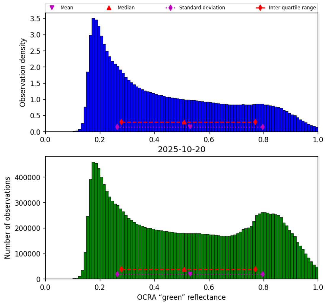
Figure 50: Histogram of “OCRA “green” reflectance” for 2025-10-20 to 2025-10-20
