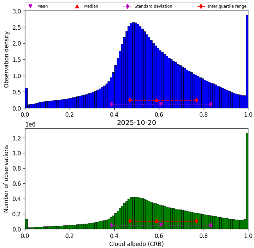
Figure 42: Histogram of “Cloud albedo (CRB)” for 2025-10-20 to 2025-10-20
