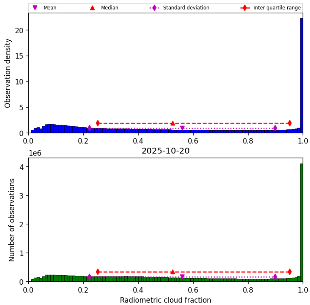
Figure 37: Histogram of “Radiometric cloud fraction” for 2025-10-20 to 2025-10-20
