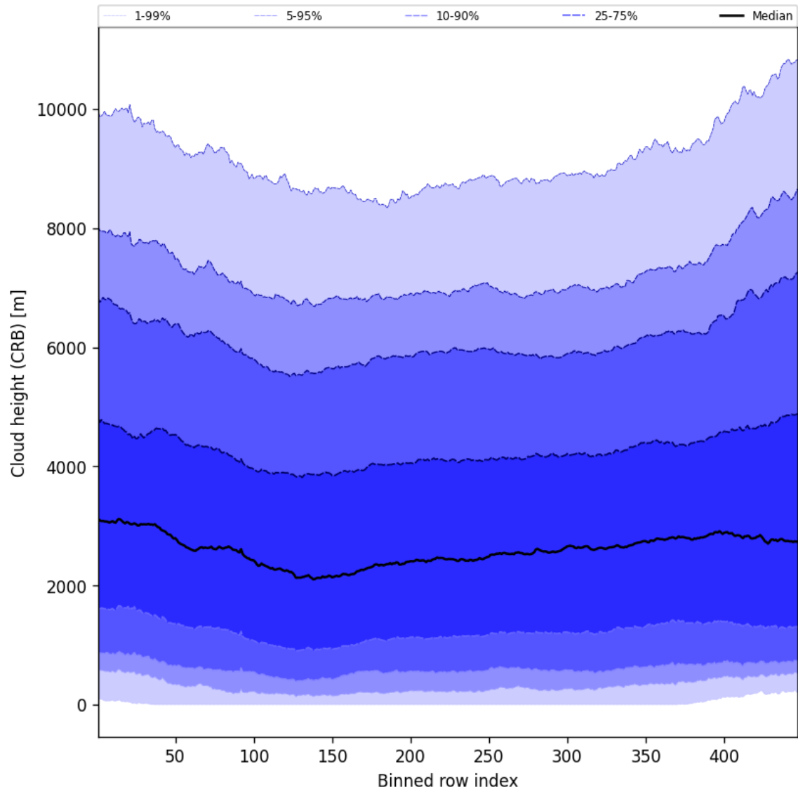
Figure 57: Along track statistics of “Cloud height (CRB)” for 2025-10-20 to 2025-10-20
