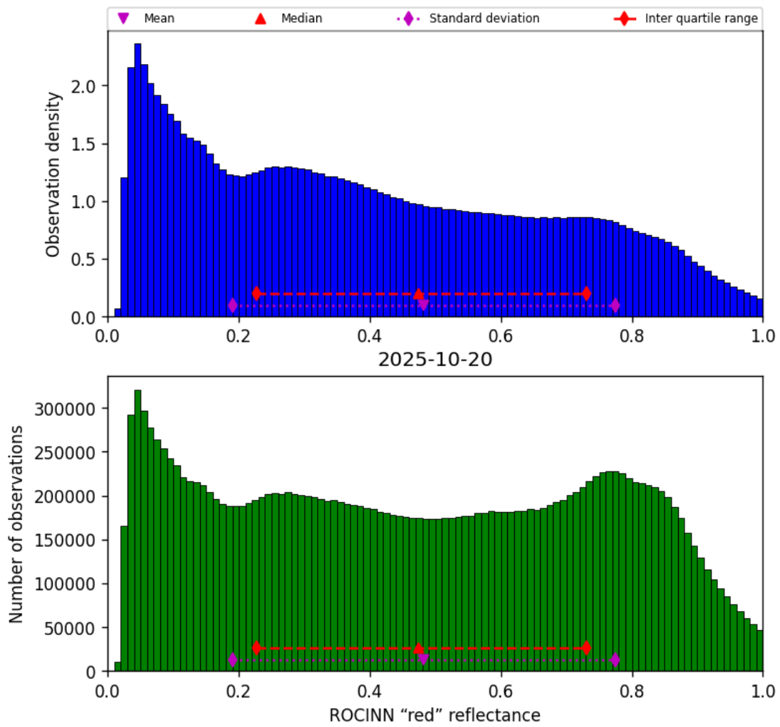
Figure 51: Histogram of “ROCINN “red” reflectance” for 2025-10-20 to 2025-10-20
