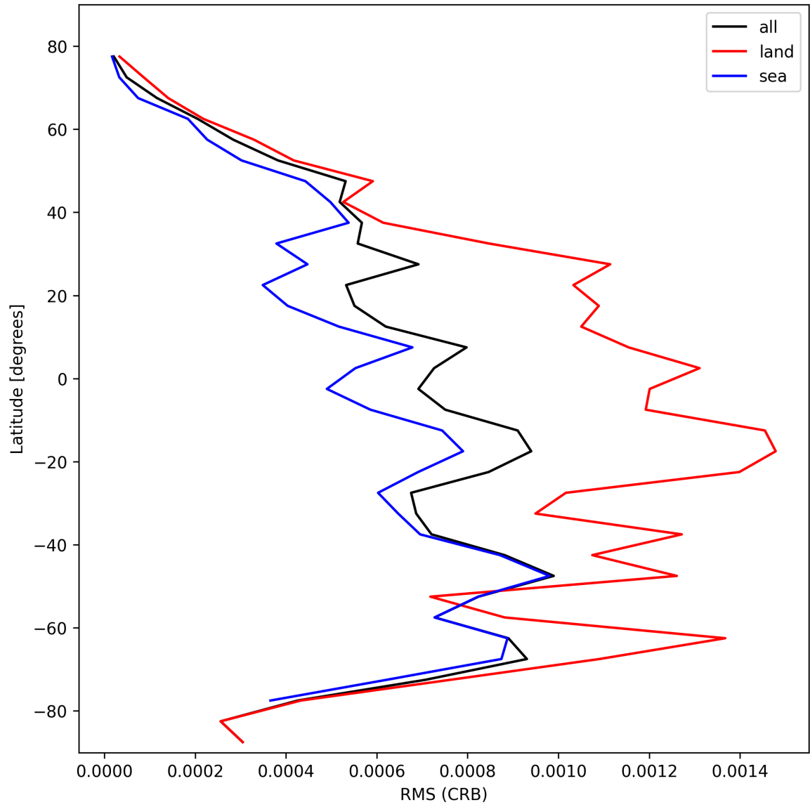
Figure 30: Zonal average of “RMS (CRB)” for 2025-10-20 to 2025-10-20.
