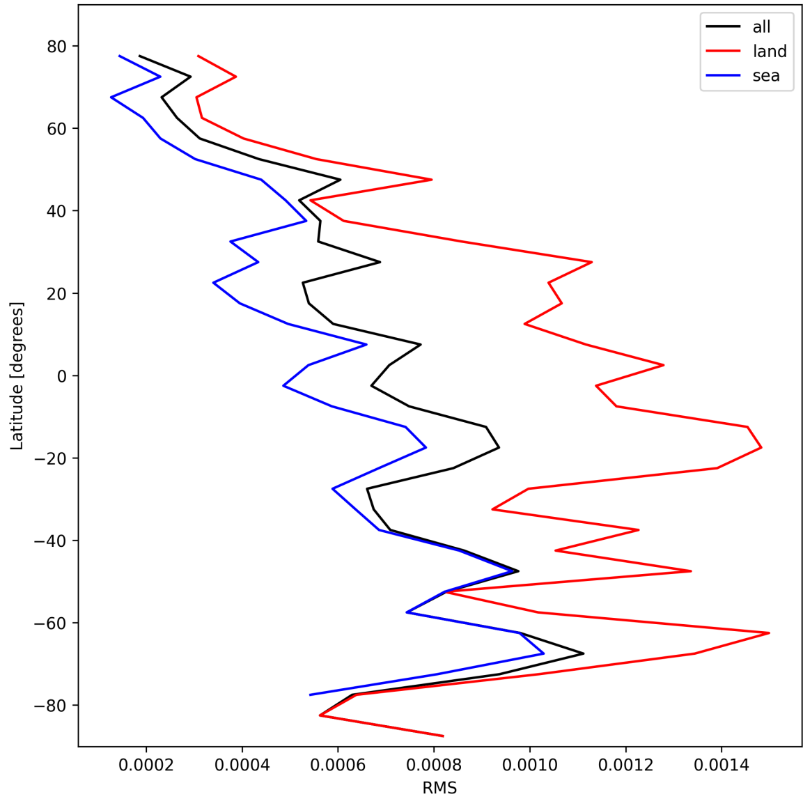
Figure 29: Zonal average of “RMS” for 2025-10-20 to 2025-10-20.
