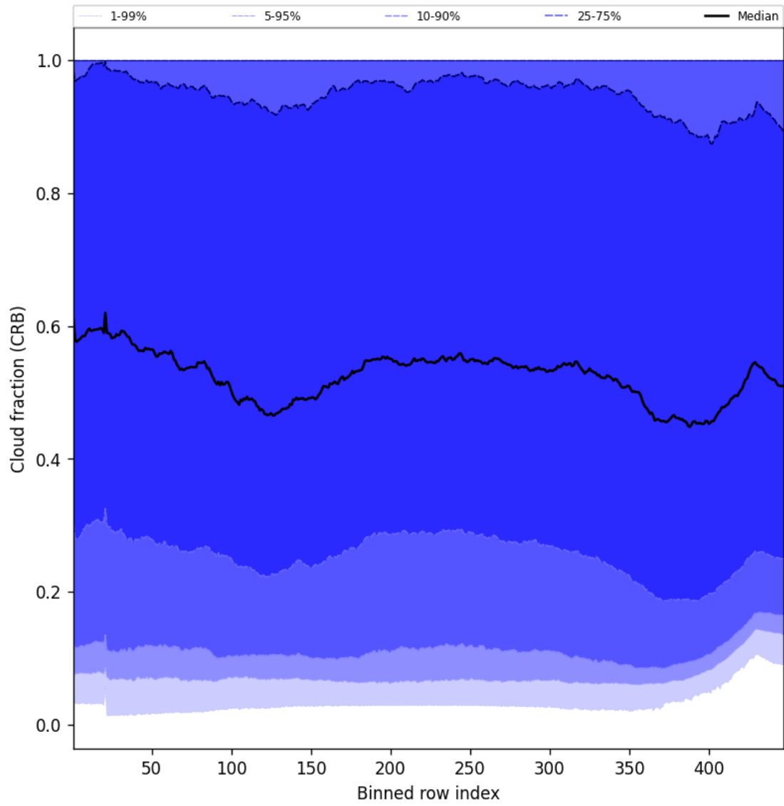
Figure 56: Along track statistics of “Cloud fraction (CRB)” for 2025-10-20 to 2025-10-20
