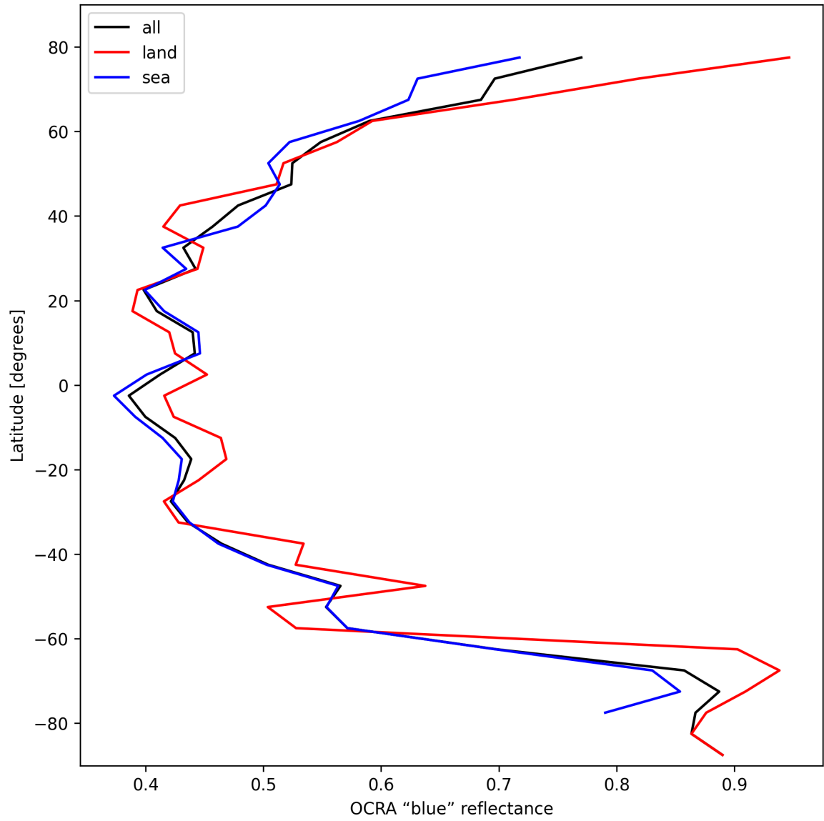
Figure 33: Zonal average of “OCRA “blue” reflectance” for 2025-10-20 to 2025-10-20.
