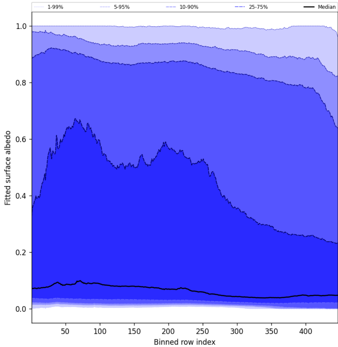
Figure 59: Along track statistics of “Fitted surface albedo” for 2025-10-20 to 2025-10-20
