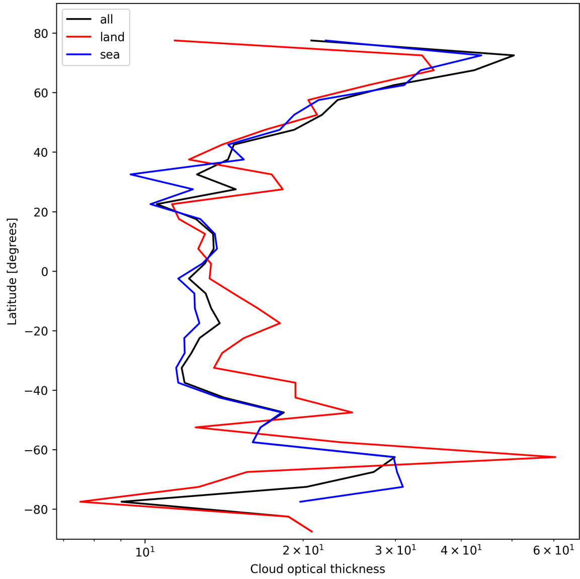
Figure 23: Zonal average of “Cloud optical thickness” for 2025-10-20 to 2025-10-20.
