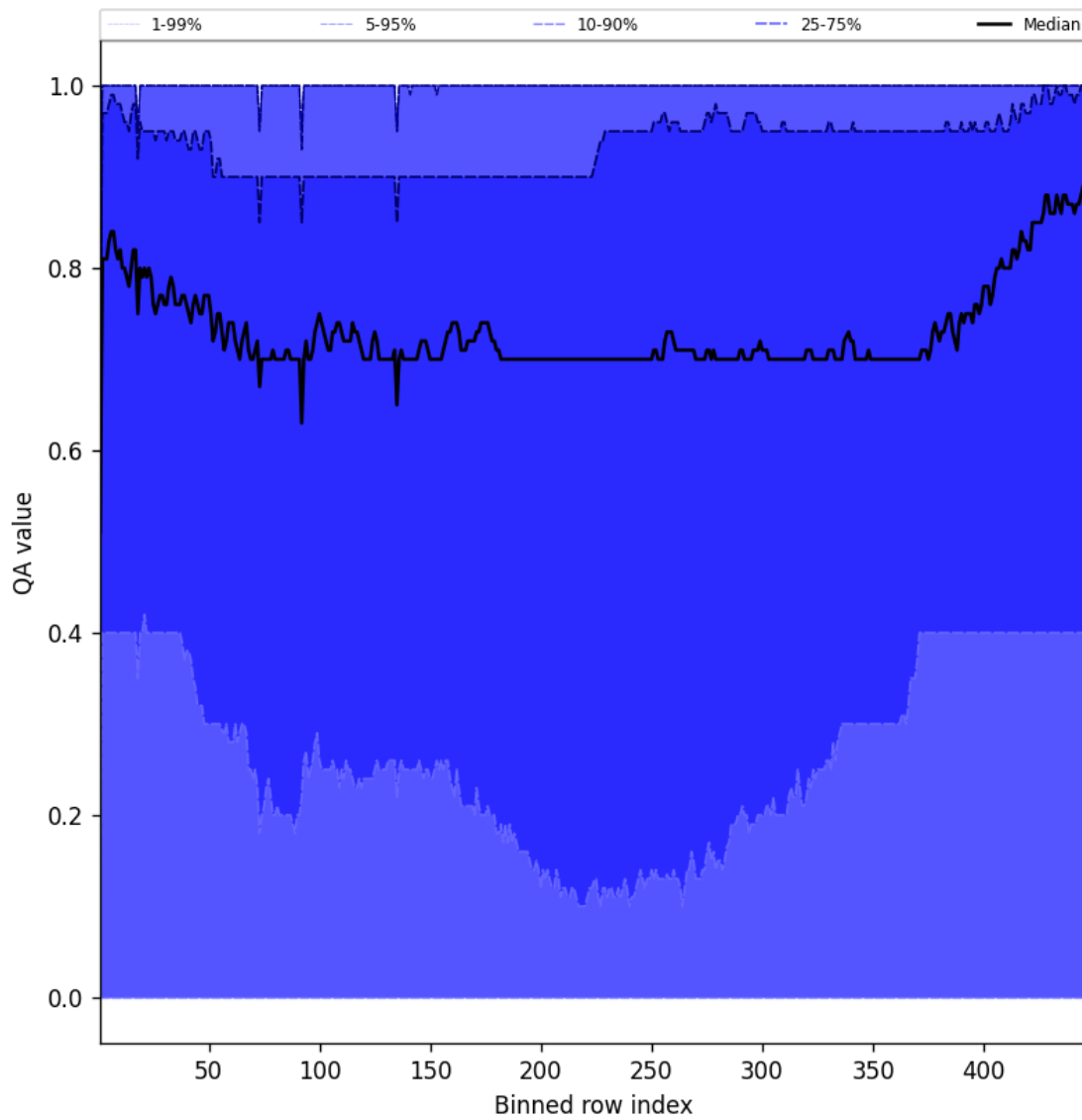
Figure 52: Along track statistics of "QA value" for 2025-10-20 to 2025-10-20
