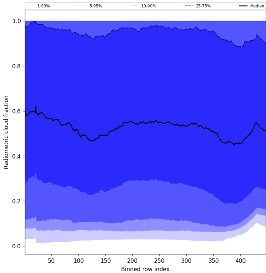
Figure 53: Along track statistics of “Radiometric cloud fraction” for 2025-10-20 to 2025-10-20
