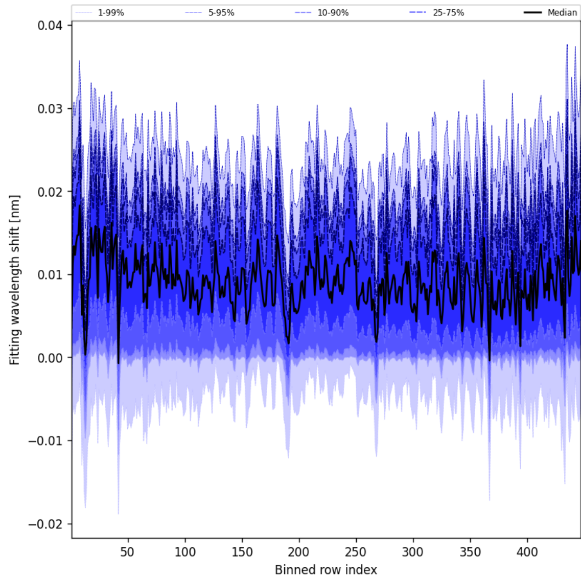
Figure 63: Along track statistics of “Fitting wavelength shift” for 2025-10-20 to 2025-10-20
