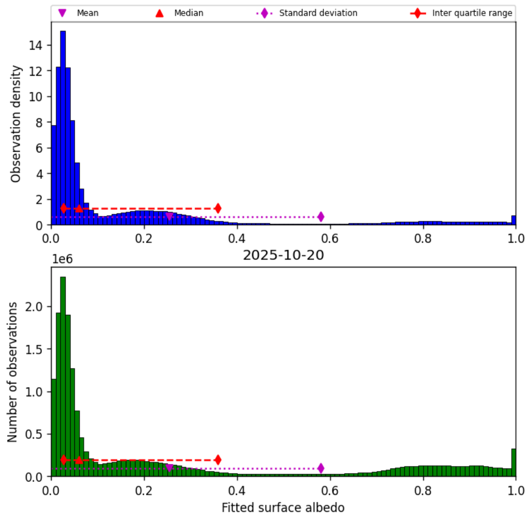
Figure 43: Histogram of “Fitted surface albedo” for 2025-10-20 to 2025-10-20
