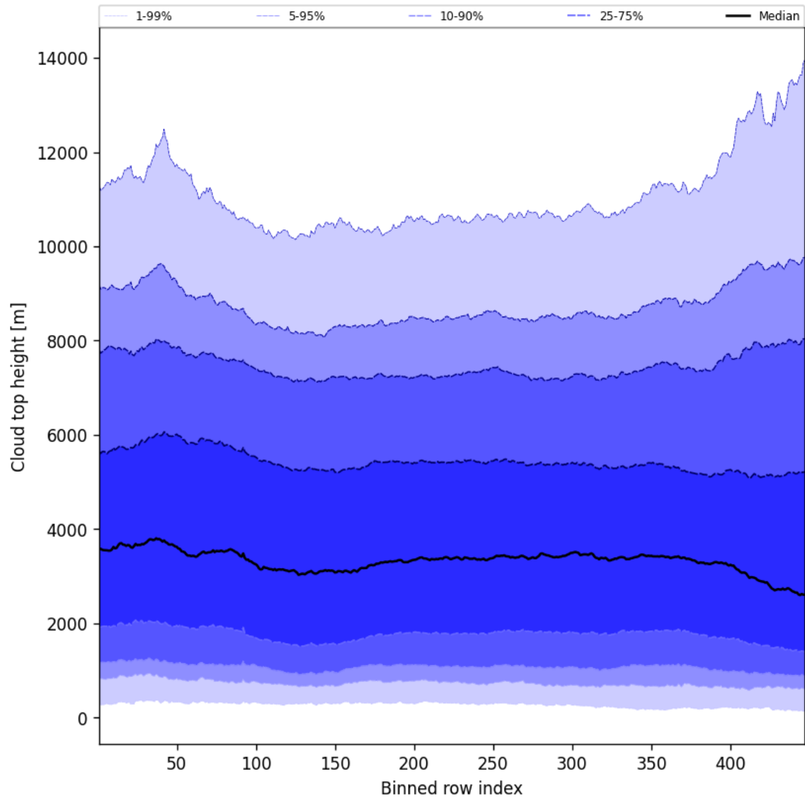
Figure 54: Along track statistics of “Cloud top height” for 2025-10-20 to 2025-10-20
