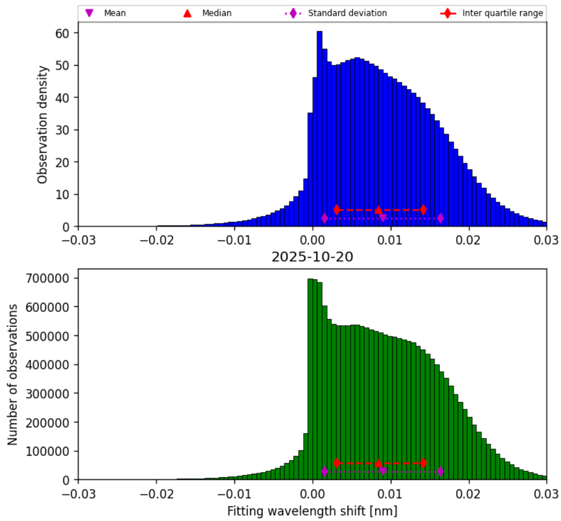
Figure 47: Histogram of “Fitting wavelength shift” for 2025-10-20 to 2025-10-20
