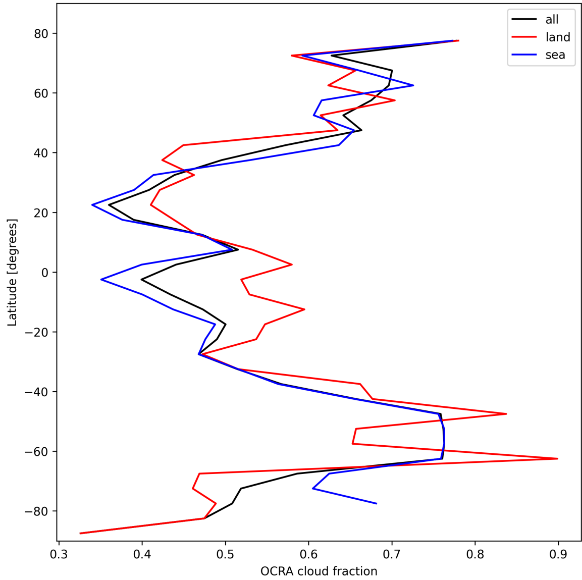
Figure 32: Zonal average of “OCRA cloud fraction” for 2025-10-20 to 2025-10-20.
