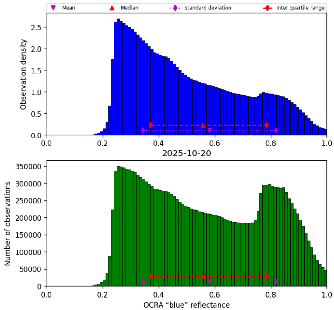
Figure 49: Histogram of “OCRA “blue” reflectance” for 2025-10-20 to 2025-10-20
