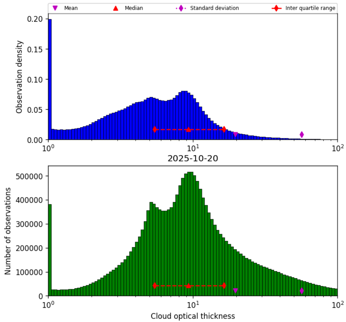
Figure 39: Histogram of “Cloud optical thickness” for 2025-10-20 to 2025-10-20
