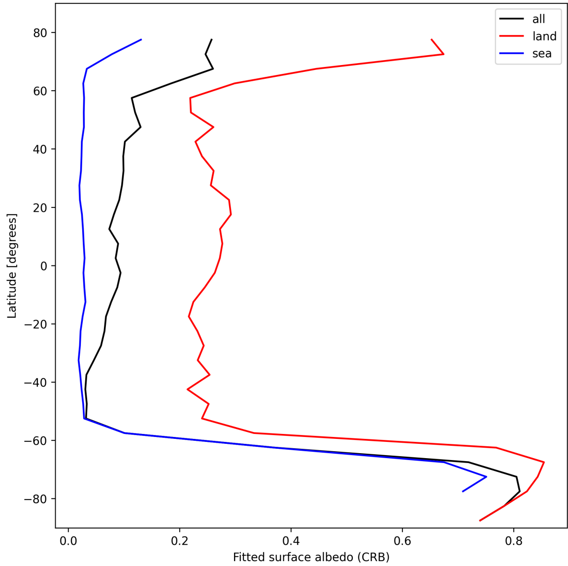
Figure 28: Zonal average of “Fitted surface albedo (CRB)” for 2025-10-20 to 2025-10-20.
