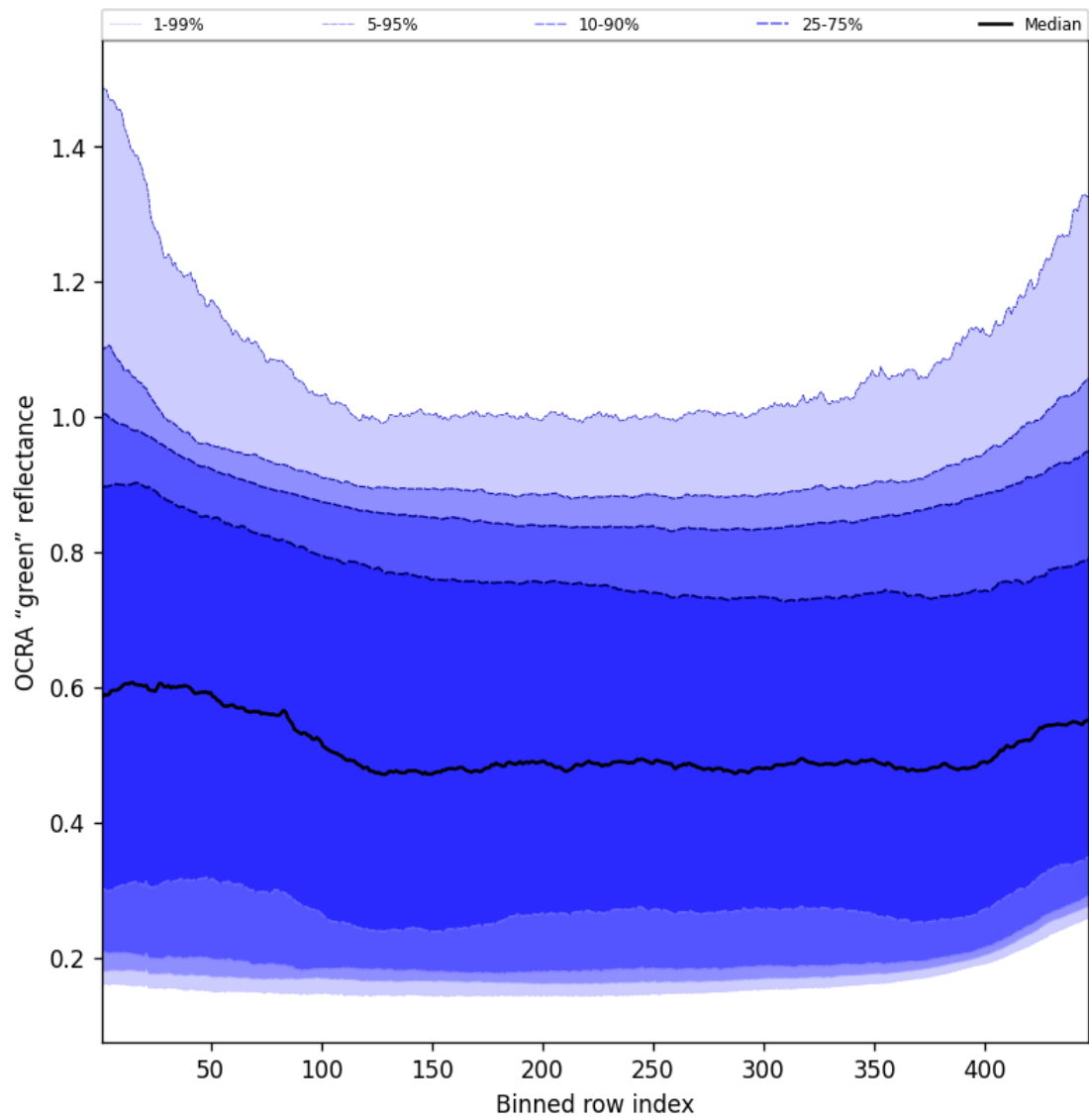
Figure 66: Along track statistics of “OCRA “green” reflectance” for 2025-10-20 to 2025-10-20
