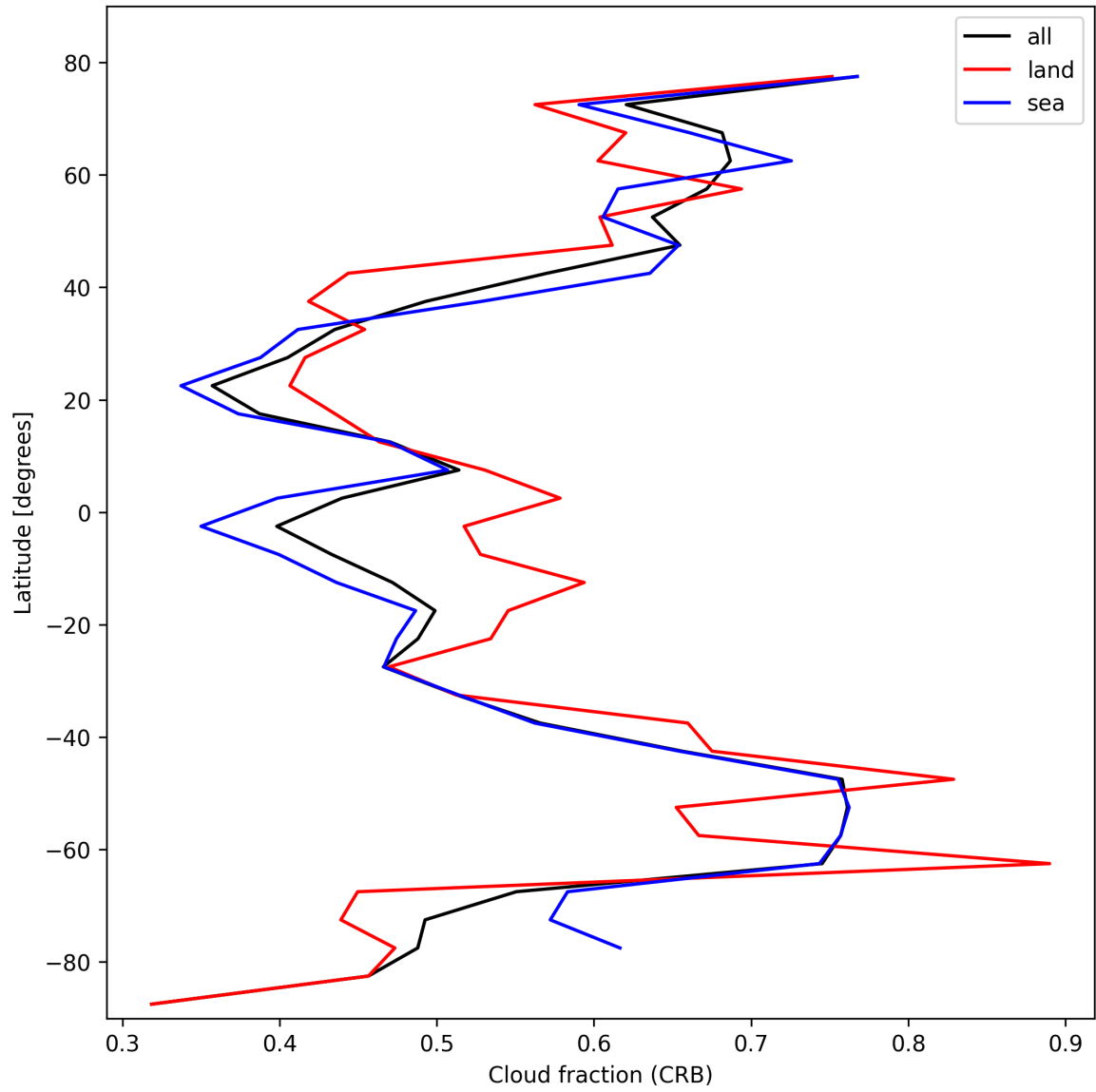
Figure 24: Zonal average of “Cloud fraction (CRB)” for 2025-10-20 to 2025-10-20.
