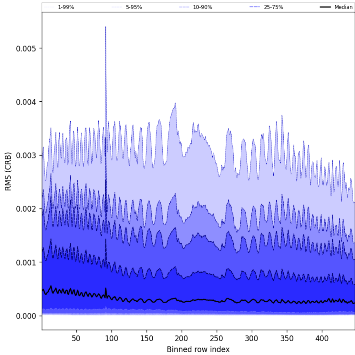
Figure 62: Along track statistics of “RMS (CRB)” for 2025-10-20 to 2025-10-20
