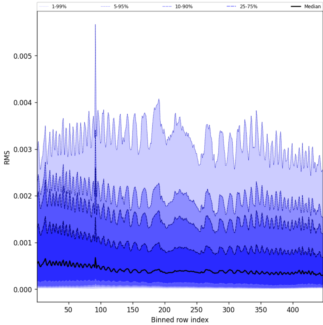
Figure 61: Along track statistics of “RMS” for 2025-10-20 to 2025-10-20
