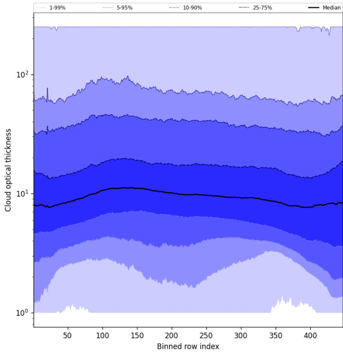
Figure 55: Along track statistics of “Cloud optical thickness” for 2025-10-20 to 2025-10-20
