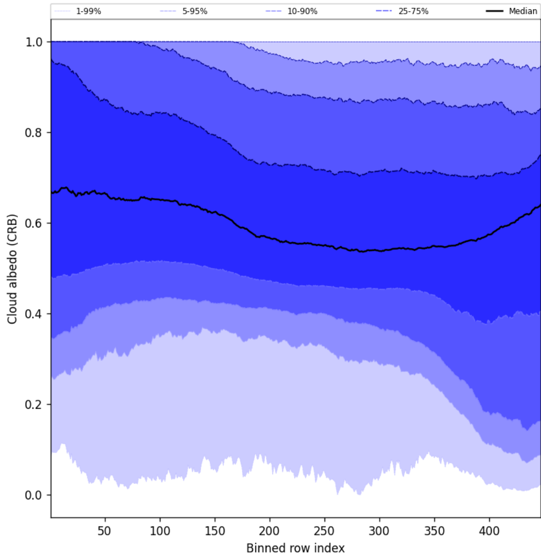
Figure 58: Along track statistics of “Cloud albedo (CRB)” for 2025-10-20 to 2025-10-20
