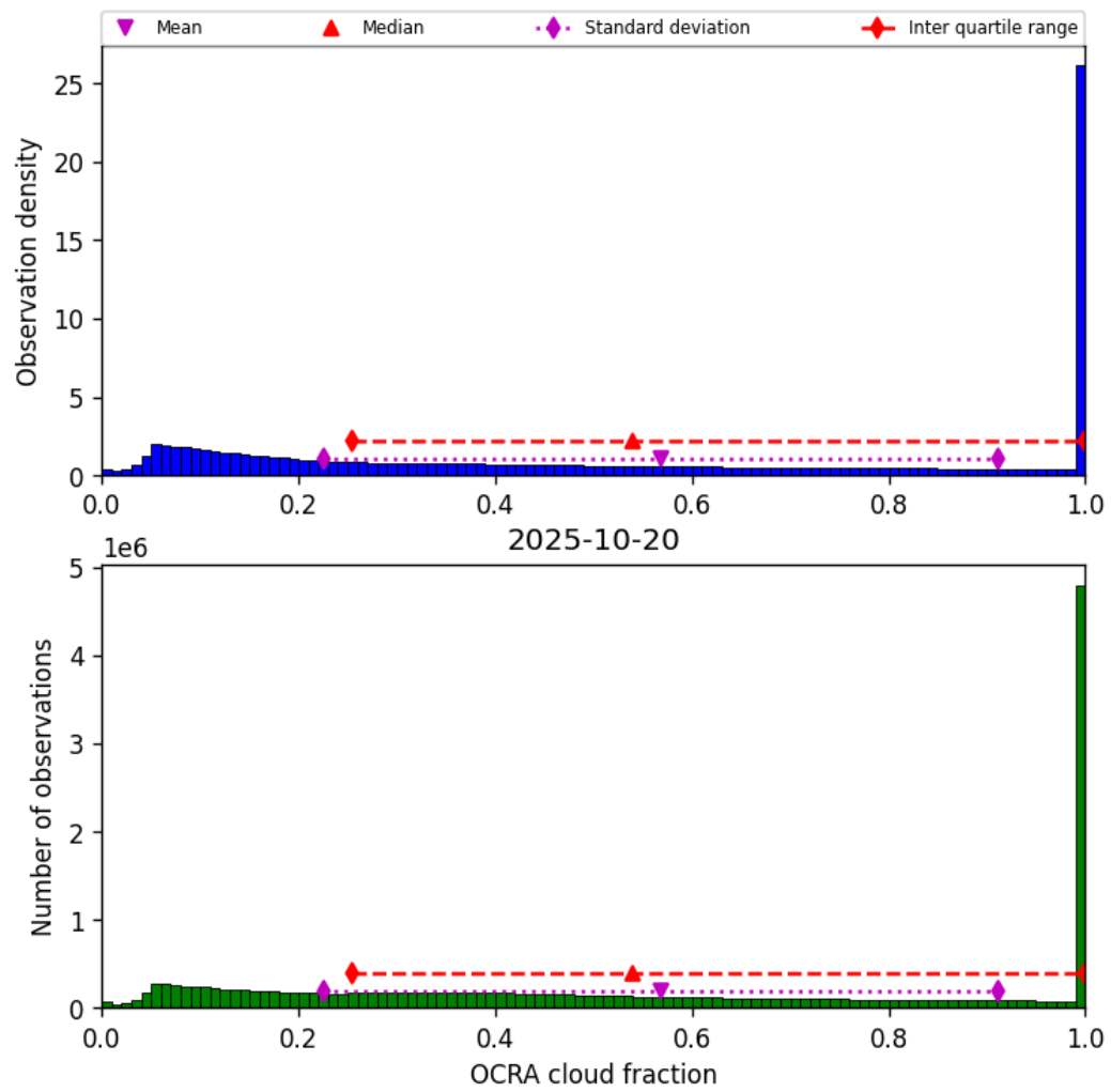
Figure 48: Histogram of “OCRA cloud fraction” for 2025-10-20 to 2025-10-20
