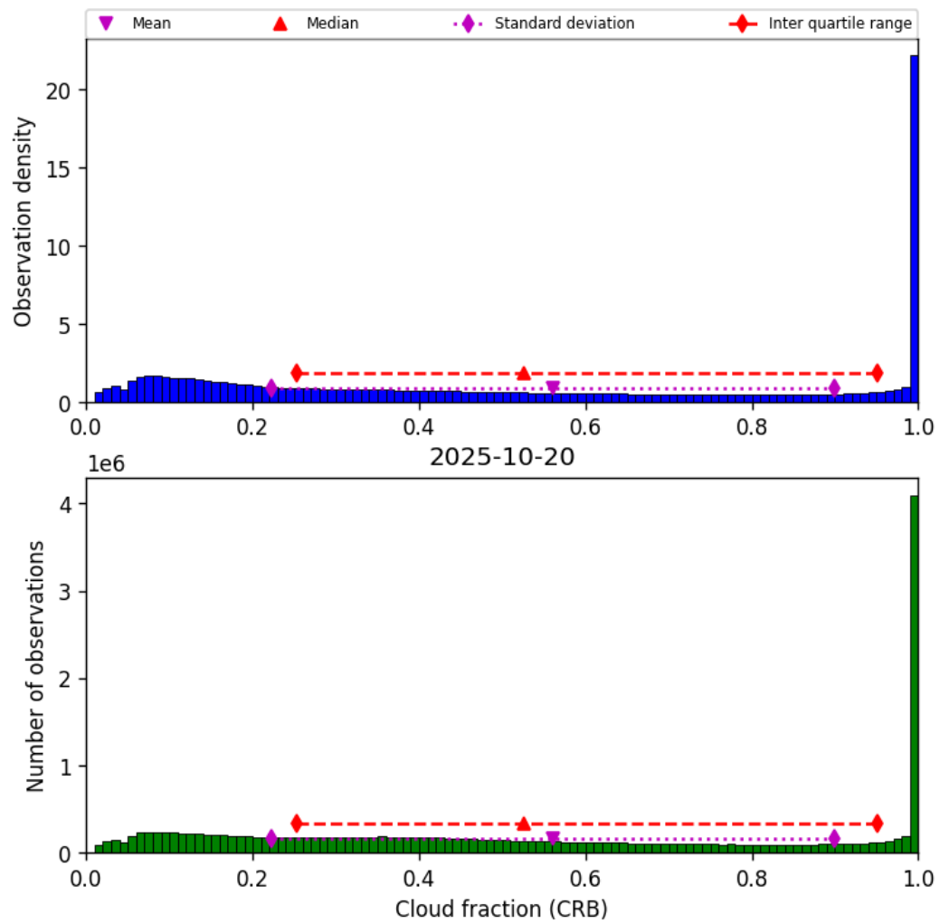
Figure 40: Histogram of “Cloud fraction (CRB)” for 2025-10-20 to 2025-10-20
