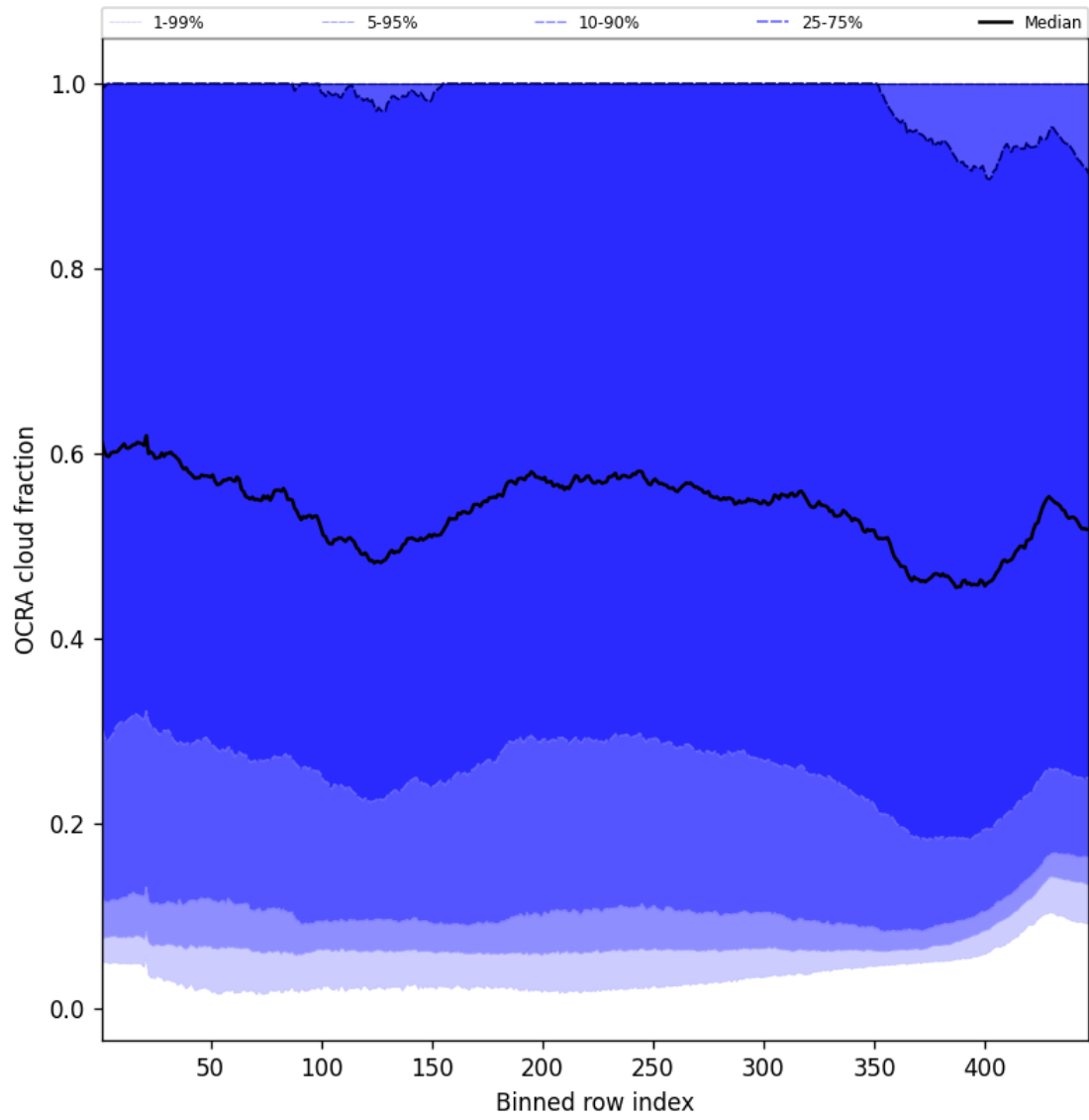
Figure 64: Along track statistics of “OCRA cloud fraction” for 2025-10-20 to 2025-10-20
