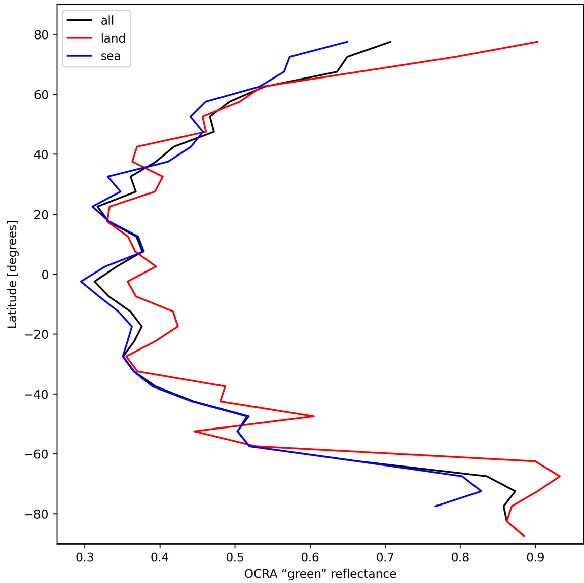
Figure 34: Zonal average of “OCRA “green” reflectance” for 2025-10-20 to 2025-10-20.
