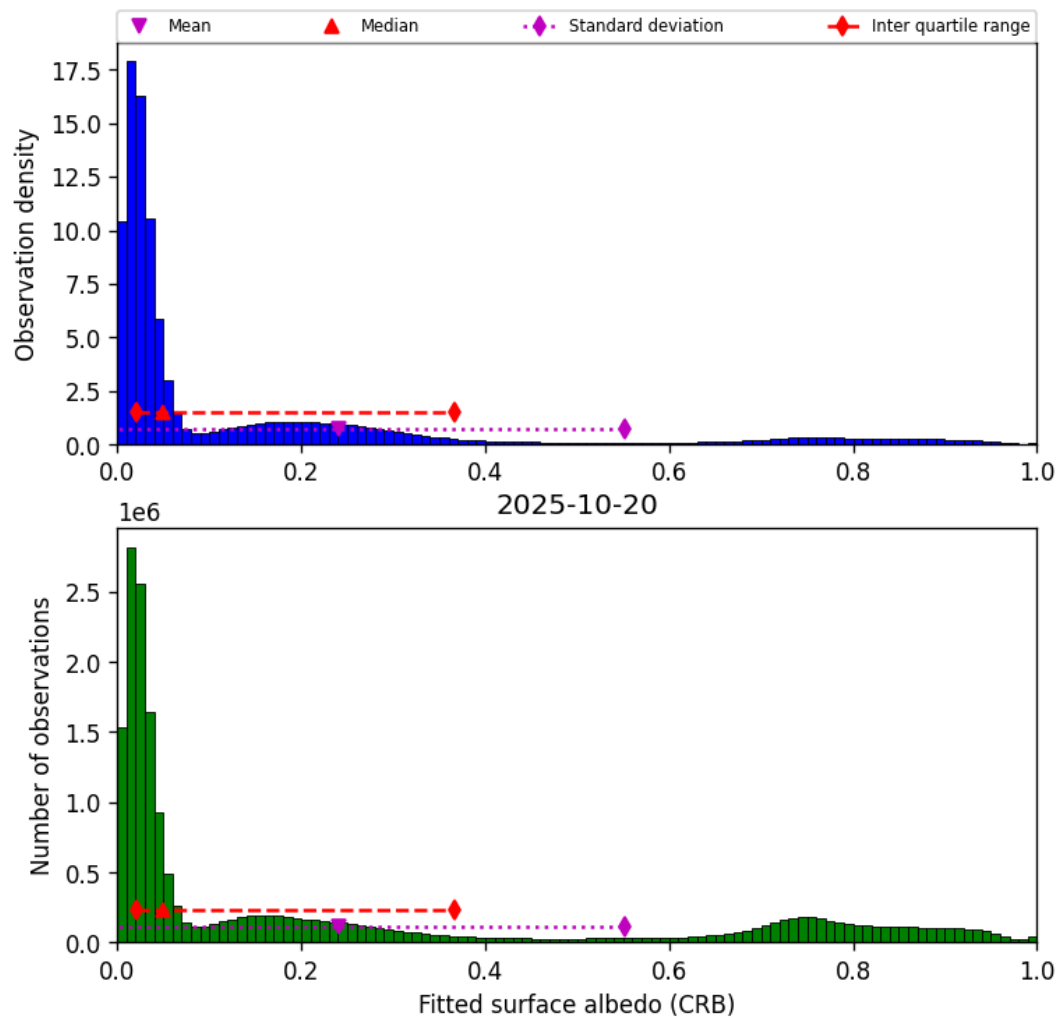
Figure 44: Histogram of “Fitted surface albedo (CRB)” for 2025-10-20 to 2025-10-20
