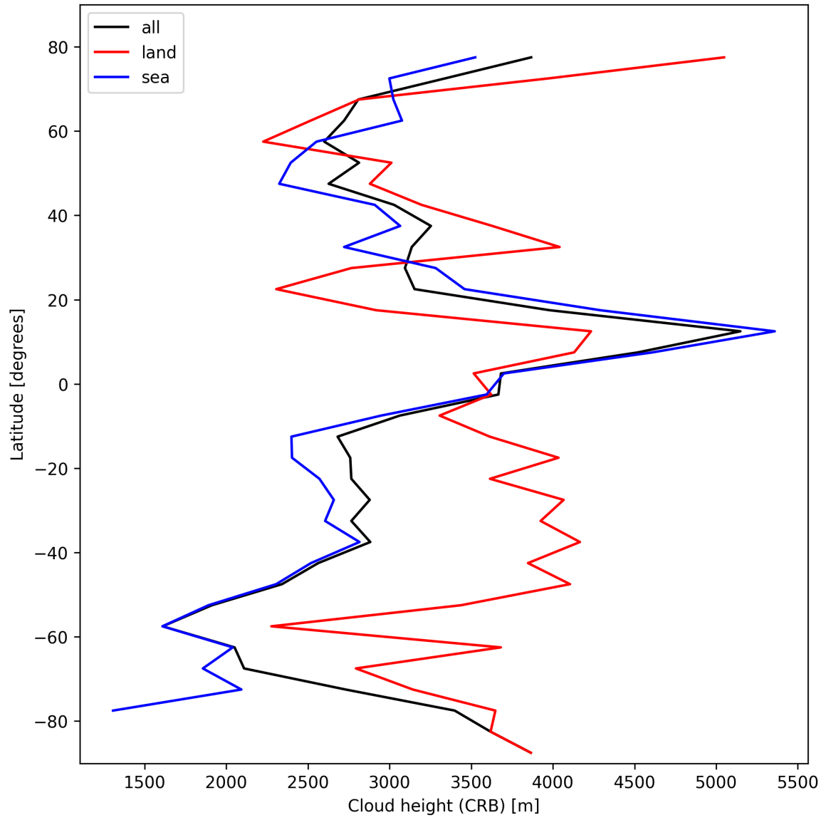
Figure 25: Zonal average of “Cloud height (CRB)” for 2025-10-20 to 2025-10-20.
