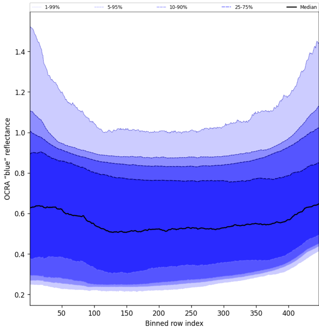
Figure 65: Along track statistics of “OCRA “blue” reflectance” for 2025-10-20 to 2025-10-20
