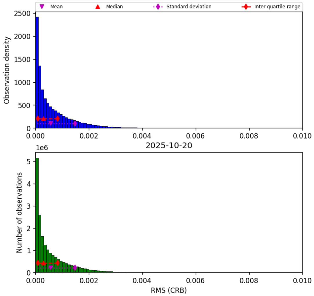
Figure 46: Histogram of “RMS (CRB)” for 2025-10-20 to 2025-10-20
