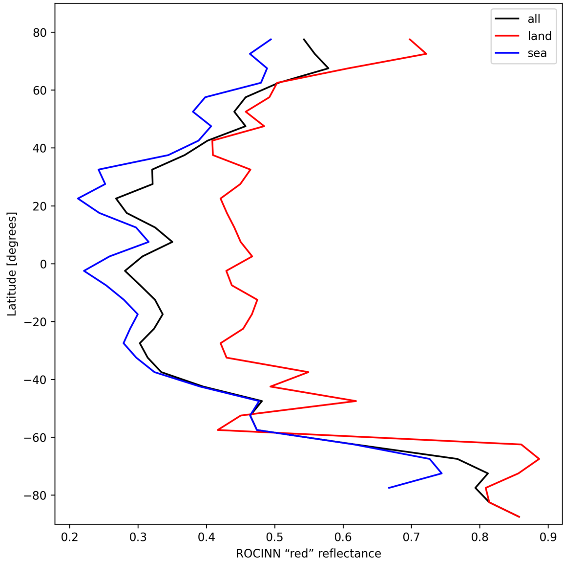
Figure 35: Zonal average of “ROCINN “red” reflectance” for 2025-10-20 to 2025-10-20.
