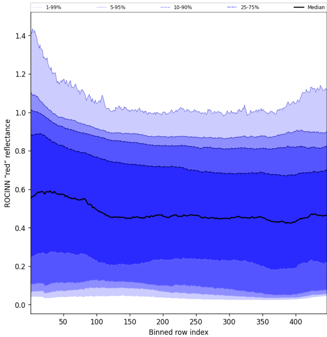
Figure 67: Along track statistics of "ROCINN "red" reflectance" for 2025-10-20 to 2025-10-20
