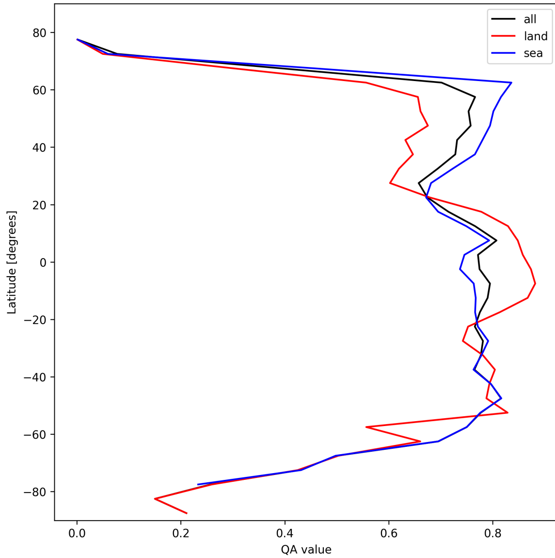
Figure 20: Zonal average of “QA value” for 2025-10-20 to 2025-10-20.
