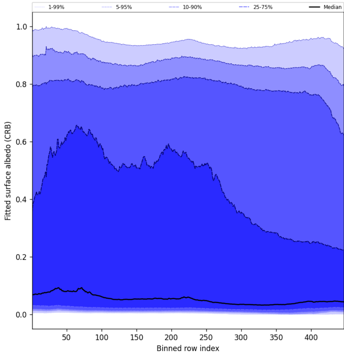
Figure 60: Along track statistics of “Fitted surface albedo (CRB)” for 2025-10-20 to 2025-10-20
