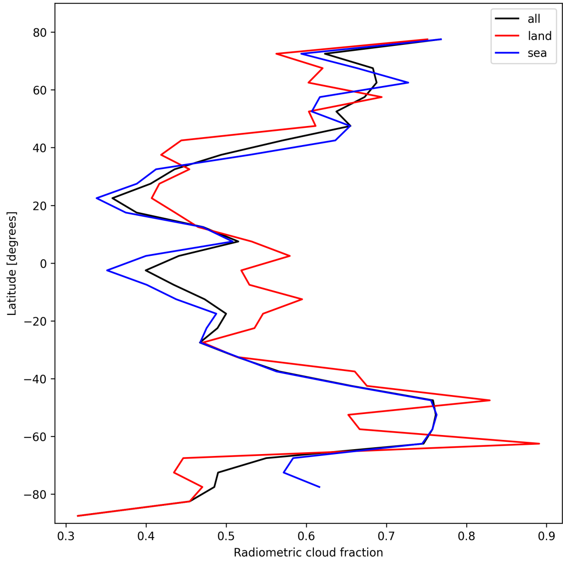
Figure 21: Zonal average of “Radiometric cloud fraction” for 2025-10-20 to 2025-10-20.
