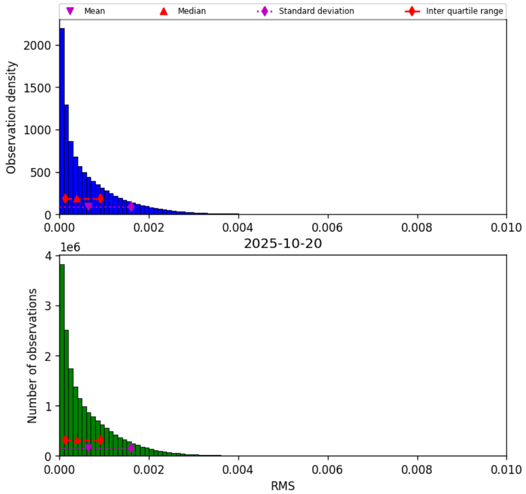
Figure 45: Histogram of “RMS” for 2025-10-20 to 2025-10-20
