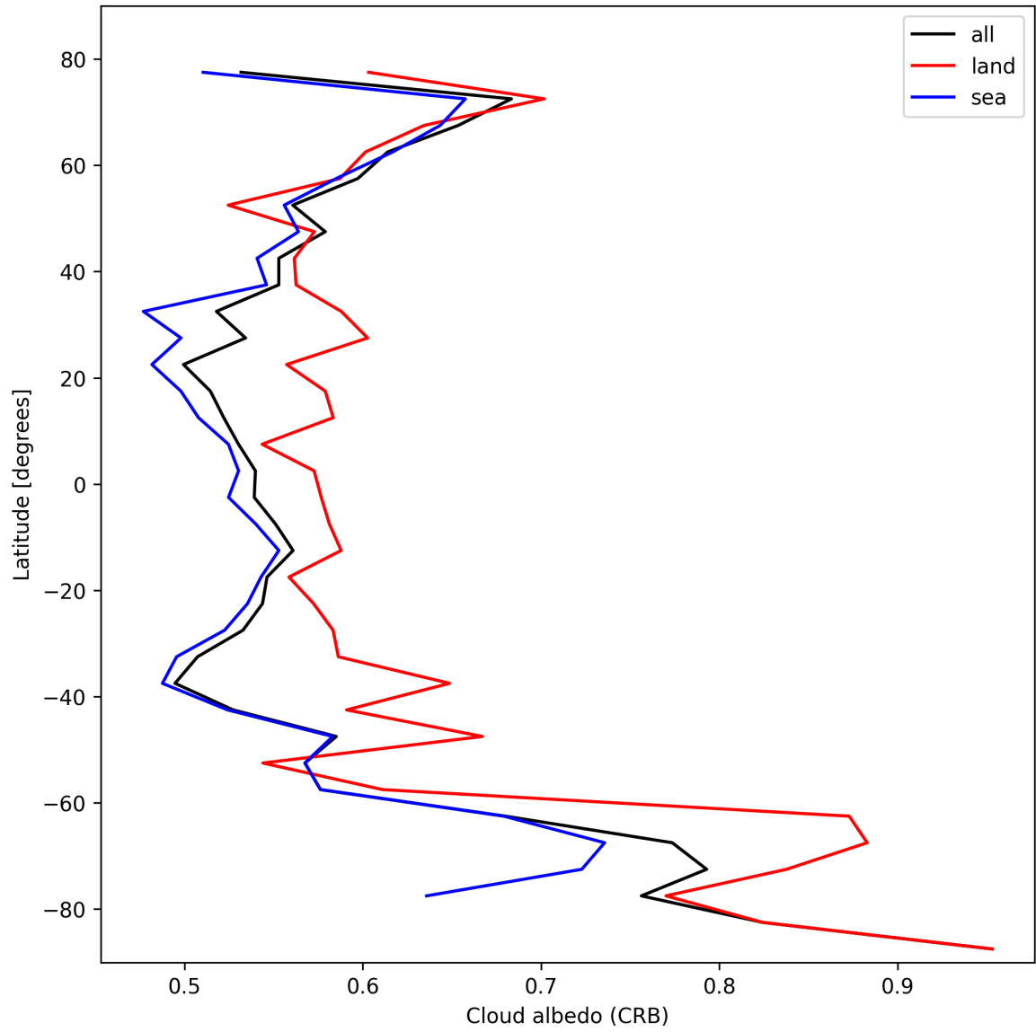
Figure 26: Zonal average of “Cloud albedo (CRB)” for 2025-10-20 to 2025-10-20.
