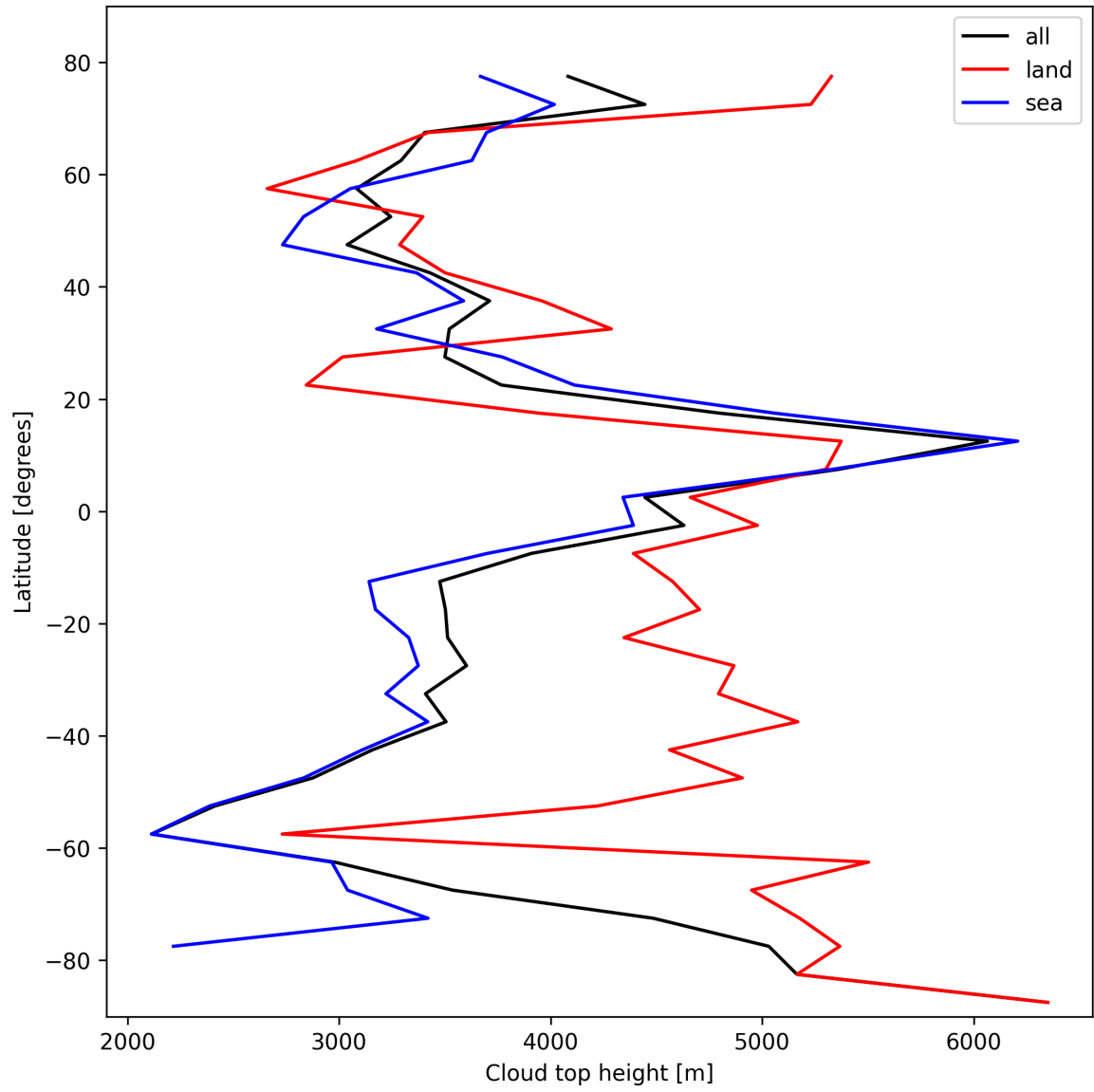
Figure 22: Zonal average of “Cloud top height” for 2025-10-20 to 2025-10-20.
