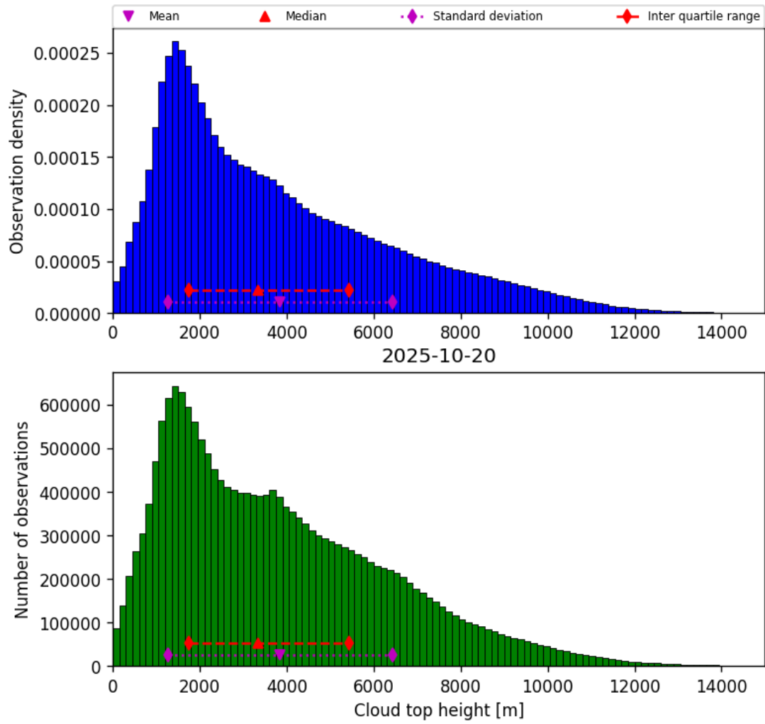
Figure 38: Histogram of “Cloud top height” for 2025-10-20 to 2025-10-20
