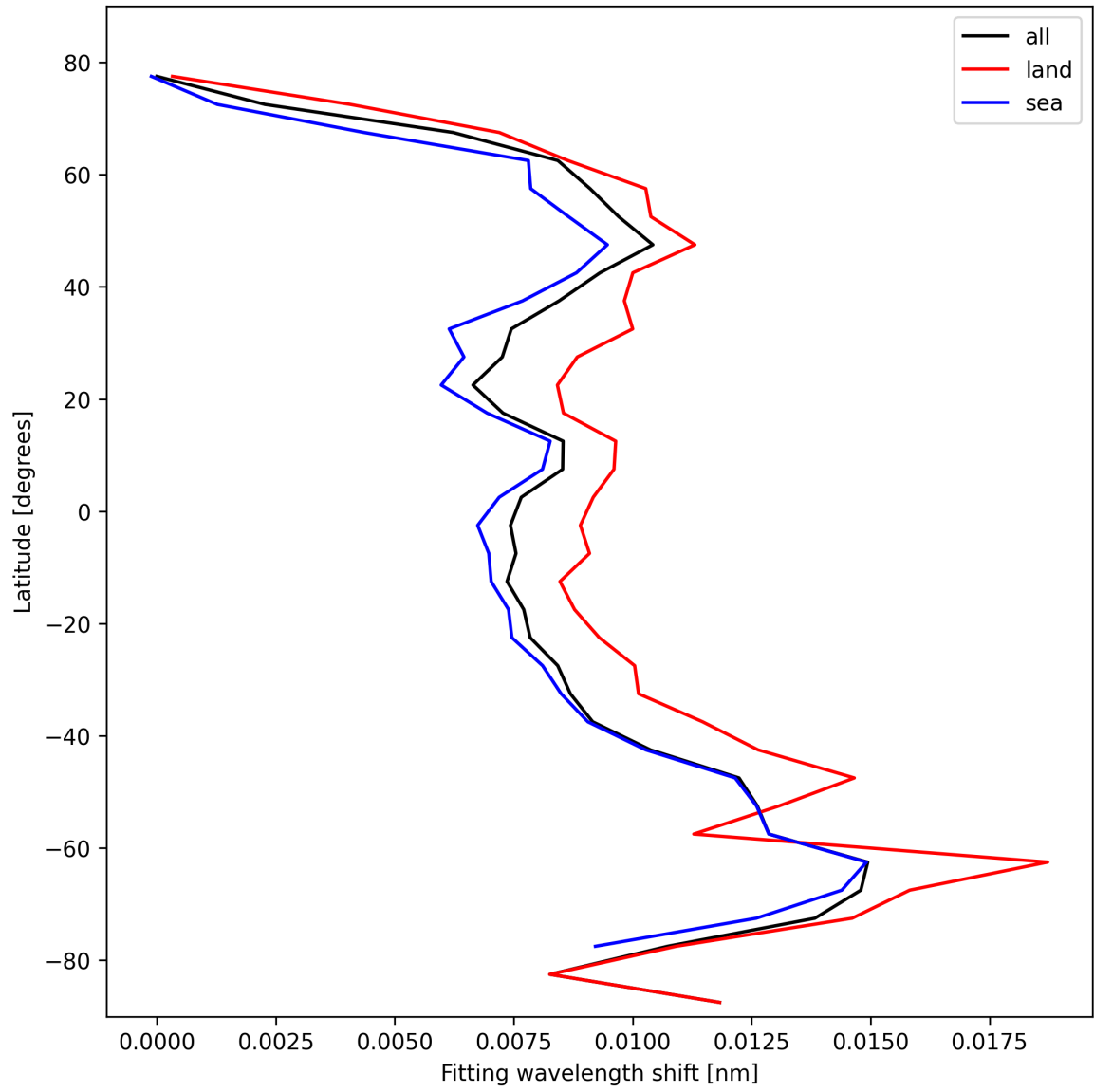
Figure 31: Zonal average of “Fitting wavelength shift” for 2025-10-20 to 2025-10-20.
