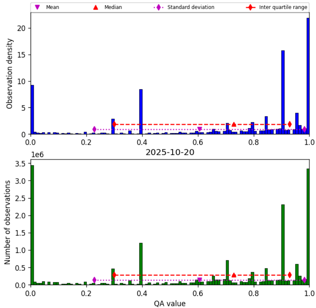
Figure 36: Histogram of “QA value” for 2025-10-20 to 2025-10-20
