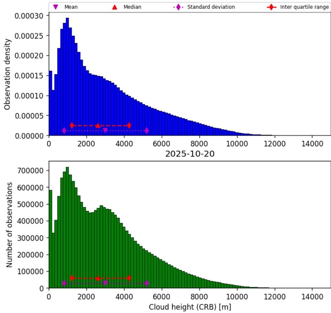
Figure 41: Histogram of “Cloud height (CRB)” for 2025-10-20 to 2025-10-20
