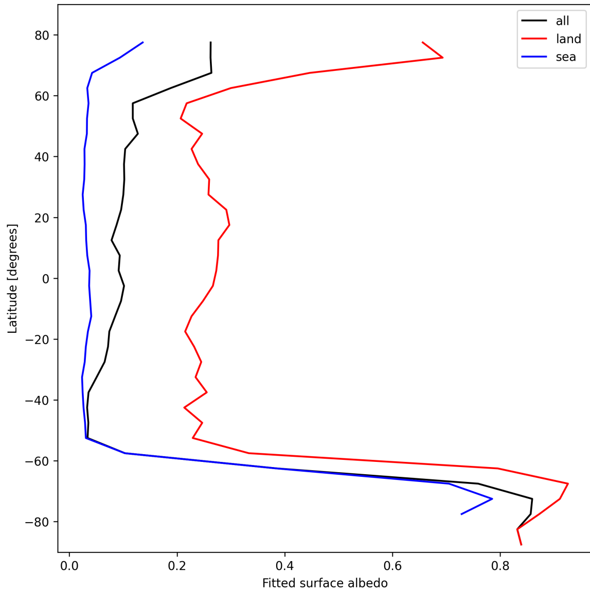
Figure 27: Zonal average of “Fitted surface albedo” for 2025-10-20 to 2025-10-20.
