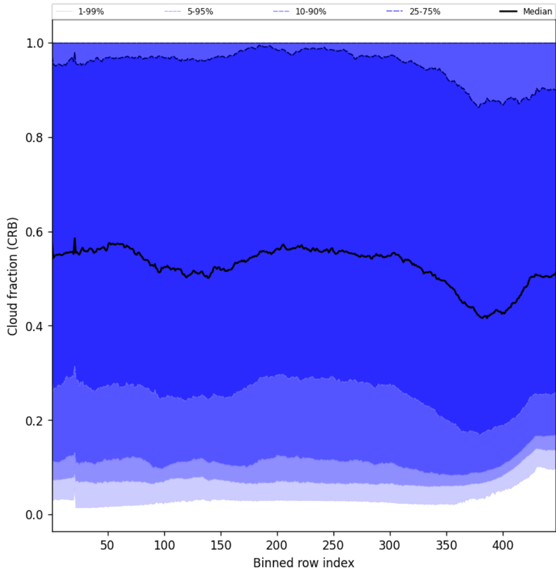
Figure 56: Along track statistics of “Cloud fraction (CRB)” for 2025-10-21 to 2025-10-22
