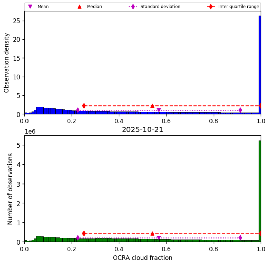
Figure 48: Histogram of “OCRA cloud fraction” for 2025-10-21 to 2025-10-22
