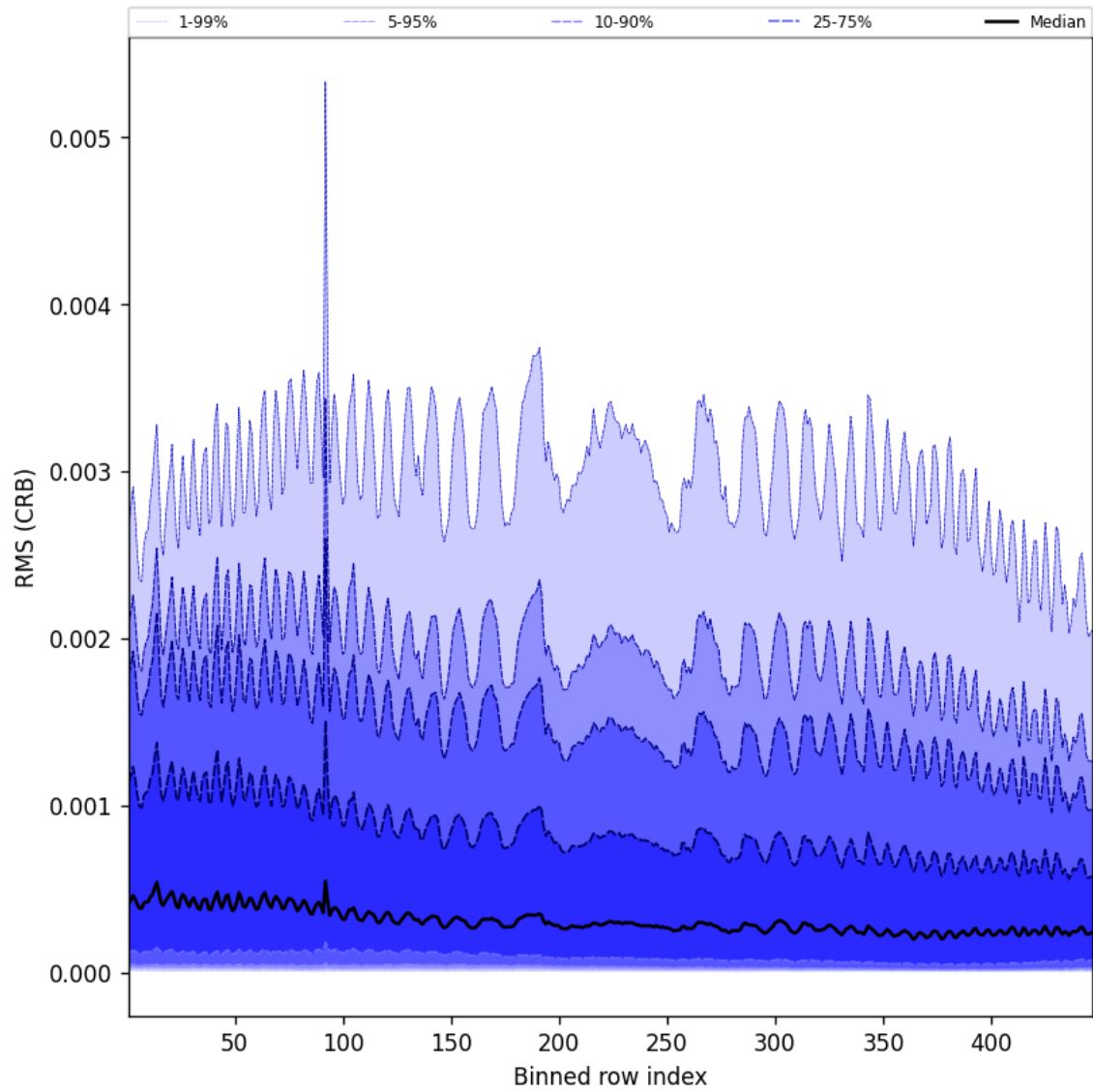
Figure 62: Along track statistics of “RMS (CRB)” for 2025-10-21 to 2025-10-22
