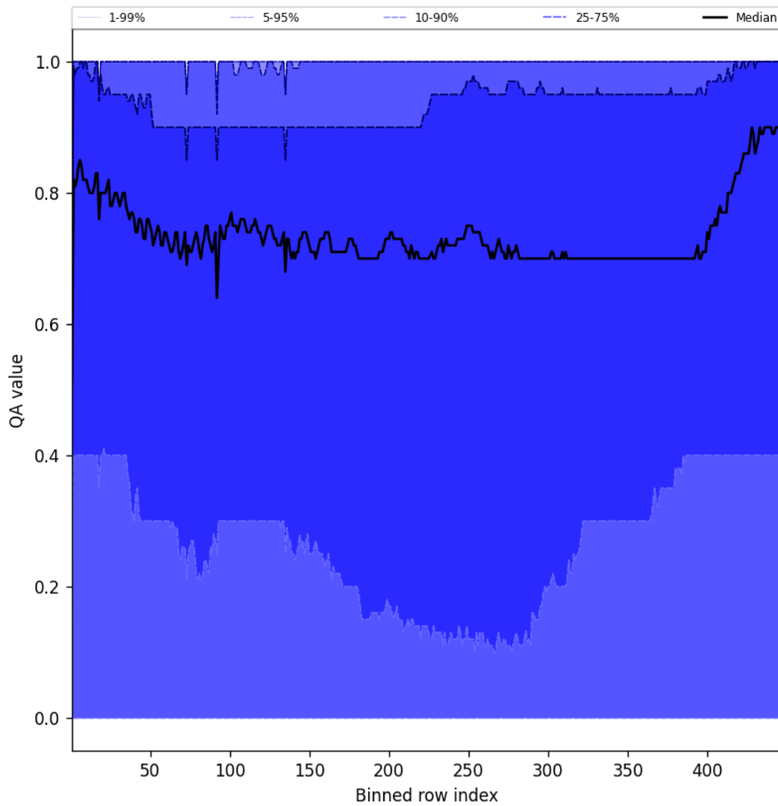
Figure 52: Along track statistics of “QA value” for 2025-10-21 to 2025-10-22
