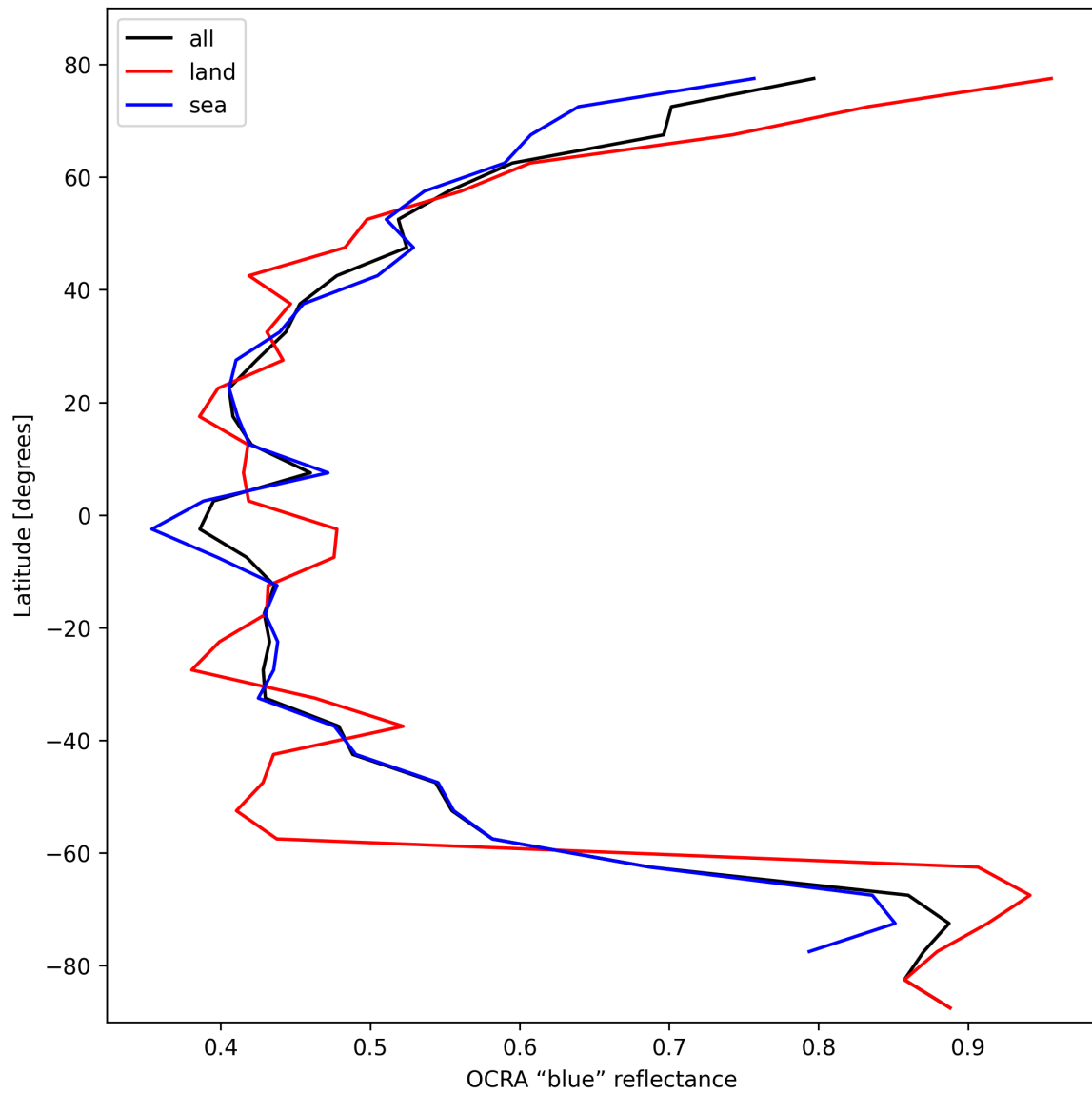
Figure 33: Zonal average of “OCRA “blue” reflectance” for 2025-10-21 to 2025-10-22.
