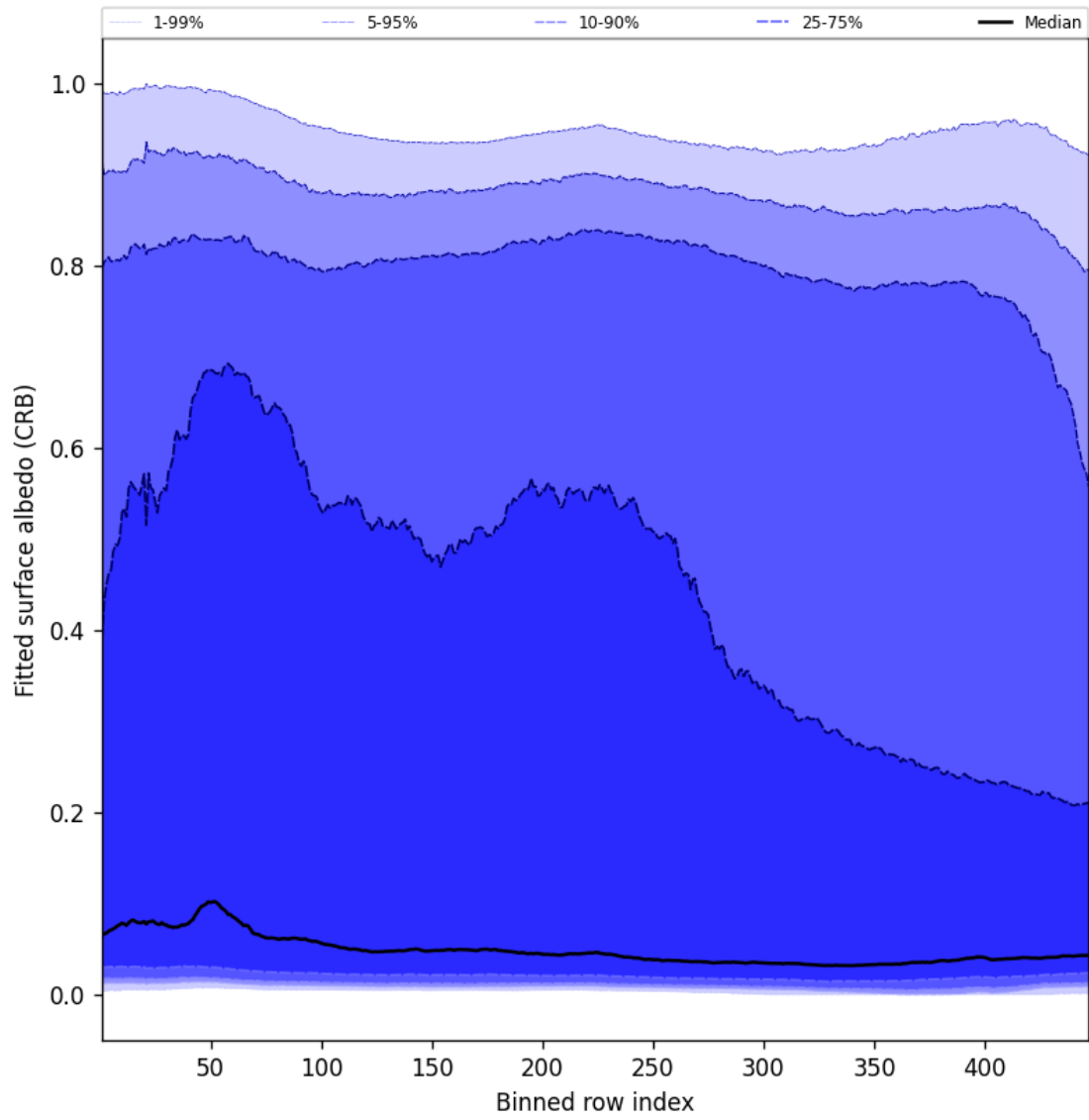
Figure 60: Along track statistics of “Fitted surface albedo (CRB)” for 2025-10-21 to 2025-10-22
