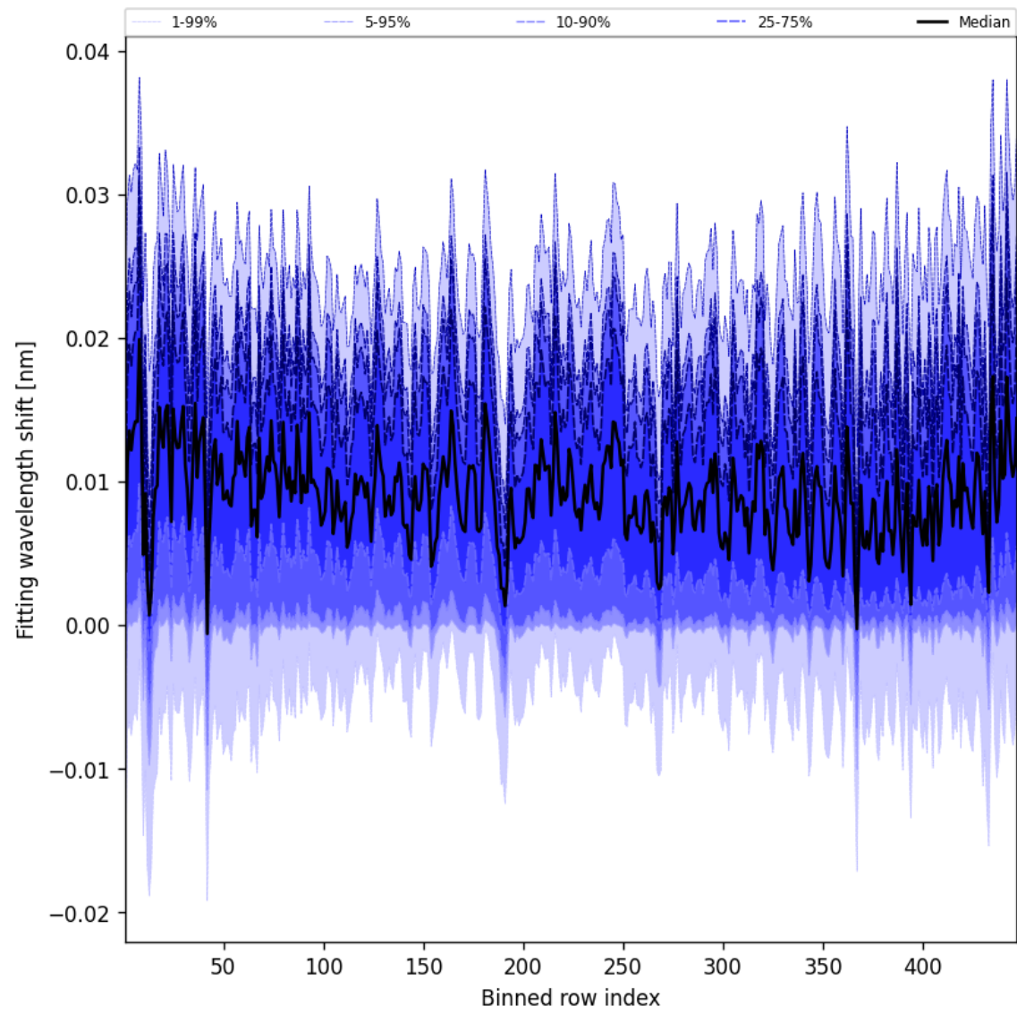
Figure 63: Along track statistics of “Fitting wavelength shift” for 2025-10-21 to 2025-10-22
