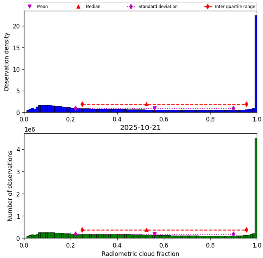
Figure 37: Histogram of “Radiometric cloud fraction” for 2025-10-21 to 2025-10-22
