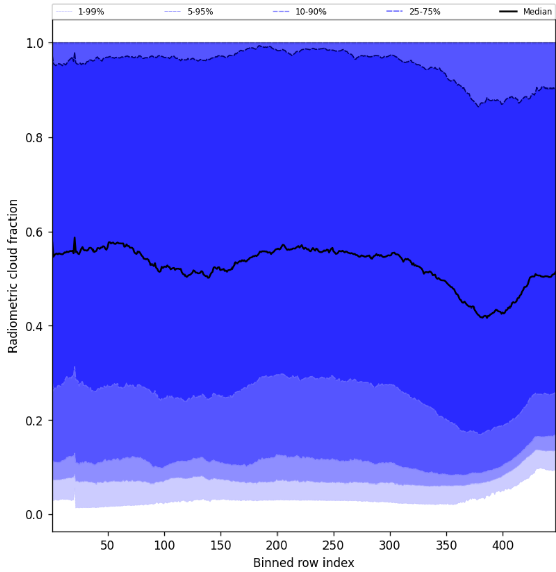
Figure 53: Along track statistics of “Radiometric cloud fraction” for 2025-10-21 to 2025-10-22
