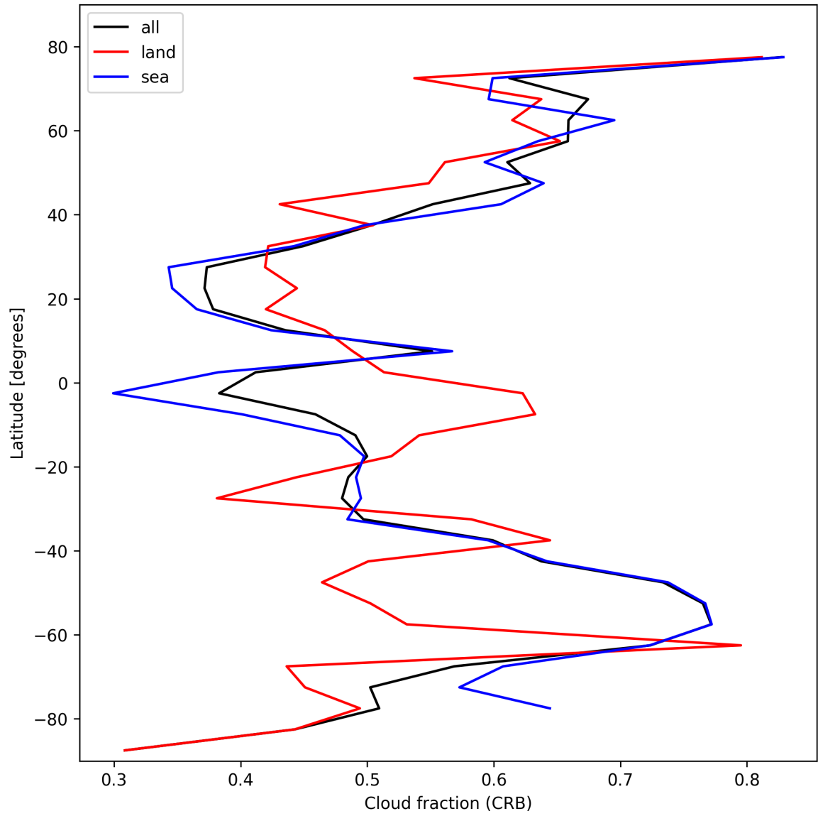
Figure 24: Zonal average of “Cloud fraction (CRB)” for 2025-10-21 to 2025-10-22.
