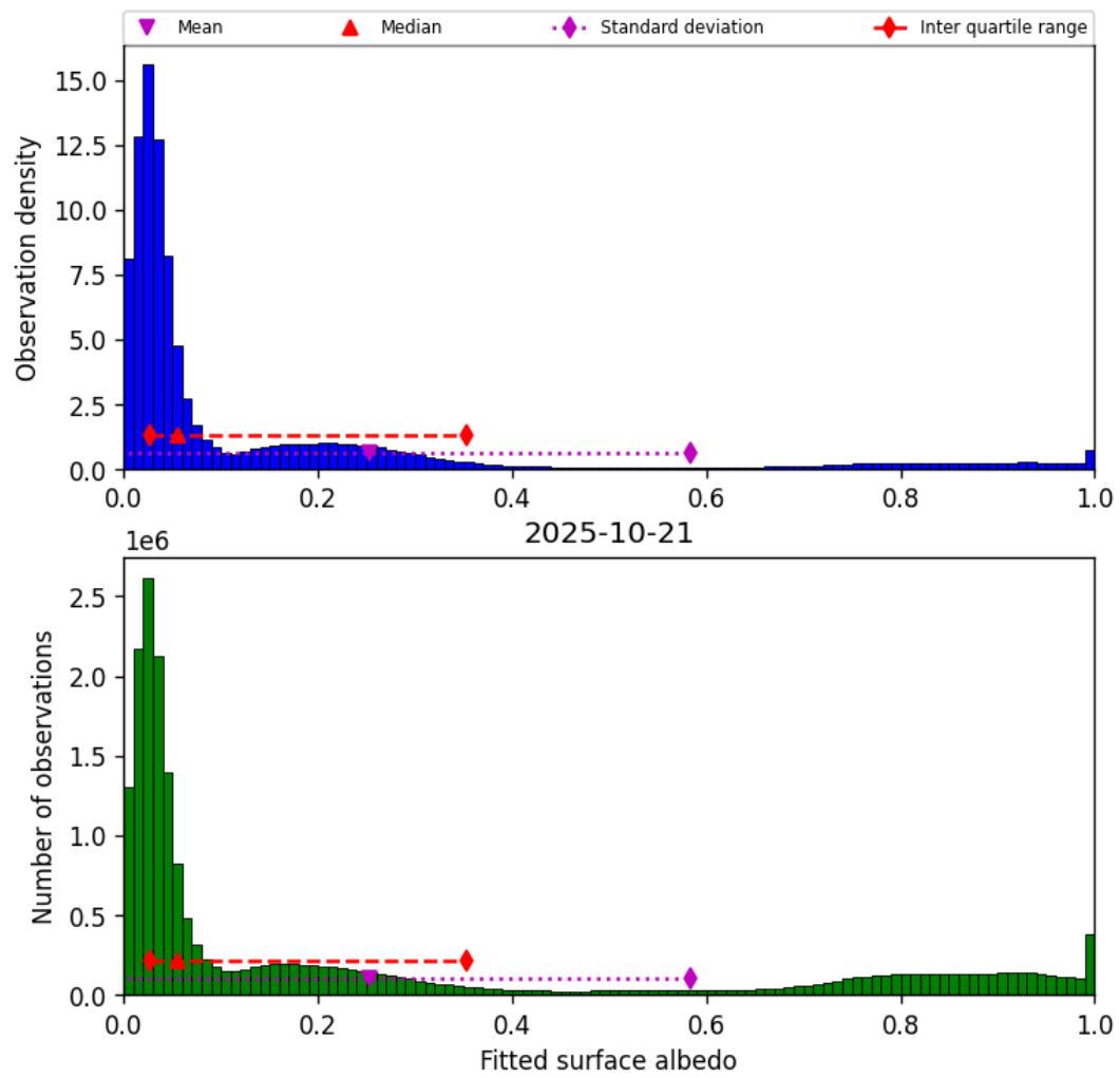
Figure 43: Histogram of “Fitted surface albedo” for 2025-10-21 to 2025-10-22
