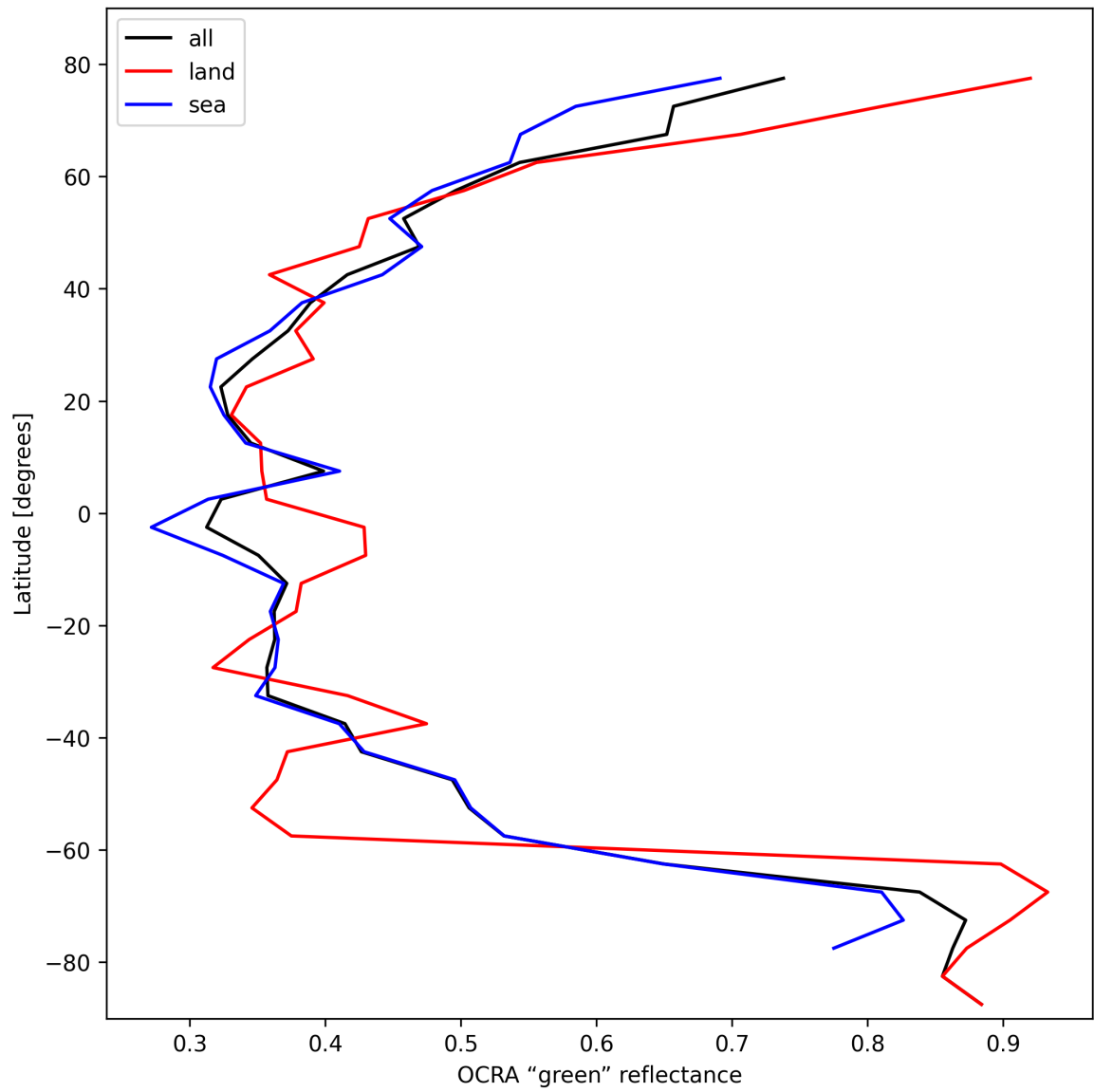
Figure 34: Zonal average of “OCRA “green” reflectance” for 2025-10-21 to 2025-10-22.
