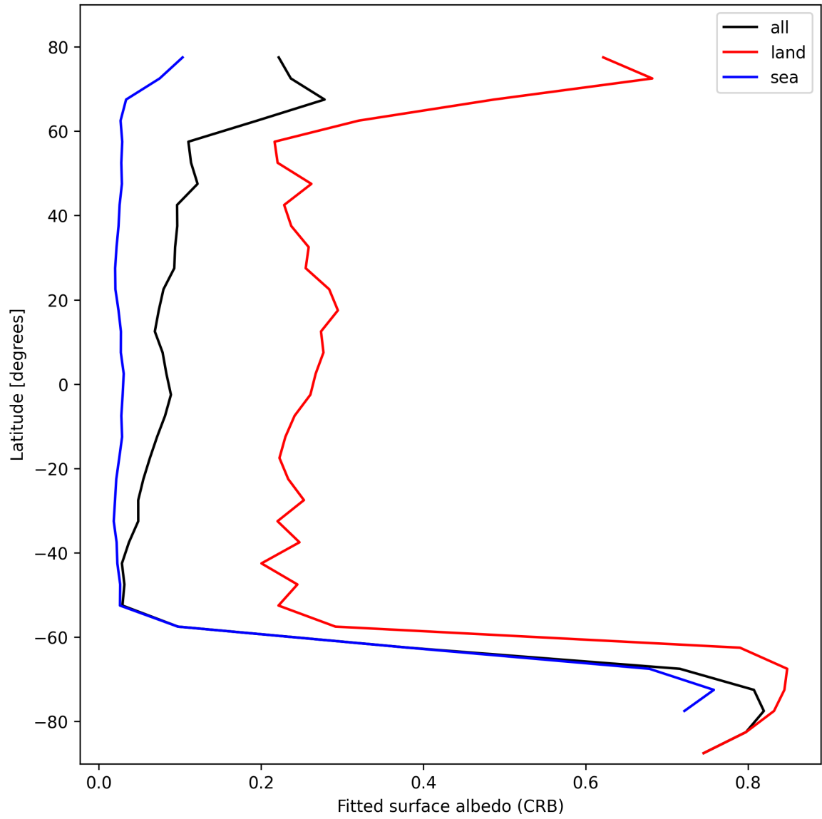
Figure 28: Zonal average of “Fitted surface albedo (CRB)” for 2025-10-21 to 2025-10-22.
