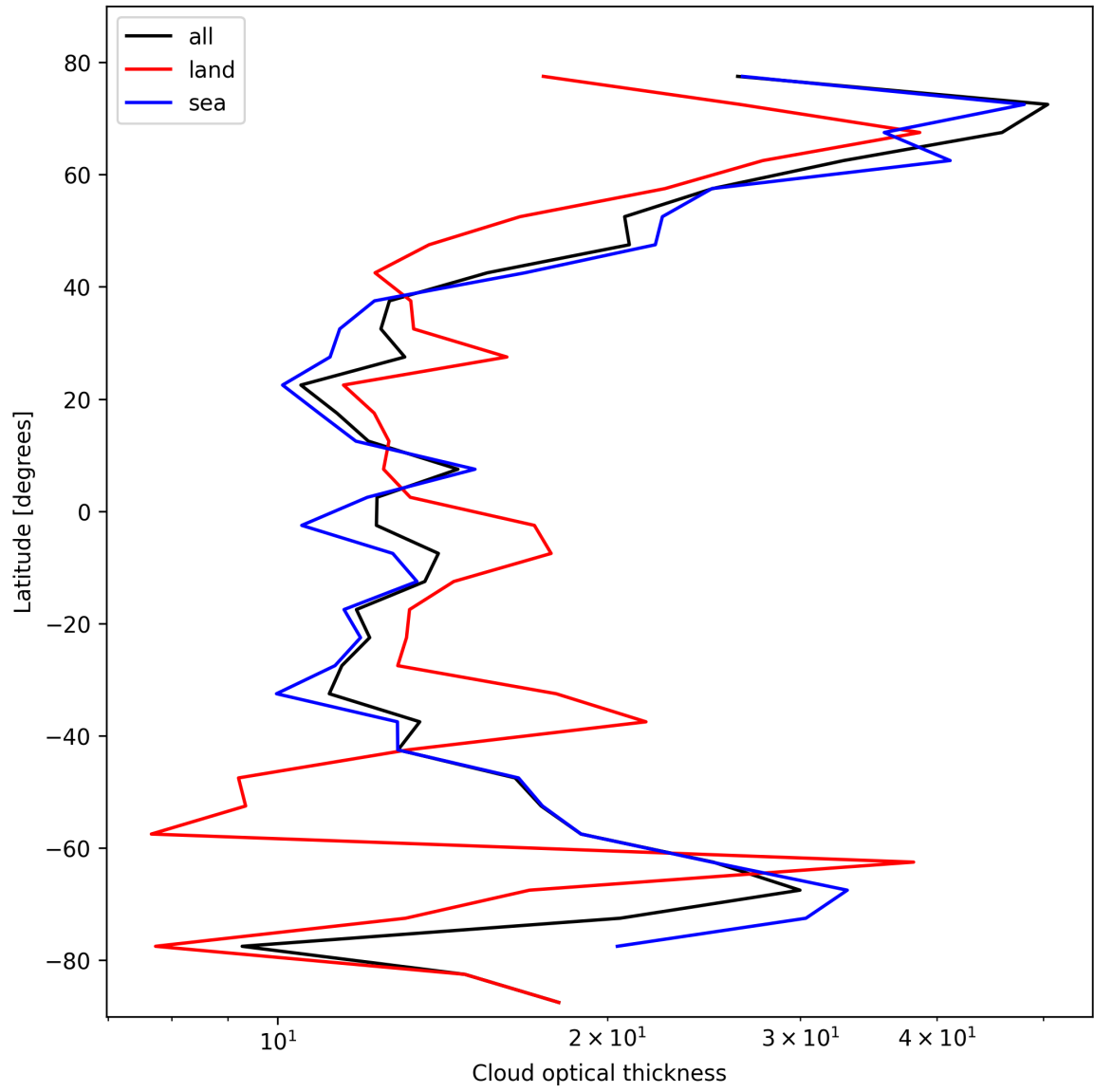
Figure 23: Zonal average of “Cloud optical thickness” for 2025-10-21 to 2025-10-22.
