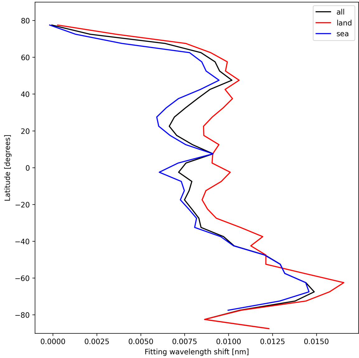
Figure 31: Zonal average of “Fitting wavelength shift” for 2025-10-21 to 2025-10-22.
