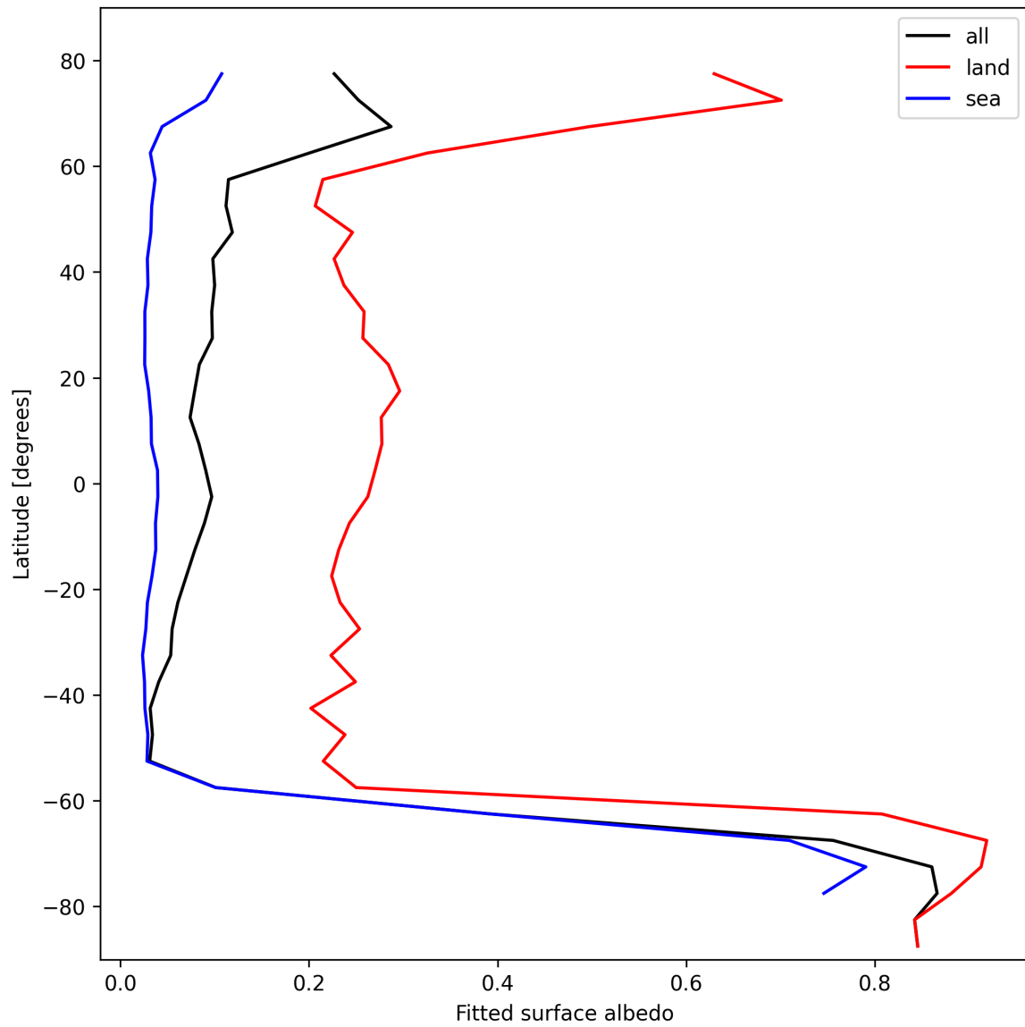
Figure 27: Zonal average of “Fitted surface albedo” for 2025-10-21 to 2025-10-22.
