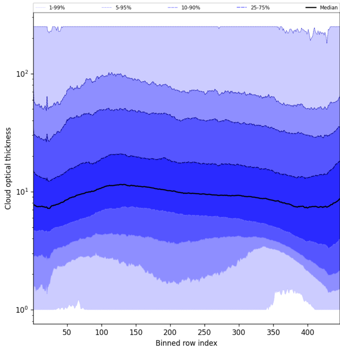
Figure 55: Along track statistics of “Cloud optical thickness” for 2025-10-21 to 2025-10-22
