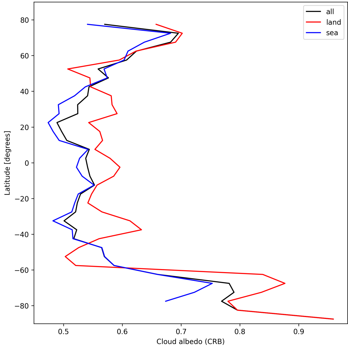
Figure 26: Zonal average of “Cloud albedo (CRB)” for 2025-10-21 to 2025-10-22.
