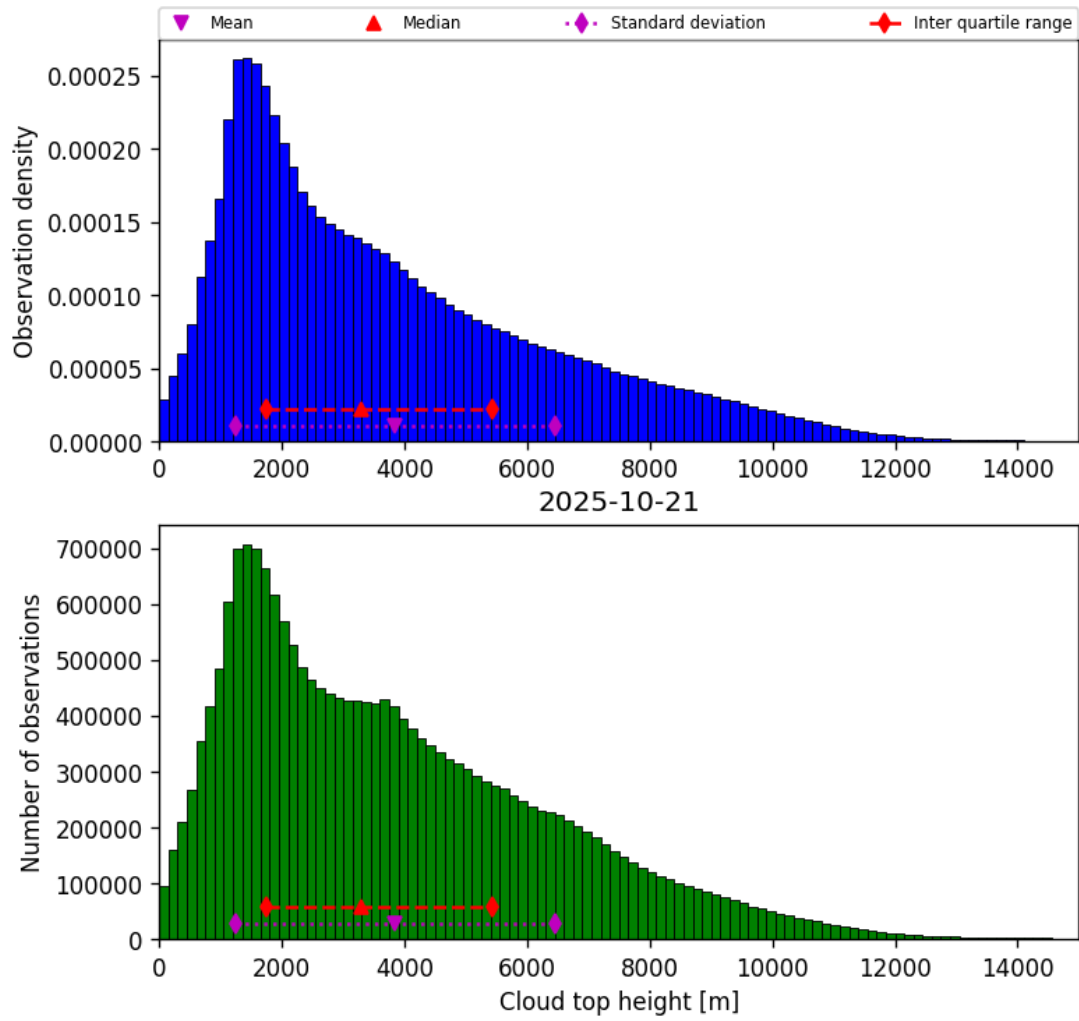
Figure 38: Histogram of “Cloud top height” for 2025-10-21 to 2025-10-22
