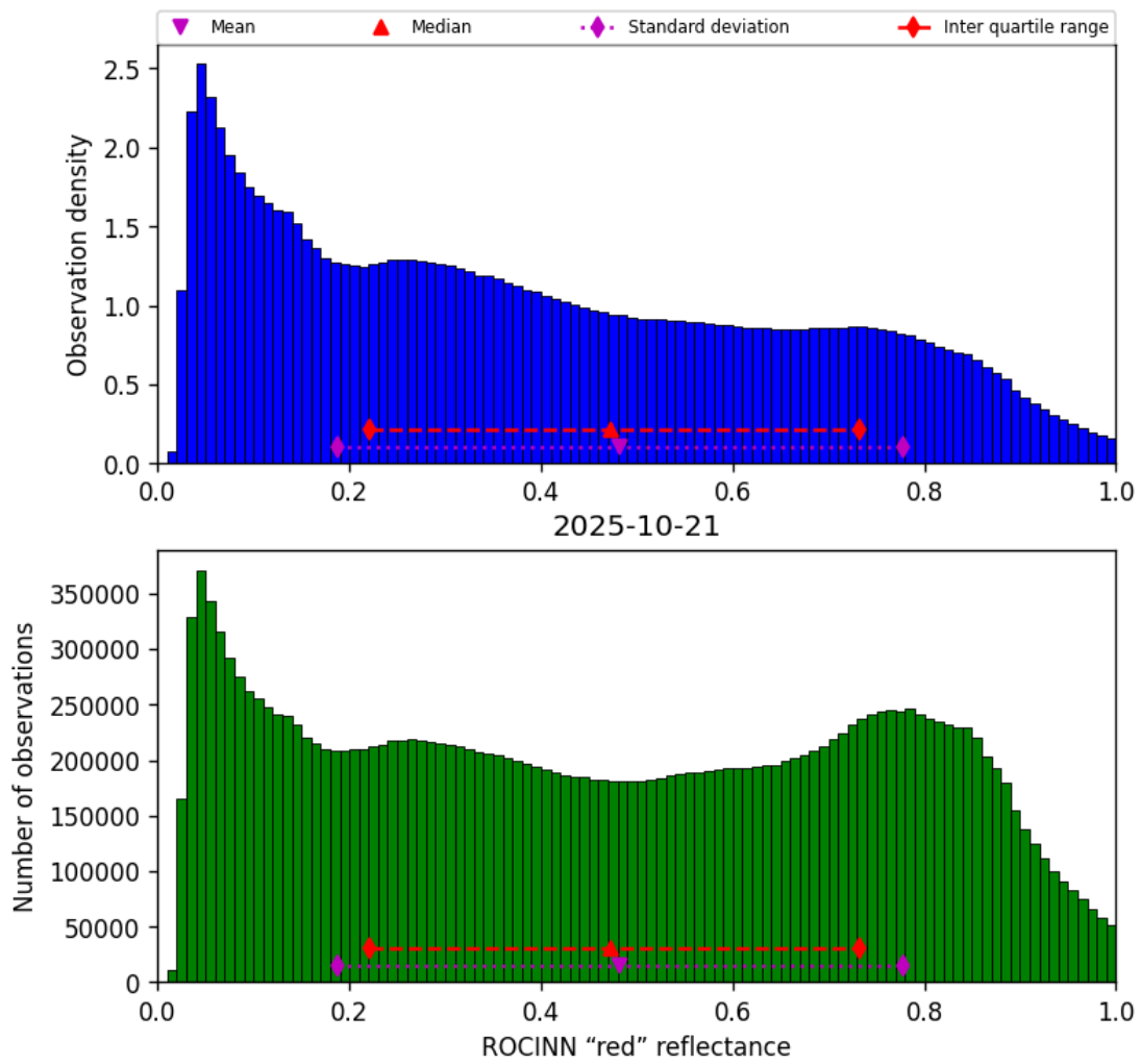
Figure 51: Histogram of “ROCINN “red” reflectance” for 2025-10-21 to 2025-10-22
