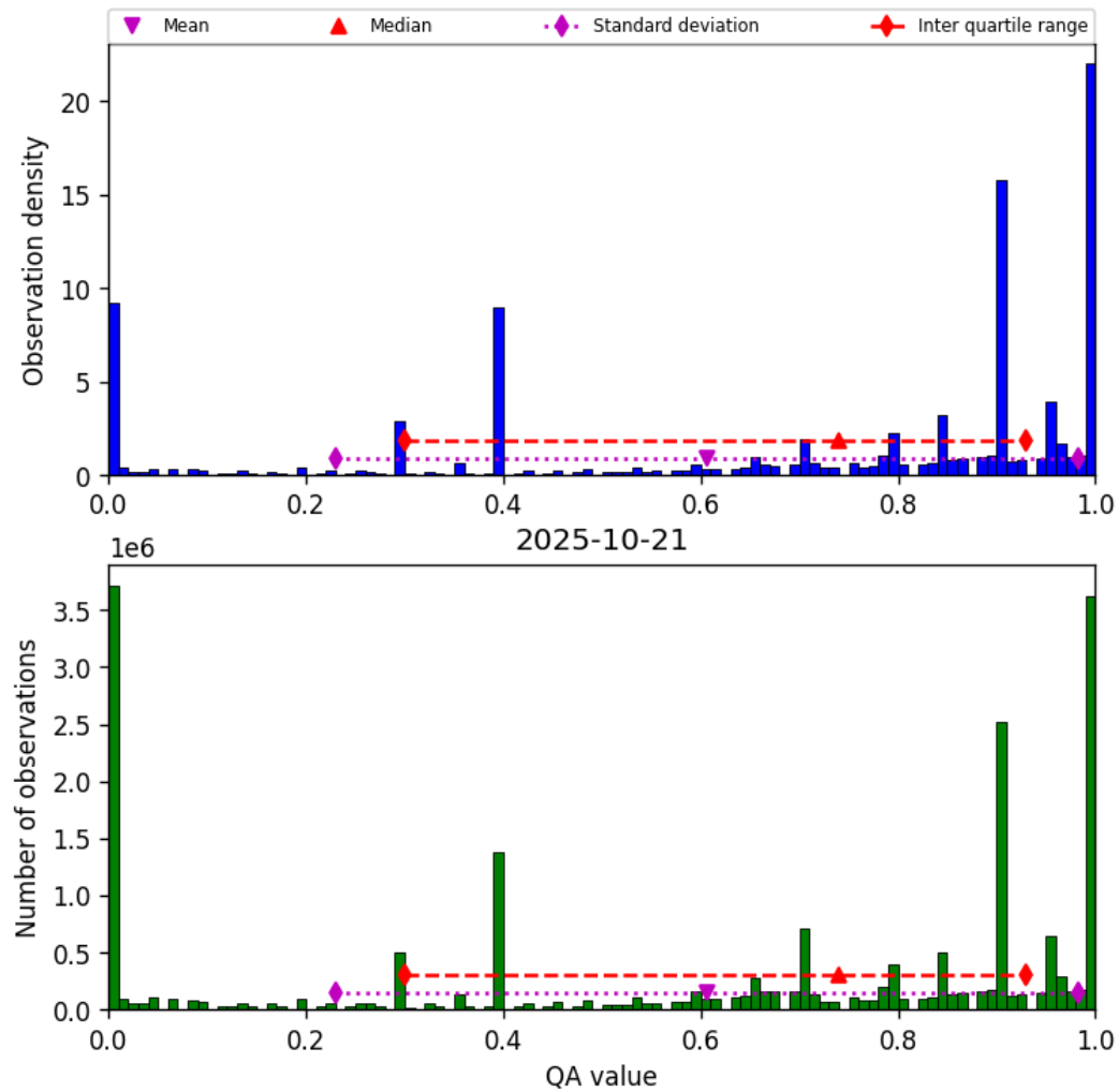
Figure 36: Histogram of “QA value” for 2025-10-21 to 2025-10-22
