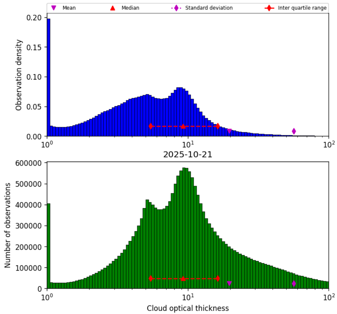
Figure 39: Histogram of “Cloud optical thickness” for 2025-10-21 to 2025-10-22
