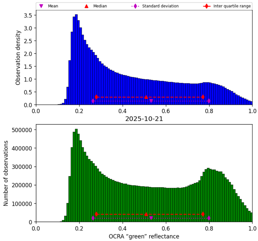
Figure 50: Histogram of “OCRA “green” reflectance” for 2025-10-21 to 2025-10-22
