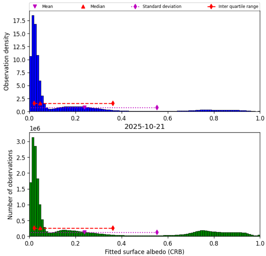
Figure 44: Histogram of “Fitted surface albedo (CRB)” for 2025-10-21 to 2025-10-22
