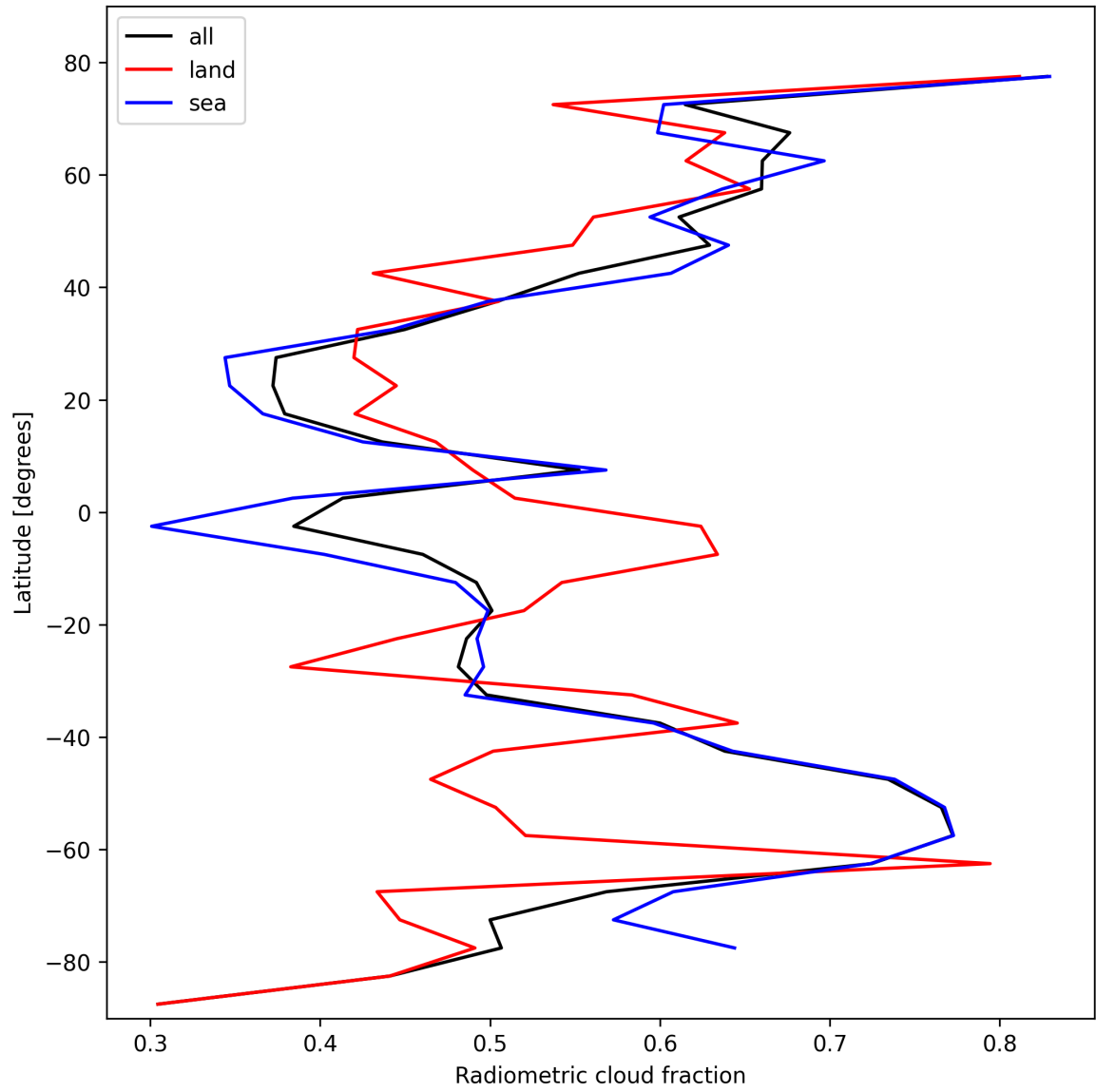
Figure 21: Zonal average of “Radiometric cloud fraction” for 2025-10-21 to 2025-10-22.
