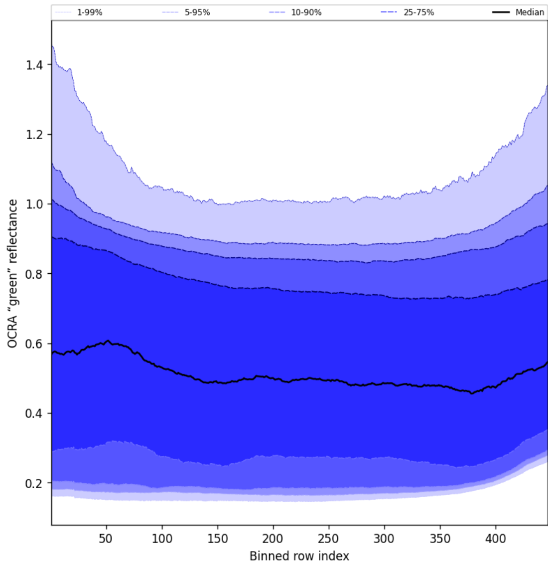
Figure 66: Along track statistics of "OCRA "green" reflectance" for 2025-10-21 to 2025-10-22
