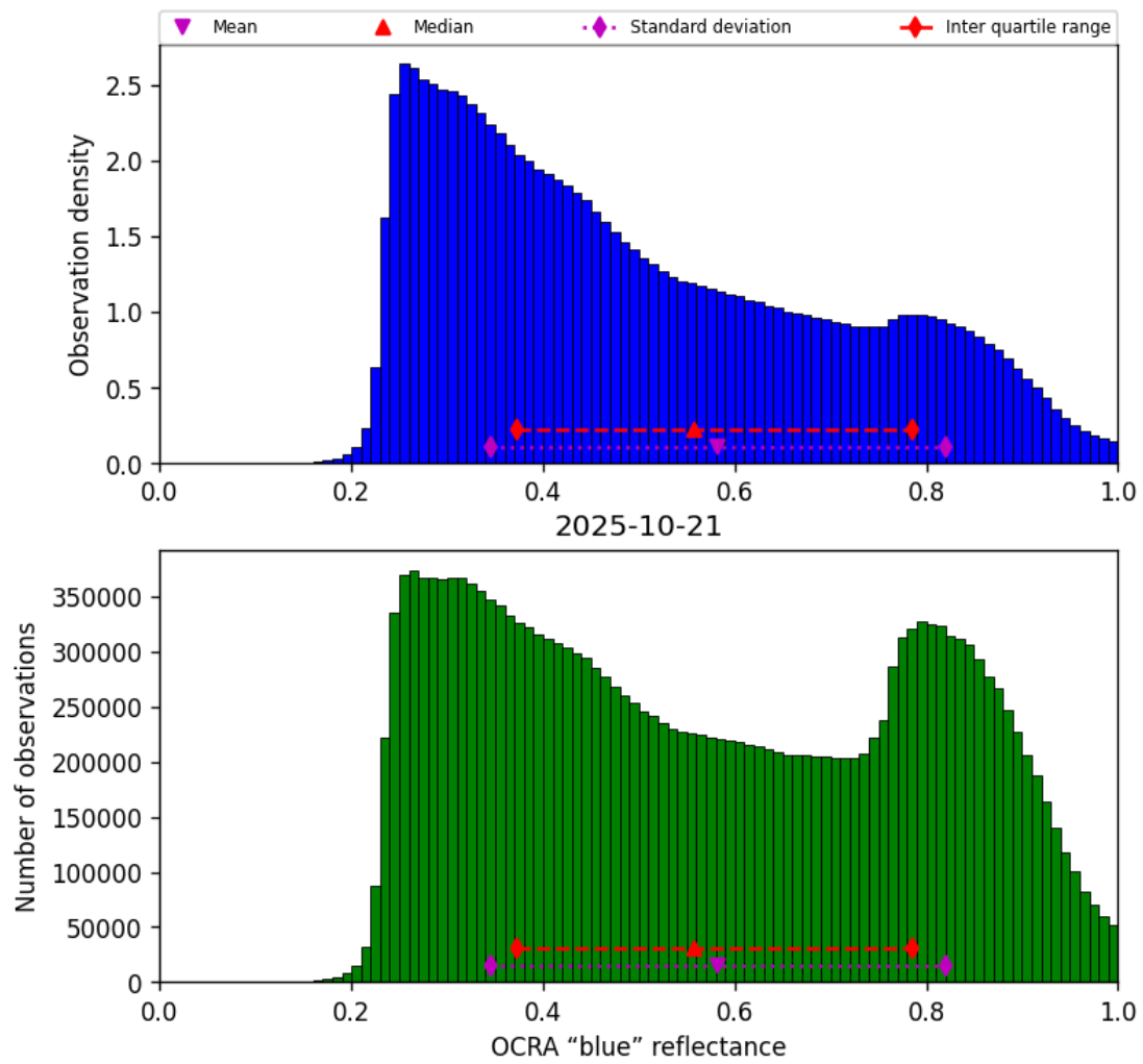
Figure 49: Histogram of “OCRA “blue” reflectance” for 2025-10-21 to 2025-10-22
