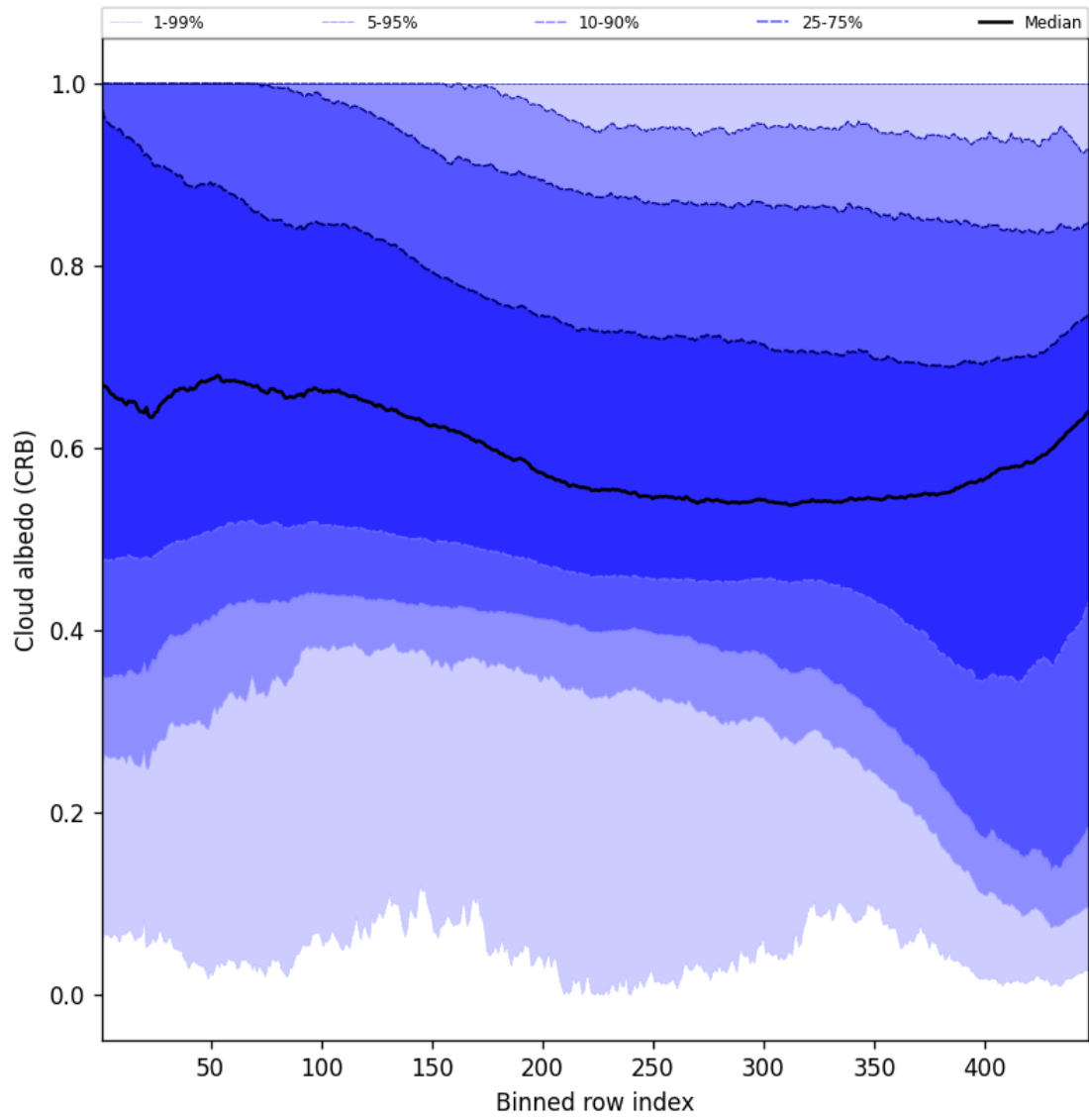
Figure 58: Along track statistics of “Cloud albedo (CRB)” for 2025-10-21 to 2025-10-22
