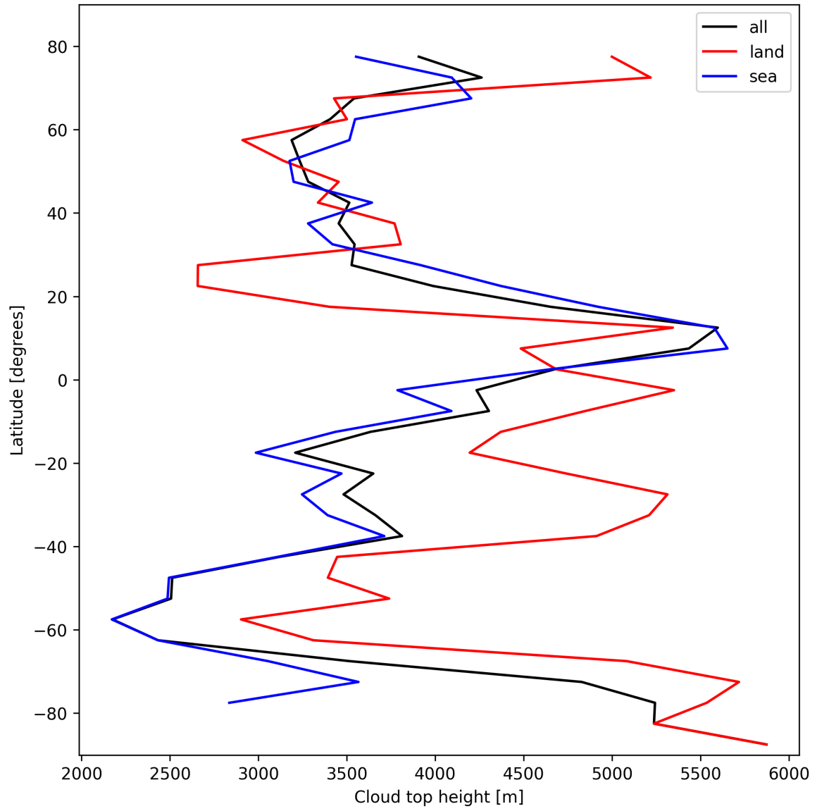
Figure 22: Zonal average of “Cloud top height” for 2025-10-21 to 2025-10-22.
