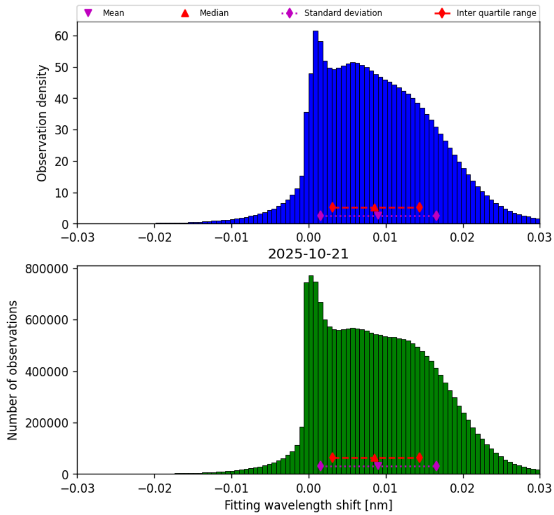
Figure 47: Histogram of “Fitting wavelength shift” for 2025-10-21 to 2025-10-22
