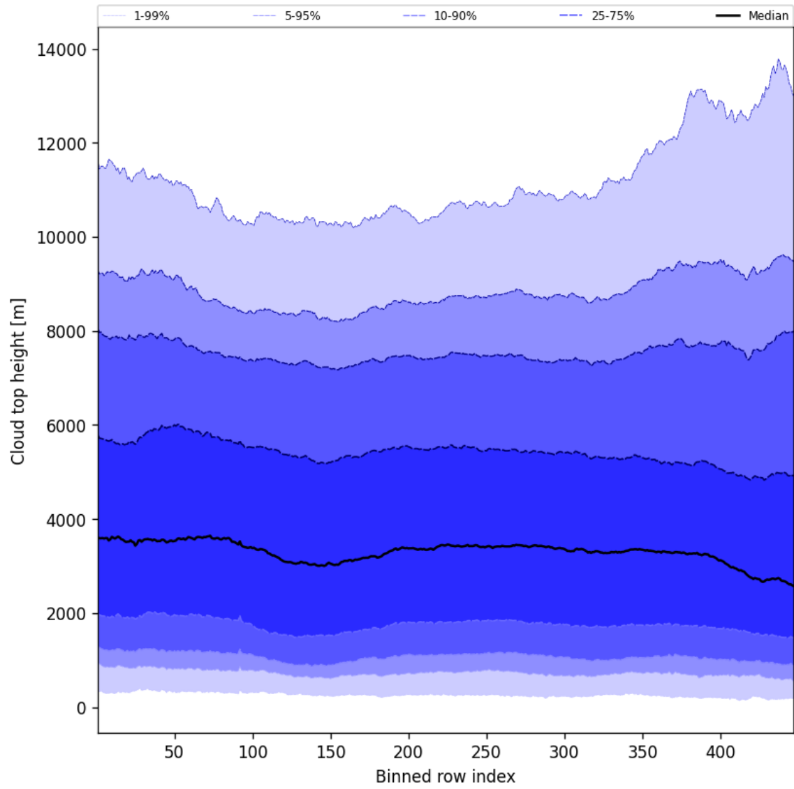
Figure 54: Along track statistics of “Cloud top height” for 2025-10-21 to 2025-10-22
