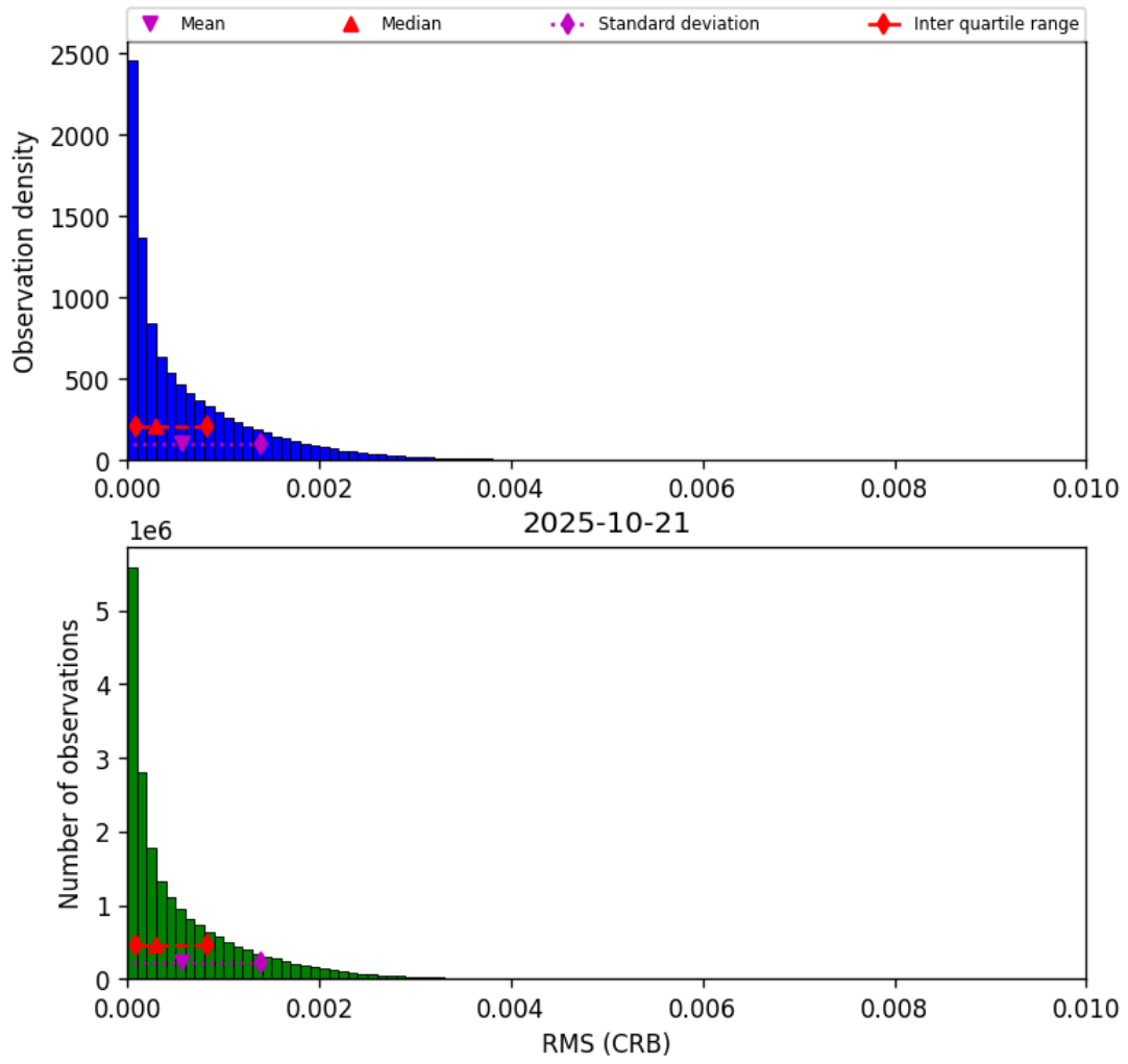
Figure 46: Histogram of “RMS (CRB)” for 2025-10-21 to 2025-10-22
