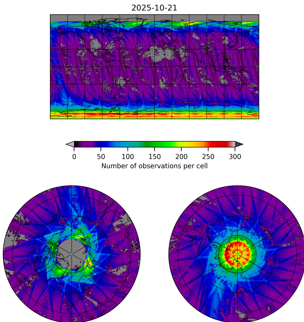
Figure 19: Map of the number of observations for 2025-10-21 to 2025-10-22
