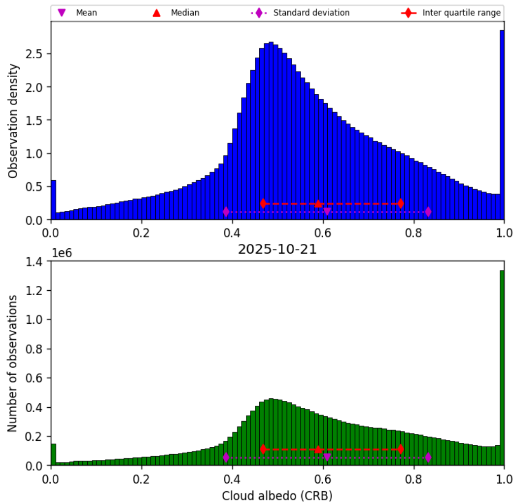
Figure 42: Histogram of “Cloud albedo (CRB)” for 2025-10-21 to 2025-10-22
