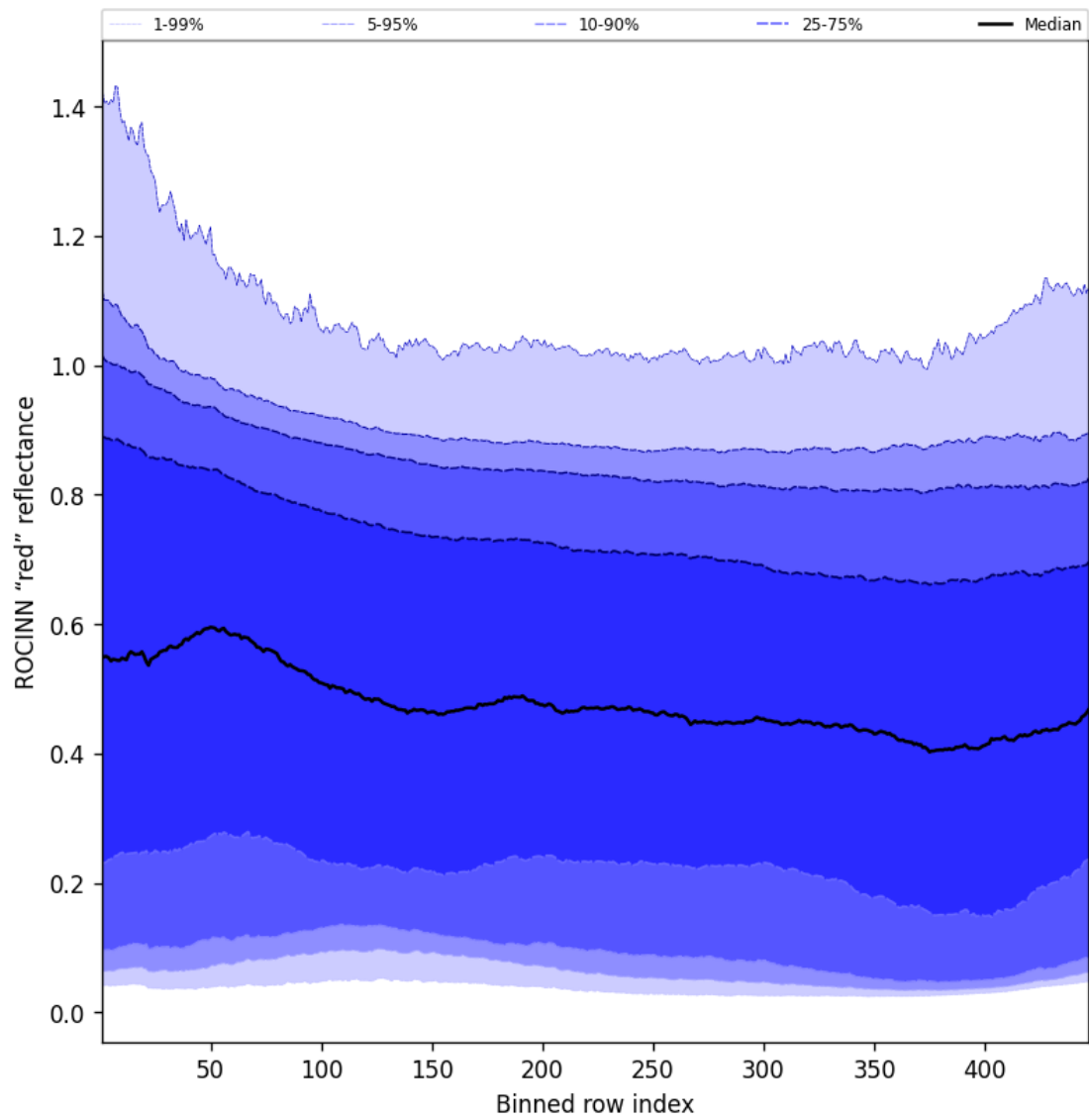
Figure 67: Along track statistics of "ROCINN "red" reflectance" for 2025-10-21 to 2025-10-22
