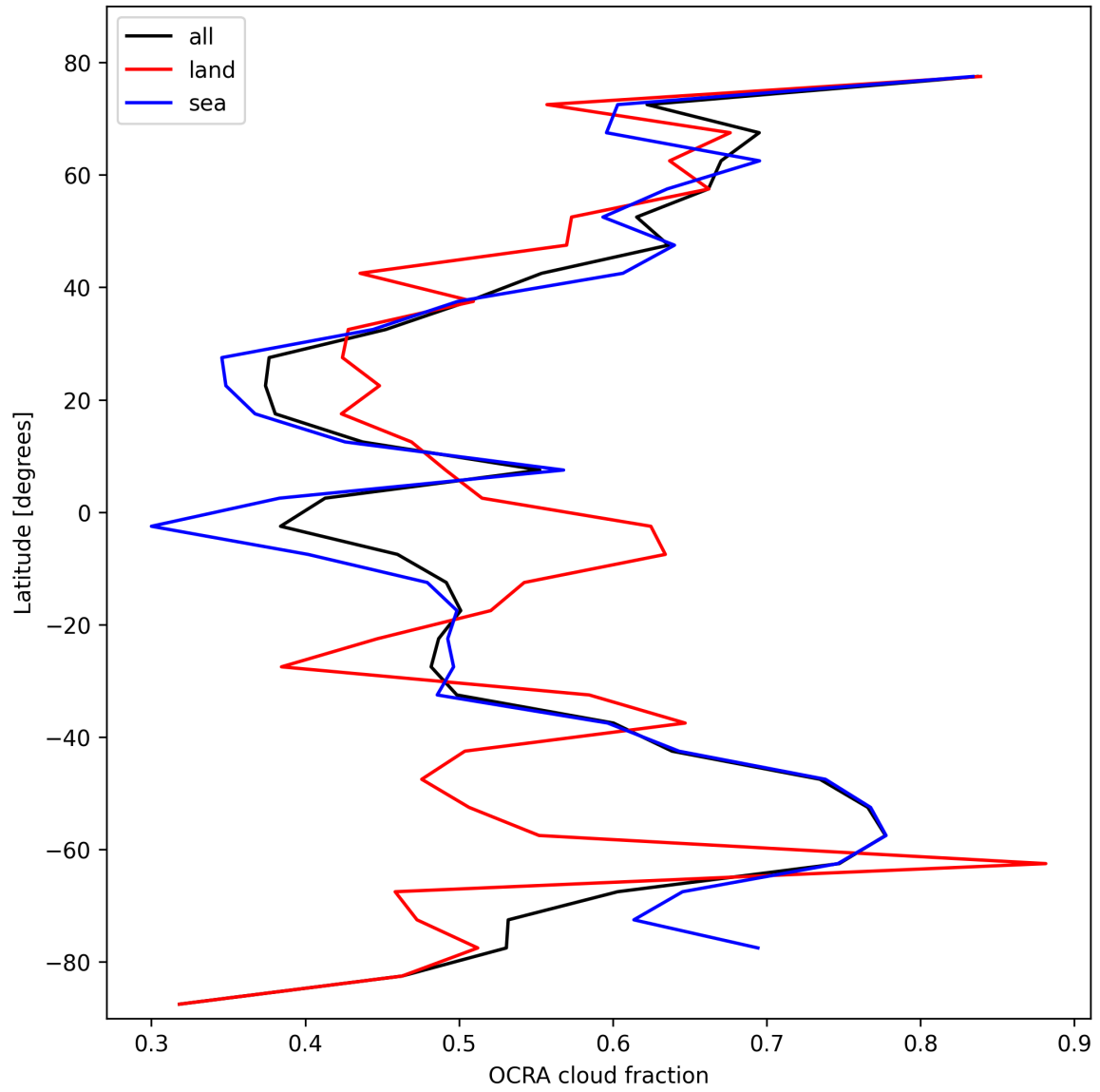
Figure 32: Zonal average of “OCRA cloud fraction” for 2025-10-21 to 2025-10-22.
