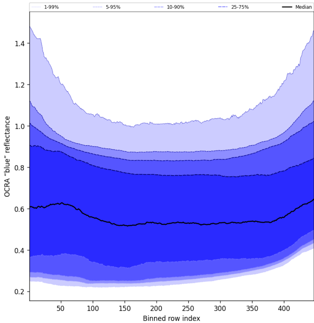
Figure 65: Along track statistics of “OCRA “blue” reflectance” for 2025-10-21 to 2025-10-22
