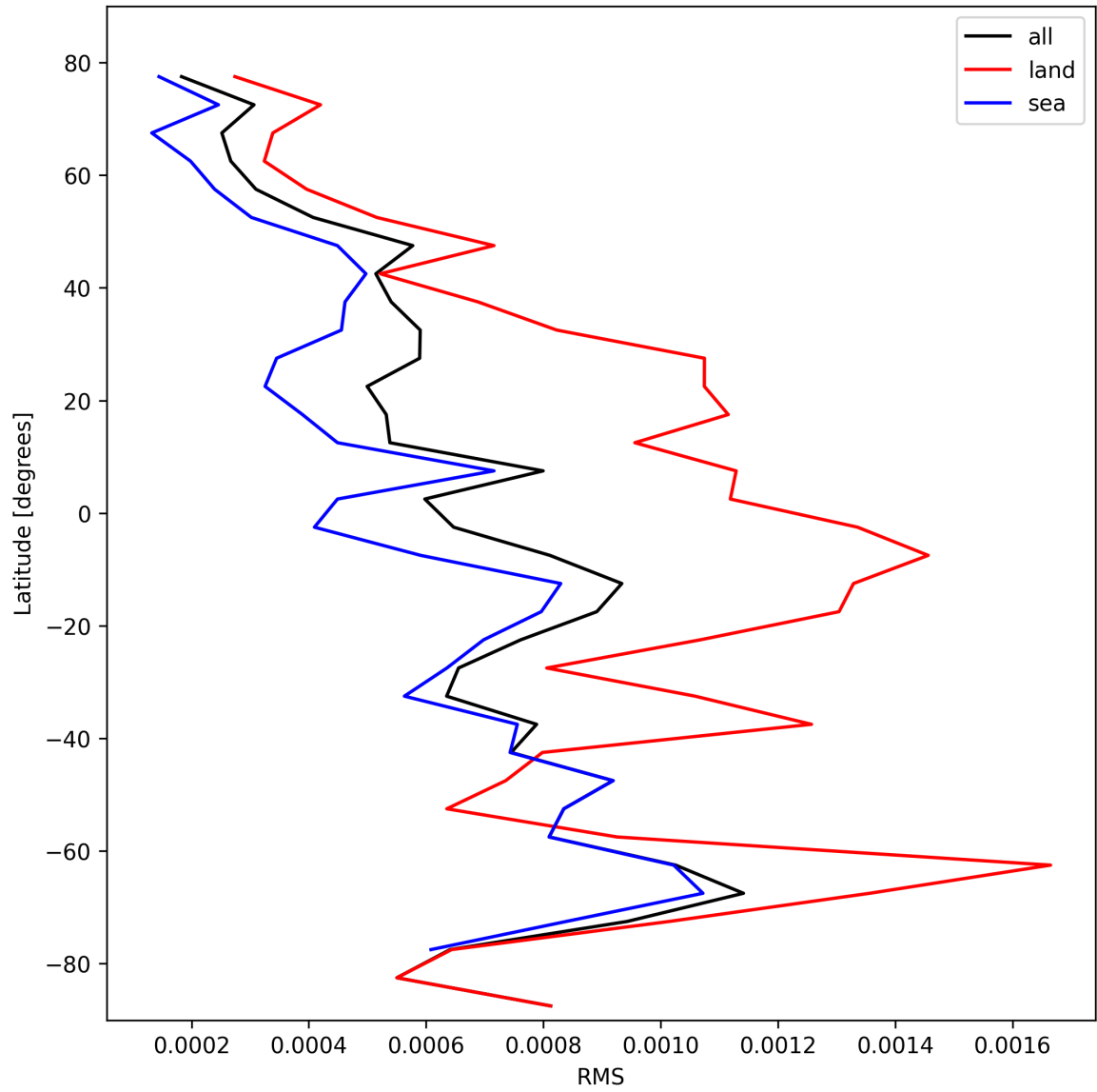
Figure 29: Zonal average of “RMS” for 2025-10-21 to 2025-10-22.
