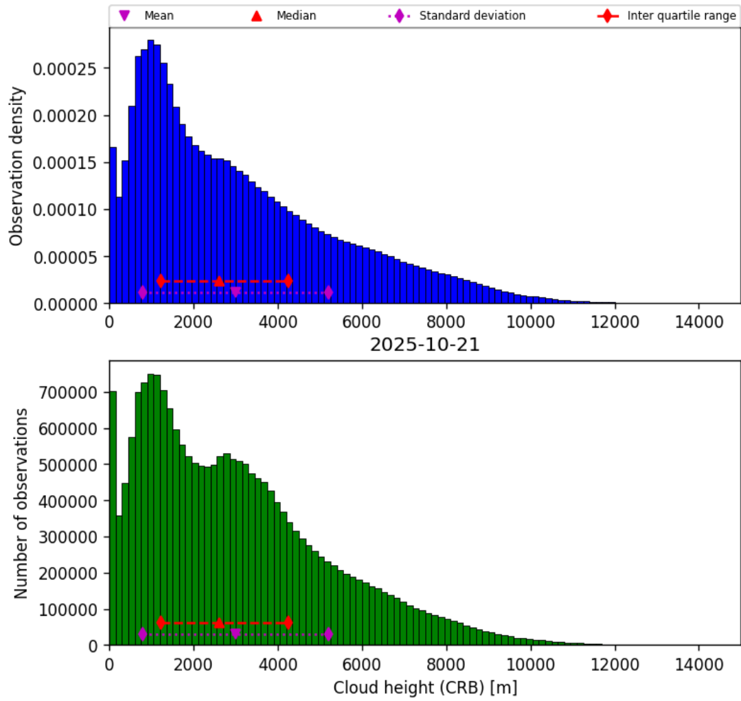
Figure 41: Histogram of “Cloud height (CRB)” for 2025-10-21 to 2025-10-22
