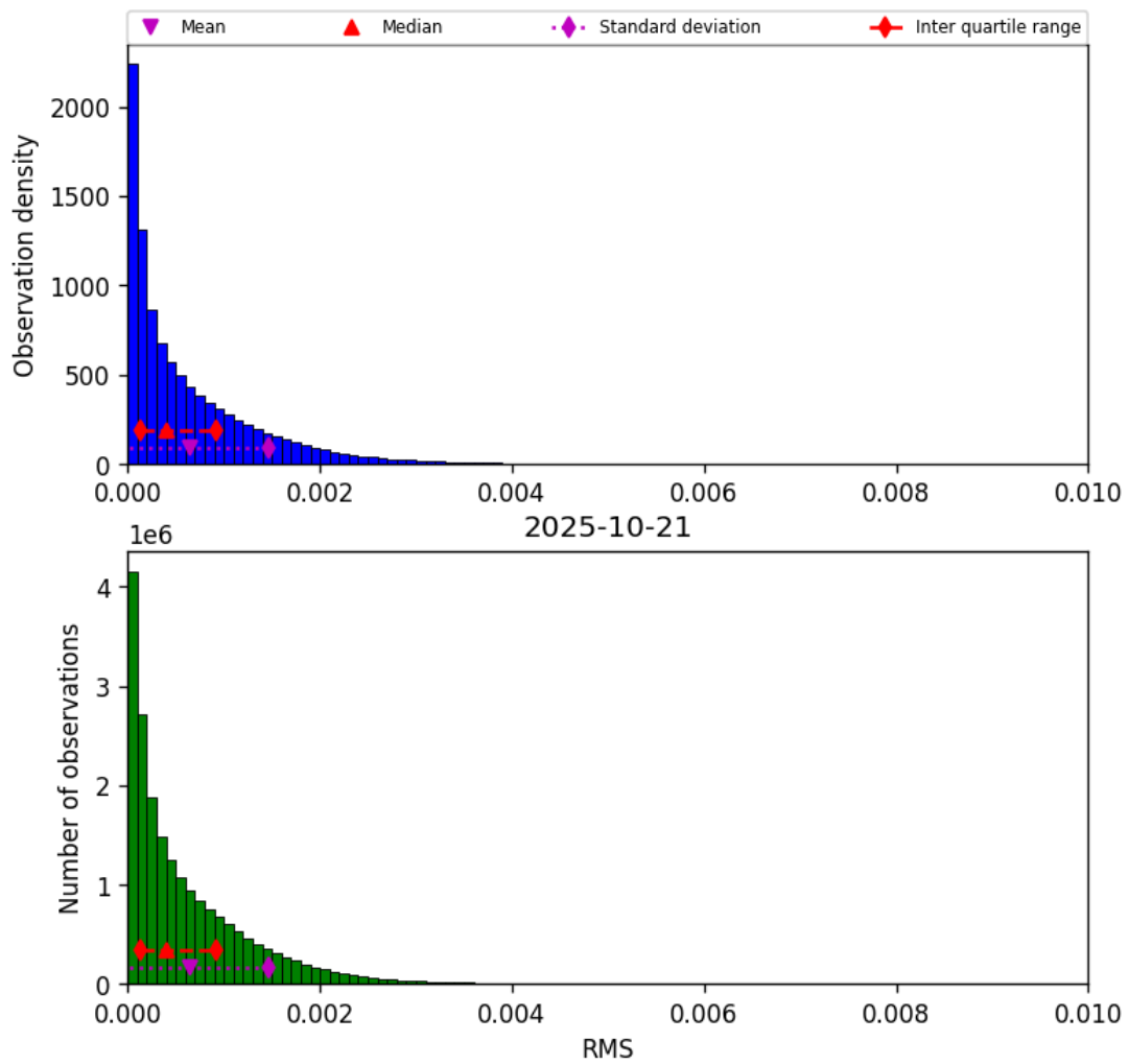
Figure 45: Histogram of “RMS” for 2025-10-21 to 2025-10-22
