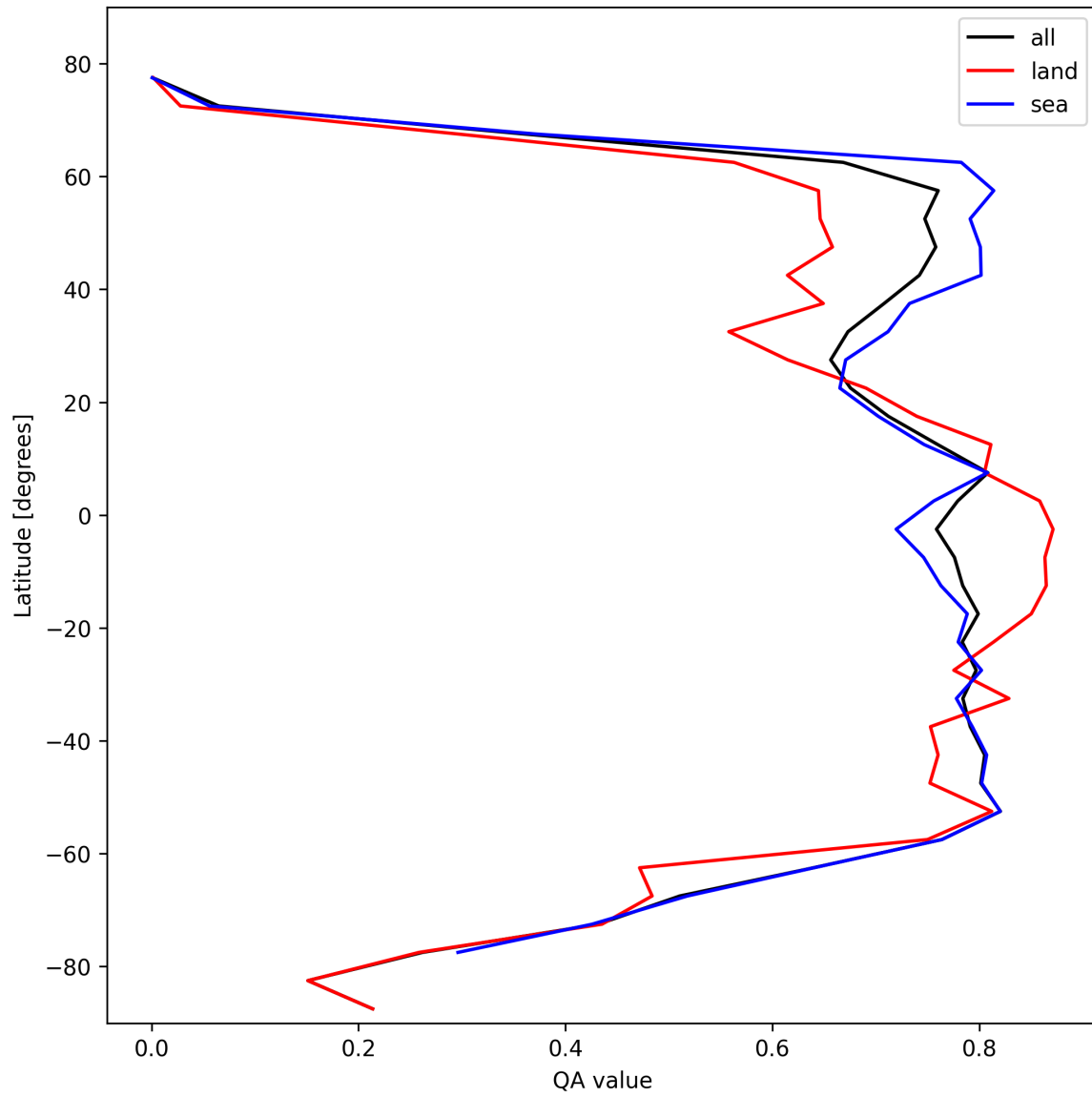
Figure 20: Zonal average of “QA value” for 2025-10-21 to 2025-10-22.
