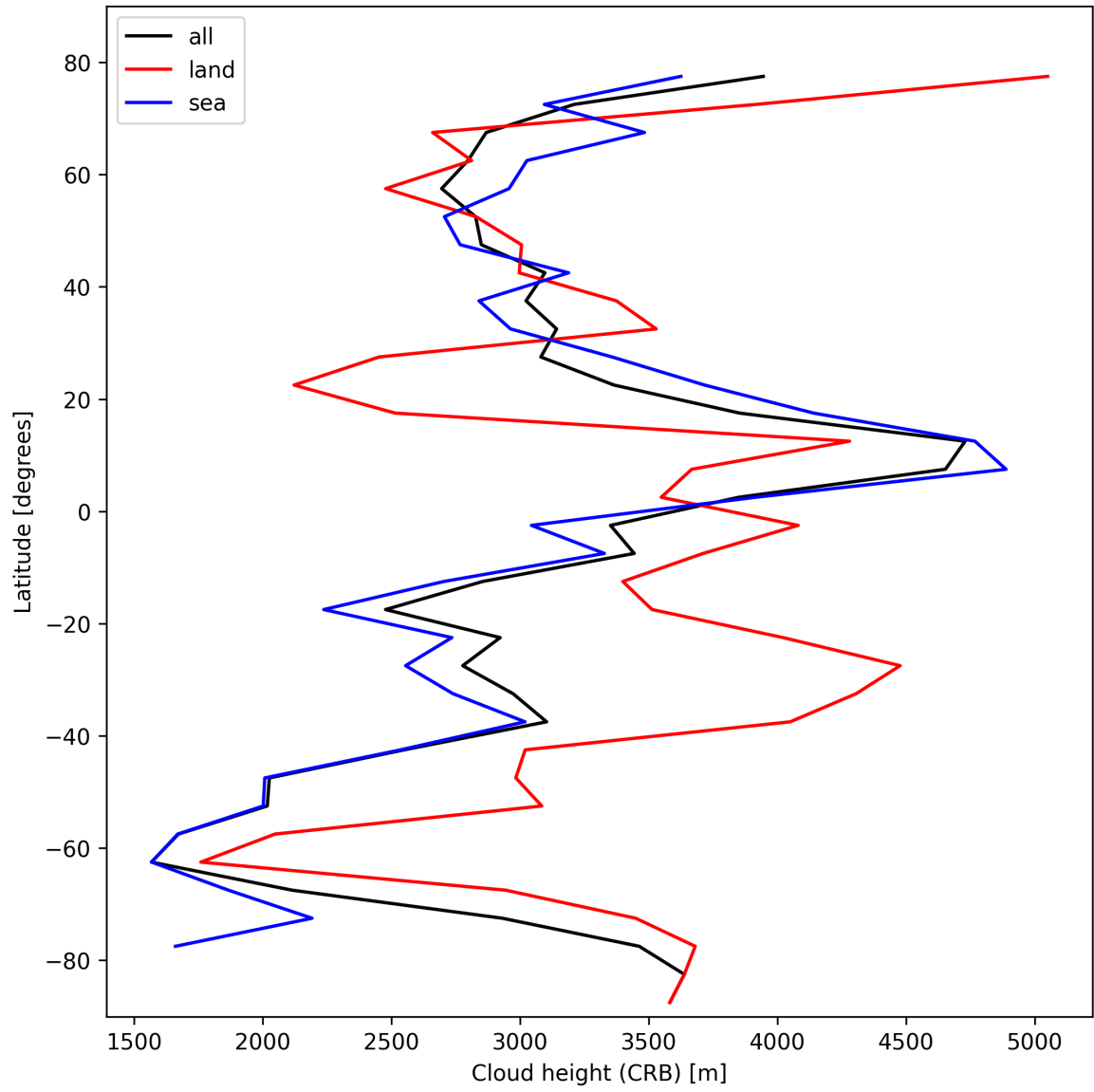
Figure 25: Zonal average of “Cloud height (CRB)” for 2025-10-21 to 2025-10-22.
