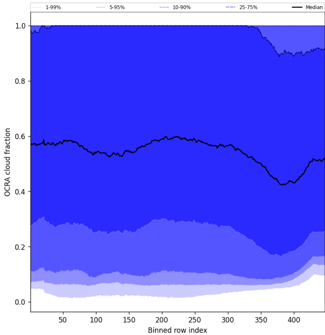
Figure 64: Along track statistics of “OCRA cloud fraction” for 2025-10-21 to 2025-10-22
