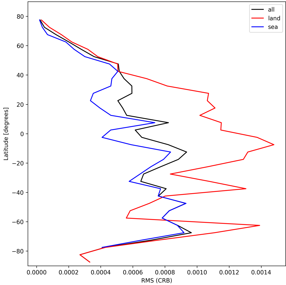
Figure 30: Zonal average of “RMS (CRB)” for 2025-10-21 to 2025-10-22.
