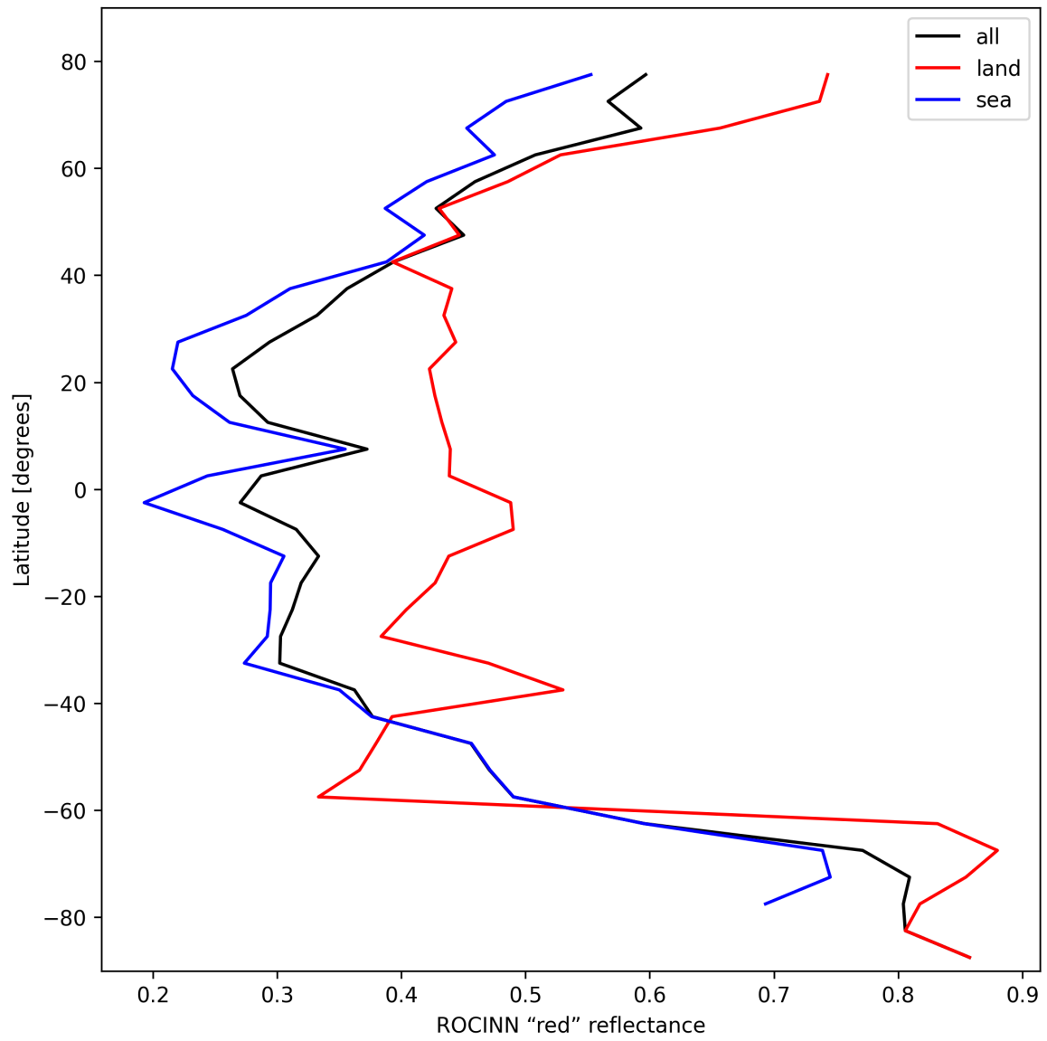
Figure 35: Zonal average of “ROCINN “red” reflectance” for 2025-10-21 to 2025-10-22.
