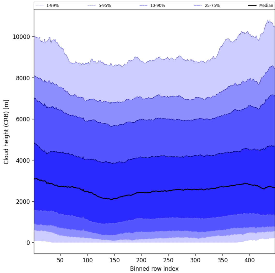
Figure 57: Along track statistics of “Cloud height (CRB)” for 2025-10-21 to 2025-10-22
