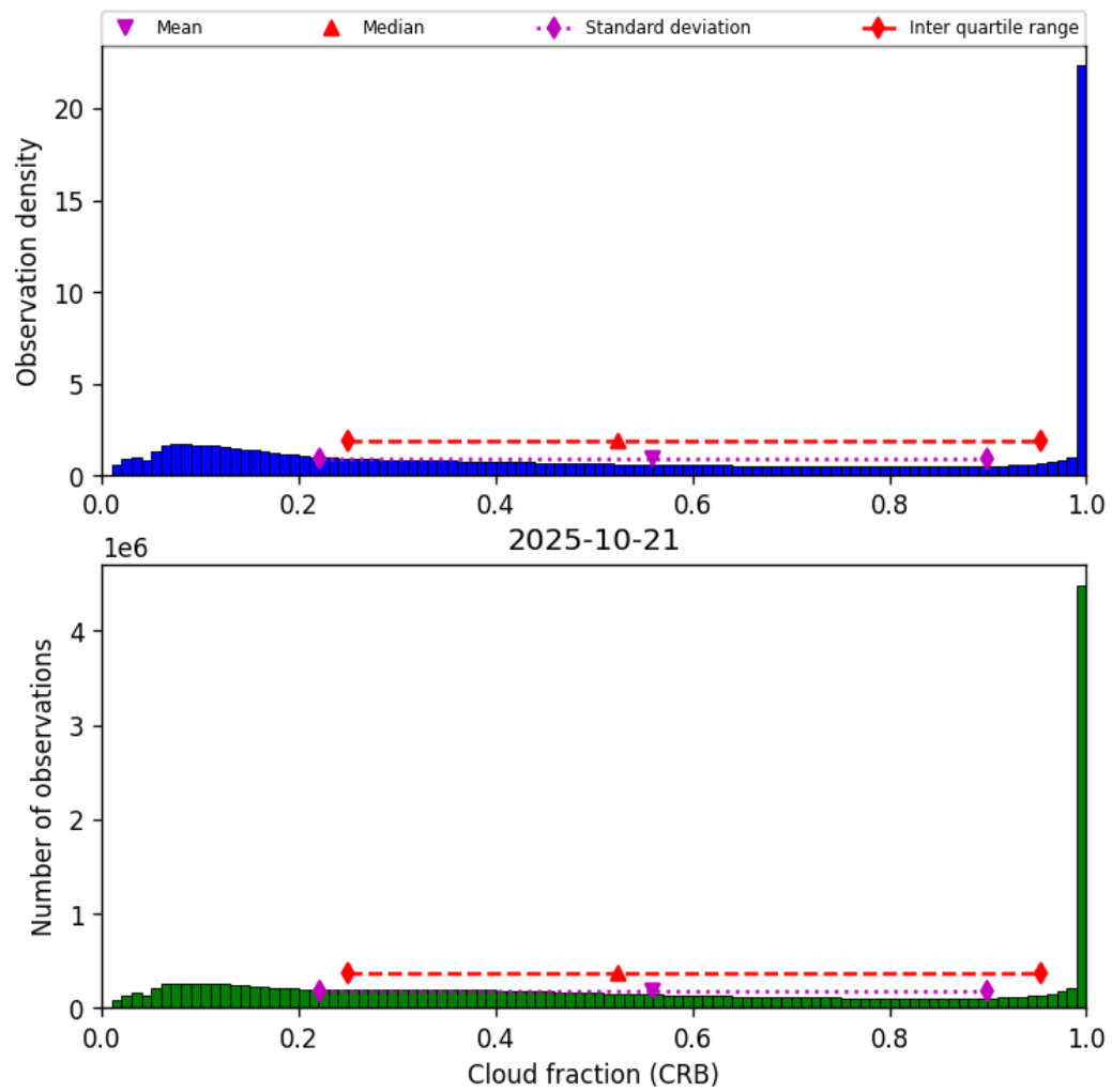
Figure 40: Histogram of “Cloud fraction (CRB)” for 2025-10-21 to 2025-10-22
