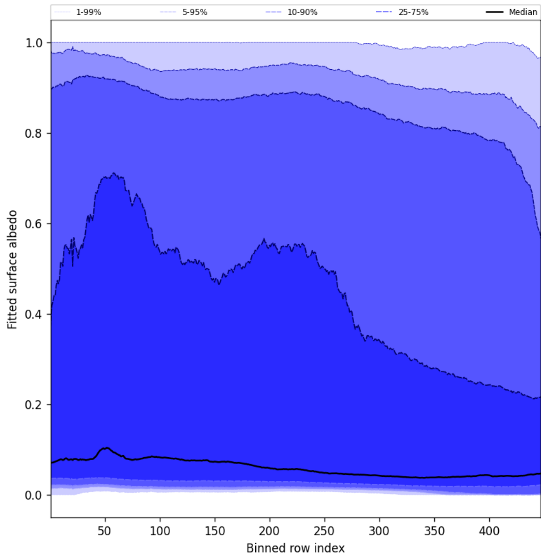
Figure 59: Along track statistics of “Fitted surface albedo” for 2025-10-21 to 2025-10-22
