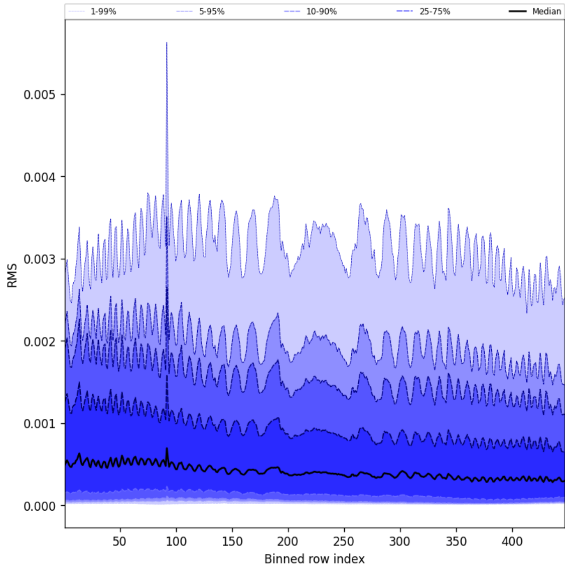
Figure 61: Along track statistics of “RMS” for 2025-10-21 to 2025-10-22
