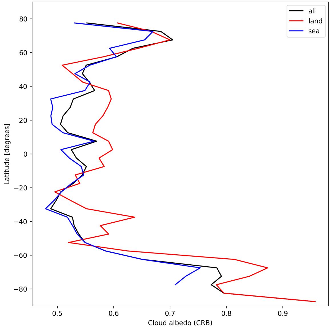
Figure 26: Zonal average of “Cloud albedo (CRB)” for 2025-10-22 to 2025-10-23.
