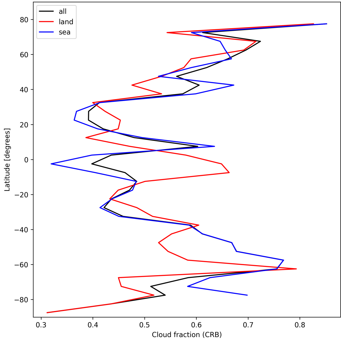
Figure 24: Zonal average of “Cloud fraction (CRB)” for 2025-10-22 to 2025-10-23.
