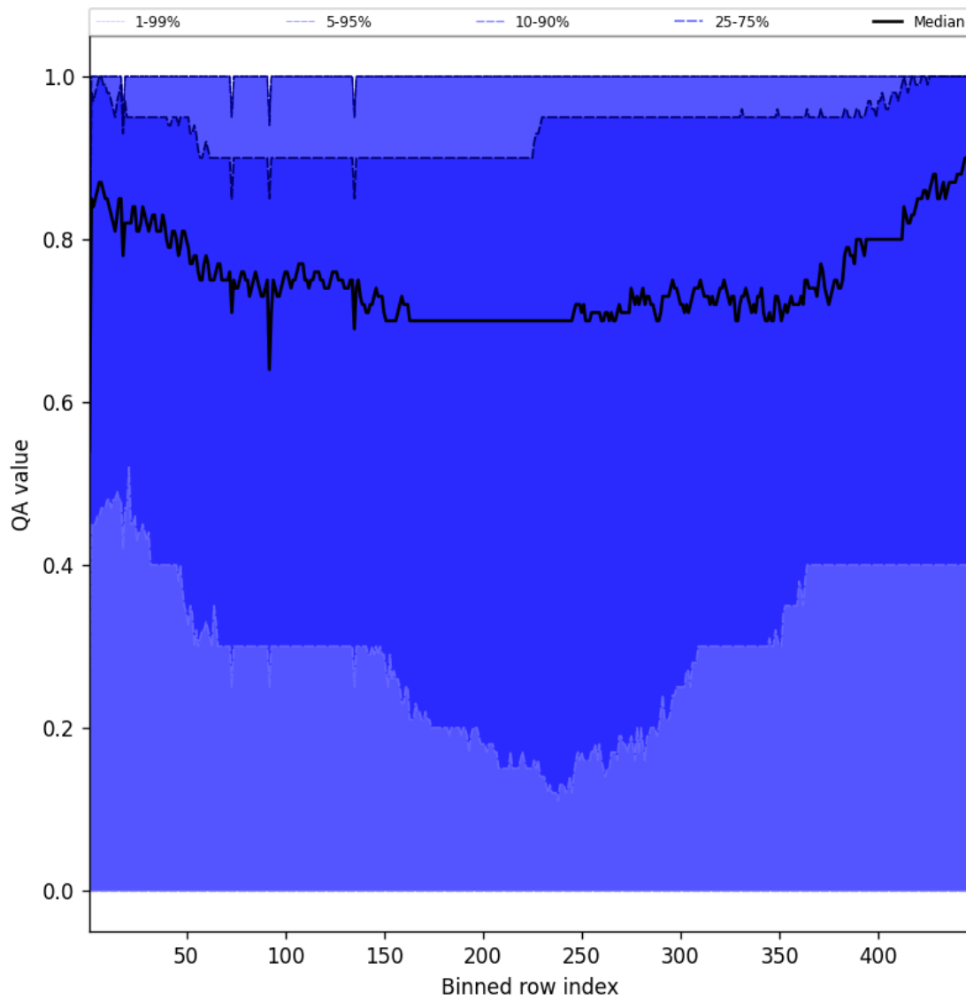
Figure 52: Along track statistics of “QA value” for 2025-10-22 to 2025-10-23
