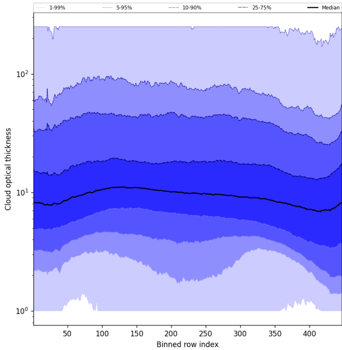
Figure 55: Along track statistics of “Cloud optical thickness” for 2025-10-22 to 2025-10-23
