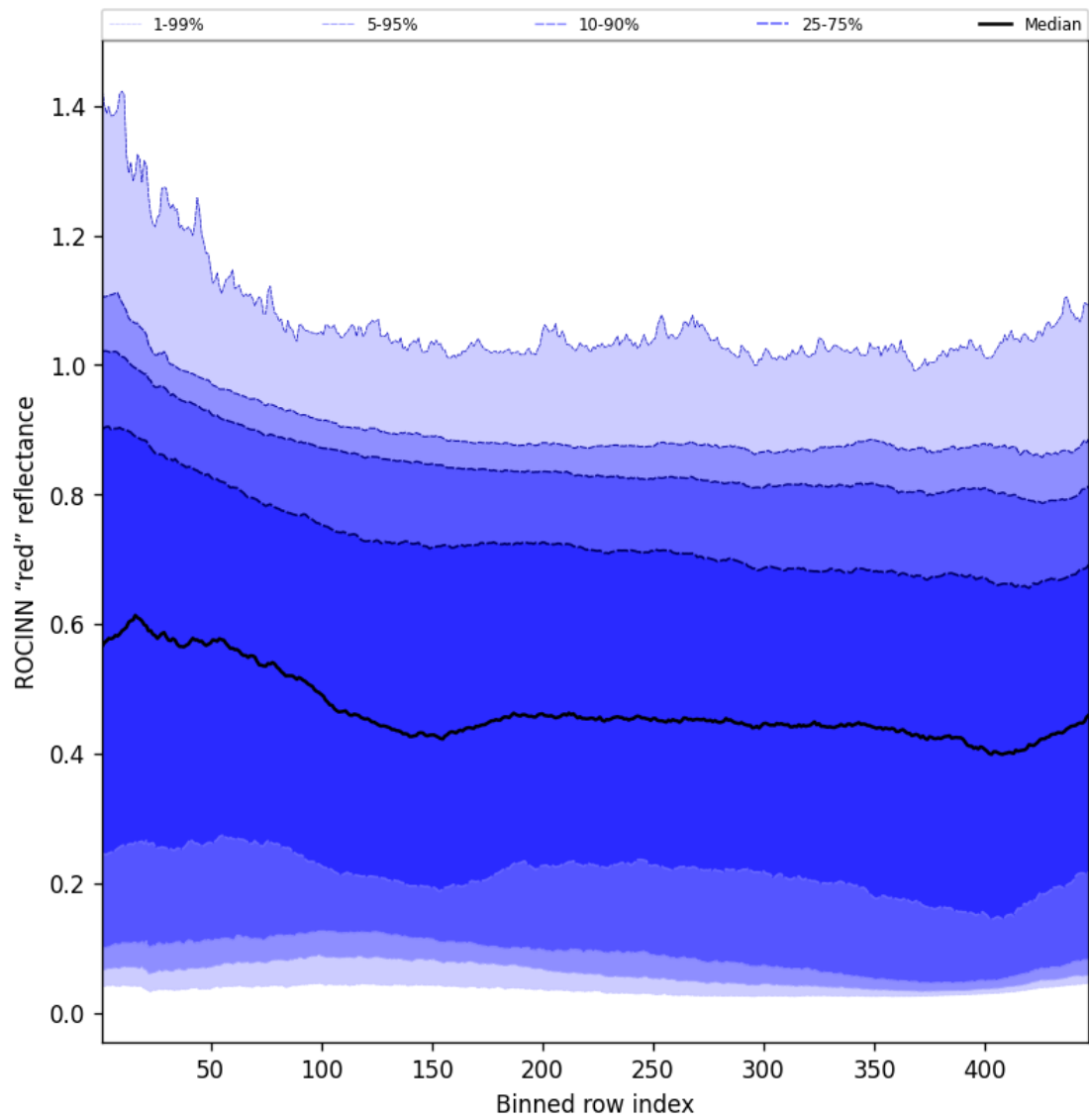
Figure 67: Along track statistics of "ROCINN "red" reflectance" for 2025-10-22 to 2025-10-23
