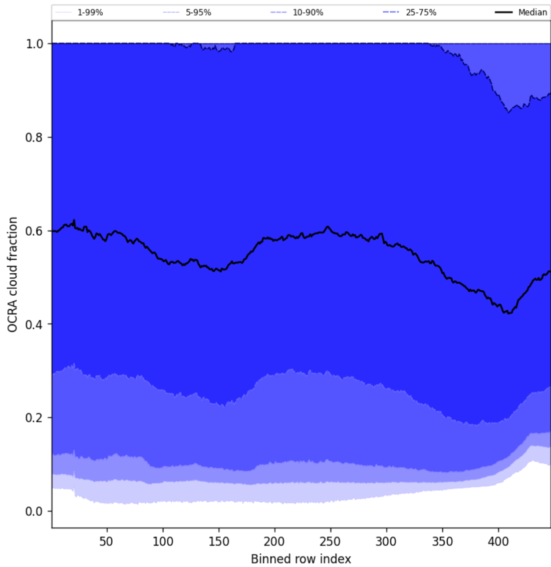
Figure 64: Along track statistics of “OCRA cloud fraction” for 2025-10-22 to 2025-10-23
