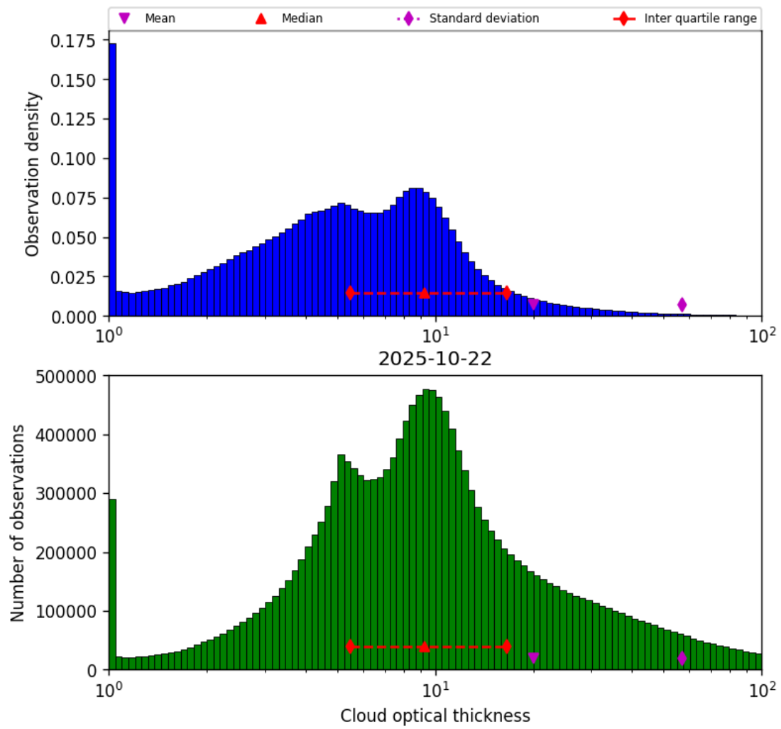
Figure 39: Histogram of “Cloud optical thickness” for 2025-10-22 to 2025-10-23
