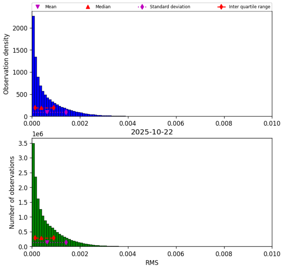
Figure 45: Histogram of “RMS” for 2025-10-22 to 2025-10-23
