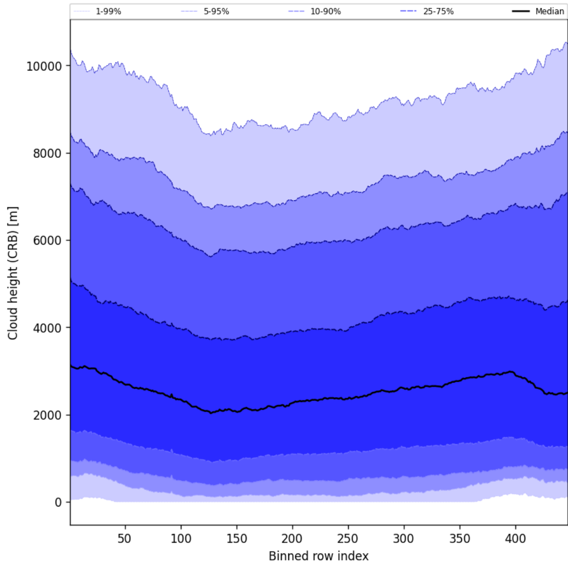
Figure 57: Along track statistics of “Cloud height (CRB)” for 2025-10-22 to 2025-10-23
