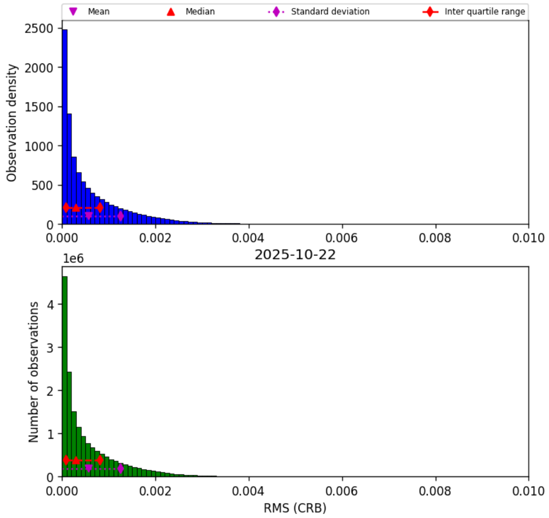
Figure 46: Histogram of “RMS (CRB)” for 2025-10-22 to 2025-10-23
