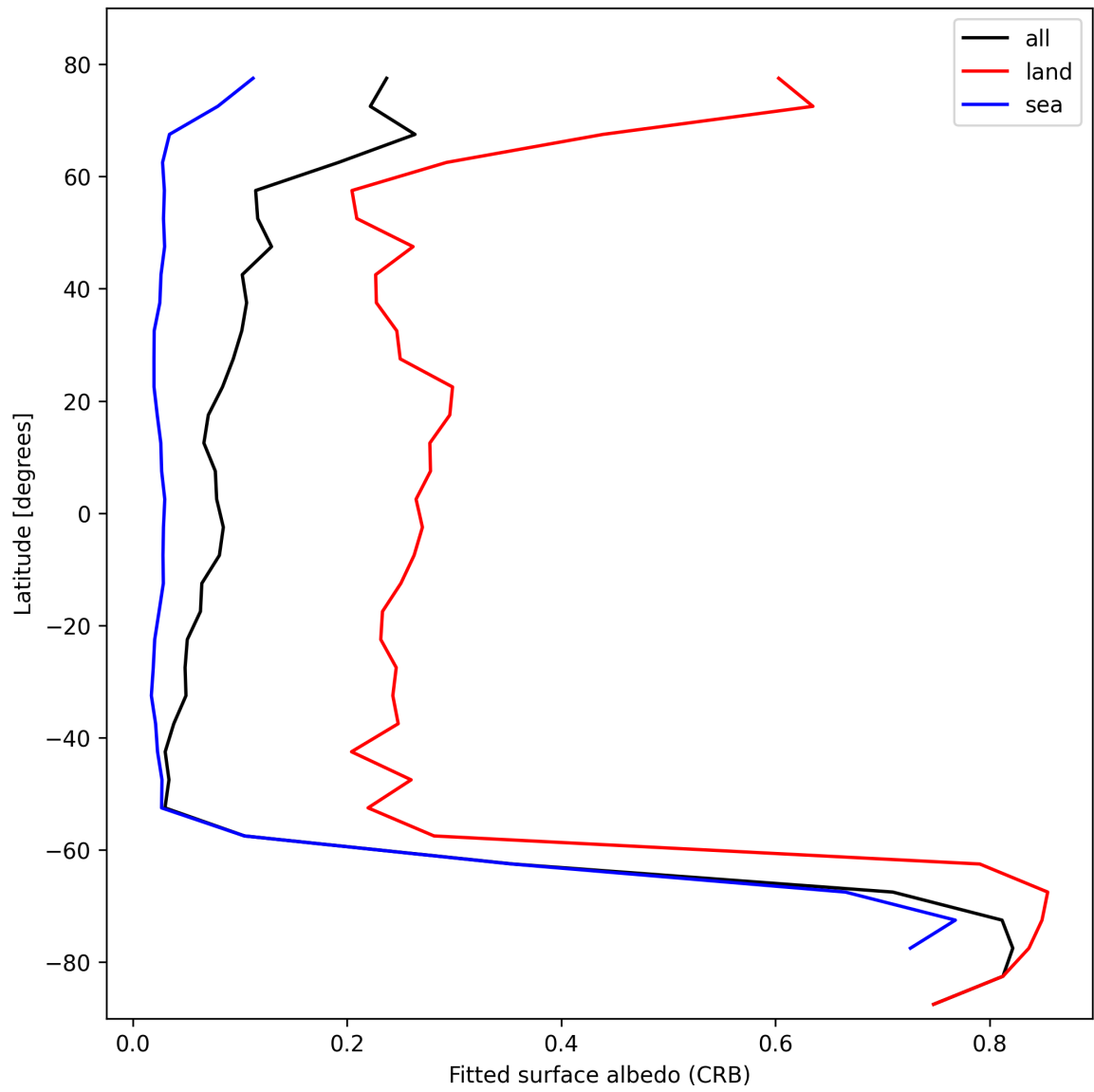
Figure 28: Zonal average of “Fitted surface albedo (CRB)” for 2025-10-22 to 2025-10-23.
