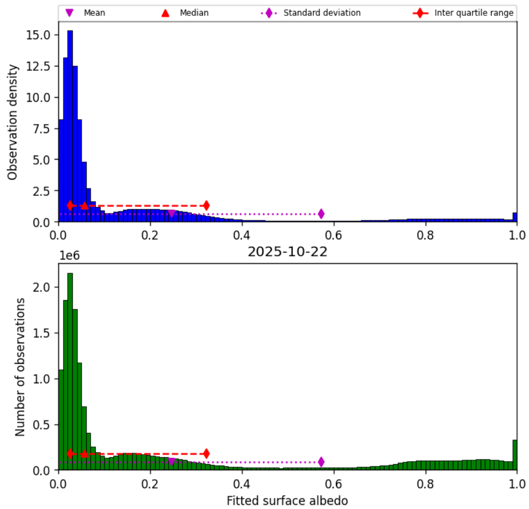
Figure 43: Histogram of “Fitted surface albedo” for 2025-10-22 to 2025-10-23
