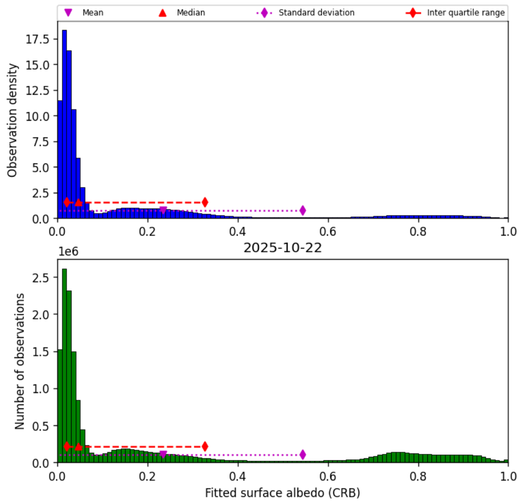
Figure 44: Histogram of “Fitted surface albedo (CRB)” for 2025-10-22 to 2025-10-23
