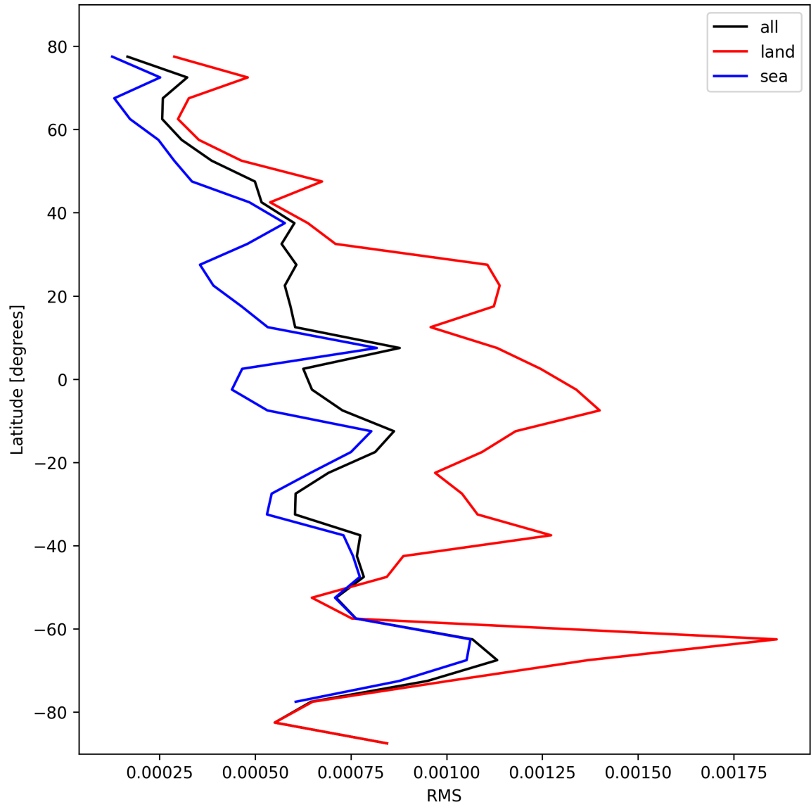
Figure 29: Zonal average of “RMS” for 2025-10-22 to 2025-10-23.
