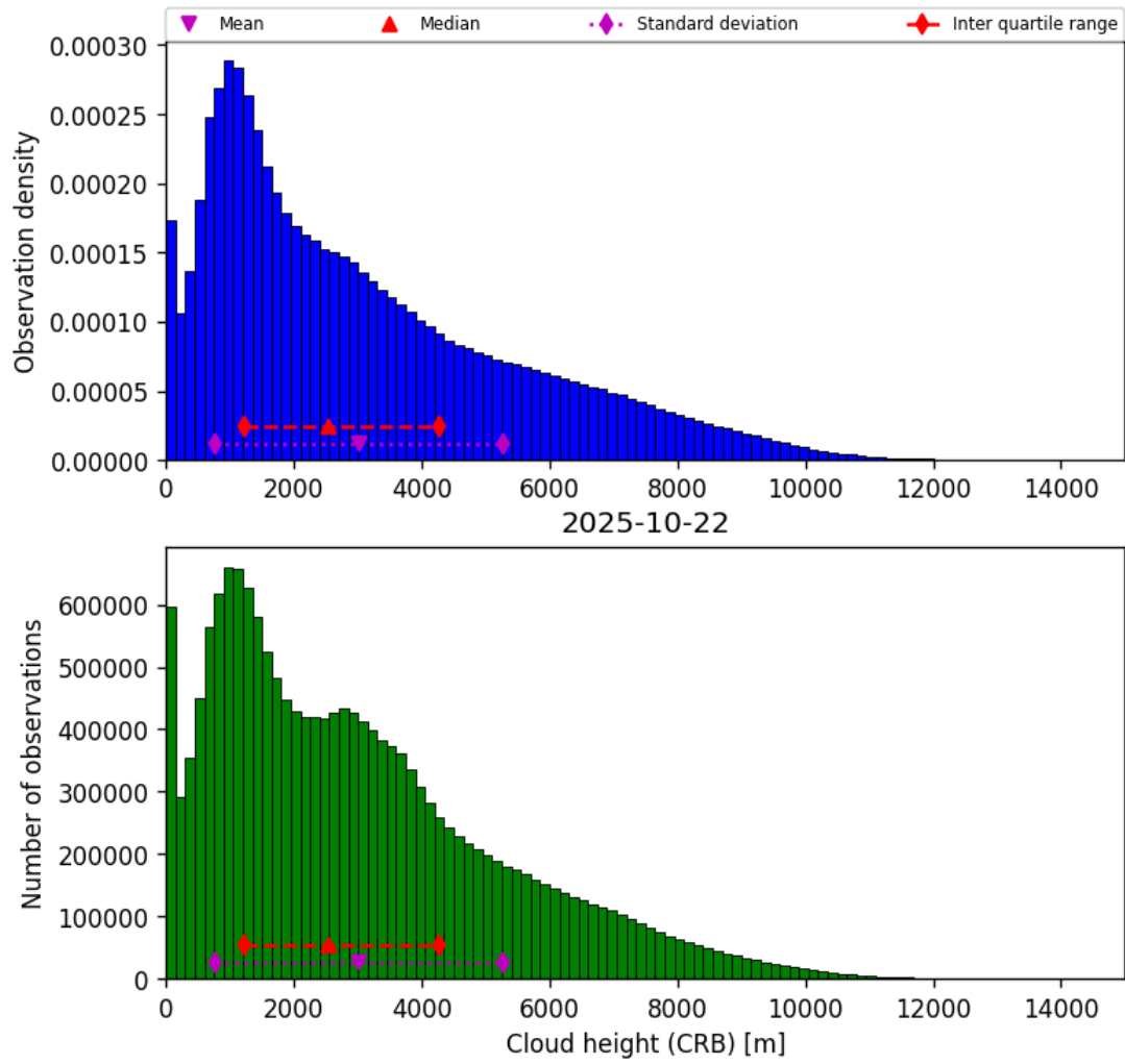
Figure 41: Histogram of “Cloud height (CRB)” for 2025-10-22 to 2025-10-23
