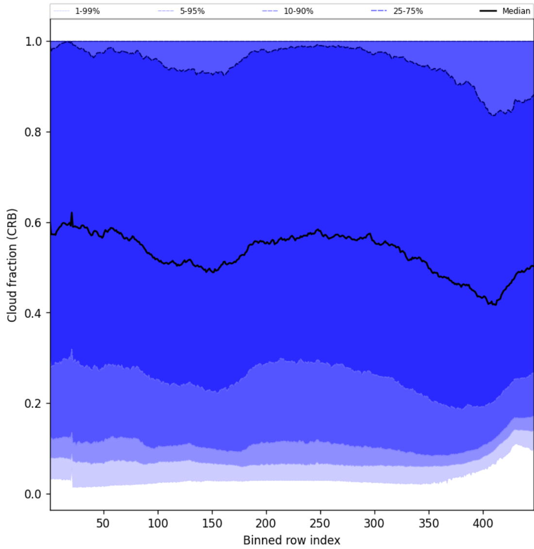
Figure 56: Along track statistics of “Cloud fraction (CRB)” for 2025-10-22 to 2025-10-23
