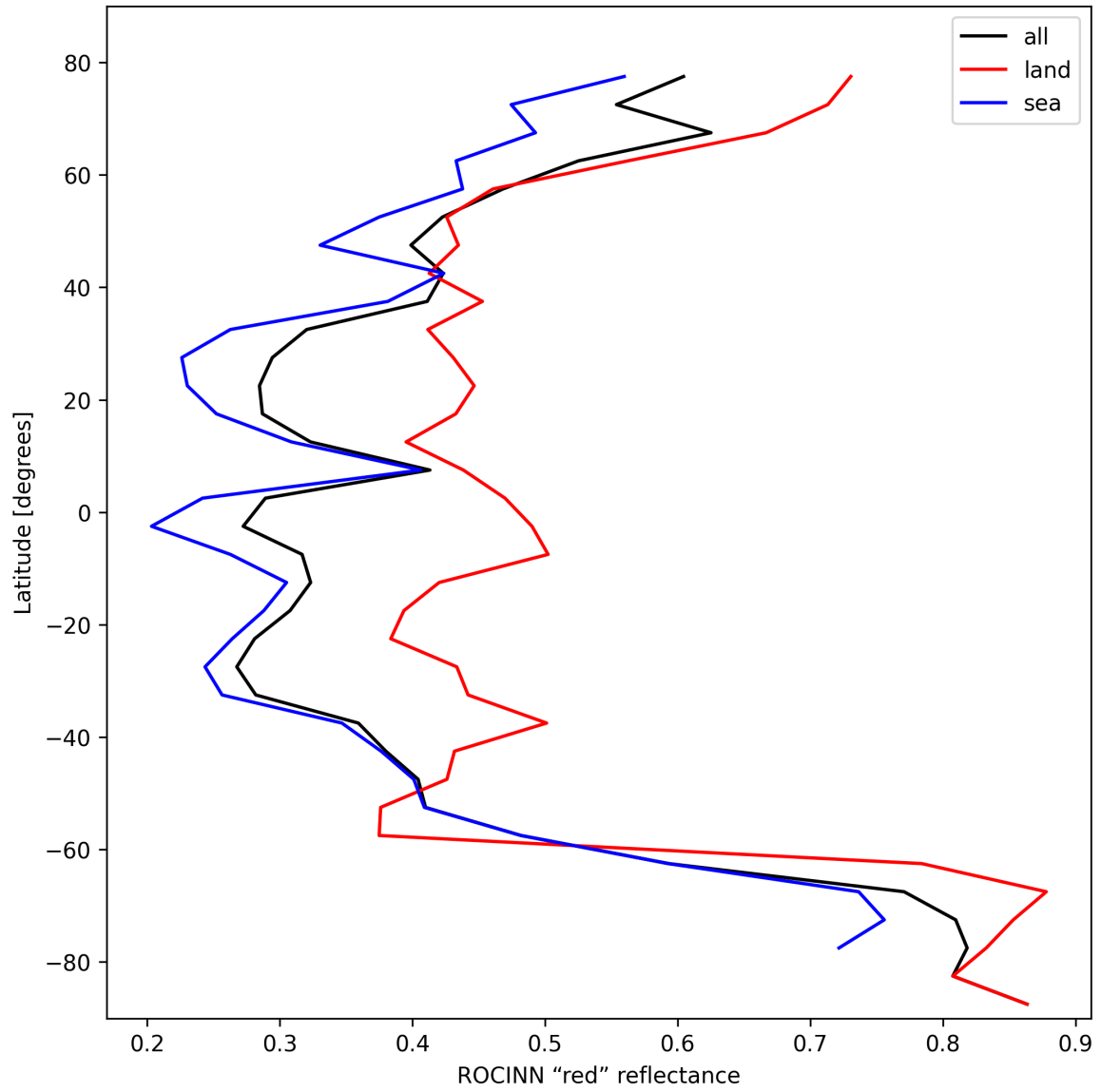
Figure 35: Zonal average of “ROCINN “red” reflectance” for 2025-10-22 to 2025-10-23.
