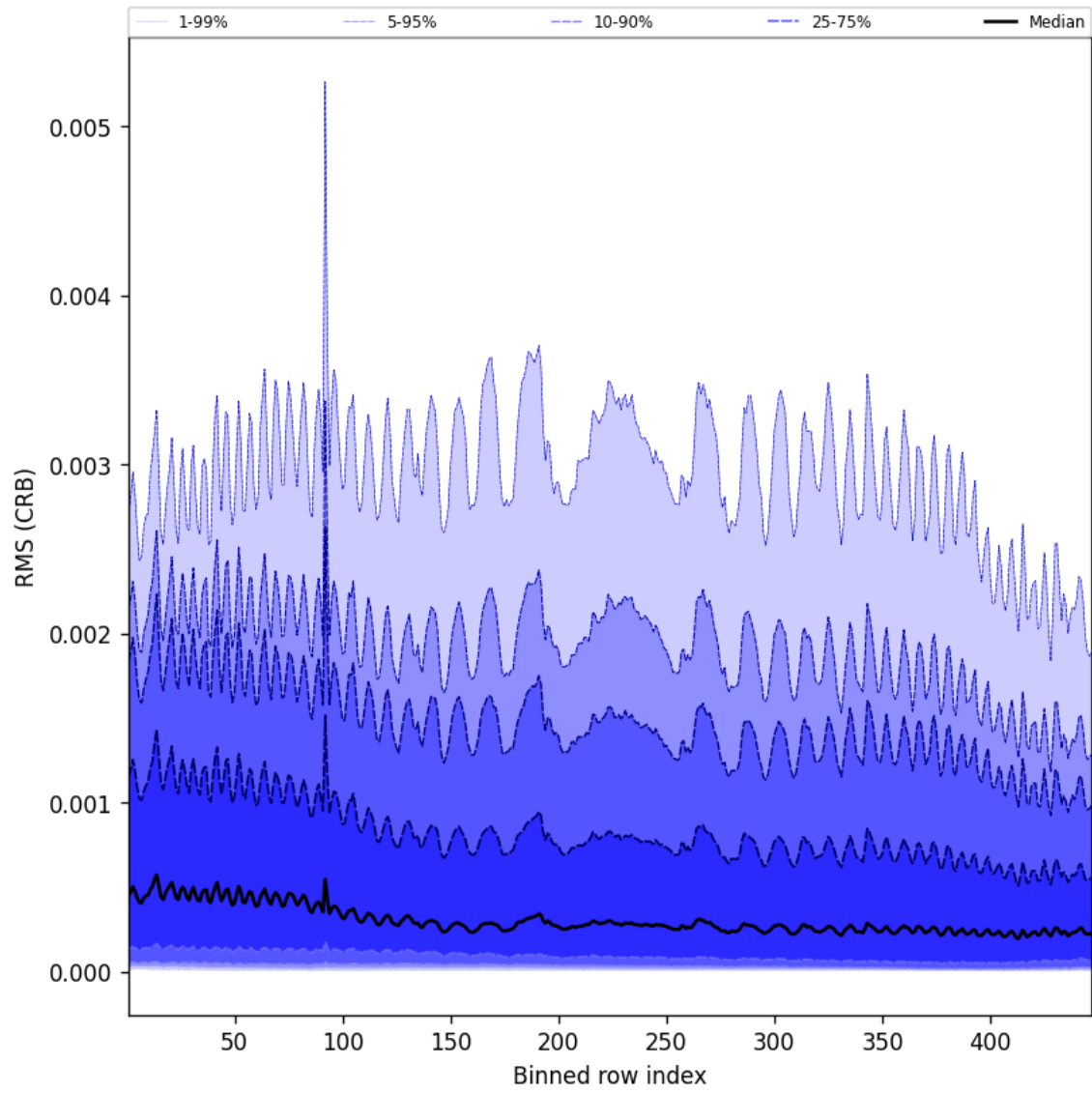
Figure 62: Along track statistics of “RMS (CRB)” for 2025-10-22 to 2025-10-23
