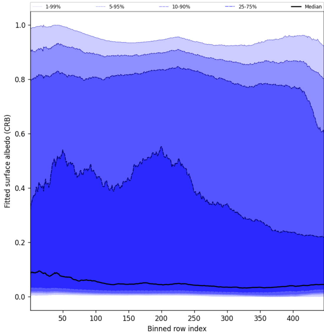
Figure 60: Along track statistics of “Fitted surface albedo (CRB)” for 2025-10-22 to 2025-10-23
