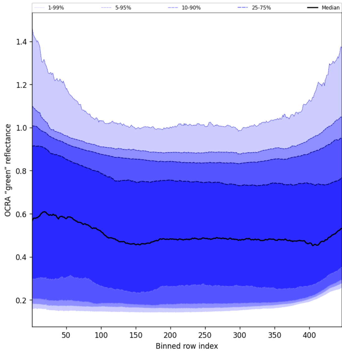
Figure 66: Along track statistics of “OCRA “green” reflectance” for 2025-10-22 to 2025-10-23
