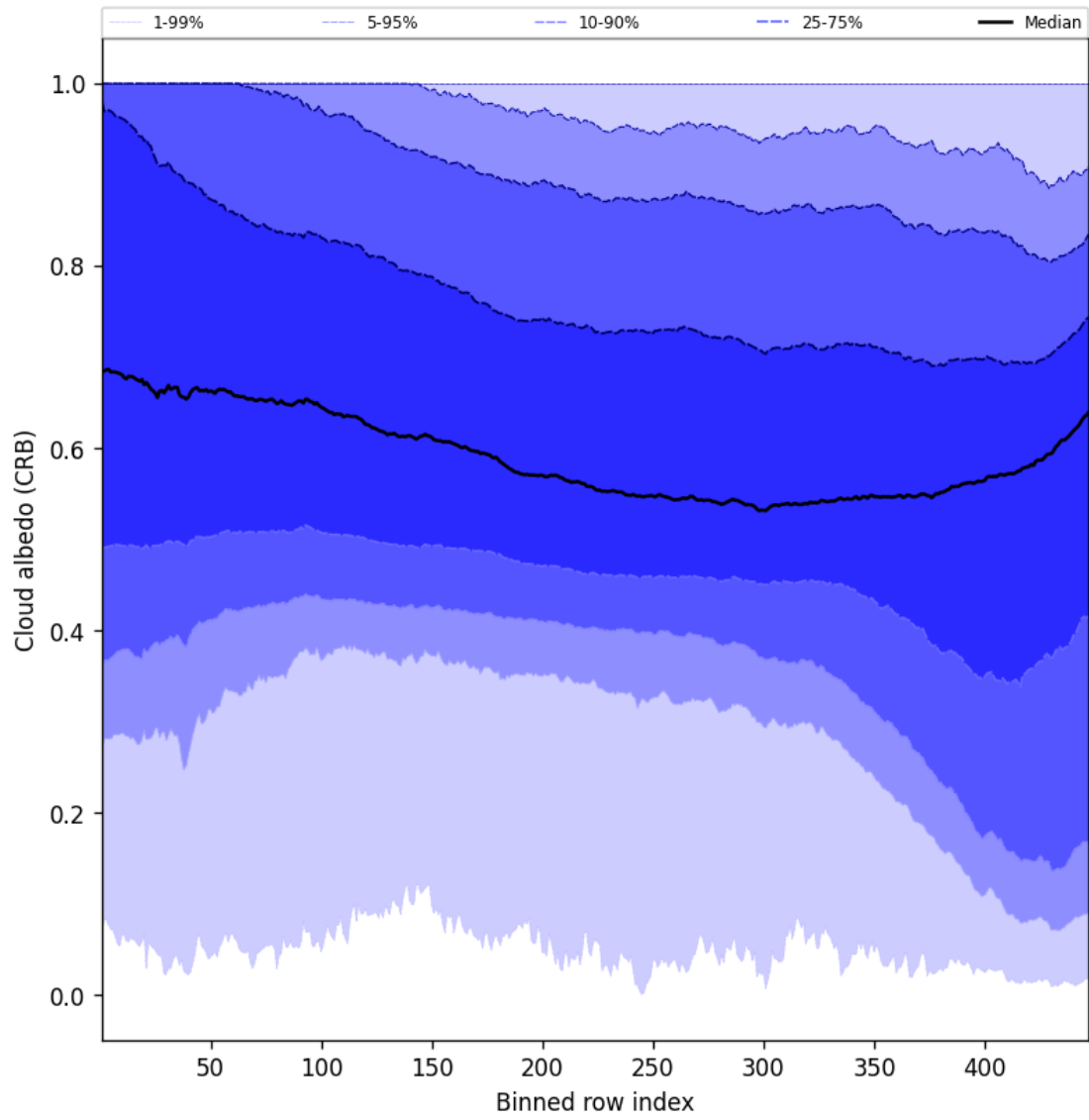
Figure 58: Along track statistics of “Cloud albedo (CRB)” for 2025-10-22 to 2025-10-23
