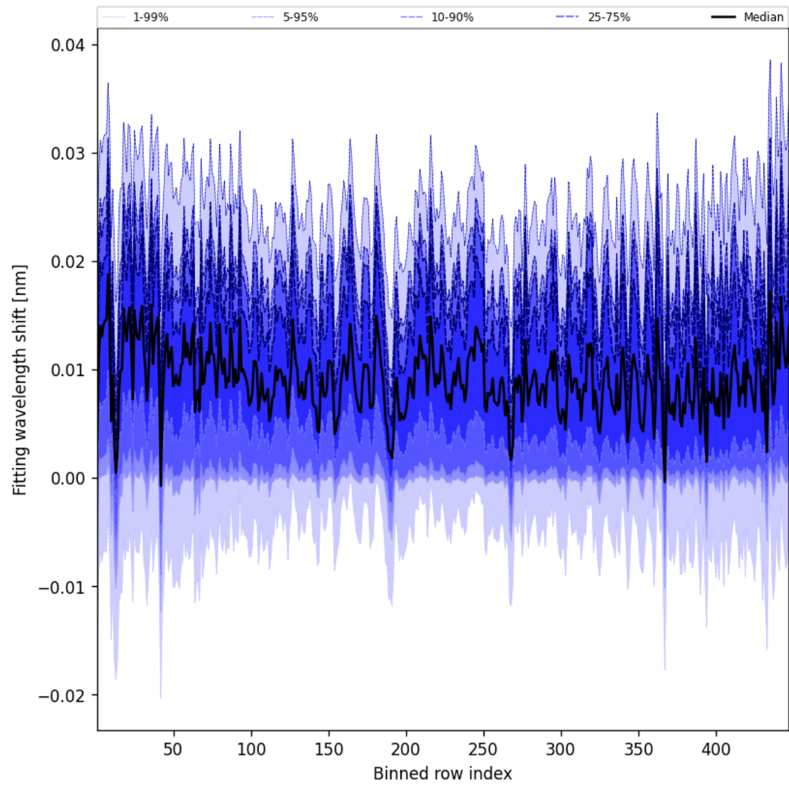
Figure 63: Along track statistics of “Fitting wavelength shift” for 2025-10-22 to 2025-10-23
