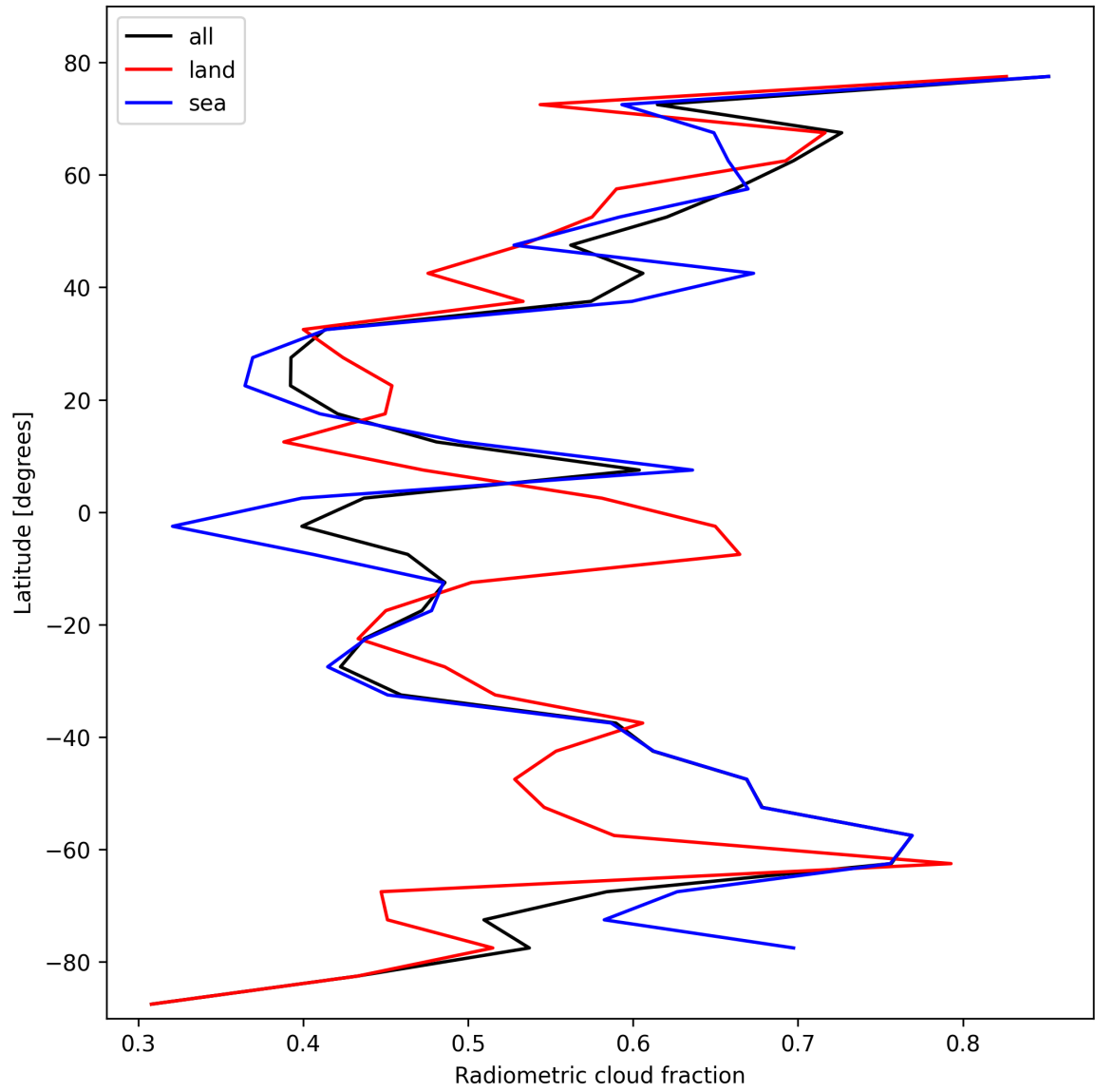
Figure 21: Zonal average of “Radiometric cloud fraction” for 2025-10-22 to 2025-10-23.
