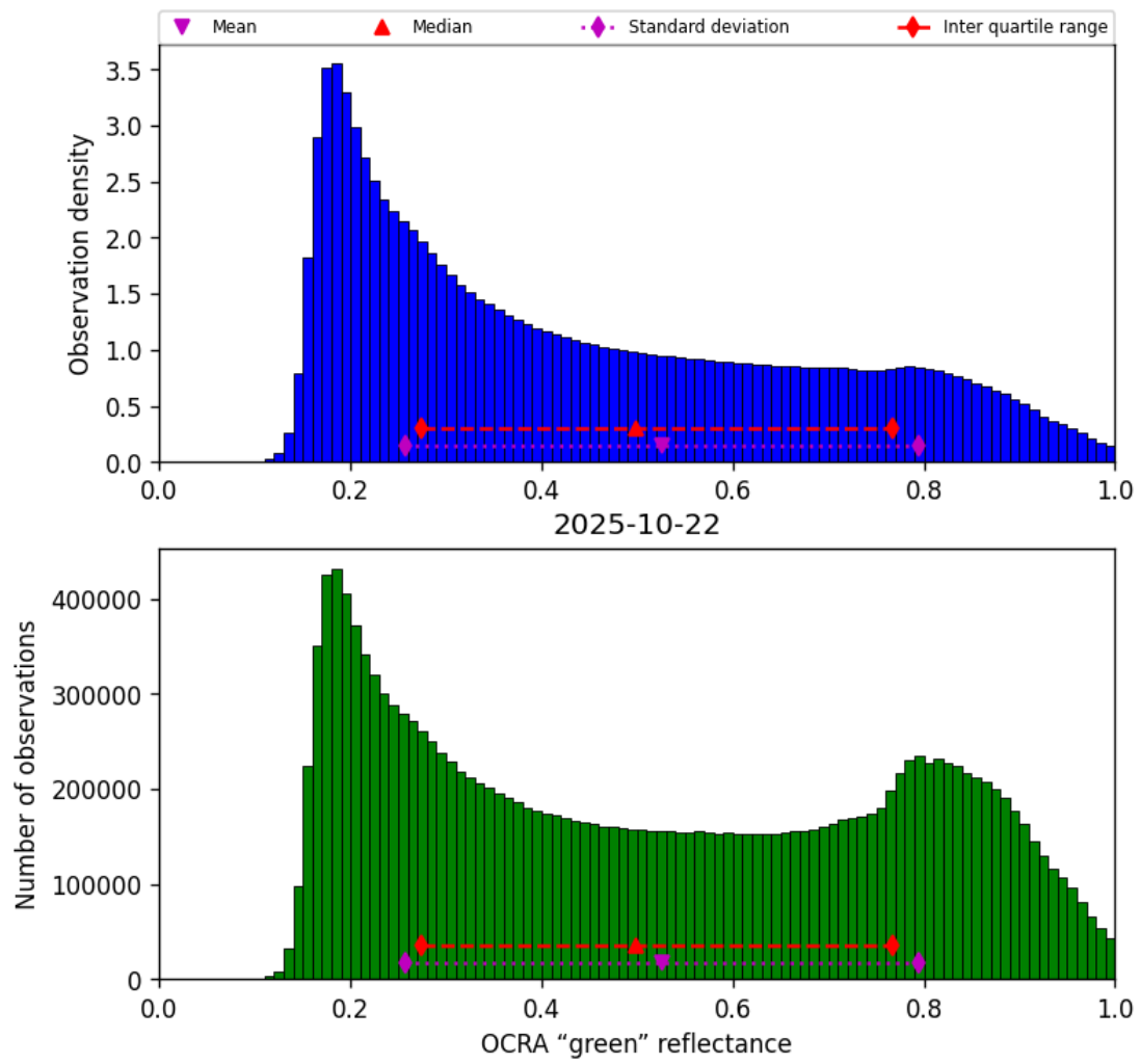
Figure 50: Histogram of “OCRA “green” reflectance” for 2025-10-22 to 2025-10-23
