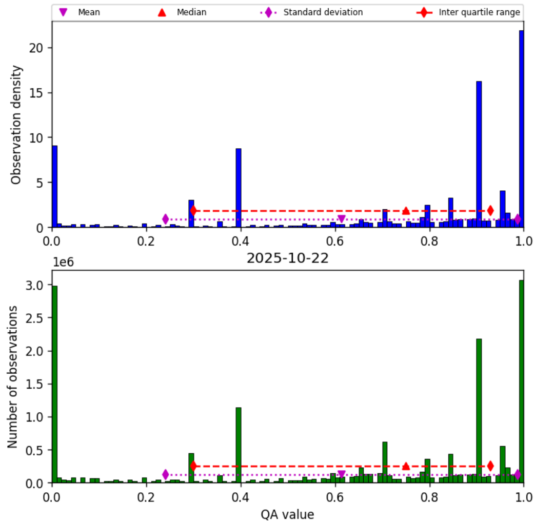
Figure 36: Histogram of “QA value” for 2025-10-22 to 2025-10-23
