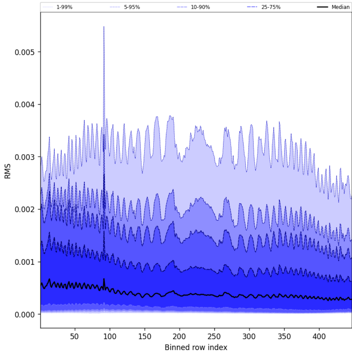
Figure 61: Along track statistics of “RMS” for 2025-10-22 to 2025-10-23
