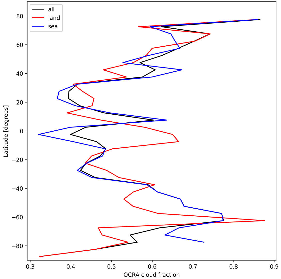
Figure 32: Zonal average of “OCRA cloud fraction” for 2025-10-22 to 2025-10-23.
