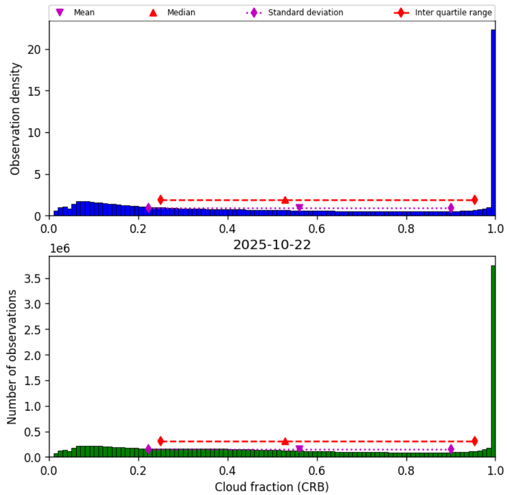
Figure 40: Histogram of “Cloud fraction (CRB)” for 2025-10-22 to 2025-10-23
