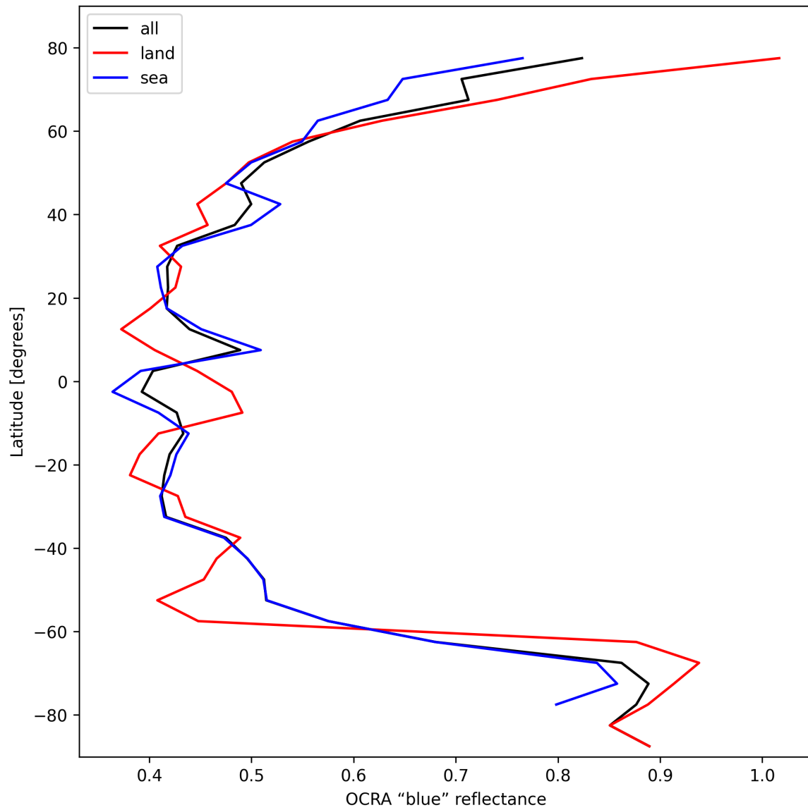
Figure 33: Zonal average of “OCRA “blue” reflectance” for 2025-10-22 to 2025-10-23.
