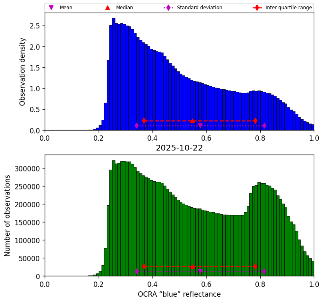
Figure 49: Histogram of “OCRA “blue” reflectance” for 2025-10-22 to 2025-10-23
