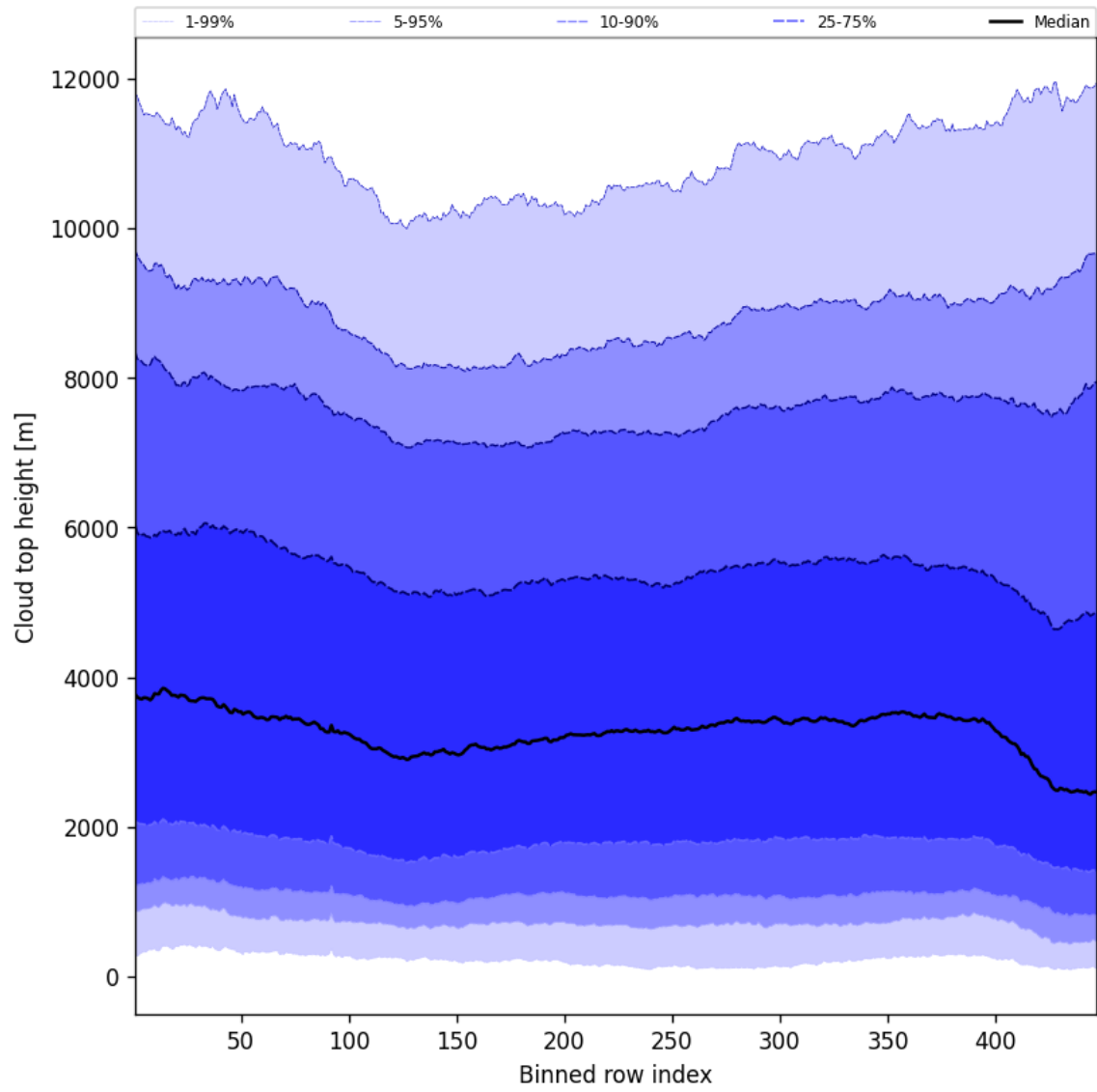
Figure 54: Along track statistics of “Cloud top height” for 2025-10-22 to 2025-10-23
