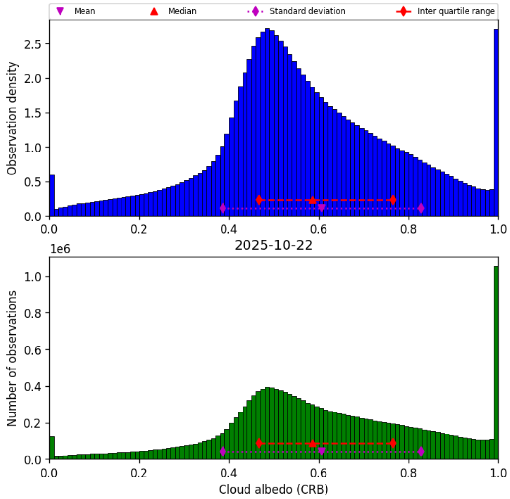
Figure 42: Histogram of “Cloud albedo (CRB)” for 2025-10-22 to 2025-10-23
