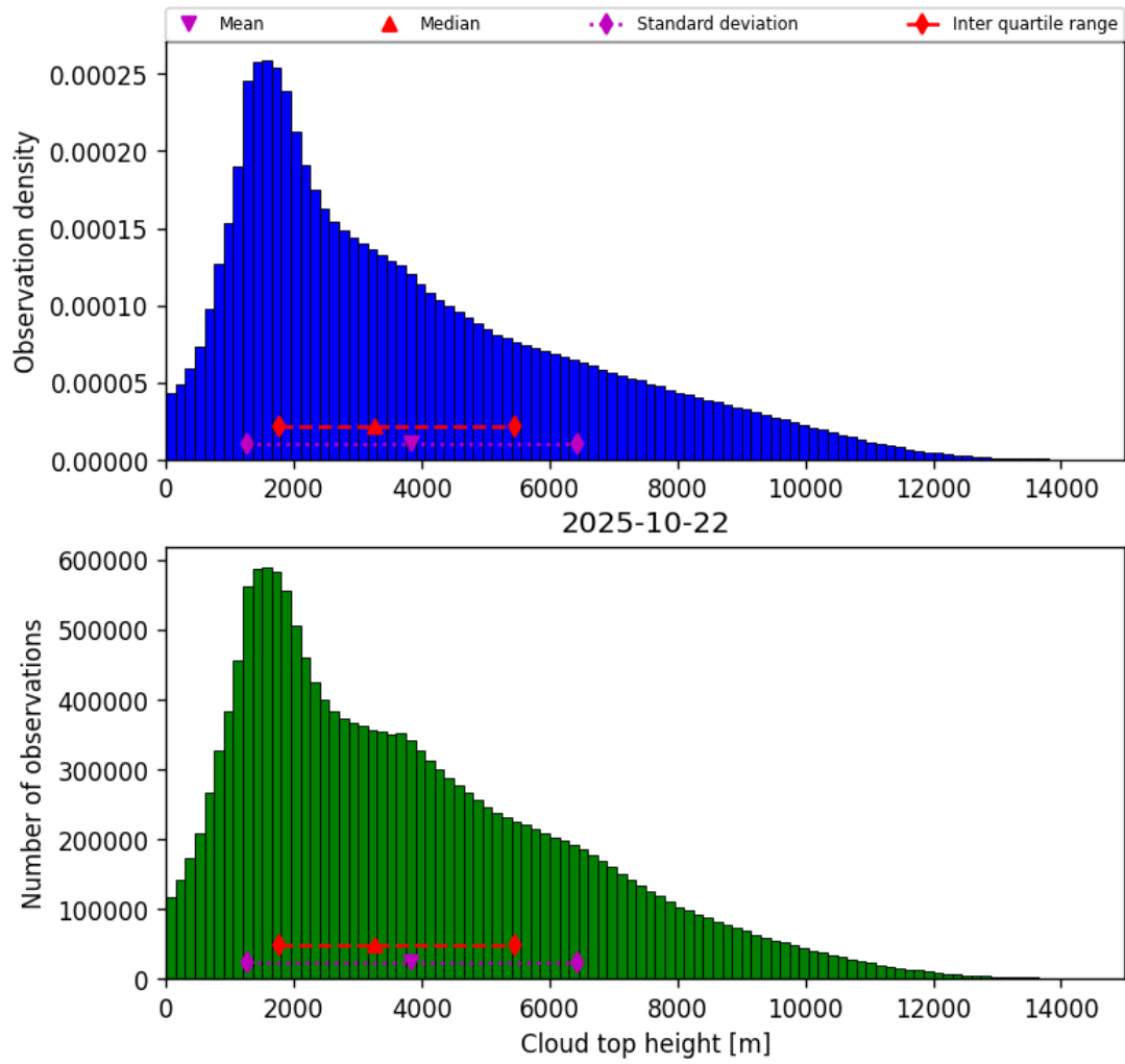
Figure 38: Histogram of “Cloud top height” for 2025-10-22 to 2025-10-23
