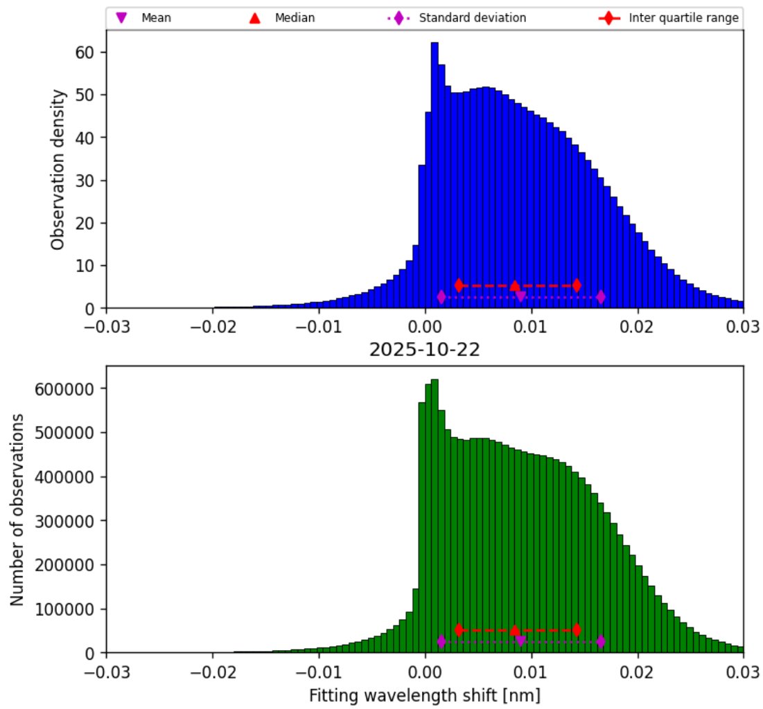
Figure 47: Histogram of “Fitting wavelength shift” for 2025-10-22 to 2025-10-23
