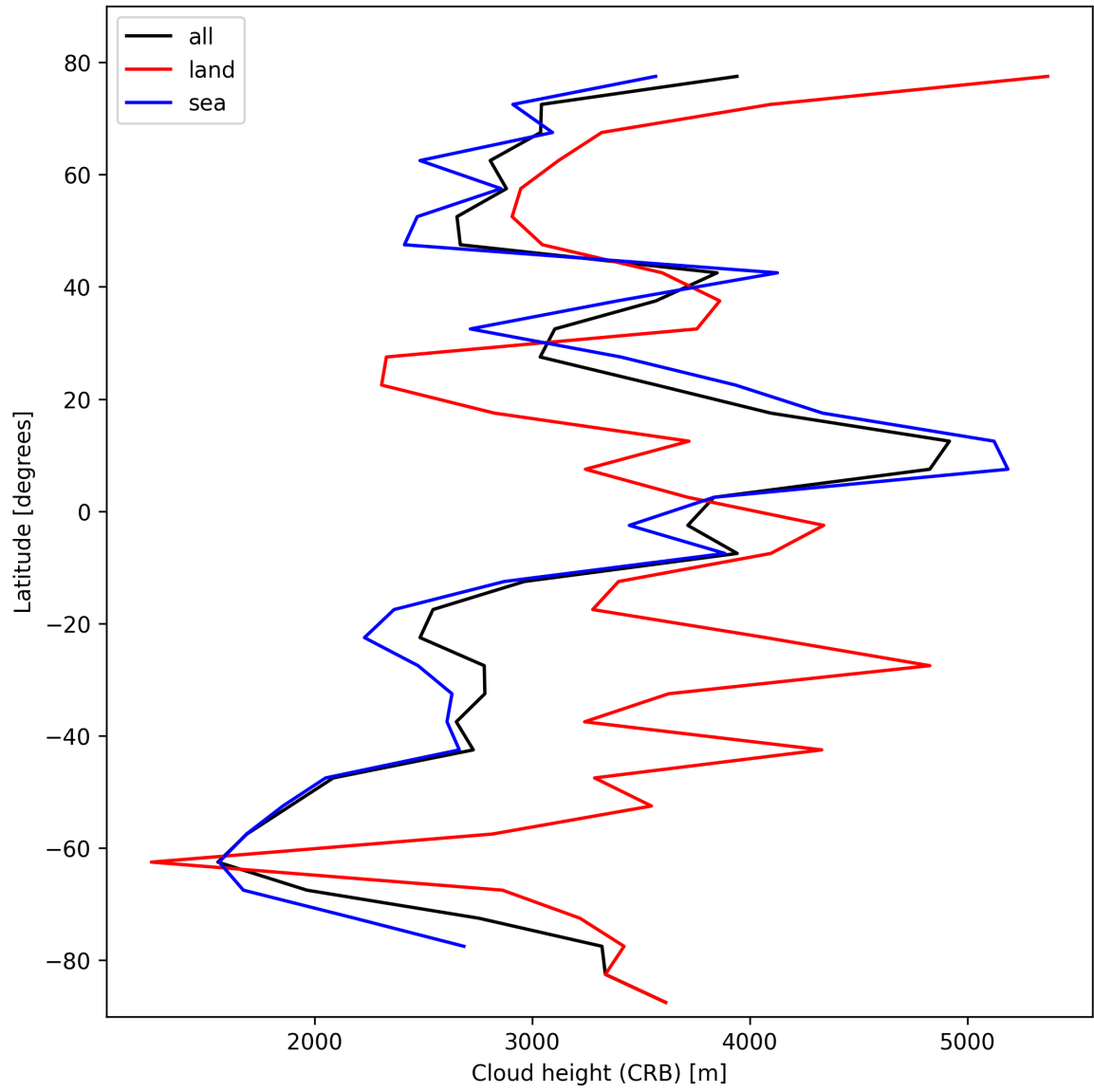
Figure 25: Zonal average of “Cloud height (CRB)” for 2025-10-22 to 2025-10-23.
