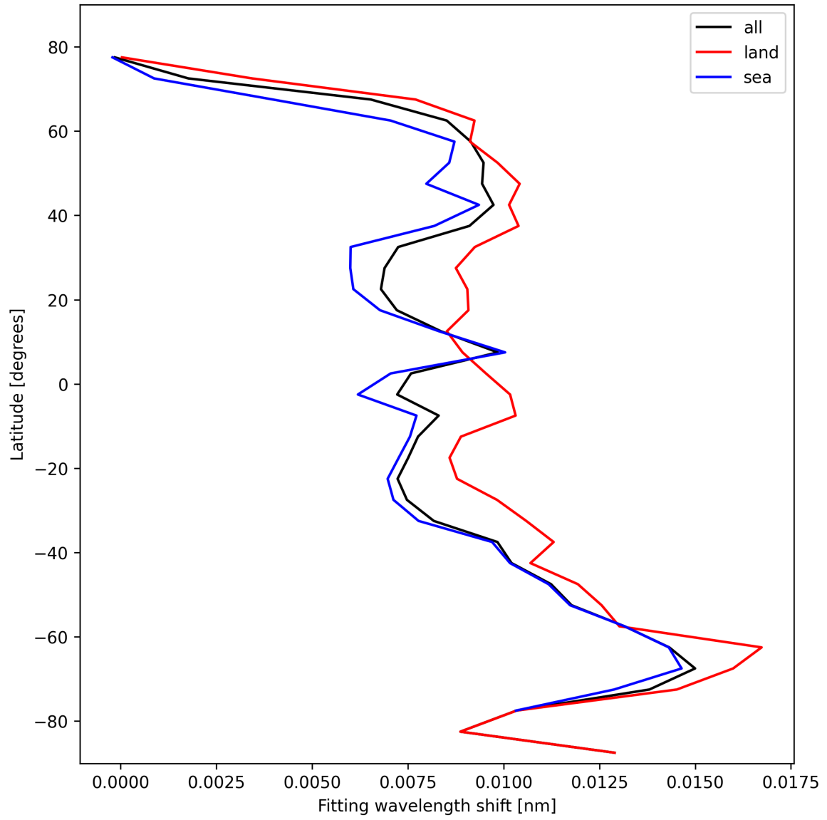
Figure 31: Zonal average of “Fitting wavelength shift” for 2025-10-22 to 2025-10-23.
