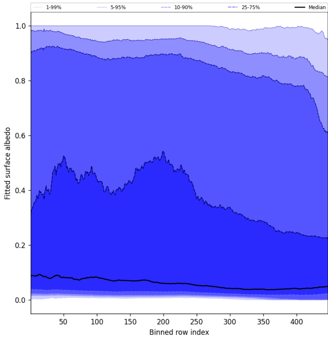
Figure 59: Along track statistics of “Fitted surface albedo” for 2025-10-22 to 2025-10-23
