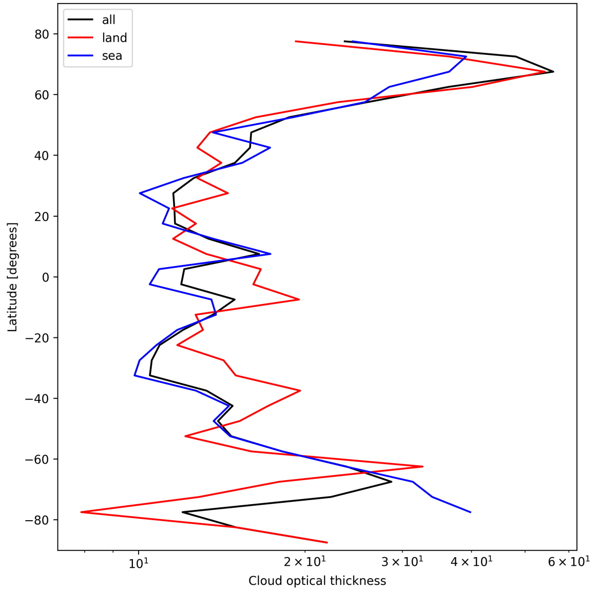
Figure 23: Zonal average of “Cloud optical thickness” for 2025-10-22 to 2025-10-23.
