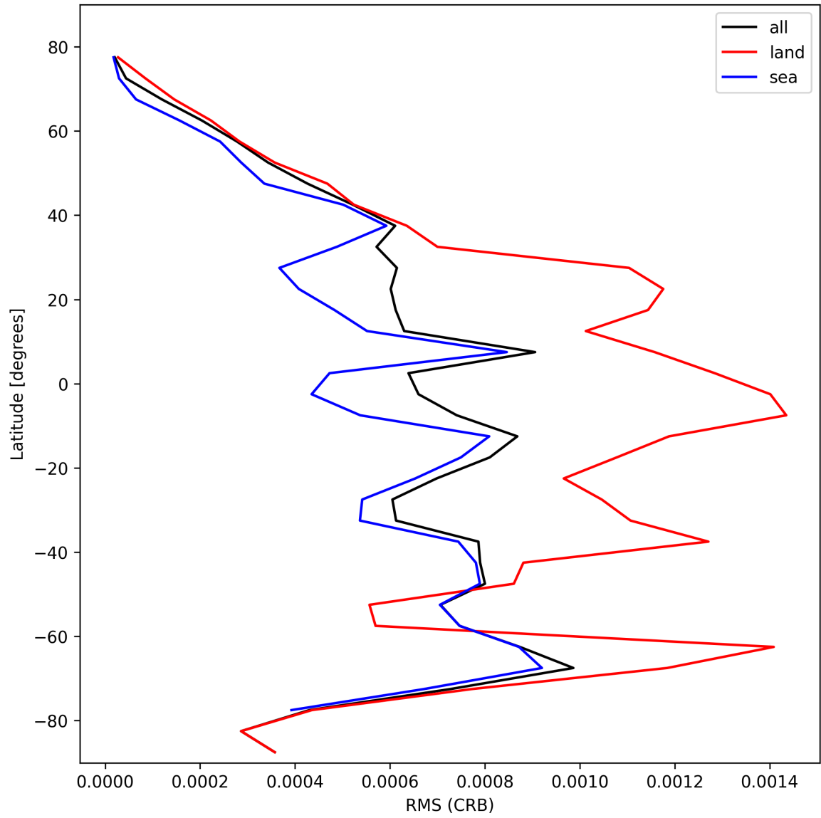
Figure 30: Zonal average of “RMS (CRB)” for 2025-10-22 to 2025-10-23.
