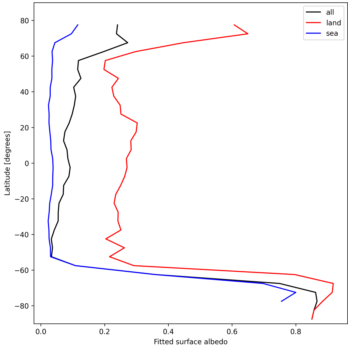
Figure 27: Zonal average of “Fitted surface albedo” for 2025-10-22 to 2025-10-23.
