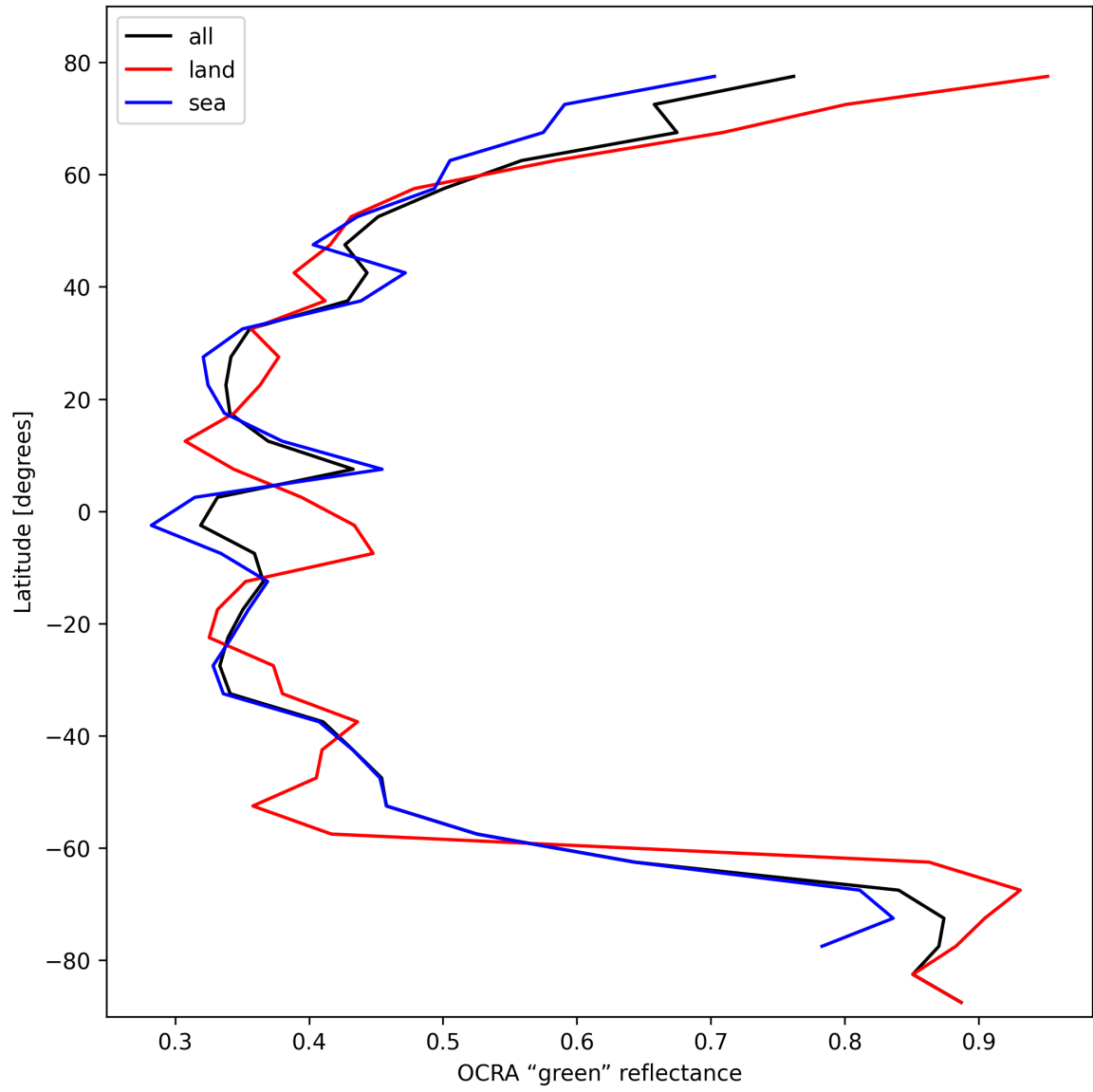
Figure 34: Zonal average of “OCRA “green” reflectance” for 2025-10-22 to 2025-10-23.
