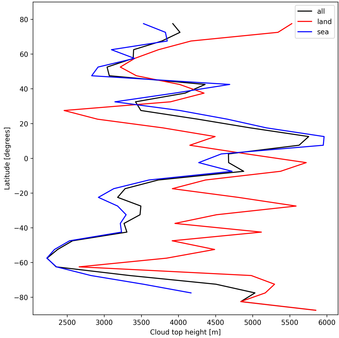
Figure 22: Zonal average of “Cloud top height” for 2025-10-22 to 2025-10-23.
