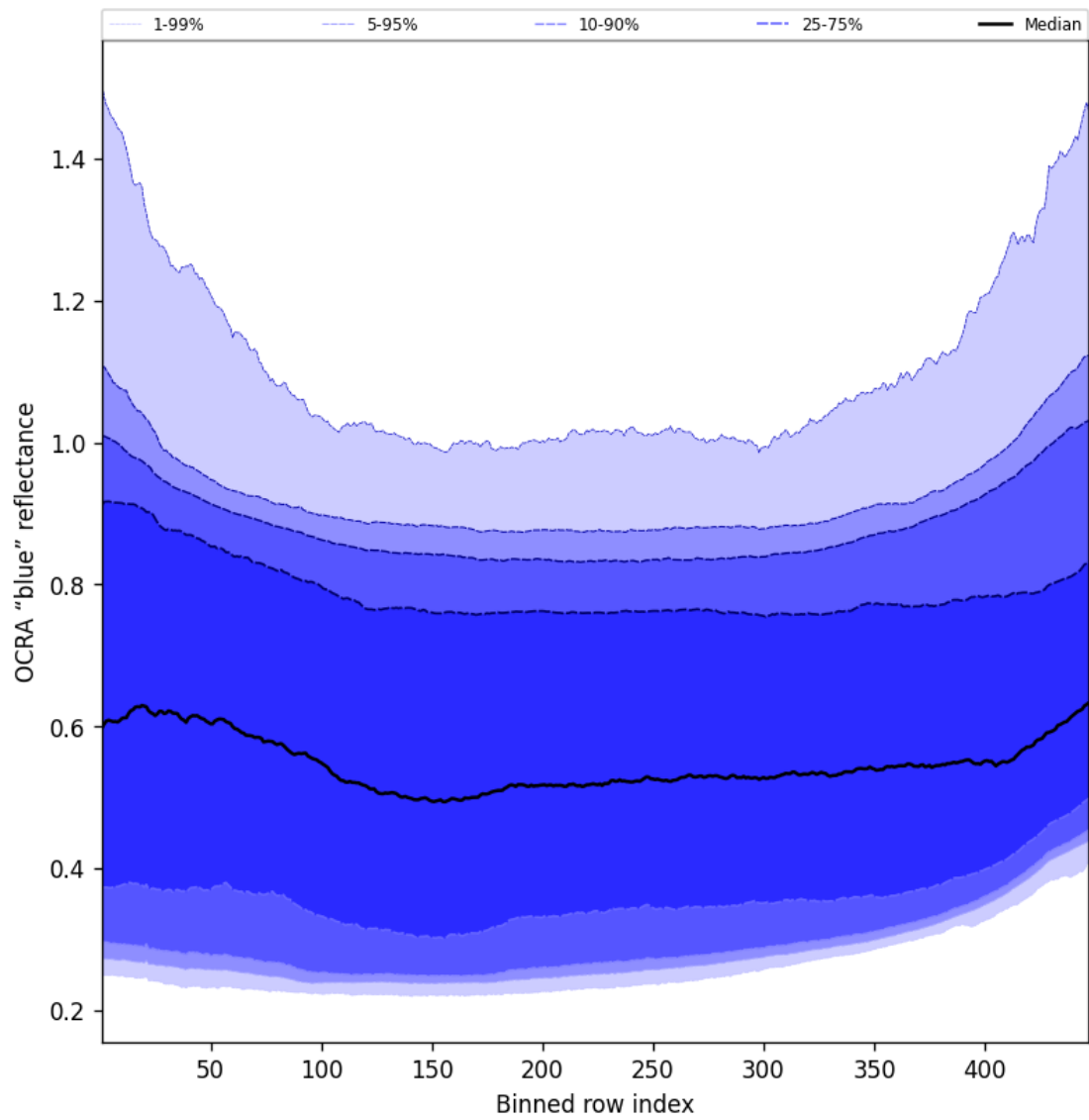
Figure 65: Along track statistics of “OCRA “blue” reflectance” for 2025-10-22 to 2025-10-23
