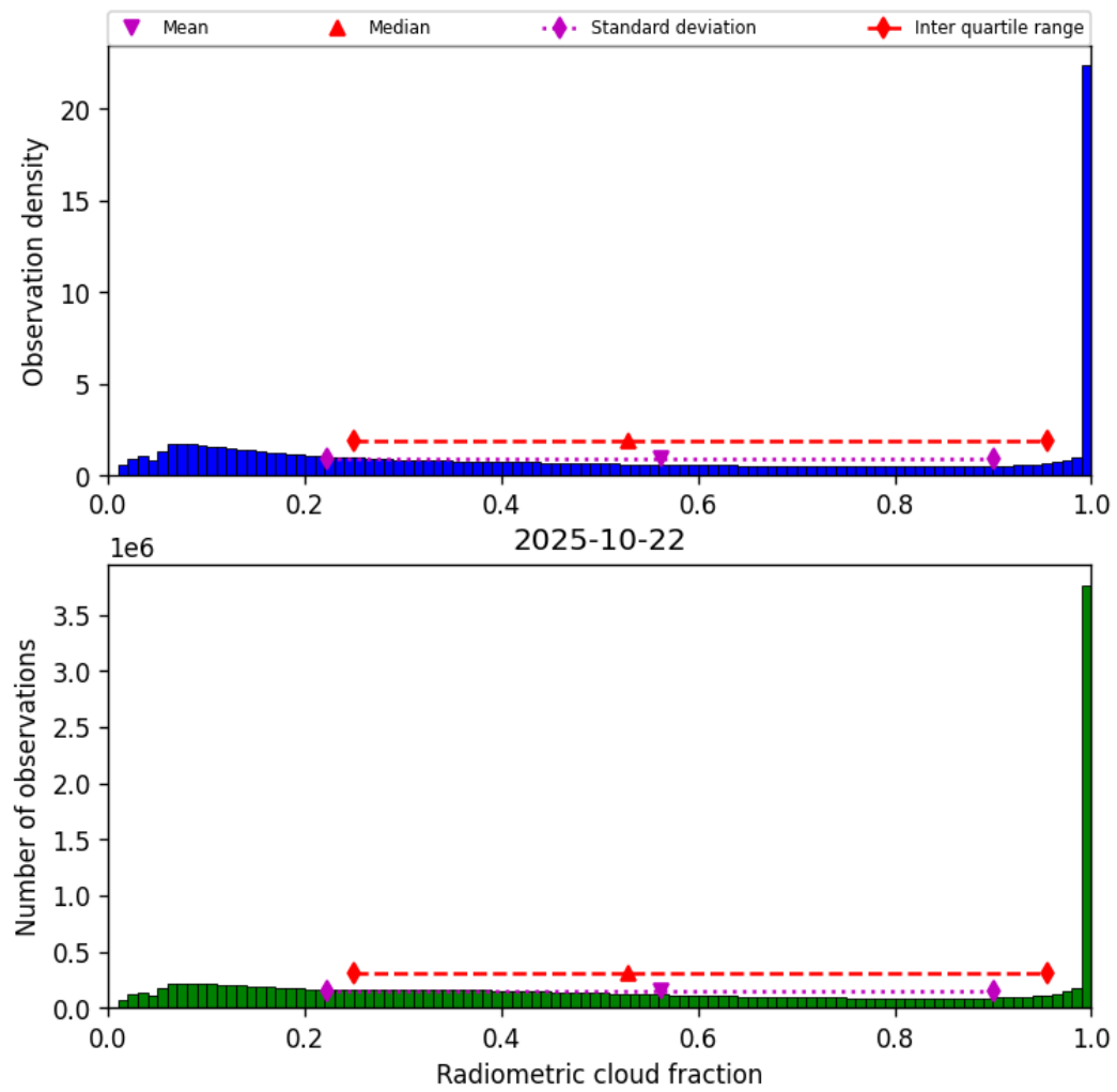
Figure 37: Histogram of “Radiometric cloud fraction” for 2025-10-22 to 2025-10-23
