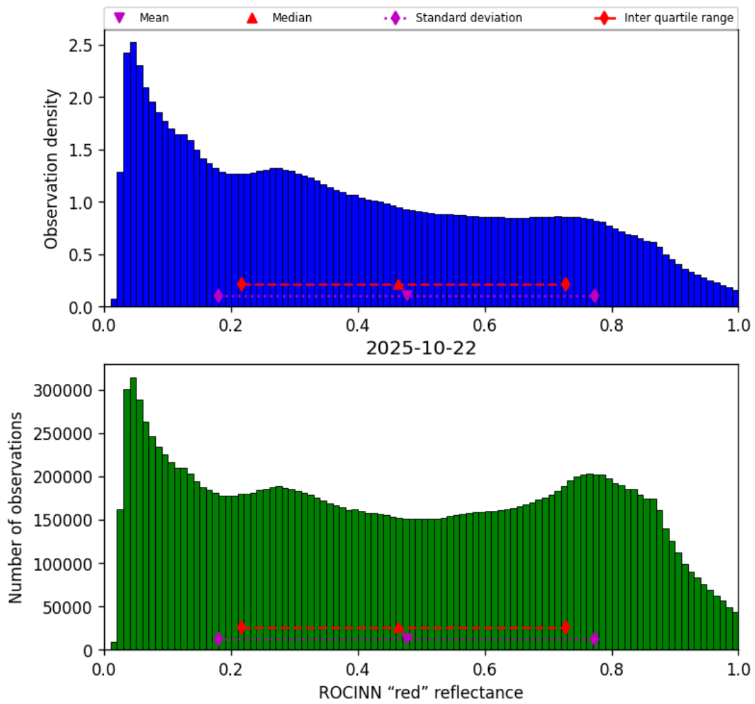
Figure 51: Histogram of “ROCINN “red” reflectance” for 2025-10-22 to 2025-10-23
