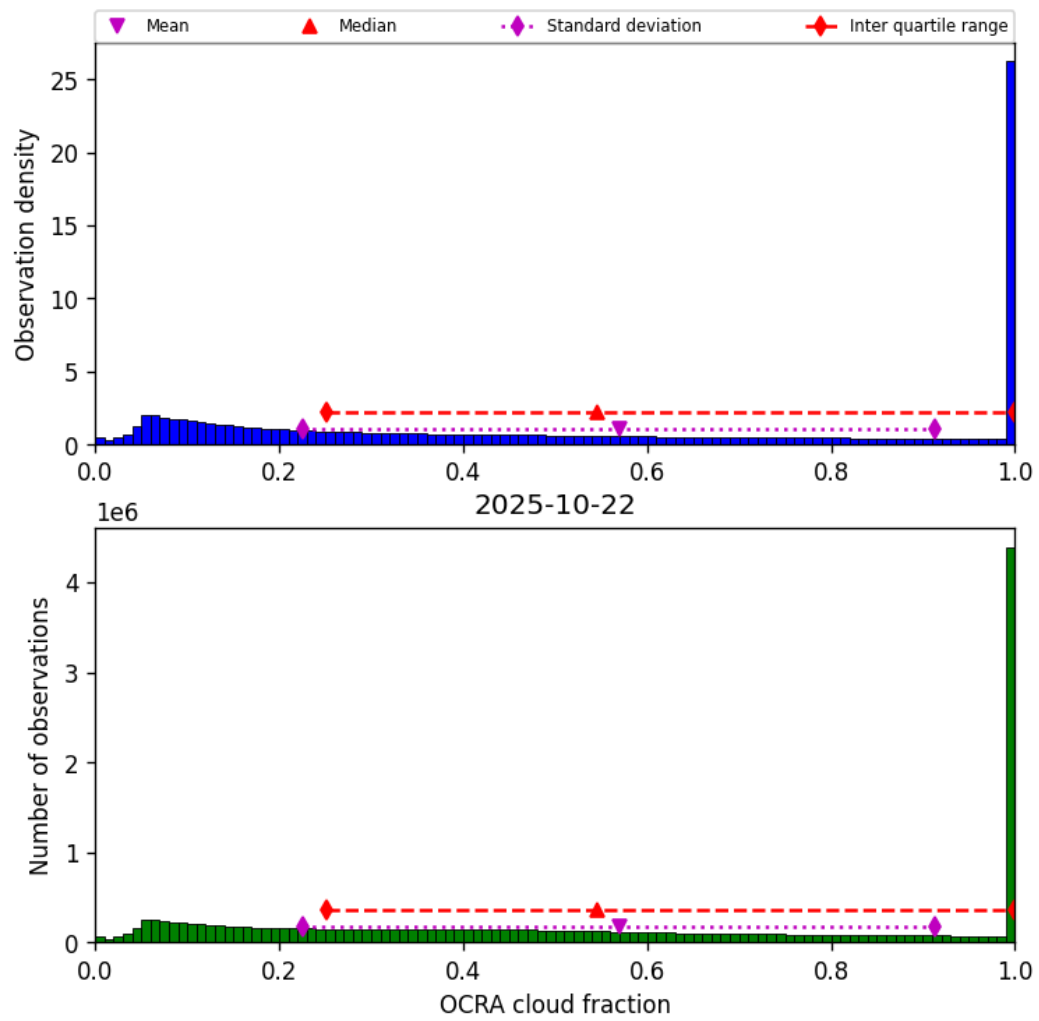
Figure 48: Histogram of “OCRA cloud fraction” for 2025-10-22 to 2025-10-23
