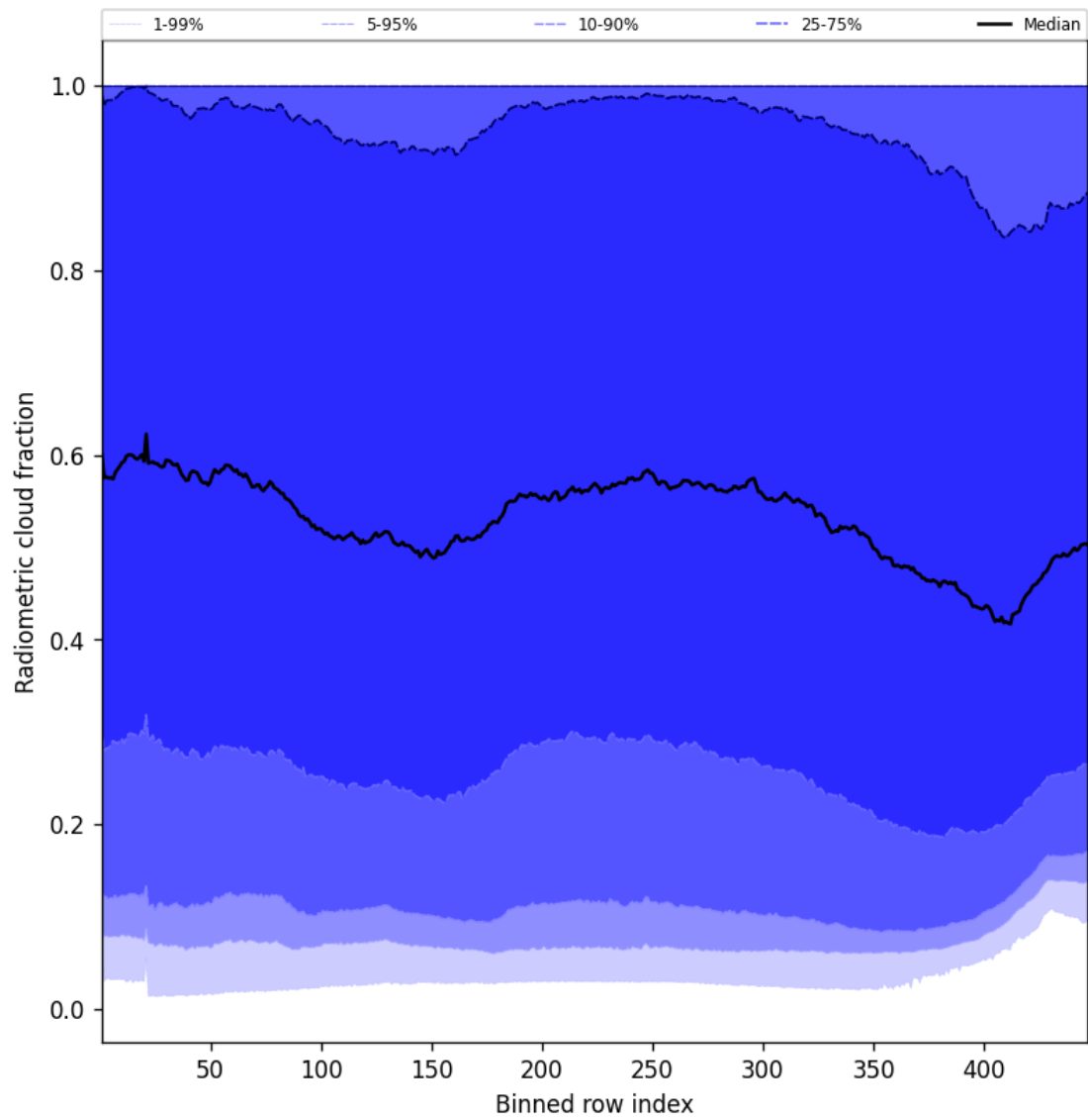
Figure 53: Along track statistics of “Radiometric cloud fraction” for 2025-10-22 to 2025-10-23
