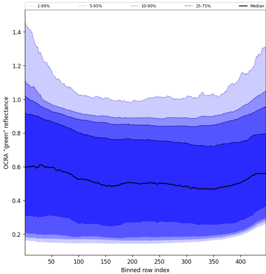
Figure 66: Along track statistics of “OCRA “green” reflectance” for 2025-10-24 to 2025-10-25
