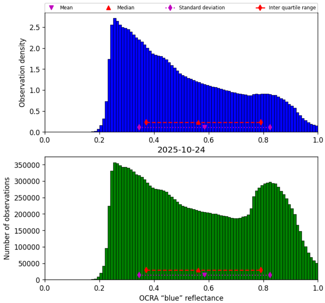
Figure 49: Histogram of “OCRA “blue” reflectance” for 2025-10-24 to 2025-10-25
