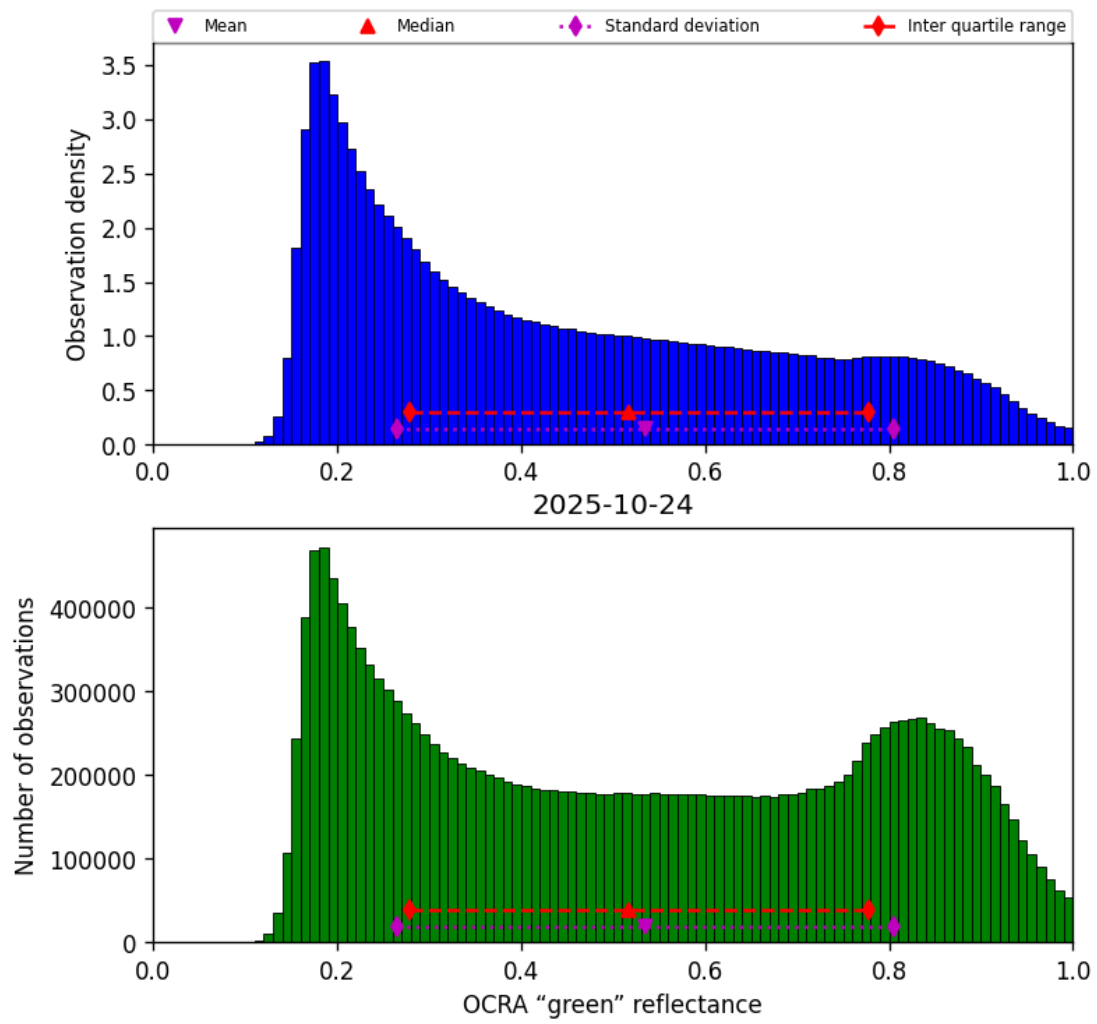
Figure 50: Histogram of “OCRA “green” reflectance” for 2025-10-24 to 2025-10-25
