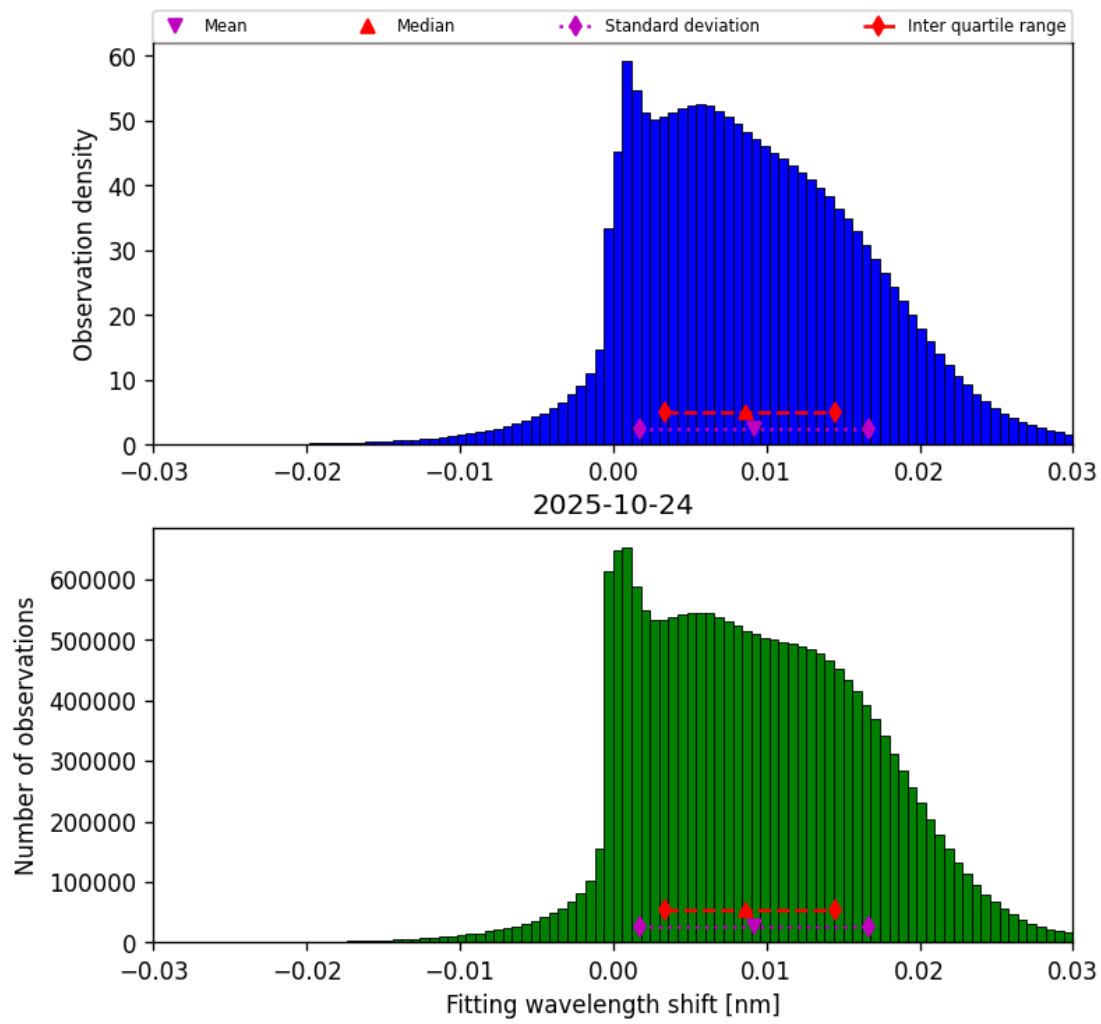
Figure 47: Histogram of “Fitting wavelength shift” for 2025-10-24 to 2025-10-25
