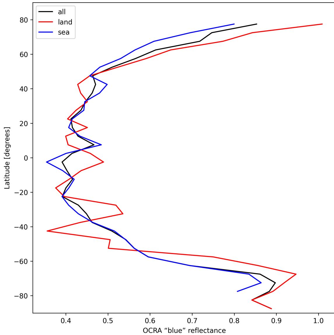
Figure 33: Zonal average of “OCRA “blue” reflectance” for 2025-10-24 to 2025-10-25.
