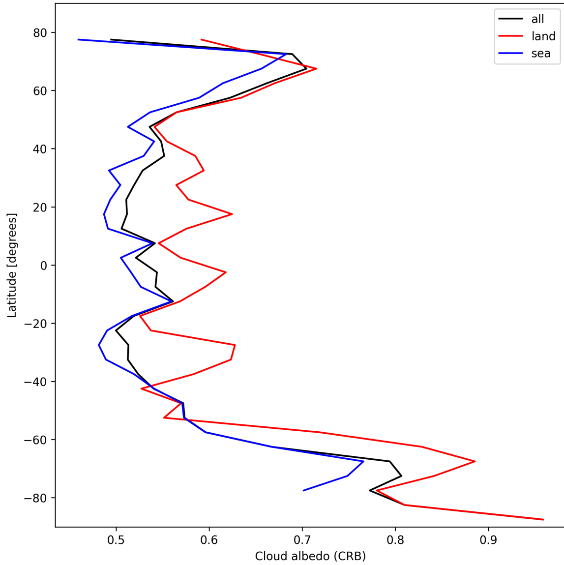
Figure 26: Zonal average of “Cloud albedo (CRB)” for 2025-10-24 to 2025-10-25.
