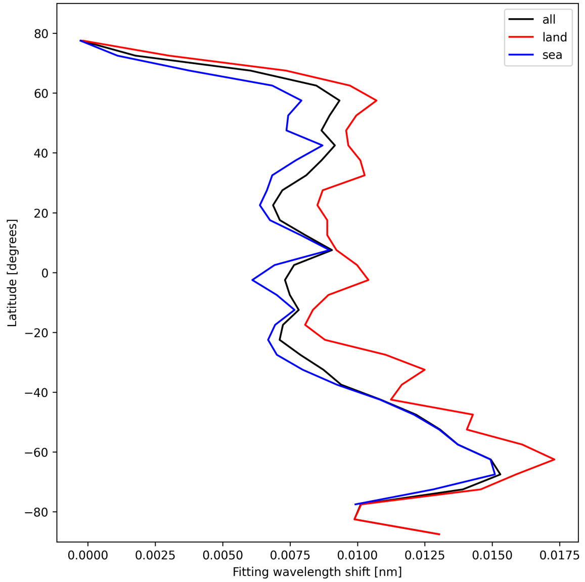
Figure 31: Zonal average of “Fitting wavelength shift” for 2025-10-24 to 2025-10-25.
