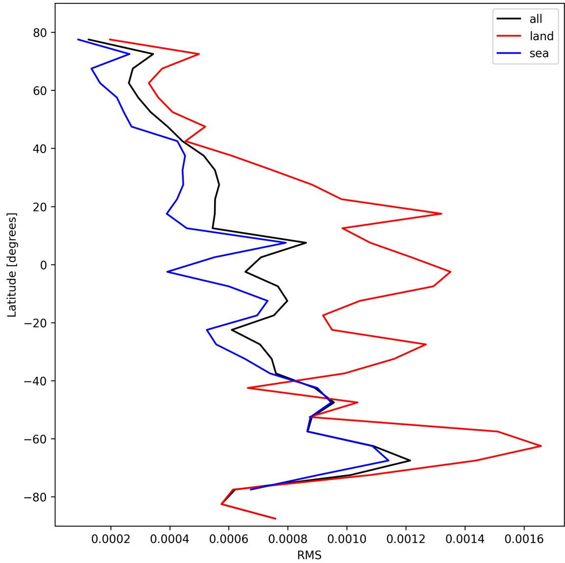
Figure 29: Zonal average of “RMS” for 2025-10-24 to 2025-10-25.
