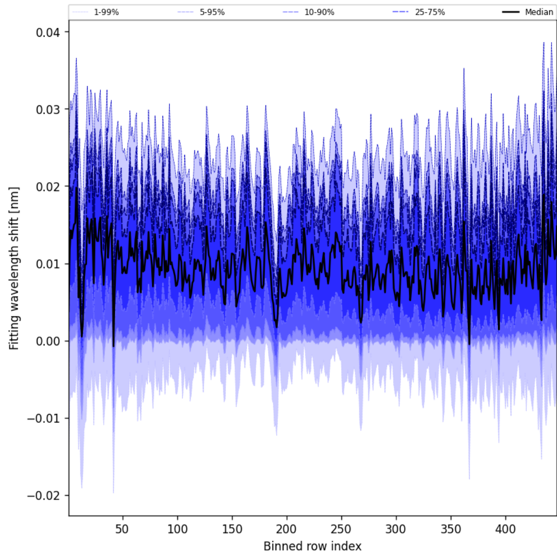
Figure 63: Along track statistics of “Fitting wavelength shift” for 2025-10-24 to 2025-10-25
