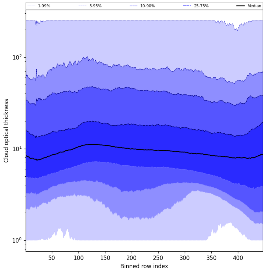
Figure 55: Along track statistics of “Cloud optical thickness” for 2025-10-24 to 2025-10-25
