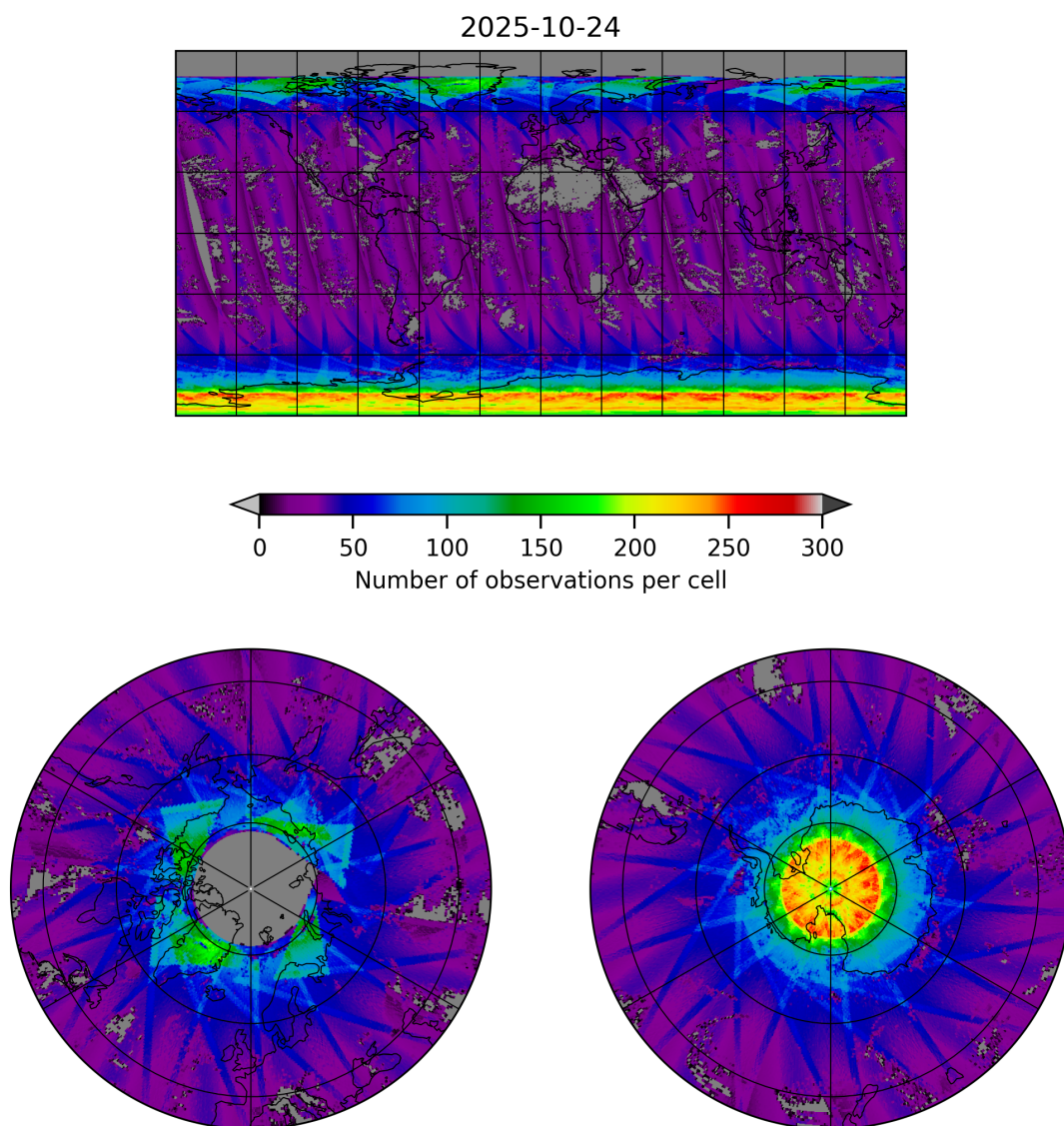
Figure 19: Map of the number of observations for 2025-10-24 to 2025-10-25
