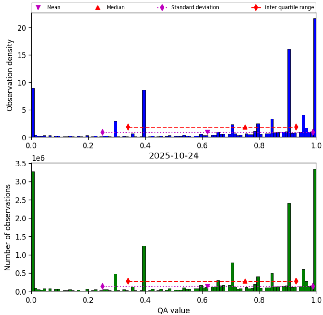
Figure 36: Histogram of “QA value” for 2025-10-24 to 2025-10-25
