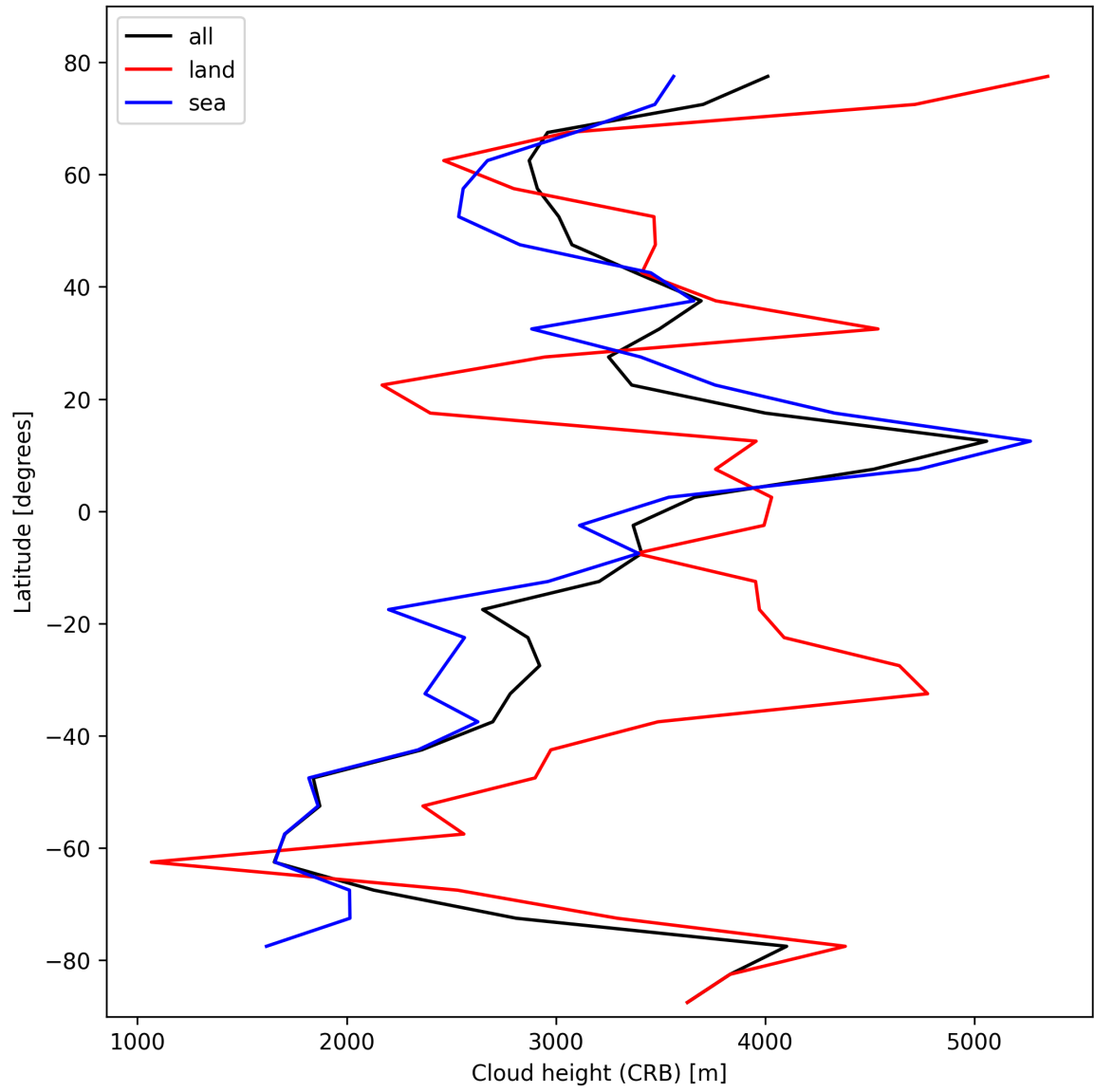
Figure 25: Zonal average of “Cloud height (CRB)” for 2025-10-24 to 2025-10-25.
