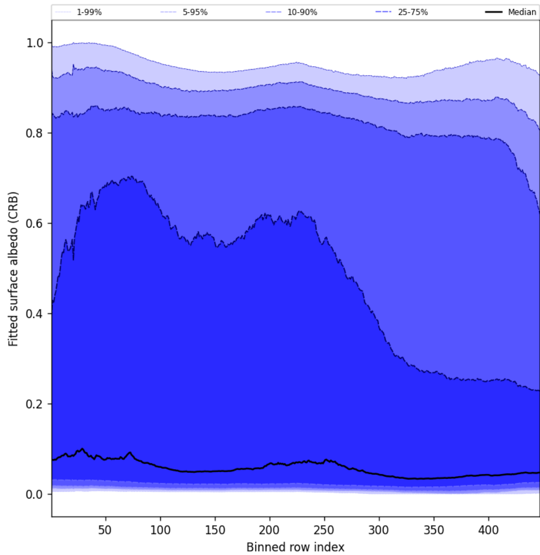
Figure 60: Along track statistics of “Fitted surface albedo (CRB)” for 2025-10-24 to 2025-10-25
