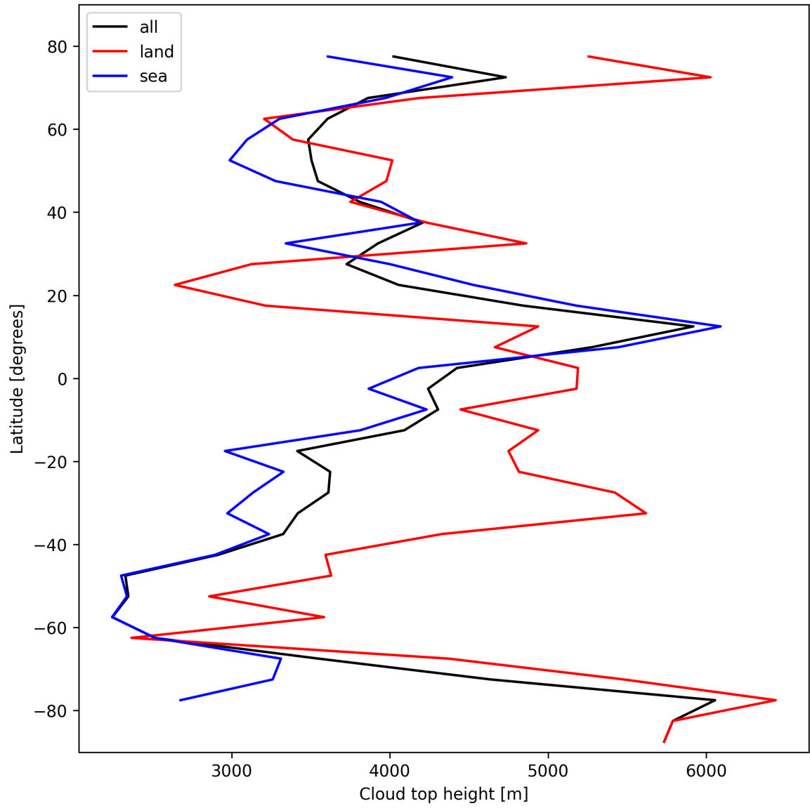
Figure 22: Zonal average of “Cloud top height” for 2025-10-24 to 2025-10-25.
