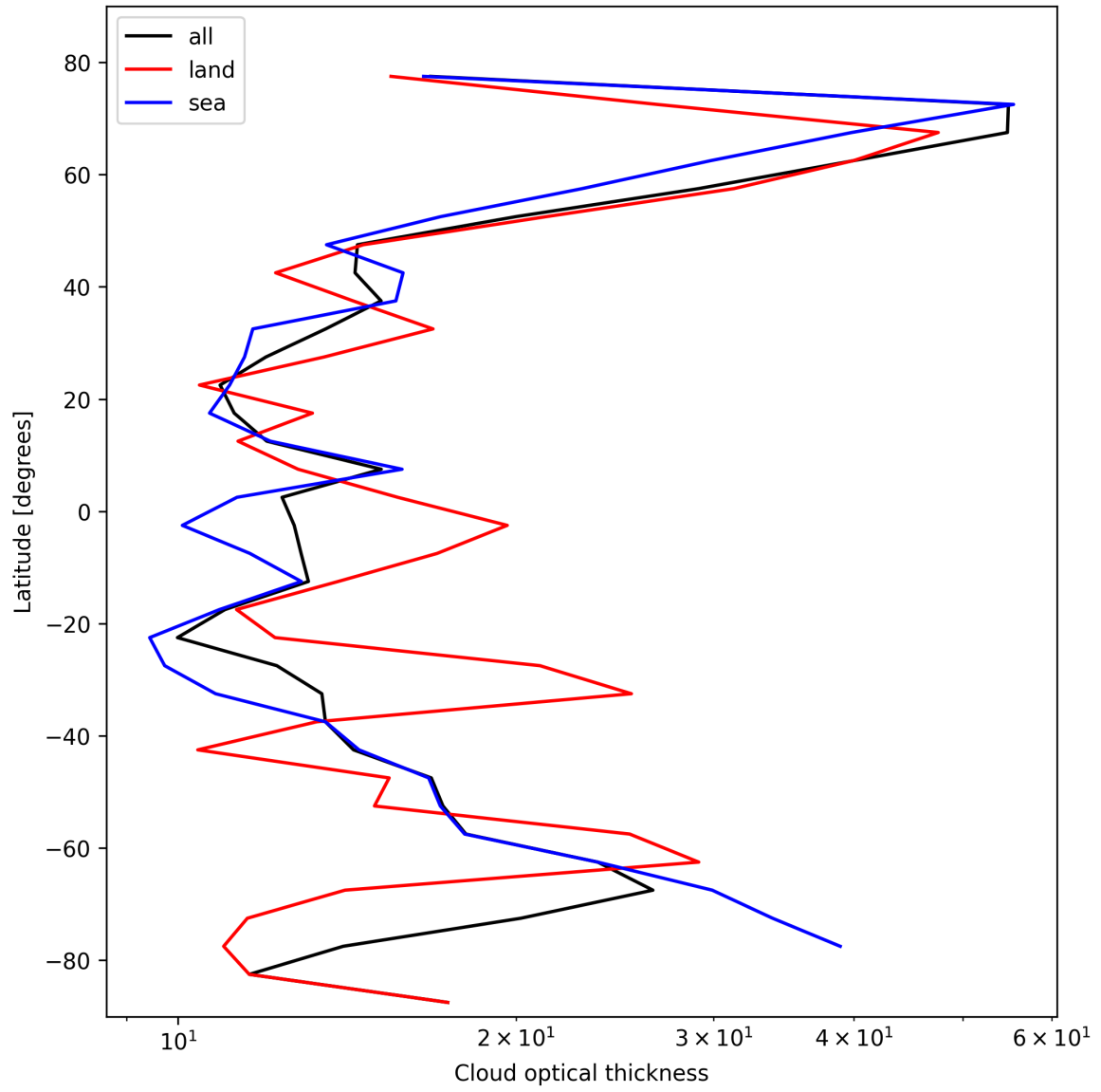
Figure 23: Zonal average of “Cloud optical thickness” for 2025-10-24 to 2025-10-25.
