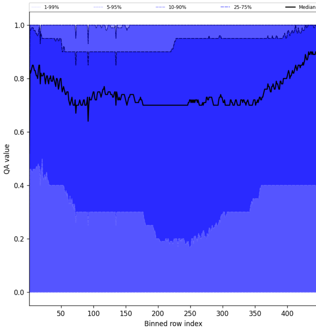
Figure 52: Along track statistics of “QA value” for 2025-10-24 to 2025-10-25
