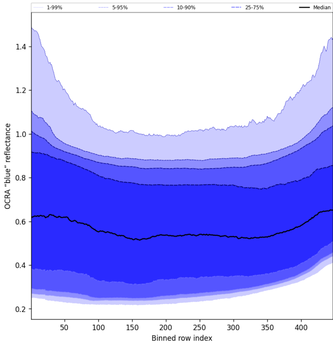
Figure 65: Along track statistics of “OCRA “blue” reflectance” for 2025-10-24 to 2025-10-25
