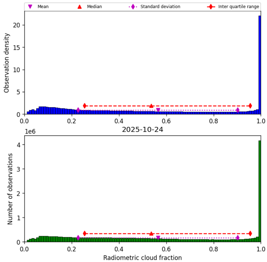
Figure 37: Histogram of “Radiometric cloud fraction” for 2025-10-24 to 2025-10-25
