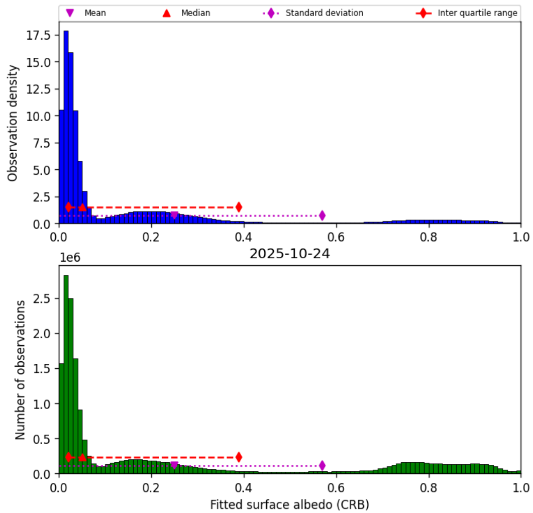
Figure 44: Histogram of “Fitted surface albedo (CRB)” for 2025-10-24 to 2025-10-25
