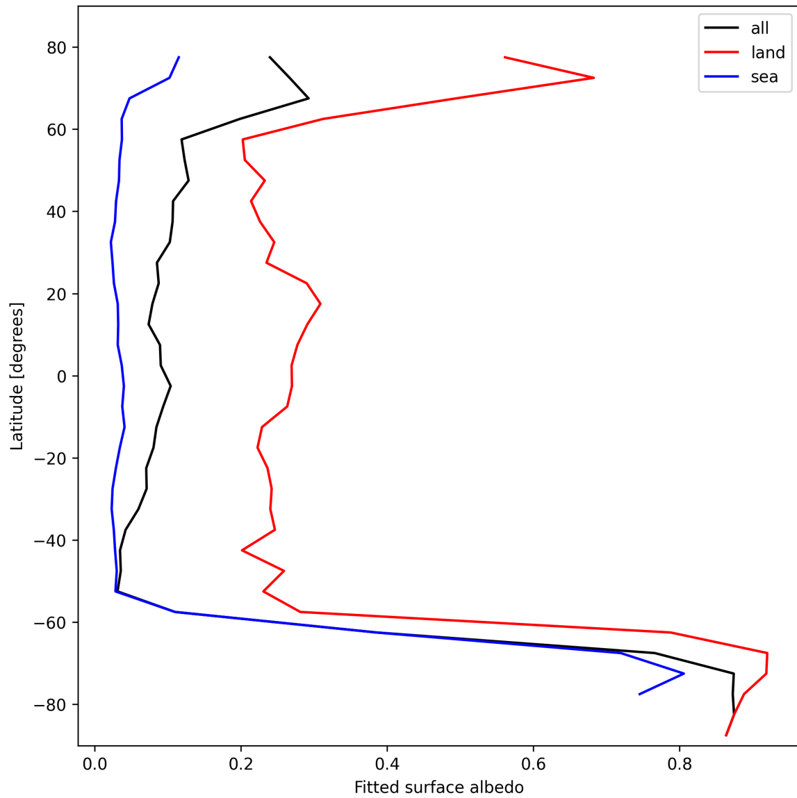
Figure 27: Zonal average of “Fitted surface albedo” for 2025-10-24 to 2025-10-25.
