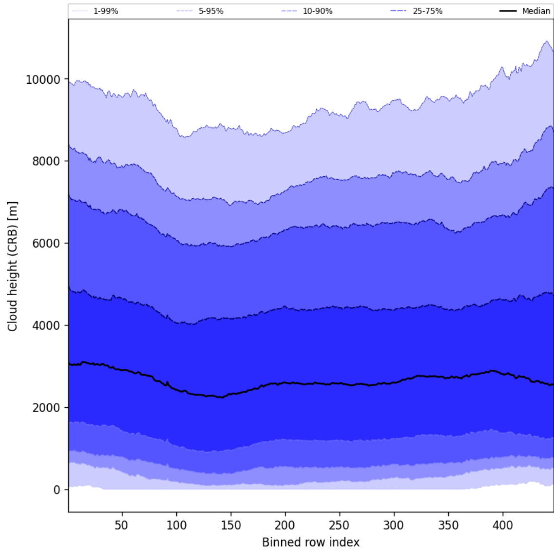
Figure 57: Along track statistics of “Cloud height (CRB)” for 2025-10-24 to 2025-10-25
