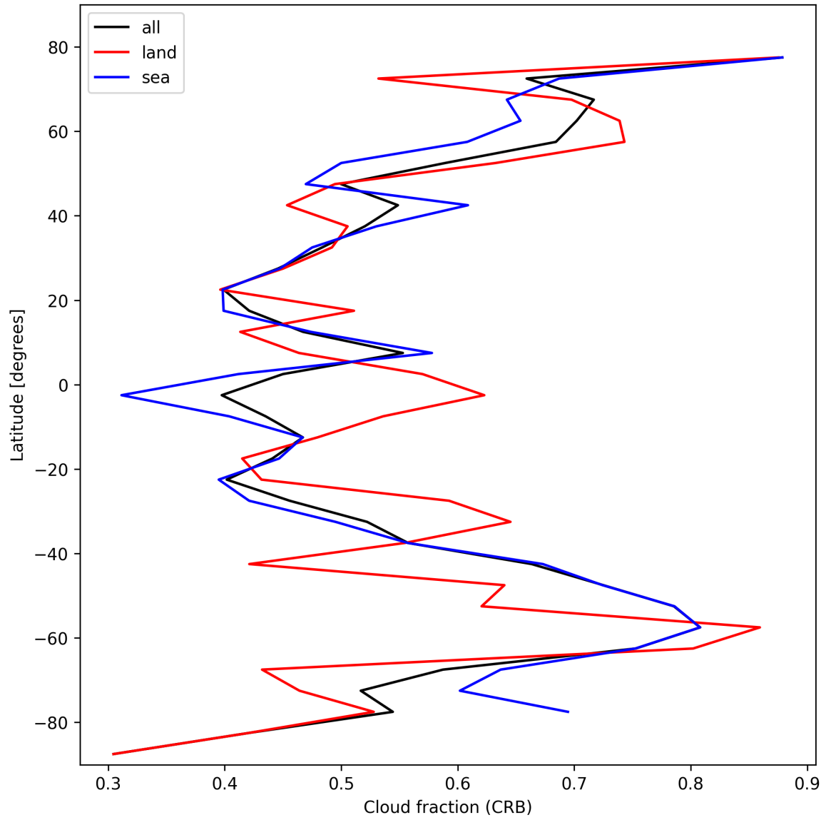
Figure 24: Zonal average of “Cloud fraction (CRB)” for 2025-10-24 to 2025-10-25.
