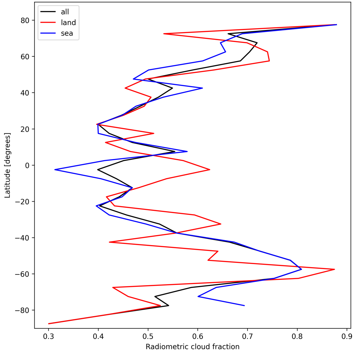
Figure 21: Zonal average of “Radiometric cloud fraction” for 2025-10-24 to 2025-10-25.
