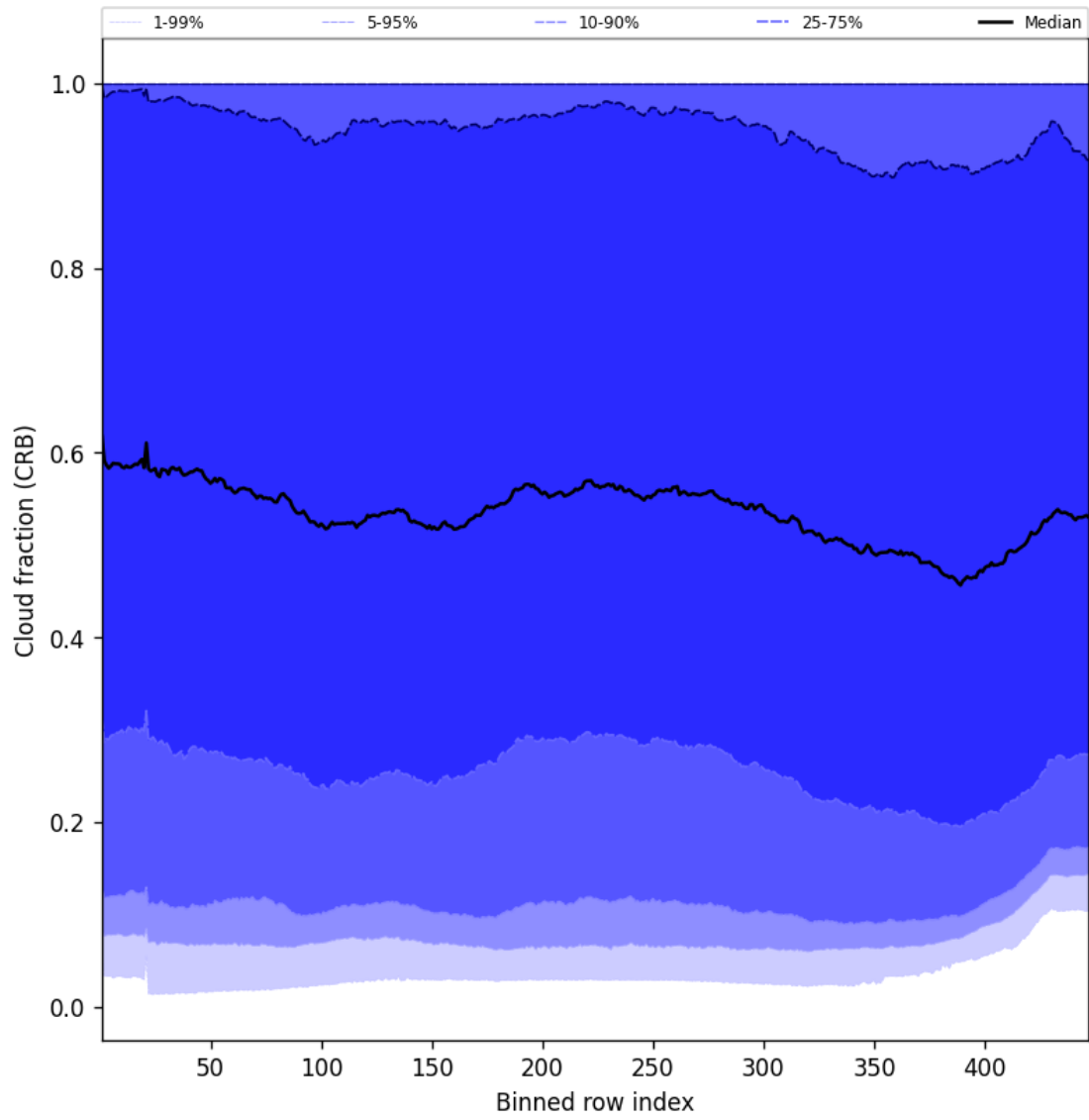
Figure 56: Along track statistics of “Cloud fraction (CRB)” for 2025-10-24 to 2025-10-25
