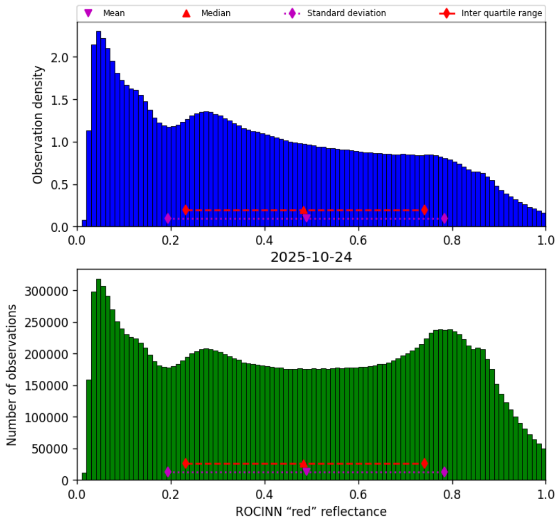
Figure 51: Histogram of “ROCINN “red” reflectance” for 2025-10-24 to 2025-10-25
