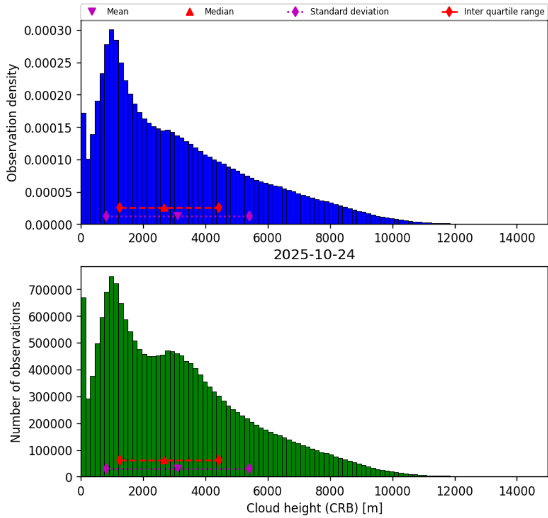
Figure 41: Histogram of “Cloud height (CRB)” for 2025-10-24 to 2025-10-25
