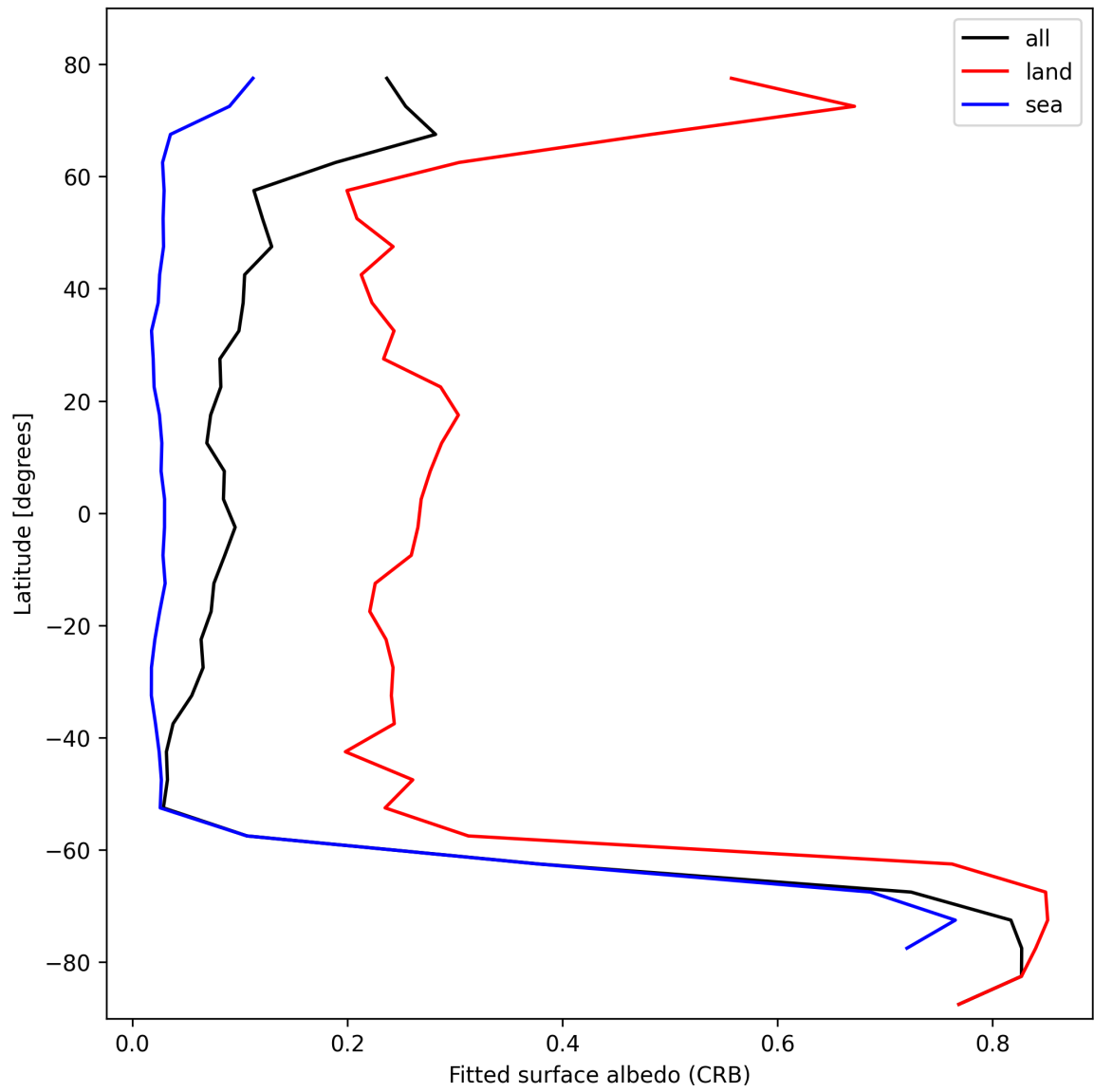
Figure 28: Zonal average of “Fitted surface albedo (CRB)” for 2025-10-24 to 2025-10-25.
