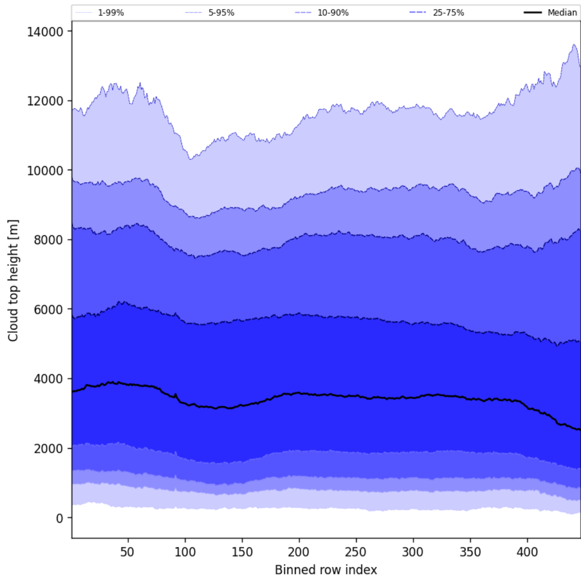
Figure 54: Along track statistics of “Cloud top height” for 2025-10-24 to 2025-10-25
