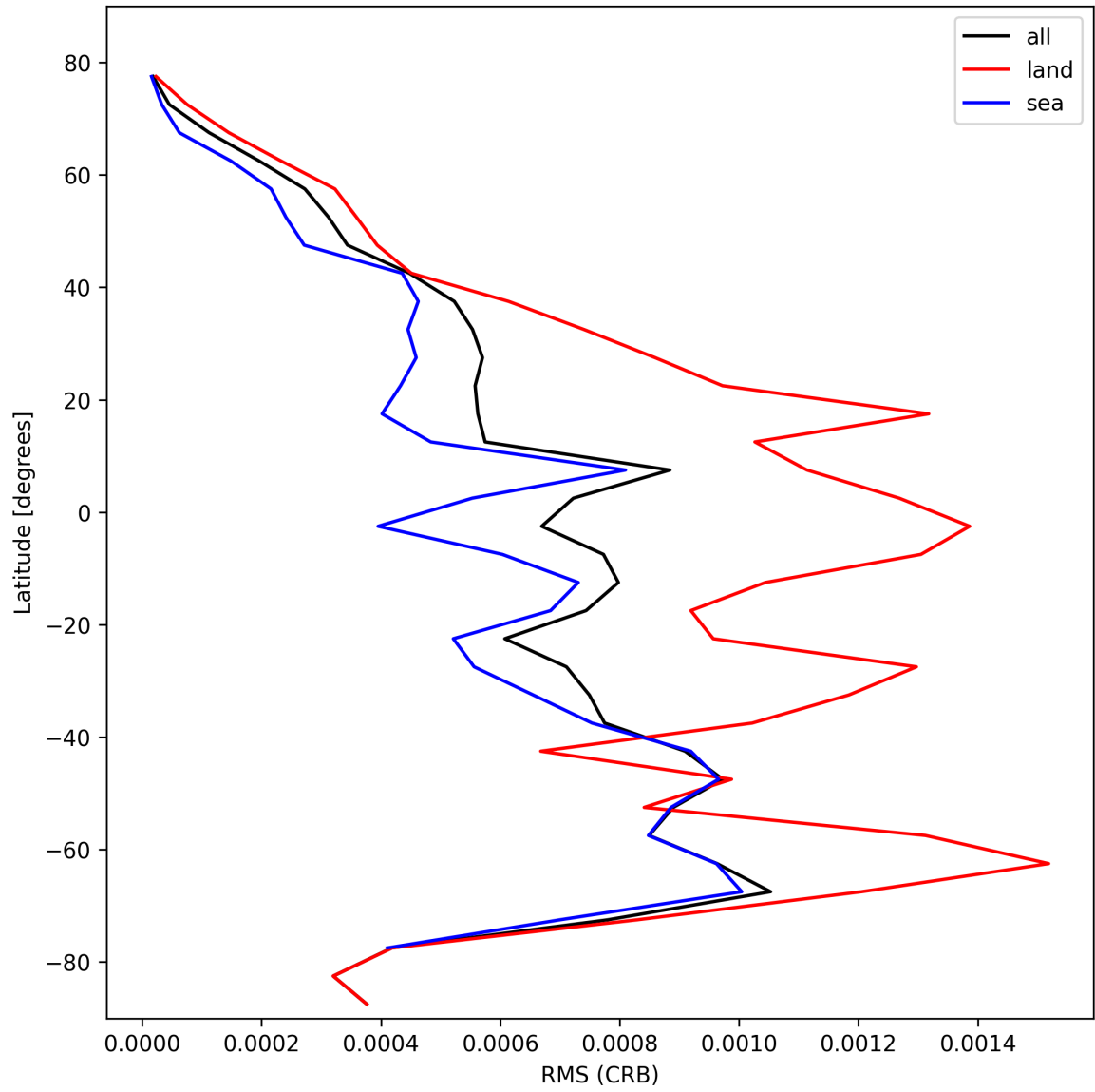
Figure 30: Zonal average of “RMS (CRB)” for 2025-10-24 to 2025-10-25.
