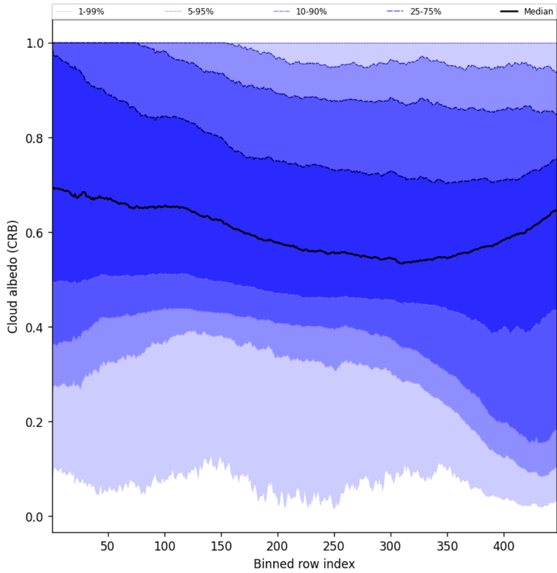
Figure 58: Along track statistics of “Cloud albedo (CRB)” for 2025-10-24 to 2025-10-25
