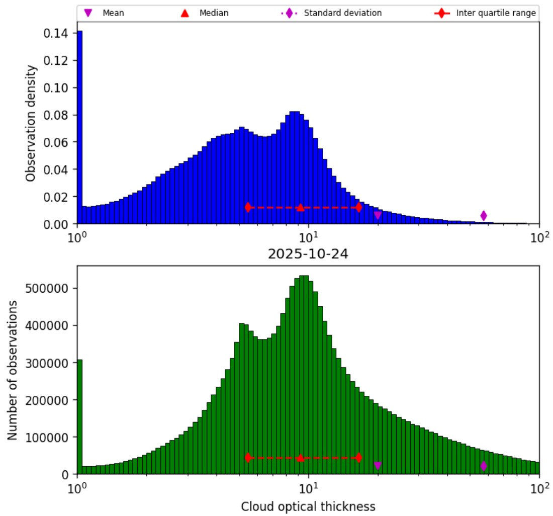
Figure 39: Histogram of “Cloud optical thickness” for 2025-10-24 to 2025-10-25
