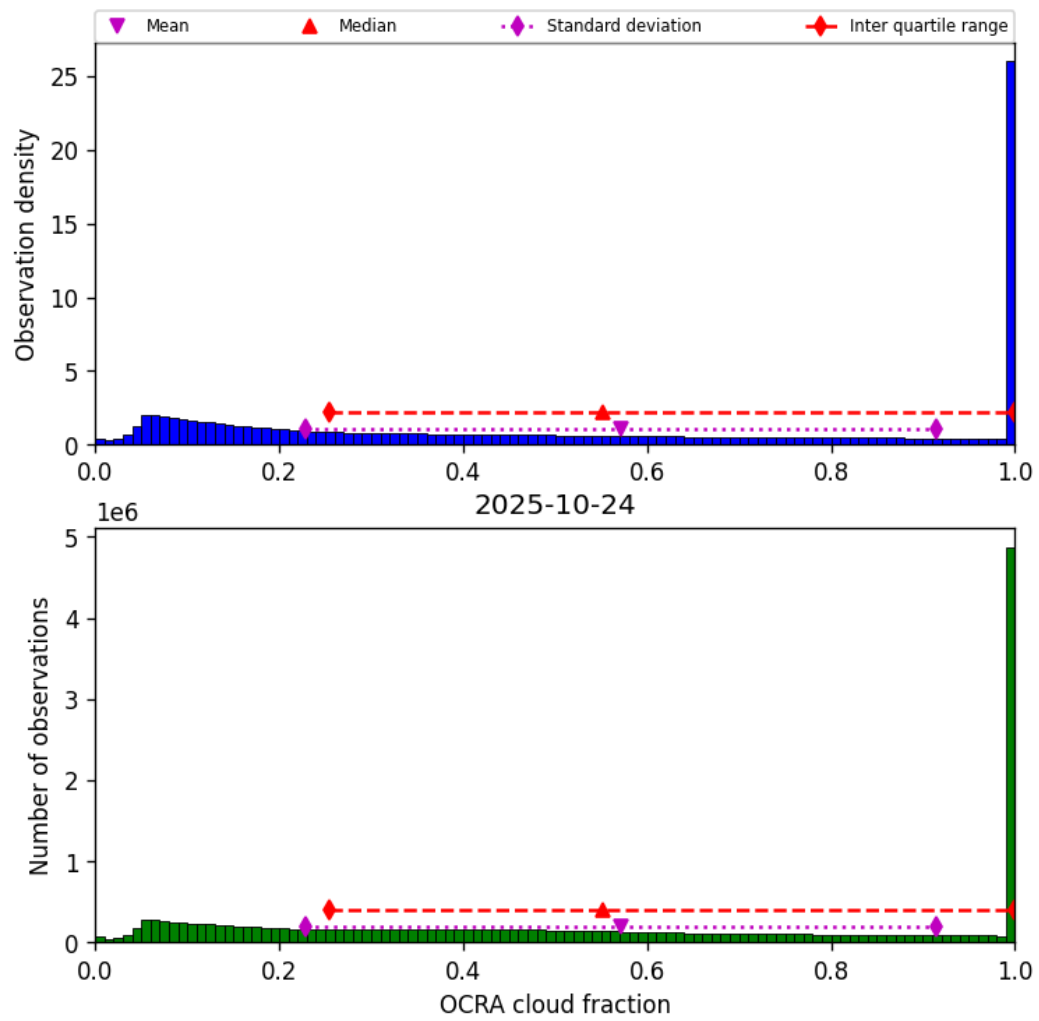
Figure 48: Histogram of “OCRA cloud fraction” for 2025-10-24 to 2025-10-25
