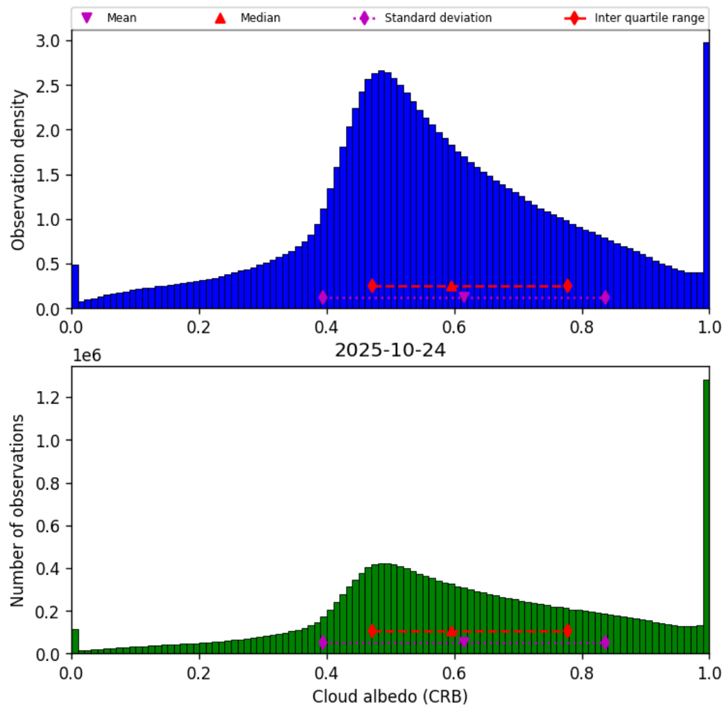
Figure 42: Histogram of “Cloud albedo (CRB)” for 2025-10-24 to 2025-10-25
