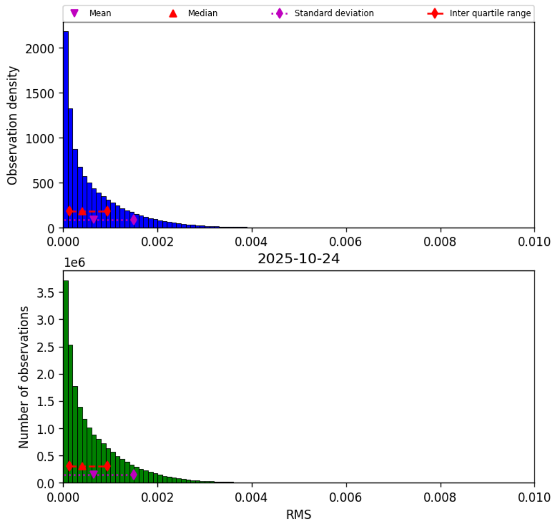
Figure 45: Histogram of “RMS” for 2025-10-24 to 2025-10-25
