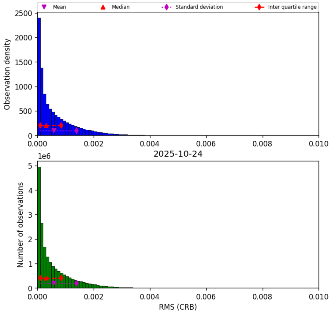
Figure 46: Histogram of “RMS (CRB)” for 2025-10-24 to 2025-10-25
