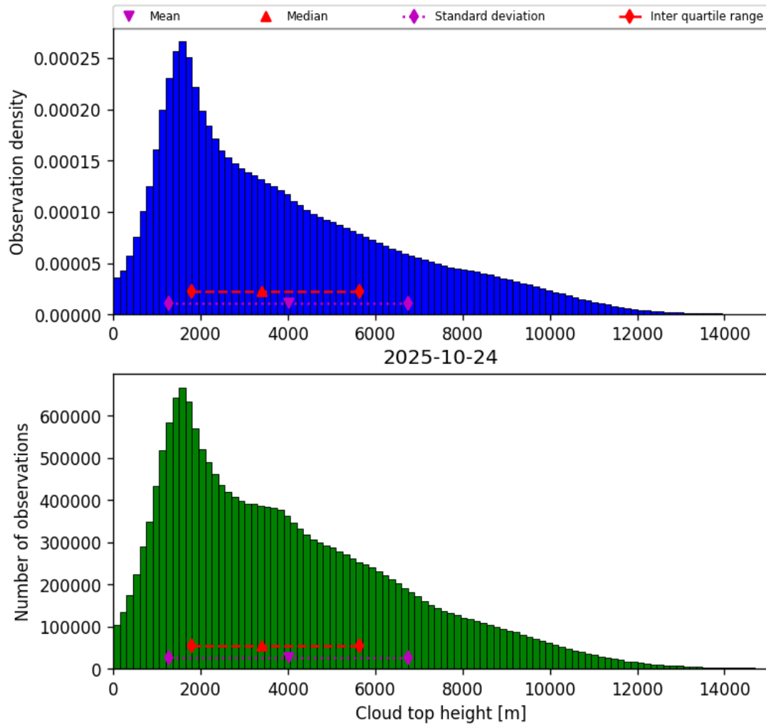
Figure 38: Histogram of “Cloud top height” for 2025-10-24 to 2025-10-25
