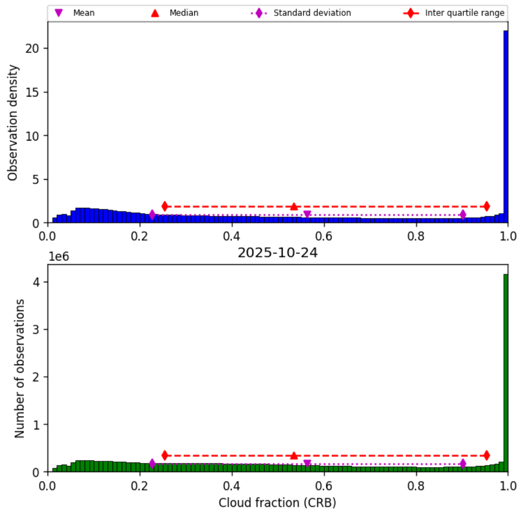
Figure 40: Histogram of “Cloud fraction (CRB)” for 2025-10-24 to 2025-10-25
