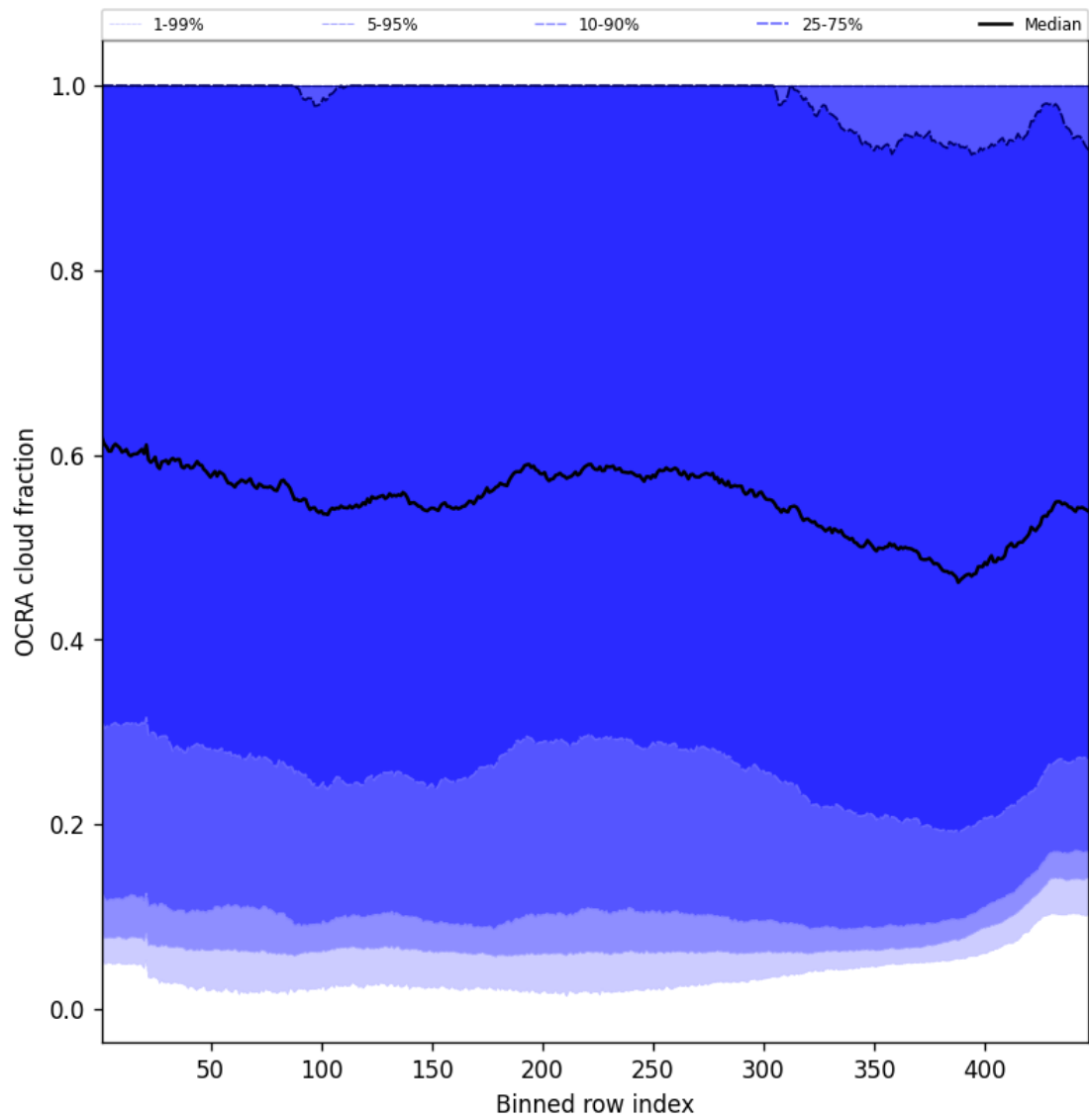
Figure 64: Along track statistics of “OCRA cloud fraction” for 2025-10-24 to 2025-10-25
