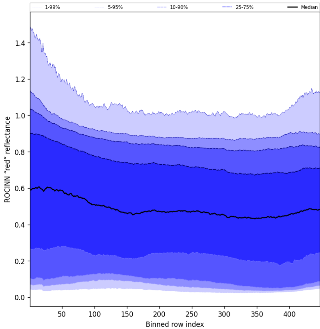
Figure 67: Along track statistics of "ROCINN "red" reflectance" for 2025-10-24 to 2025-10-25
