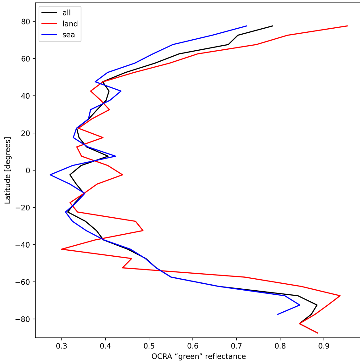
Figure 34: Zonal average of “OCRA “green” reflectance” for 2025-10-24 to 2025-10-25.
