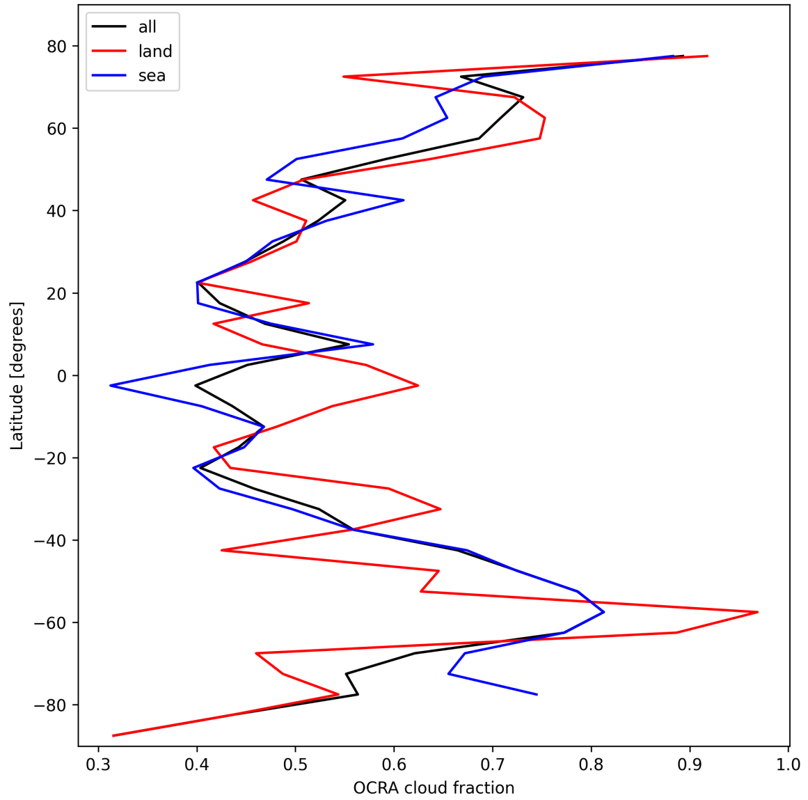
Figure 32: Zonal average of “OCRA cloud fraction” for 2025-10-24 to 2025-10-25.
