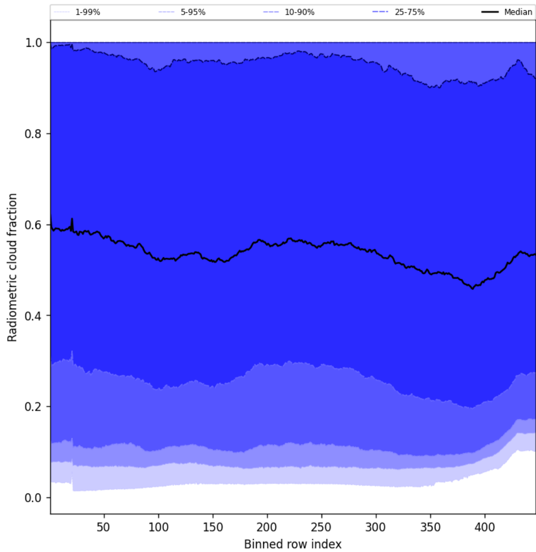
Figure 53: Along track statistics of “Radiometric cloud fraction” for 2025-10-24 to 2025-10-25
