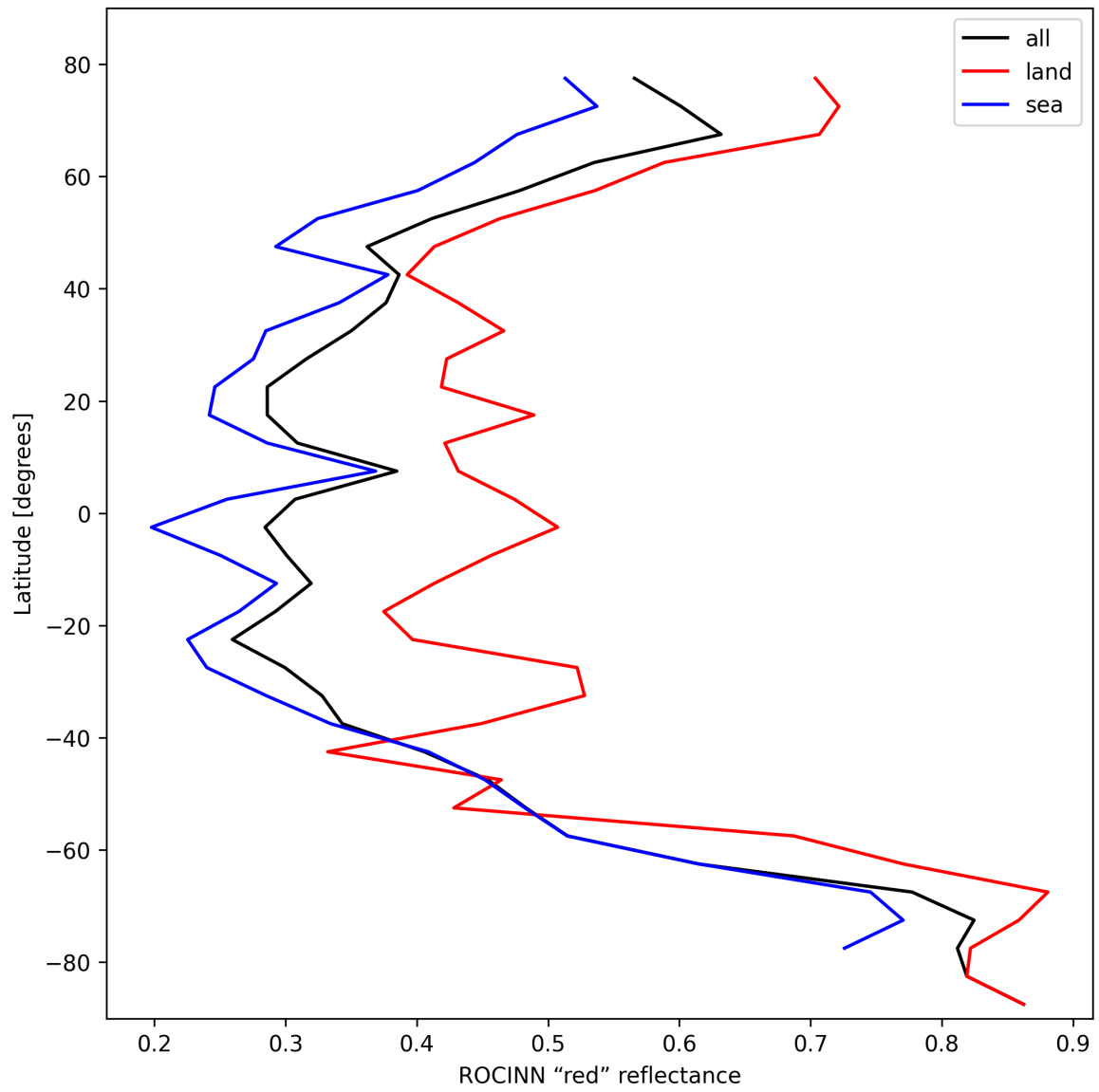
Figure 35: Zonal average of “ROCINN “red” reflectance” for 2025-10-24 to 2025-10-25.
