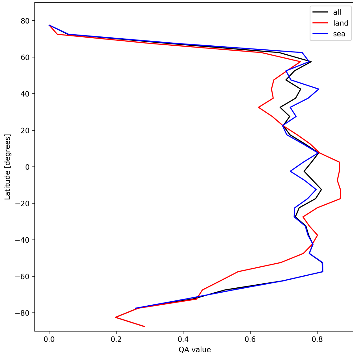
Figure 20: Zonal average of “QA value” for 2025-10-24 to 2025-10-25.
