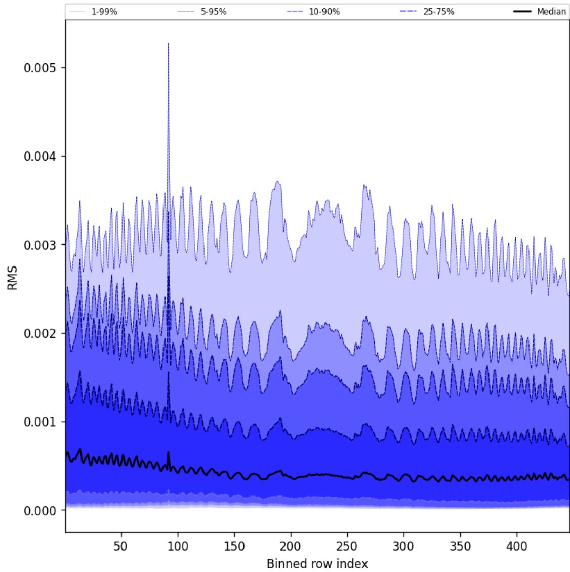
Figure 61: Along track statistics of “RMS” for 2025-10-24 to 2025-10-25
