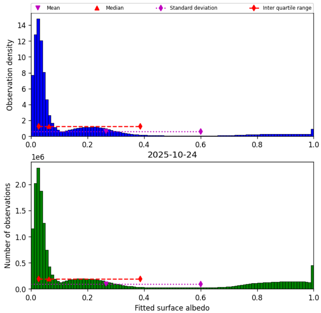
Figure 43: Histogram of “Fitted surface albedo” for 2025-10-24 to 2025-10-25
