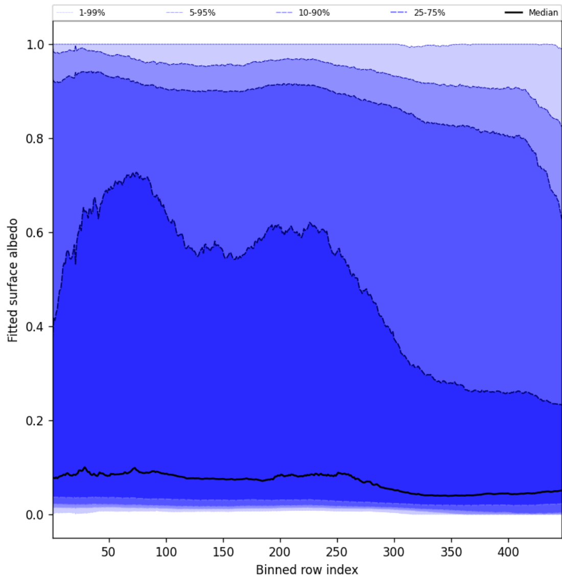
Figure 59: Along track statistics of “Fitted surface albedo” for 2025-10-24 to 2025-10-25
