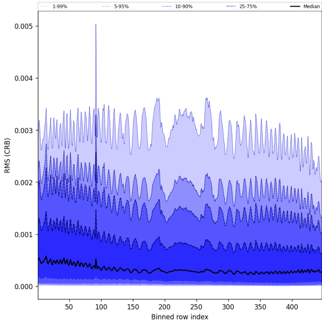
Figure 62: Along track statistics of “RMS (CRB)” for 2025-10-24 to 2025-10-25
