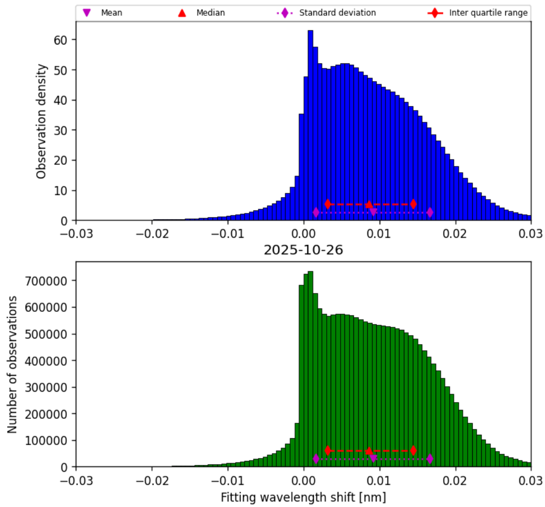
Figure 47: Histogram of “Fitting wavelength shift” for 2025-10-26 to 2025-10-27
