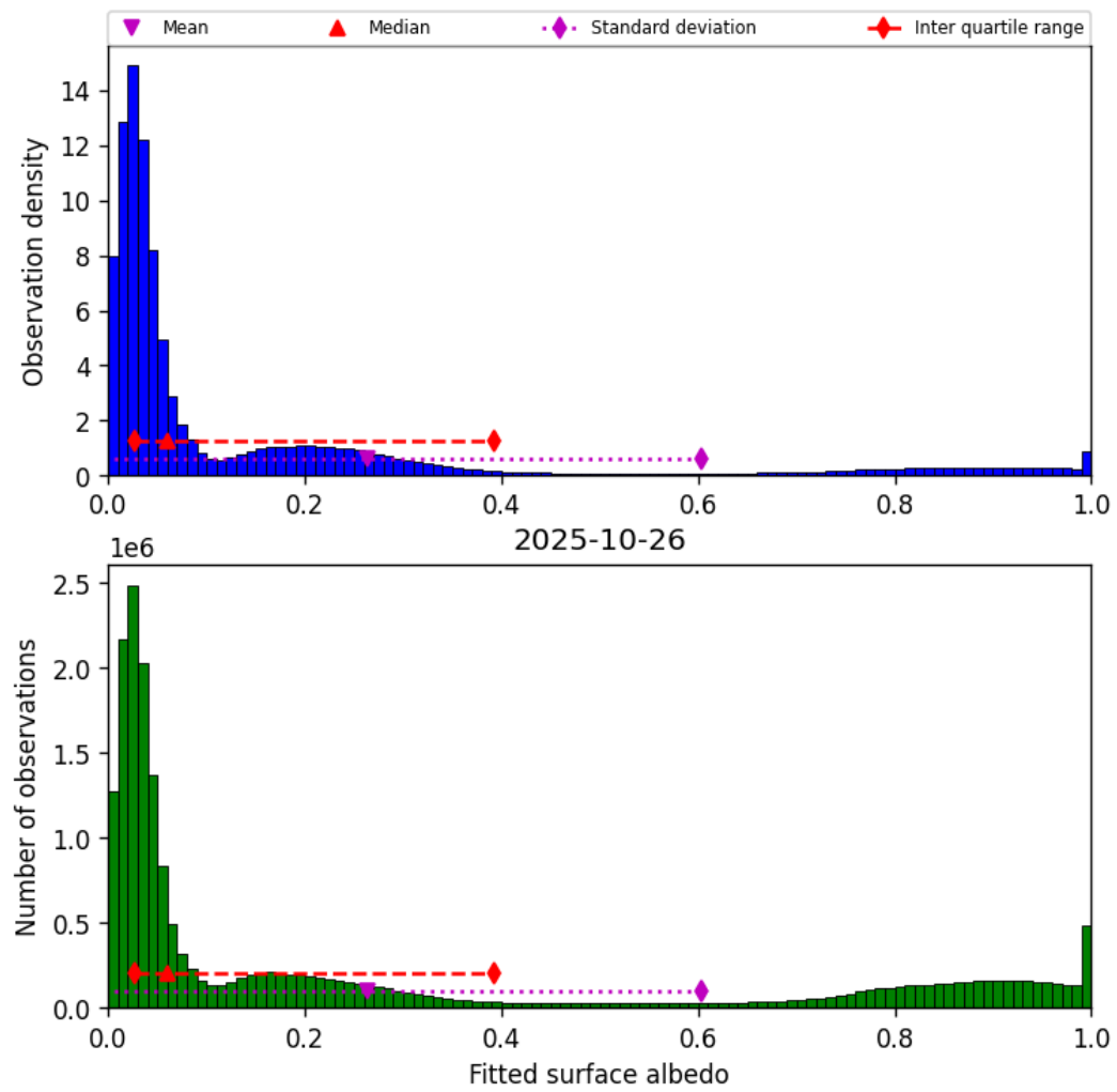
Figure 43: Histogram of “Fitted surface albedo” for 2025-10-26 to 2025-10-27
