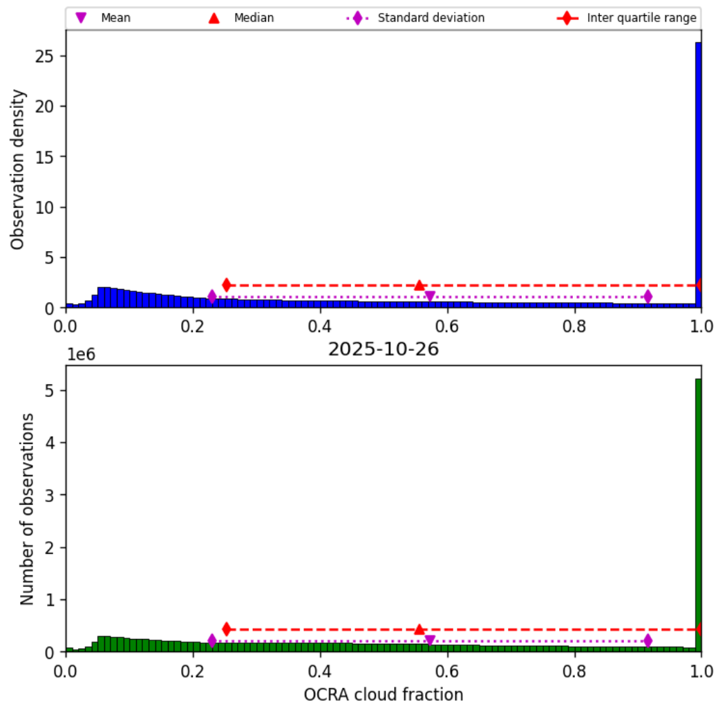
Figure 48: Histogram of “OCRA cloud fraction” for 2025-10-26 to 2025-10-27
