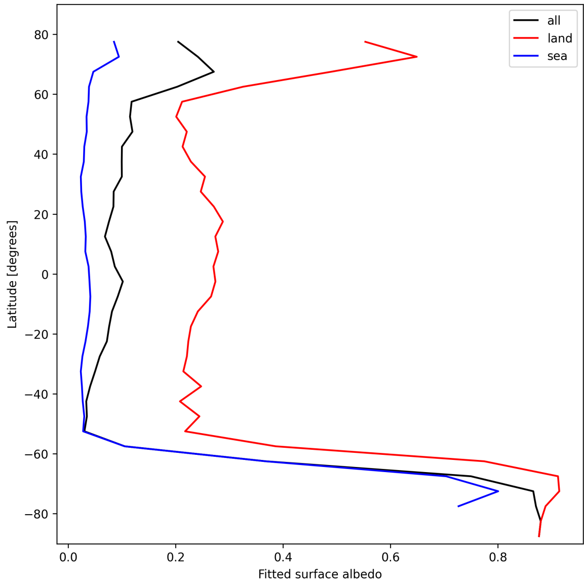
Figure 27: Zonal average of “Fitted surface albedo” for 2025-10-26 to 2025-10-27.
