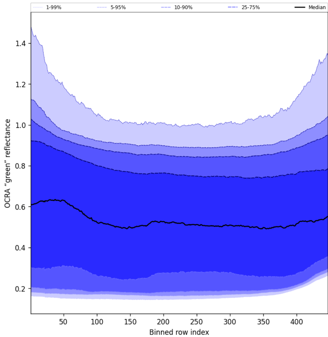
Figure 66: Along track statistics of “OCRA “green” reflectance” for 2025-10-26 to 2025-10-27
