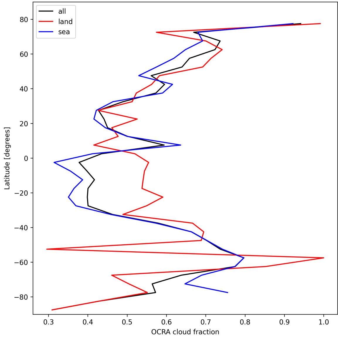
Figure 32: Zonal average of “OCRA cloud fraction” for 2025-10-26 to 2025-10-27.
