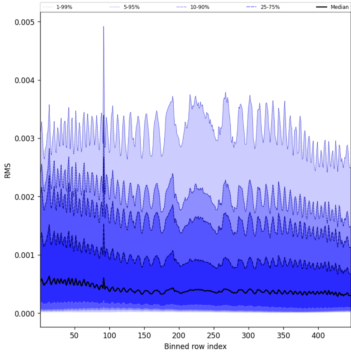
Figure 61: Along track statistics of “RMS” for 2025-10-26 to 2025-10-27
