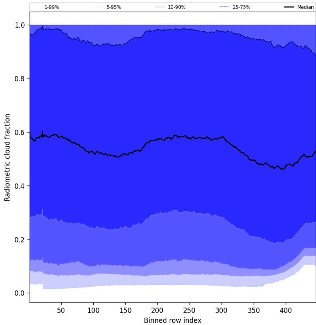
Figure 53: Along track statistics of “Radiometric cloud fraction” for 2025-10-26 to 2025-10-27
