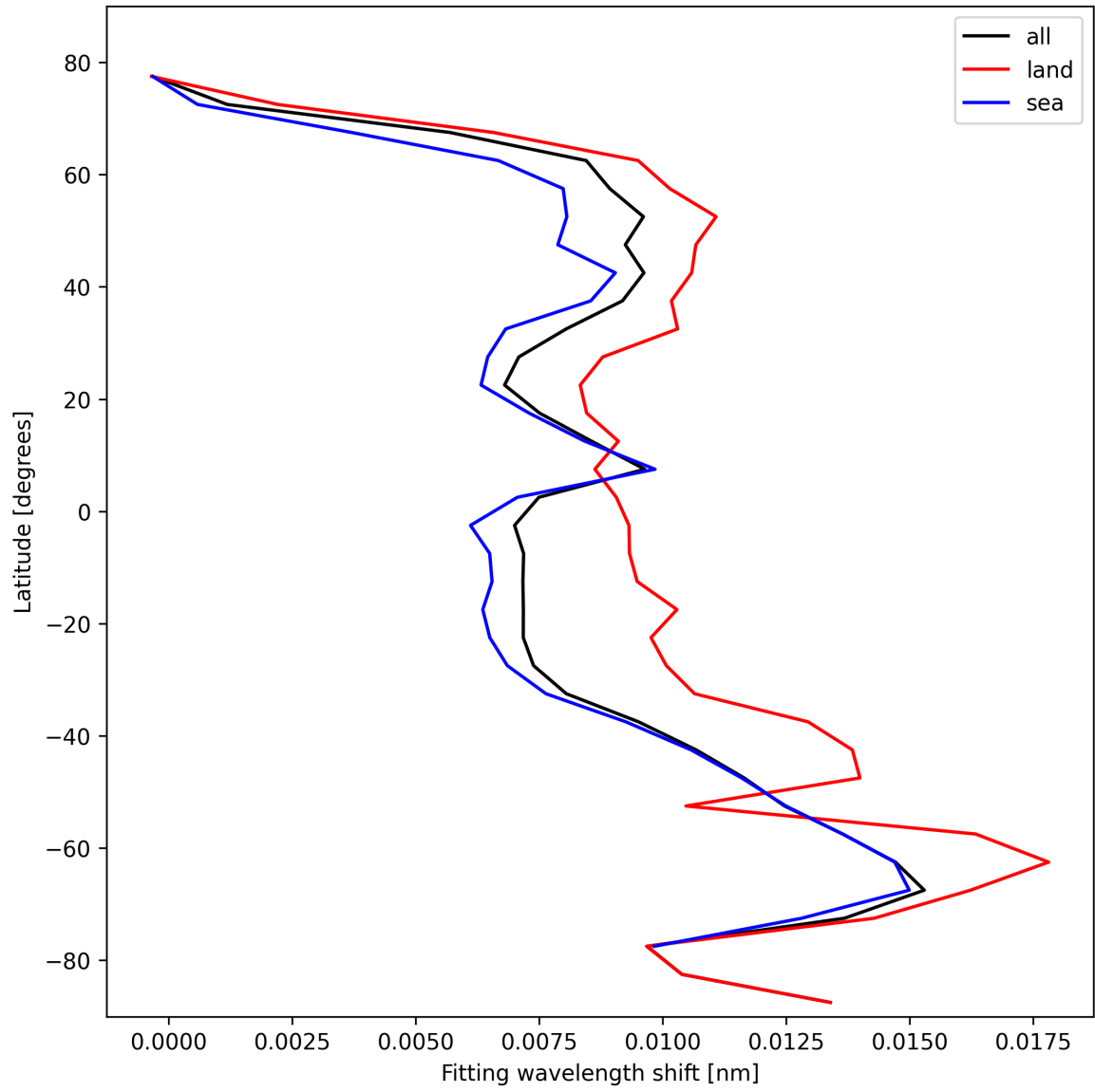
Figure 31: Zonal average of “Fitting wavelength shift” for 2025-10-26 to 2025-10-27.
