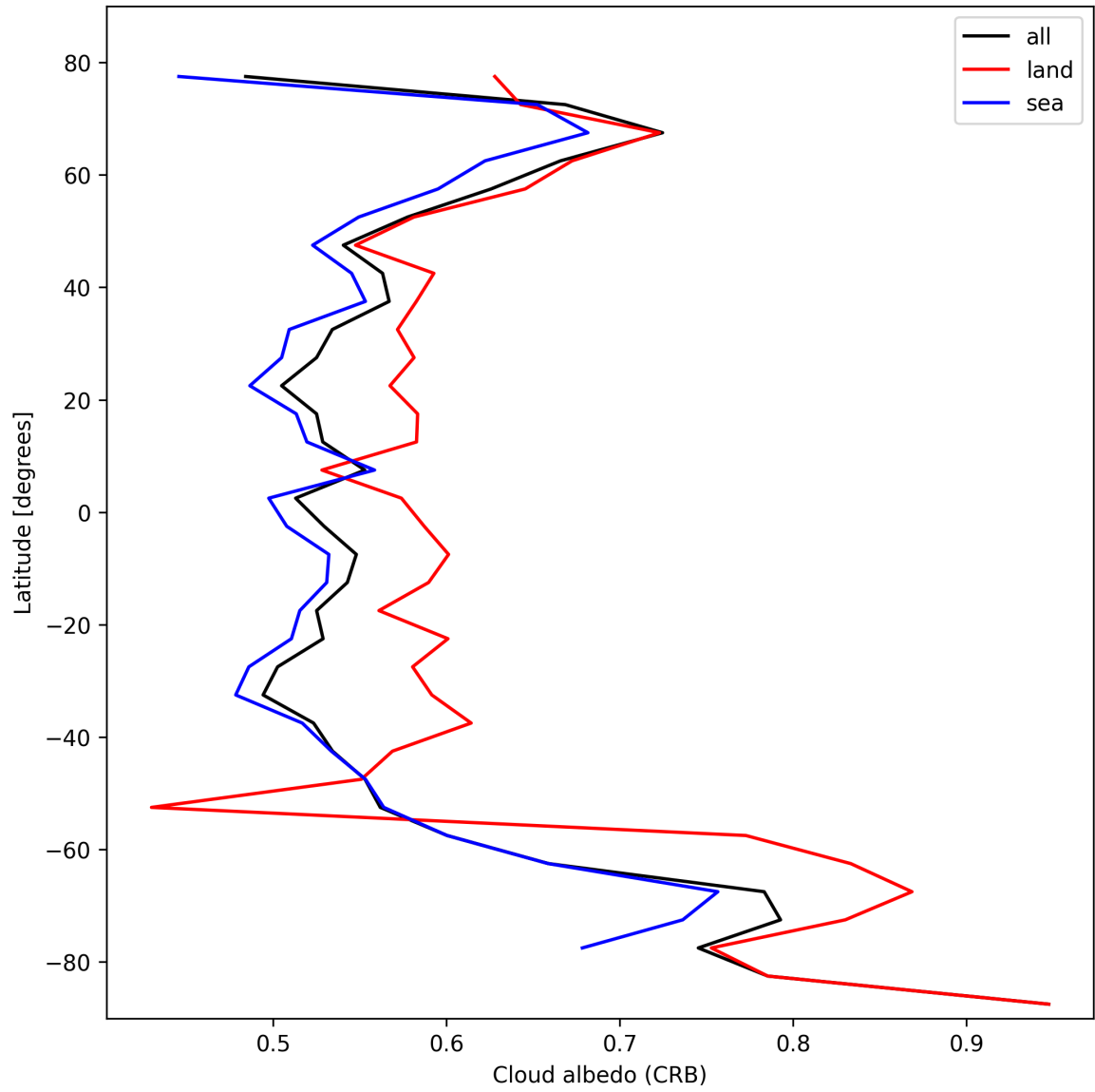
Figure 26: Zonal average of “Cloud albedo (CRB)” for 2025-10-26 to 2025-10-27.
