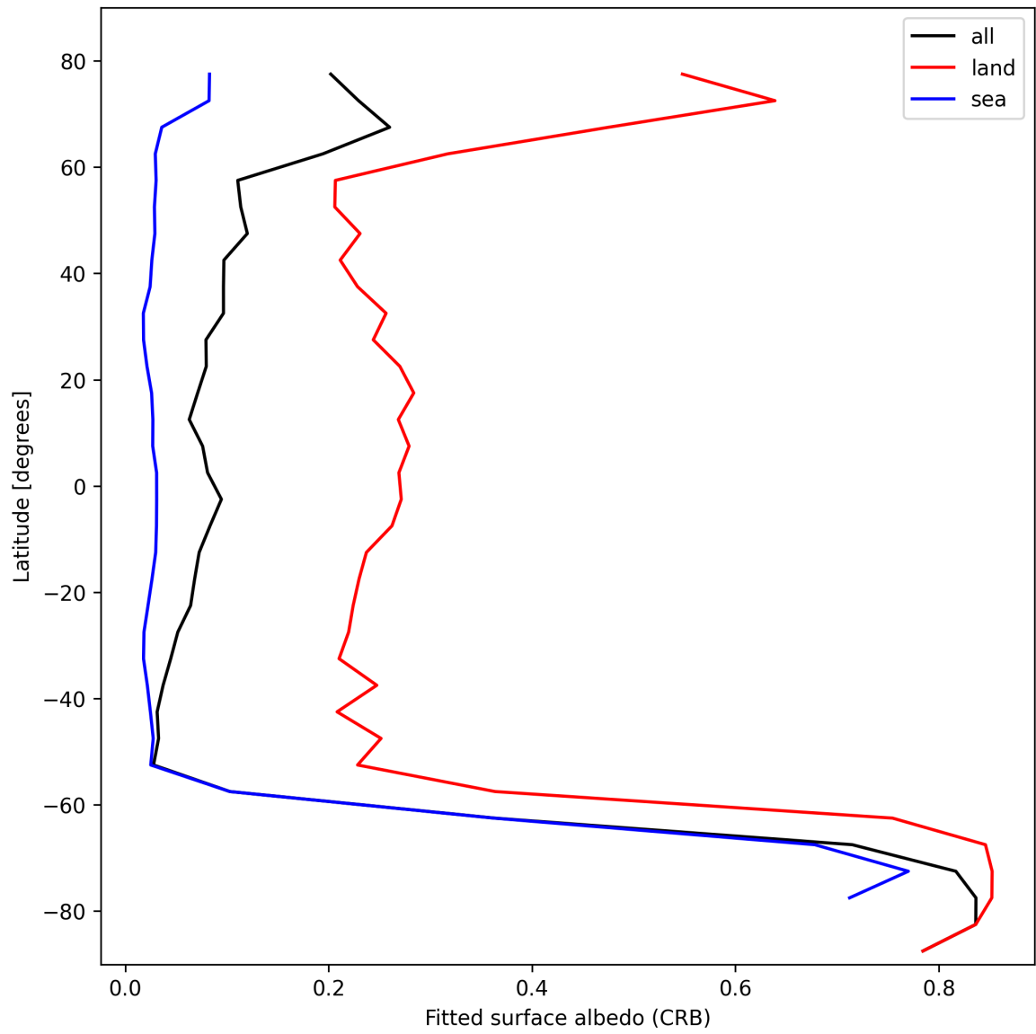
Figure 28: Zonal average of “Fitted surface albedo (CRB)” for 2025-10-26 to 2025-10-27.
