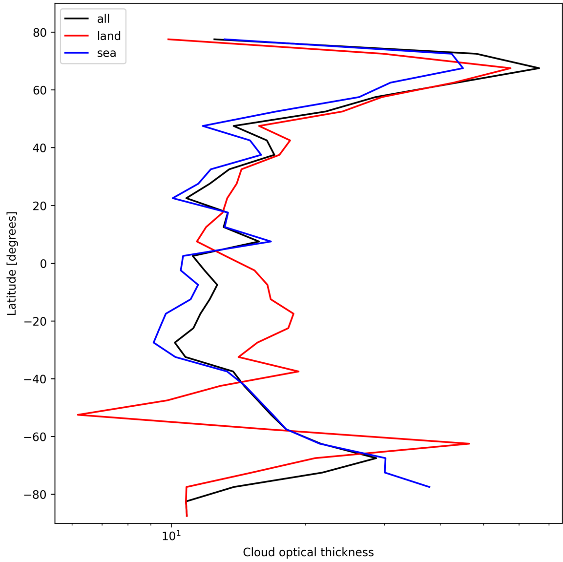
Figure 23: Zonal average of “Cloud optical thickness” for 2025-10-26 to 2025-10-27.
