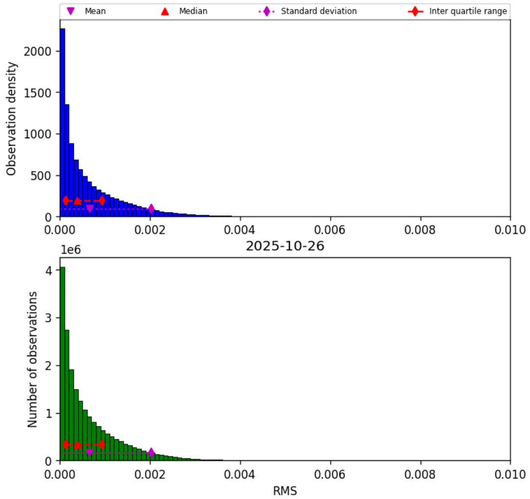
Figure 45: Histogram of “RMS” for 2025-10-26 to 2025-10-27
