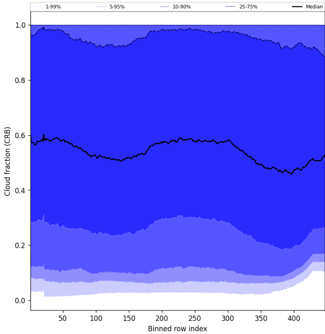
Figure 56: Along track statistics of “Cloud fraction (CRB)” for 2025-10-26 to 2025-10-27
