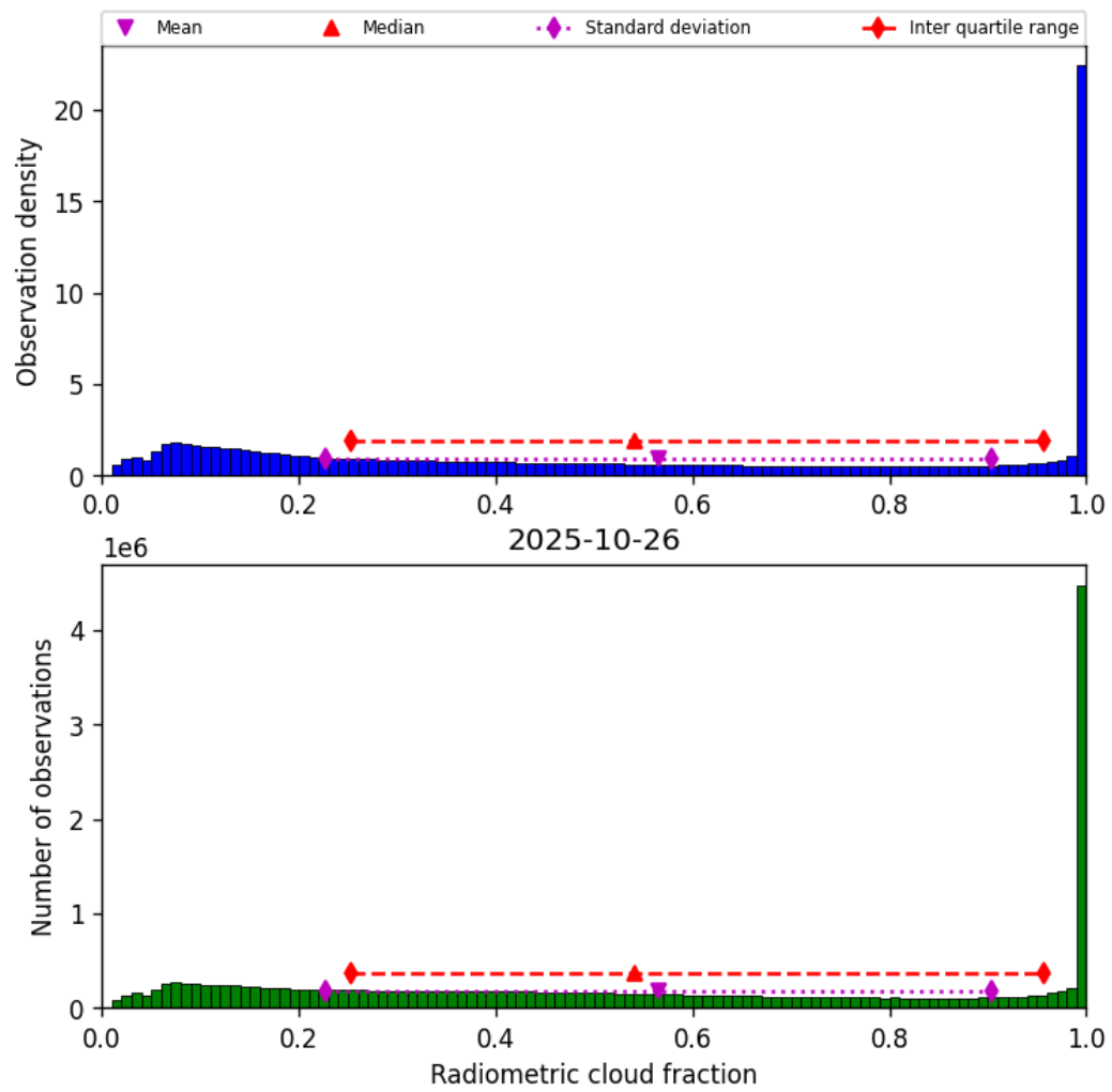
Figure 37: Histogram of “Radiometric cloud fraction” for 2025-10-26 to 2025-10-27
