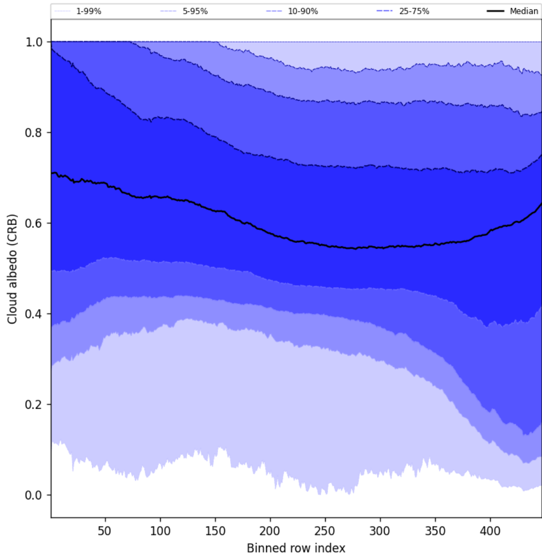
Figure 58: Along track statistics of “Cloud albedo (CRB)” for 2025-10-26 to 2025-10-27
