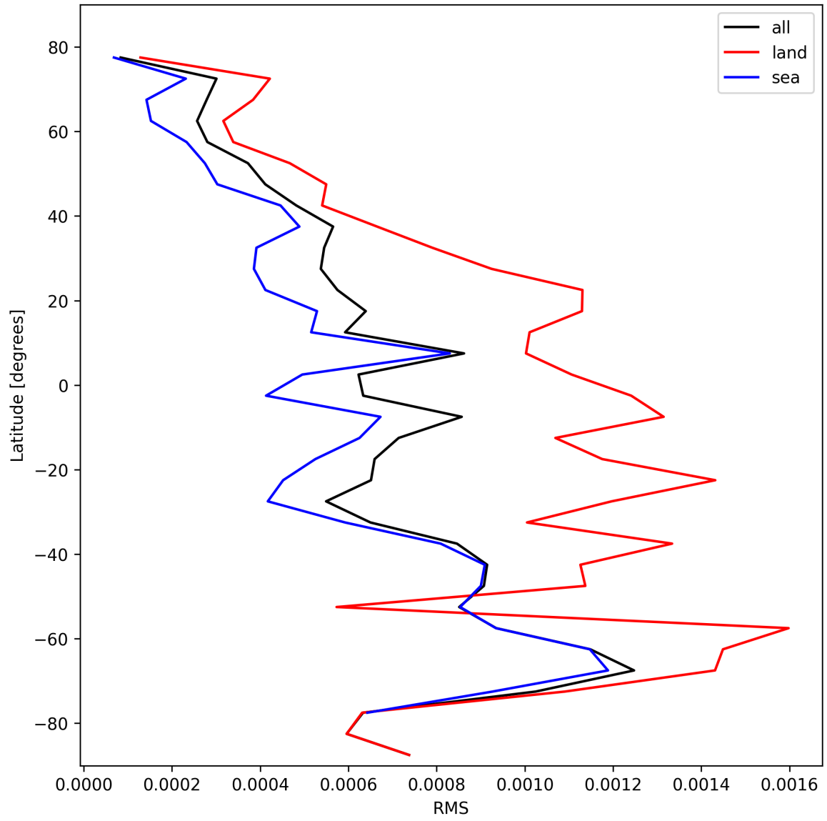
Figure 29: Zonal average of “RMS” for 2025-10-26 to 2025-10-27.
