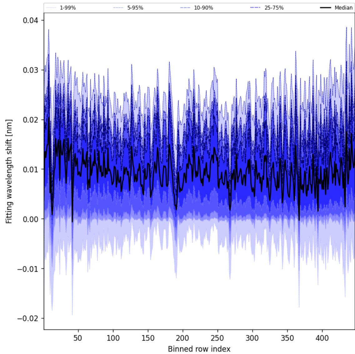
Figure 63: Along track statistics of “Fitting wavelength shift” for 2025-10-26 to 2025-10-27
