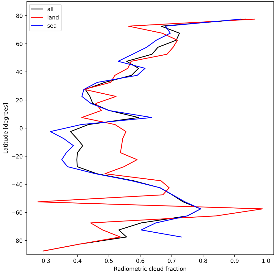
Figure 21: Zonal average of “Radiometric cloud fraction” for 2025-10-26 to 2025-10-27.
