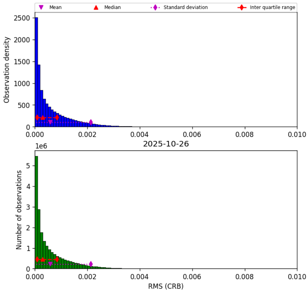
Figure 46: Histogram of “RMS (CRB)” for 2025-10-26 to 2025-10-27
