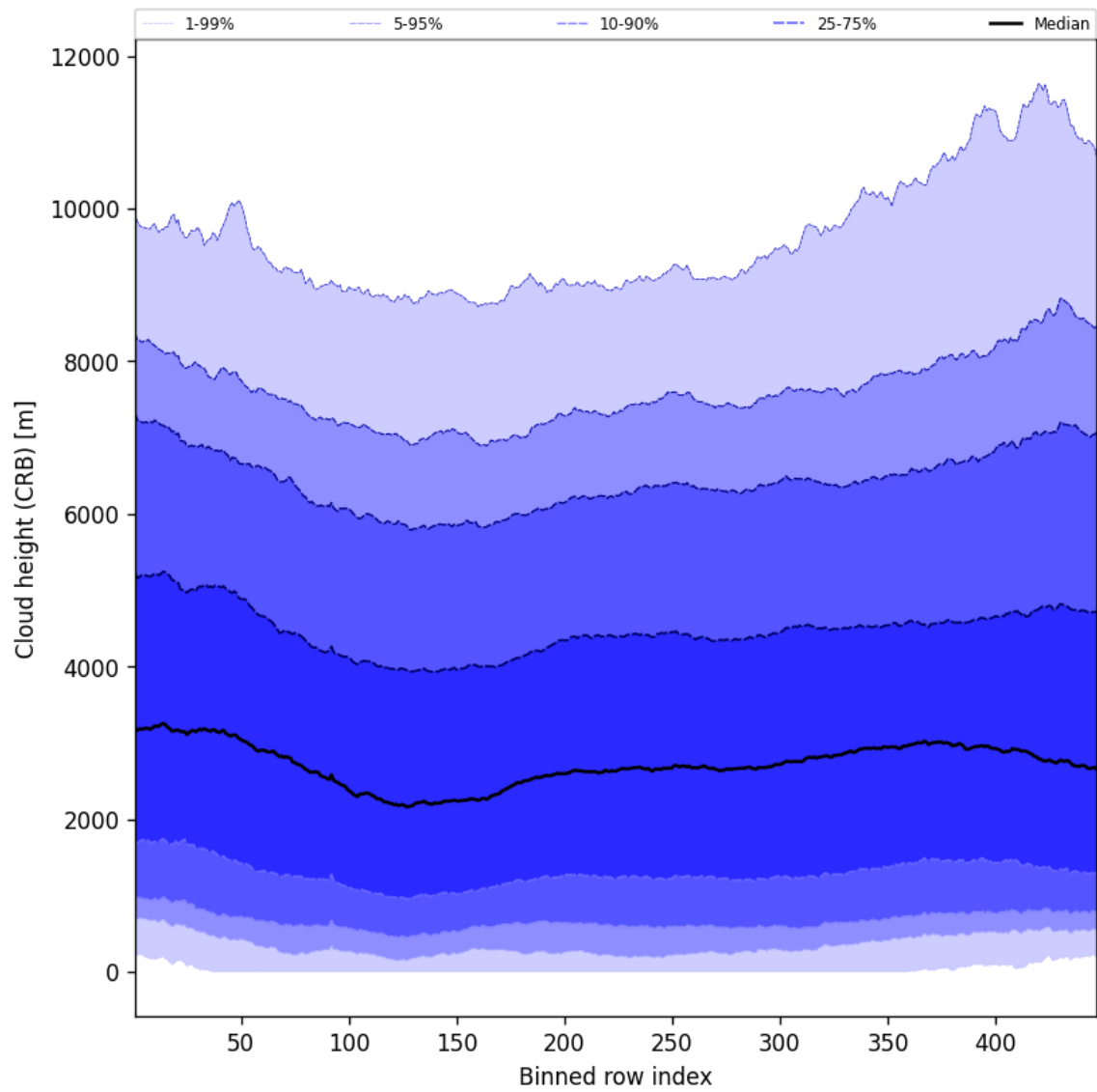
Figure 57: Along track statistics of “Cloud height (CRB)” for 2025-10-26 to 2025-10-27
