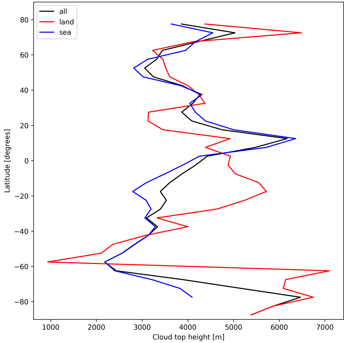
Figure 22: Zonal average of “Cloud top height” for 2025-10-26 to 2025-10-27.
