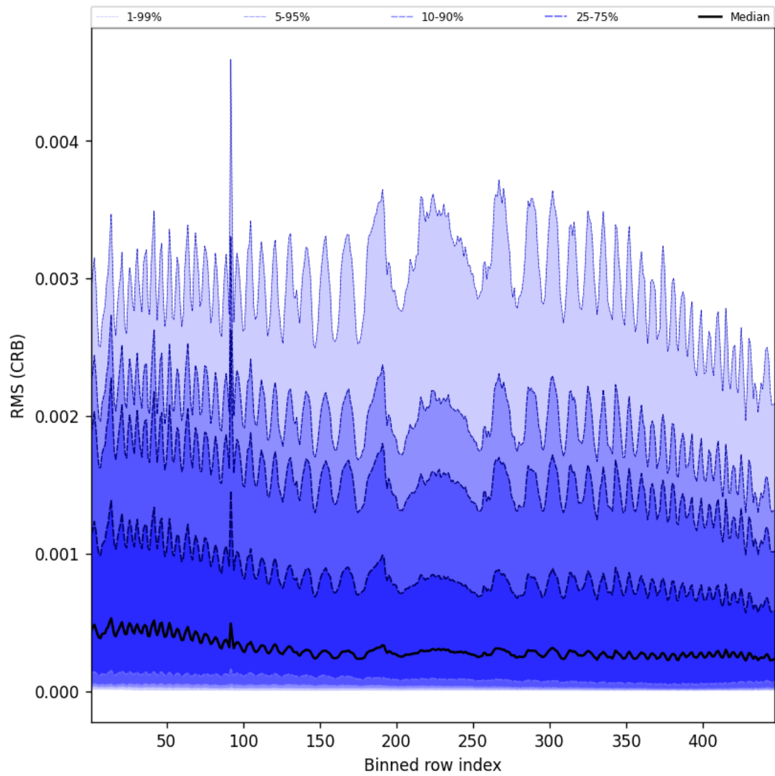
Figure 62: Along track statistics of “RMS (CRB)” for 2025-10-26 to 2025-10-27
