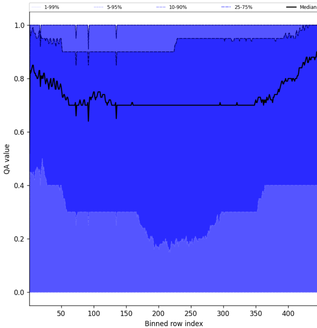
Figure 52: Along track statistics of “QA value” for 2025-10-26 to 2025-10-27
