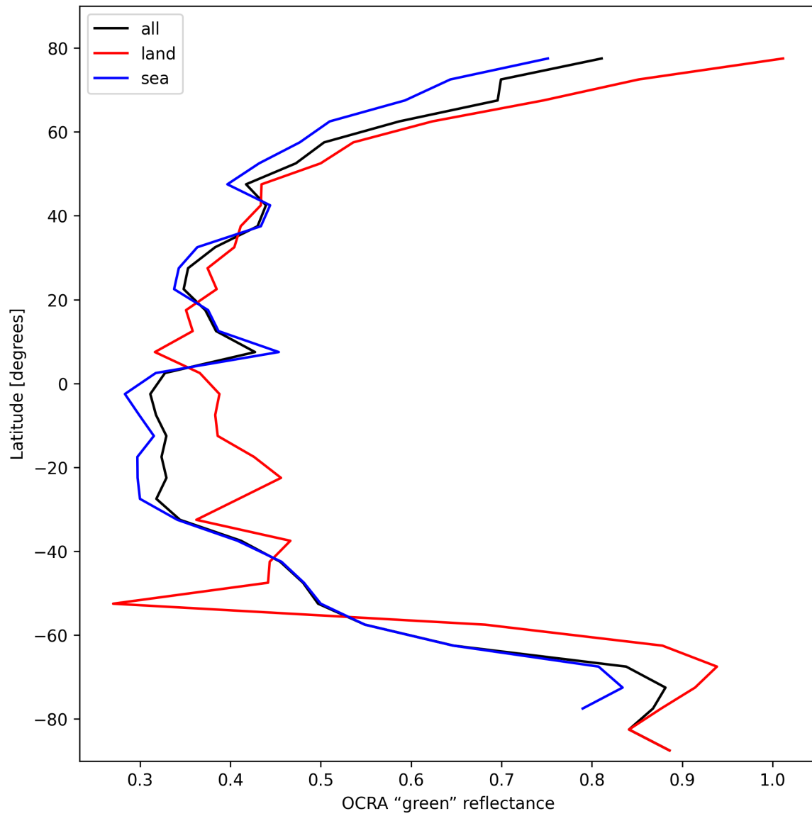
Figure 34: Zonal average of “OCRA “green” reflectance” for 2025-10-26 to 2025-10-27.
