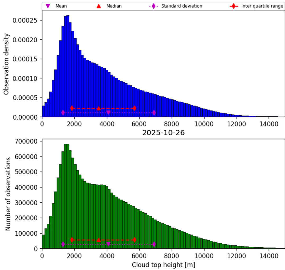
Figure 38: Histogram of “Cloud top height” for 2025-10-26 to 2025-10-27
