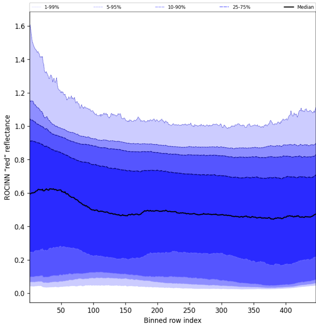
Figure 67: Along track statistics of "ROCINN "red" reflectance" for 2025-10-26 to 2025-10-27
