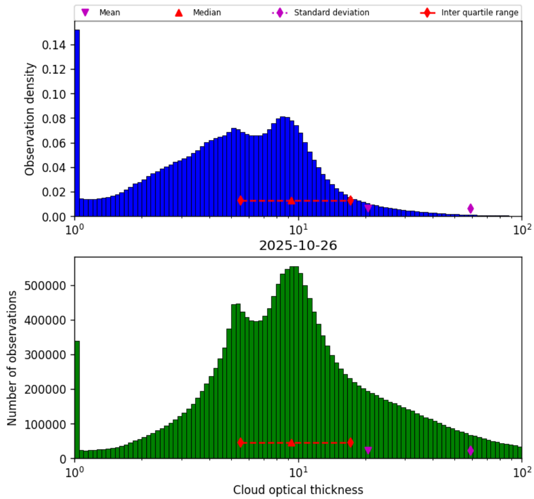
Figure 39: Histogram of “Cloud optical thickness” for 2025-10-26 to 2025-10-27
