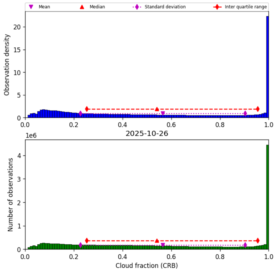
Figure 40: Histogram of “Cloud fraction (CRB)” for 2025-10-26 to 2025-10-27
