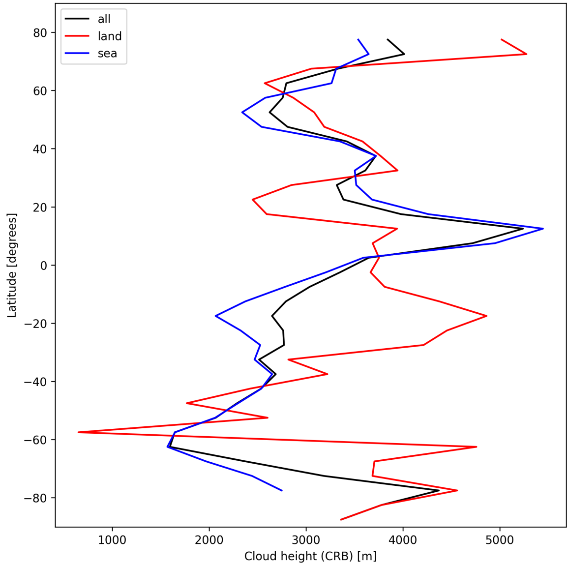
Figure 25: Zonal average of “Cloud height (CRB)” for 2025-10-26 to 2025-10-27.
