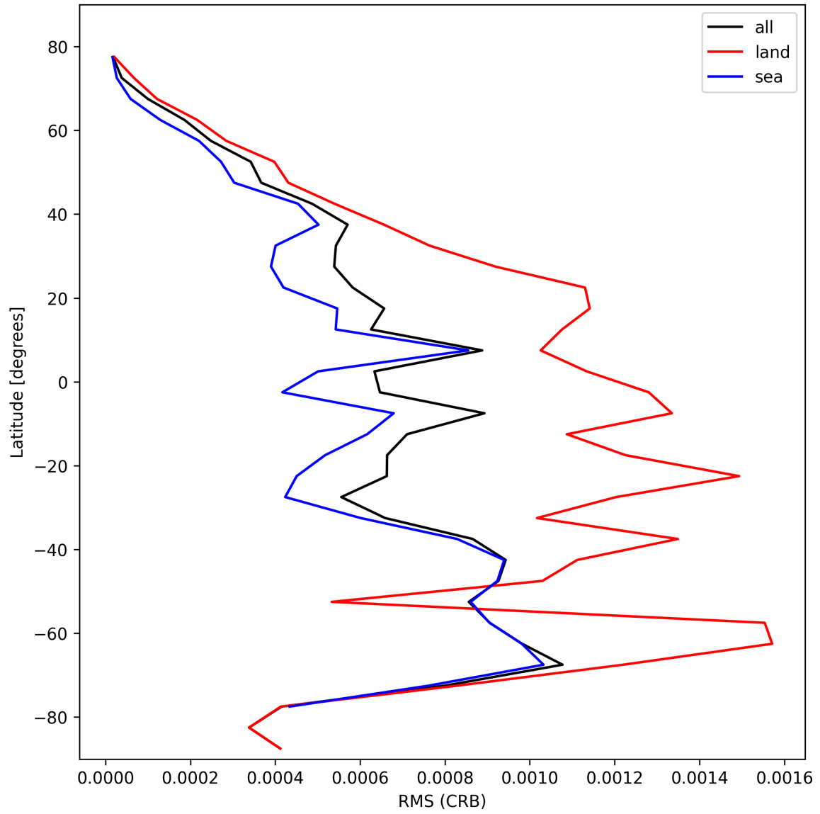
Figure 30: Zonal average of “RMS (CRB)” for 2025-10-26 to 2025-10-27.
