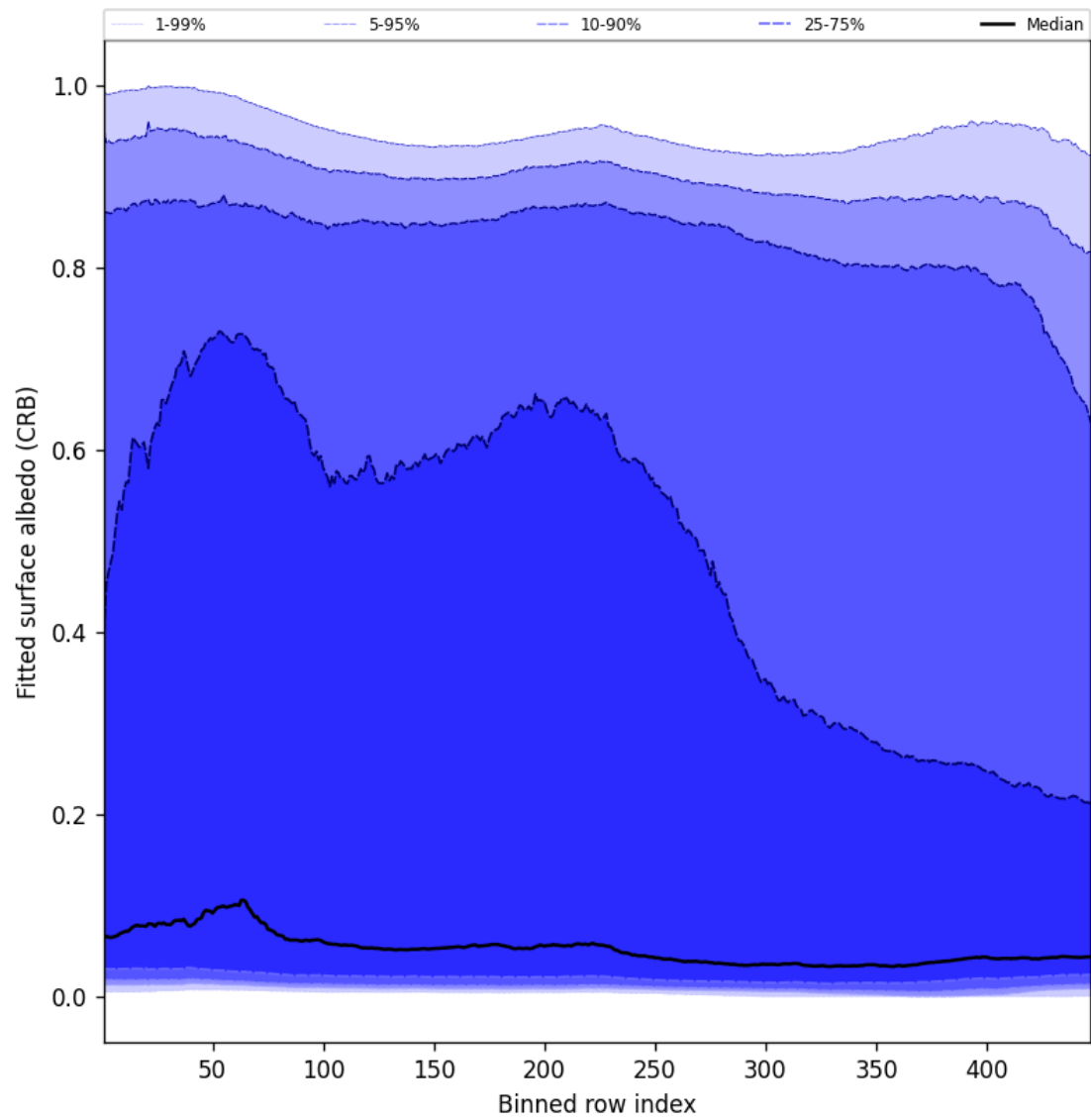
Figure 60: Along track statistics of “Fitted surface albedo (CRB)” for 2025-10-26 to 2025-10-27
