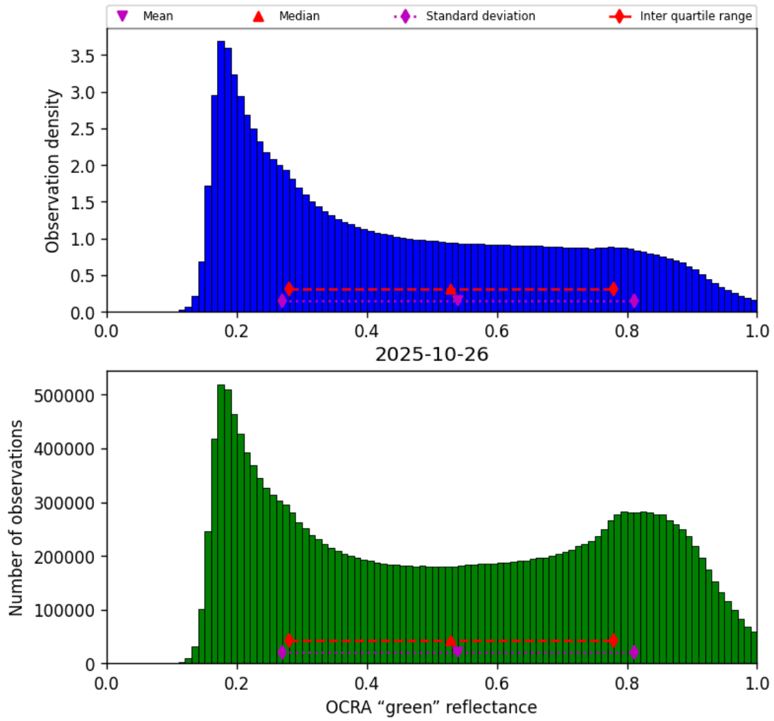
Figure 50: Histogram of “OCRA “green” reflectance” for 2025-10-26 to 2025-10-27
