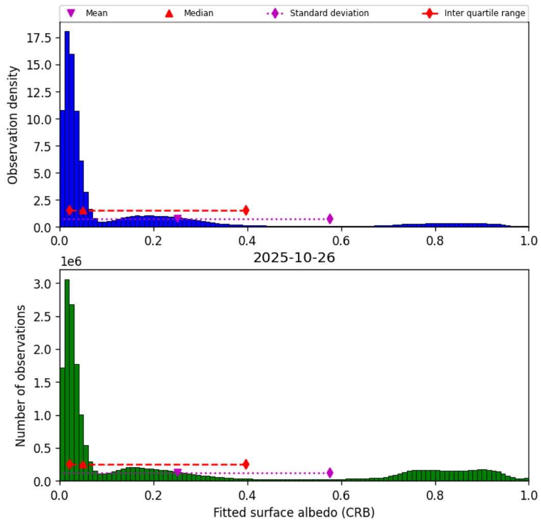
Figure 44: Histogram of “Fitted surface albedo (CRB)” for 2025-10-26 to 2025-10-27
