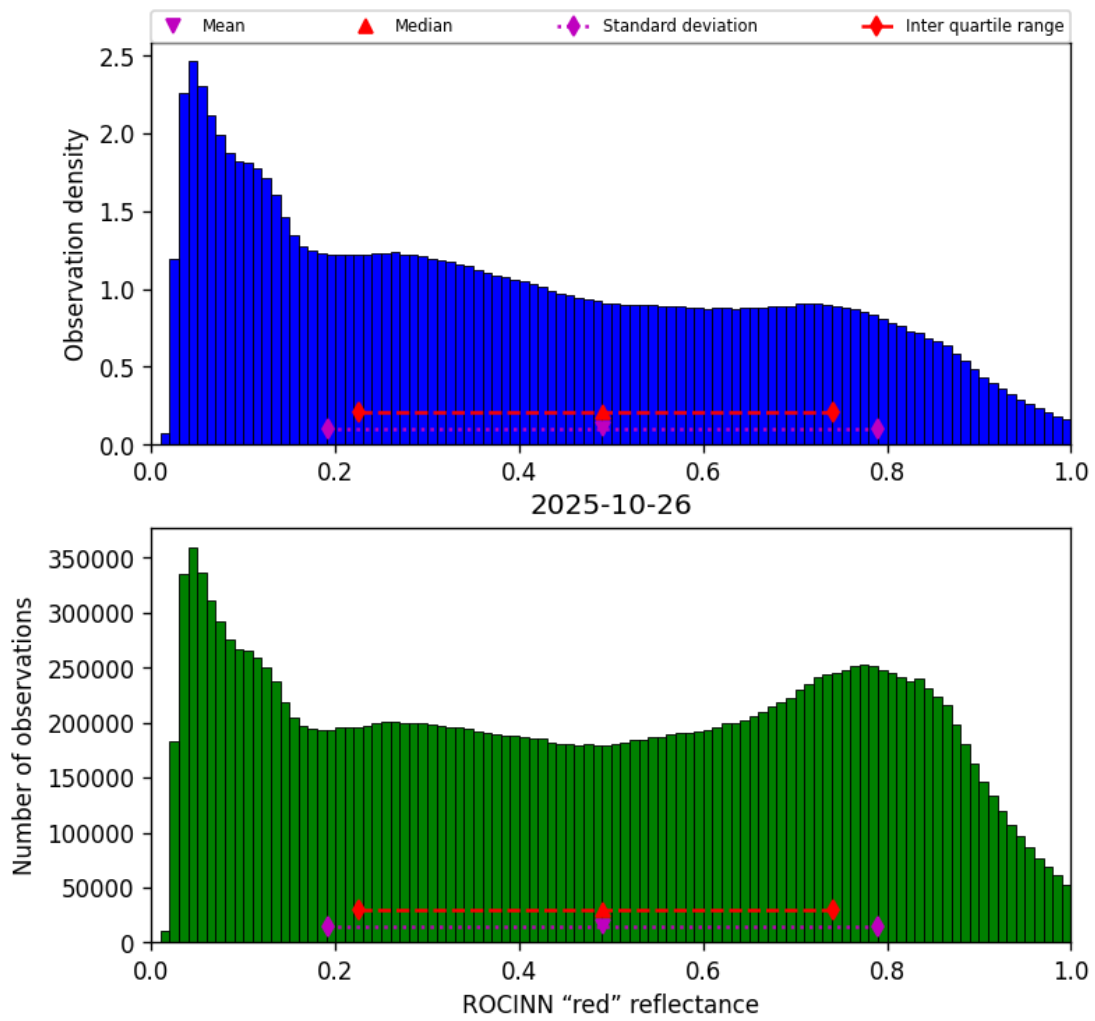
Figure 51: Histogram of “ROCINN “red” reflectance” for 2025-10-26 to 2025-10-27
