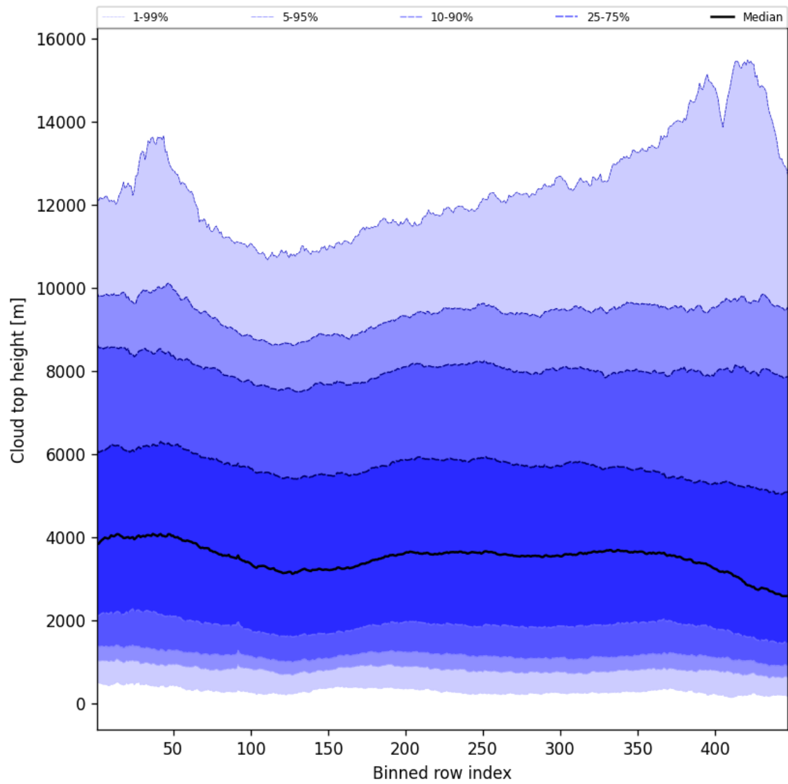
Figure 54: Along track statistics of “Cloud top height” for 2025-10-26 to 2025-10-27
