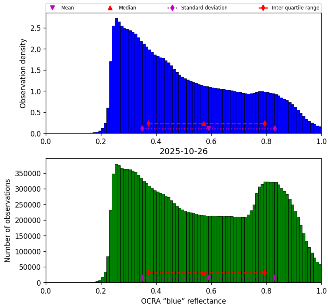
Figure 49: Histogram of “OCRA “blue” reflectance” for 2025-10-26 to 2025-10-27
