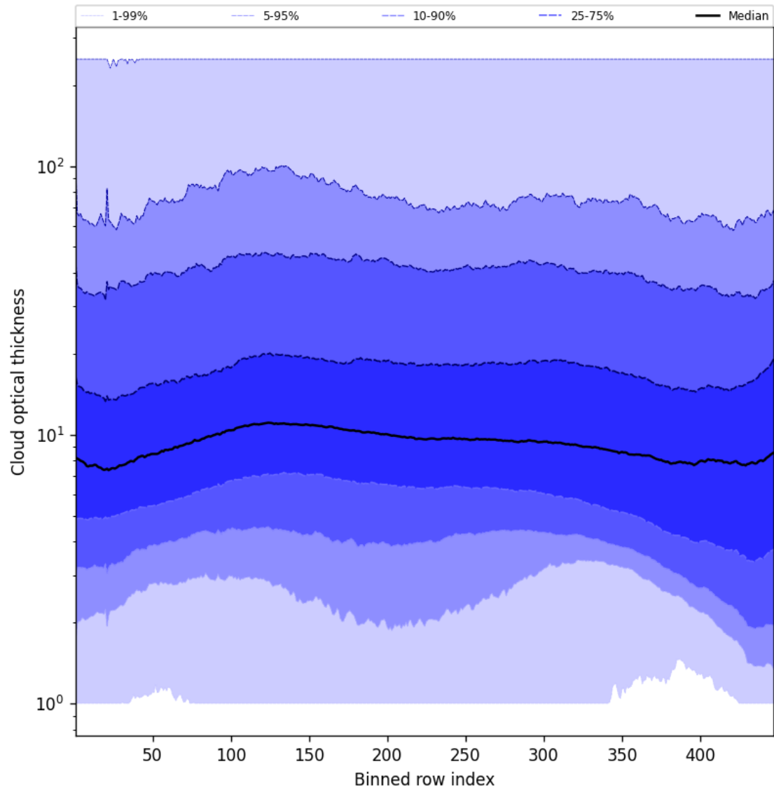
Figure 55: Along track statistics of “Cloud optical thickness” for 2025-10-26 to 2025-10-27
