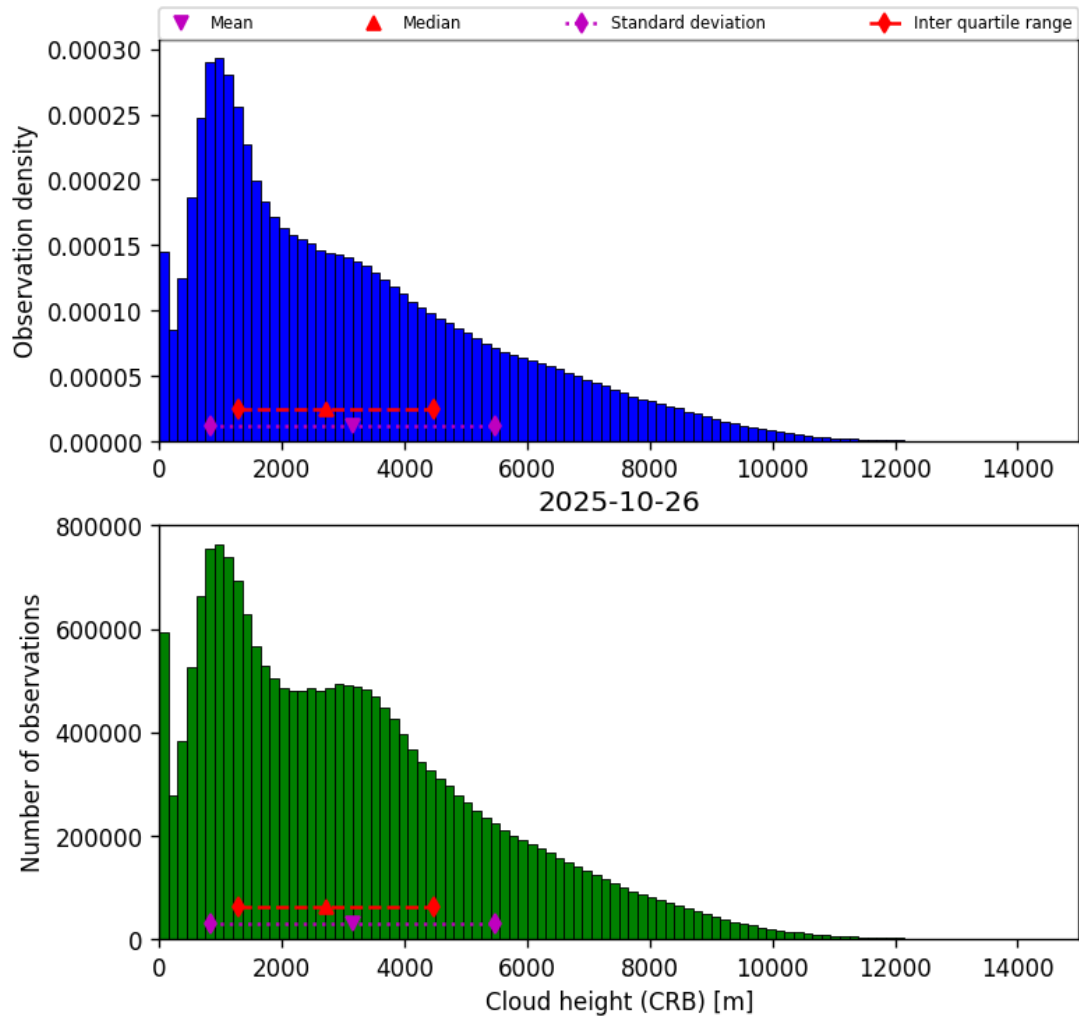
Figure 41: Histogram of “Cloud height (CRB)” for 2025-10-26 to 2025-10-27
