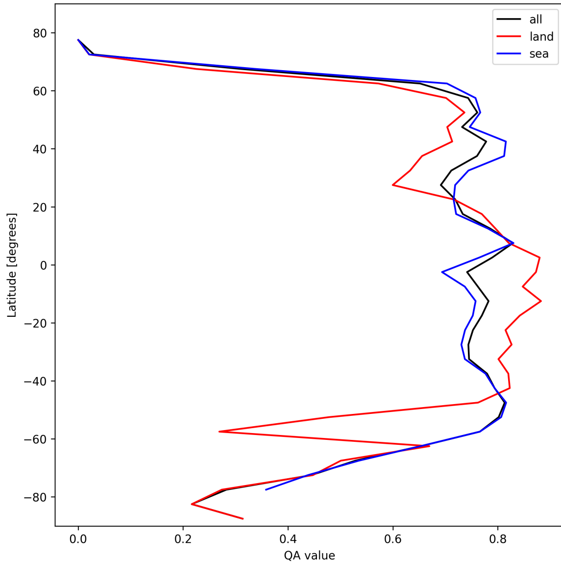
Figure 20: Zonal average of “QA value” for 2025-10-26 to 2025-10-27.
