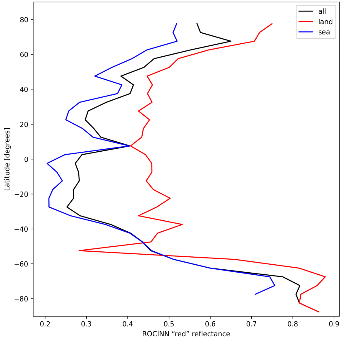
Figure 35: Zonal average of “ROCINN “red” reflectance” for 2025-10-26 to 2025-10-27.
