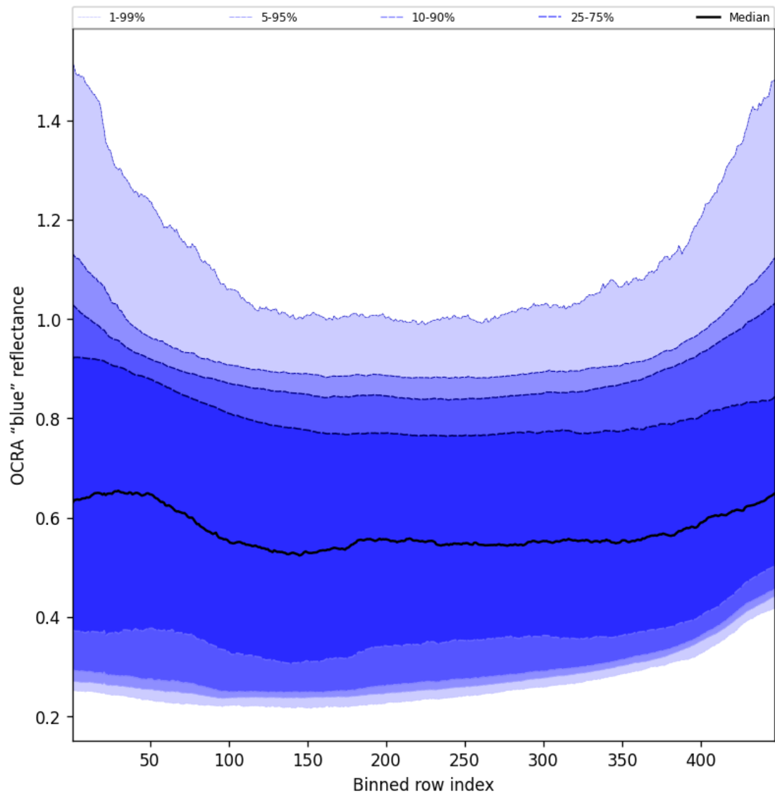
Figure 65: Along track statistics of “OCRA “blue” reflectance” for 2025-10-26 to 2025-10-27
