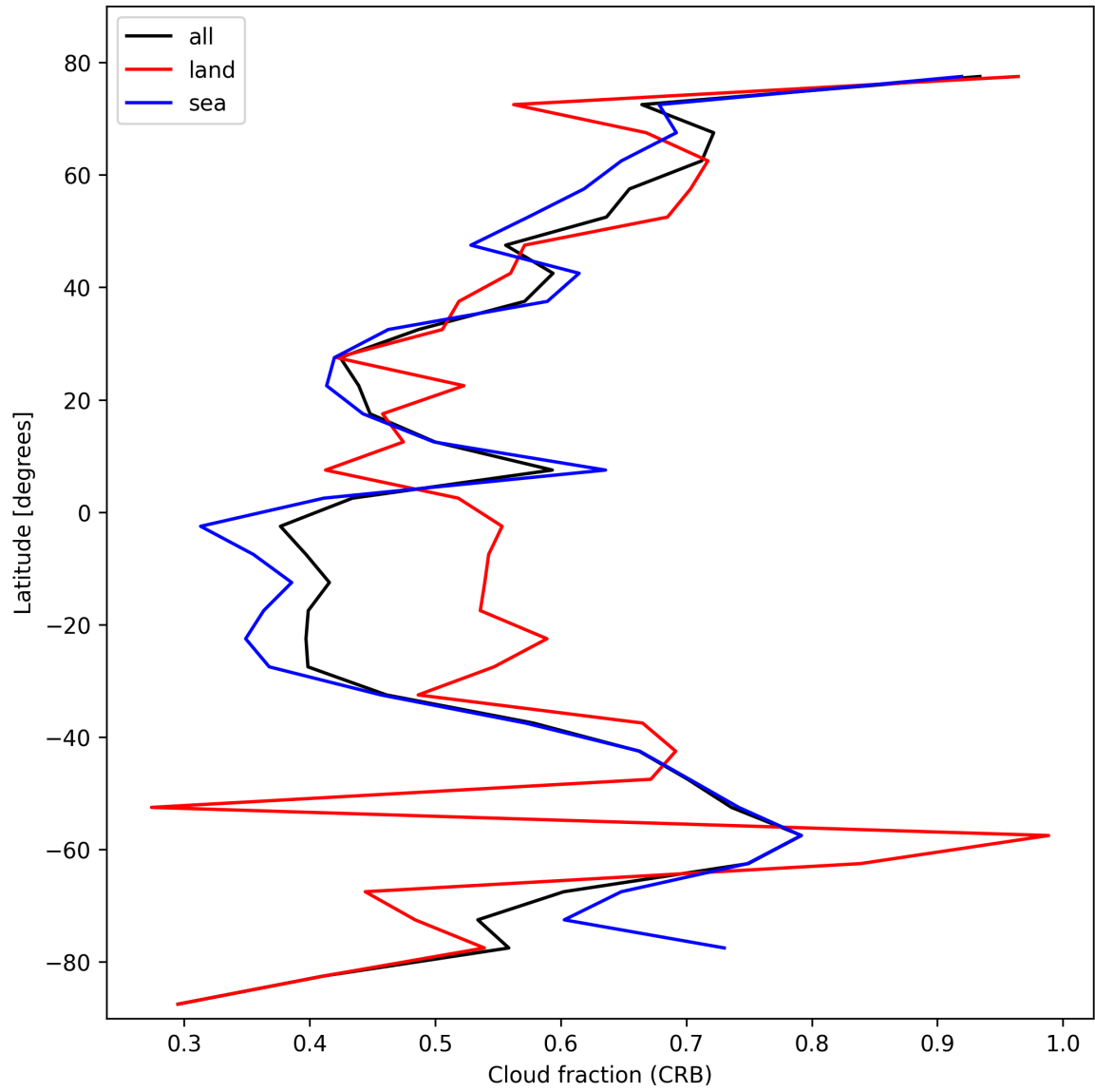
Figure 24: Zonal average of “Cloud fraction (CRB)” for 2025-10-26 to 2025-10-27.
