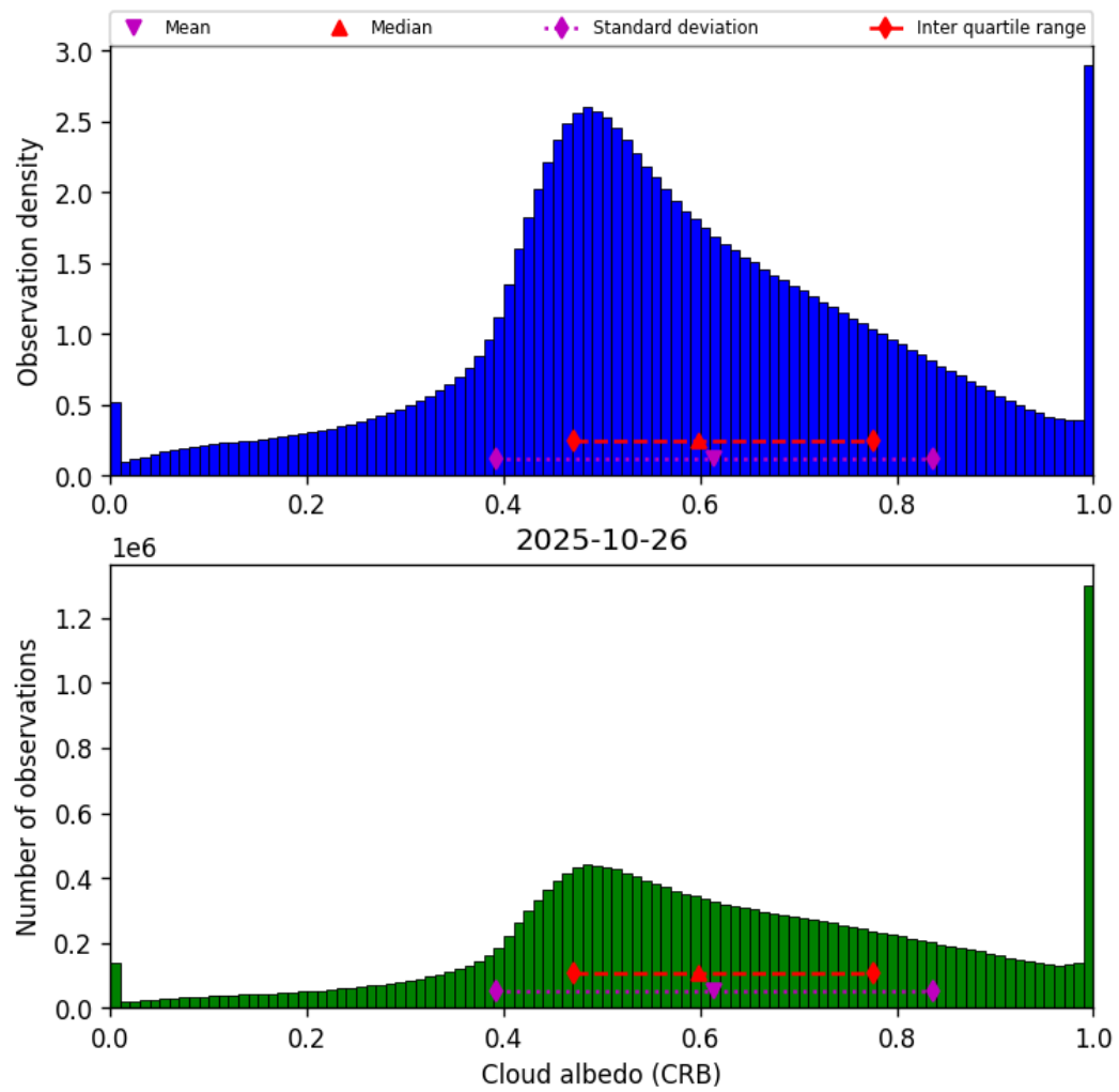
Figure 42: Histogram of “Cloud albedo (CRB)” for 2025-10-26 to 2025-10-27
