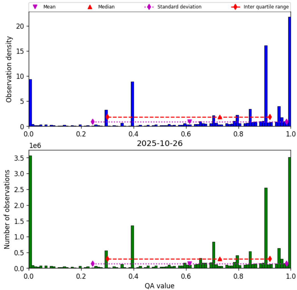
Figure 36: Histogram of “QA value” for 2025-10-26 to 2025-10-27
