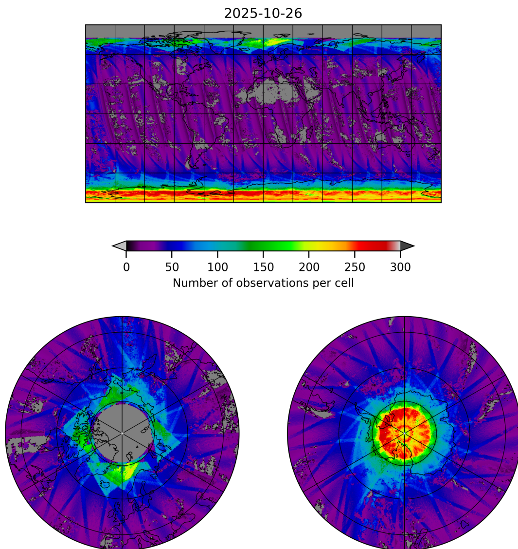
Figure 19: Map of the number of observations for 2025-10-26 to 2025-10-27
