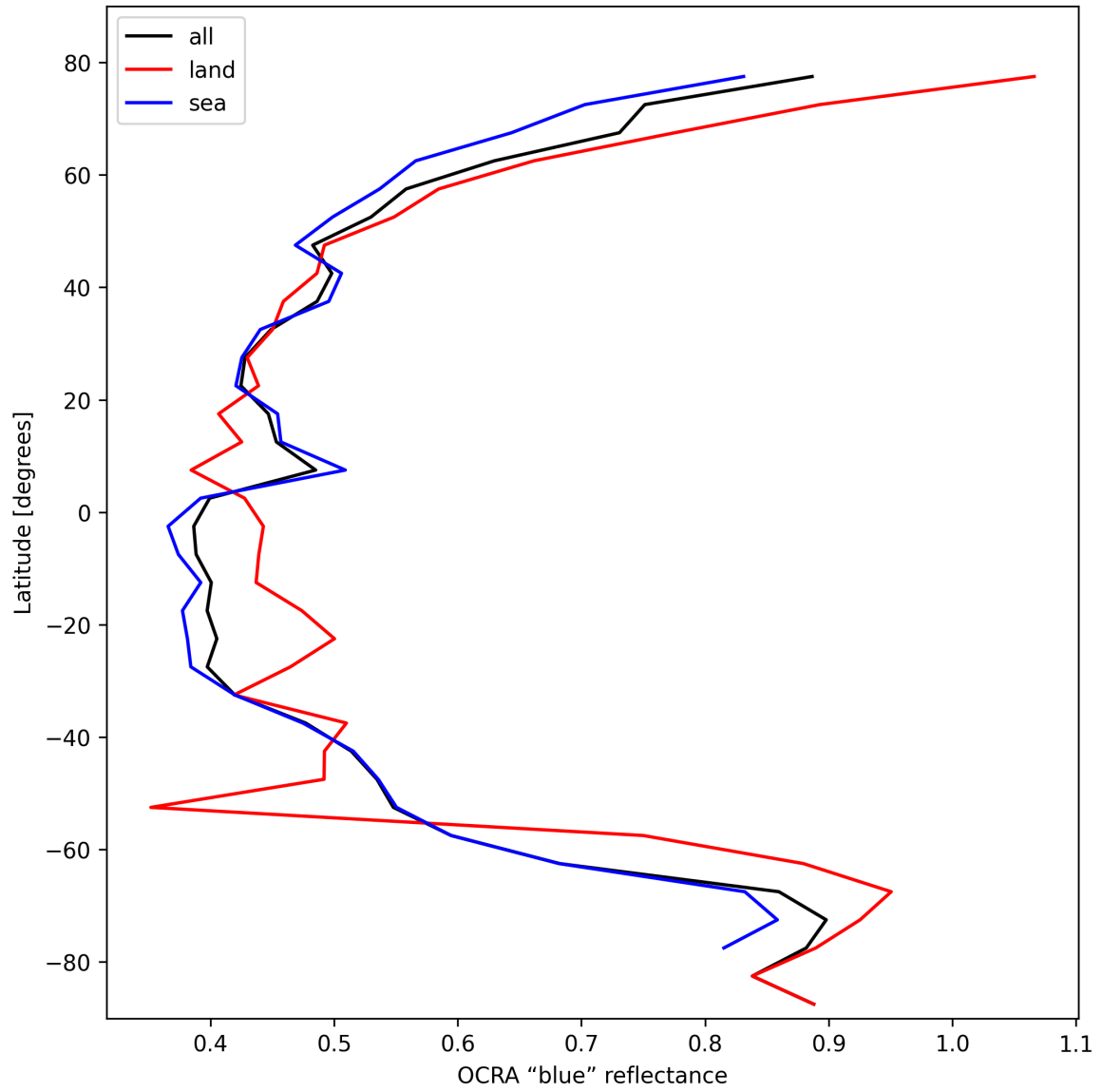
Figure 33: Zonal average of “OCRA “blue” reflectance” for 2025-10-26 to 2025-10-27.
