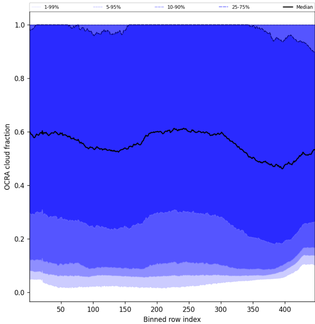
Figure 64: Along track statistics of “OCRA cloud fraction” for 2025-10-26 to 2025-10-27
