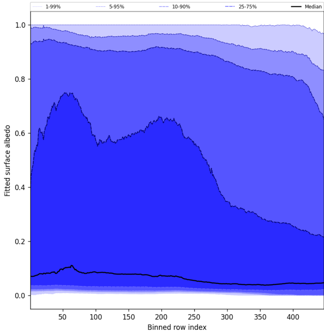
Figure 59: Along track statistics of “Fitted surface albedo” for 2025-10-26 to 2025-10-27
