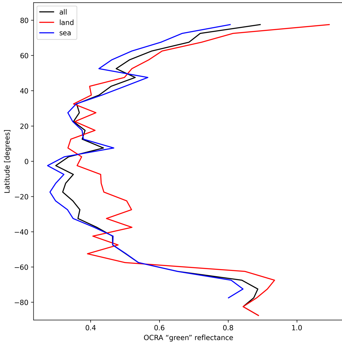
Figure 34: Zonal average of “OCRA “green” reflectance” for 2025-10-27 to 2025-10-28.
