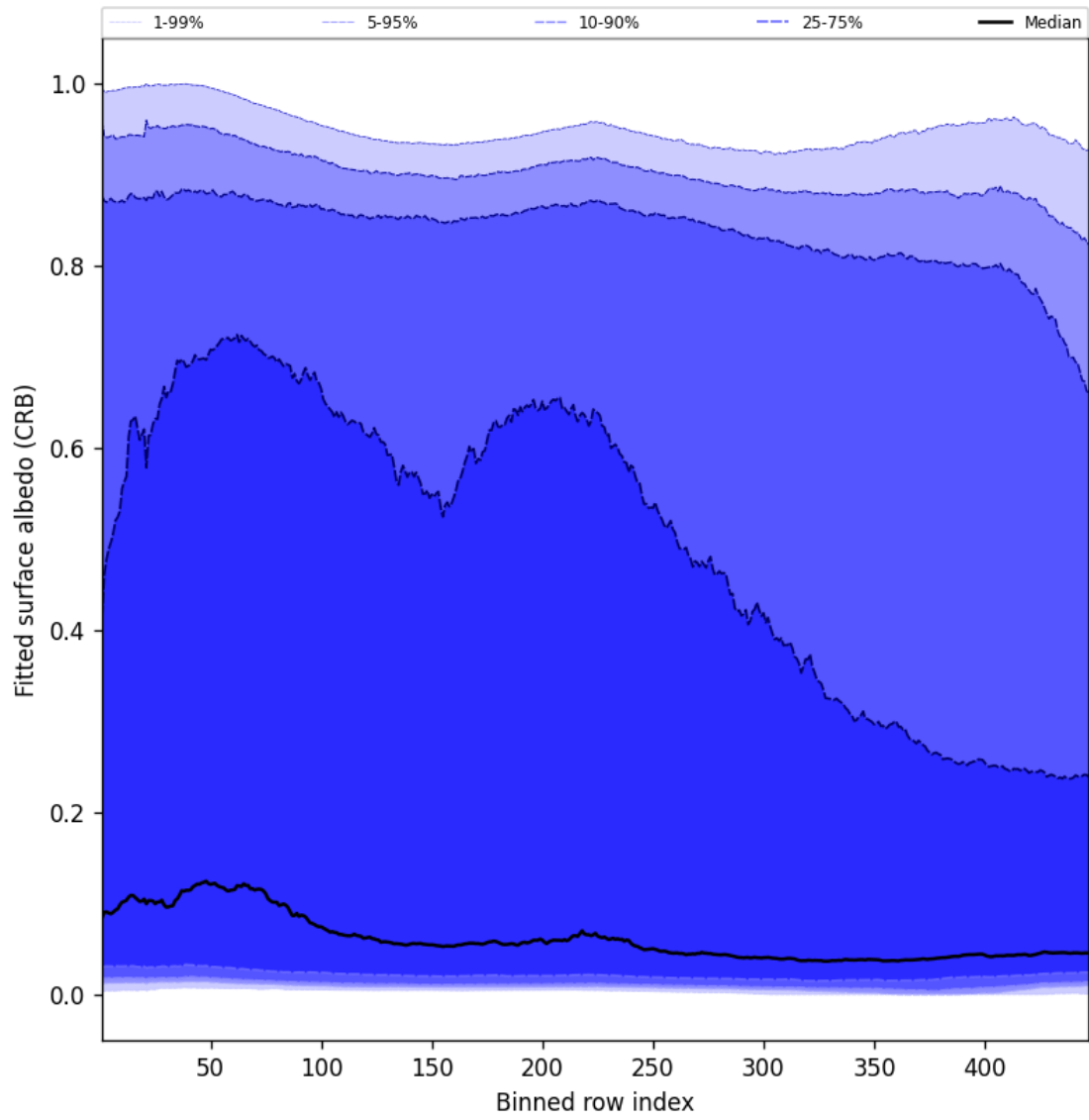
Figure 60: Along track statistics of “Fitted surface albedo (CRB)” for 2025-10-27 to 2025-10-28
