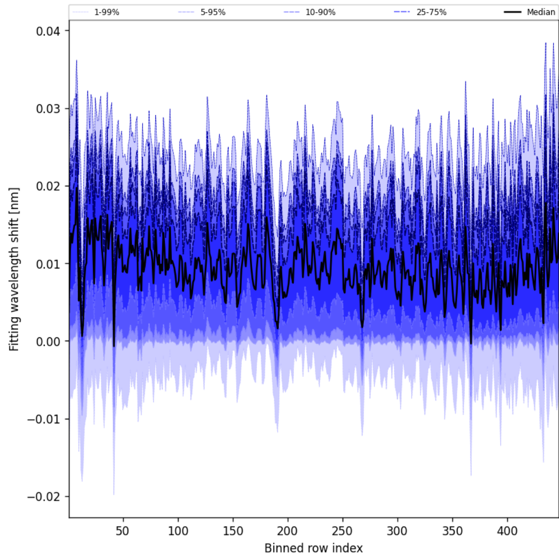
Figure 63: Along track statistics of “Fitting wavelength shift” for 2025-10-27 to 2025-10-28
