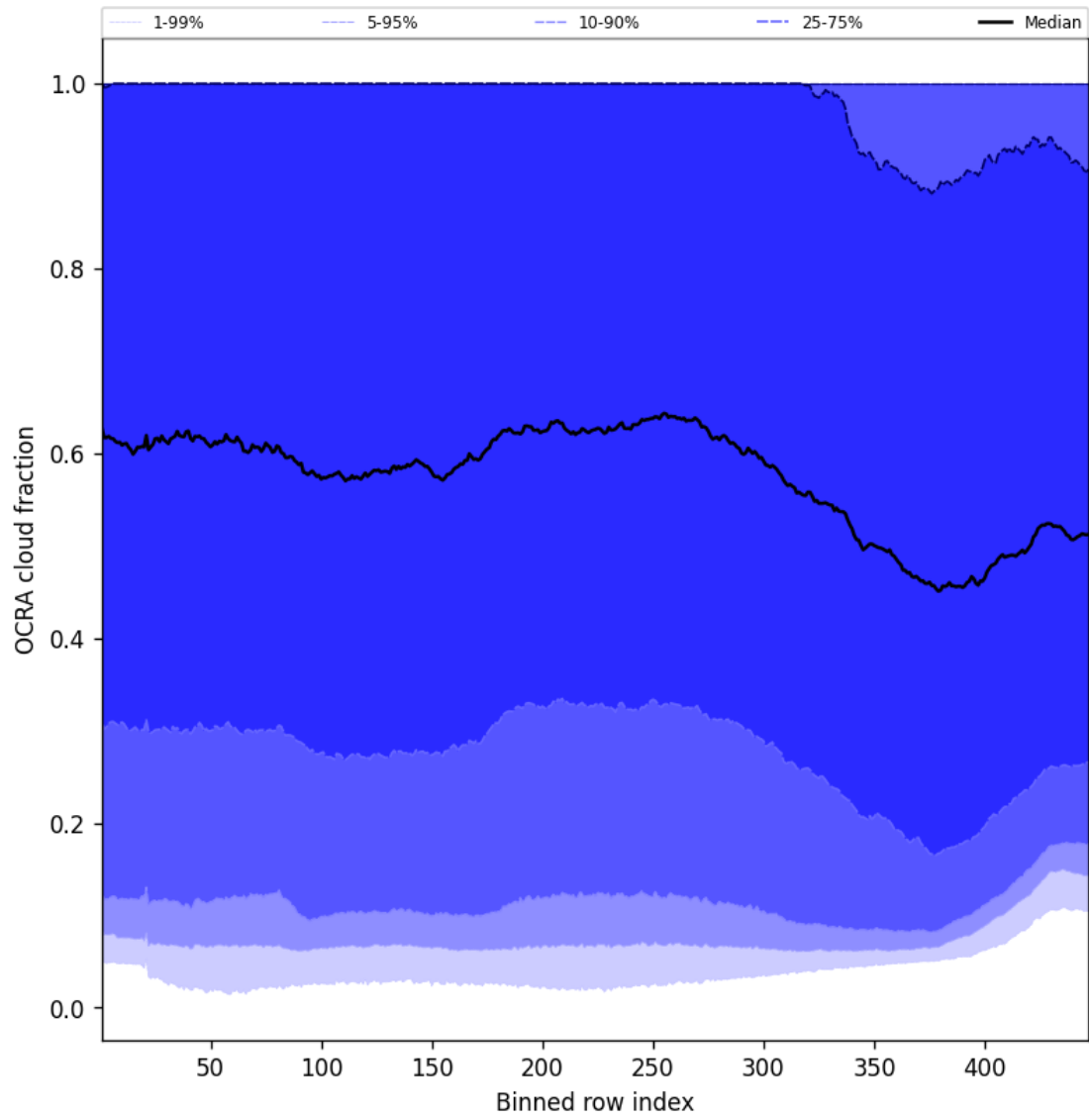
Figure 64: Along track statistics of “OCRA cloud fraction” for 2025-10-27 to 2025-10-28
