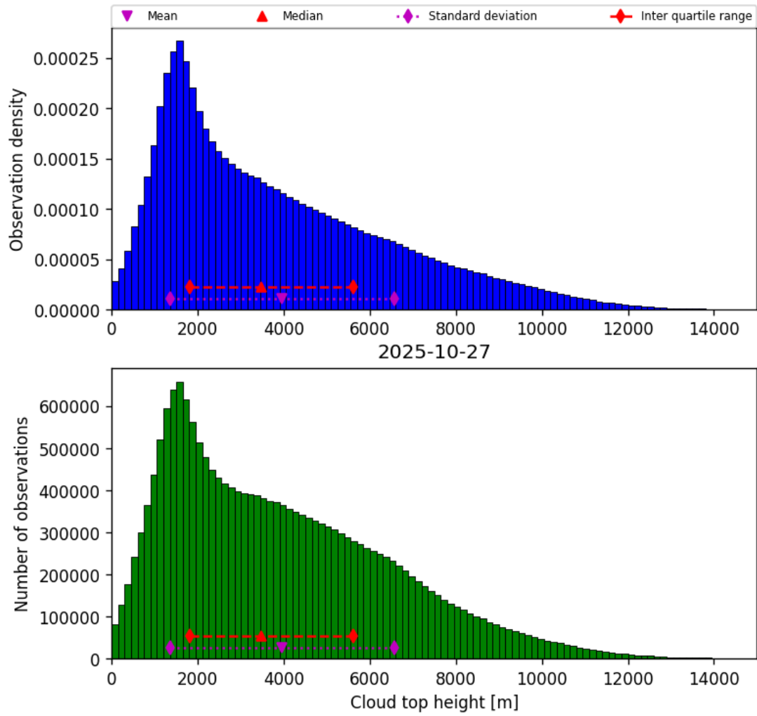
Figure 38: Histogram of “Cloud top height” for 2025-10-27 to 2025-10-28
