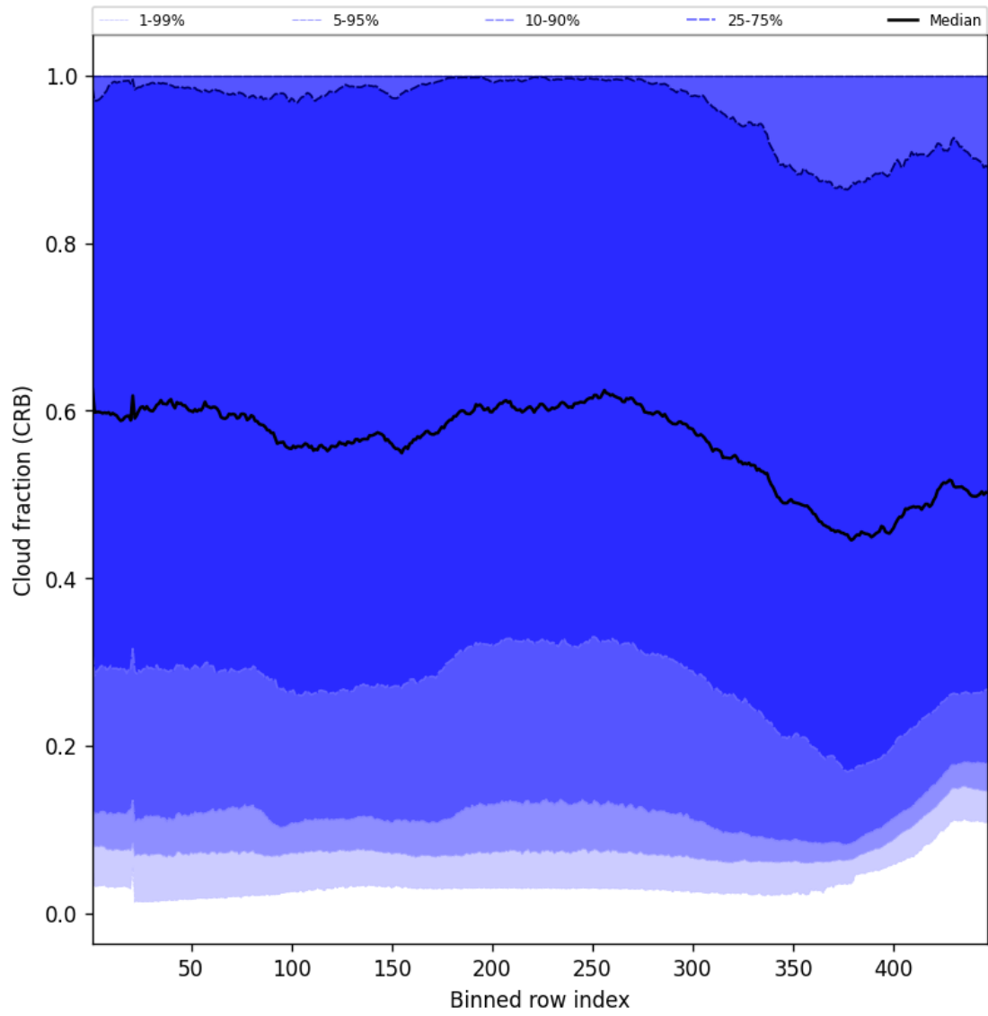
Figure 56: Along track statistics of “Cloud fraction (CRB)” for 2025-10-27 to 2025-10-28
