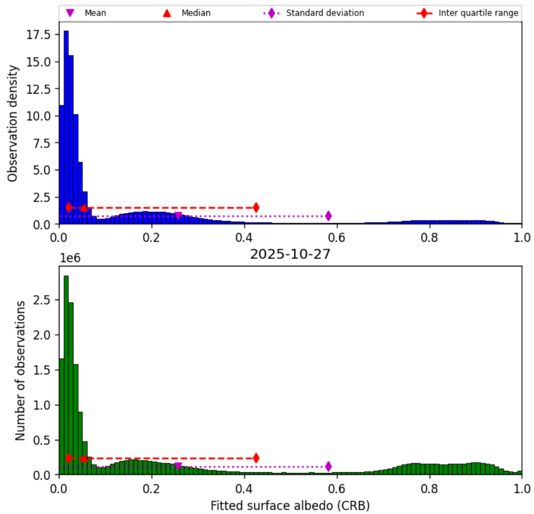
Figure 44: Histogram of “Fitted surface albedo (CRB)” for 2025-10-27 to 2025-10-28
