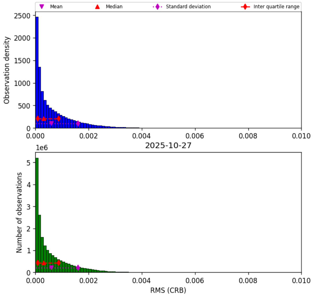
Figure 46: Histogram of “RMS (CRB)” for 2025-10-27 to 2025-10-28
