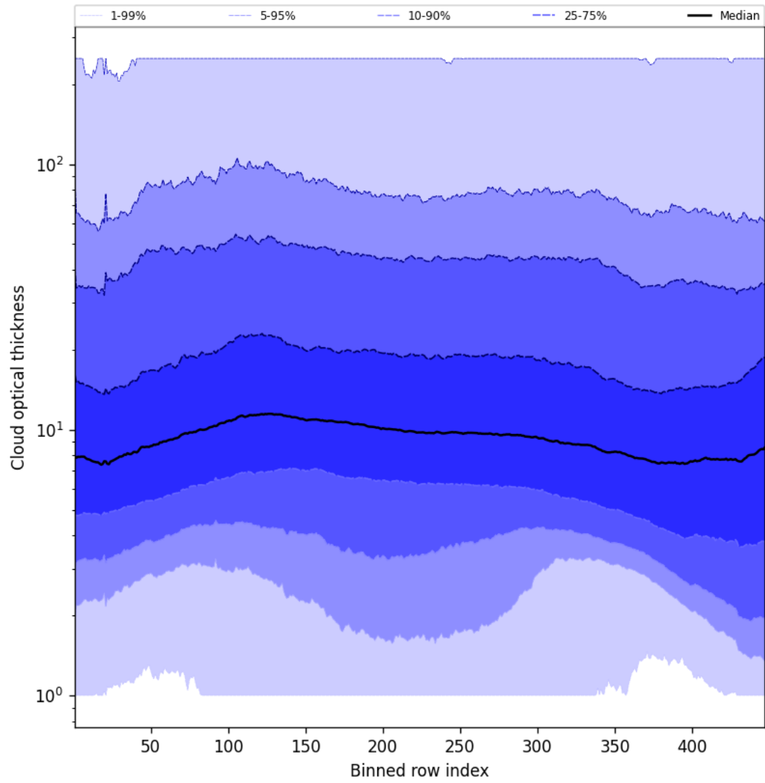
Figure 55: Along track statistics of “Cloud optical thickness” for 2025-10-27 to 2025-10-28
