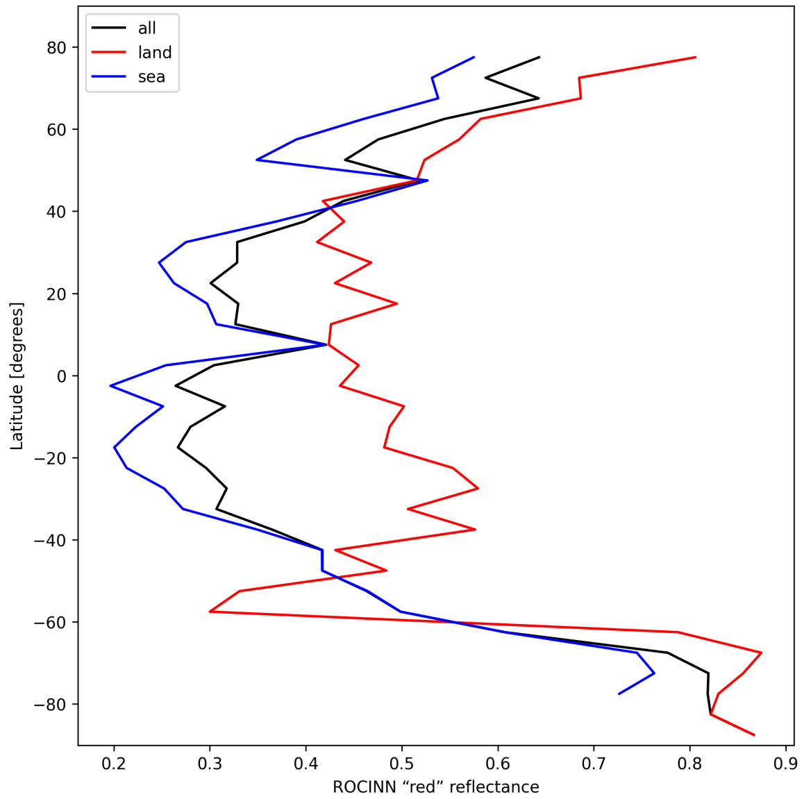
Figure 35: Zonal average of “ROCINN “red” reflectance” for 2025-10-27 to 2025-10-28.
