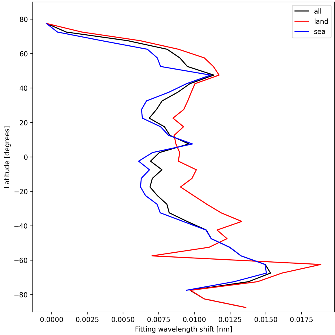
Figure 31: Zonal average of “Fitting wavelength shift” for 2025-10-27 to 2025-10-28.
