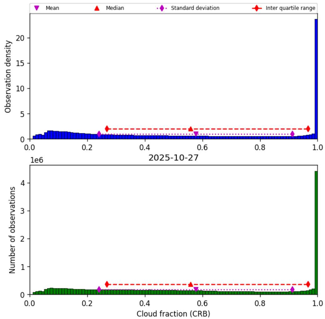
Figure 40: Histogram of “Cloud fraction (CRB)” for 2025-10-27 to 2025-10-28
