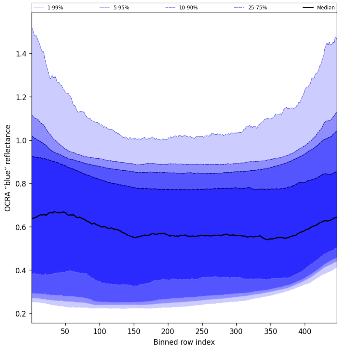
Figure 65: Along track statistics of “OCRA “blue” reflectance” for 2025-10-27 to 2025-10-28
