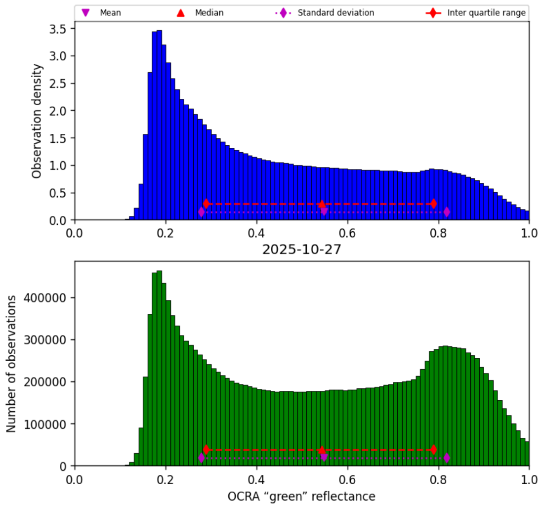
Figure 50: Histogram of “OCRA “green” reflectance” for 2025-10-27 to 2025-10-28
