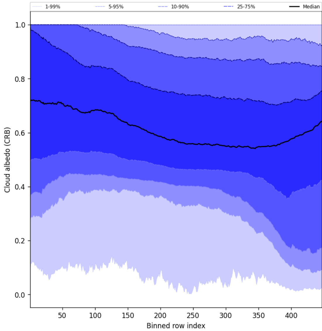
Figure 58: Along track statistics of “Cloud albedo (CRB)” for 2025-10-27 to 2025-10-28
