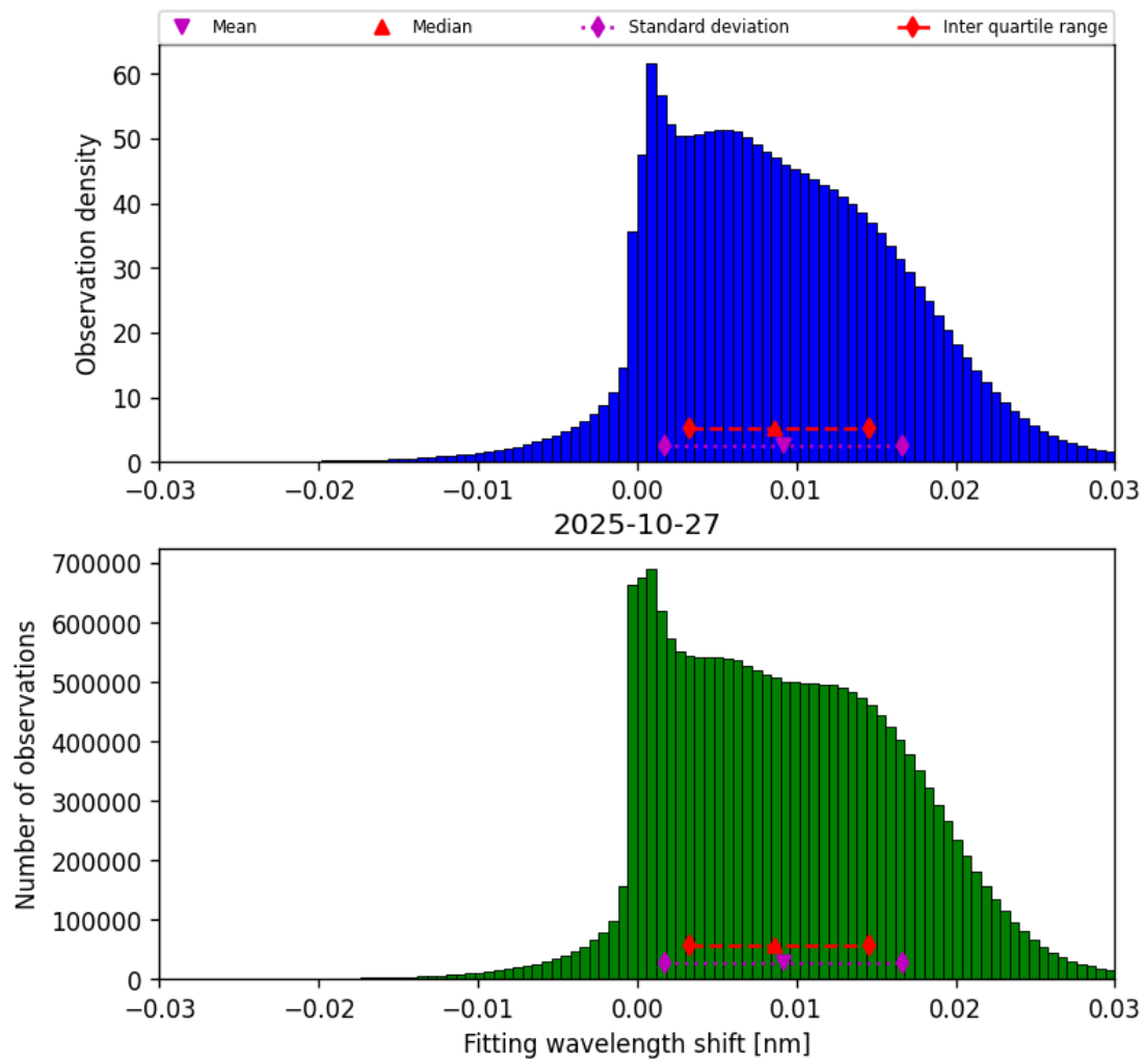
Figure 47: Histogram of “Fitting wavelength shift” for 2025-10-27 to 2025-10-28
