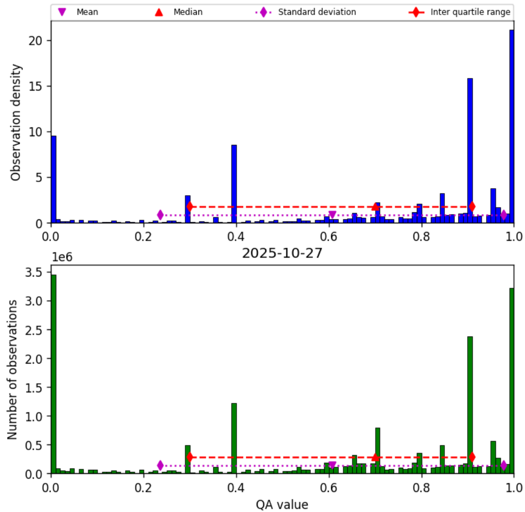
Figure 36: Histogram of “QA value” for 2025-10-27 to 2025-10-28
