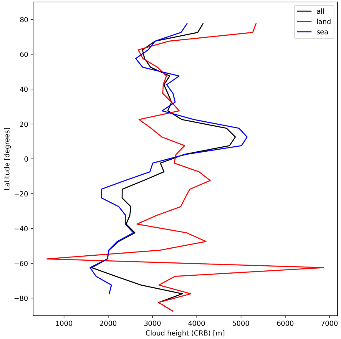
Figure 25: Zonal average of “Cloud height (CRB)” for 2025-10-27 to 2025-10-28.
