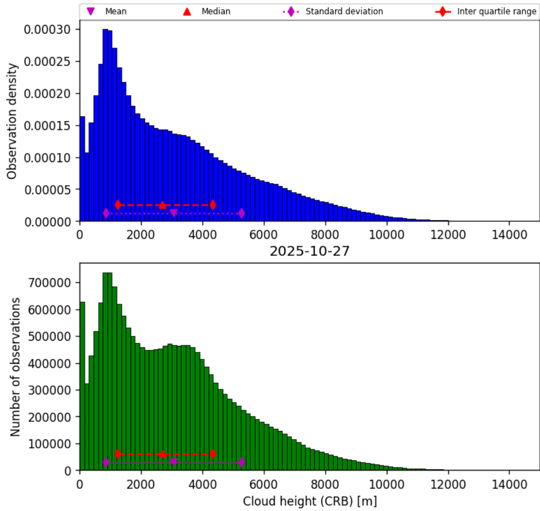
Figure 41: Histogram of “Cloud height (CRB)” for 2025-10-27 to 2025-10-28
