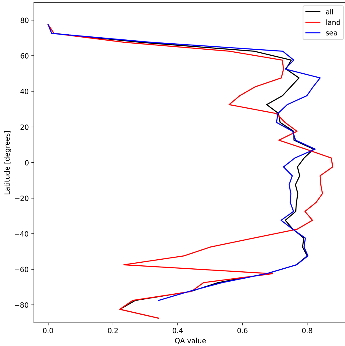
Figure 20: Zonal average of “QA value” for 2025-10-27 to 2025-10-28.
