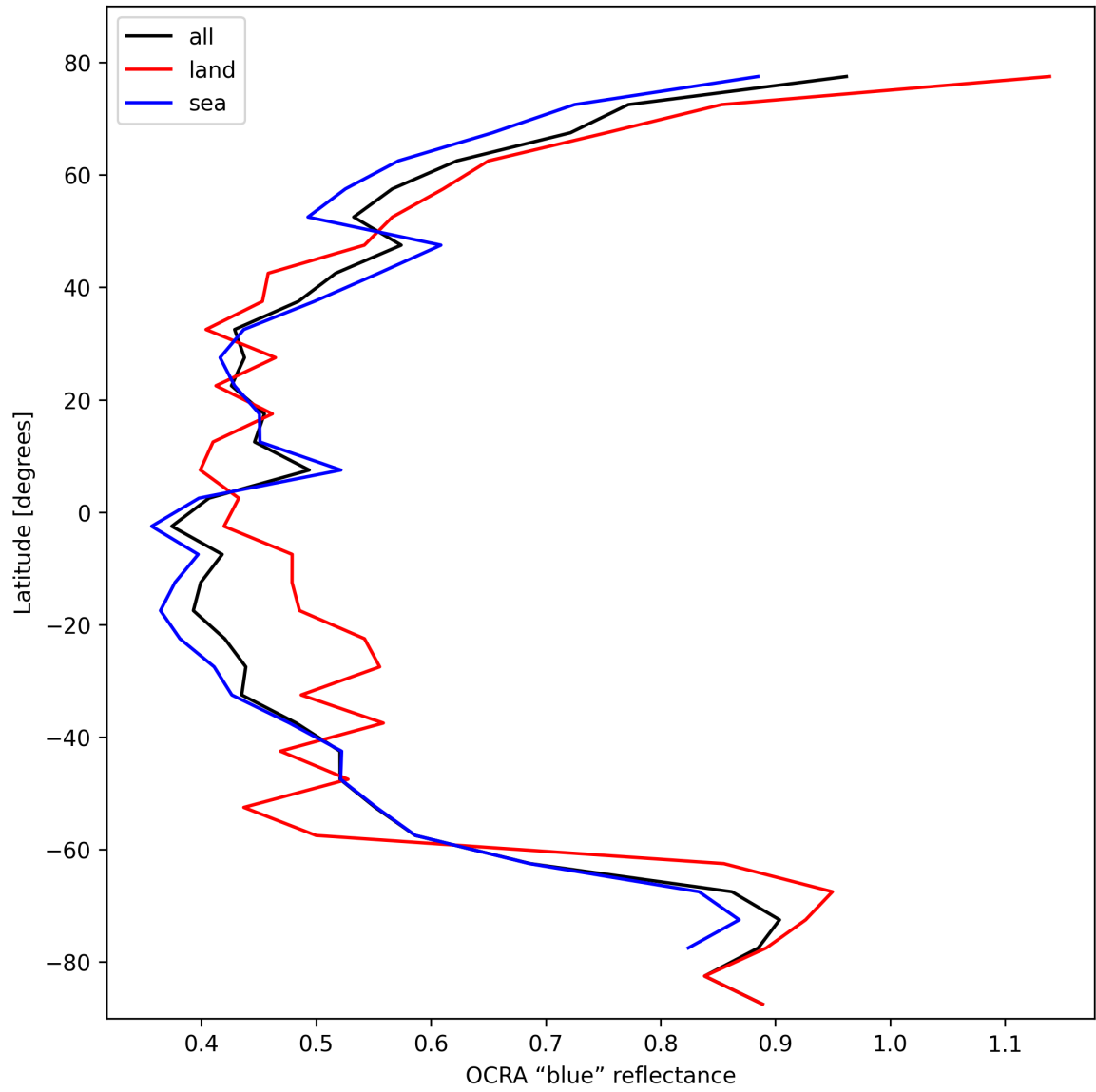
Figure 33: Zonal average of “OCRA “blue” reflectance” for 2025-10-27 to 2025-10-28.
