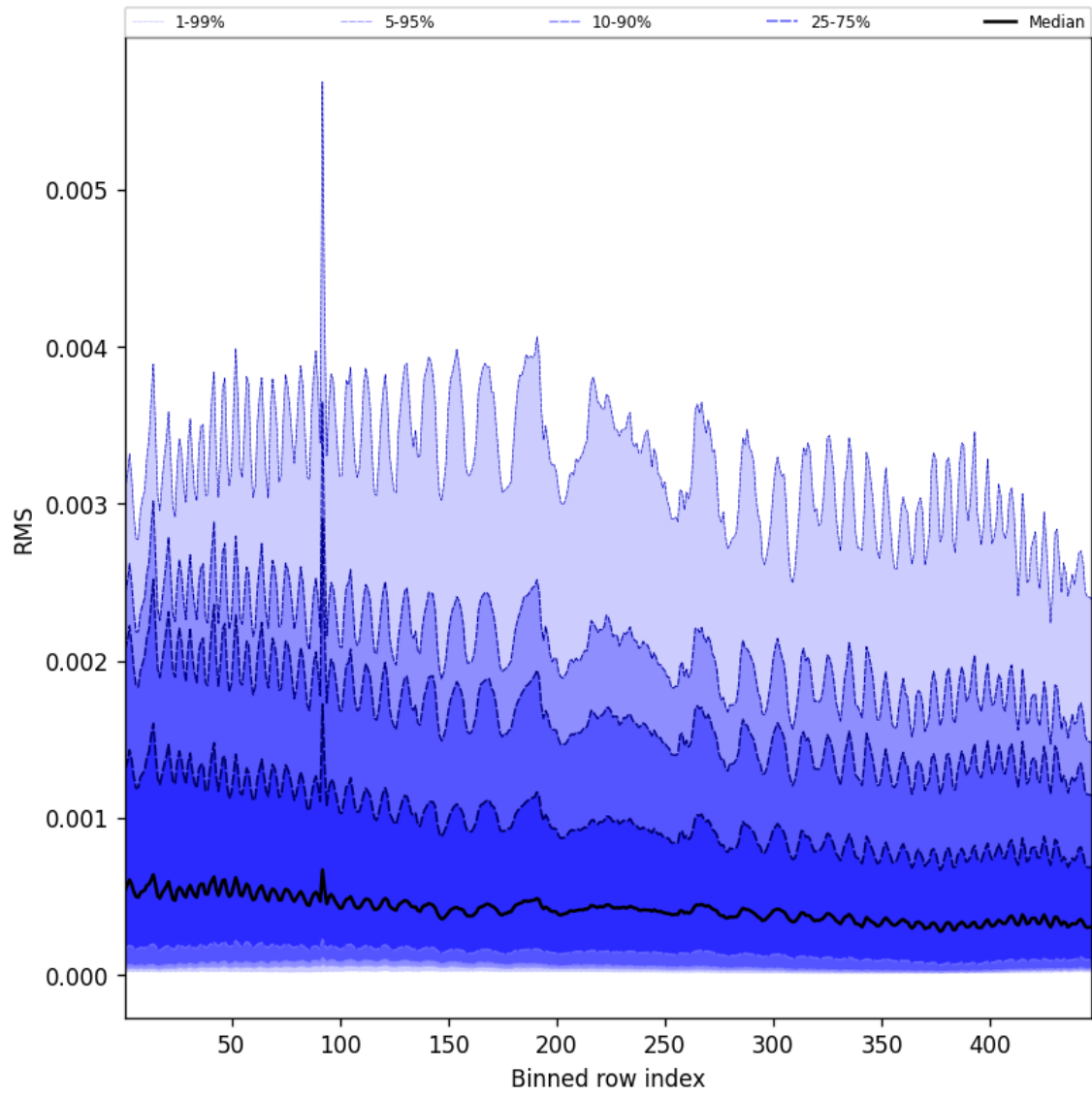
Figure 61: Along track statistics of “RMS” for 2025-10-27 to 2025-10-28
