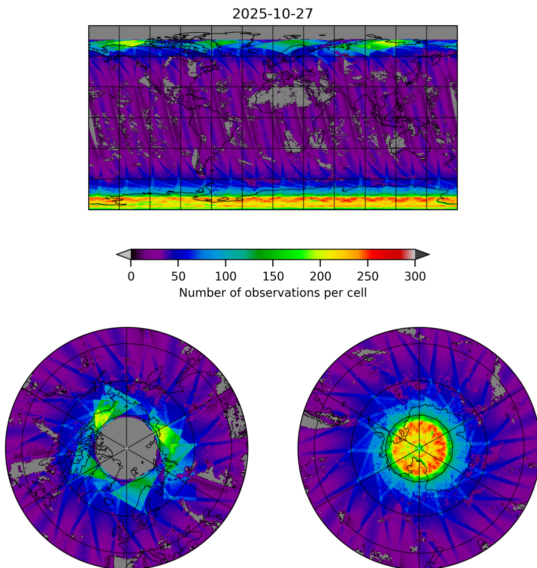
Figure 19: Map of the number of observations for 2025-10-27 to 2025-10-28
