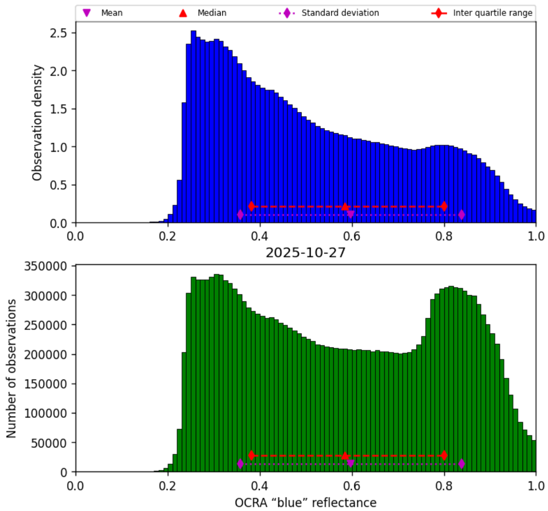
Figure 49: Histogram of “OCRA “blue” reflectance” for 2025-10-27 to 2025-10-28
