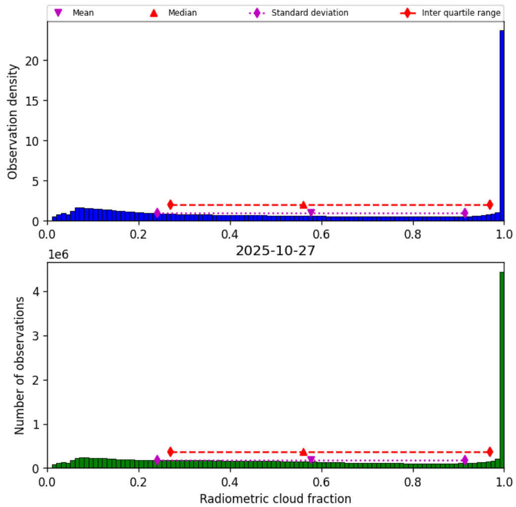
Figure 37: Histogram of “Radiometric cloud fraction” for 2025-10-27 to 2025-10-28
