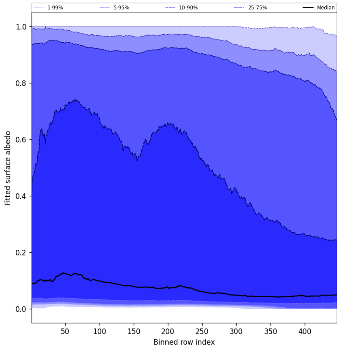
Figure 59: Along track statistics of “Fitted surface albedo” for 2025-10-27 to 2025-10-28
