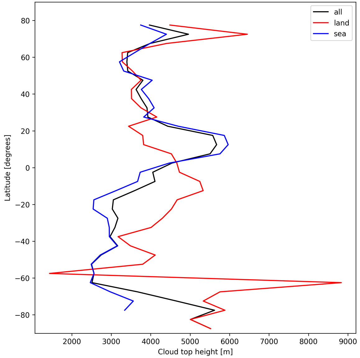
Figure 22: Zonal average of “Cloud top height” for 2025-10-27 to 2025-10-28.
