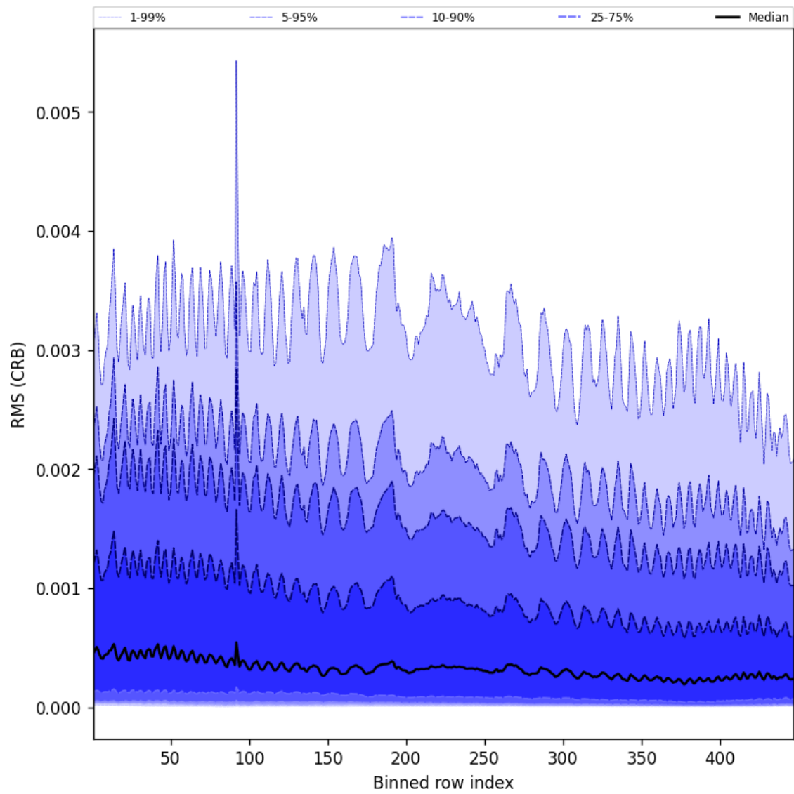
Figure 62: Along track statistics of “RMS (CRB)” for 2025-10-27 to 2025-10-28
