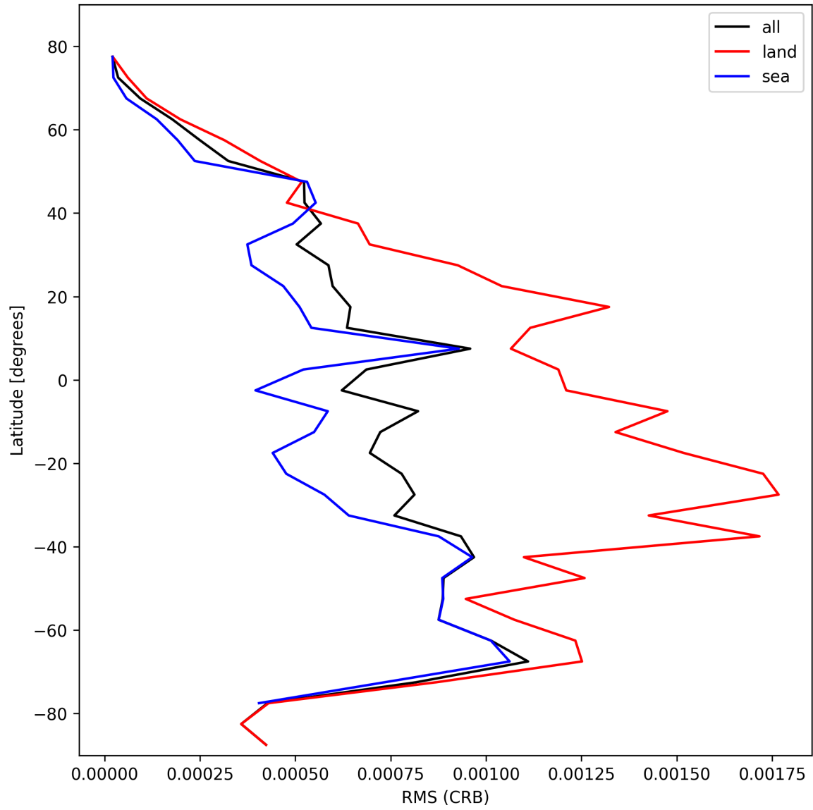
Figure 30: Zonal average of “RMS (CRB)” for 2025-10-27 to 2025-10-28.
