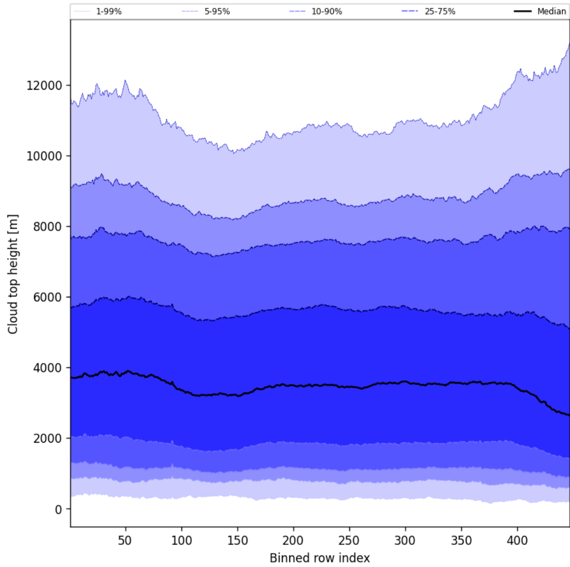
Figure 54: Along track statistics of “Cloud top height” for 2025-10-27 to 2025-10-28
