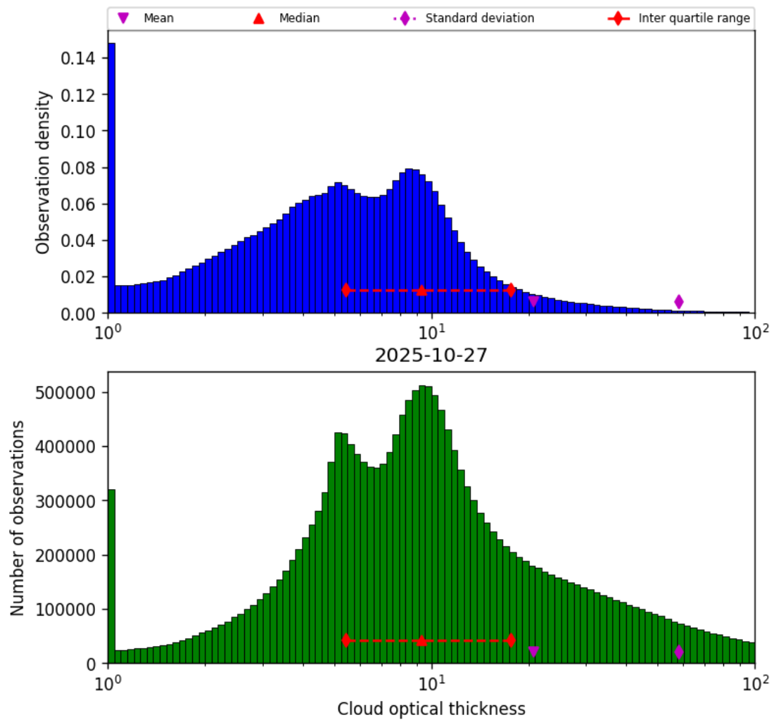
Figure 39: Histogram of “Cloud optical thickness” for 2025-10-27 to 2025-10-28
