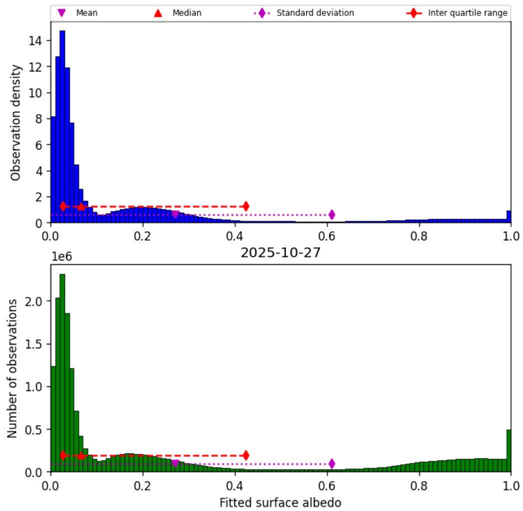
Figure 43: Histogram of “Fitted surface albedo” for 2025-10-27 to 2025-10-28
