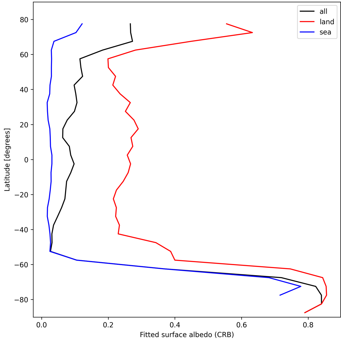
Figure 28: Zonal average of “Fitted surface albedo (CRB)” for 2025-10-27 to 2025-10-28.
