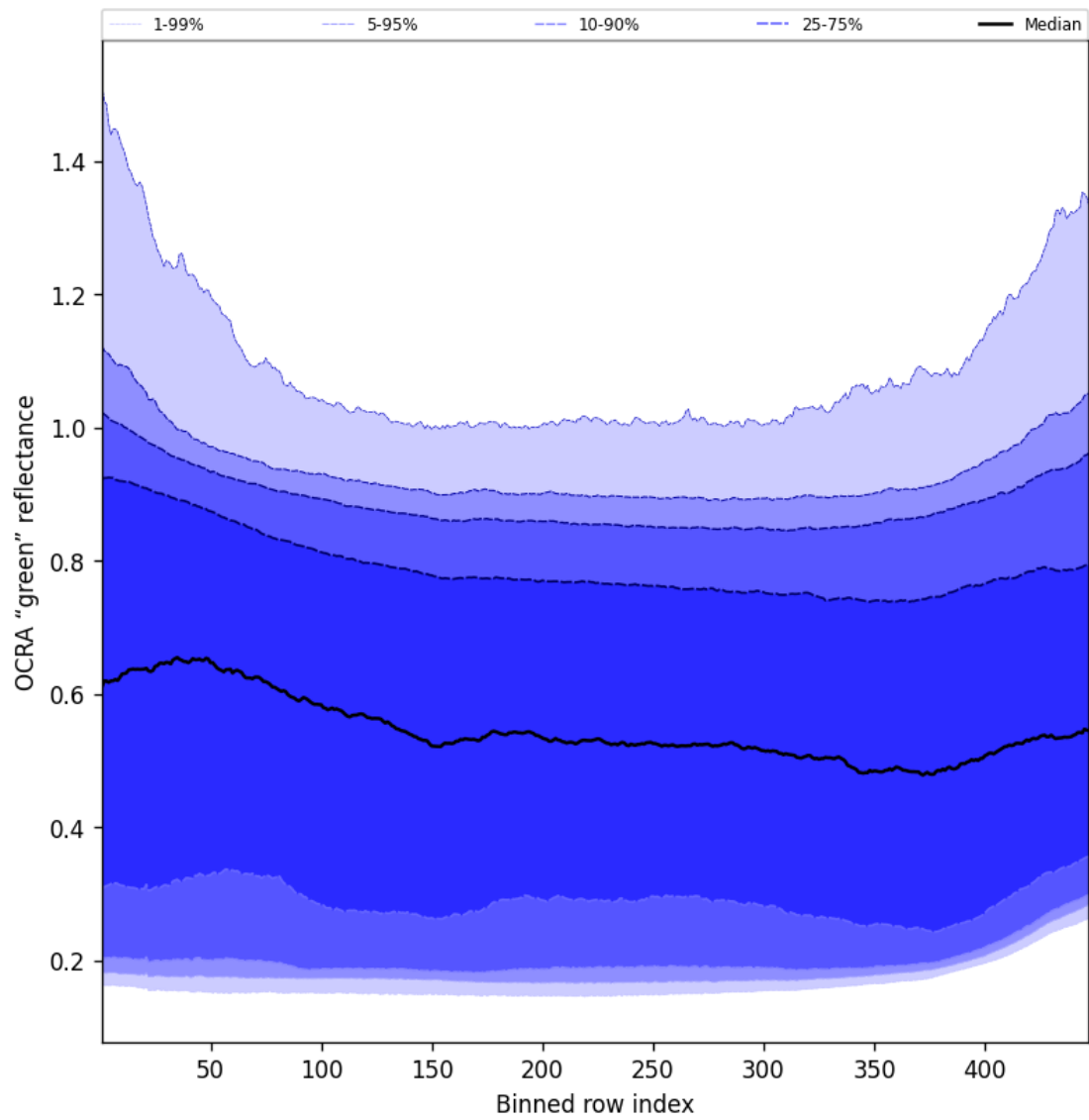
Figure 66: Along track statistics of “OCRA “green” reflectance” for 2025-10-27 to 2025-10-28
