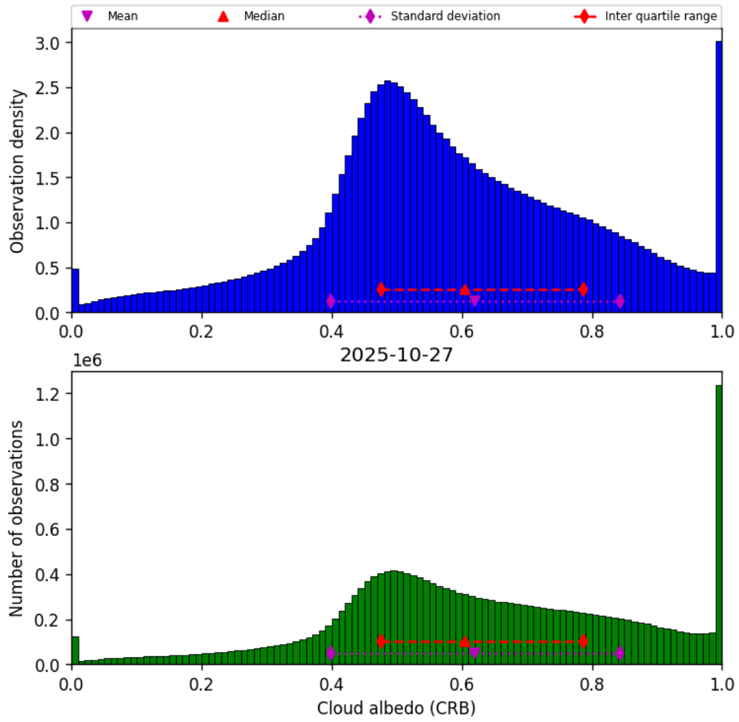
Figure 42: Histogram of “Cloud albedo (CRB)” for 2025-10-27 to 2025-10-28
