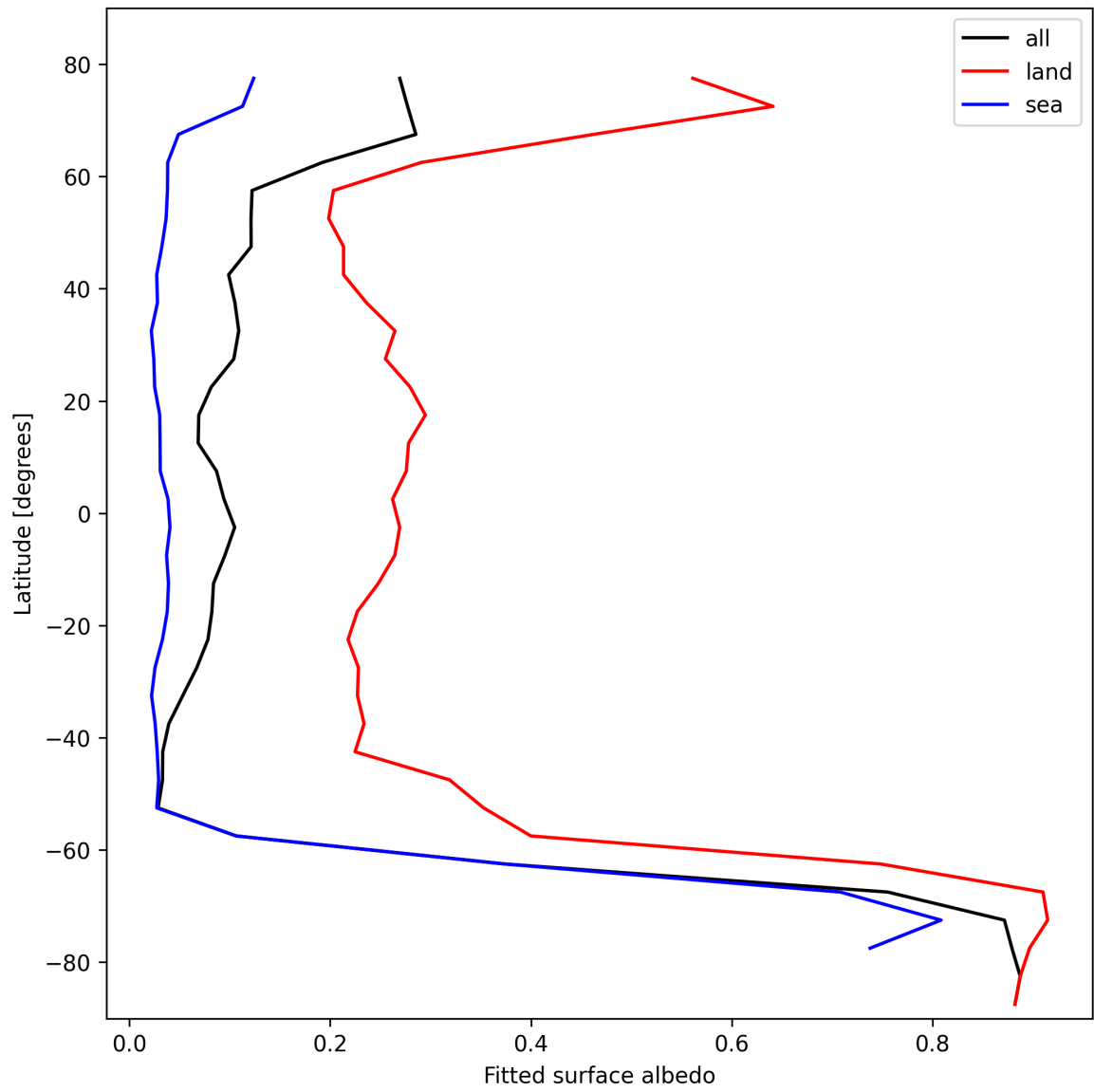
Figure 27: Zonal average of “Fitted surface albedo” for 2025-10-27 to 2025-10-28.
