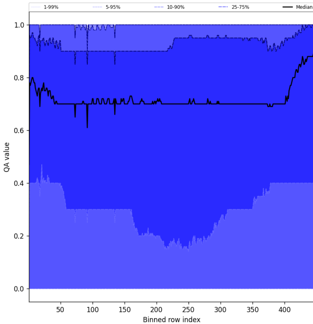
Figure 52: Along track statistics of “QA value” for 2025-10-27 to 2025-10-28
