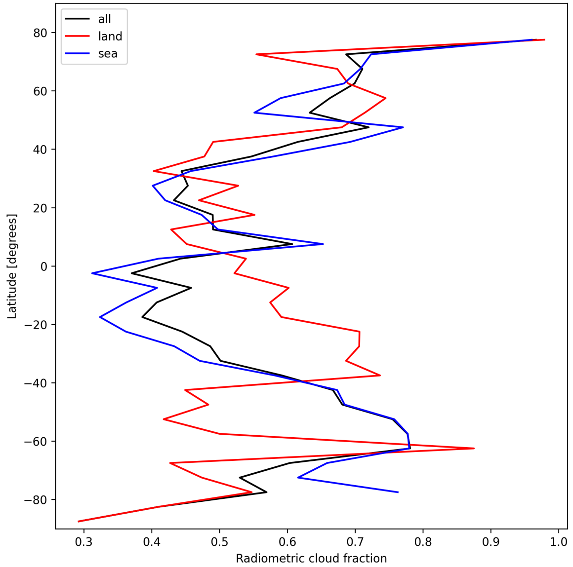
Figure 21: Zonal average of “Radiometric cloud fraction” for 2025-10-27 to 2025-10-28.
