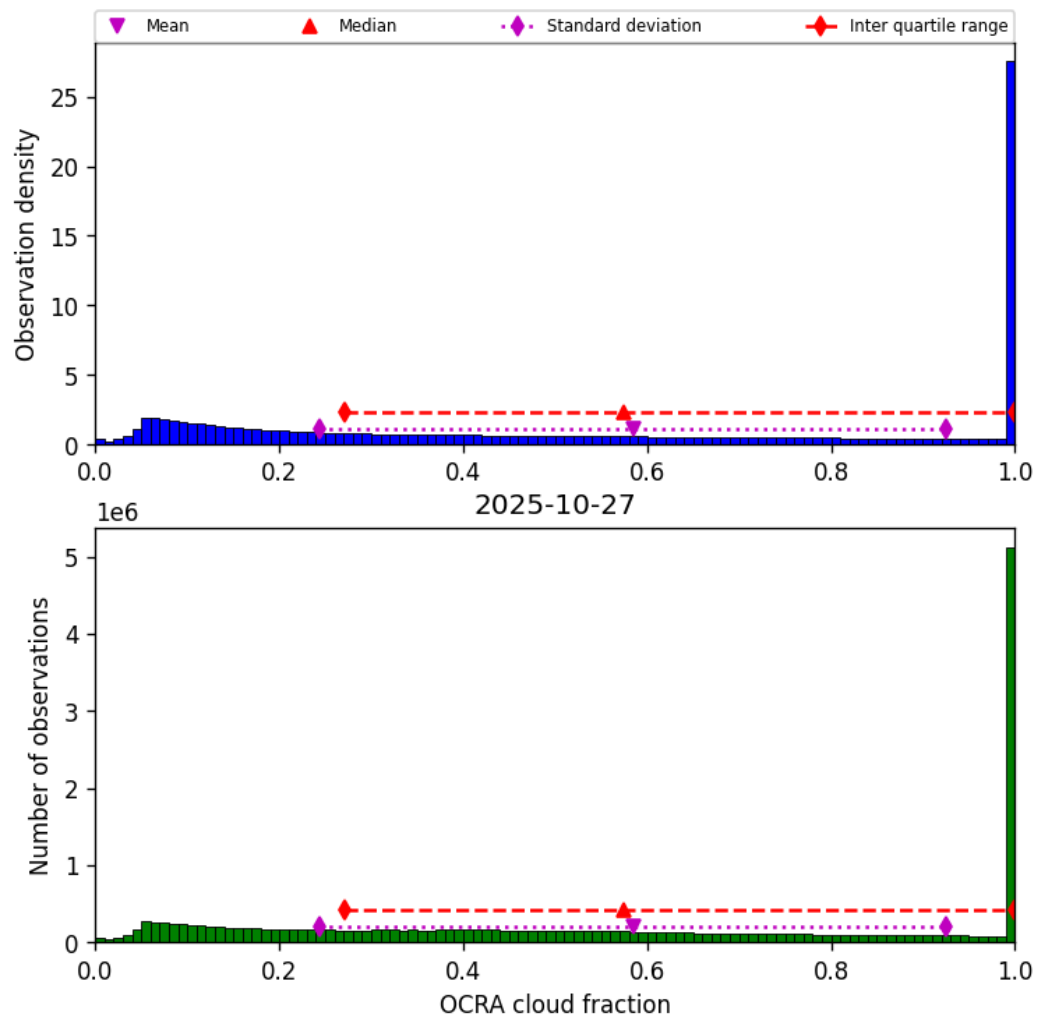
Figure 48: Histogram of “OCRA cloud fraction” for 2025-10-27 to 2025-10-28
