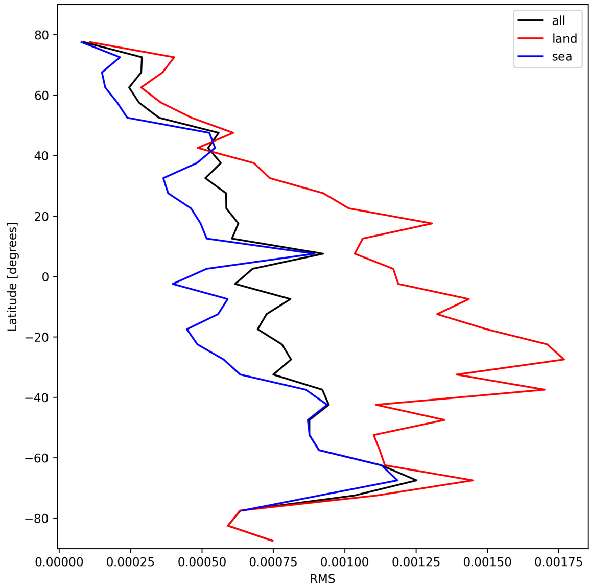
Figure 29: Zonal average of “RMS” for 2025-10-27 to 2025-10-28.
