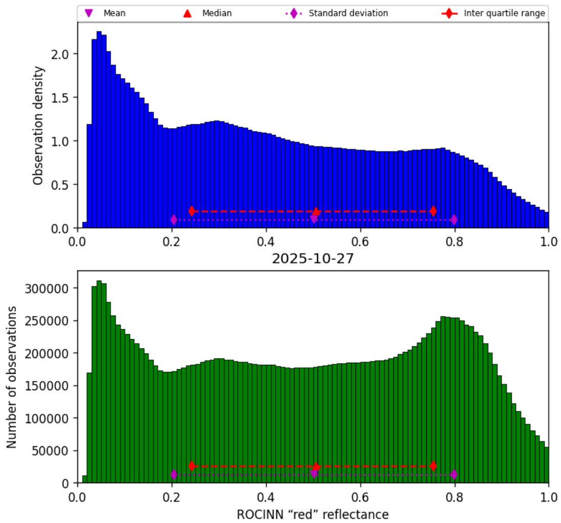
Figure 51: Histogram of “ROCINN “red” reflectance” for 2025-10-27 to 2025-10-28
