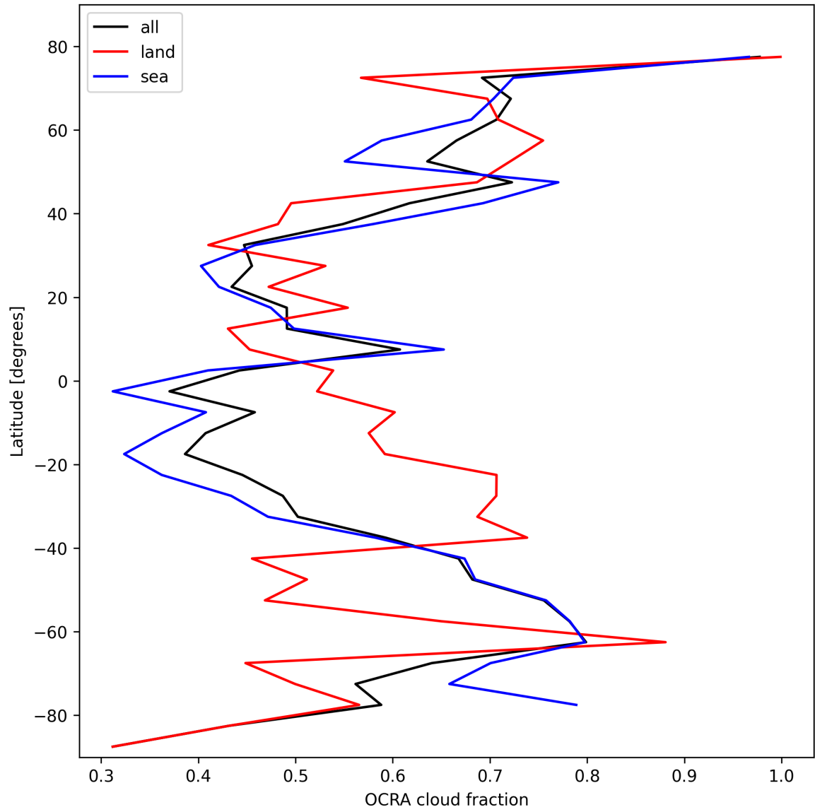
Figure 32: Zonal average of “OCRA cloud fraction” for 2025-10-27 to 2025-10-28.
