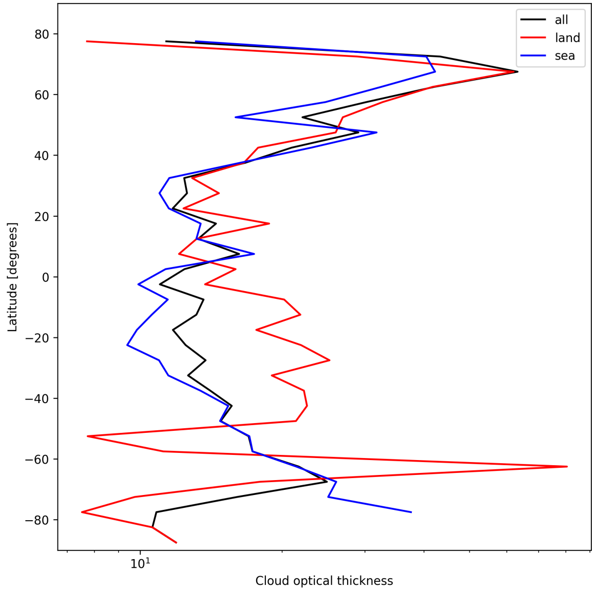
Figure 23: Zonal average of “Cloud optical thickness” for 2025-10-27 to 2025-10-28.
