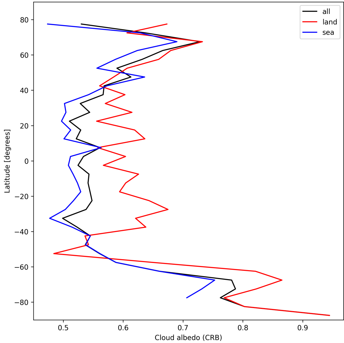
Figure 26: Zonal average of “Cloud albedo (CRB)” for 2025-10-27 to 2025-10-28.
