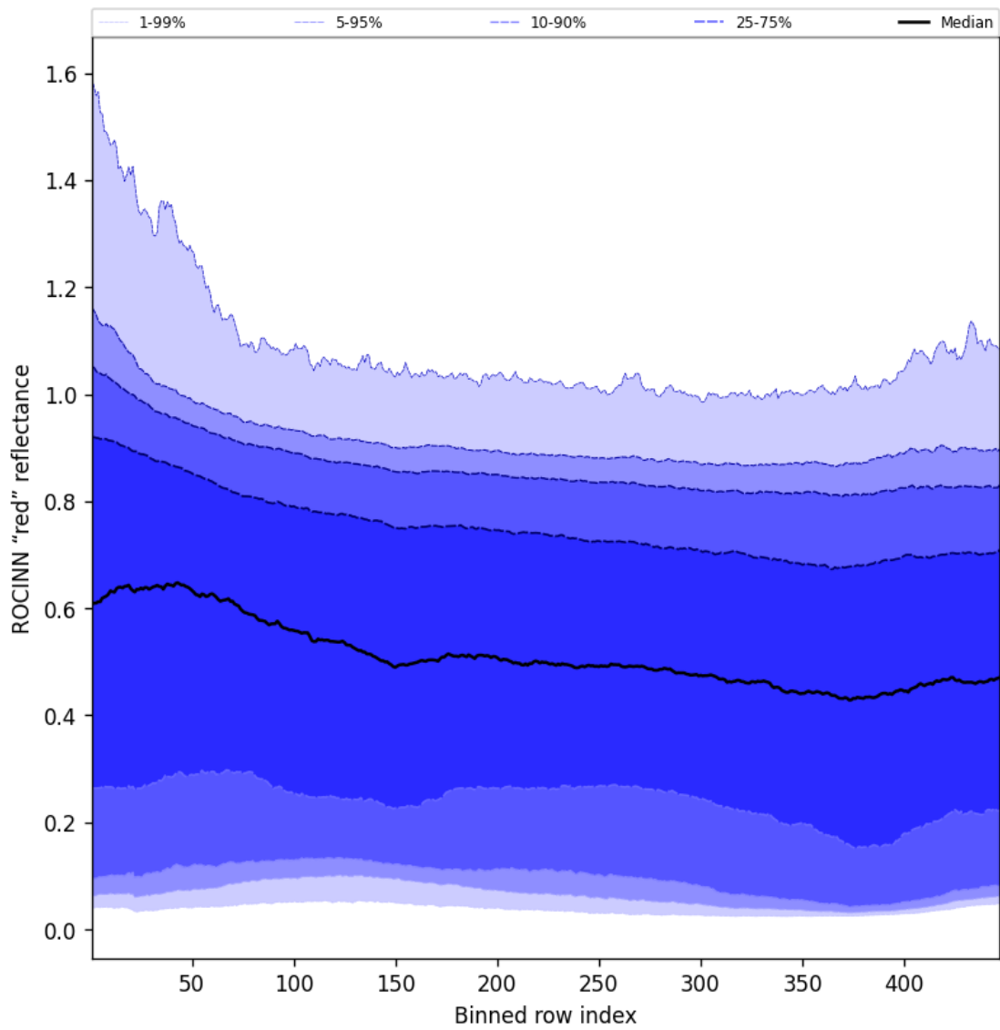
Figure 67: Along track statistics of “ROCINN “red” reflectance” for 2025-10-27 to 2025-10-28
