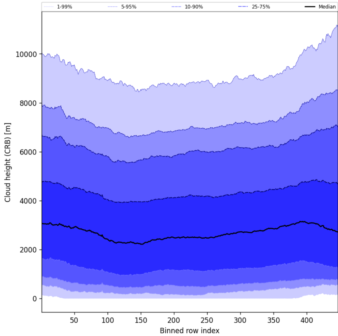
Figure 57: Along track statistics of “Cloud height (CRB)” for 2025-10-27 to 2025-10-28
