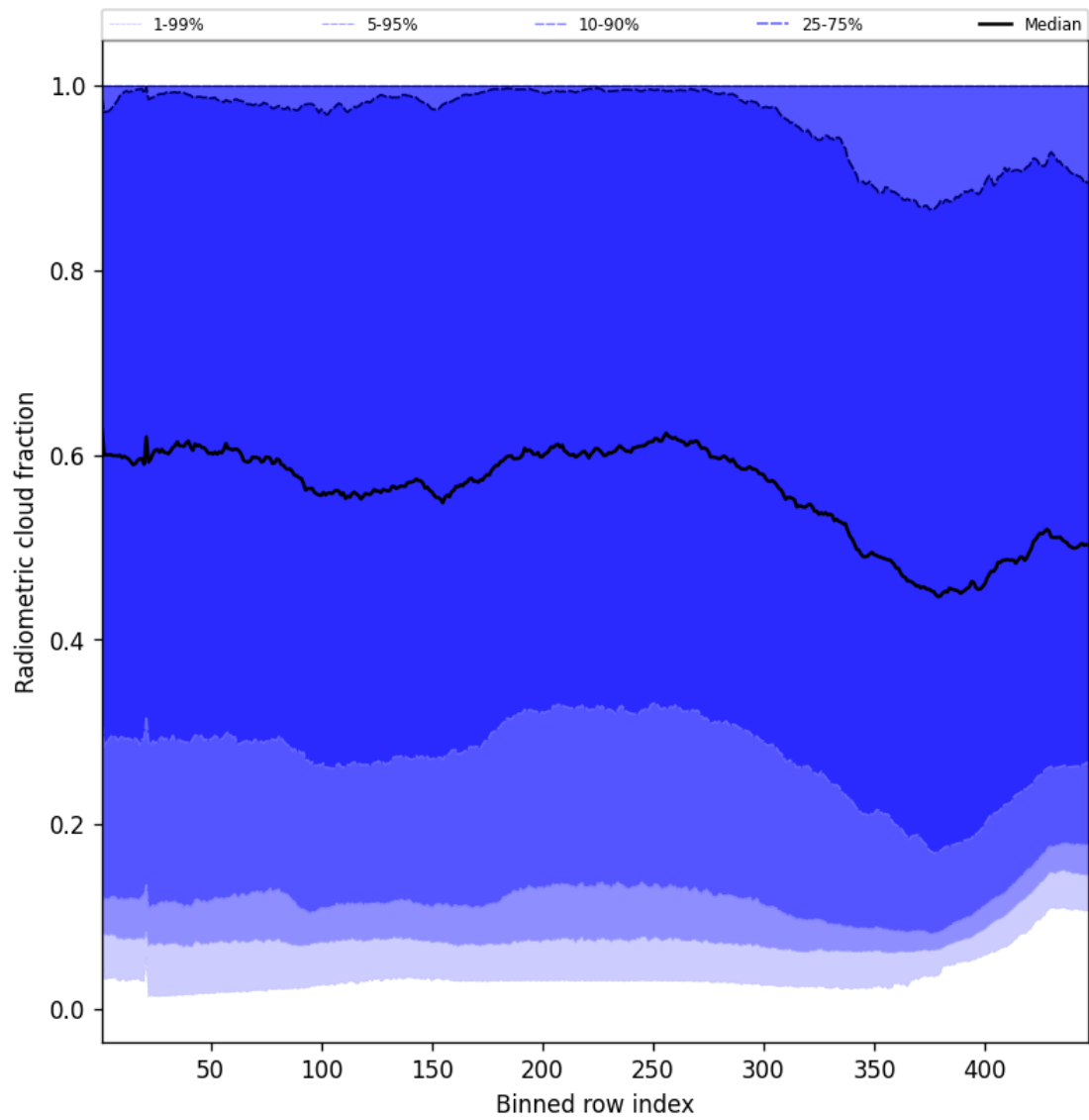
Figure 53: Along track statistics of “Radiometric cloud fraction” for 2025-10-27 to 2025-10-28
