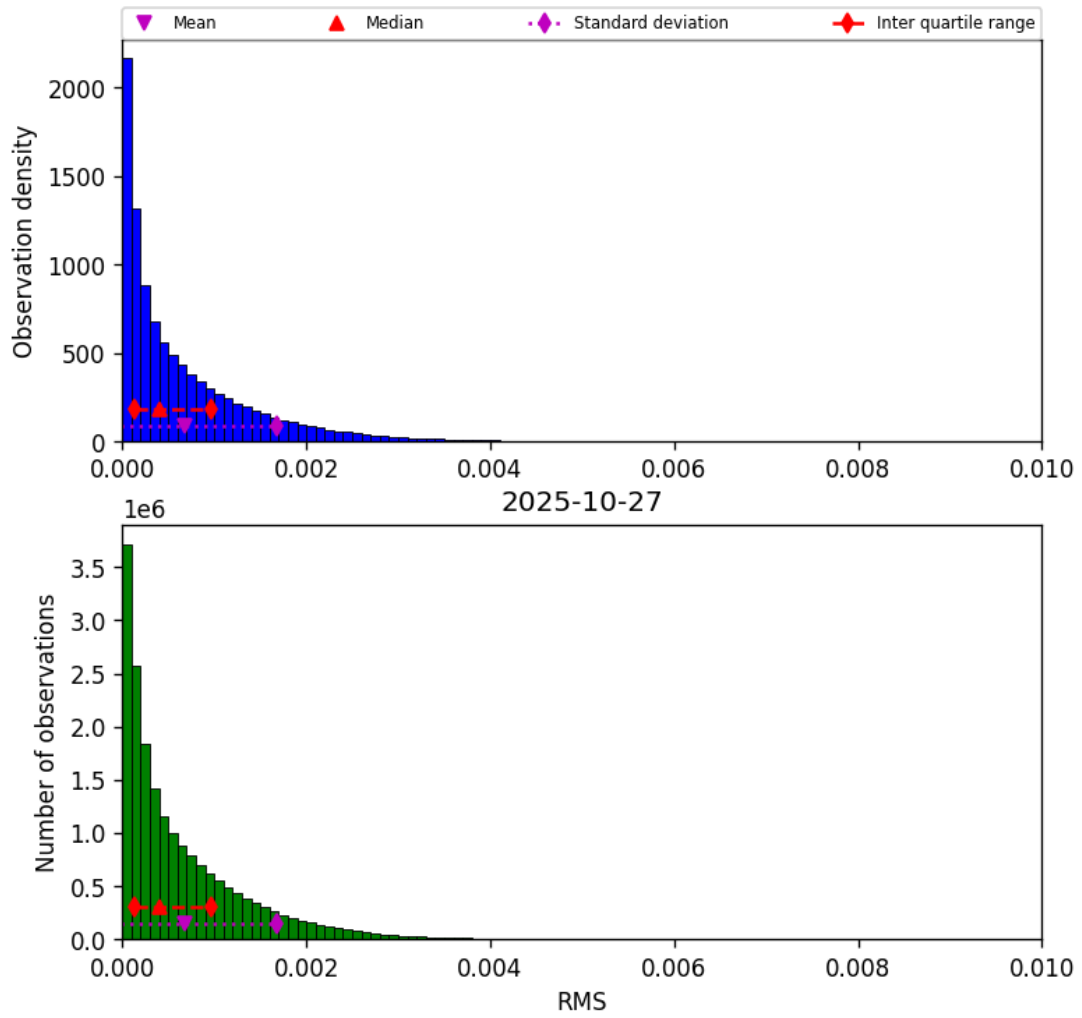
Figure 45: Histogram of “RMS” for 2025-10-27 to 2025-10-28
