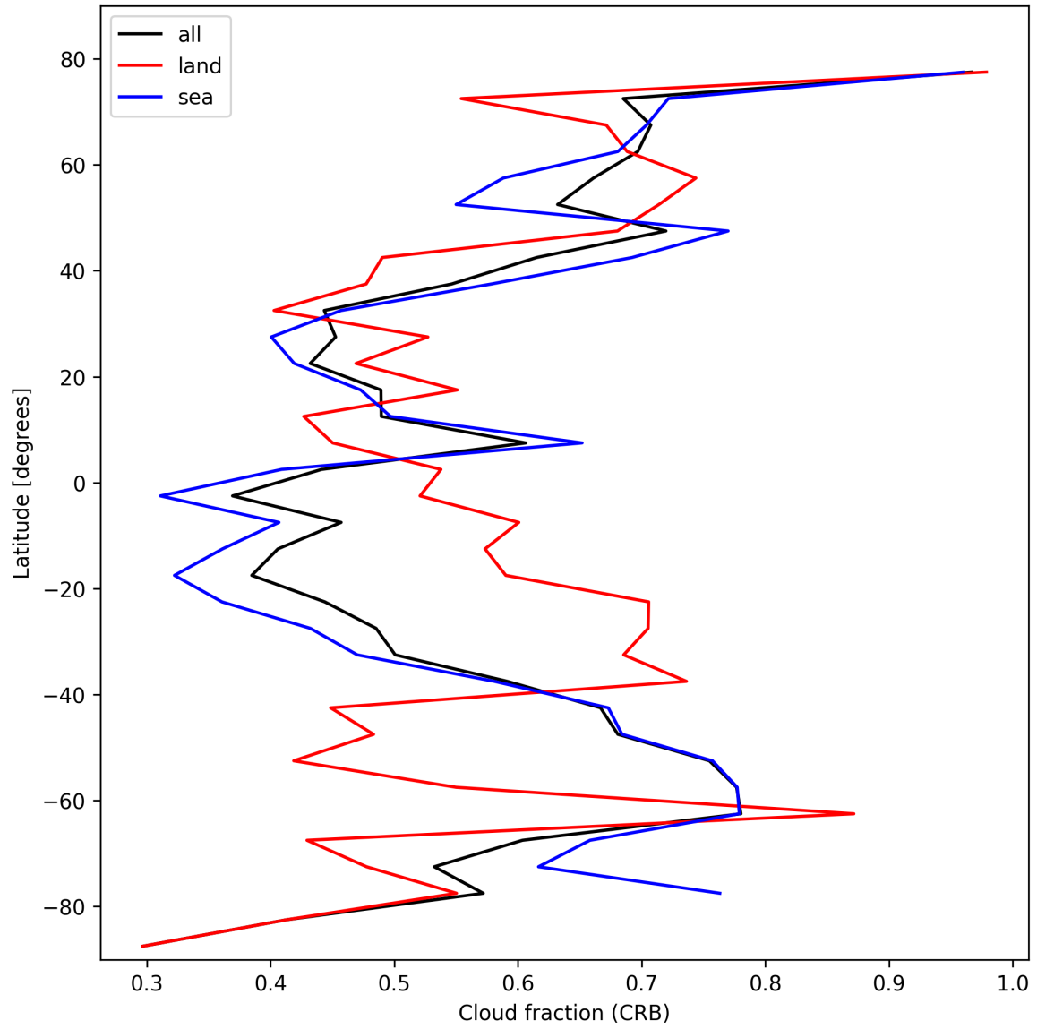
Figure 24: Zonal average of “Cloud fraction (CRB)” for 2025-10-27 to 2025-10-28.
