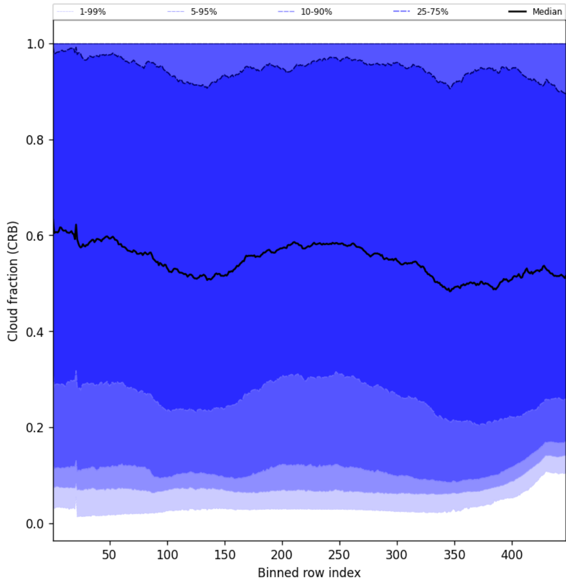
Figure 56: Along track statistics of “Cloud fraction (CRB)” for 2025-10-29 to 2025-10-30
