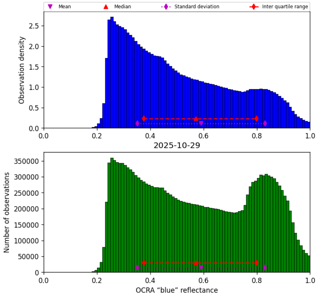
Figure 49: Histogram of “OCRA “blue” reflectance” for 2025-10-29 to 2025-10-30
