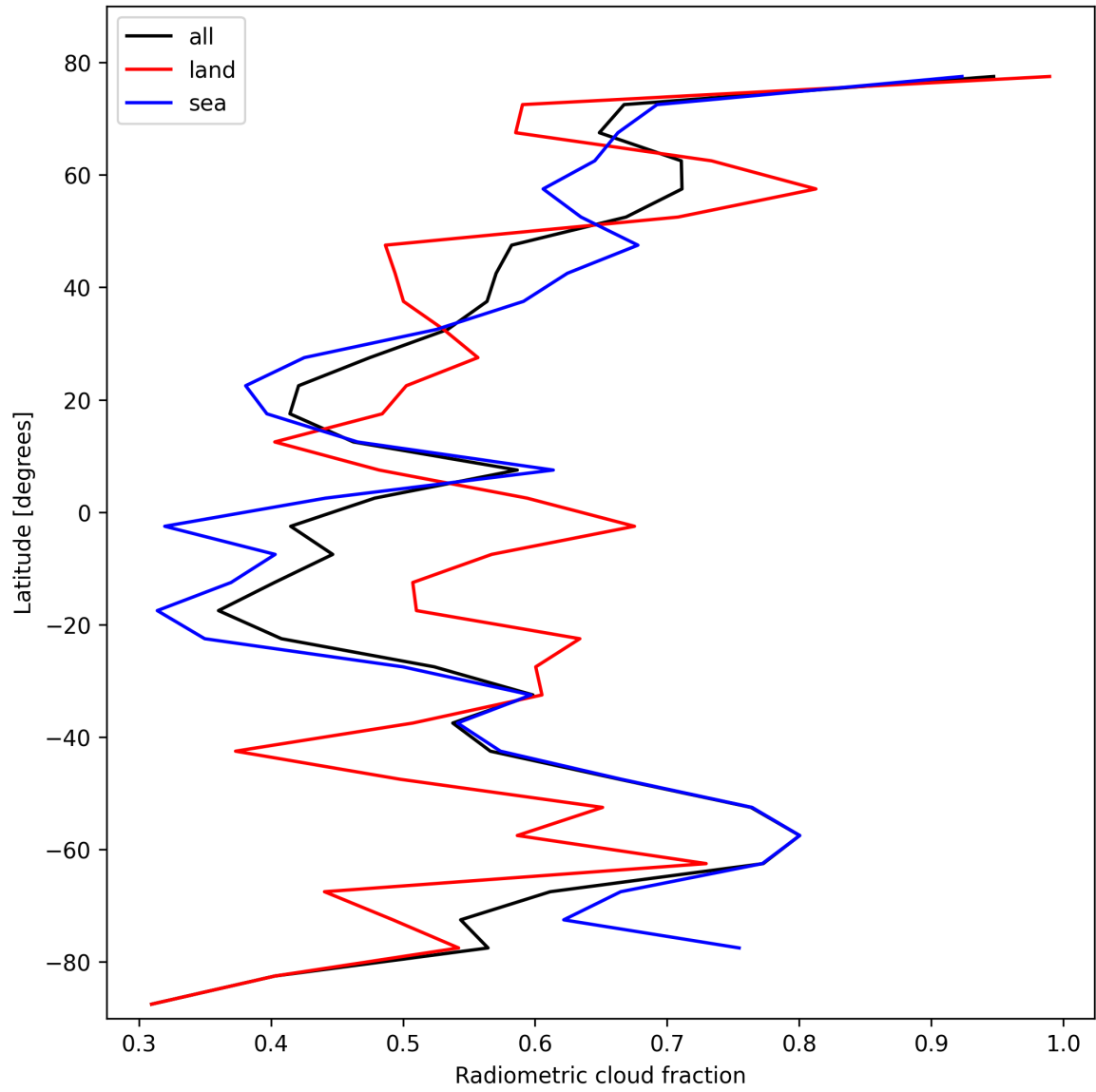
Figure 21: Zonal average of “Radiometric cloud fraction” for 2025-10-29 to 2025-10-30.
