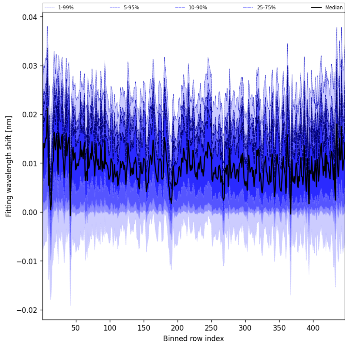
Figure 63: Along track statistics of “Fitting wavelength shift” for 2025-10-29 to 2025-10-30
