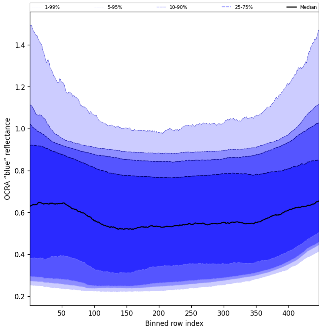
Figure 65: Along track statistics of “OCRA “blue” reflectance” for 2025-10-29 to 2025-10-30
