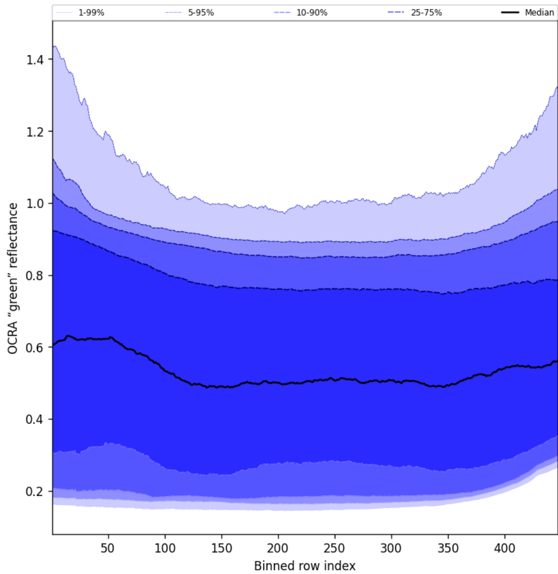
Figure 66: Along track statistics of “OCRA “green” reflectance” for 2025-10-29 to 2025-10-30
