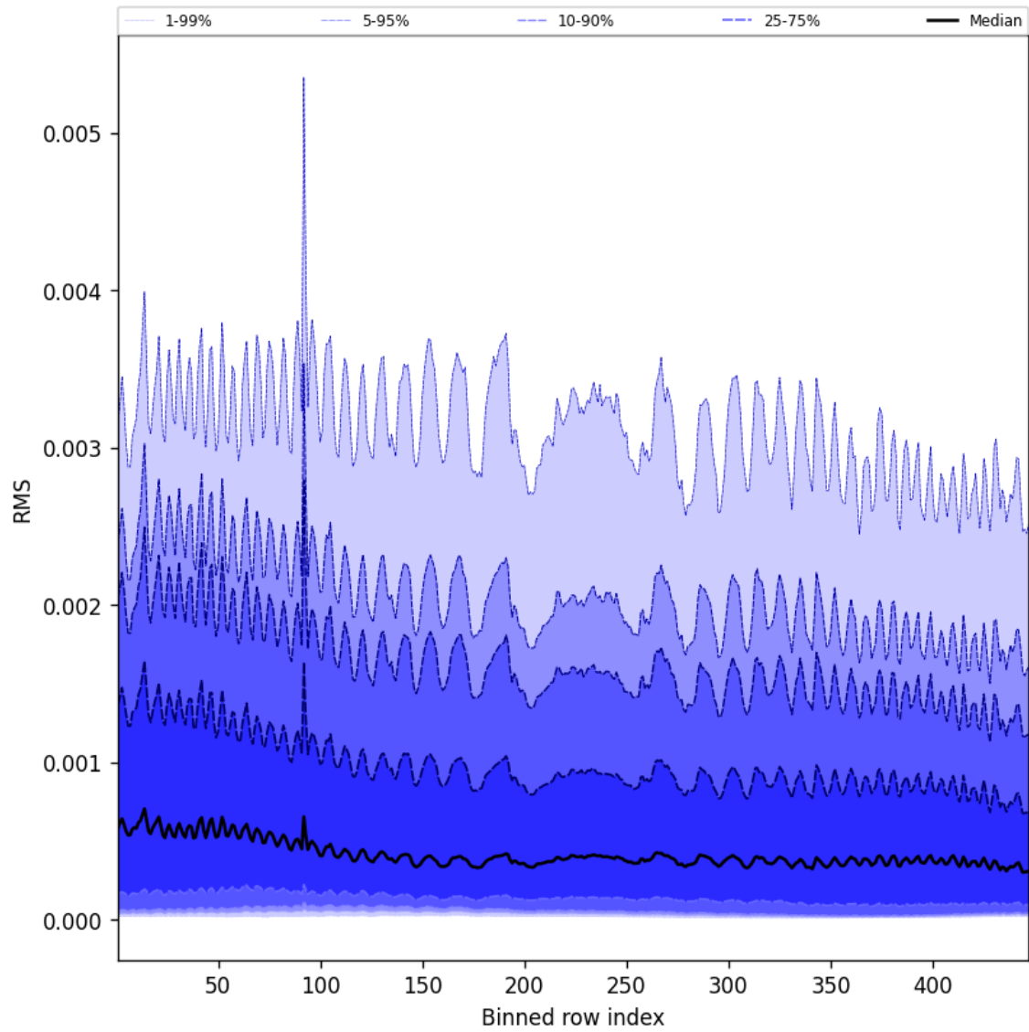
Figure 61: Along track statistics of “RMS” for 2025-10-29 to 2025-10-30
