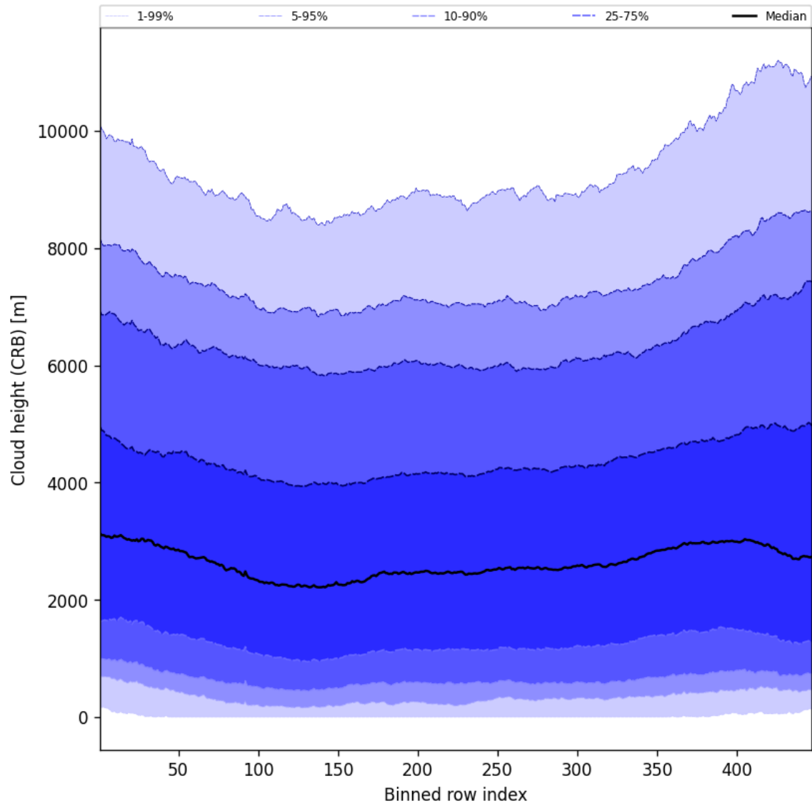
Figure 57: Along track statistics of “Cloud height (CRB)” for 2025-10-29 to 2025-10-30
