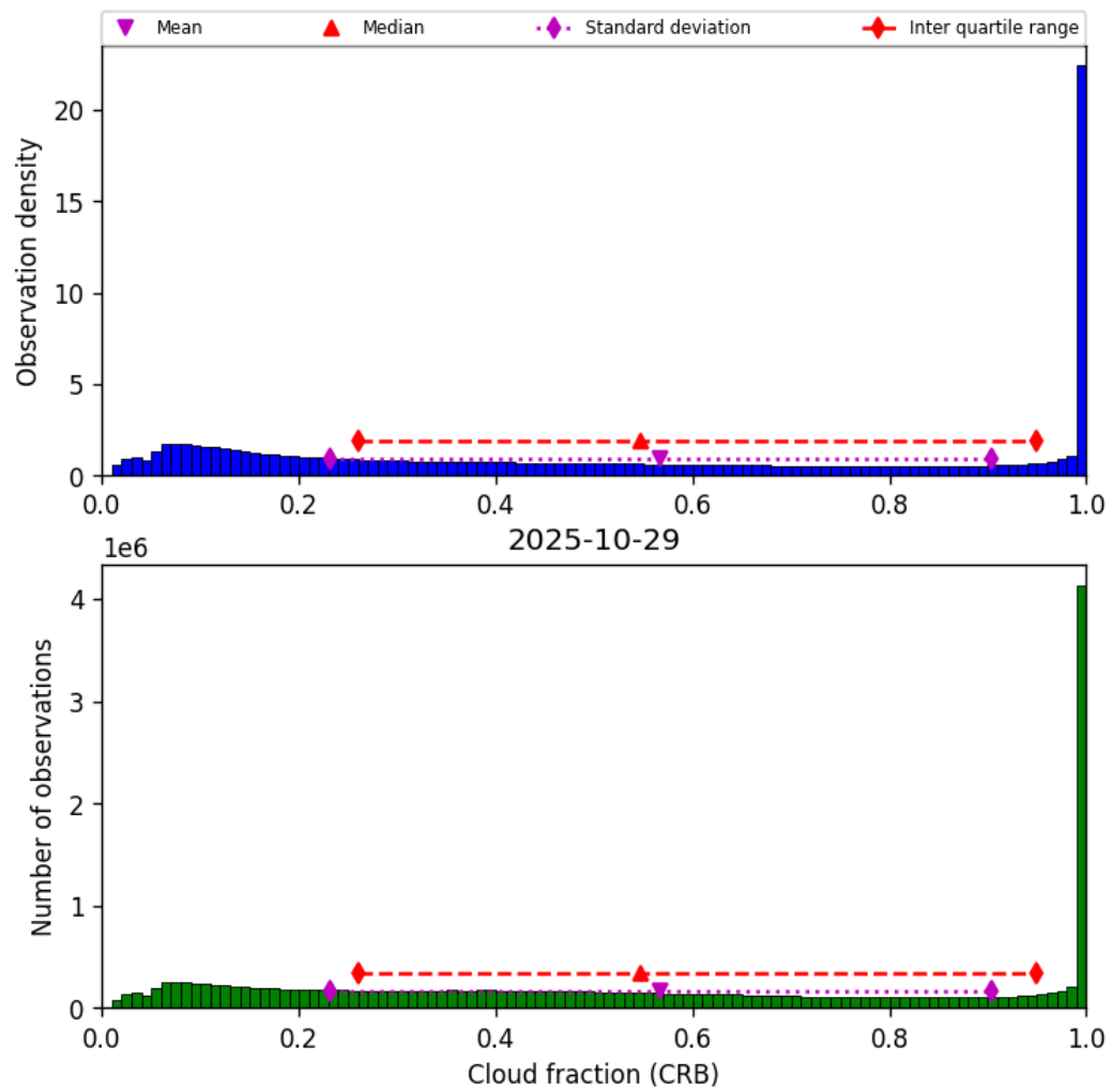
Figure 40: Histogram of “Cloud fraction (CRB)” for 2025-10-29 to 2025-10-30
