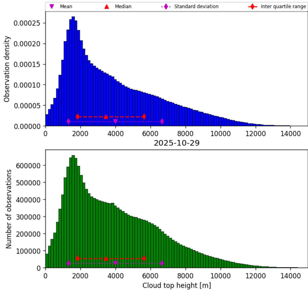
Figure 38: Histogram of “Cloud top height” for 2025-10-29 to 2025-10-30
