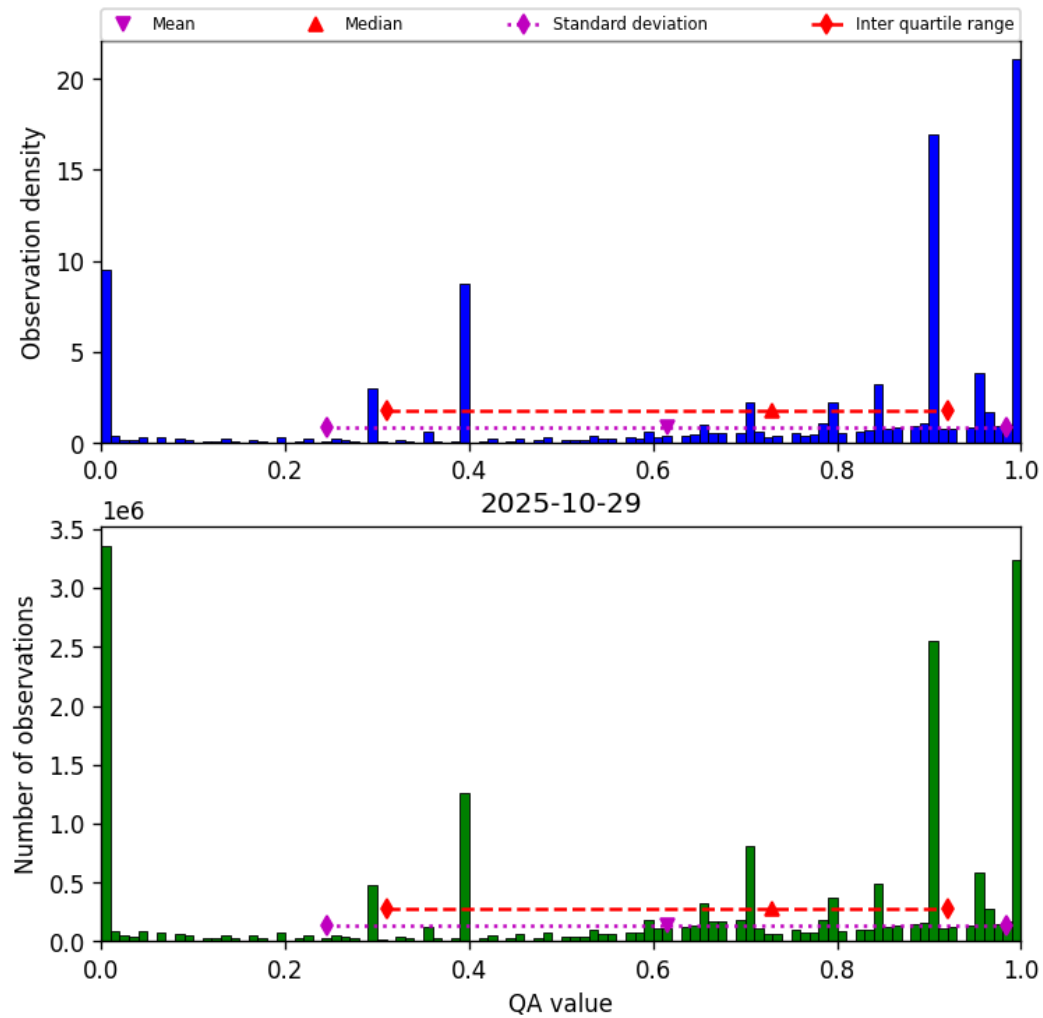
Figure 36: Histogram of “QA value” for 2025-10-29 to 2025-10-30
