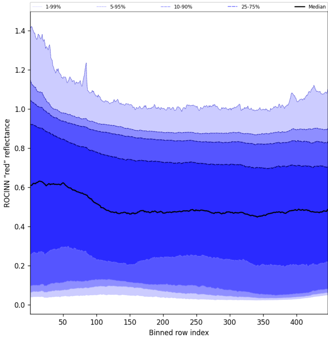
Figure 67: Along track statistics of “ROCINN “red” reflectance” for 2025-10-29 to 2025-10-30
