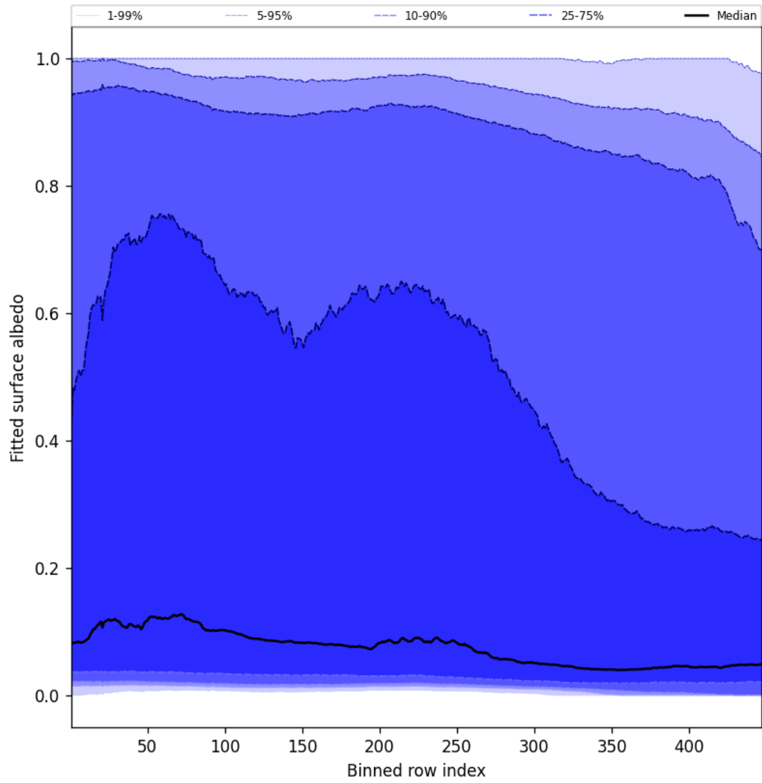
Figure 59: Along track statistics of “Fitted surface albedo” for 2025-10-29 to 2025-10-30
