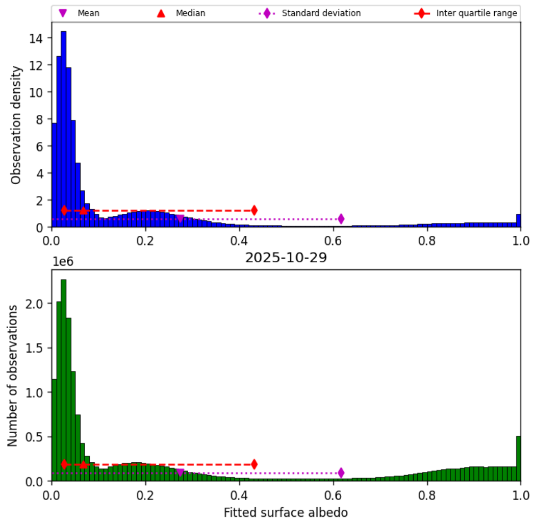
Figure 43: Histogram of “Fitted surface albedo” for 2025-10-29 to 2025-10-30
