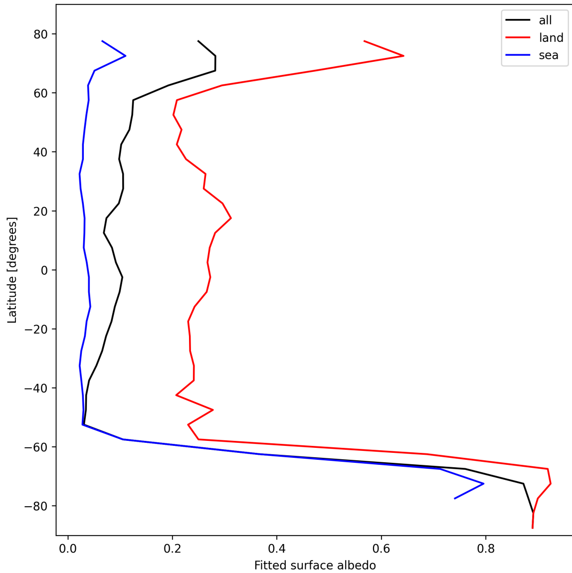
Figure 27: Zonal average of “Fitted surface albedo” for 2025-10-29 to 2025-10-30.
