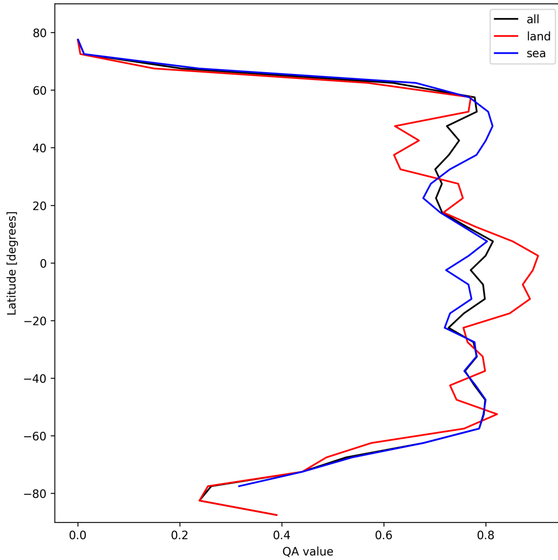
Figure 20: Zonal average of “QA value” for 2025-10-29 to 2025-10-30.
