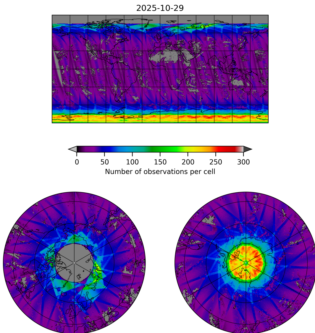
Figure 19: Map of the number of observations for 2025-10-29 to 2025-10-30
