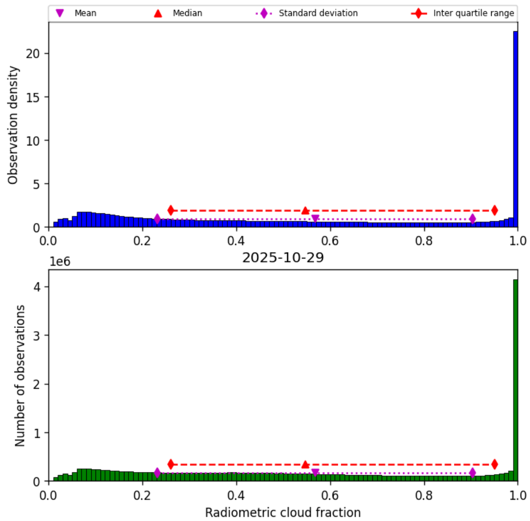
Figure 37: Histogram of “Radiometric cloud fraction” for 2025-10-29 to 2025-10-30
