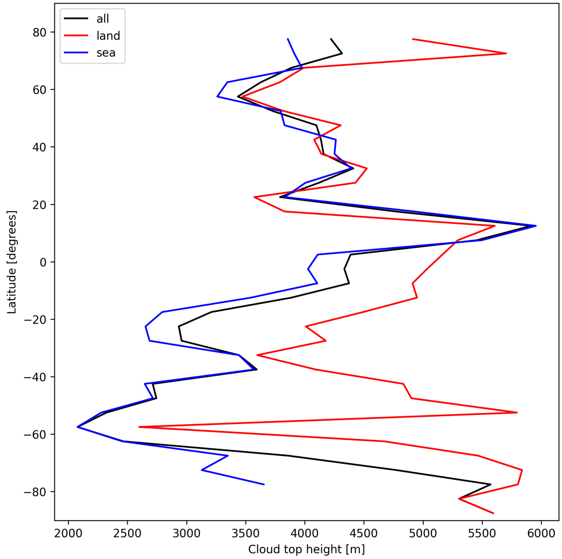
Figure 22: Zonal average of “Cloud top height” for 2025-10-29 to 2025-10-30.
