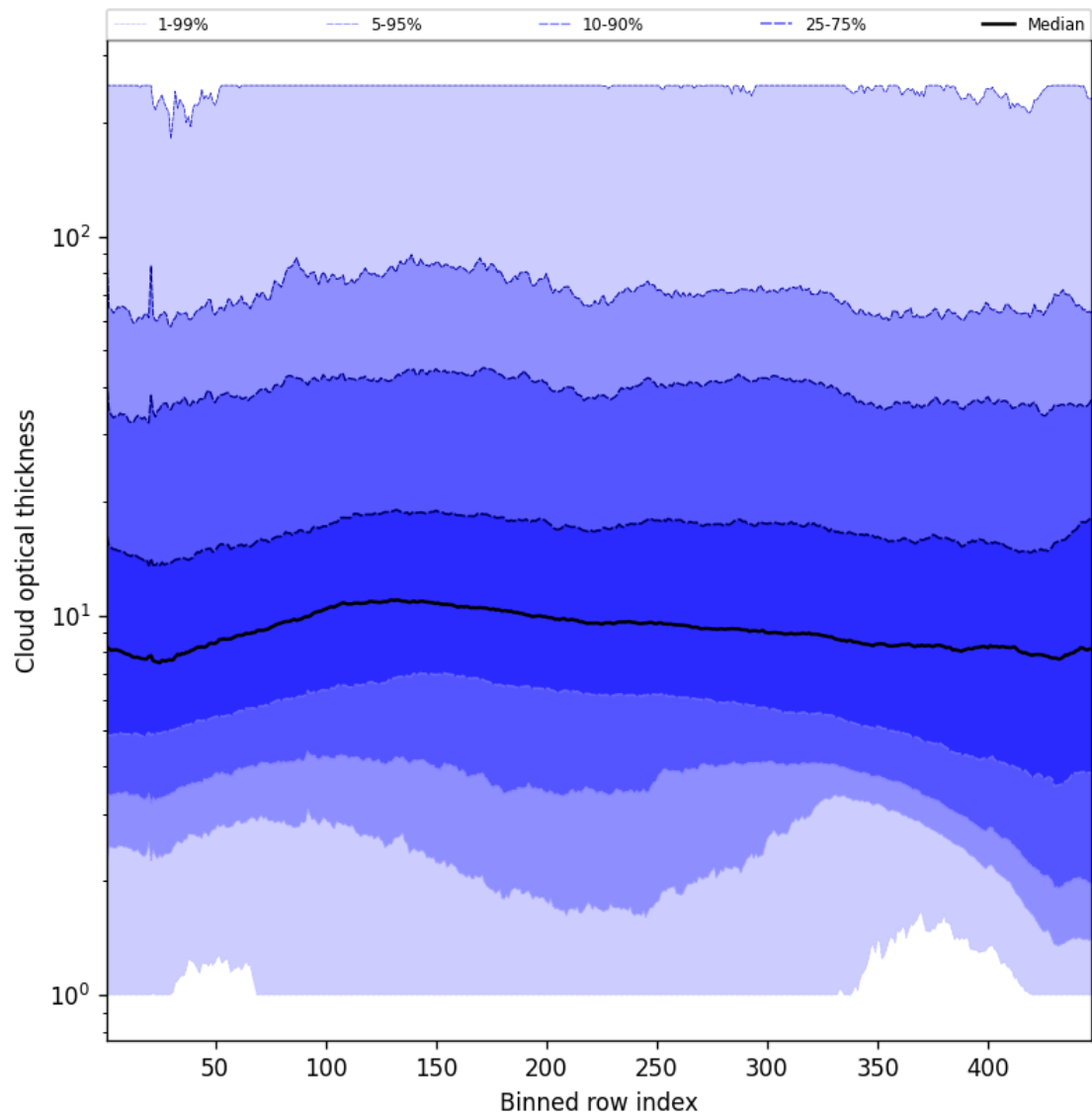
Figure 55: Along track statistics of “Cloud optical thickness” for 2025-10-29 to 2025-10-30
