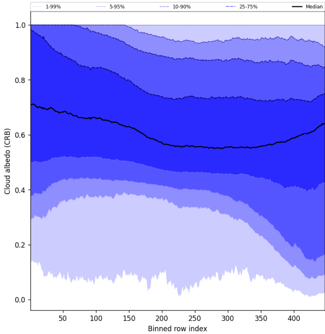
Figure 58: Along track statistics of “Cloud albedo (CRB)” for 2025-10-29 to 2025-10-30
