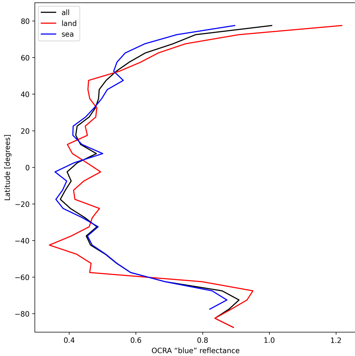
Figure 33: Zonal average of “OCRA “blue” reflectance” for 2025-10-29 to 2025-10-30.
