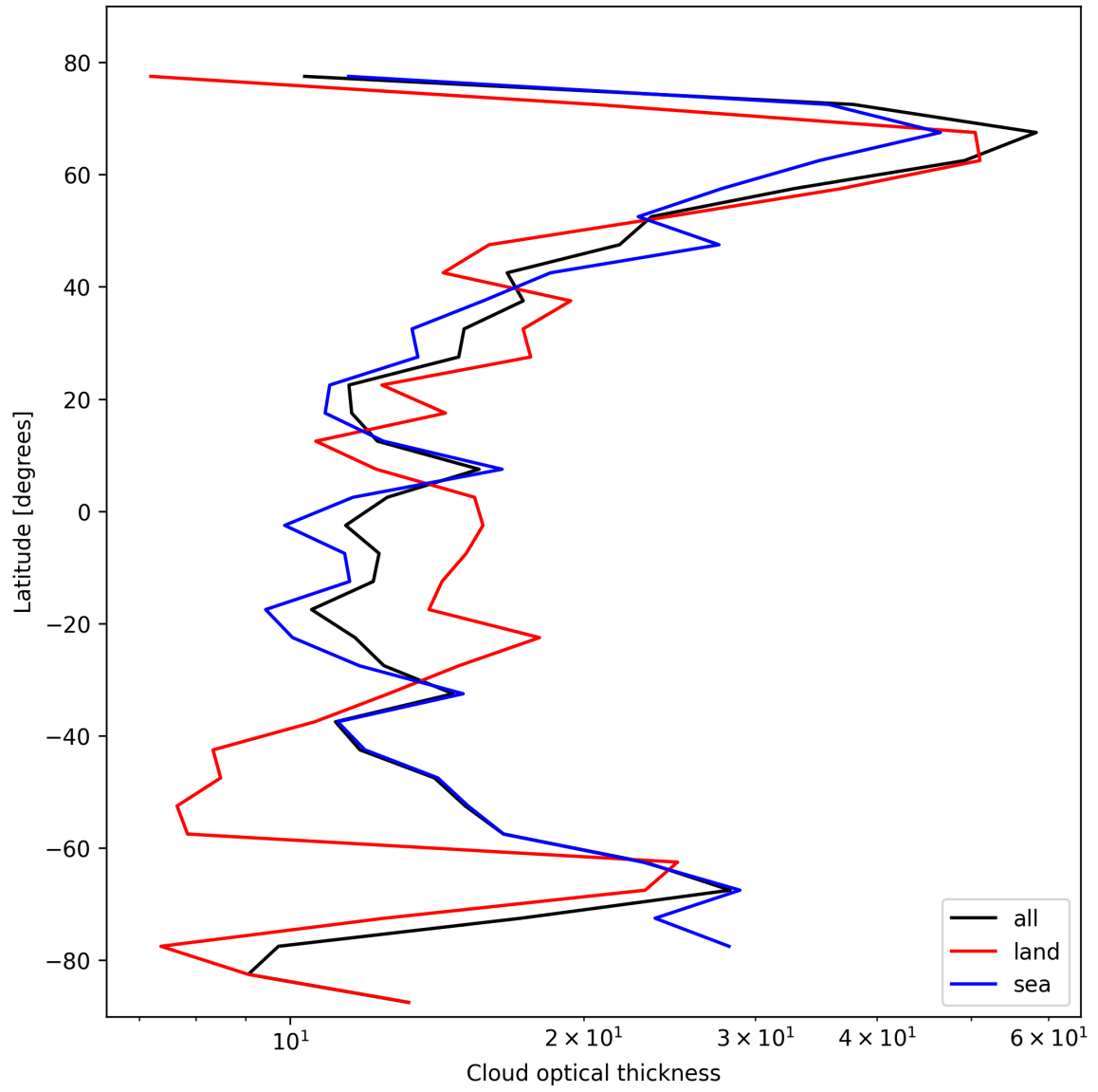
Figure 23: Zonal average of “Cloud optical thickness” for 2025-10-29 to 2025-10-30.
