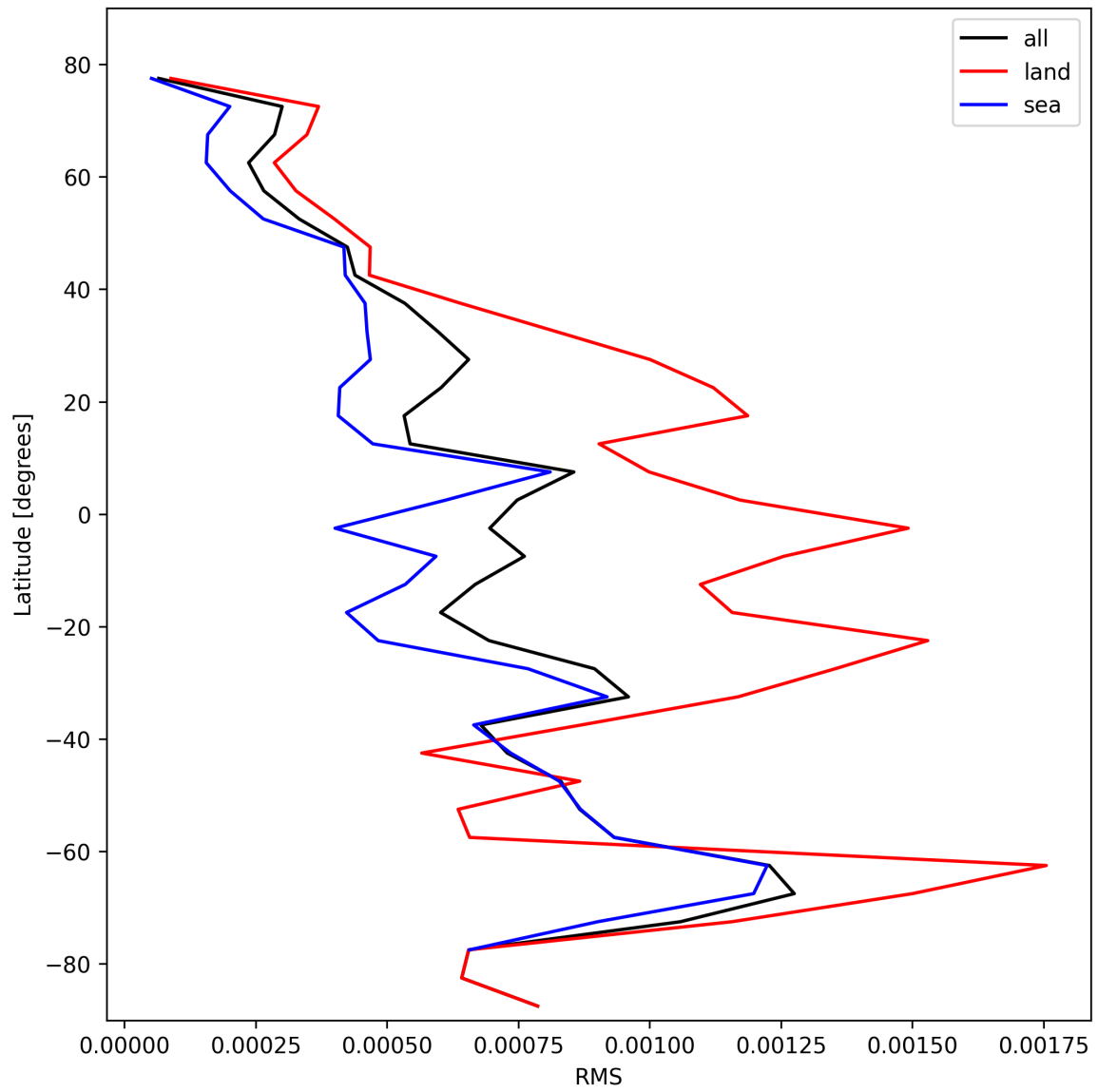
Figure 29: Zonal average of “RMS” for 2025-10-29 to 2025-10-30.
