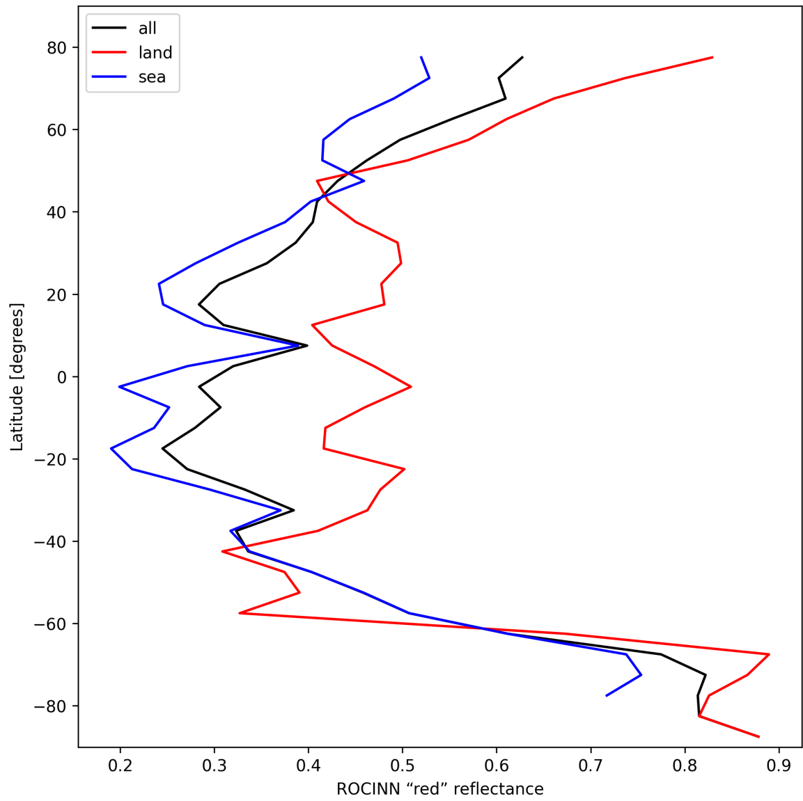
Figure 35: Zonal average of “ROCINN “red” reflectance” for 2025-10-29 to 2025-10-30.
