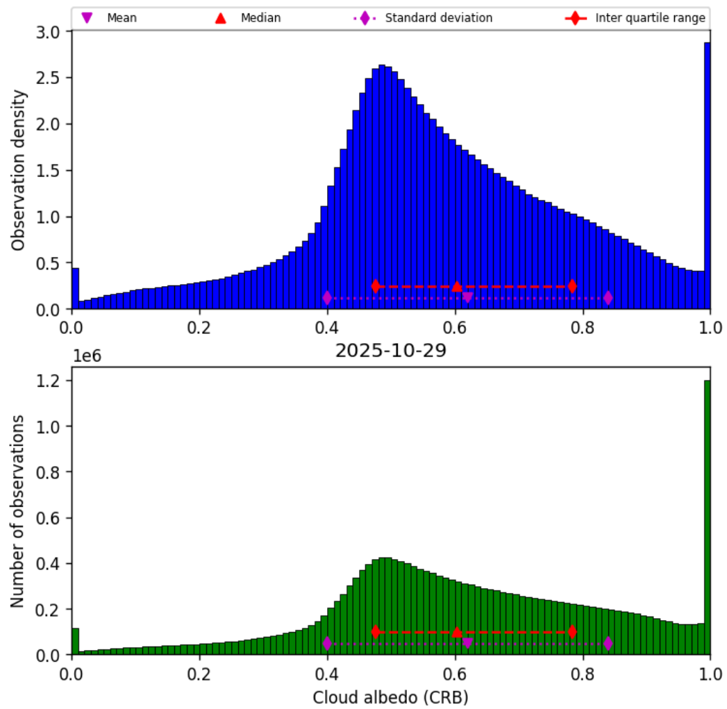
Figure 42: Histogram of “Cloud albedo (CRB)” for 2025-10-29 to 2025-10-30
