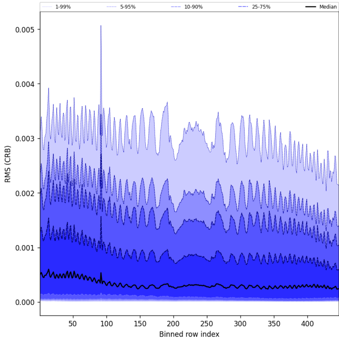
Figure 62: Along track statistics of “RMS (CRB)” for 2025-10-29 to 2025-10-30
