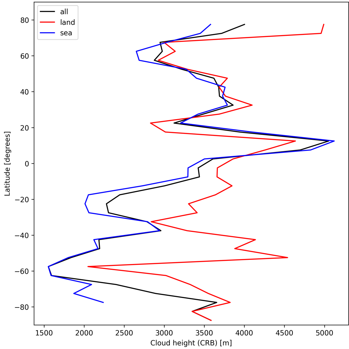
Figure 25: Zonal average of “Cloud height (CRB)” for 2025-10-29 to 2025-10-30.
