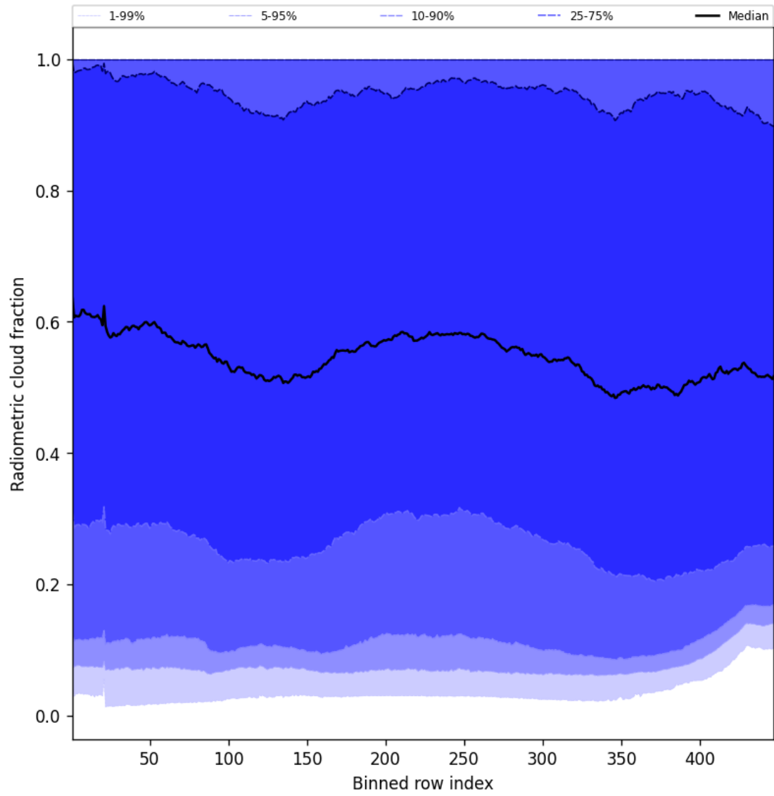
Figure 53: Along track statistics of “Radiometric cloud fraction” for 2025-10-29 to 2025-10-30
