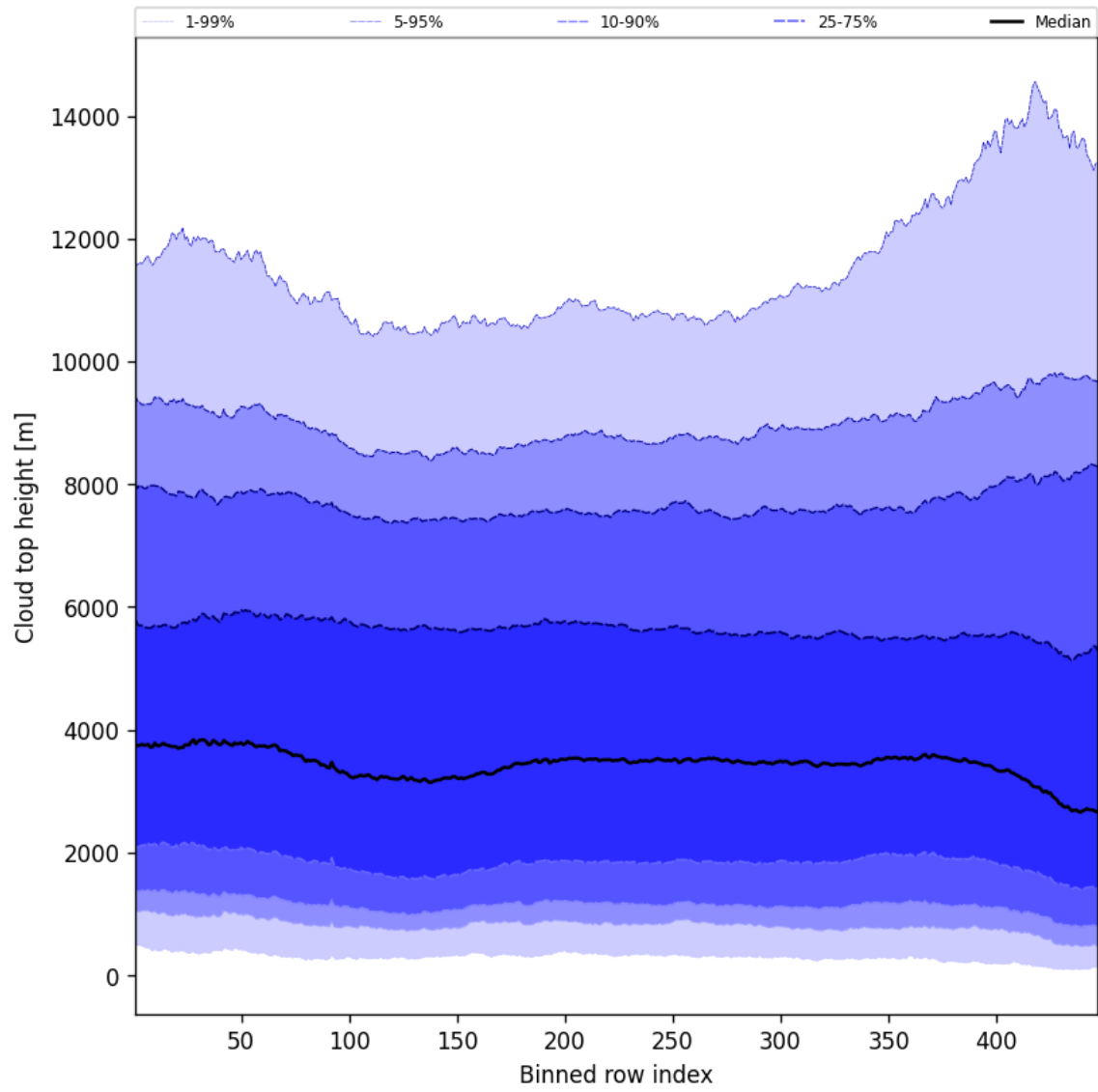
Figure 54: Along track statistics of “Cloud top height” for 2025-10-29 to 2025-10-30
