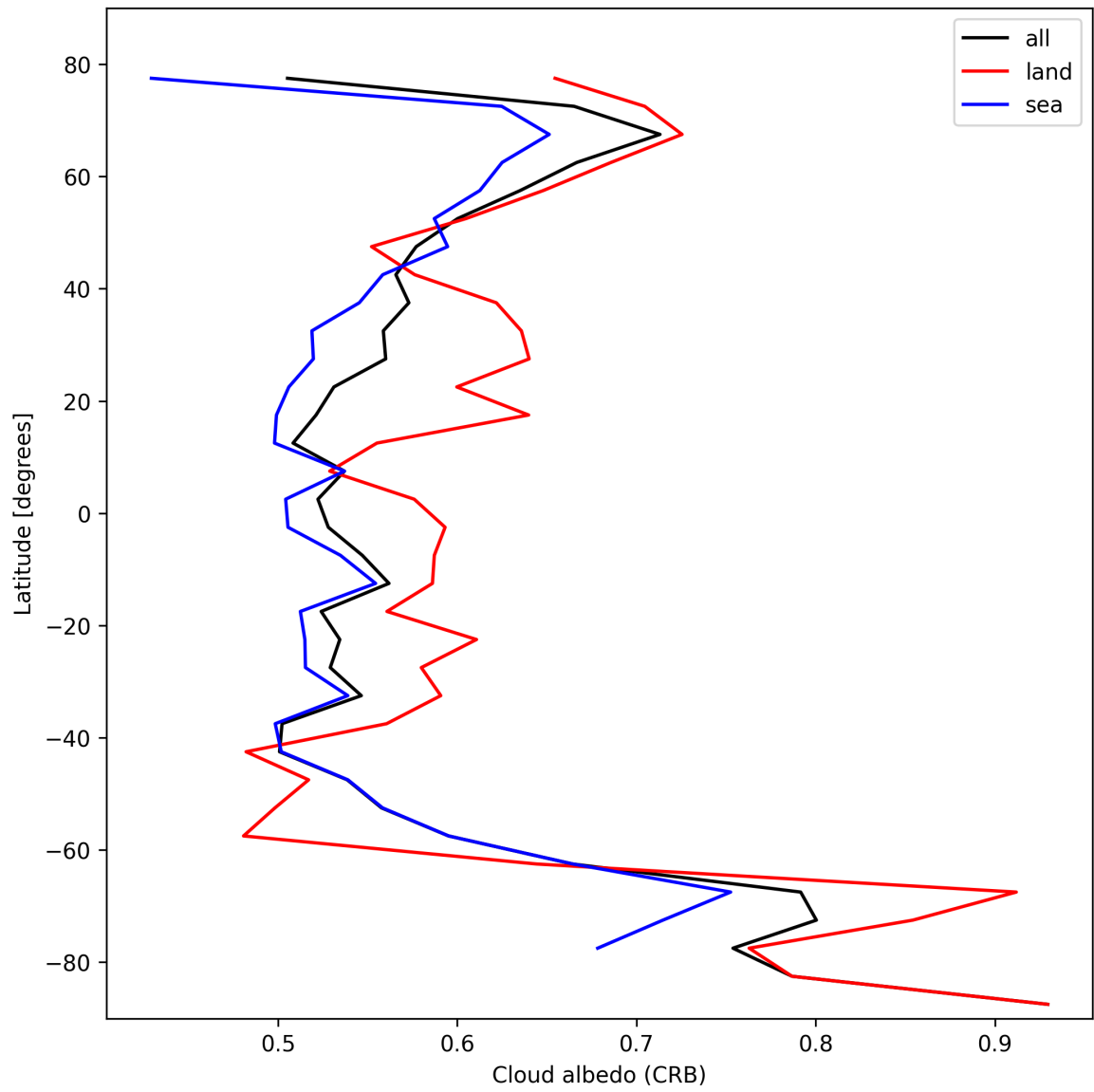
Figure 26: Zonal average of “Cloud albedo (CRB)” for 2025-10-29 to 2025-10-30.
