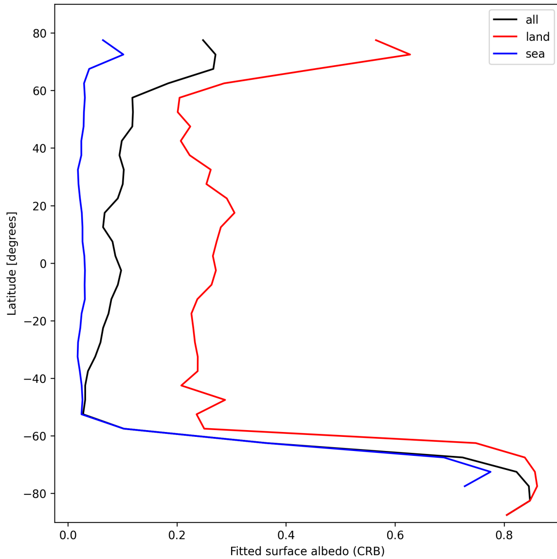
Figure 28: Zonal average of “Fitted surface albedo (CRB)” for 2025-10-29 to 2025-10-30.
