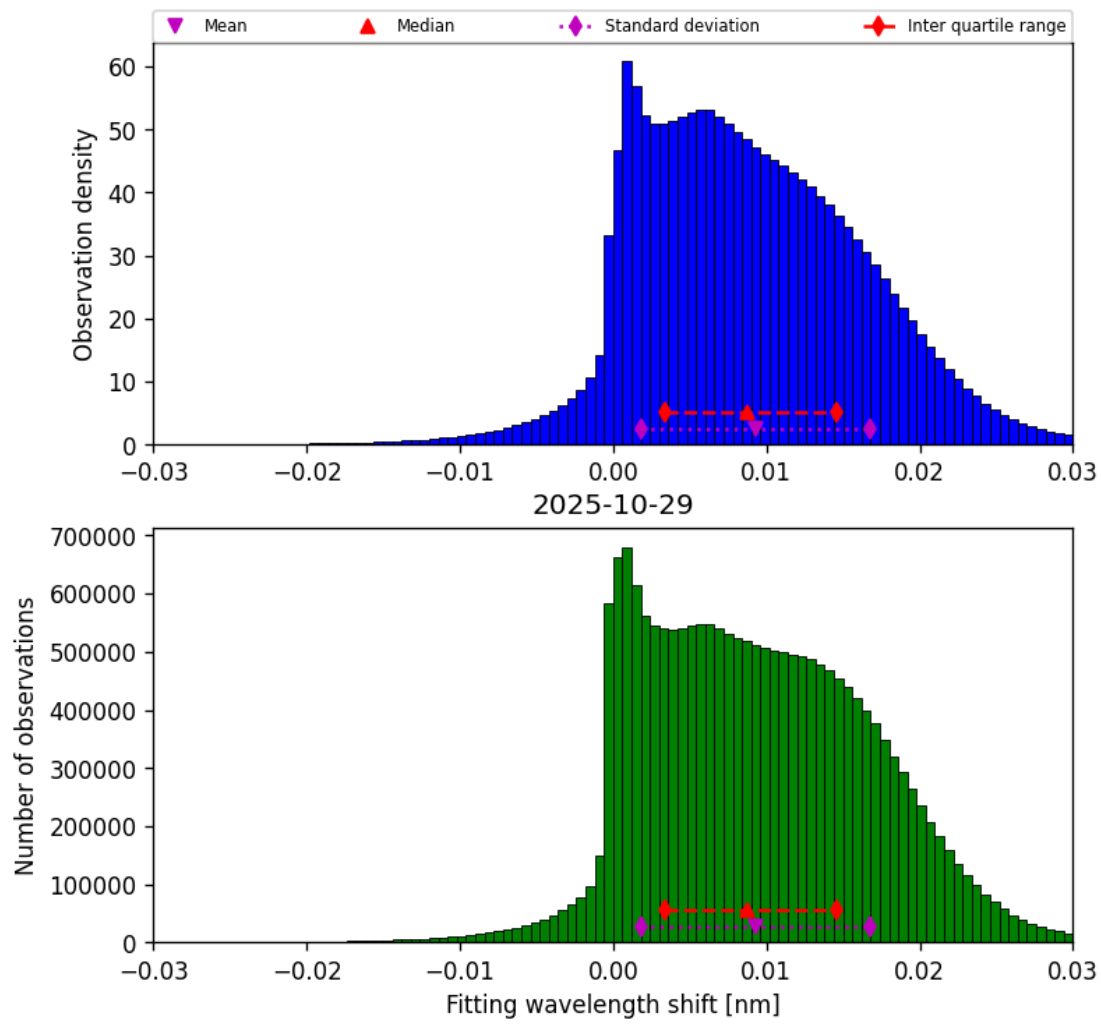
Figure 47: Histogram of “Fitting wavelength shift” for 2025-10-29 to 2025-10-30
