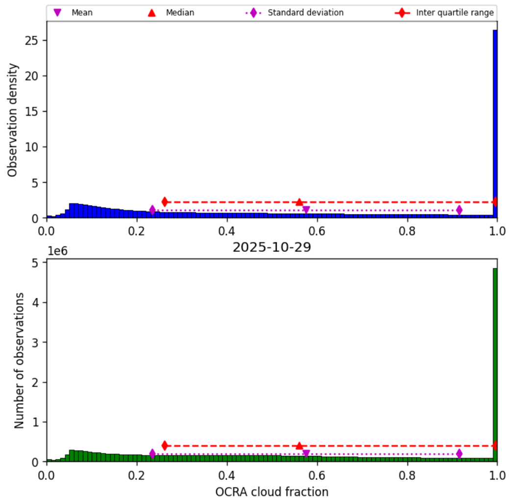
Figure 48: Histogram of “OCRA cloud fraction” for 2025-10-29 to 2025-10-30
