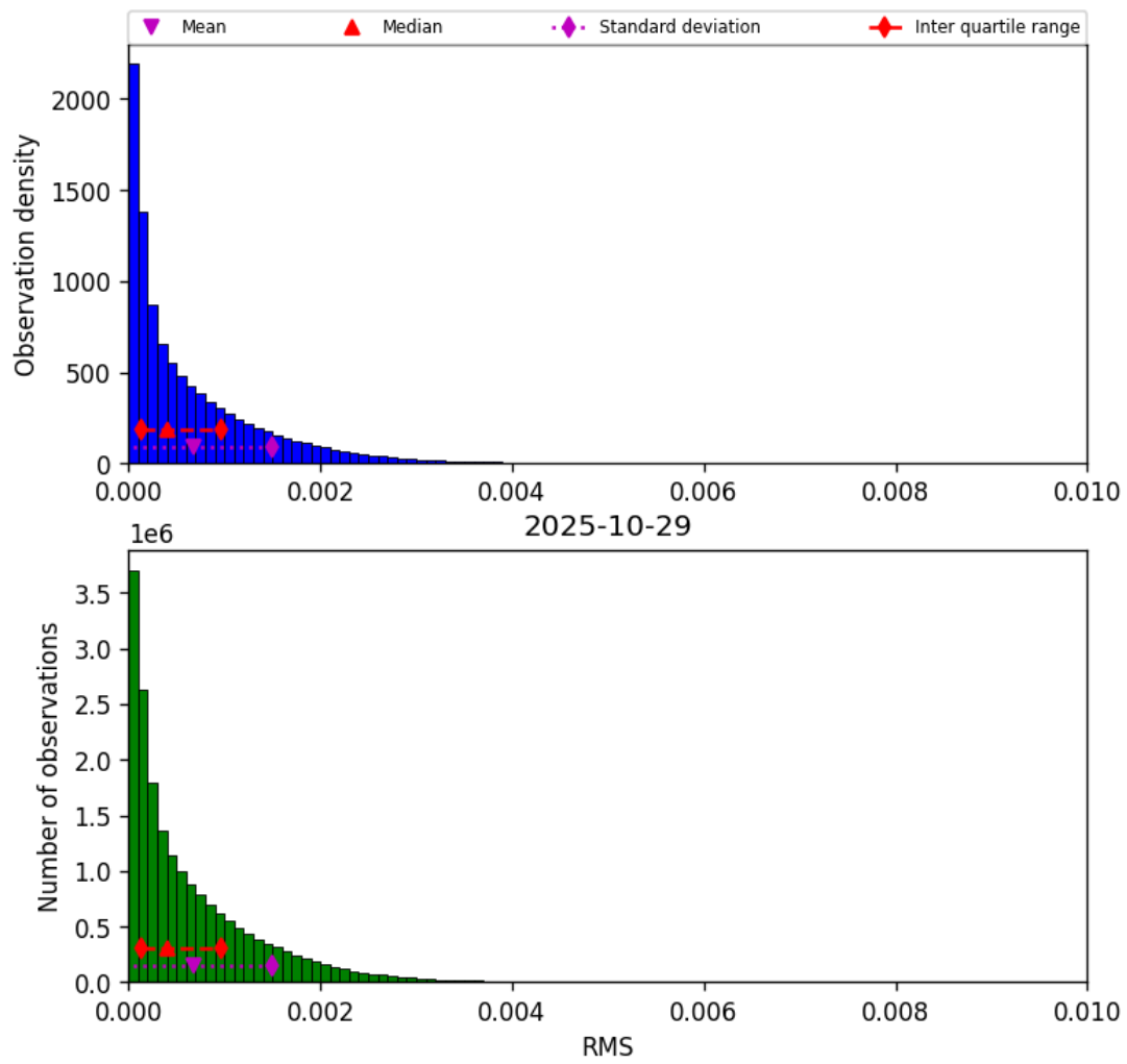
Figure 45: Histogram of “RMS” for 2025-10-29 to 2025-10-30
