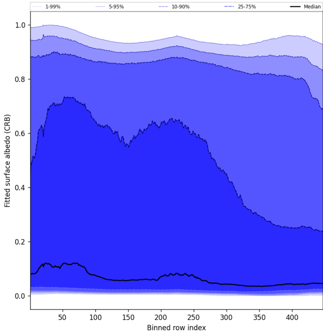
Figure 60: Along track statistics of “Fitted surface albedo (CRB)” for 2025-10-29 to 2025-10-30
