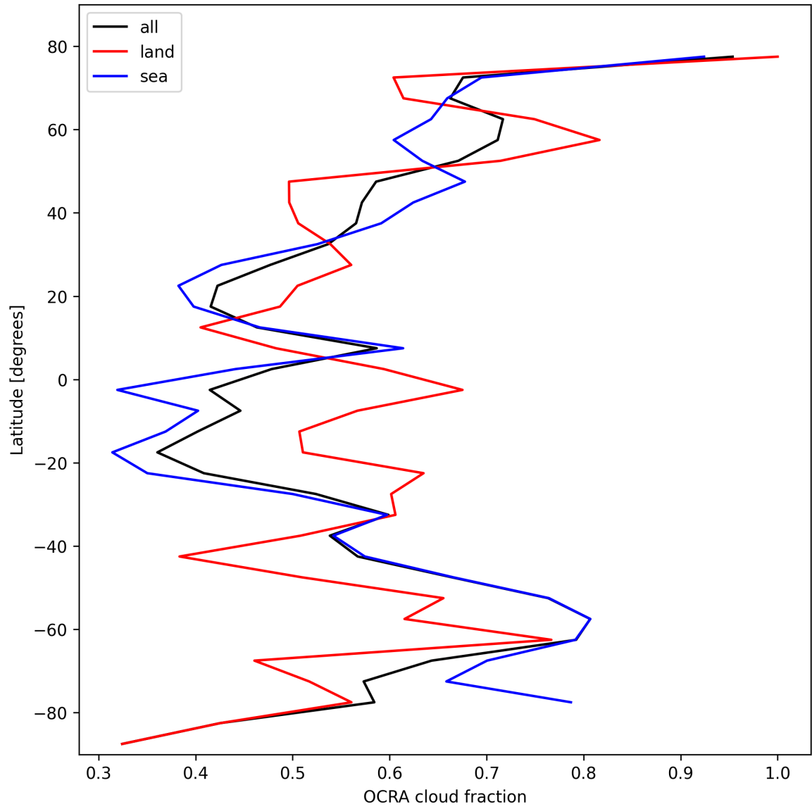
Figure 32: Zonal average of “OCRA cloud fraction” for 2025-10-29 to 2025-10-30.
