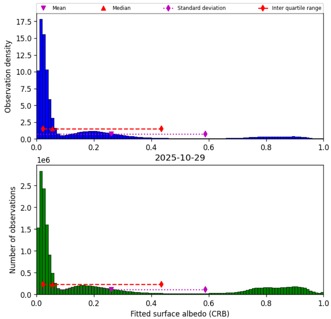
Figure 44: Histogram of “Fitted surface albedo (CRB)” for 2025-10-29 to 2025-10-30
