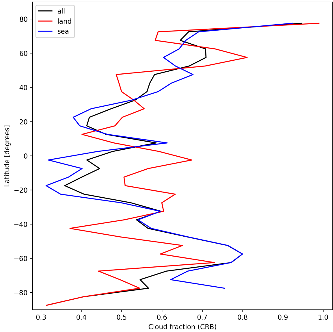
Figure 24: Zonal average of “Cloud fraction (CRB)” for 2025-10-29 to 2025-10-30.
