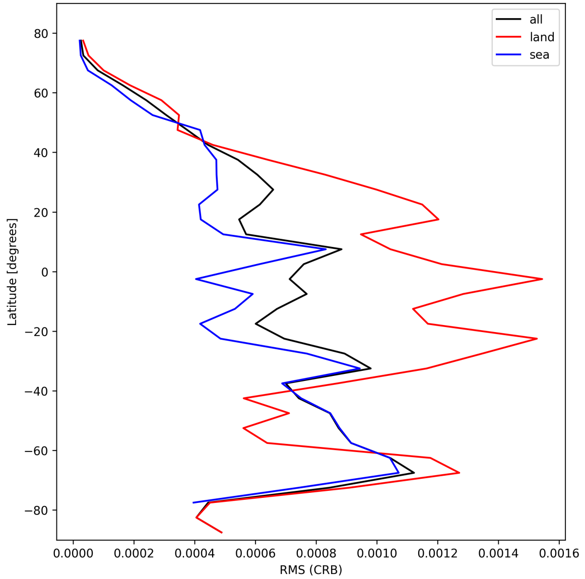
Figure 30: Zonal average of "RMS (CRB)" for 2025-10-29 to 2025-10-30.
