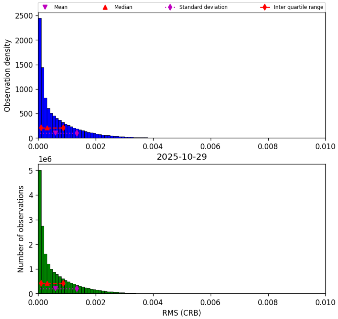
Figure 46: Histogram of “RMS (CRB)” for 2025-10-29 to 2025-10-30
