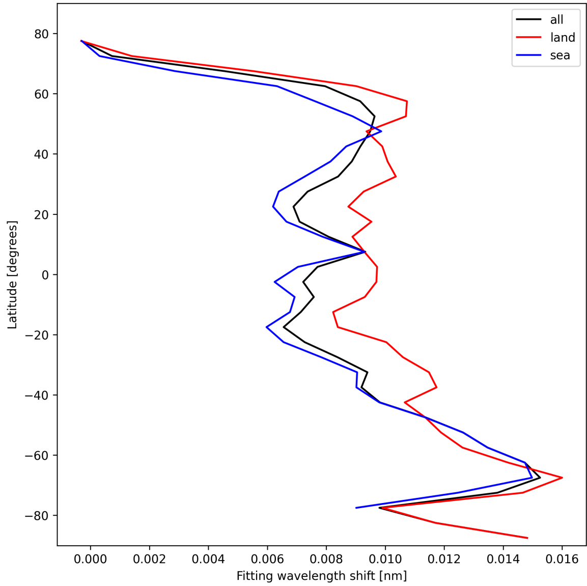
Figure 31: Zonal average of “Fitting wavelength shift” for 2025-10-29 to 2025-10-30.
