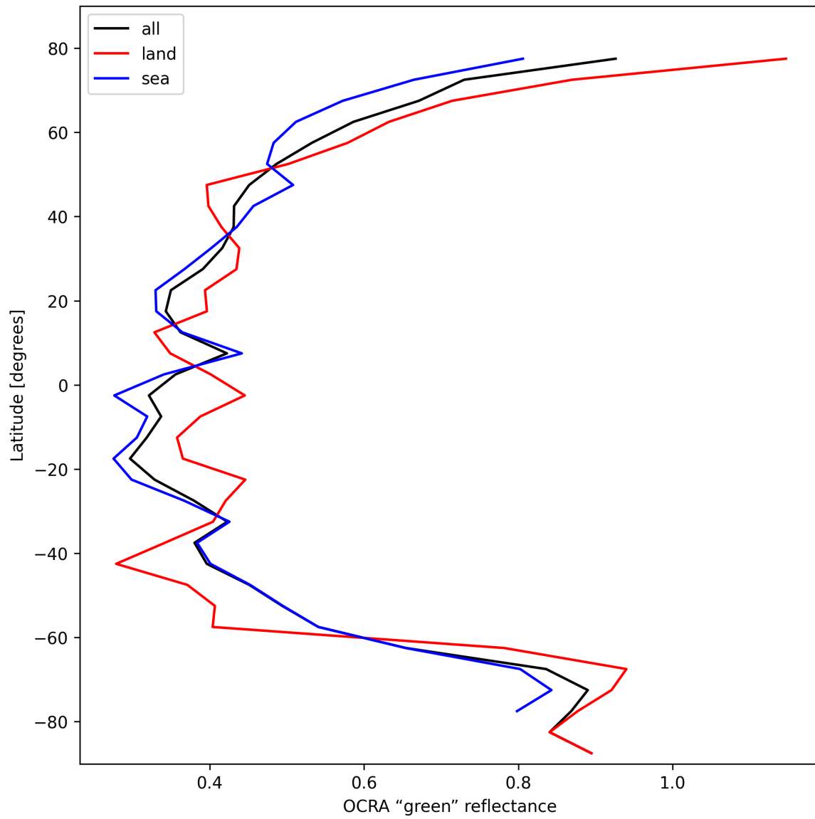
Figure 34: Zonal average of “OCRA “green” reflectance” for 2025-10-29 to 2025-10-30.
