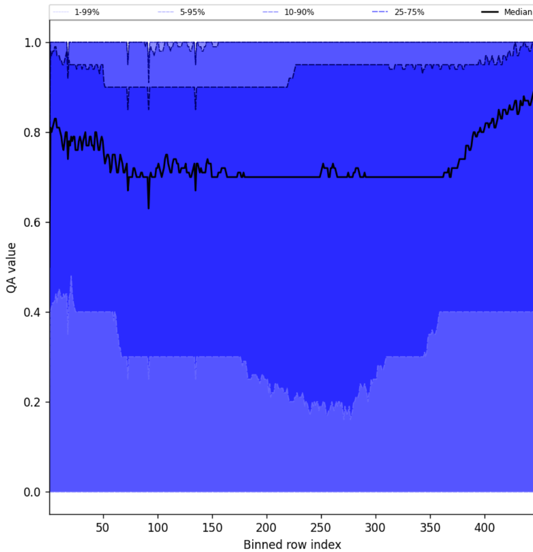
Figure 52: Along track statistics of “QA value” for 2025-10-29 to 2025-10-30
