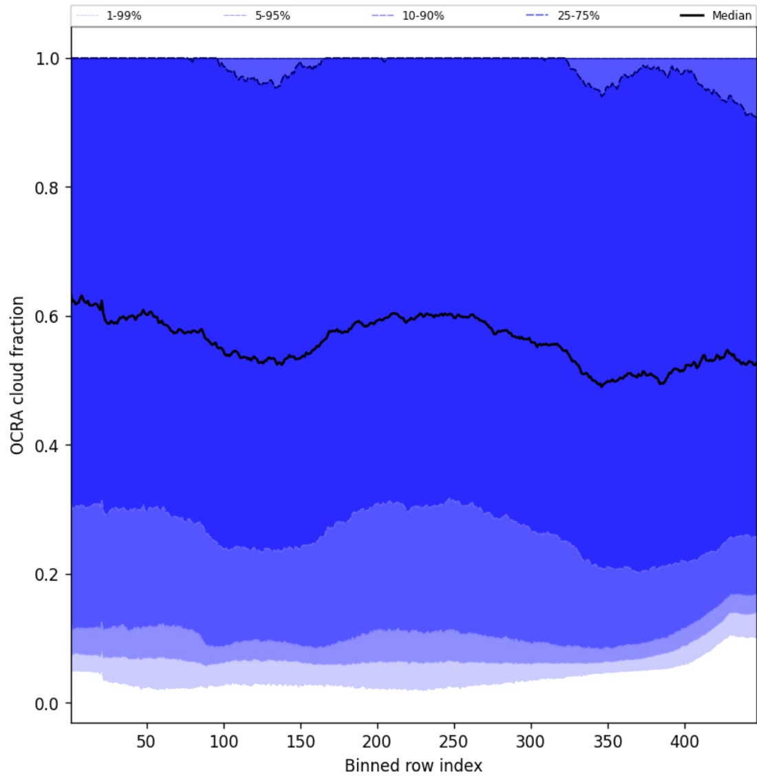
Figure 64: Along track statistics of “OCRA cloud fraction” for 2025-10-29 to 2025-10-30
