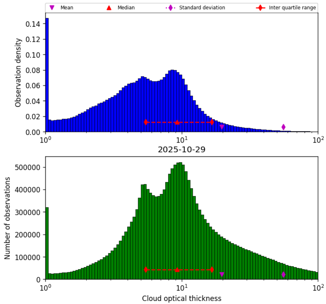
Figure 39: Histogram of “Cloud optical thickness” for 2025-10-29 to 2025-10-30
