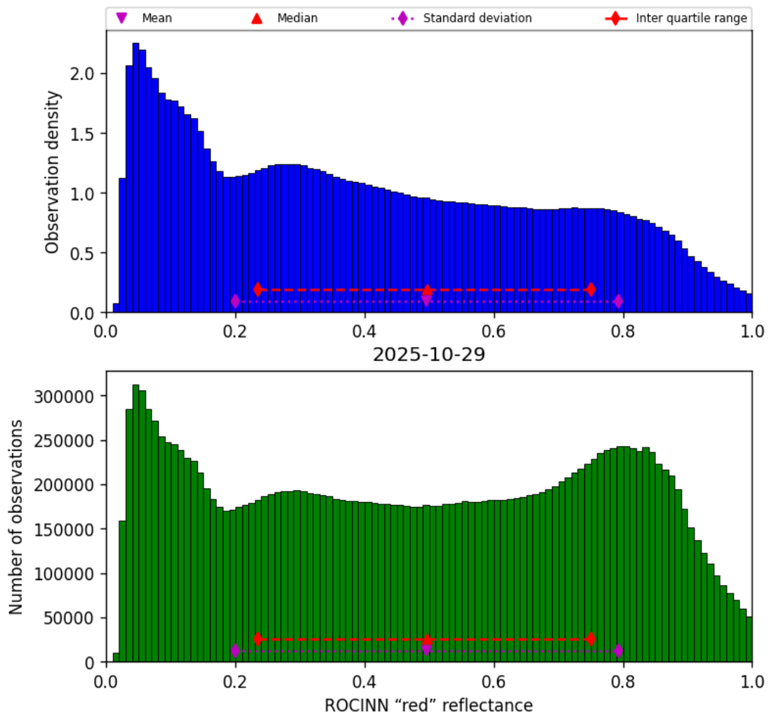
Figure 51: Histogram of “ROCINN “red” reflectance” for 2025-10-29 to 2025-10-30
