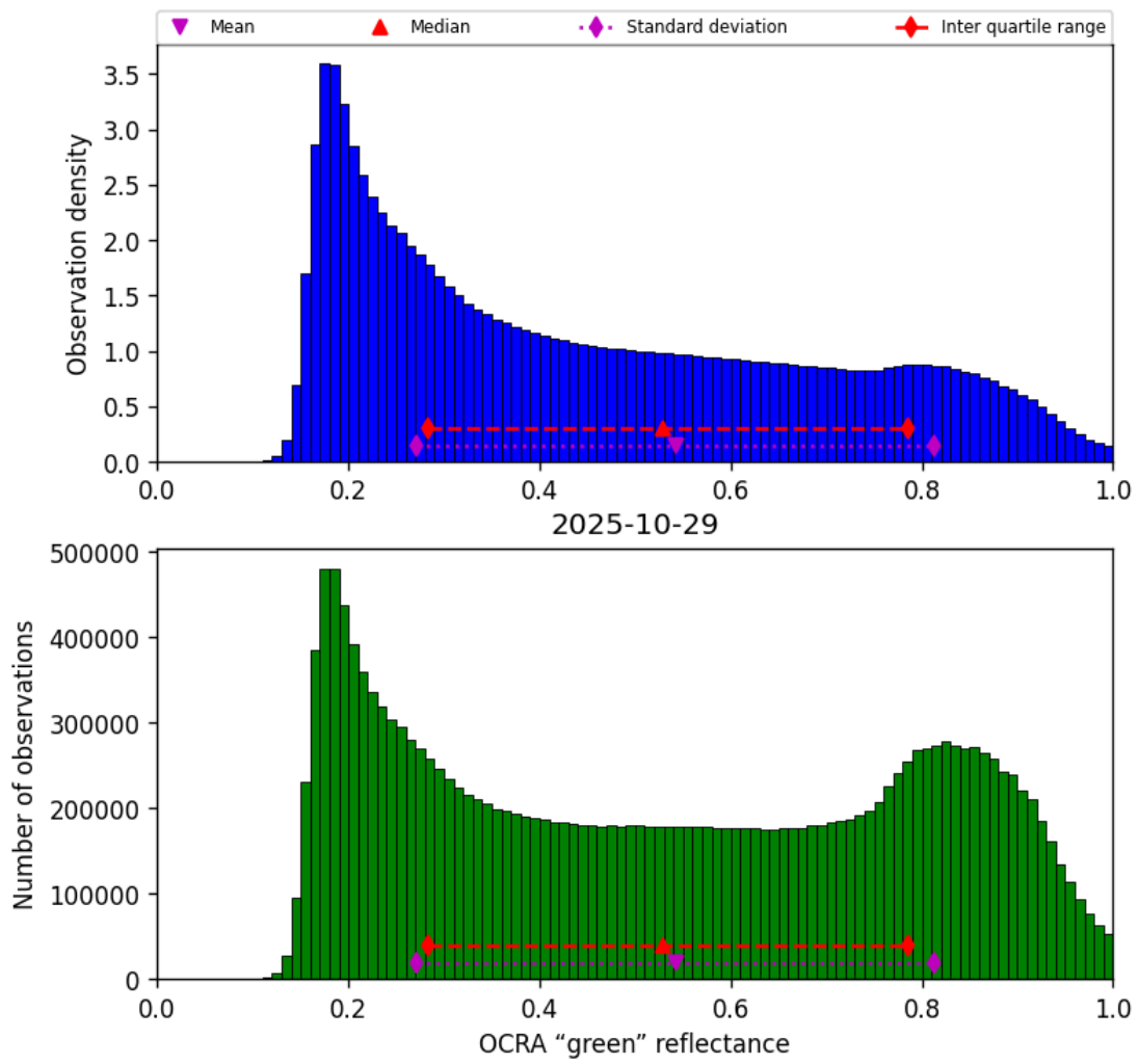
Figure 50: Histogram of “OCRA “green” reflectance” for 2025-10-29 to 2025-10-30
