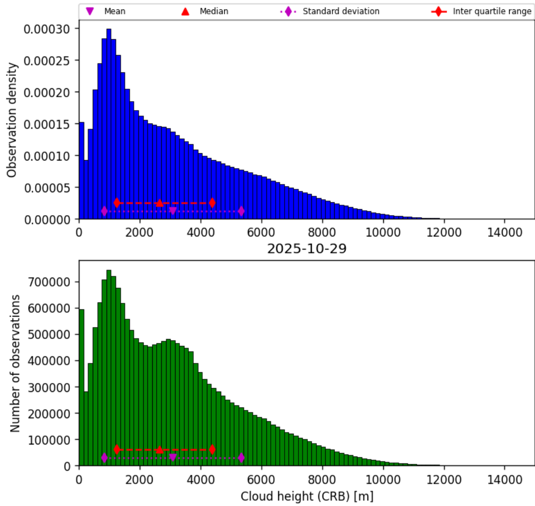
Figure 41: Histogram of “Cloud height (CRB)” for 2025-10-29 to 2025-10-30
