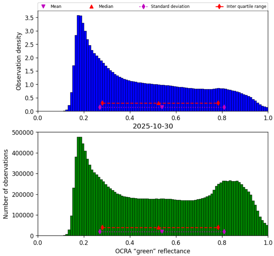
Figure 50: Histogram of “OCRA “green” reflectance” for 2025-10-30 to 2025-10-30
