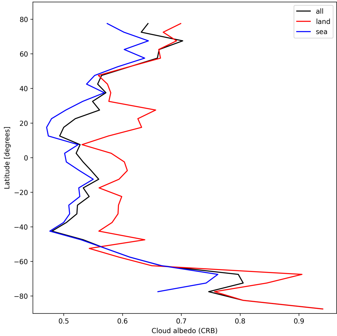
Figure 26: Zonal average of “Cloud albedo (CRB)” for 2025-10-30 to 2025-10-30.
