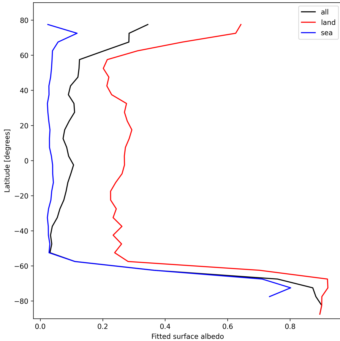
Figure 27: Zonal average of “Fitted surface albedo” for 2025-10-30 to 2025-10-30.
