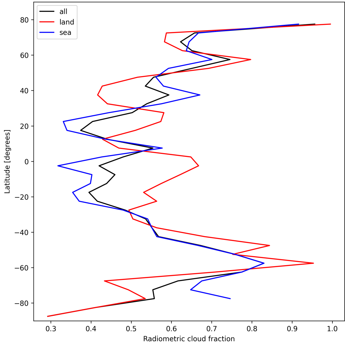
Figure 21: Zonal average of “Radiometric cloud fraction” for 2025-10-30 to 2025-10-30.
