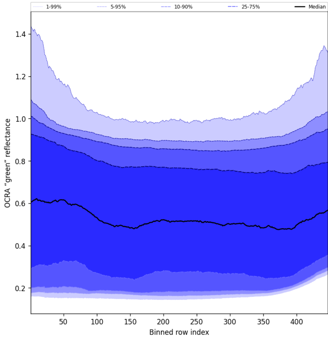
Figure 66: Along track statistics of “OCRA “green” reflectance” for 2025-10-30 to 2025-10-30
