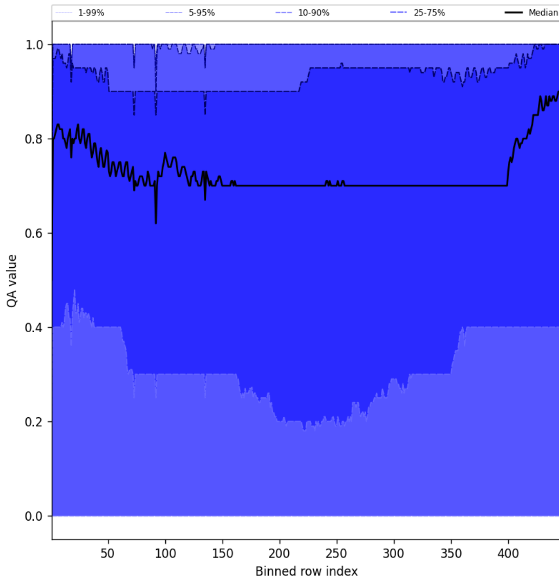
Figure 52: Along track statistics of “QA value” for 2025-10-30 to 2025-10-30
