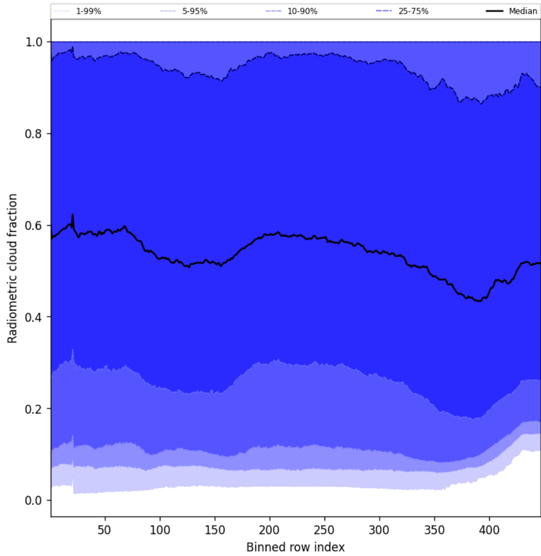
Figure 53: Along track statistics of “Radiometric cloud fraction” for 2025-10-30 to 2025-10-30
