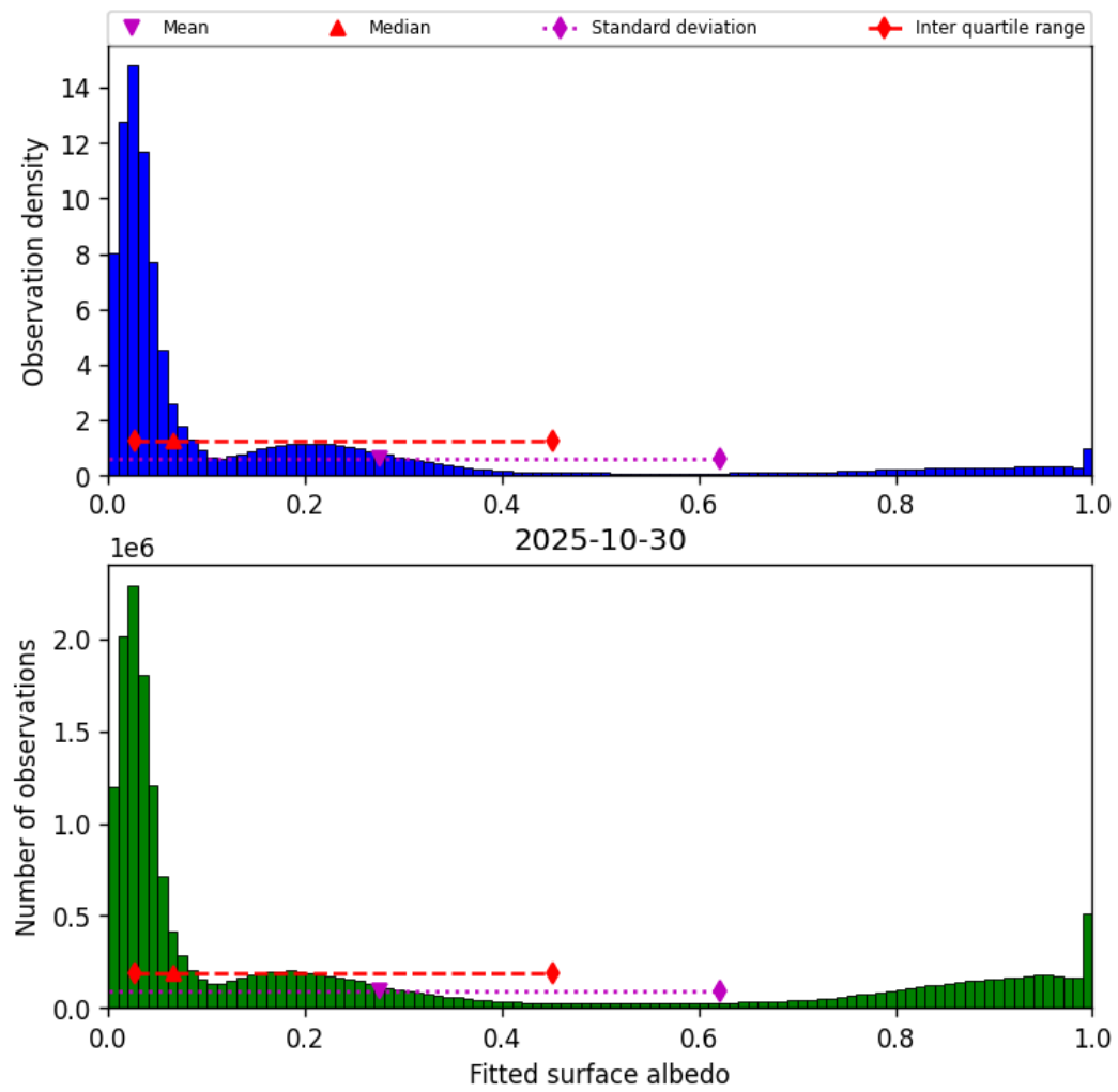
Figure 43: Histogram of “Fitted surface albedo” for 2025-10-30 to 2025-10-30
