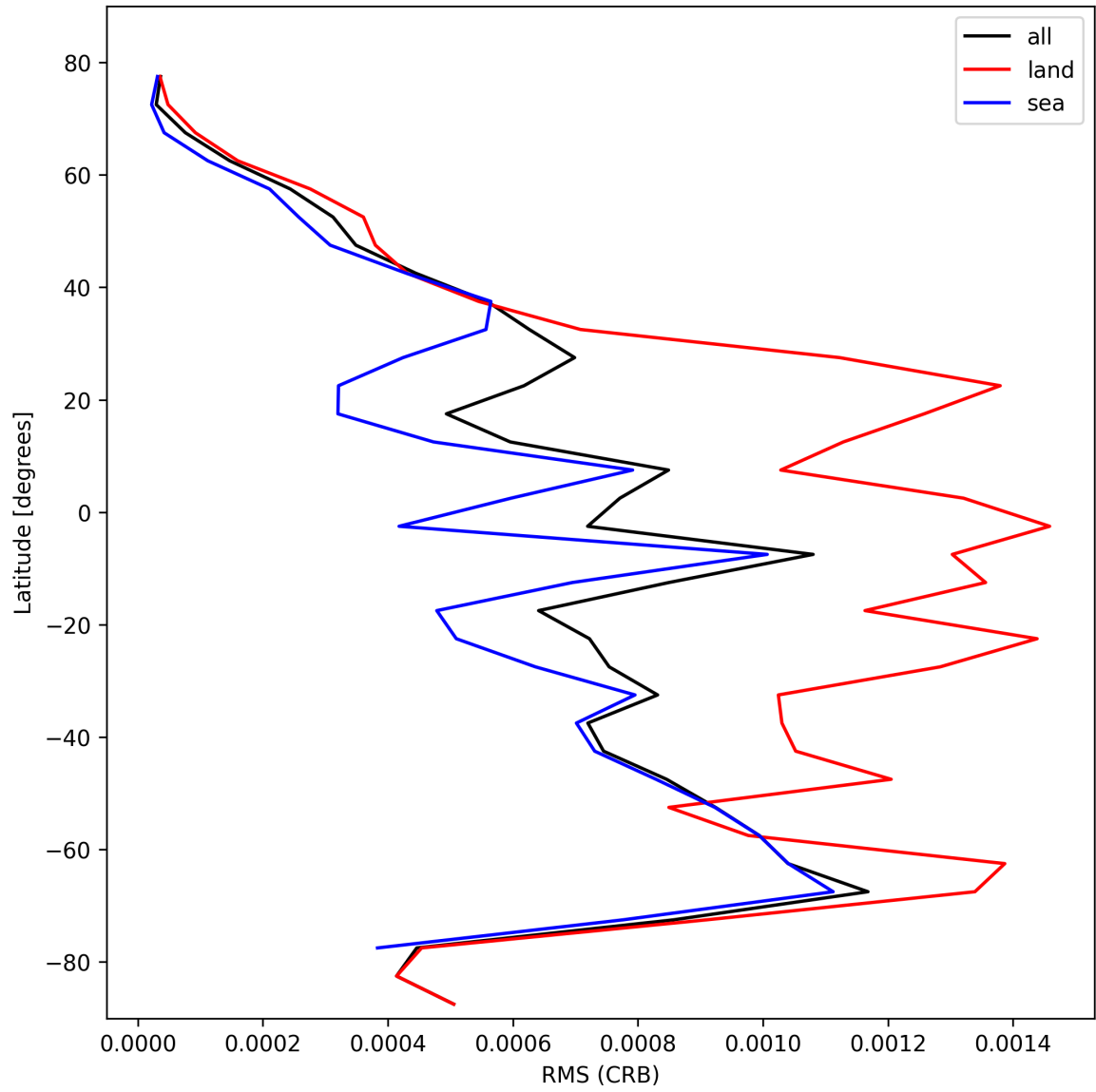
Figure 30: Zonal average of “RMS (CRB)” for 2025-10-30 to 2025-10-30.
