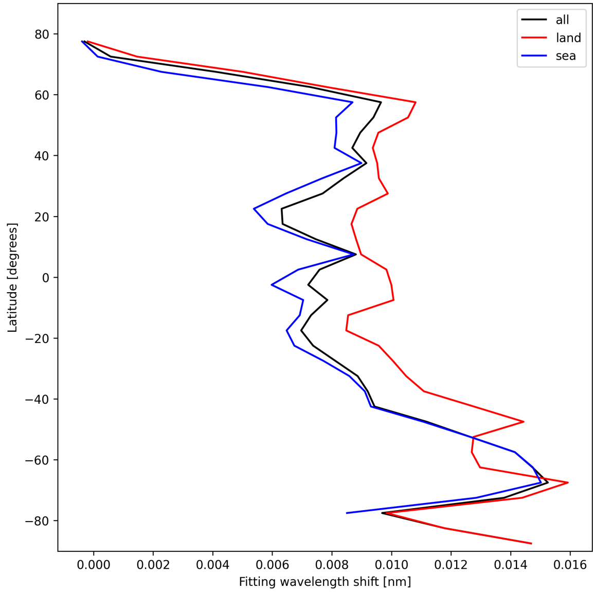
Figure 31: Zonal average of “Fitting wavelength shift” for 2025-10-30 to 2025-10-30.
