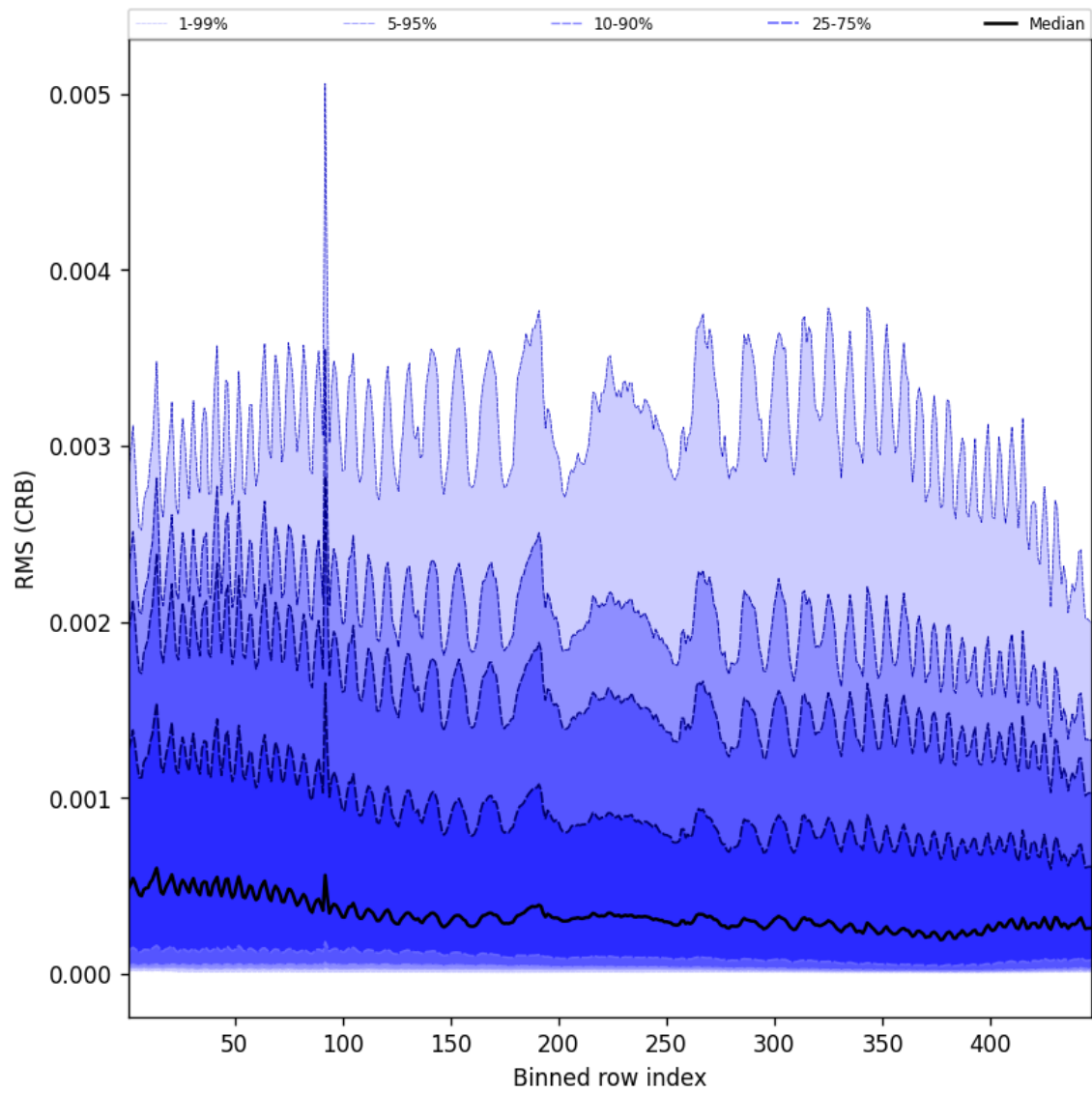
Figure 62: Along track statistics of “RMS (CRB)” for 2025-10-30 to 2025-10-30
