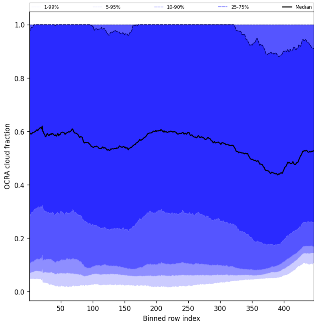
Figure 64: Along track statistics of “OCRA cloud fraction” for 2025-10-30 to 2025-10-30
