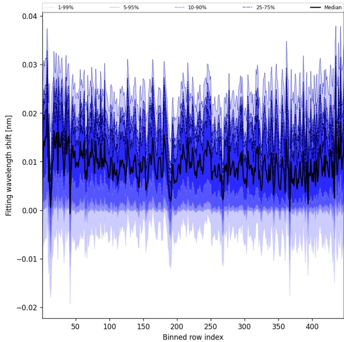
Figure 63: Along track statistics of “Fitting wavelength shift” for 2025-10-30 to 2025-10-30
