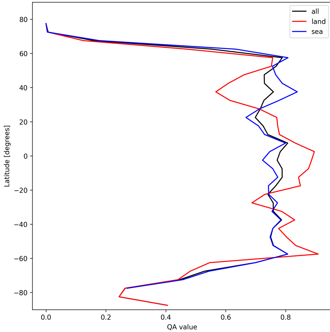
Figure 20: Zonal average of “QA value” for 2025-10-30 to 2025-10-30.
