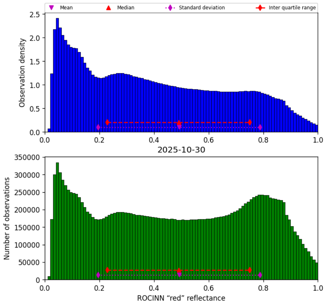
Figure 51: Histogram of “ROCINN “red” reflectance” for 2025-10-30 to 2025-10-30
