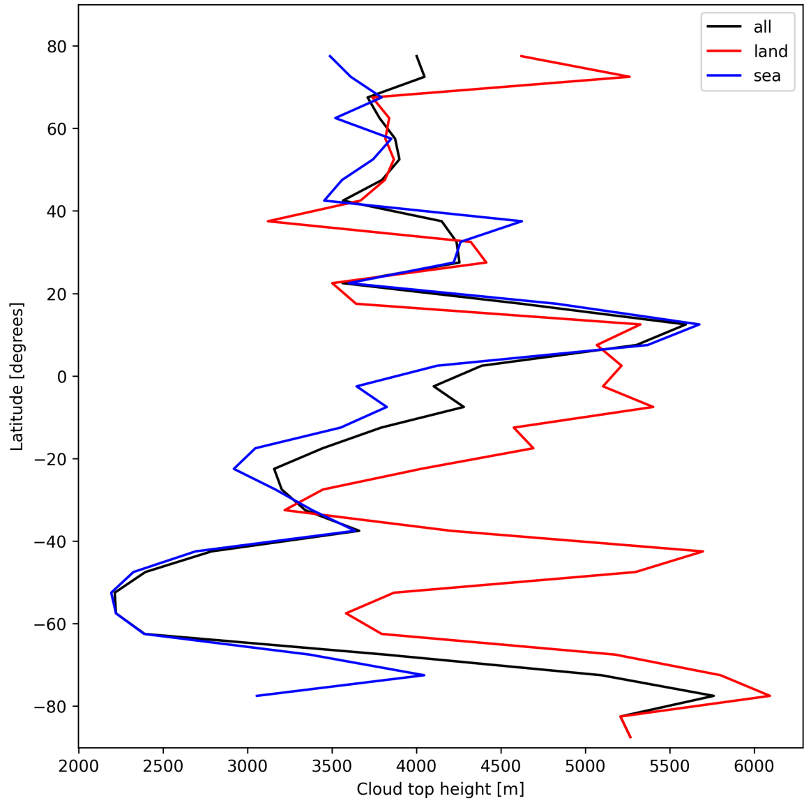
Figure 22: Zonal average of “Cloud top height” for 2025-10-30 to 2025-10-30.
