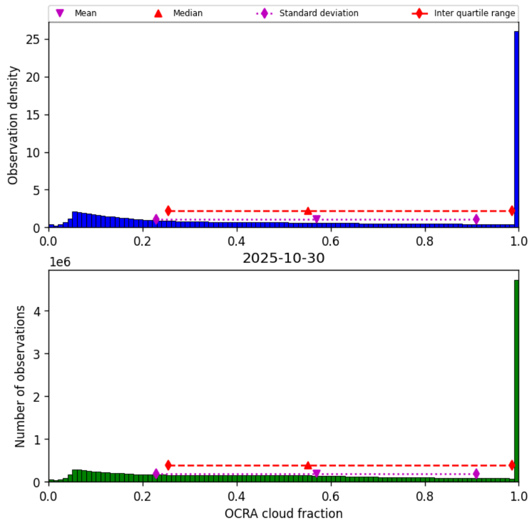
Figure 48: Histogram of “OCRA cloud fraction” for 2025-10-30 to 2025-10-30
