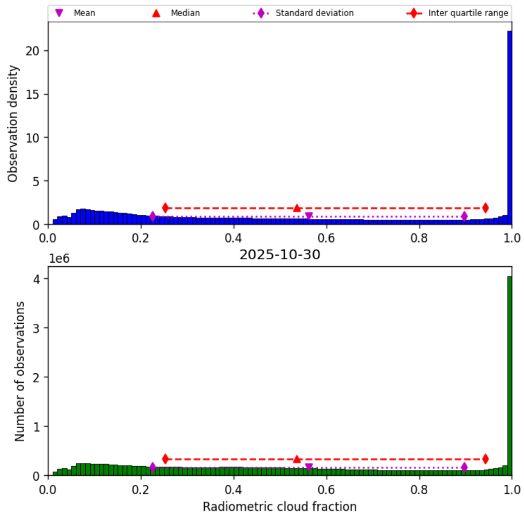
Figure 37: Histogram of “Radiometric cloud fraction” for 2025-10-30 to 2025-10-30
