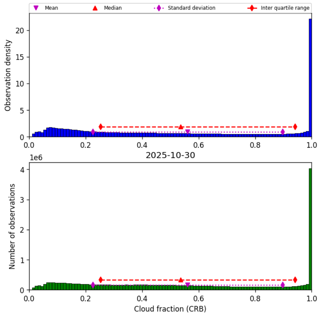
Figure 40: Histogram of “Cloud fraction (CRB)” for 2025-10-30 to 2025-10-30
