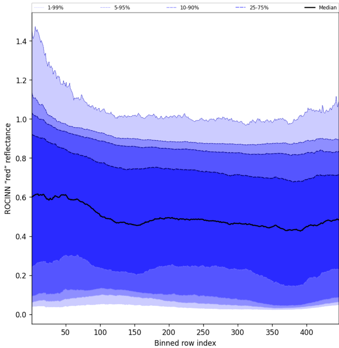
Figure 67: Along track statistics of “ROCINN “red” reflectance” for 2025-10-30 to 2025-10-30
