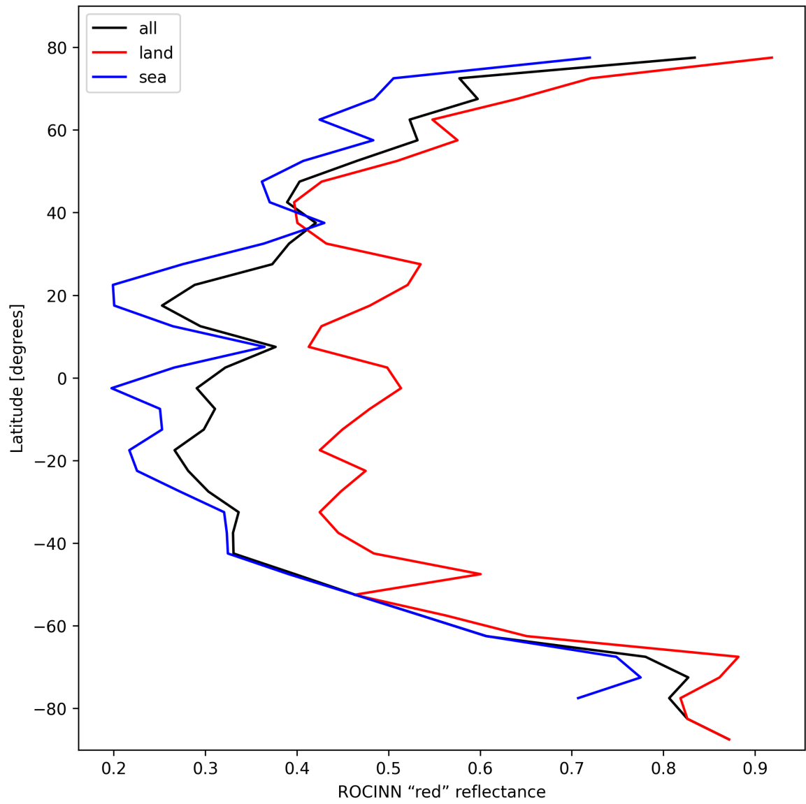
Figure 35: Zonal average of “ROCINN “red” reflectance” for 2025-10-30 to 2025-10-30.
