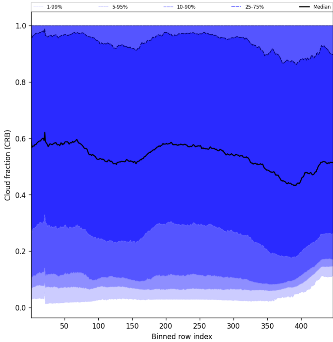
Figure 56: Along track statistics of “Cloud fraction (CRB)” for 2025-10-30 to 2025-10-30
