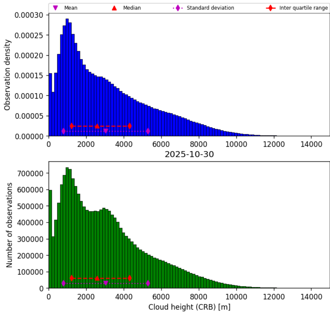
Figure 41: Histogram of “Cloud height (CRB)” for 2025-10-30 to 2025-10-30
