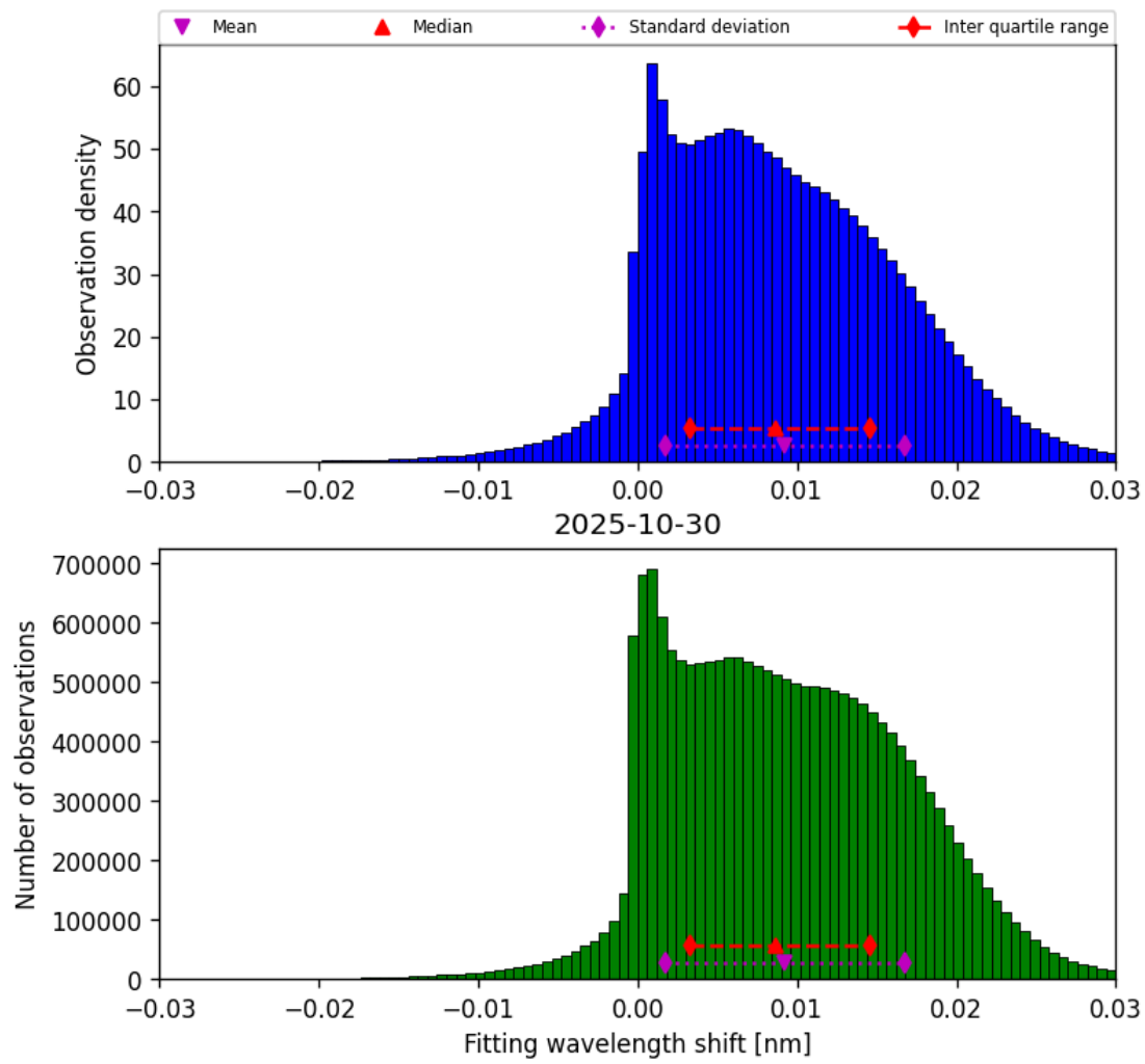
Figure 47: Histogram of “Fitting wavelength shift” for 2025-10-30 to 2025-10-30
