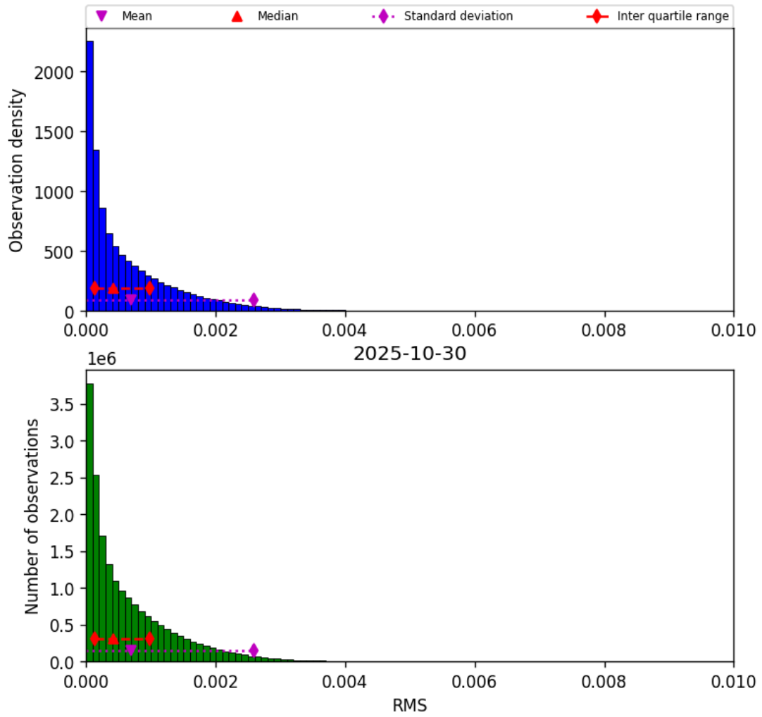
Figure 45: Histogram of “RMS” for 2025-10-30 to 2025-10-30
