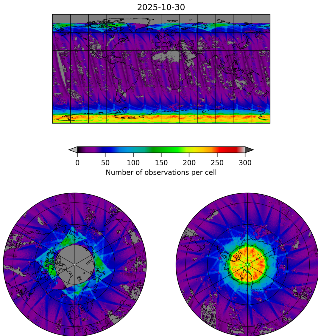
Figure 19: Map of the number of observations for 2025-10-30 to 2025-10-30
