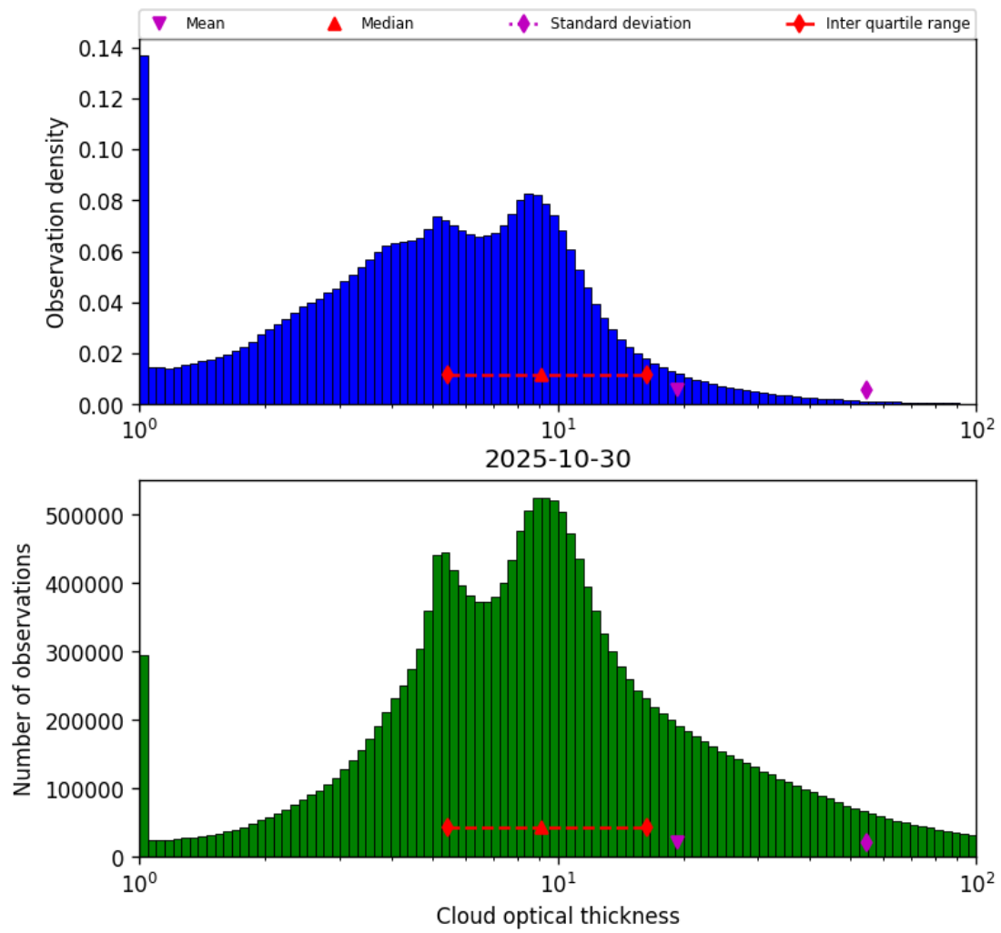
Figure 39: Histogram of “Cloud optical thickness” for 2025-10-30 to 2025-10-30
