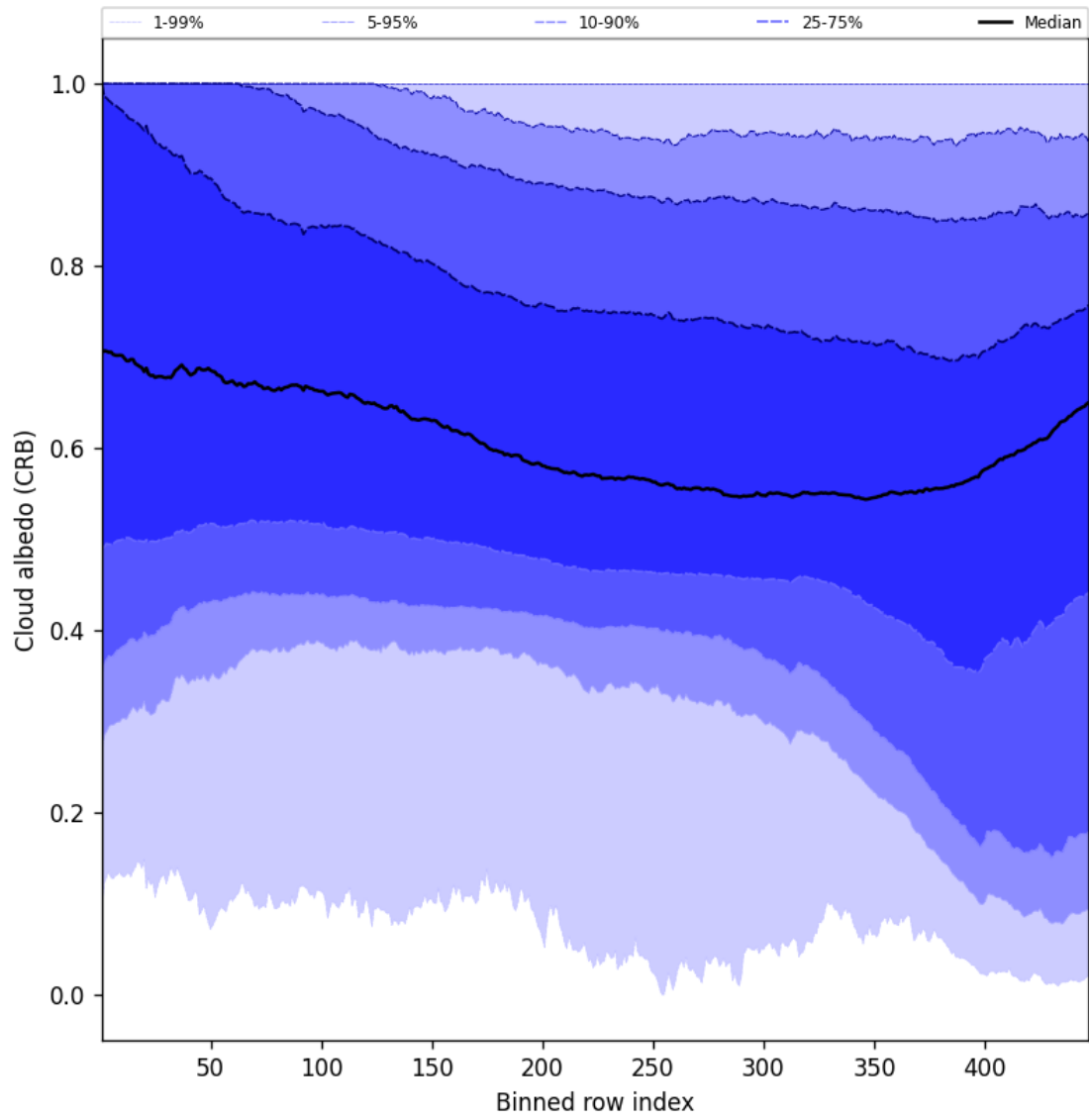
Figure 58: Along track statistics of “Cloud albedo (CRB)” for 2025-10-30 to 2025-10-30
