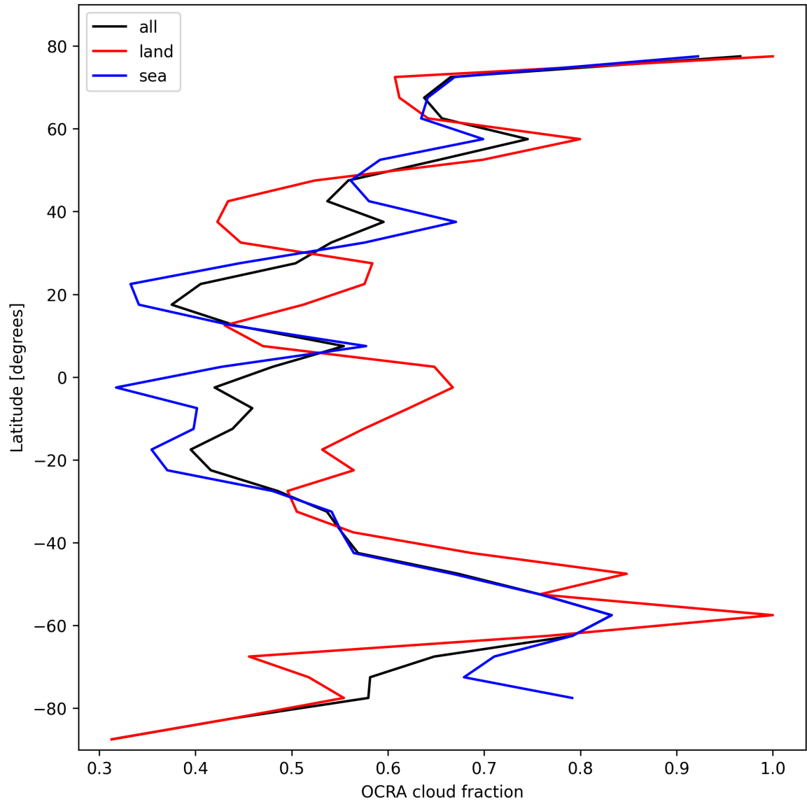
Figure 32: Zonal average of “OCRA cloud fraction” for 2025-10-30 to 2025-10-30.
