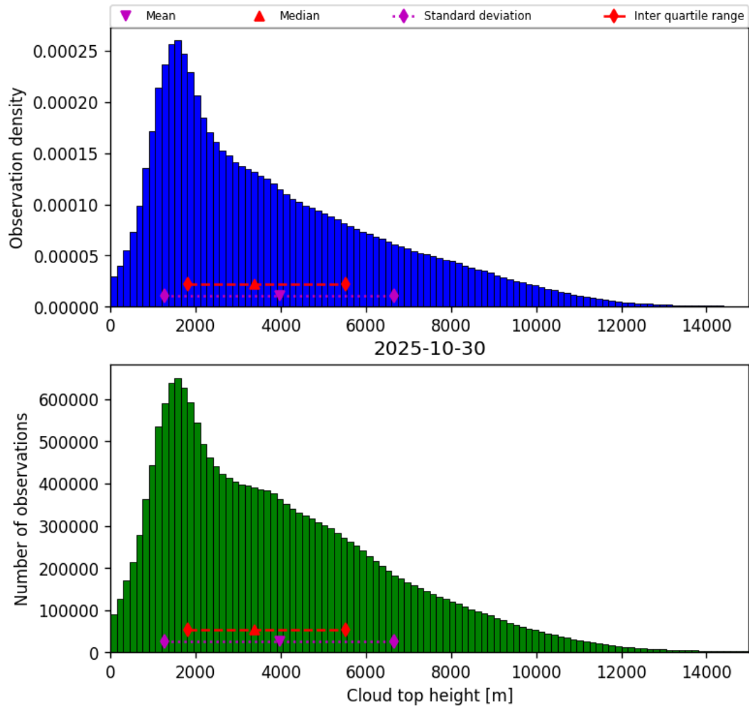
Figure 38: Histogram of “Cloud top height” for 2025-10-30 to 2025-10-30
