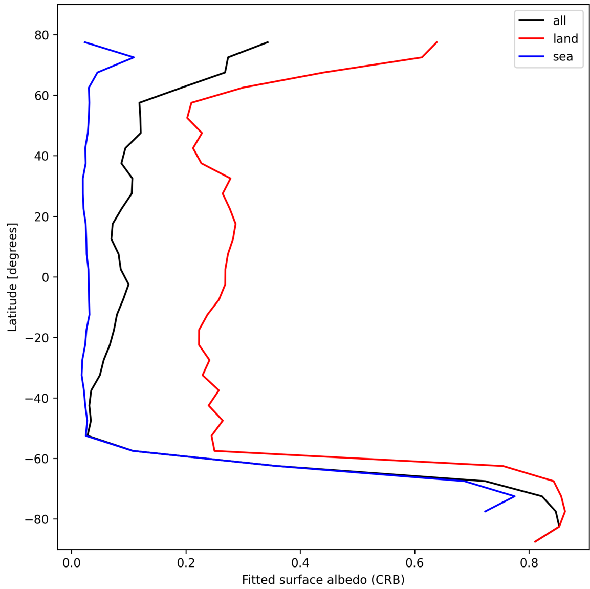
Figure 28: Zonal average of “Fitted surface albedo (CRB)” for 2025-10-30 to 2025-10-30.
