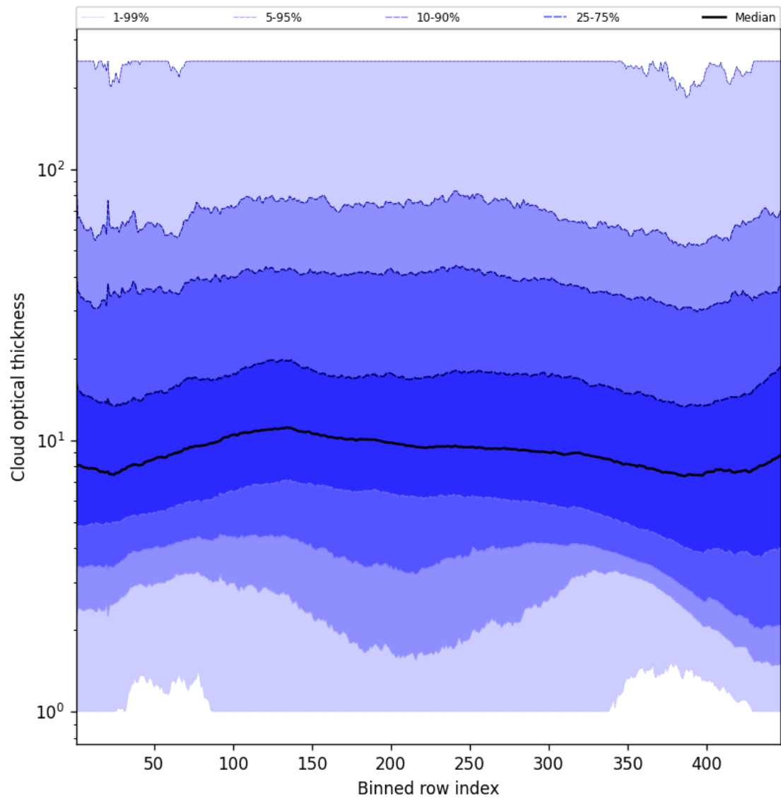
Figure 55: Along track statistics of “Cloud optical thickness” for 2025-10-30 to 2025-10-30
