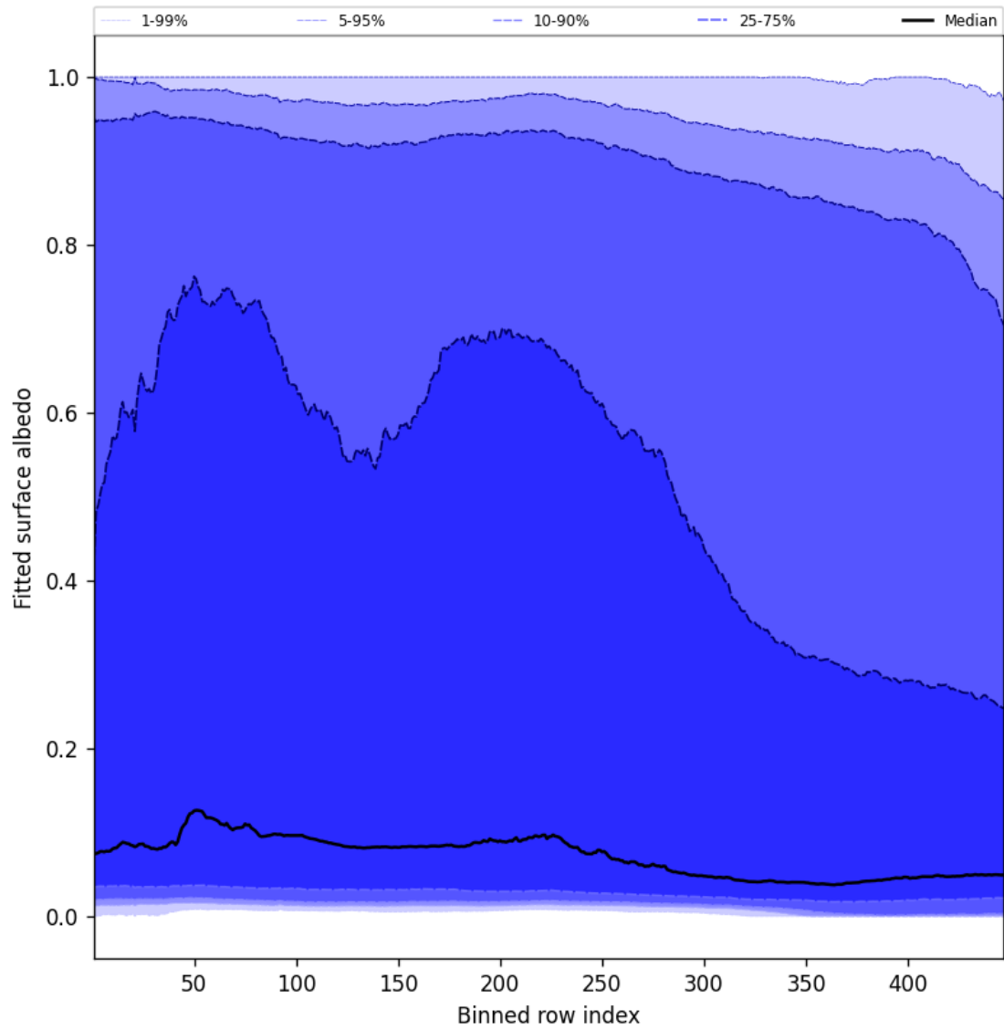
Figure 59: Along track statistics of “Fitted surface albedo” for 2025-10-30 to 2025-10-30
