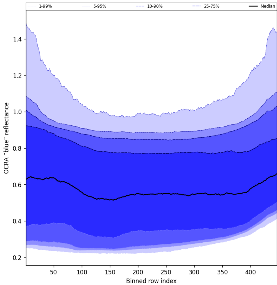
Figure 65: Along track statistics of “OCRA “blue” reflectance” for 2025-10-30 to 2025-10-30
