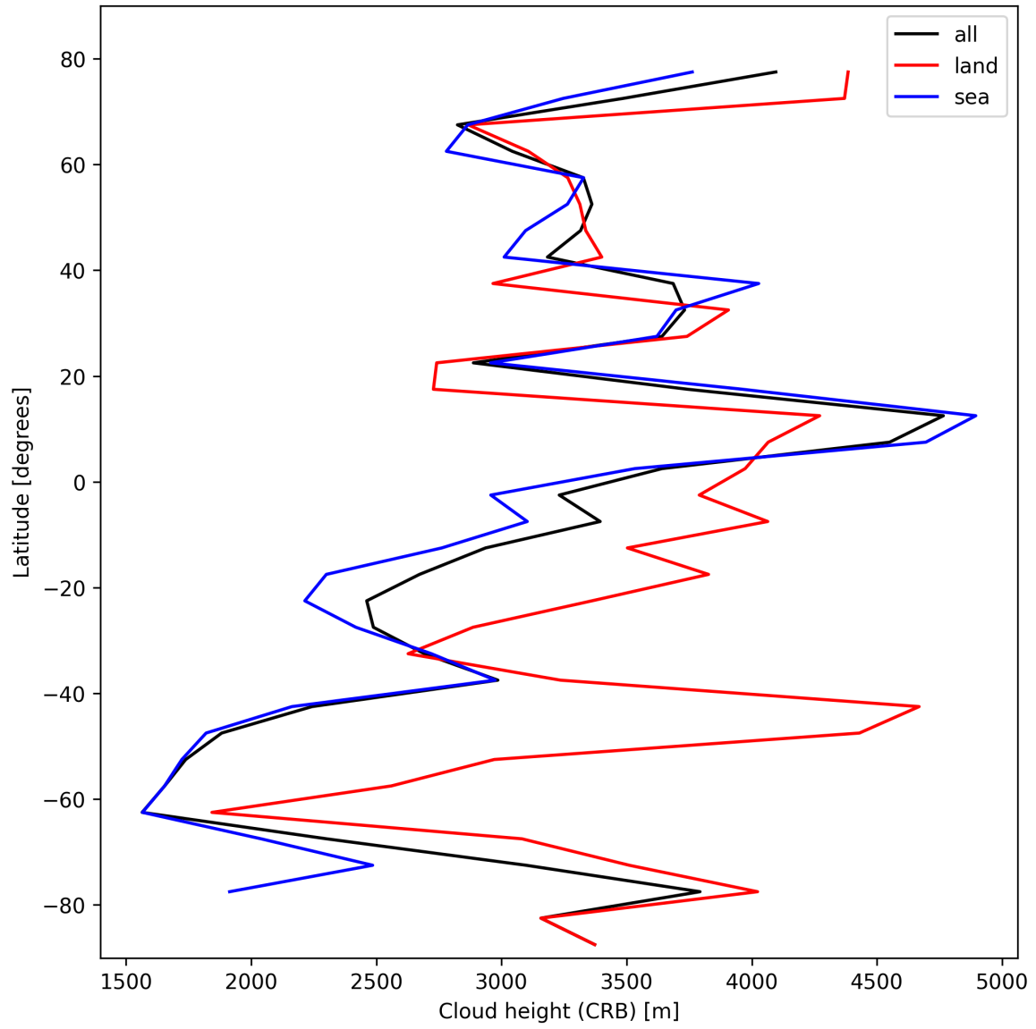
Figure 25: Zonal average of “Cloud height (CRB)” for 2025-10-30 to 2025-10-30.
