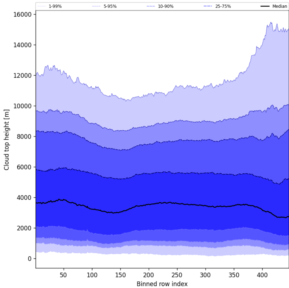
Figure 54: Along track statistics of “Cloud top height” for 2025-10-30 to 2025-10-30
