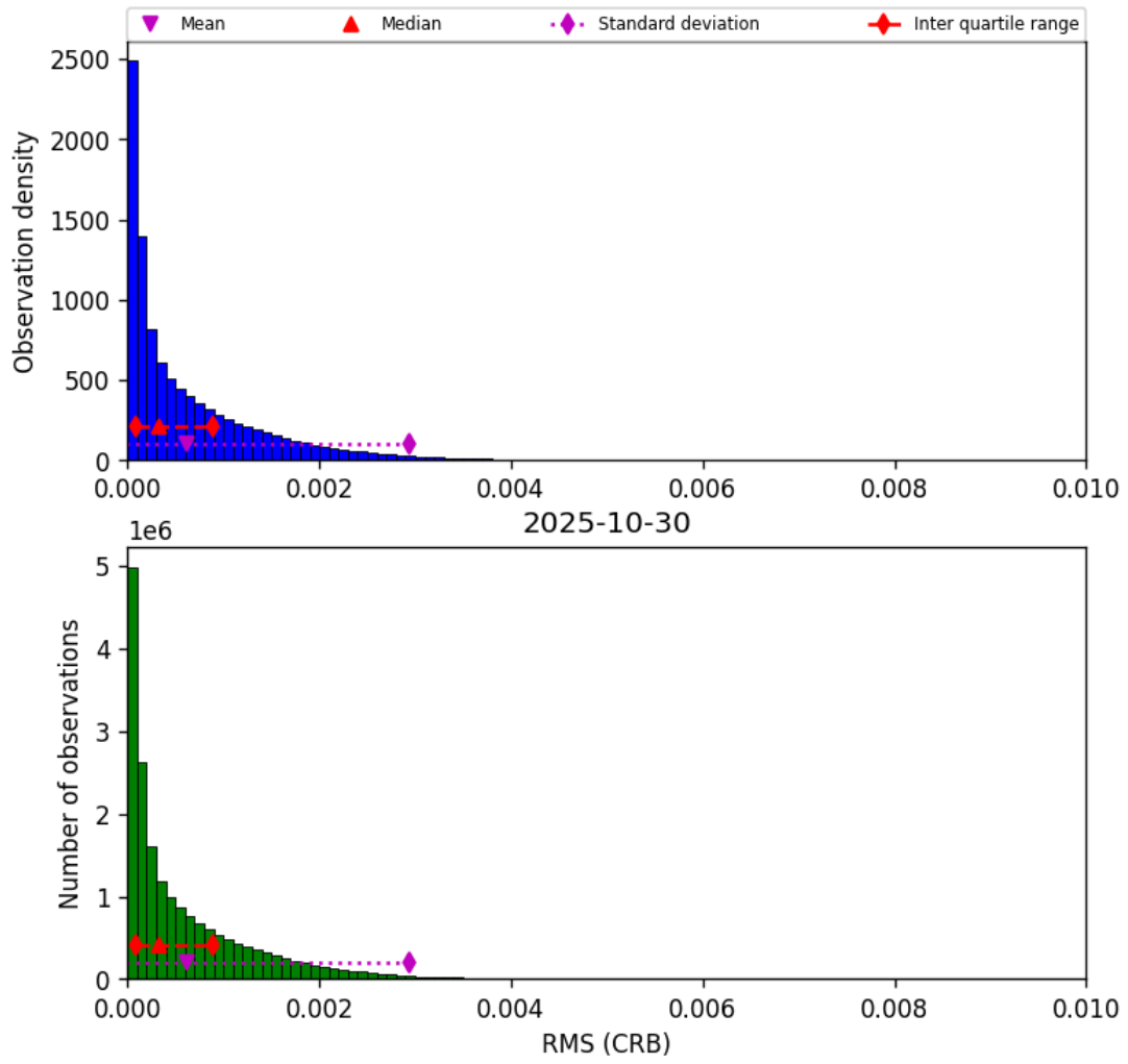
Figure 46: Histogram of “RMS (CRB)” for 2025-10-30 to 2025-10-30
