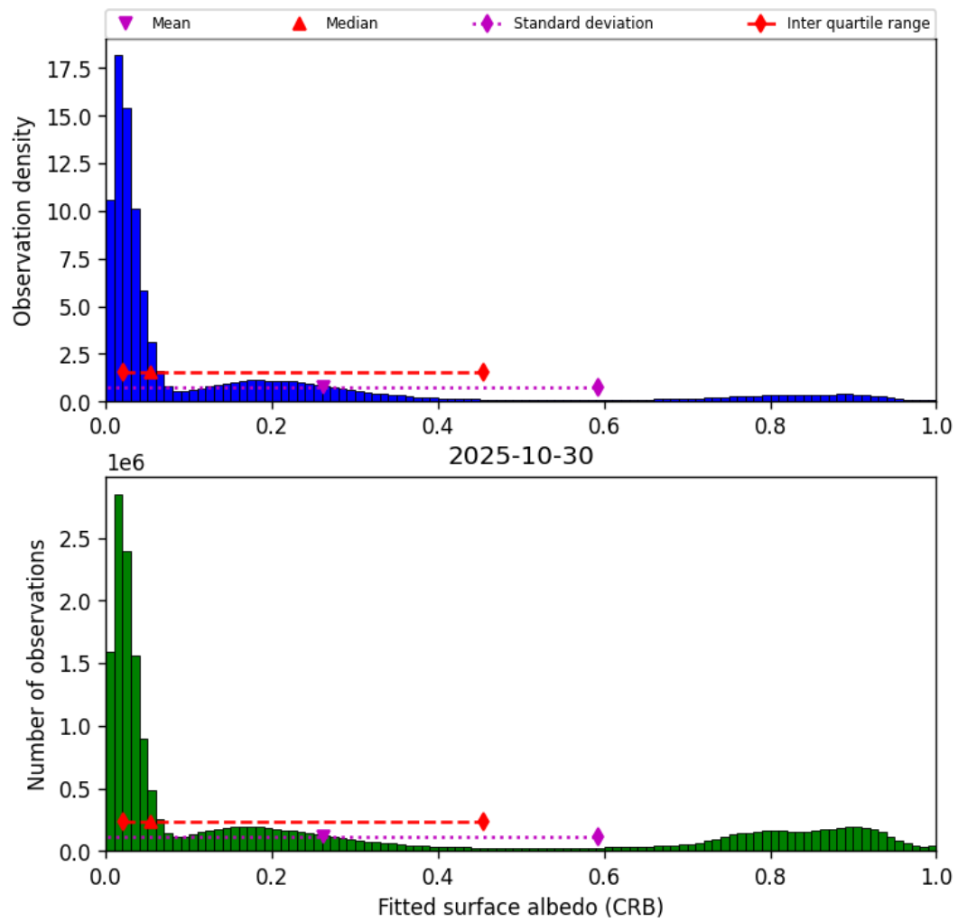
Figure 44: Histogram of “Fitted surface albedo (CRB)” for 2025-10-30 to 2025-10-30
