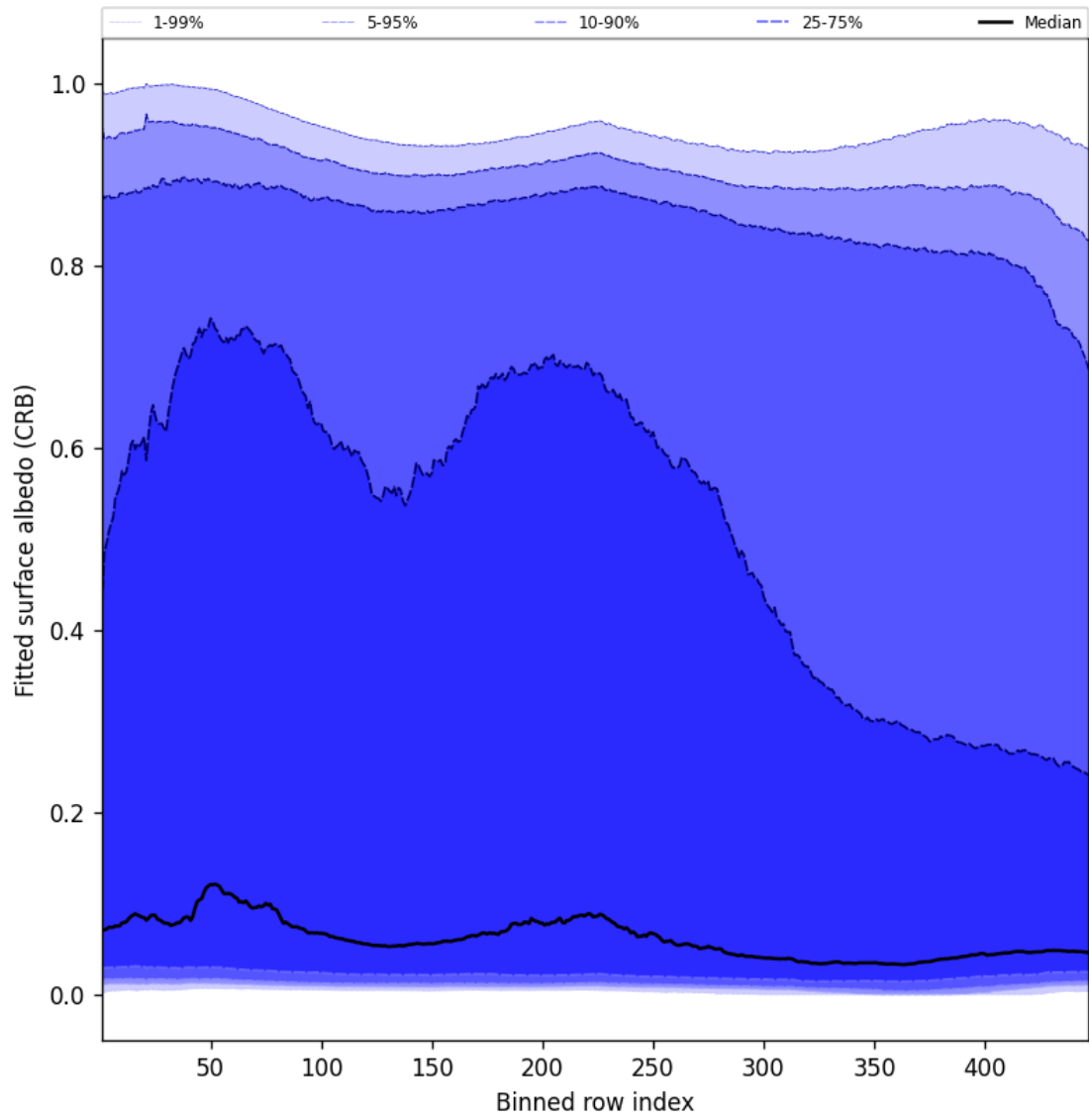
Figure 60: Along track statistics of “Fitted surface albedo (CRB)” for 2025-10-30 to 2025-10-30
