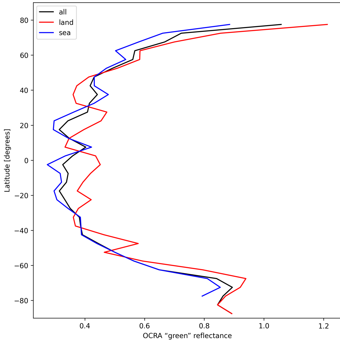
Figure 34: Zonal average of “OCRA “green” reflectance” for 2025-10-30 to 2025-10-30.
