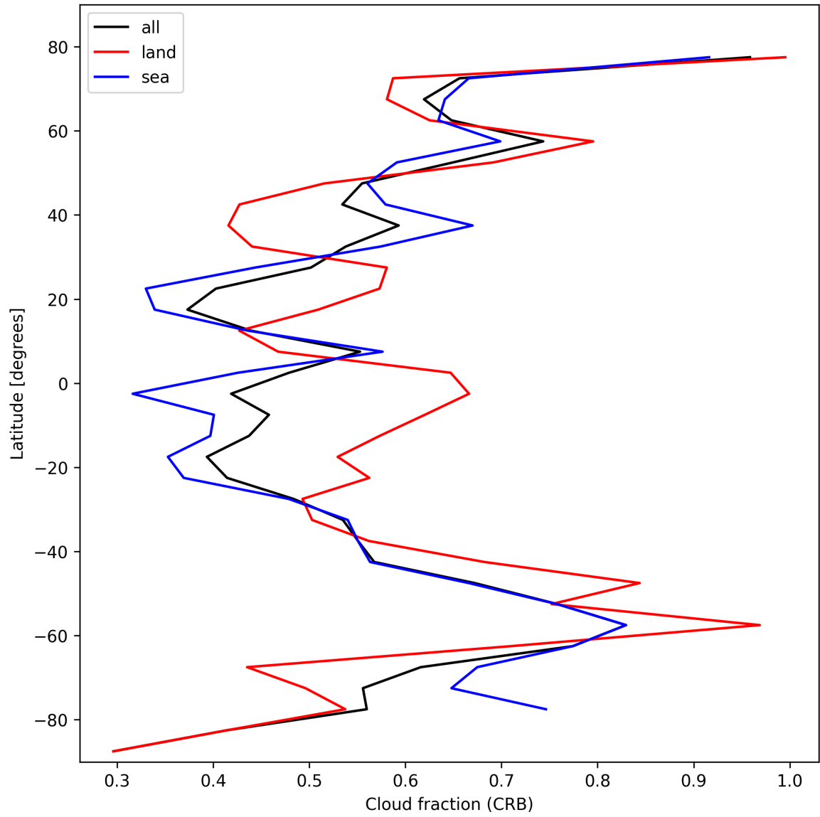
Figure 24: Zonal average of “Cloud fraction (CRB)” for 2025-10-30 to 2025-10-30.
