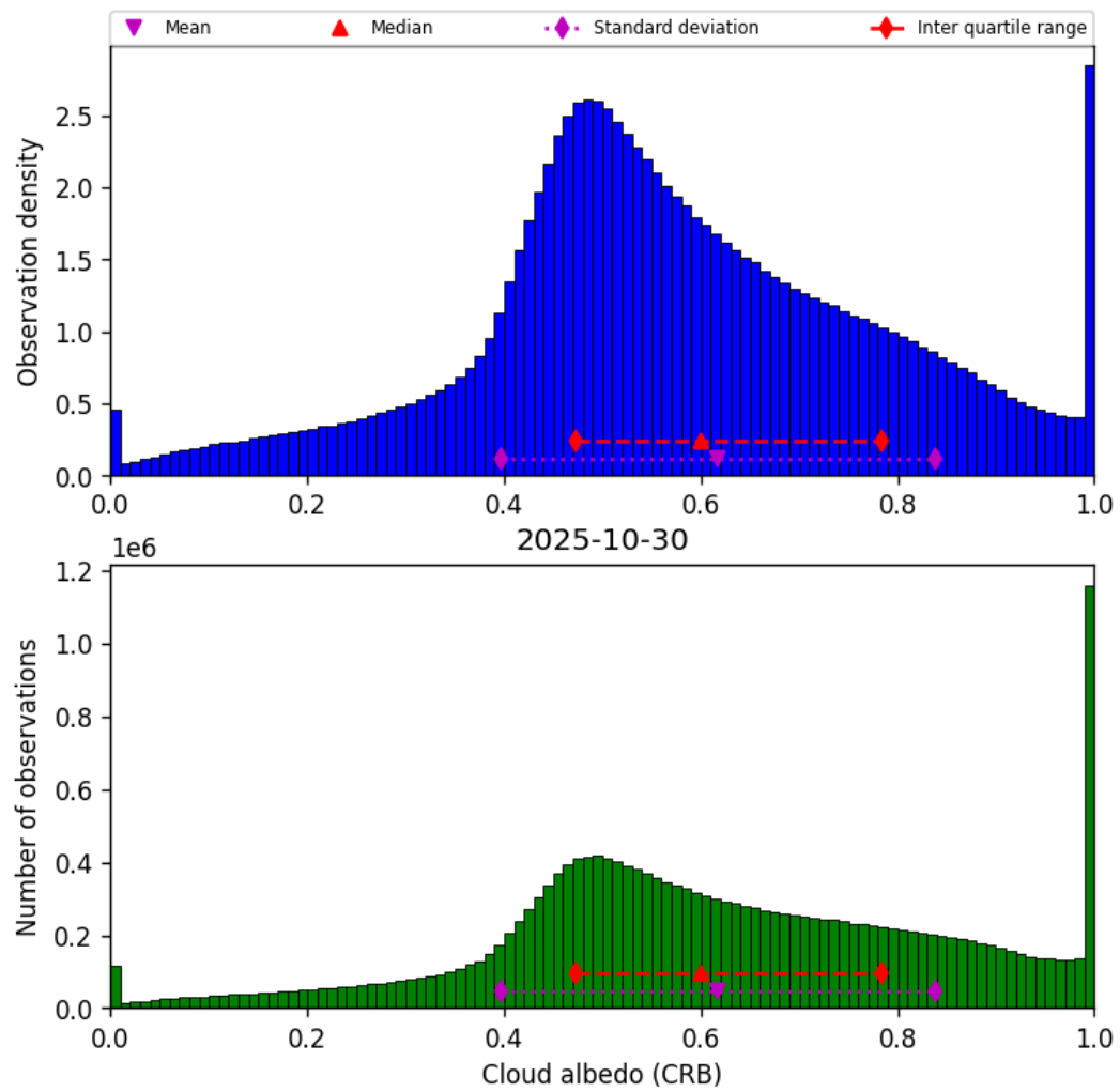
Figure 42: Histogram of “Cloud albedo (CRB)” for 2025-10-30 to 2025-10-30
