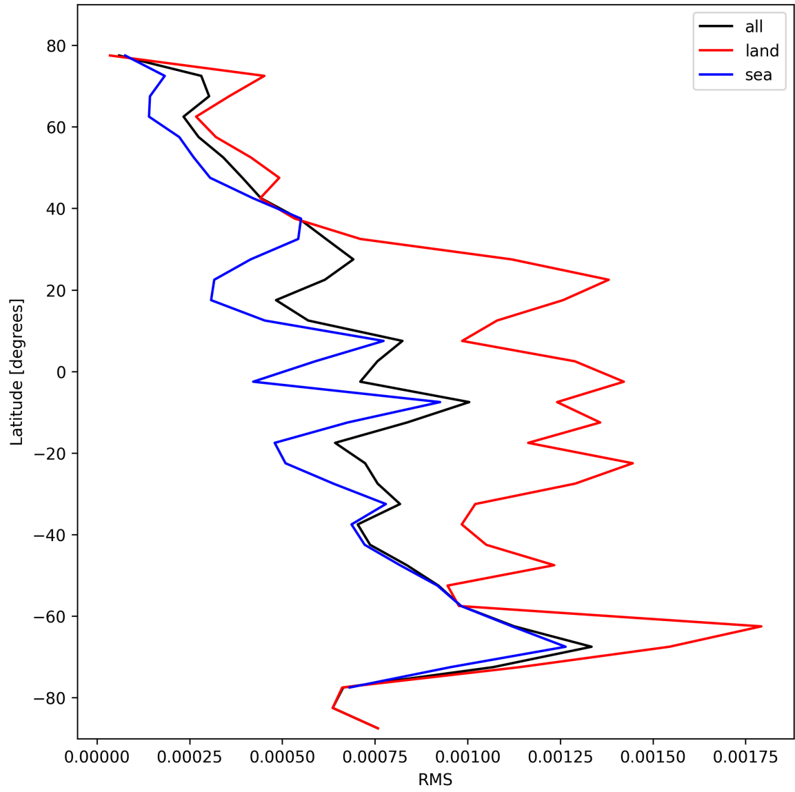
Figure 29: Zonal average of “RMS” for 2025-10-30 to 2025-10-30.
