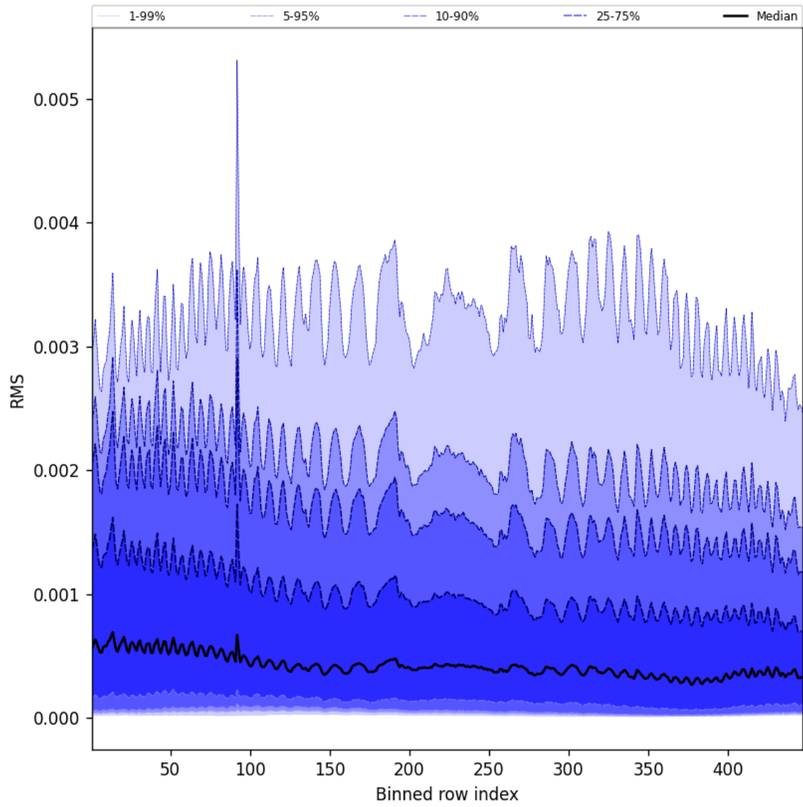
Figure 61: Along track statistics of “RMS” for 2025-10-30 to 2025-10-30
