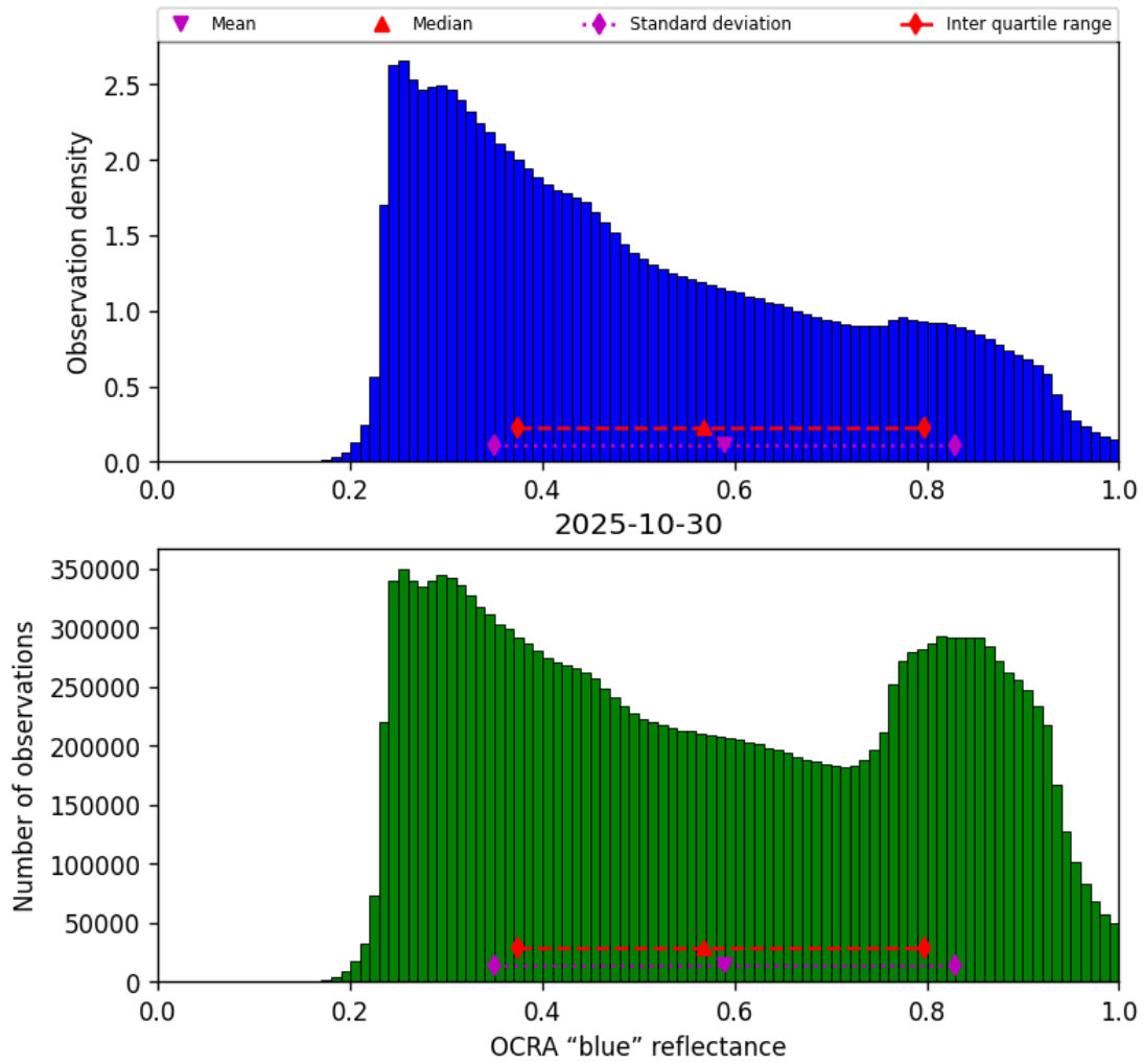
Figure 49: Histogram of “OCRA “blue” reflectance” for 2025-10-30 to 2025-10-30
