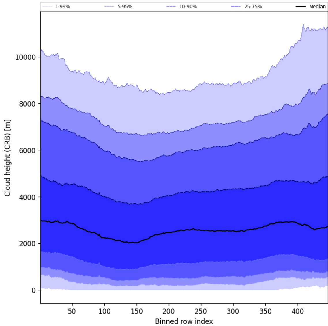
Figure 57: Along track statistics of “Cloud height (CRB)” for 2025-10-30 to 2025-10-30
