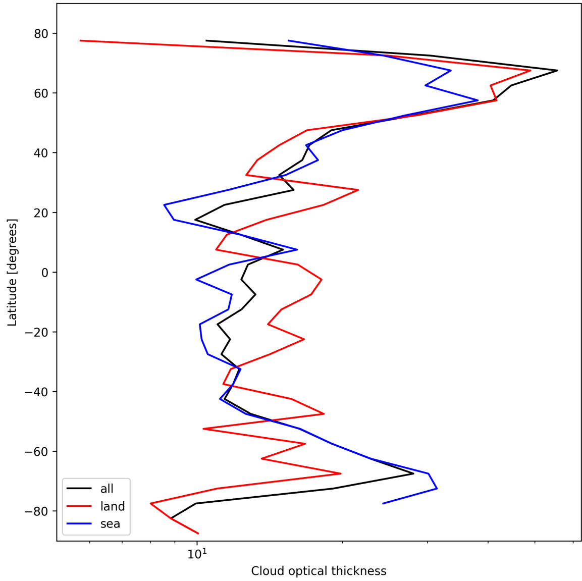
Figure 23: Zonal average of “Cloud optical thickness” for 2025-10-30 to 2025-10-30.
