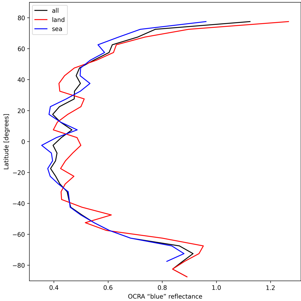
Figure 33: Zonal average of “OCRA “blue” reflectance” for 2025-10-30 to 2025-10-30.
