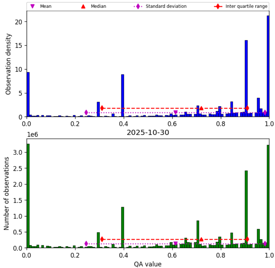
Figure 36: Histogram of “QA value” for 2025-10-30 to 2025-10-30
