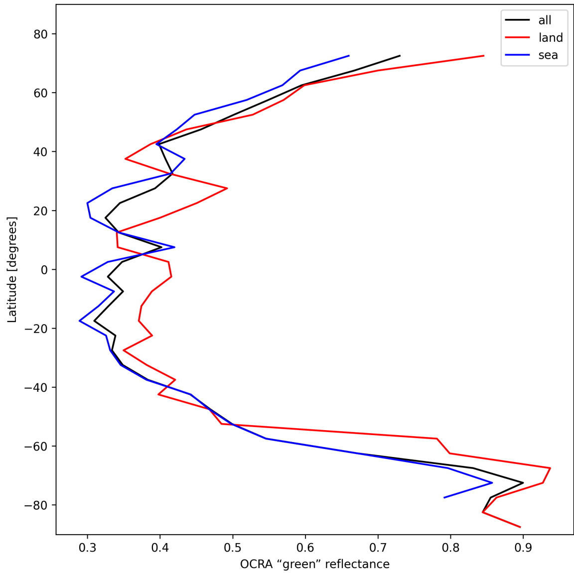
Figure 34: Zonal average of “OCRA “green” reflectance” for 2025-10-31 to 2025-10-31.
