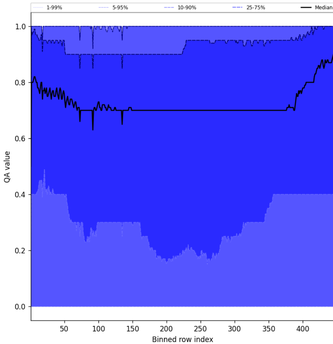
Figure 52: Along track statistics of “QA value” for 2025-10-31 to 2025-10-31
