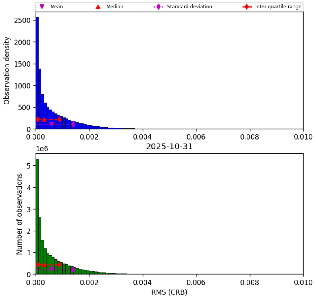
Figure 46: Histogram of “RMS (CRB)” for 2025-10-31 to 2025-10-31
