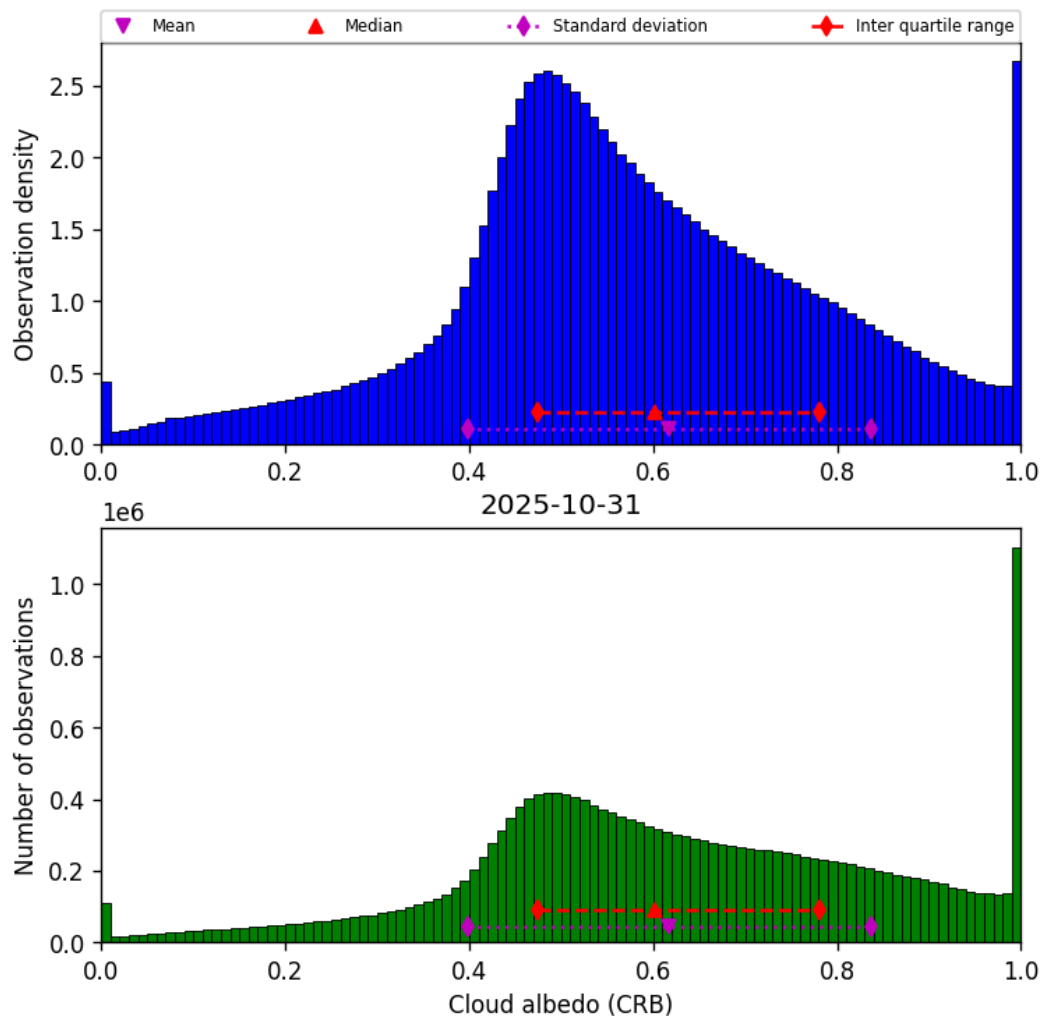
Figure 42: Histogram of “Cloud albedo (CRB)” for 2025-10-31 to 2025-10-31
