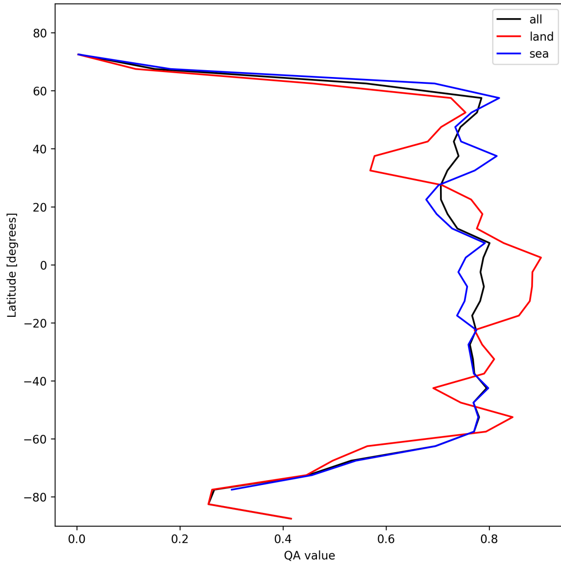
Figure 20: Zonal average of “QA value” for 2025-10-31 to 2025-10-31.
