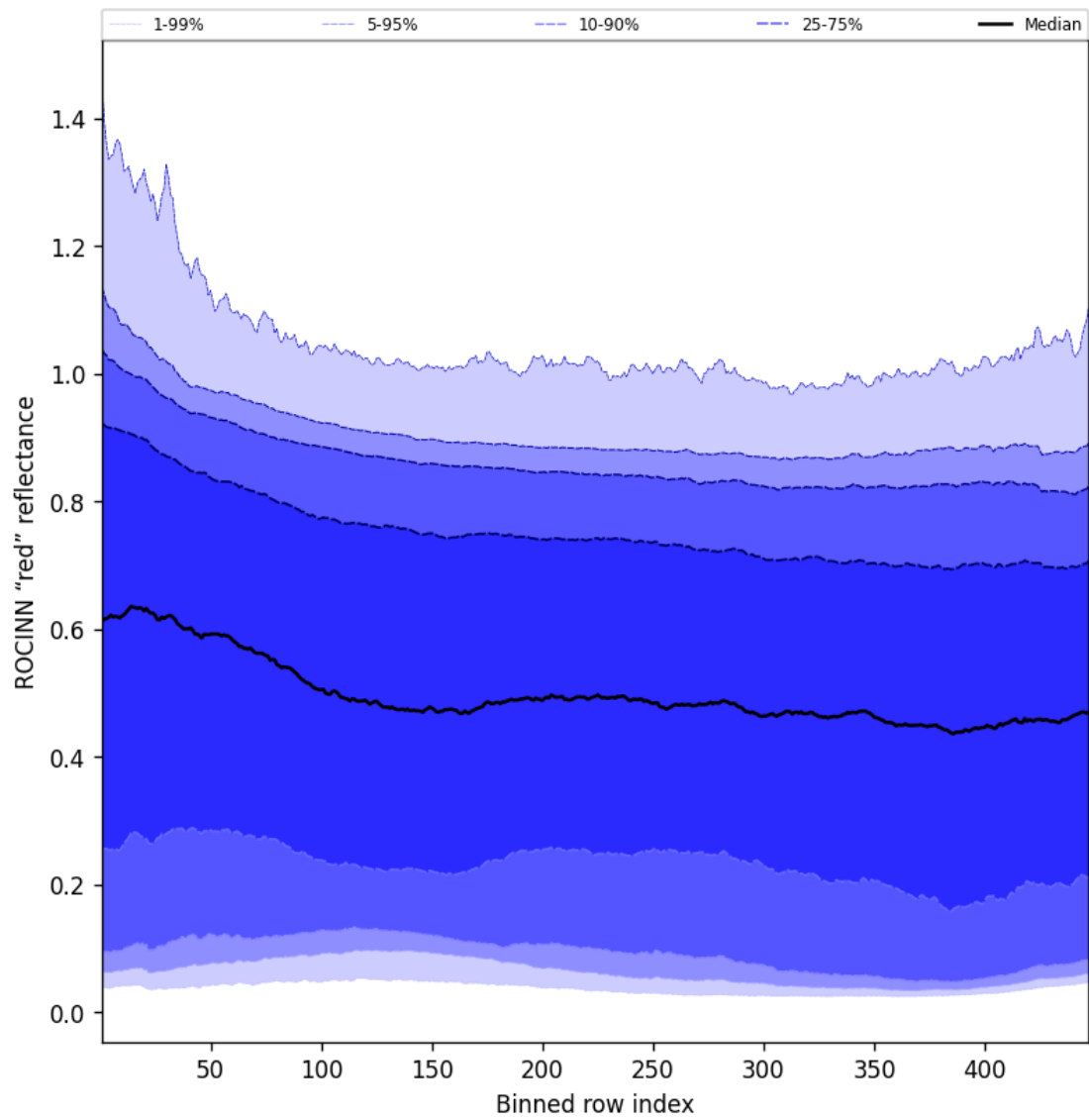
Figure 67: Along track statistics of "ROCINN "red" reflectance" for 2025-10-31 to 2025-10-31
