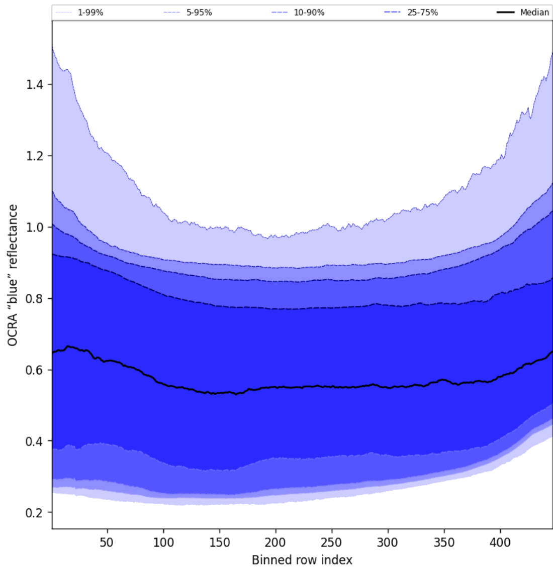
Figure 65: Along track statistics of "OCRA "blue" reflectance" for 2025-10-31 to 2025-10-31
