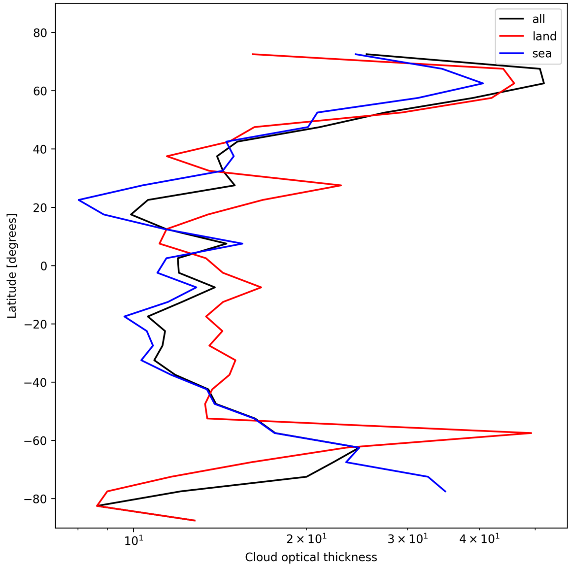
Figure 23: Zonal average of “Cloud optical thickness” for 2025-10-31 to 2025-10-31.
