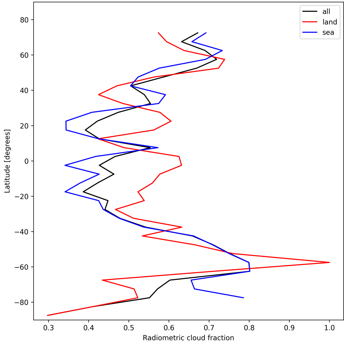
Figure 21: Zonal average of “Radiometric cloud fraction” for 2025-10-31 to 2025-10-31.
