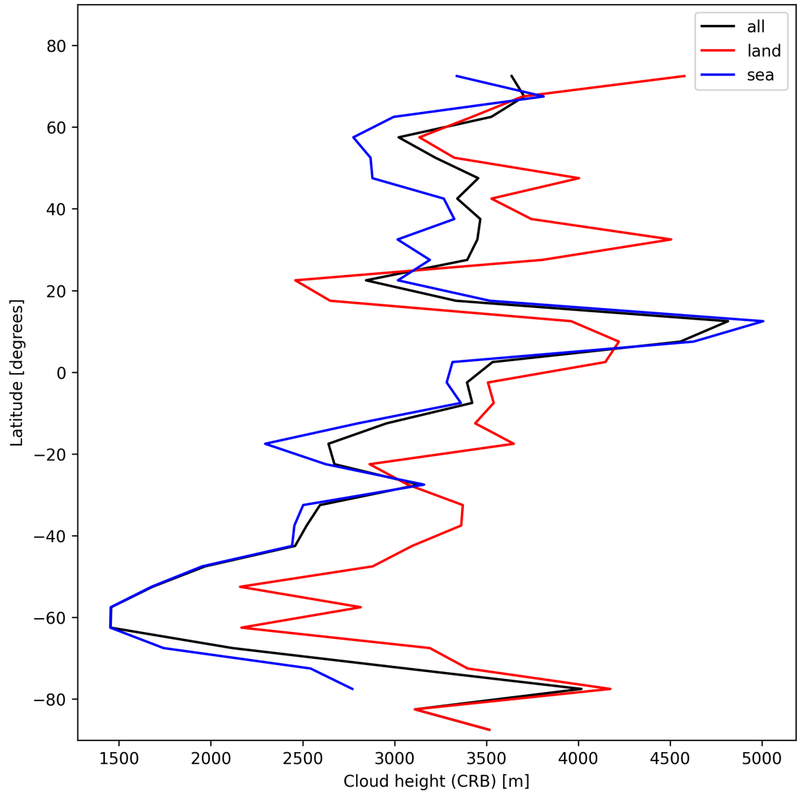
Figure 25: Zonal average of “Cloud height (CRB)” for 2025-10-31 to 2025-10-31.
