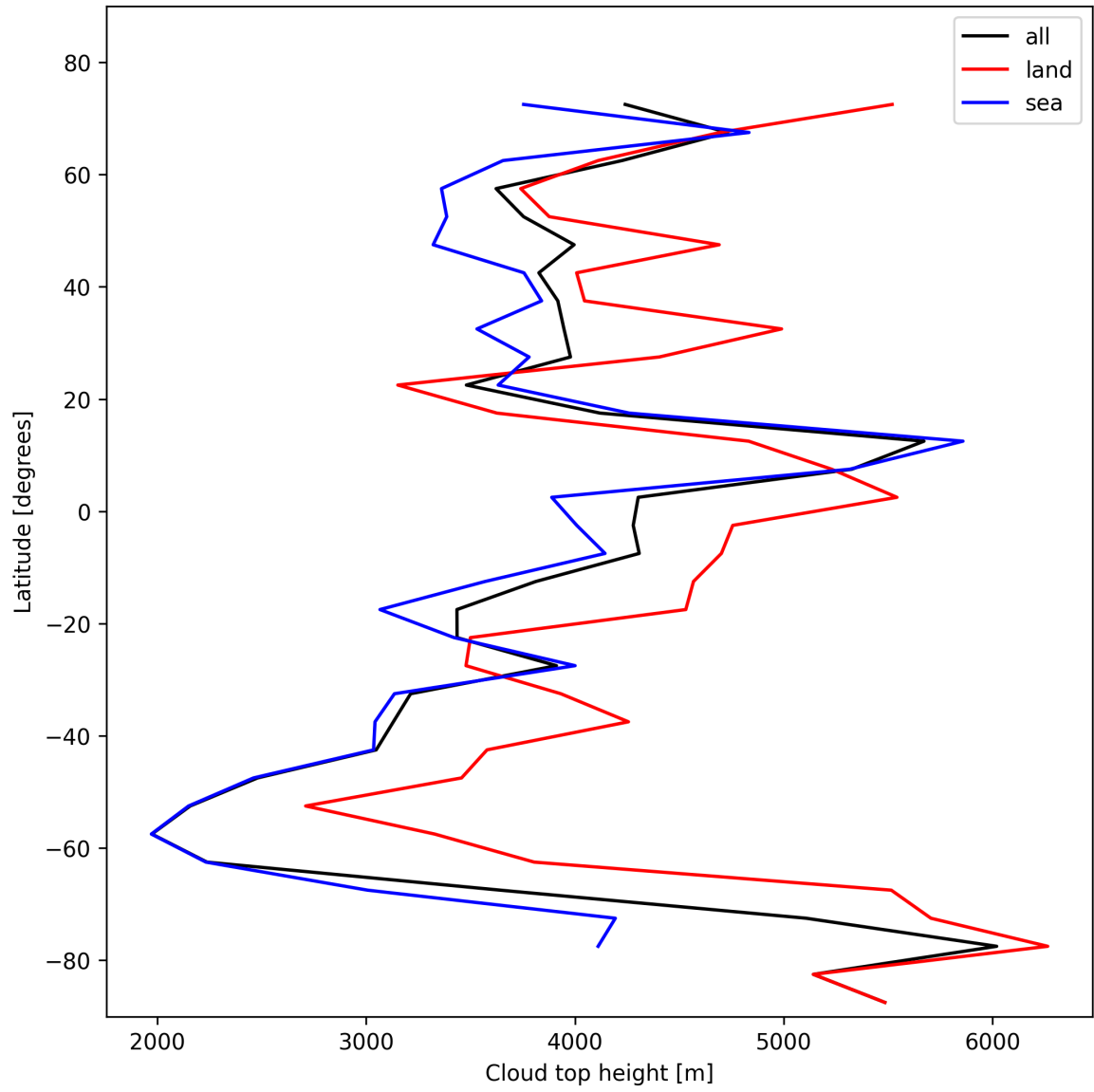
Figure 22: Zonal average of “Cloud top height” for 2025-10-31 to 2025-10-31.
