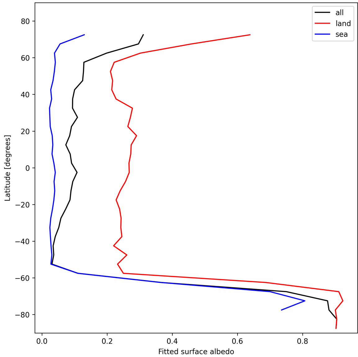
Figure 27: Zonal average of “Fitted surface albedo” for 2025-10-31 to 2025-10-31.
