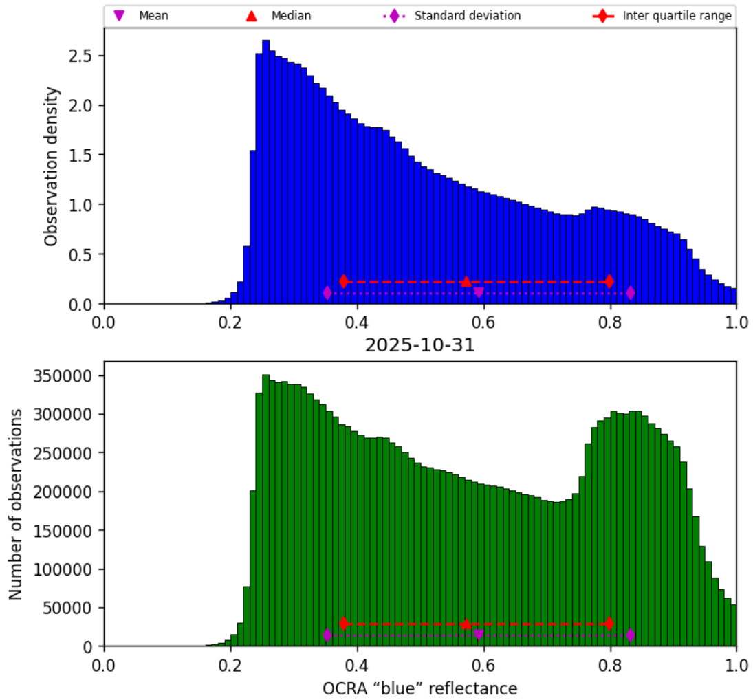
Figure 49: Histogram of “OCRA “blue” reflectance” for 2025-10-31 to 2025-10-31
