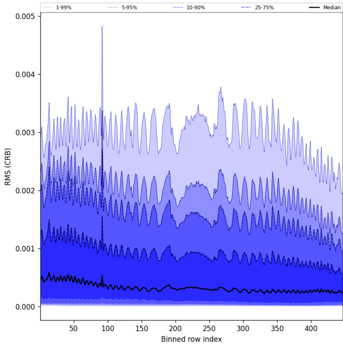
Figure 62: Along track statistics of “RMS (CRB)” for 2025-10-31 to 2025-10-31
