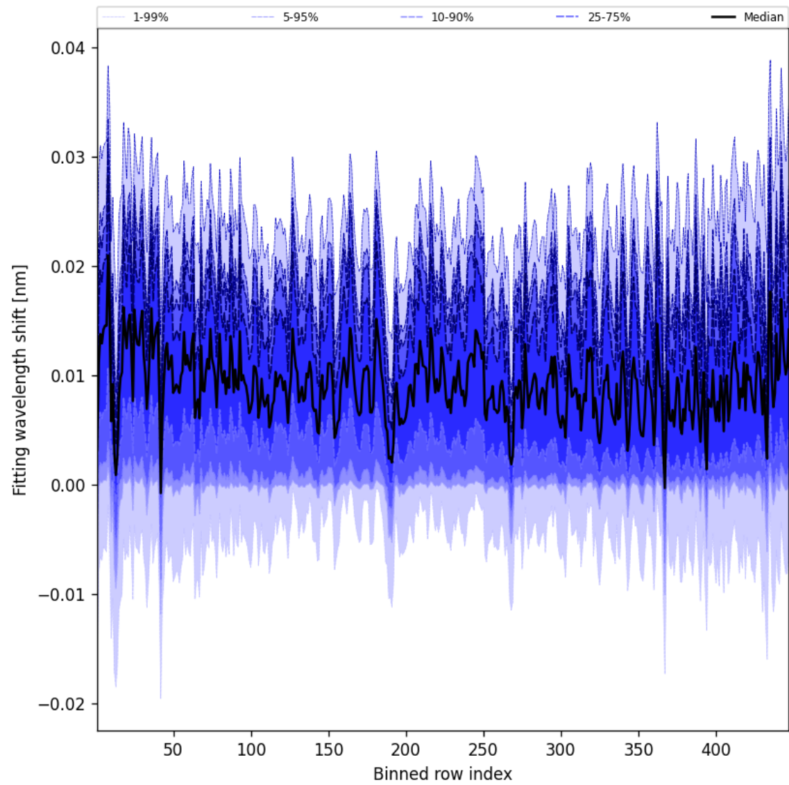
Figure 63: Along track statistics of “Fitting wavelength shift” for 2025-10-31 to 2025-10-31
