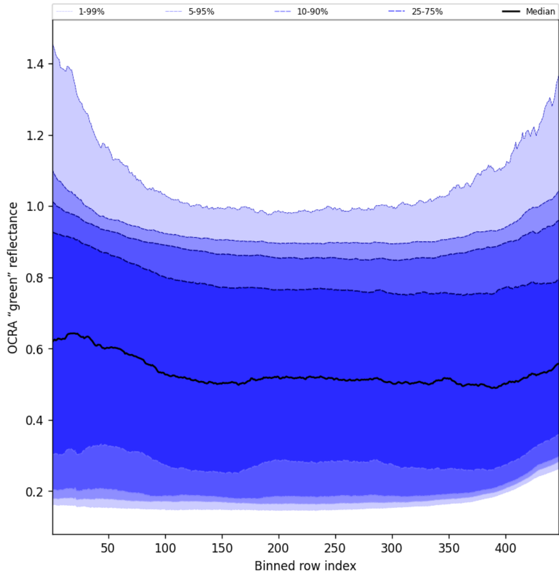
Figure 66: Along track statistics of “OCRA “green” reflectance” for 2025-10-31 to 2025-10-31
