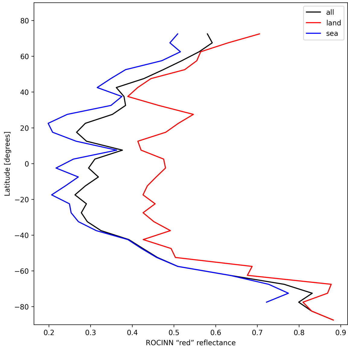
Figure 35: Zonal average of "ROCINN "red" reflectance" for 2025-10-31 to 2025-10-31.
