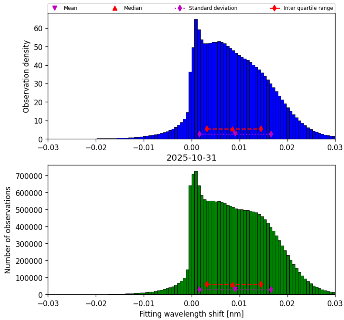
Figure 47: Histogram of “Fitting wavelength shift” for 2025-10-31 to 2025-10-31
