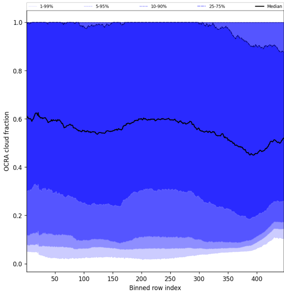
Figure 64: Along track statistics of “OCRA cloud fraction” for 2025-10-31 to 2025-10-31
