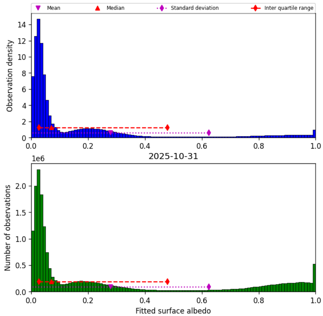
Figure 43: Histogram of “Fitted surface albedo” for 2025-10-31 to 2025-10-31
