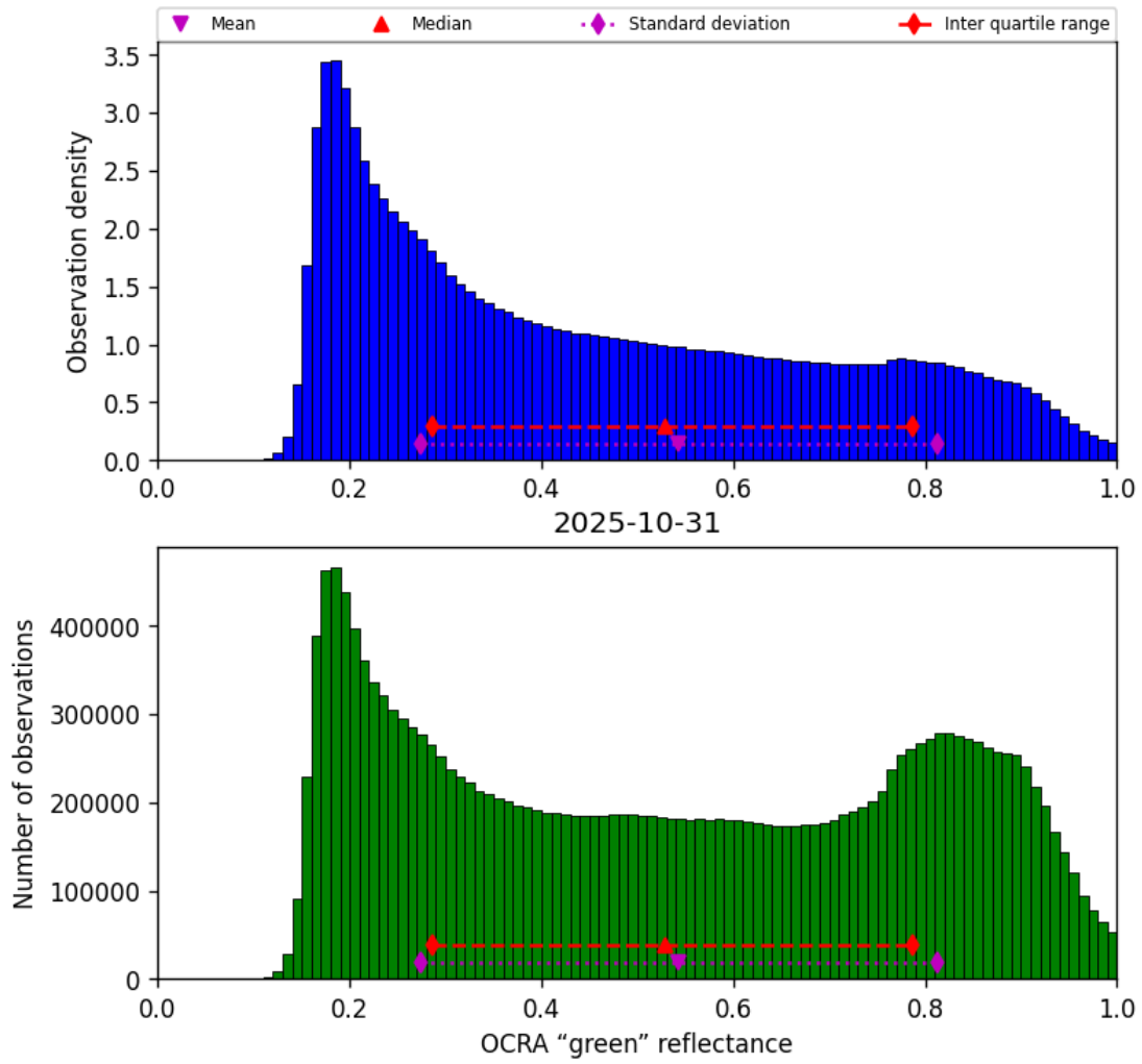
Figure 50: Histogram of “OCRA “green” reflectance” for 2025-10-31 to 2025-10-31
