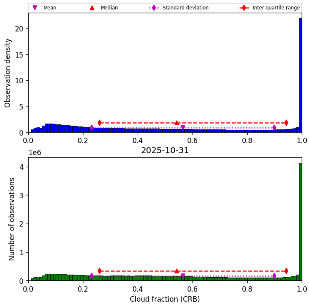
Figure 40: Histogram of “Cloud fraction (CRB)” for 2025-10-31 to 2025-10-31
