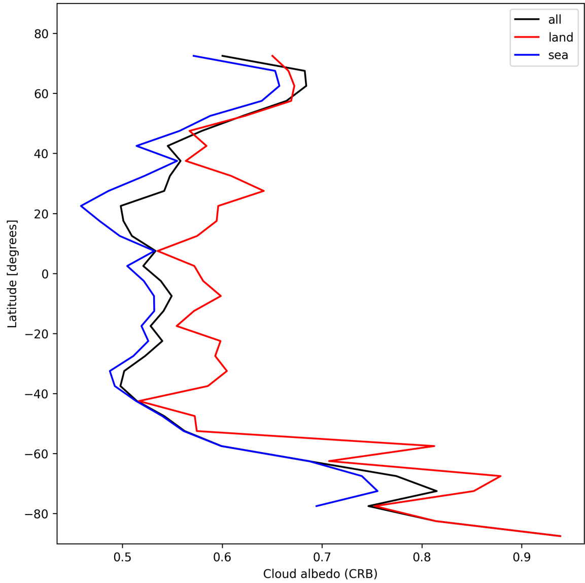
Figure 26: Zonal average of “Cloud albedo (CRB)” for 2025-10-31 to 2025-10-31.
