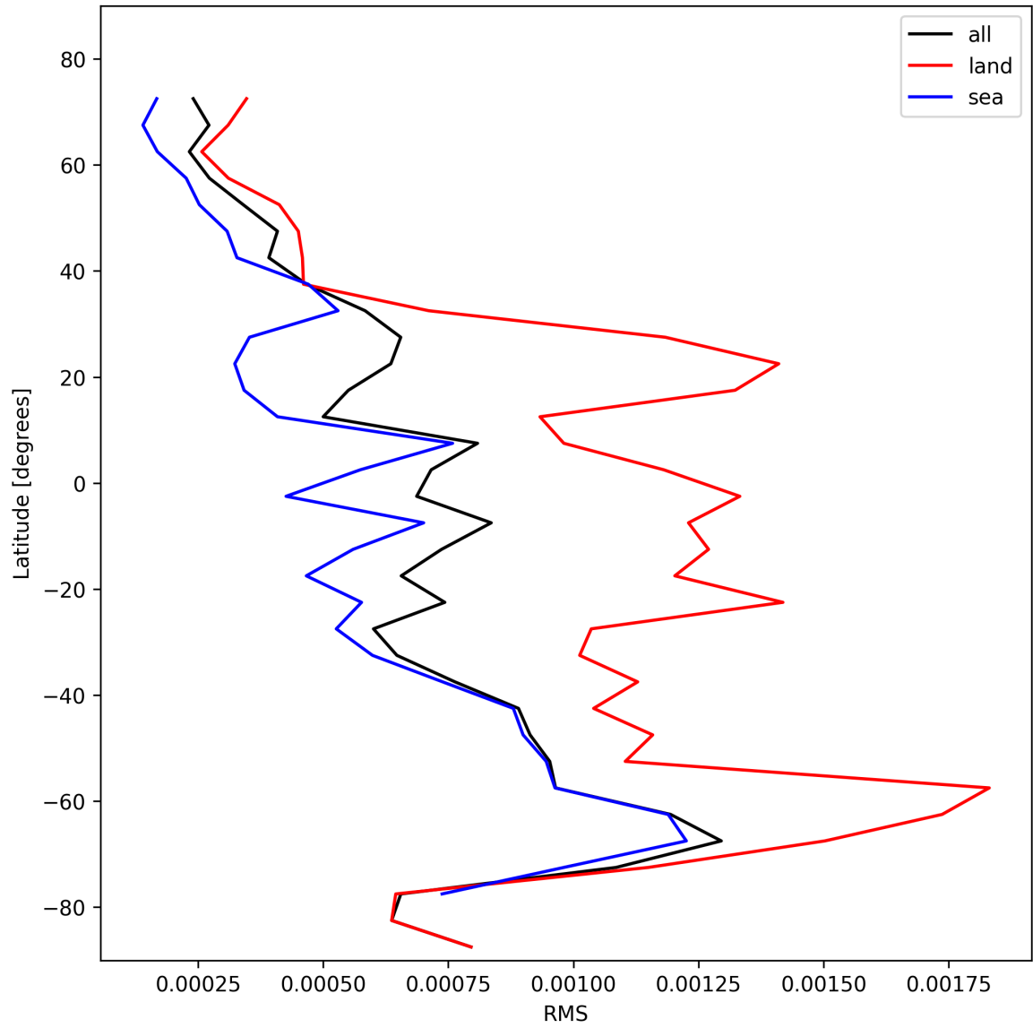
Figure 29: Zonal average of “RMS” for 2025-10-31 to 2025-10-31.
