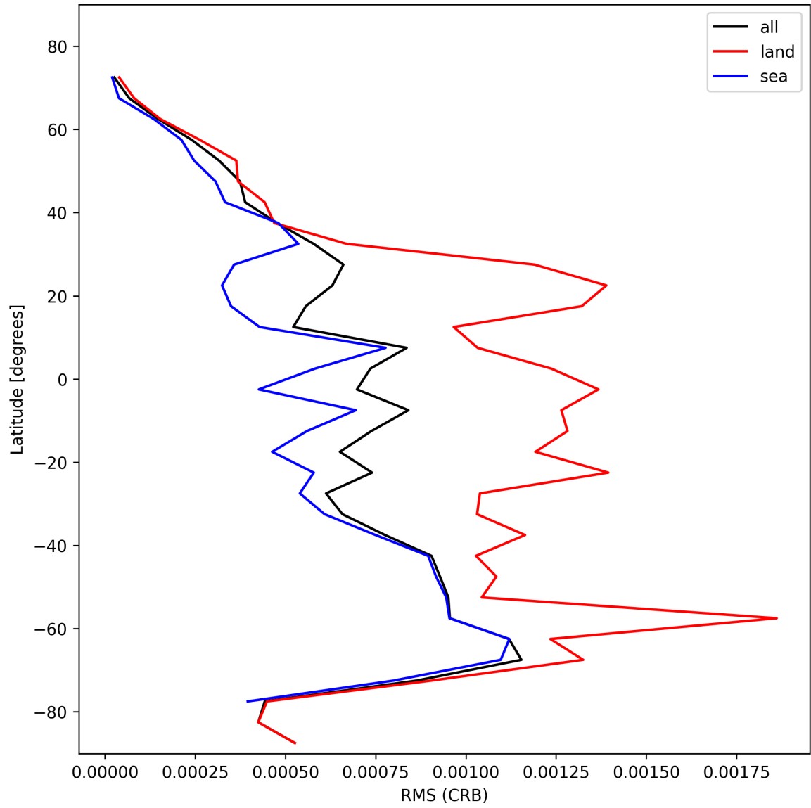
Figure 30: Zonal average of “RMS (CRB)” for 2025-10-31 to 2025-10-31.
