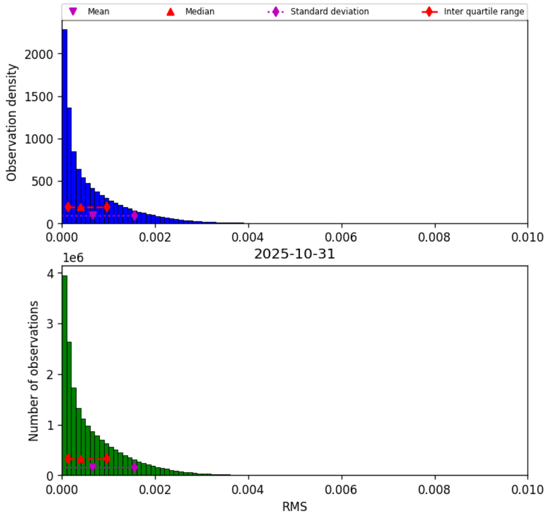
Figure 45: Histogram of “RMS” for 2025-10-31 to 2025-10-31
