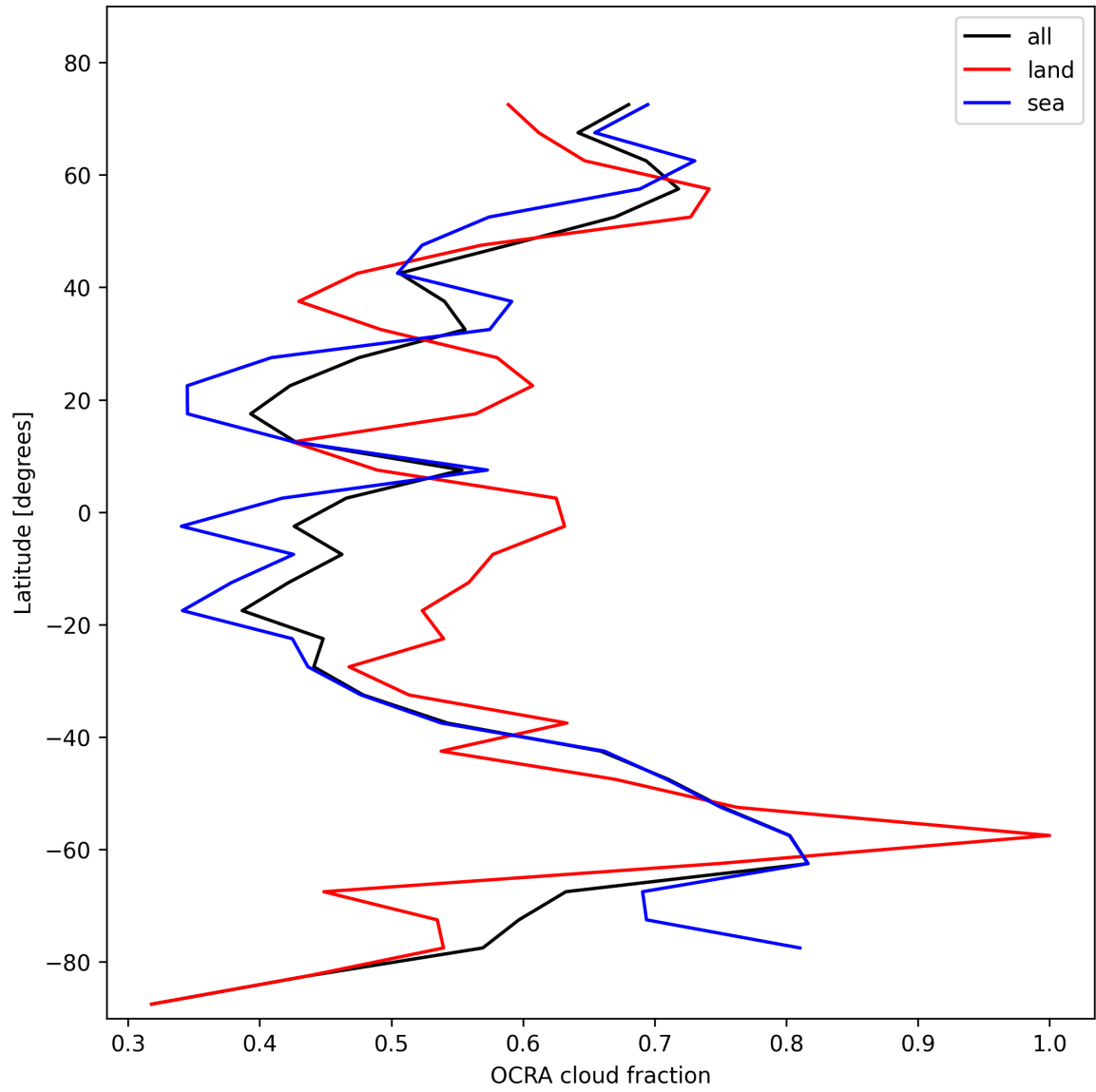
Figure 32: Zonal average of “OCRA cloud fraction” for 2025-10-31 to 2025-10-31.
