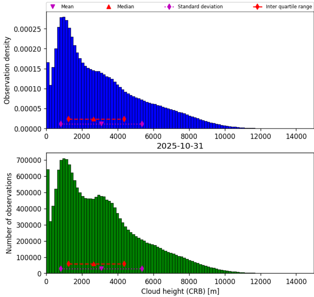
Figure 41: Histogram of “Cloud height (CRB)” for 2025-10-31 to 2025-10-31
