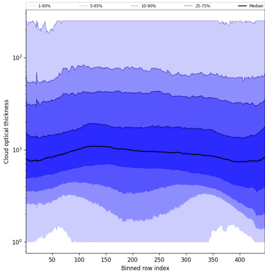
Figure 55: Along track statistics of “Cloud optical thickness” for 2025-10-31 to 2025-10-31
