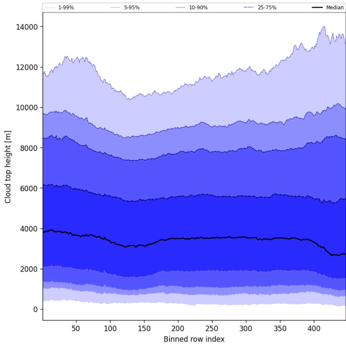
Figure 54: Along track statistics of “Cloud top height” for 2025-10-31 to 2025-10-31
