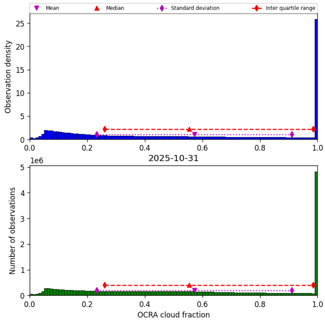
Figure 48: Histogram of “OCRA cloud fraction” for 2025-10-31 to 2025-10-31
