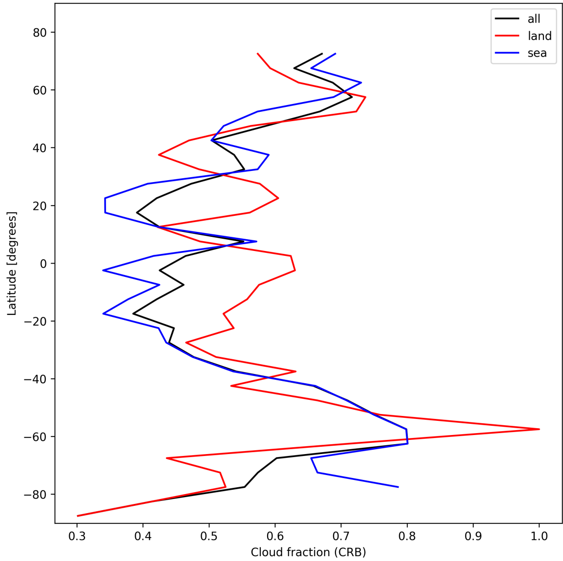
Figure 24: Zonal average of “Cloud fraction (CRB)” for 2025-10-31 to 2025-10-31.
