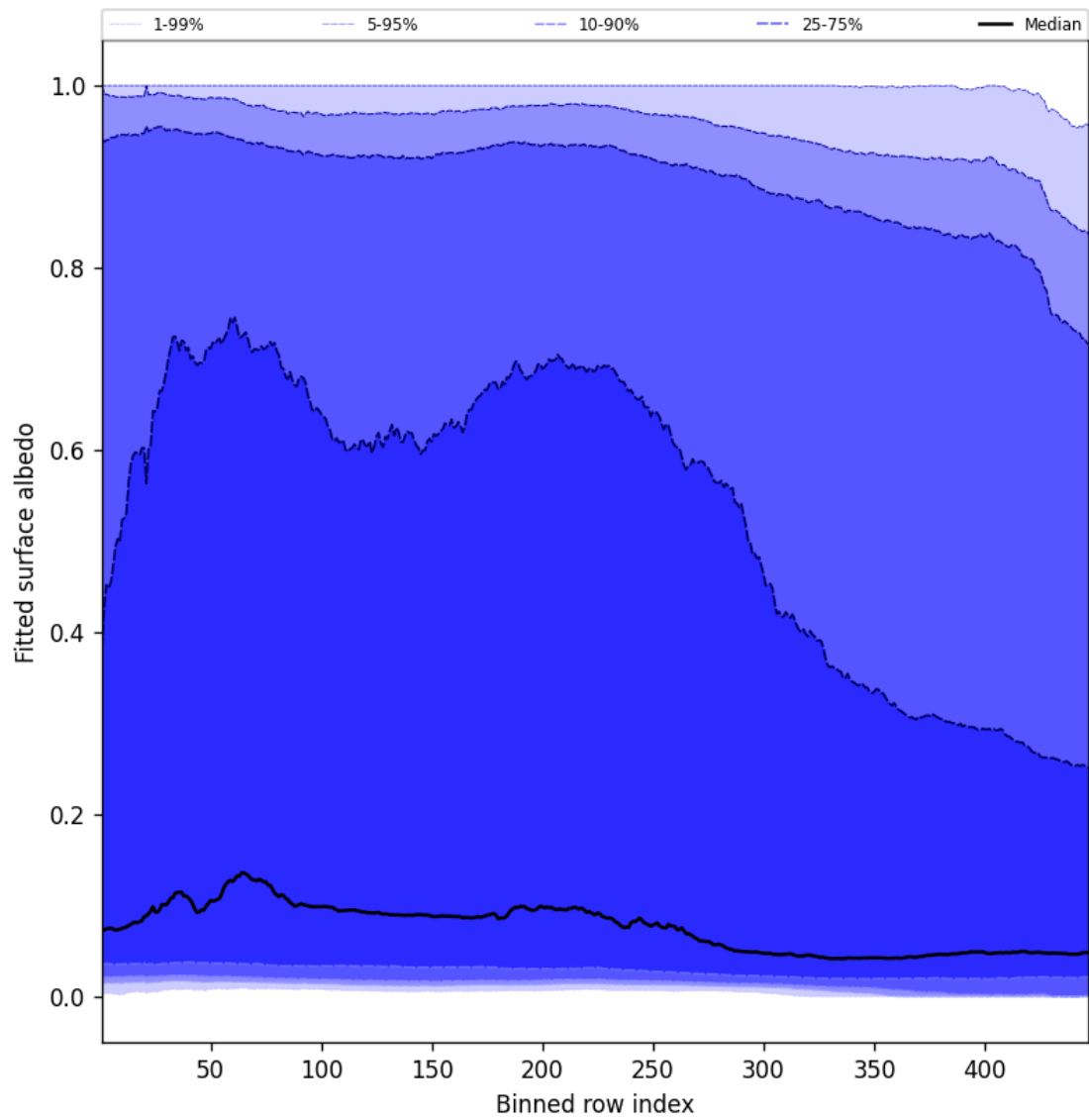
Figure 59: Along track statistics of “Fitted surface albedo” for 2025-10-31 to 2025-10-31
