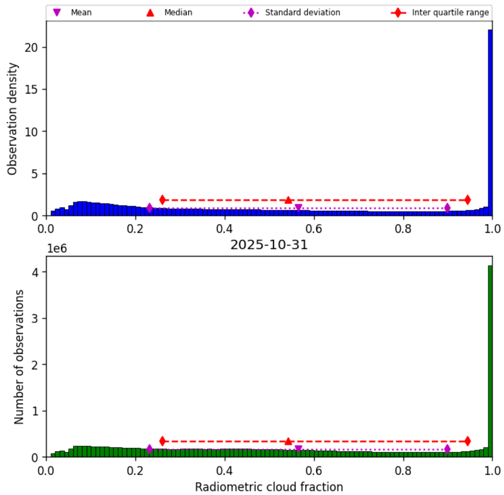
Figure 37: Histogram of “Radiometric cloud fraction” for 2025-10-31 to 2025-10-31
