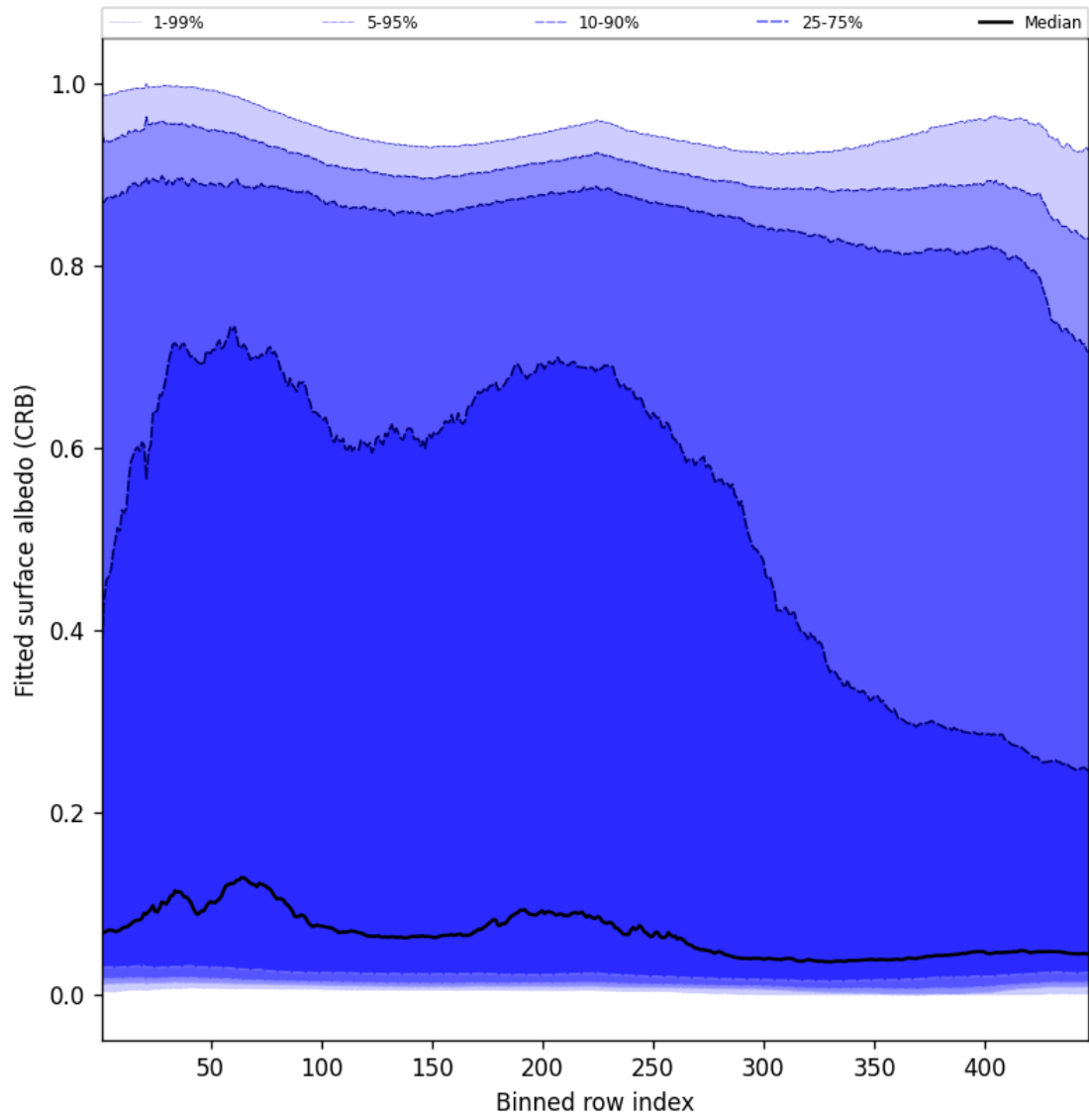
Figure 60: Along track statistics of “Fitted surface albedo (CRB)” for 2025-10-31 to 2025-10-31
