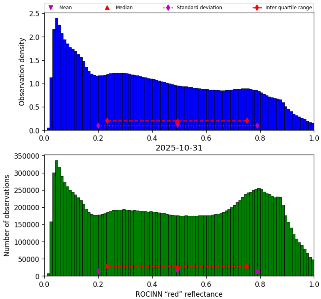
Figure 51: Histogram of “ROCINN “red” reflectance” for 2025-10-31 to 2025-10-31
