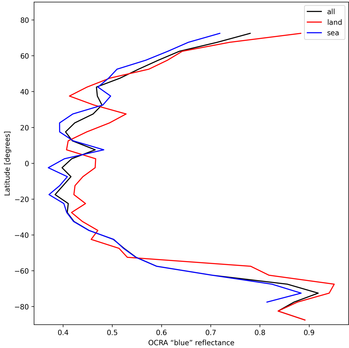
Figure 33: Zonal average of “OCRA “blue” reflectance” for 2025-10-31 to 2025-10-31.
