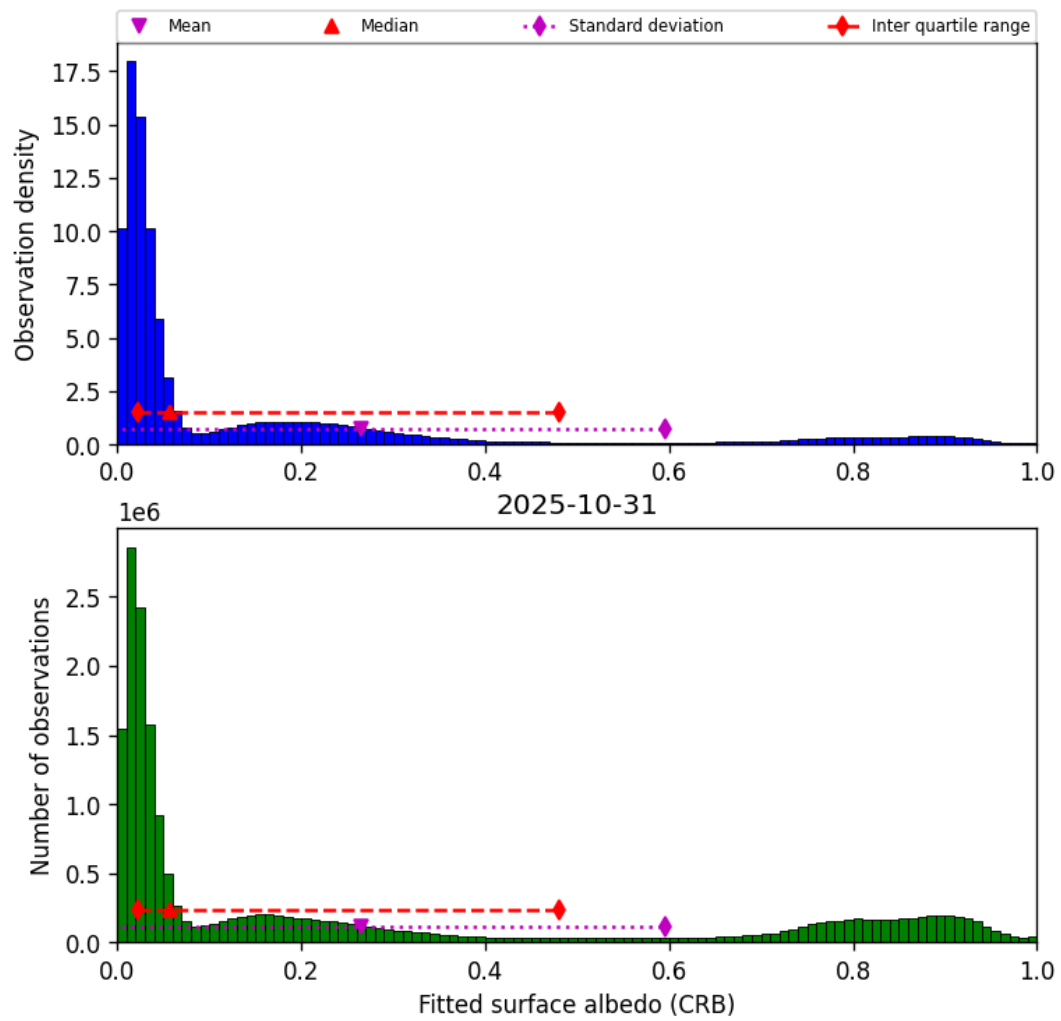
Figure 44: Histogram of “Fitted surface albedo (CRB)” for 2025-10-31 to 2025-10-31
