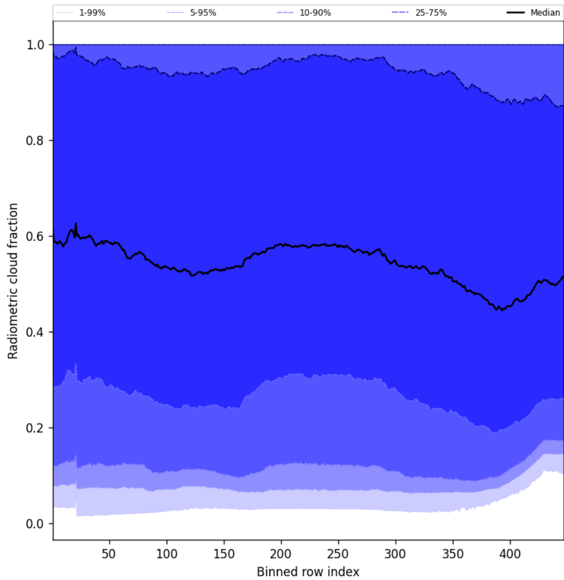
Figure 53: Along track statistics of “Radiometric cloud fraction” for 2025-10-31 to 2025-10-31
