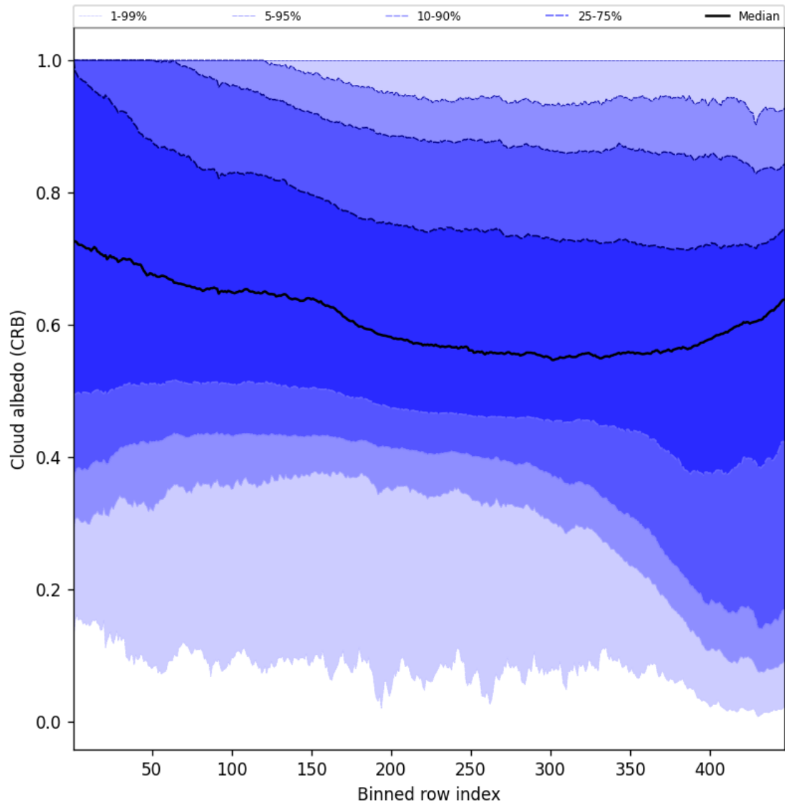
Figure 58: Along track statistics of “Cloud albedo (CRB)” for 2025-10-31 to 2025-10-31
