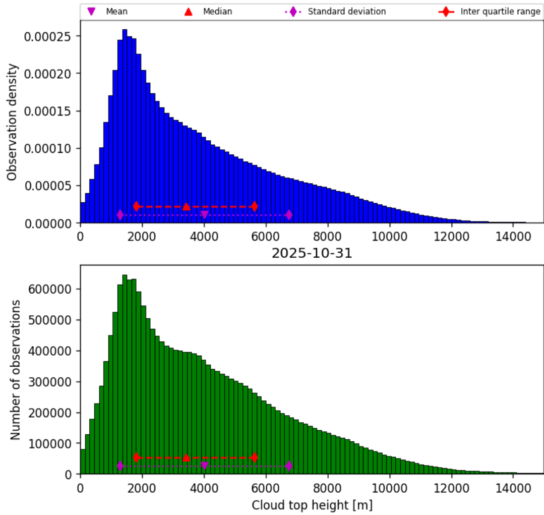
Figure 38: Histogram of “Cloud top height” for 2025-10-31 to 2025-10-31
