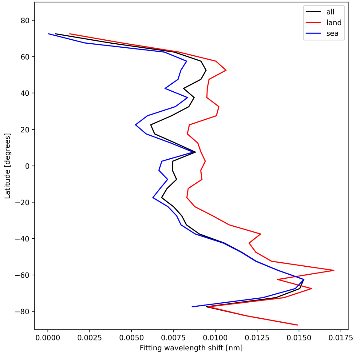
Figure 31: Zonal average of “Fitting wavelength shift” for 2025-10-31 to 2025-10-31.
