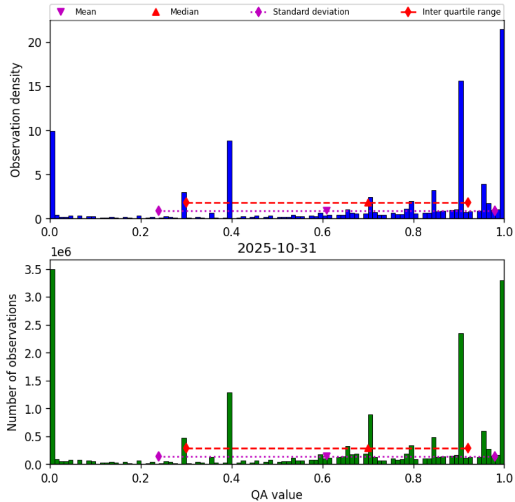
Figure 36: Histogram of “QA value” for 2025-10-31 to 2025-10-31
