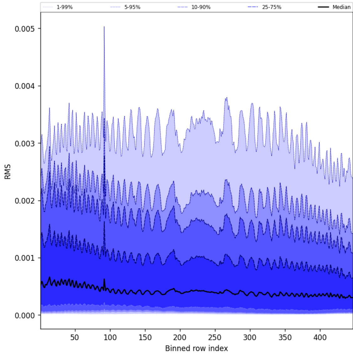
Figure 61: Along track statistics of “RMS” for 2025-10-31 to 2025-10-31
