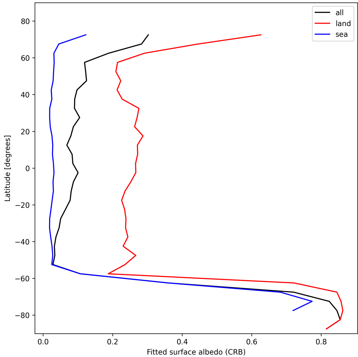
Figure 28: Zonal average of “Fitted surface albedo (CRB)” for 2025-10-31 to 2025-10-31.
