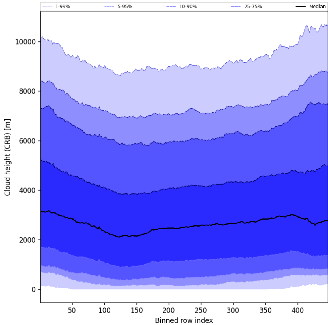
Figure 57: Along track statistics of “Cloud height (CRB)” for 2025-10-31 to 2025-10-31
