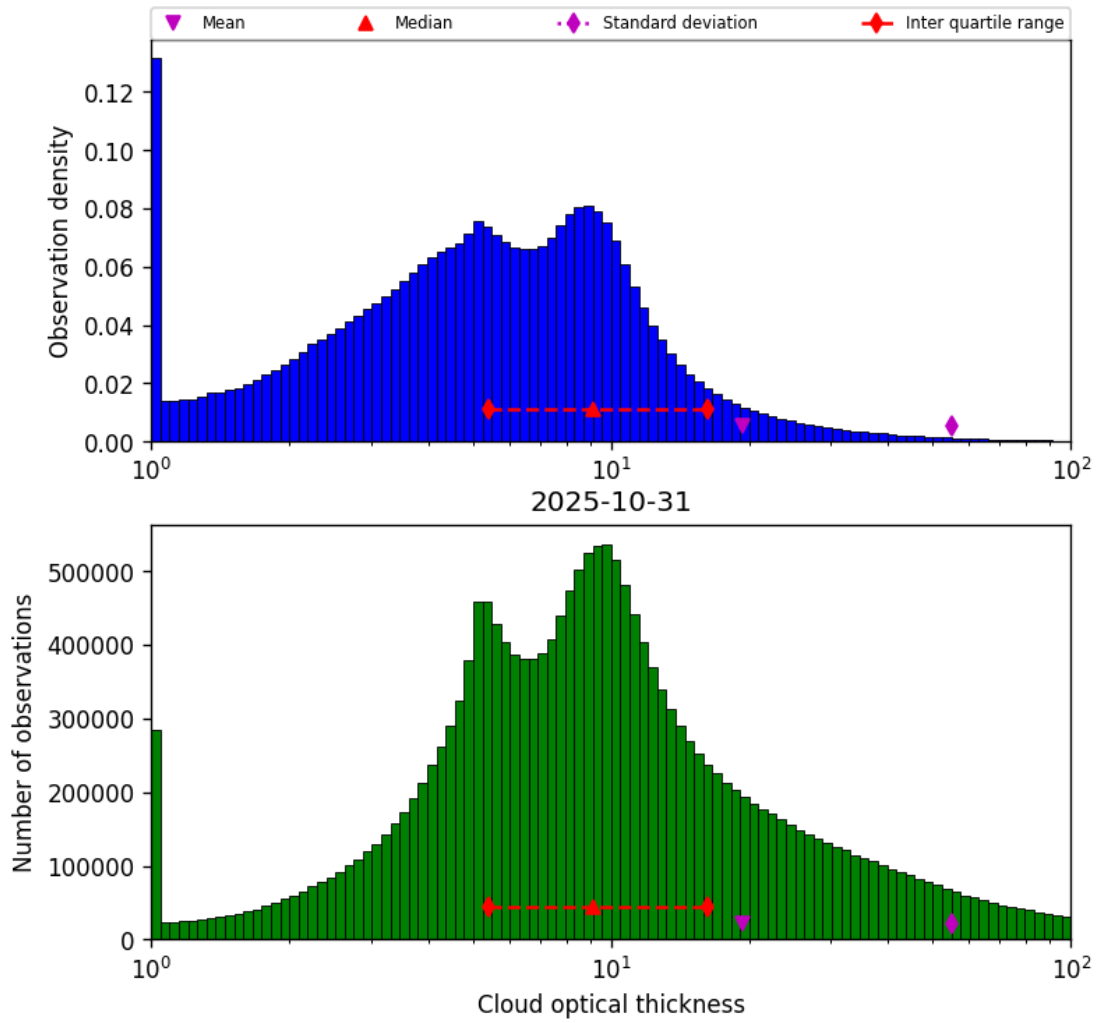
Figure 39: Histogram of “Cloud optical thickness” for 2025-10-31 to 2025-10-31
