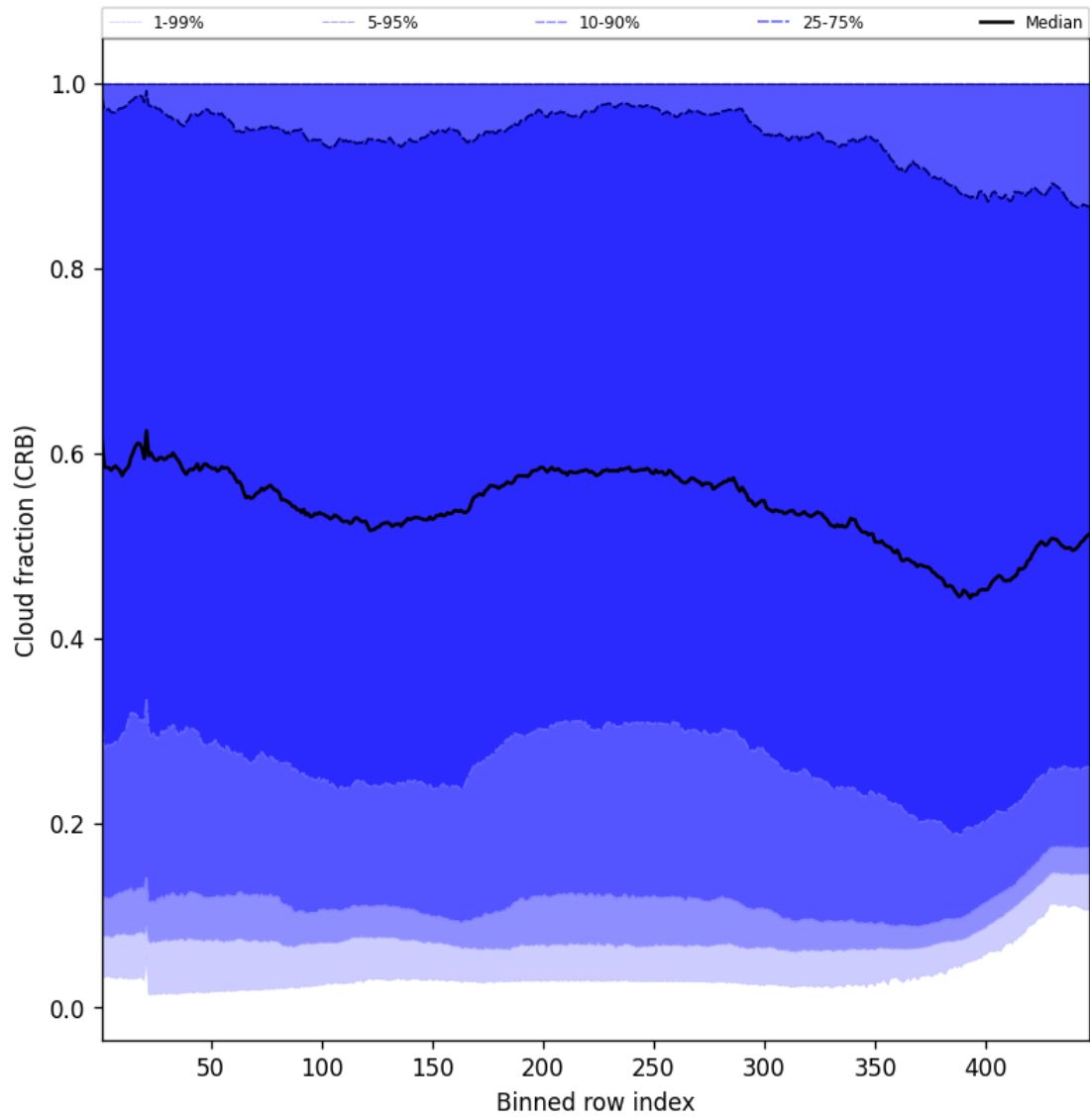
Figure 56: Along track statistics of “Cloud fraction (CRB)” for 2025-10-31 to 2025-10-31
