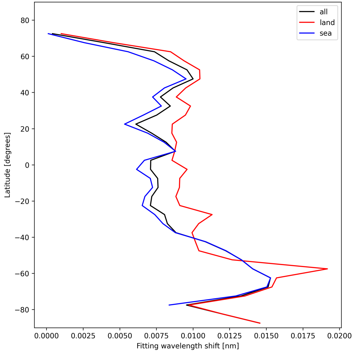
Figure 31: Zonal average of “Fitting wavelength shift” for 2025-11-01 to 2025-11-02.
