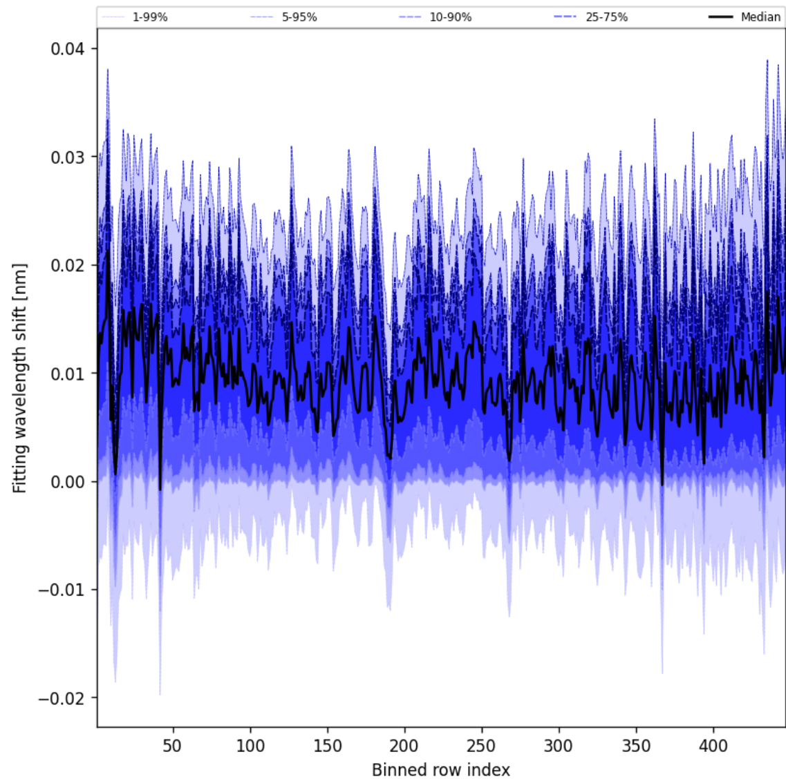
Figure 63: Along track statistics of “Fitting wavelength shift” for 2025-11-01 to 2025-11-02
