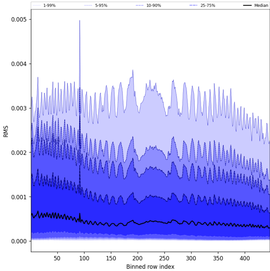
Figure 61: Along track statistics of “RMS” for 2025-11-01 to 2025-11-02
