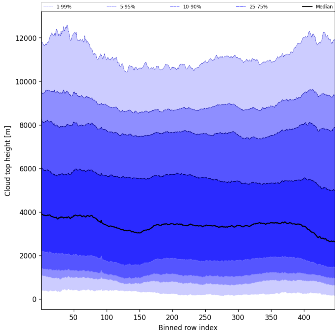
Figure 54: Along track statistics of “Cloud top height” for 2025-11-01 to 2025-11-02
