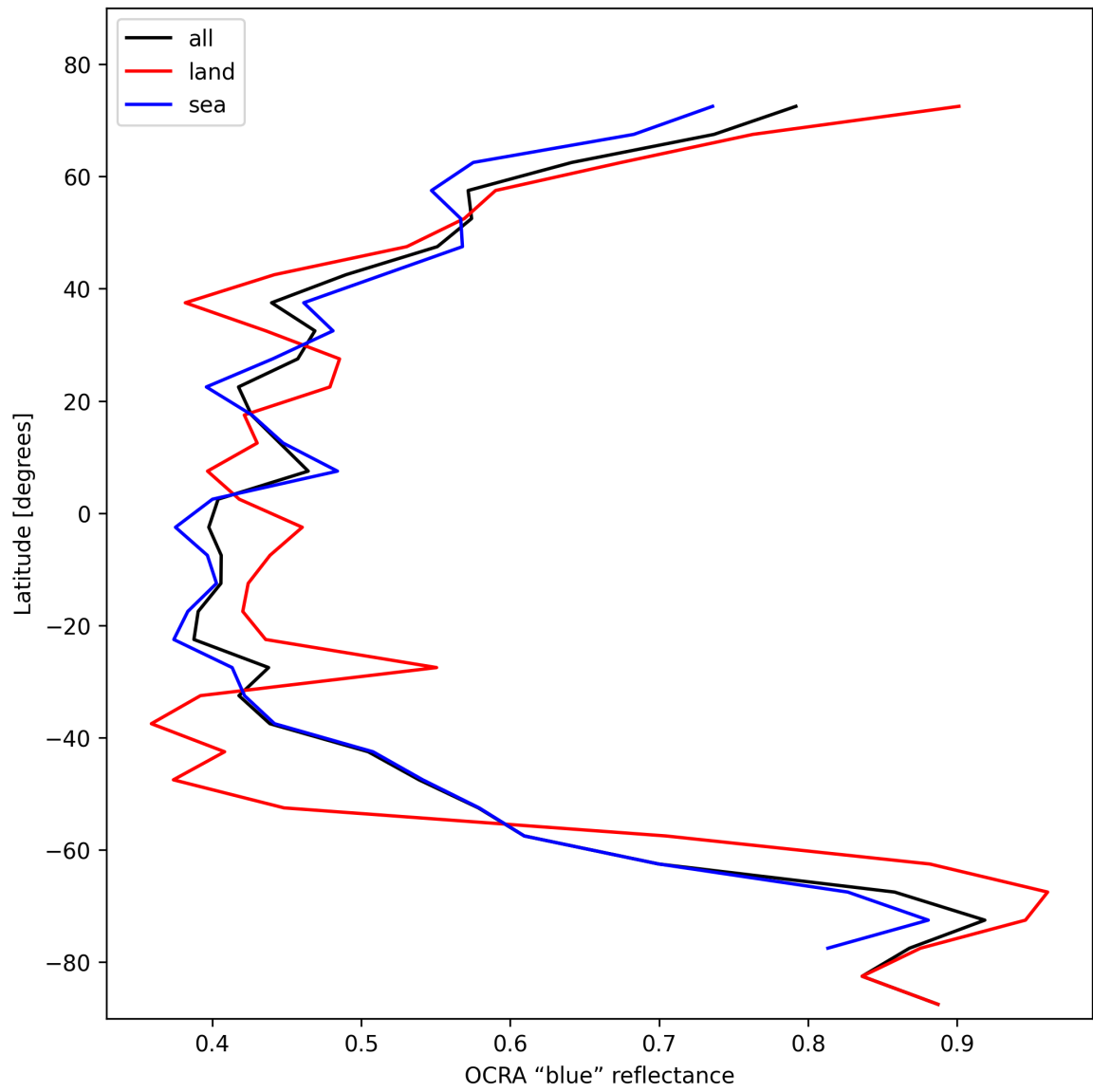
Figure 33: Zonal average of “OCRA “blue” reflectance” for 2025-11-01 to 2025-11-02.
