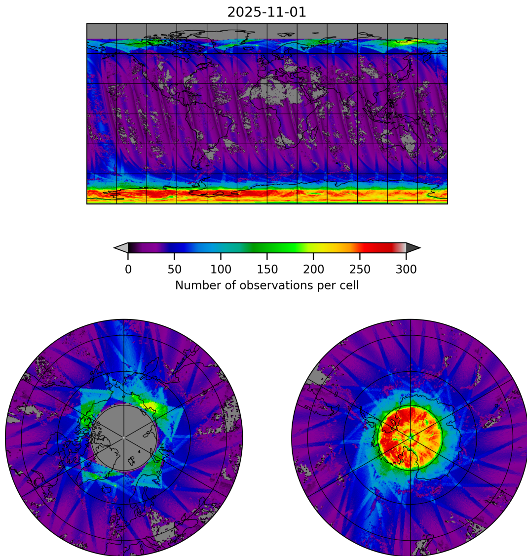
Figure 19: Map of the number of observations for 2025-11-01 to 2025-11-02
