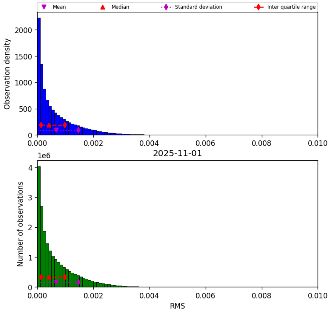
Figure 45: Histogram of “RMS” for 2025-11-01 to 2025-11-02
