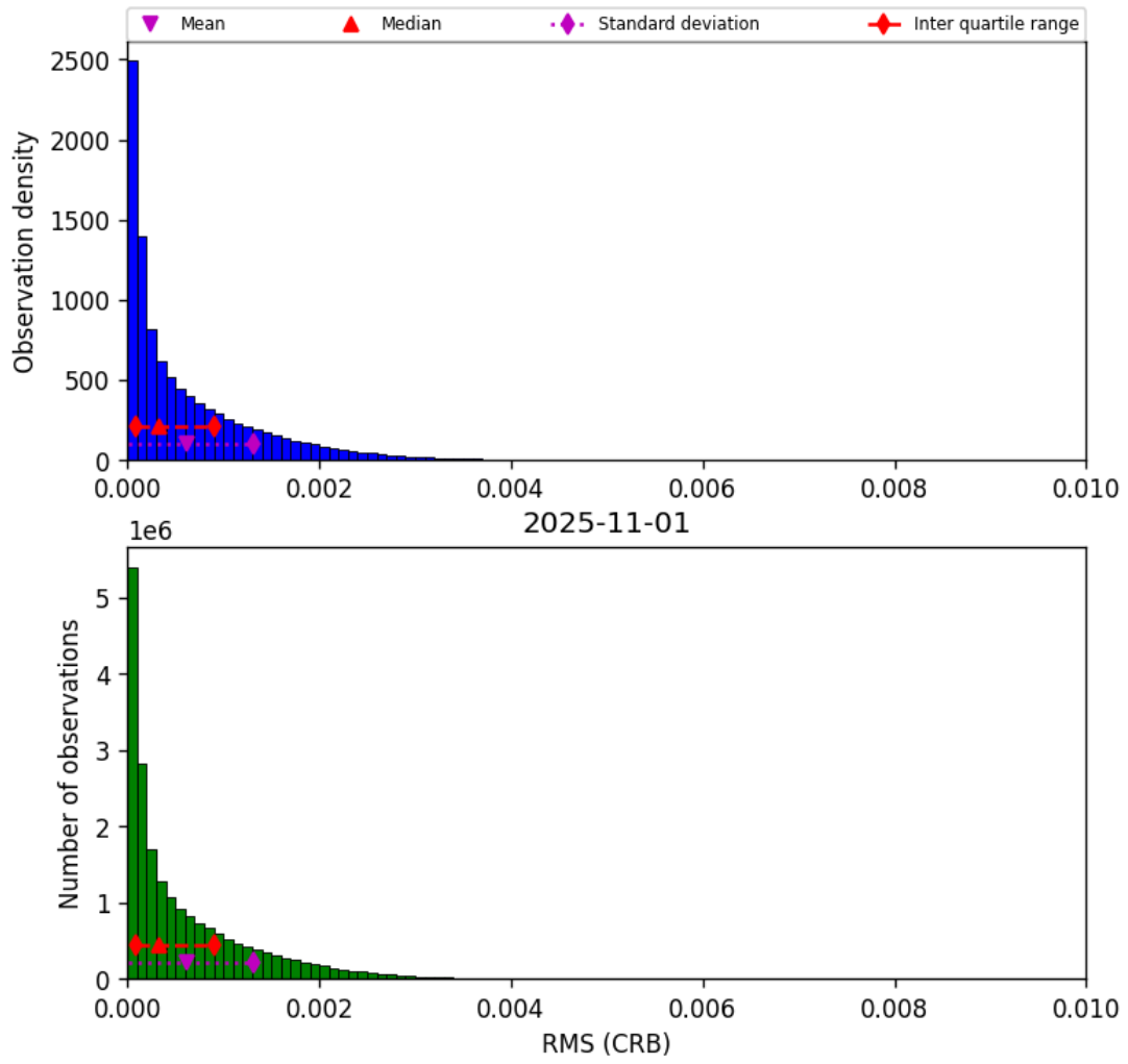
Figure 46: Histogram of “RMS (CRB)” for 2025-11-01 to 2025-11-02
