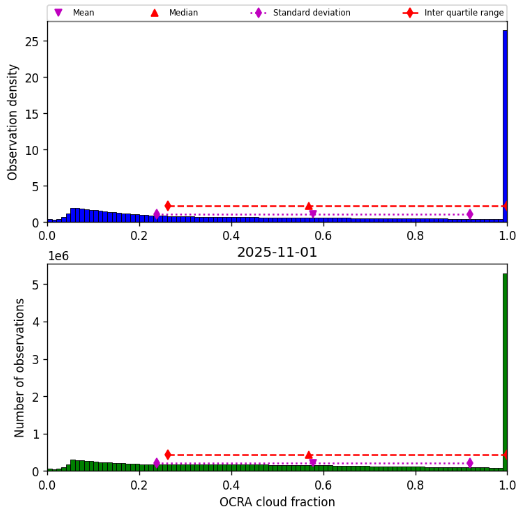
Figure 48: Histogram of “OCRA cloud fraction” for 2025-11-01 to 2025-11-02
