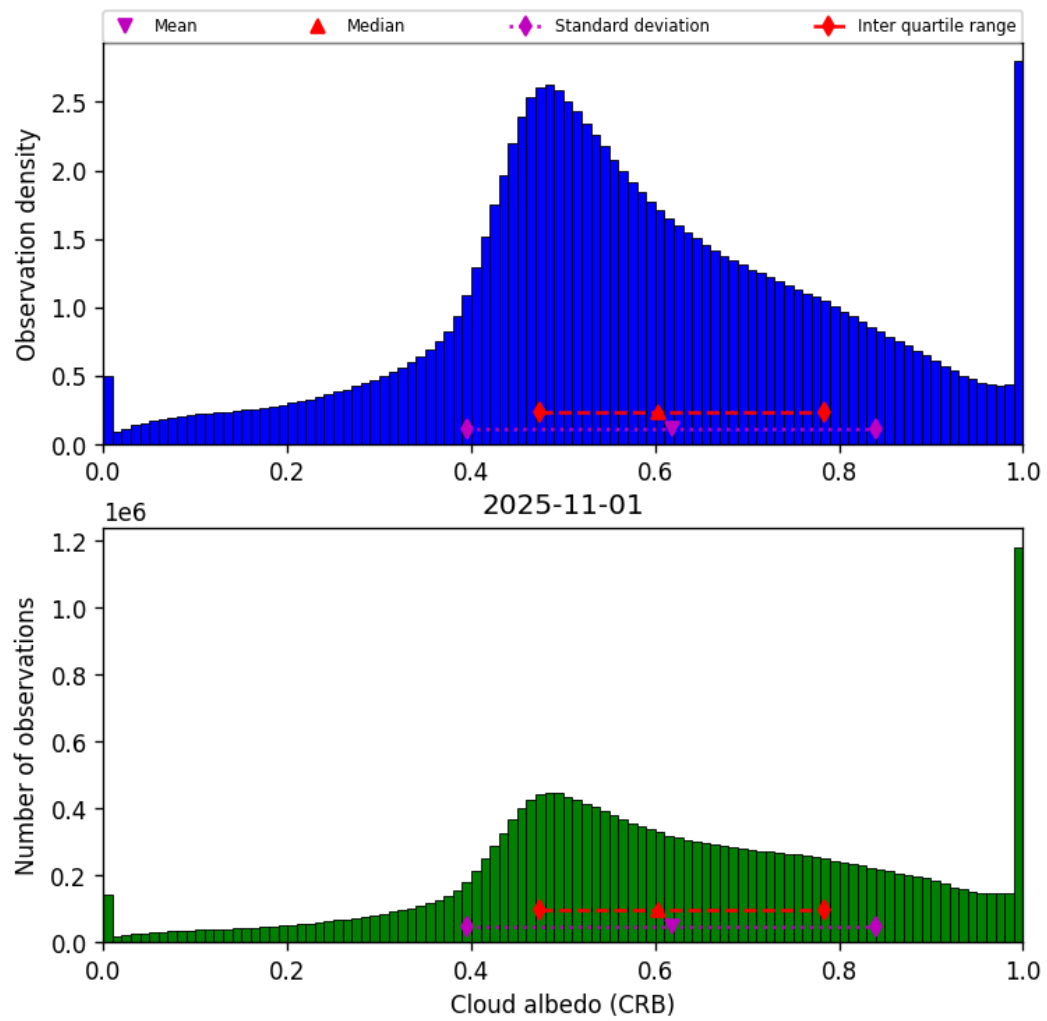
Figure 42: Histogram of “Cloud albedo (CRB)” for 2025-11-01 to 2025-11-02
