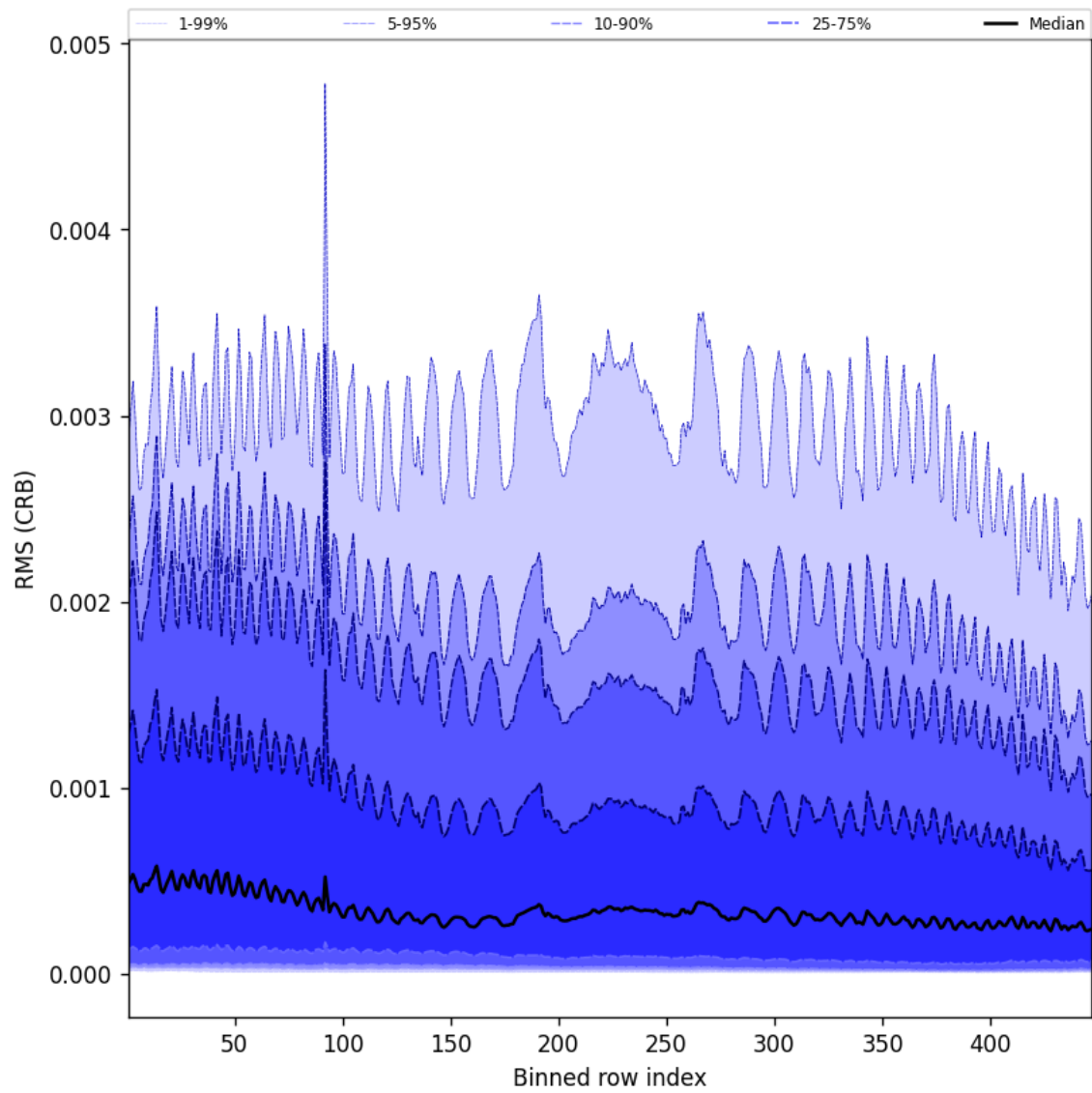
Figure 62: Along track statistics of “RMS (CRB)” for 2025-11-01 to 2025-11-02
