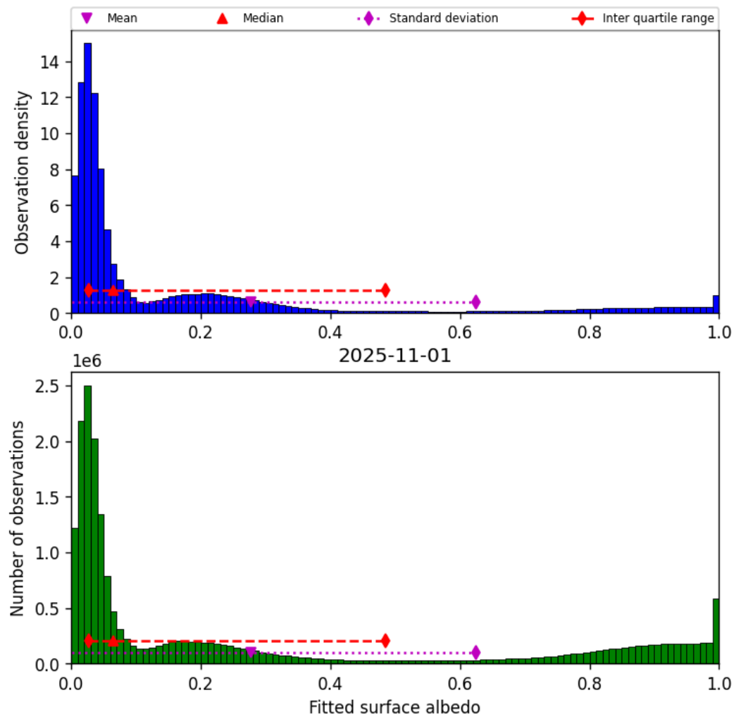
Figure 43: Histogram of “Fitted surface albedo” for 2025-11-01 to 2025-11-02
