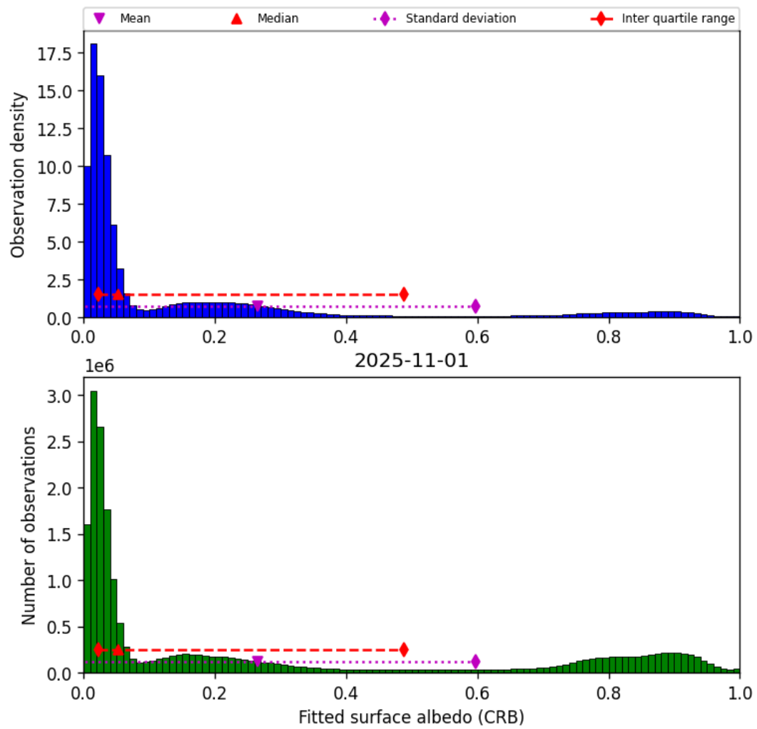
Figure 44: Histogram of “Fitted surface albedo (CRB)” for 2025-11-01 to 2025-11-02
