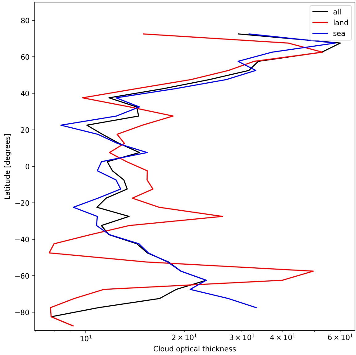
Figure 23: Zonal average of “Cloud optical thickness” for 2025-11-01 to 2025-11-02.
