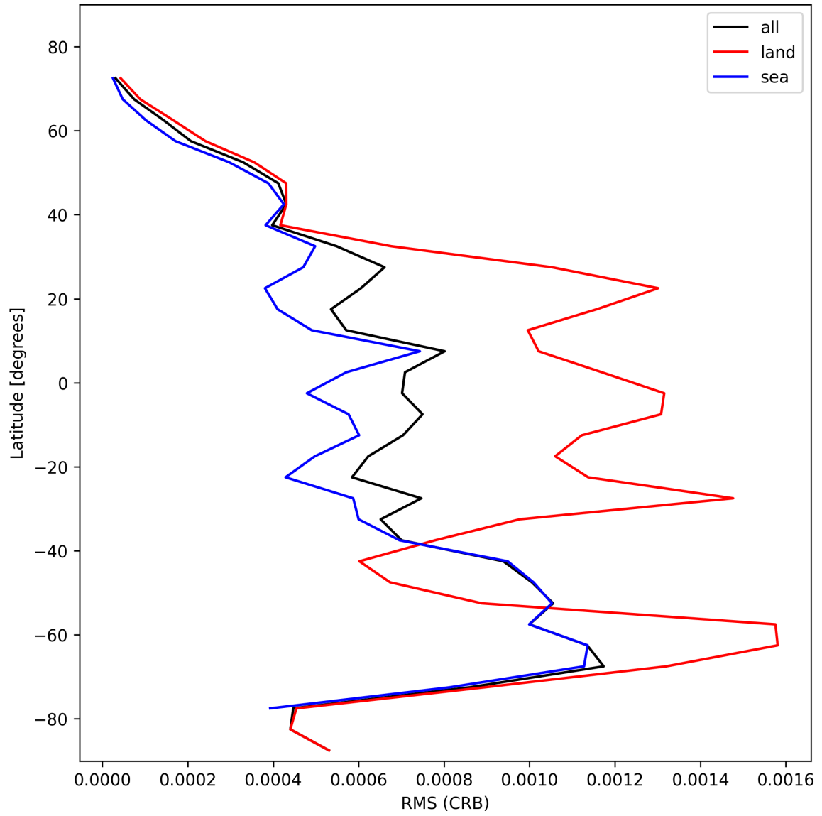
Figure 30: Zonal average of “RMS (CRB)” for 2025-11-01 to 2025-11-02.
