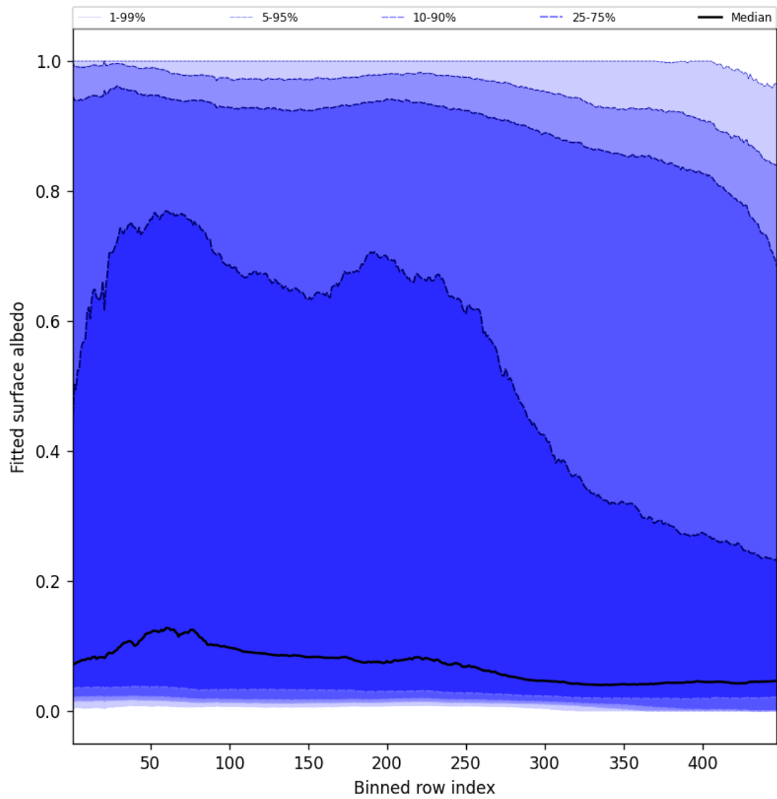
Figure 59: Along track statistics of “Fitted surface albedo” for 2025-11-01 to 2025-11-02
