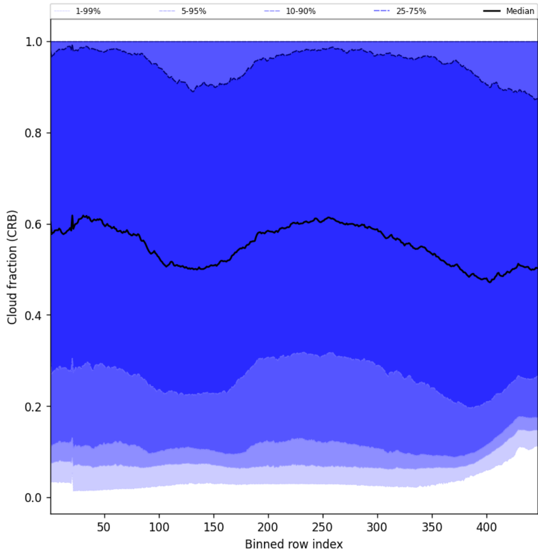
Figure 56: Along track statistics of “Cloud fraction (CRB)” for 2025-11-01 to 2025-11-02
