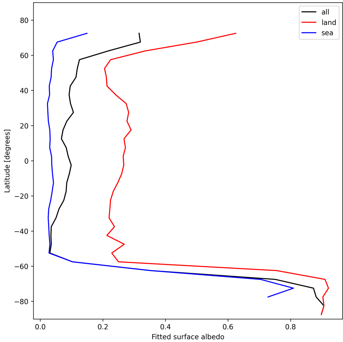
Figure 27: Zonal average of “Fitted surface albedo” for 2025-11-01 to 2025-11-02.
