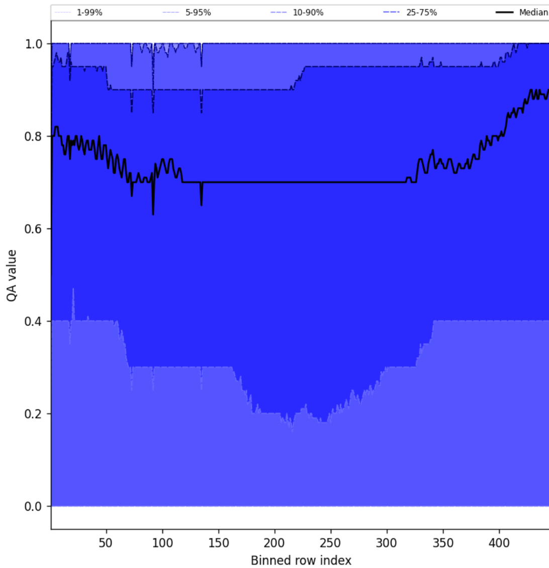
Figure 52: Along track statistics of “QA value” for 2025-11-01 to 2025-11-02
