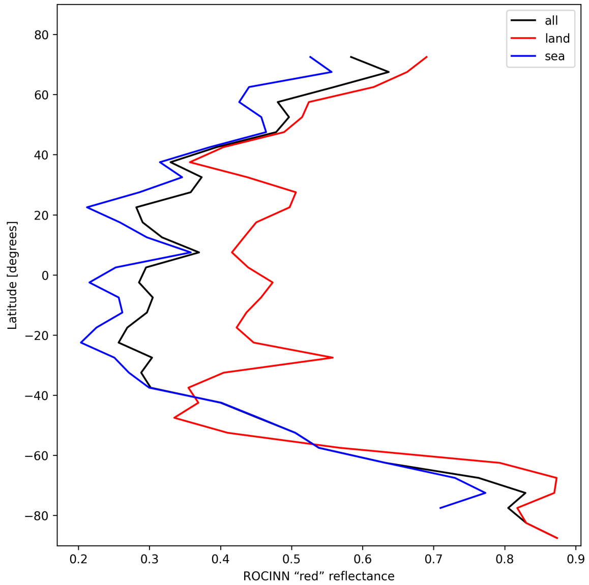
Figure 35: Zonal average of “ROCINN “red” reflectance” for 2025-11-01 to 2025-11-02.
