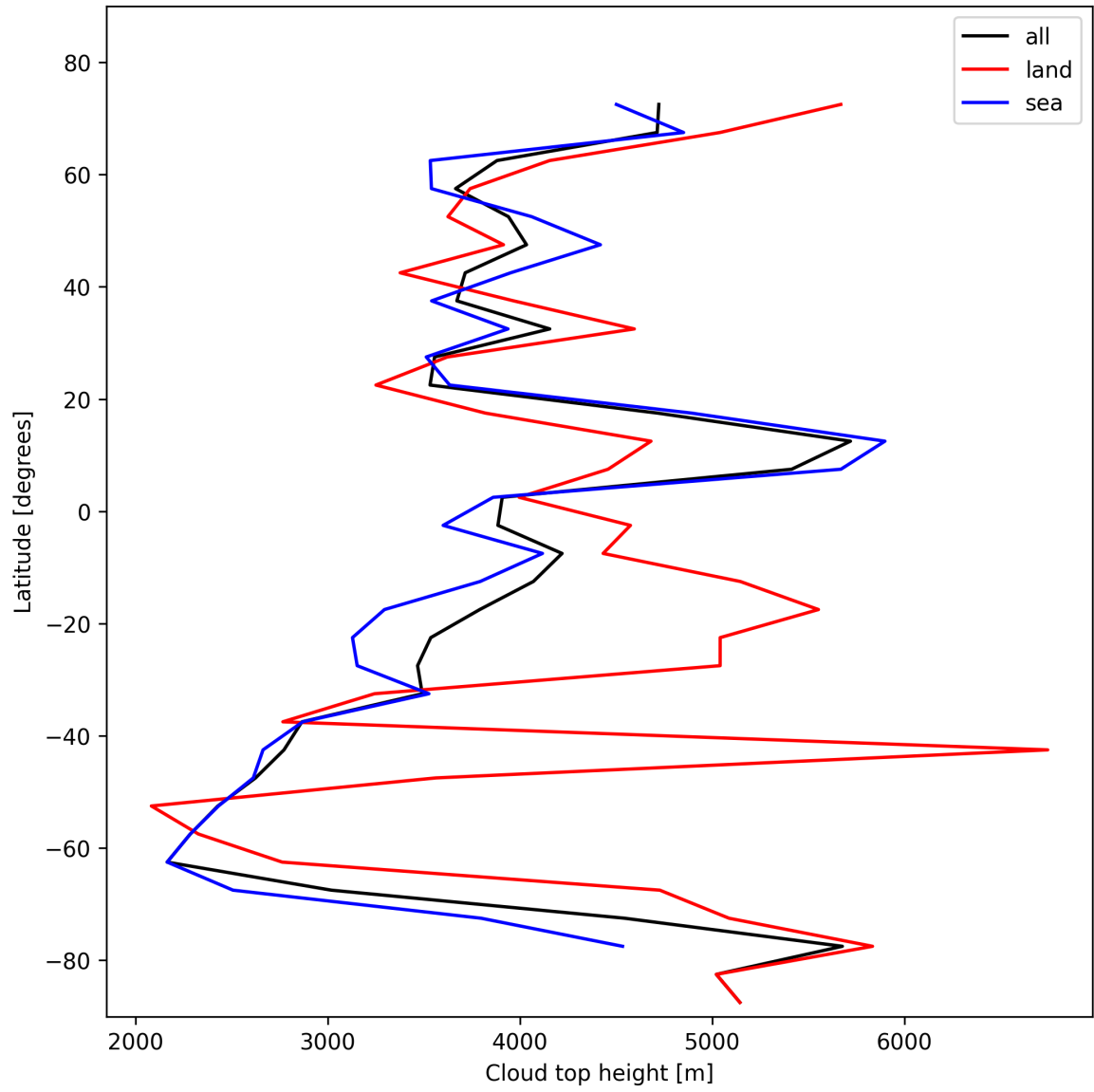
Figure 22: Zonal average of “Cloud top height” for 2025-11-01 to 2025-11-02.
