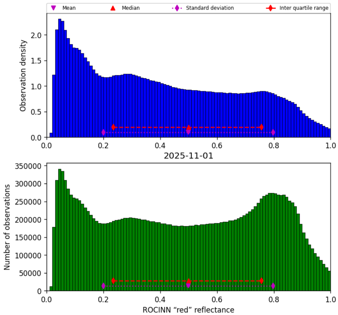
Figure 51: Histogram of “ROCINN “red” reflectance” for 2025-11-01 to 2025-11-02
