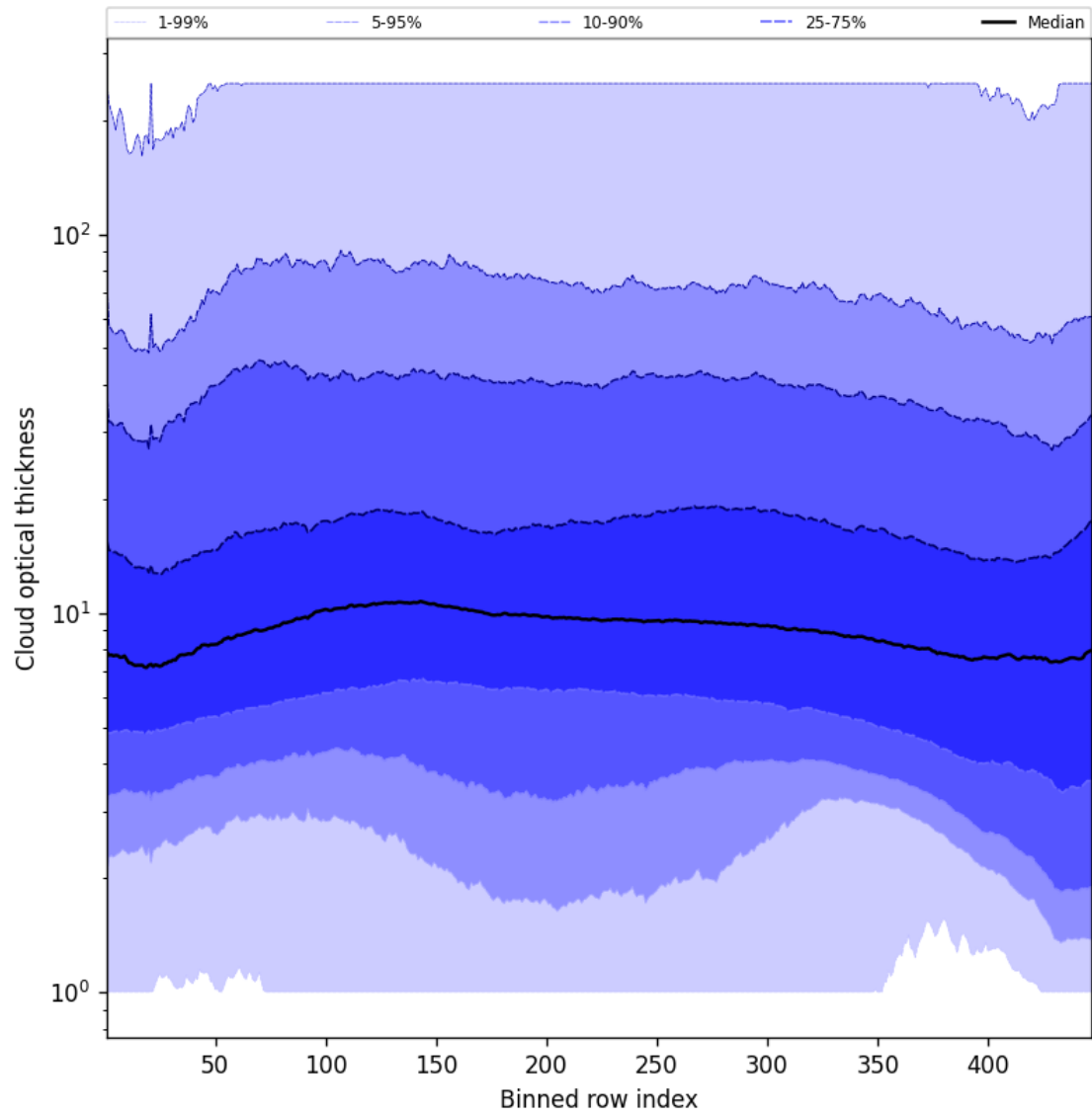
Figure 55: Along track statistics of “Cloud optical thickness” for 2025-11-01 to 2025-11-02
