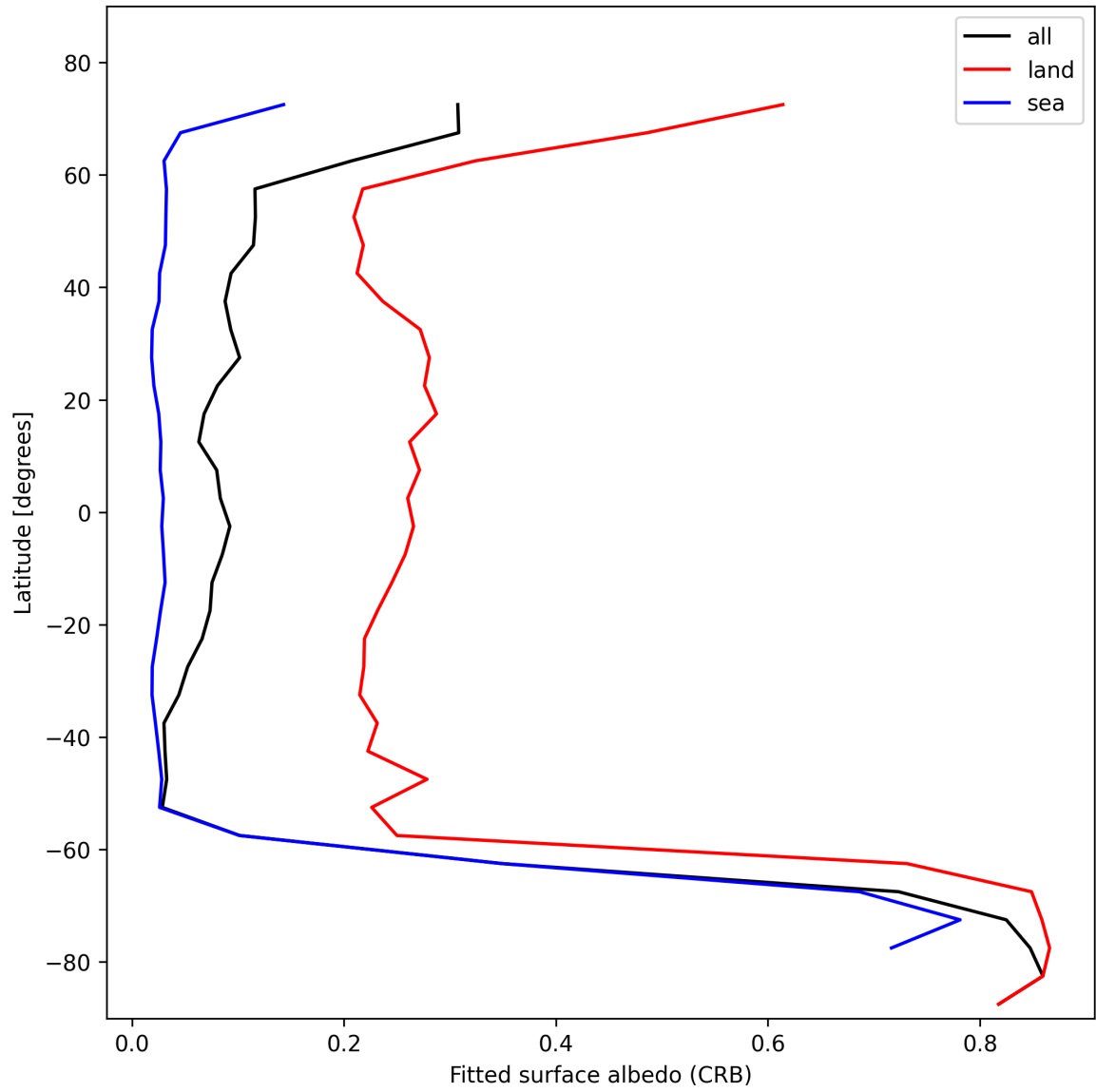
Figure 28: Zonal average of “Fitted surface albedo (CRB)” for 2025-11-01 to 2025-11-02.
