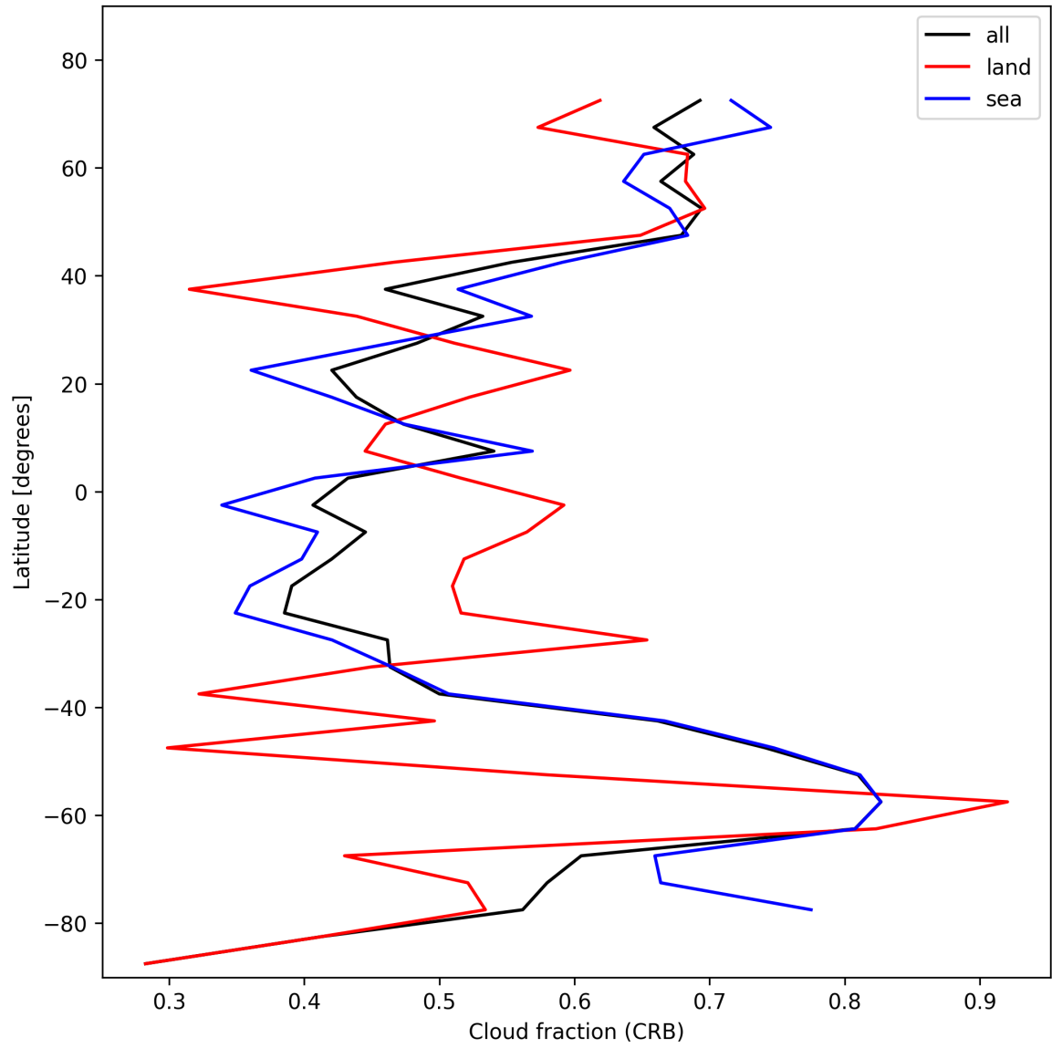
Figure 24: Zonal average of “Cloud fraction (CRB)” for 2025-11-01 to 2025-11-02.
