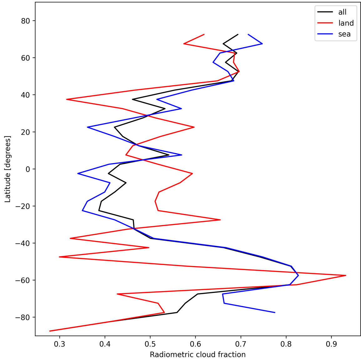
Figure 21: Zonal average of “Radiometric cloud fraction” for 2025-11-01 to 2025-11-02.
