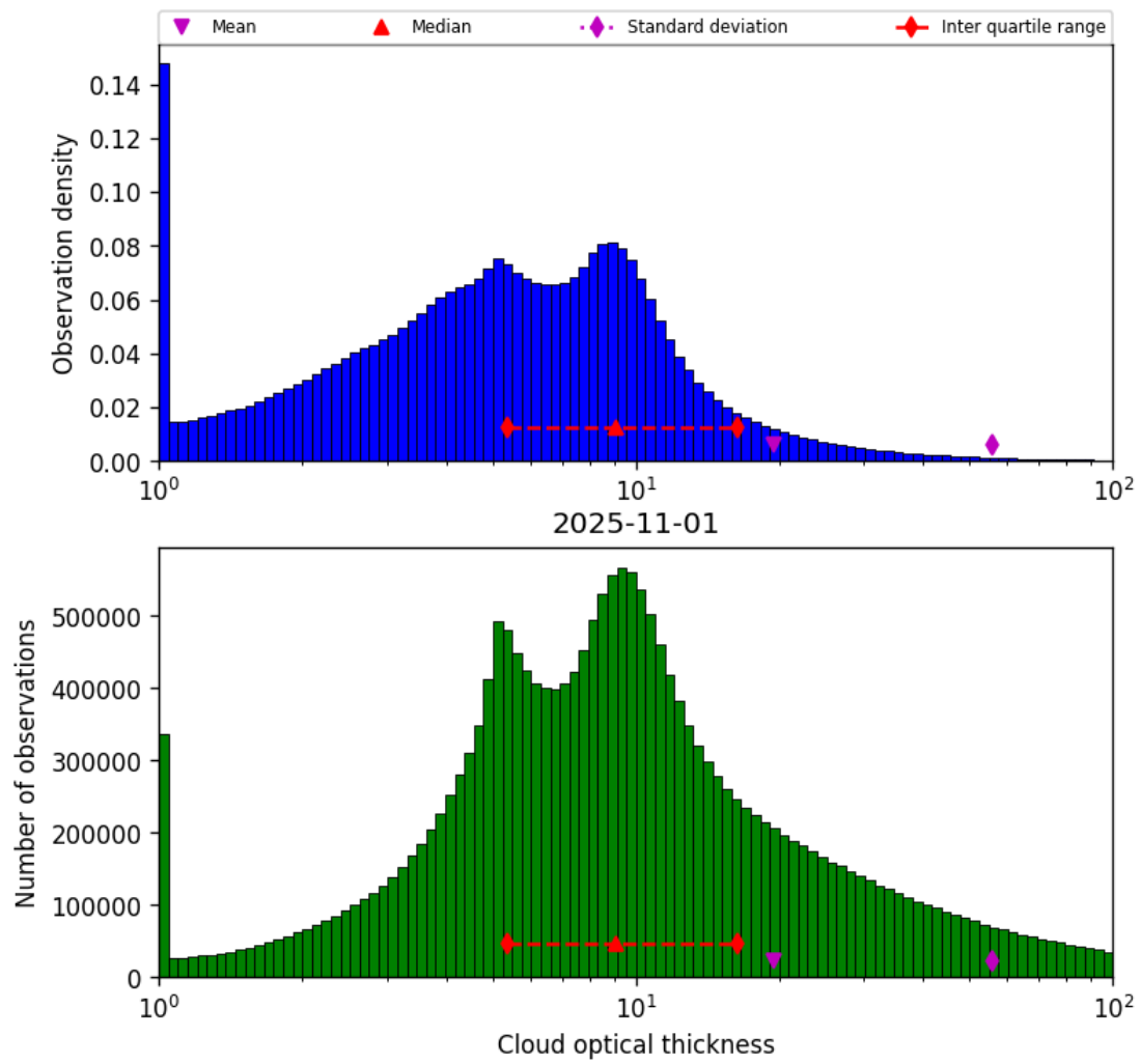
Figure 39: Histogram of “Cloud optical thickness” for 2025-11-01 to 2025-11-02
