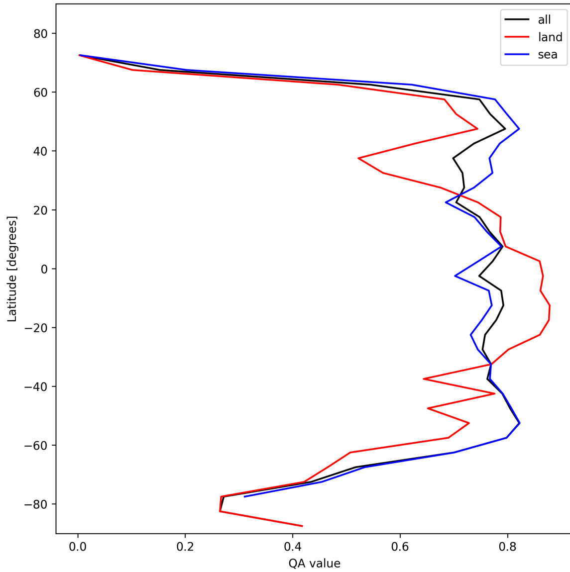
Figure 20: Zonal average of “QA value” for 2025-11-01 to 2025-11-02.
