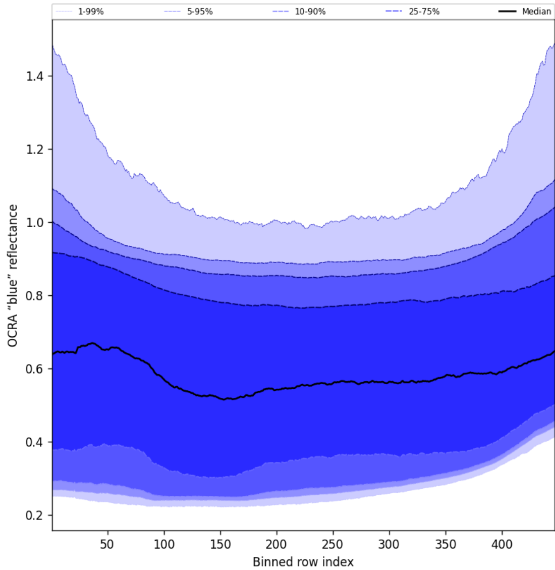
Figure 65: Along track statistics of “OCRA “blue” reflectance” for 2025-11-01 to 2025-11-02
