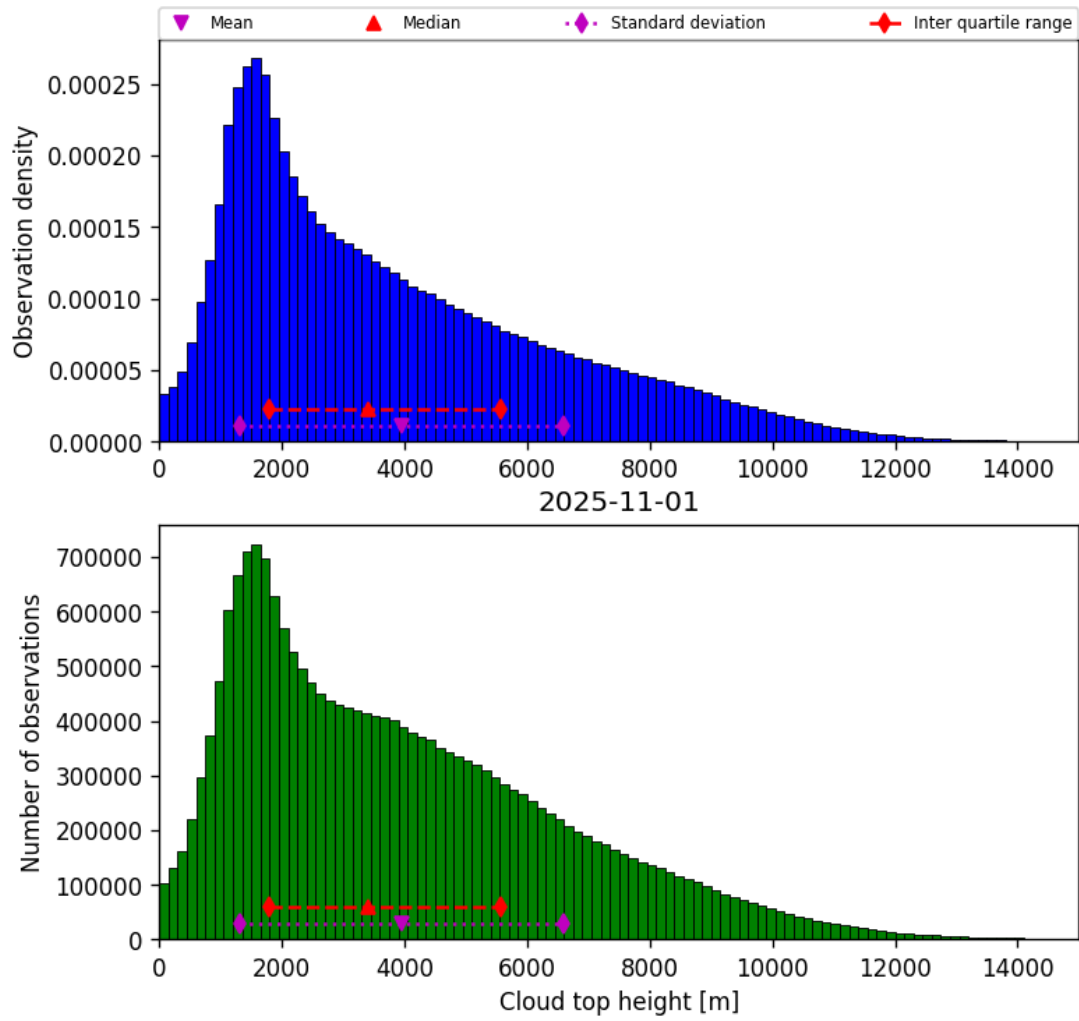
Figure 38: Histogram of “Cloud top height” for 2025-11-01 to 2025-11-02
