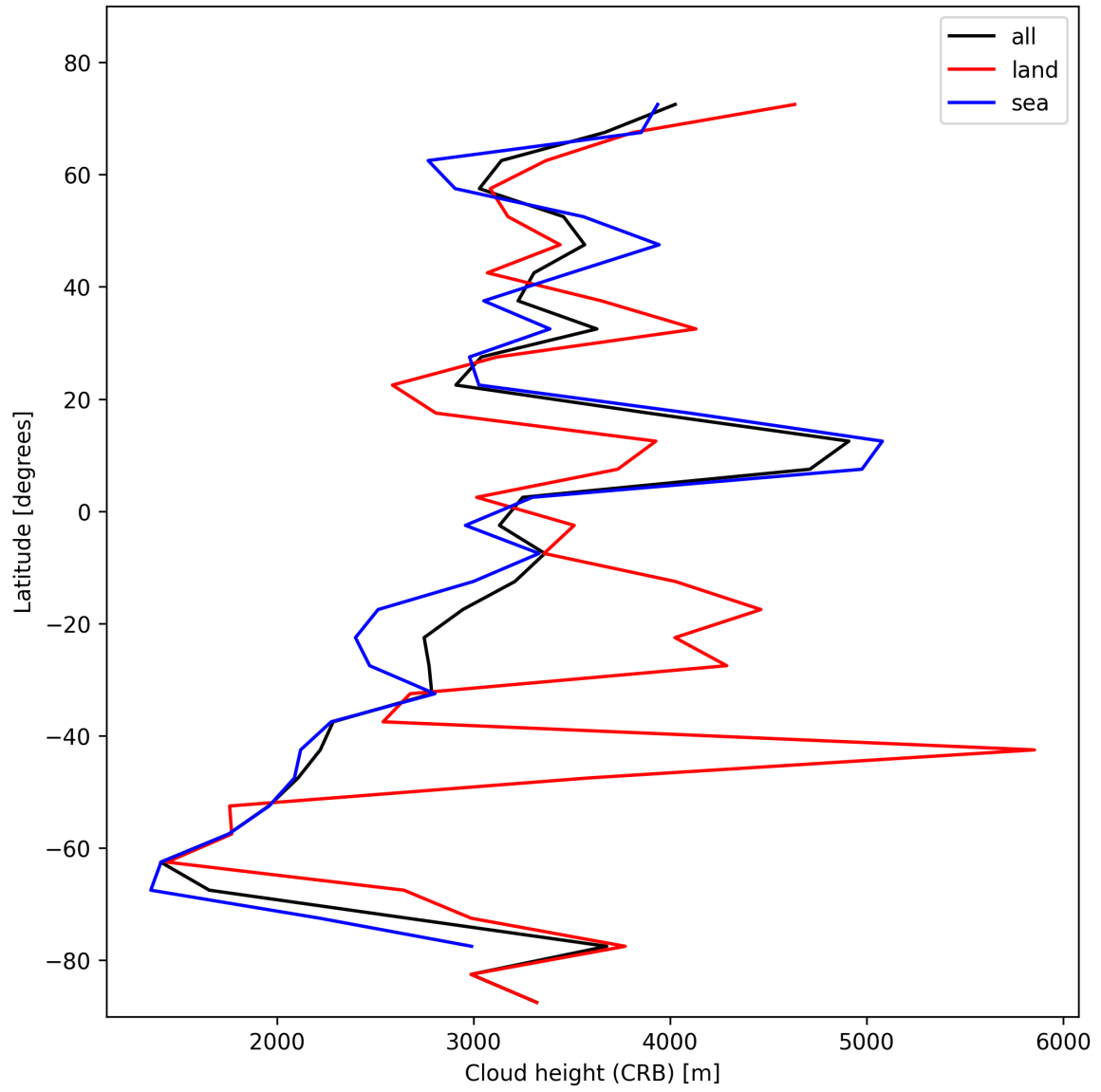
Figure 25: Zonal average of “Cloud height (CRB)” for 2025-11-01 to 2025-11-02.
