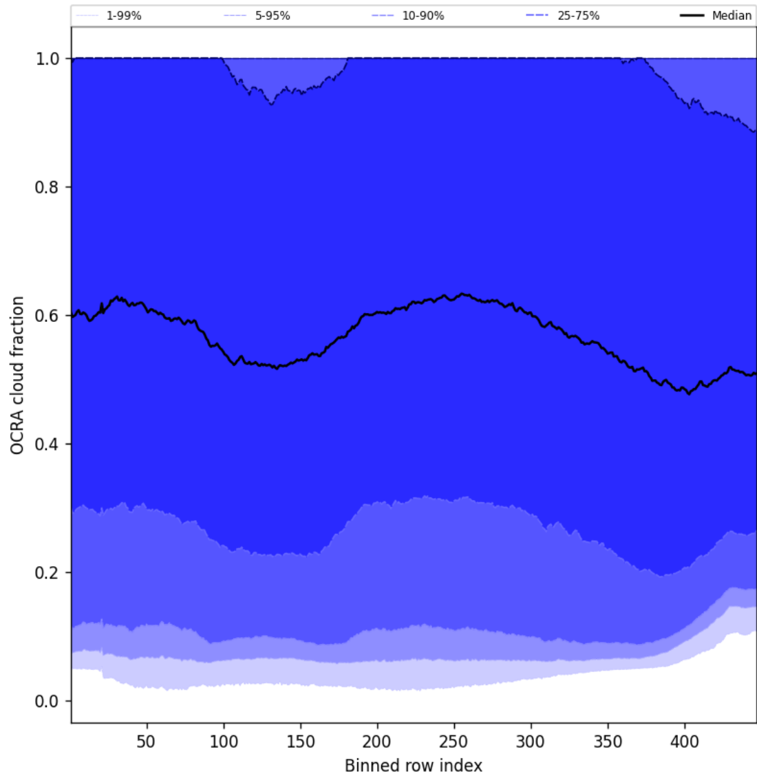
Figure 64: Along track statistics of “OCRA cloud fraction” for 2025-11-01 to 2025-11-02
