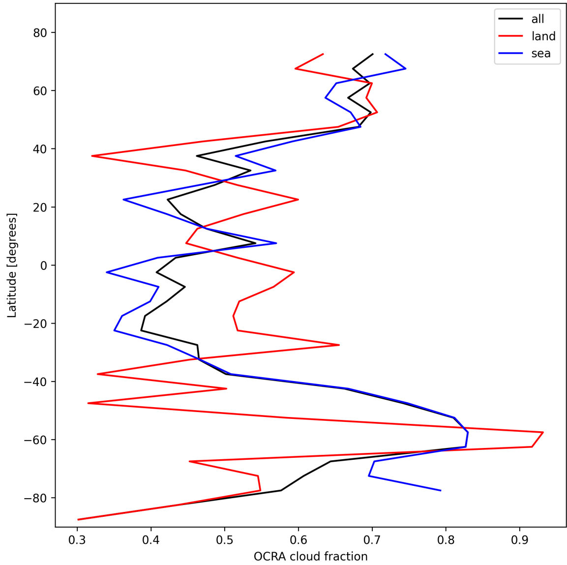
Figure 32: Zonal average of “OCRA cloud fraction” for 2025-11-01 to 2025-11-02.
