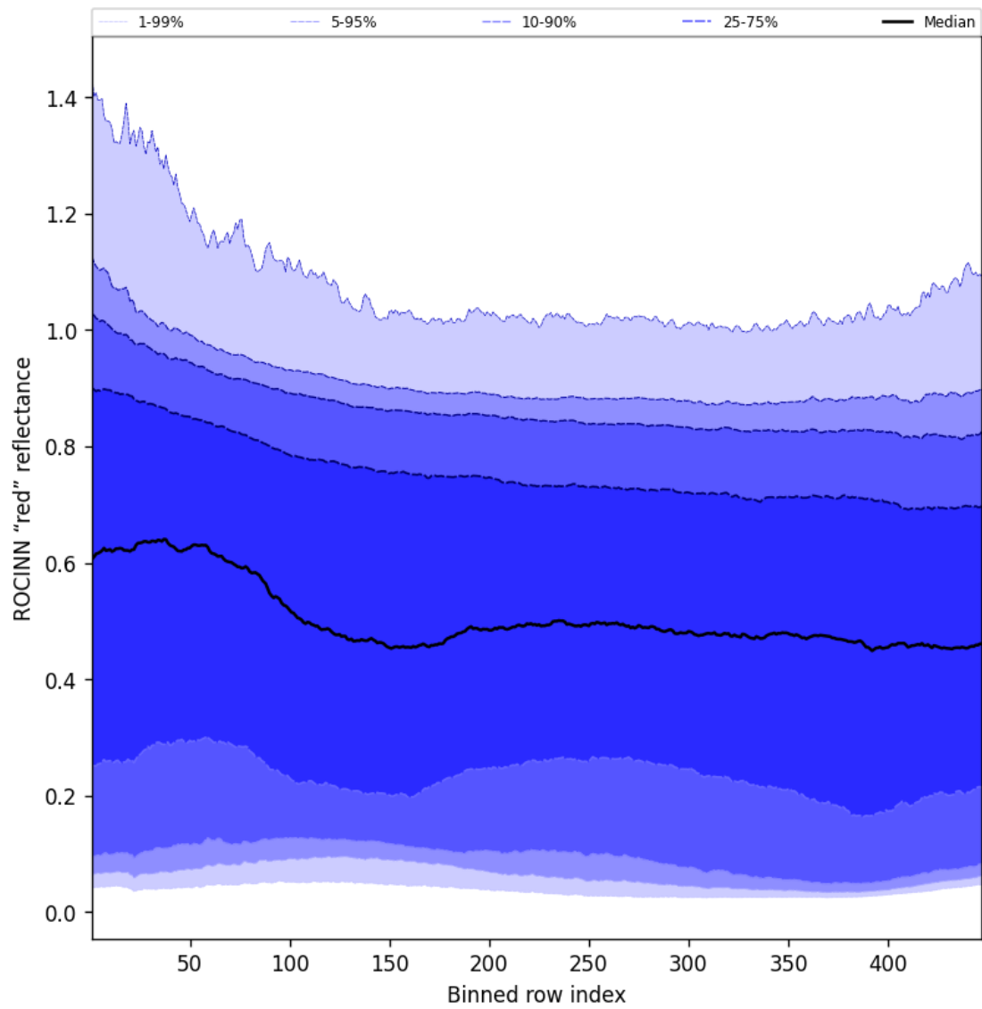
Figure 67: Along track statistics of "ROCINN "red" reflectance" for 2025-11-01 to 2025-11-02
