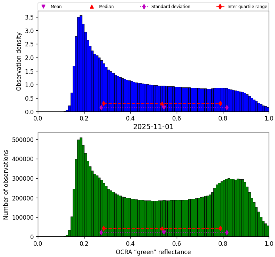
Figure 50: Histogram of “OCRA “green” reflectance” for 2025-11-01 to 2025-11-02
