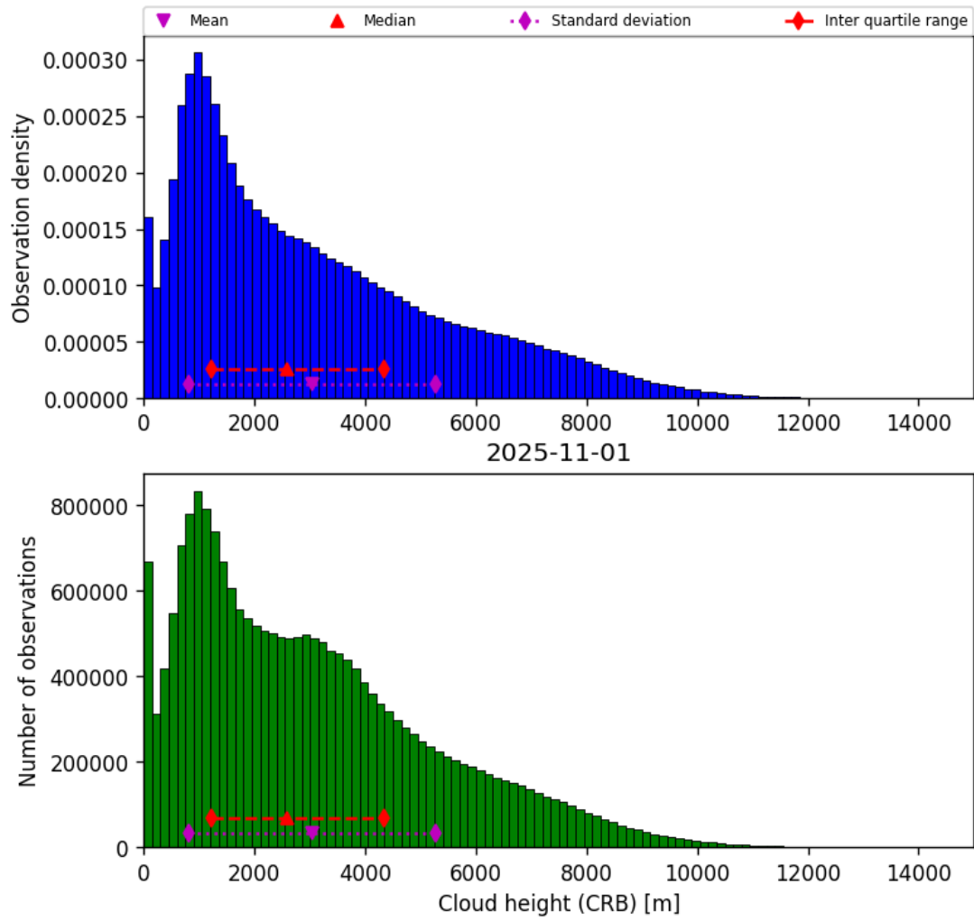
Figure 41: Histogram of “Cloud height (CRB)” for 2025-11-01 to 2025-11-02
