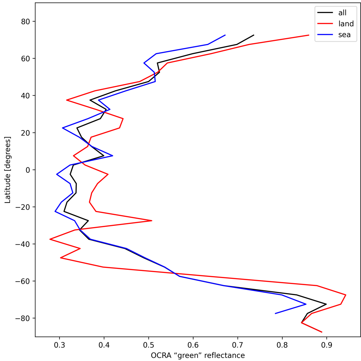
Figure 34: Zonal average of “OCRA “green” reflectance” for 2025-11-01 to 2025-11-02.
