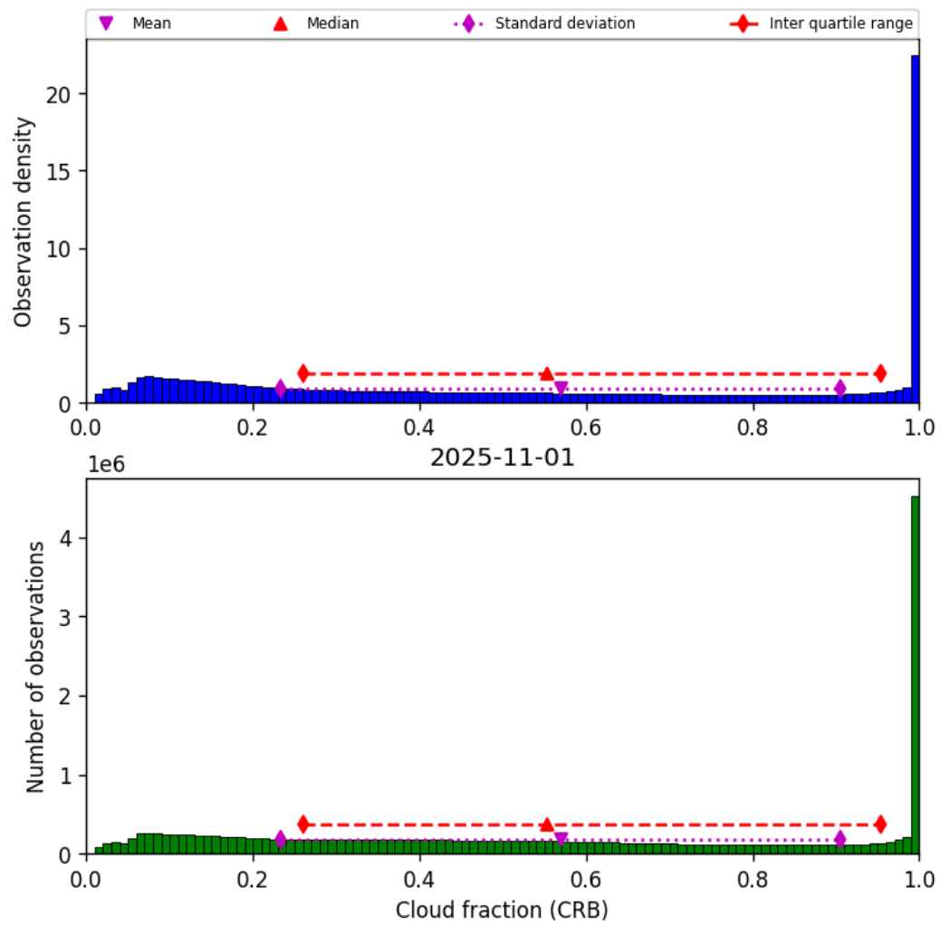
Figure 40: Histogram of “Cloud fraction (CRB)” for 2025-11-01 to 2025-11-02
