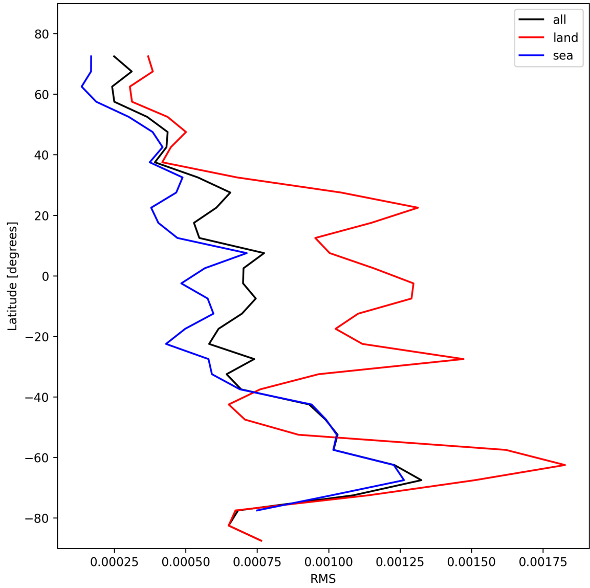
Figure 29: Zonal average of “RMS” for 2025-11-01 to 2025-11-02.
