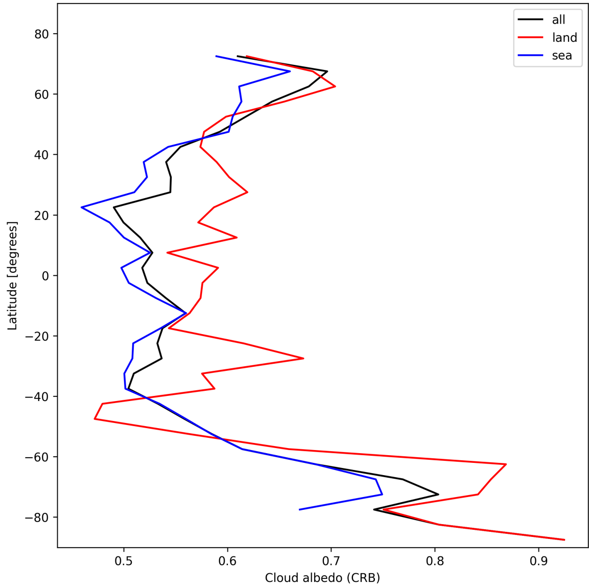
Figure 26: Zonal average of “Cloud albedo (CRB)” for 2025-11-01 to 2025-11-02.
