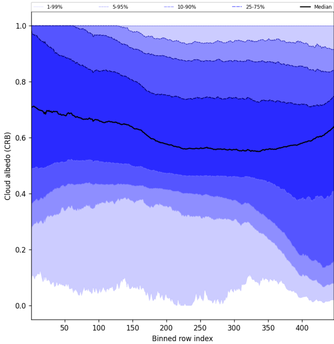
Figure 58: Along track statistics of “Cloud albedo (CRB)” for 2025-11-01 to 2025-11-02
