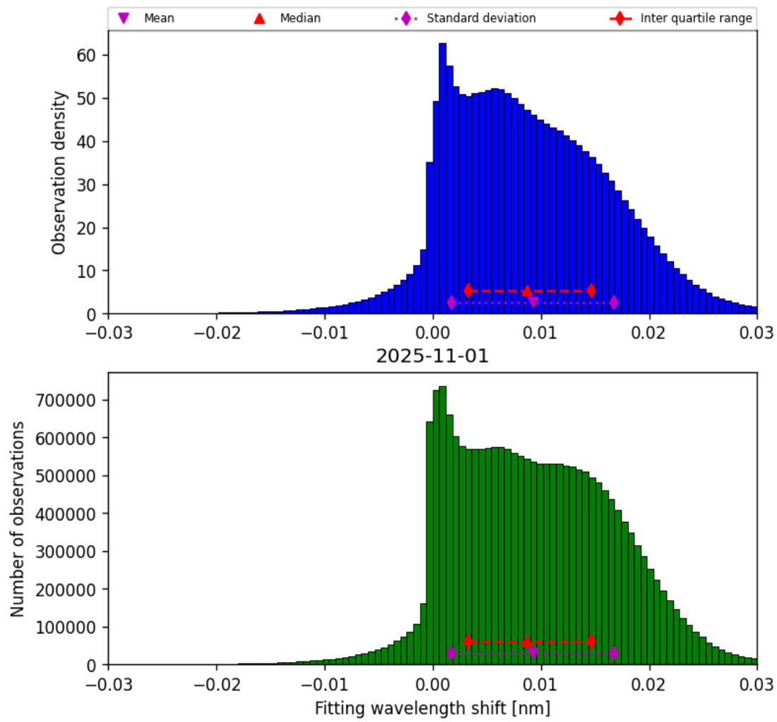
Figure 47: Histogram of “Fitting wavelength shift” for 2025-11-01 to 2025-11-02
