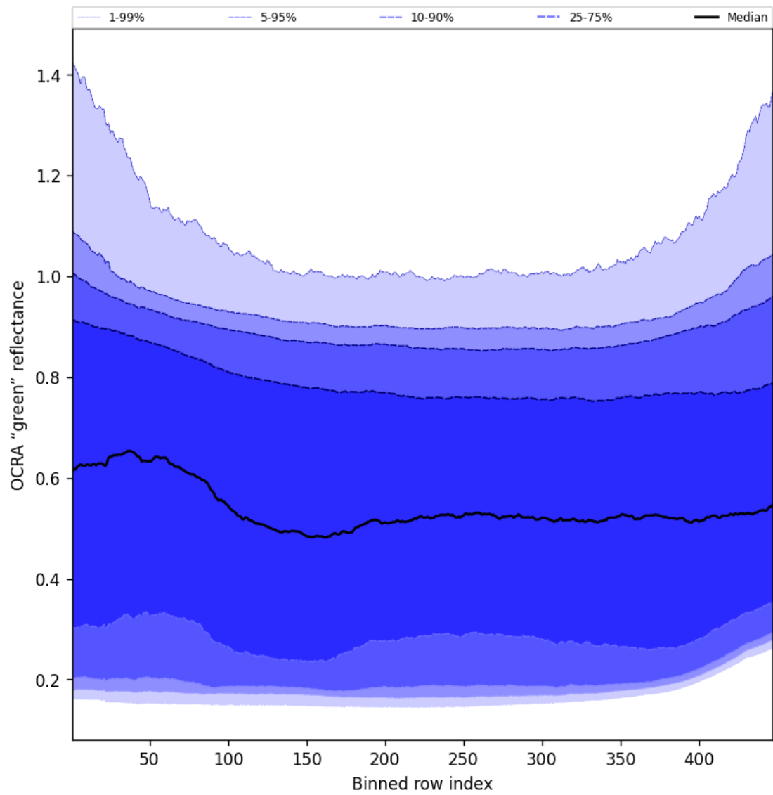
Figure 66: Along track statistics of “OCRA “green” reflectance” for 2025-11-01 to 2025-11-02
