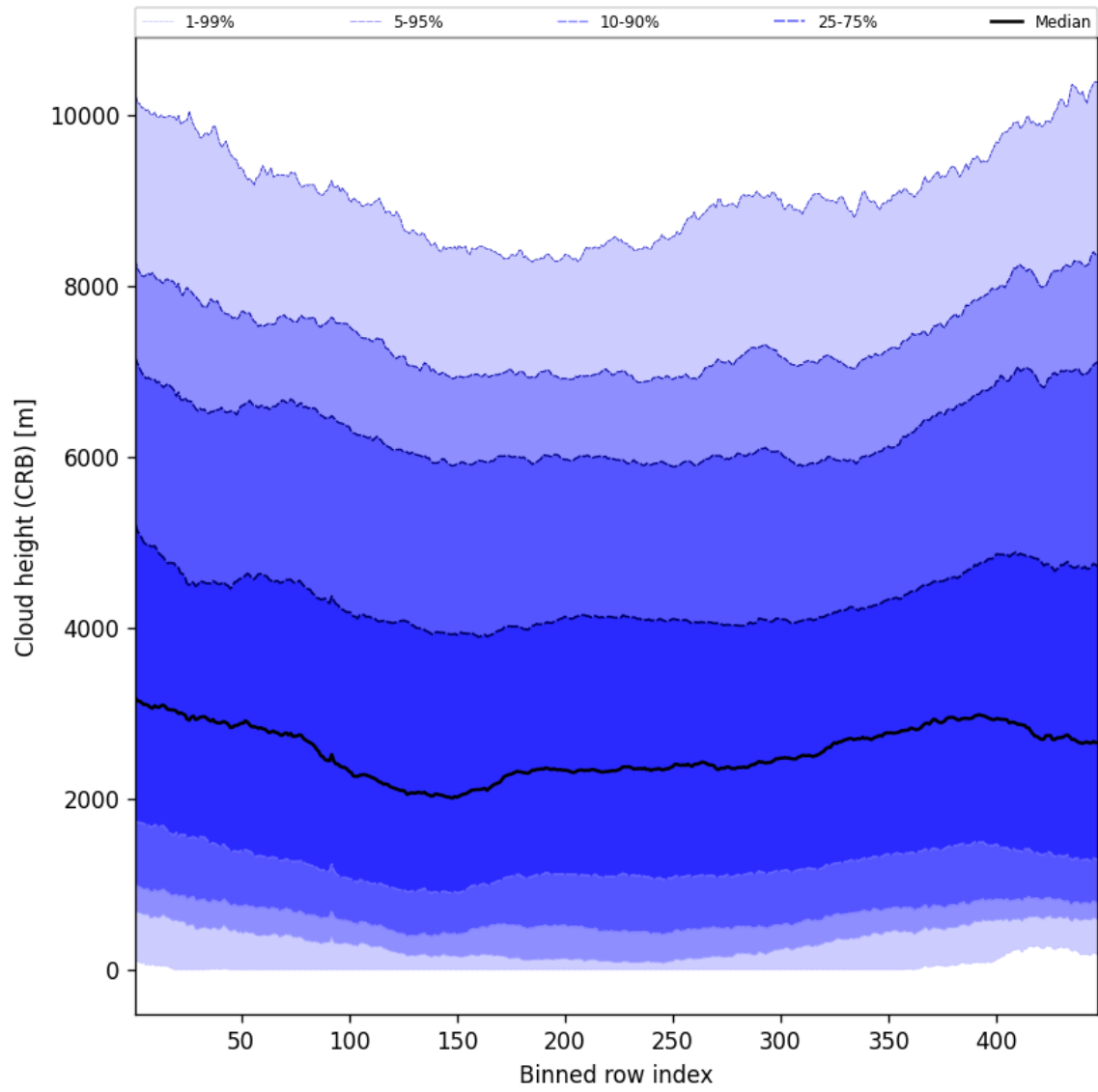
Figure 57: Along track statistics of “Cloud height (CRB)” for 2025-11-01 to 2025-11-02
