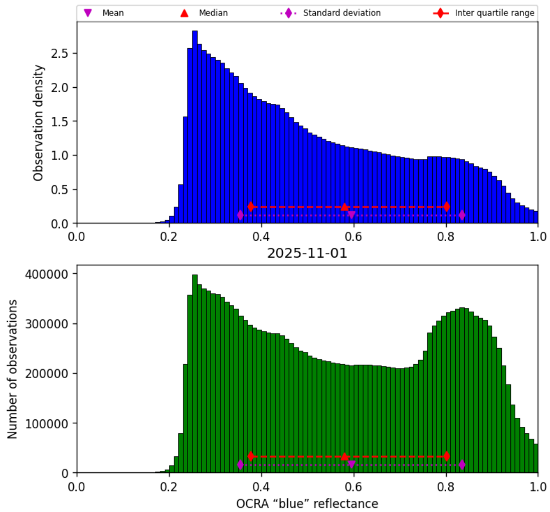
Figure 49: Histogram of “OCRA “blue” reflectance” for 2025-11-01 to 2025-11-02
