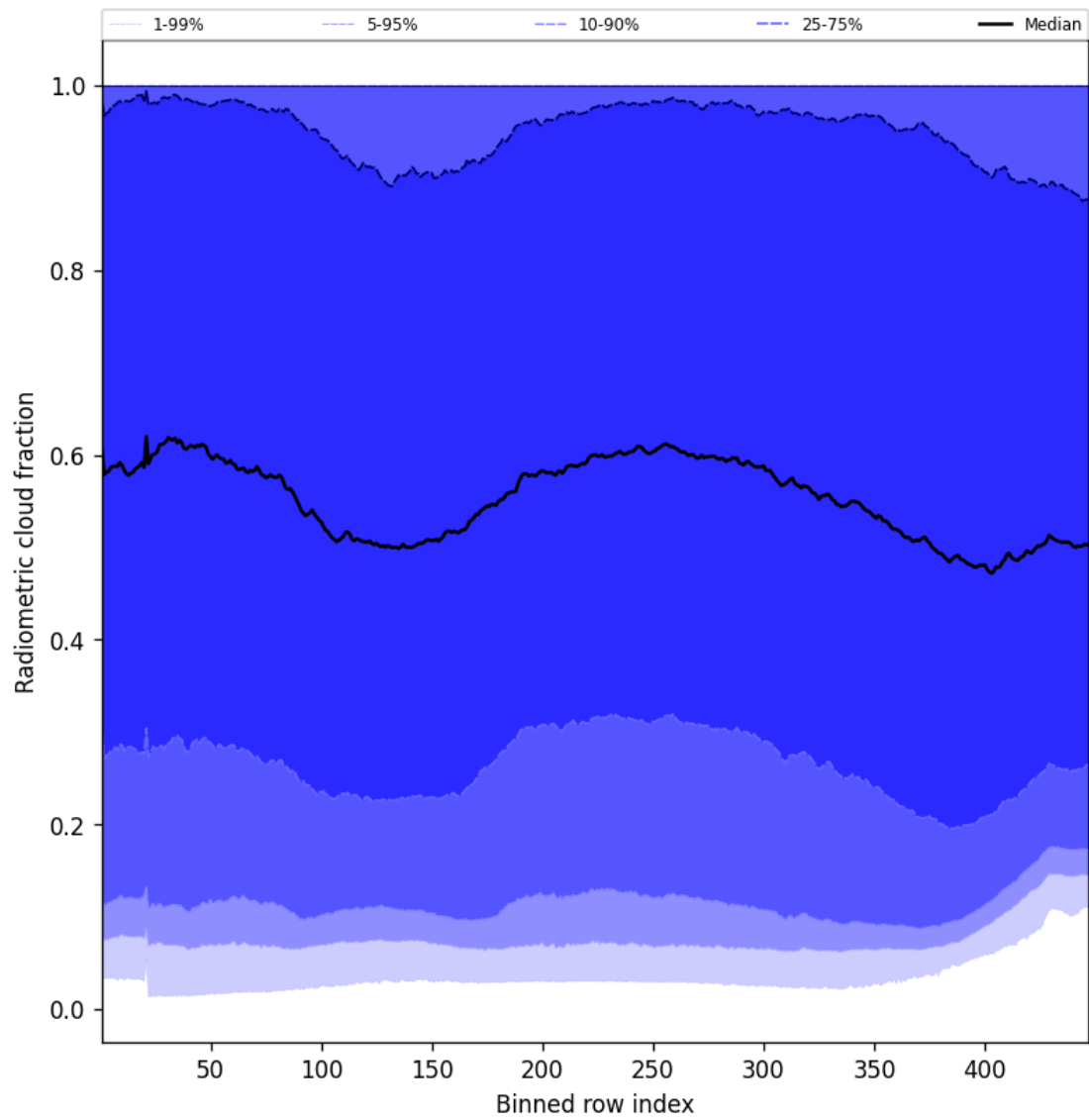
Figure 53: Along track statistics of “Radiometric cloud fraction” for 2025-11-01 to 2025-11-02
