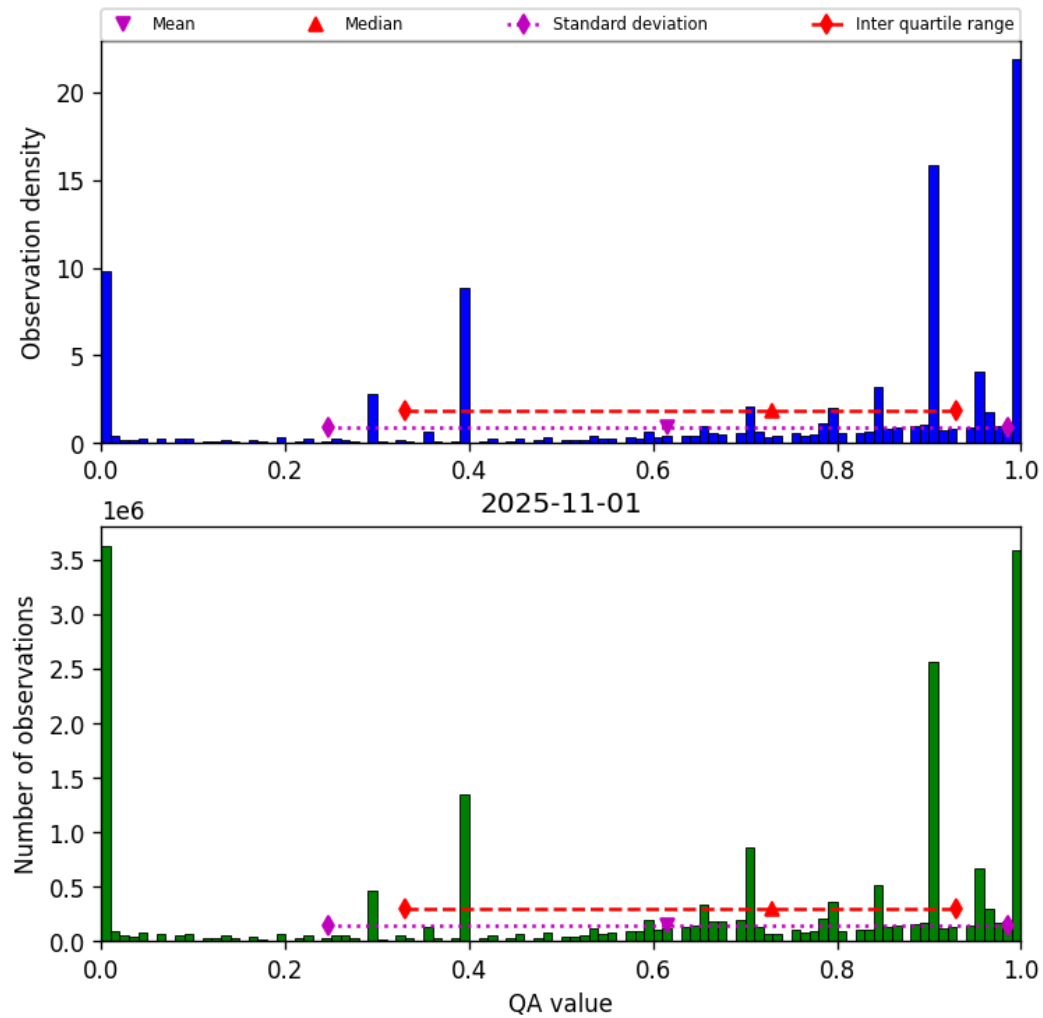
Figure 36: Histogram of “QA value” for 2025-11-01 to 2025-11-02
