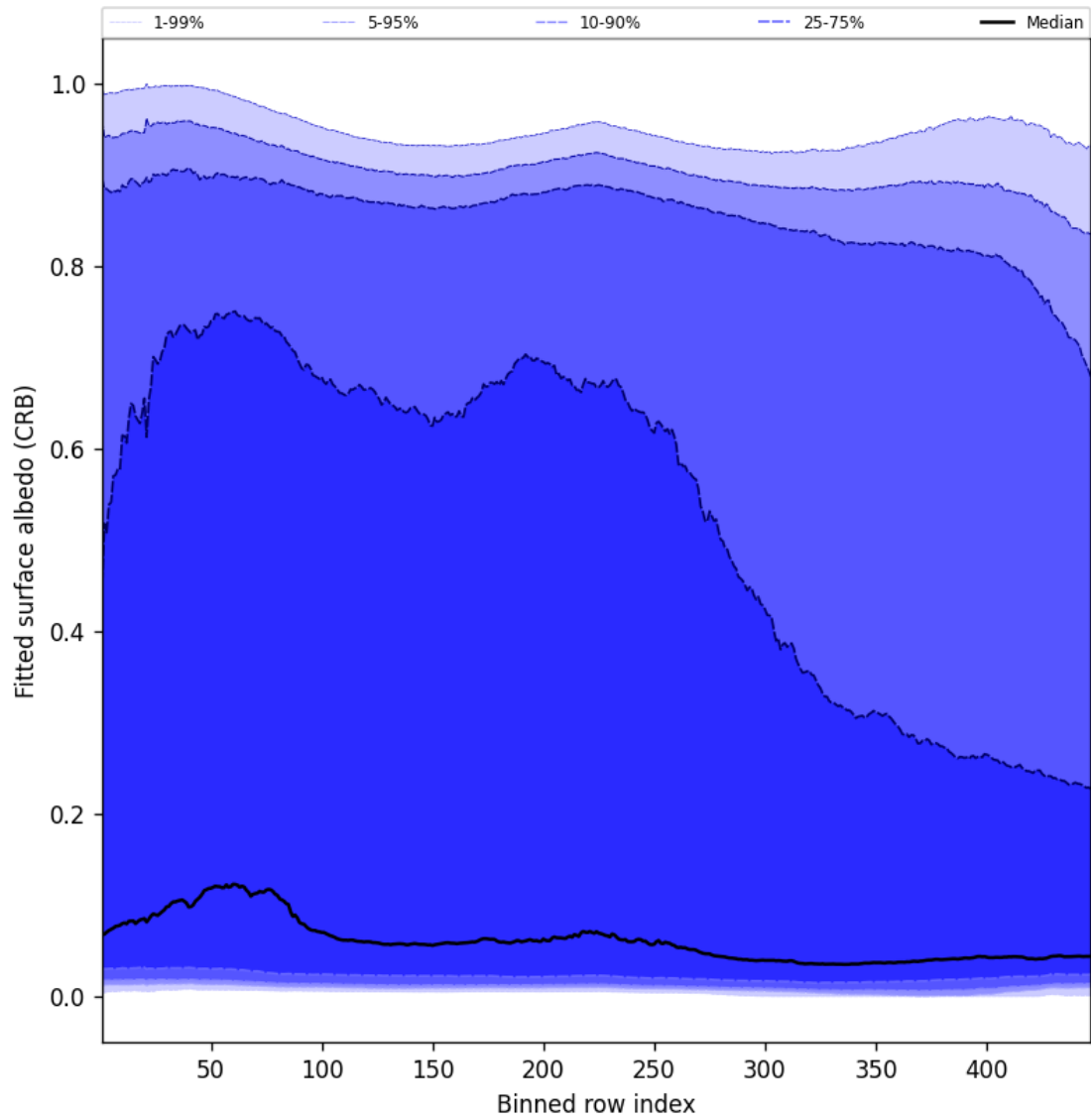
Figure 60: Along track statistics of “Fitted surface albedo (CRB)” for 2025-11-01 to 2025-11-02
