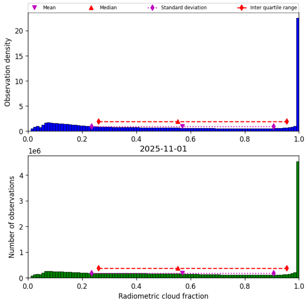
Figure 37: Histogram of “Radiometric cloud fraction” for 2025-11-01 to 2025-11-02
