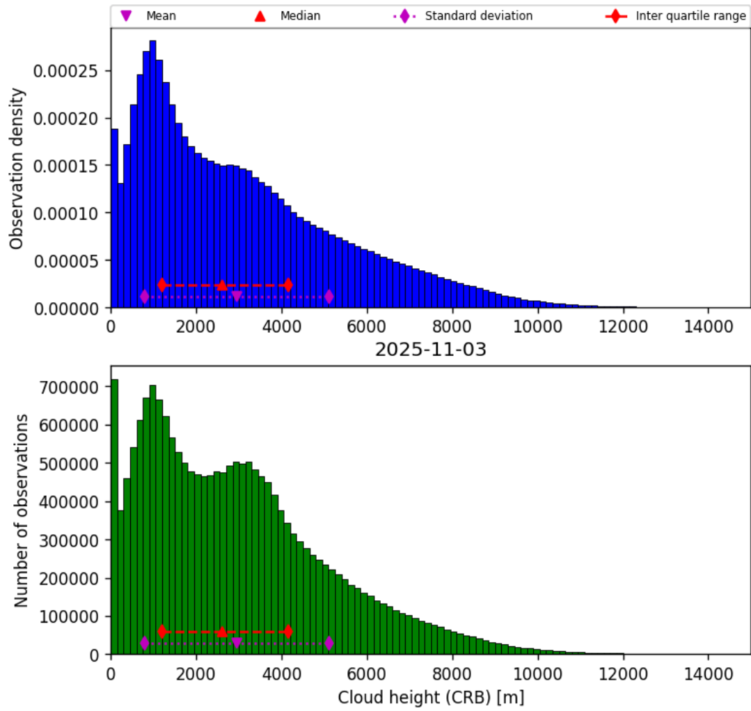
Figure 41: Histogram of “Cloud height (CRB)” for 2025-11-03 to 2025-11-04
