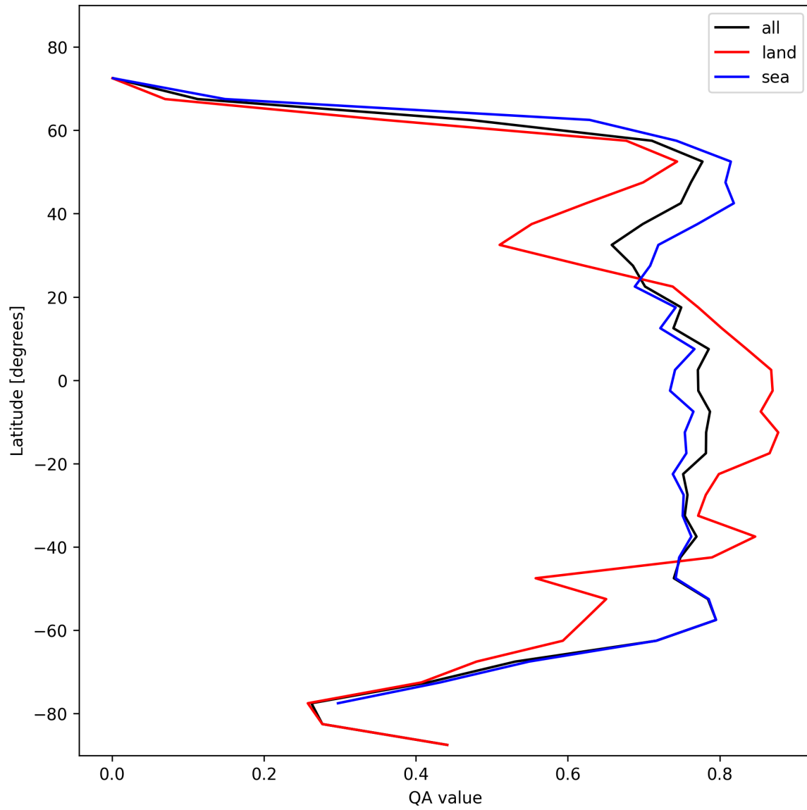
Figure 20: Zonal average of “QA value” for 2025-11-03 to 2025-11-04.
