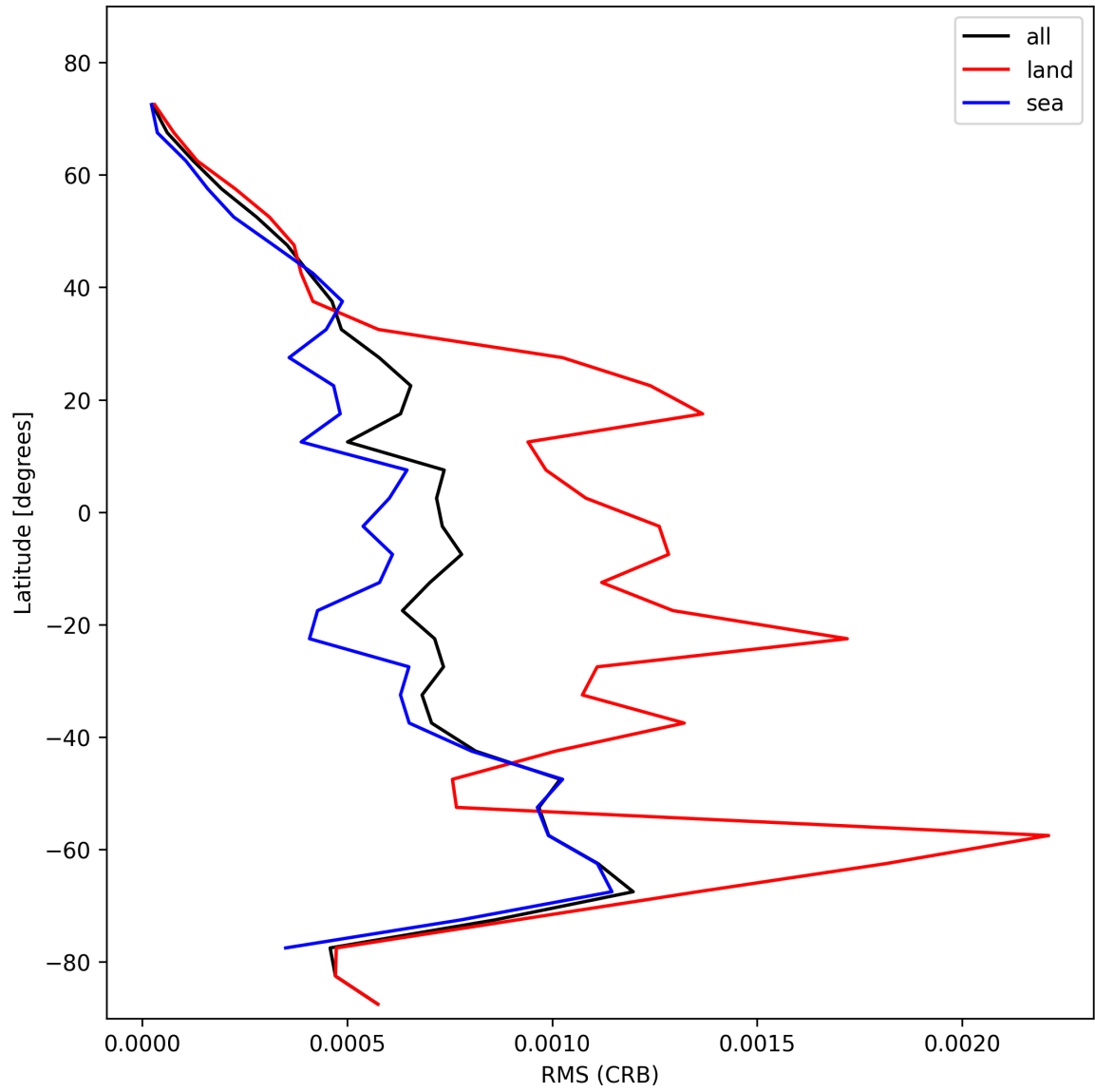
Figure 30: Zonal average of “RMS (CRB)” for 2025-11-03 to 2025-11-04.
