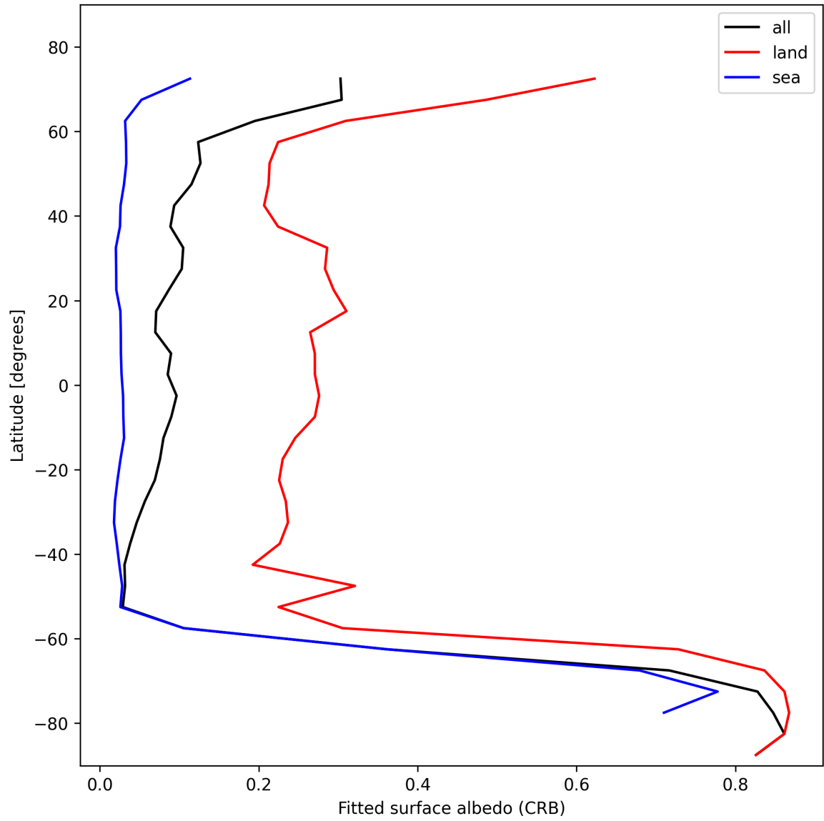
Figure 28: Zonal average of “Fitted surface albedo (CRB)” for 2025-11-03 to 2025-11-04.
