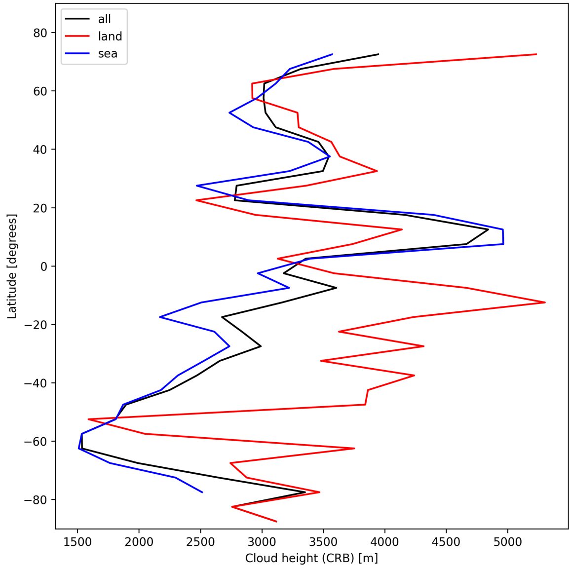
Figure 25: Zonal average of “Cloud height (CRB)” for 2025-11-03 to 2025-11-04.
