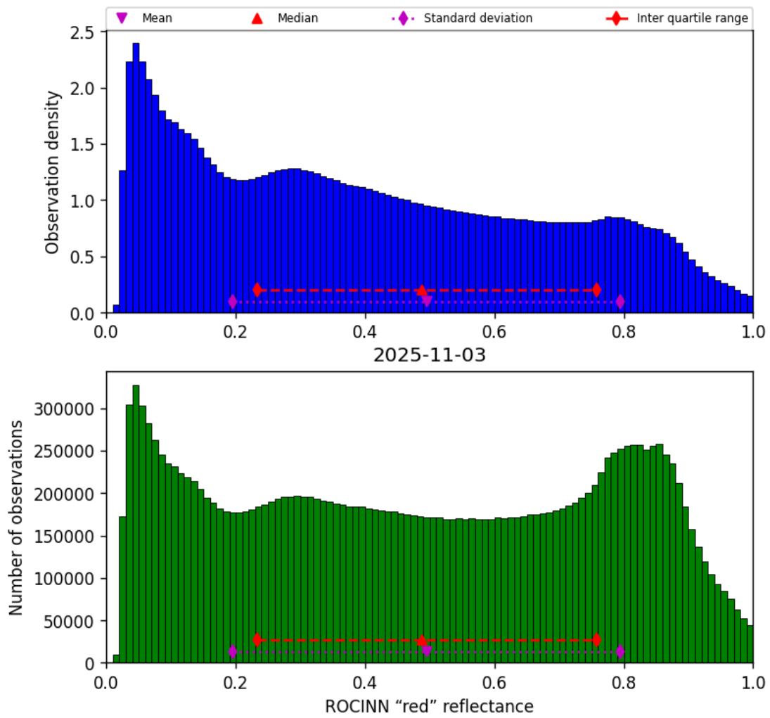
Figure 51: Histogram of “ROCINN “red” reflectance” for 2025-11-03 to 2025-11-04
