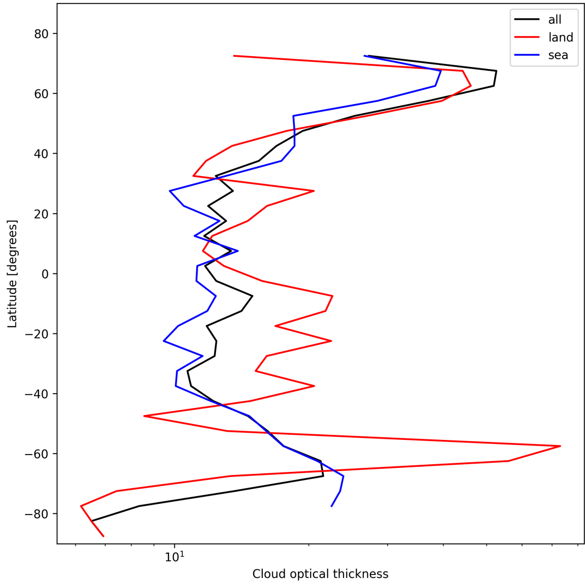
Figure 23: Zonal average of “Cloud optical thickness” for 2025-11-03 to 2025-11-04.
