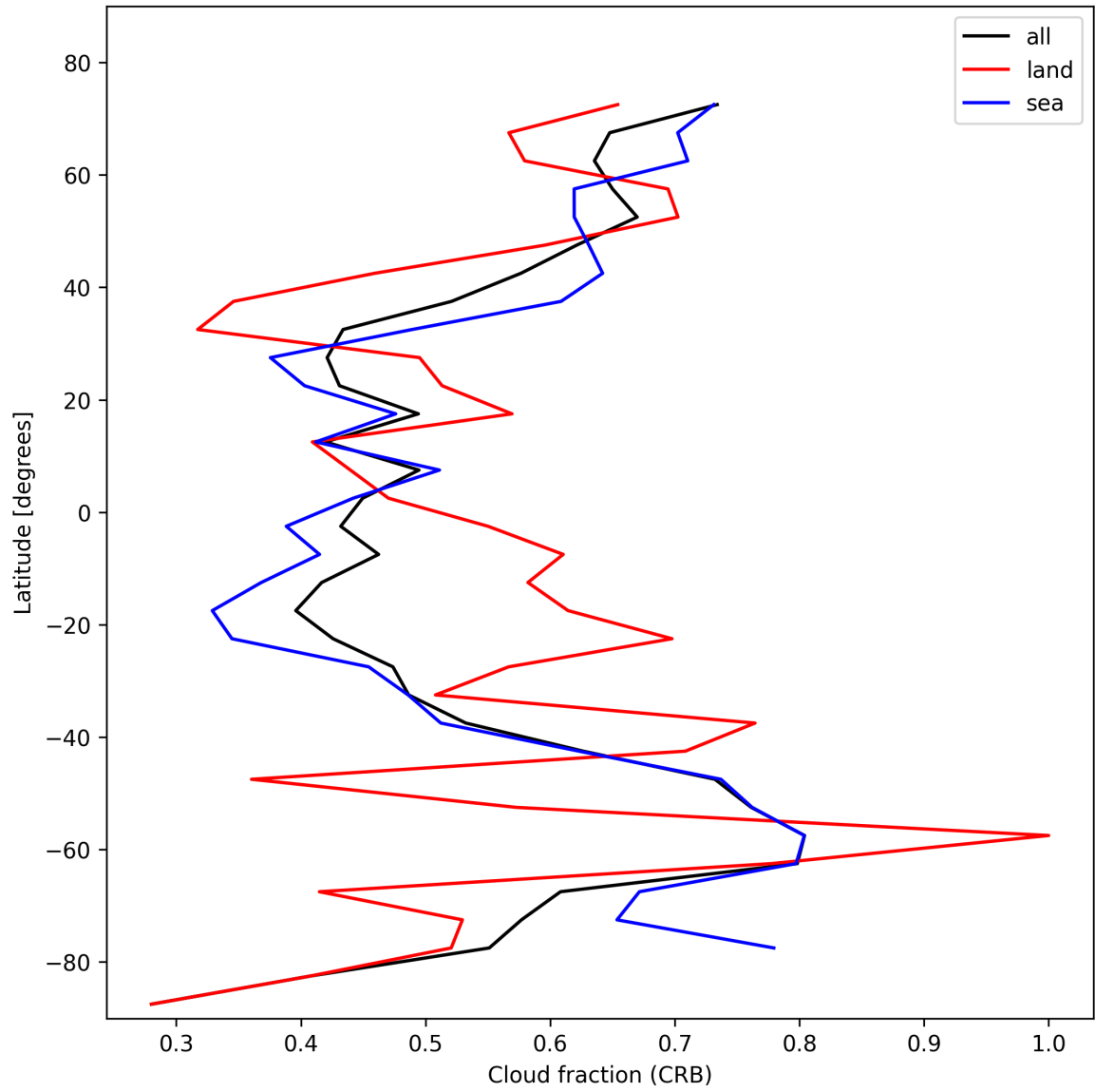
Figure 24: Zonal average of “Cloud fraction (CRB)” for 2025-11-03 to 2025-11-04.
