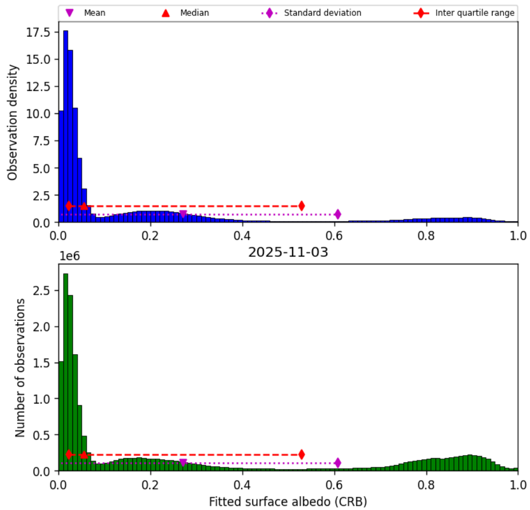
Figure 44: Histogram of “Fitted surface albedo (CRB)” for 2025-11-03 to 2025-11-04
