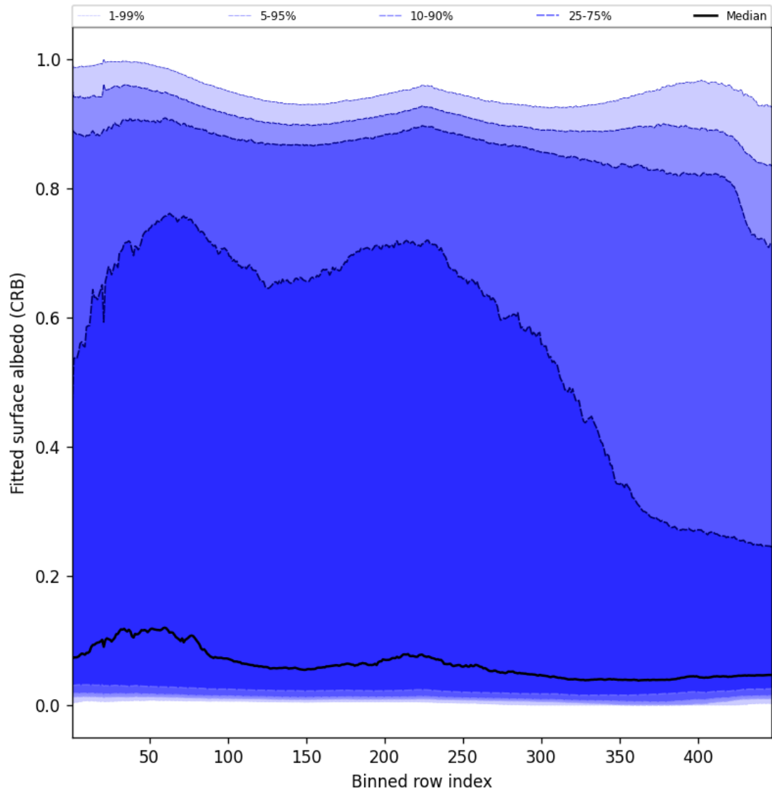
Figure 60: Along track statistics of “Fitted surface albedo (CRB)” for 2025-11-03 to 2025-11-04
