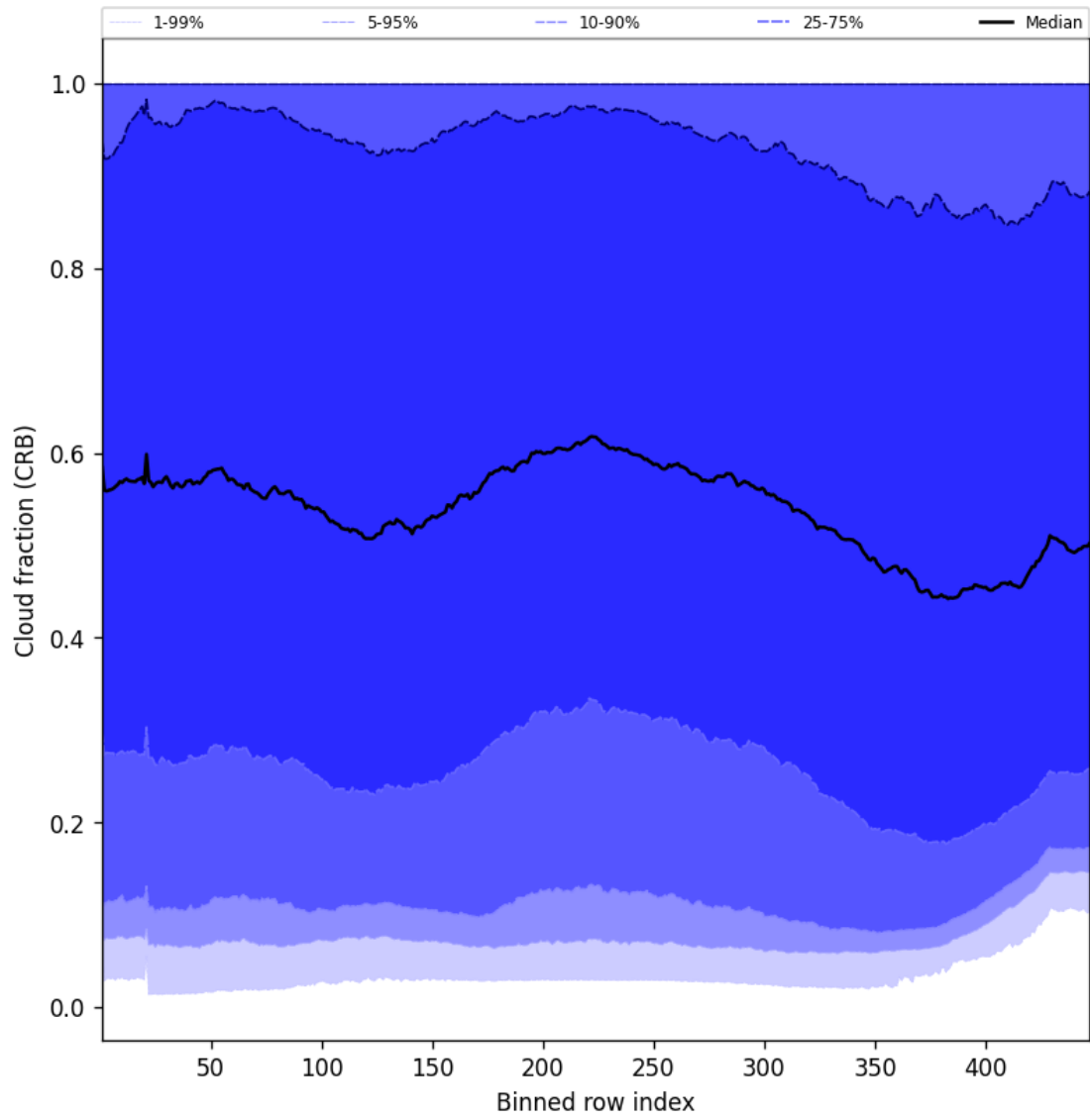
Figure 56: Along track statistics of “Cloud fraction (CRB)” for 2025-11-03 to 2025-11-04
