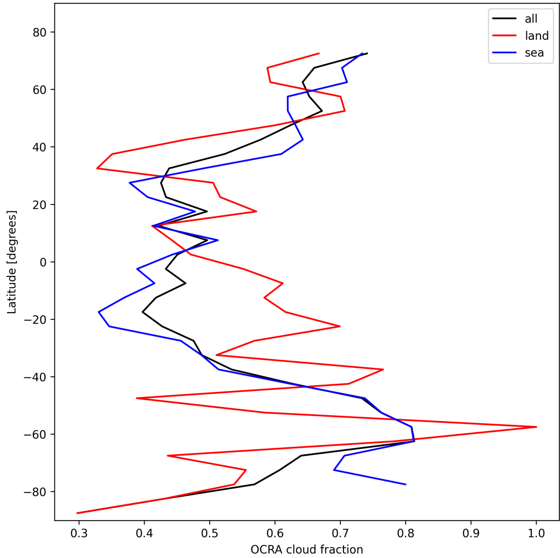
Figure 32: Zonal average of “OCRA cloud fraction” for 2025-11-03 to 2025-11-04.
