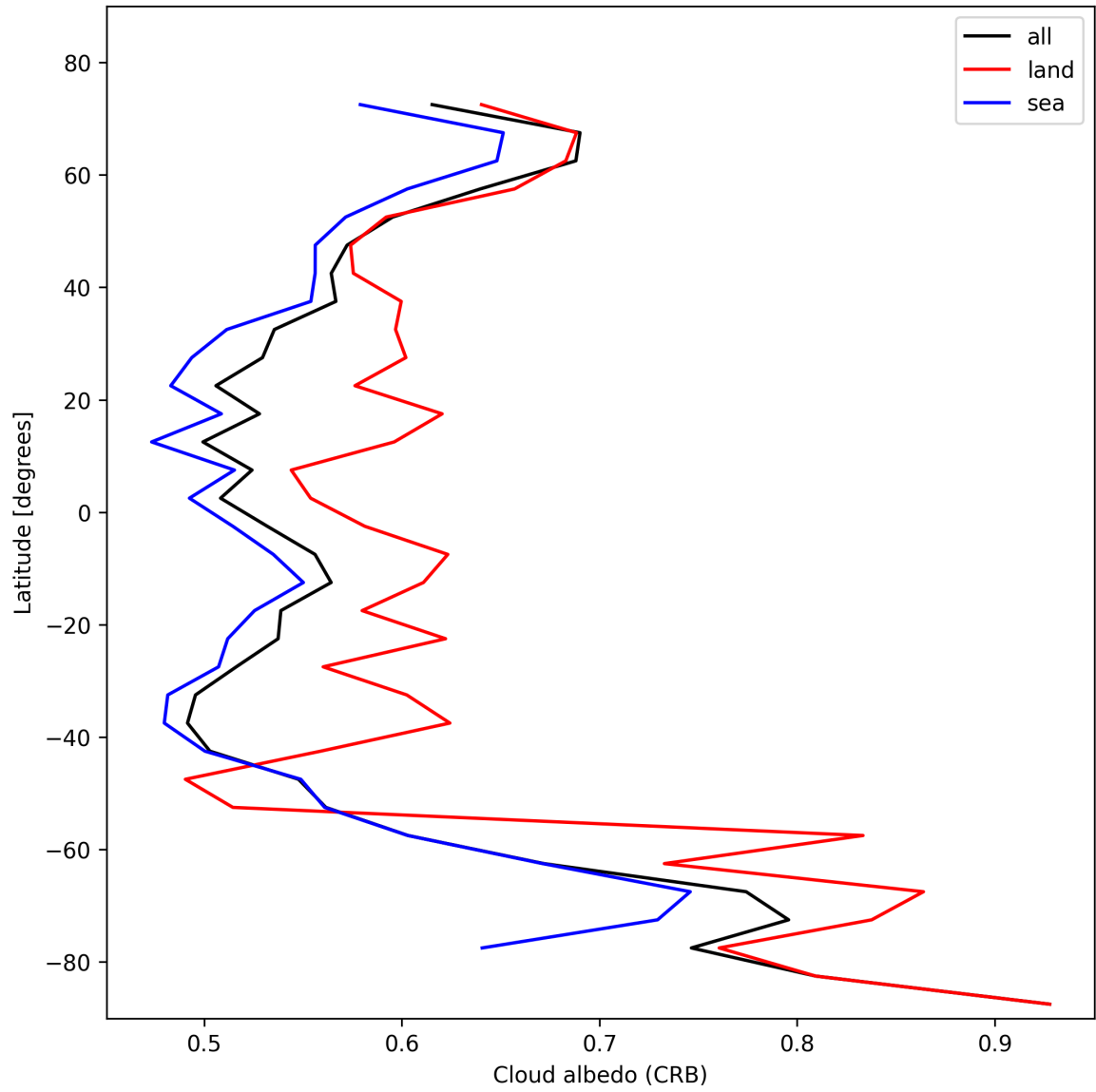
Figure 26: Zonal average of “Cloud albedo (CRB)” for 2025-11-03 to 2025-11-04.
