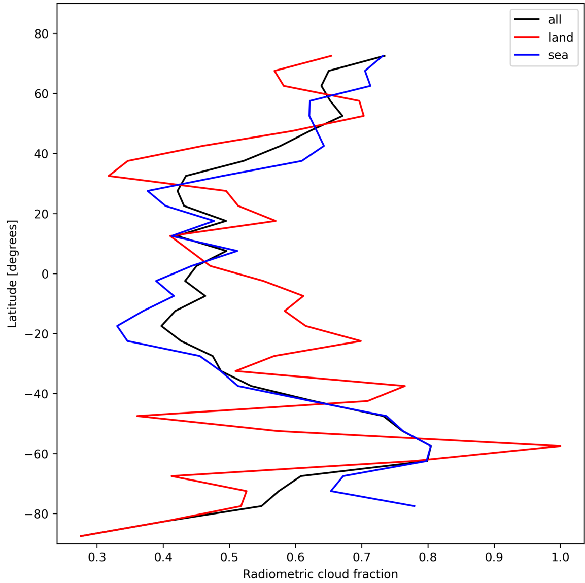
Figure 21: Zonal average of “Radiometric cloud fraction” for 2025-11-03 to 2025-11-04.
