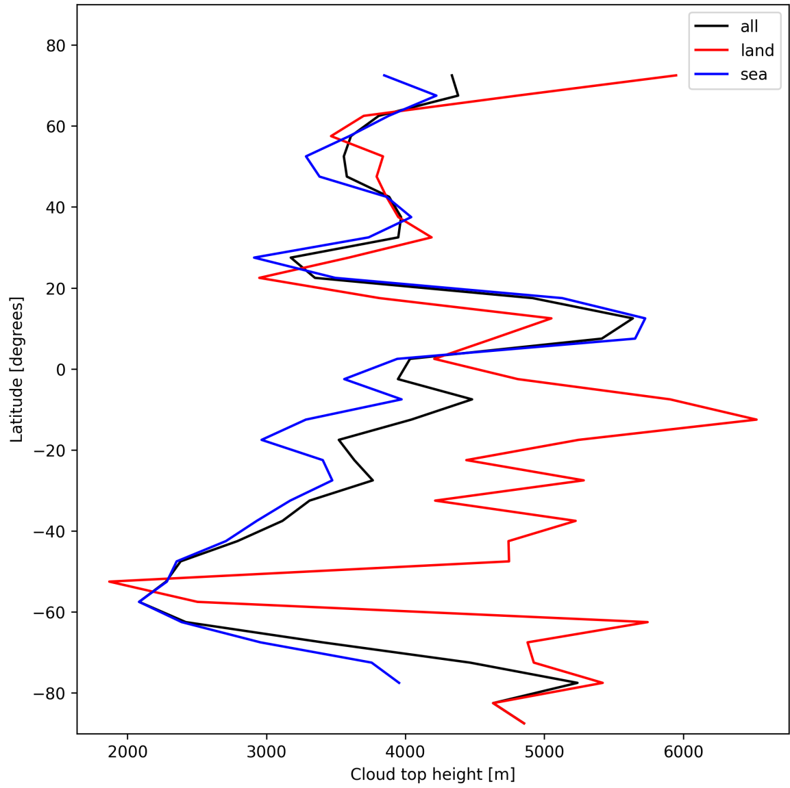
Figure 22: Zonal average of “Cloud top height” for 2025-11-03 to 2025-11-04.
