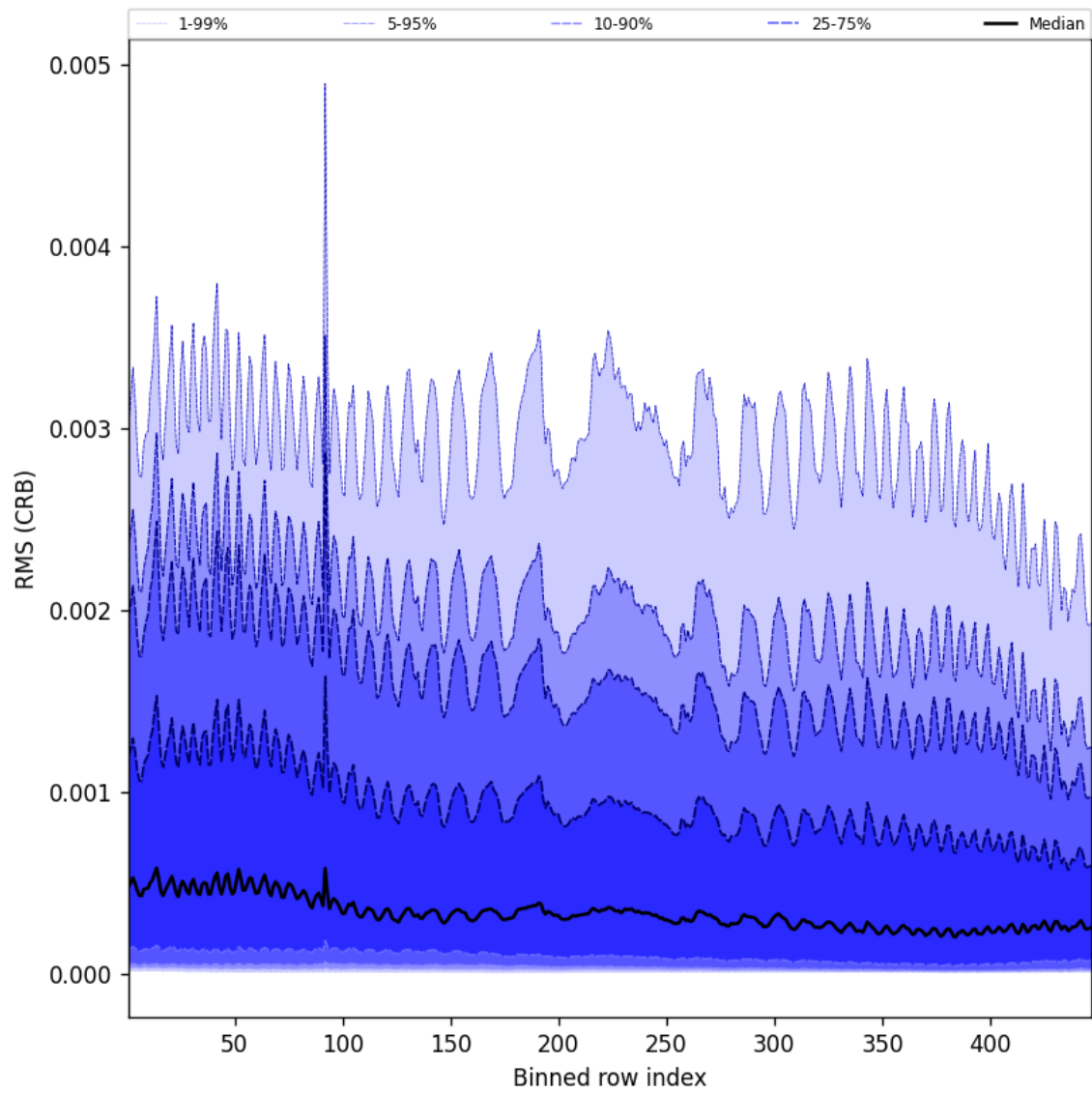
Figure 62: Along track statistics of “RMS (CRB)” for 2025-11-03 to 2025-11-04
