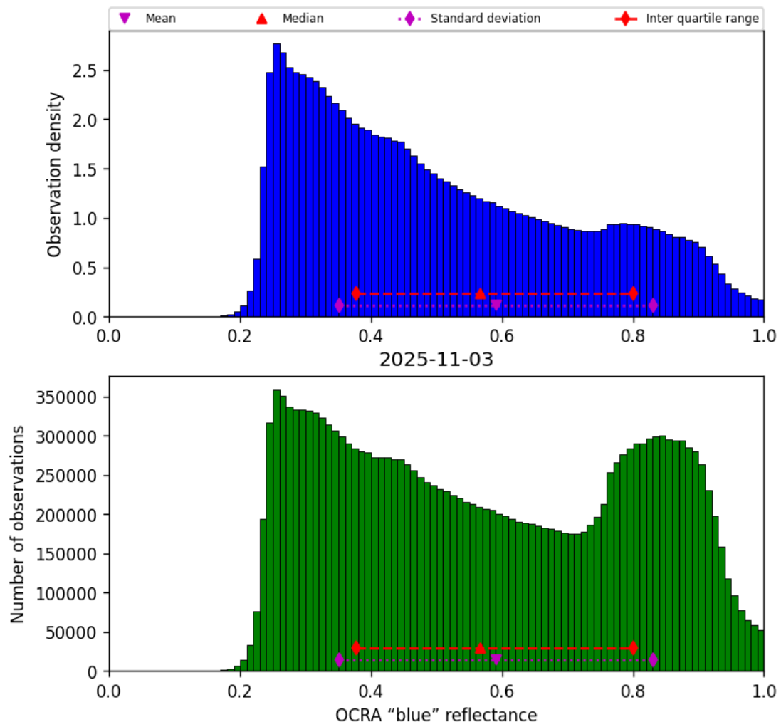
Figure 49: Histogram of “OCRA “blue” reflectance” for 2025-11-03 to 2025-11-04
