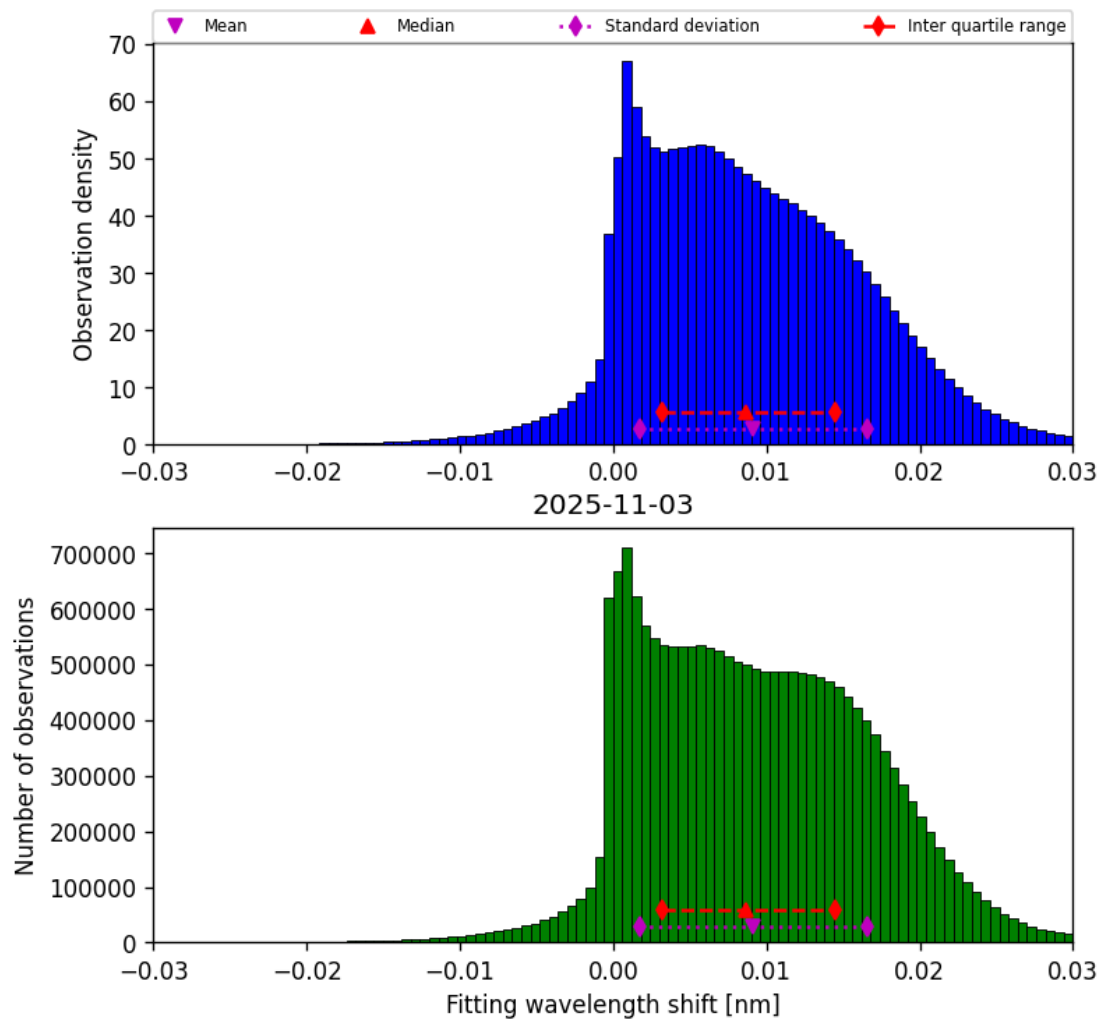
Figure 47: Histogram of “Fitting wavelength shift” for 2025-11-03 to 2025-11-04
