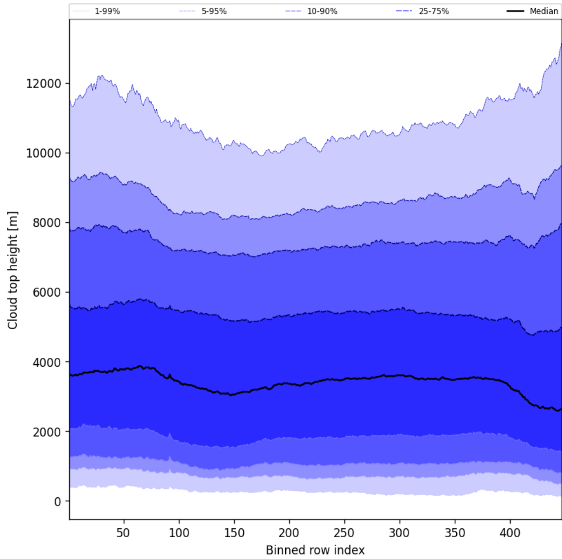
Figure 54: Along track statistics of “Cloud top height” for 2025-11-03 to 2025-11-04
