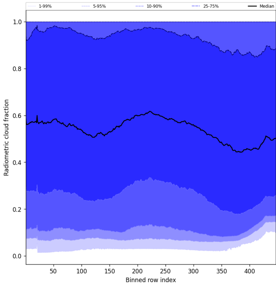
Figure 53: Along track statistics of “Radiometric cloud fraction” for 2025-11-03 to 2025-11-04
