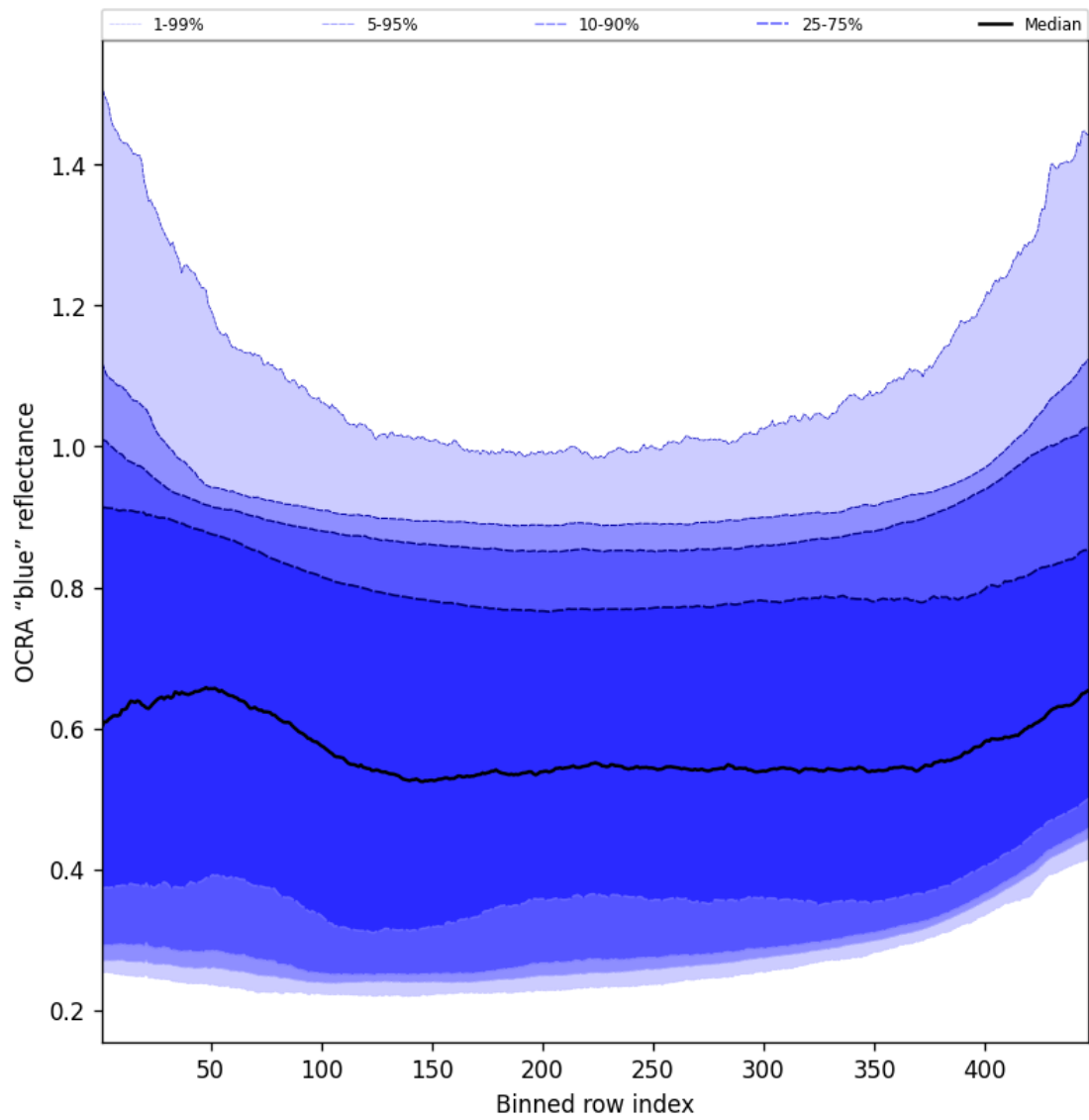
Figure 65: Along track statistics of “OCRA “blue” reflectance” for 2025-11-03 to 2025-11-04
