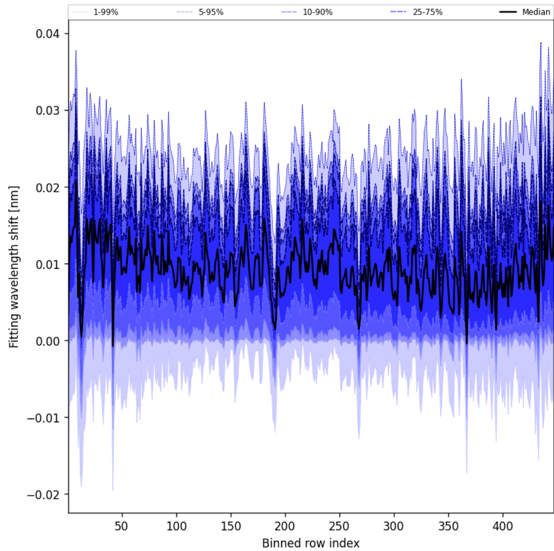
Figure 63: Along track statistics of “Fitting wavelength shift” for 2025-11-03 to 2025-11-04
