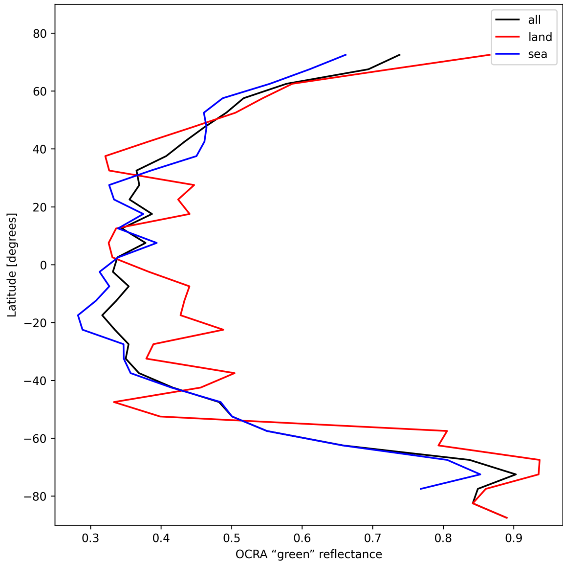
Figure 34: Zonal average of “OCRA “green” reflectance” for 2025-11-03 to 2025-11-04.
