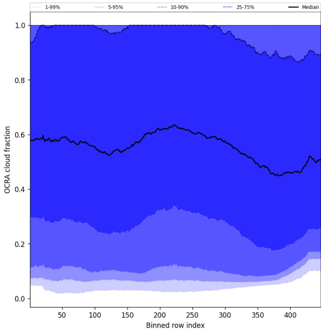
Figure 64: Along track statistics of “OCRA cloud fraction” for 2025-11-03 to 2025-11-04
