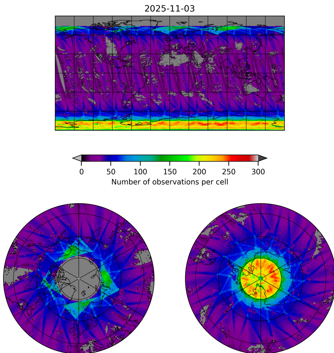
Figure 19: Map of the number of observations for 2025-11-03 to 2025-11-04
