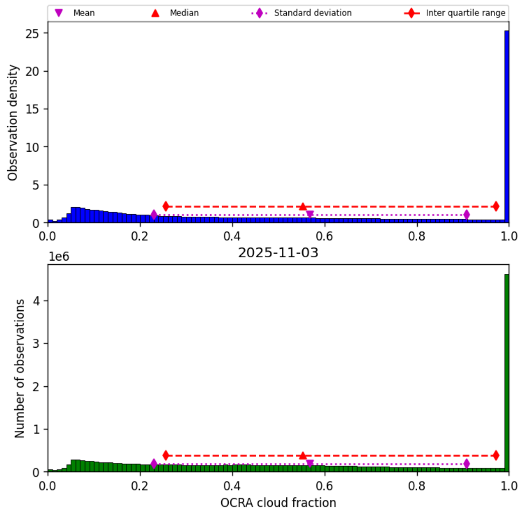
Figure 48: Histogram of “OCRA cloud fraction” for 2025-11-03 to 2025-11-04
