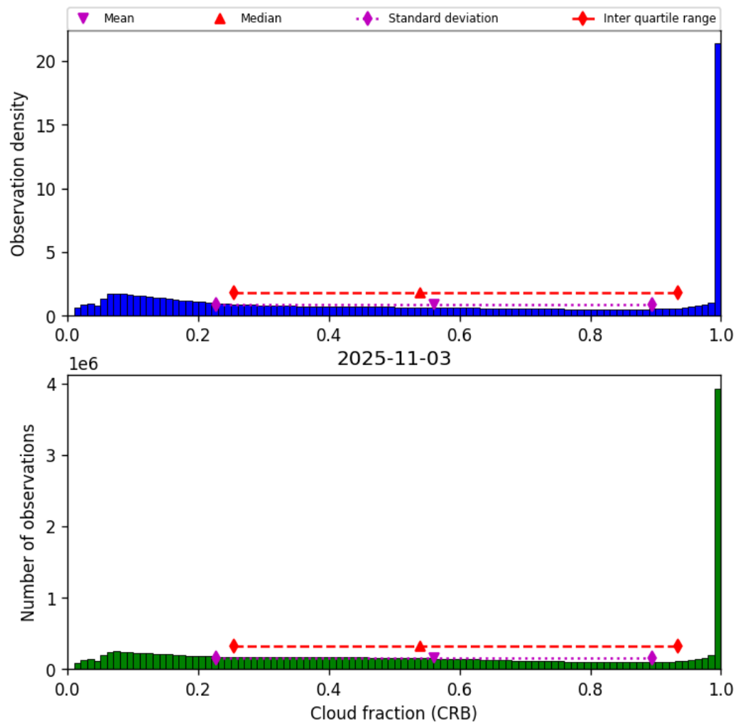
Figure 40: Histogram of "Cloud fraction (CRB)" for 2025-11-03 to 2025-11-04
