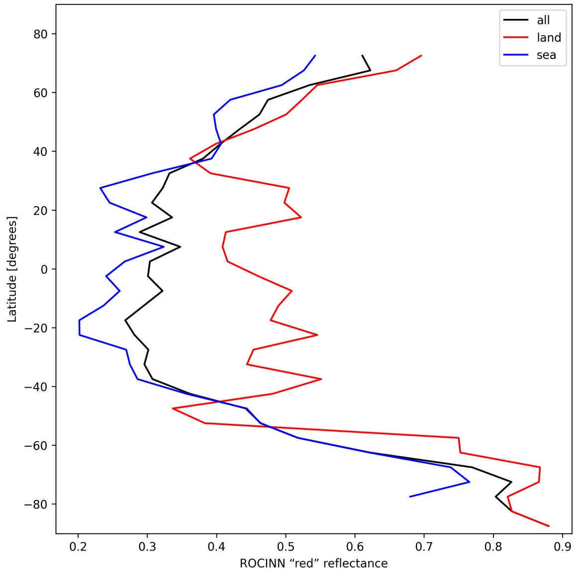
Figure 35: Zonal average of "ROCINN "red" reflectance" for 2025-11-03 to 2025-11-04.
