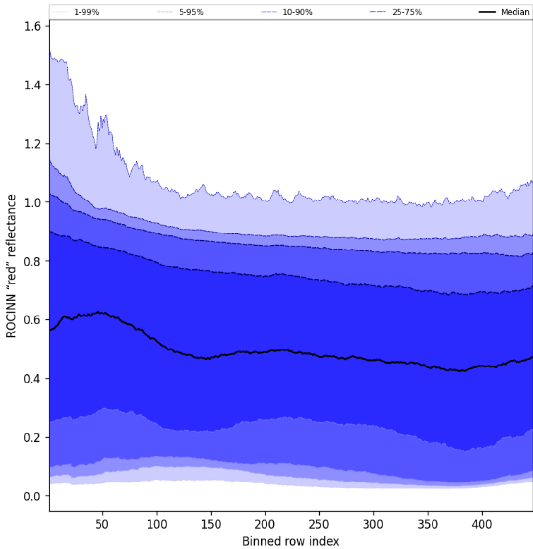
Figure 67: Along track statistics of "ROCINN "red" reflectance" for 2025-11-03 to 2025-11-04
