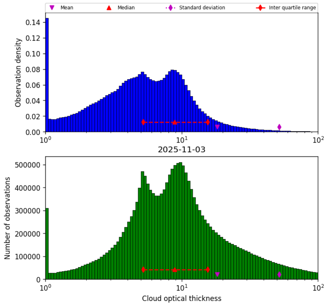
Figure 39: Histogram of “Cloud optical thickness” for 2025-11-03 to 2025-11-04
