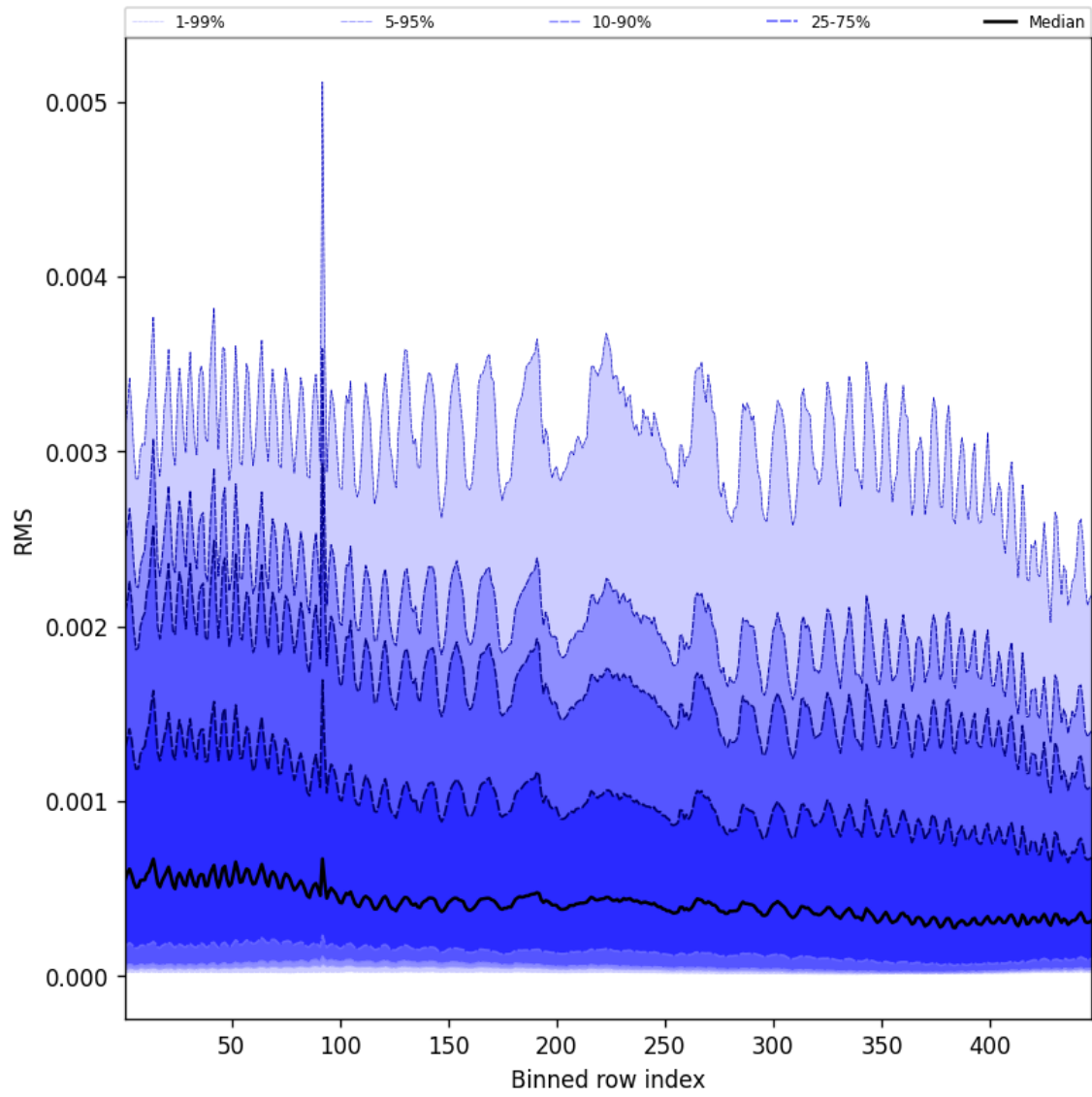
Figure 61: Along track statistics of “RMS” for 2025-11-03 to 2025-11-04
