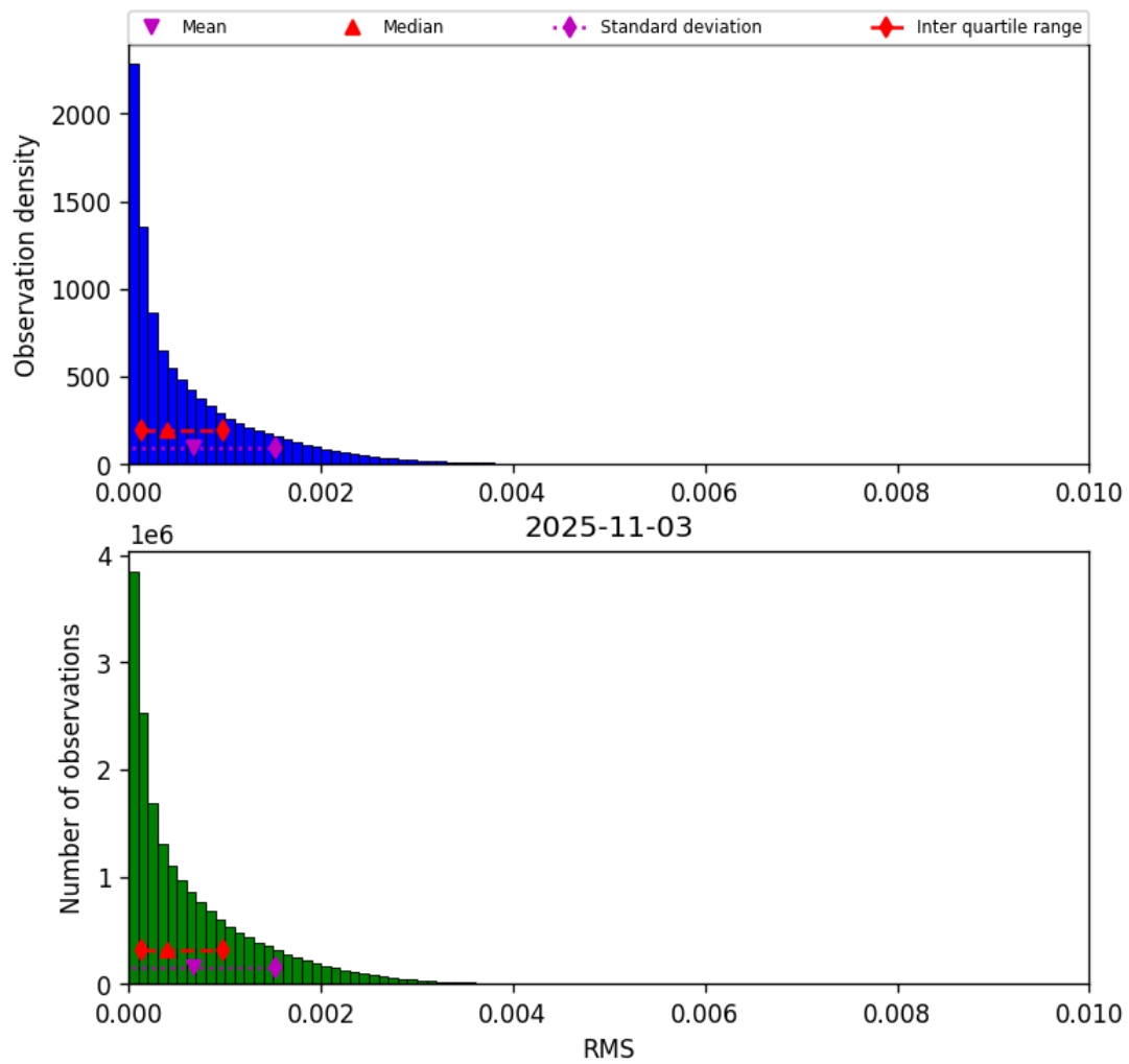
Figure 45: Histogram of “RMS” for 2025-11-03 to 2025-11-04
