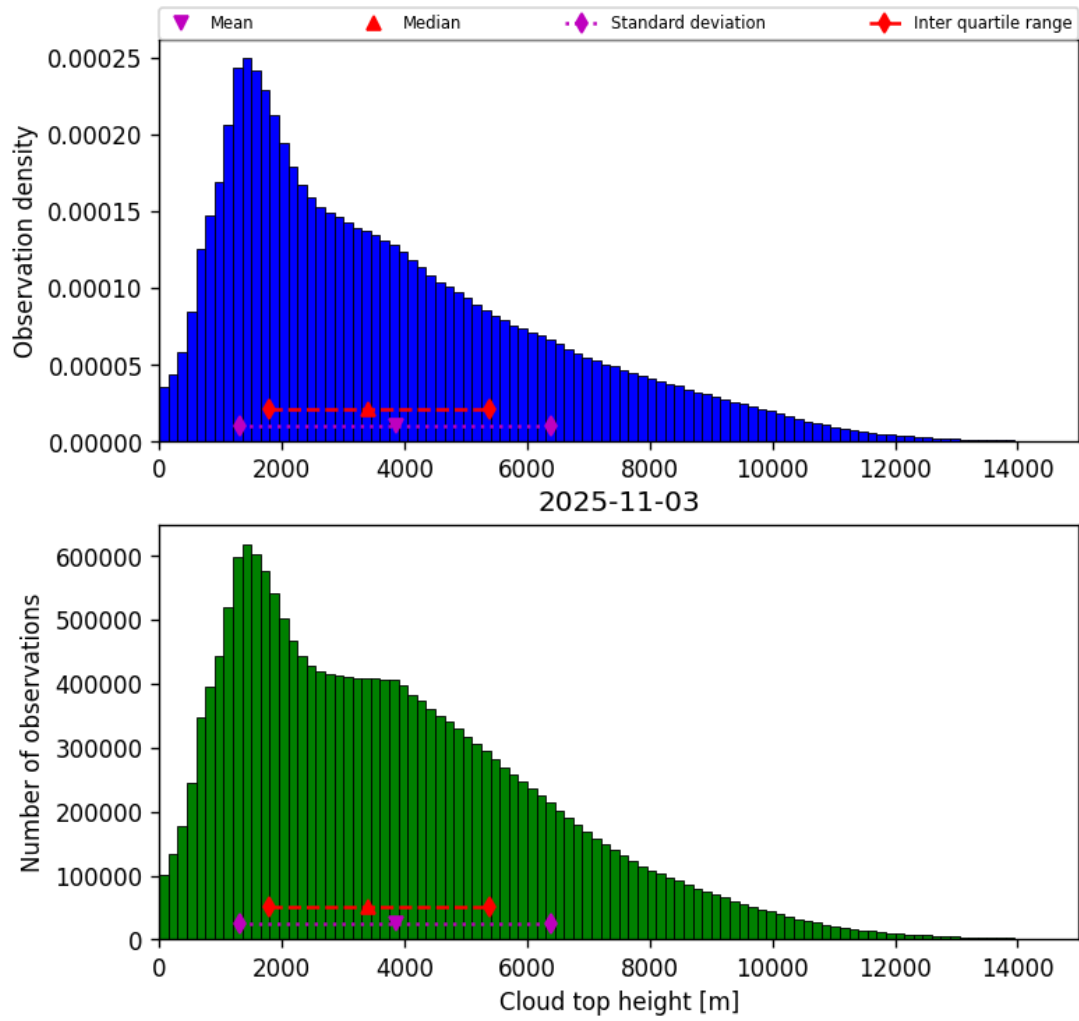
Figure 38: Histogram of “Cloud top height” for 2025-11-03 to 2025-11-04
