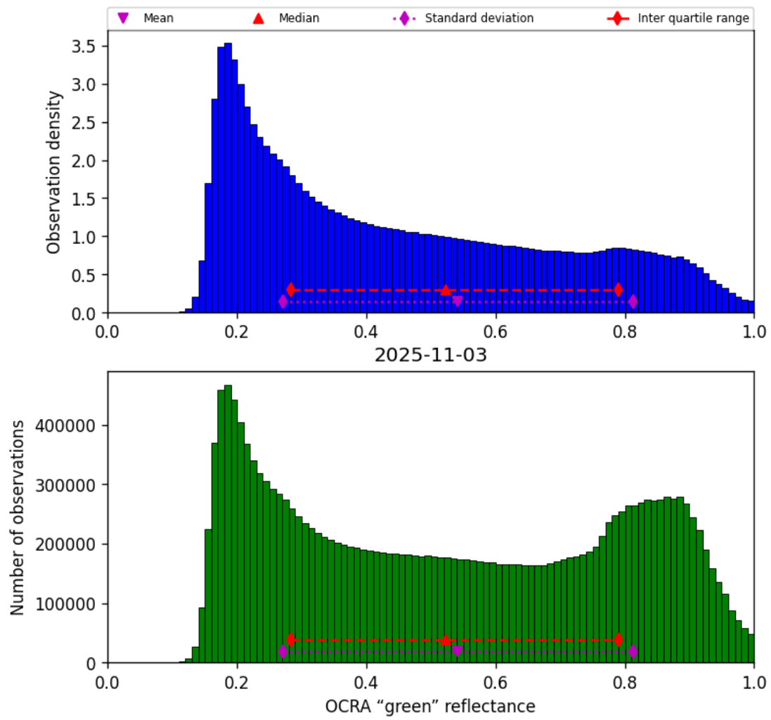
Figure 50: Histogram of “OCRA “green” reflectance” for 2025-11-03 to 2025-11-04
