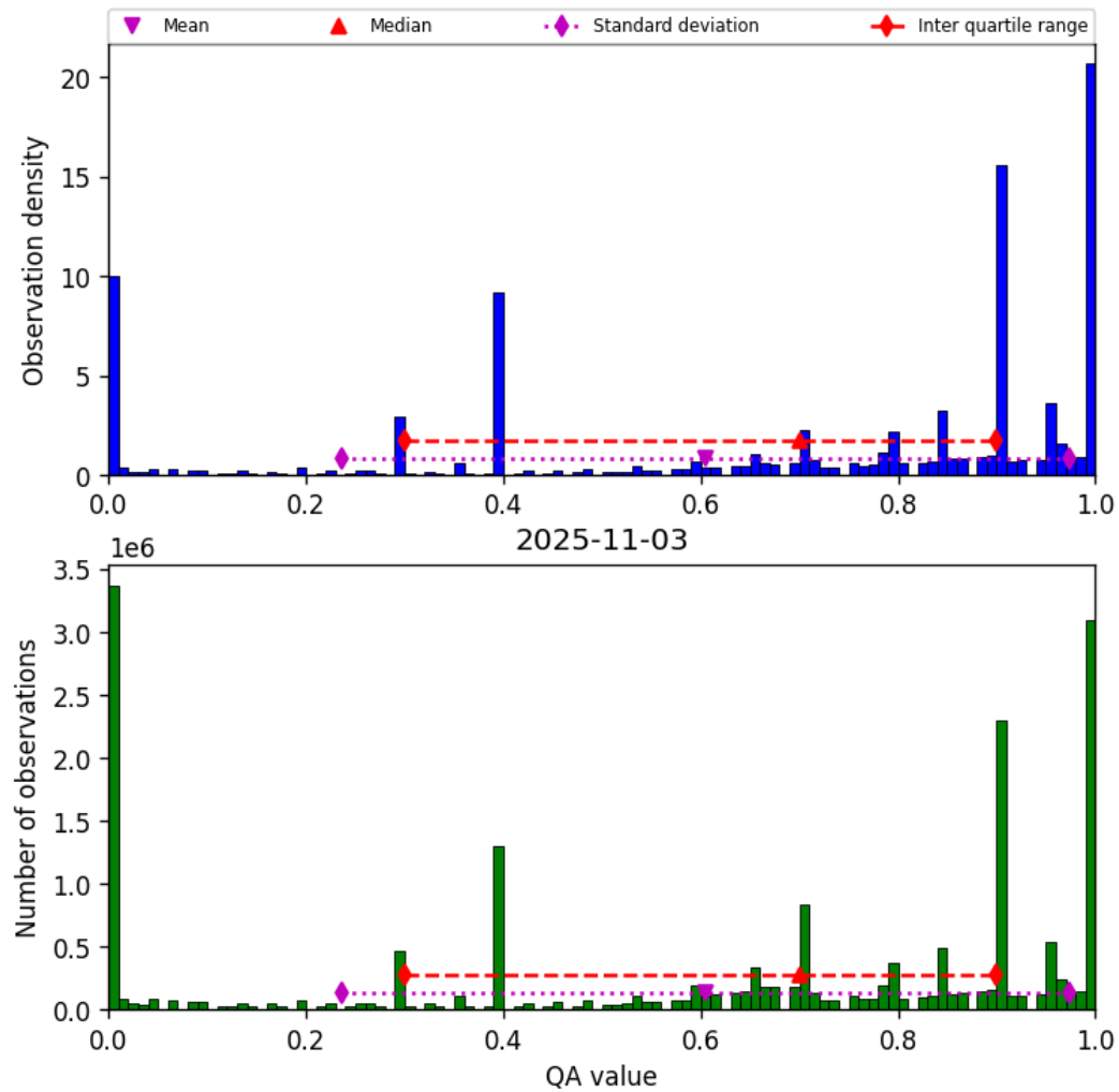
Figure 36: Histogram of “QA value” for 2025-11-03 to 2025-11-04
