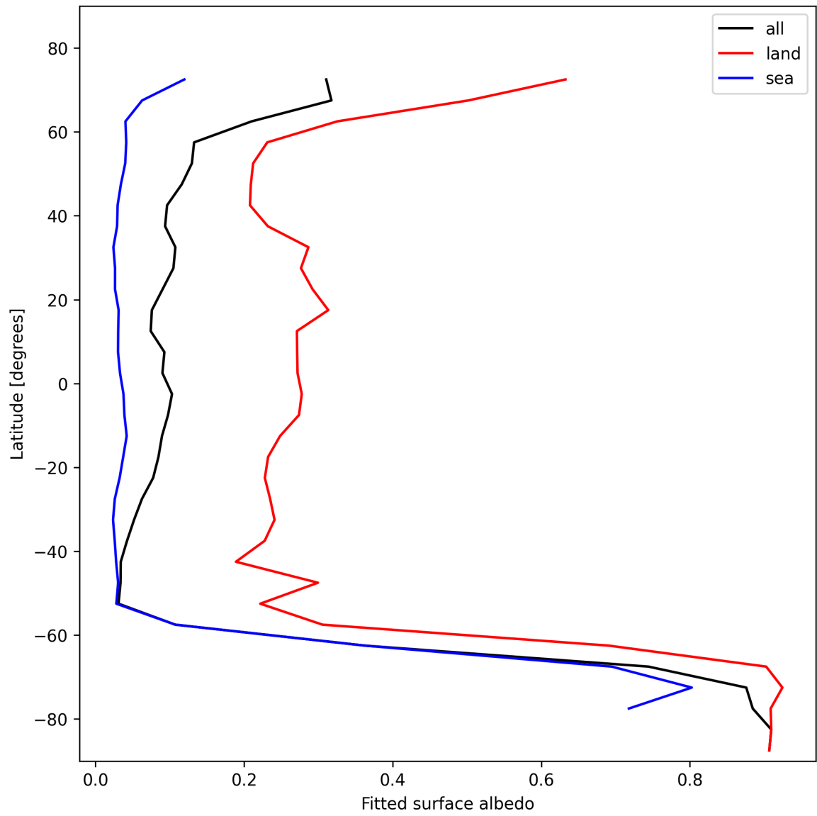
Figure 27: Zonal average of “Fitted surface albedo” for 2025-11-03 to 2025-11-04.
