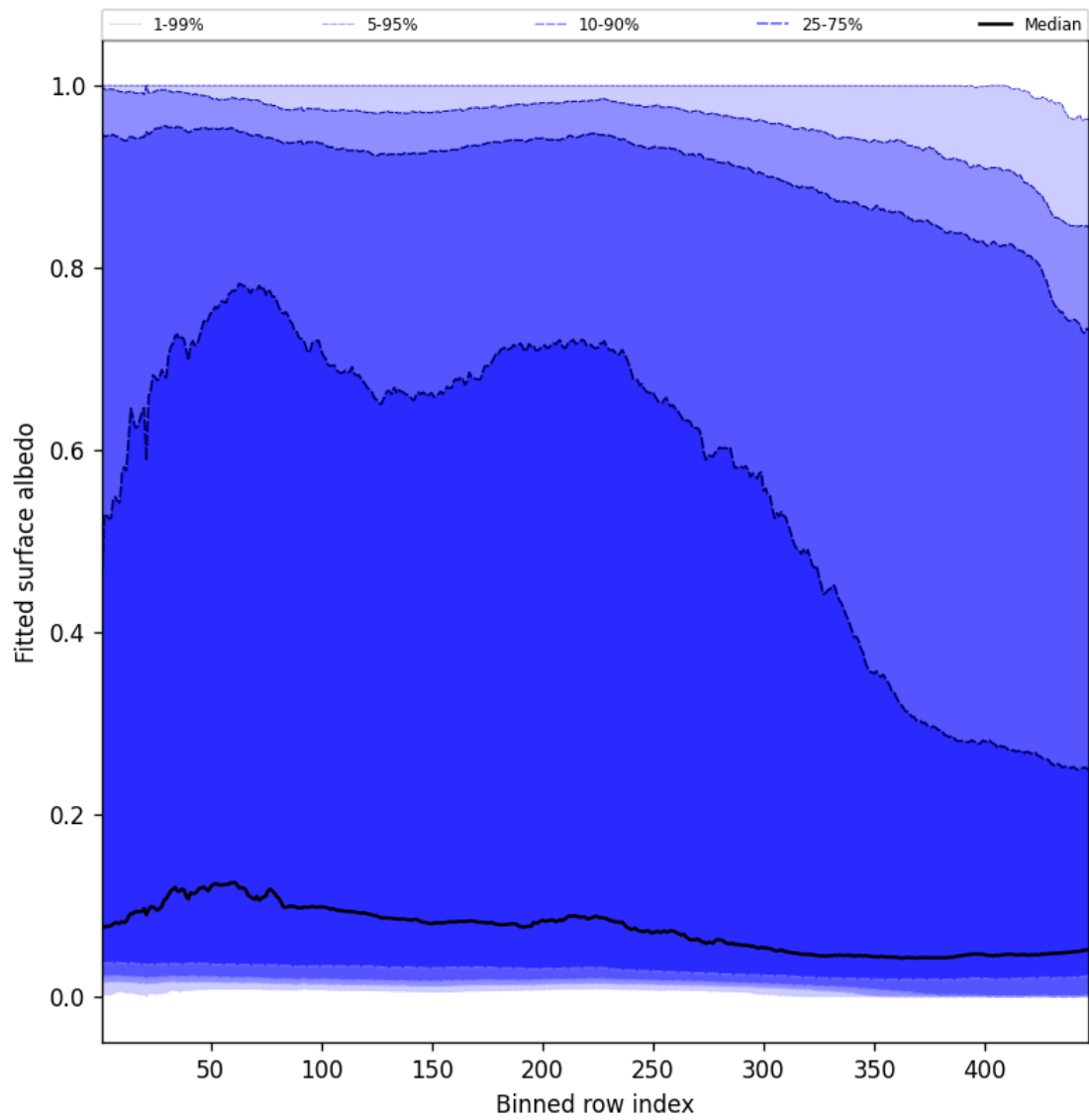
Figure 59: Along track statistics of “Fitted surface albedo” for 2025-11-03 to 2025-11-04
