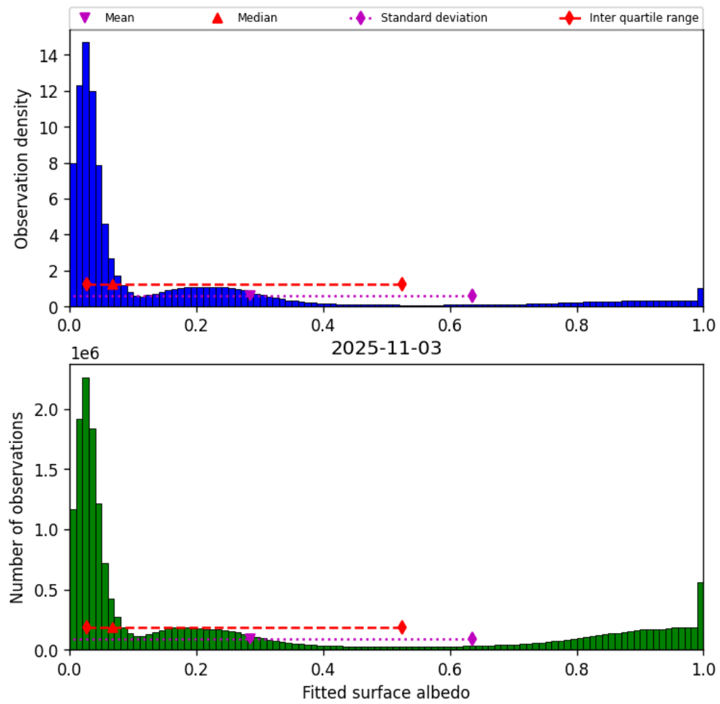
Figure 43: Histogram of “Fitted surface albedo” for 2025-11-03 to 2025-11-04
