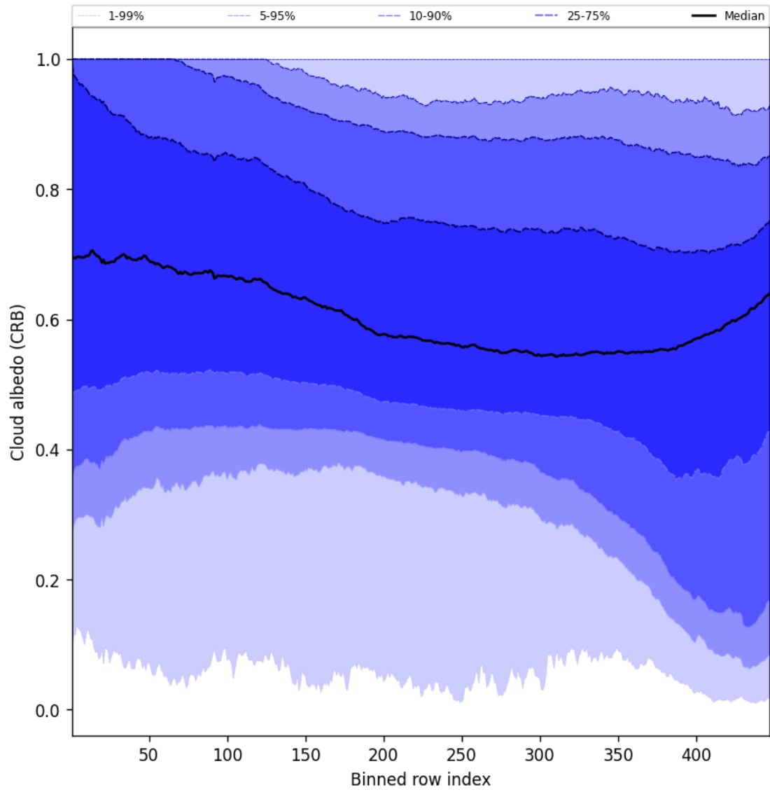
Figure 58: Along track statistics of “Cloud albedo (CRB)” for 2025-11-03 to 2025-11-04
