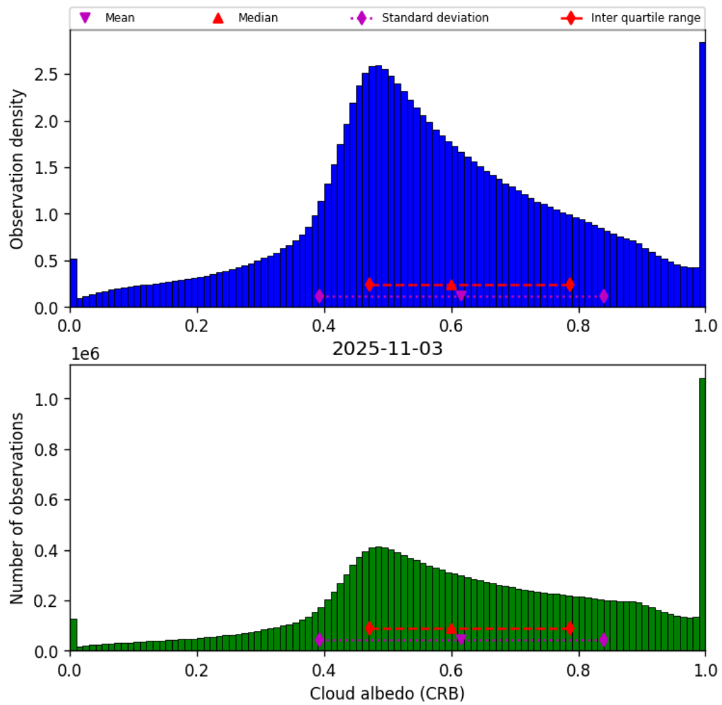
Figure 42: Histogram of “Cloud albedo (CRB)” for 2025-11-03 to 2025-11-04
