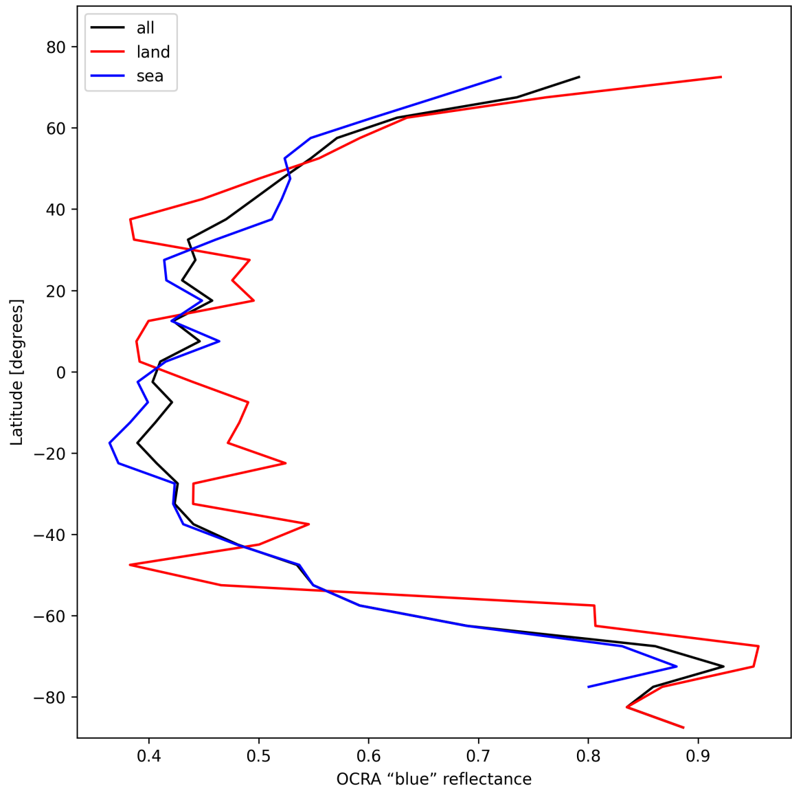
Figure 33: Zonal average of "OCRA "blue" reflectance" for 2025-11-03 to 2025-11-04.
