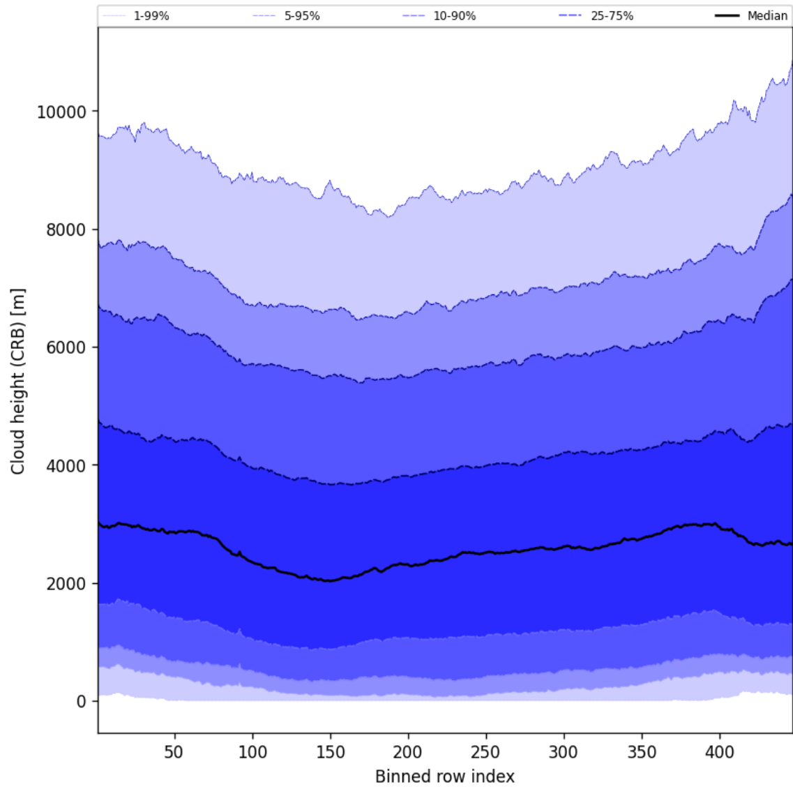
Figure 57: Along track statistics of “Cloud height (CRB)” for 2025-11-03 to 2025-11-04
