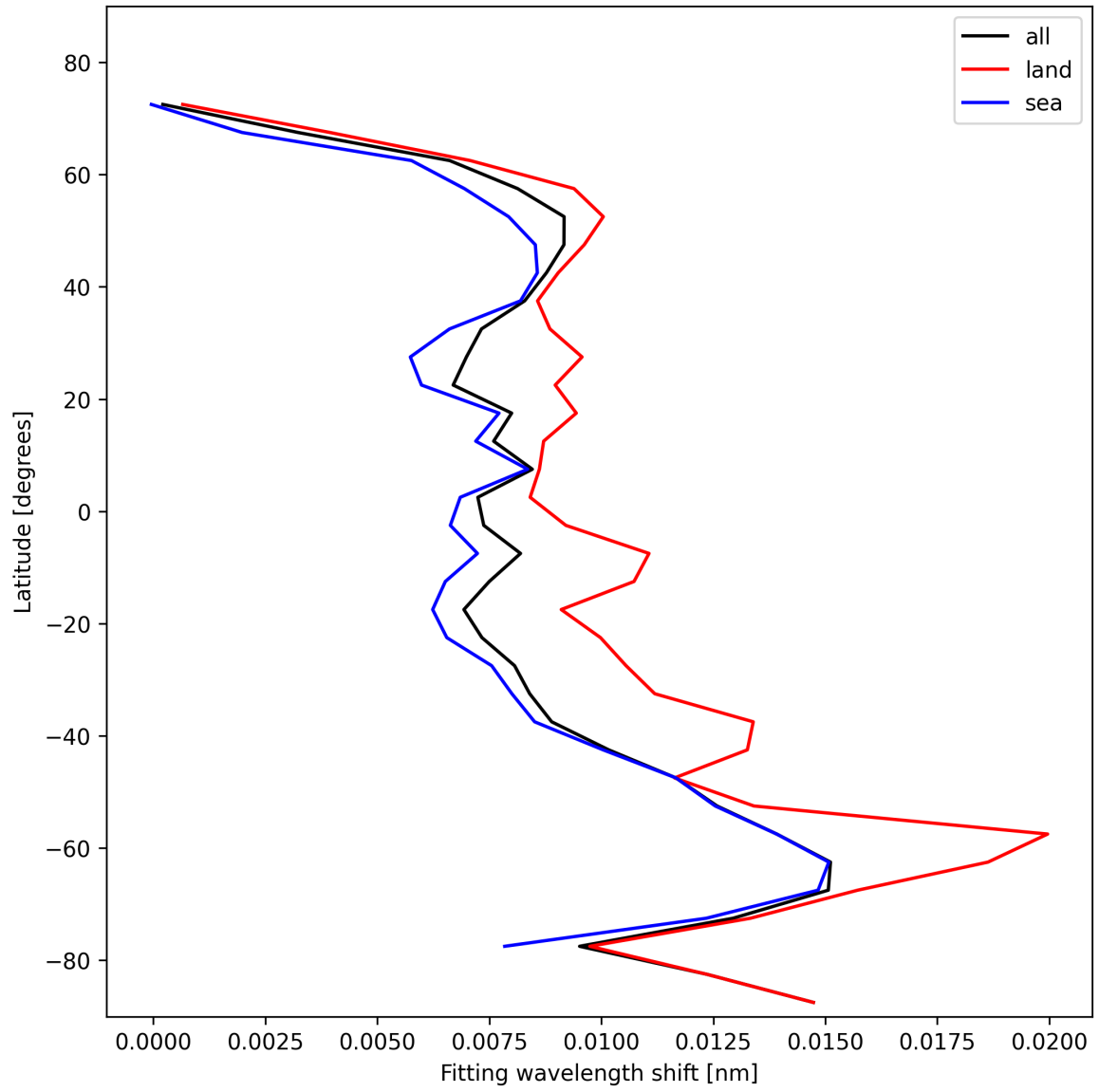
Figure 31: Zonal average of “Fitting wavelength shift” for 2025-11-03 to 2025-11-04.
