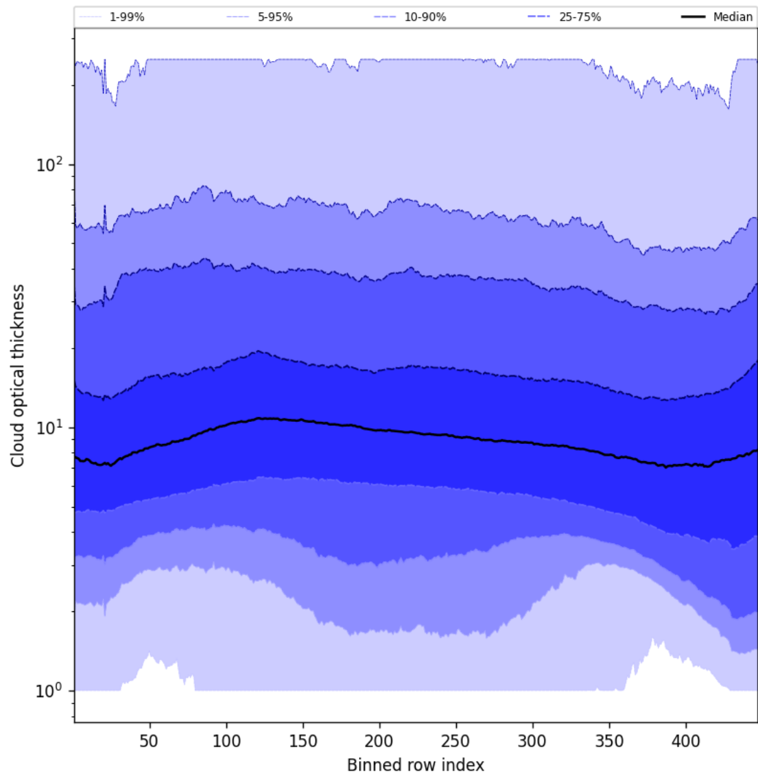
Figure 55: Along track statistics of “Cloud optical thickness” for 2025-11-03 to 2025-11-04
