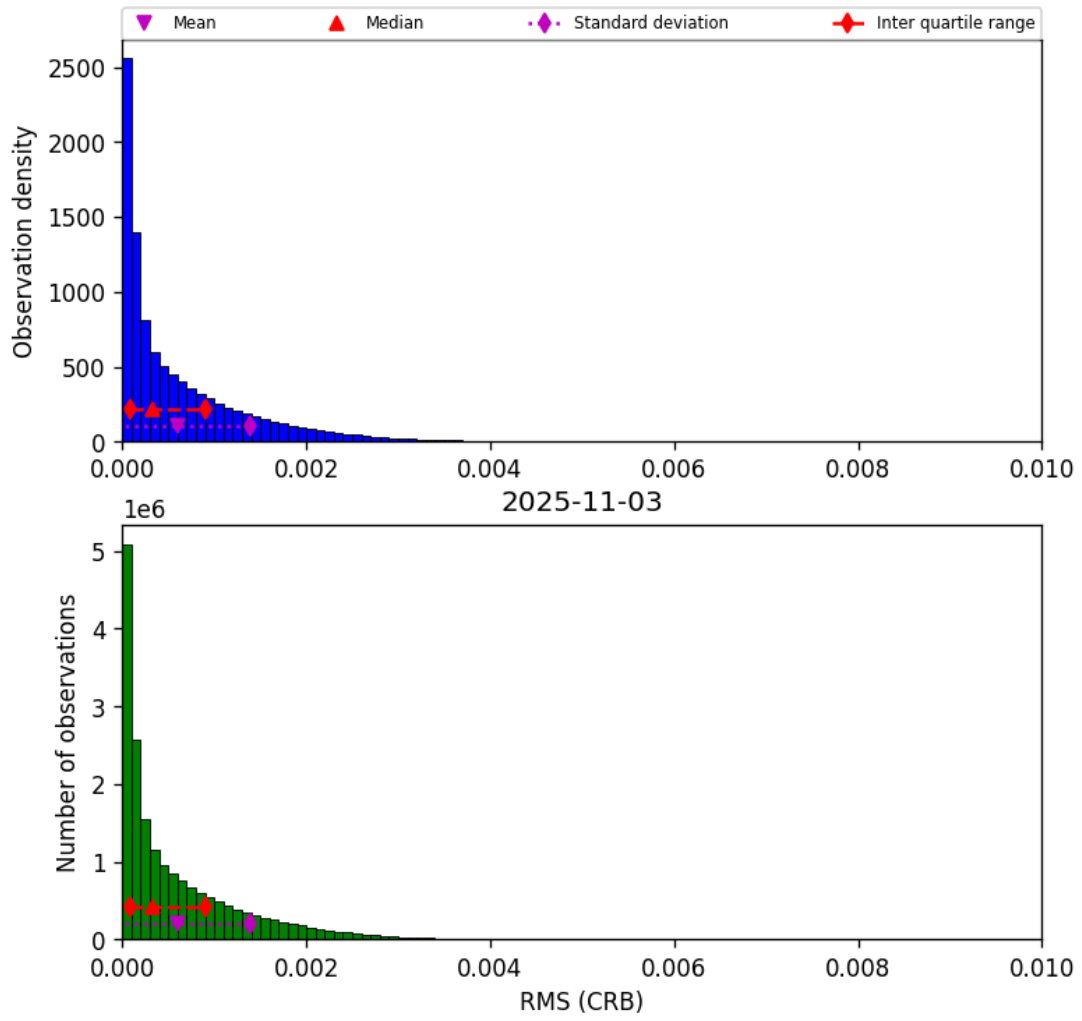
Figure 46: Histogram of “RMS (CRB)” for 2025-11-03 to 2025-11-04
