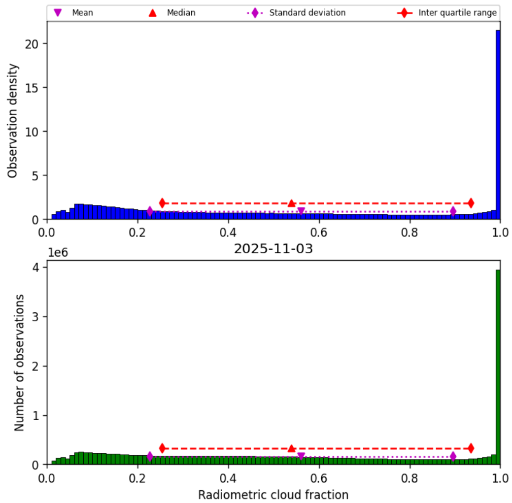
Figure 37: Histogram of “Radiometric cloud fraction” for 2025-11-03 to 2025-11-04
