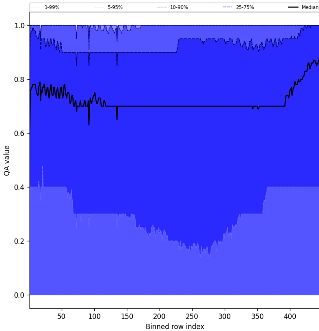
Figure 52: Along track statistics of "QA value" for 2025-11-03 to 2025-11-04
