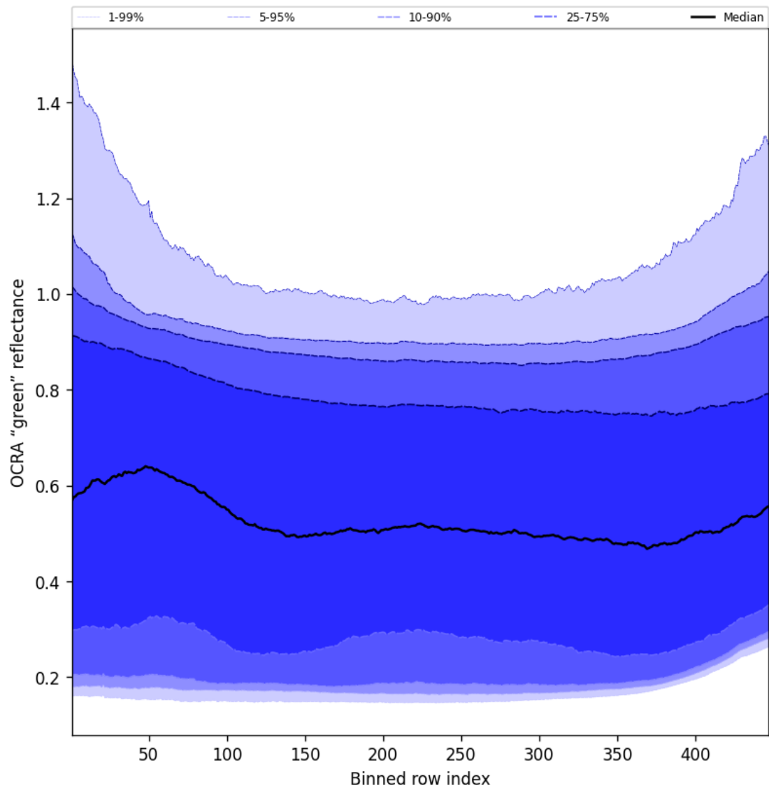
Figure 66: Along track statistics of “OCRA “green” reflectance” for 2025-11-03 to 2025-11-04
