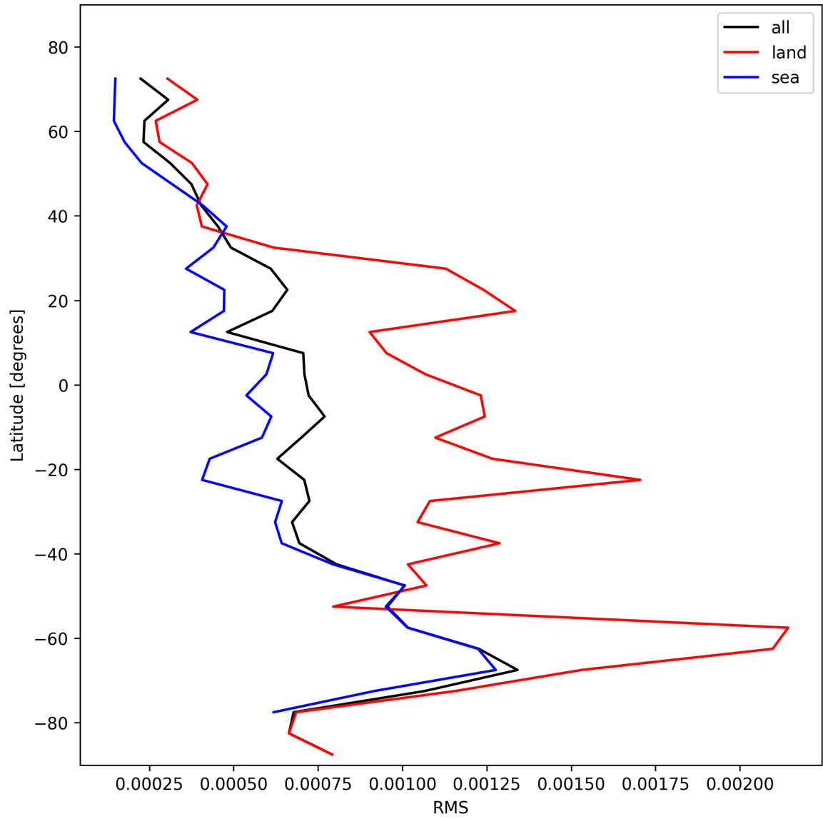
Figure 29: Zonal average of “RMS” for 2025-11-03 to 2025-11-04.
