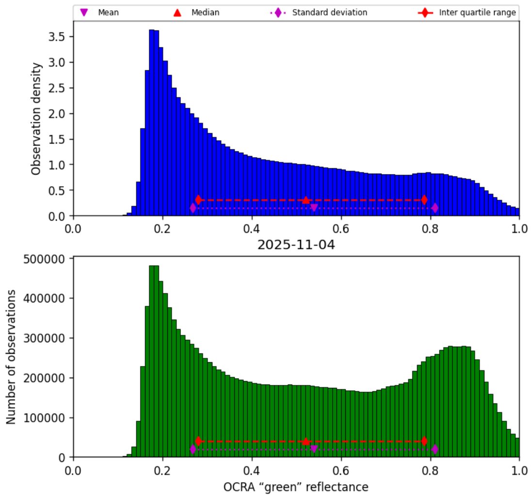
Figure 50: Histogram of “OCRA “green” reflectance” for 2025-11-04 to 2025-11-05
