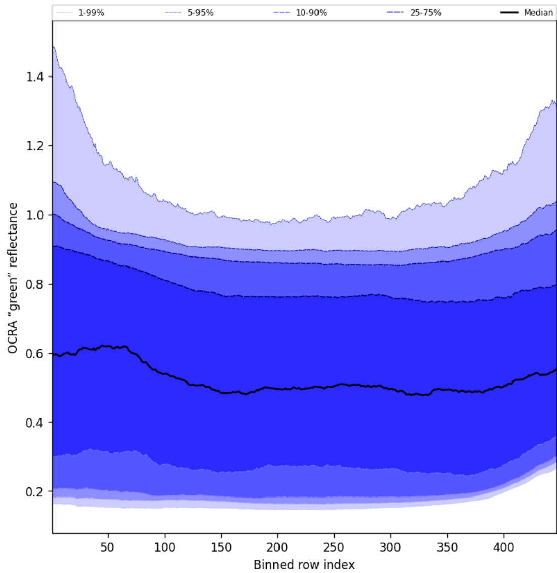
Figure 66: Along track statistics of “OCRA “green” reflectance” for 2025-11-04 to 2025-11-05
