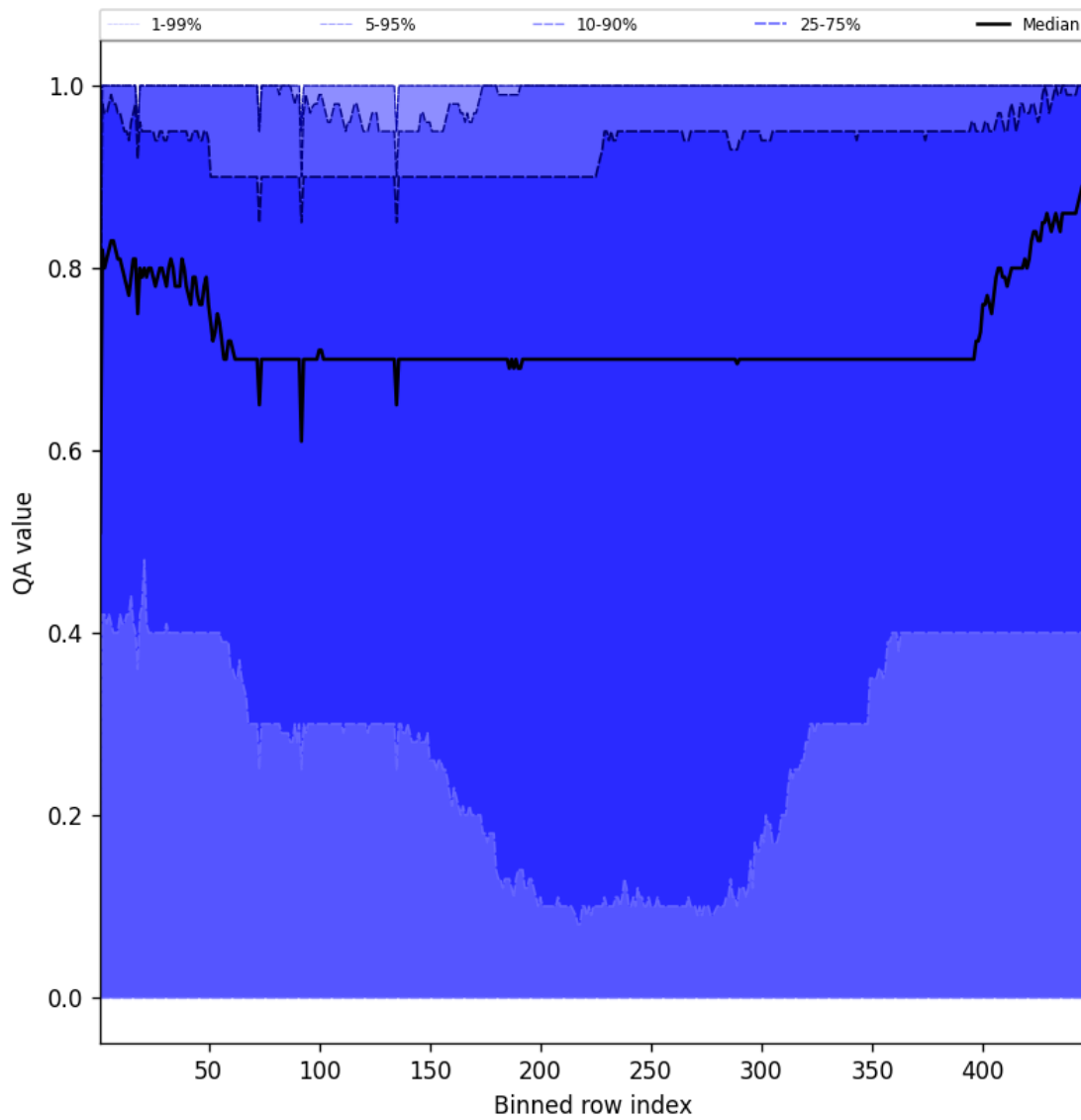
Figure 52: Along track statistics of “QA value” for 2025-11-04 to 2025-11-05
