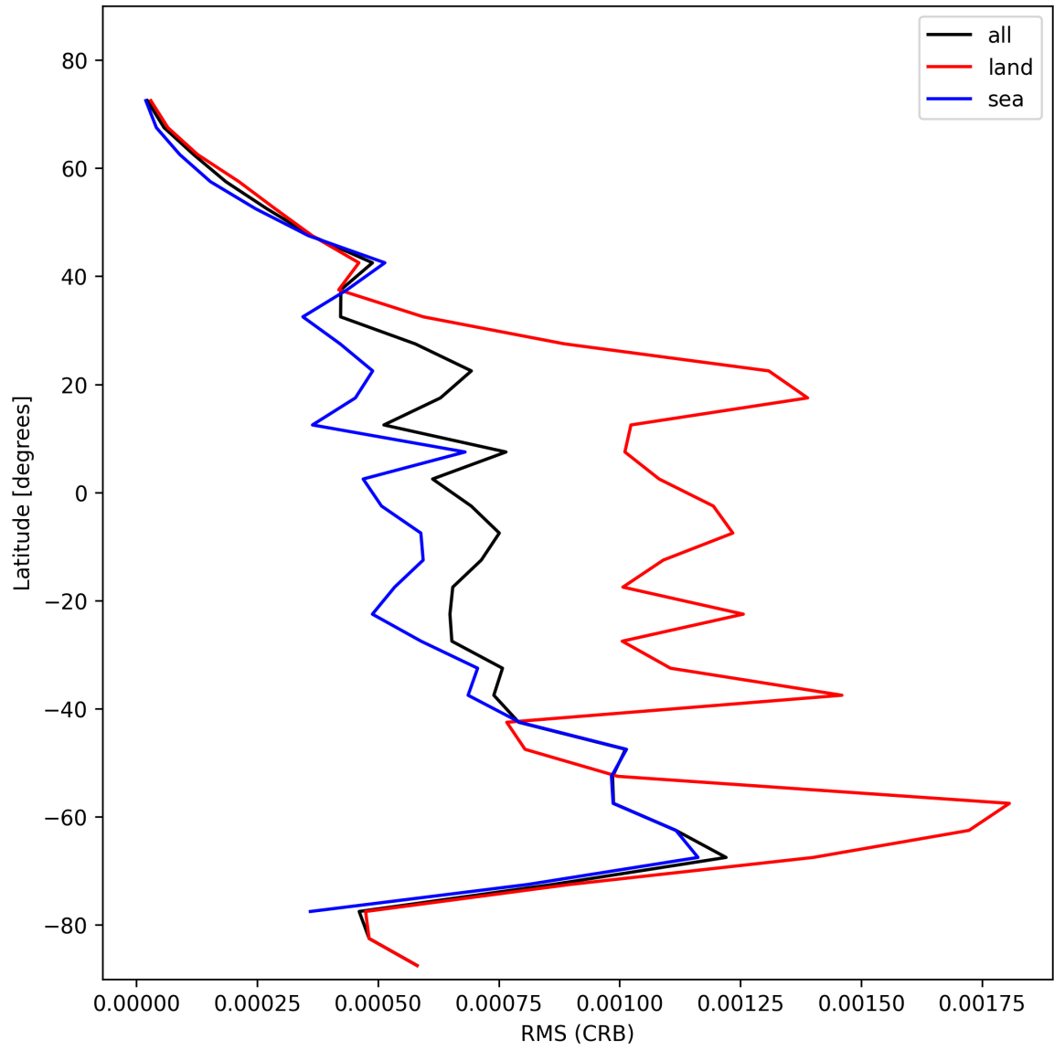
Figure 30: Zonal average of "RMS (CRB)" for 2025-11-04 to 2025-11-05.
