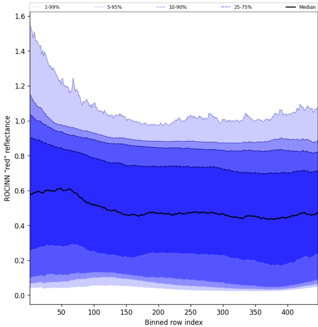
Figure 67: Along track statistics of “ROCINN “red” reflectance” for 2025-11-04 to 2025-11-05
