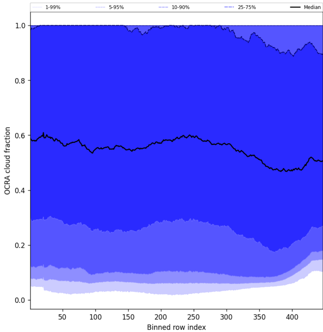
Figure 64: Along track statistics of “OCRA cloud fraction” for 2025-11-04 to 2025-11-05
