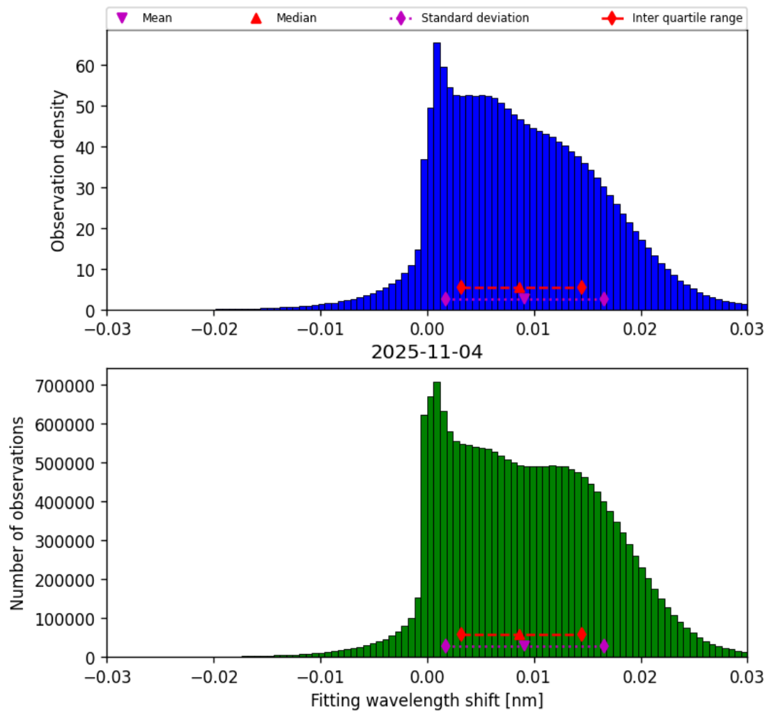
Figure 47: Histogram of “Fitting wavelength shift” for 2025-11-04 to 2025-11-05
