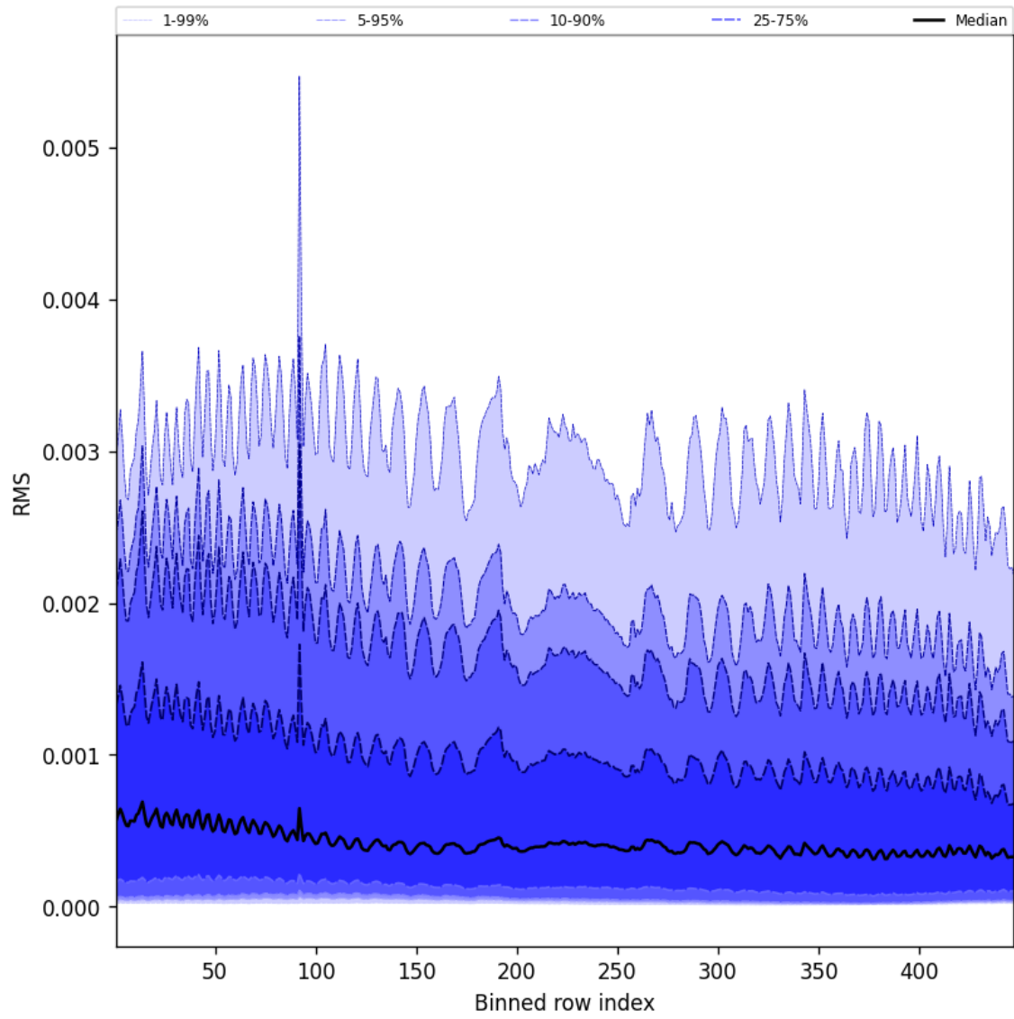
Figure 61: Along track statistics of “RMS” for 2025-11-04 to 2025-11-05
