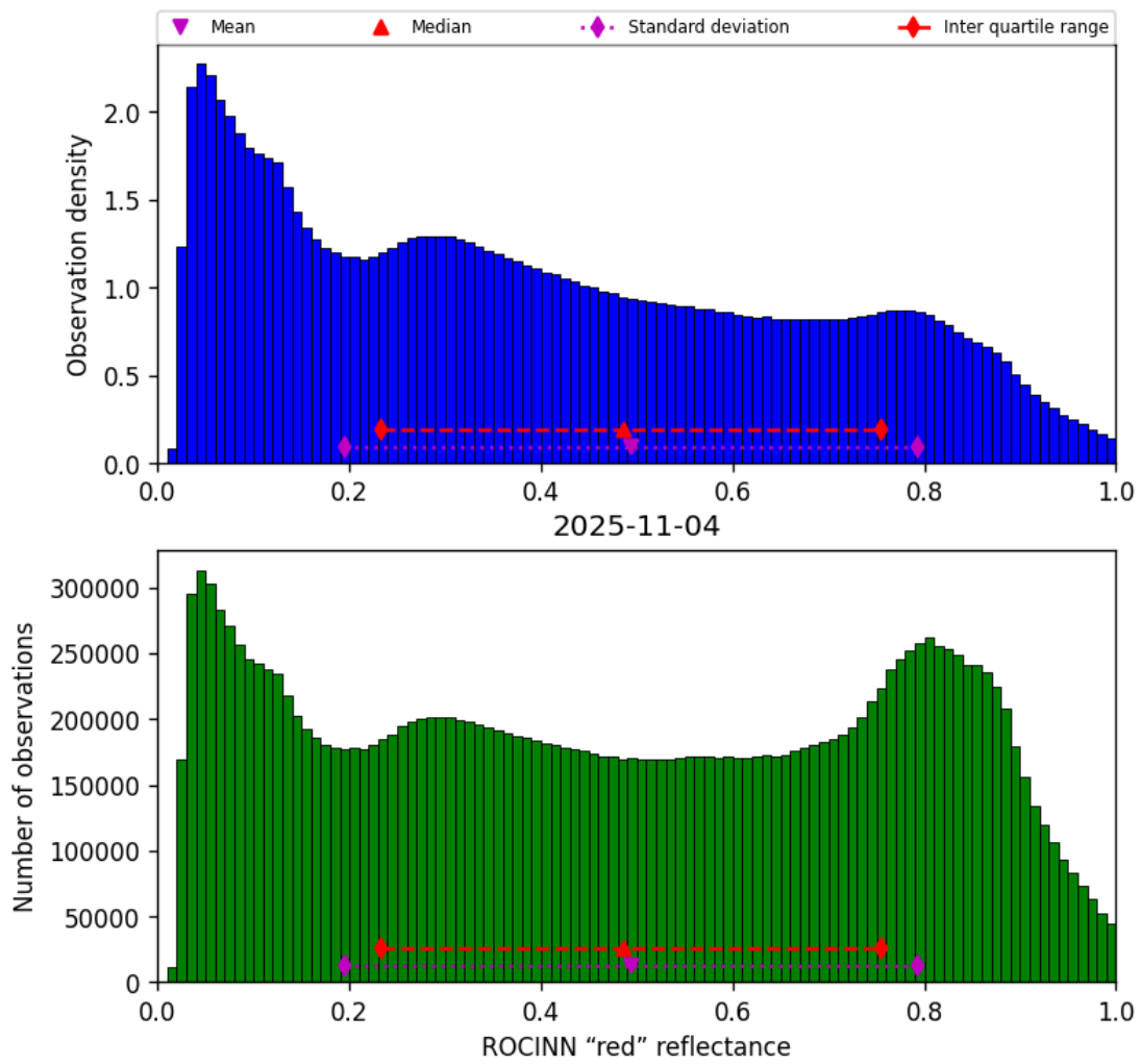
Figure 51: Histogram of “ROCINN “red” reflectance” for 2025-11-04 to 2025-11-05
