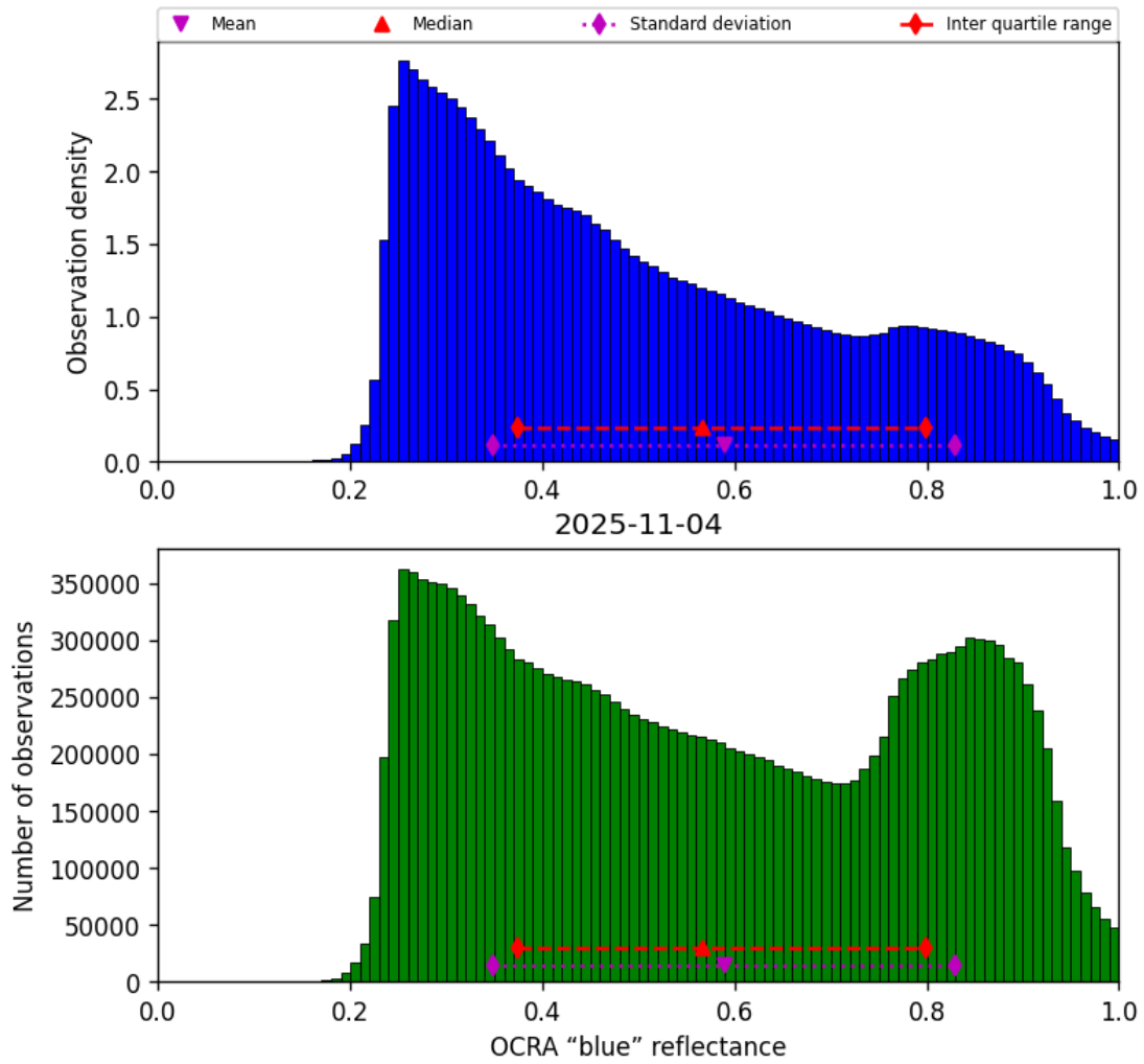
Figure 49: Histogram of “OCRA “blue” reflectance” for 2025-11-04 to 2025-11-05
