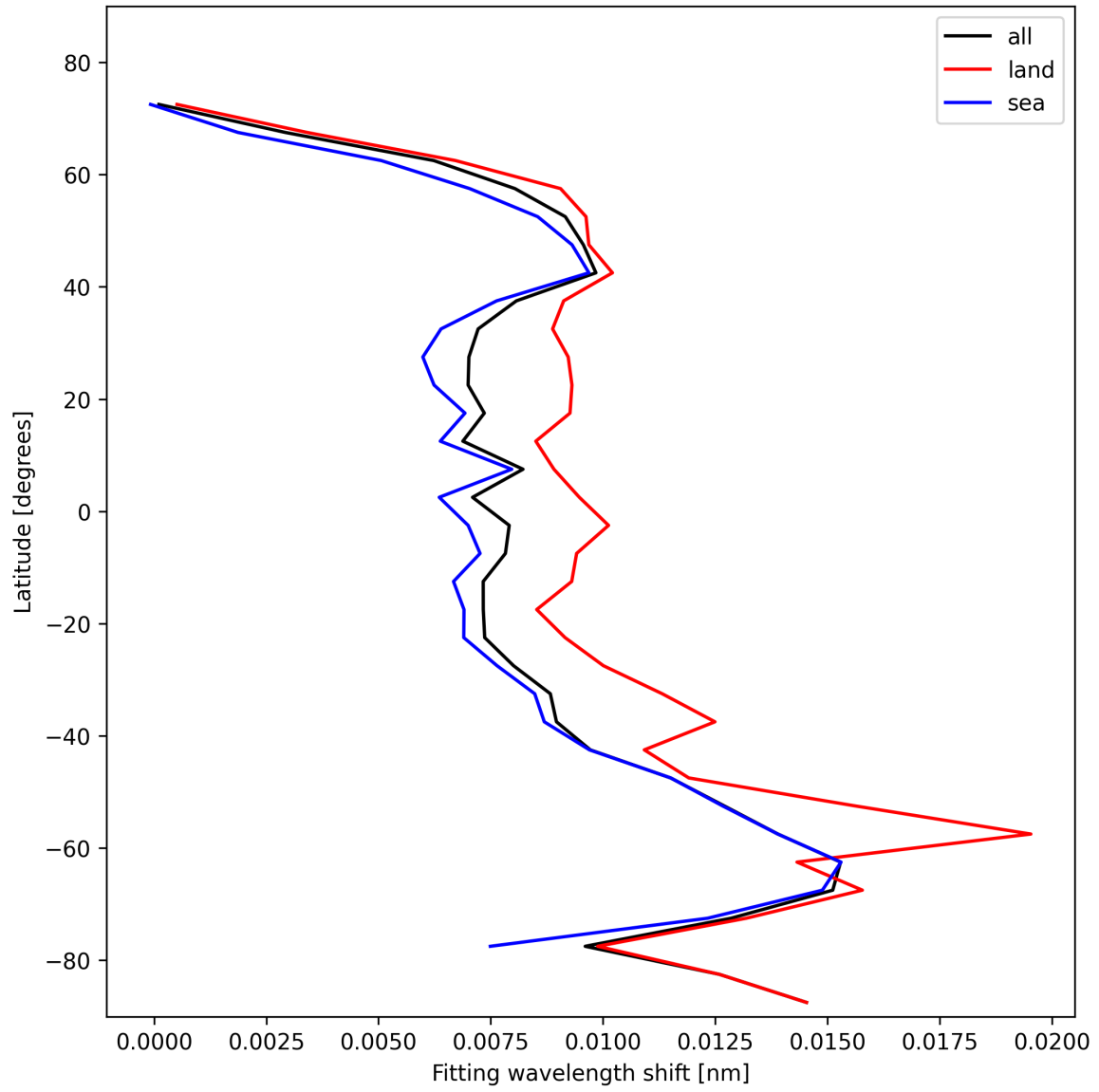
Figure 31: Zonal average of “Fitting wavelength shift” for 2025-11-04 to 2025-11-05.
