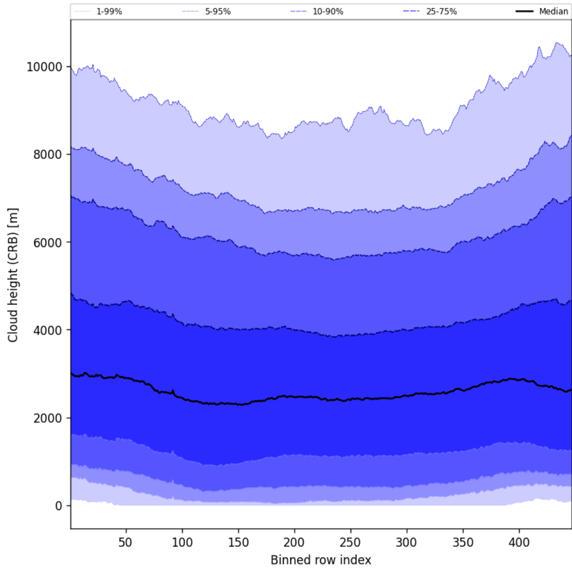
Figure 57: Along track statistics of “Cloud height (CRB)” for 2025-11-04 to 2025-11-05
