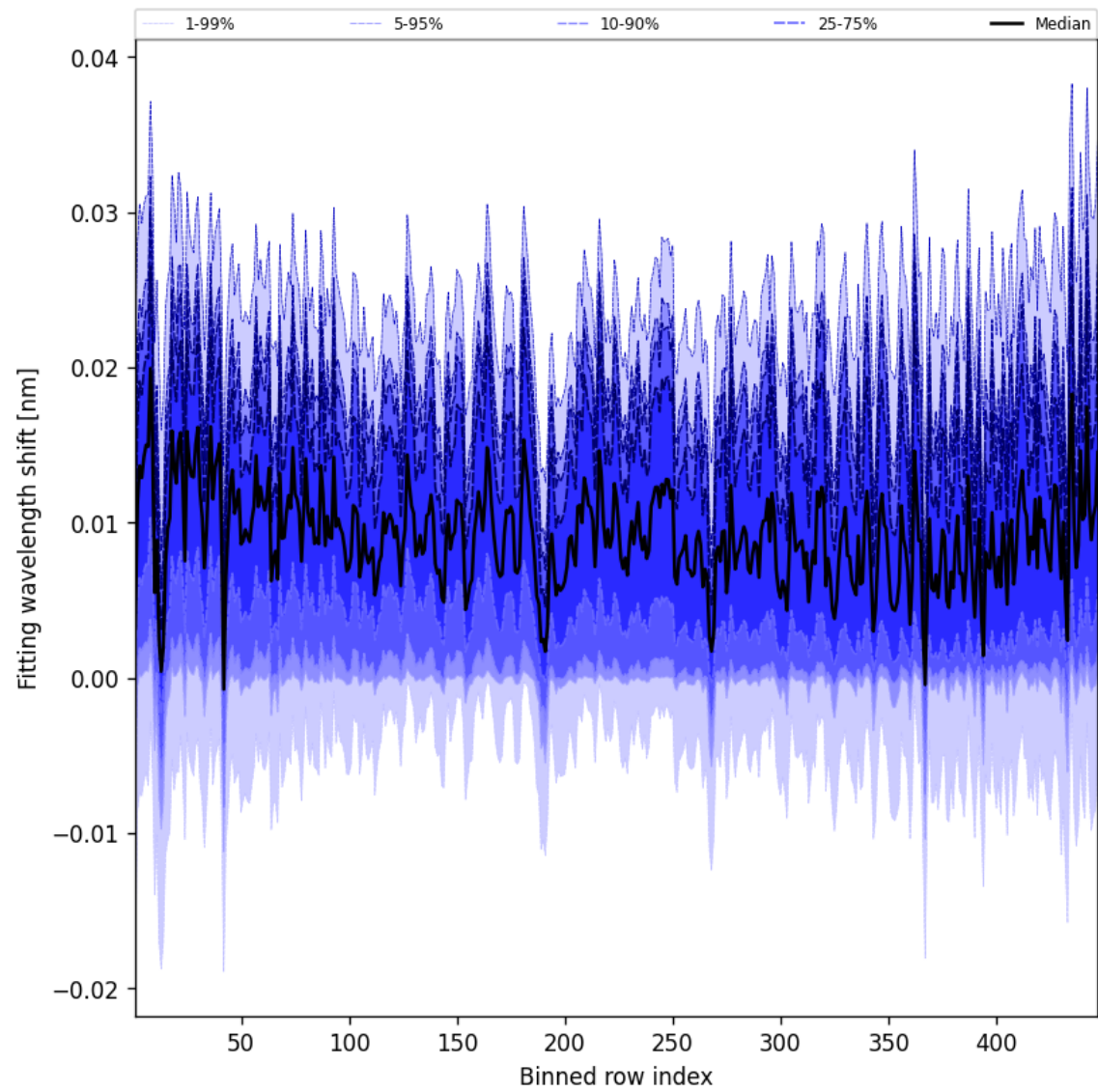
Figure 63: Along track statistics of “Fitting wavelength shift” for 2025-11-04 to 2025-11-05
