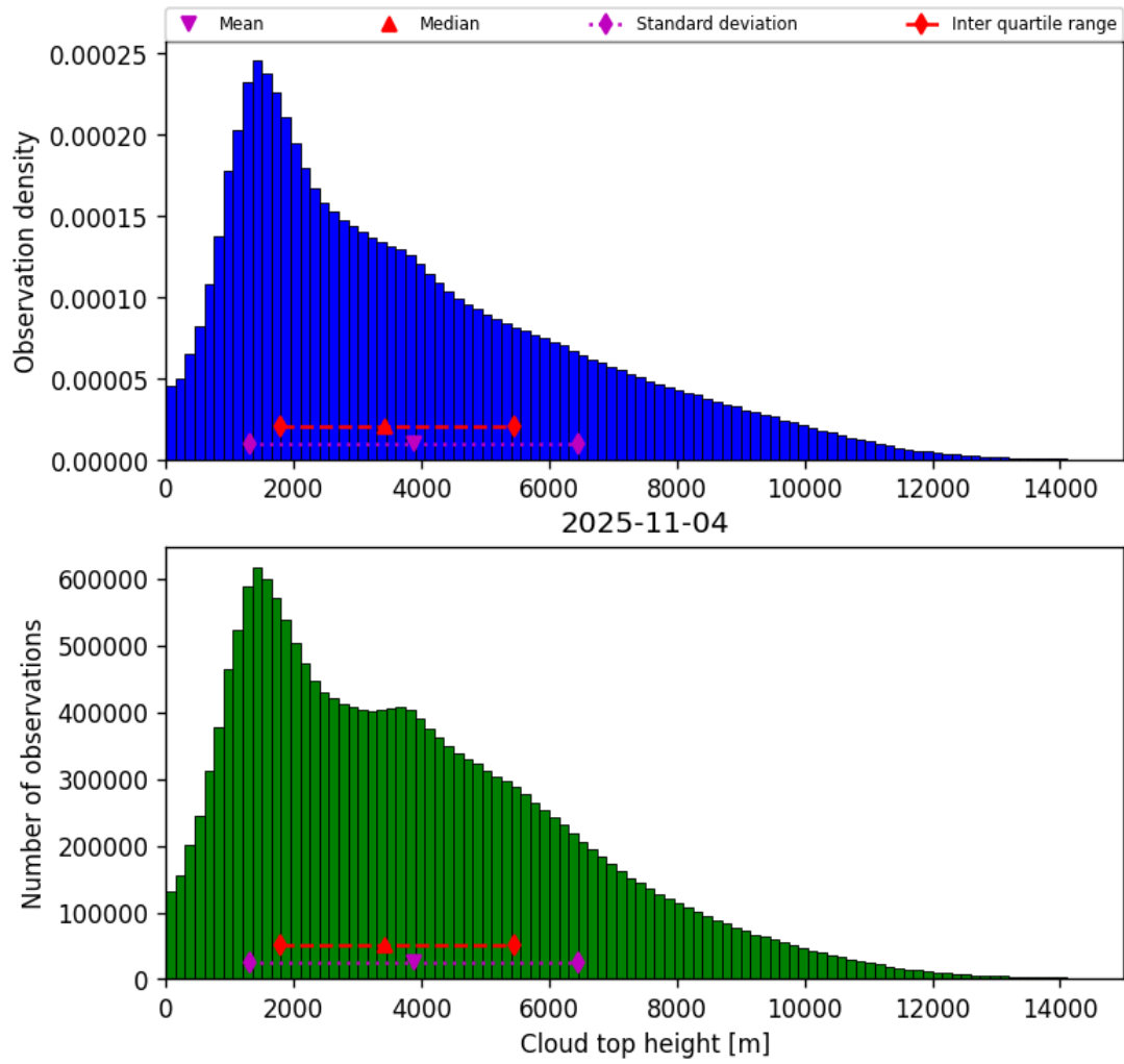
Figure 38: Histogram of “Cloud top height” for 2025-11-04 to 2025-11-05
