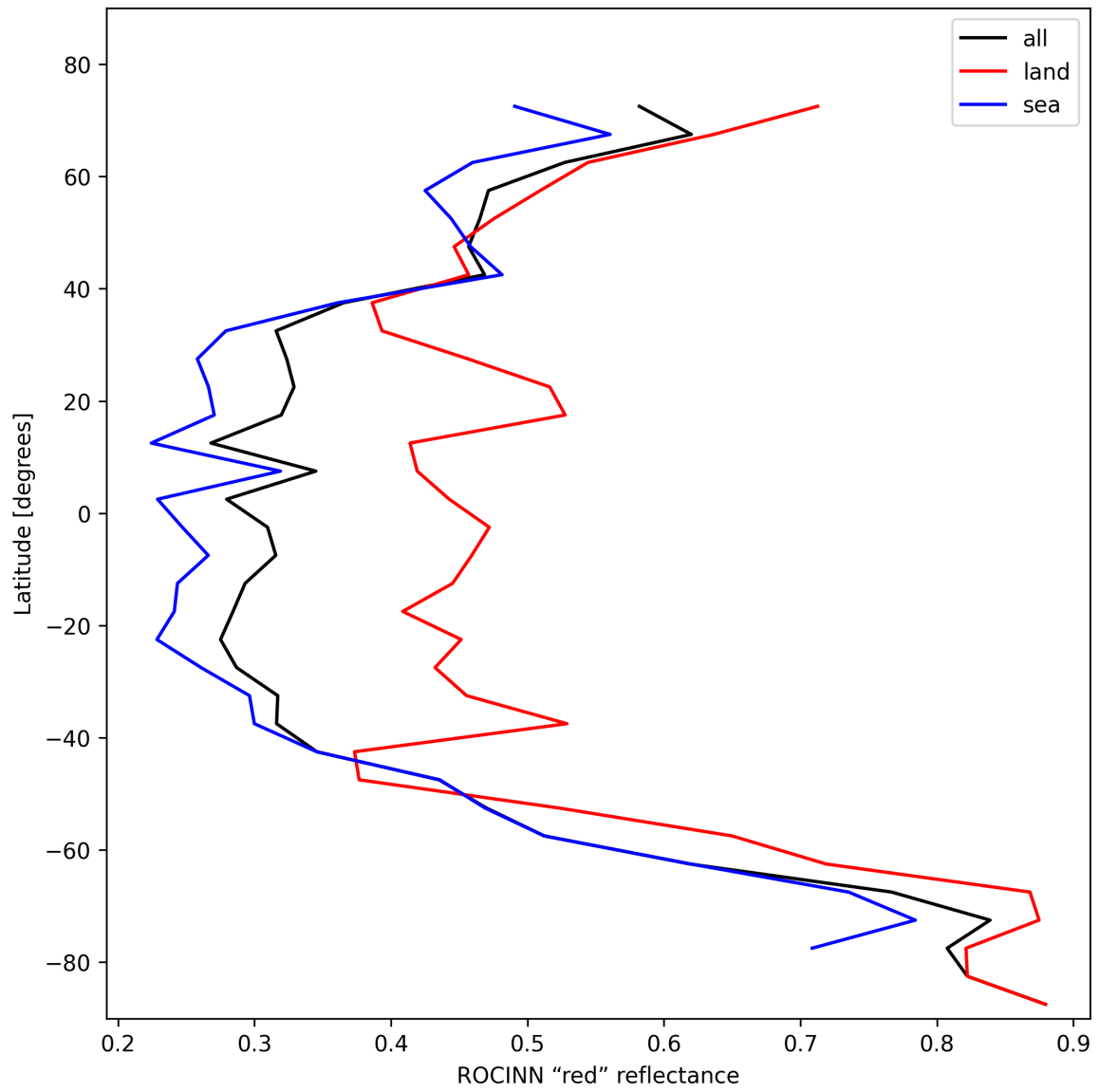
Figure 35: Zonal average of “ROCINN “red” reflectance” for 2025-11-04 to 2025-11-05.
