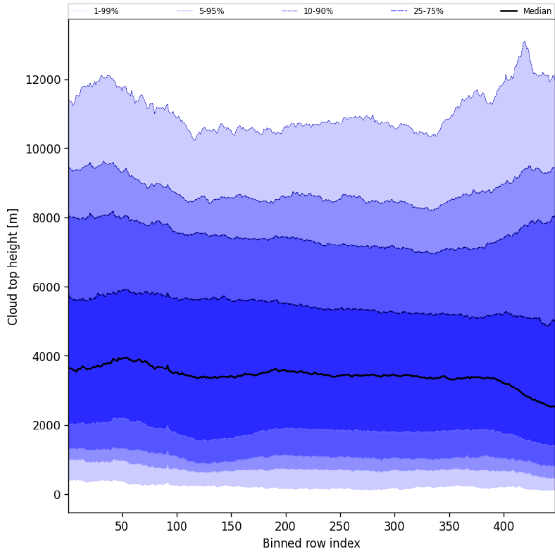
Figure 54: Along track statistics of “Cloud top height” for 2025-11-04 to 2025-11-05
