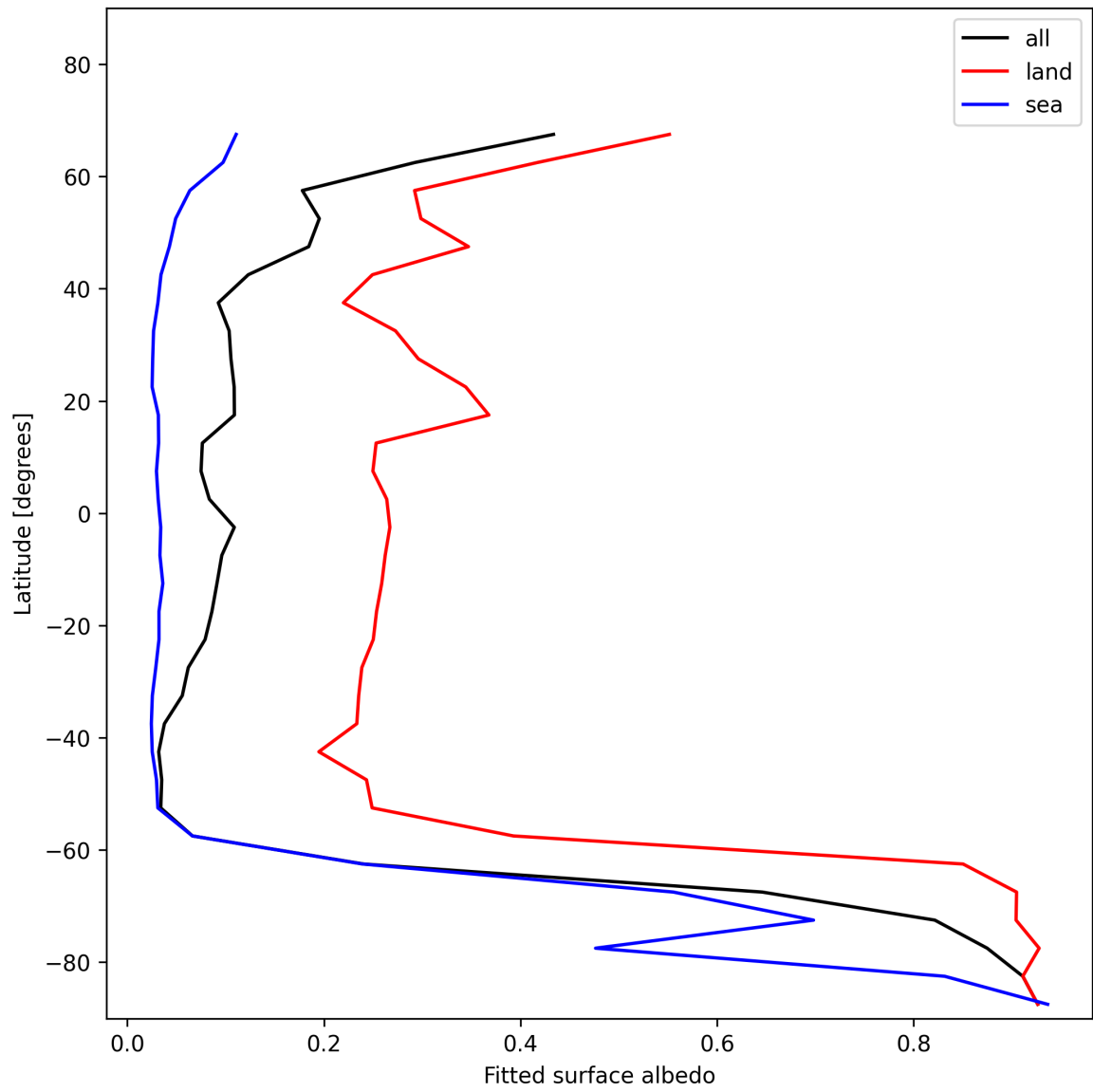
Figure 27: Zonal average of “Fitted surface albedo” for 2025-12-01 to 2025-12-01.
