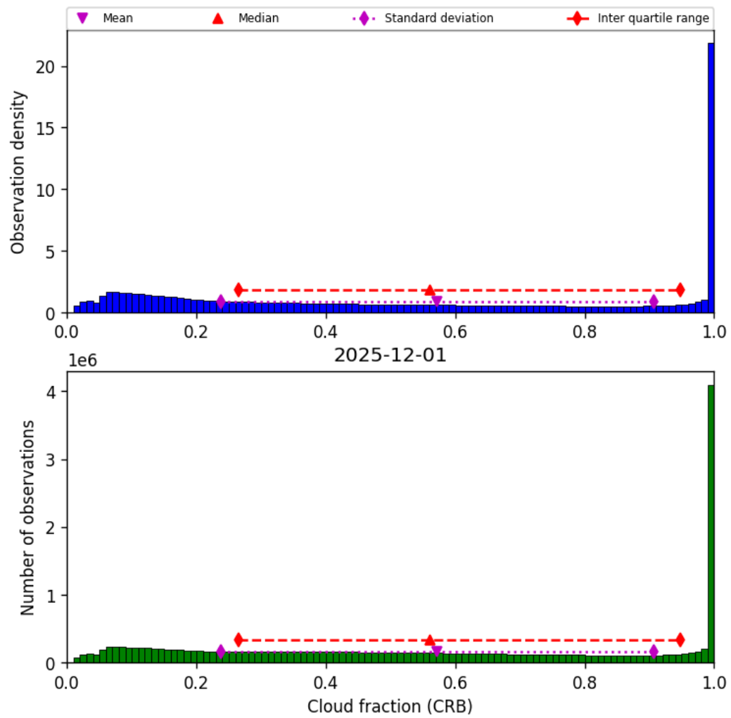
Figure 40: Histogram of “Cloud fraction (CRB)” for 2025-12-01 to 2025-12-01
