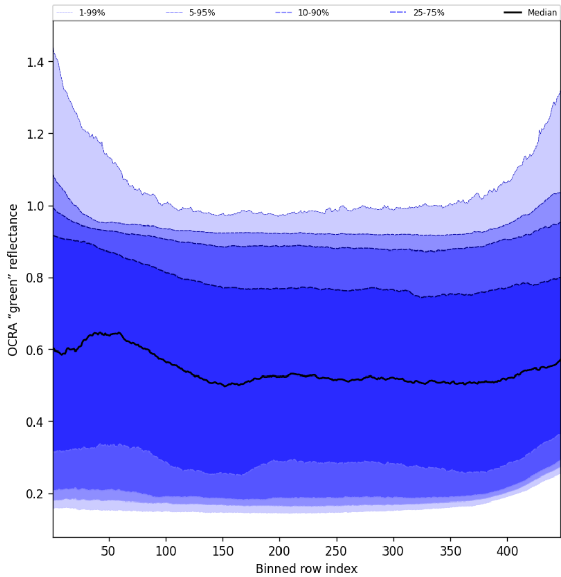
Figure 66: Along track statistics of “OCRA “green” reflectance” for 2025-12-01 to 2025-12-01
