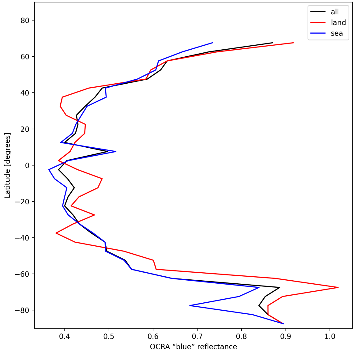
Figure 33: Zonal average of “OCRA “blue” reflectance” for 2025-12-01 to 2025-12-01.
