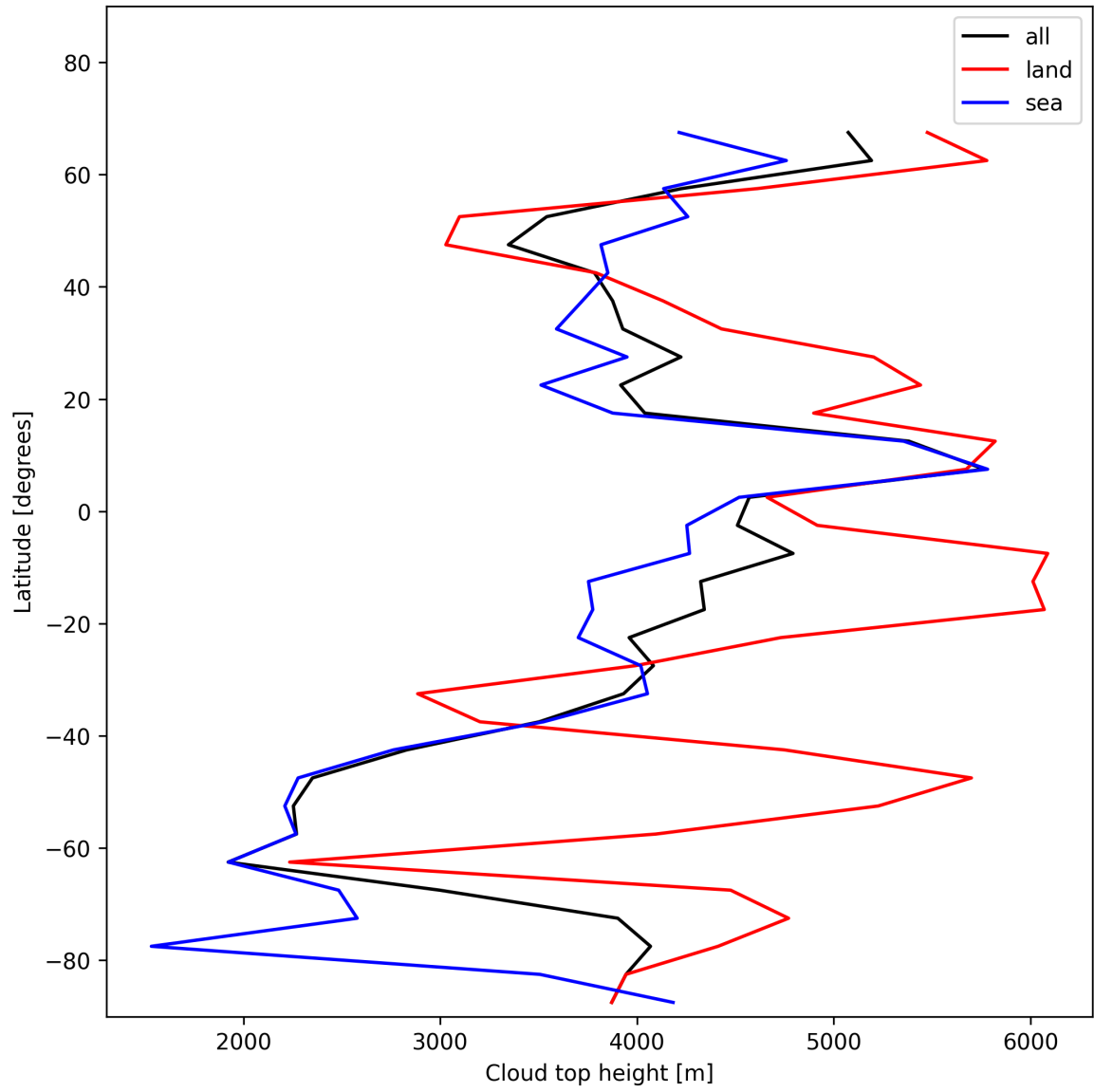
Figure 22: Zonal average of “Cloud top height” for 2025-12-01 to 2025-12-01.
