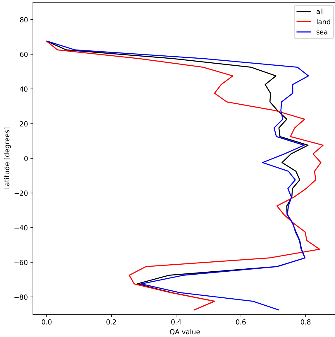
Figure 20: Zonal average of “QA value” for 2025-12-01 to 2025-12-01.
