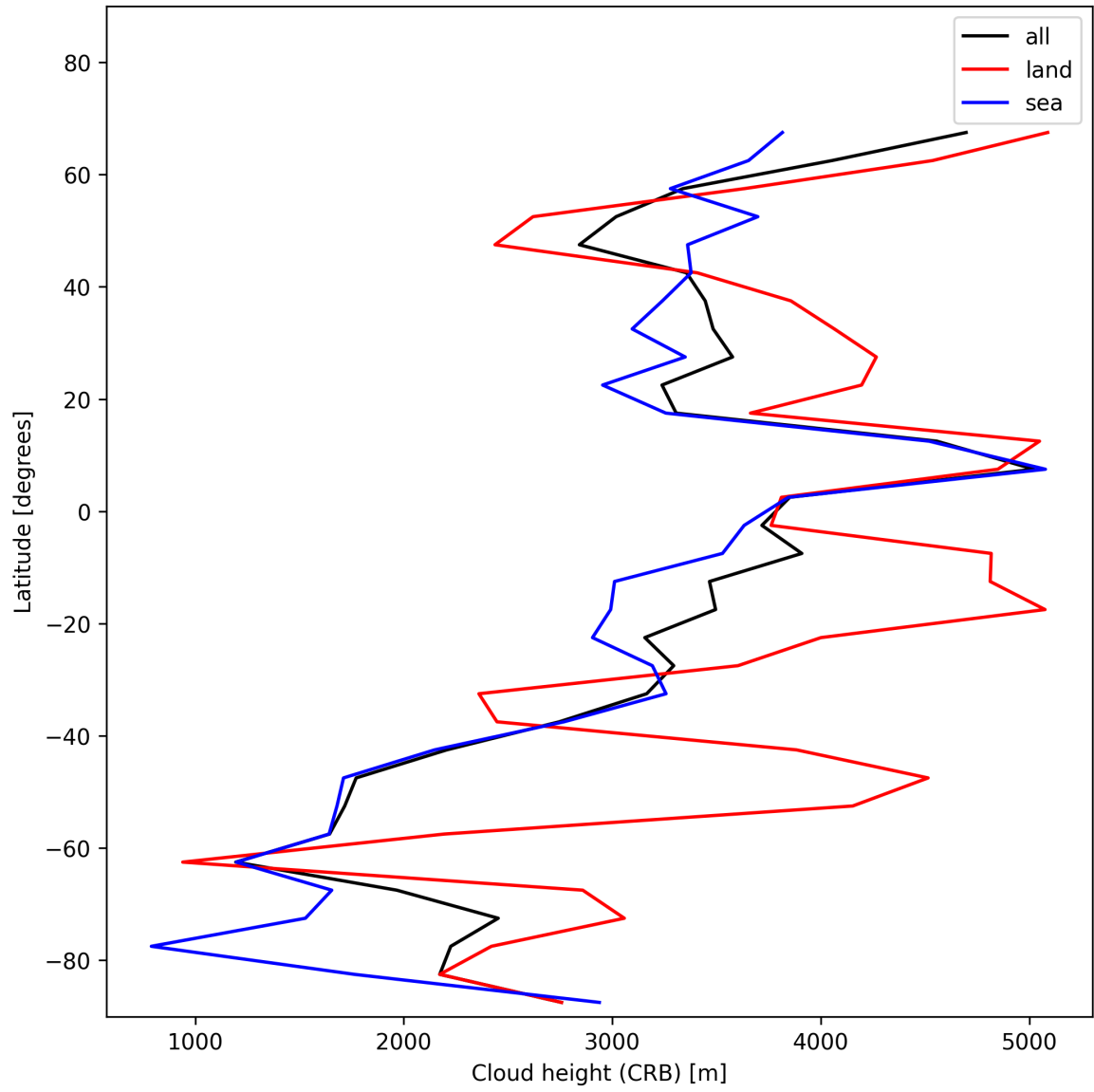
Figure 25: Zonal average of “Cloud height (CRB)” for 2025-12-01 to 2025-12-01.
