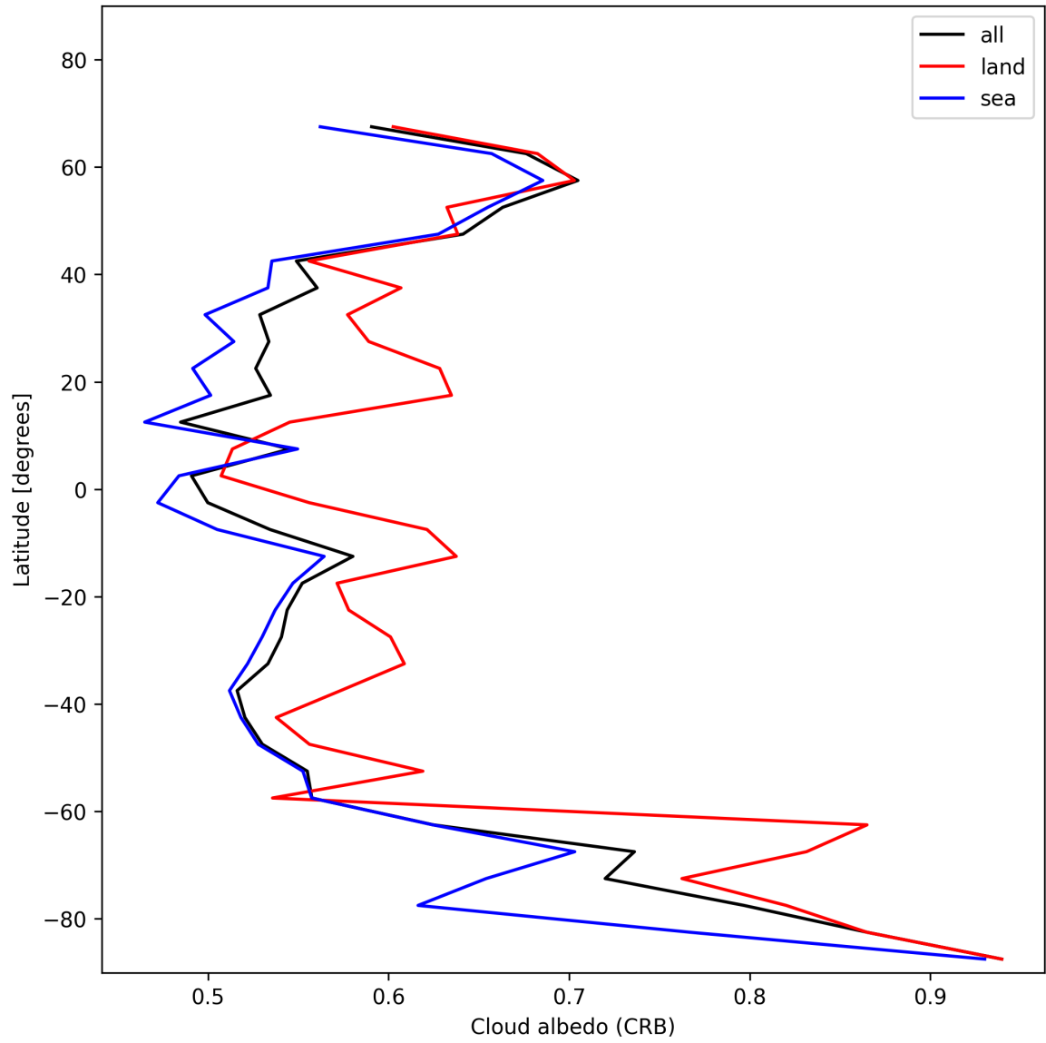
Figure 26: Zonal average of “Cloud albedo (CRB)” for 2025-12-01 to 2025-12-01.
