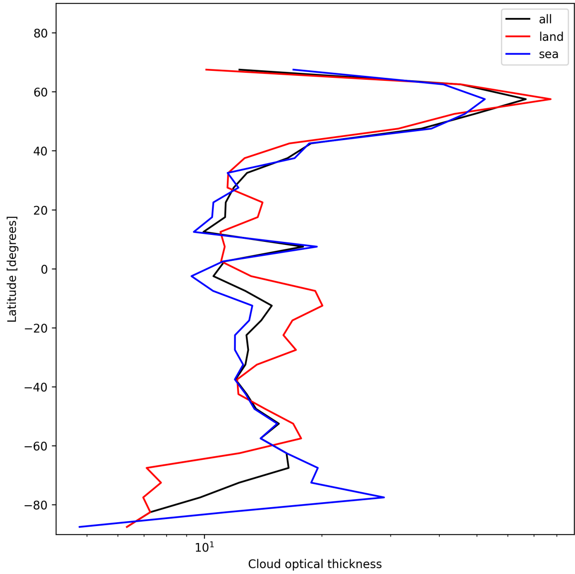
Figure 23: Zonal average of “Cloud optical thickness” for 2025-12-01 to 2025-12-01.
