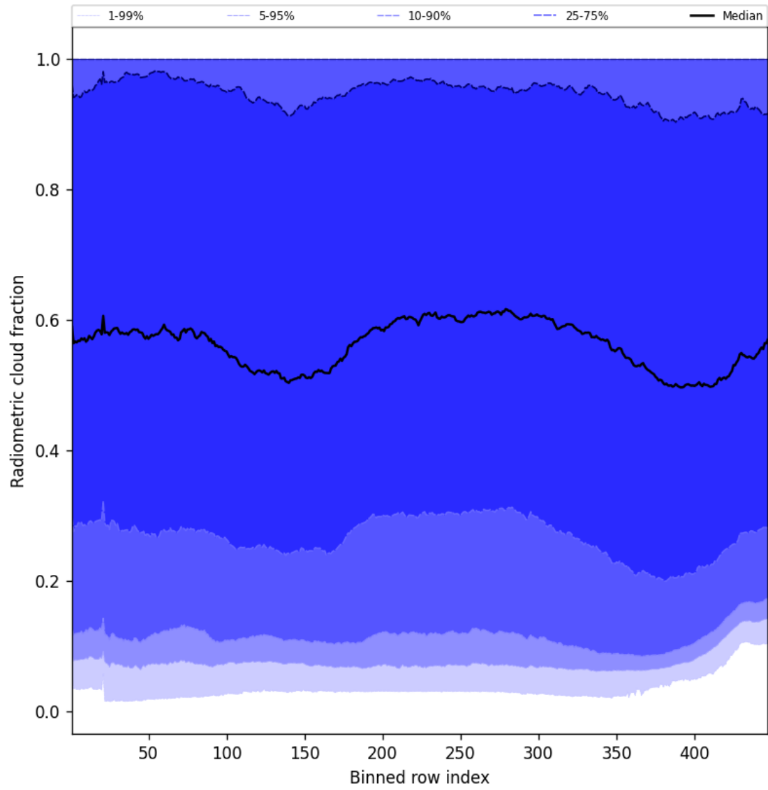
Figure 53: Along track statistics of “Radiometric cloud fraction” for 2025-12-01 to 2025-12-01
