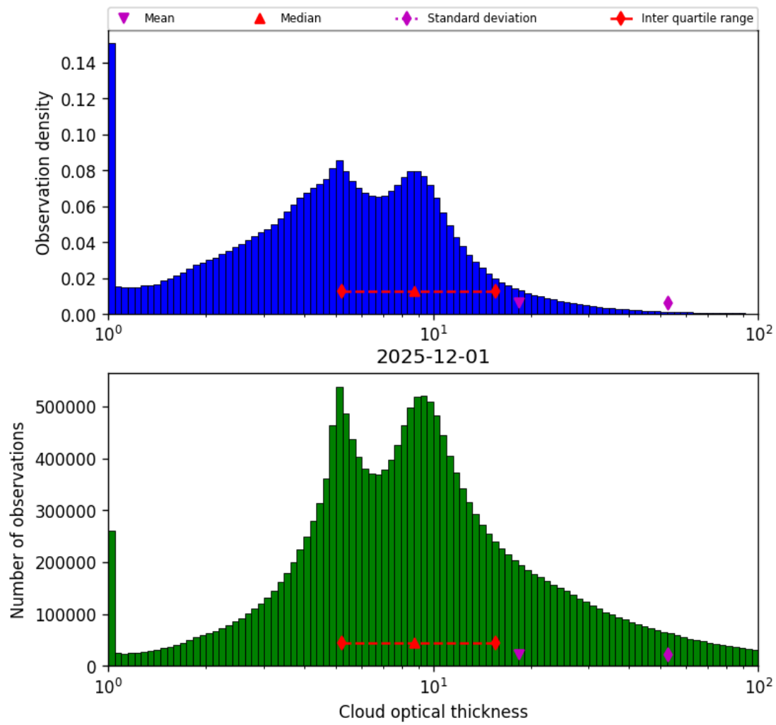
Figure 39: Histogram of “Cloud optical thickness” for 2025-12-01 to 2025-12-01
