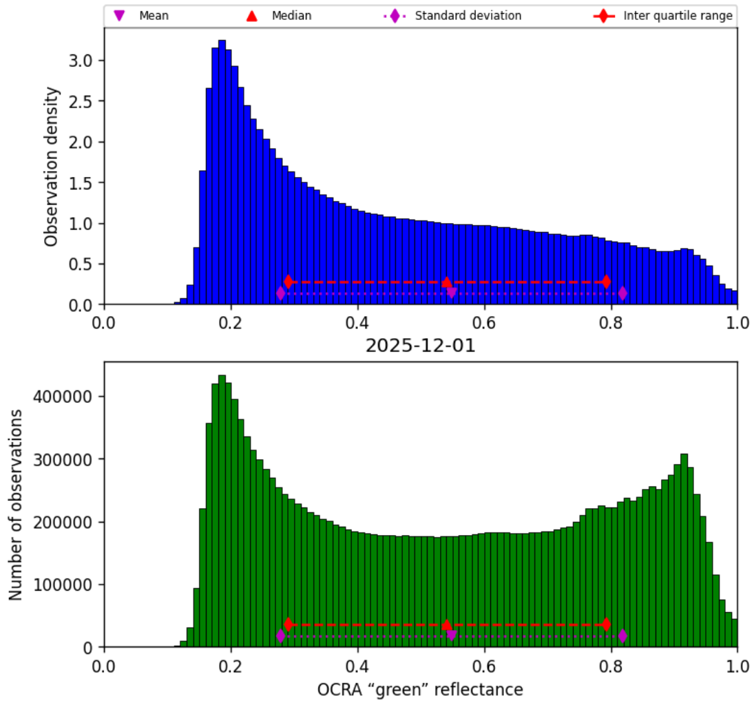
Figure 50: Histogram of “OCRA “green” reflectance” for 2025-12-01 to 2025-12-01
