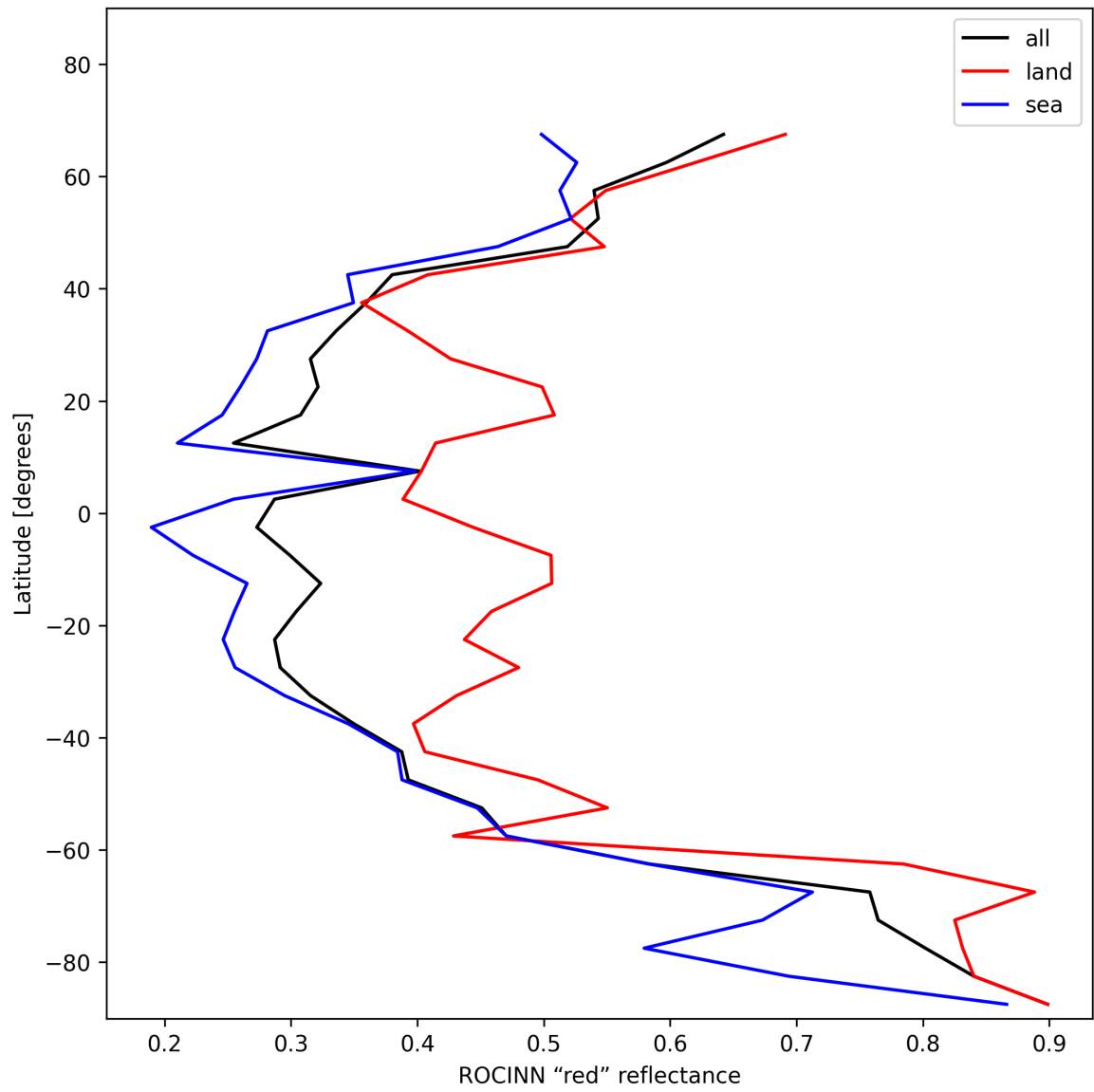
Figure 35: Zonal average of “ROCINN “red” reflectance” for 2025-12-01 to 2025-12-01.
