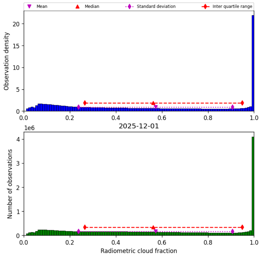
Figure 37: Histogram of “Radiometric cloud fraction” for 2025-12-01 to 2025-12-01
