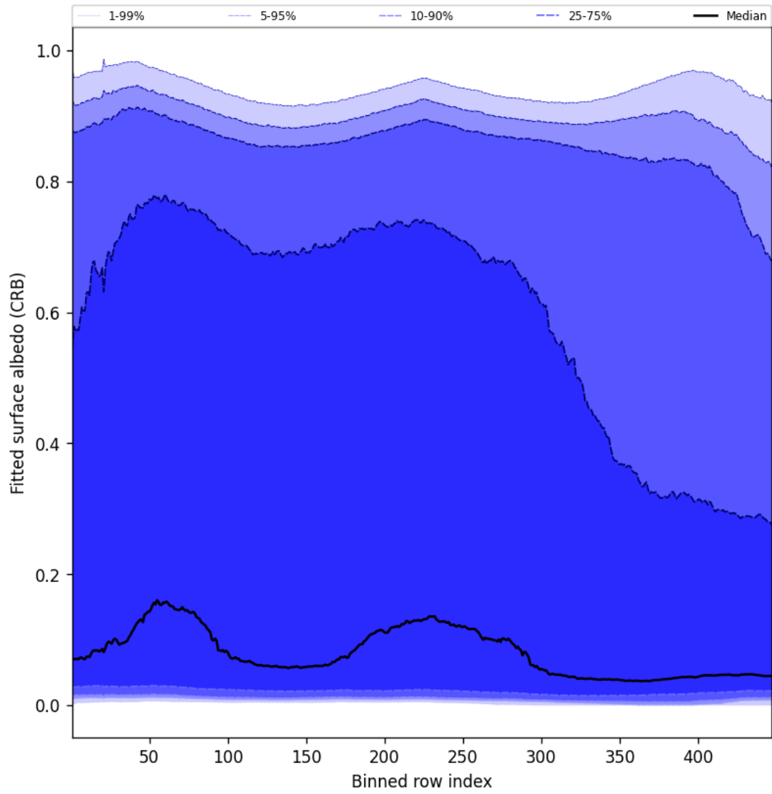
Figure 60: Along track statistics of “Fitted surface albedo (CRB)” for 2025-12-01 to 2025-12-01
