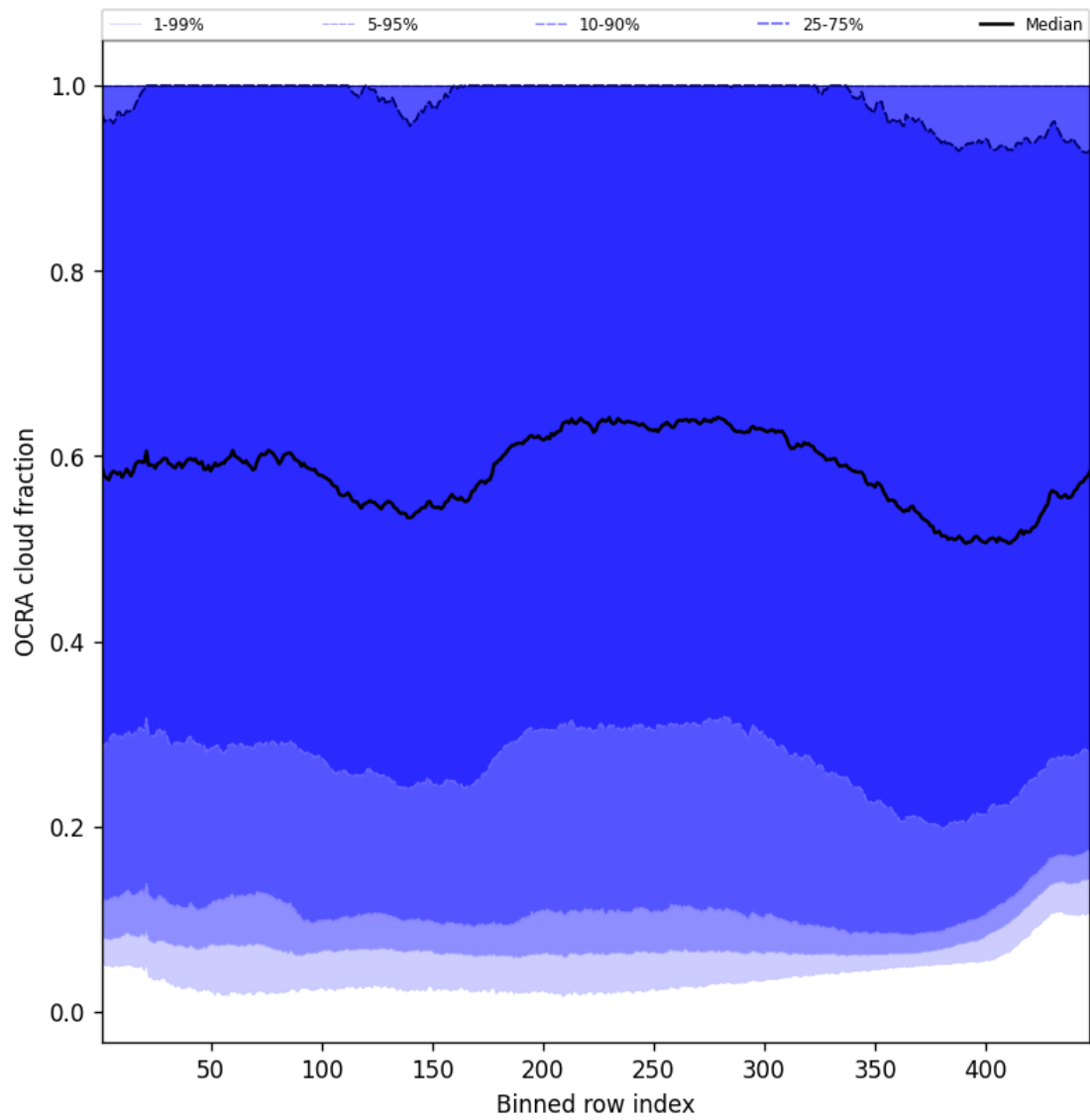
Figure 64: Along track statistics of “OCRA cloud fraction” for 2025-12-01 to 2025-12-01
