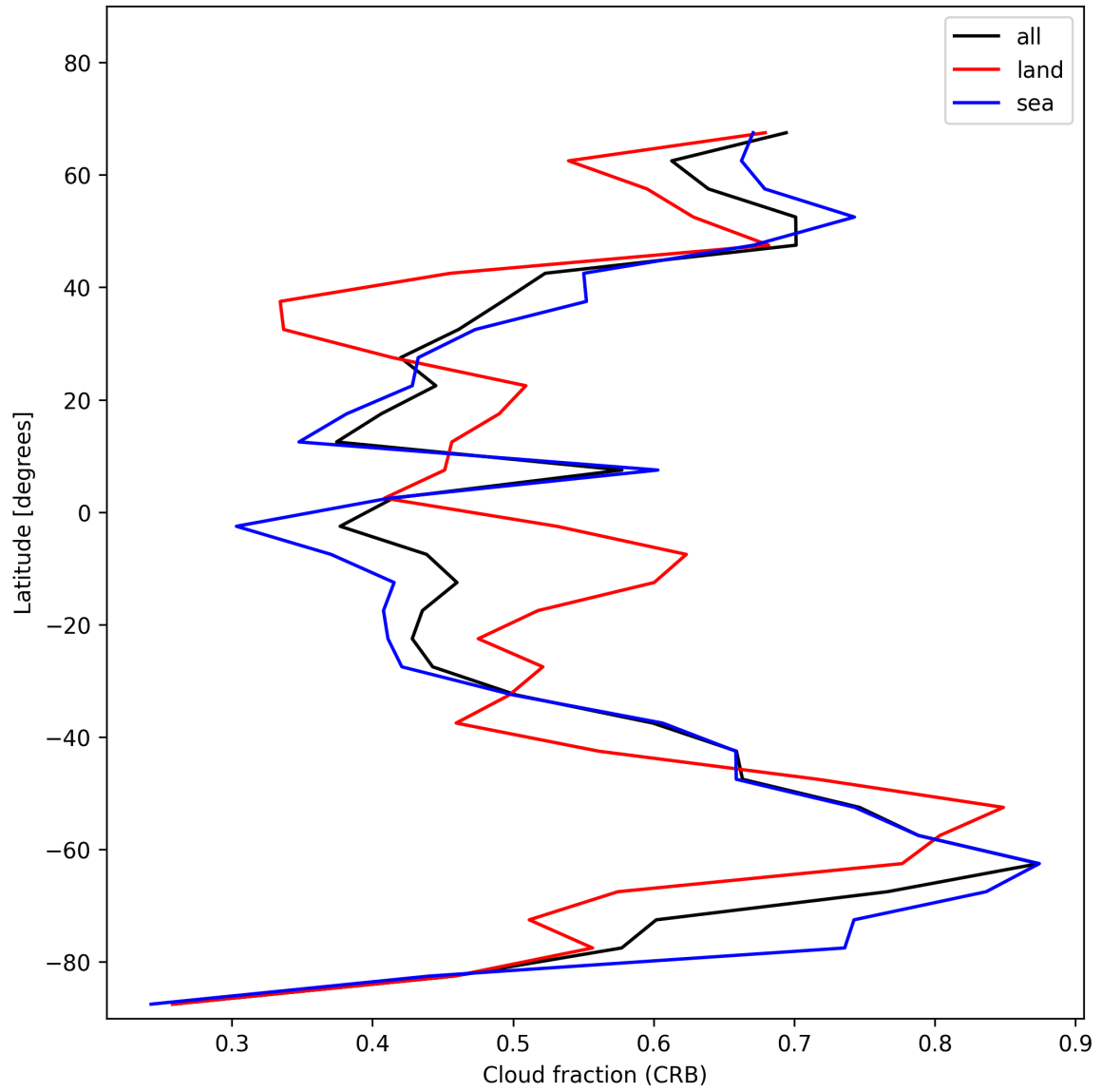
Figure 24: Zonal average of “Cloud fraction (CRB)” for 2025-12-01 to 2025-12-01.
