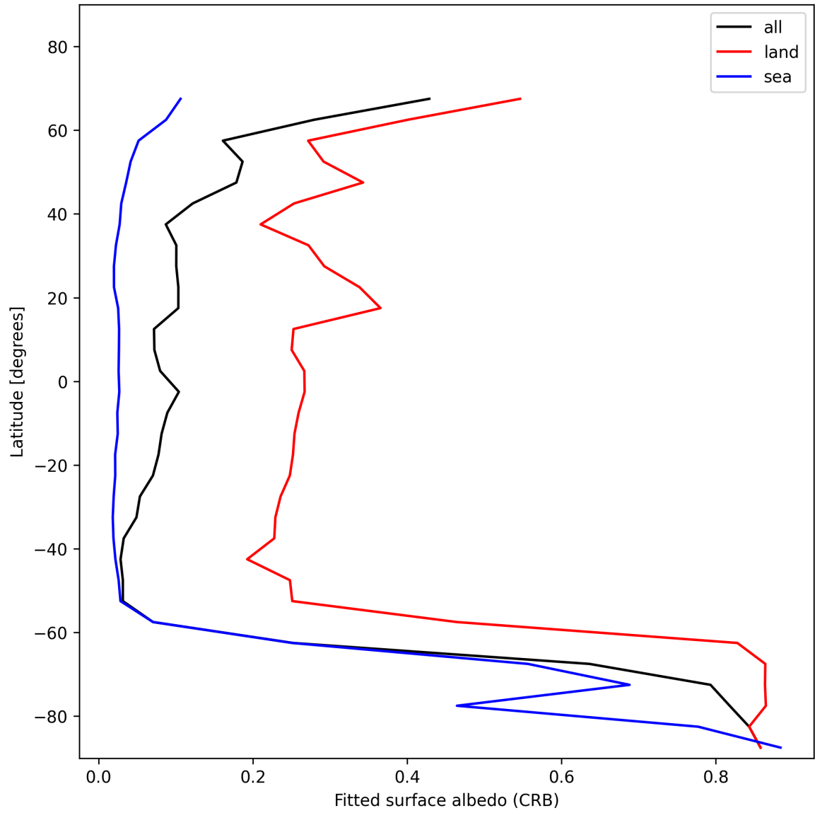
Figure 28: Zonal average of “Fitted surface albedo (CRB)” for 2025-12-01 to 2025-12-01.
