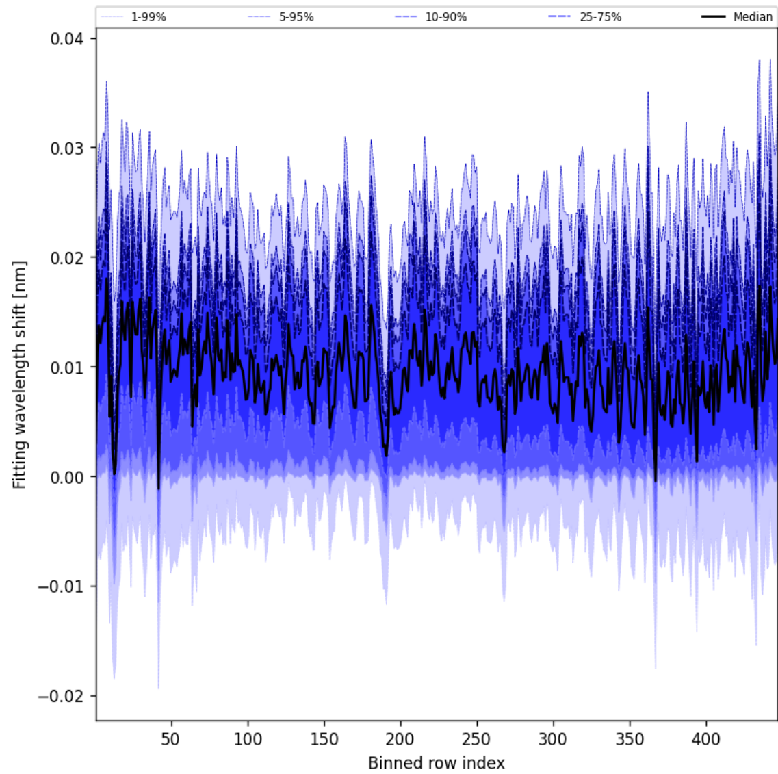
Figure 63: Along track statistics of “Fitting wavelength shift” for 2025-12-01 to 2025-12-01
