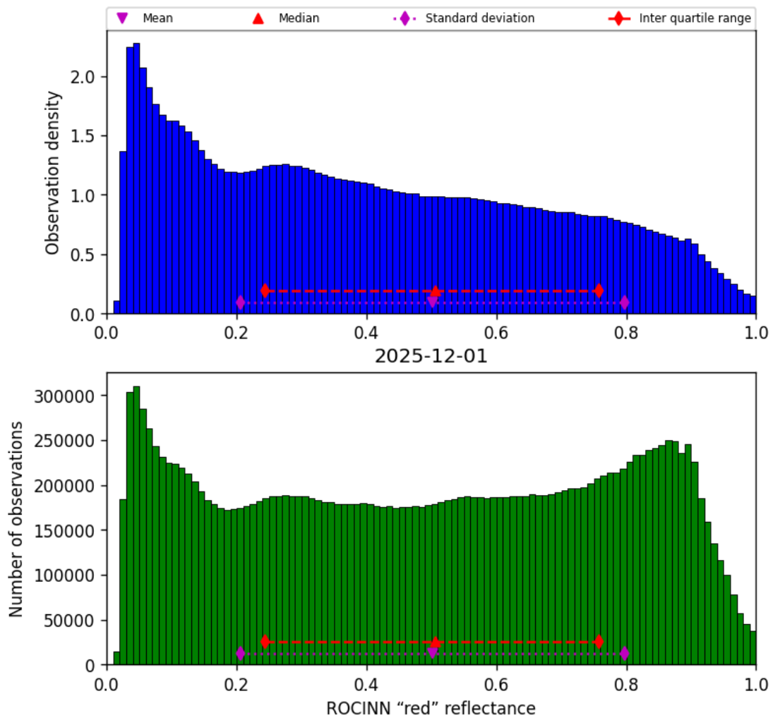
Figure 51: Histogram of “ROCINN “red” reflectance” for 2025-12-01 to 2025-12-01
