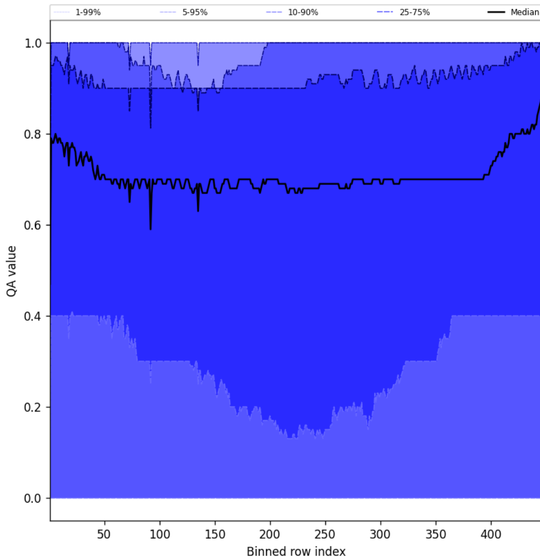
Figure 52: Along track statistics of “QA value” for 2025-12-01 to 2025-12-01
