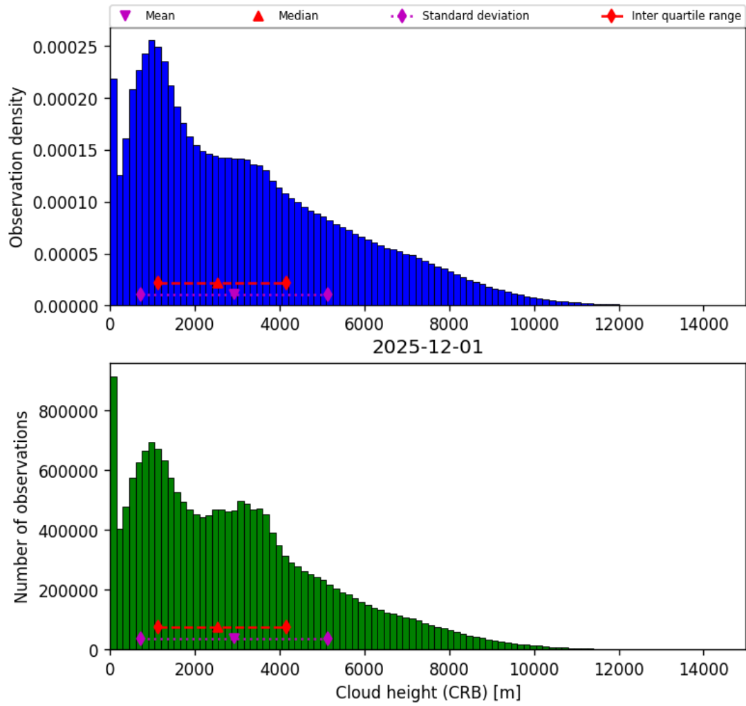
Figure 41: Histogram of “Cloud height (CRB)” for 2025-12-01 to 2025-12-01
