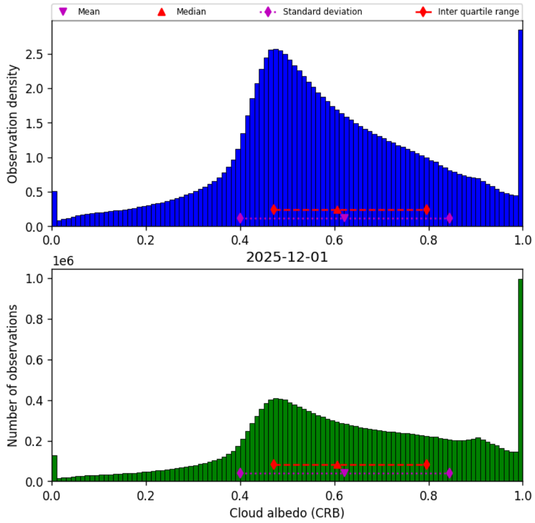
Figure 42: Histogram of “Cloud albedo (CRB)” for 2025-12-01 to 2025-12-01
