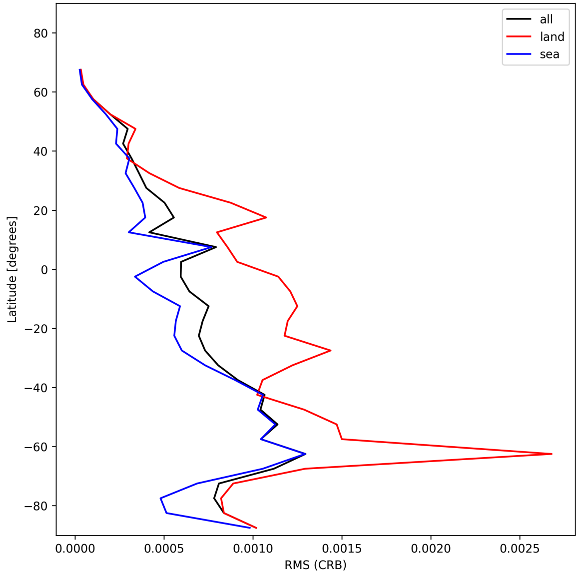
Figure 30: Zonal average of “RMS (CRB)” for 2025-12-01 to 2025-12-01.
