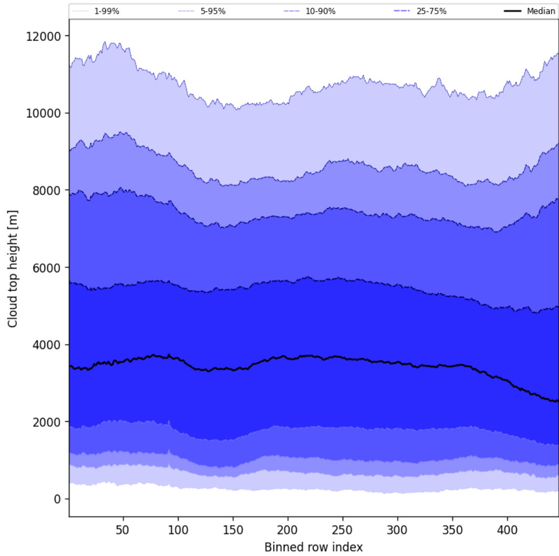
Figure 54: Along track statistics of “Cloud top height” for 2025-12-01 to 2025-12-01
