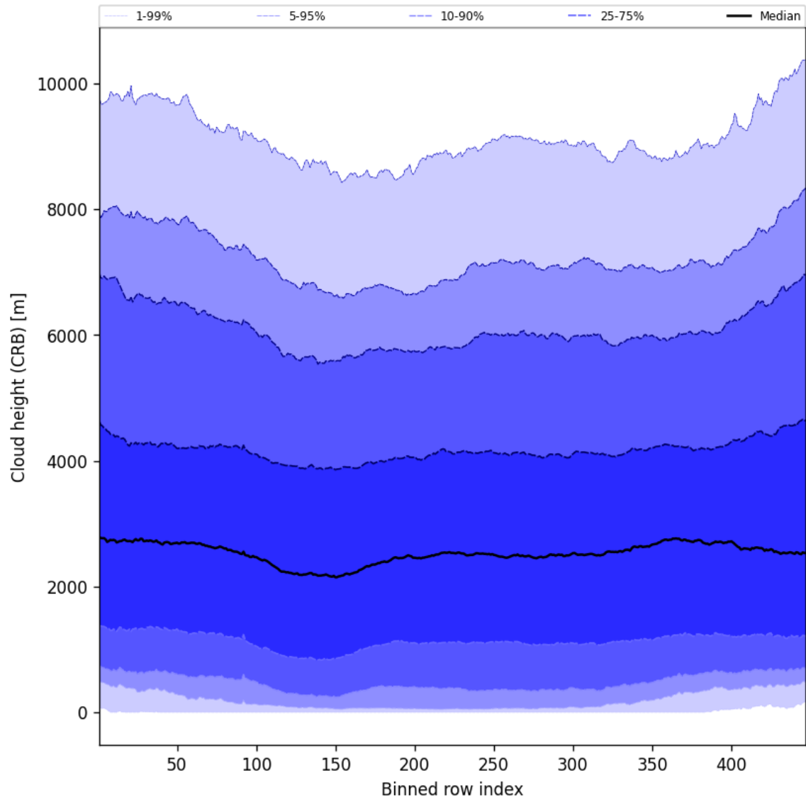
Figure 57: Along track statistics of “Cloud height (CRB)” for 2025-12-01 to 2025-12-01
