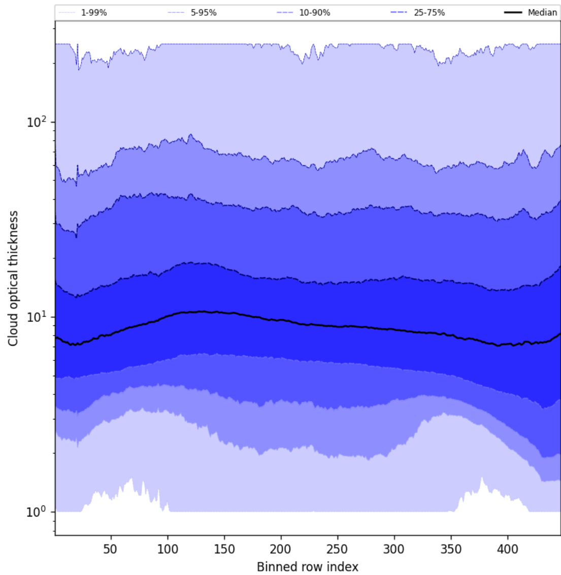
Figure 55: Along track statistics of “Cloud optical thickness” for 2025-12-01 to 2025-12-01
