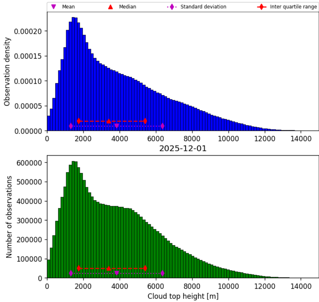
Figure 38: Histogram of “Cloud top height” for 2025-12-01 to 2025-12-01
