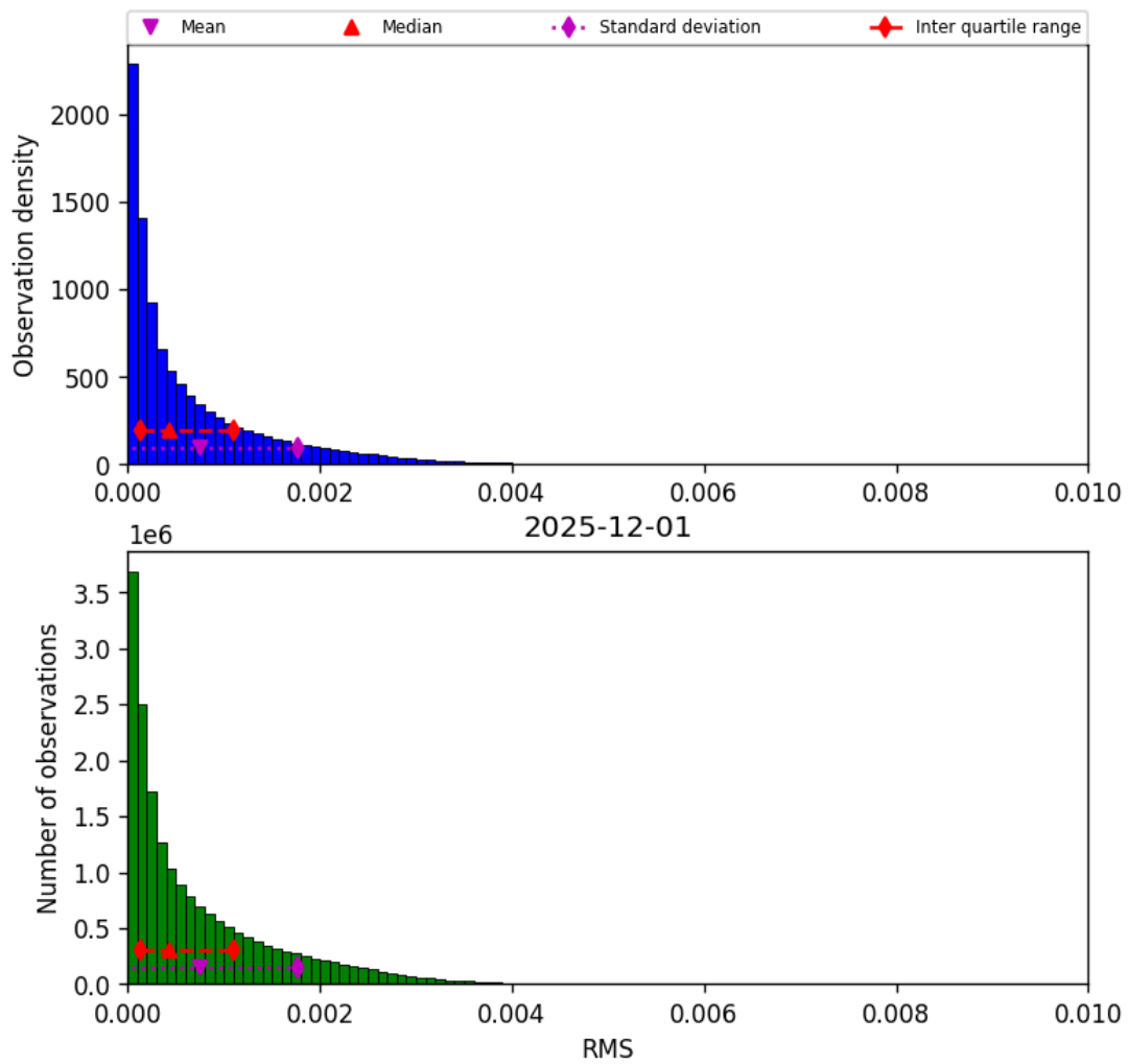
Figure 45: Histogram of “RMS” for 2025-12-01 to 2025-12-01
