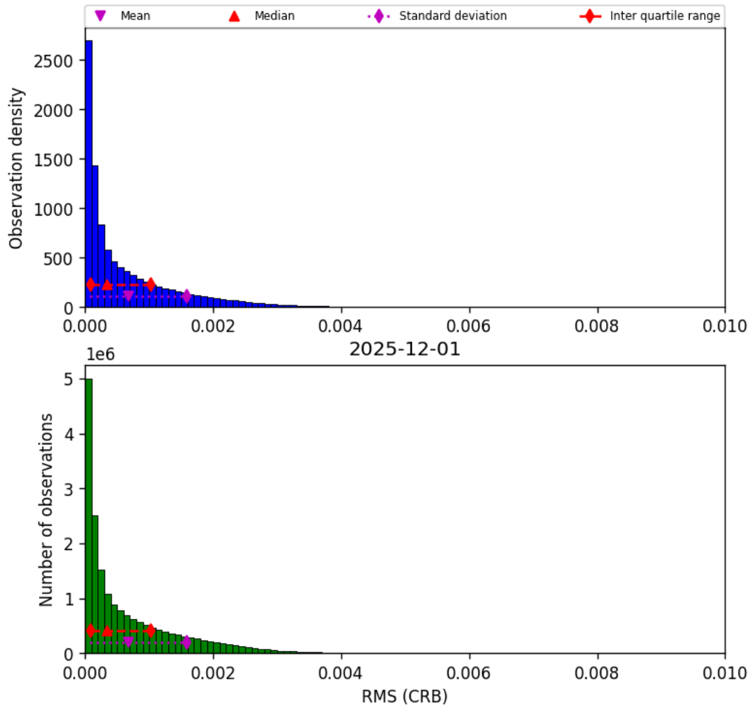
Figure 46: Histogram of “RMS (CRB)” for 2025-12-01 to 2025-12-01
