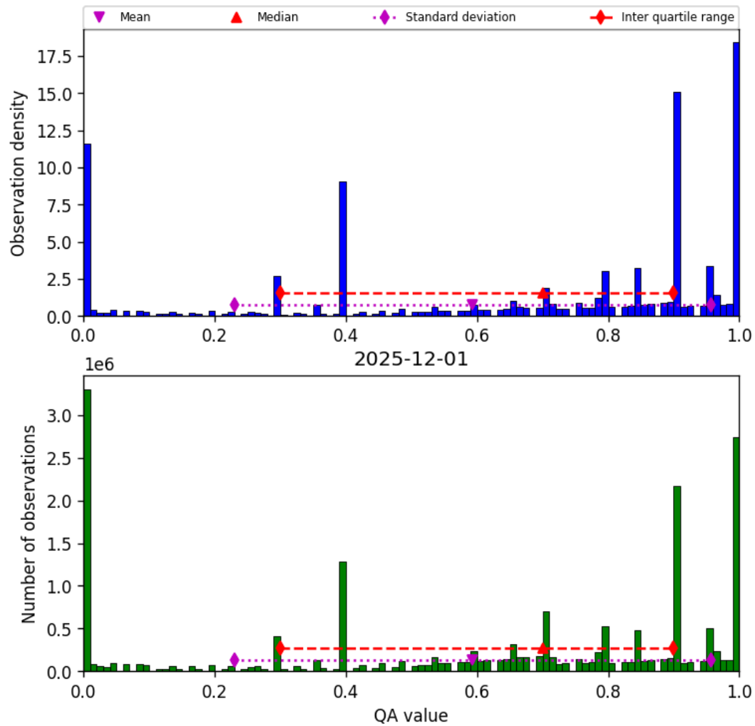
Figure 36: Histogram of “QA value” for 2025-12-01 to 2025-12-01
