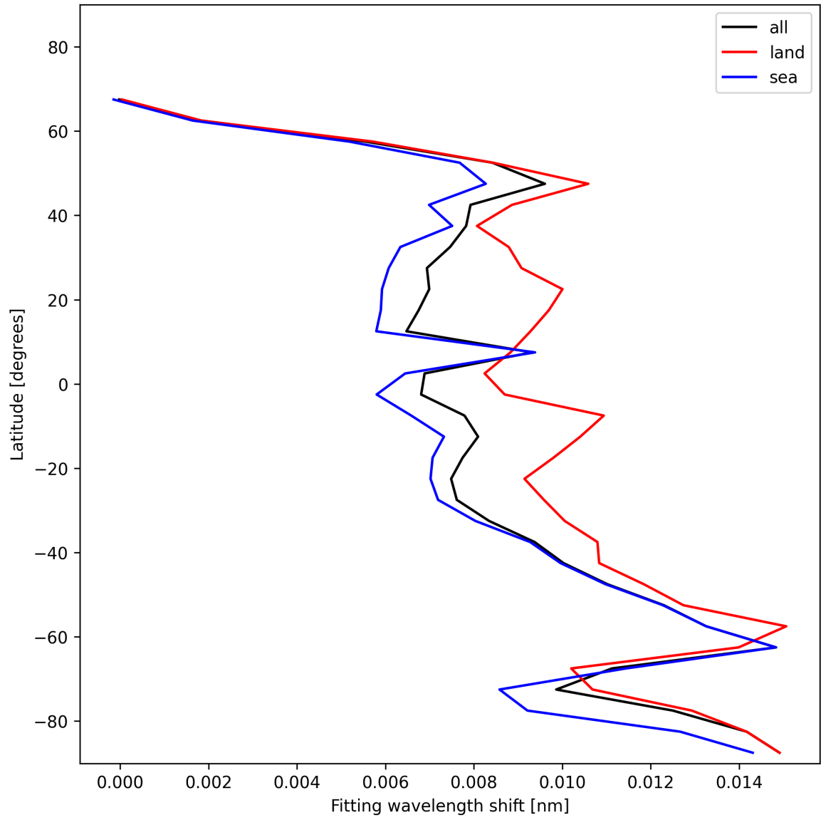
Figure 31: Zonal average of “Fitting wavelength shift” for 2025-12-01 to 2025-12-01.
