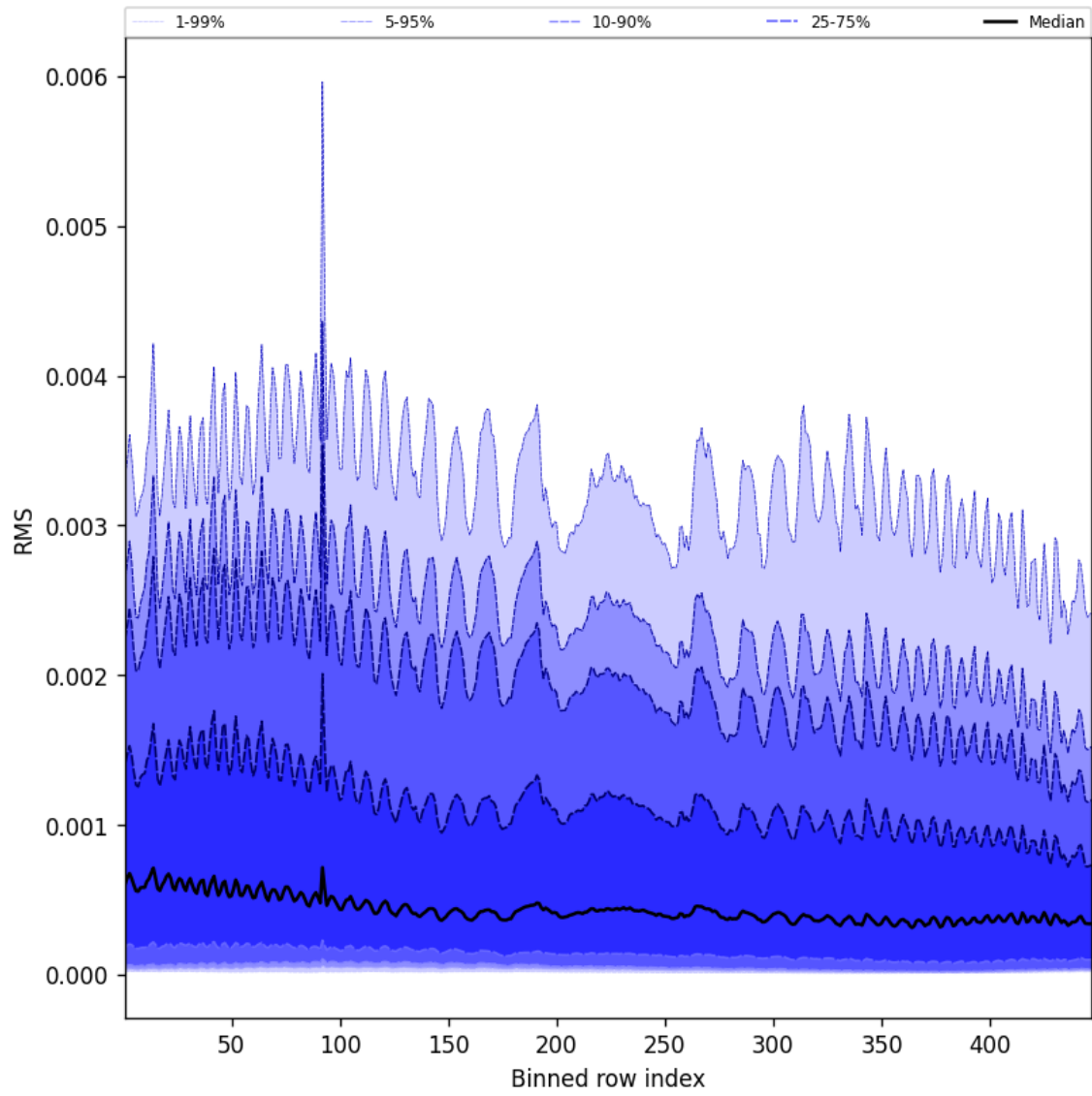
Figure 61: Along track statistics of “RMS” for 2025-12-01 to 2025-12-01
