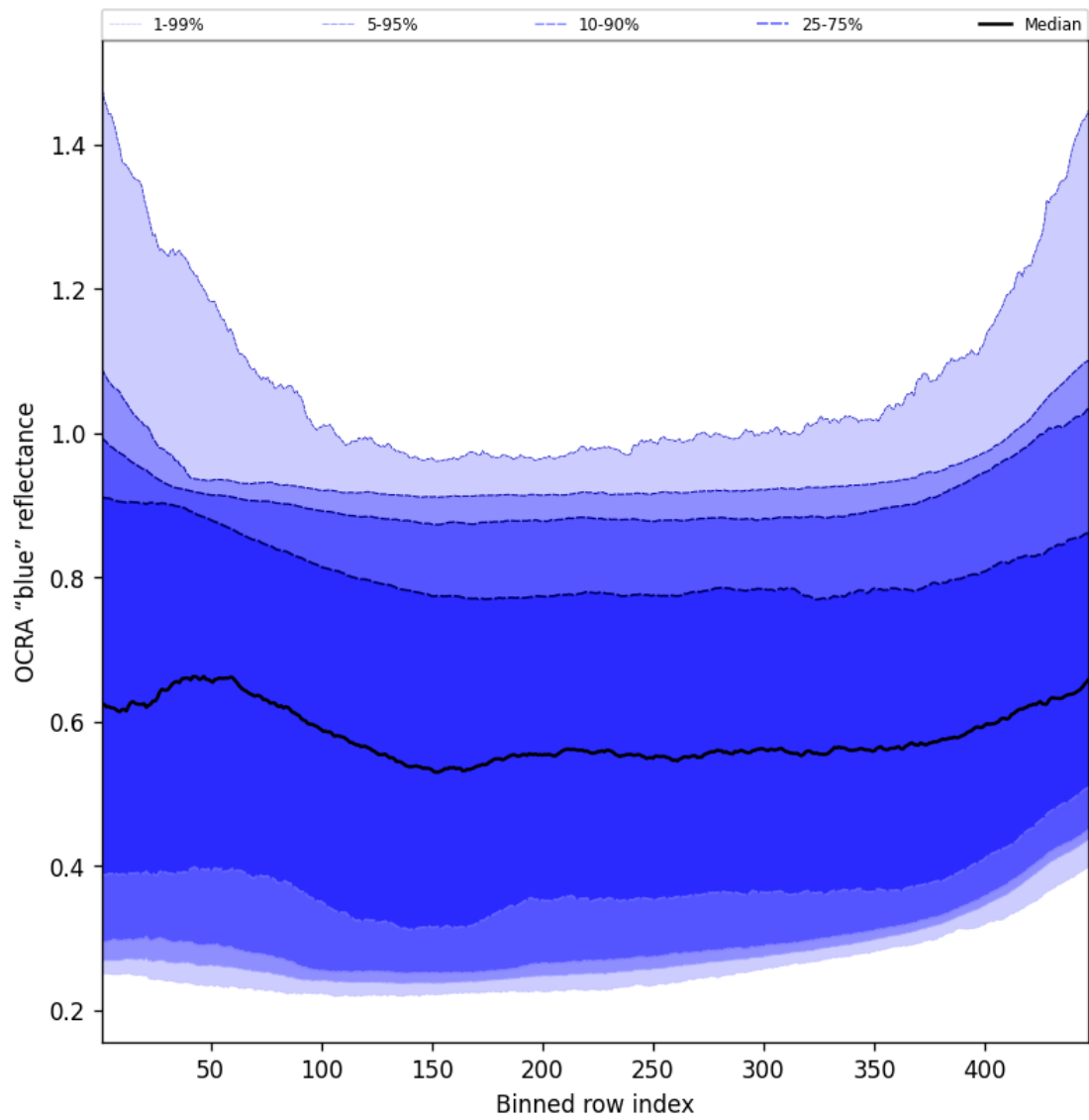
Figure 65: Along track statistics of "OCRA "blue" reflectance" for 2025-12-01 to 2025-12-01
