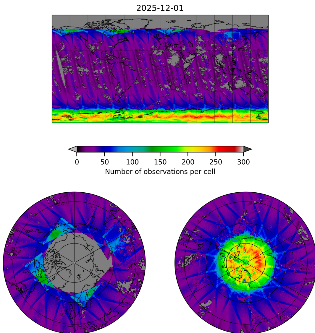
Figure 19: Map of the number of observations for 2025-12-01 to 2025-12-01
