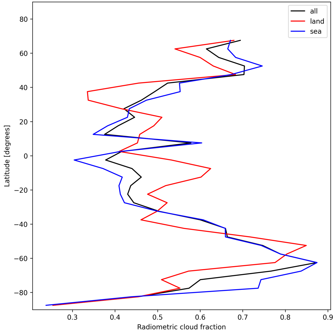
Figure 21: Zonal average of “Radiometric cloud fraction” for 2025-12-01 to 2025-12-01.
