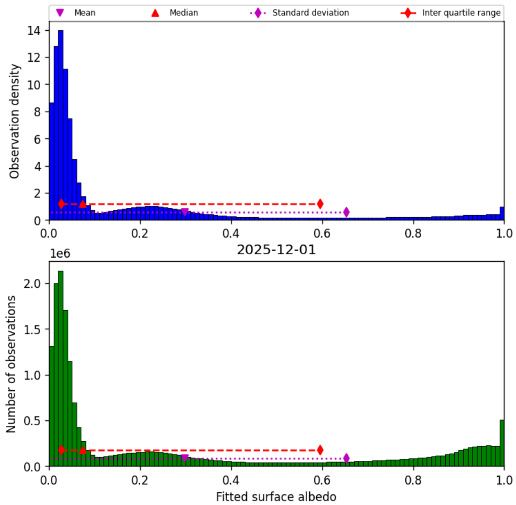
Figure 43: Histogram of “Fitted surface albedo” for 2025-12-01 to 2025-12-01
