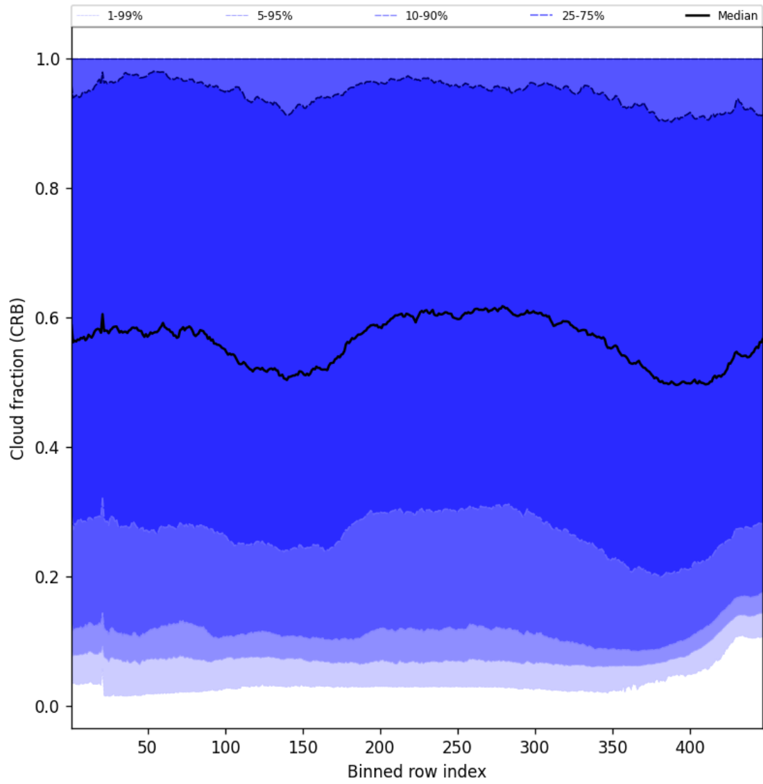
Figure 56: Along track statistics of “Cloud fraction (CRB)” for 2025-12-01 to 2025-12-01
