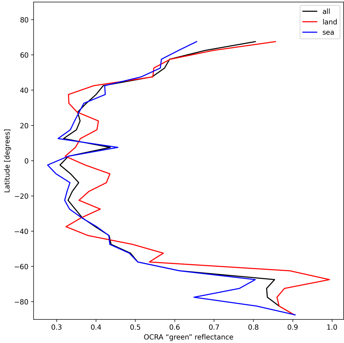
Figure 34: Zonal average of “OCRA “green” reflectance” for 2025-12-01 to 2025-12-01.
