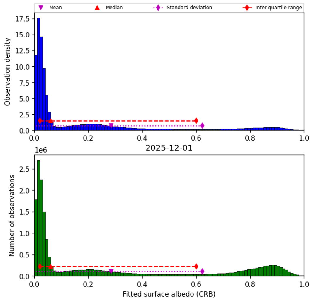
Figure 44: Histogram of “Fitted surface albedo (CRB)” for 2025-12-01 to 2025-12-01
