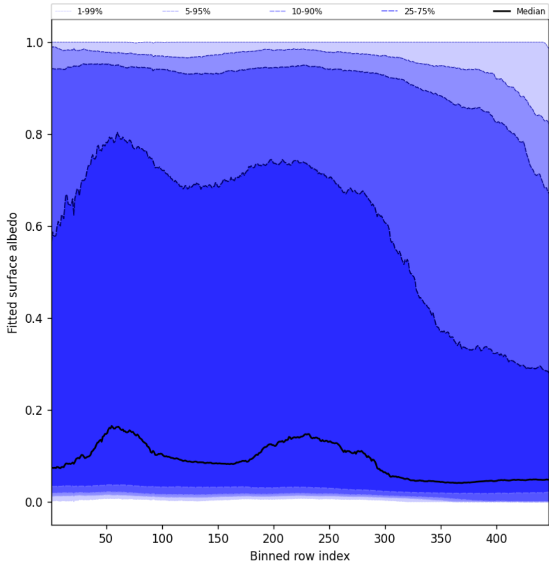
Figure 59: Along track statistics of “Fitted surface albedo” for 2025-12-01 to 2025-12-01
