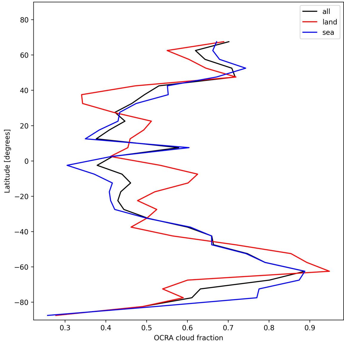
Figure 32: Zonal average of “OCRA cloud fraction” for 2025-12-01 to 2025-12-01.
