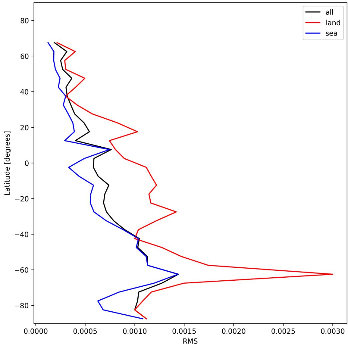
Figure 29: Zonal average of “RMS” for 2025-12-01 to 2025-12-01.
