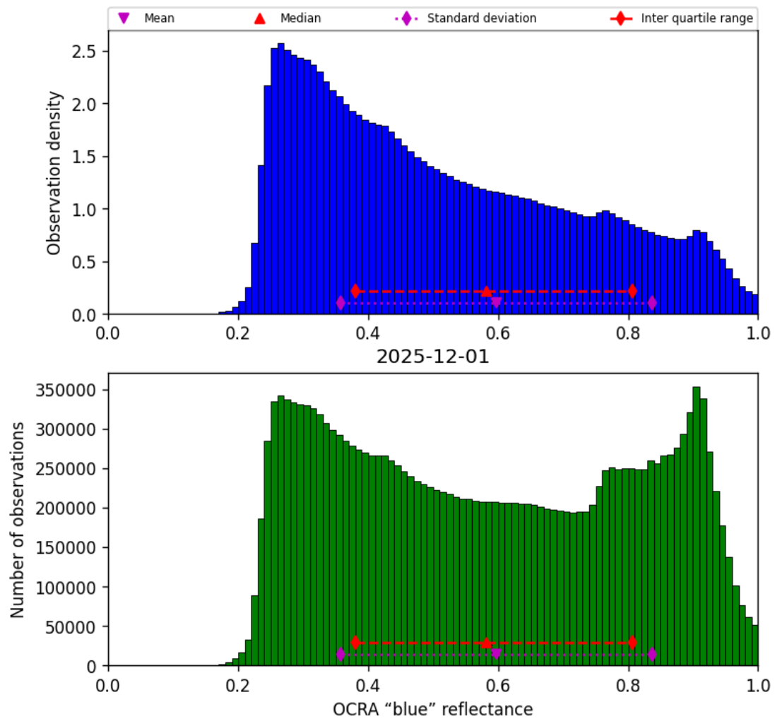
Figure 49: Histogram of “OCRA “blue” reflectance” for 2025-12-01 to 2025-12-01
