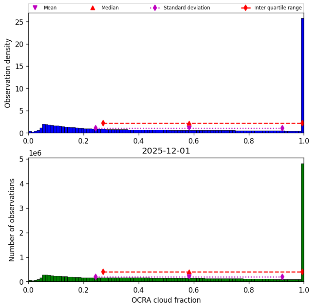
Figure 48: Histogram of “OCRA cloud fraction” for 2025-12-01 to 2025-12-01
