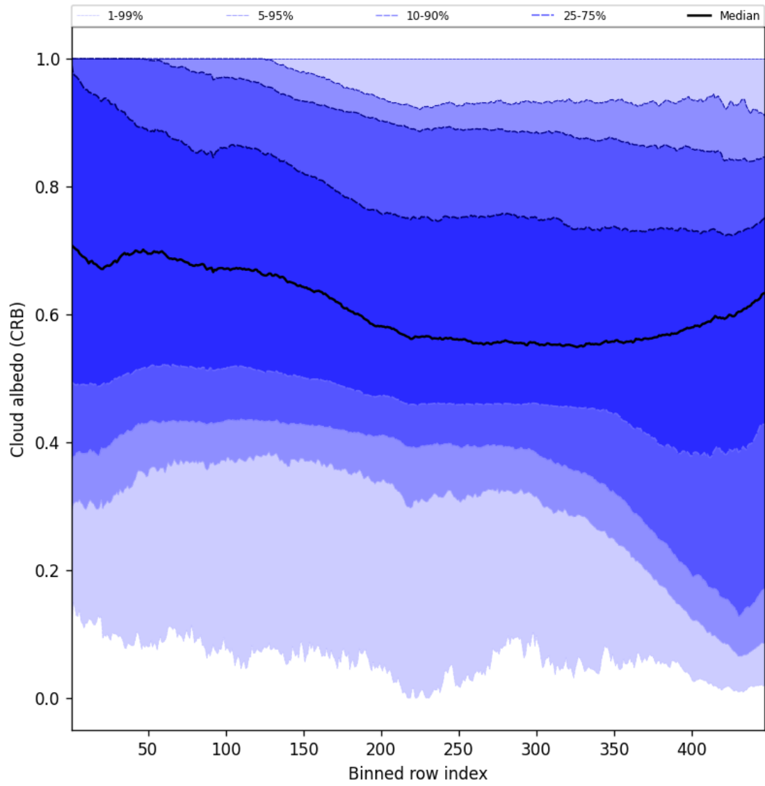
Figure 58: Along track statistics of “Cloud albedo (CRB)” for 2025-12-01 to 2025-12-01
