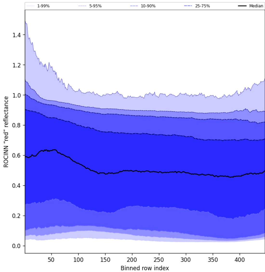
Figure 67: Along track statistics of "ROCINN "red" reflectance" for 2025-12-01 to 2025-12-01
