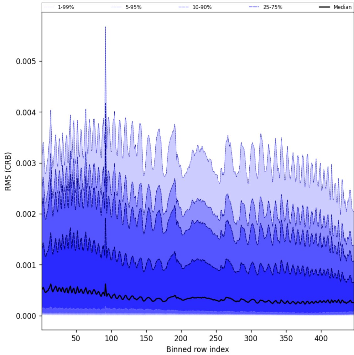
Figure 62: Along track statistics of “RMS (CRB)” for 2025-12-01 to 2025-12-01
