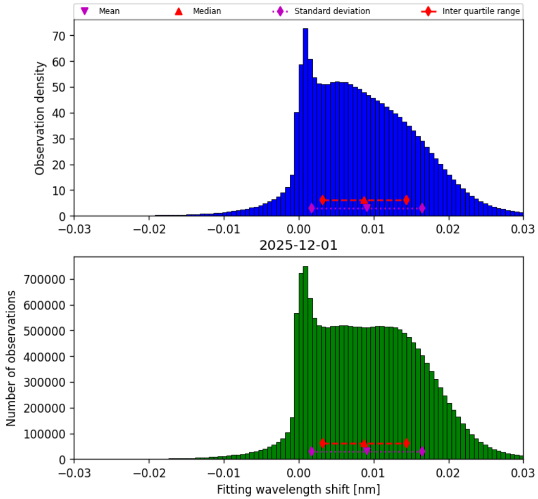
Figure 47: Histogram of “Fitting wavelength shift” for 2025-12-01 to 2025-12-01
