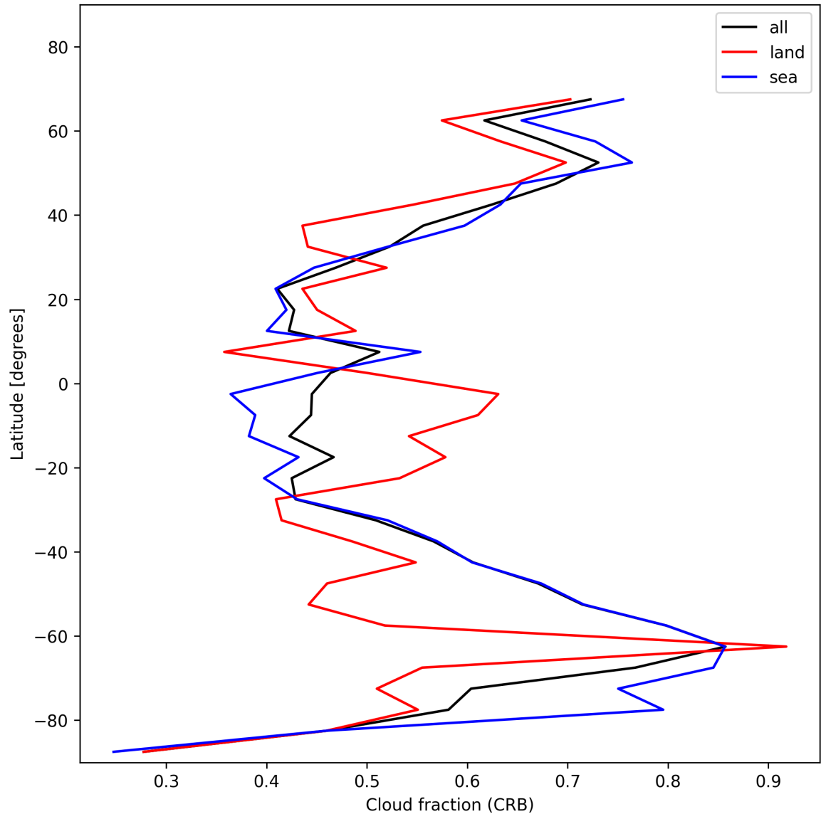
Figure 24: Zonal average of “Cloud fraction (CRB)” for 2025-12-02 to 2025-12-02.
