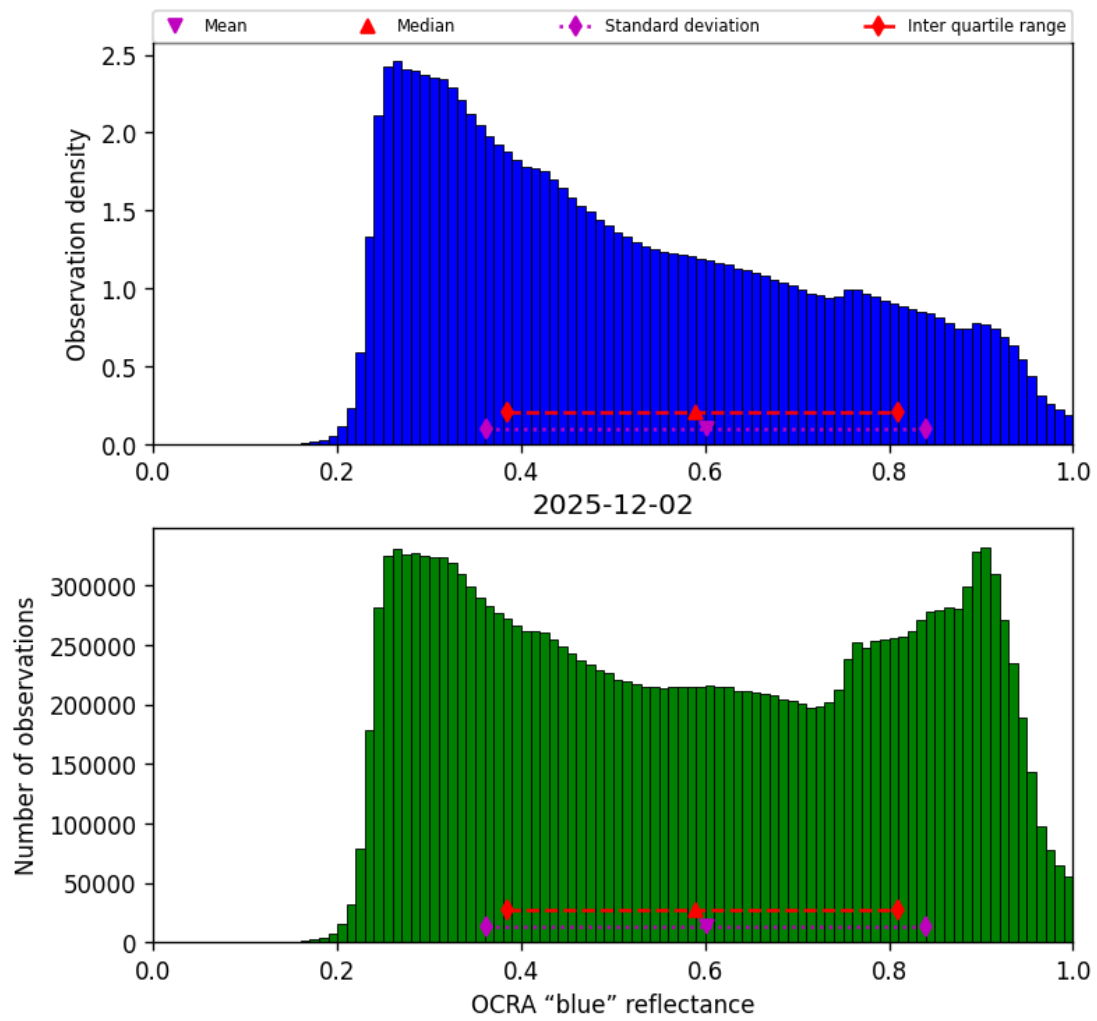
Figure 49: Histogram of “OCRA “blue” reflectance” for 2025-12-02 to 2025-12-02
