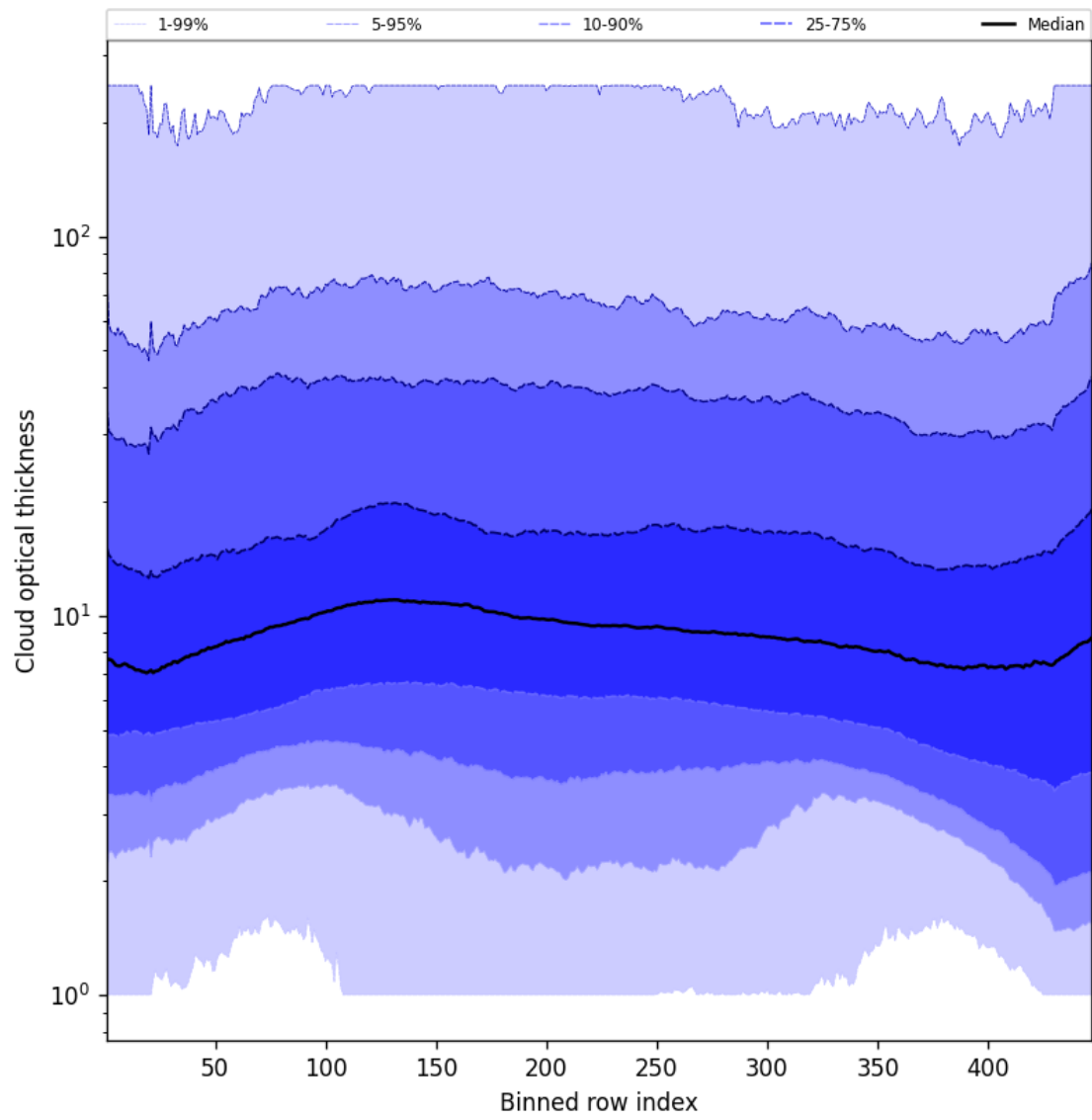
Figure 55: Along track statistics of “Cloud optical thickness” for 2025-12-02 to 2025-12-02
