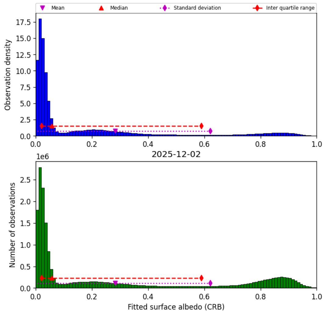
Figure 44: Histogram of “Fitted surface albedo (CRB)” for 2025-12-02 to 2025-12-02
