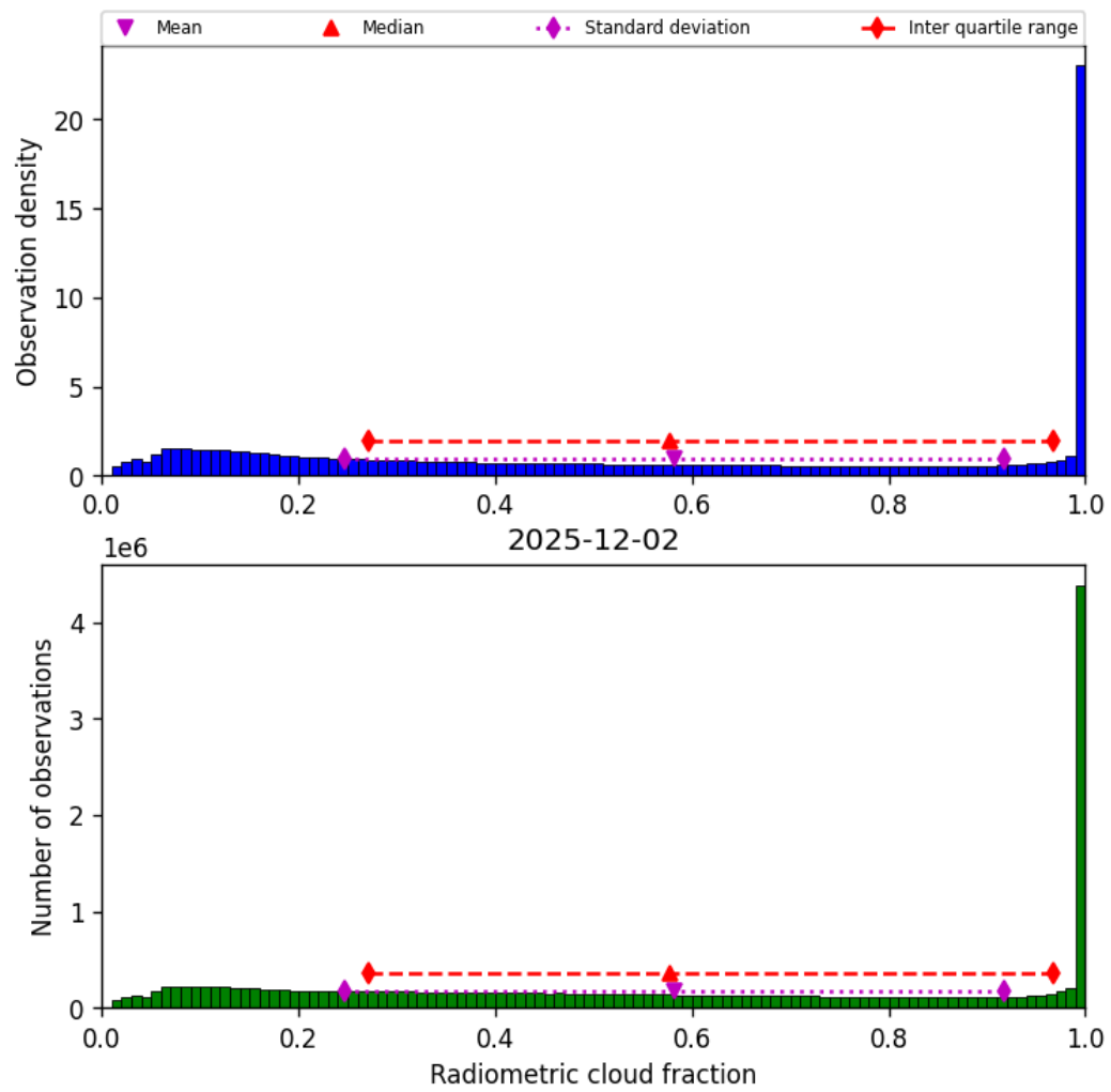
Figure 37: Histogram of “Radiometric cloud fraction” for 2025-12-02 to 2025-12-02
