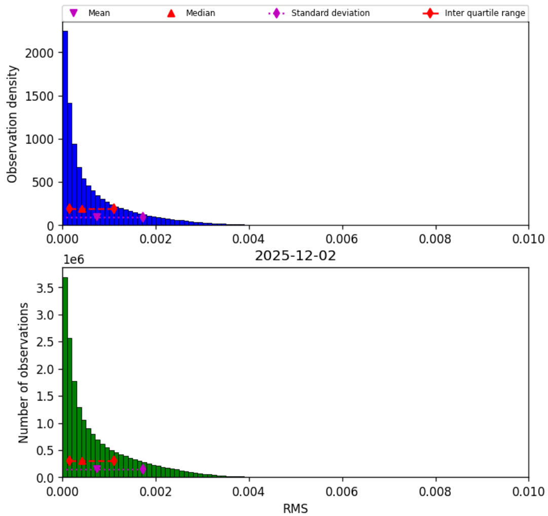
Figure 45: Histogram of “RMS” for 2025-12-02 to 2025-12-02
