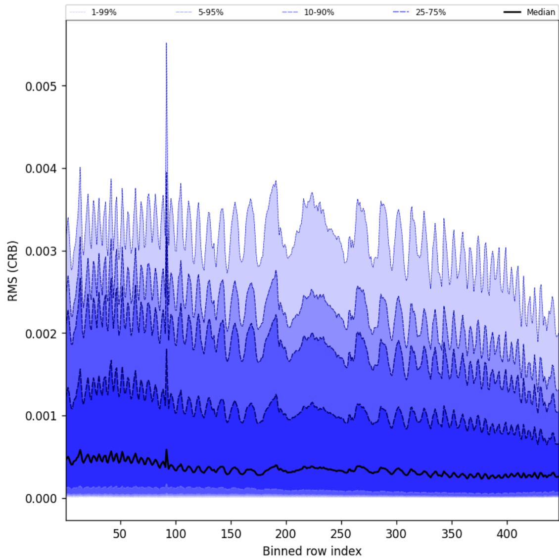
Figure 62: Along track statistics of “RMS (CRB)” for 2025-12-02 to 2025-12-02
