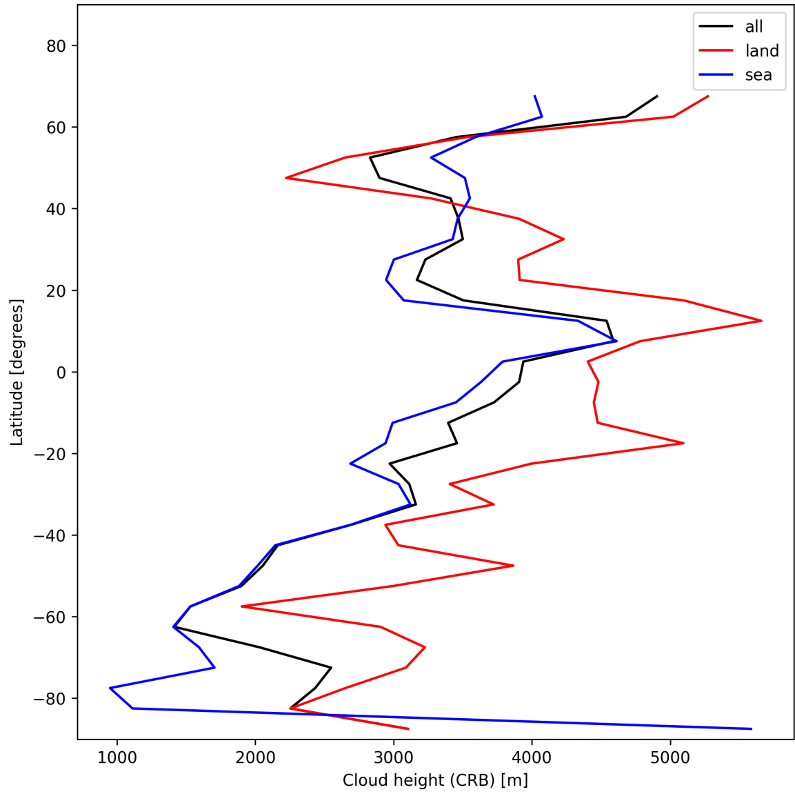
Figure 25: Zonal average of “Cloud height (CRB)” for 2025-12-02 to 2025-12-02.
