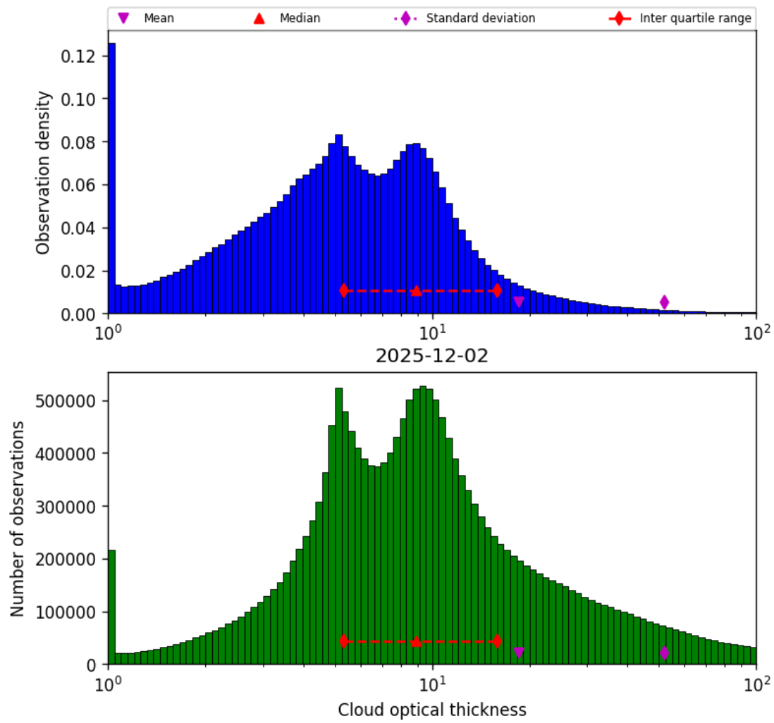
Figure 39: Histogram of “Cloud optical thickness” for 2025-12-02 to 2025-12-02
