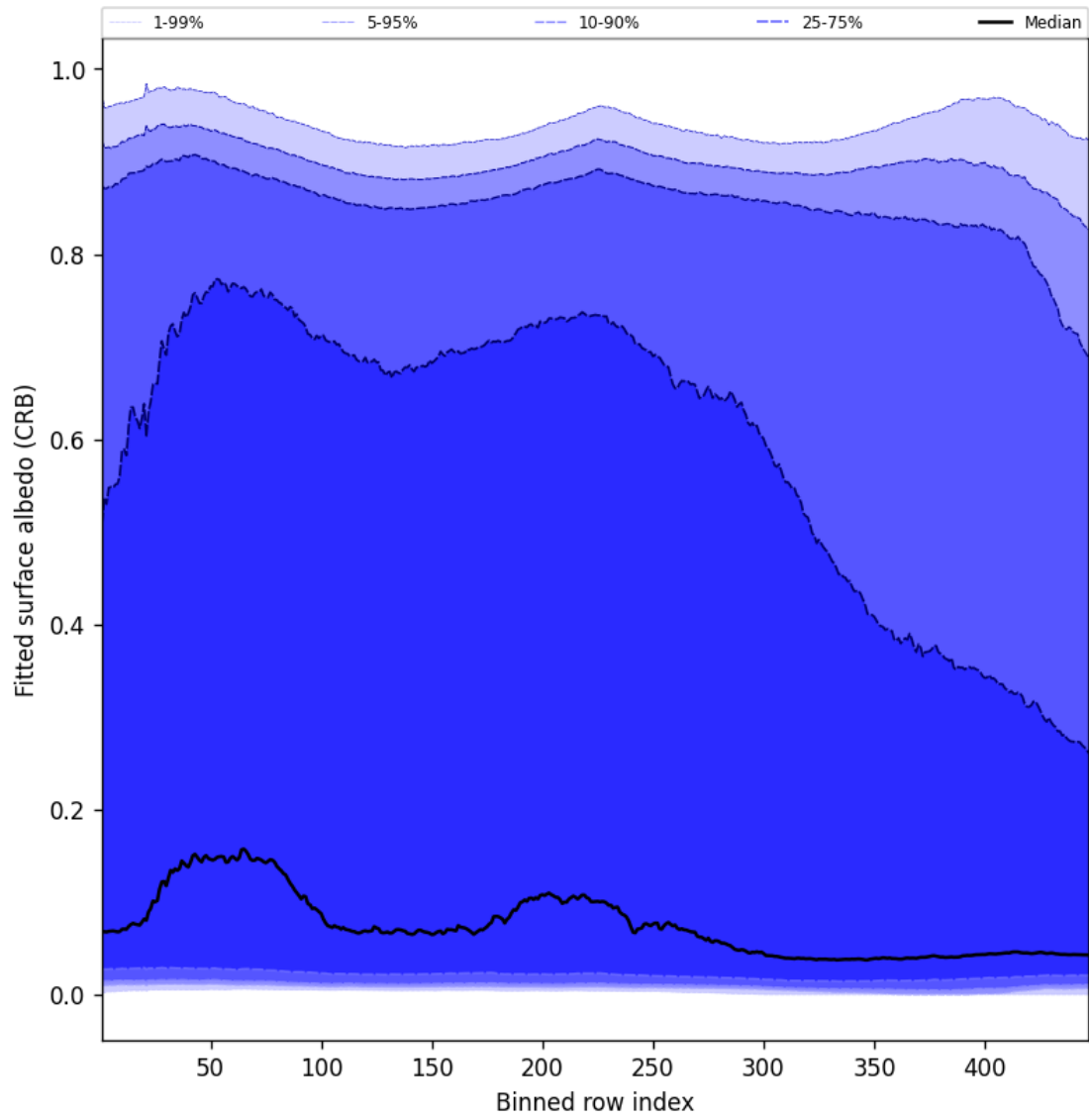
Figure 60: Along track statistics of “Fitted surface albedo (CRB)” for 2025-12-02 to 2025-12-02
