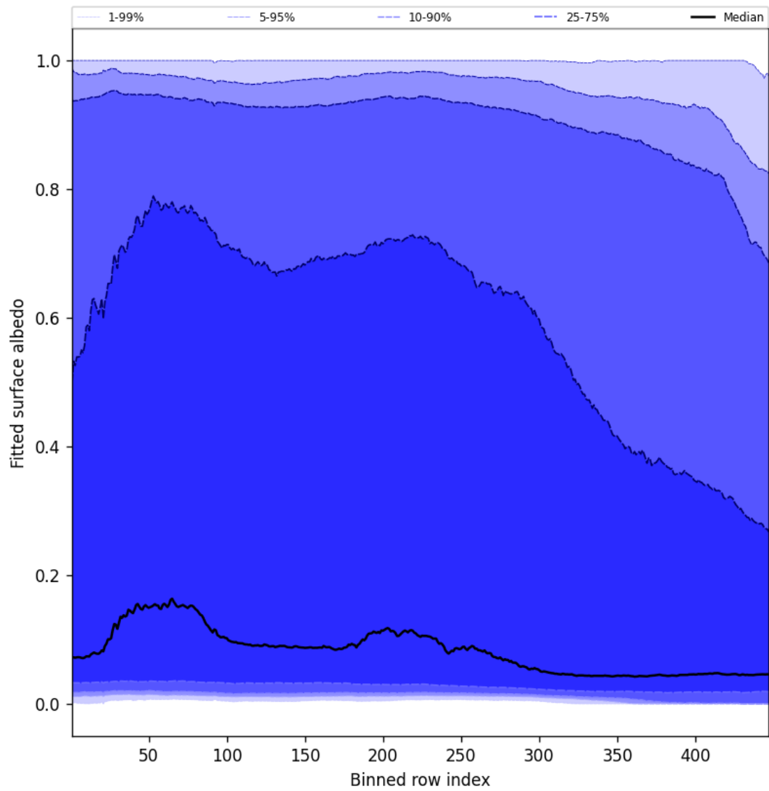
Figure 59: Along track statistics of “Fitted surface albedo” for 2025-12-02 to 2025-12-02
