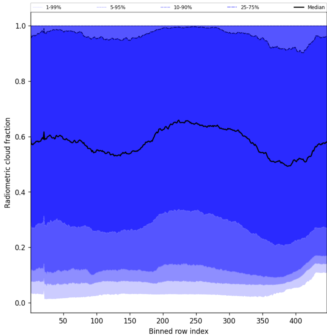
Figure 53: Along track statistics of “Radiometric cloud fraction” for 2025-12-02 to 2025-12-02
