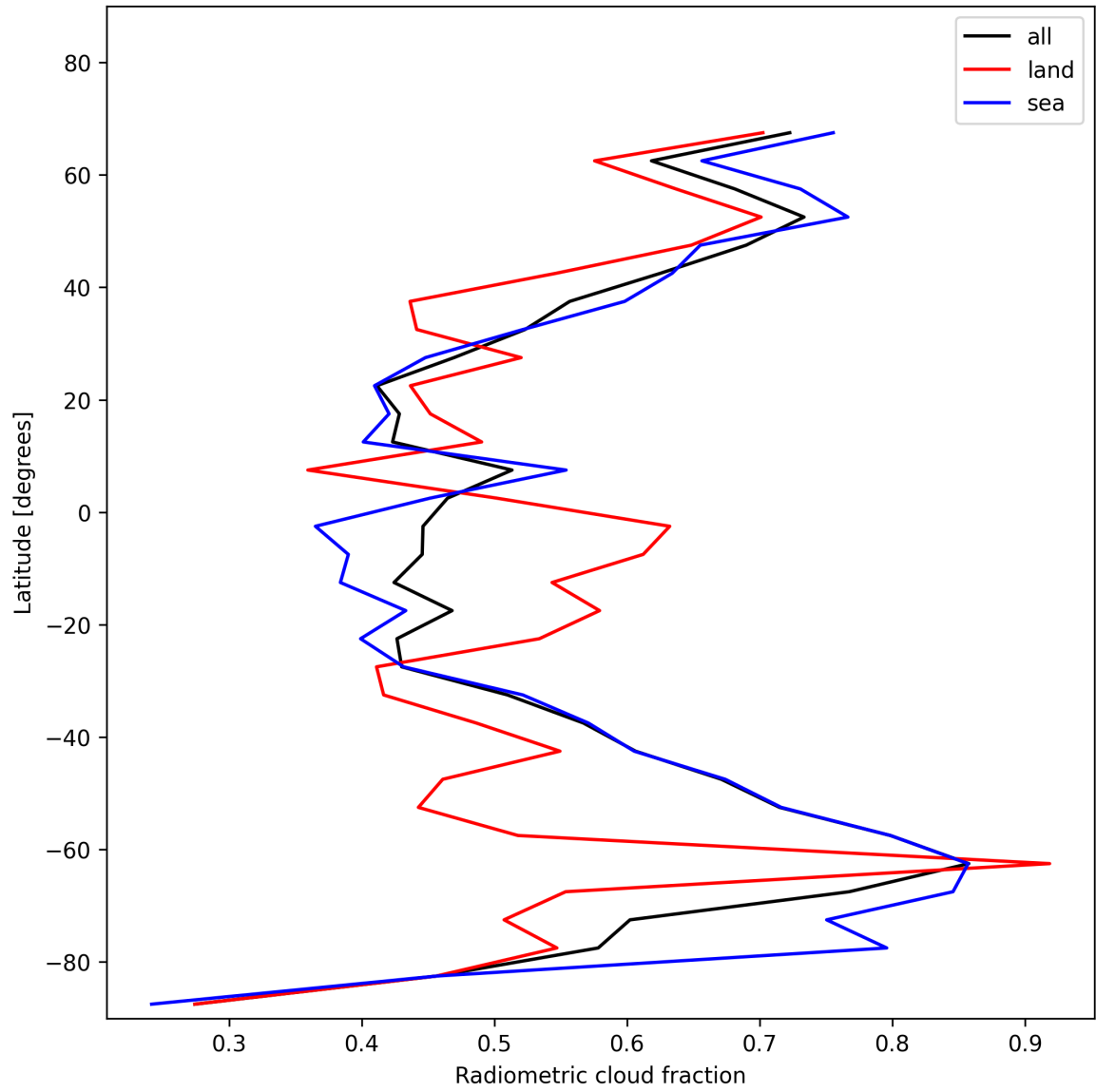
Figure 21: Zonal average of “Radiometric cloud fraction” for 2025-12-02 to 2025-12-02.
