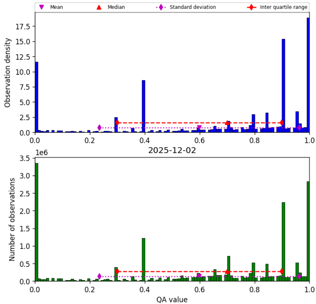
Figure 36: Histogram of “QA value” for 2025-12-02 to 2025-12-02
