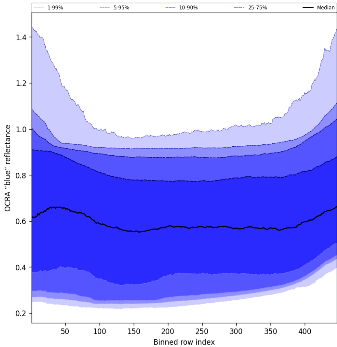
Figure 65: Along track statistics of “OCRA “blue” reflectance” for 2025-12-02 to 2025-12-02
