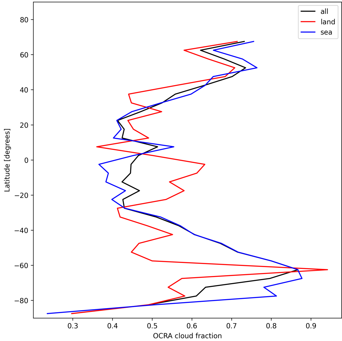
Figure 32: Zonal average of “OCRA cloud fraction” for 2025-12-02 to 2025-12-02.
