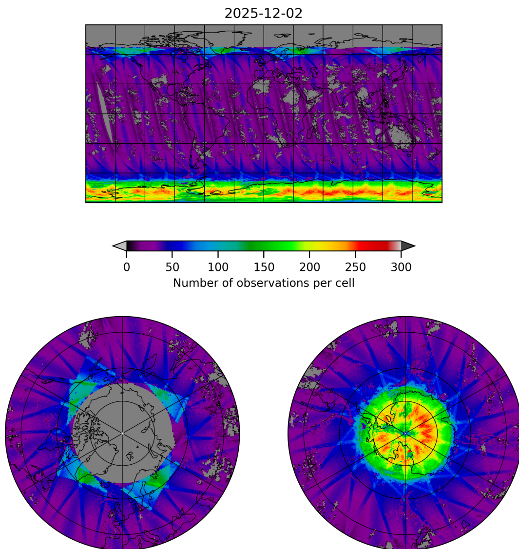
Figure 19: Map of the number of observations for 2025-12-02 to 2025-12-02
