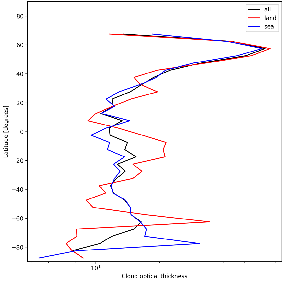
Figure 23: Zonal average of “Cloud optical thickness” for 2025-12-02 to 2025-12-02.
