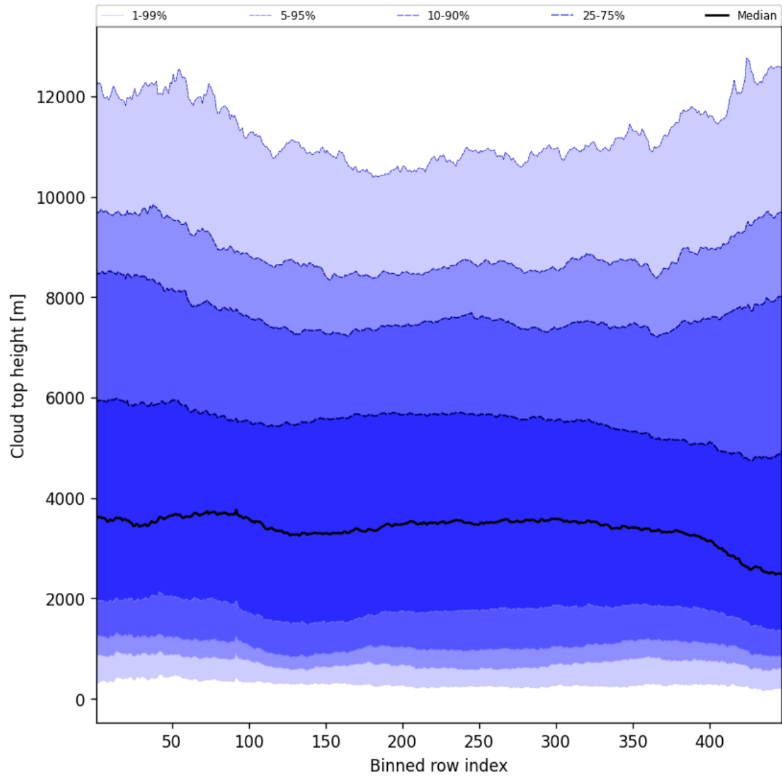
Figure 54: Along track statistics of “Cloud top height” for 2025-12-02 to 2025-12-02
