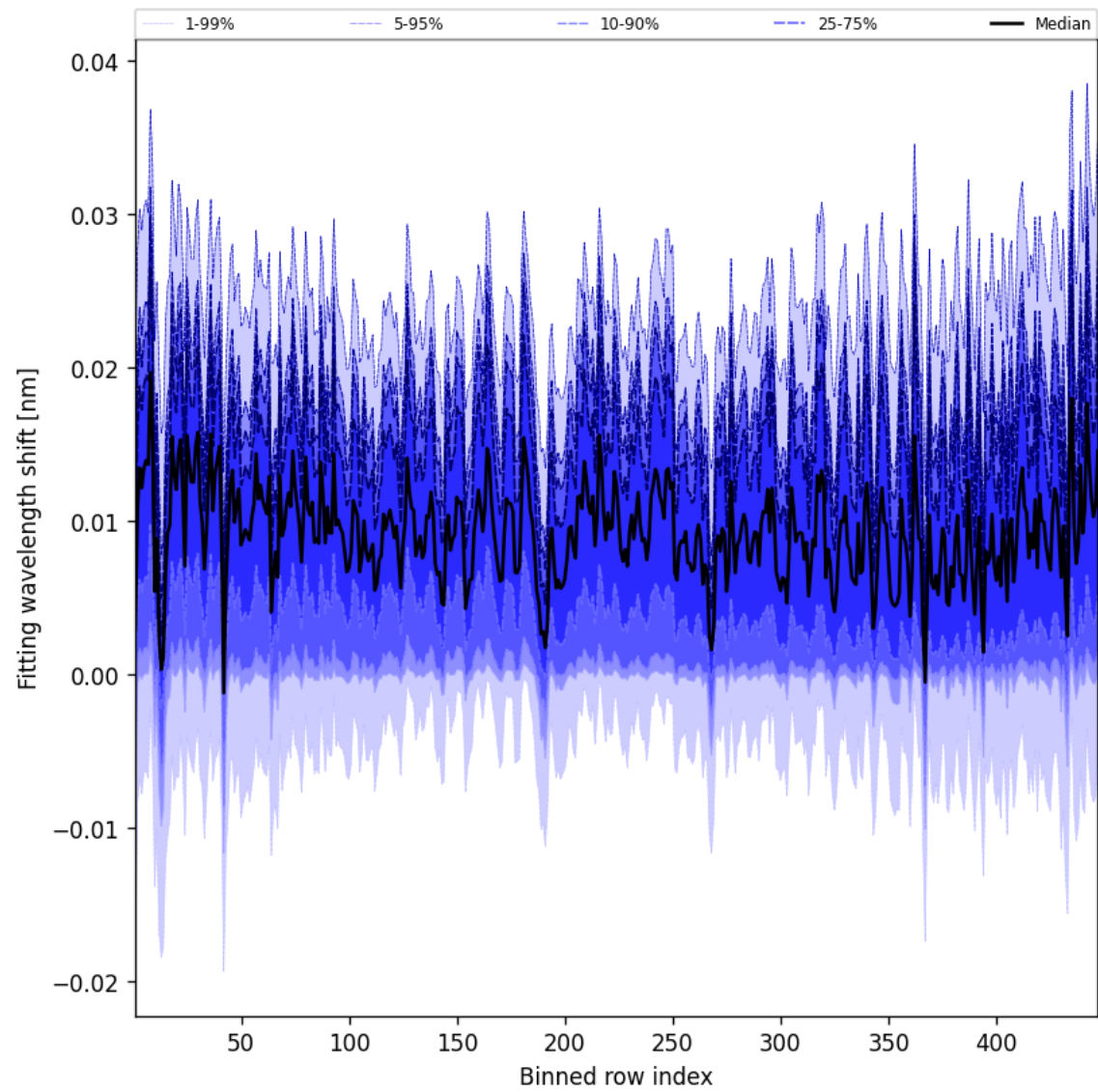
Figure 63: Along track statistics of “Fitting wavelength shift” for 2025-12-02 to 2025-12-02
