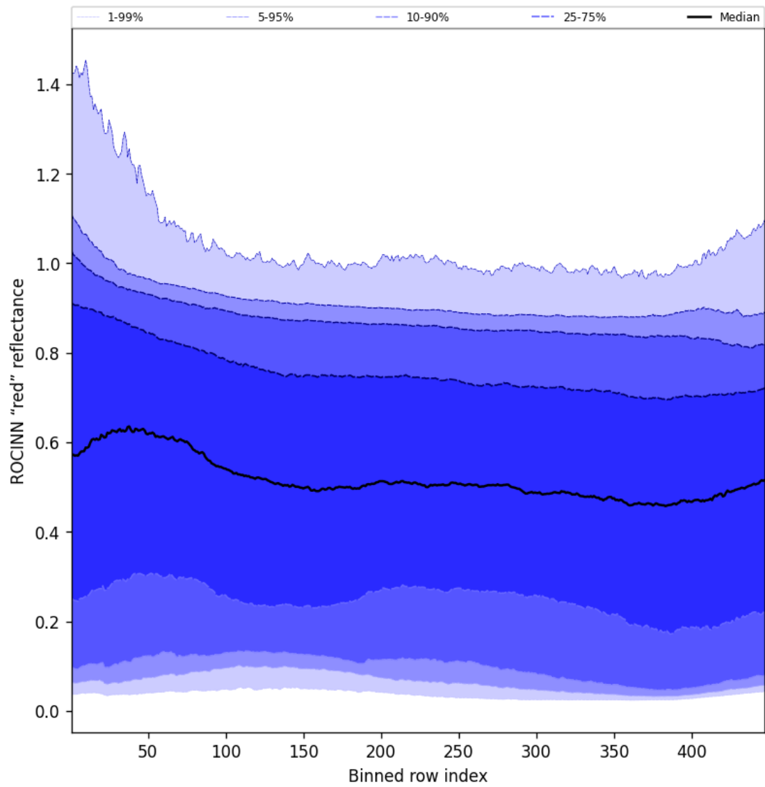
Figure 67: Along track statistics of "ROCINN "red" reflectance" for 2025-12-02 to 2025-12-02
