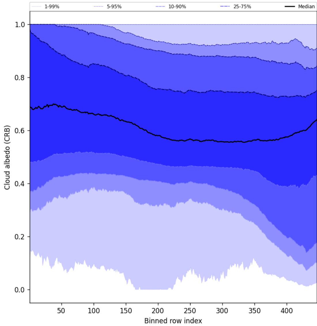
Figure 58: Along track statistics of “Cloud albedo (CRB)” for 2025-12-02 to 2025-12-02
