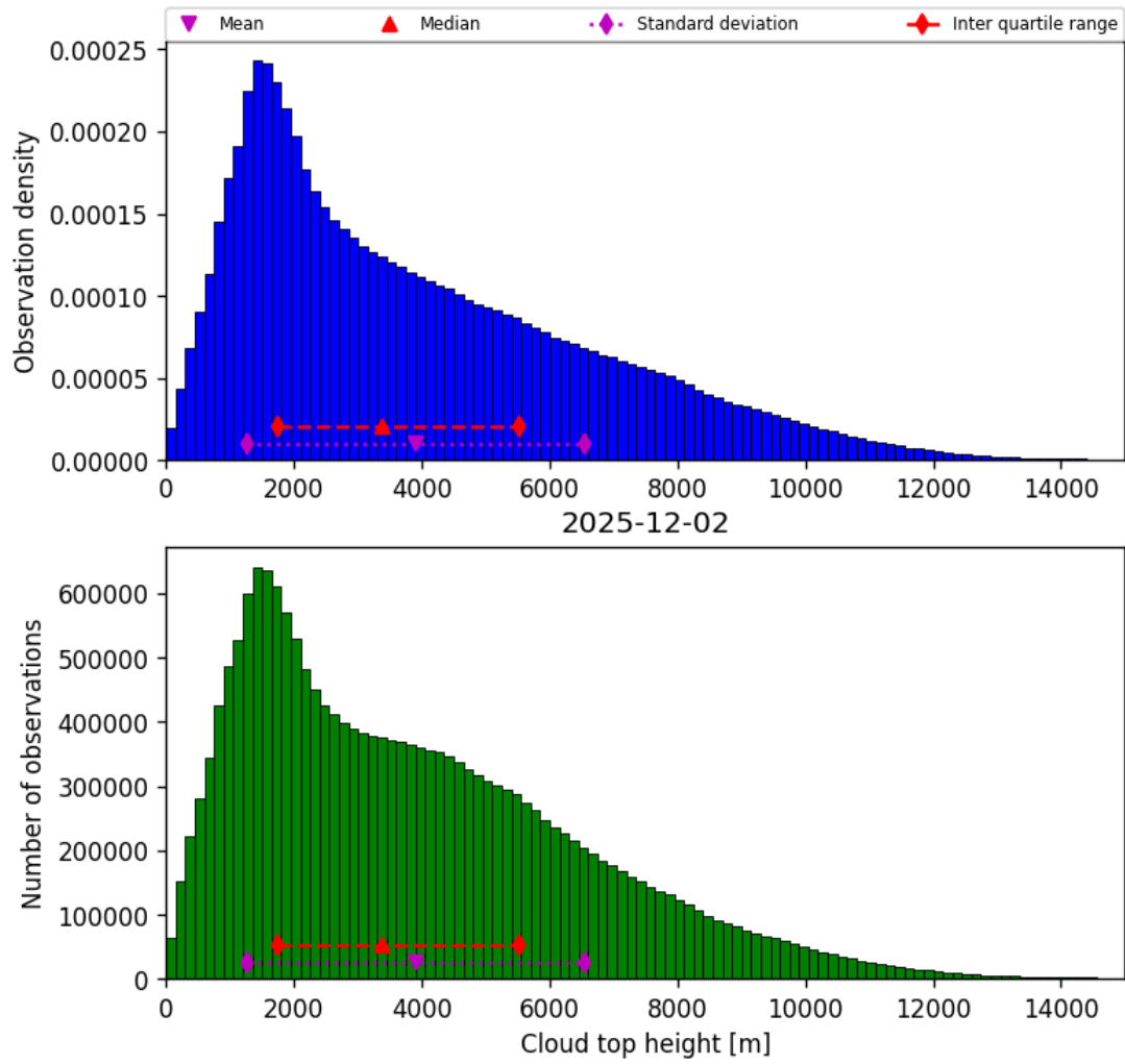
Figure 38: Histogram of “Cloud top height” for 2025-12-02 to 2025-12-02
