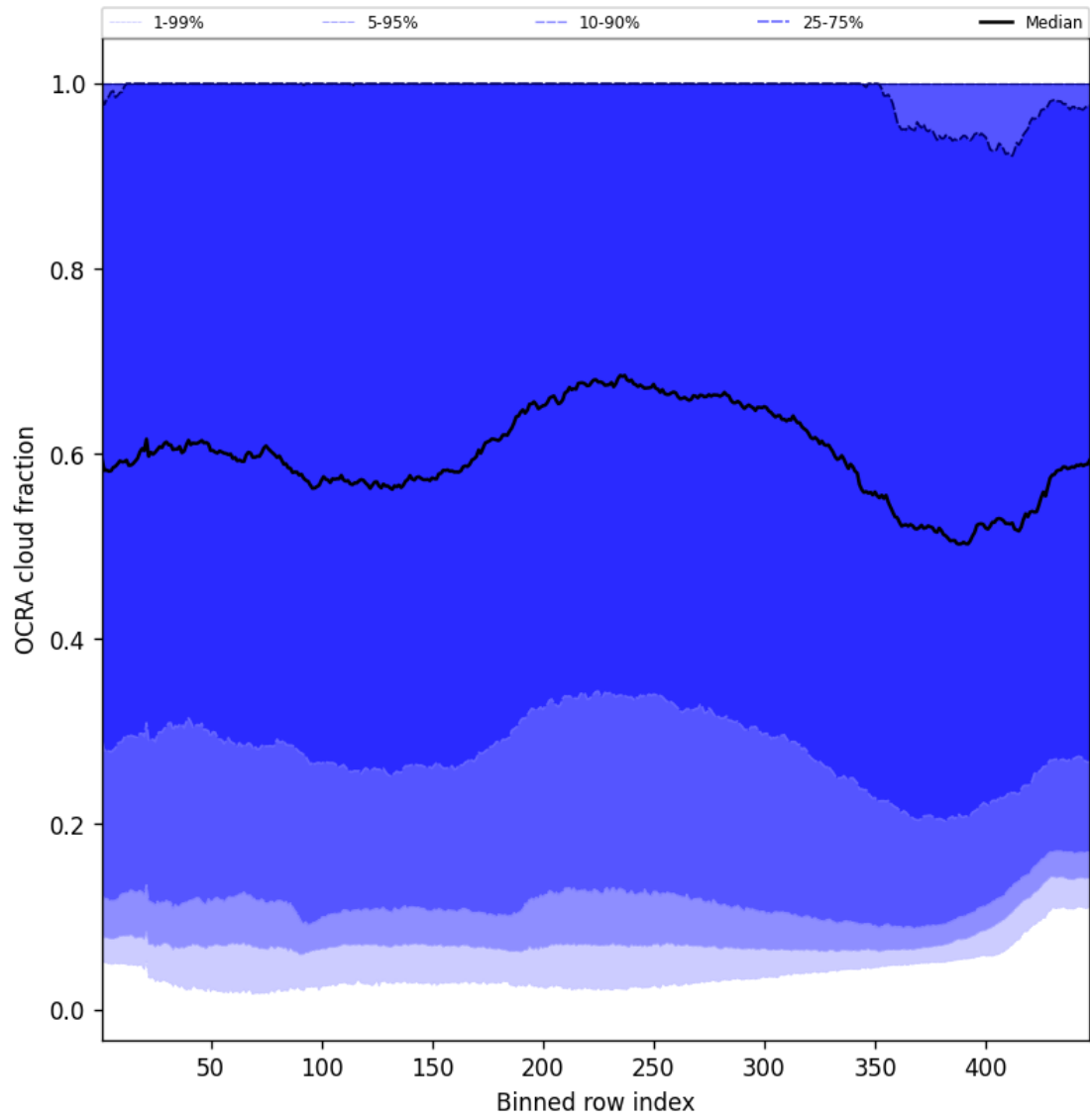
Figure 64: Along track statistics of “OCRA cloud fraction” for 2025-12-02 to 2025-12-02
