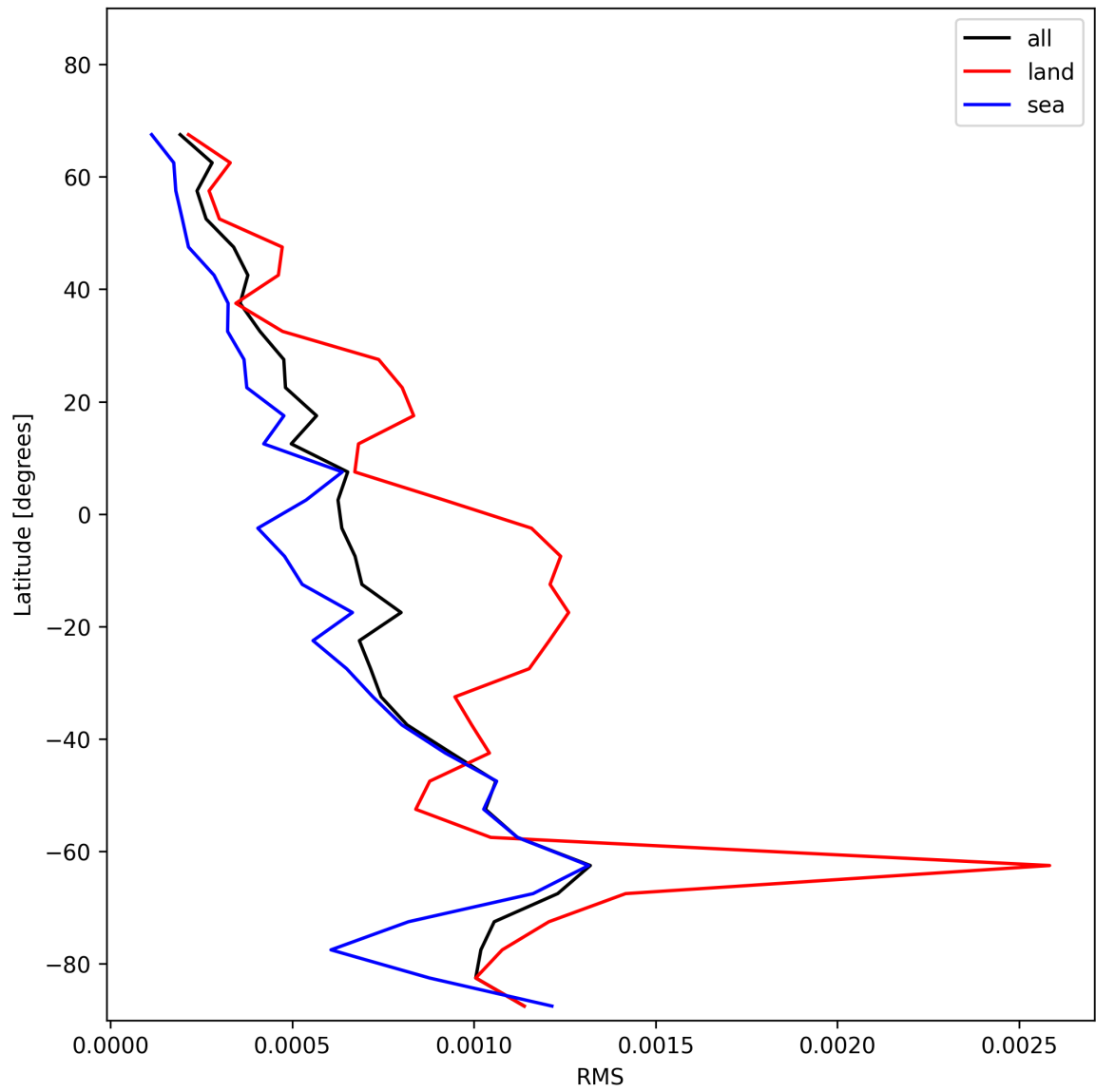
Figure 29: Zonal average of “RMS” for 2025-12-02 to 2025-12-02.
