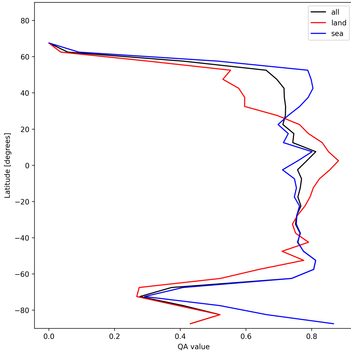
Figure 20: Zonal average of “QA value” for 2025-12-02 to 2025-12-02.
