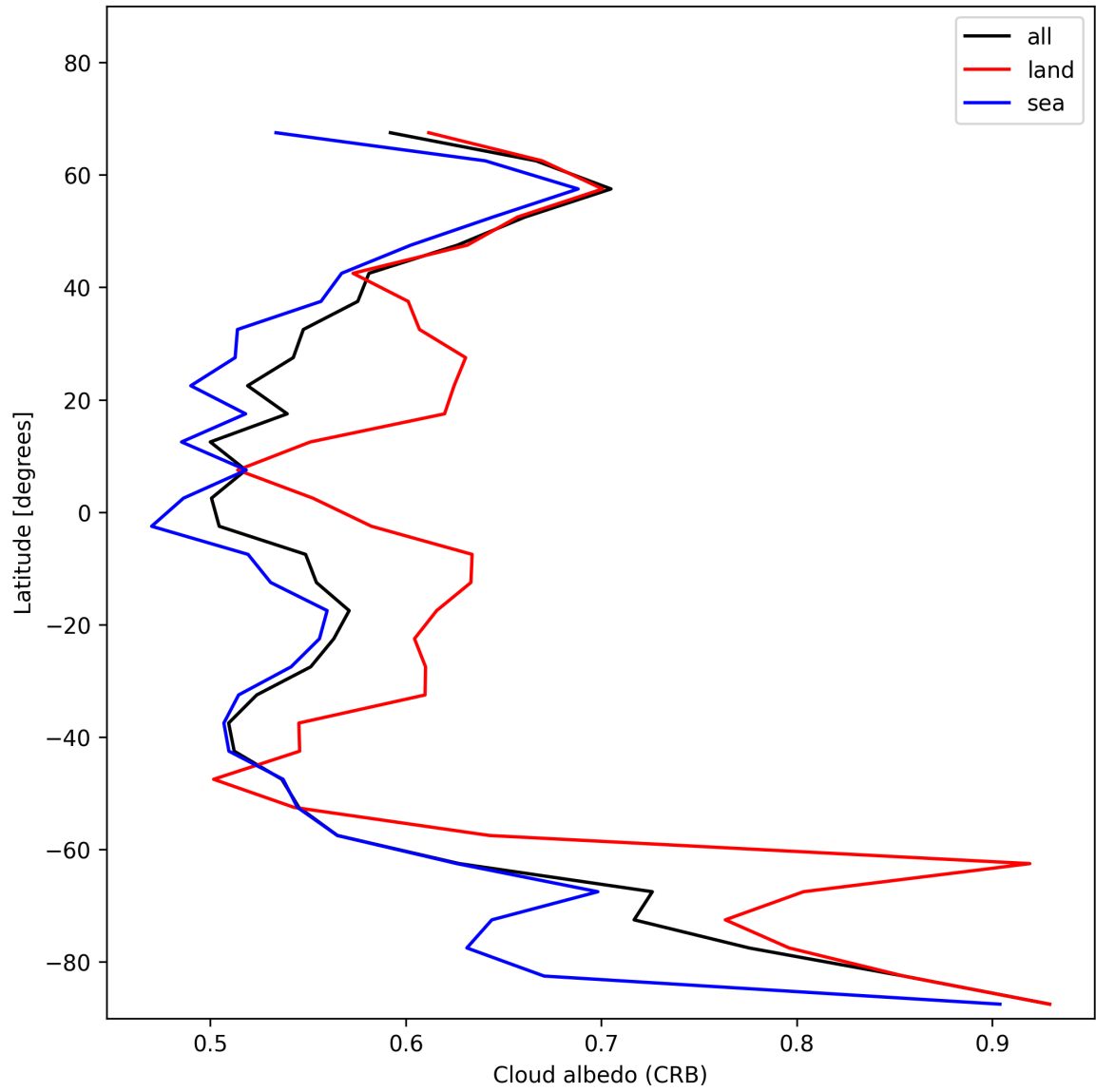
Figure 26: Zonal average of “Cloud albedo (CRB)” for 2025-12-02 to 2025-12-02.
