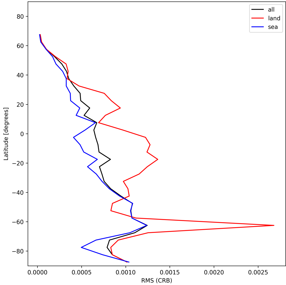
Figure 30: Zonal average of “RMS (CRB)” for 2025-12-02 to 2025-12-02.
