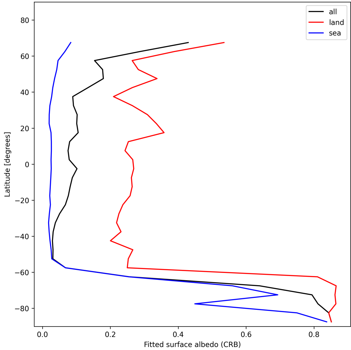
Figure 28: Zonal average of “Fitted surface albedo (CRB)” for 2025-12-02 to 2025-12-02.
