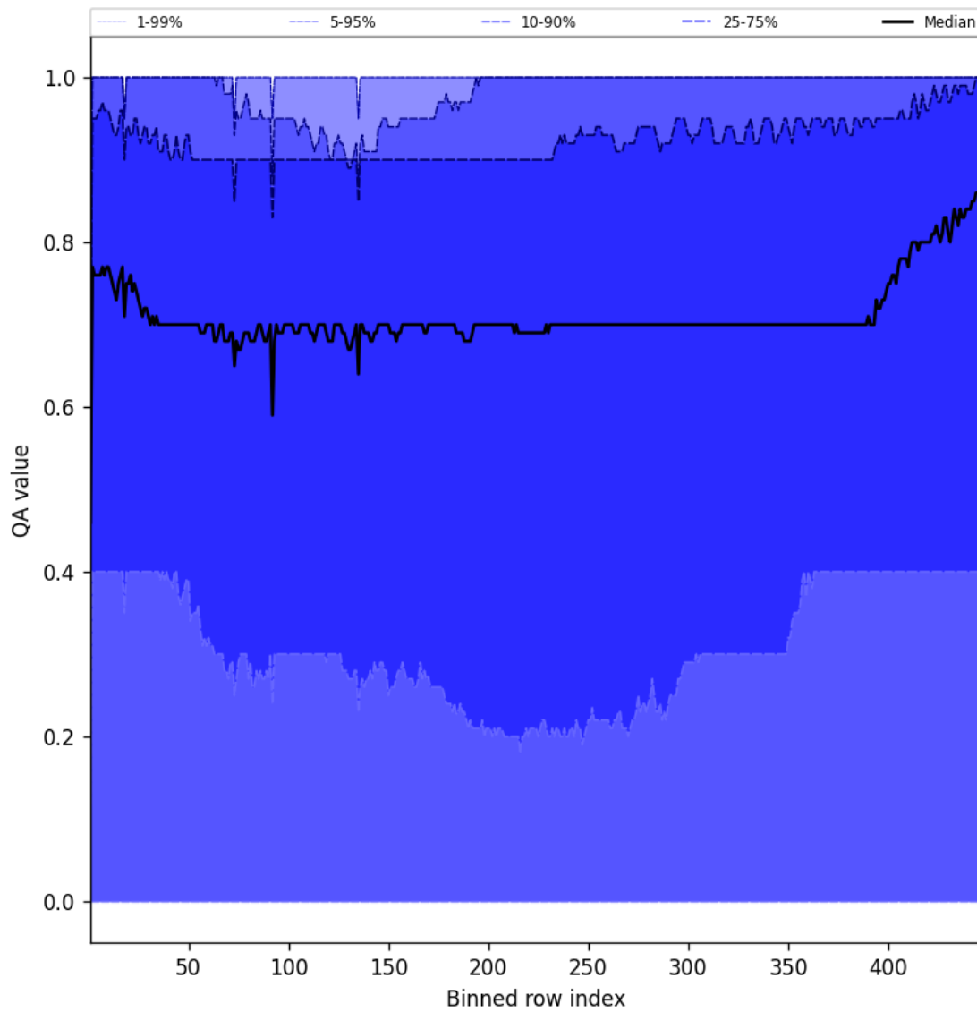
Figure 52: Along track statistics of “QA value” for 2025-12-02 to 2025-12-02
