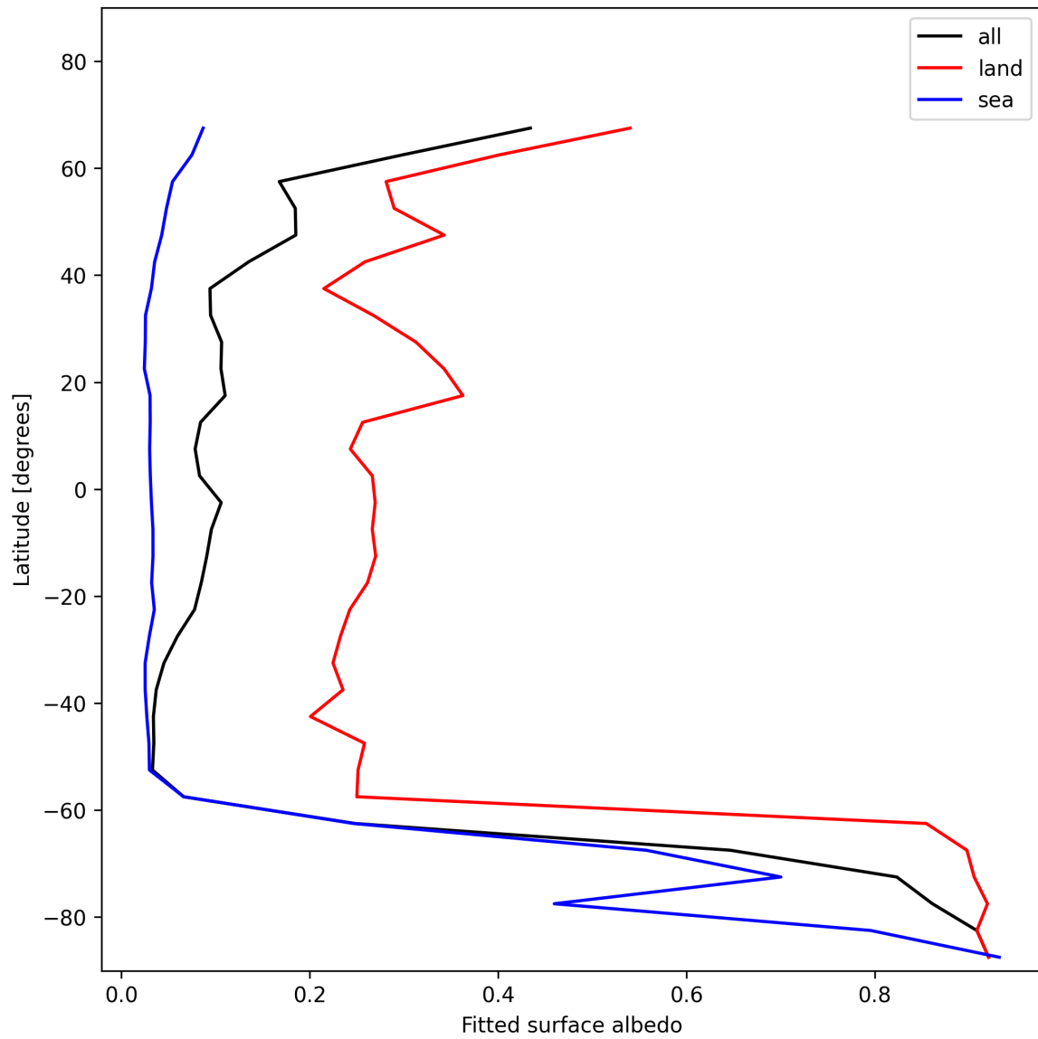
Figure 27: Zonal average of “Fitted surface albedo” for 2025-12-02 to 2025-12-02.
