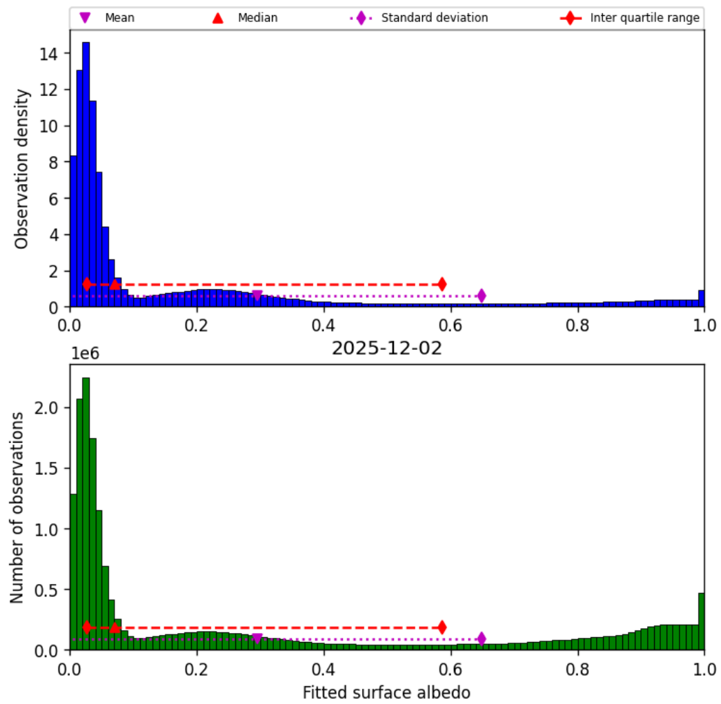
Figure 43: Histogram of “Fitted surface albedo” for 2025-12-02 to 2025-12-02
