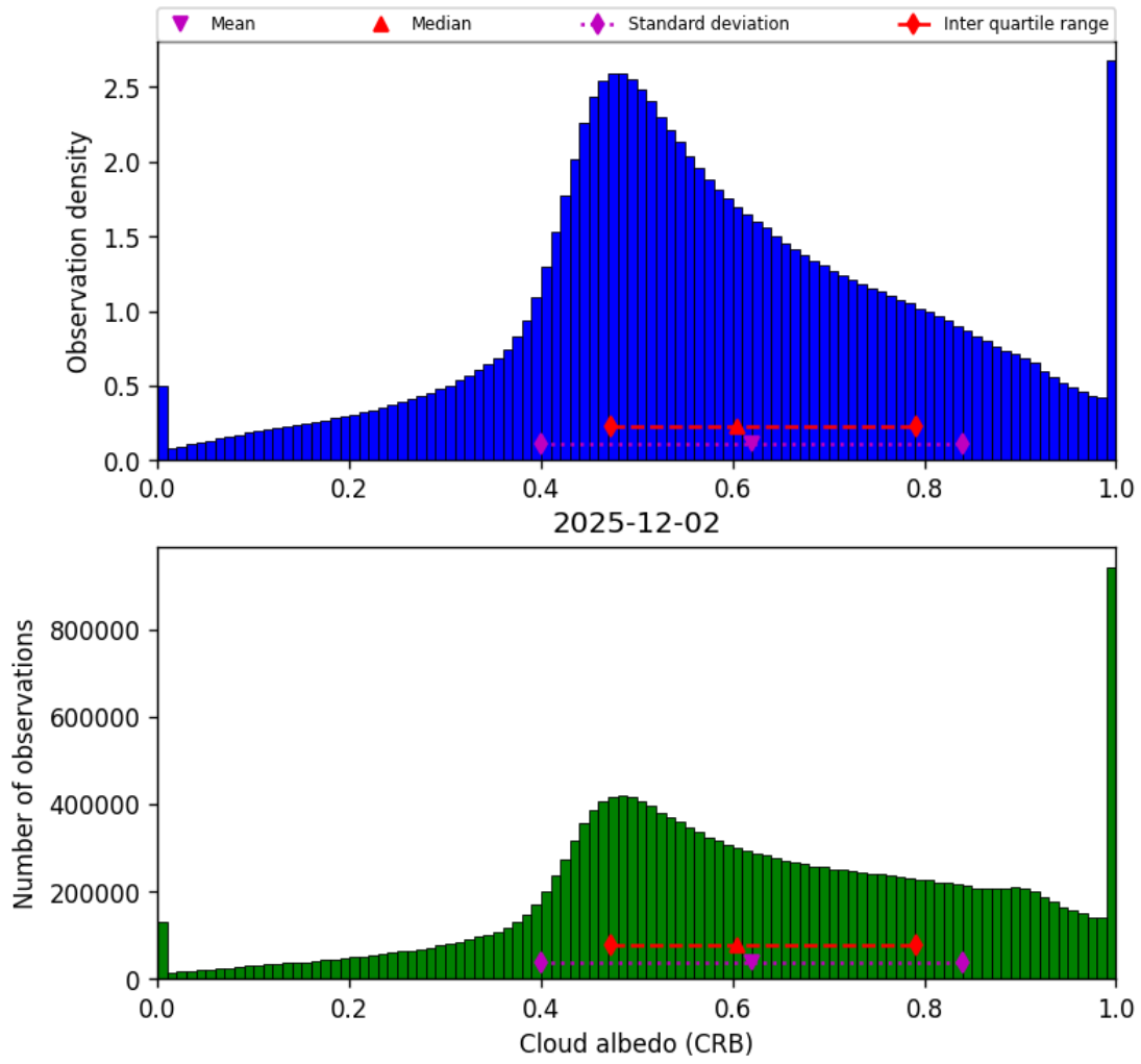
Figure 42: Histogram of “Cloud albedo (CRB)” for 2025-12-02 to 2025-12-02
