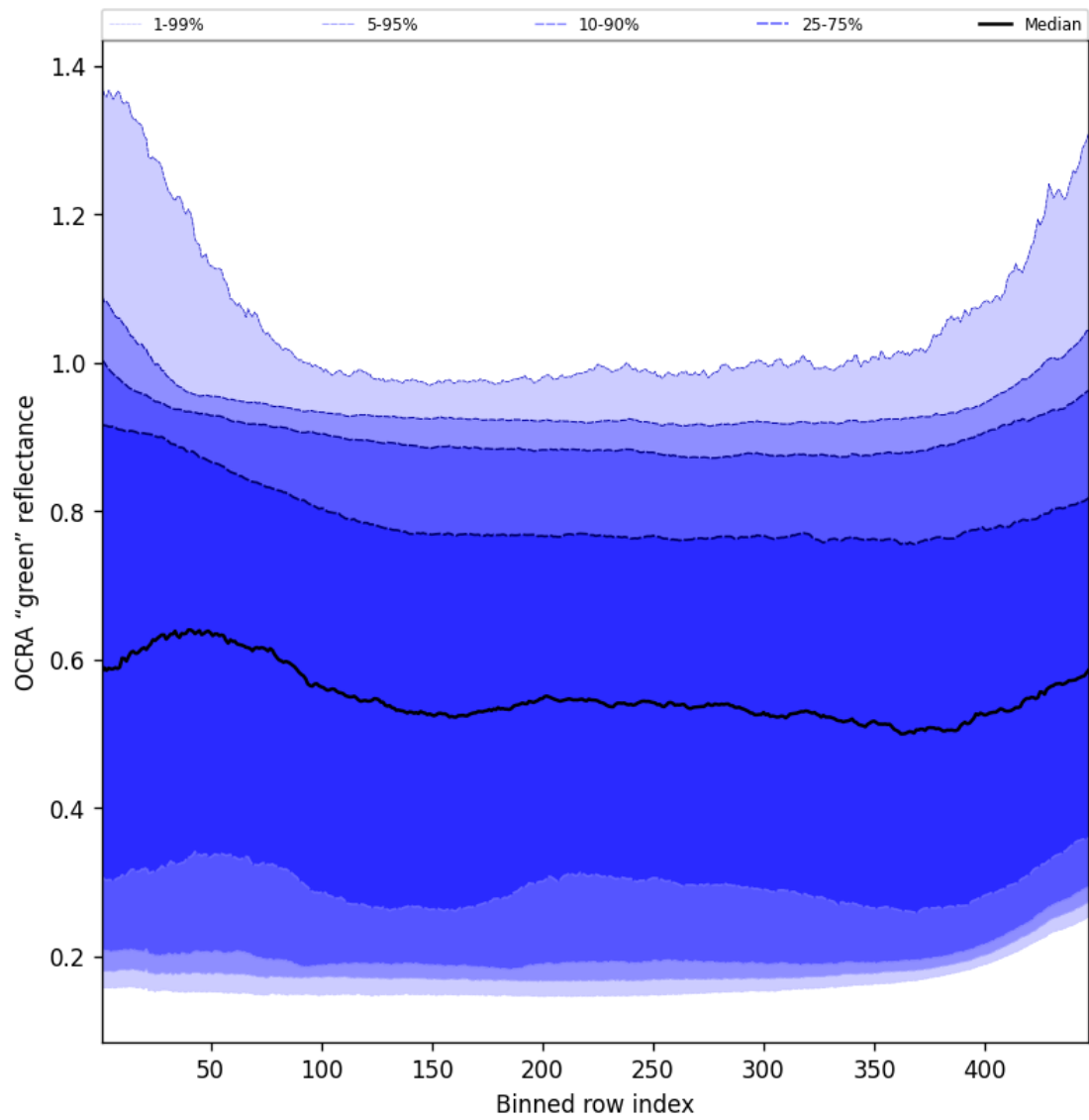
Figure 66: Along track statistics of “OCRA “green” reflectance” for 2025-12-02 to 2025-12-02
