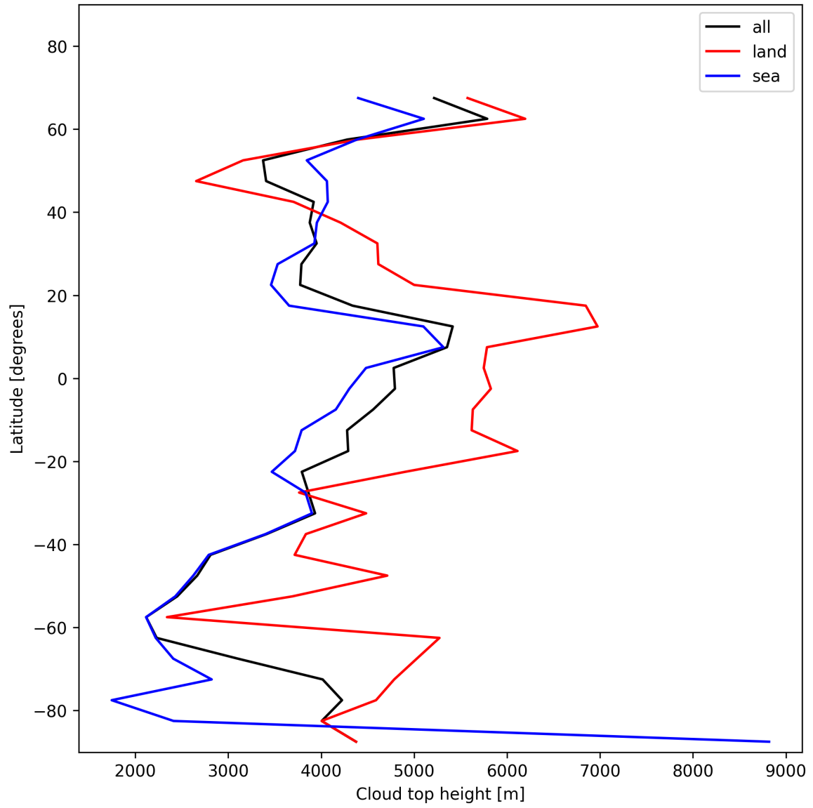
Figure 22: Zonal average of “Cloud top height” for 2025-12-02 to 2025-12-02.
