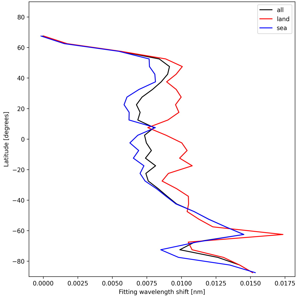
Figure 31: Zonal average of “Fitting wavelength shift” for 2025-12-02 to 2025-12-02.
