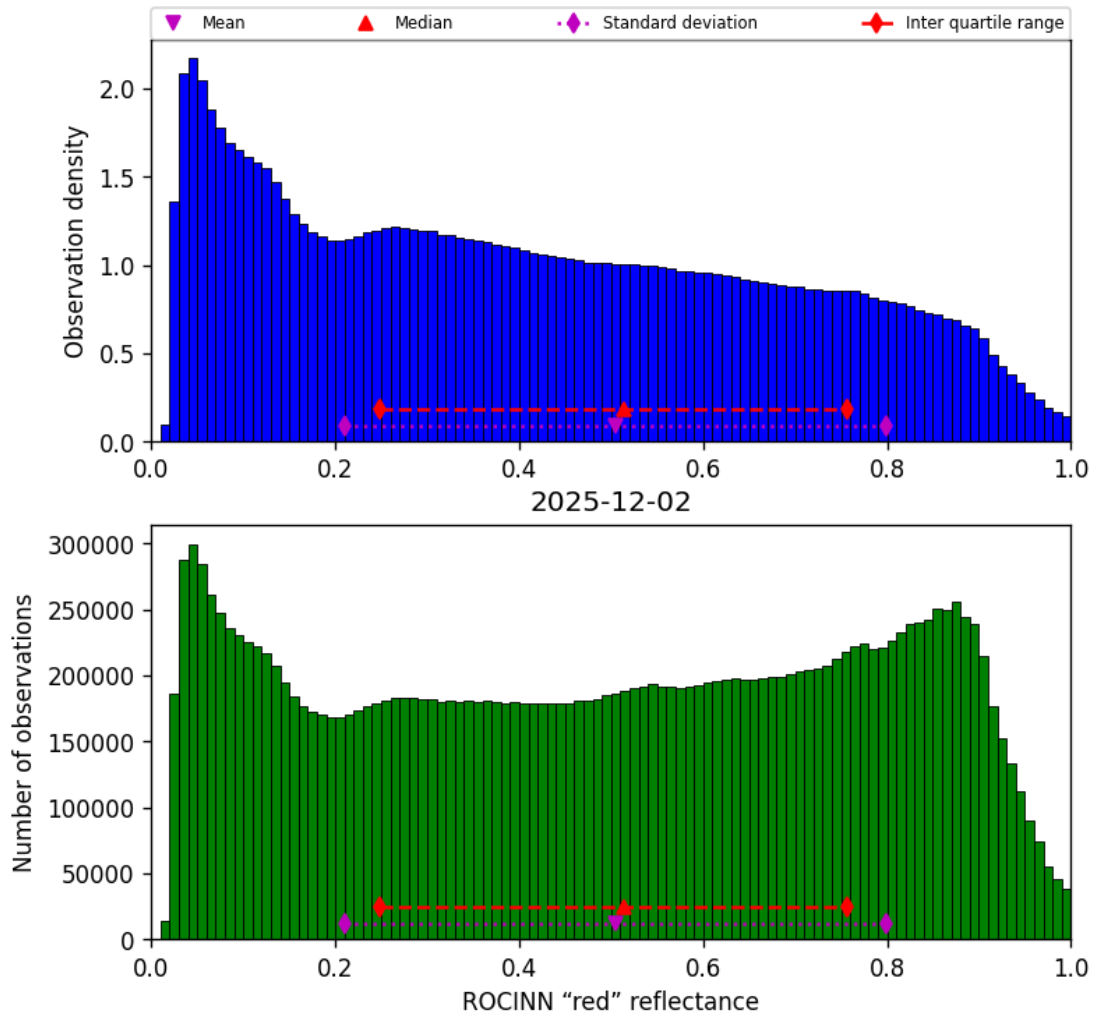
Figure 51: Histogram of “ROCINN “red” reflectance” for 2025-12-02 to 2025-12-02
