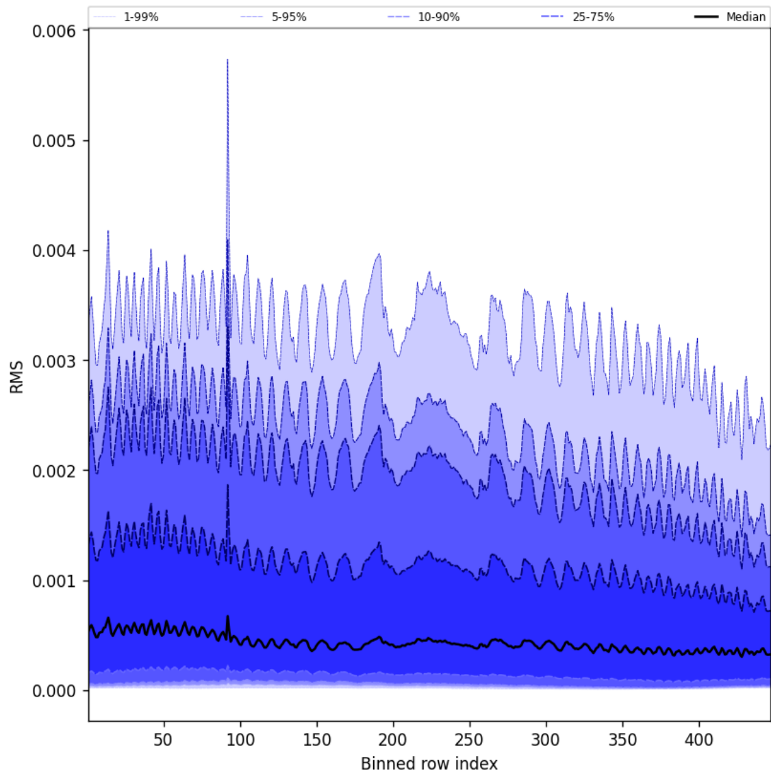
Figure 61: Along track statistics of “RMS” for 2025-12-02 to 2025-12-02
