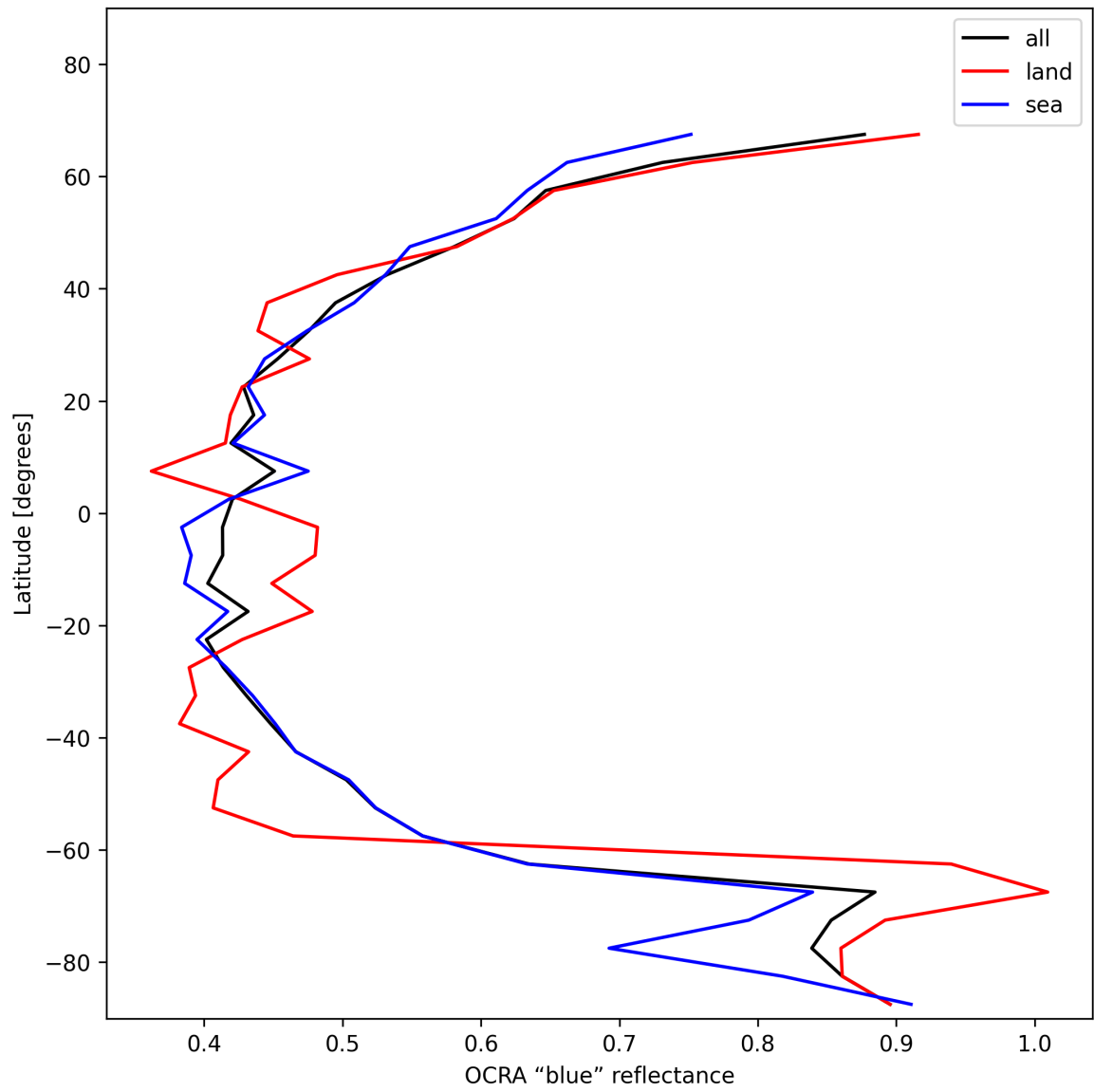
Figure 33: Zonal average of “OCRA “blue” reflectance” for 2025-12-02 to 2025-12-02.
