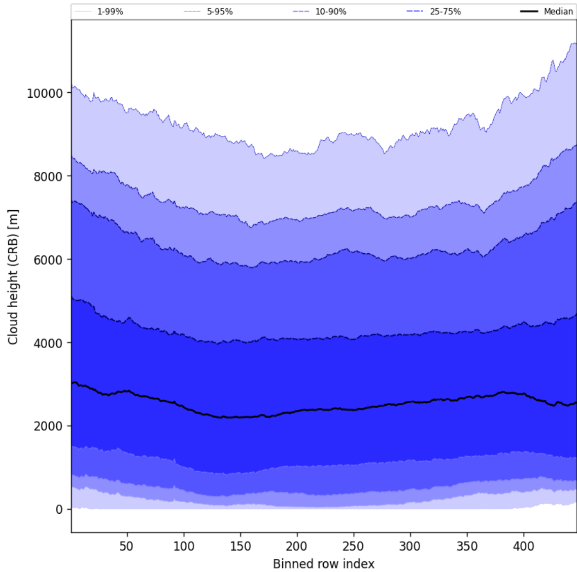
Figure 57: Along track statistics of “Cloud height (CRB)” for 2025-12-02 to 2025-12-02
