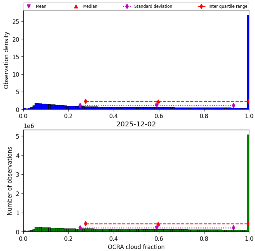
Figure 48: Histogram of “OCRA cloud fraction” for 2025-12-02 to 2025-12-02
