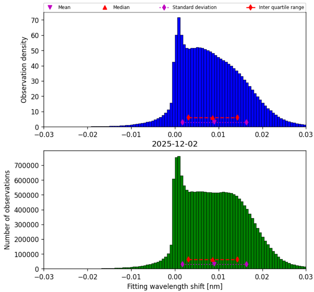
Figure 47: Histogram of “Fitting wavelength shift” for 2025-12-02 to 2025-12-02
