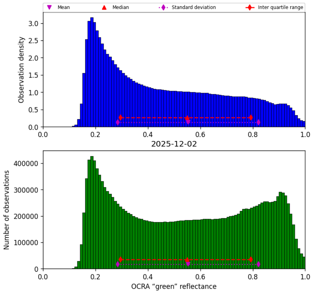
Figure 50: Histogram of “OCRA “green” reflectance” for 2025-12-02 to 2025-12-02
