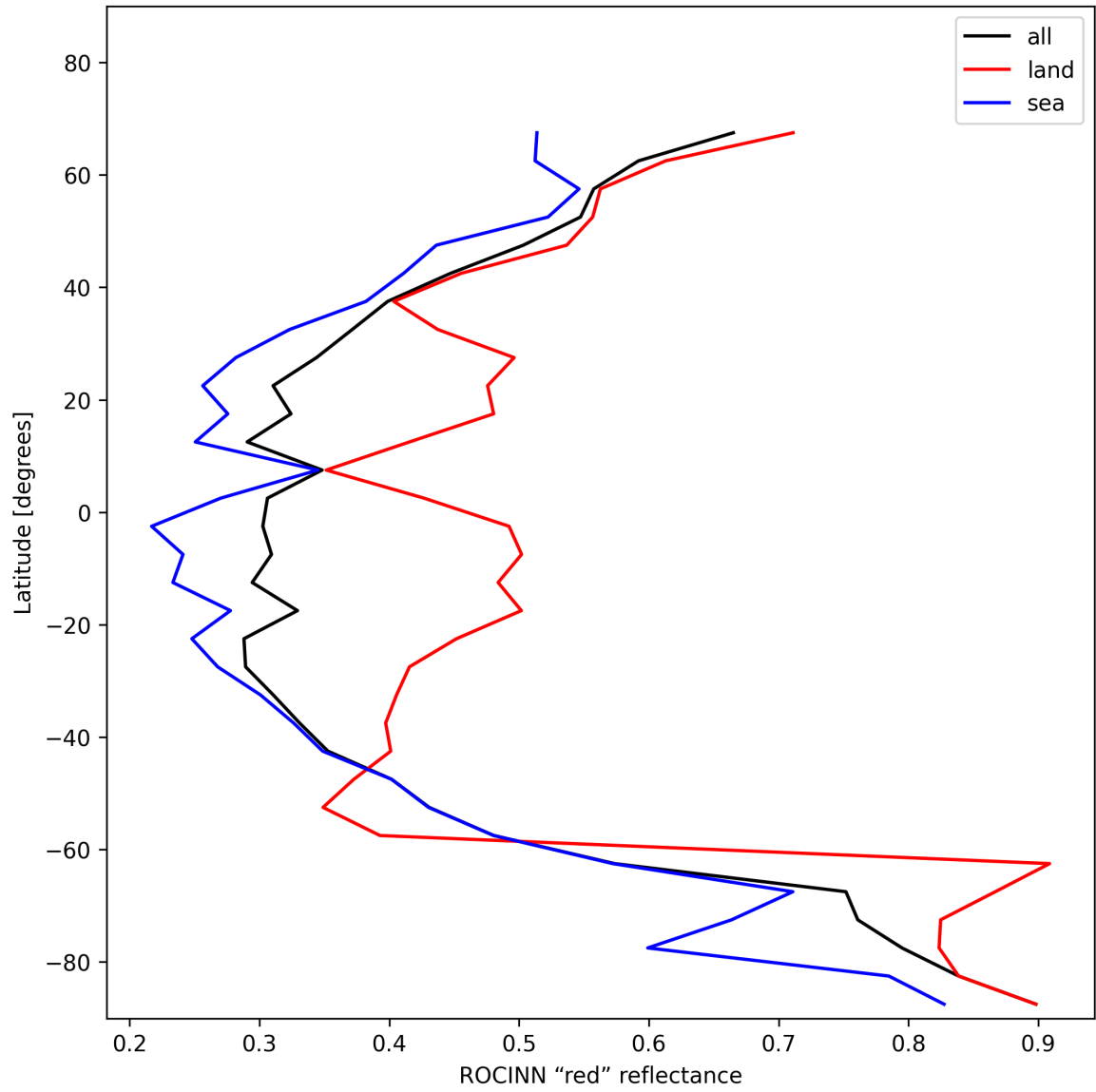
Figure 35: Zonal average of “ROCINN “red” reflectance” for 2025-12-02 to 2025-12-02.
