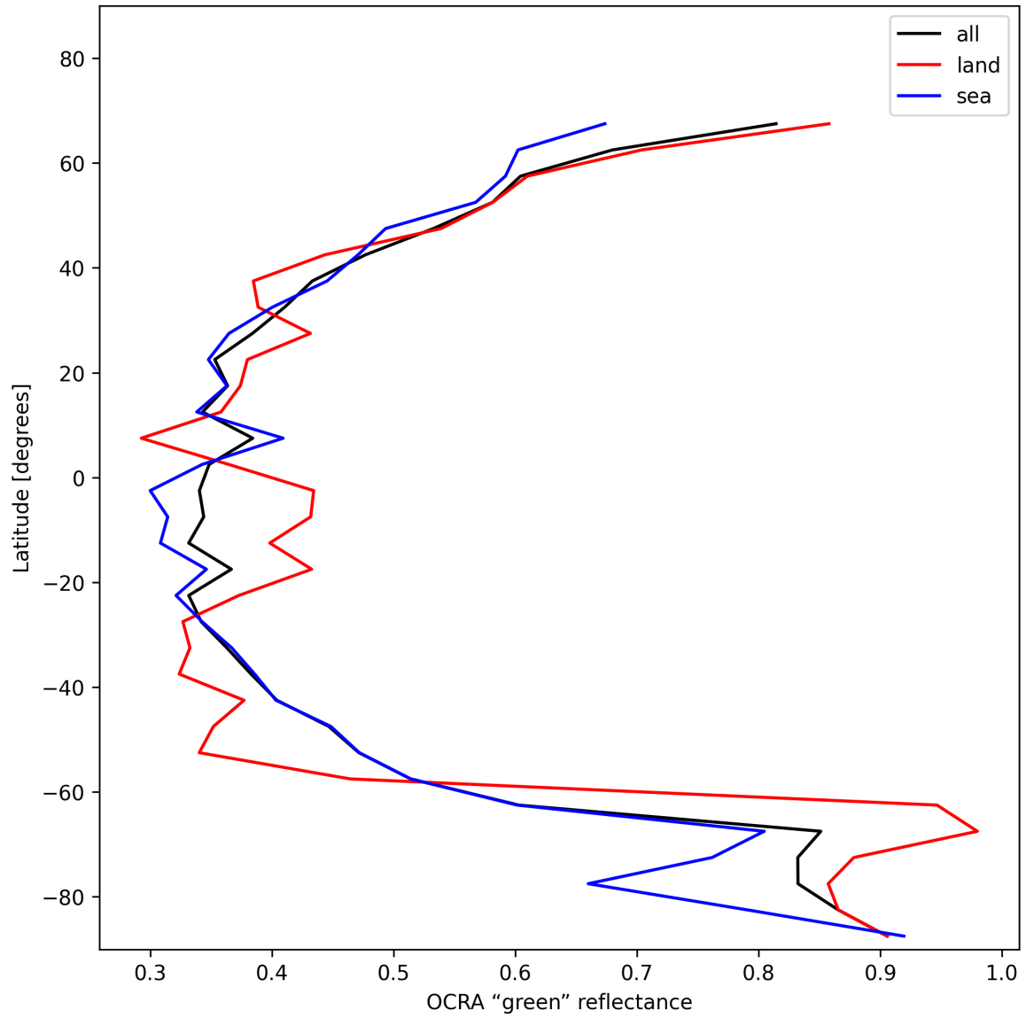
Figure 34: Zonal average of “OCRA “green” reflectance” for 2025-12-02 to 2025-12-02.
