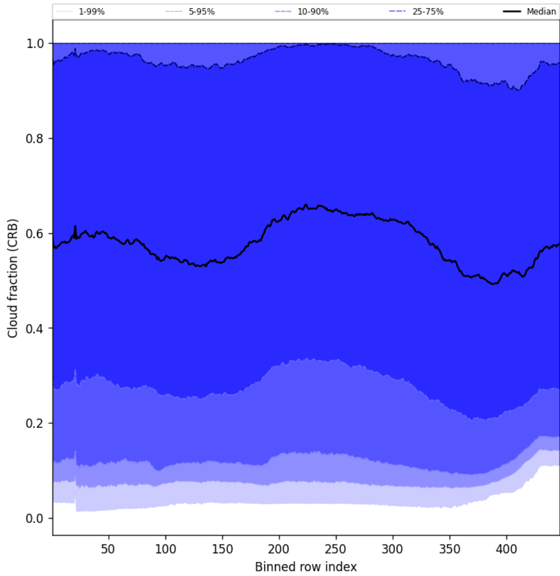
Figure 56: Along track statistics of “Cloud fraction (CRB)” for 2025-12-02 to 2025-12-02
