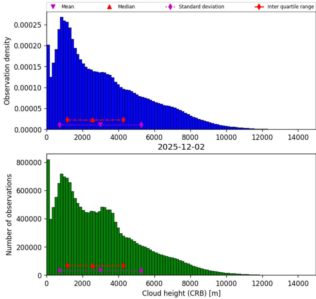
Figure 41: Histogram of “Cloud height (CRB)” for 2025-12-02 to 2025-12-02
