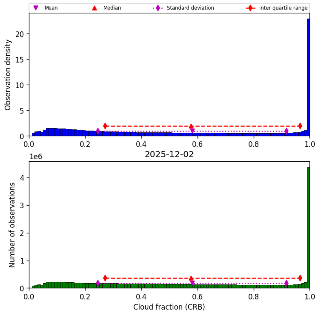
Figure 40: Histogram of “Cloud fraction (CRB)” for 2025-12-02 to 2025-12-02
