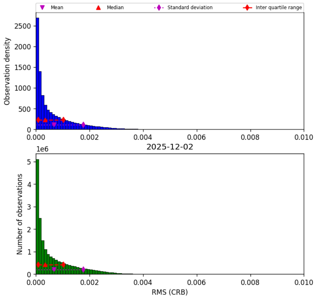
Figure 46: Histogram of “RMS (CRB)” for 2025-12-02 to 2025-12-02
