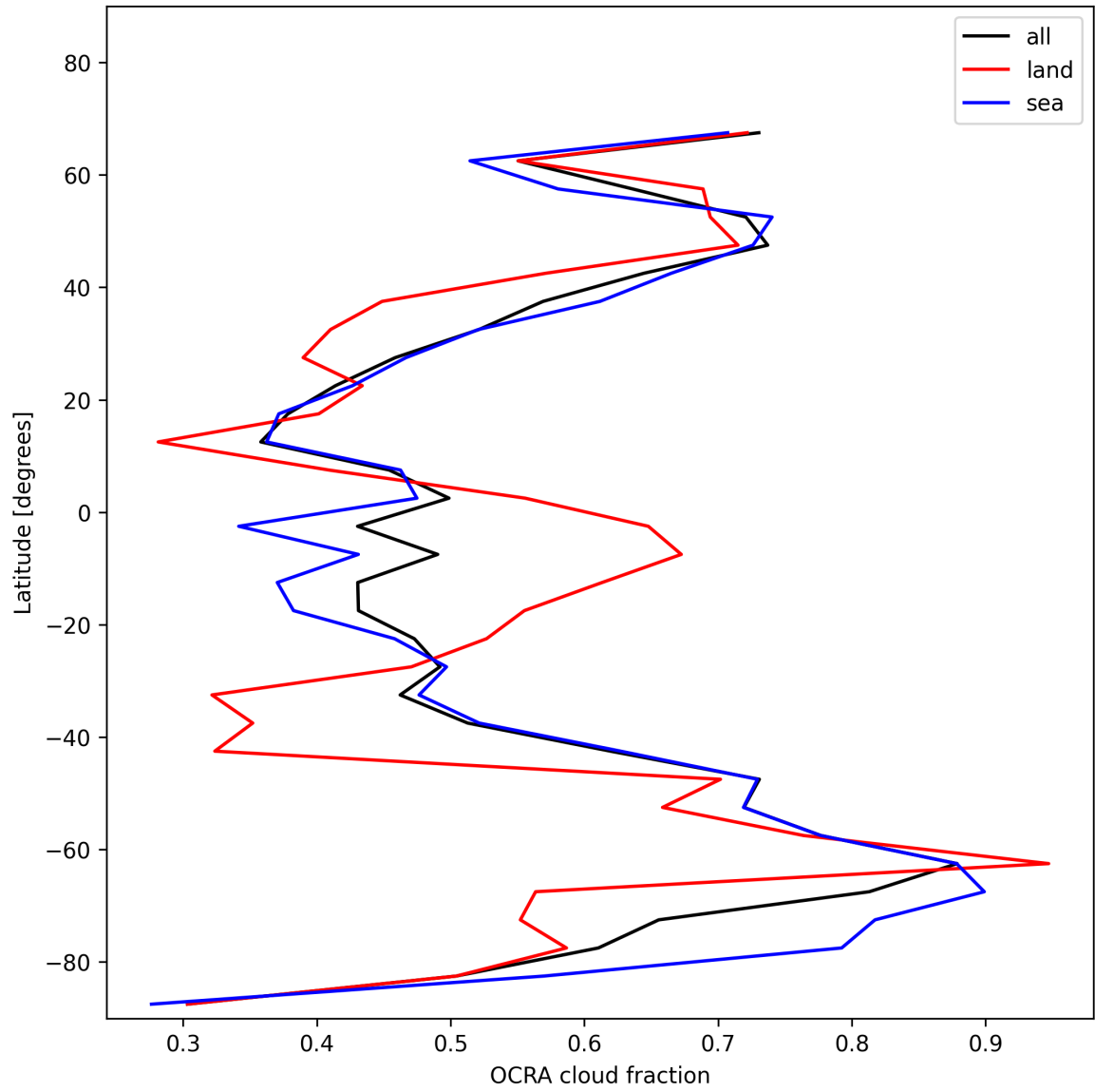
Figure 32: Zonal average of “OCRA cloud fraction” for 2025-12-04 to 2025-12-05.
