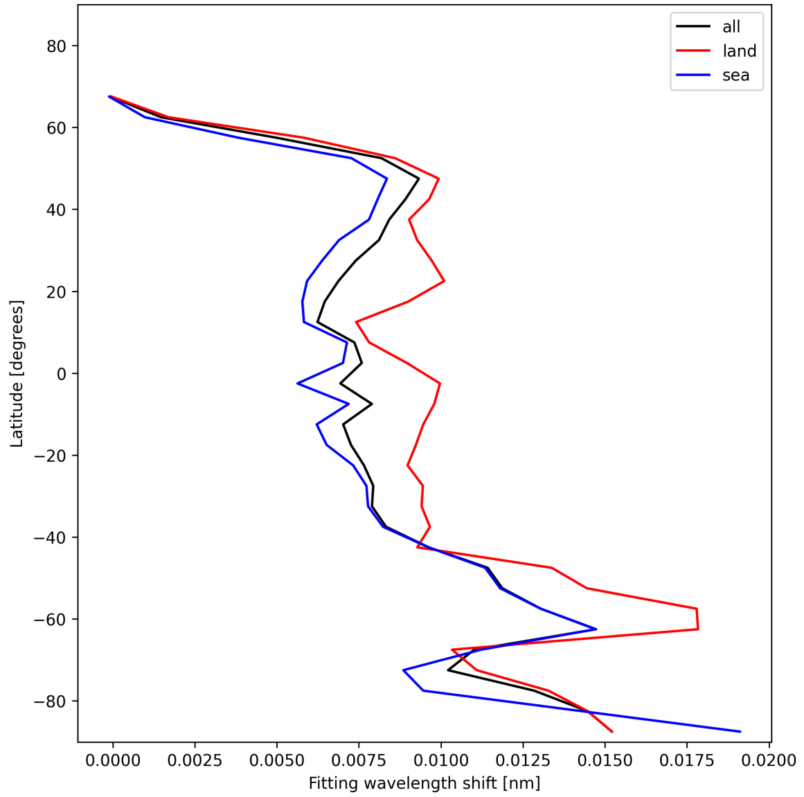
Figure 31: Zonal average of “Fitting wavelength shift” for 2025-12-04 to 2025-12-05.
