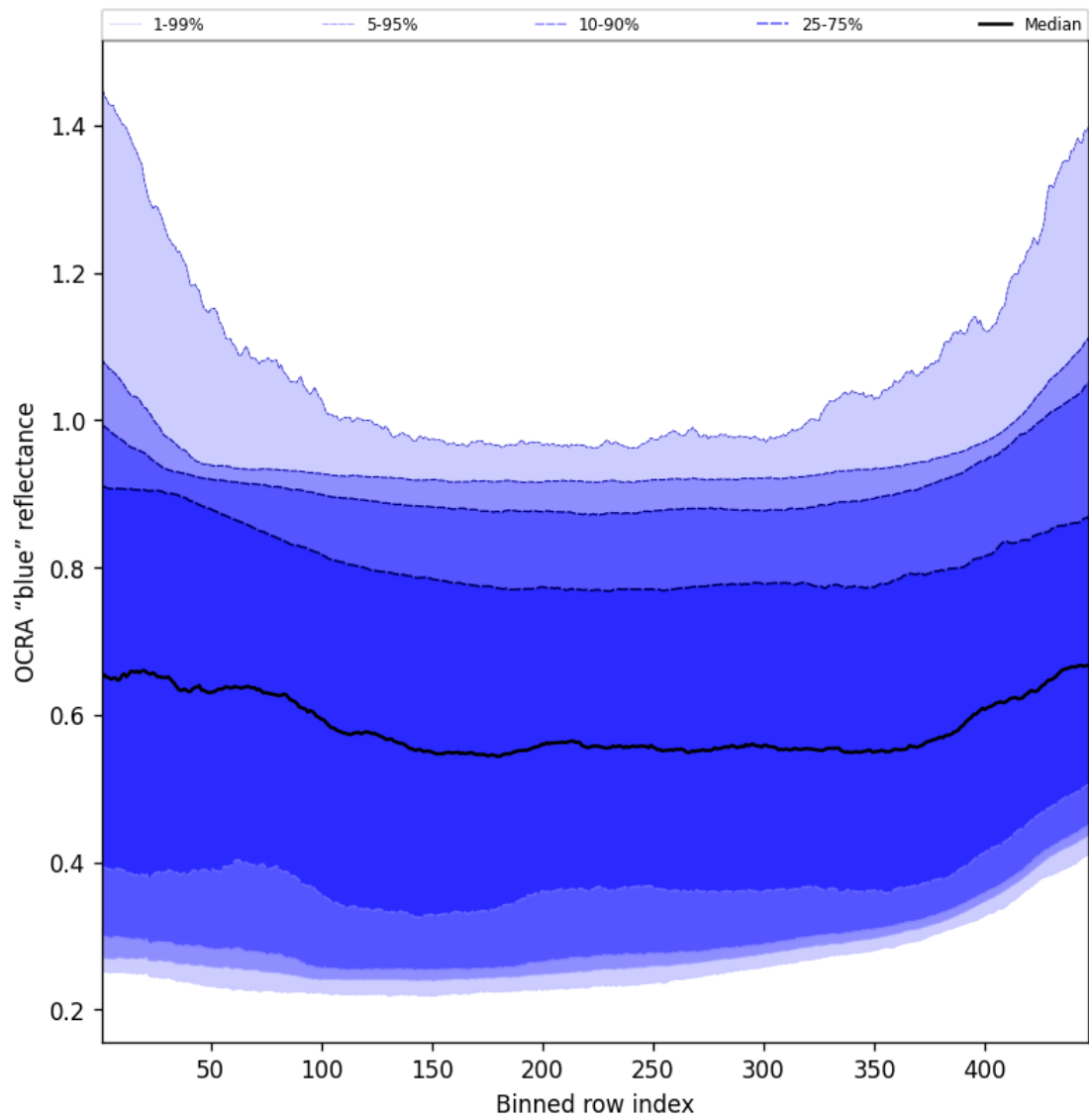
Figure 65: Along track statistics of "OCRA "blue" reflectance" for 2025-12-04 to 2025-12-05
