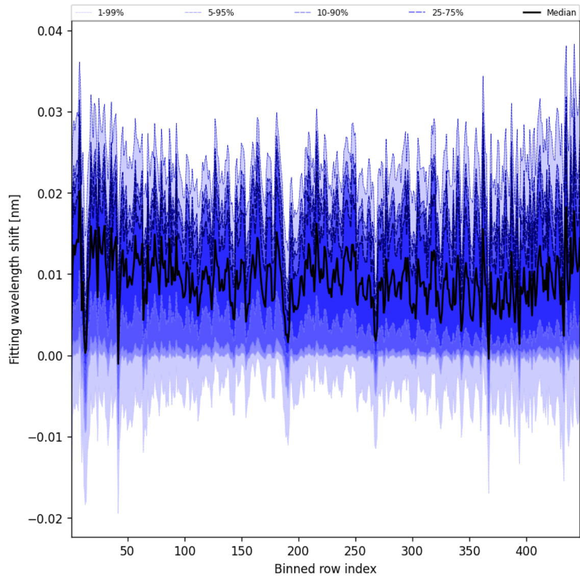
Figure 63: Along track statistics of “Fitting wavelength shift” for 2025-12-04 to 2025-12-05
