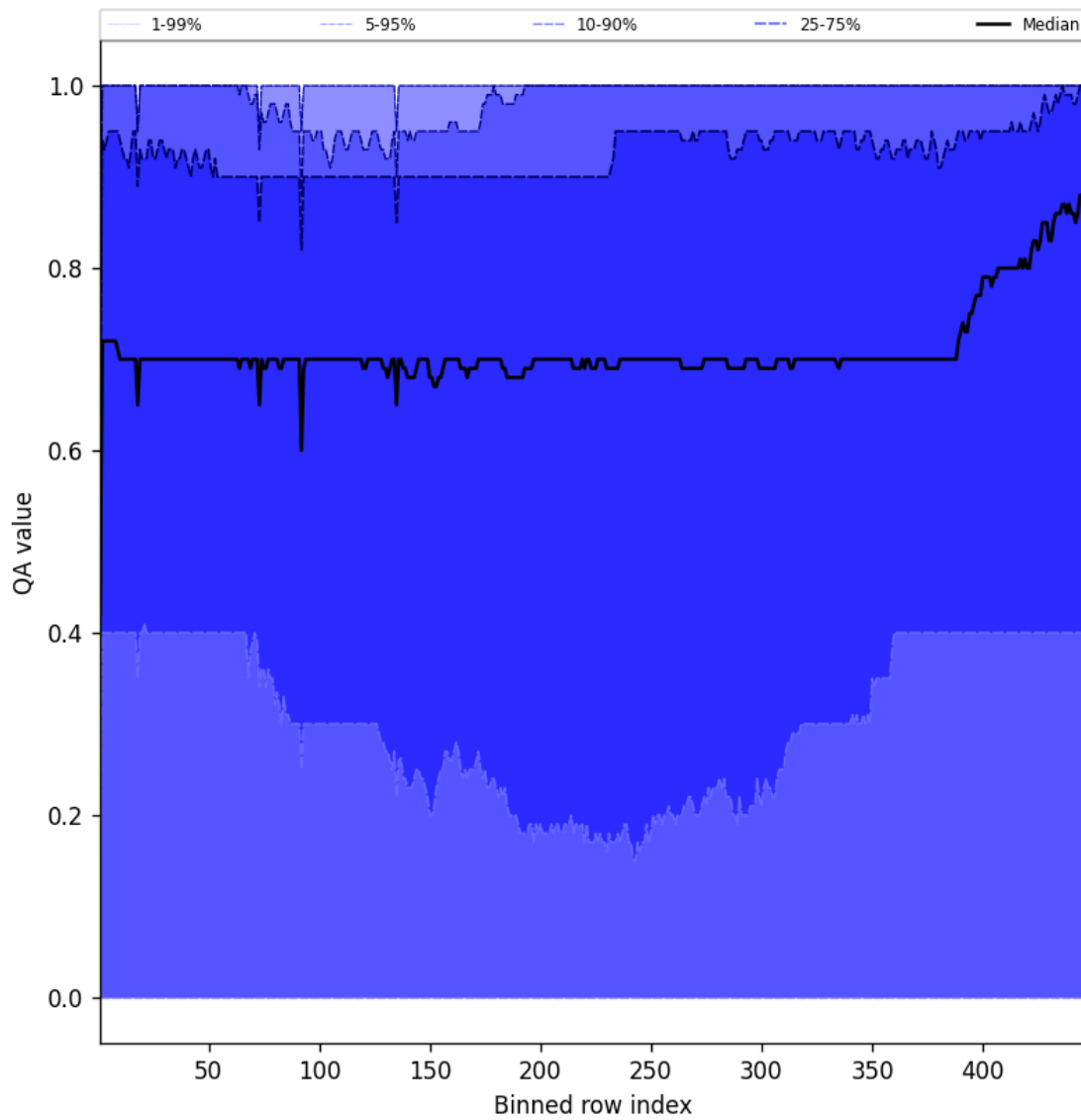
Figure 52: Along track statistics of “QA value” for 2025-12-04 to 2025-12-05
