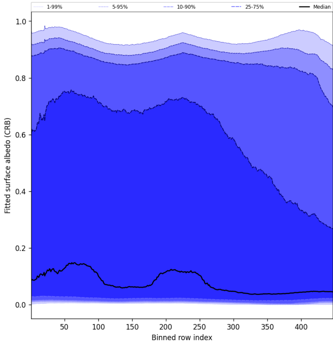
Figure 60: Along track statistics of “Fitted surface albedo (CRB)” for 2025-12-04 to 2025-12-05
