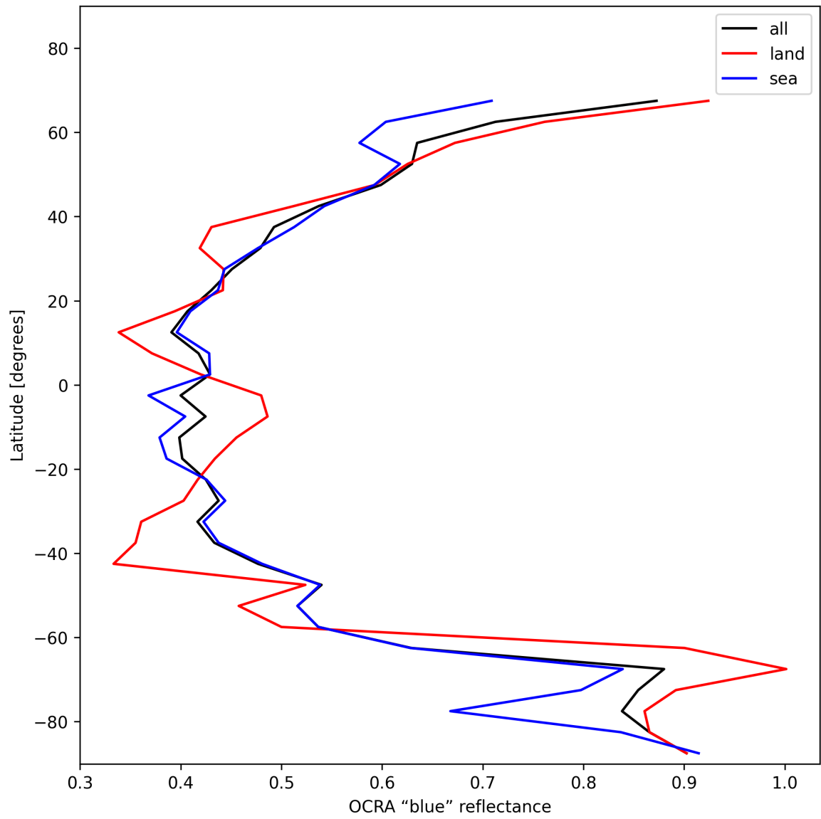
Figure 33: Zonal average of “OCRA “blue” reflectance” for 2025-12-04 to 2025-12-05.
