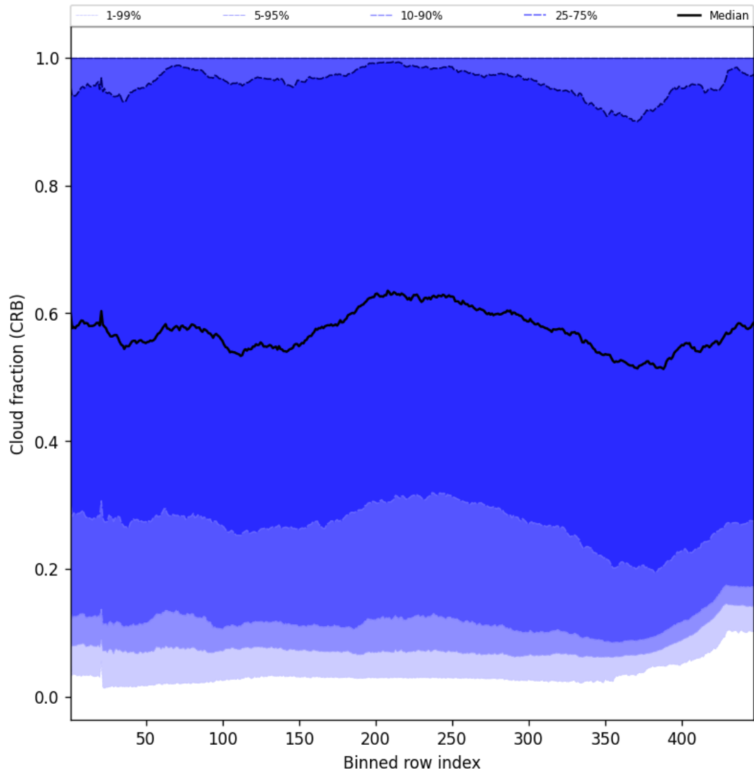
Figure 56: Along track statistics of “Cloud fraction (CRB)” for 2025-12-04 to 2025-12-05
