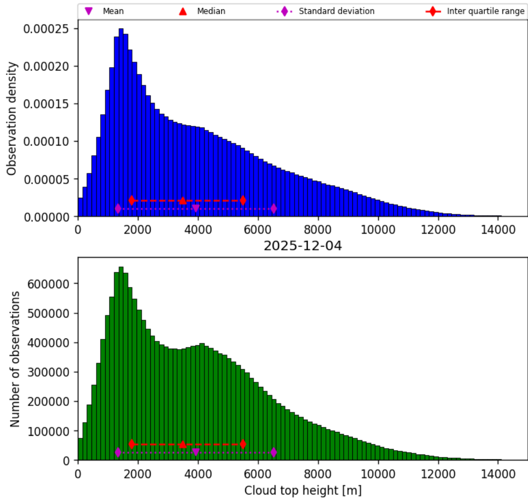
Figure 38: Histogram of “Cloud top height” for 2025-12-04 to 2025-12-05
