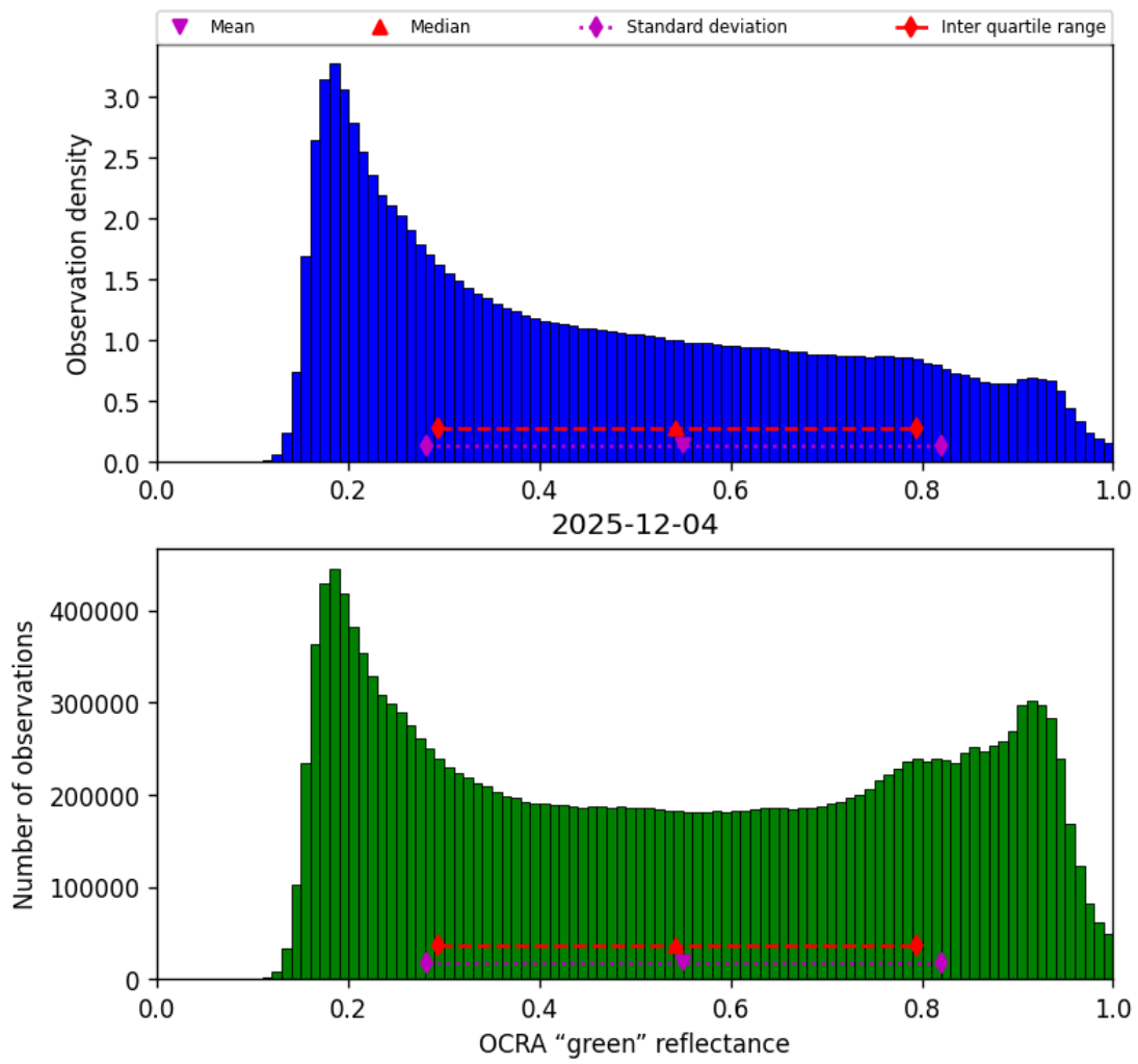
Figure 50: Histogram of “OCRA “green” reflectance” for 2025-12-04 to 2025-12-05
