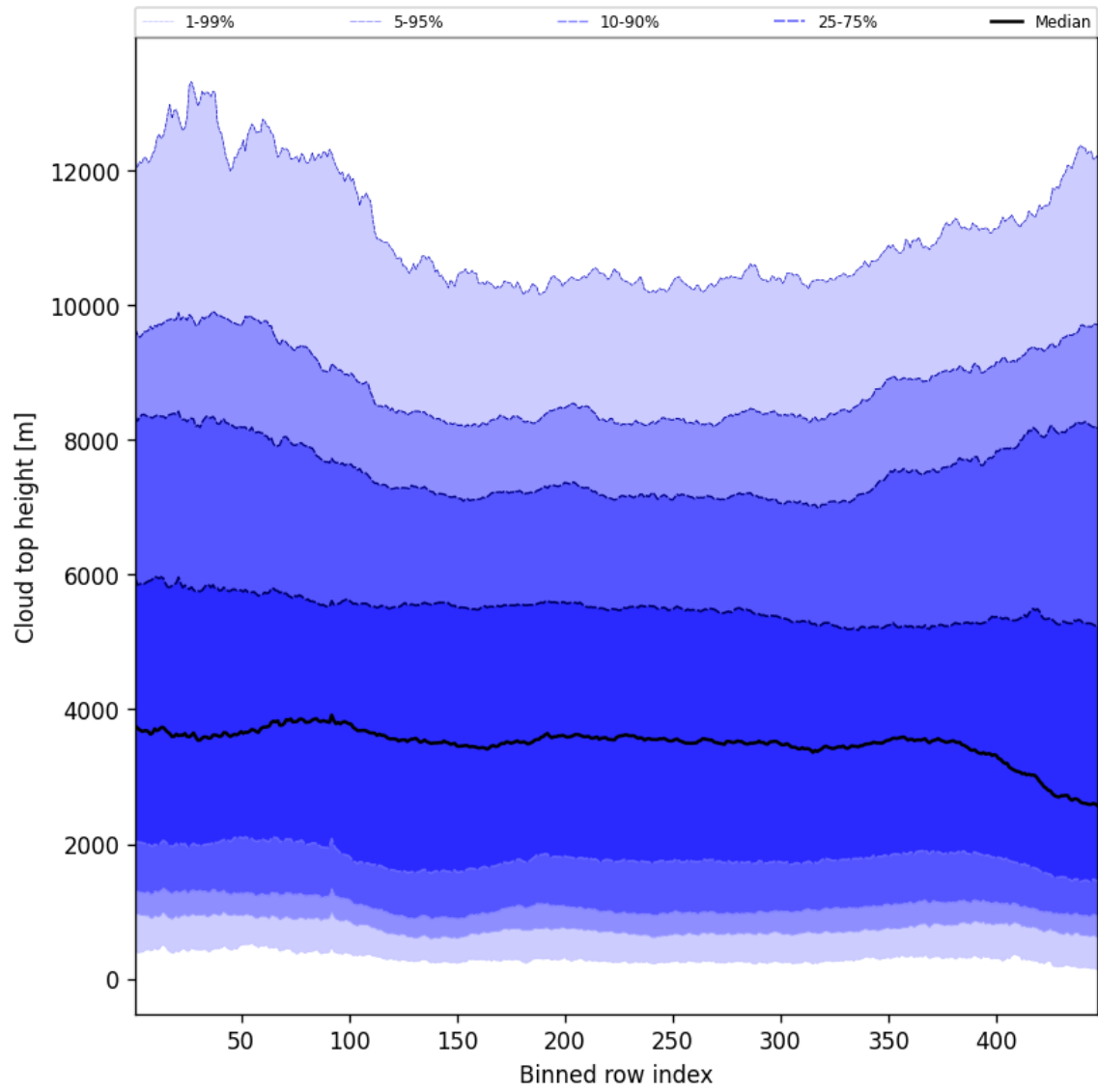
Figure 54: Along track statistics of “Cloud top height” for 2025-12-04 to 2025-12-05
