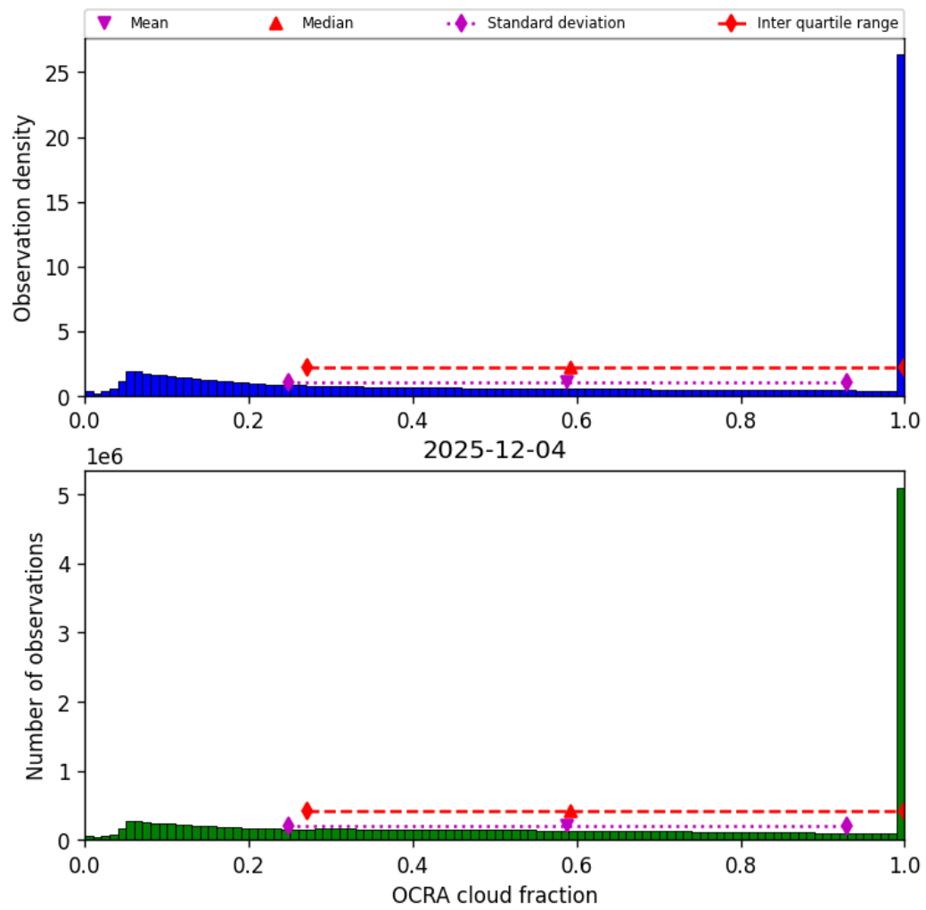
Figure 48: Histogram of “OCRA cloud fraction” for 2025-12-04 to 2025-12-05
