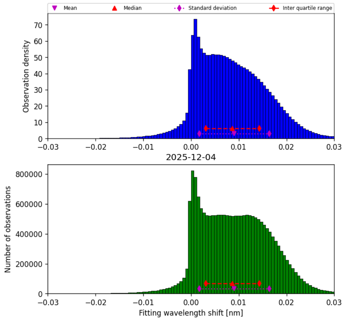
Figure 47: Histogram of “Fitting wavelength shift” for 2025-12-04 to 2025-12-05
