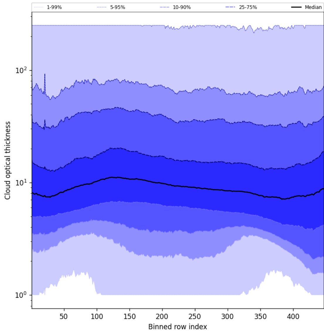
Figure 55: Along track statistics of “Cloud optical thickness” for 2025-12-04 to 2025-12-05
