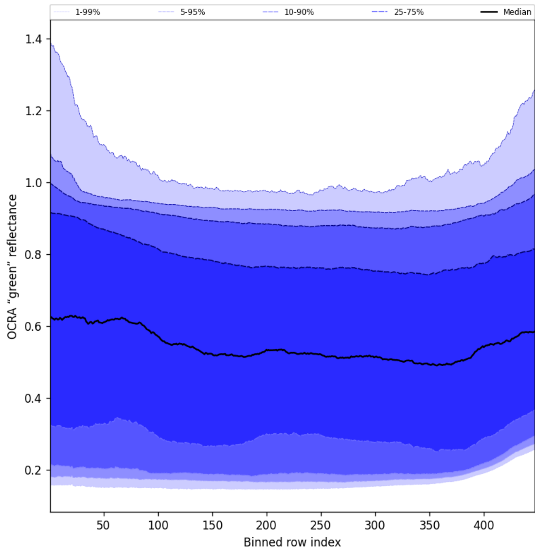
Figure 66: Along track statistics of “OCRA “green” reflectance” for 2025-12-04 to 2025-12-05
