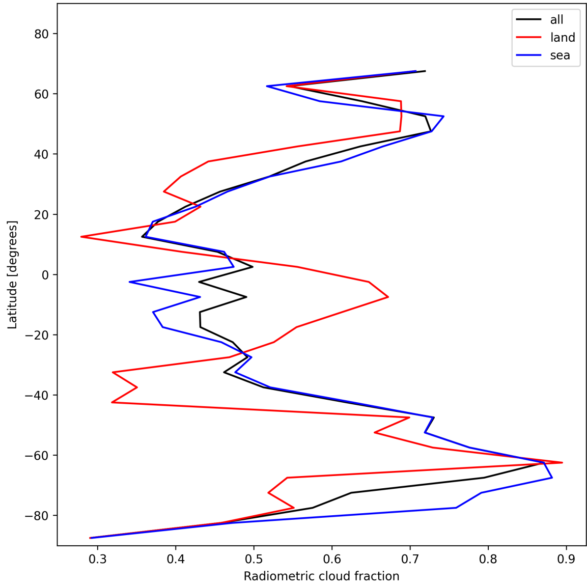
Figure 21: Zonal average of “Radiometric cloud fraction” for 2025-12-04 to 2025-12-05.
