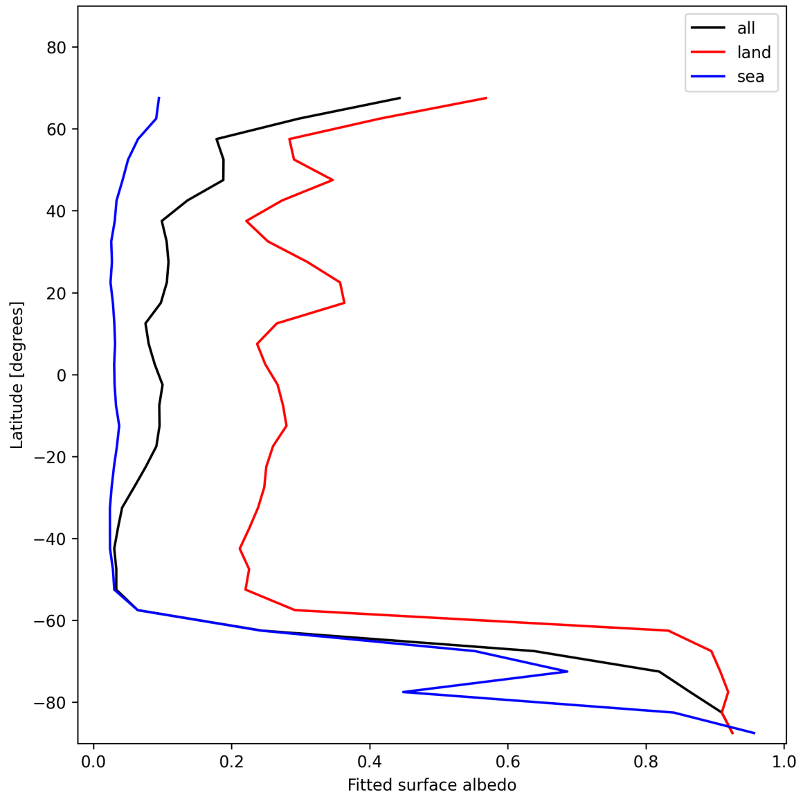
Figure 27: Zonal average of “Fitted surface albedo” for 2025-12-04 to 2025-12-05.
