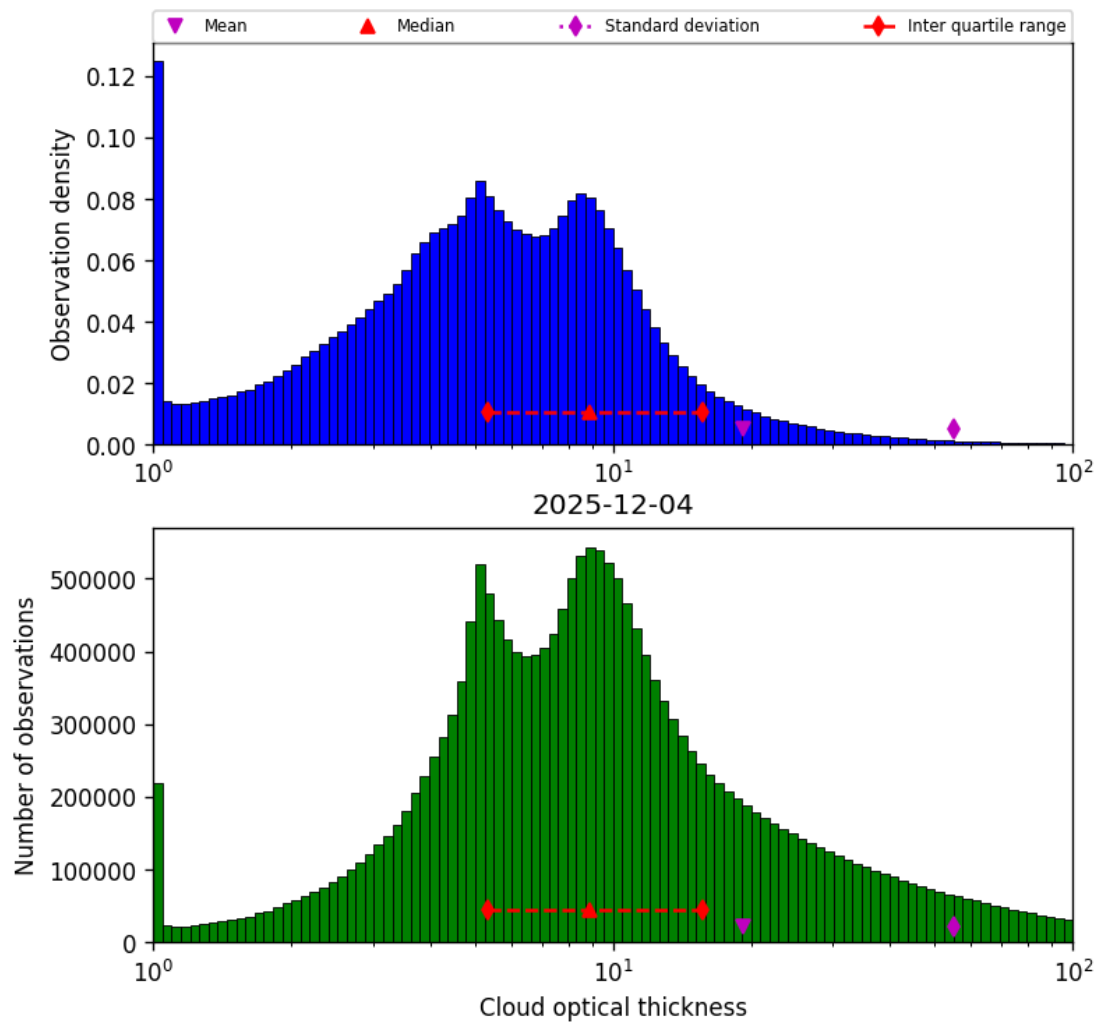
Figure 39: Histogram of “Cloud optical thickness” for 2025-12-04 to 2025-12-05
