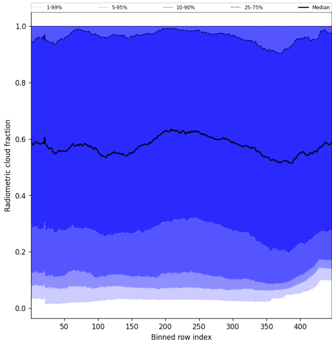
Figure 53: Along track statistics of “Radiometric cloud fraction” for 2025-12-04 to 2025-12-05
