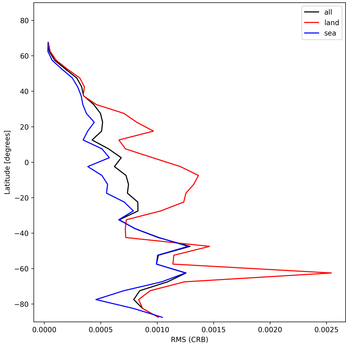
Figure 30: Zonal average of “RMS (CRB)” for 2025-12-04 to 2025-12-05.
