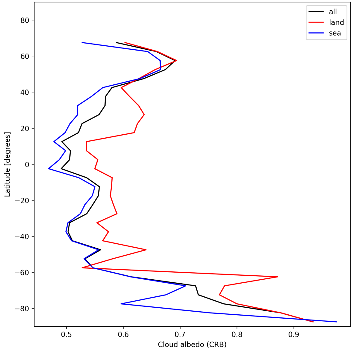
Figure 26: Zonal average of “Cloud albedo (CRB)” for 2025-12-04 to 2025-12-05.
