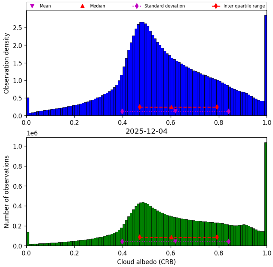
Figure 42: Histogram of “Cloud albedo (CRB)” for 2025-12-04 to 2025-12-05
