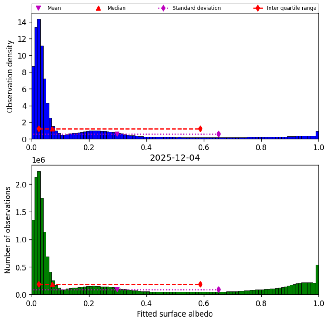
Figure 43: Histogram of “Fitted surface albedo” for 2025-12-04 to 2025-12-05
