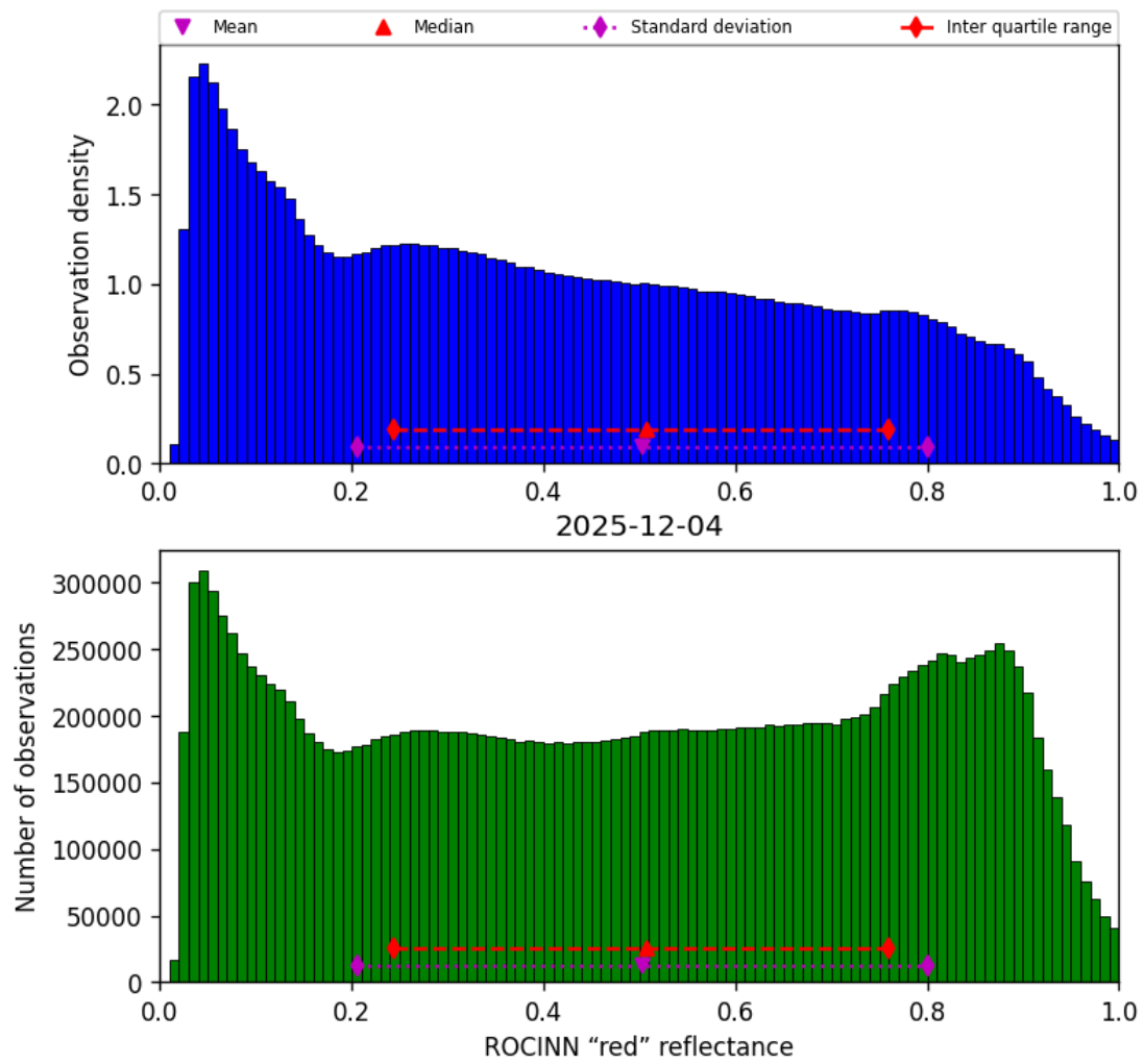
Figure 51: Histogram of “ROCINN “red” reflectance” for 2025-12-04 to 2025-12-05
