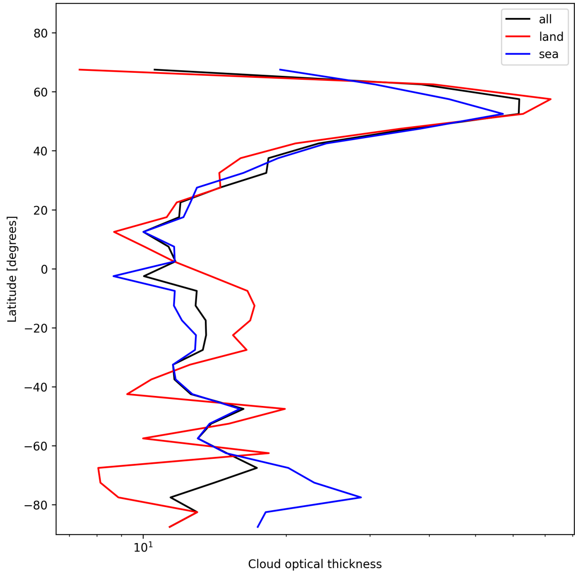
Figure 23: Zonal average of “Cloud optical thickness” for 2025-12-04 to 2025-12-05.
