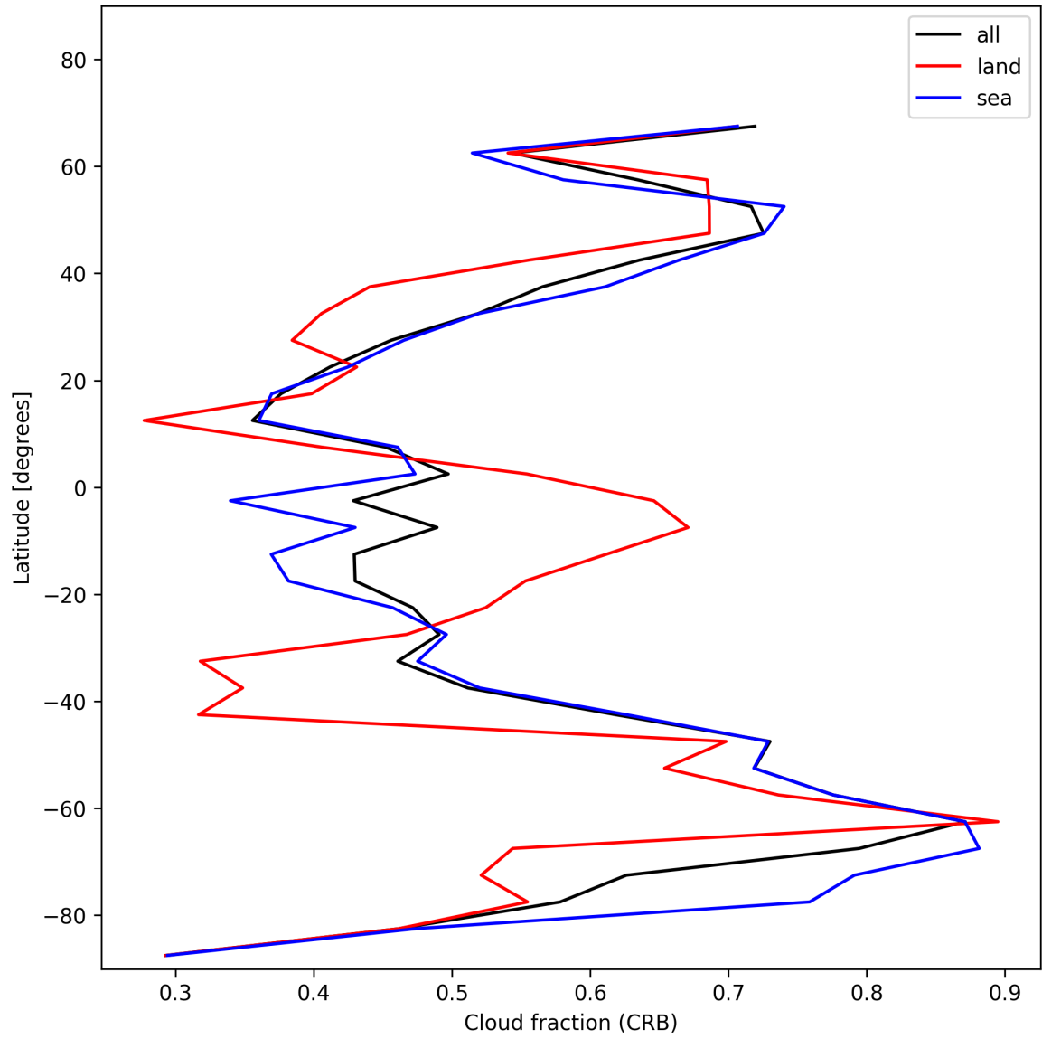
Figure 24: Zonal average of “Cloud fraction (CRB)” for 2025-12-04 to 2025-12-05.
