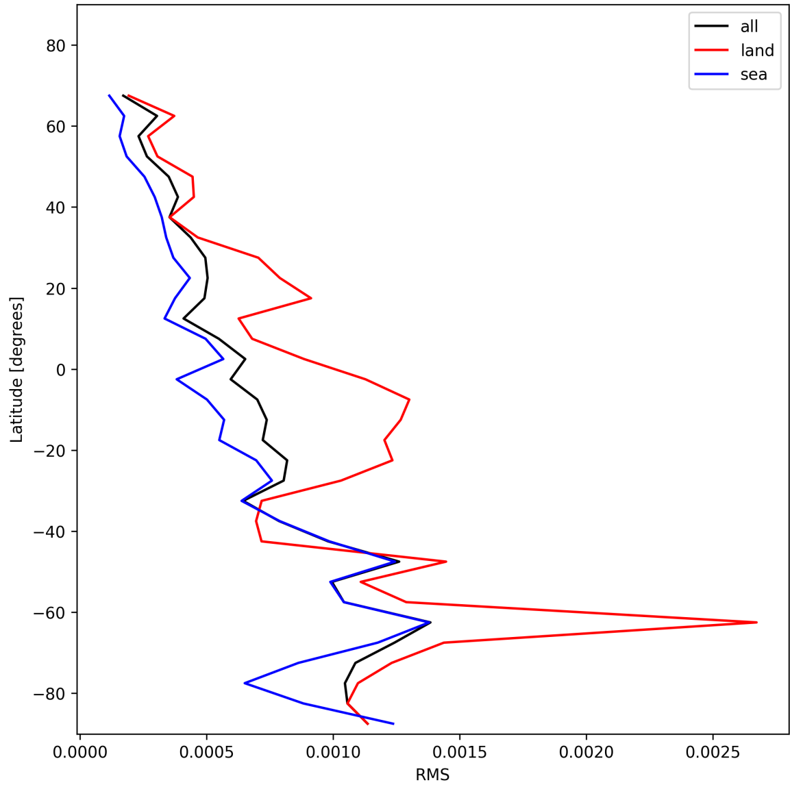
Figure 29: Zonal average of “RMS” for 2025-12-04 to 2025-12-05.
