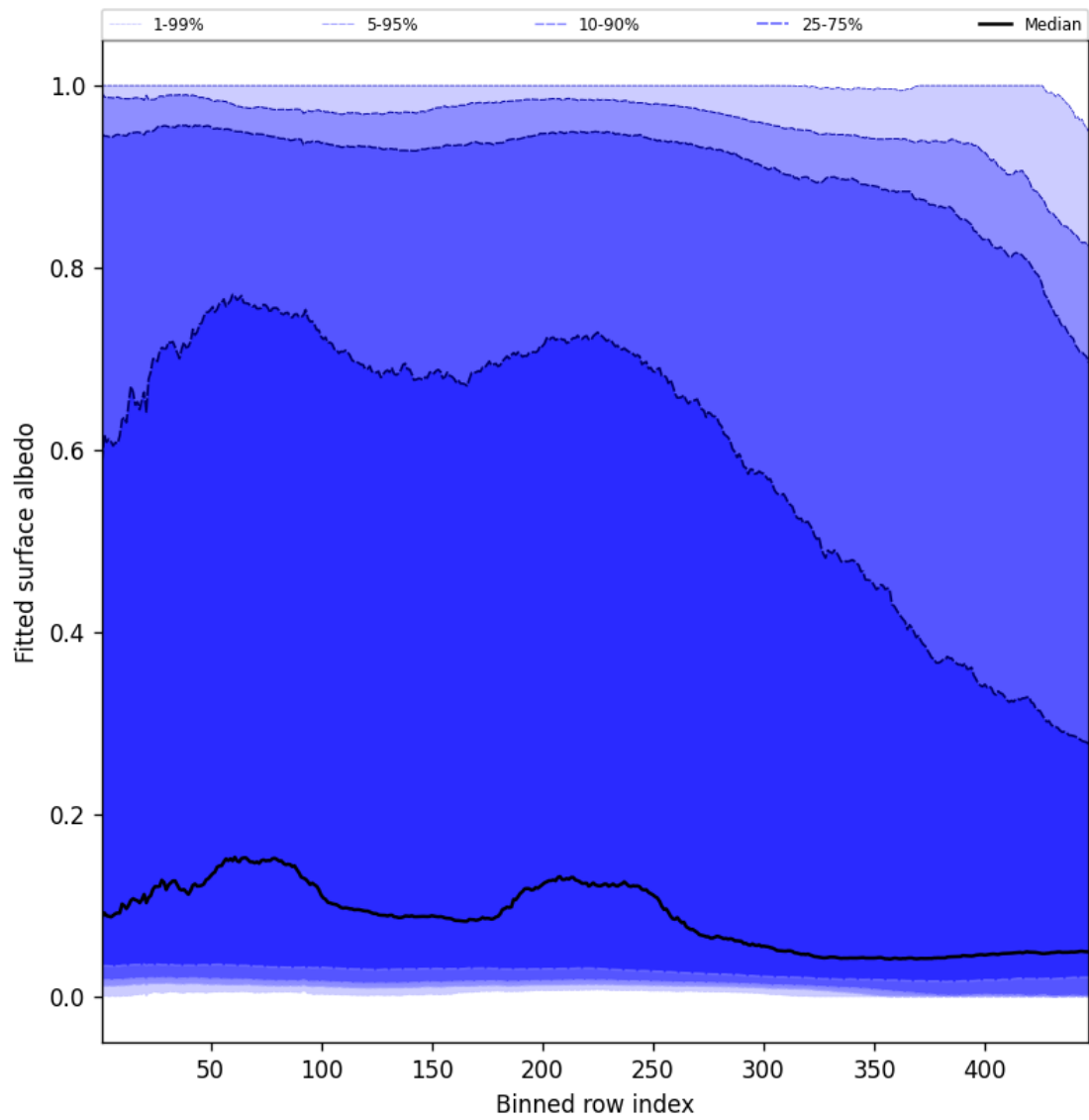
Figure 59: Along track statistics of “Fitted surface albedo” for 2025-12-04 to 2025-12-05
