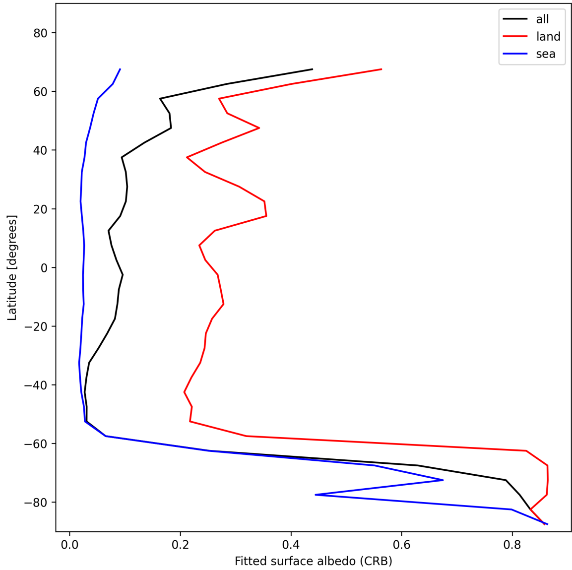
Figure 28: Zonal average of “Fitted surface albedo (CRB)” for 2025-12-04 to 2025-12-05.
