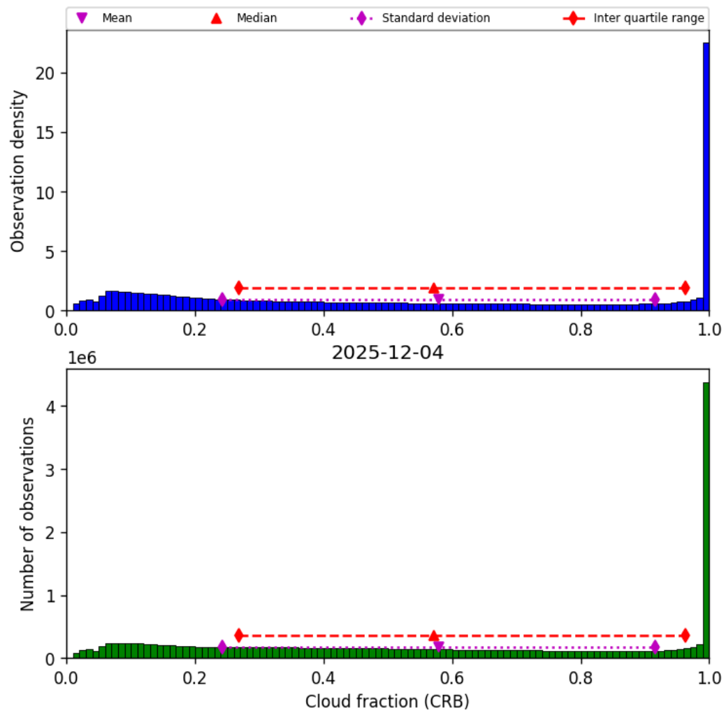
Figure 40: Histogram of “Cloud fraction (CRB)” for 2025-12-04 to 2025-12-05
