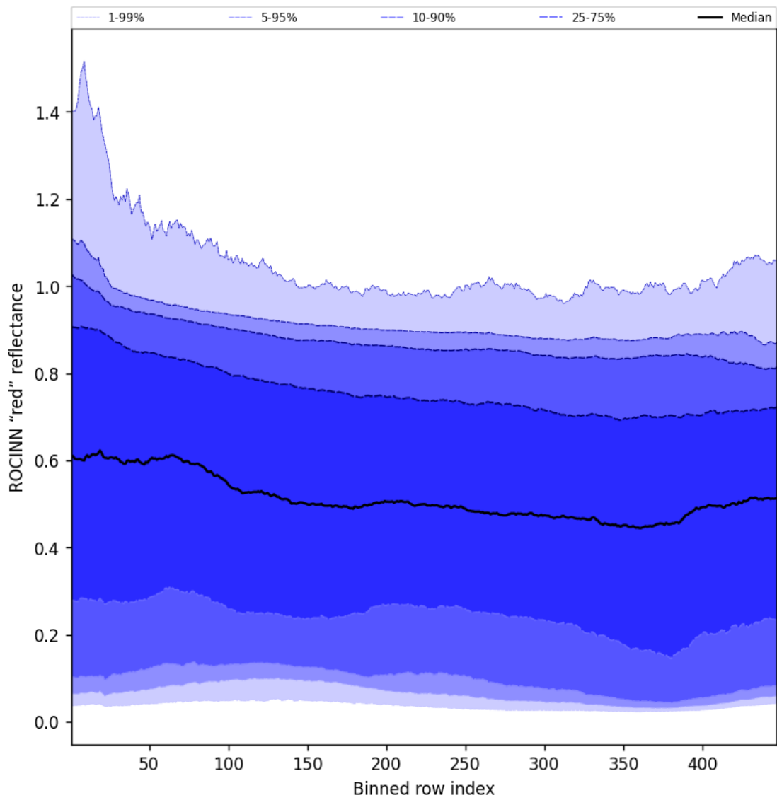
Figure 67: Along track statistics of “ROCINN “red” reflectance” for 2025-12-04 to 2025-12-05
