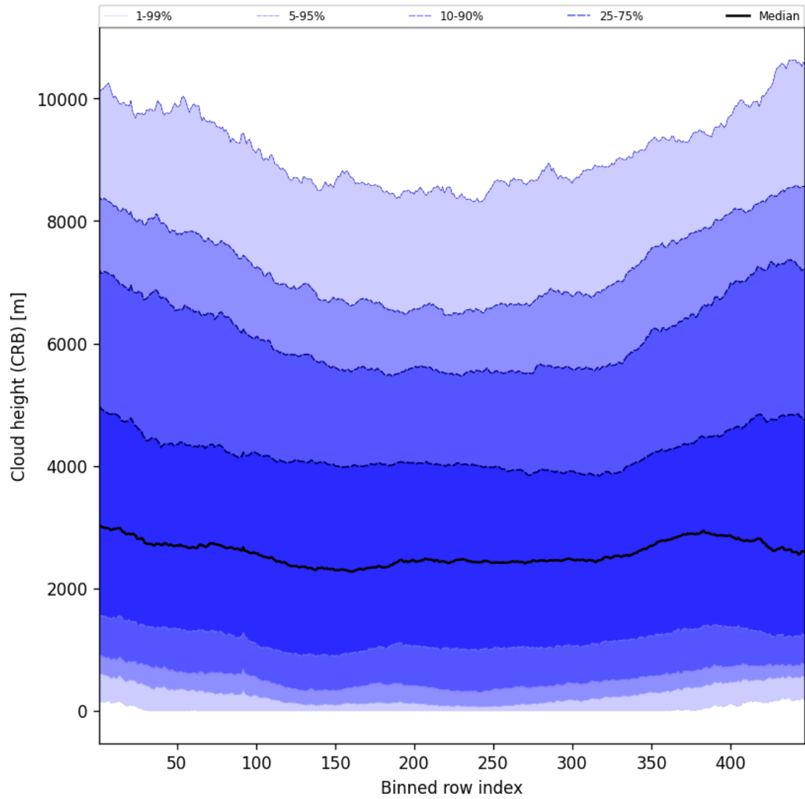
Figure 57: Along track statistics of “Cloud height (CRB)” for 2025-12-04 to 2025-12-05
