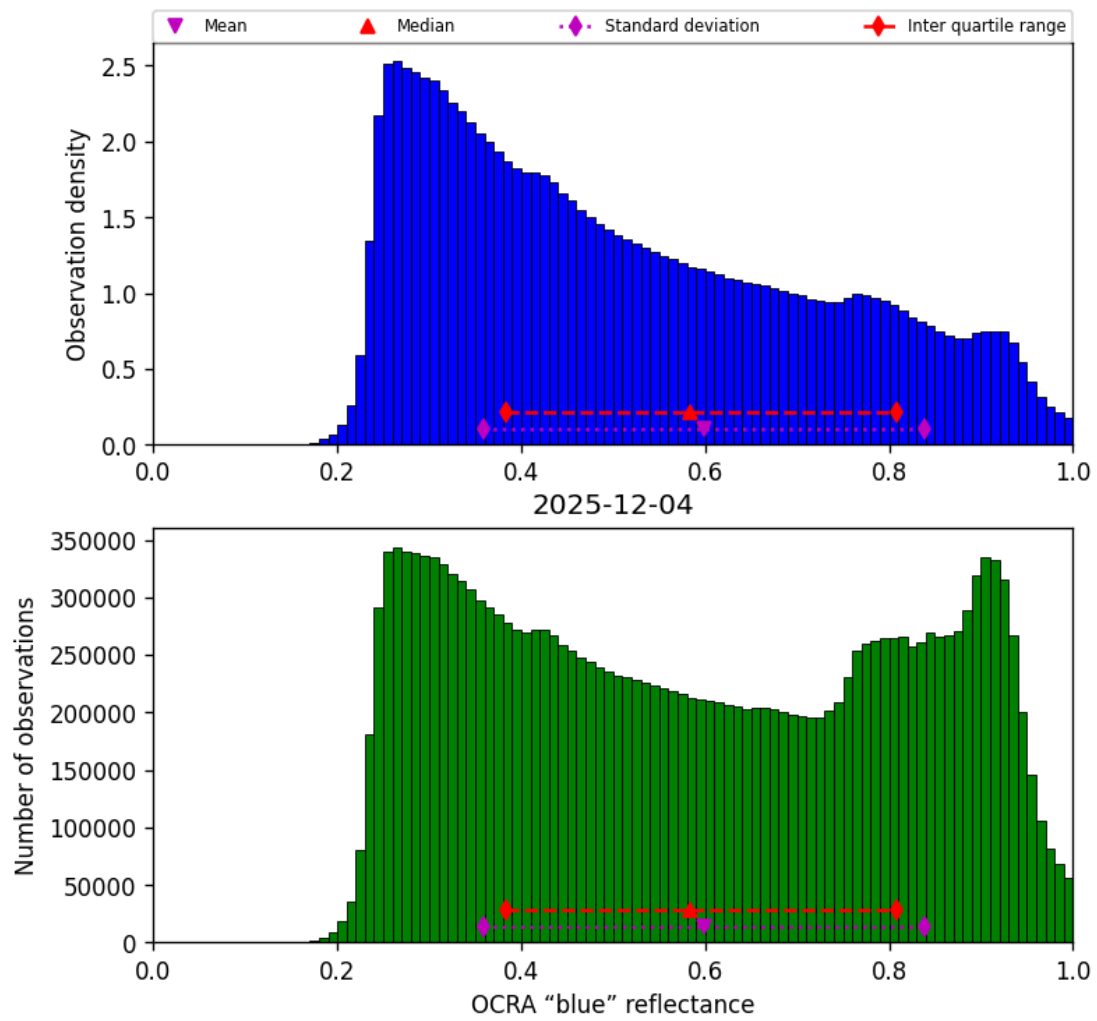
Figure 49: Histogram of "OCRA "blue" reflectance" for 2025-12-04 to 2025-12-05
