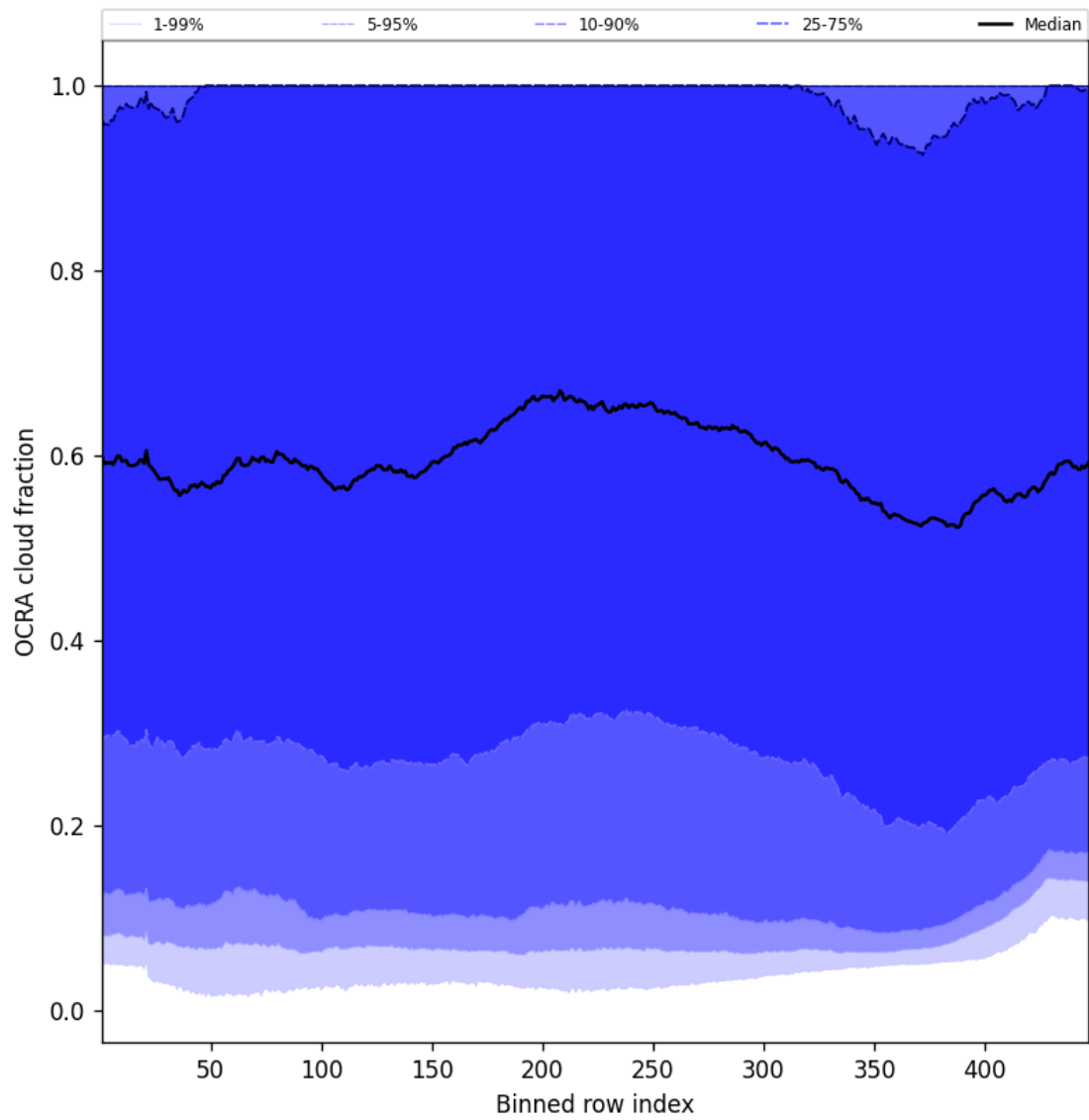
Figure 64: Along track statistics of “OCRA cloud fraction” for 2025-12-04 to 2025-12-05
