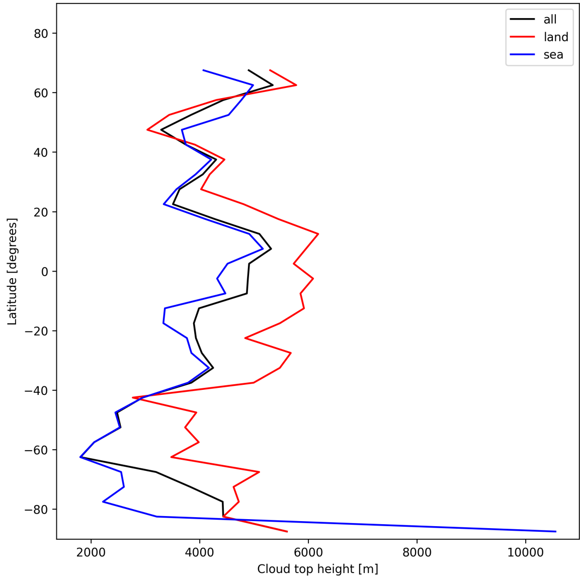
Figure 22: Zonal average of “Cloud top height” for 2025-12-04 to 2025-12-05.
