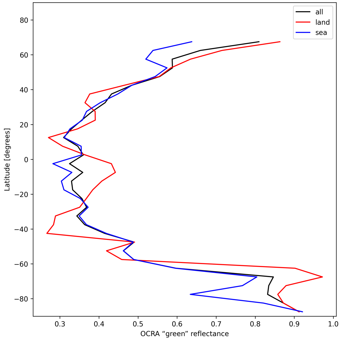
Figure 34: Zonal average of "OCRA "green" reflectance" for 2025-12-04 to 2025-12-05.
