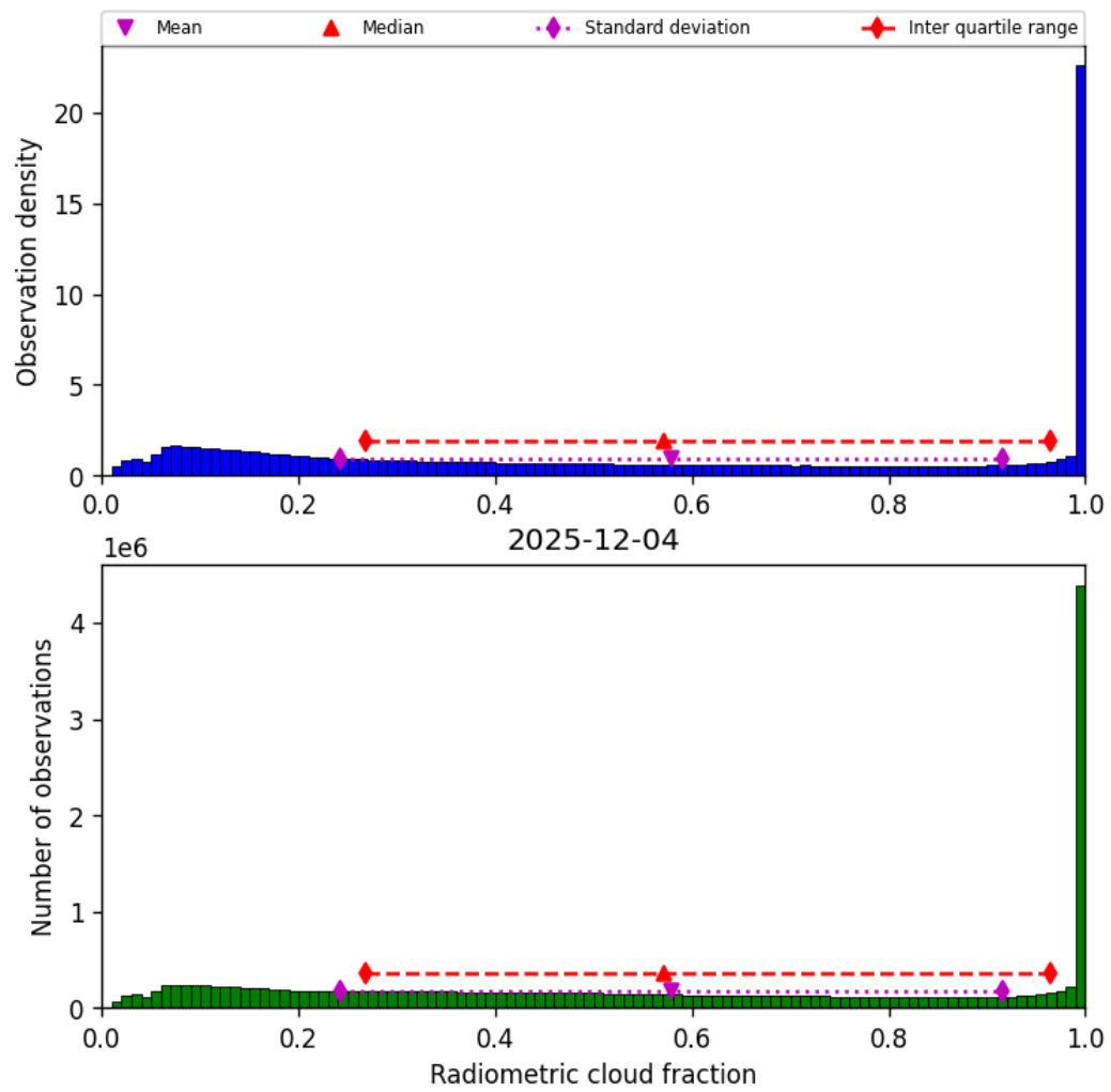
Figure 37: Histogram of “Radiometric cloud fraction” for 2025-12-04 to 2025-12-05
