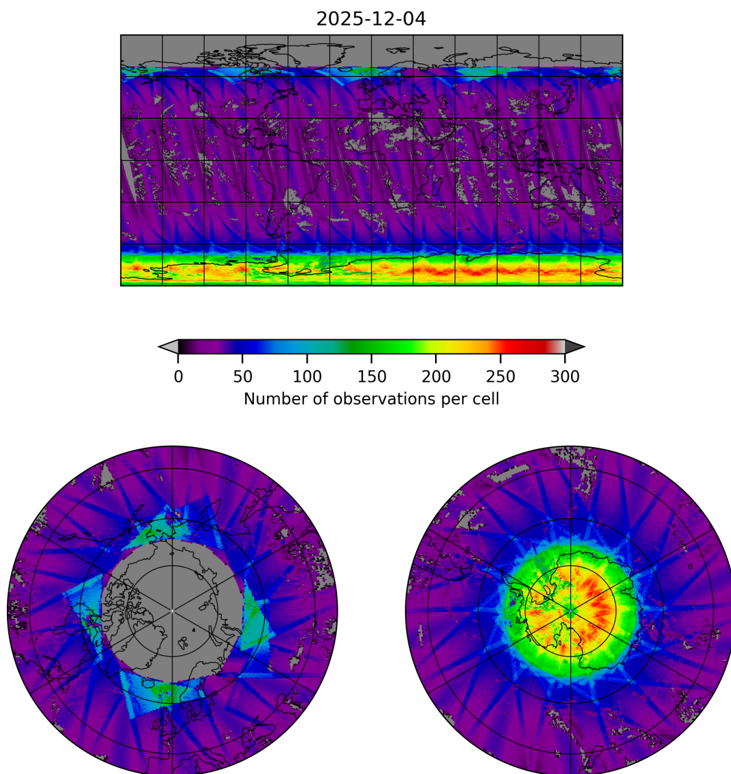
Figure 19: Map of the number of observations for 2025-12-04 to 2025-12-05
