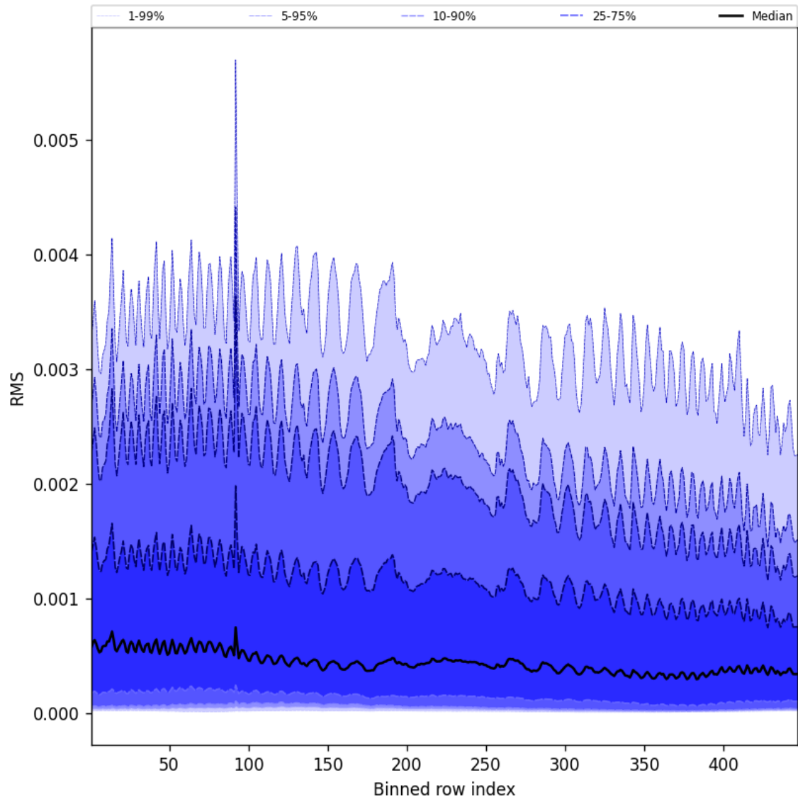
Figure 61: Along track statistics of “RMS” for 2025-12-04 to 2025-12-05
