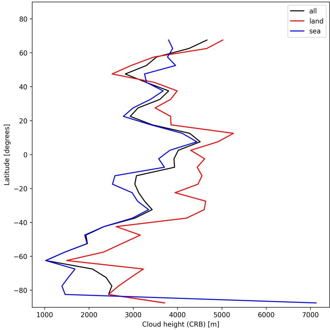
Figure 25: Zonal average of “Cloud height (CRB)” for 2025-12-04 to 2025-12-05.
