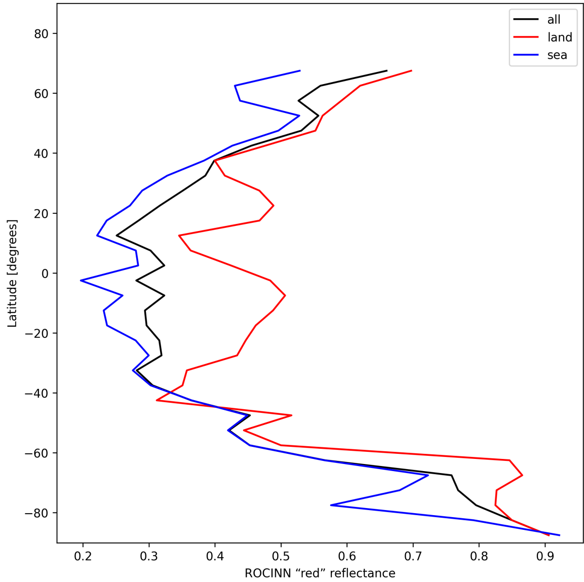
Figure 35: Zonal average of "ROCINN "red" reflectance" for 2025-12-04 to 2025-12-05.
