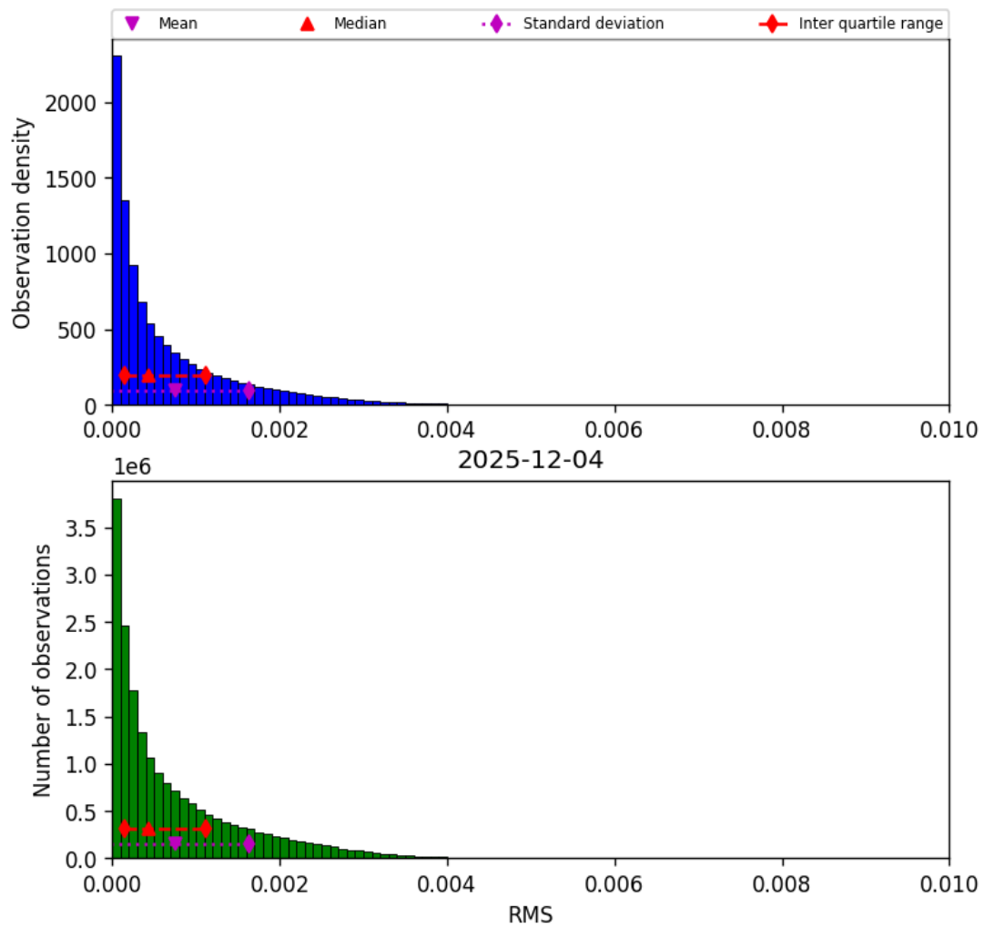
Figure 45: Histogram of “RMS” for 2025-12-04 to 2025-12-05
