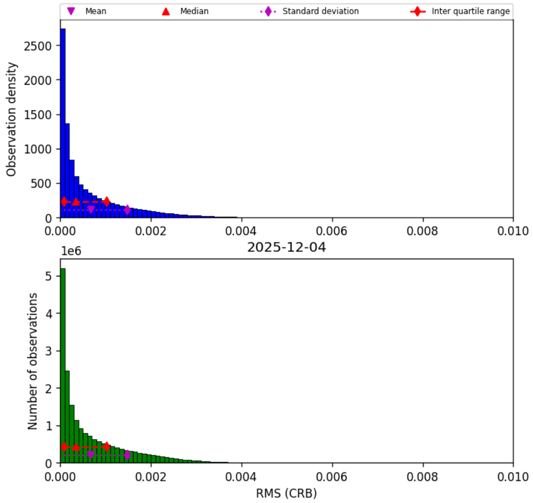
Figure 46: Histogram of “RMS (CRB)” for 2025-12-04 to 2025-12-05
