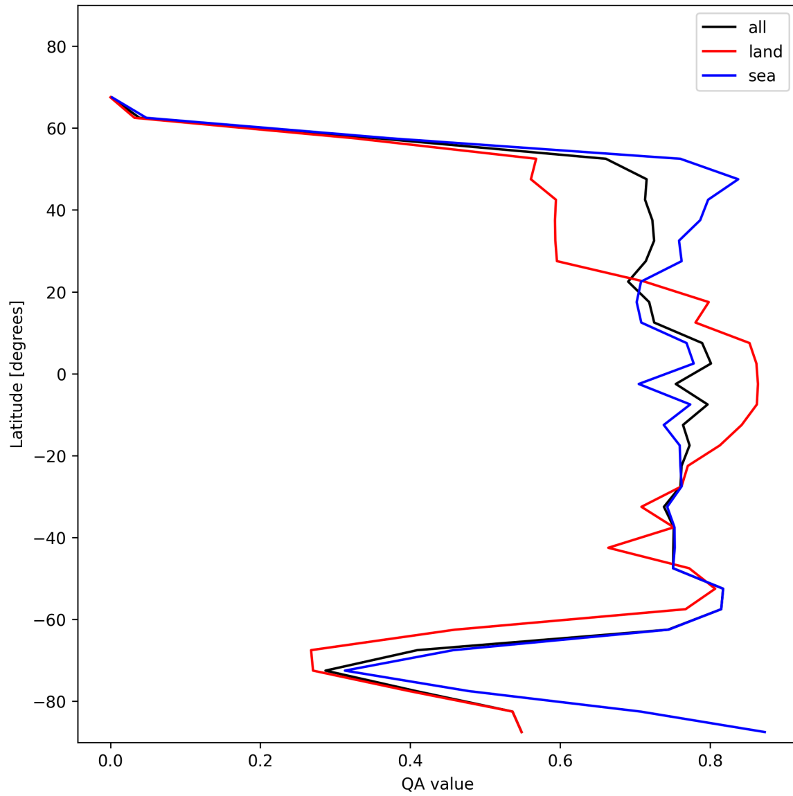
Figure 20: Zonal average of “QA value” for 2025-12-04 to 2025-12-05.
