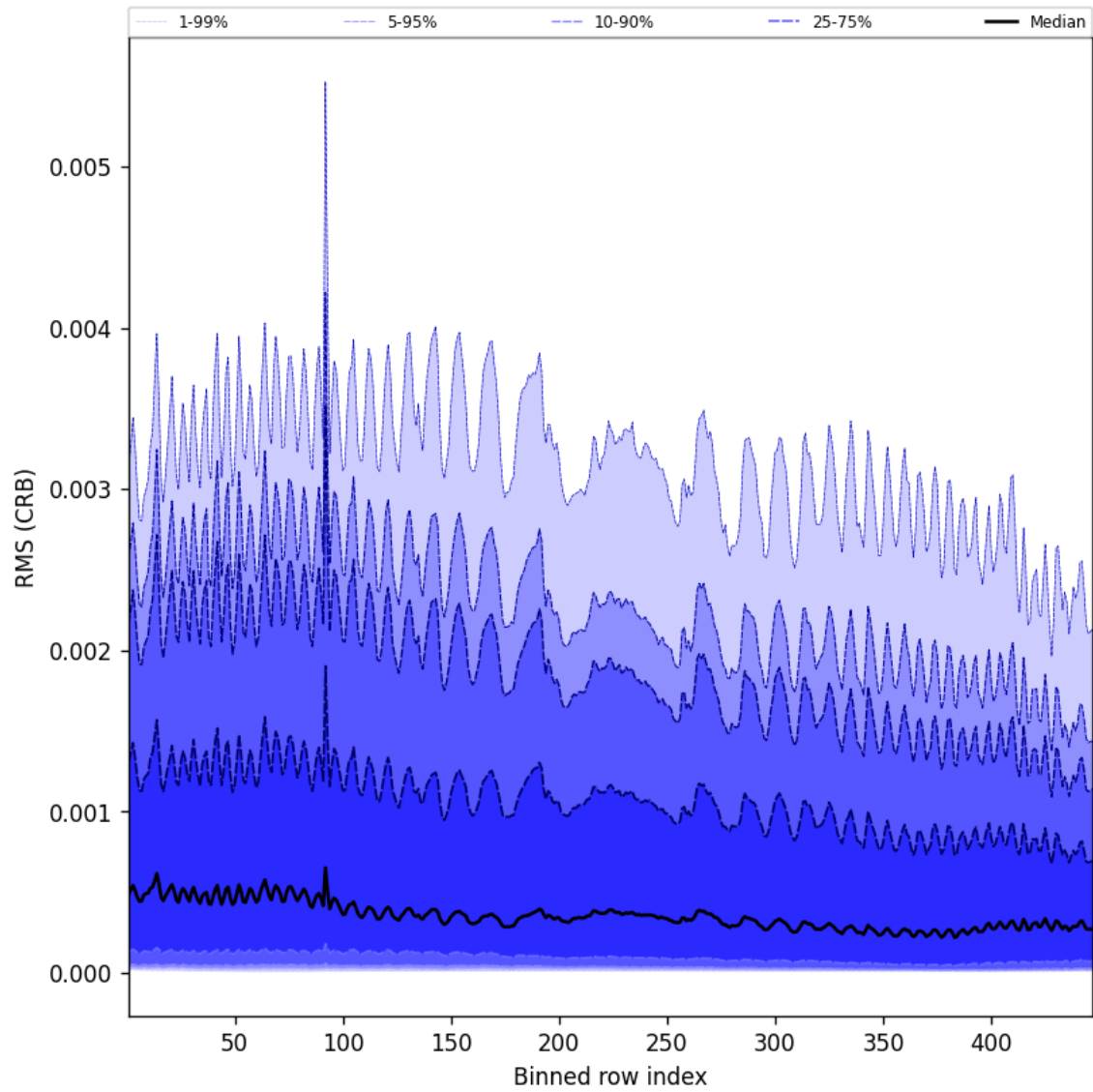
Figure 62: Along track statistics of “RMS (CRB)” for 2025-12-04 to 2025-12-05
