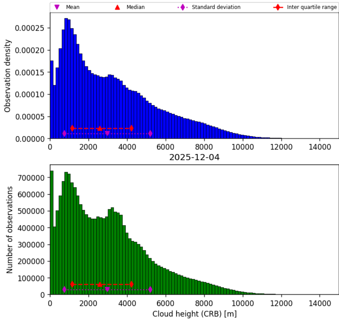
Figure 41: Histogram of “Cloud height (CRB)” for 2025-12-04 to 2025-12-05
