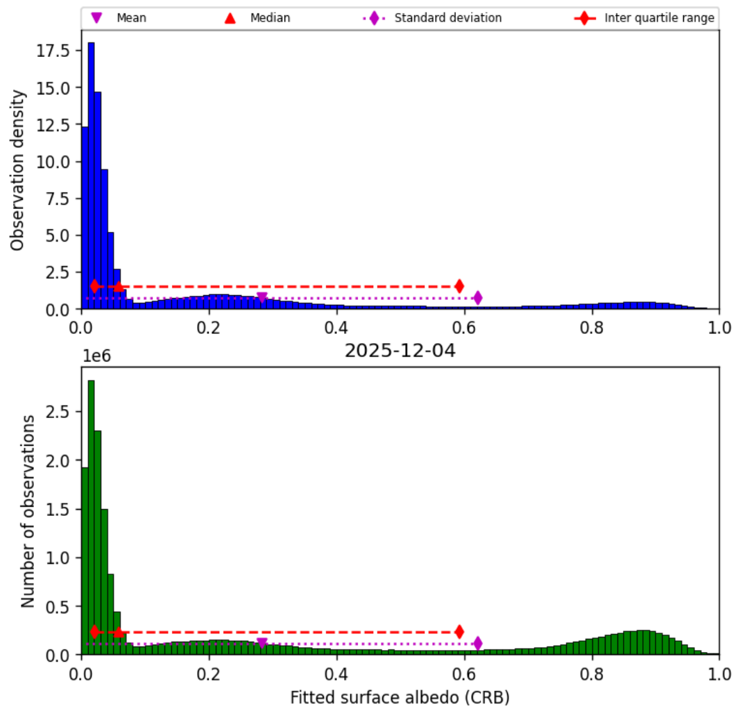
Figure 44: Histogram of “Fitted surface albedo (CRB)” for 2025-12-04 to 2025-12-05
