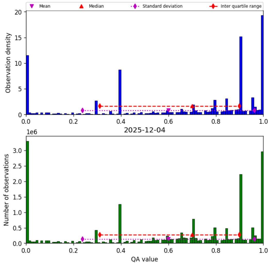
Figure 36: Histogram of “QA value” for 2025-12-04 to 2025-12-05
