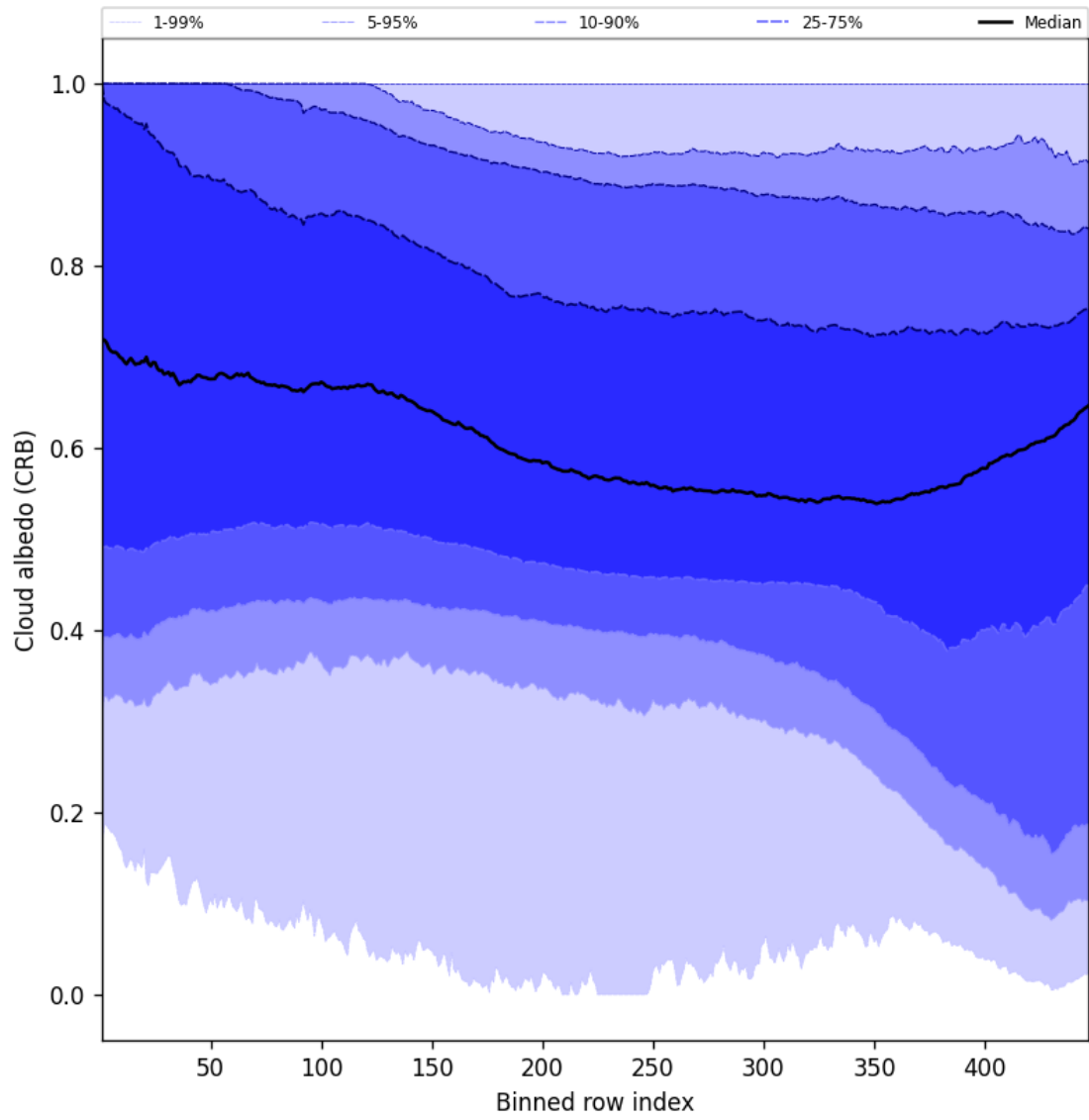
Figure 58: Along track statistics of “Cloud albedo (CRB)” for 2025-12-04 to 2025-12-05
