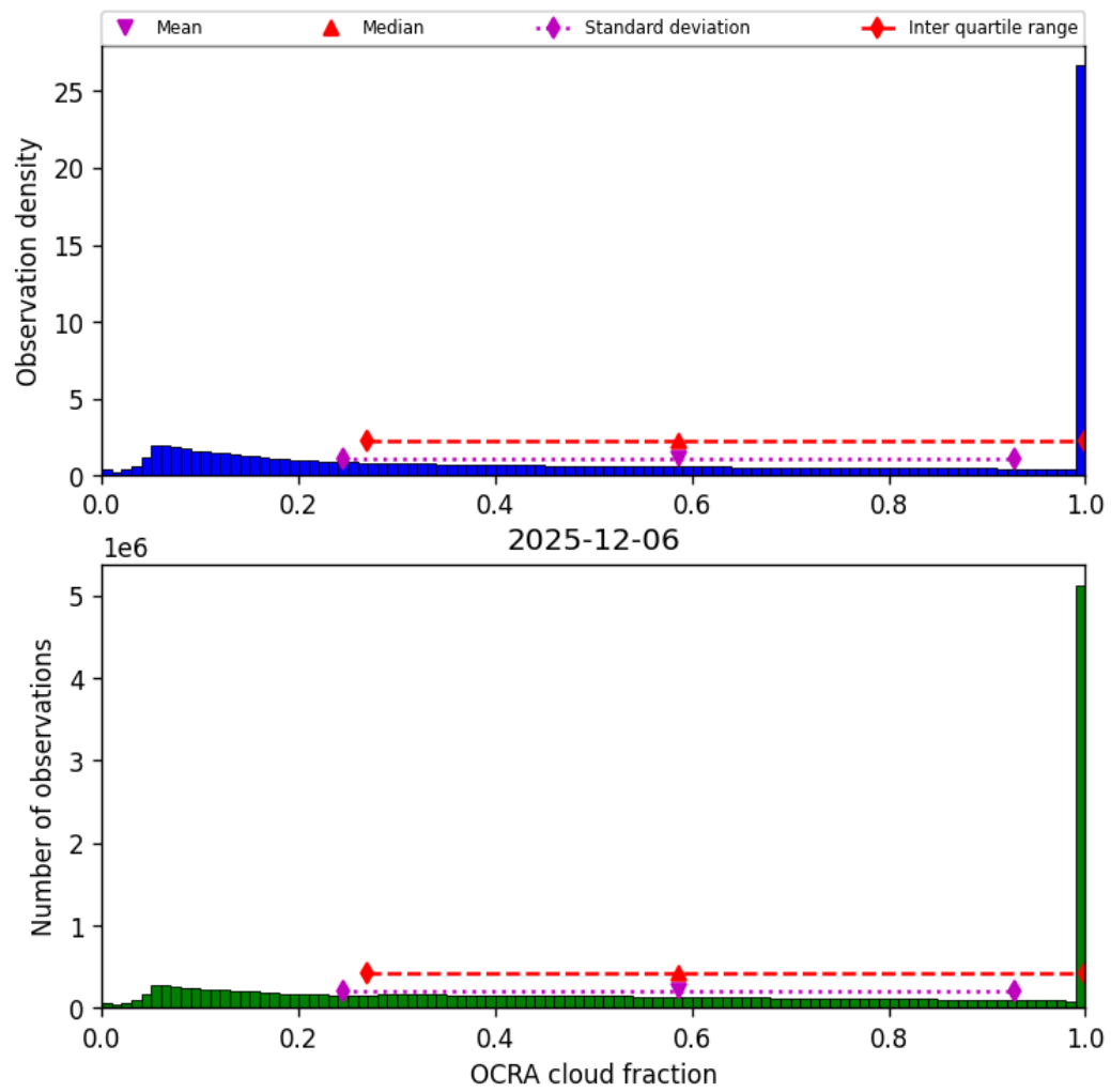
Figure 48: Histogram of “OCRA cloud fraction” for 2025-12-06 to 2025-12-07
