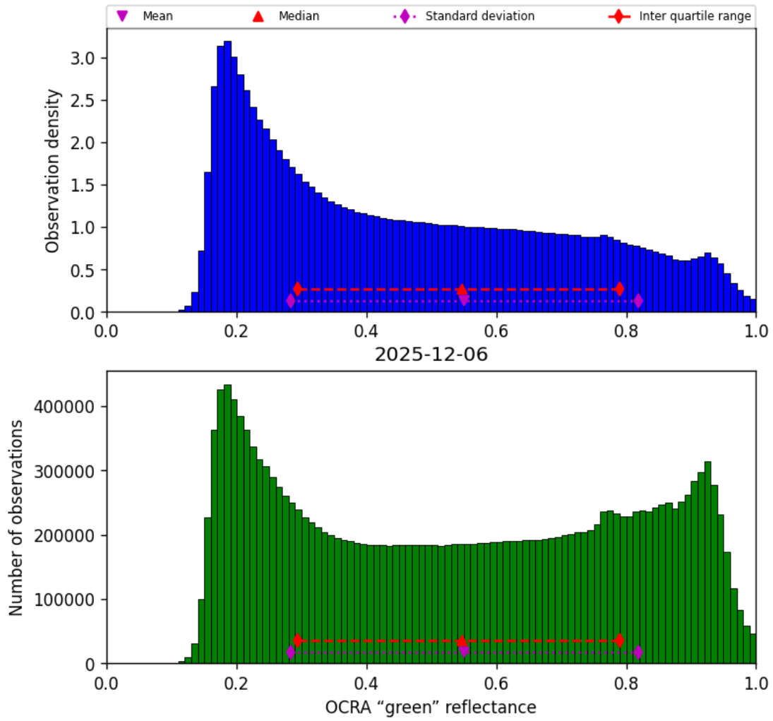
Figure 50: Histogram of “OCRA “green” reflectance” for 2025-12-06 to 2025-12-07
