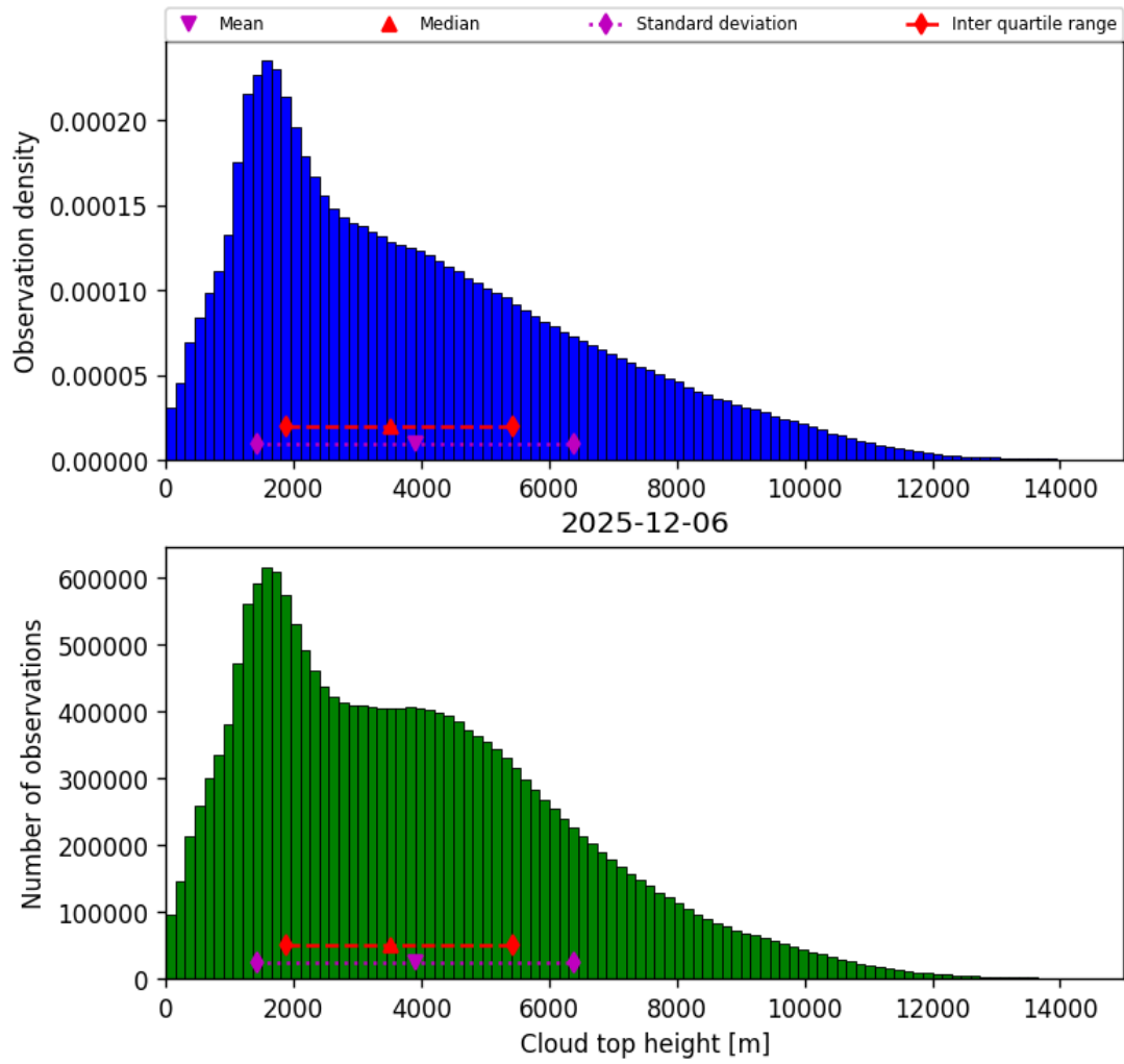
Figure 38: Histogram of “Cloud top height” for 2025-12-06 to 2025-12-07
