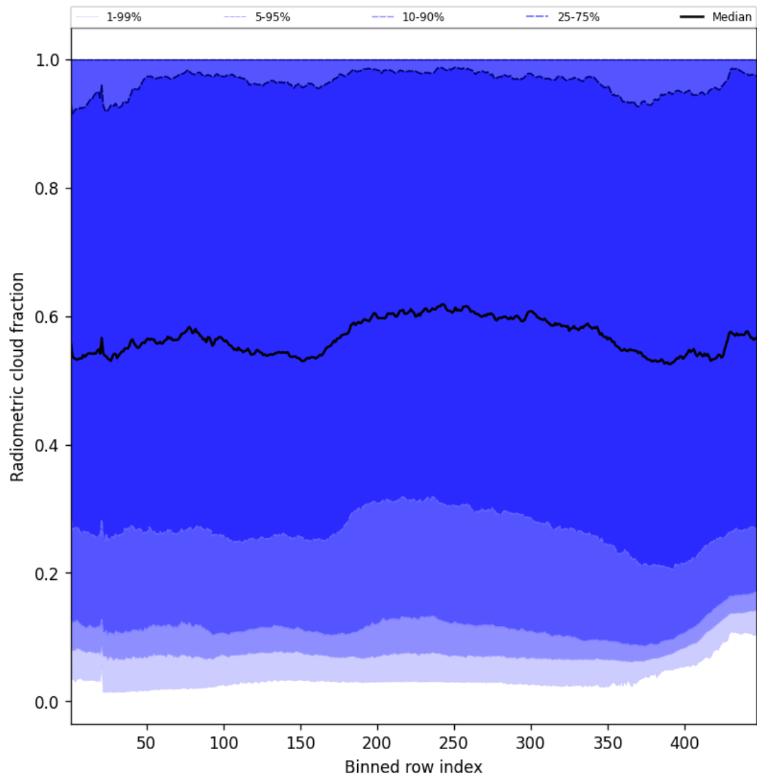
Figure 53: Along track statistics of “Radiometric cloud fraction” for 2025-12-06 to 2025-12-07
