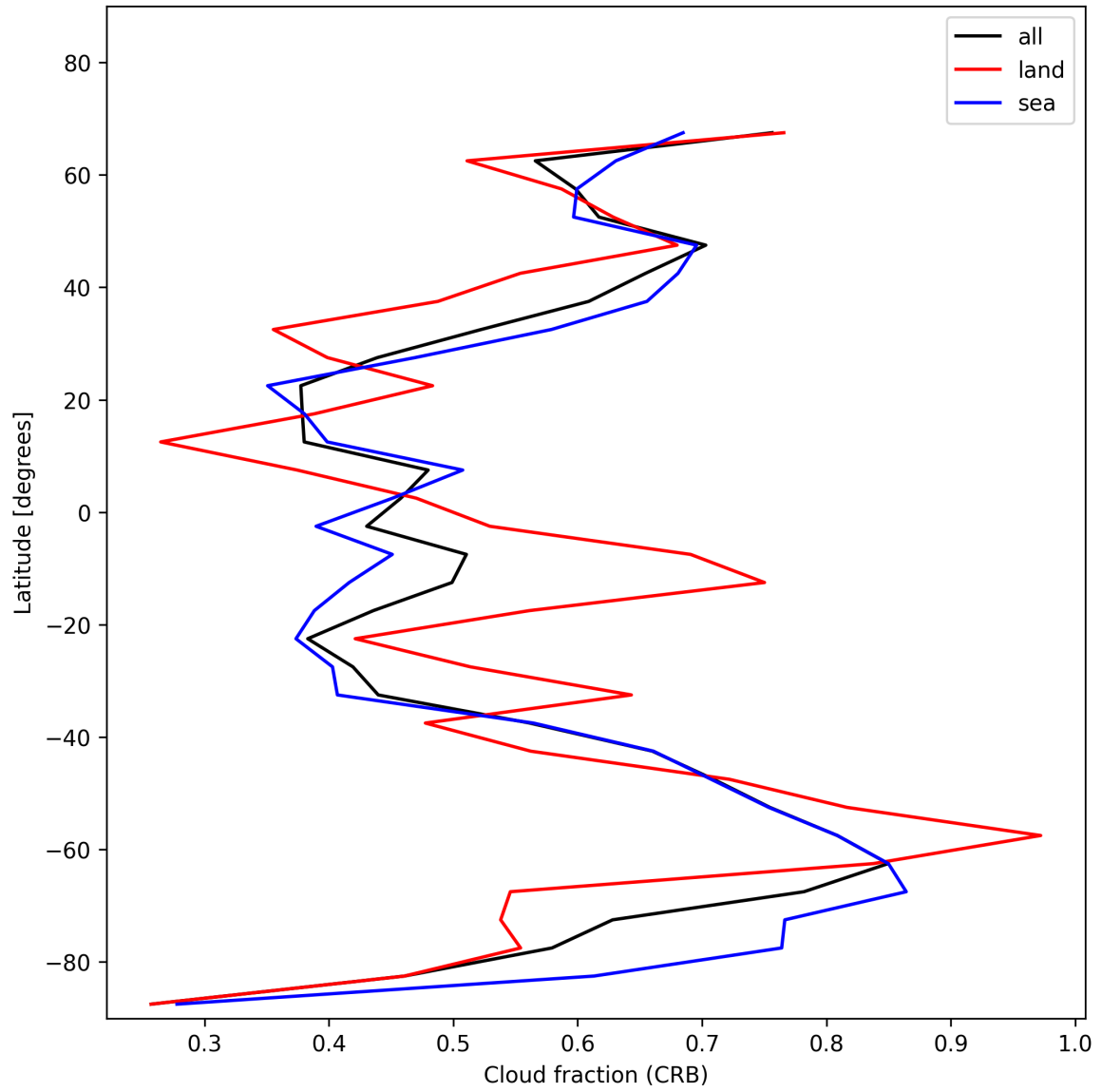
Figure 24: Zonal average of “Cloud fraction (CRB)” for 2025-12-06 to 2025-12-07.
