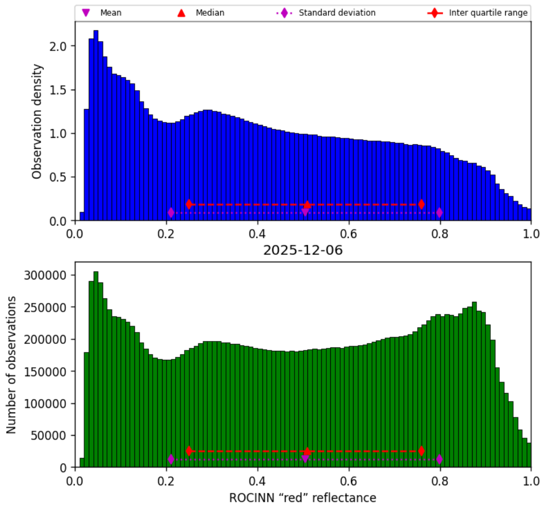
Figure 51: Histogram of “ROCINN “red” reflectance” for 2025-12-06 to 2025-12-07
