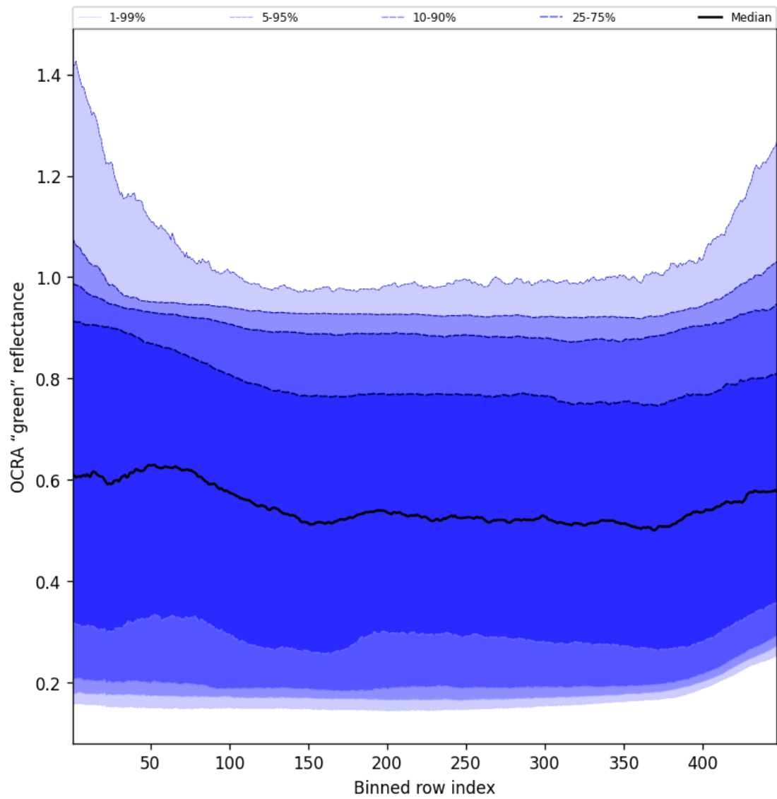
Figure 66: Along track statistics of "OCRA "green" reflectance" for 2025-12-06 to 2025-12-07
