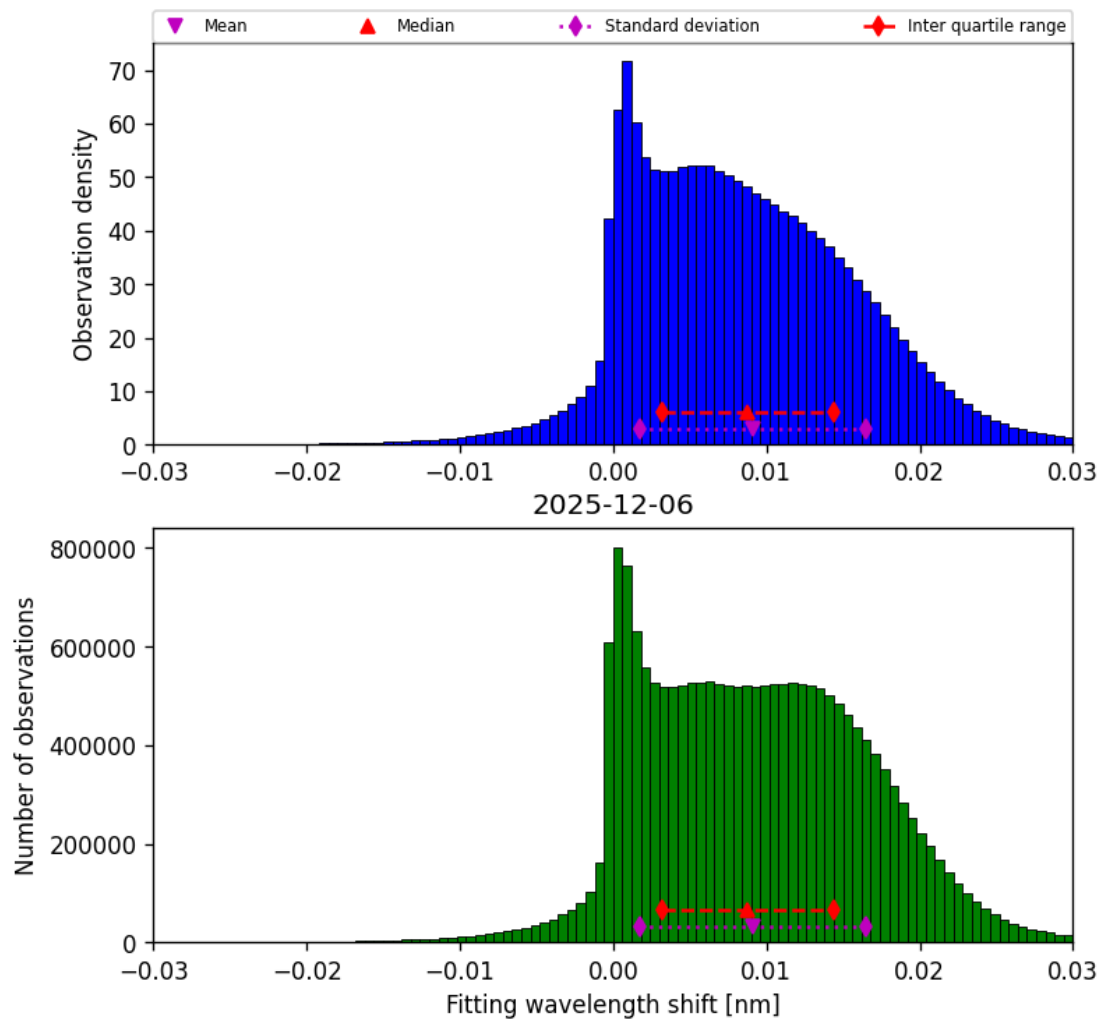
Figure 47: Histogram of “Fitting wavelength shift” for 2025-12-06 to 2025-12-07
