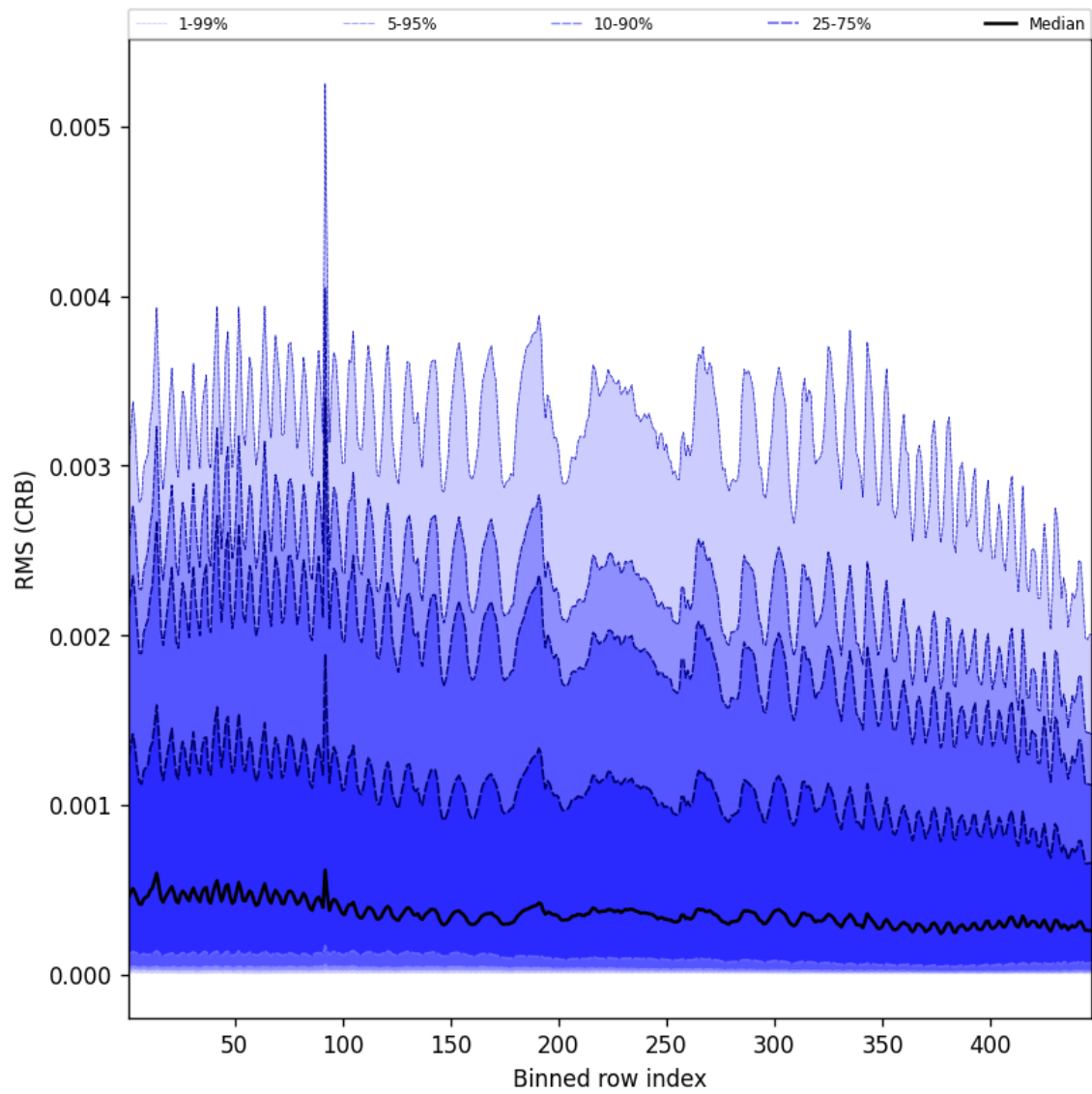
Figure 62: Along track statistics of “RMS (CRB)” for 2025-12-06 to 2025-12-07
