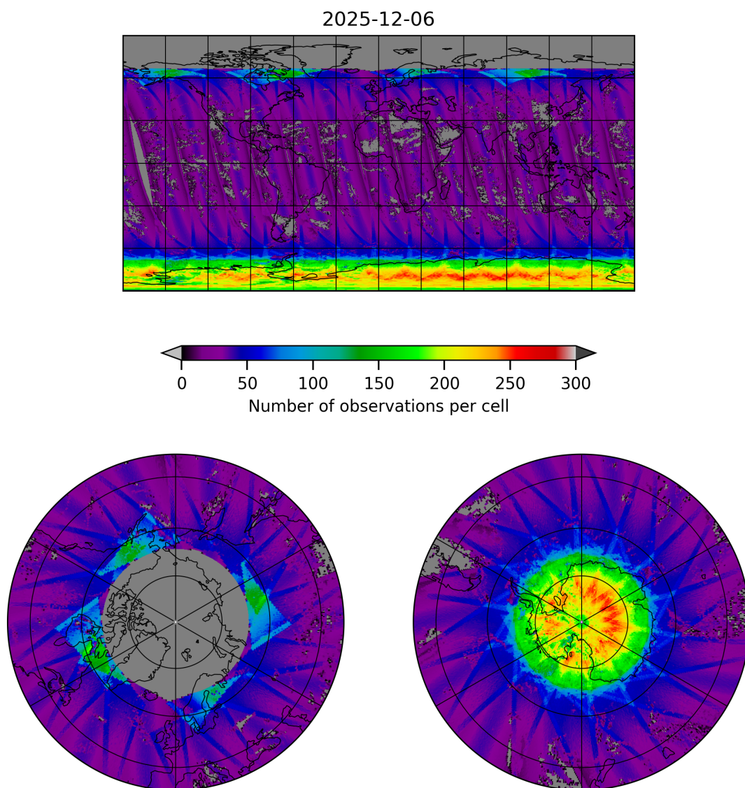
Figure 19: Map of the number of observations for 2025-12-06 to 2025-12-07
