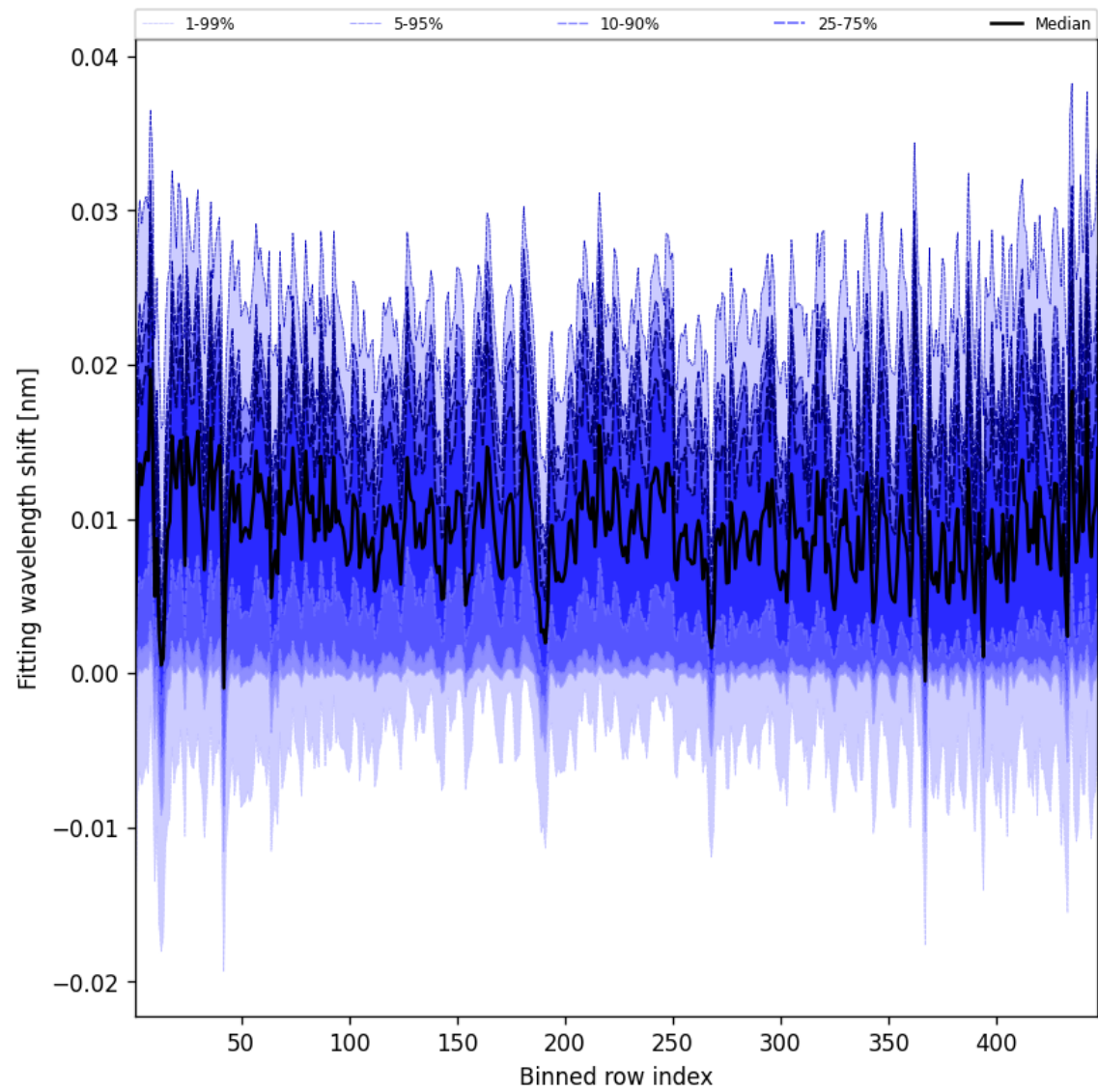
Figure 63: Along track statistics of “Fitting wavelength shift” for 2025-12-06 to 2025-12-07
