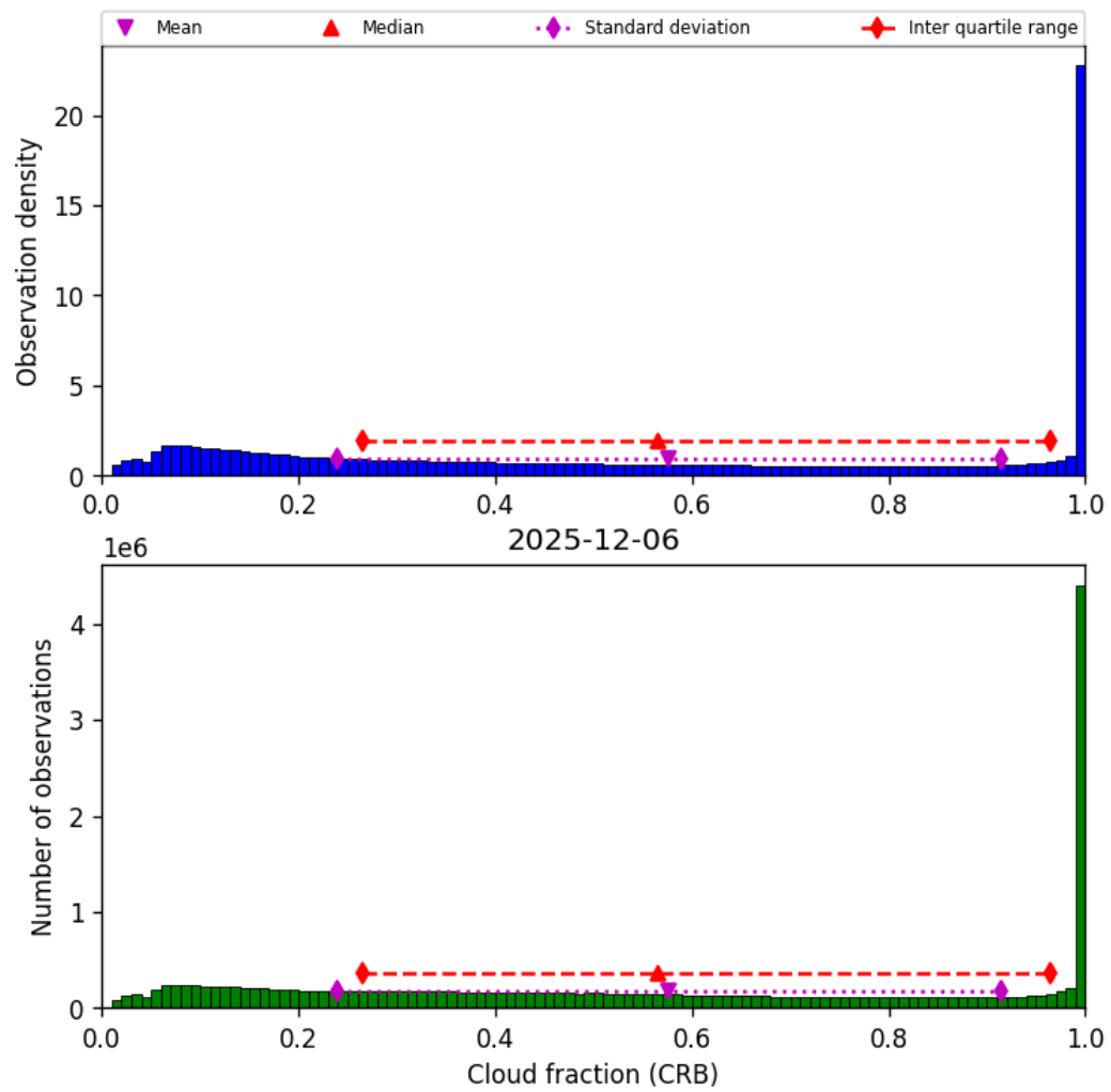
Figure 40: Histogram of “Cloud fraction (CRB)” for 2025-12-06 to 2025-12-07
