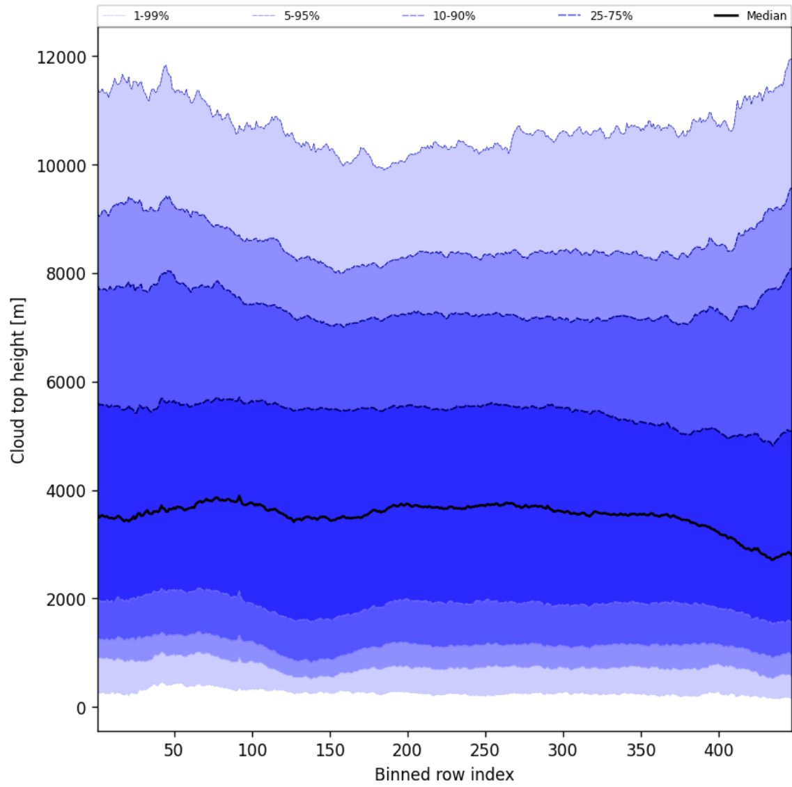
Figure 54: Along track statistics of “Cloud top height” for 2025-12-06 to 2025-12-07
