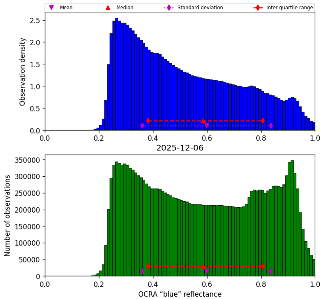
Figure 49: Histogram of “OCRA “blue” reflectance” for 2025-12-06 to 2025-12-07
