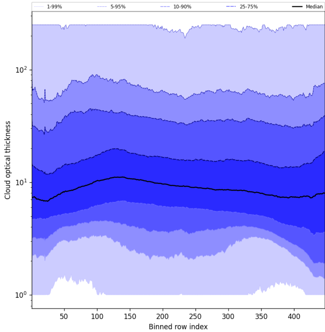
Figure 55: Along track statistics of “Cloud optical thickness” for 2025-12-06 to 2025-12-07
