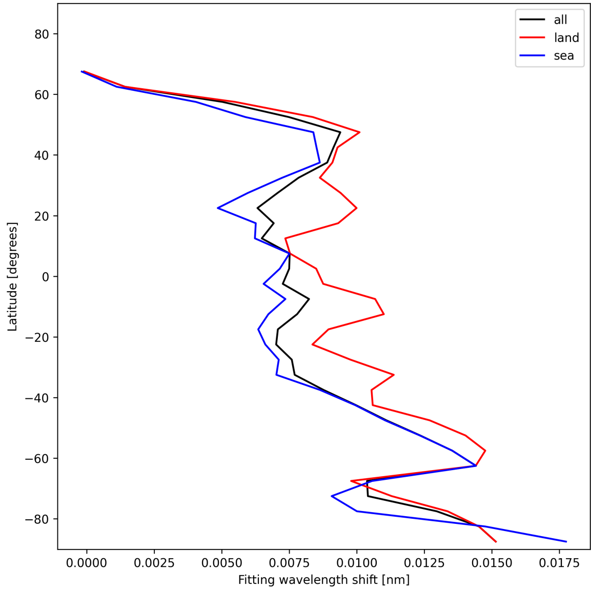
Figure 31: Zonal average of “Fitting wavelength shift” for 2025-12-06 to 2025-12-07.
