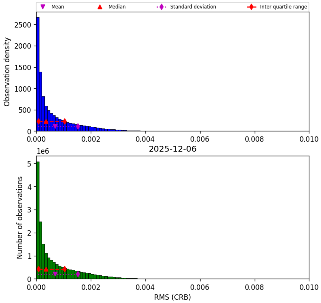
Figure 46: Histogram of “RMS (CRB)” for 2025-12-06 to 2025-12-07
