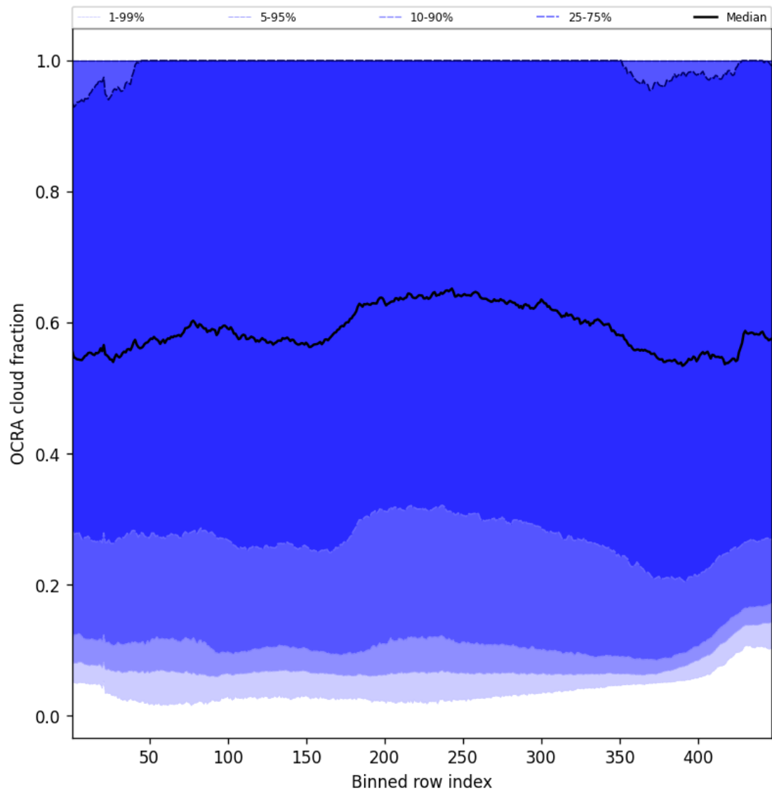
Figure 64: Along track statistics of “OCRA cloud fraction” for 2025-12-06 to 2025-12-07
