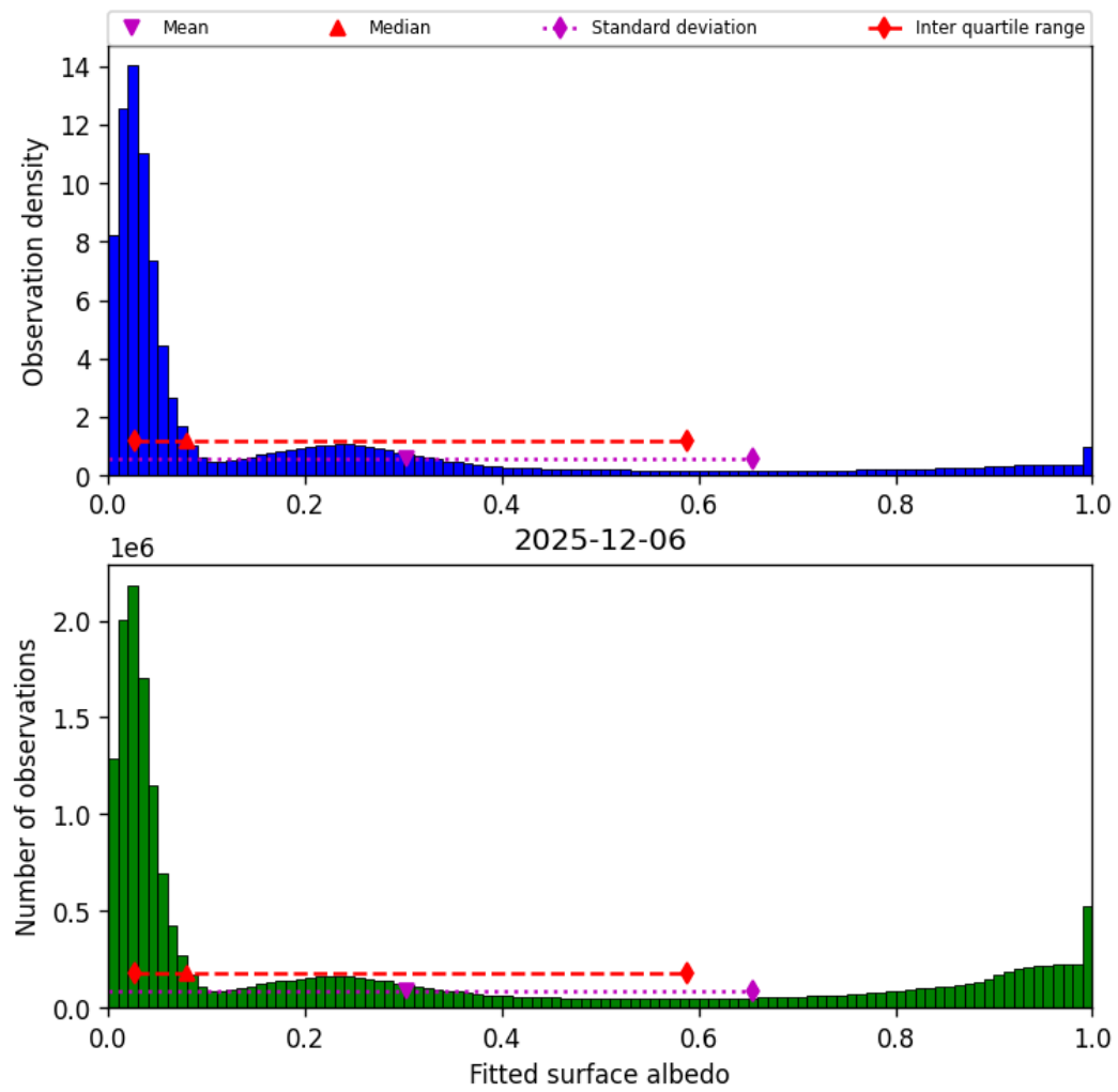
Figure 43: Histogram of “Fitted surface albedo” for 2025-12-06 to 2025-12-07
