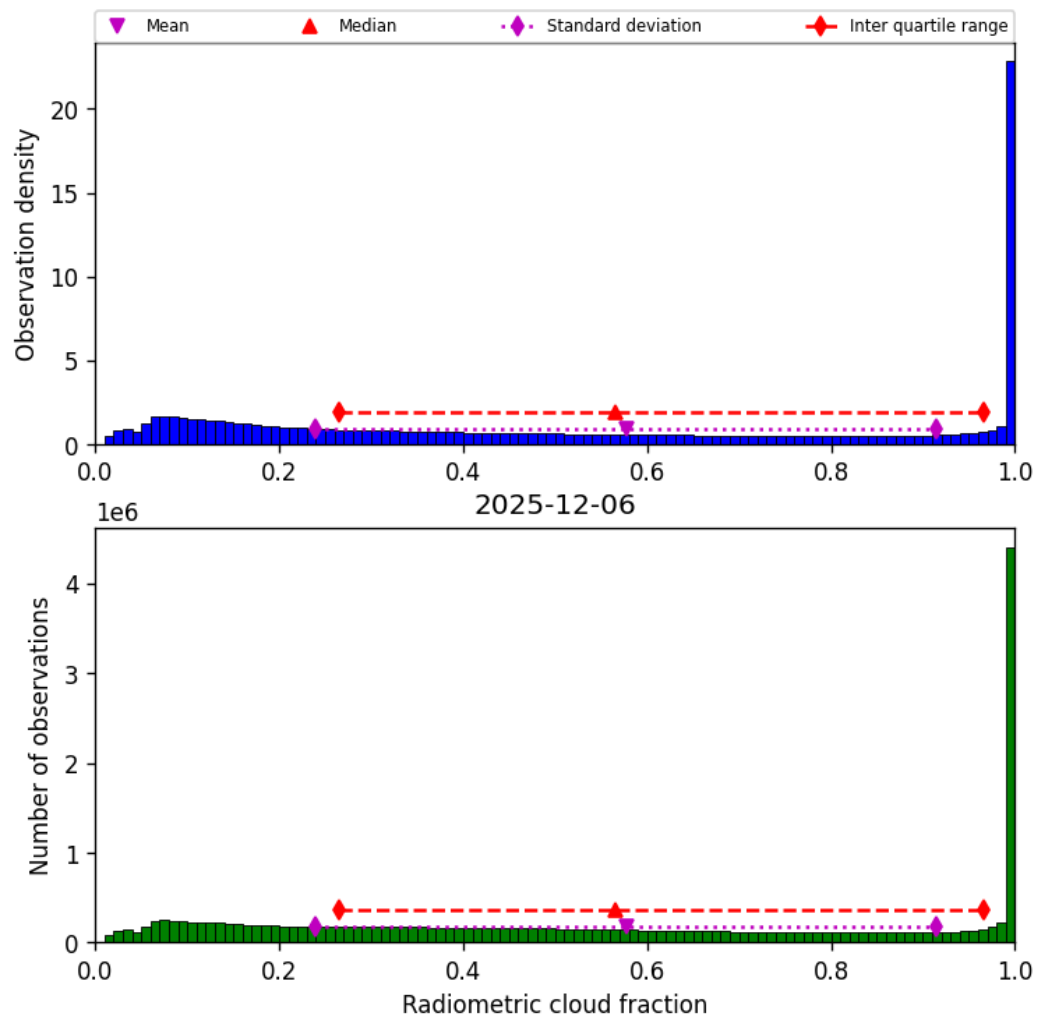
Figure 37: Histogram of “Radiometric cloud fraction” for 2025-12-06 to 2025-12-07
