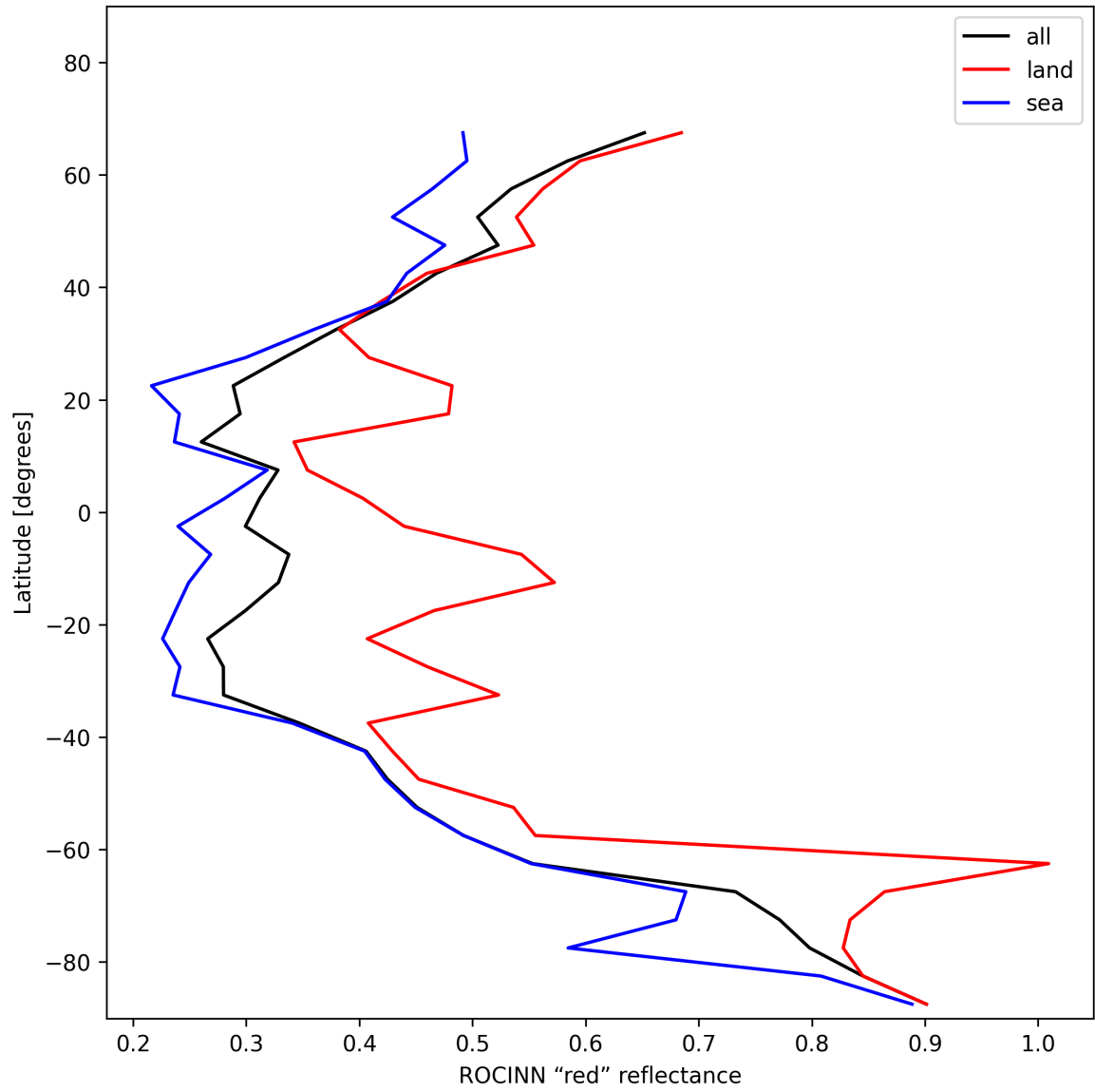
Figure 35: Zonal average of “ROCINN “red” reflectance” for 2025-12-06 to 2025-12-07.
