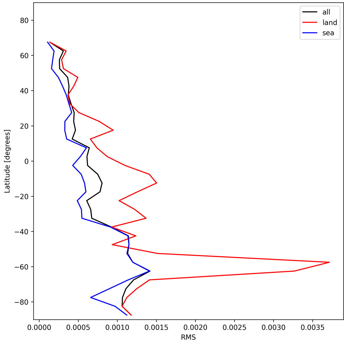
Figure 29: Zonal average of “RMS” for 2025-12-06 to 2025-12-07.
