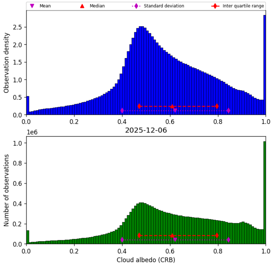
Figure 42: Histogram of “Cloud albedo (CRB)” for 2025-12-06 to 2025-12-07
