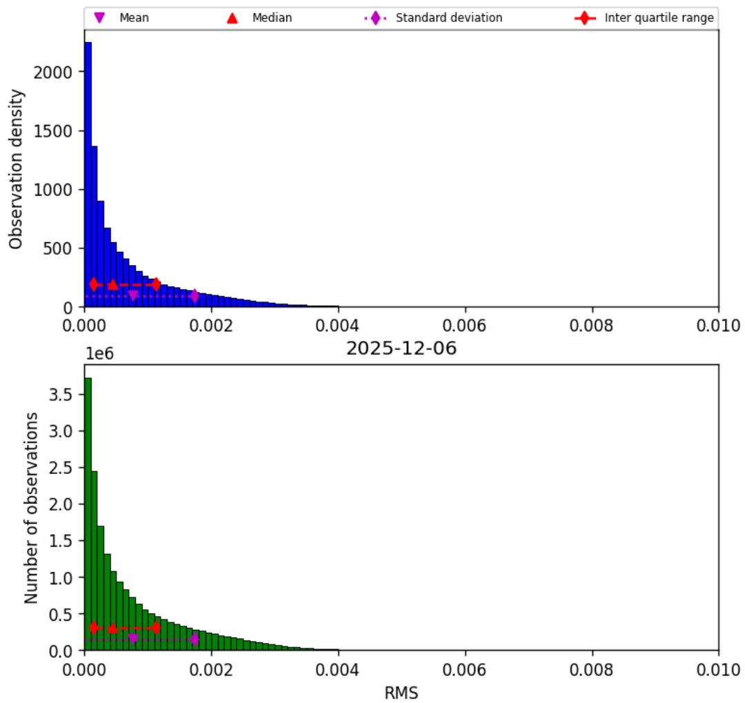
Figure 45: Histogram of “RMS” for 2025-12-06 to 2025-12-07
