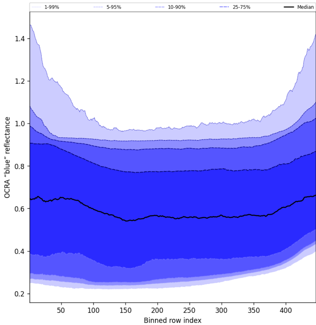
Figure 65: Along track statistics of “OCRA “blue” reflectance” for 2025-12-06 to 2025-12-07
