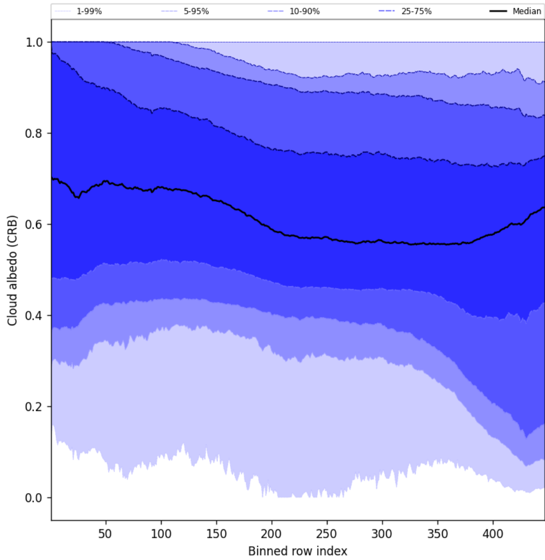
Figure 58: Along track statistics of “Cloud albedo (CRB)” for 2025-12-06 to 2025-12-07
