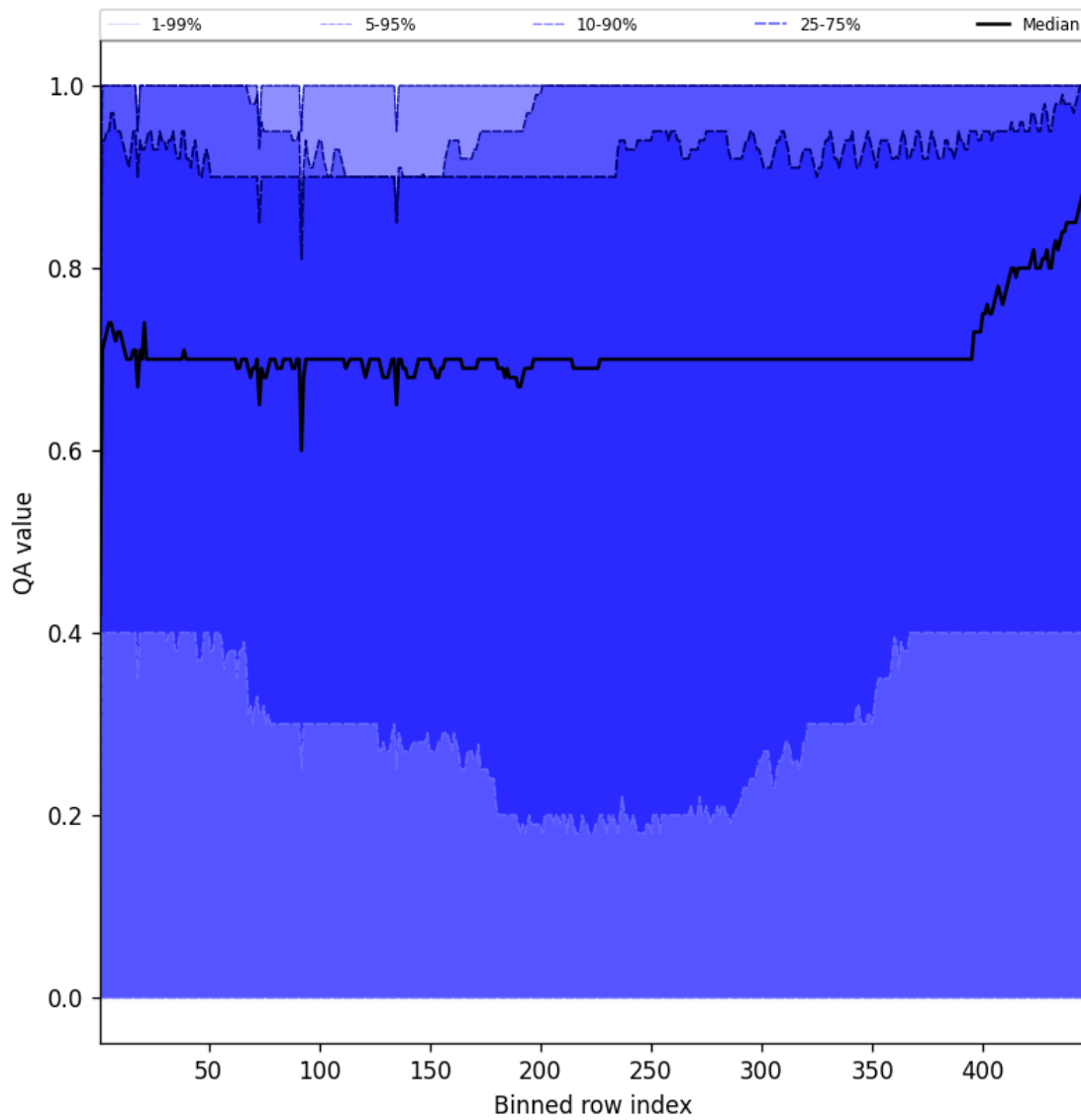
Figure 52: Along track statistics of “QA value” for 2025-12-06 to 2025-12-07
