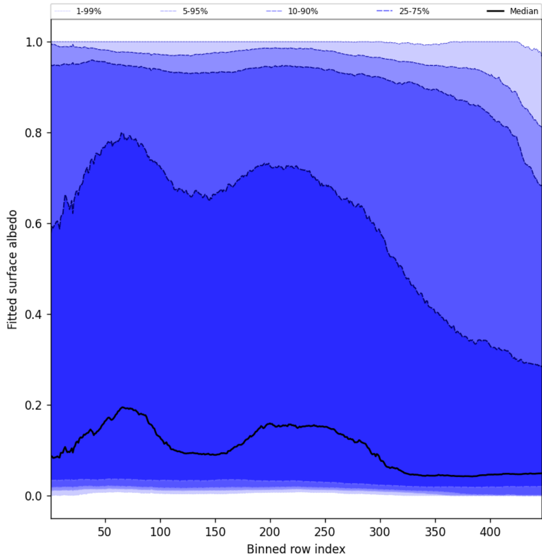
Figure 59: Along track statistics of “Fitted surface albedo” for 2025-12-06 to 2025-12-07
