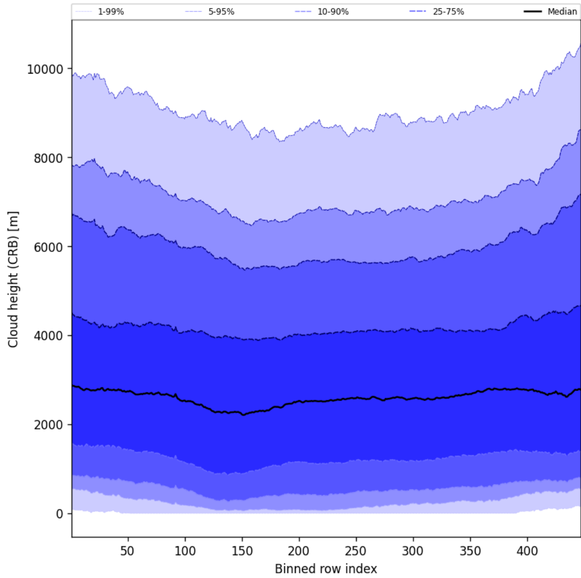
Figure 57: Along track statistics of “Cloud height (CRB)” for 2025-12-06 to 2025-12-07
