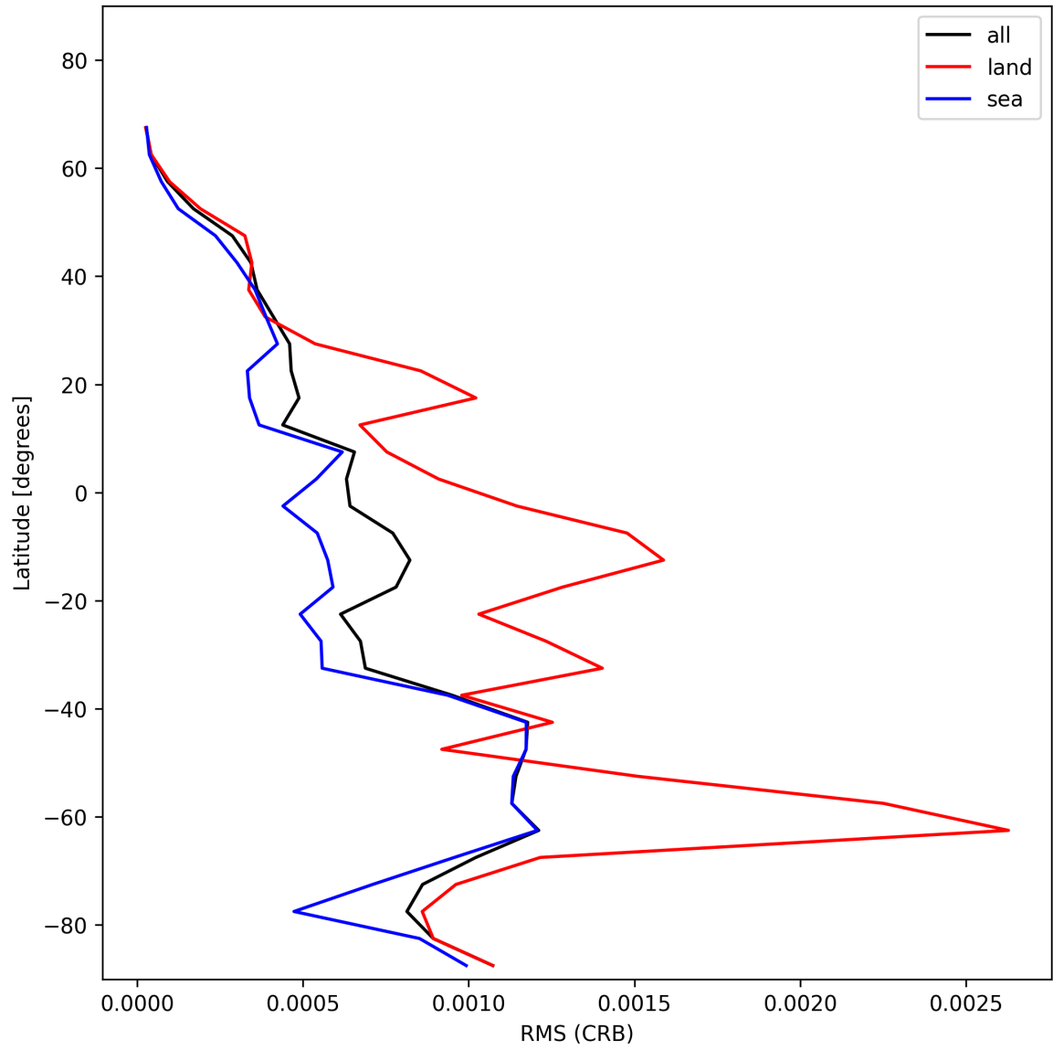
Figure 30: Zonal average of “RMS (CRB)” for 2025-12-06 to 2025-12-07.
