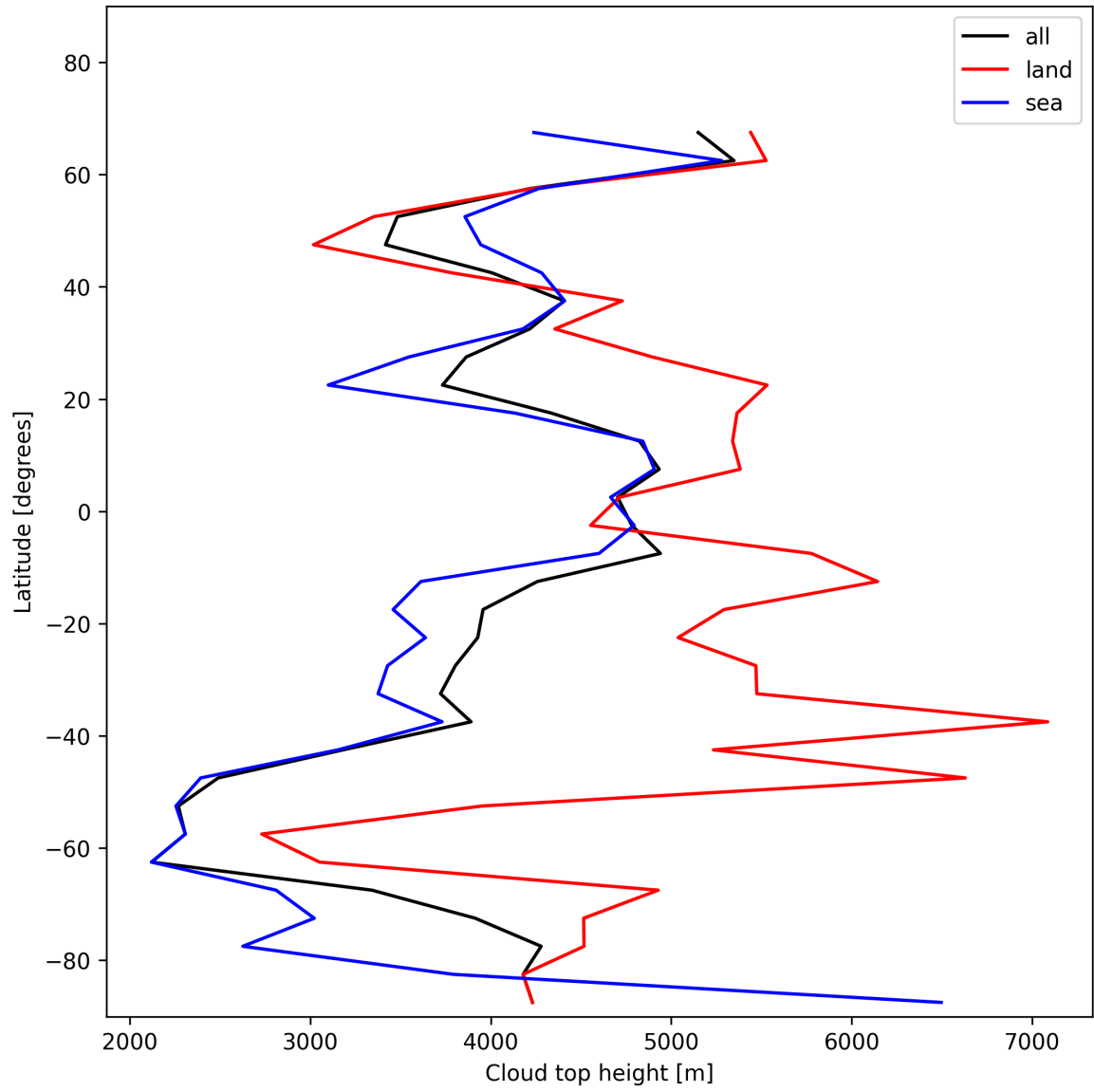
Figure 22: Zonal average of “Cloud top height” for 2025-12-06 to 2025-12-07.
