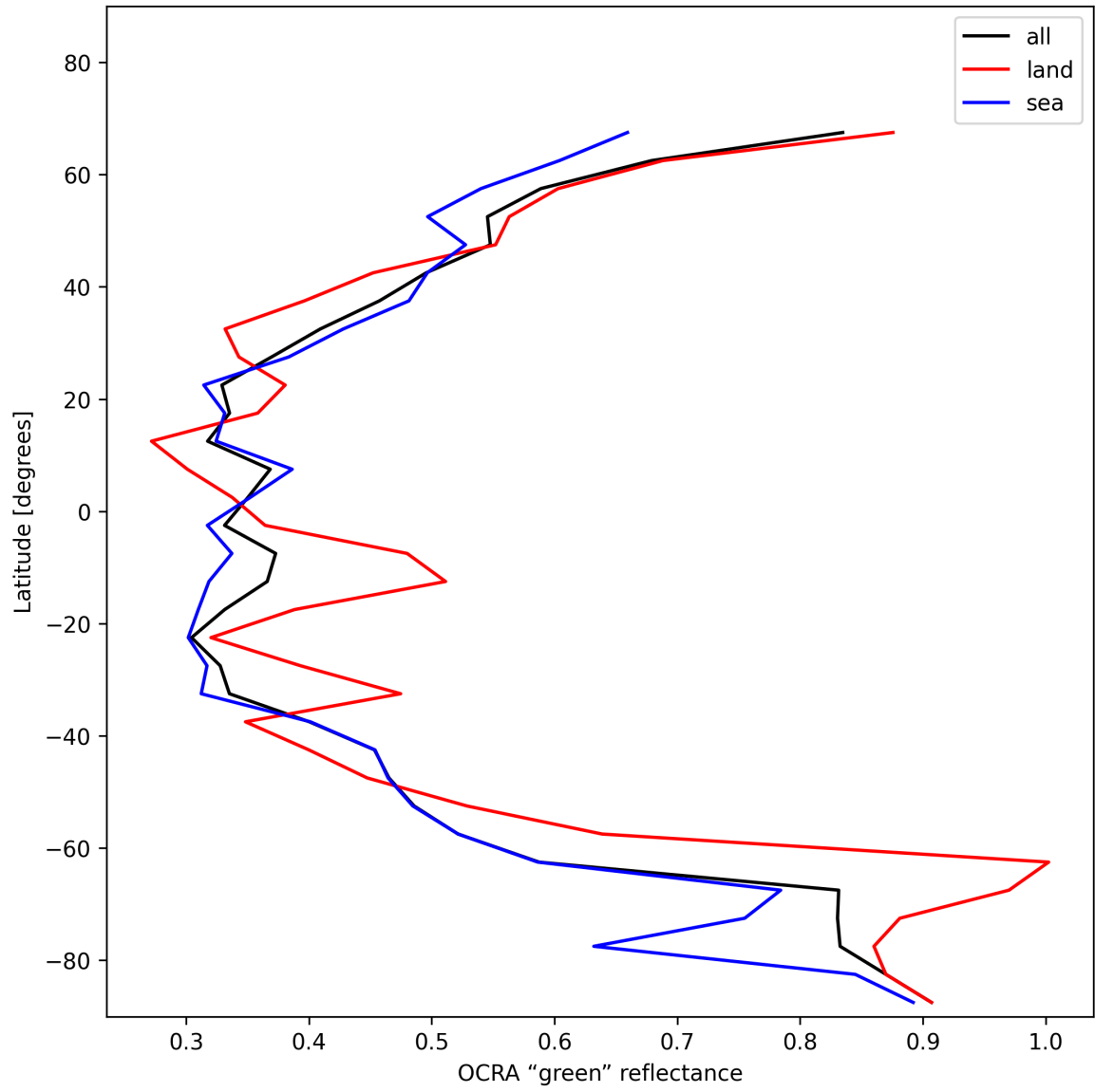
Figure 34: Zonal average of “OCRA “green” reflectance” for 2025-12-06 to 2025-12-07.
