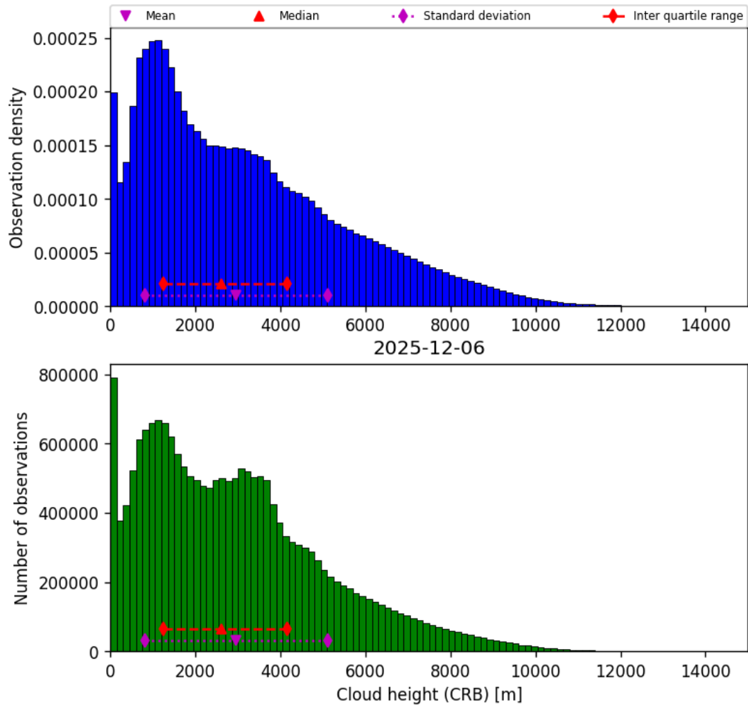
Figure 41: Histogram of “Cloud height (CRB)” for 2025-12-06 to 2025-12-07
