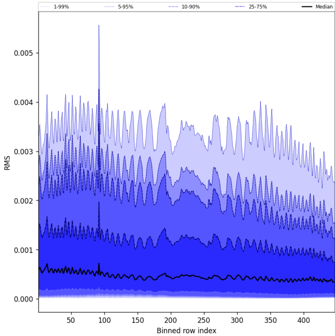
Figure 61: Along track statistics of “RMS” for 2025-12-06 to 2025-12-07
