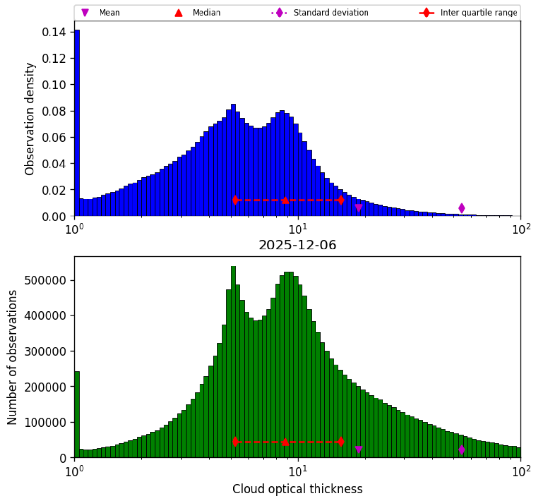
Figure 39: Histogram of “Cloud optical thickness” for 2025-12-06 to 2025-12-07
