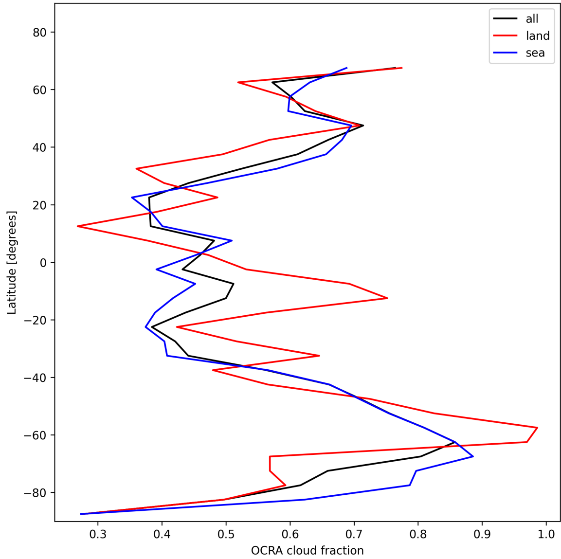
Figure 32: Zonal average of “OCRA cloud fraction” for 2025-12-06 to 2025-12-07.
