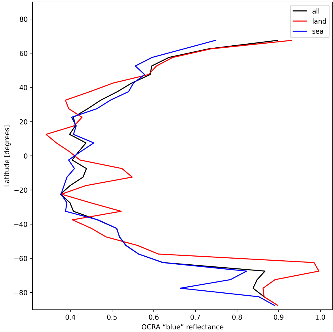
Figure 33: Zonal average of “OCRA “blue” reflectance” for 2025-12-06 to 2025-12-07.
