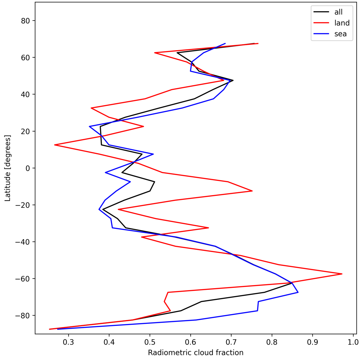
Figure 21: Zonal average of “Radiometric cloud fraction” for 2025-12-06 to 2025-12-07.
