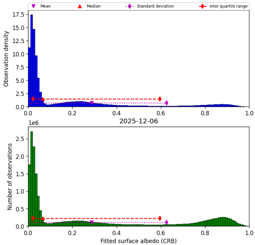
Figure 44: Histogram of “Fitted surface albedo (CRB)” for 2025-12-06 to 2025-12-07
