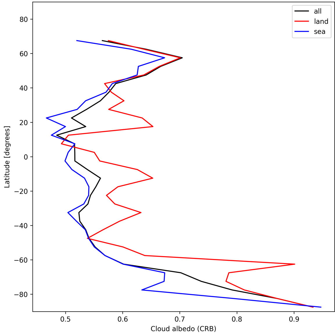
Figure 26: Zonal average of “Cloud albedo (CRB)” for 2025-12-06 to 2025-12-07.
