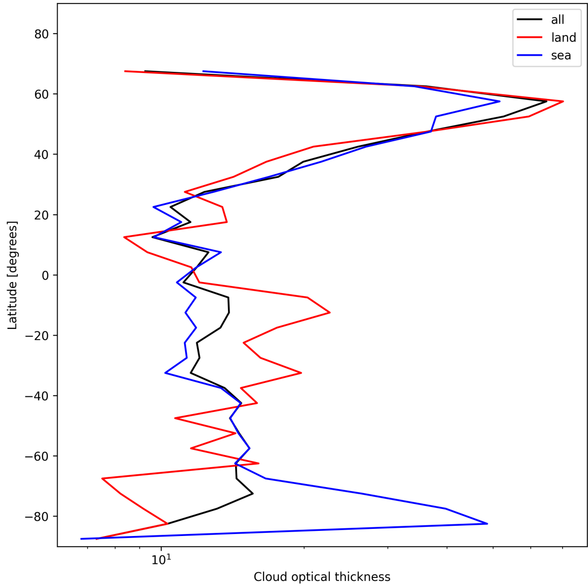
Figure 23: Zonal average of “Cloud optical thickness” for 2025-12-06 to 2025-12-07.
