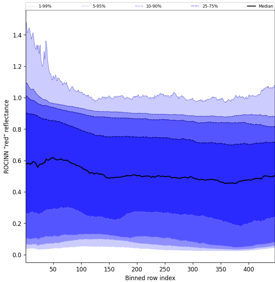
Figure 67: Along track statistics of "ROCINN "red" reflectance" for 2025-12-06 to 2025-12-07
