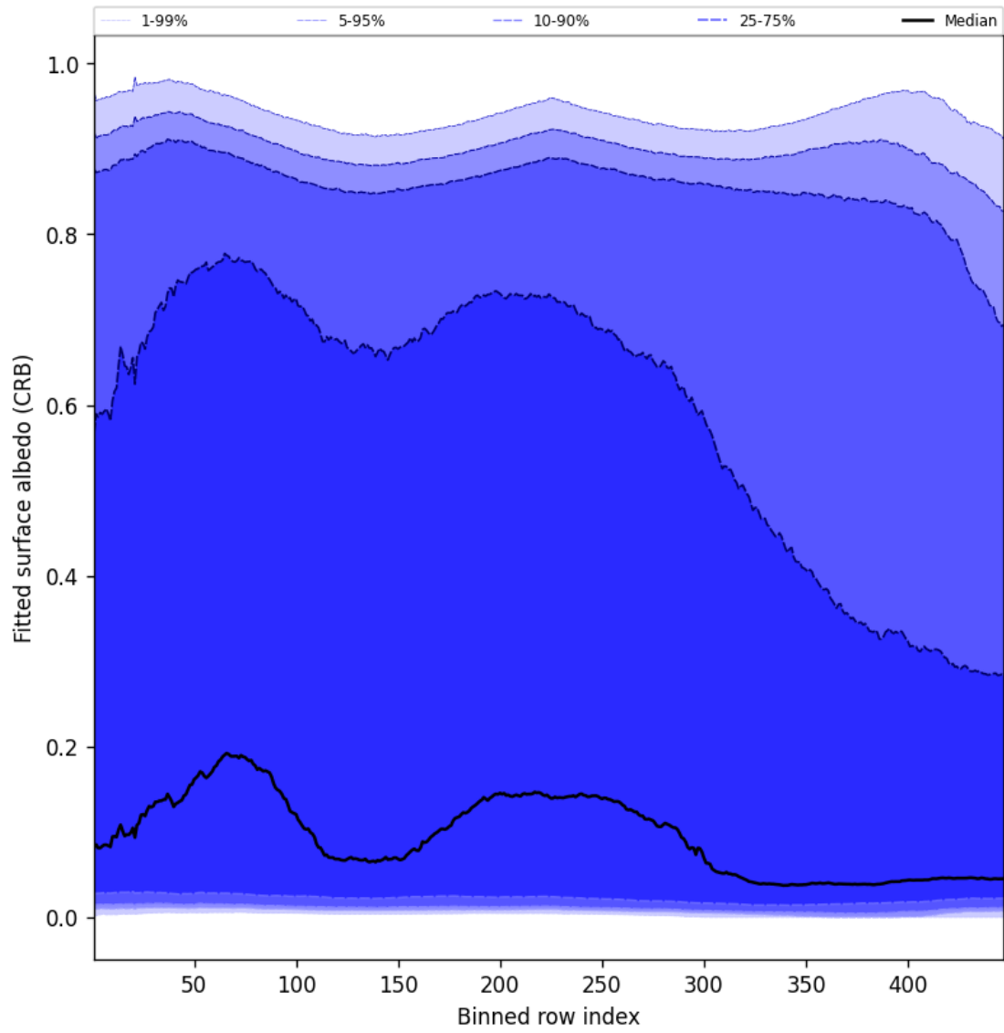
Figure 60: Along track statistics of “Fitted surface albedo (CRB)” for 2025-12-06 to 2025-12-07
