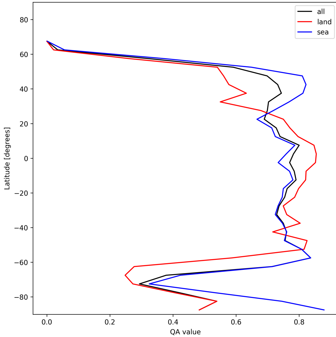
Figure 20: Zonal average of “QA value” for 2025-12-06 to 2025-12-07.
