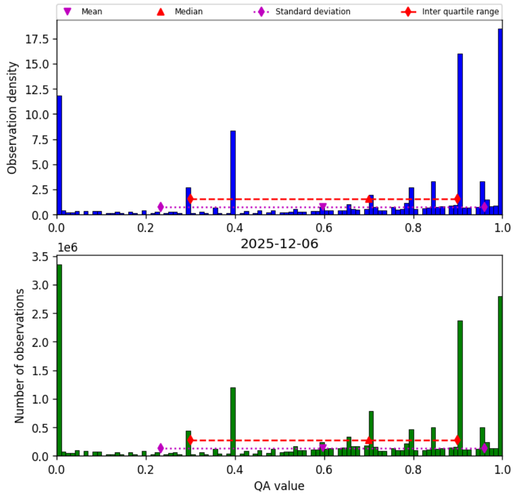
Figure 36: Histogram of “QA value” for 2025-12-06 to 2025-12-07
