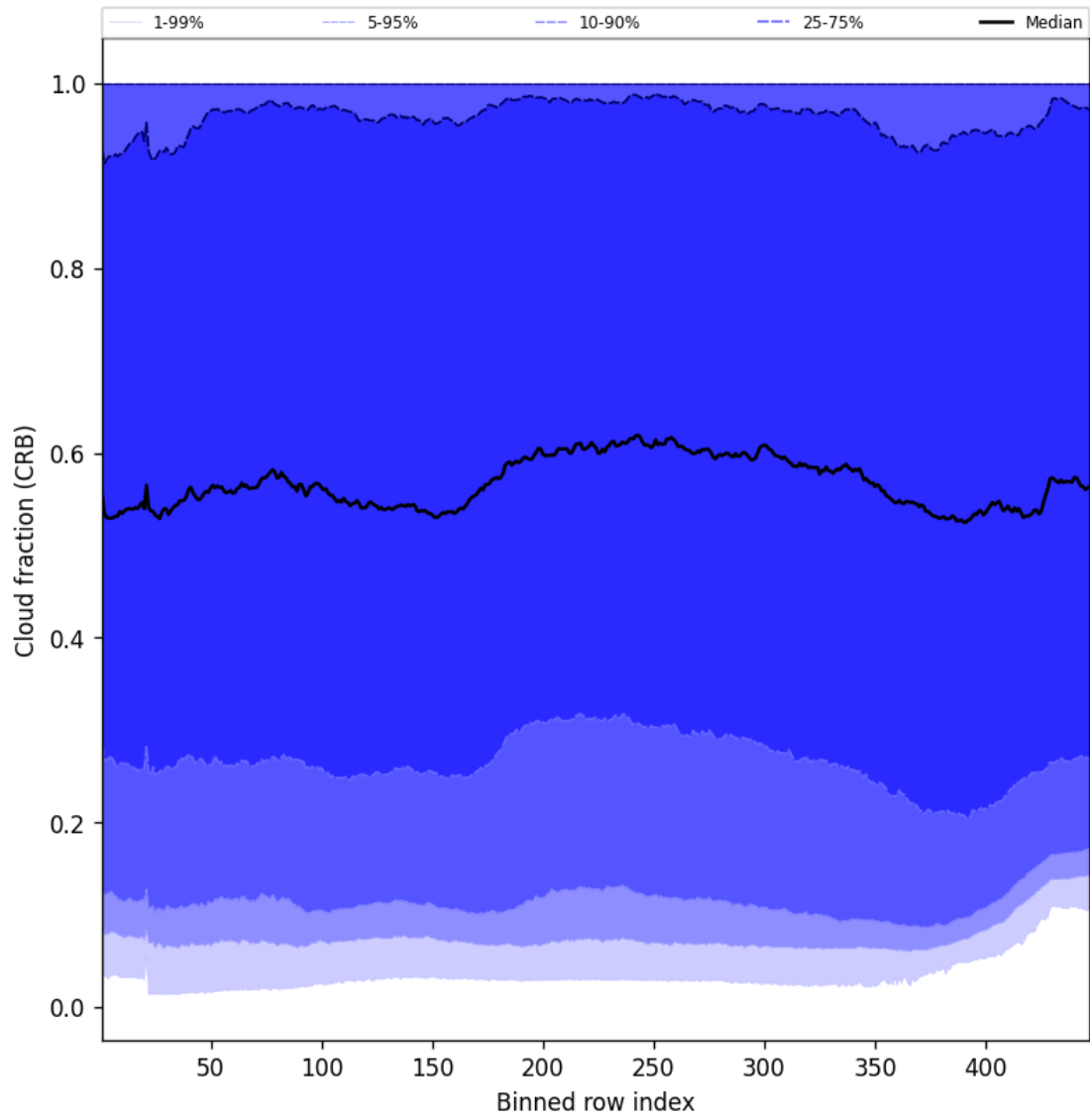
Figure 56: Along track statistics of “Cloud fraction (CRB)” for 2025-12-06 to 2025-12-07
