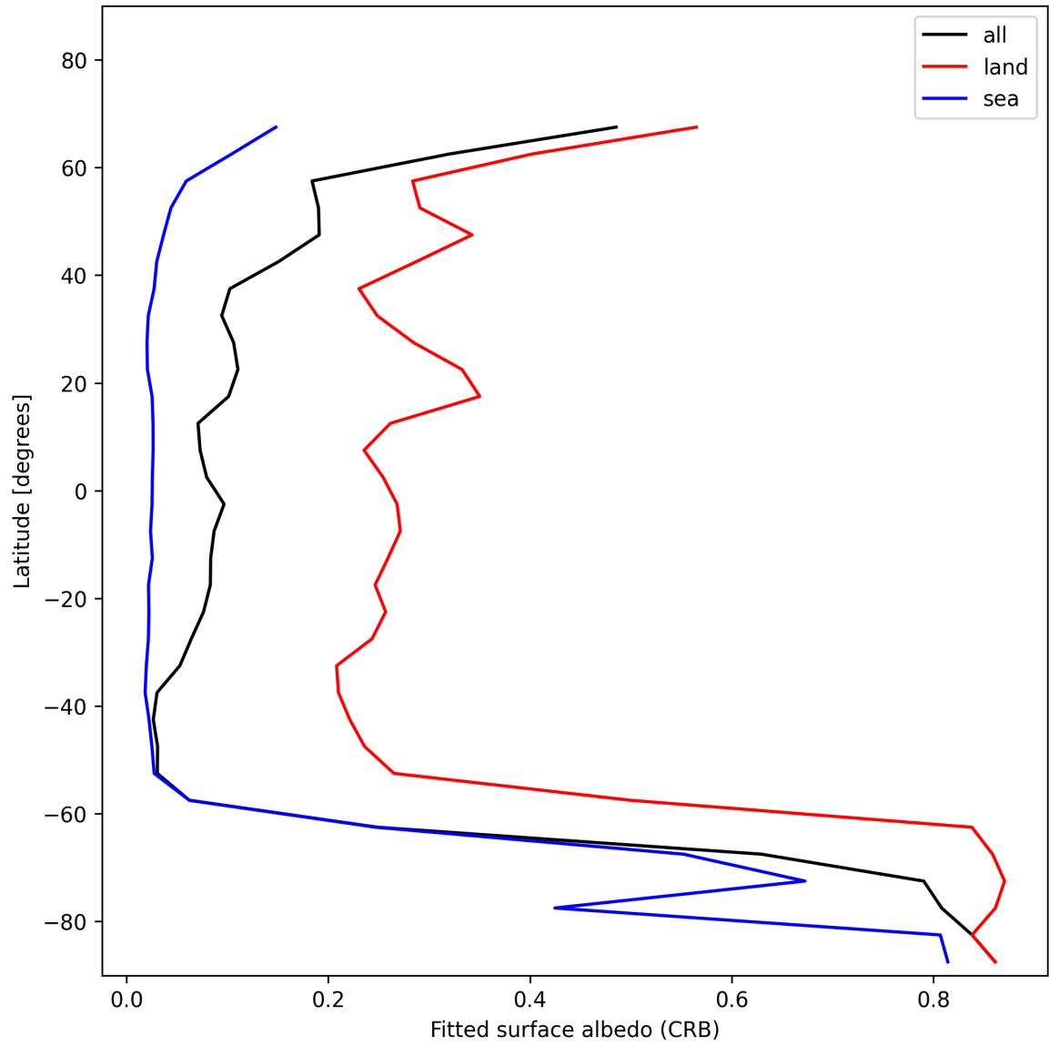
Figure 28: Zonal average of “Fitted surface albedo (CRB)” for 2025-12-06 to 2025-12-07.
