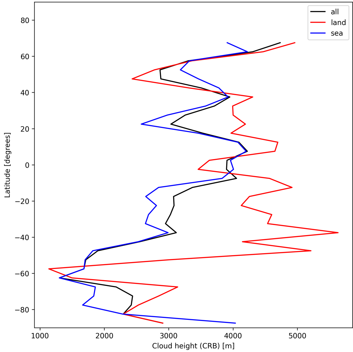
Figure 25: Zonal average of “Cloud height (CRB)” for 2025-12-06 to 2025-12-07.
