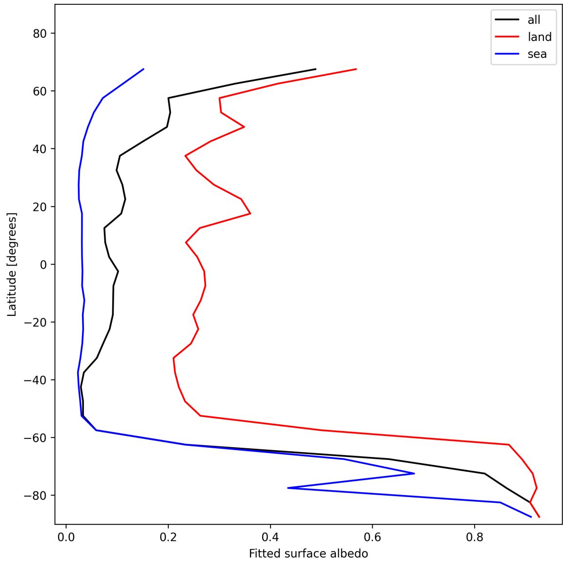
Figure 27: Zonal average of “Fitted surface albedo” for 2025-12-06 to 2025-12-07.
