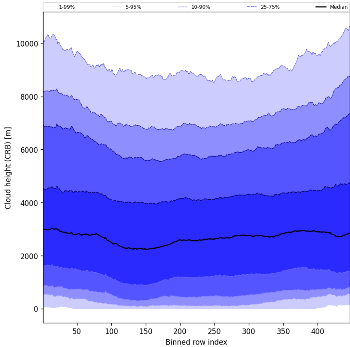
Figure 57: Along track statistics of “Cloud height (CRB)” for 2025-12-07 to 2025-12-07
