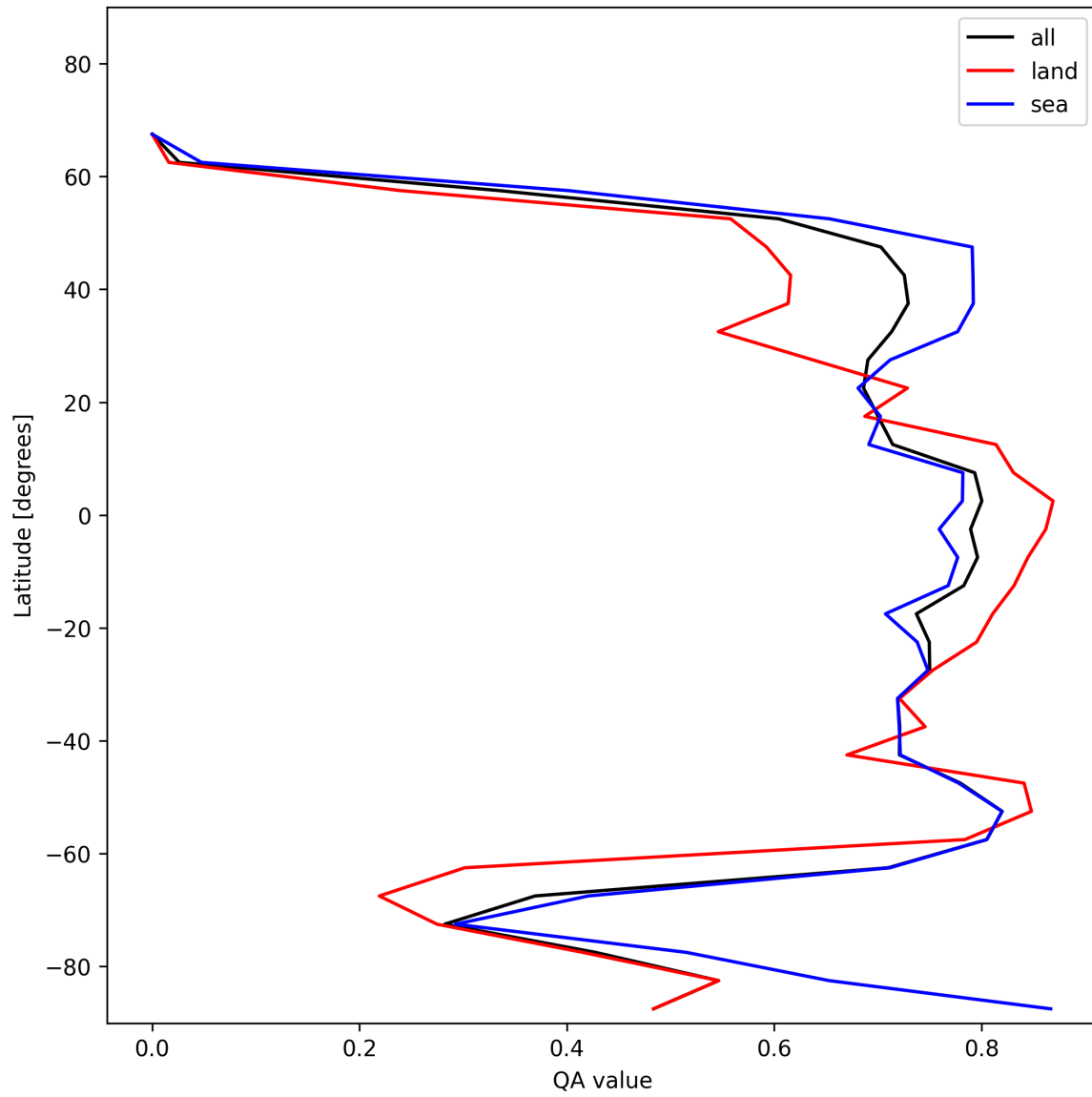
Figure 20: Zonal average of “QA value” for 2025-12-07 to 2025-12-07.
