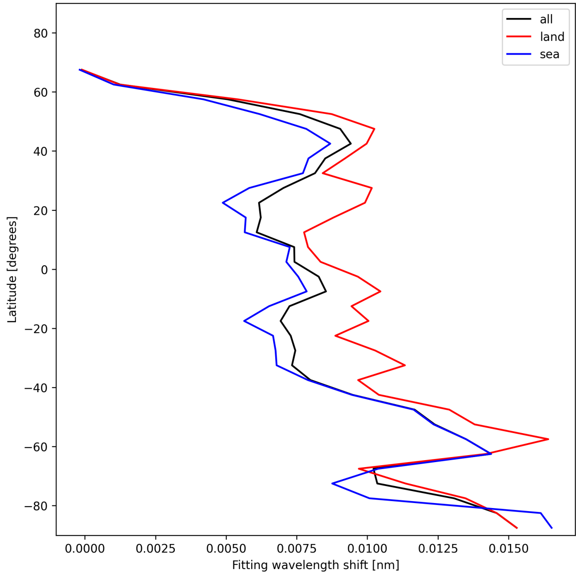
Figure 31: Zonal average of “Fitting wavelength shift” for 2025-12-07 to 2025-12-07.
