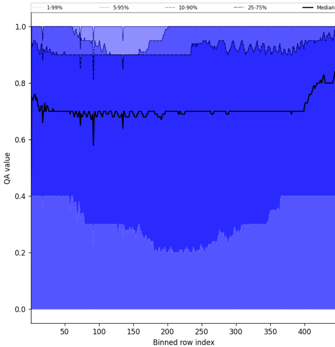
Figure 52: Along track statistics of “QA value” for 2025-12-07 to 2025-12-07
