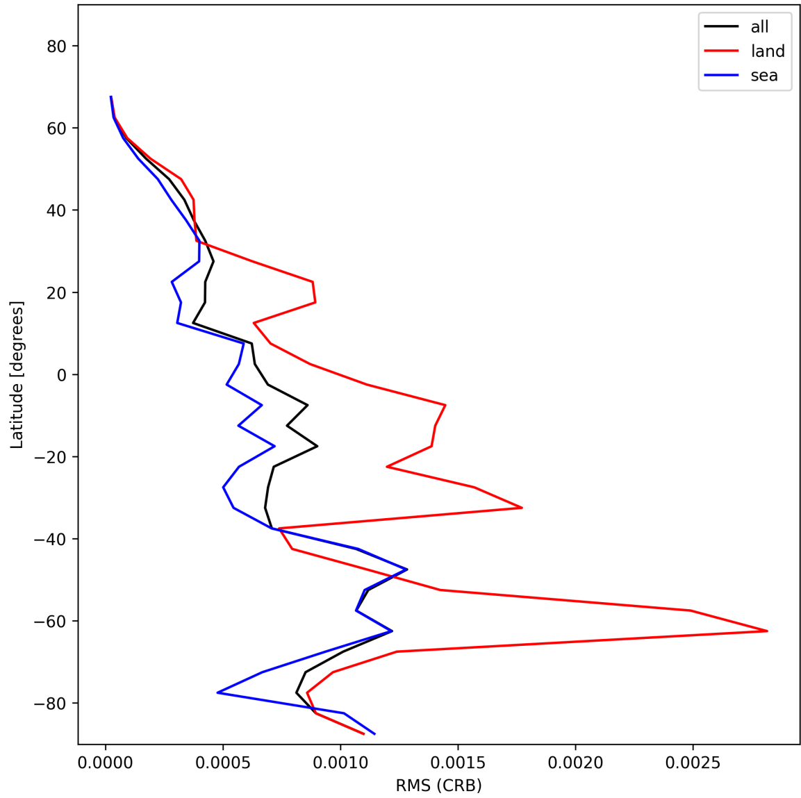
Figure 30: Zonal average of “RMS (CRB)” for 2025-12-07 to 2025-12-07.
