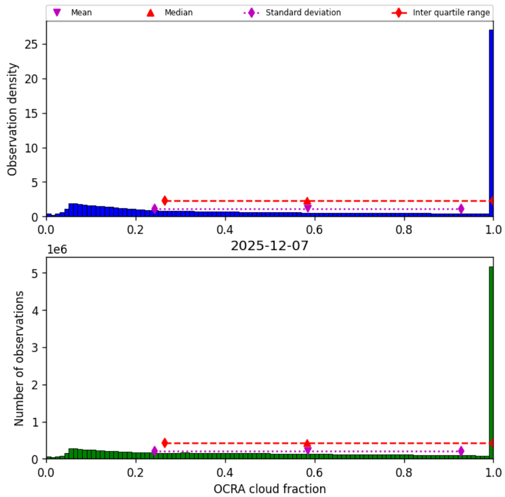
Figure 48: Histogram of “OCRA cloud fraction” for 2025-12-07 to 2025-12-07
