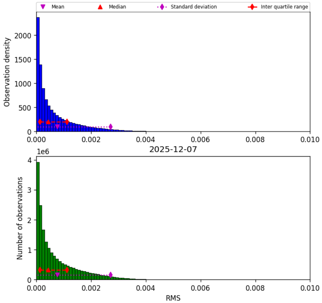
Figure 45: Histogram of “RMS” for 2025-12-07 to 2025-12-07
