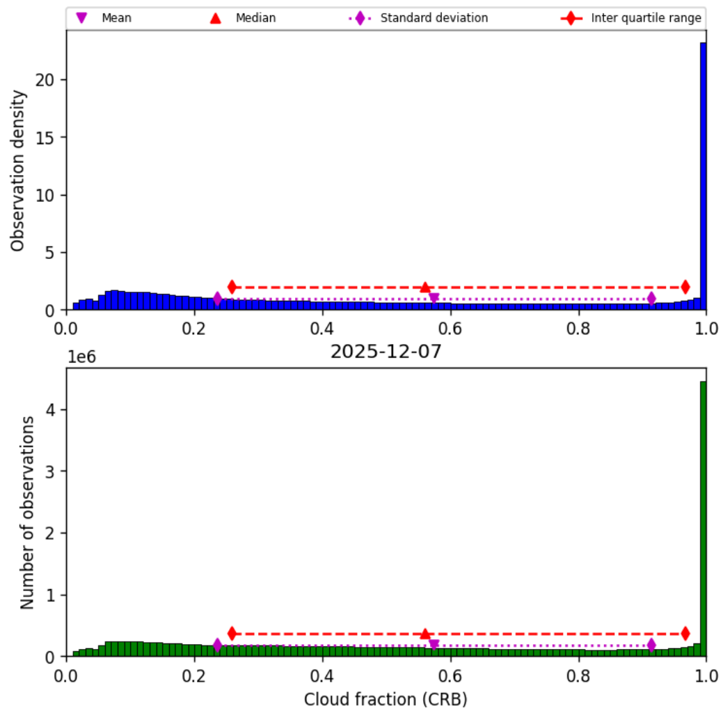
Figure 40: Histogram of “Cloud fraction (CRB)” for 2025-12-07 to 2025-12-07
