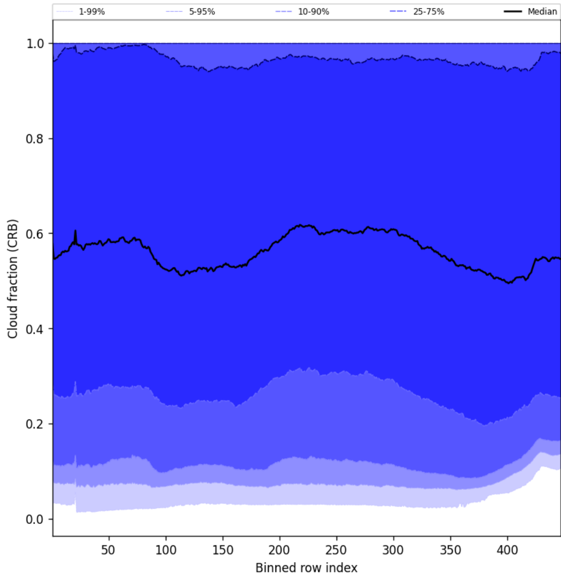
Figure 56: Along track statistics of “Cloud fraction (CRB)” for 2025-12-07 to 2025-12-07
