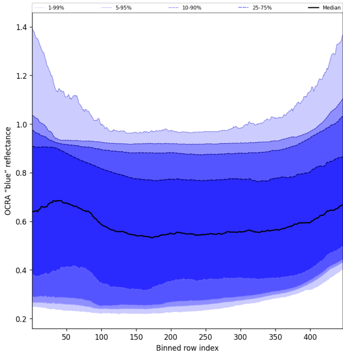
Figure 65: Along track statistics of "OCRA "blue" reflectance" for 2025-12-07 to 2025-12-07
