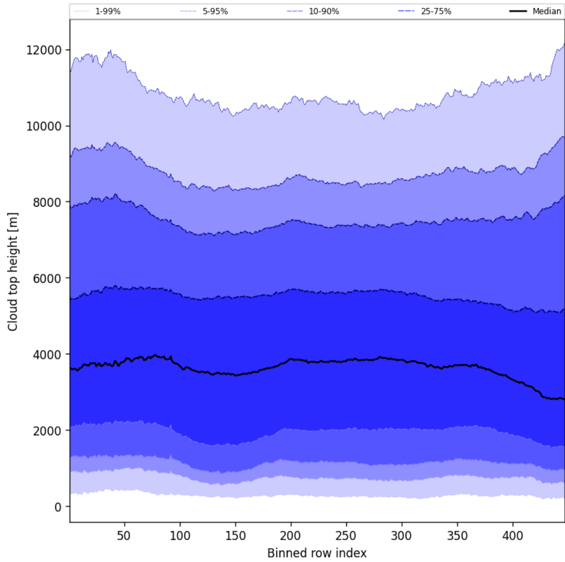
Figure 54: Along track statistics of “Cloud top height” for 2025-12-07 to 2025-12-07
