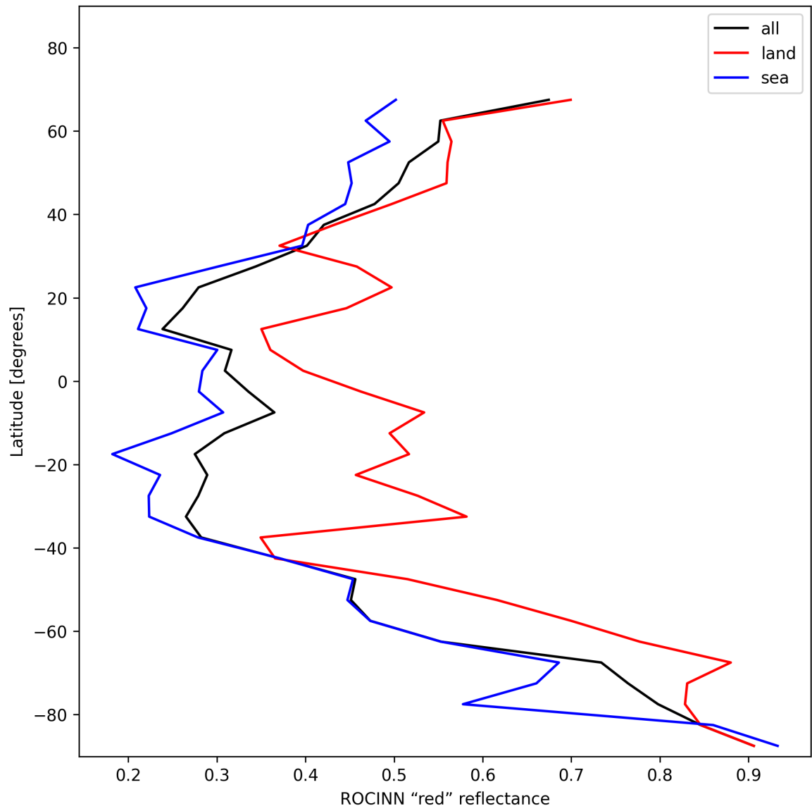
Figure 35: Zonal average of “ROCINN “red” reflectance” for 2025-12-07 to 2025-12-07.
