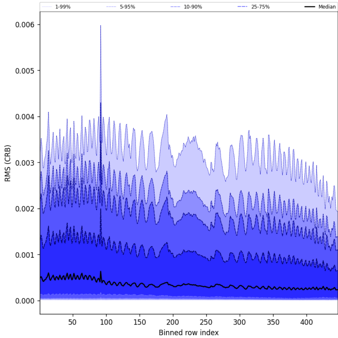
Figure 62: Along track statistics of “RMS (CRB)” for 2025-12-07 to 2025-12-07
