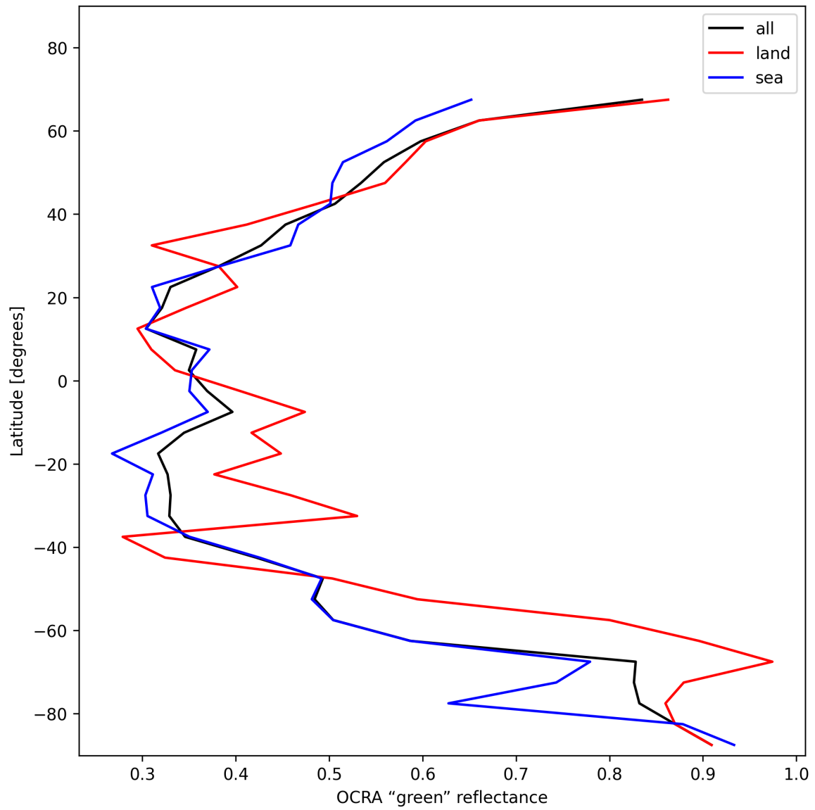
Figure 34: Zonal average of “OCRA “green” reflectance” for 2025-12-07 to 2025-12-07.
