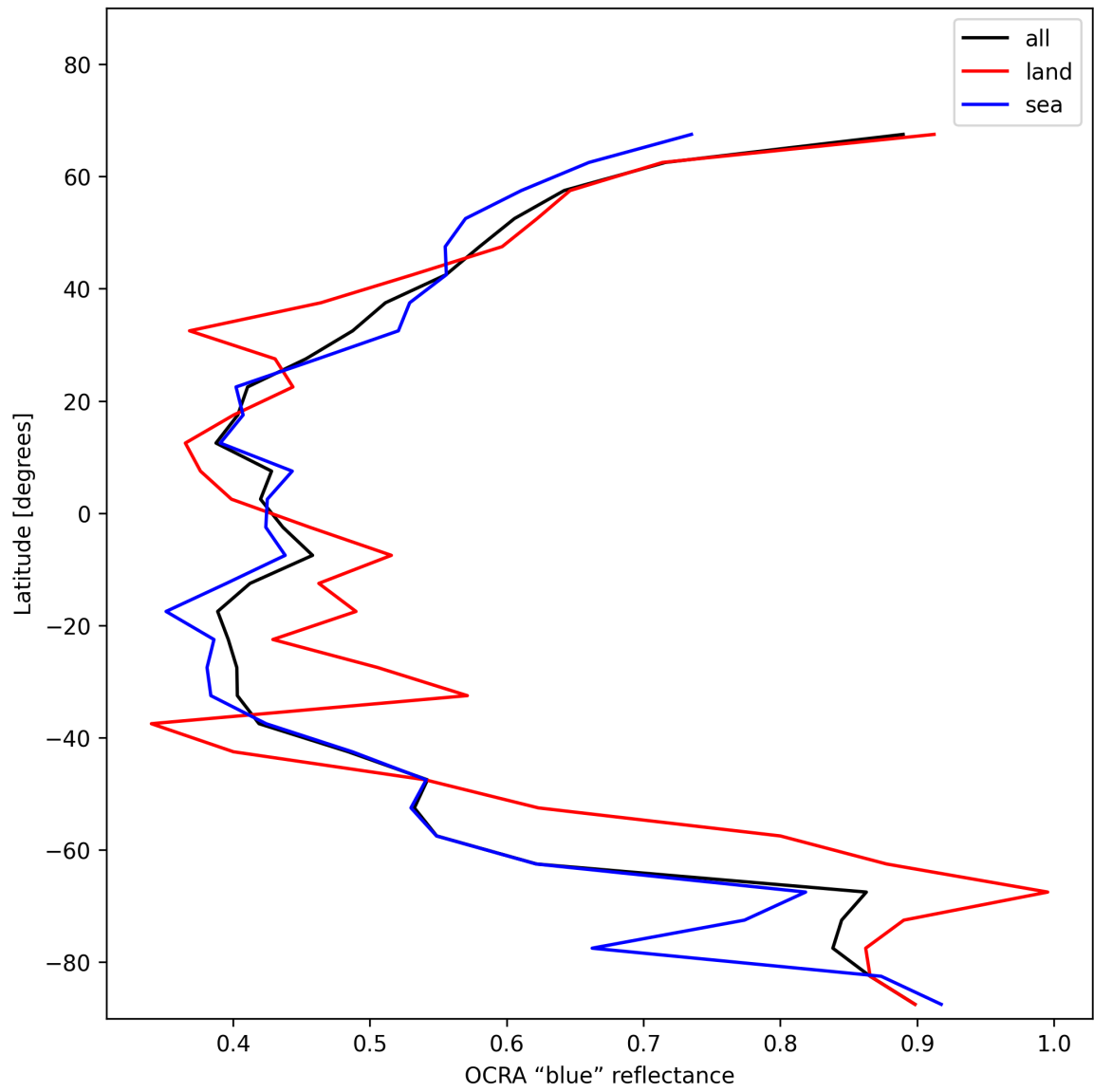
Figure 33: Zonal average of “OCRA “blue” reflectance” for 2025-12-07 to 2025-12-07.
