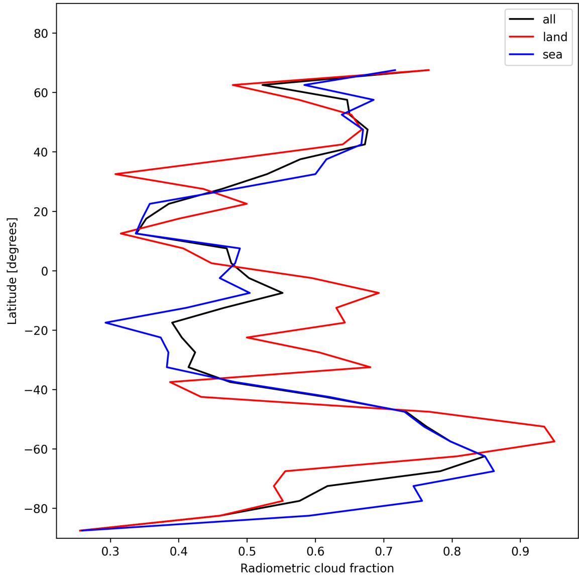
Figure 21: Zonal average of “Radiometric cloud fraction” for 2025-12-07 to 2025-12-07.
