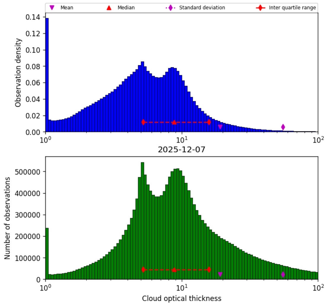
Figure 39: Histogram of “Cloud optical thickness” for 2025-12-07 to 2025-12-07
