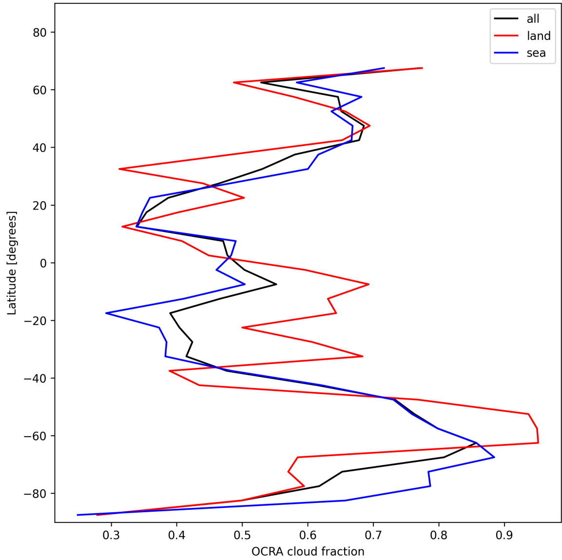
Figure 32: Zonal average of “OCRA cloud fraction” for 2025-12-07 to 2025-12-07.
