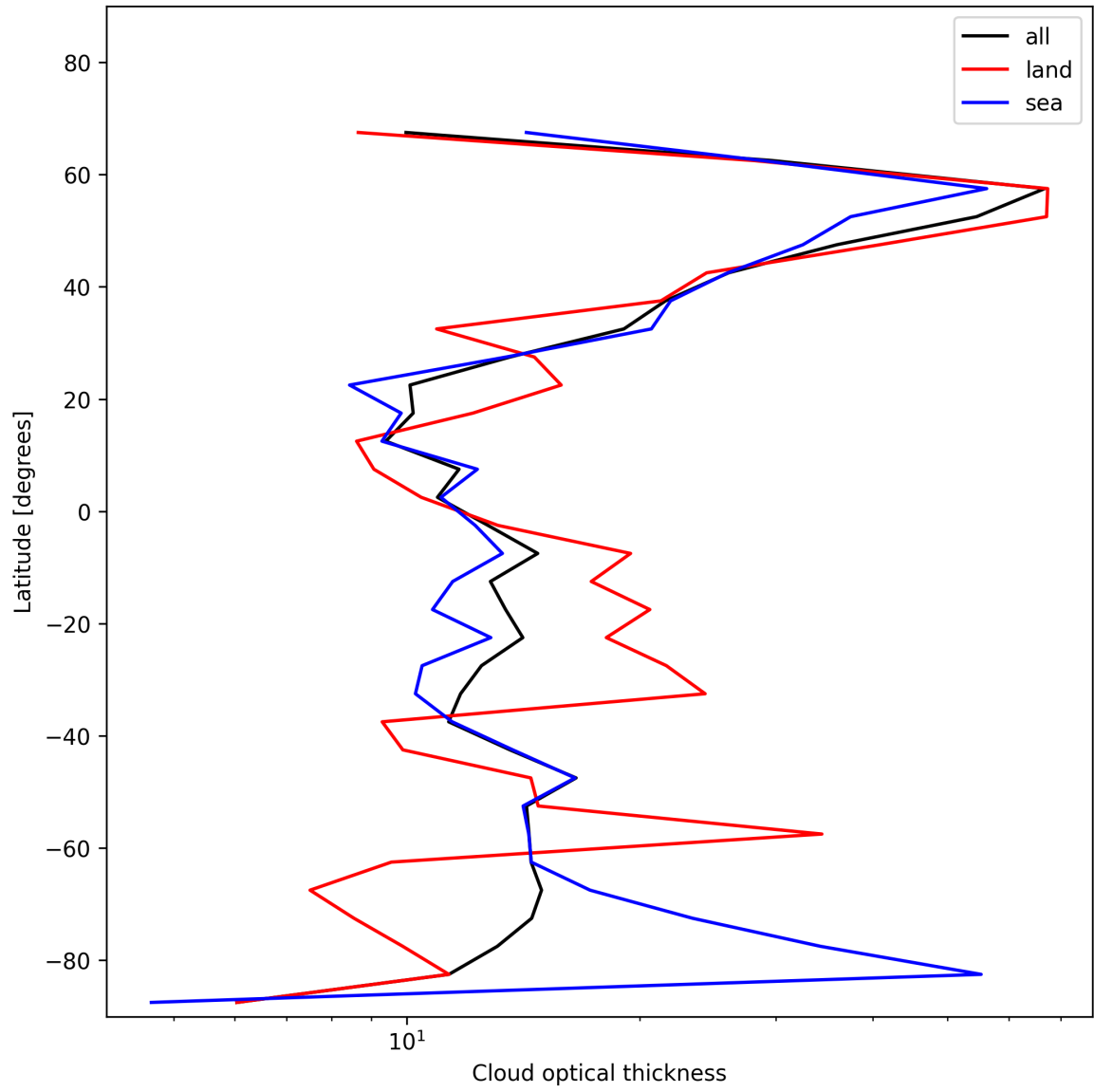
Figure 23: Zonal average of “Cloud optical thickness” for 2025-12-07 to 2025-12-07.
