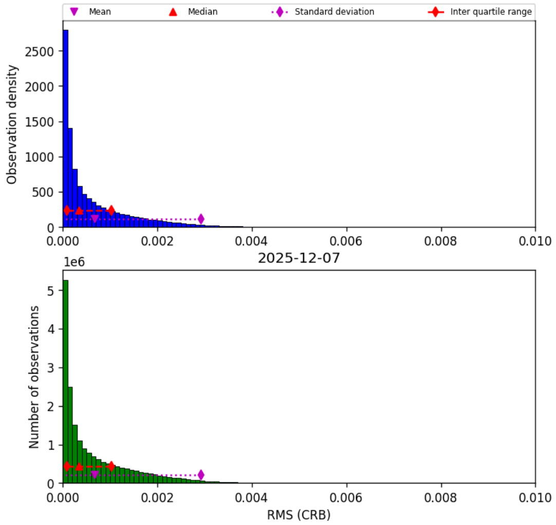
Figure 46: Histogram of “RMS (CRB)” for 2025-12-07 to 2025-12-07
