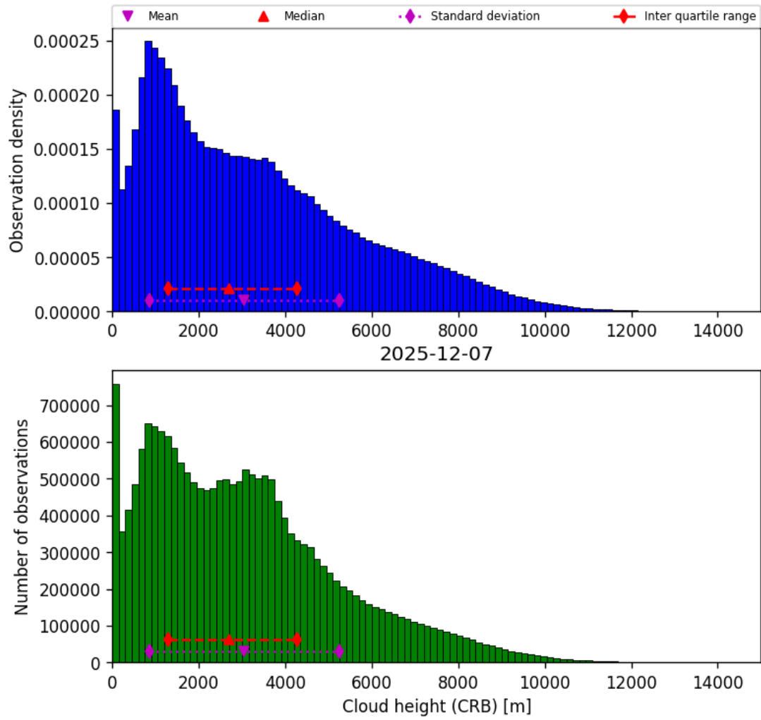
Figure 41: Histogram of “Cloud height (CRB)” for 2025-12-07 to 2025-12-07
