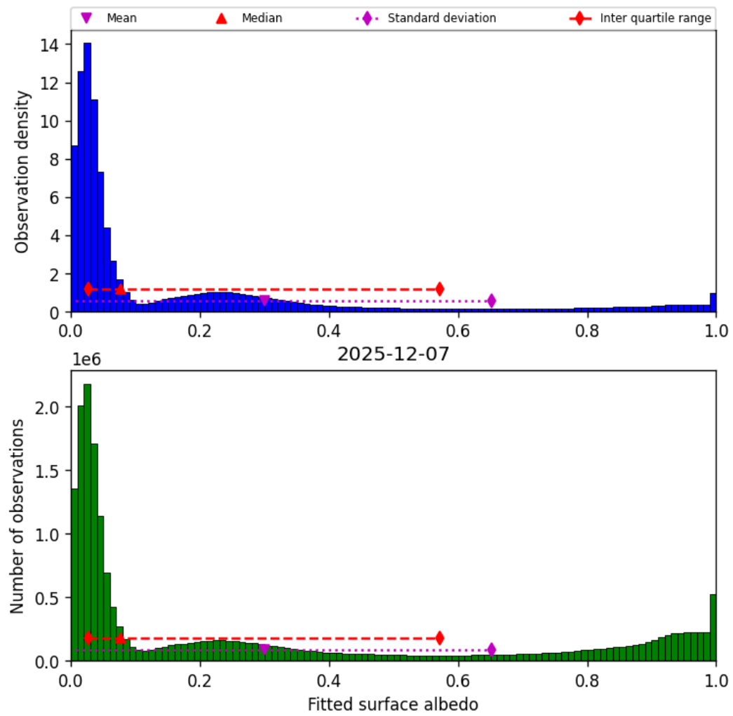
Figure 43: Histogram of “Fitted surface albedo” for 2025-12-07 to 2025-12-07
