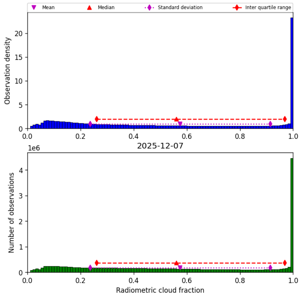
Figure 37: Histogram of “Radiometric cloud fraction” for 2025-12-07 to 2025-12-07
