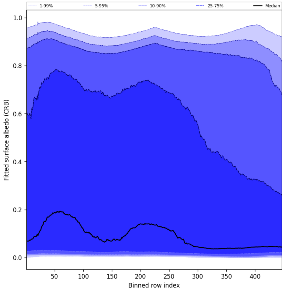
Figure 60: Along track statistics of “Fitted surface albedo (CRB)” for 2025-12-07 to 2025-12-07
