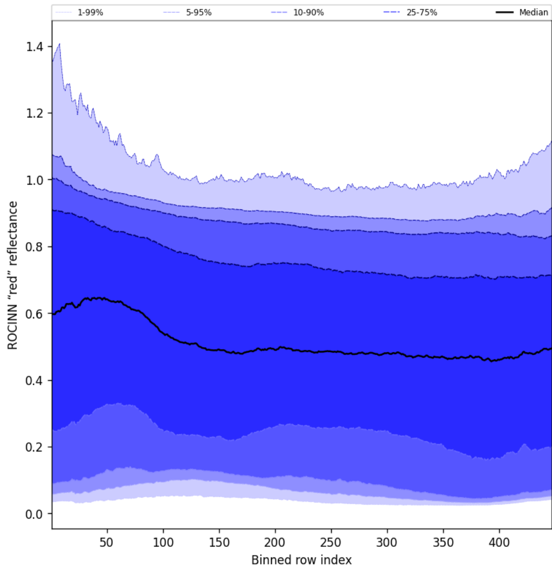
Figure 67: Along track statistics of "ROCINN "red" reflectance" for 2025-12-07 to 2025-12-07
