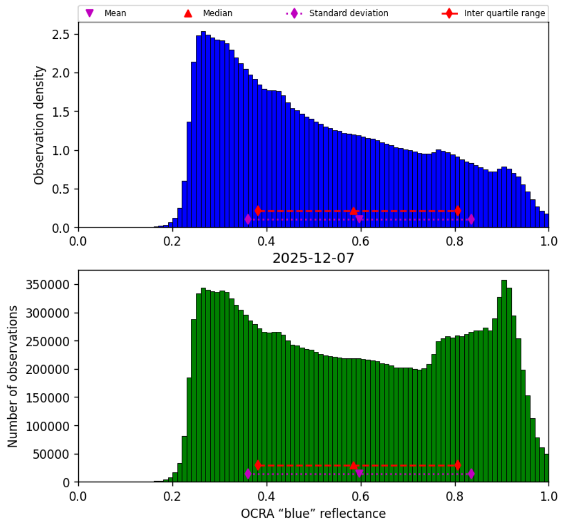
Figure 49: Histogram of “OCRA “blue” reflectance” for 2025-12-07 to 2025-12-07
