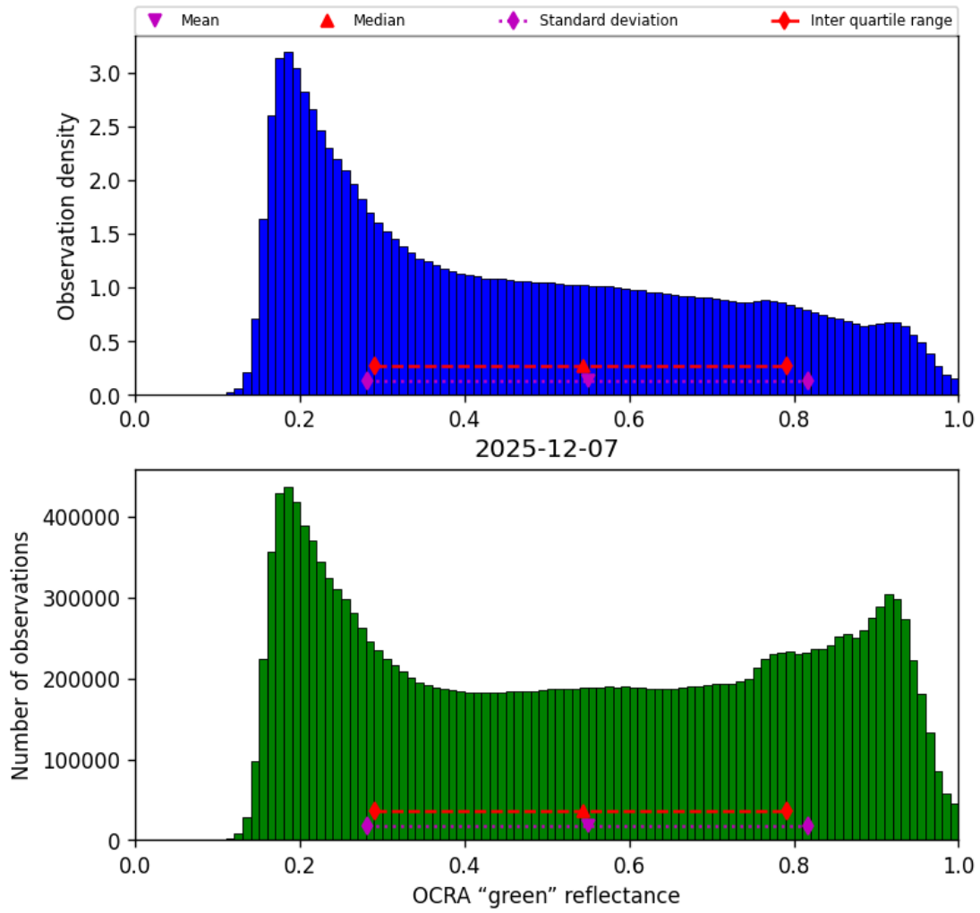
Figure 50: Histogram of “OCRA “green” reflectance” for 2025-12-07 to 2025-12-07
