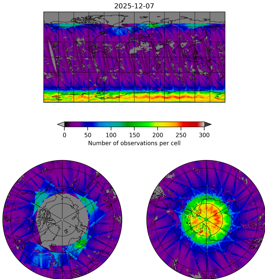
Figure 19: Map of the number of observations for 2025-12-07 to 2025-12-07
