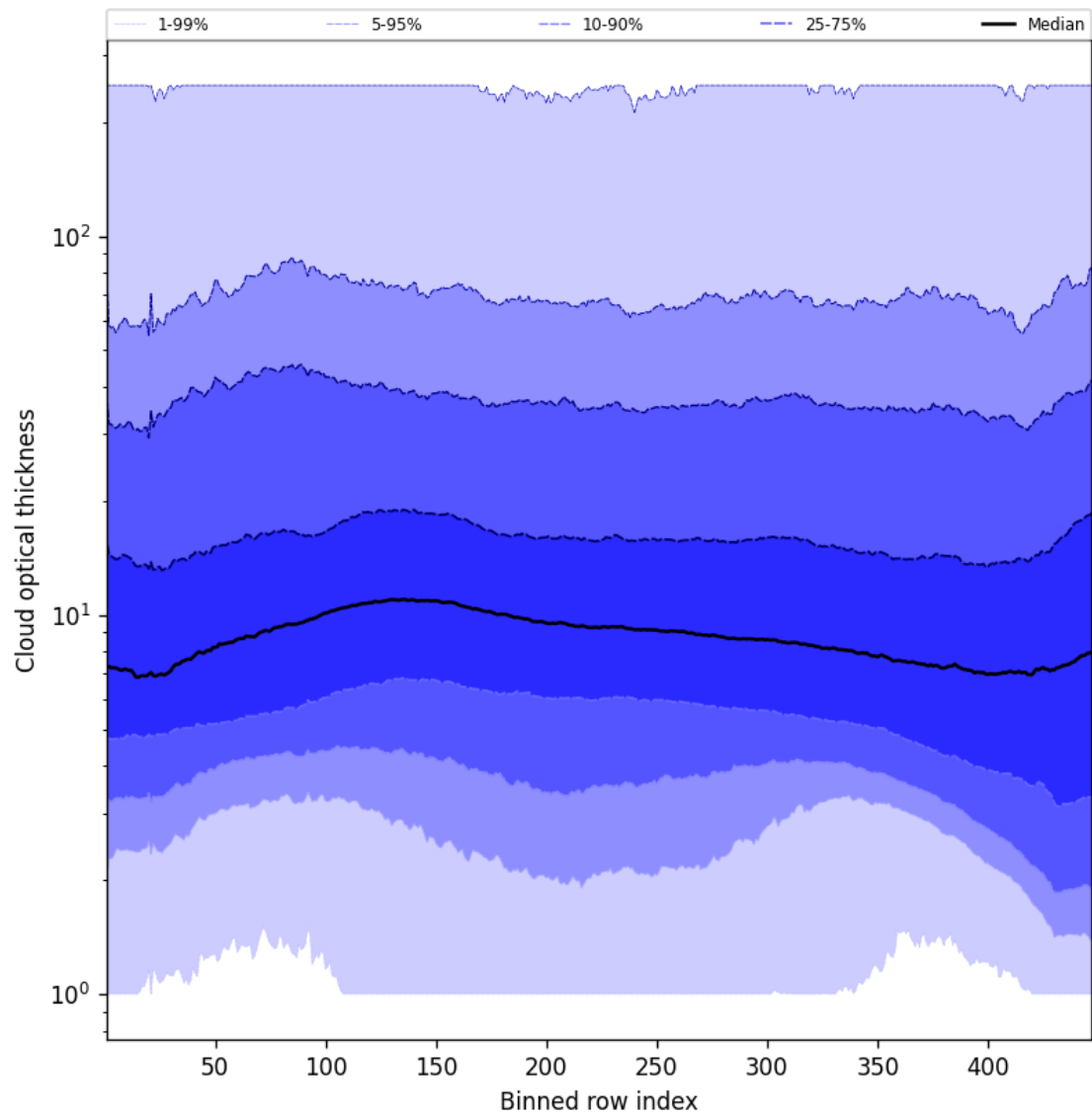
Figure 55: Along track statistics of “Cloud optical thickness” for 2025-12-07 to 2025-12-07
