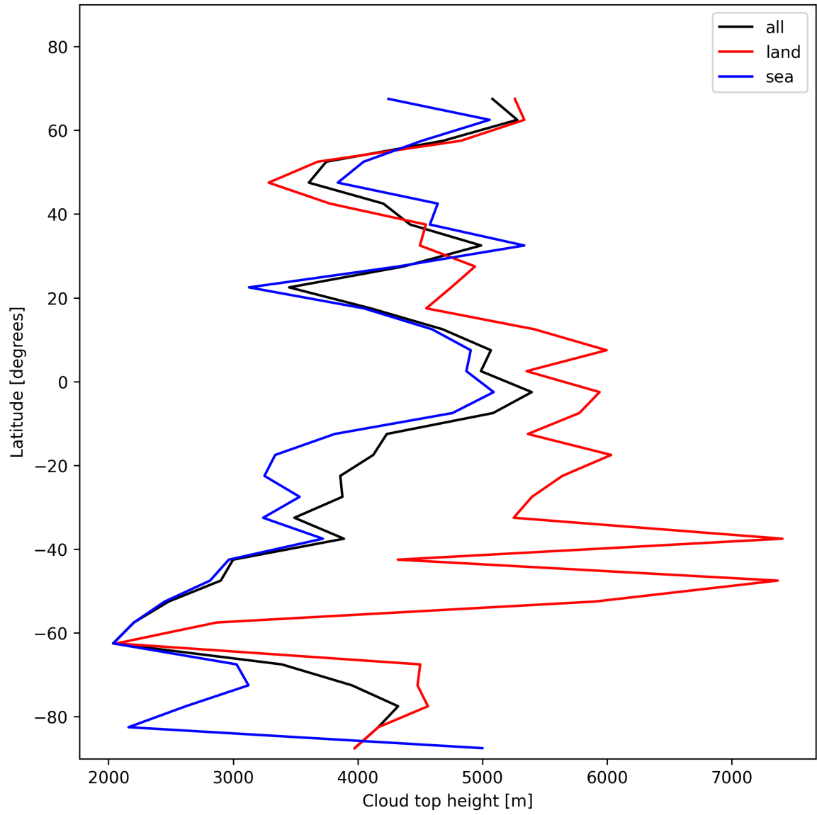
Figure 22: Zonal average of “Cloud top height” for 2025-12-07 to 2025-12-07.
