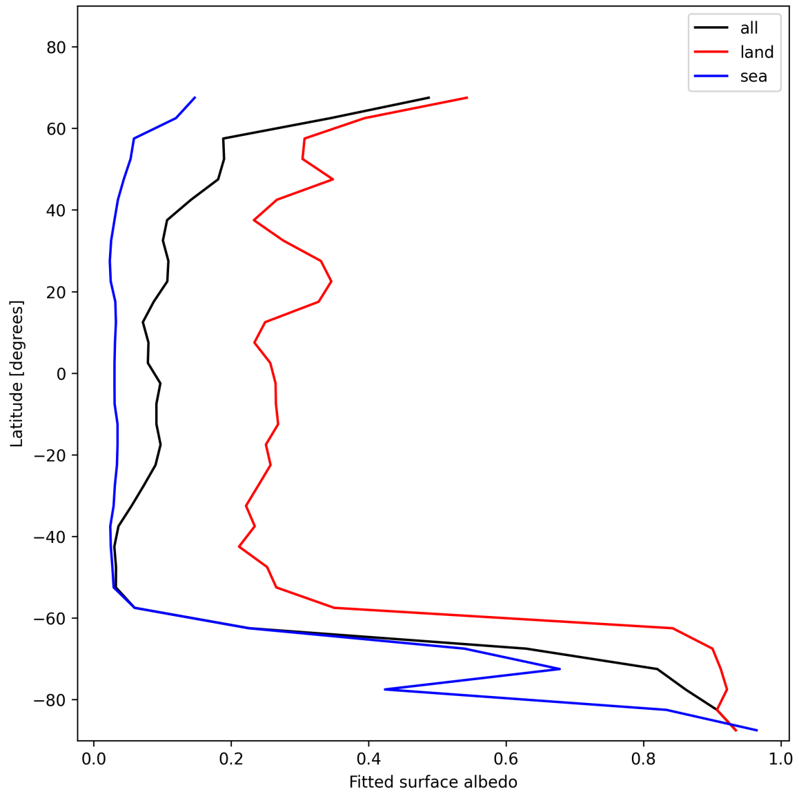
Figure 27: Zonal average of “Fitted surface albedo” for 2025-12-07 to 2025-12-07.
