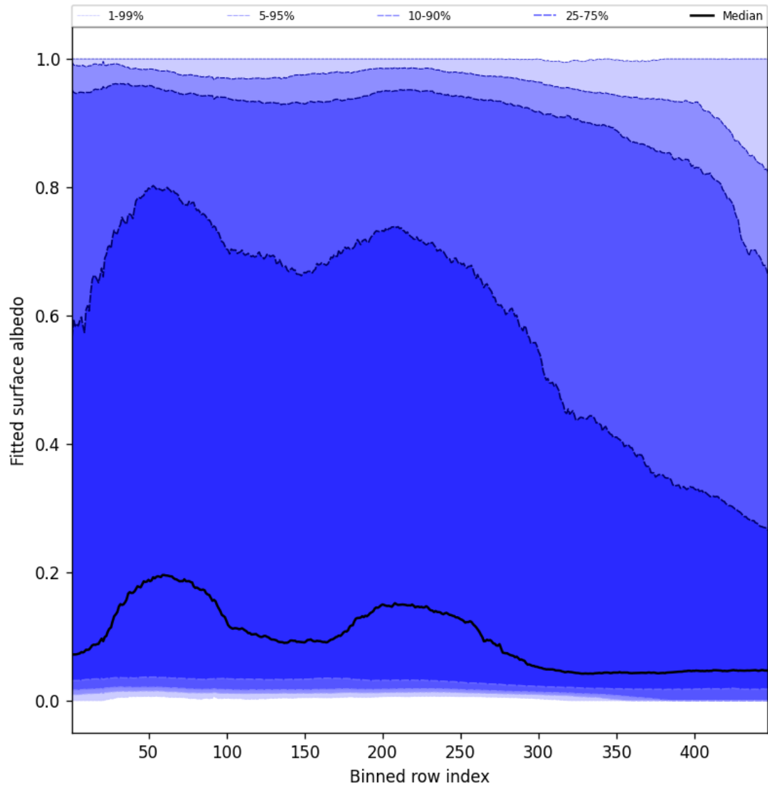
Figure 59: Along track statistics of “Fitted surface albedo” for 2025-12-07 to 2025-12-07
