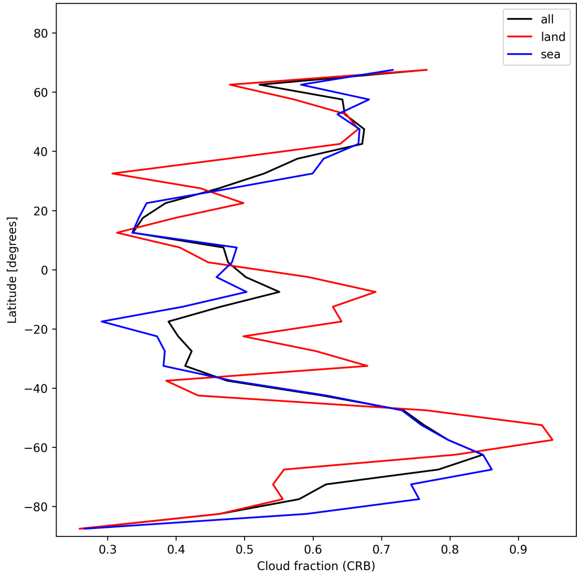
Figure 24: Zonal average of “Cloud fraction (CRB)” for 2025-12-07 to 2025-12-07.
