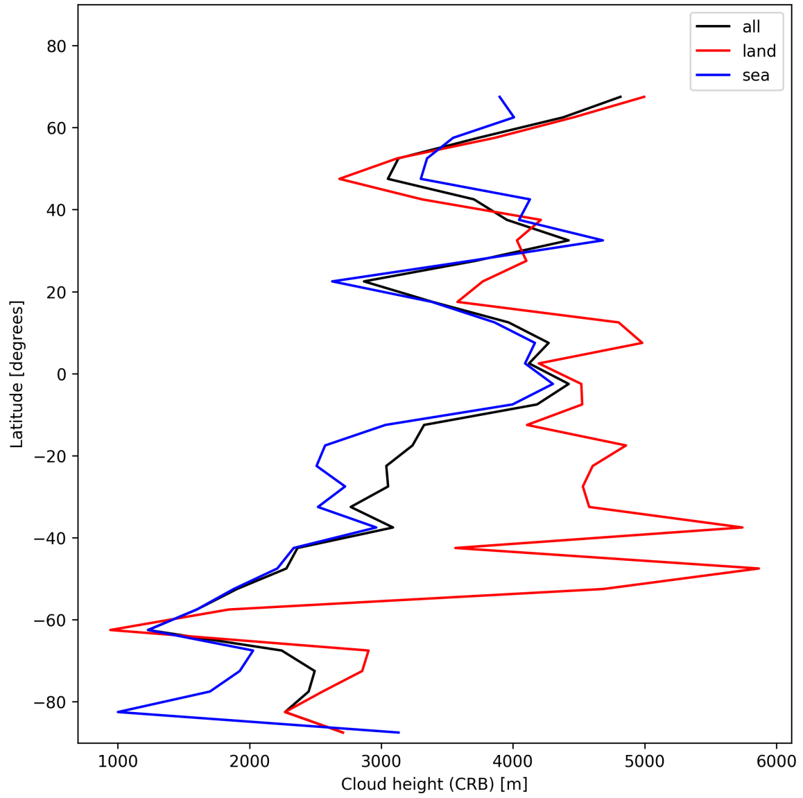
Figure 25: Zonal average of “Cloud height (CRB)” for 2025-12-07 to 2025-12-07.
