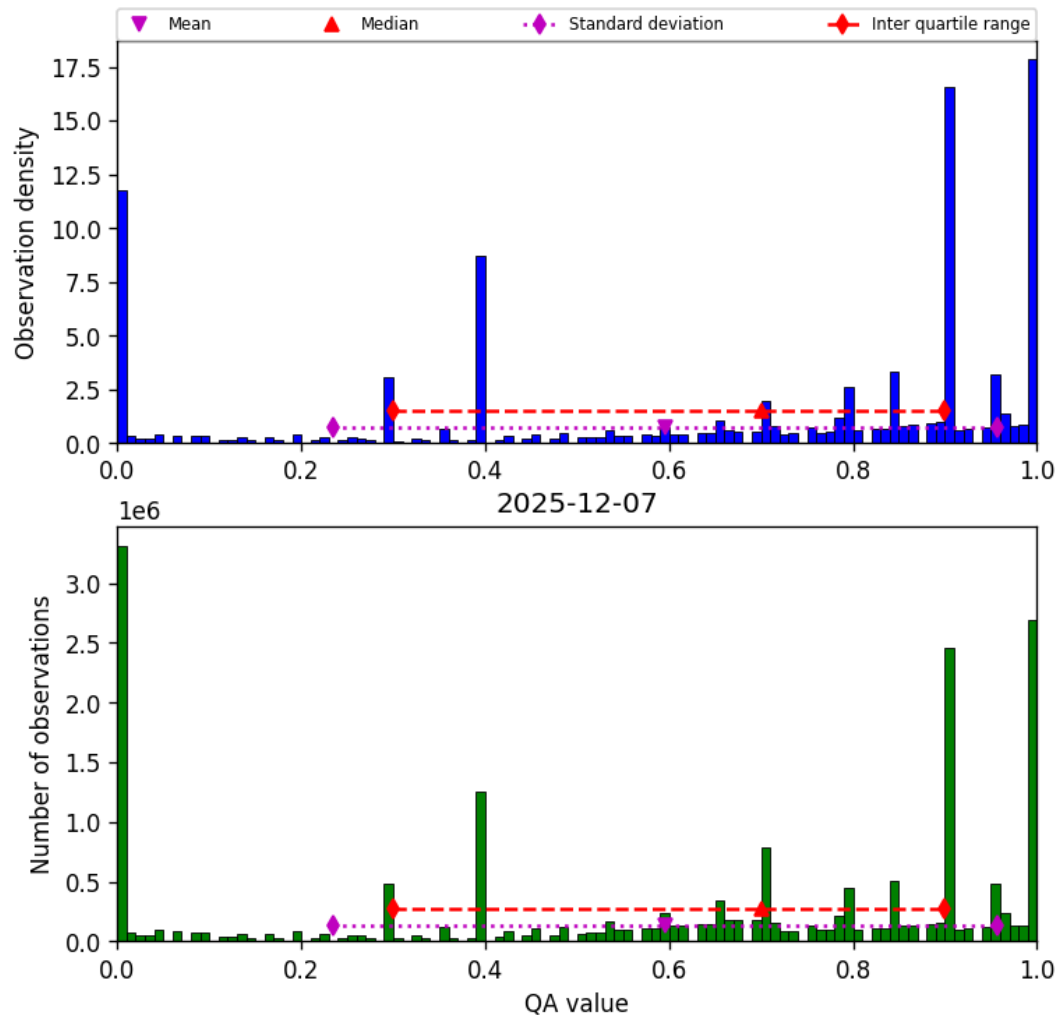
Figure 36: Histogram of “QA value” for 2025-12-07 to 2025-12-07
