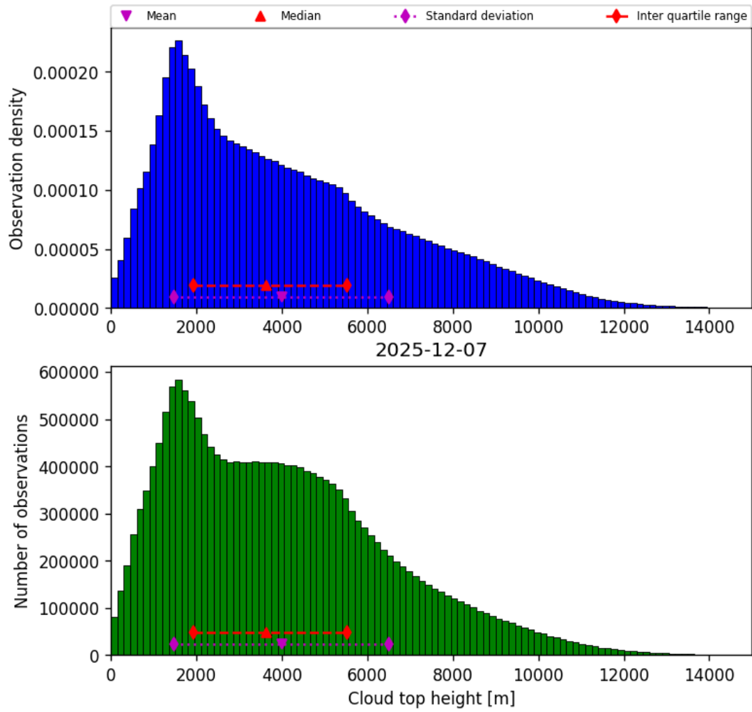
Figure 38: Histogram of “Cloud top height” for 2025-12-07 to 2025-12-07
