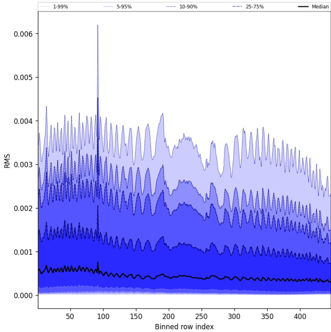
Figure 61: Along track statistics of “RMS” for 2025-12-07 to 2025-12-07
