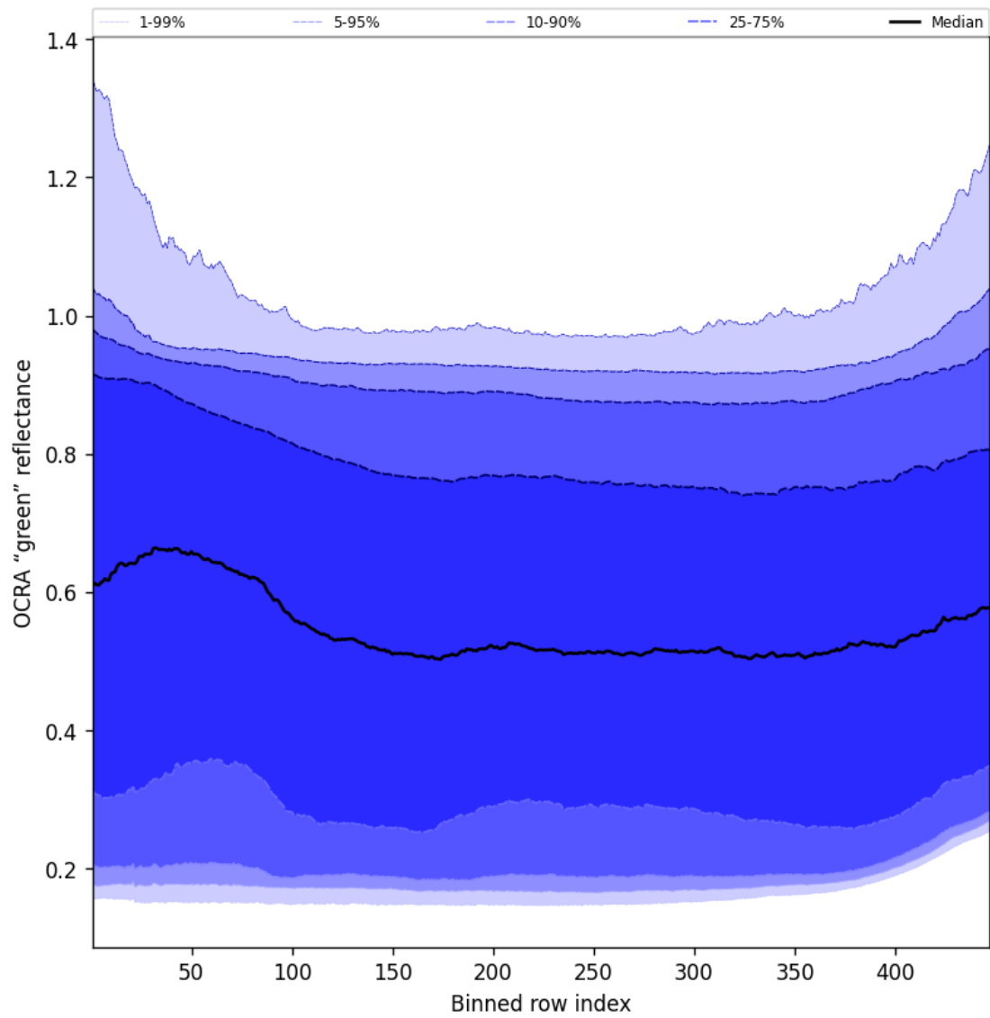
Figure 66: Along track statistics of “OCRA “green” reflectance” for 2025-12-07 to 2025-12-07
