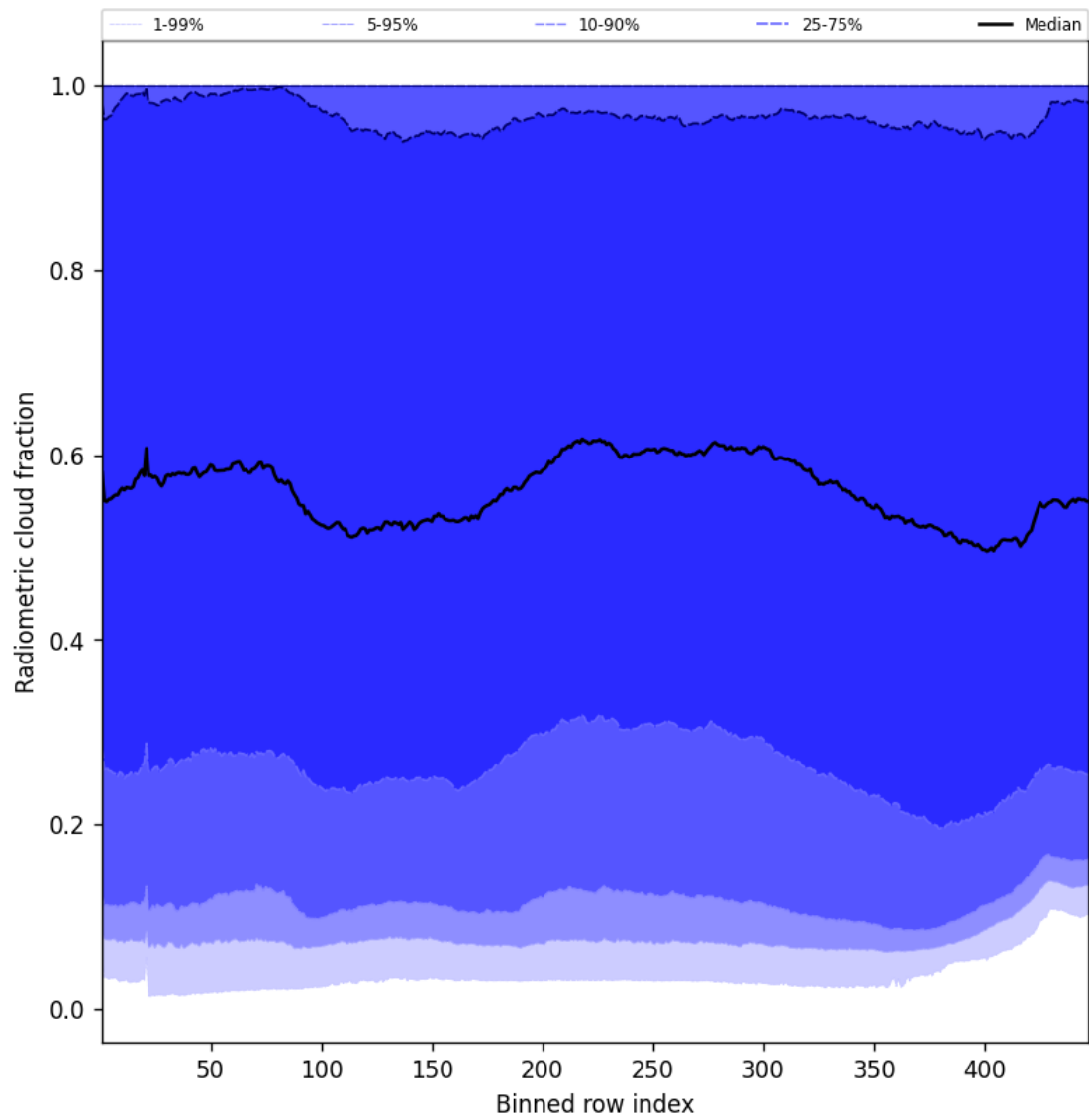
Figure 53: Along track statistics of “Radiometric cloud fraction” for 2025-12-07 to 2025-12-07
