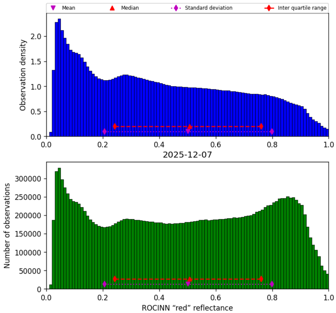
Figure 51: Histogram of “ROCINN “red” reflectance” for 2025-12-07 to 2025-12-07
