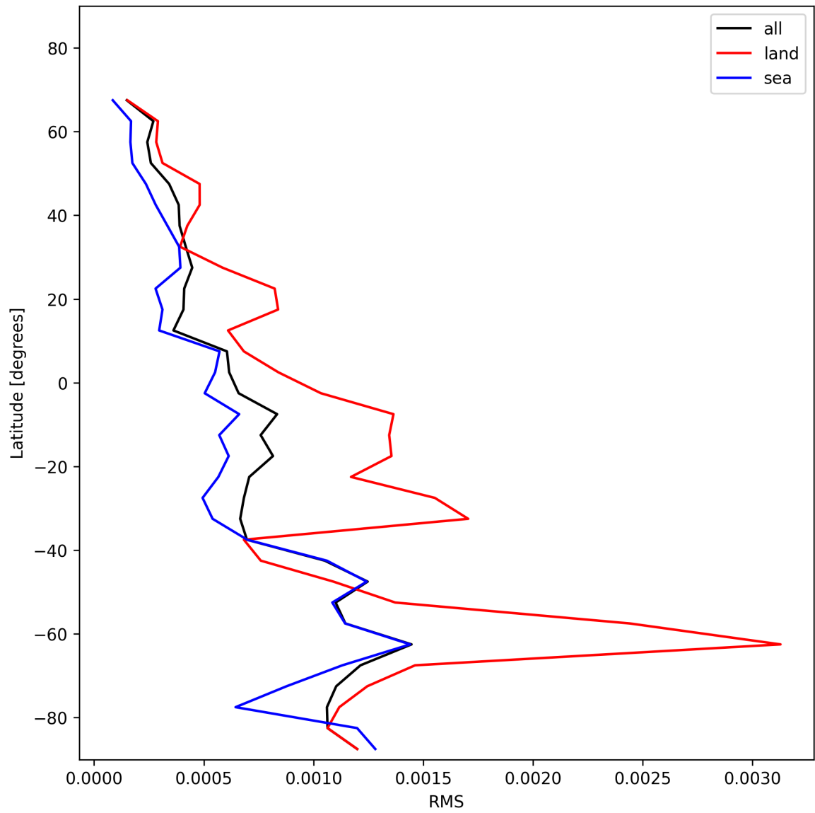
Figure 29: Zonal average of “RMS” for 2025-12-07 to 2025-12-07.
