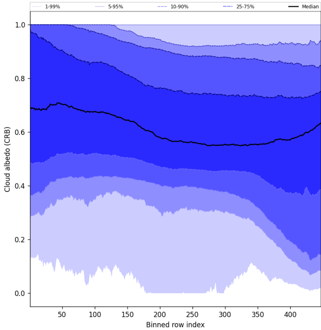
Figure 58: Along track statistics of “Cloud albedo (CRB)” for 2025-12-07 to 2025-12-07
