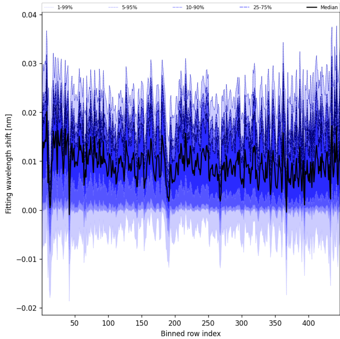
Figure 63: Along track statistics of “Fitting wavelength shift” for 2025-12-07 to 2025-12-07
