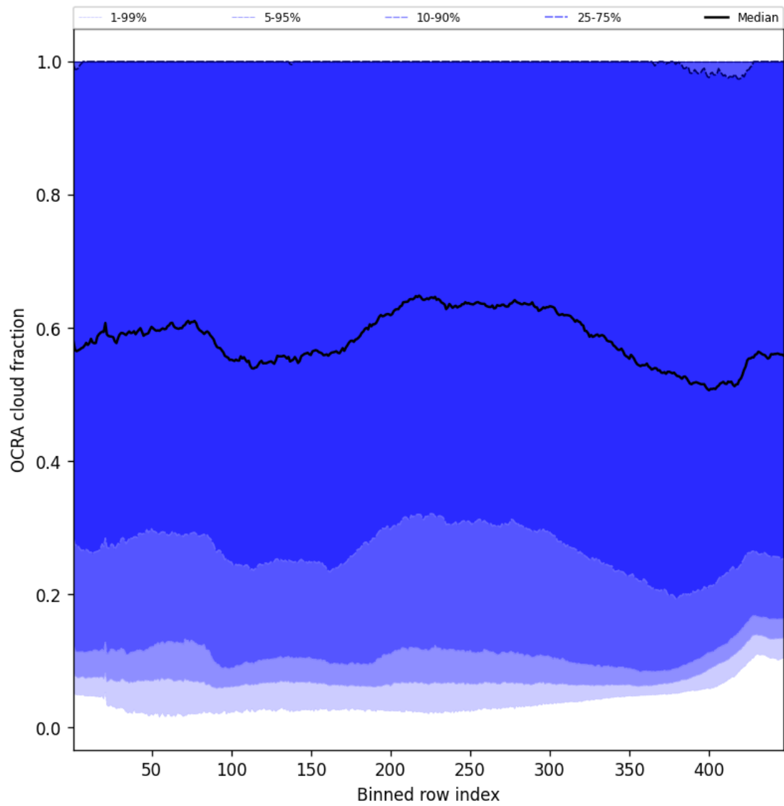
Figure 64: Along track statistics of “OCRA cloud fraction” for 2025-12-07 to 2025-12-07
