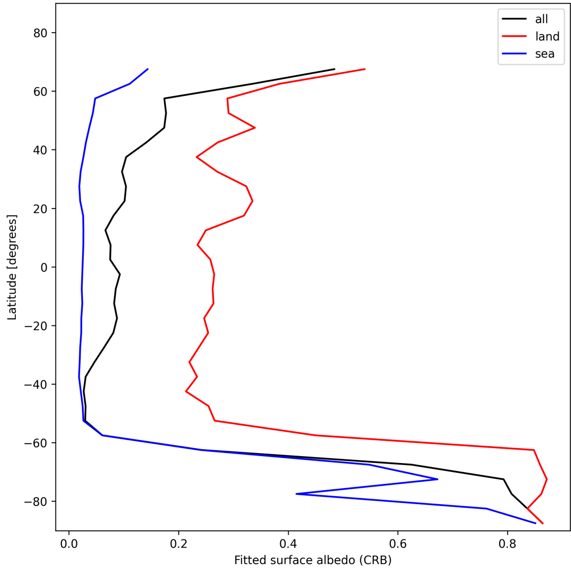
Figure 28: Zonal average of “Fitted surface albedo (CRB)” for 2025-12-07 to 2025-12-07.
