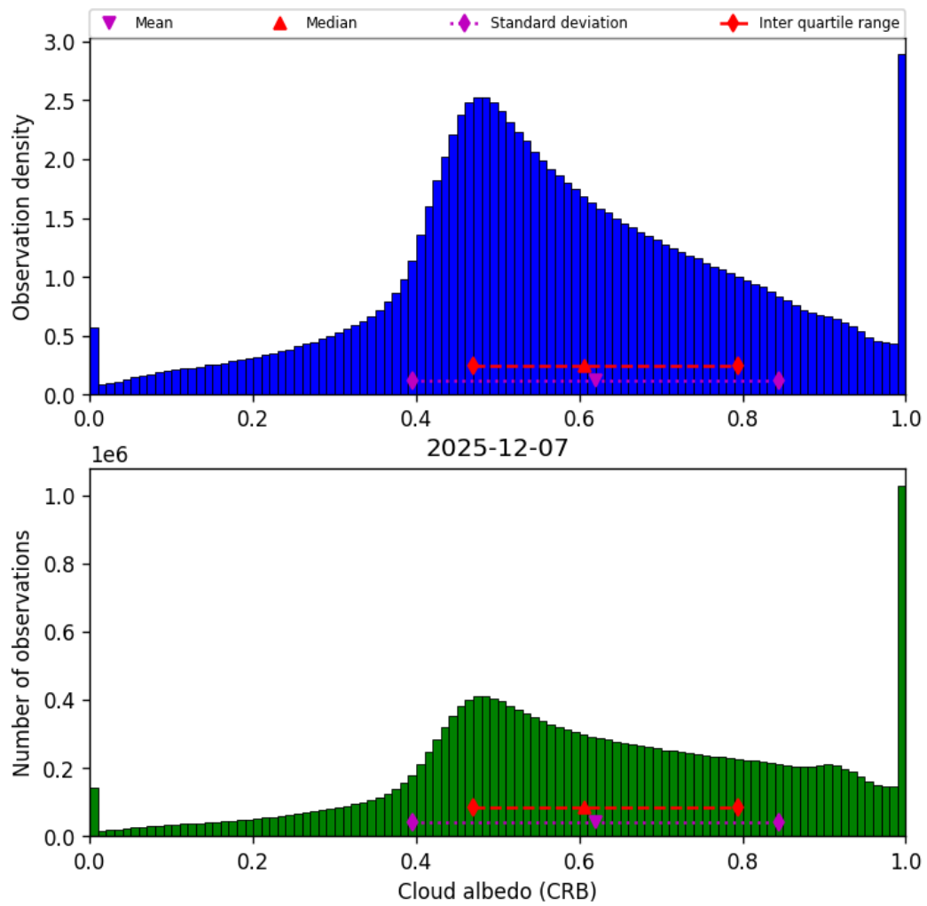
Figure 42: Histogram of “Cloud albedo (CRB)” for 2025-12-07 to 2025-12-07
