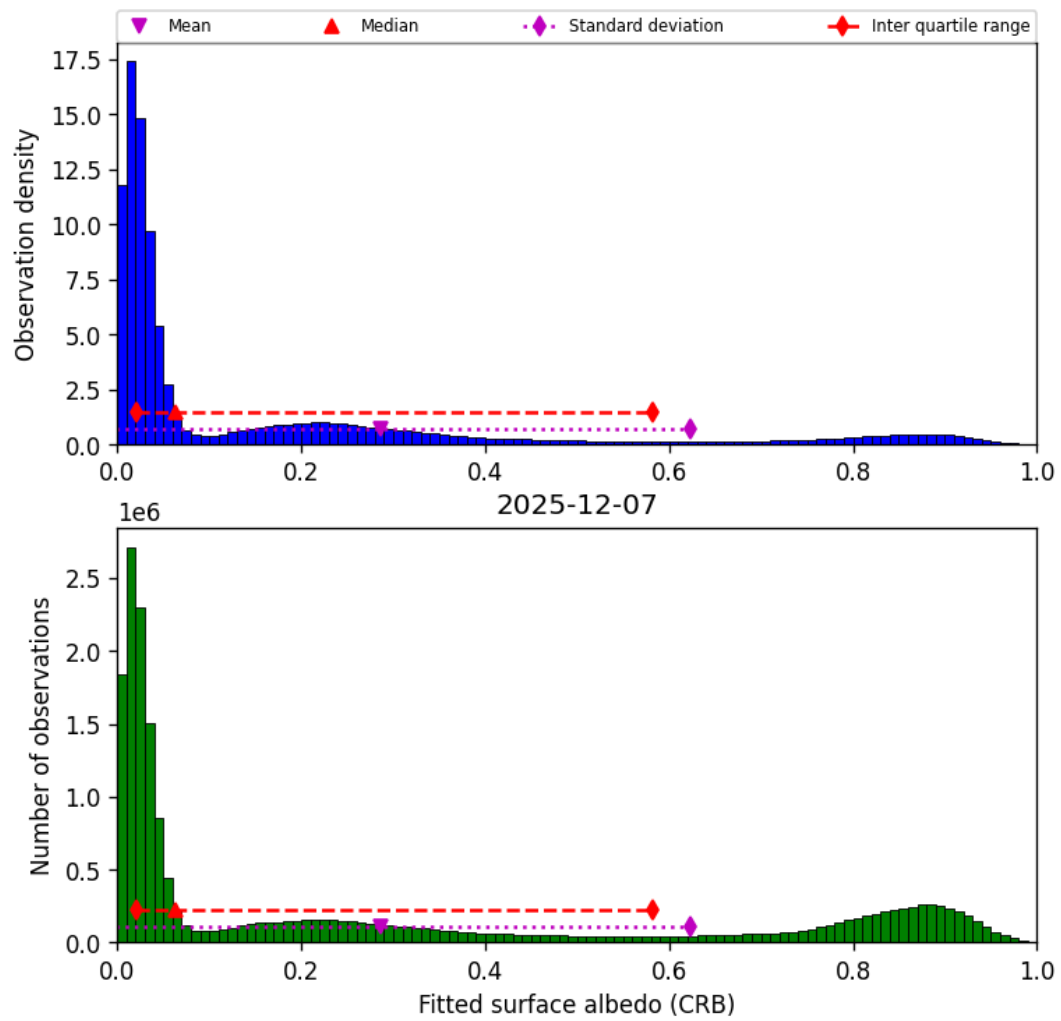
Figure 44: Histogram of “Fitted surface albedo (CRB)” for 2025-12-07 to 2025-12-07
