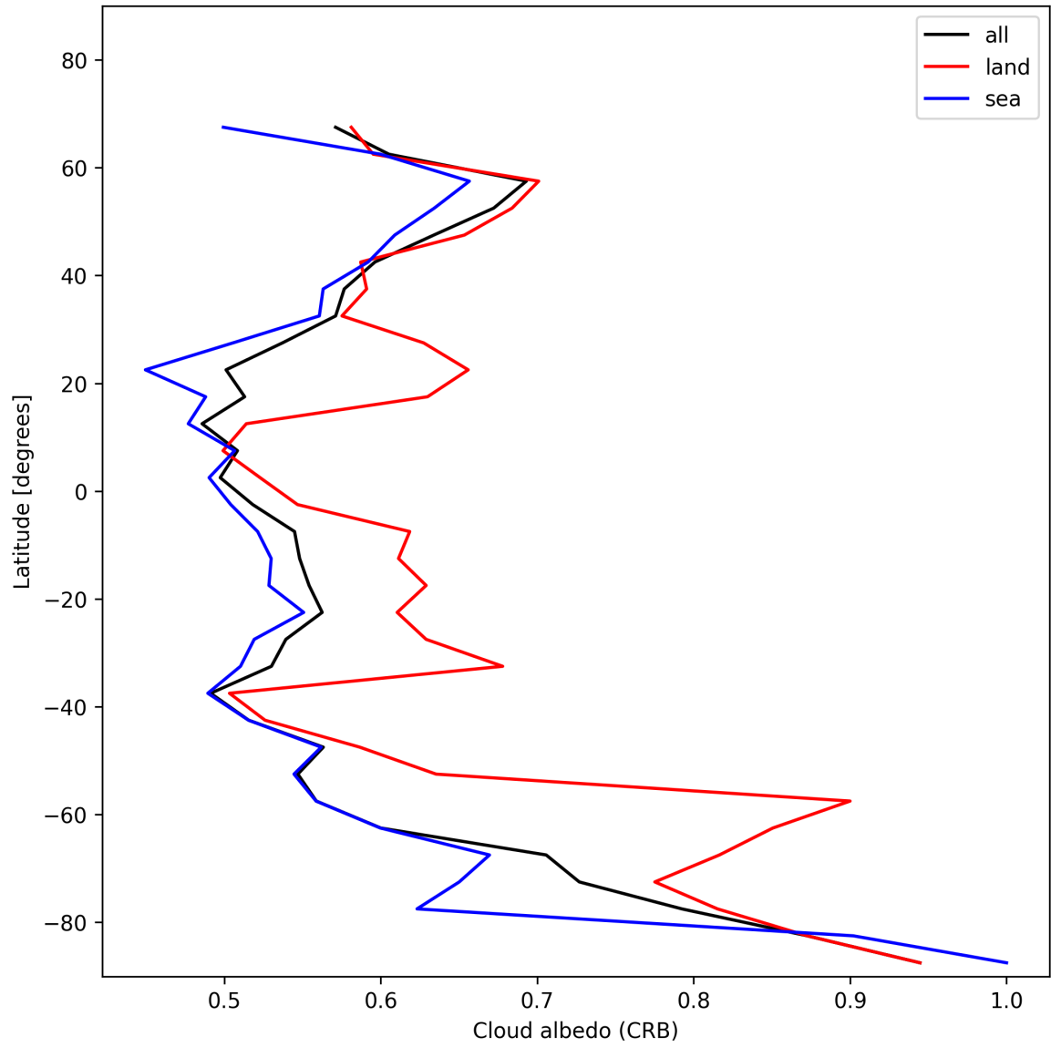
Figure 26: Zonal average of “Cloud albedo (CRB)” for 2025-12-07 to 2025-12-07.
