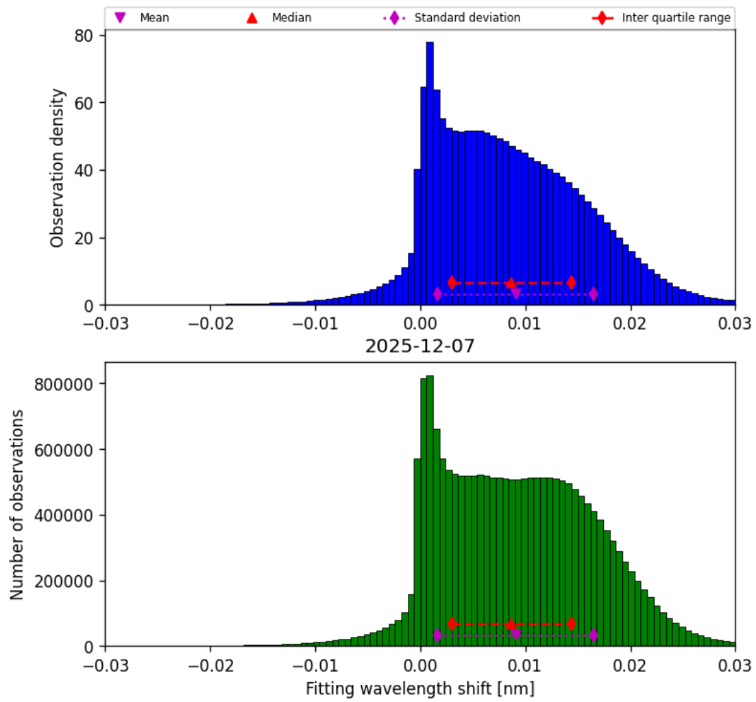
Figure 47: Histogram of “Fitting wavelength shift” for 2025-12-07 to 2025-12-07
