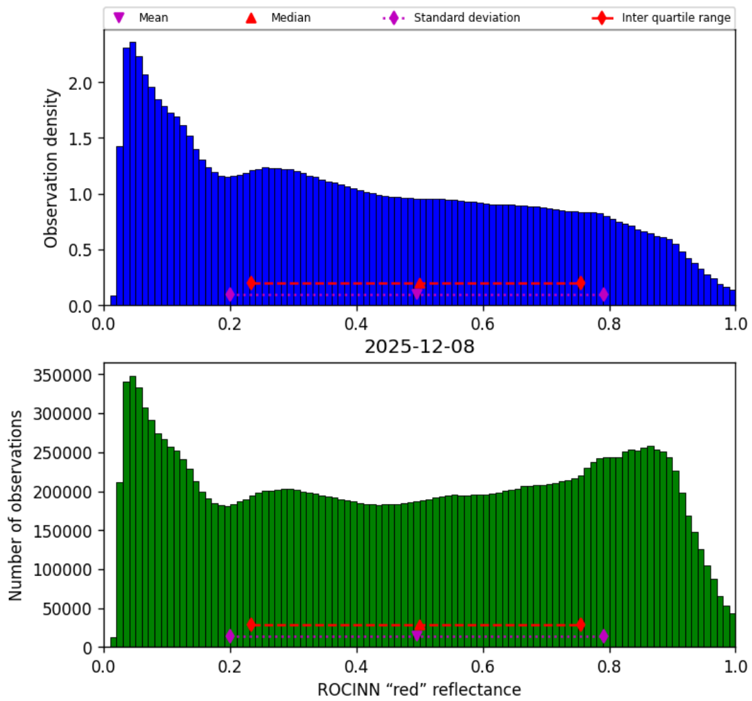
Figure 51: Histogram of “ROCINN “red” reflectance” for 2025-12-08 to 2025-12-09
