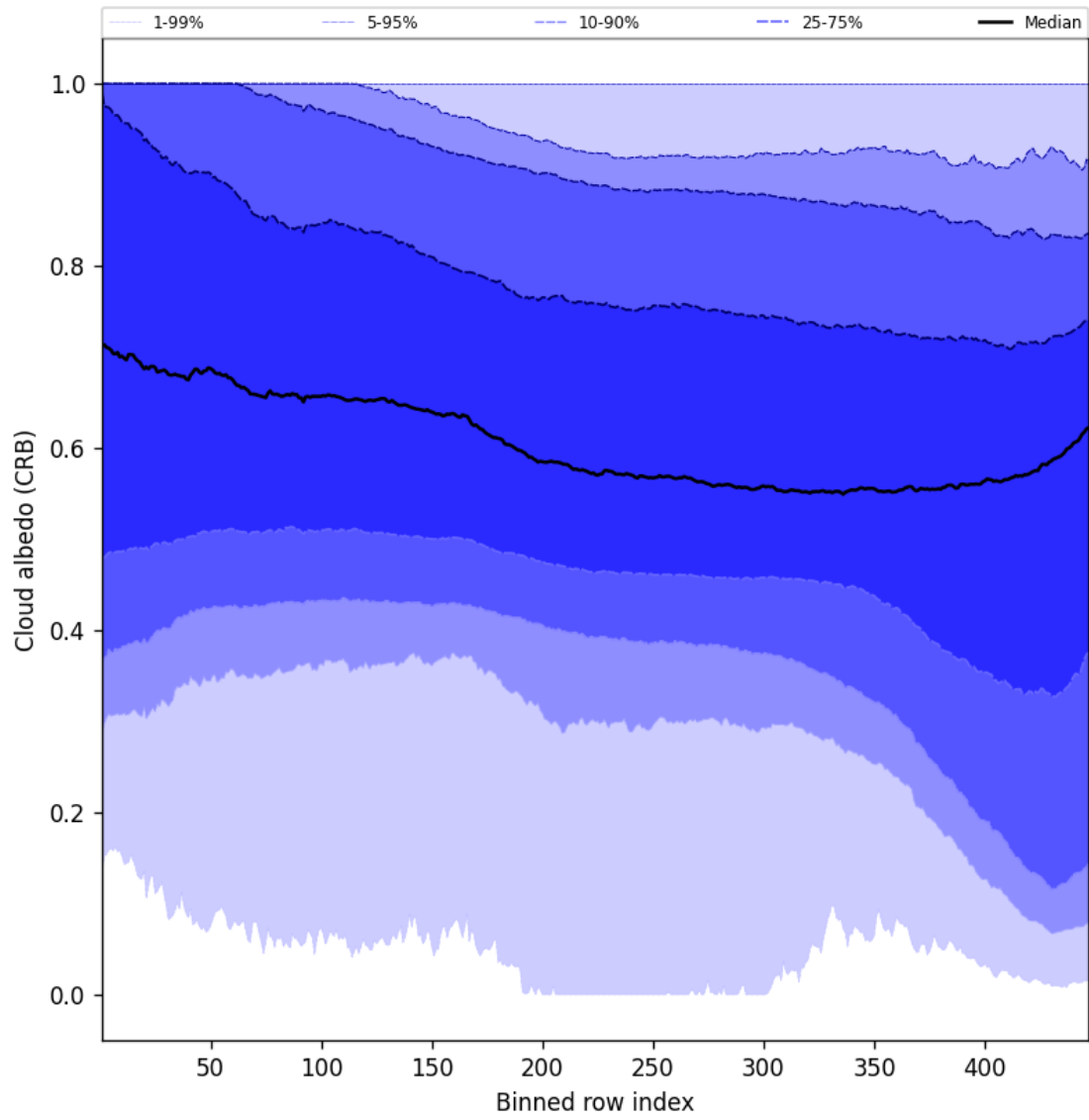
Figure 58: Along track statistics of “Cloud albedo (CRB)” for 2025-12-08 to 2025-12-09
