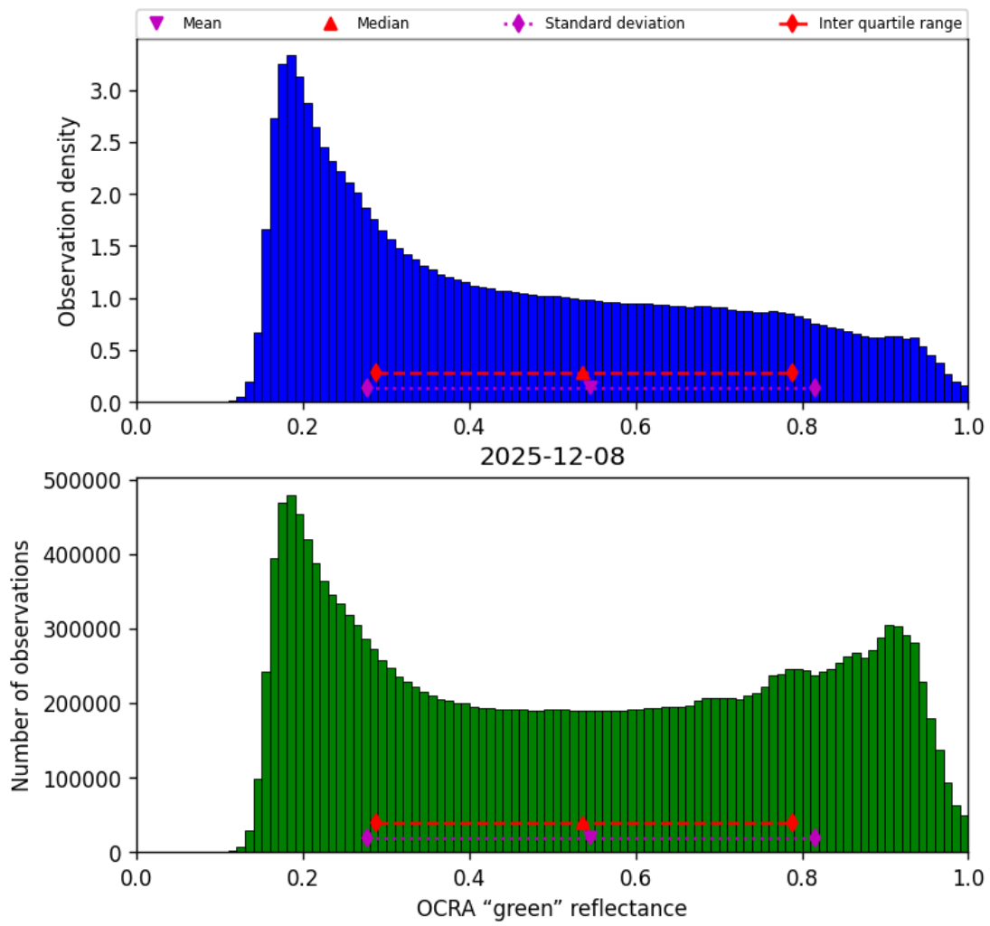
Figure 50: Histogram of “OCRA “green” reflectance” for 2025-12-08 to 2025-12-09
