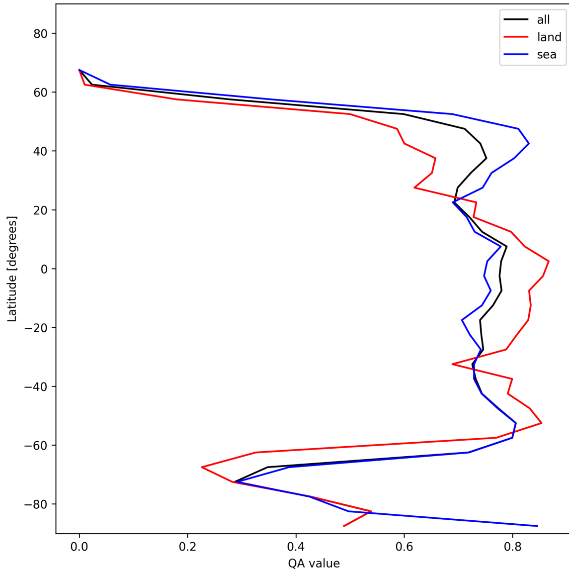
Figure 20: Zonal average of “QA value” for 2025-12-08 to 2025-12-09.
