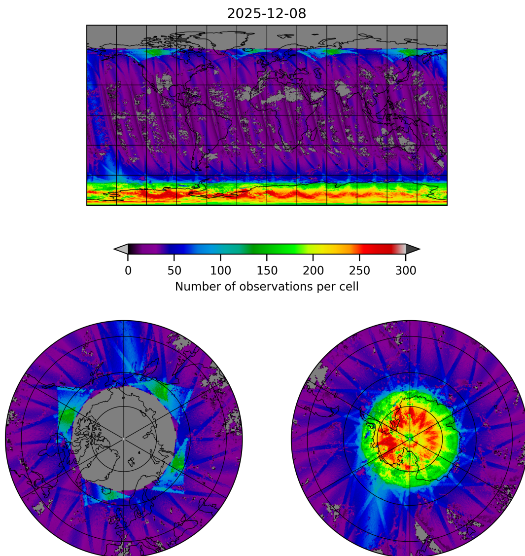
Figure 19: Map of the number of observations for 2025-12-08 to 2025-12-09
