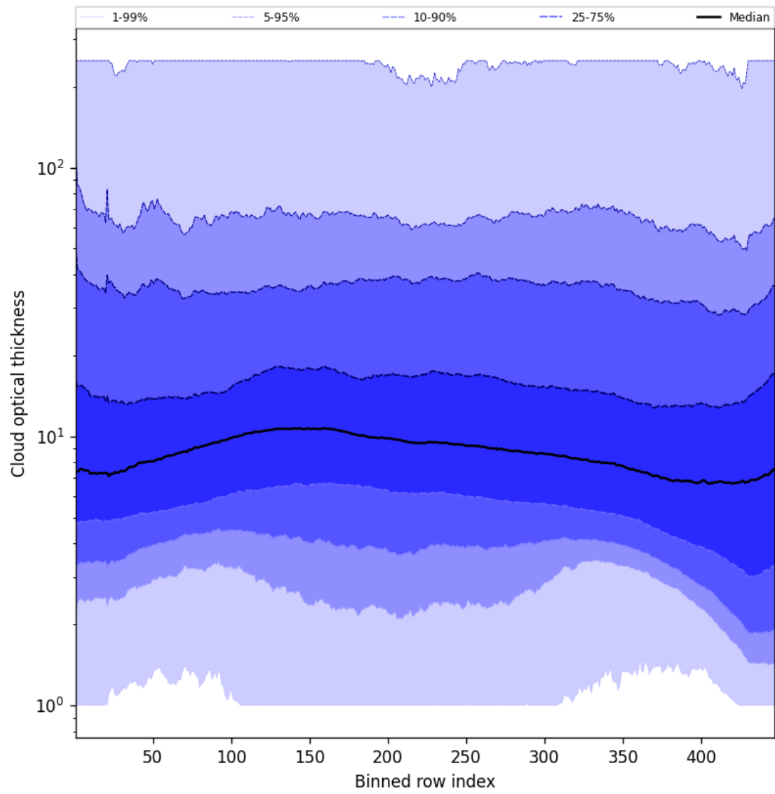
Figure 55: Along track statistics of “Cloud optical thickness” for 2025-12-08 to 2025-12-09
