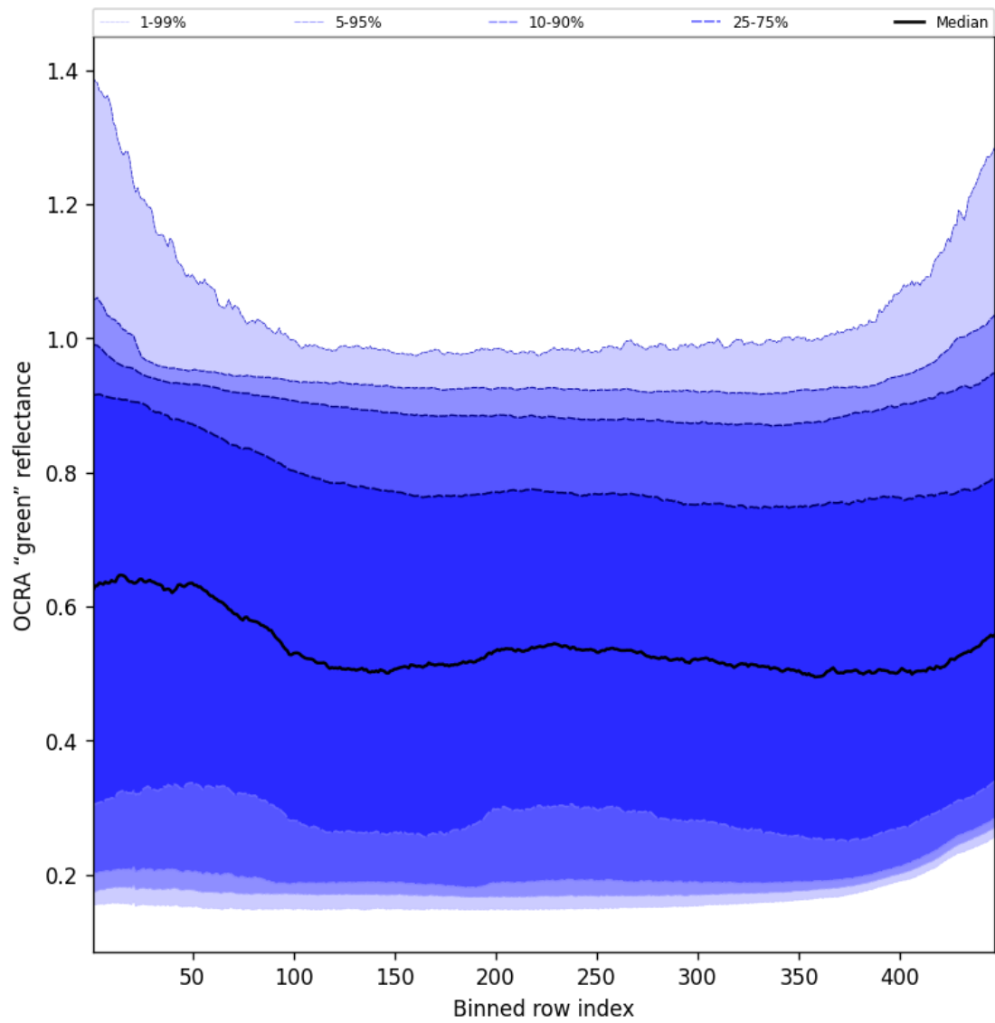
Figure 66: Along track statistics of “OCRA “green” reflectance” for 2025-12-08 to 2025-12-09
