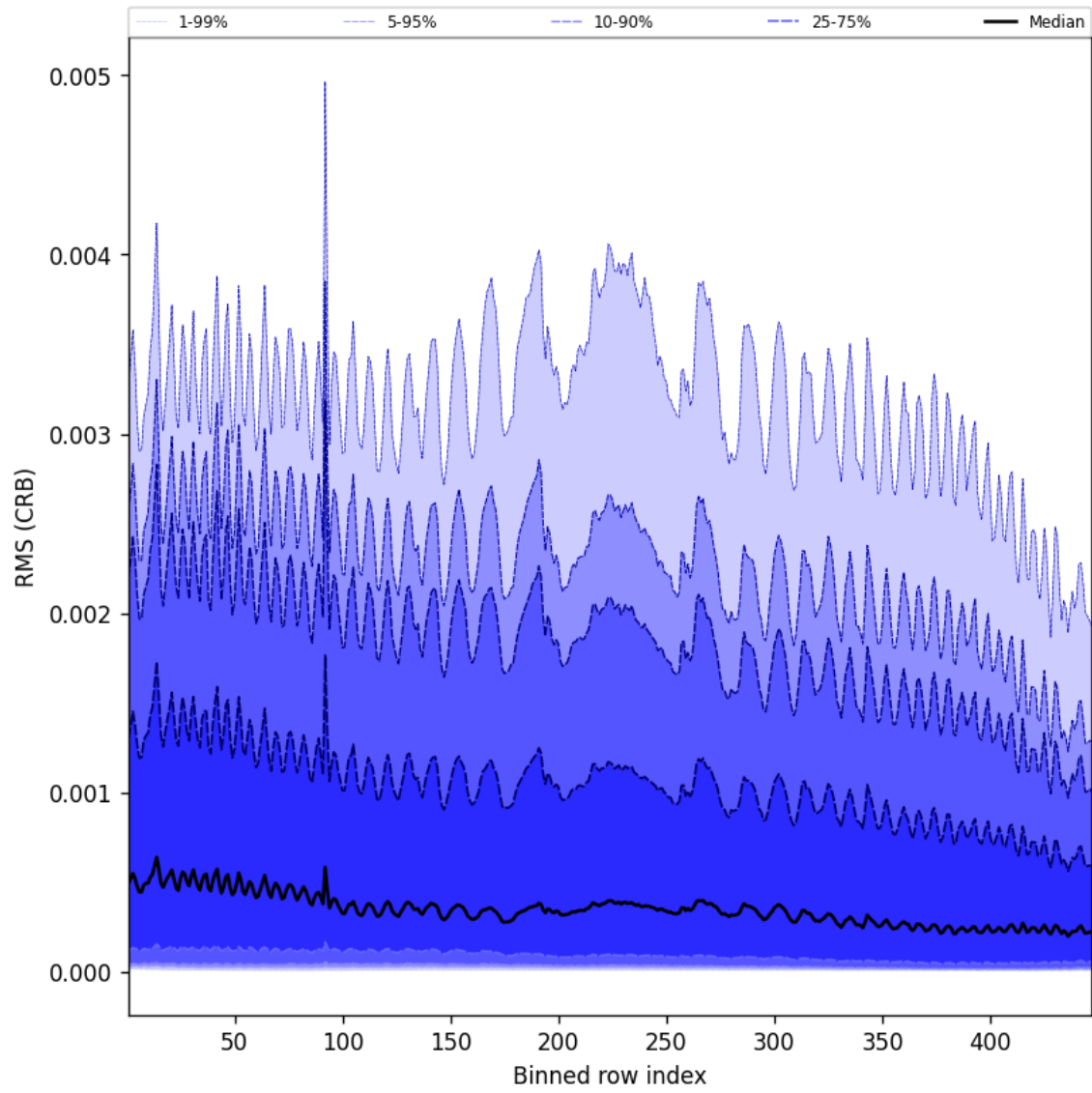
Figure 62: Along track statistics of “RMS (CRB)” for 2025-12-08 to 2025-12-09
