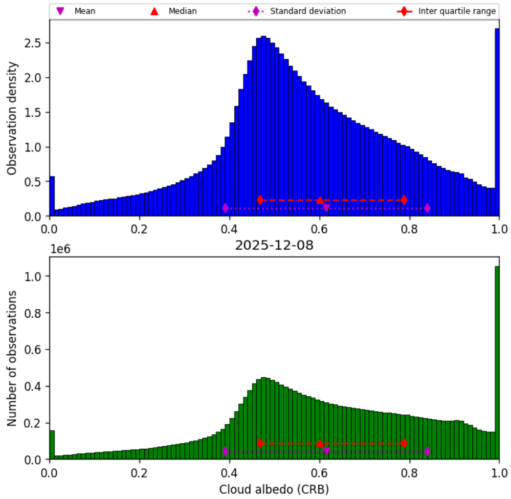
Figure 42: Histogram of “Cloud albedo (CRB)” for 2025-12-08 to 2025-12-09
