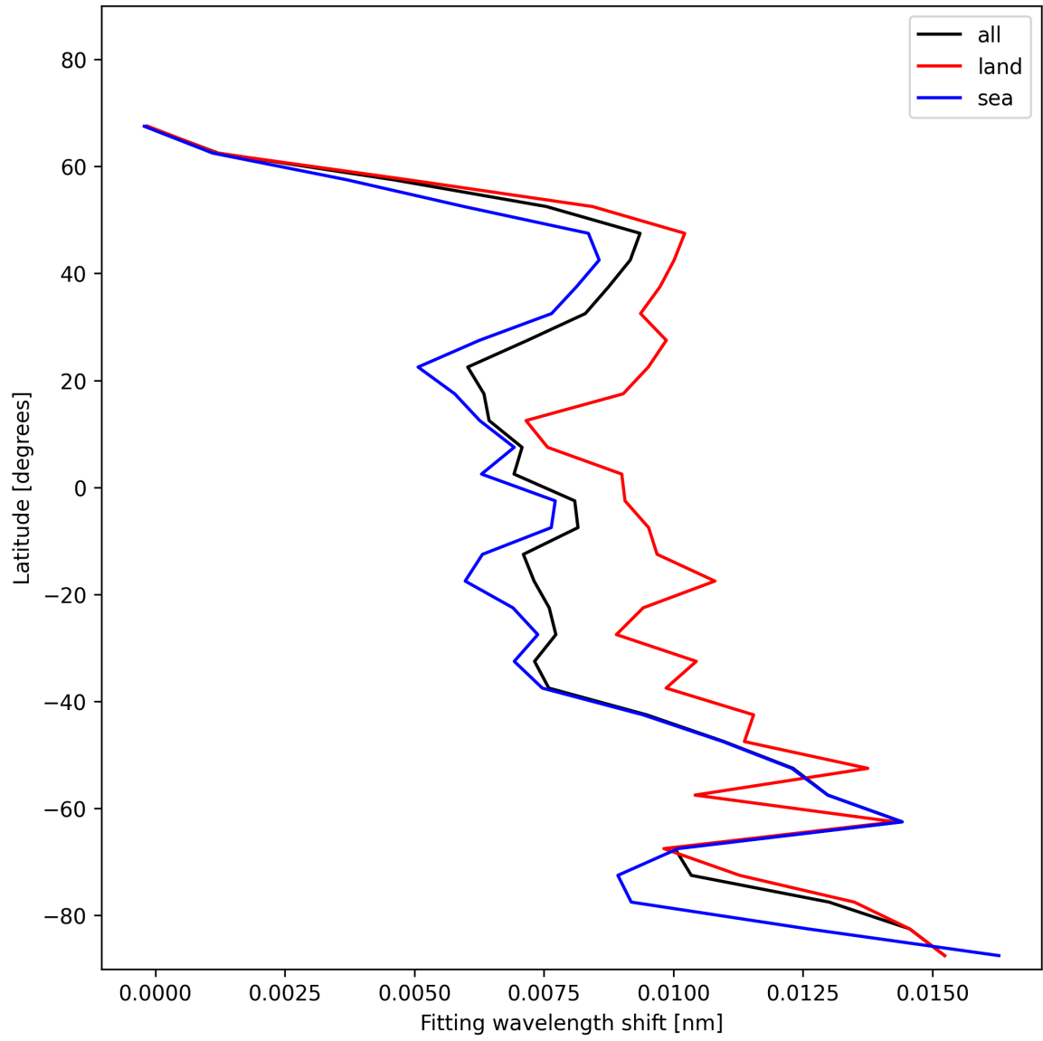
Figure 31: Zonal average of “Fitting wavelength shift” for 2025-12-08 to 2025-12-09.
