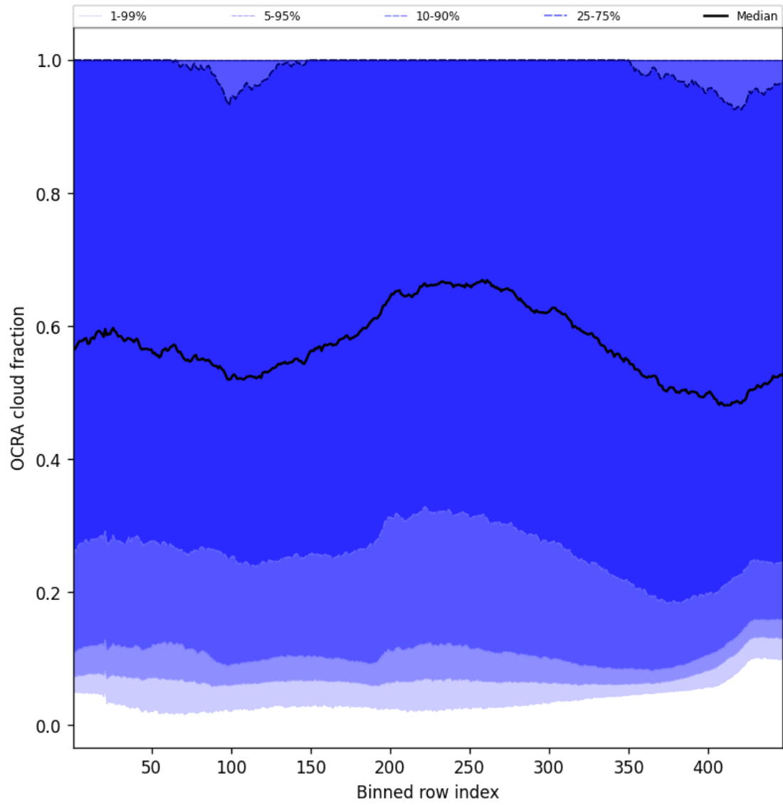
Figure 64: Along track statistics of “OCRA cloud fraction” for 2025-12-08 to 2025-12-09
