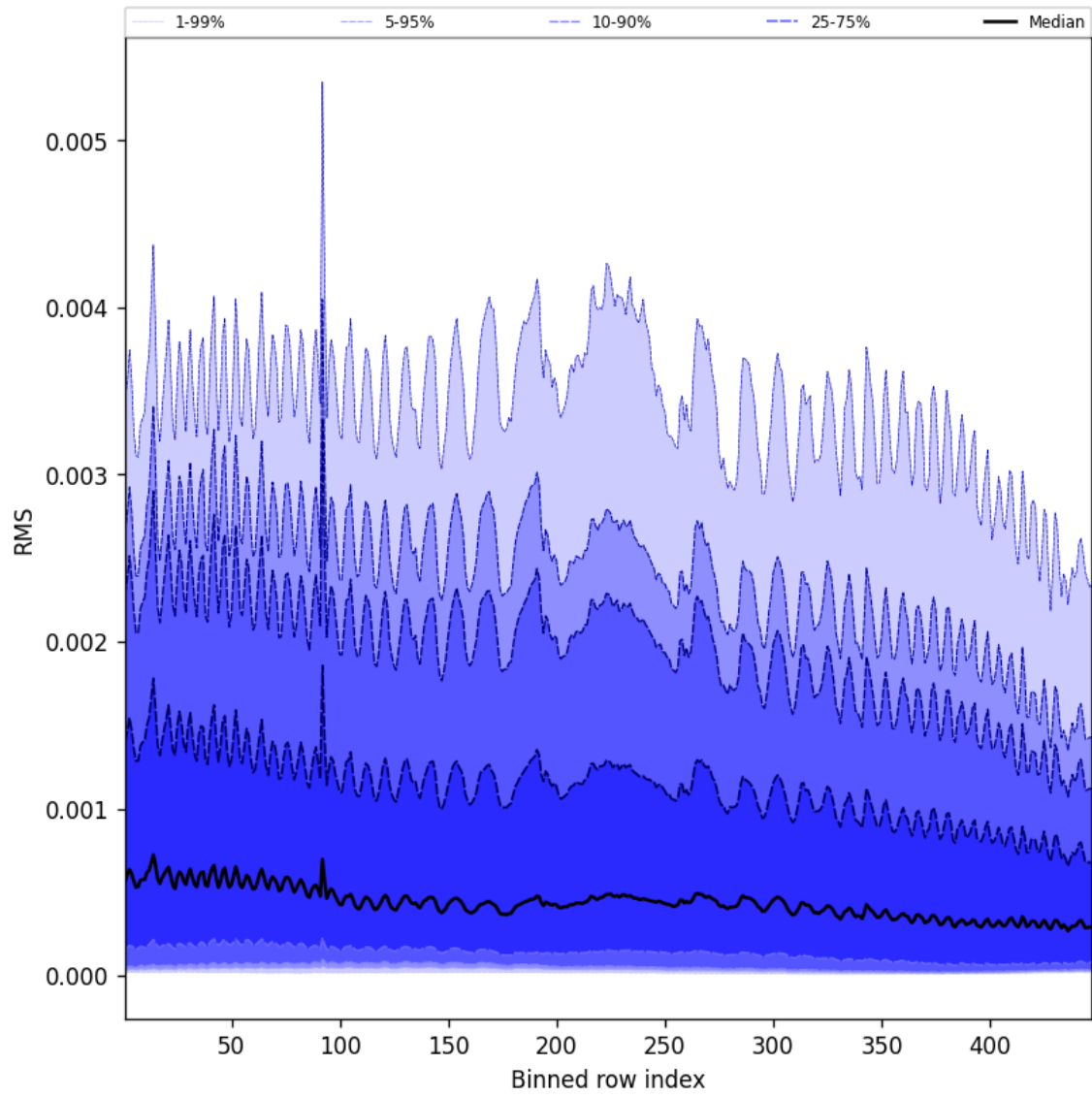
Figure 61: Along track statistics of “RMS” for 2025-12-08 to 2025-12-09
