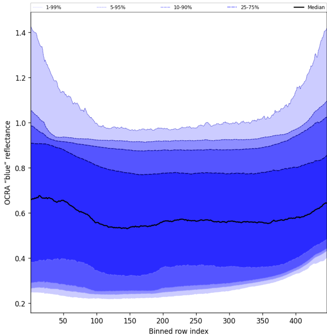
Figure 65: Along track statistics of “OCRA “blue” reflectance” for 2025-12-08 to 2025-12-09
