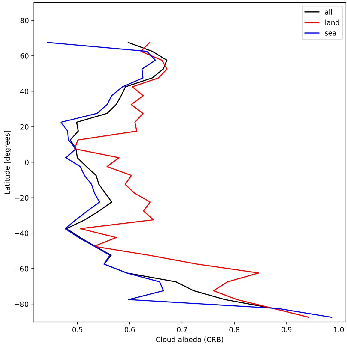
Figure 26: Zonal average of “Cloud albedo (CRB)” for 2025-12-08 to 2025-12-09.
