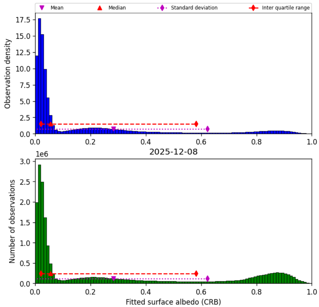
Figure 44: Histogram of “Fitted surface albedo (CRB)” for 2025-12-08 to 2025-12-09
