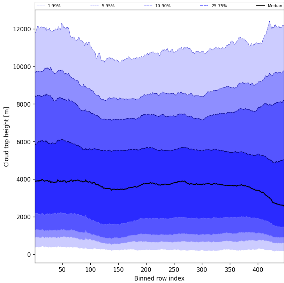
Figure 54: Along track statistics of “Cloud top height” for 2025-12-08 to 2025-12-09
