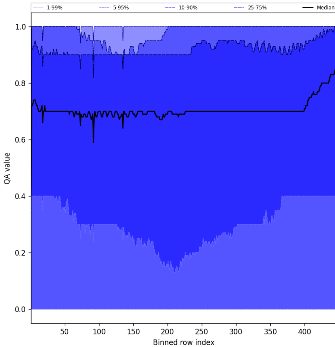
Figure 52: Along track statistics of “QA value” for 2025-12-08 to 2025-12-09
