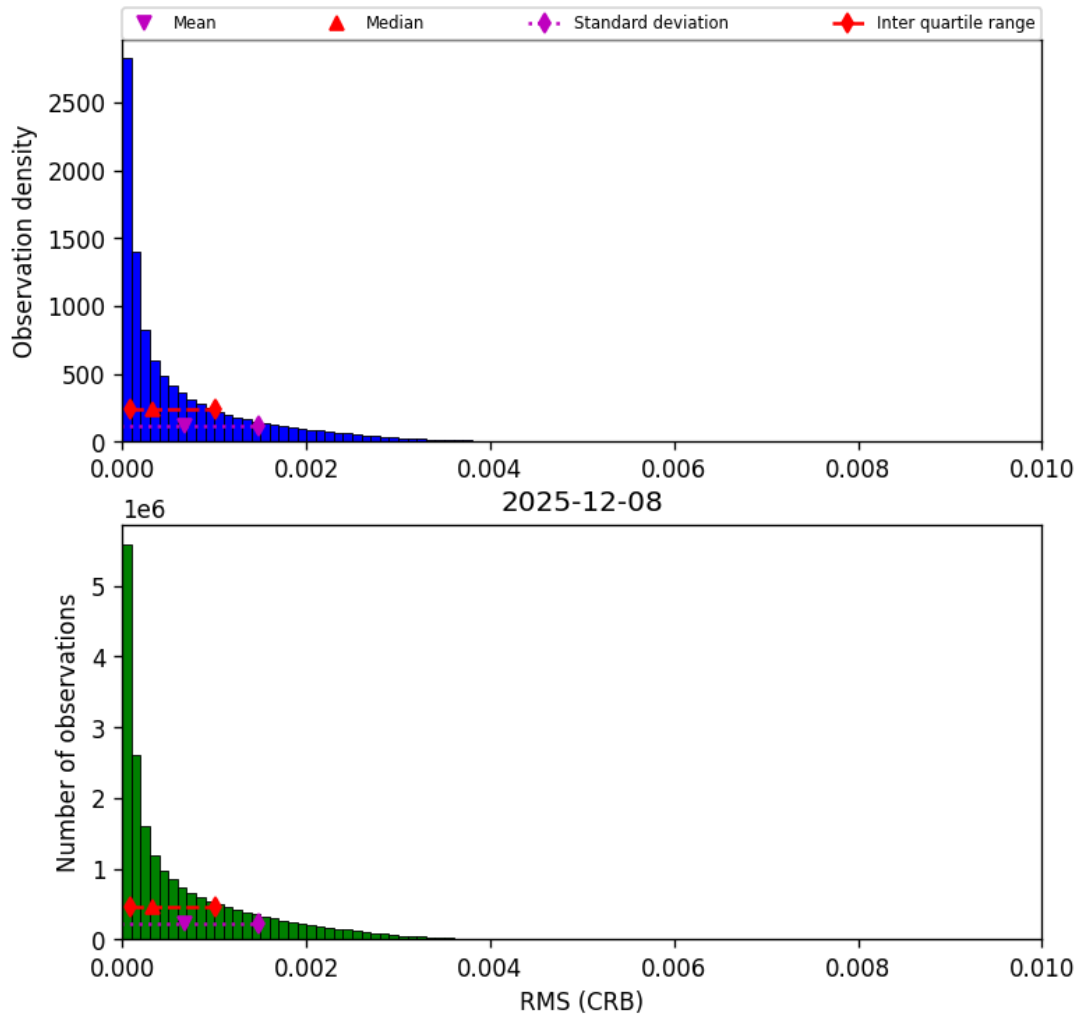
Figure 46: Histogram of "RMS (CRB)" for 2025-12-08 to 2025-12-09
