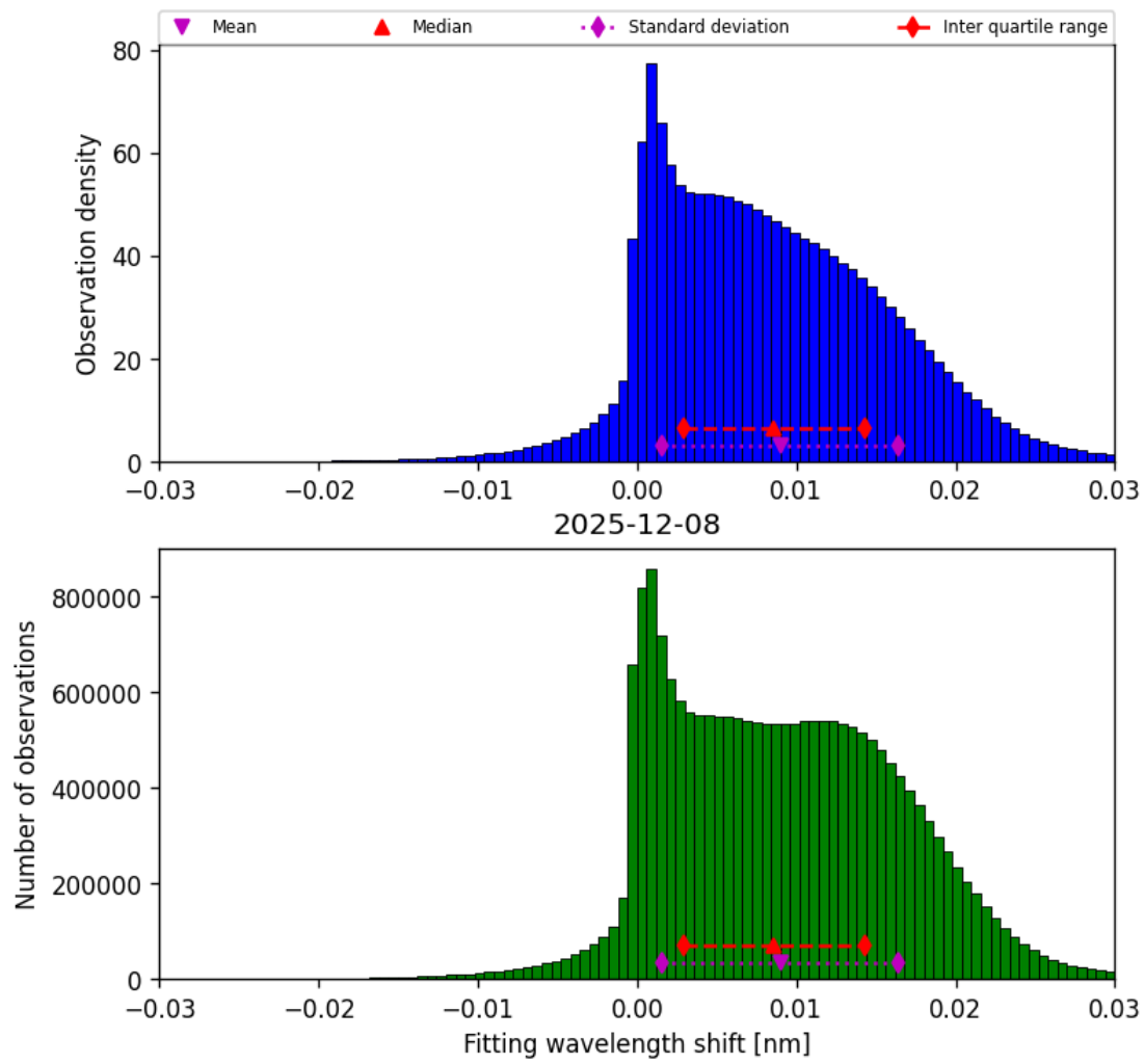
Figure 47: Histogram of “Fitting wavelength shift” for 2025-12-08 to 2025-12-09
