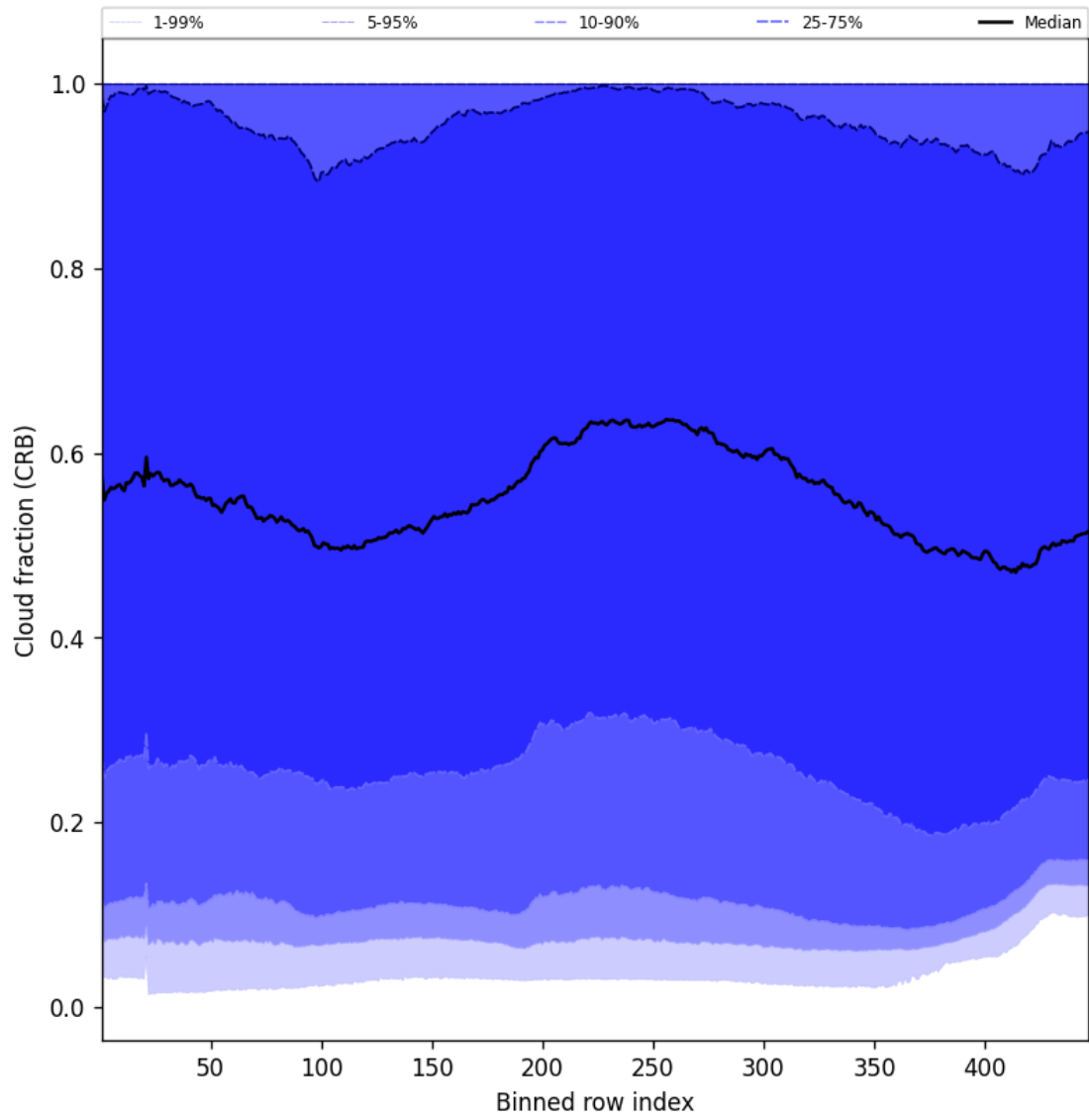
Figure 56: Along track statistics of “Cloud fraction (CRB)” for 2025-12-08 to 2025-12-09
