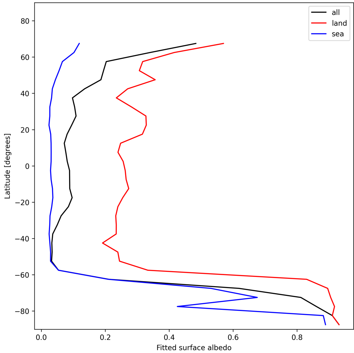
Figure 27: Zonal average of “Fitted surface albedo” for 2025-12-08 to 2025-12-09.
