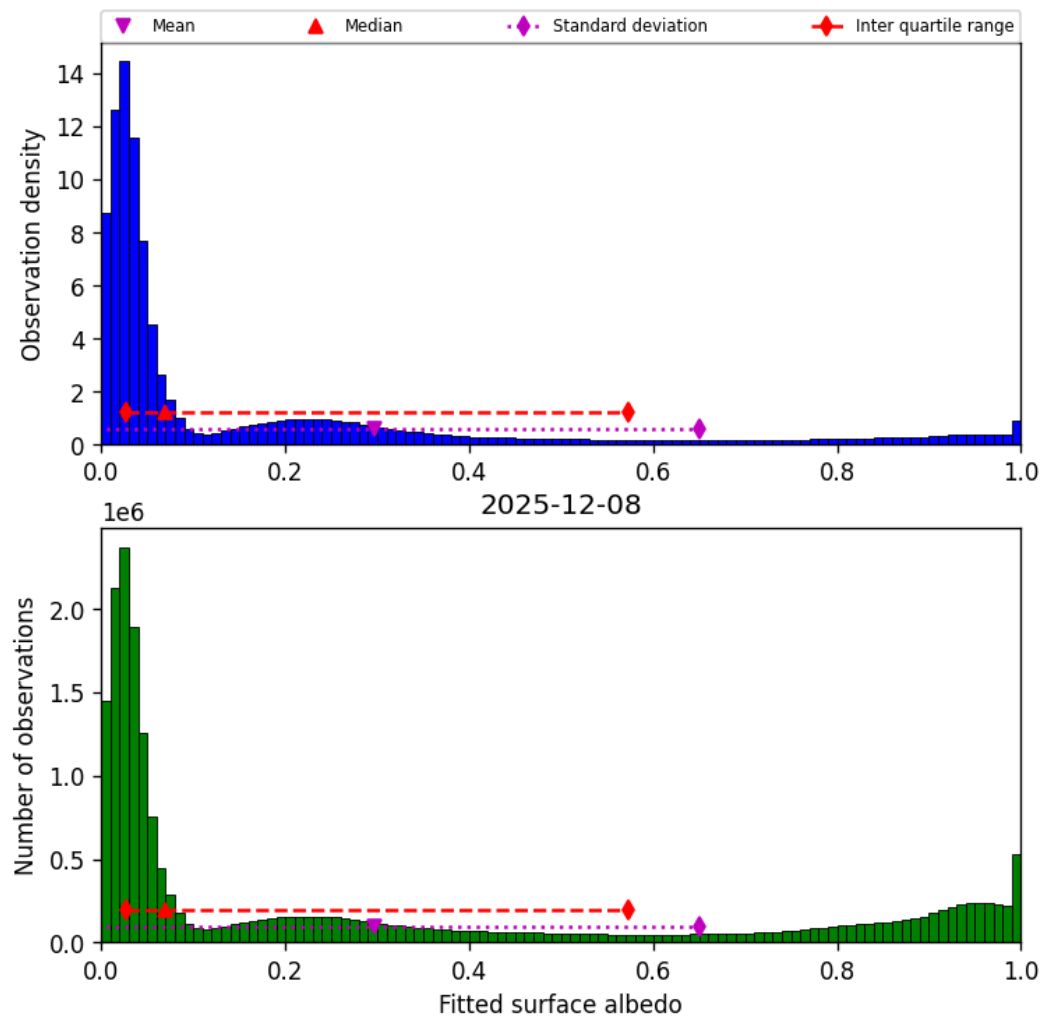
Figure 43: Histogram of “Fitted surface albedo” for 2025-12-08 to 2025-12-09
