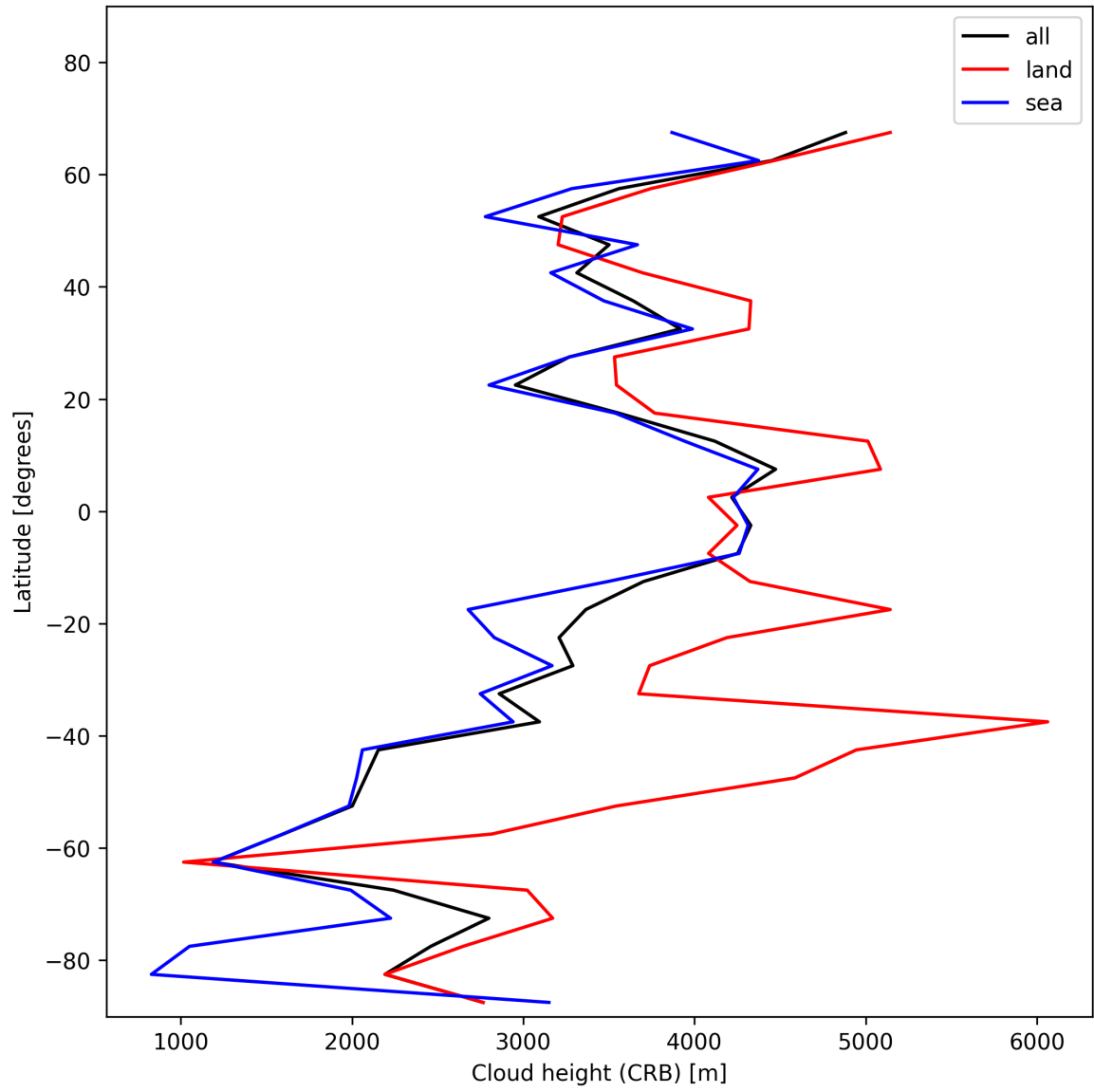
Figure 25: Zonal average of “Cloud height (CRB)” for 2025-12-08 to 2025-12-09.
