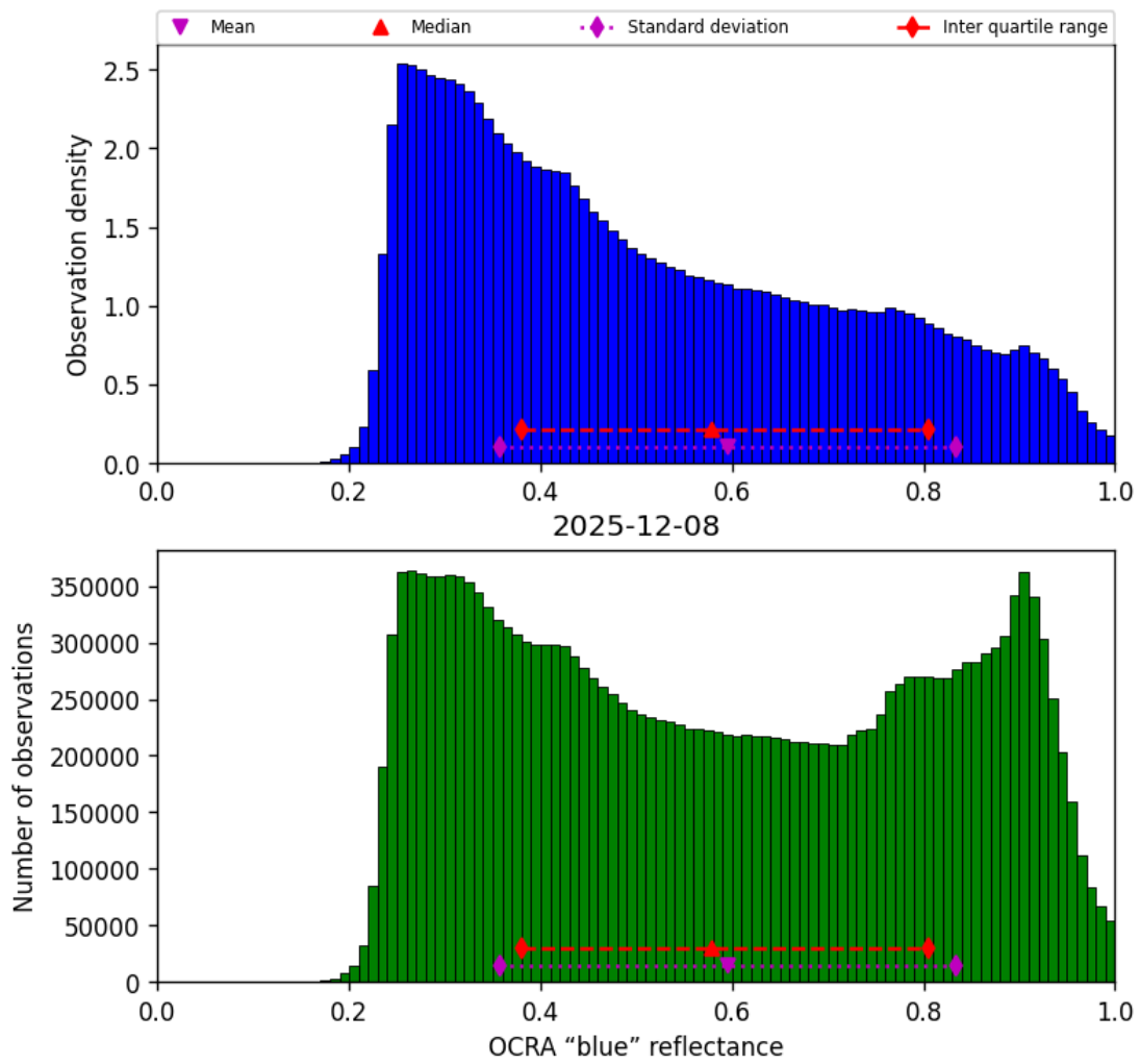
Figure 49: Histogram of “OCRA “blue” reflectance” for 2025-12-08 to 2025-12-09
