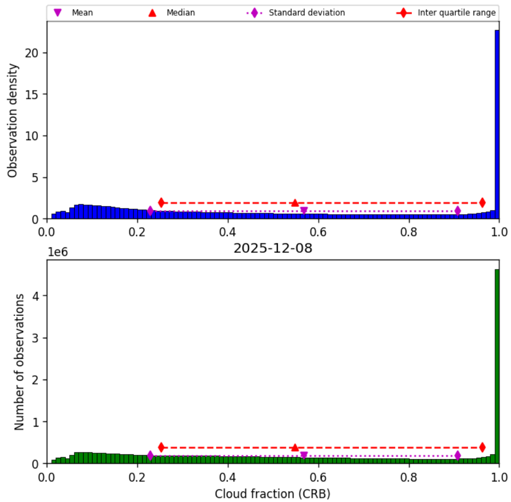
Figure 40: Histogram of “Cloud fraction (CRB)” for 2025-12-08 to 2025-12-09
