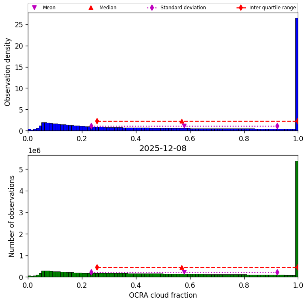
Figure 48: Histogram of “OCRA cloud fraction” for 2025-12-08 to 2025-12-09
