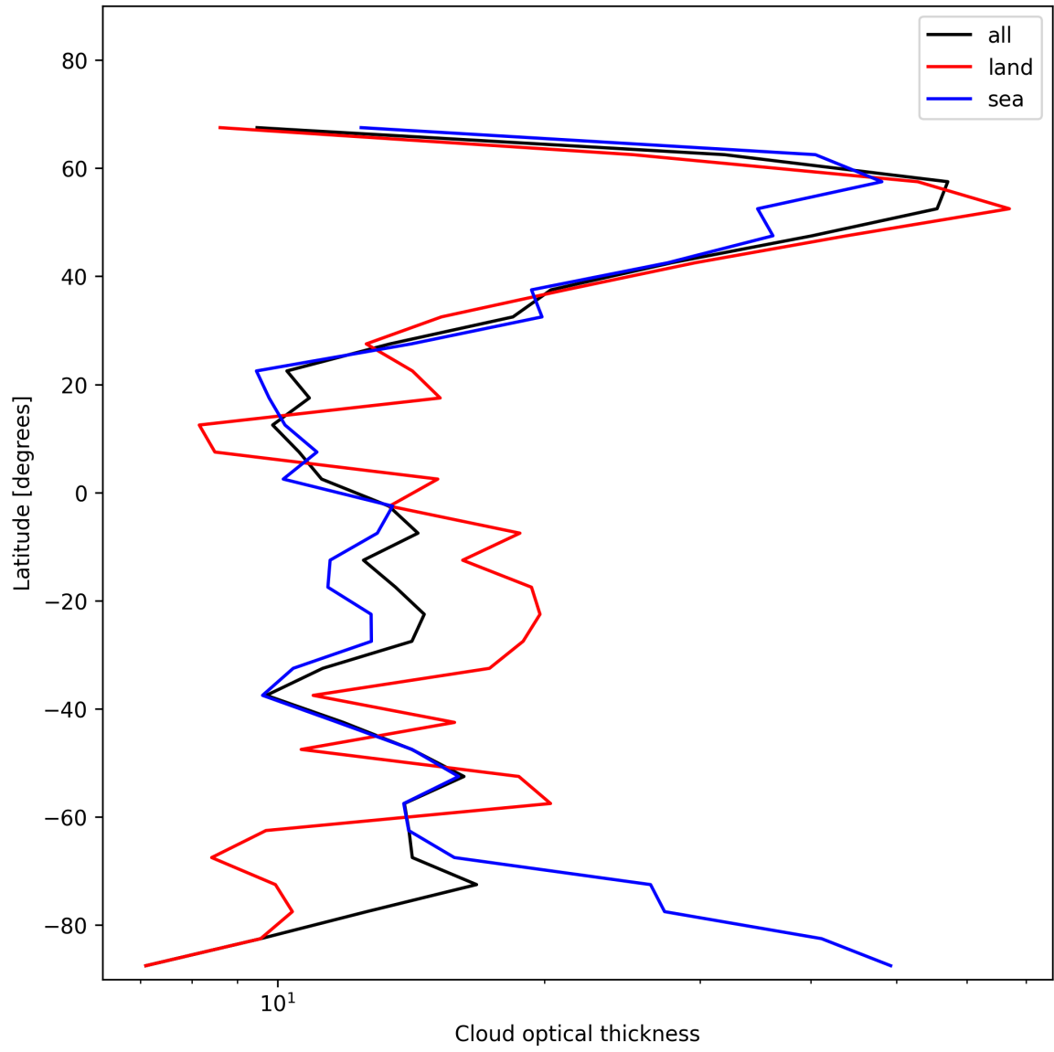
Figure 23: Zonal average of “Cloud optical thickness” for 2025-12-08 to 2025-12-09.
