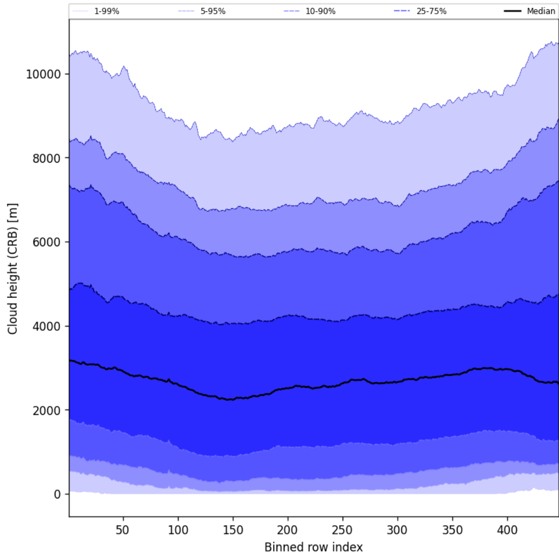
Figure 57: Along track statistics of “Cloud height (CRB)” for 2025-12-08 to 2025-12-09
