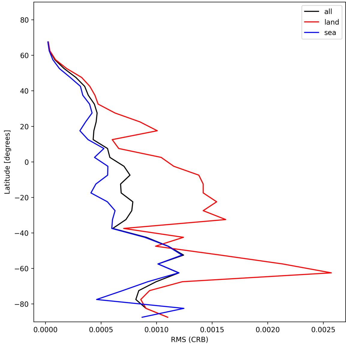
Figure 30: Zonal average of “RMS (CRB)” for 2025-12-08 to 2025-12-09.
