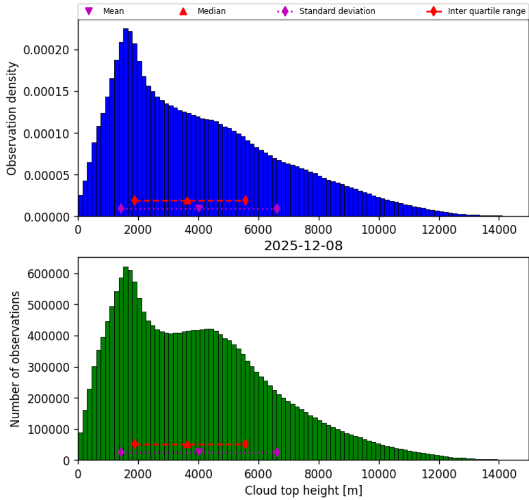
Figure 38: Histogram of “Cloud top height” for 2025-12-08 to 2025-12-09
