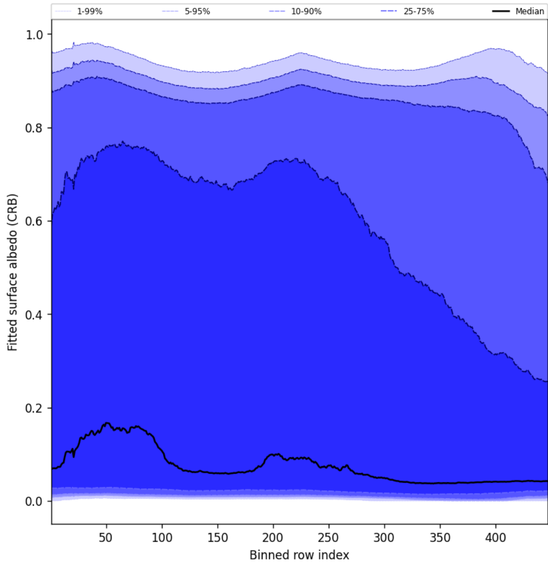
Figure 60: Along track statistics of “Fitted surface albedo (CRB)” for 2025-12-08 to 2025-12-09
