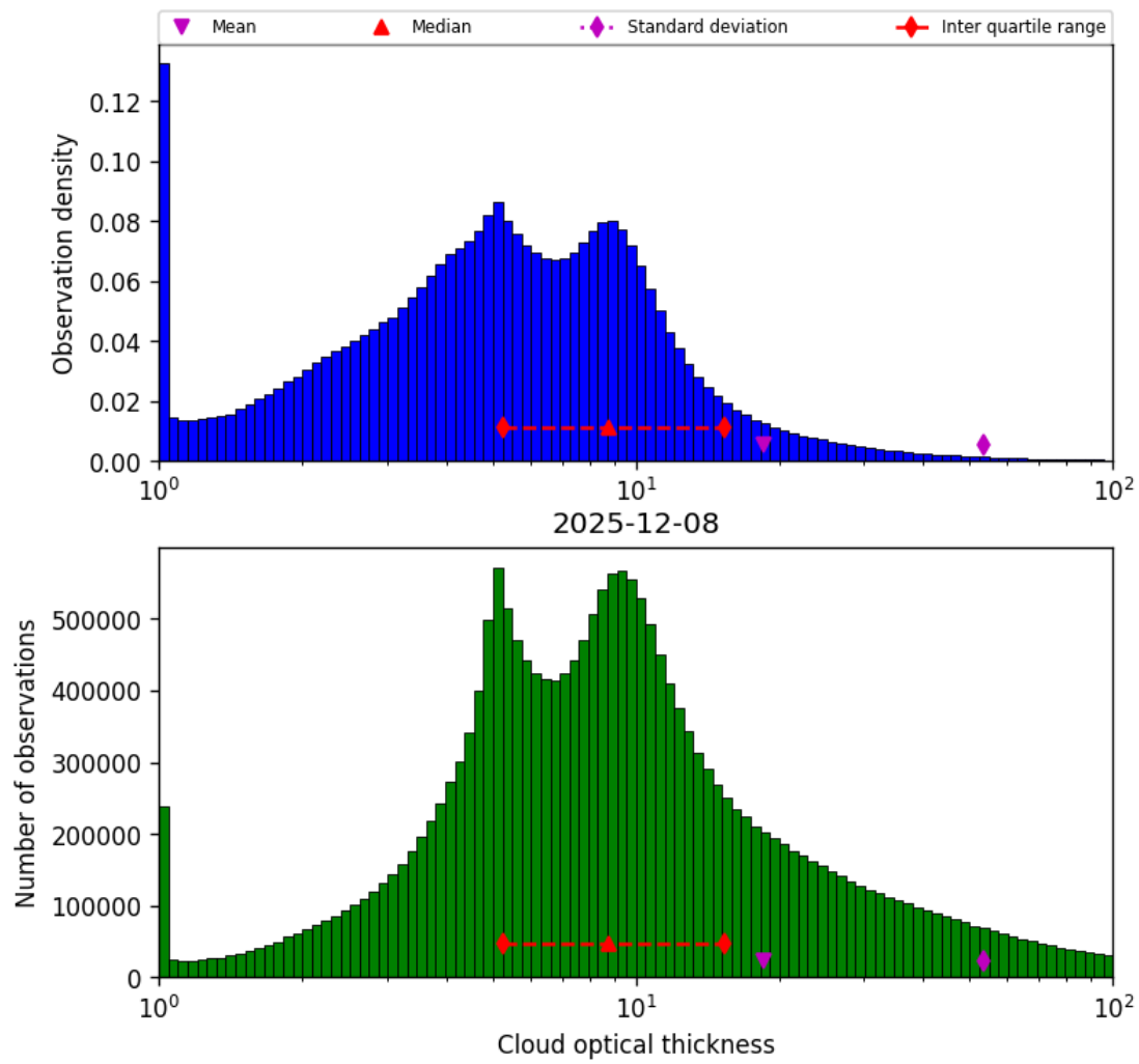
Figure 39: Histogram of “Cloud optical thickness” for 2025-12-08 to 2025-12-09
