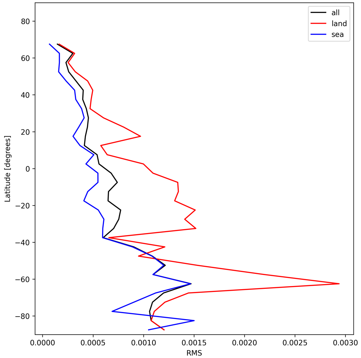
Figure 29: Zonal average of “RMS” for 2025-12-08 to 2025-12-09.
