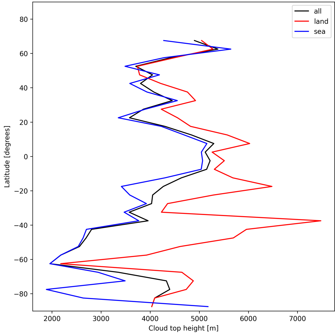
Figure 22: Zonal average of “Cloud top height” for 2025-12-08 to 2025-12-09.
