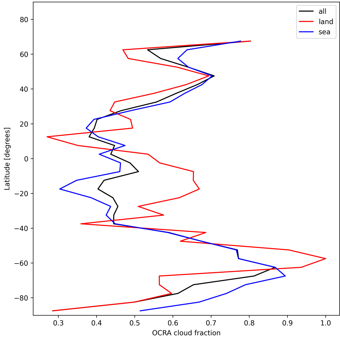
Figure 32: Zonal average of “OCRA cloud fraction” for 2025-12-08 to 2025-12-09.
