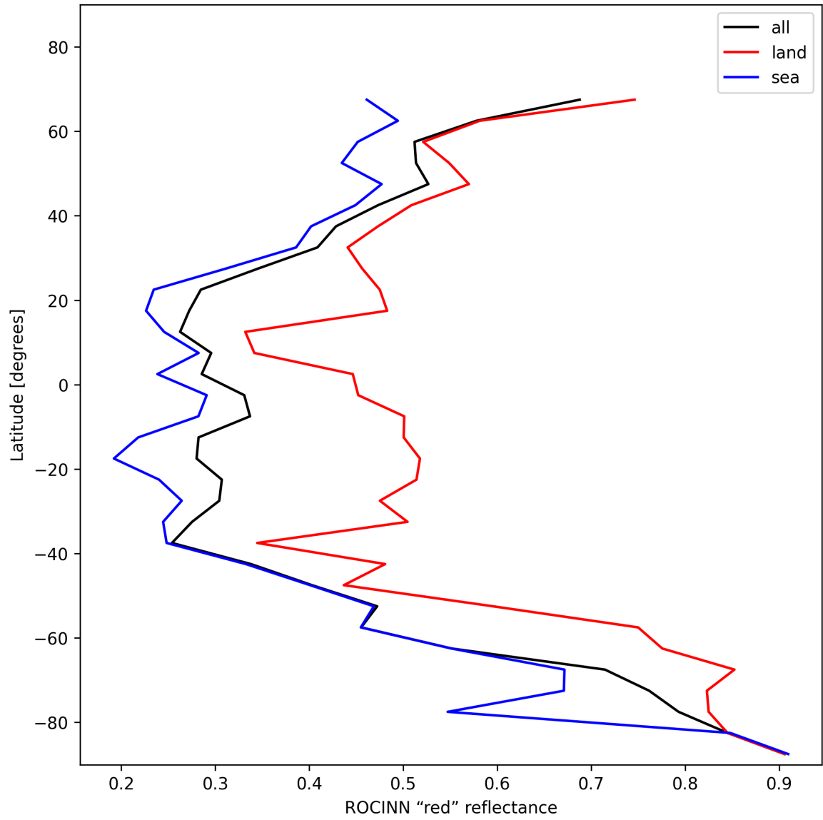
Figure 35: Zonal average of “ROCINN “red” reflectance” for 2025-12-08 to 2025-12-09.
