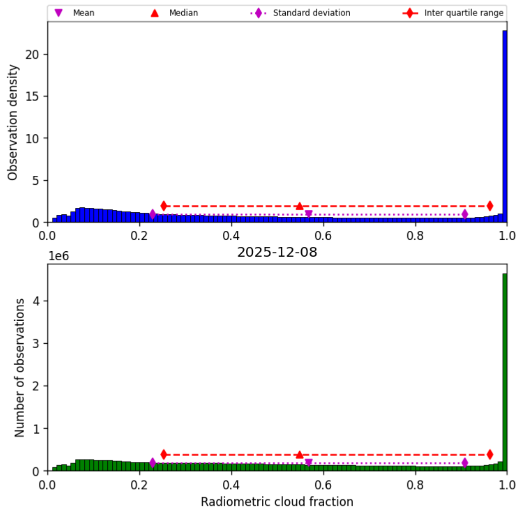
Figure 37: Histogram of “Radiometric cloud fraction” for 2025-12-08 to 2025-12-09
