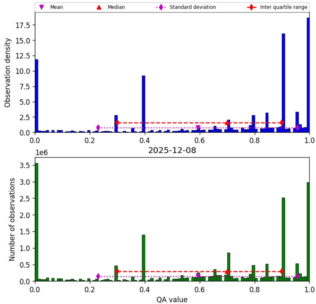
Figure 36: Histogram of “QA value” for 2025-12-08 to 2025-12-09
