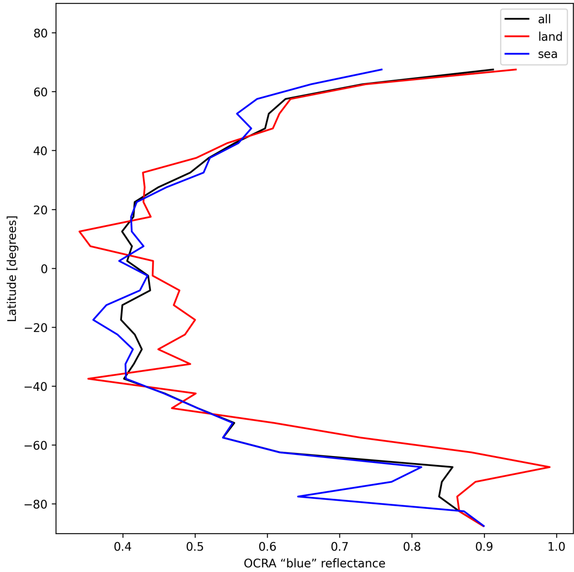
Figure 33: Zonal average of “OCRA “blue” reflectance” for 2025-12-08 to 2025-12-09.
