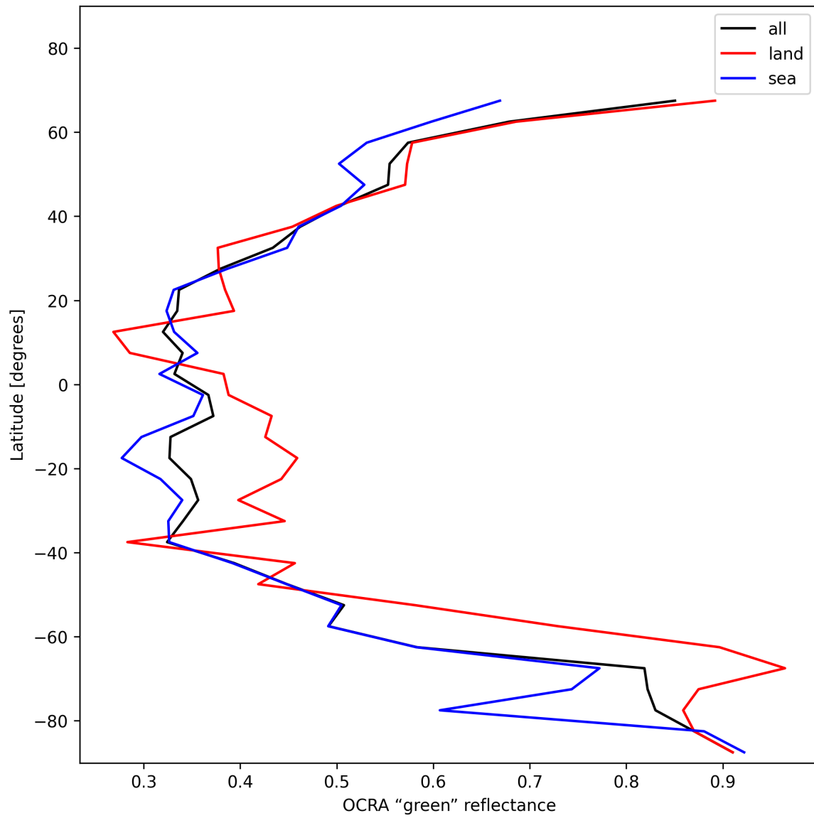
Figure 34: Zonal average of “OCRA “green” reflectance” for 2025-12-08 to 2025-12-09.
