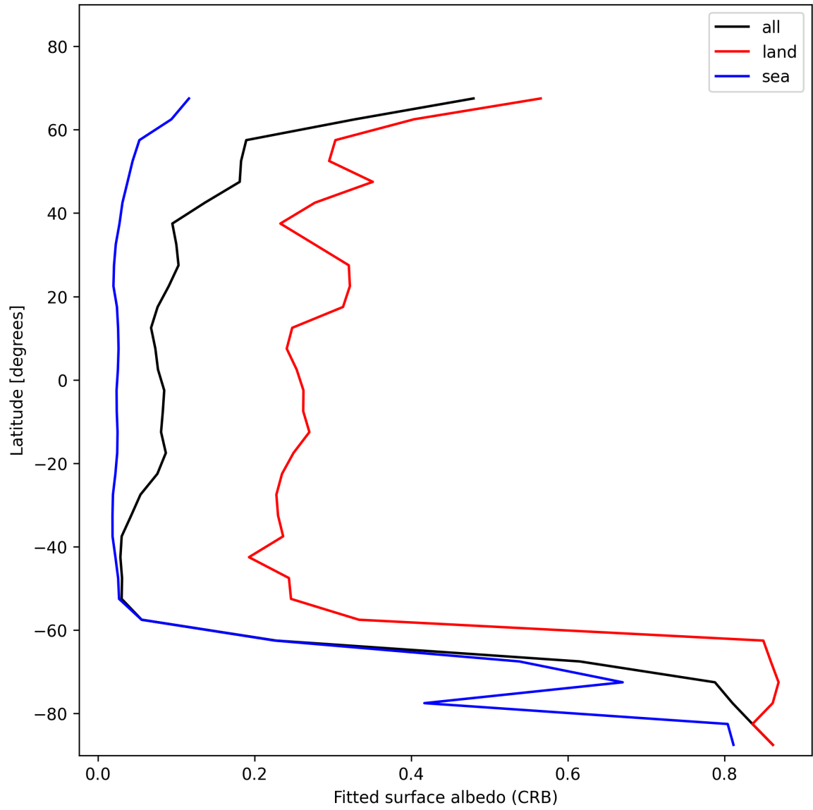
Figure 28: Zonal average of “Fitted surface albedo (CRB)” for 2025-12-08 to 2025-12-09.
