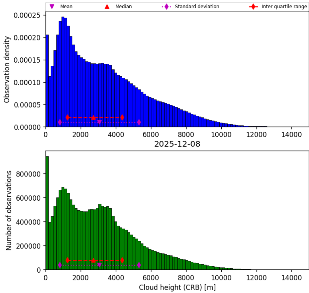
Figure 41: Histogram of “Cloud height (CRB)” for 2025-12-08 to 2025-12-09
