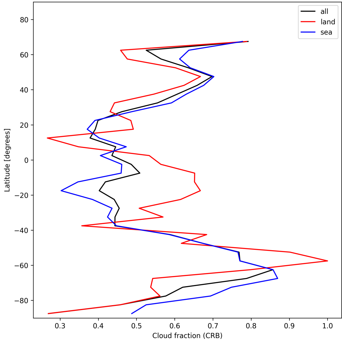
Figure 24: Zonal average of “Cloud fraction (CRB)” for 2025-12-08 to 2025-12-09.
