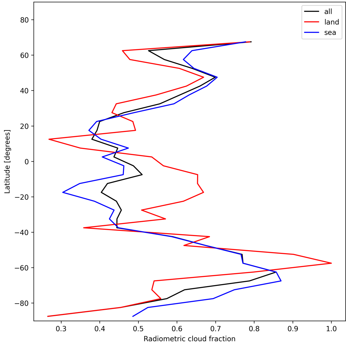
Figure 21: Zonal average of “Radiometric cloud fraction” for 2025-12-08 to 2025-12-09.
