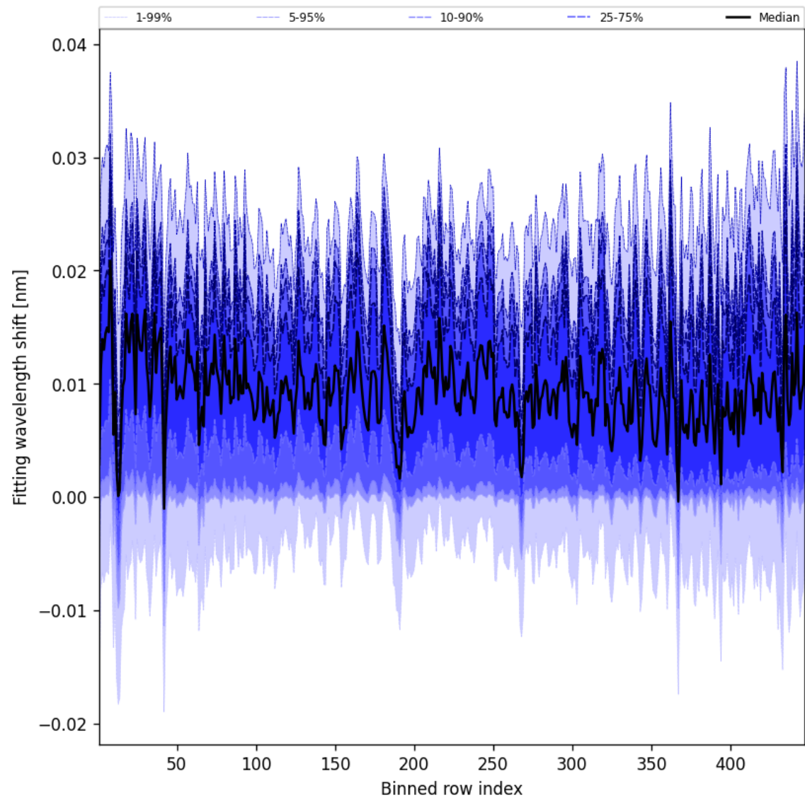
Figure 63: Along track statistics of “Fitting wavelength shift” for 2025-12-08 to 2025-12-09
