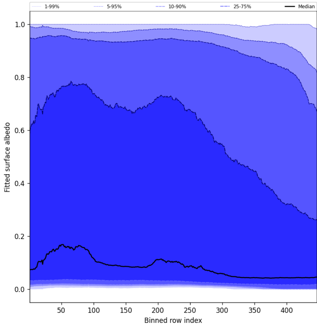
Figure 59: Along track statistics of “Fitted surface albedo” for 2025-12-08 to 2025-12-09
