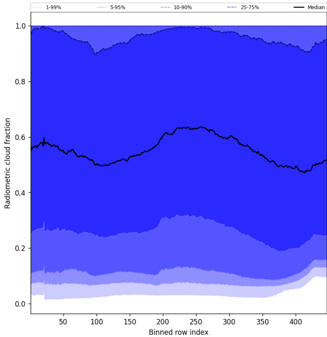
Figure 53: Along track statistics of “Radiometric cloud fraction” for 2025-12-08 to 2025-12-09
