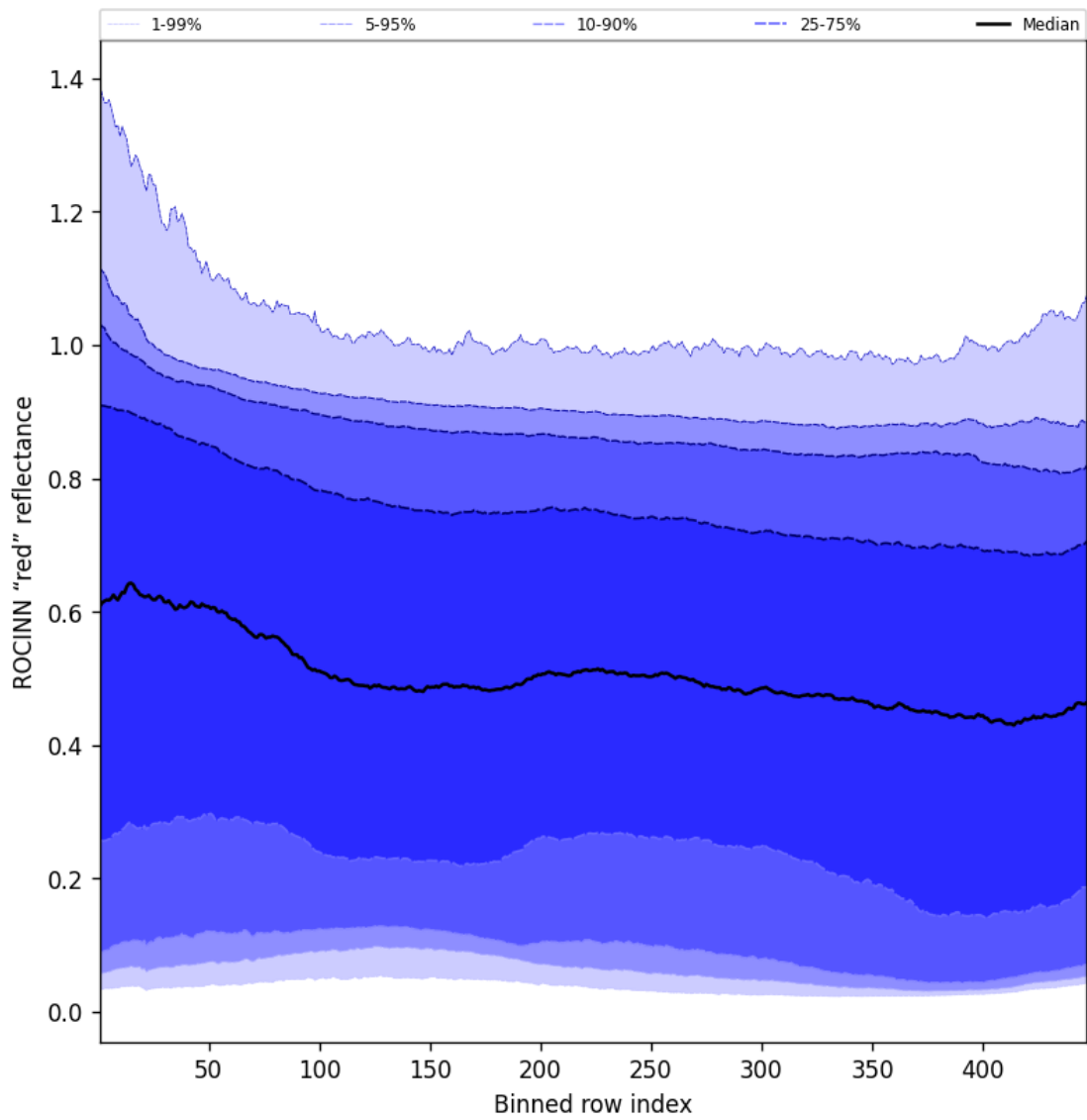
Figure 67: Along track statistics of “ROCINN “red” reflectance” for 2025-12-08 to 2025-12-09
