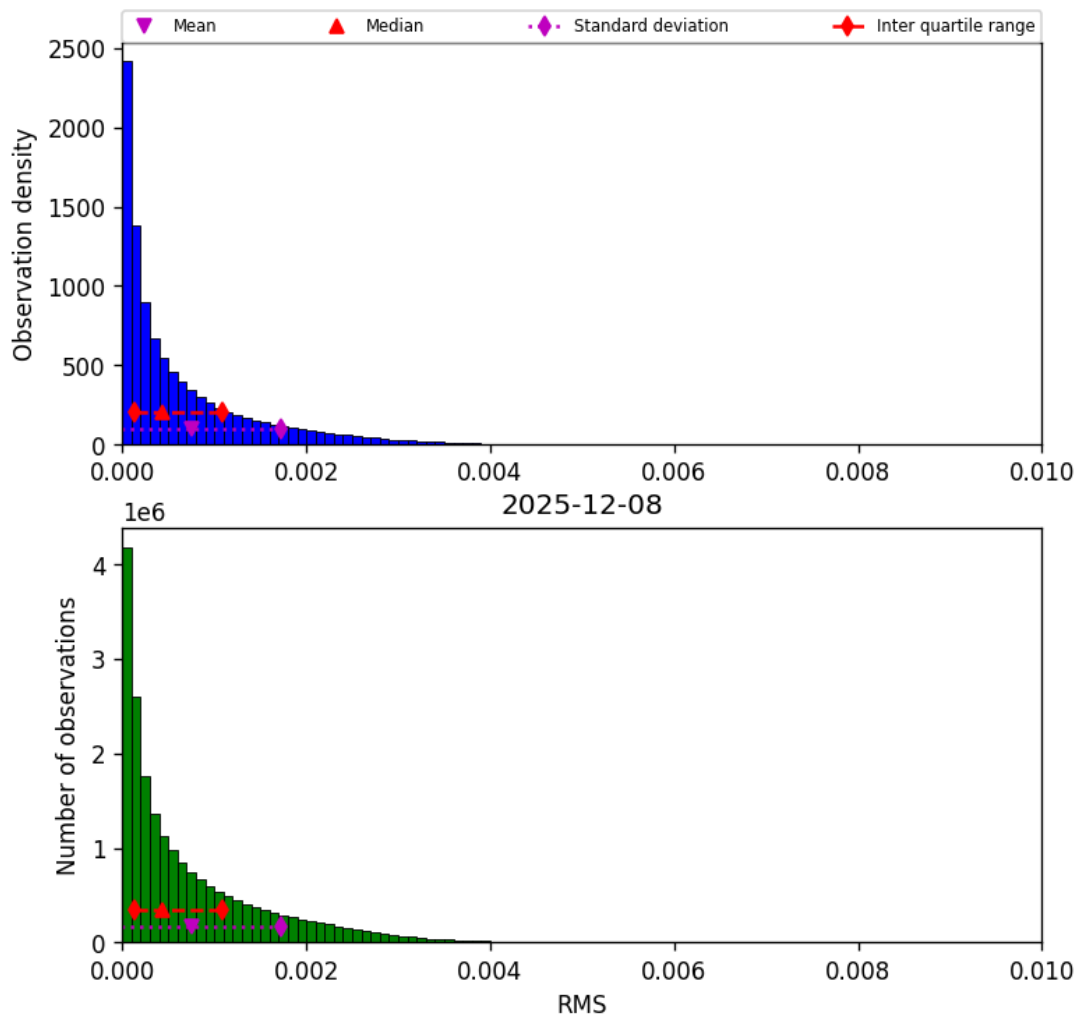
Figure 45: Histogram of “RMS” for 2025-12-08 to 2025-12-09
