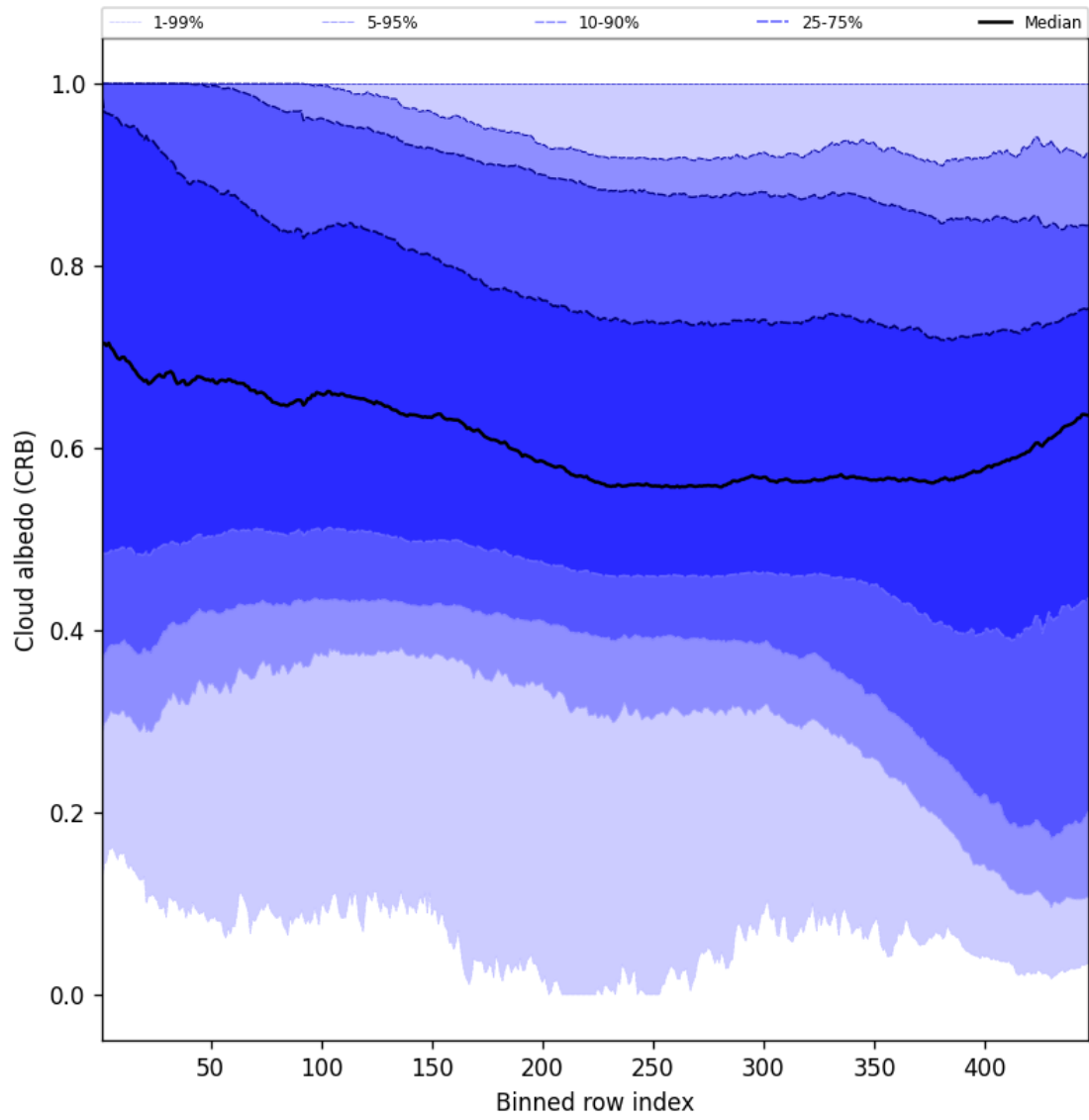
Figure 58: Along track statistics of “Cloud albedo (CRB)” for 2025-12-11 to 2025-12-12
