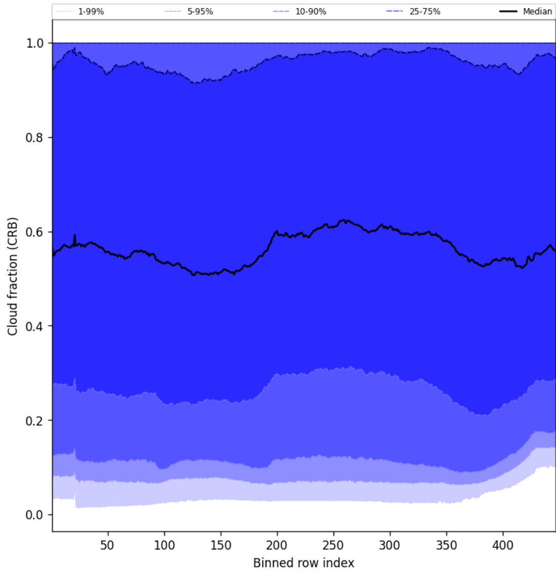
Figure 56: Along track statistics of “Cloud fraction (CRB)” for 2025-12-11 to 2025-12-12
