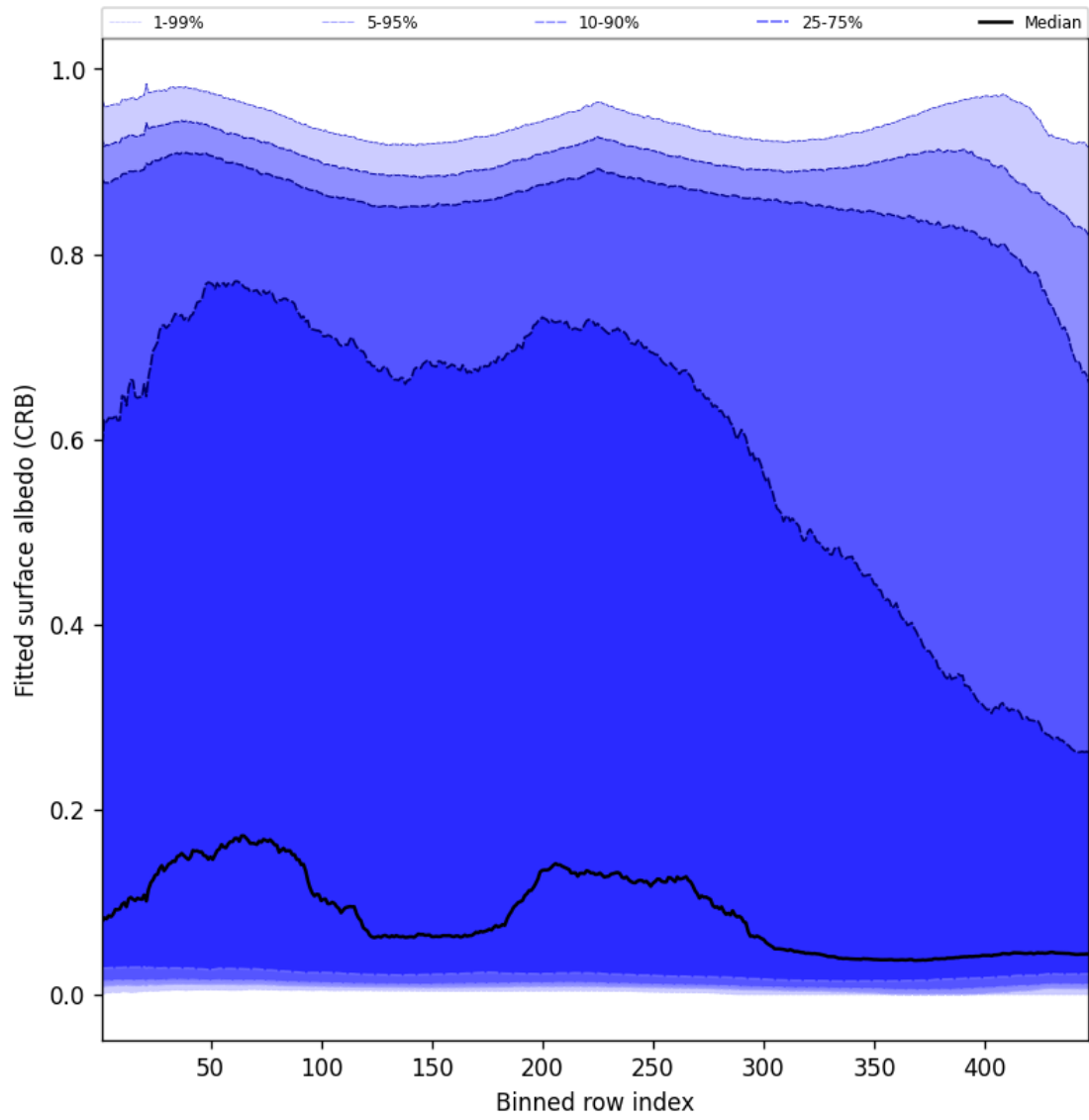
Figure 60: Along track statistics of “Fitted surface albedo (CRB)” for 2025-12-11 to 2025-12-12
