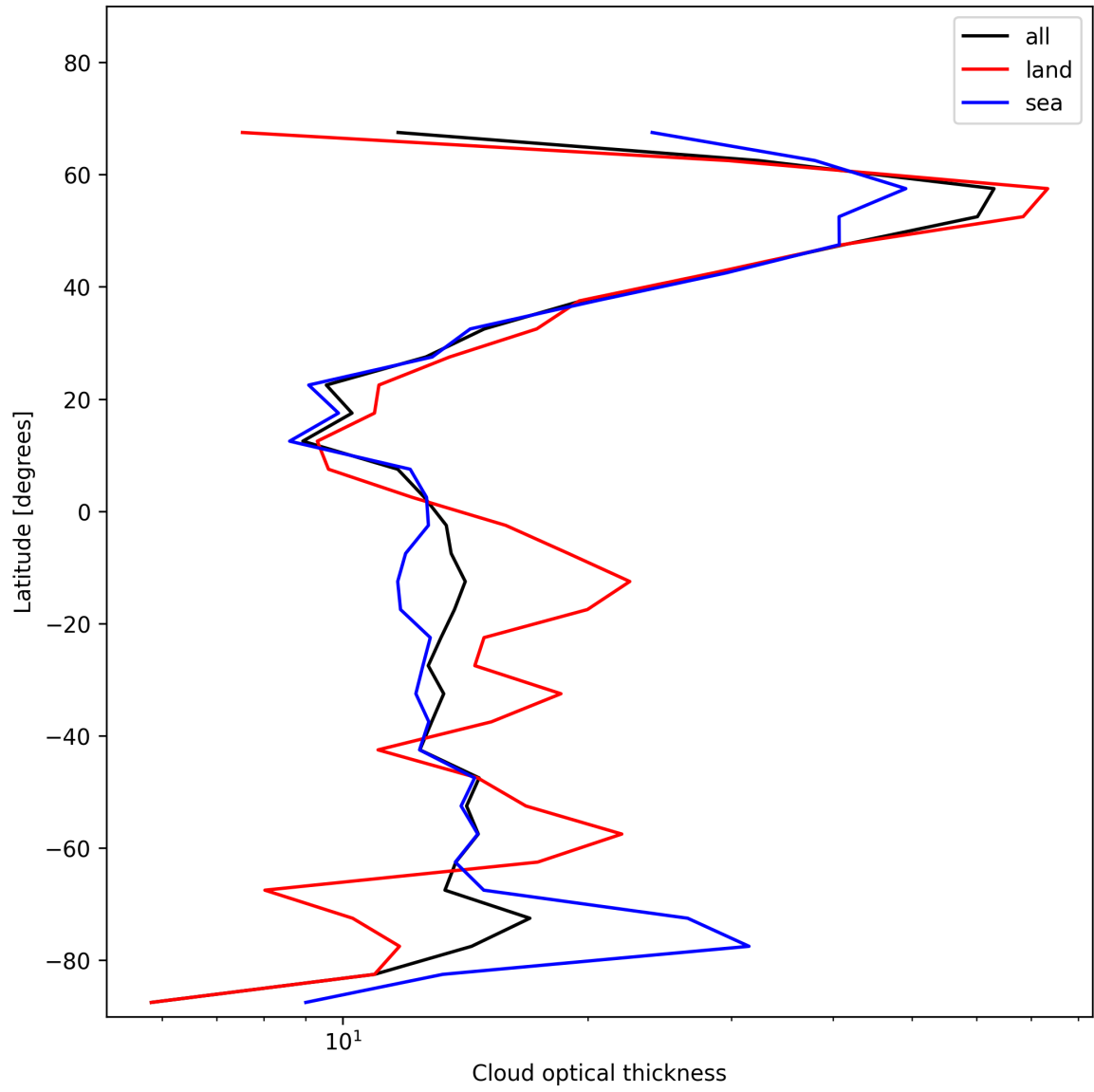
Figure 23: Zonal average of “Cloud optical thickness” for 2025-12-11 to 2025-12-12.
