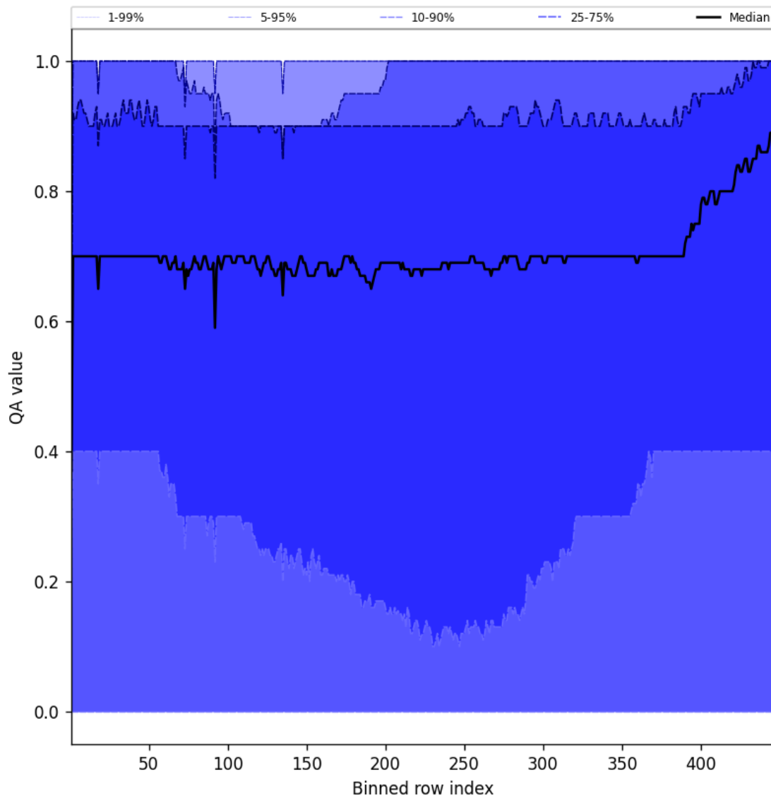
Figure 52: Along track statistics of “QA value” for 2025-12-11 to 2025-12-12
