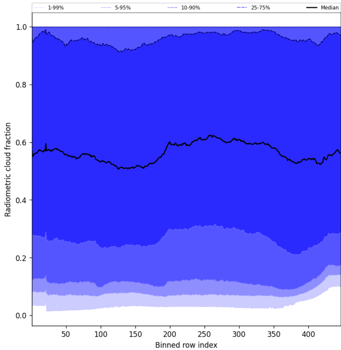
Figure 53: Along track statistics of “Radiometric cloud fraction” for 2025-12-11 to 2025-12-12
