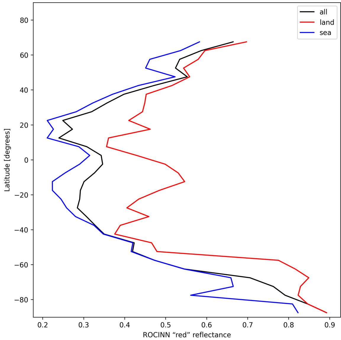
Figure 35: Zonal average of “ROCINN “red” reflectance” for 2025-12-11 to 2025-12-12.
