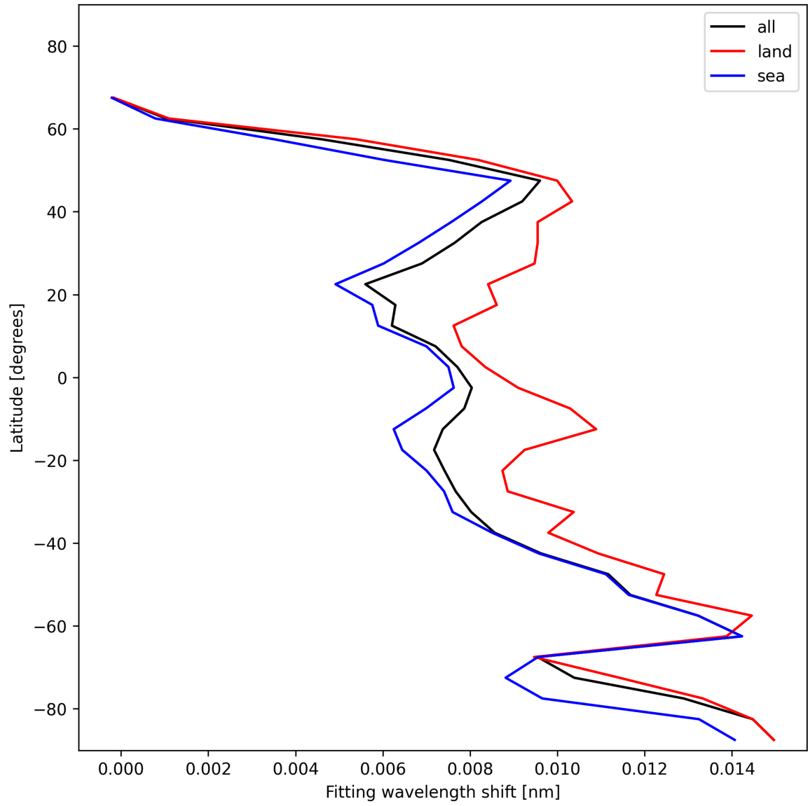
Figure 31: Zonal average of “Fitting wavelength shift” for 2025-12-11 to 2025-12-12.
