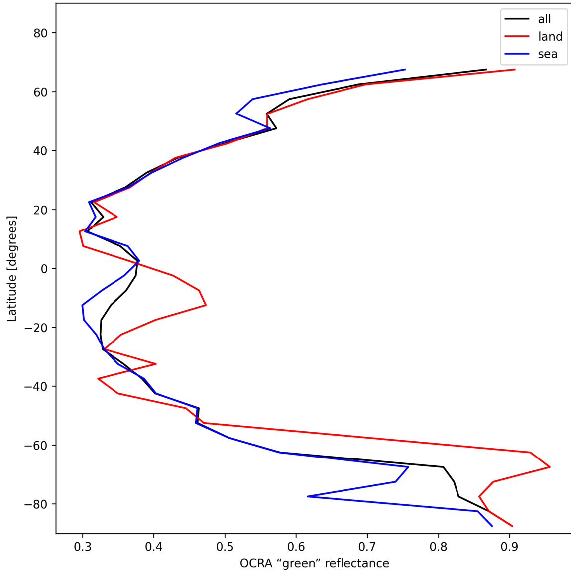
Figure 34: Zonal average of “OCRA “green” reflectance” for 2025-12-11 to 2025-12-12.
