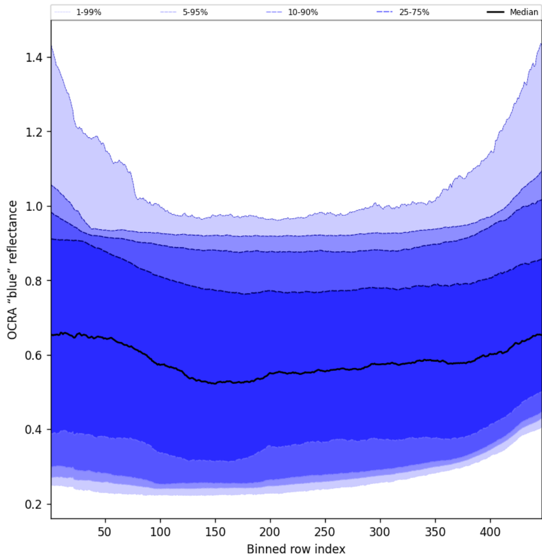
Figure 65: Along track statistics of “OCRA “blue” reflectance” for 2025-12-11 to 2025-12-12
