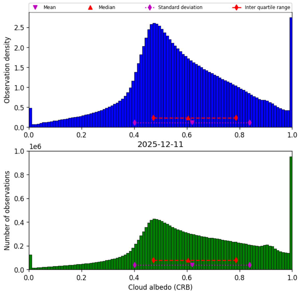
Figure 42: Histogram of “Cloud albedo (CRB)” for 2025-12-11 to 2025-12-12
