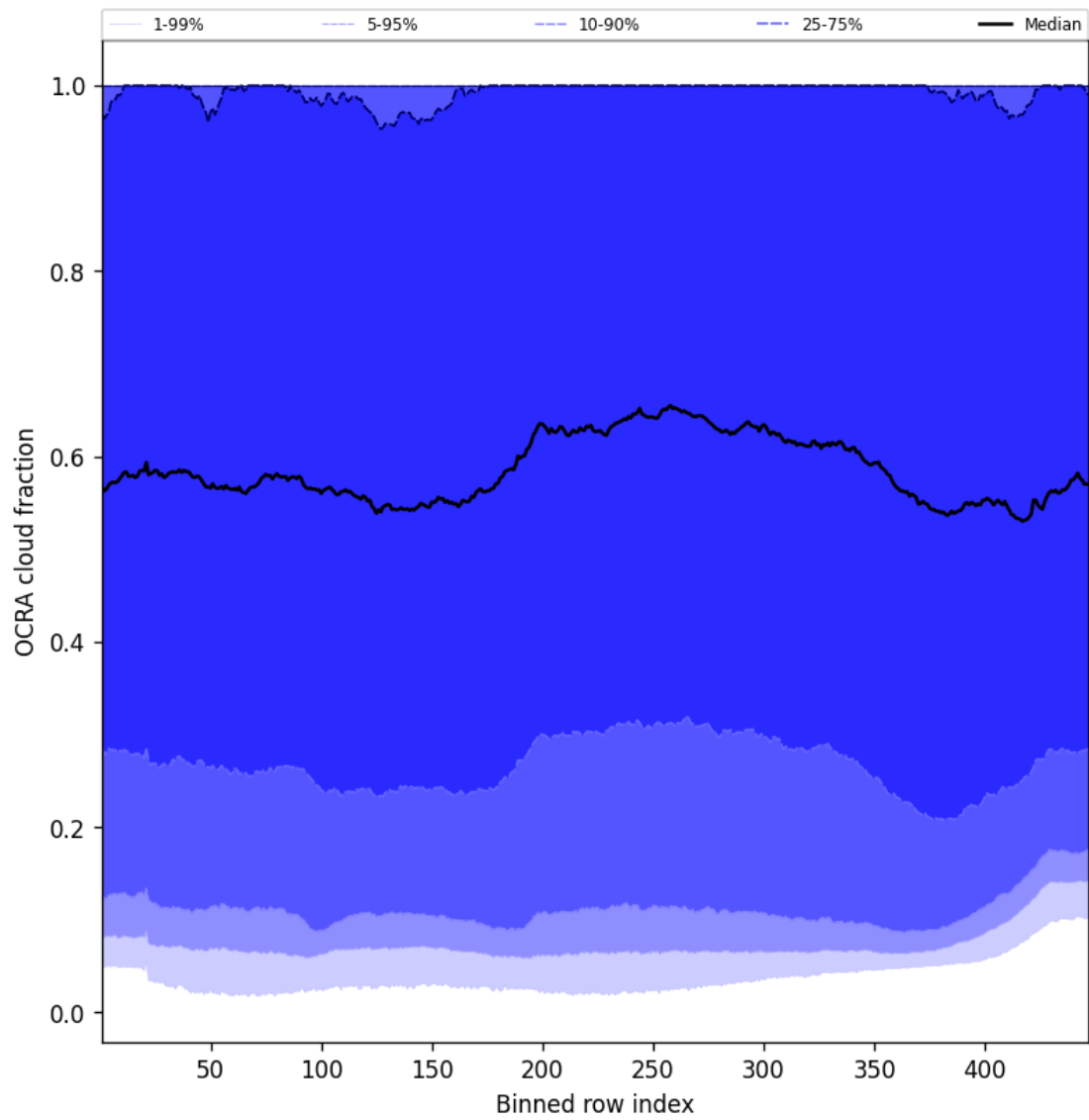
Figure 64: Along track statistics of “OCRA cloud fraction” for 2025-12-11 to 2025-12-12
