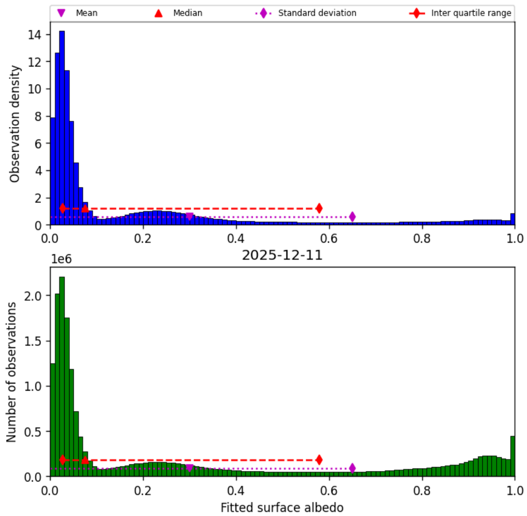
Figure 43: Histogram of “Fitted surface albedo” for 2025-12-11 to 2025-12-12
