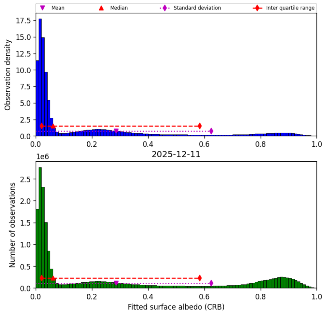
Figure 44: Histogram of “Fitted surface albedo (CRB)” for 2025-12-11 to 2025-12-12
