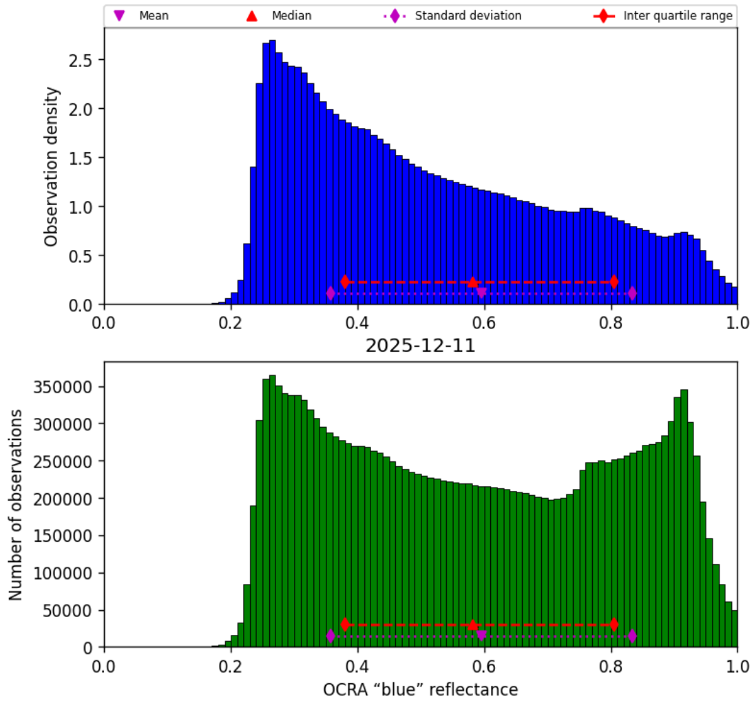
Figure 49: Histogram of “OCRA “blue” reflectance” for 2025-12-11 to 2025-12-12
