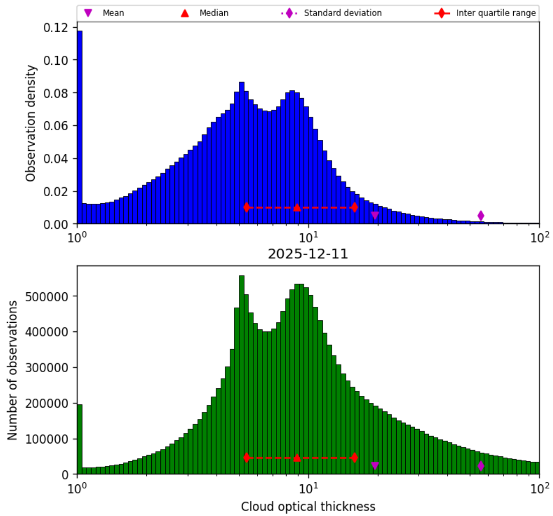
Figure 39: Histogram of “Cloud optical thickness” for 2025-12-11 to 2025-12-12
