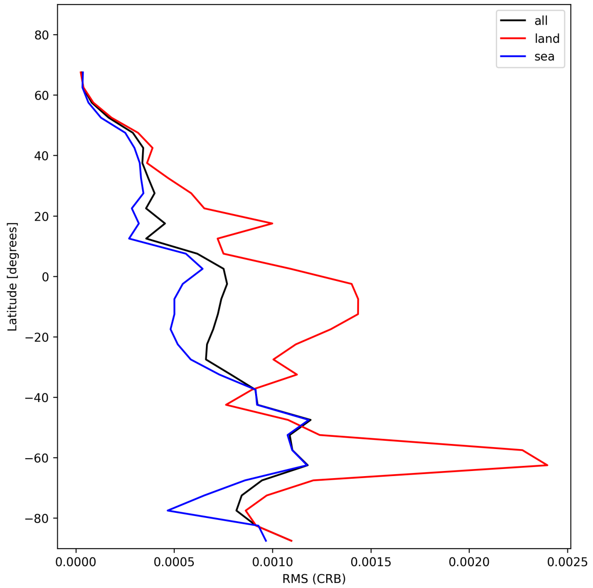
Figure 30: Zonal average of “RMS (CRB)” for 2025-12-11 to 2025-12-12.
