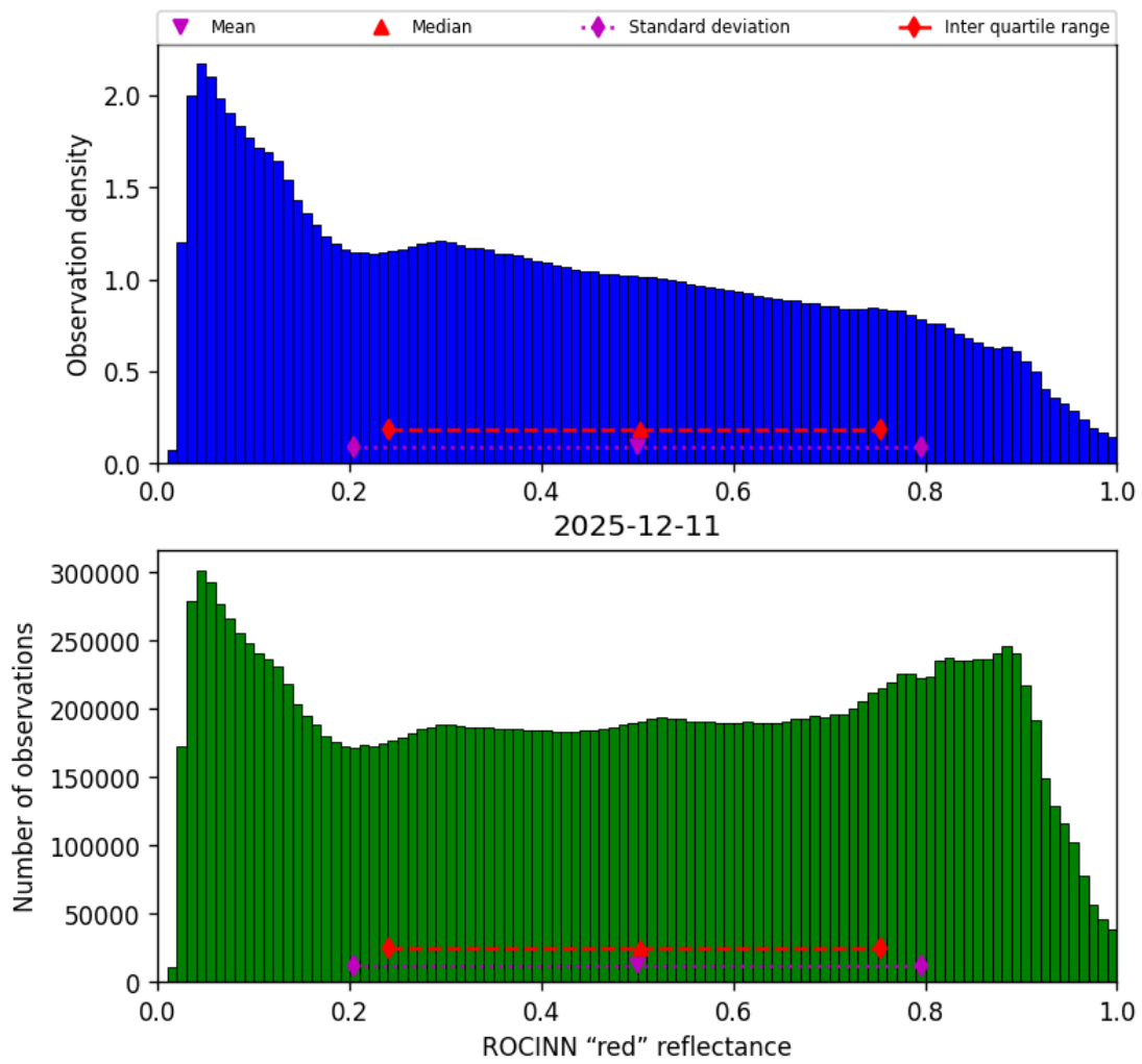
Figure 51: Histogram of “ROCINN “red” reflectance” for 2025-12-11 to 2025-12-12
