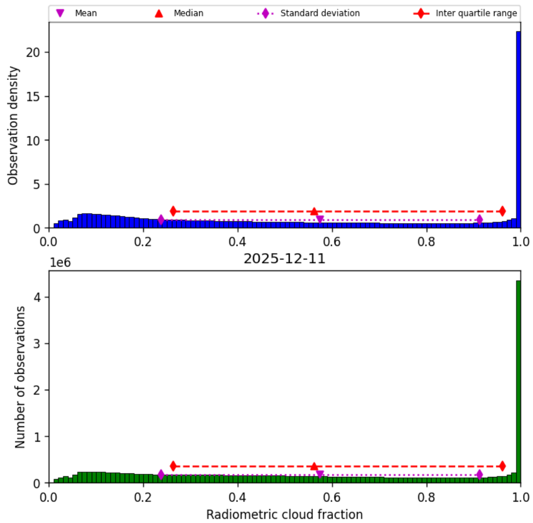
Figure 37: Histogram of “Radiometric cloud fraction” for 2025-12-11 to 2025-12-12
