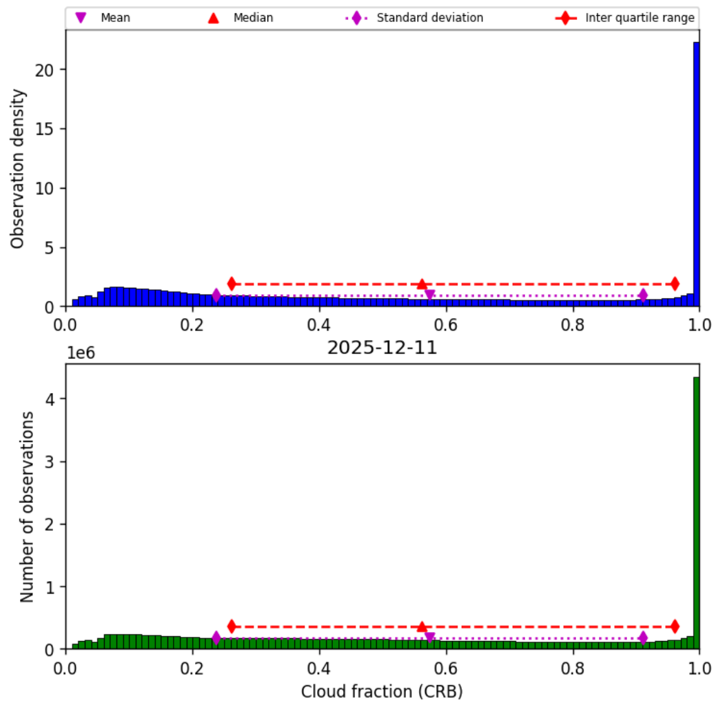
Figure 40: Histogram of “Cloud fraction (CRB)” for 2025-12-11 to 2025-12-12
