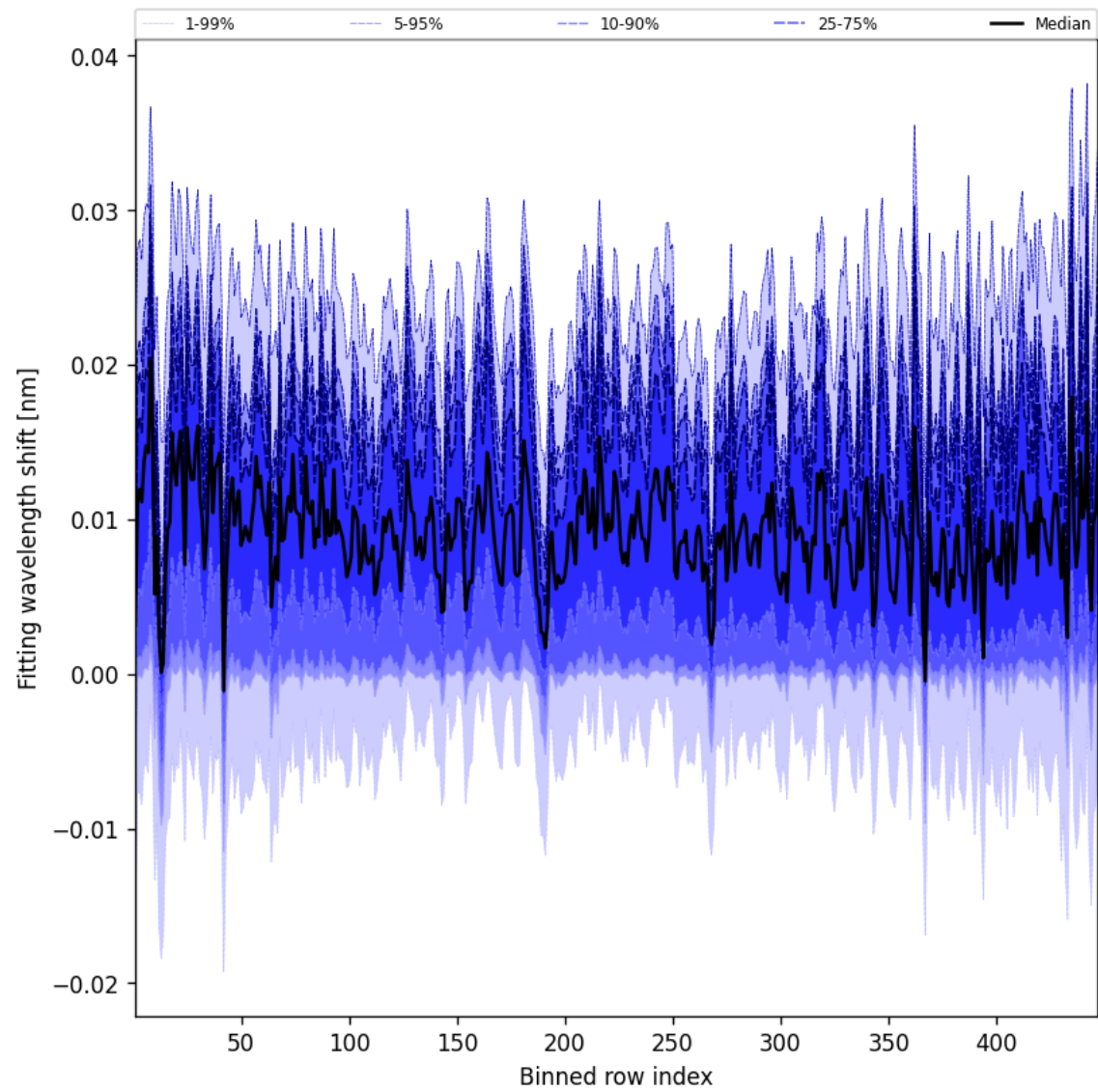
Figure 63: Along track statistics of “Fitting wavelength shift” for 2025-12-11 to 2025-12-12
