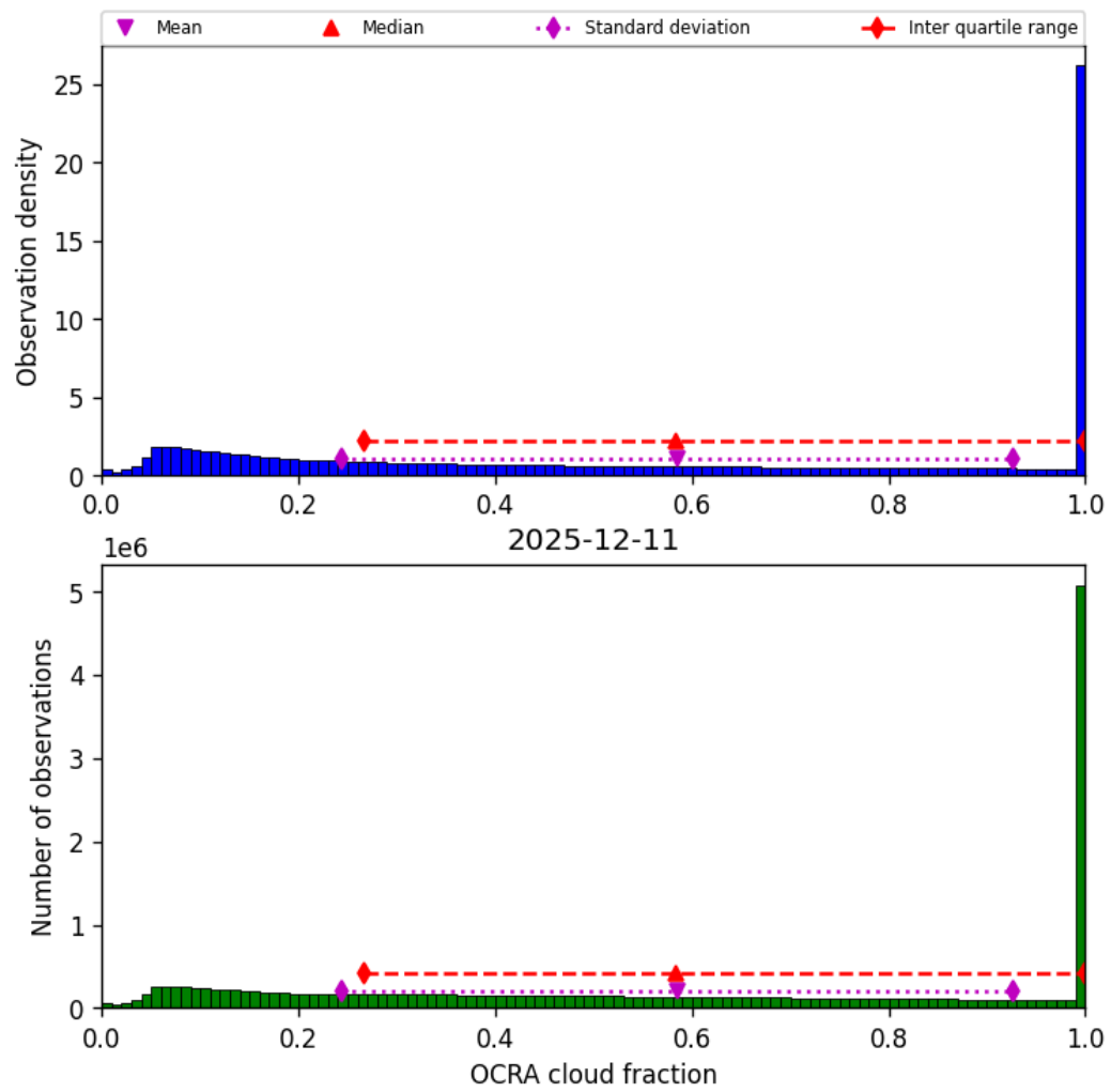
Figure 48: Histogram of “OCRA cloud fraction” for 2025-12-11 to 2025-12-12
