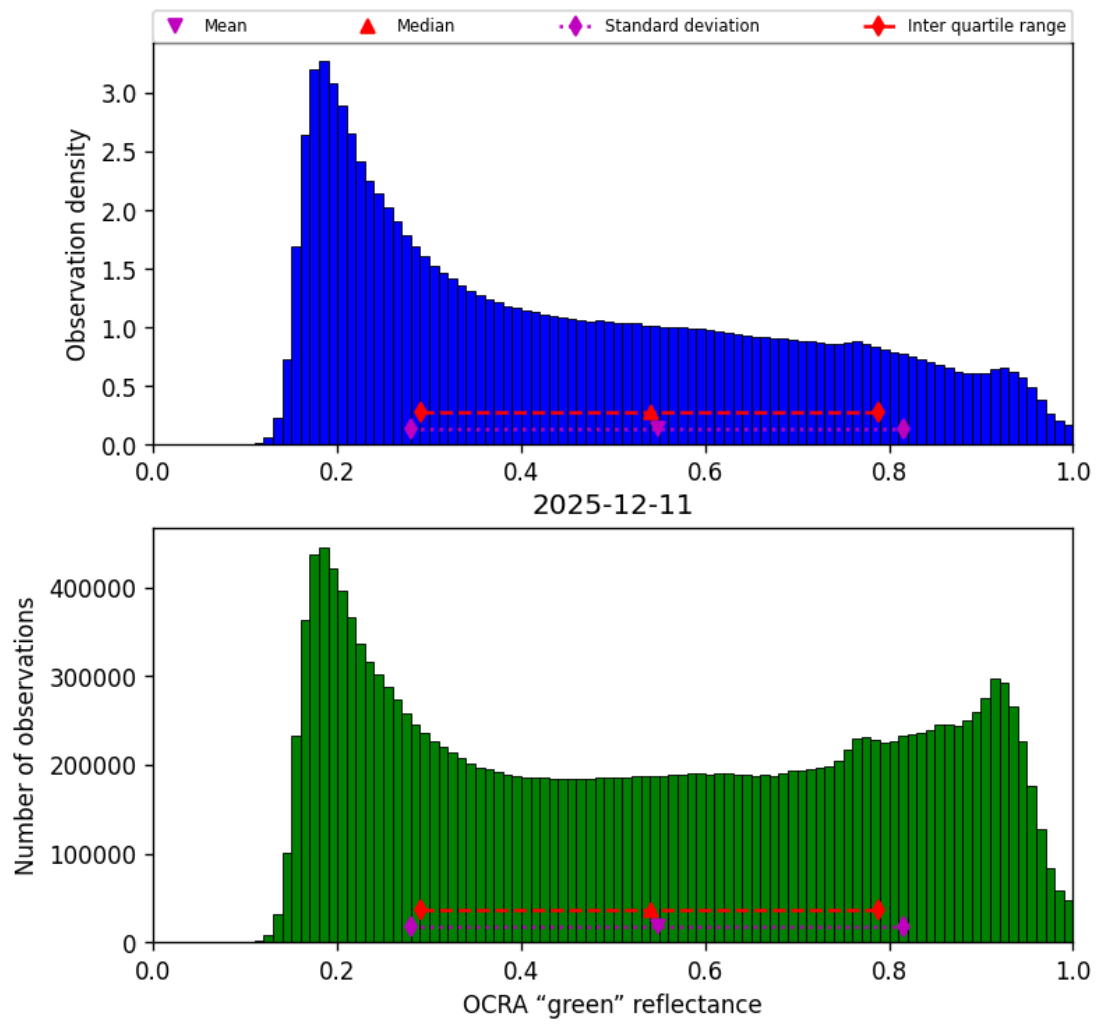
Figure 50: Histogram of “OCRA “green” reflectance” for 2025-12-11 to 2025-12-12
