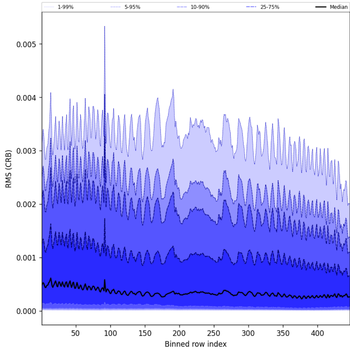
Figure 62: Along track statistics of “RMS (CRB)” for 2025-12-11 to 2025-12-12
