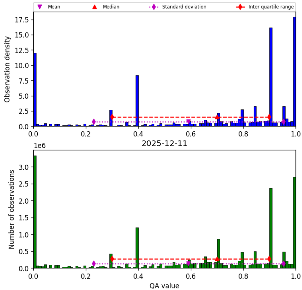
Figure 36: Histogram of “QA value” for 2025-12-11 to 2025-12-12
