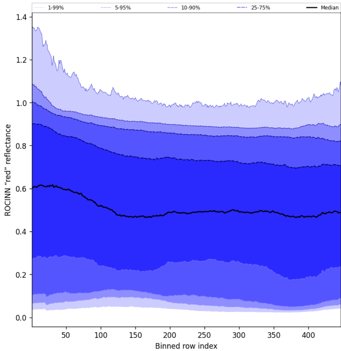
Figure 67: Along track statistics of “ROCINN “red” reflectance” for 2025-12-11 to 2025-12-12
