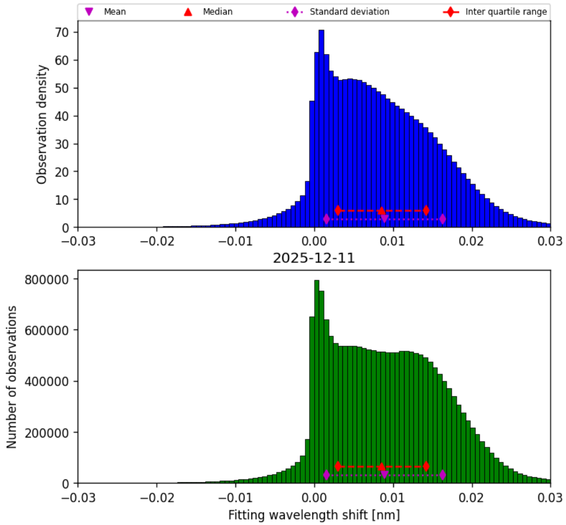
Figure 47: Histogram of “Fitting wavelength shift” for 2025-12-11 to 2025-12-12
