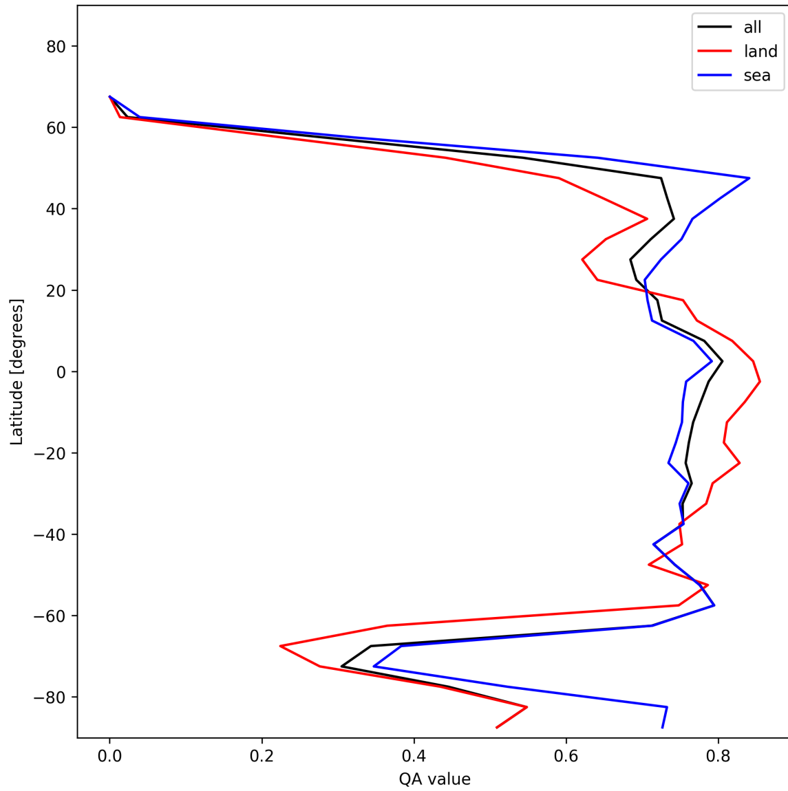
Figure 20: Zonal average of “QA value” for 2025-12-11 to 2025-12-12.
