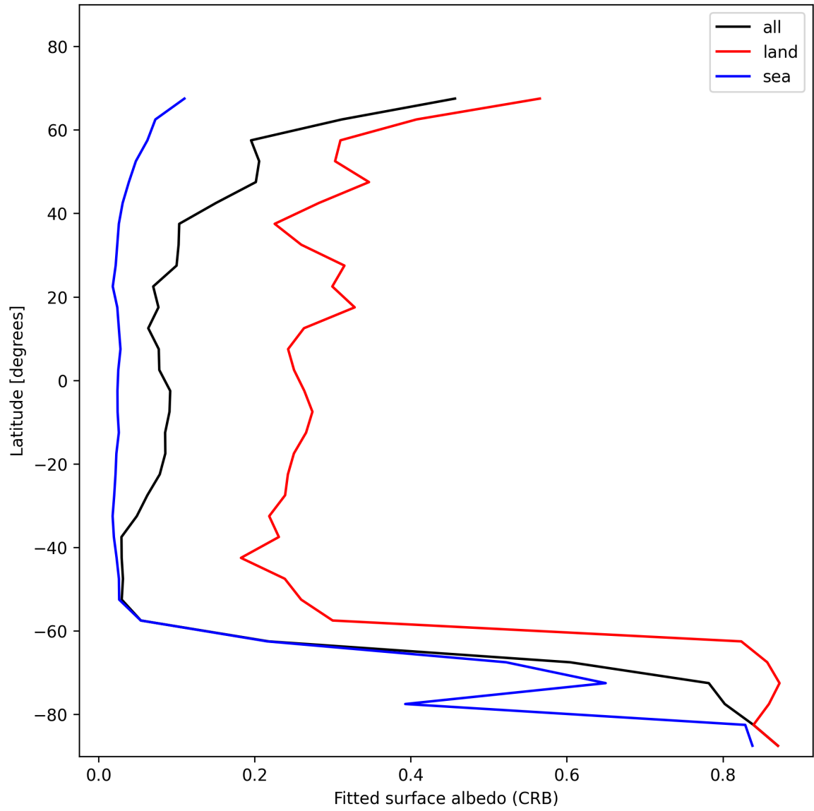
Figure 28: Zonal average of “Fitted surface albedo (CRB)” for 2025-12-11 to 2025-12-12.
