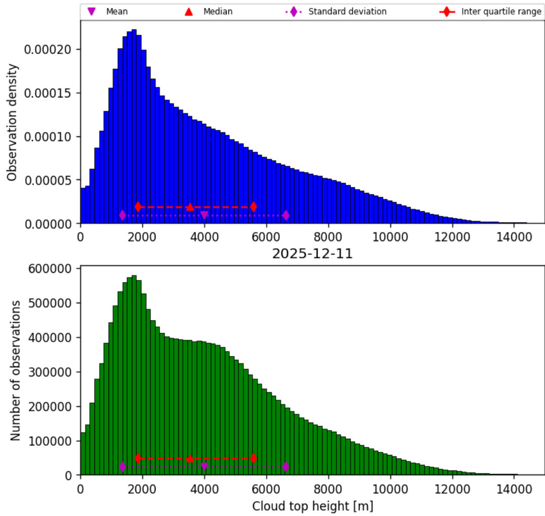
Figure 38: Histogram of “Cloud top height” for 2025-12-11 to 2025-12-12
