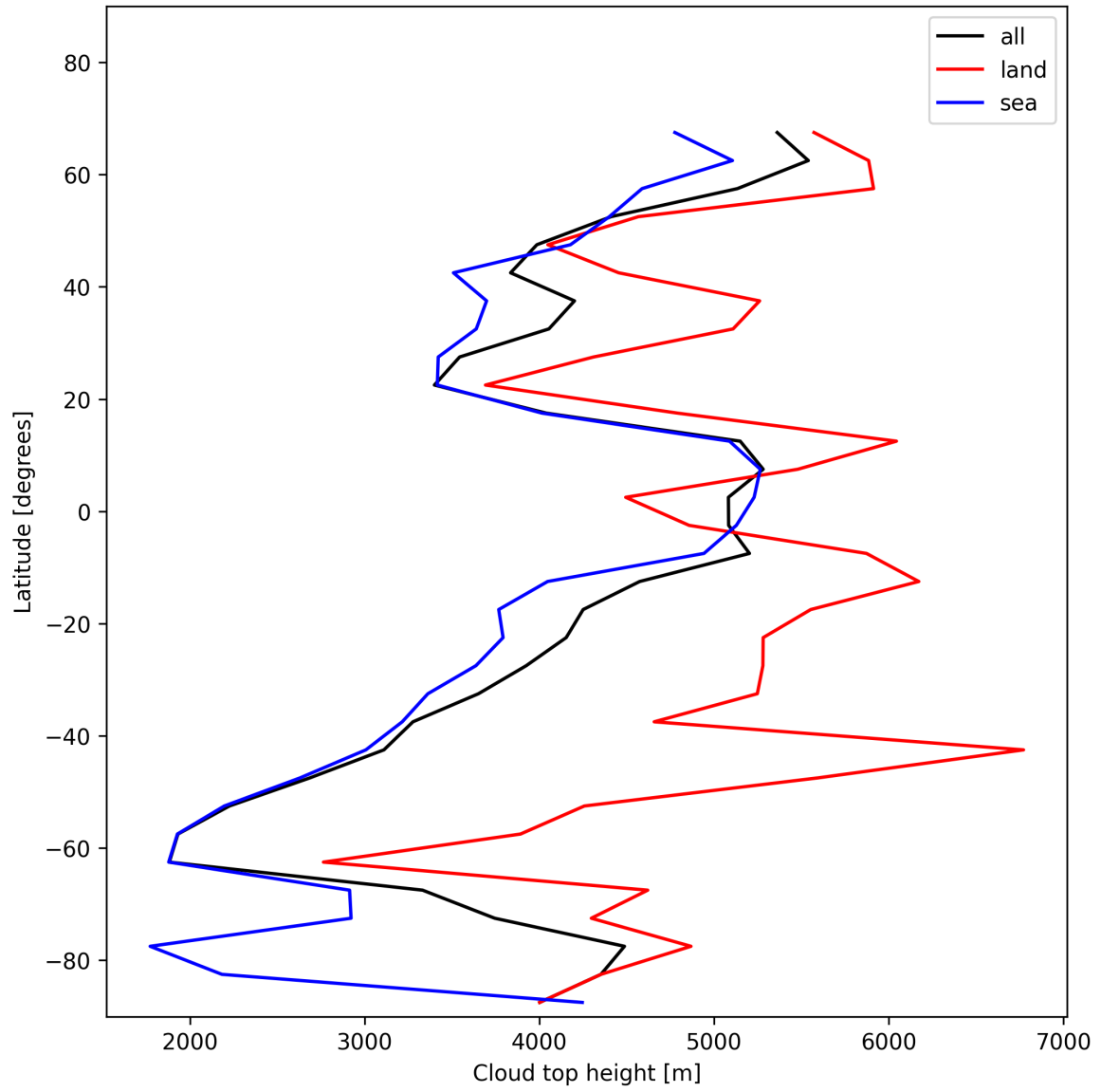
Figure 22: Zonal average of “Cloud top height” for 2025-12-11 to 2025-12-12.
