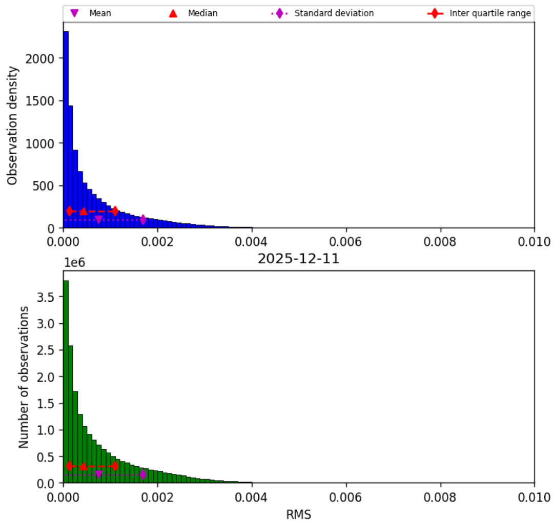
Figure 45: Histogram of “RMS” for 2025-12-11 to 2025-12-12
