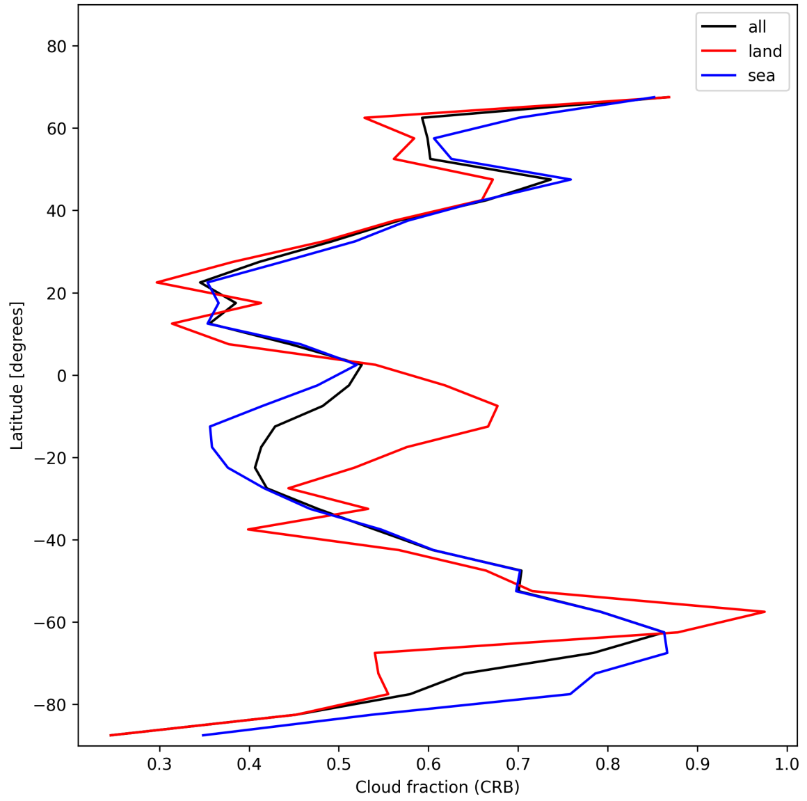
Figure 24: Zonal average of “Cloud fraction (CRB)” for 2025-12-11 to 2025-12-12.
