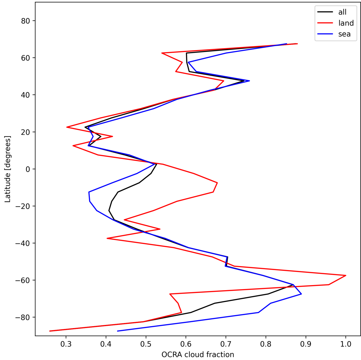
Figure 32: Zonal average of “OCRA cloud fraction” for 2025-12-11 to 2025-12-12.
