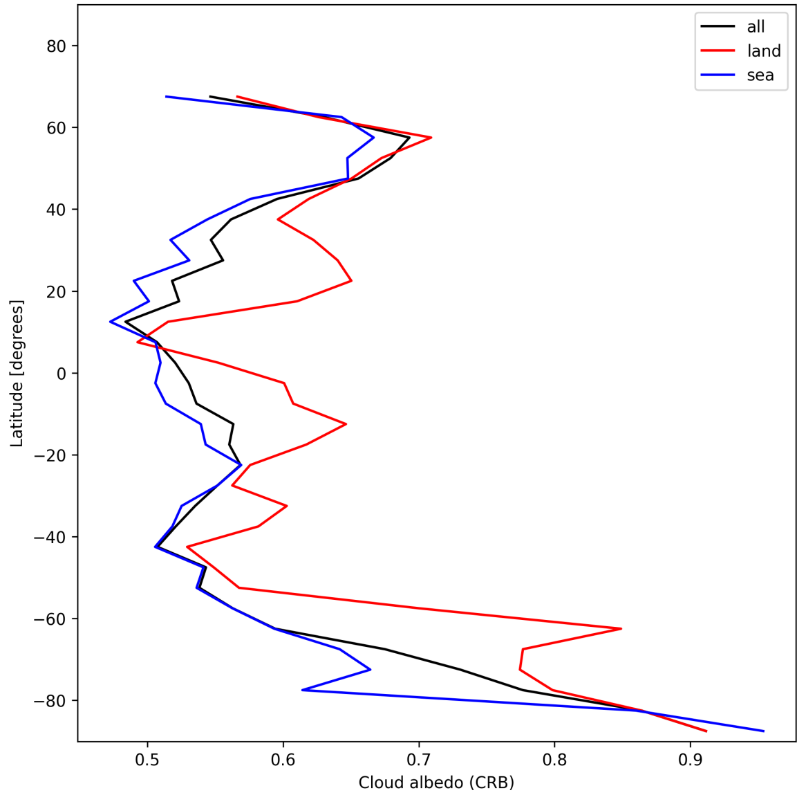
Figure 26: Zonal average of “Cloud albedo (CRB)” for 2025-12-11 to 2025-12-12.
