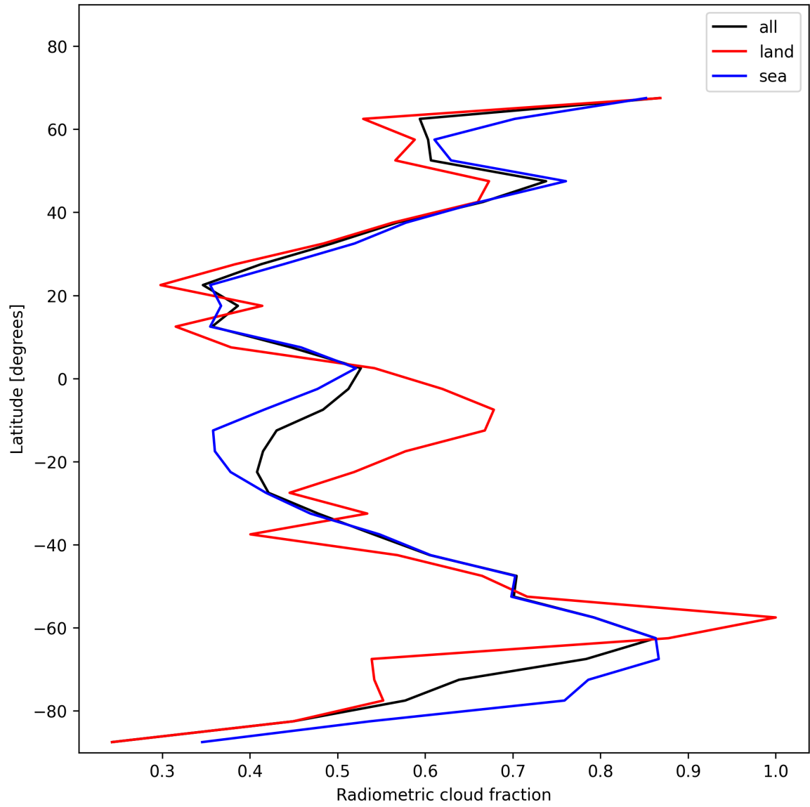
Figure 21: Zonal average of “Radiometric cloud fraction” for 2025-12-11 to 2025-12-12.
