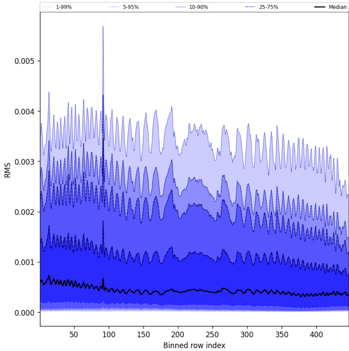
Figure 61: Along track statistics of “RMS” for 2025-12-11 to 2025-12-12
