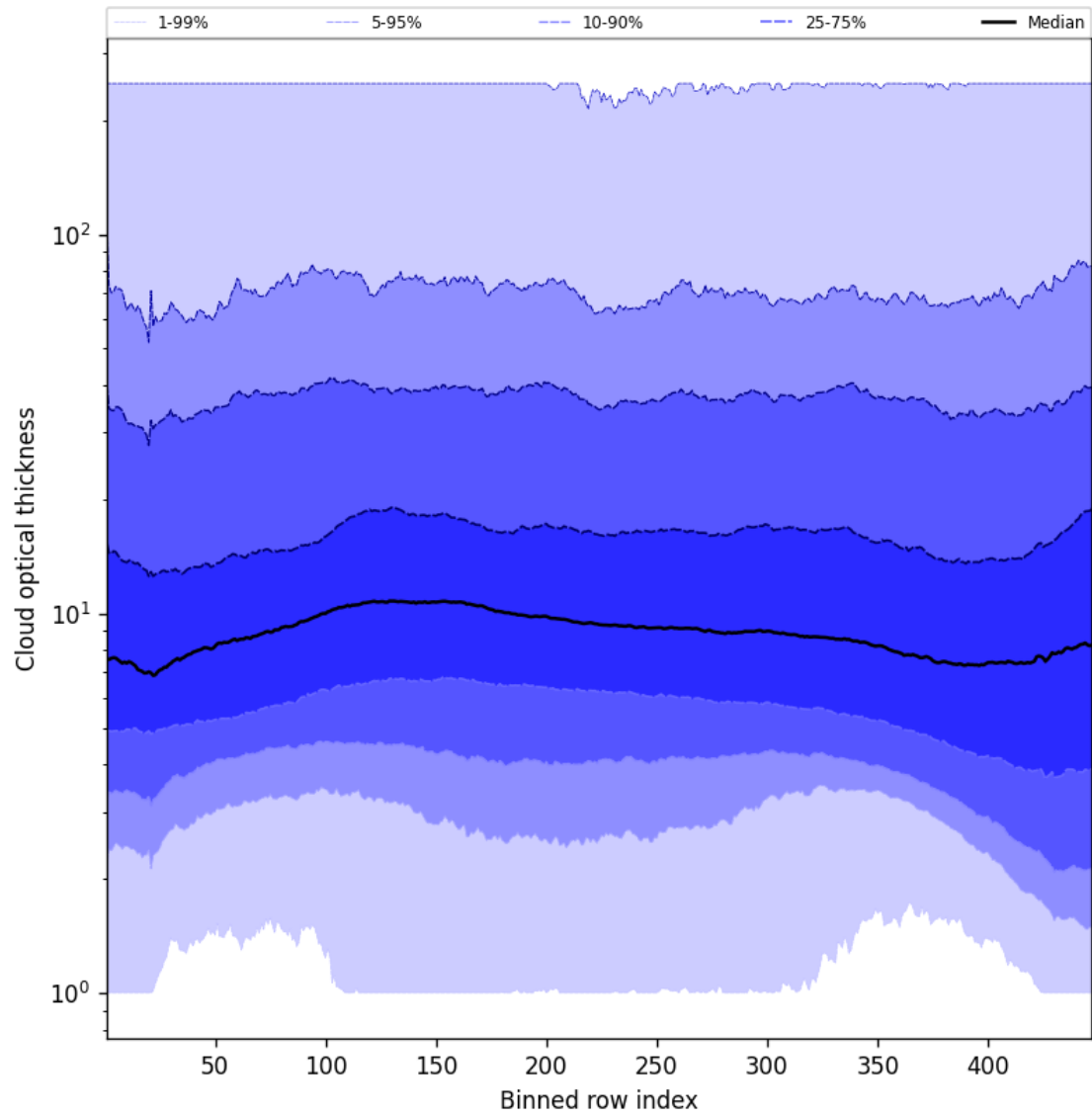
Figure 55: Along track statistics of “Cloud optical thickness” for 2025-12-11 to 2025-12-12
