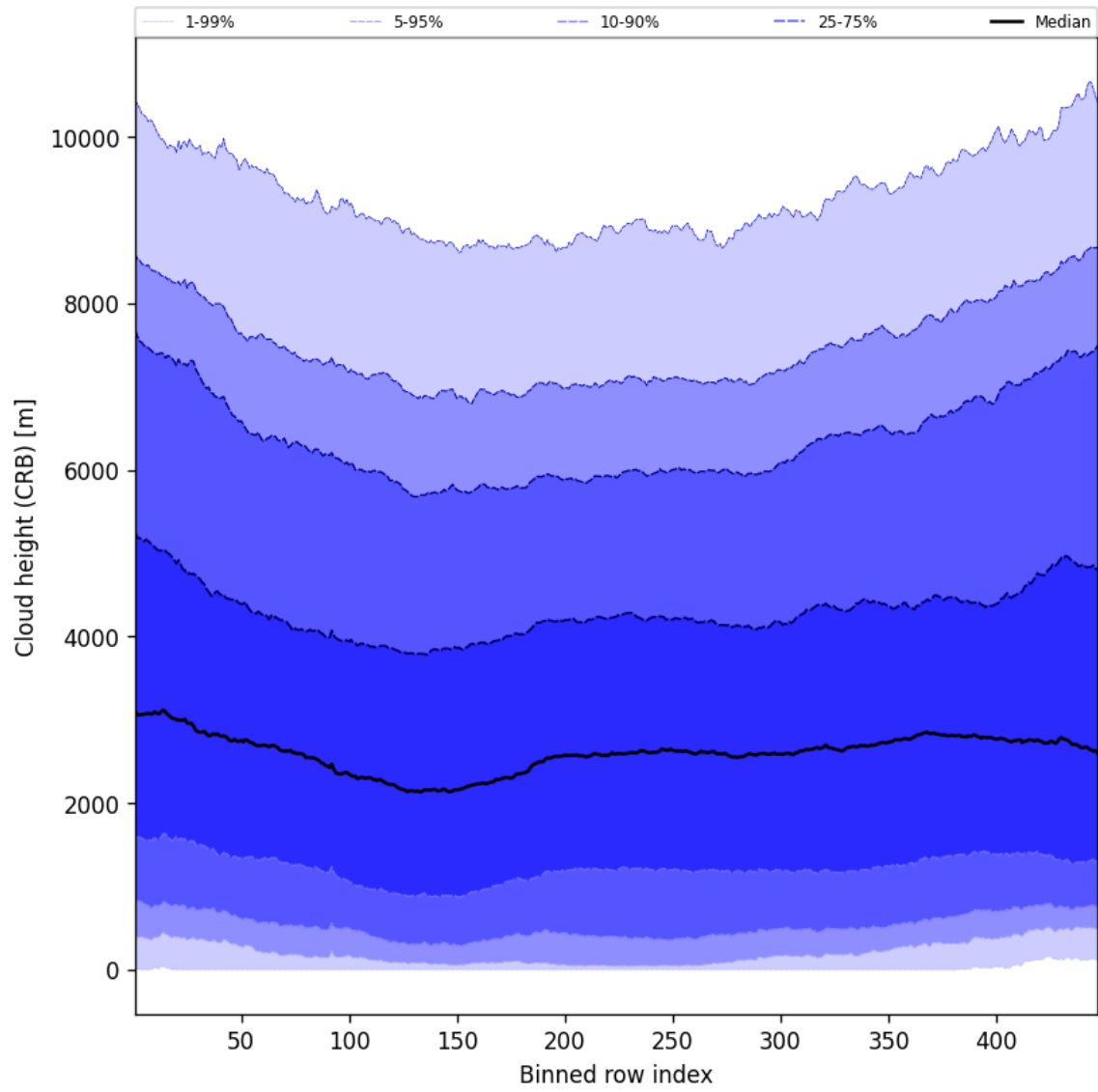
Figure 57: Along track statistics of “Cloud height (CRB)” for 2025-12-11 to 2025-12-12
