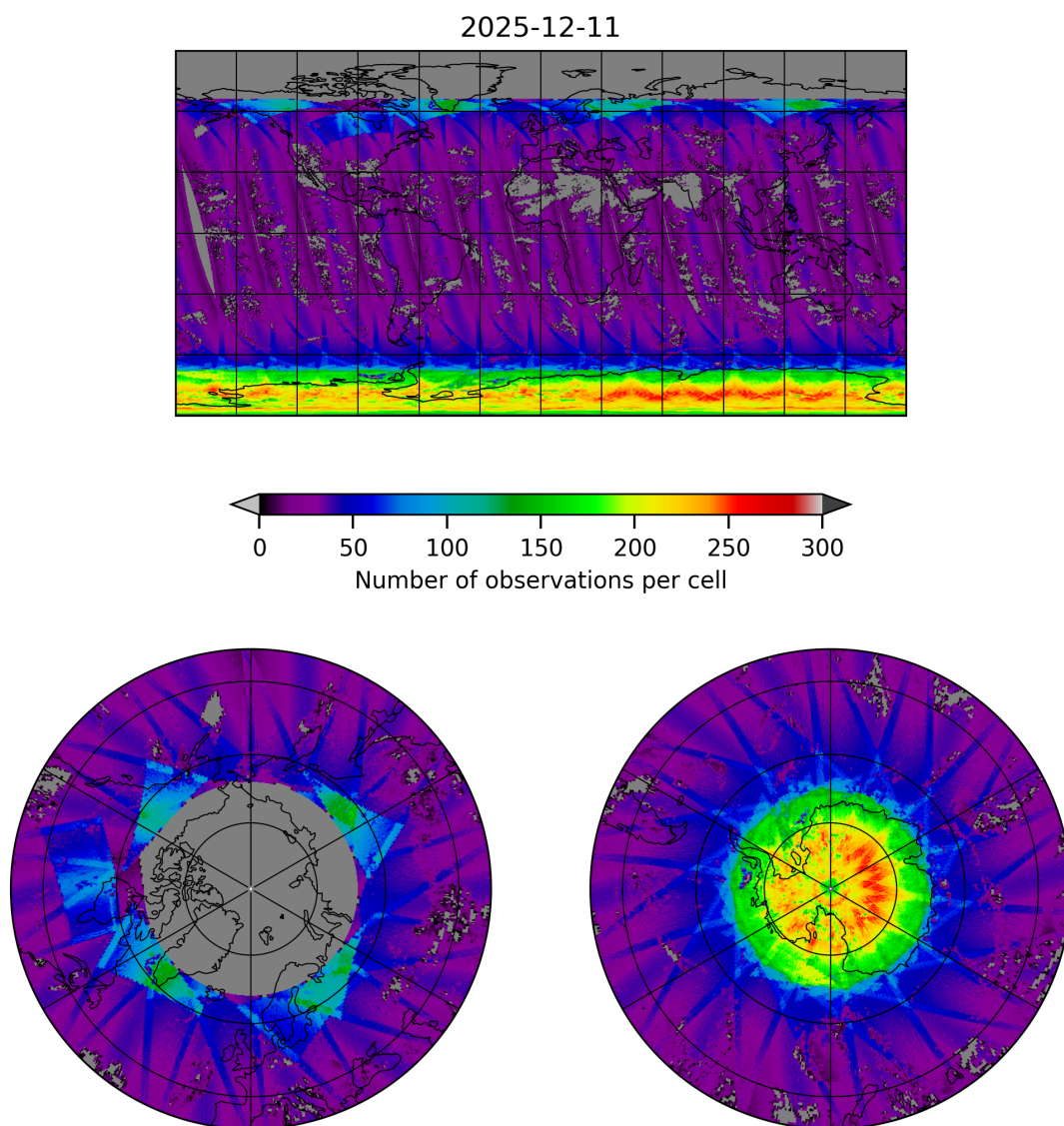
Figure 19: Map of the number of observations for 2025-12-11 to 2025-12-12
