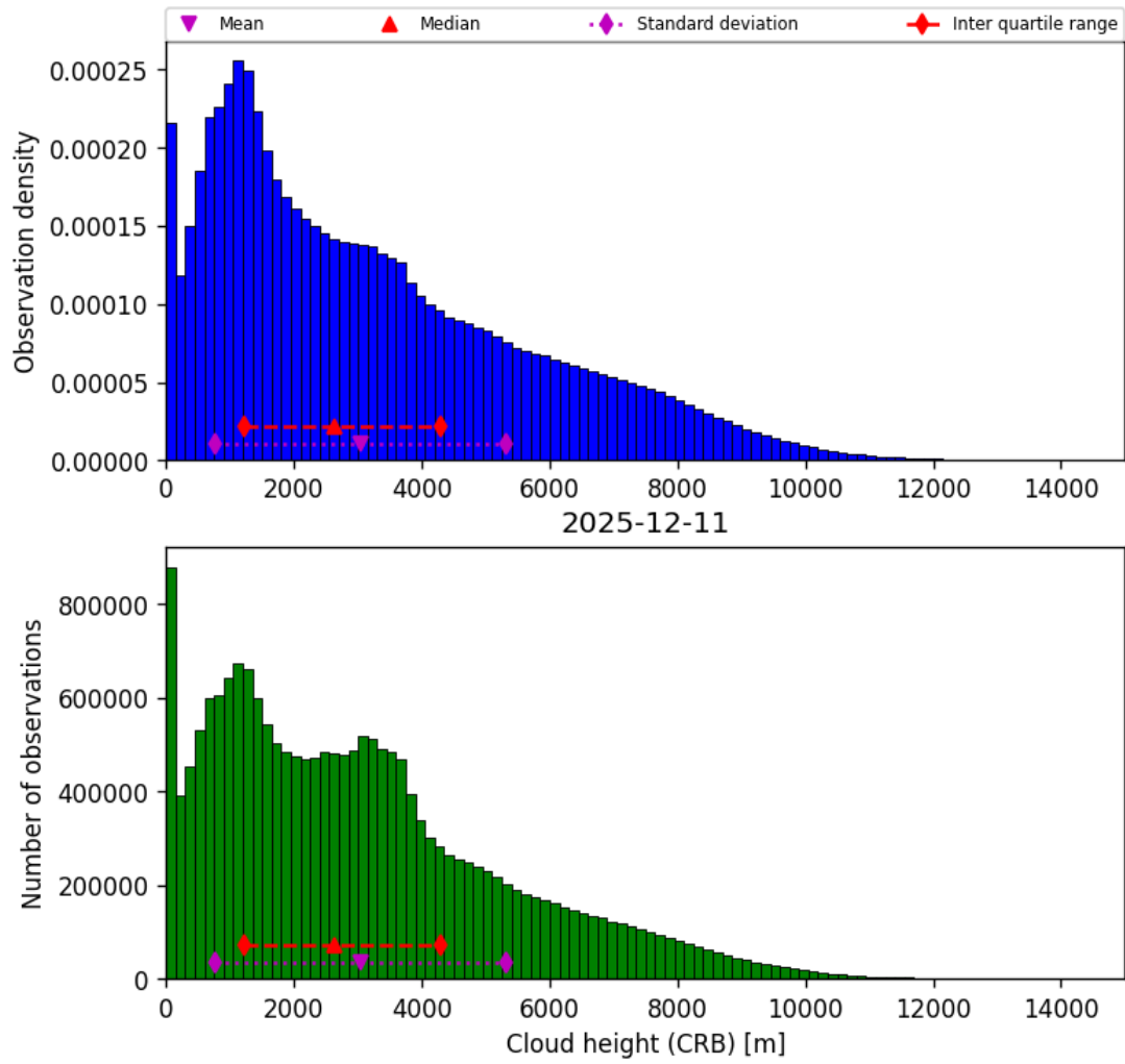
Figure 41: Histogram of “Cloud height (CRB)” for 2025-12-11 to 2025-12-12
