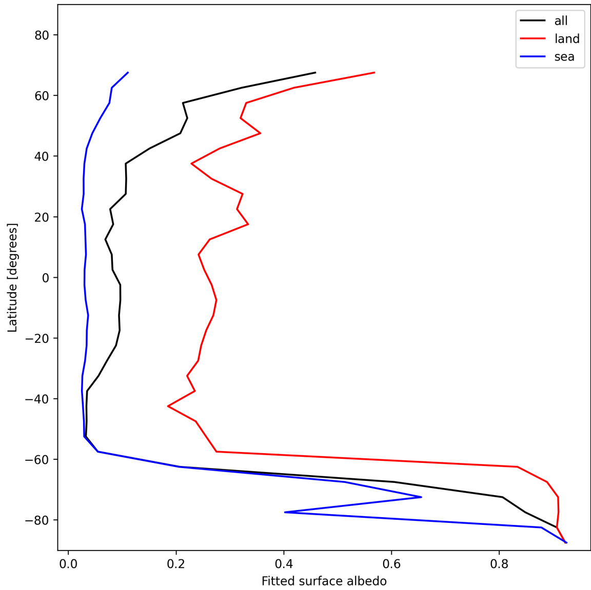
Figure 27: Zonal average of “Fitted surface albedo” for 2025-12-11 to 2025-12-12.
