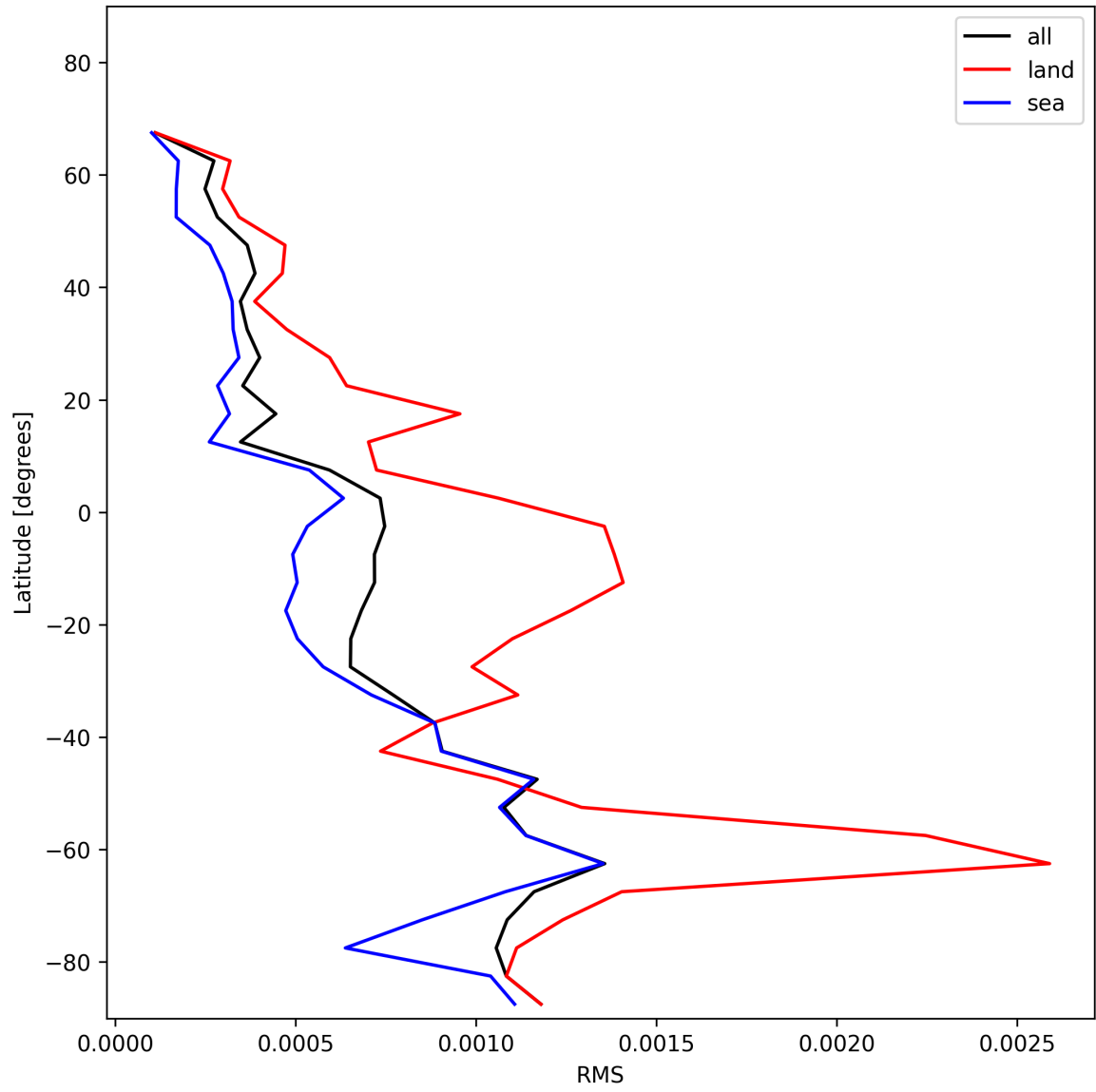
Figure 29: Zonal average of “RMS” for 2025-12-11 to 2025-12-12.
