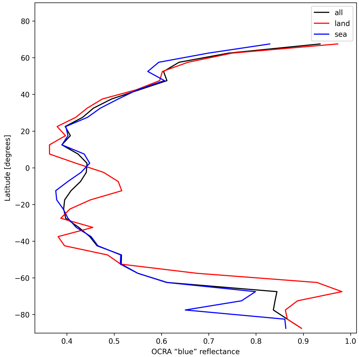
Figure 33: Zonal average of “OCRA “blue” reflectance” for 2025-12-11 to 2025-12-12.
