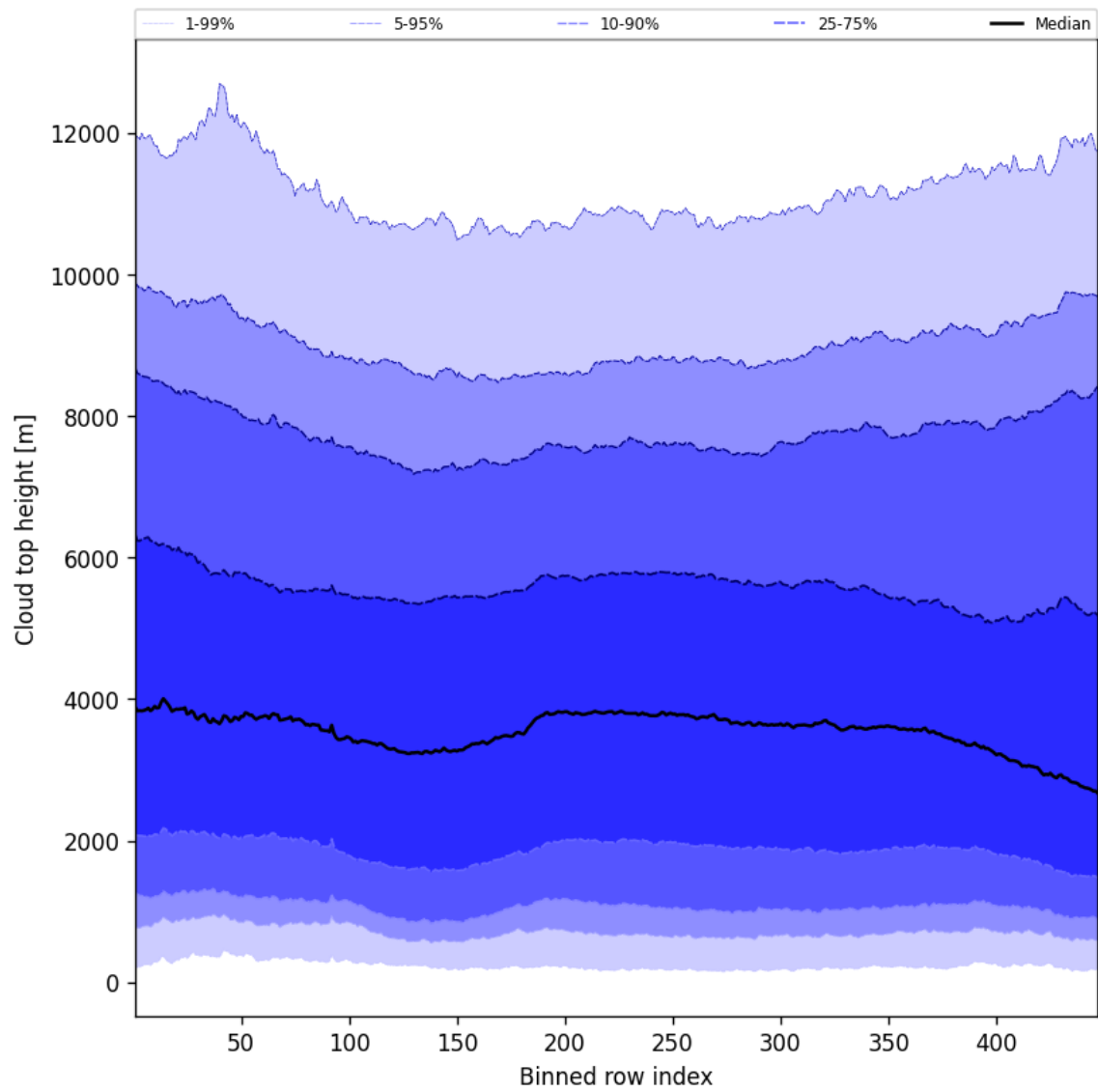
Figure 54: Along track statistics of “Cloud top height” for 2025-12-11 to 2025-12-12
