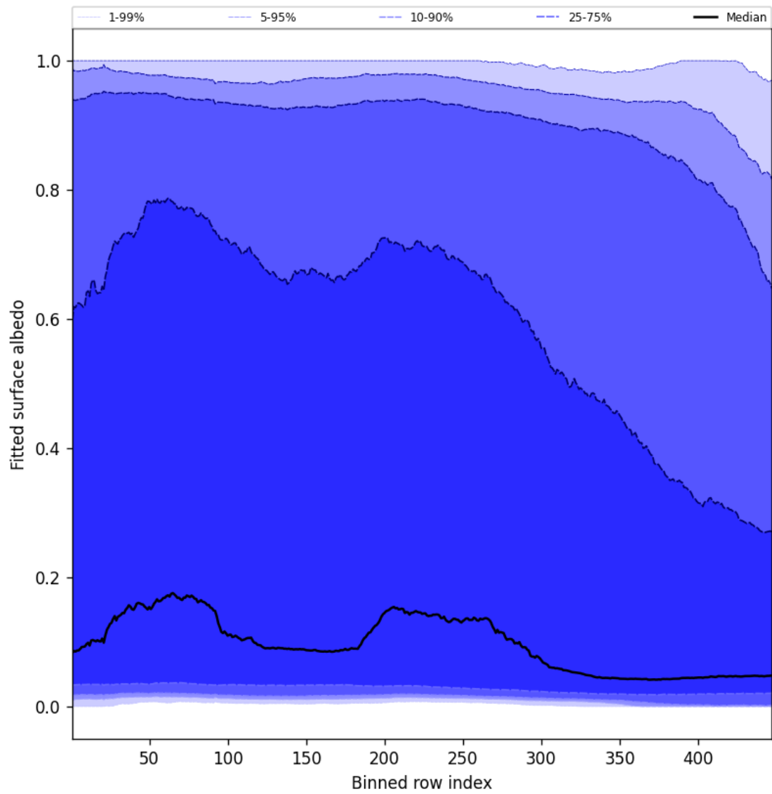
Figure 59: Along track statistics of “Fitted surface albedo” for 2025-12-11 to 2025-12-12
