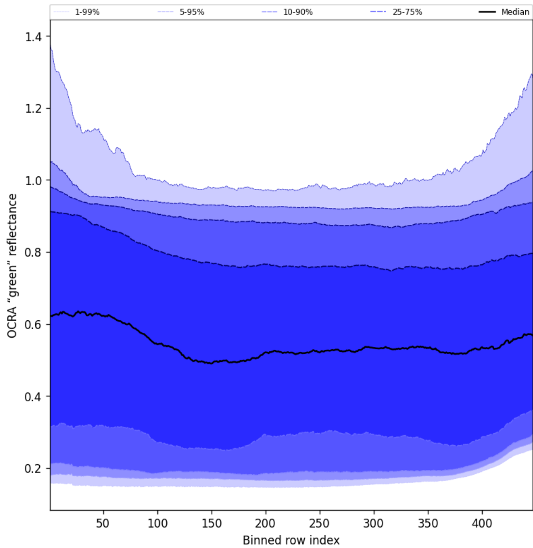
Figure 66: Along track statistics of “OCRA “green” reflectance” for 2025-12-11 to 2025-12-12
