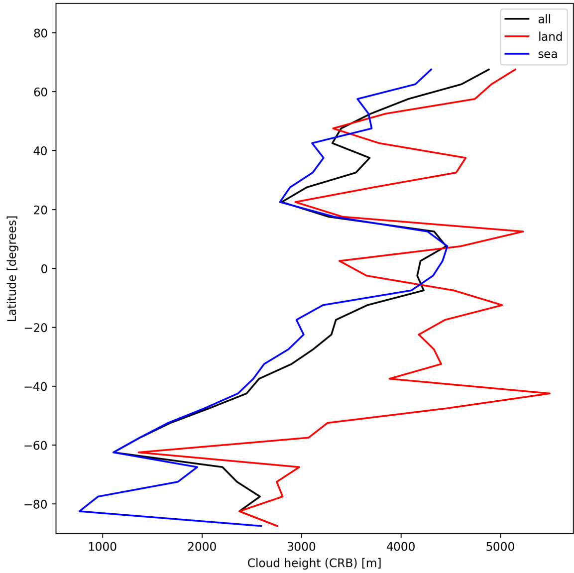
Figure 25: Zonal average of “Cloud height (CRB)” for 2025-12-11 to 2025-12-12.
