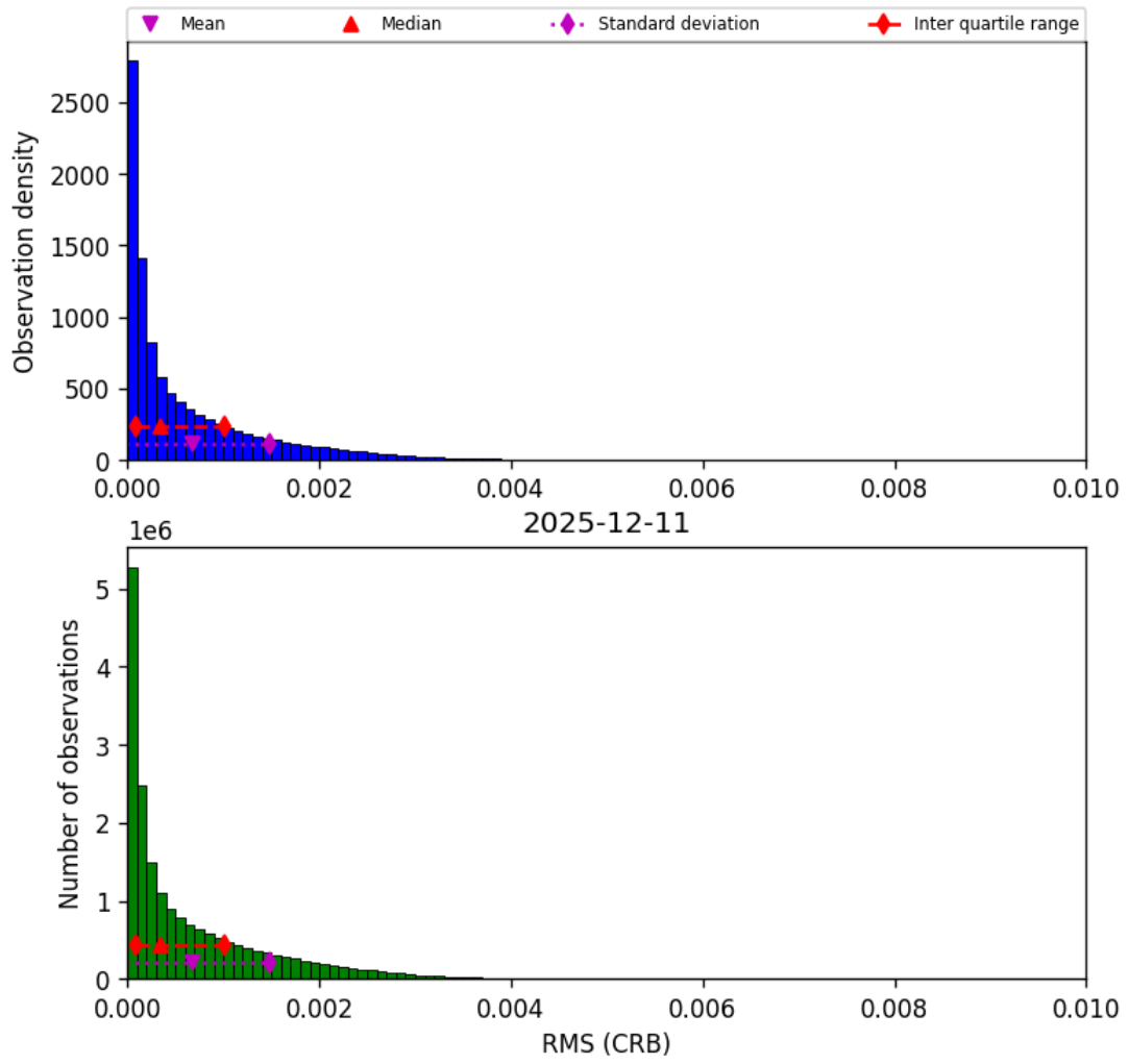
Figure 46: Histogram of “RMS (CRB)” for 2025-12-11 to 2025-12-12
