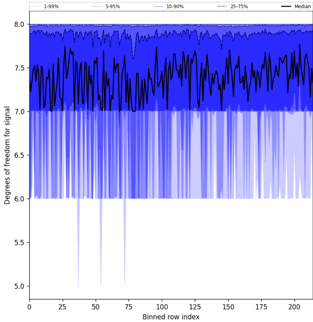
Figure 25: Along track statistics of “Degrees of freedom for signal” for 2024-12-01 to 2024-12-02
