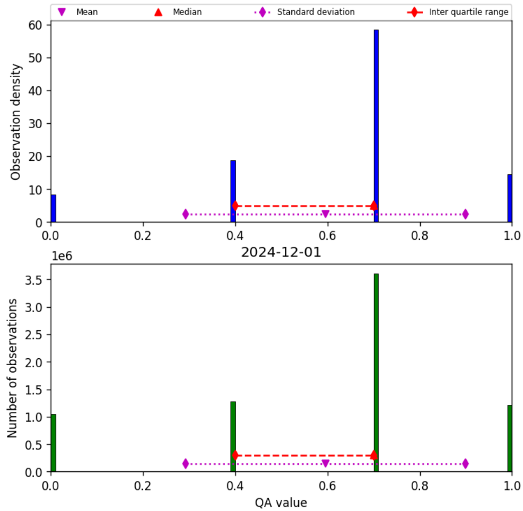
Figure 13: Histogram of “QA value” for 2024-12-01 to 2024-12-02
