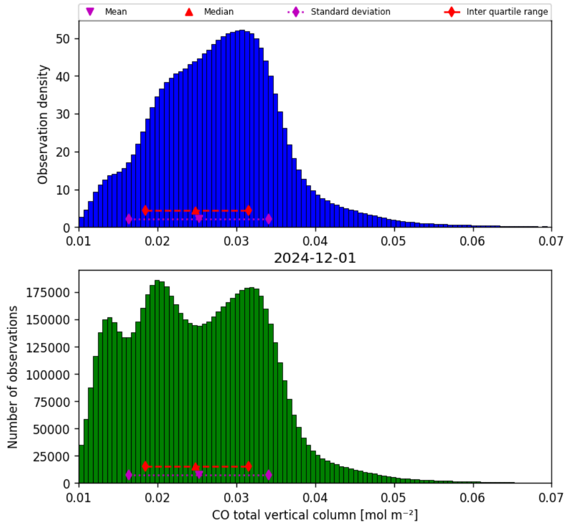
Figure 14: Histogram of “CO total vertical column” for 2024-12-01 to 2024-12-02
