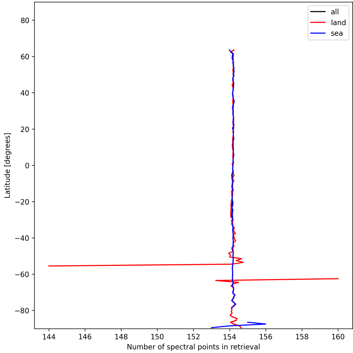
Figure 9: Zonal average of “Number of spectral points in retrieval” for 2024-12-01 to 2024-12-02.
