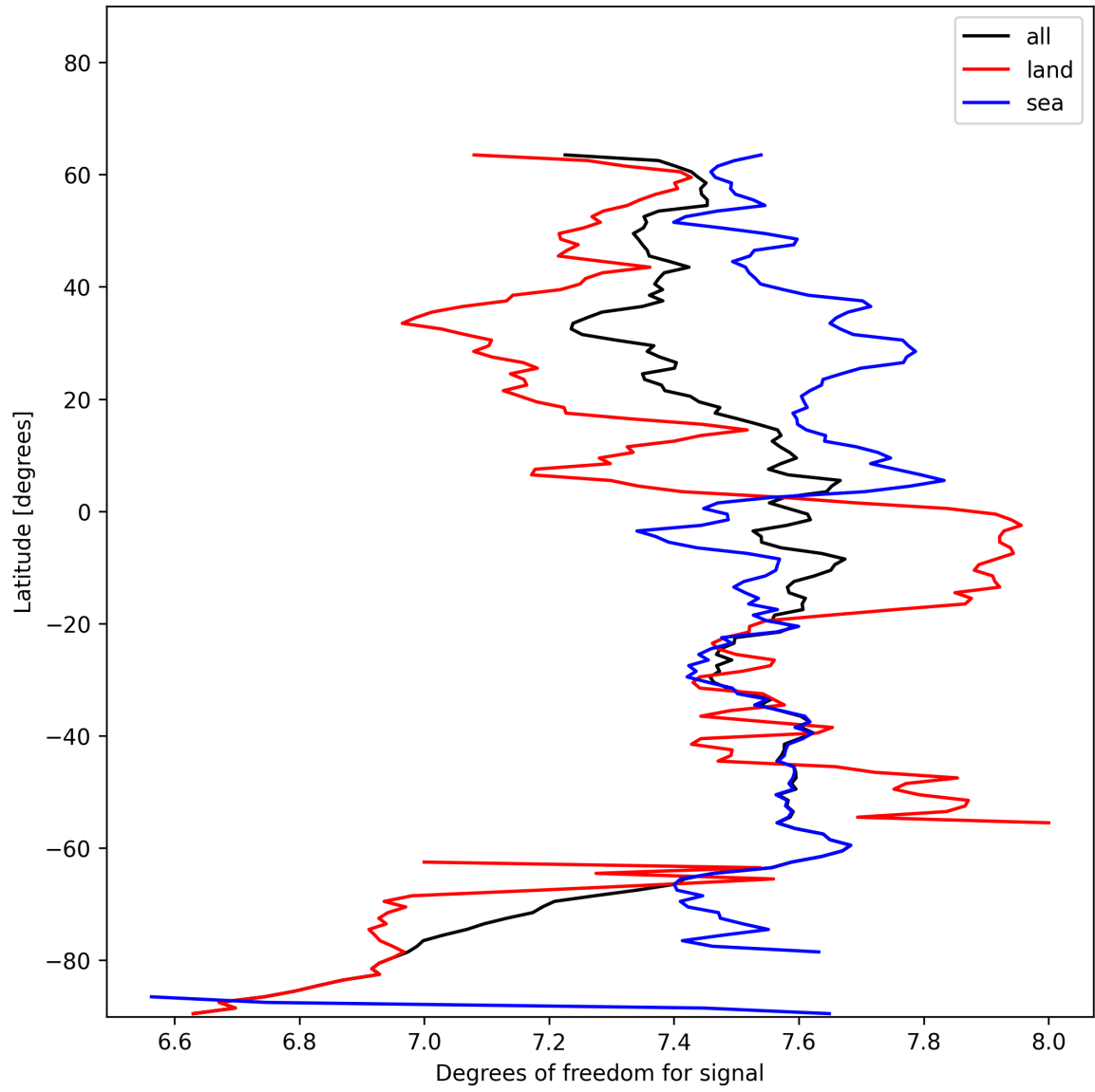
Figure 11: Zonal average of “Degrees of freedom for signal” for 2024-12-01 to 2024-12-02.
