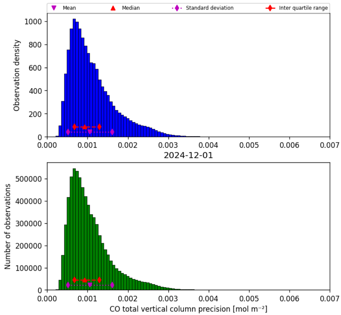
Figure 15: Histogram of “CO total vertical column precision” for 2024-12-01 to 2024-12-02
