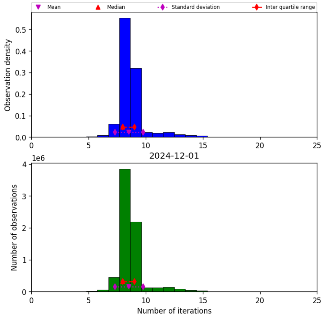
Figure 19: Histogram of “Number of iterations” for 2024-12-01 to 2024-12-02
