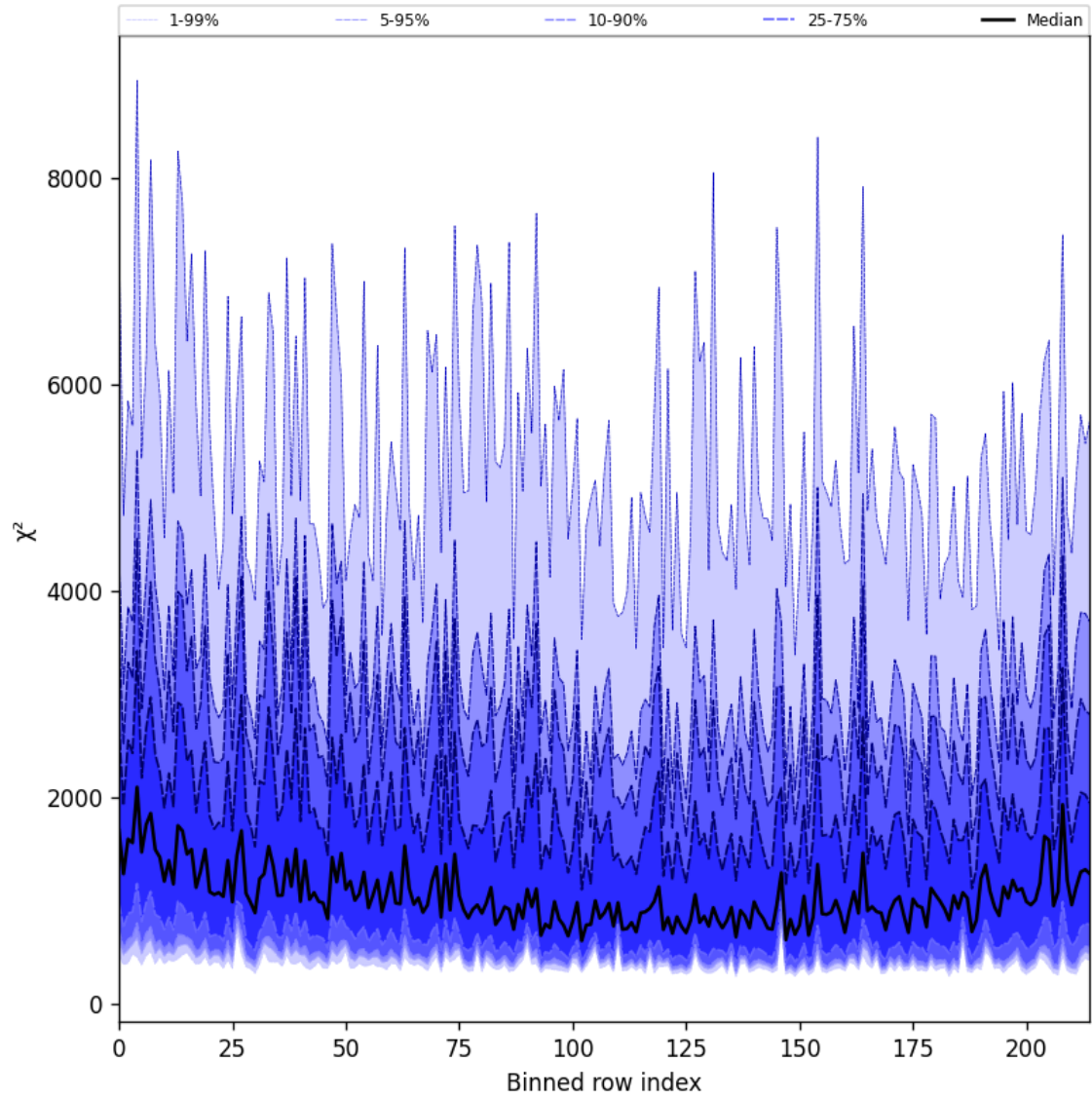
Figure 24: Along track statistics of “ \chi^2 ” for 2024-12-01 to 2024-12-02
