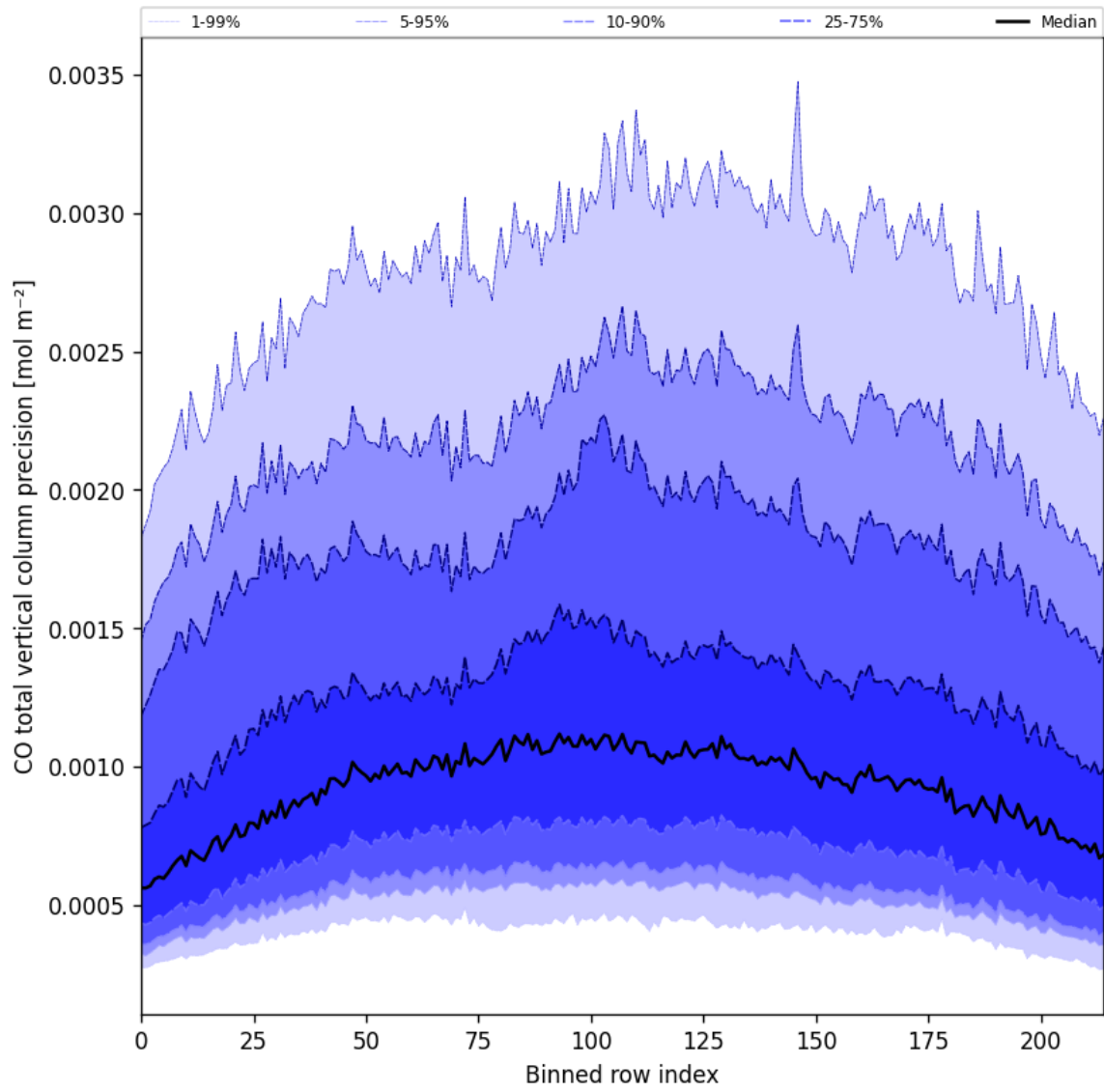
Figure 22: Along track statistics of “CO total vertical column precision” for 2024-12-01 to 2024-12-02
