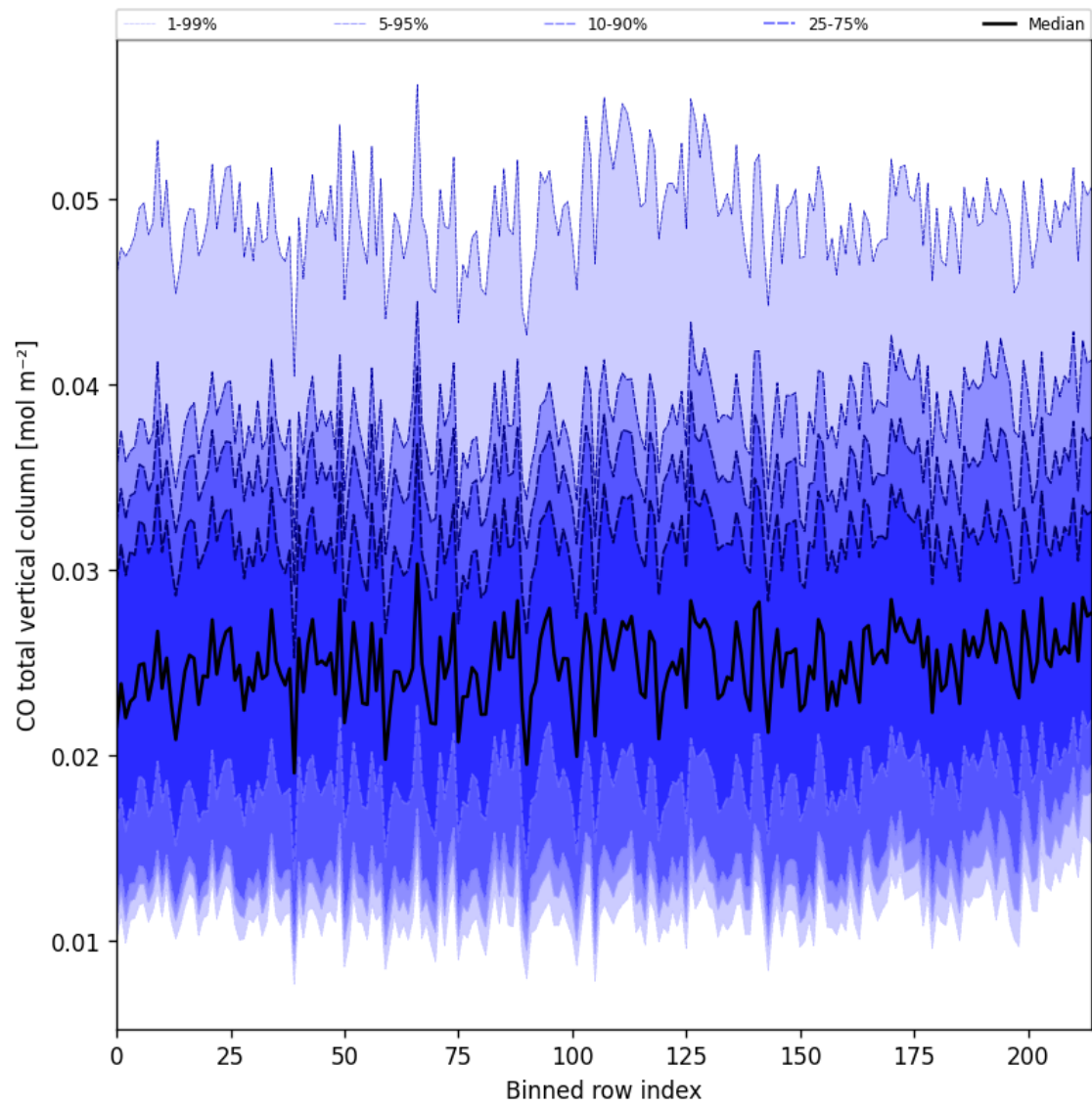
Figure 21: Along track statistics of “CO total vertical column” for 2024-12-01 to 2024-12-02
