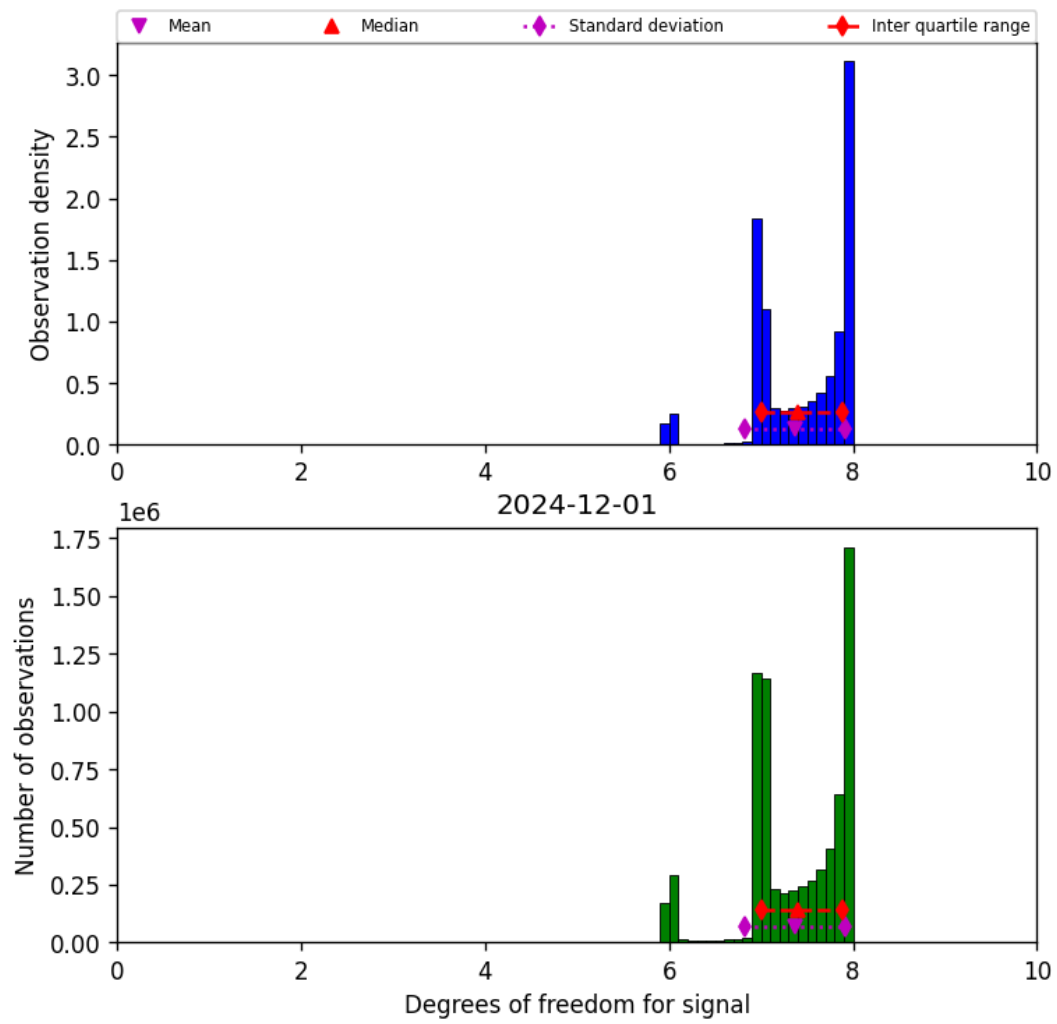
Figure 18: Histogram of “Degrees of freedom for signal” for 2024-12-01 to 2024-12-02
