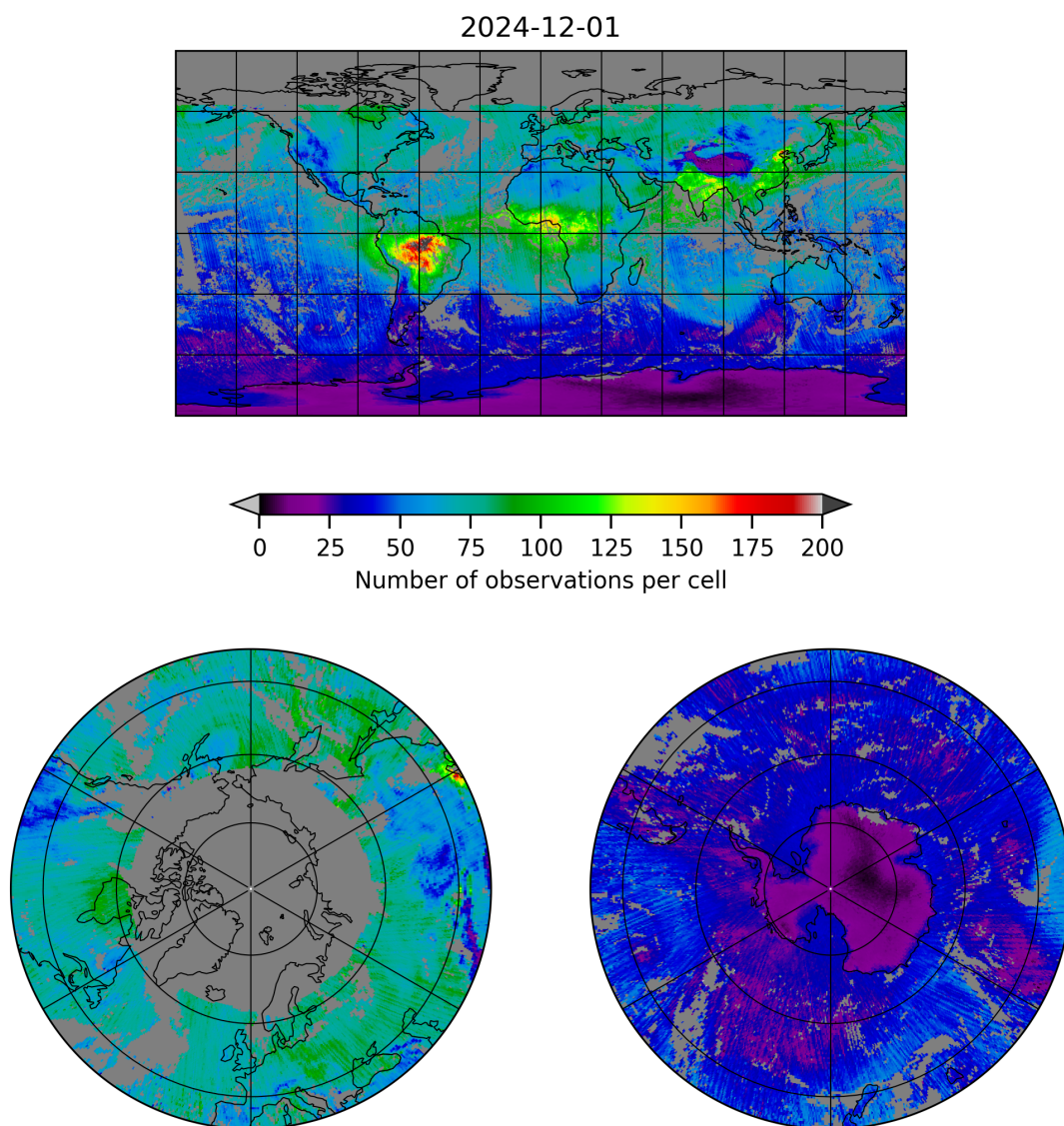
Figure 5: Map of the number of observations for 2024-12-01 to 2024-12-02
