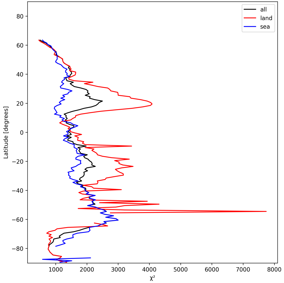
Figure 10: Zonal average of “ \chi^2 ” for 2024-12-01 to 2024-12-02.
