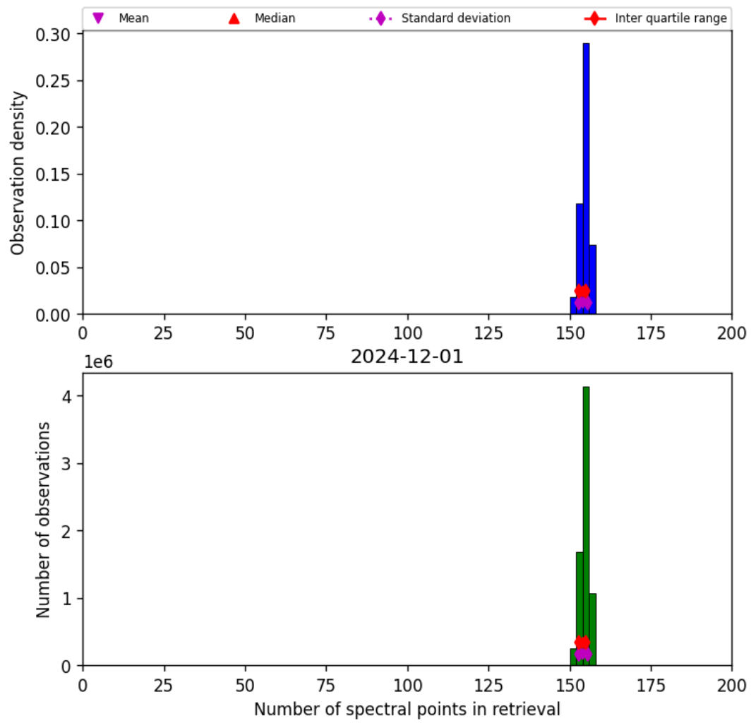
Figure 16: Histogram of “Number of spectral points in retrieval” for 2024-12-01 to 2024-12-02
