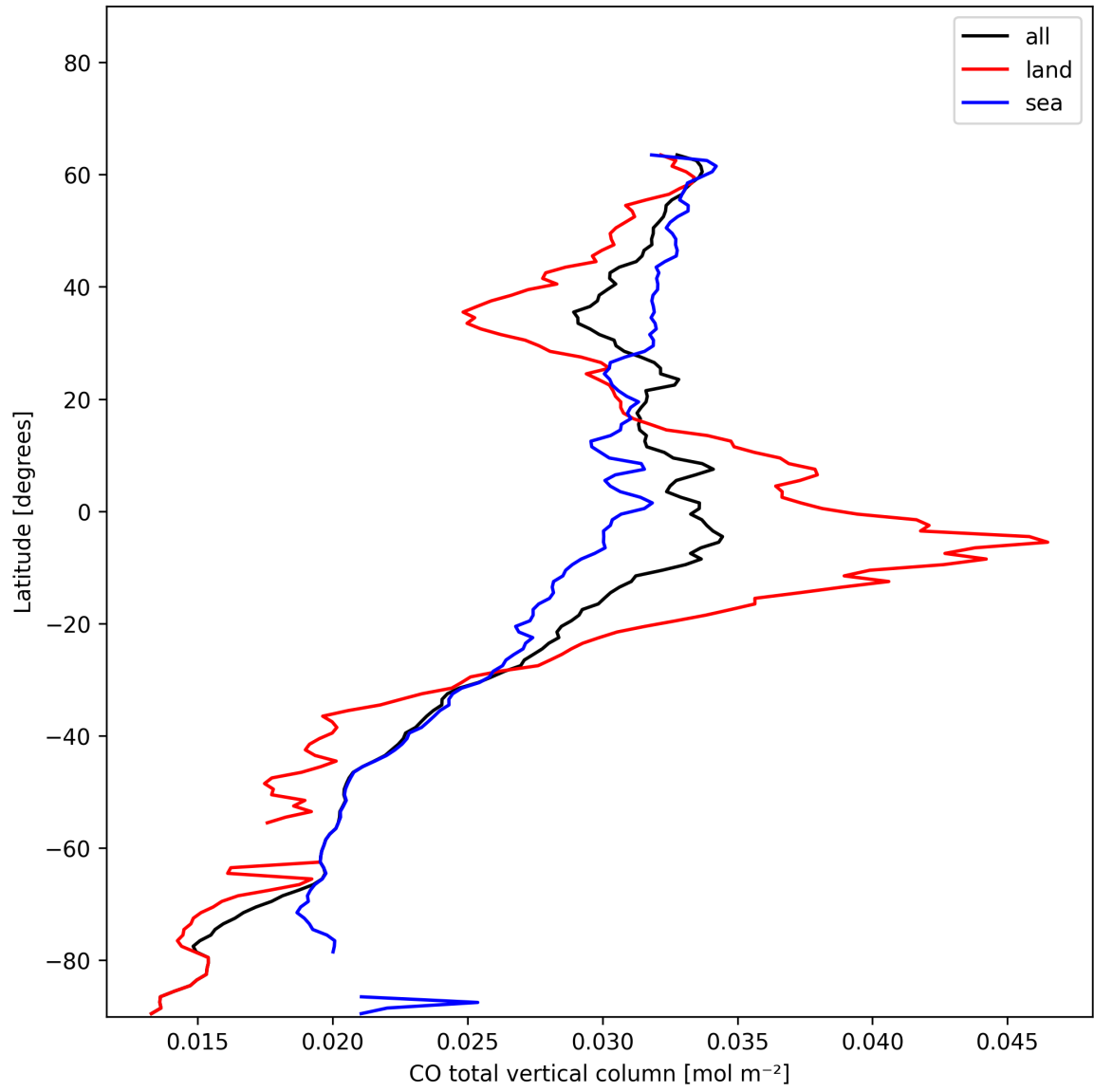
Figure 7: Zonal average of “CO total vertical column” for 2024-12-01 to 2024-12-02.
