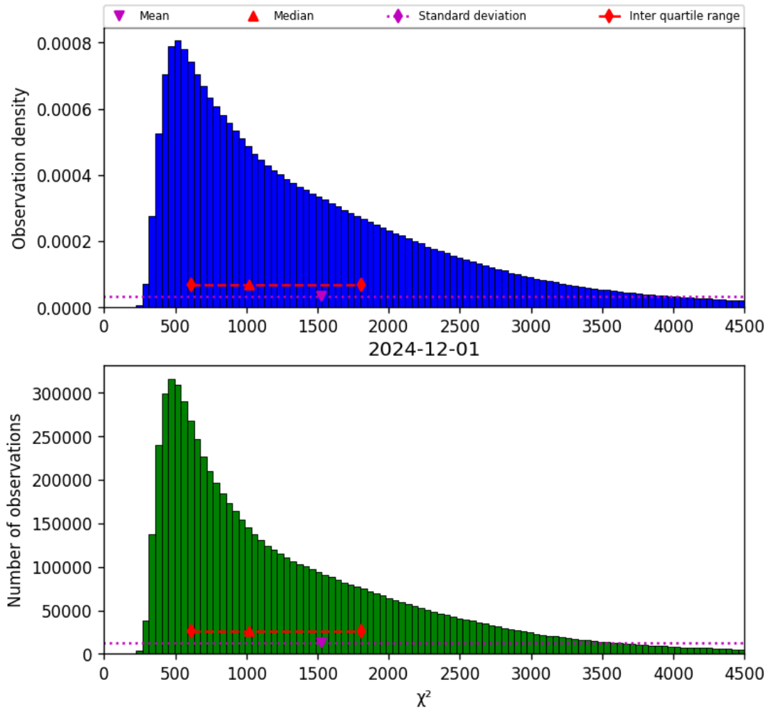
Figure 17: Histogram of “ \chi^2 ” for 2024-12-01 to 2024-12-02
