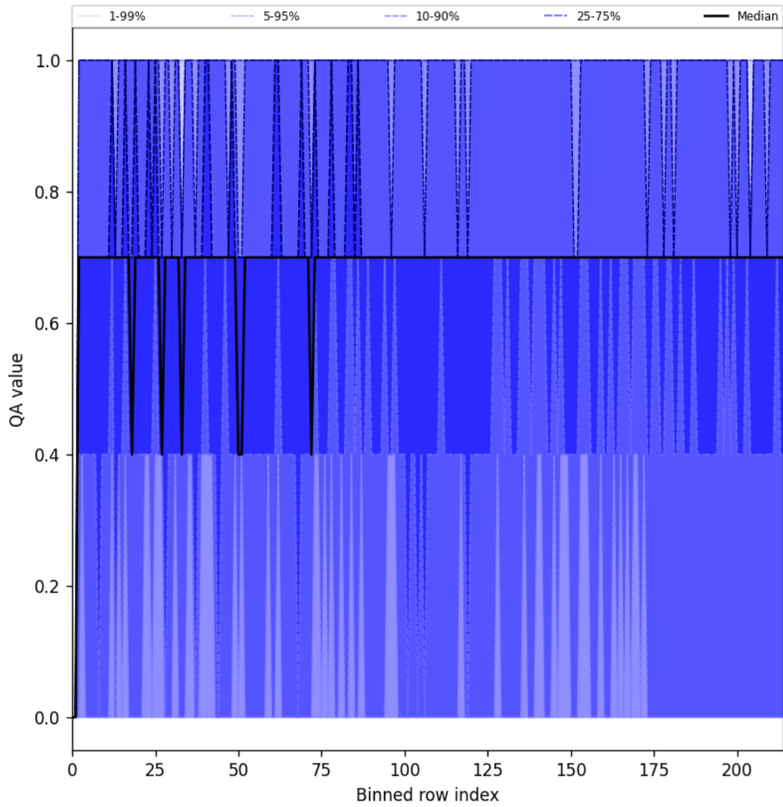
Figure 20: Along track statistics of “QA value” for 2024-12-01 to 2024-12-02
