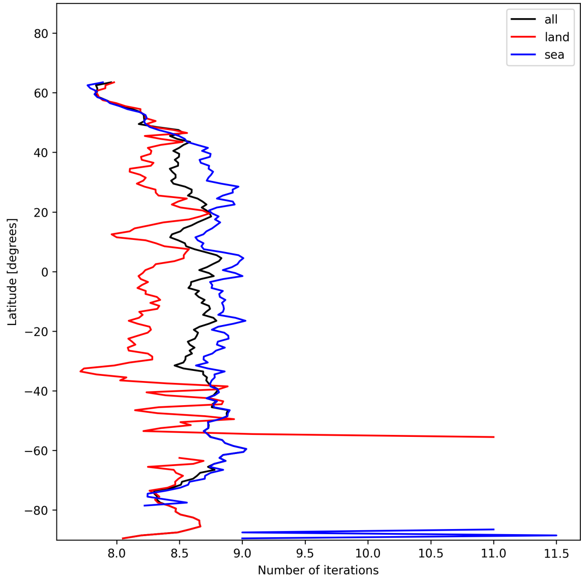
Figure 12: Zonal average of “Number of iterations” for 2024-12-01 to 2024-12-02.
