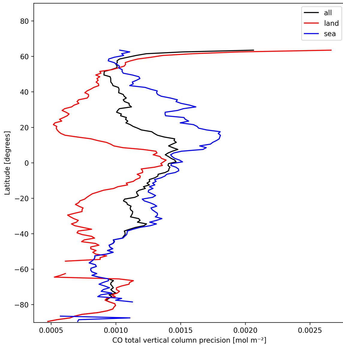
Figure 8: Zonal average of “CO total vertical column precision” for 2024-12-01 to 2024-12-02.
