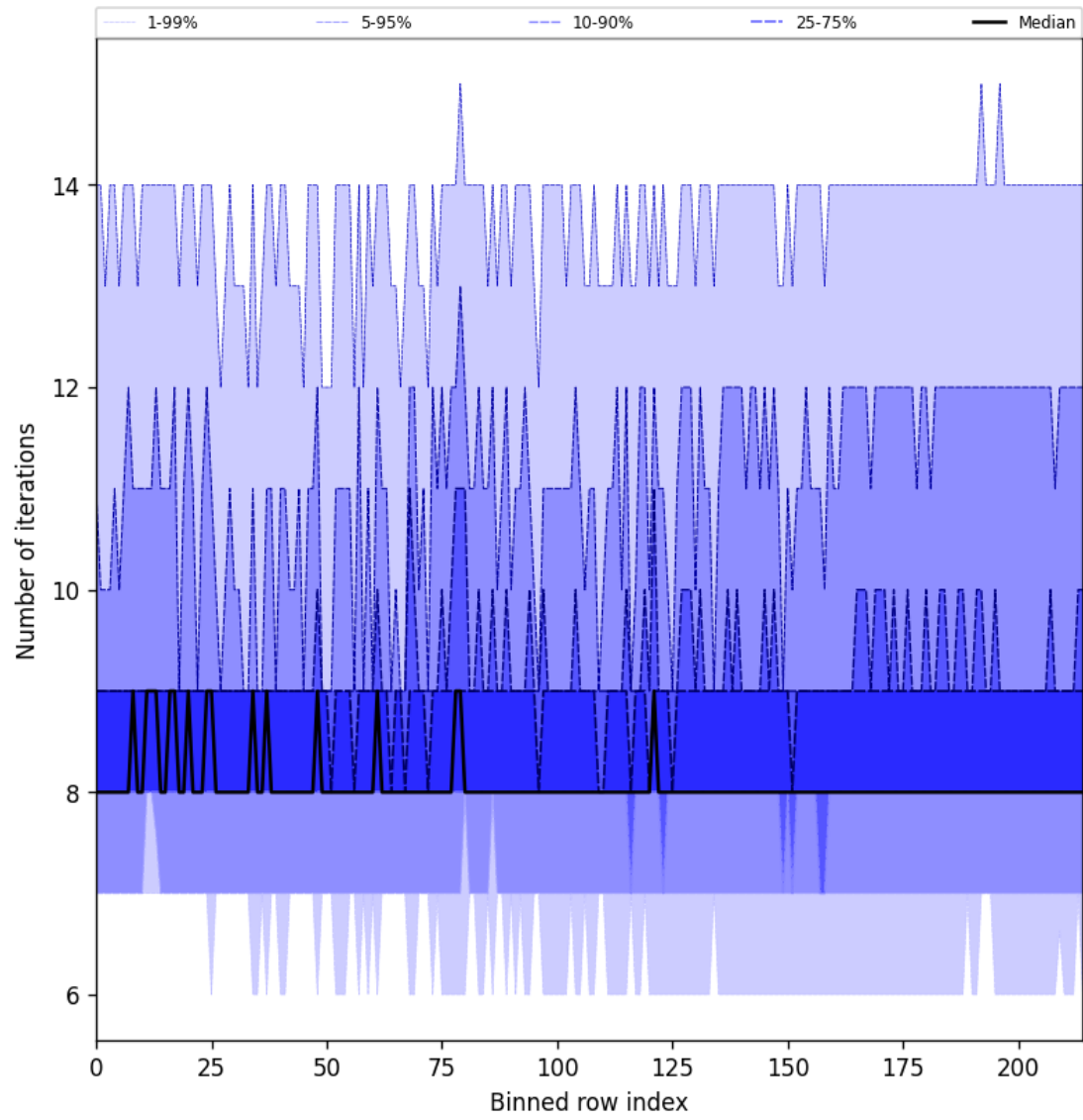
Figure 26: Along track statistics of “Number of iterations” for 2024-12-01 to 2024-12-02
