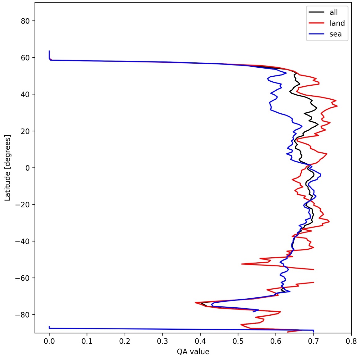
Figure 6: Zonal average of “QA value” for 2024-12-01 to 2024-12-02.
