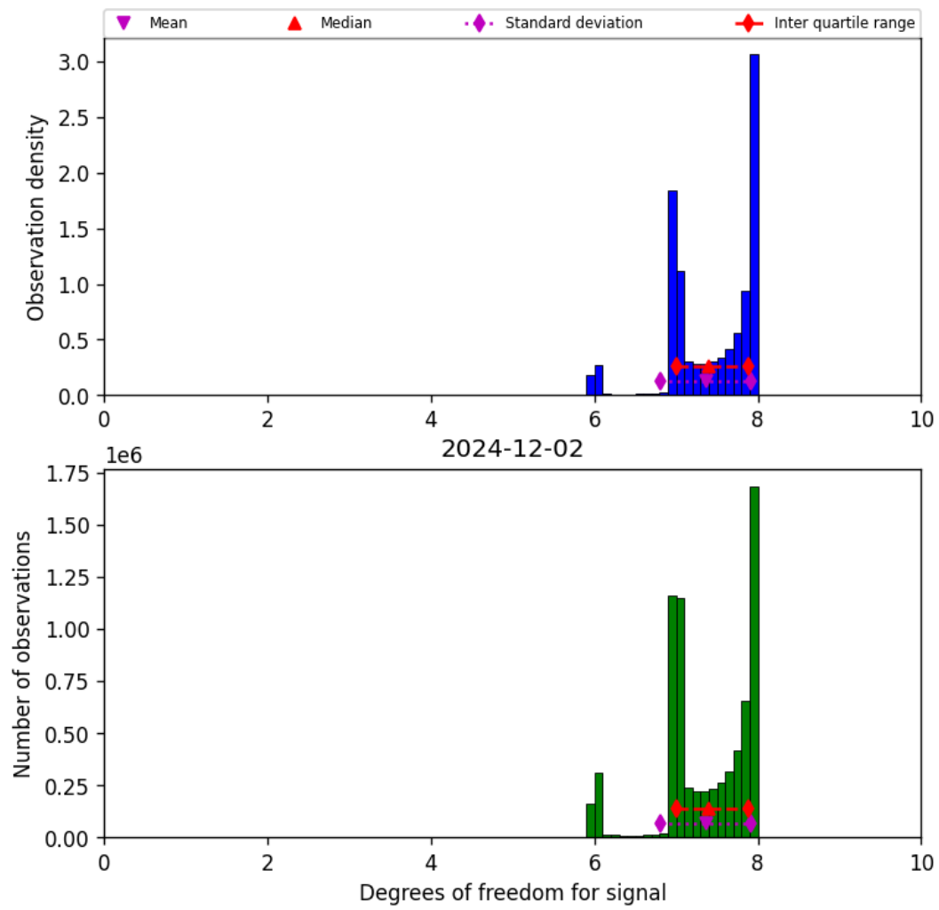
Figure 18: Histogram of “Degrees of freedom for signal” for 2024-12-02 to 2024-12-03
