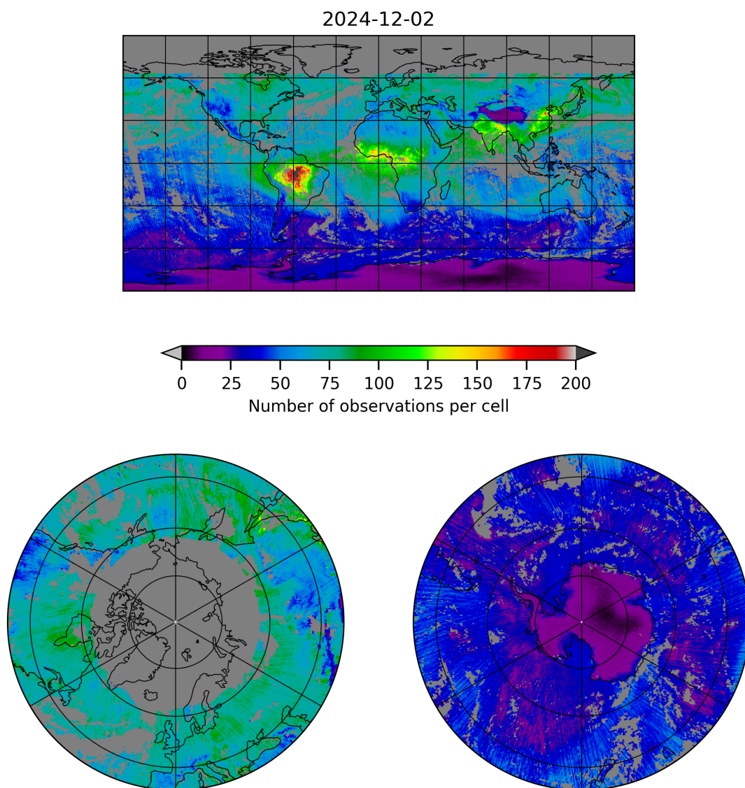
Figure 5: Map of the number of observations for 2024-12-02 to 2024-12-03
