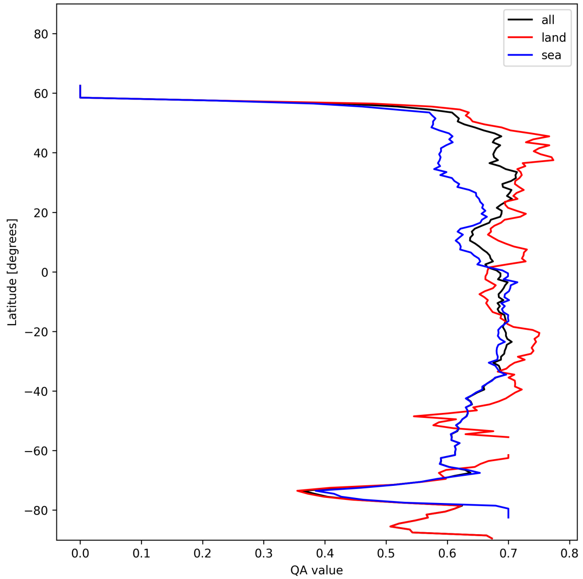
Figure 6: Zonal average of “QA value” for 2024-12-02 to 2024-12-03.
