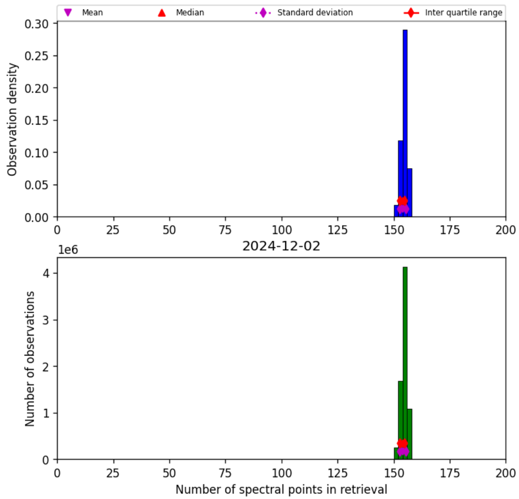
Figure 16: Histogram of “Number of spectral points in retrieval” for 2024-12-02 to 2024-12-03
