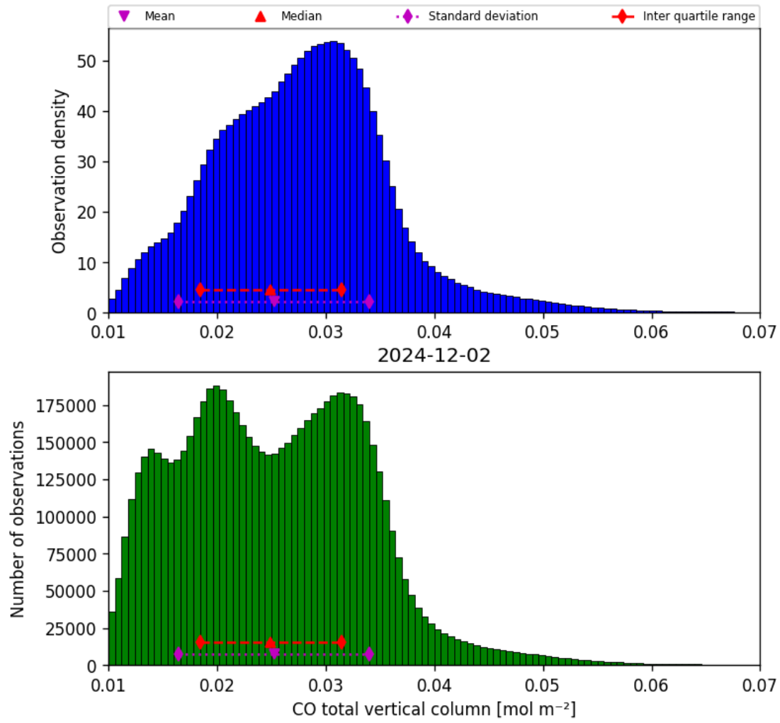
Figure 14: Histogram of “CO total vertical column” for 2024-12-02 to 2024-12-03
