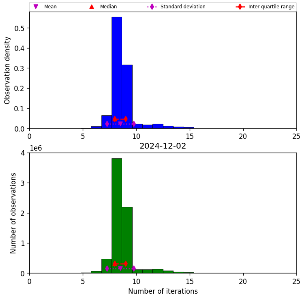
Figure 19: Histogram of “Number of iterations” for 2024-12-02 to 2024-12-03
