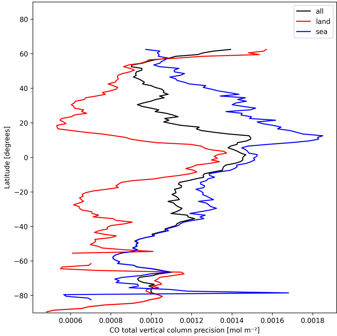
Figure 8: Zonal average of “CO total vertical column precision” for 2024-12-02 to 2024-12-03.
