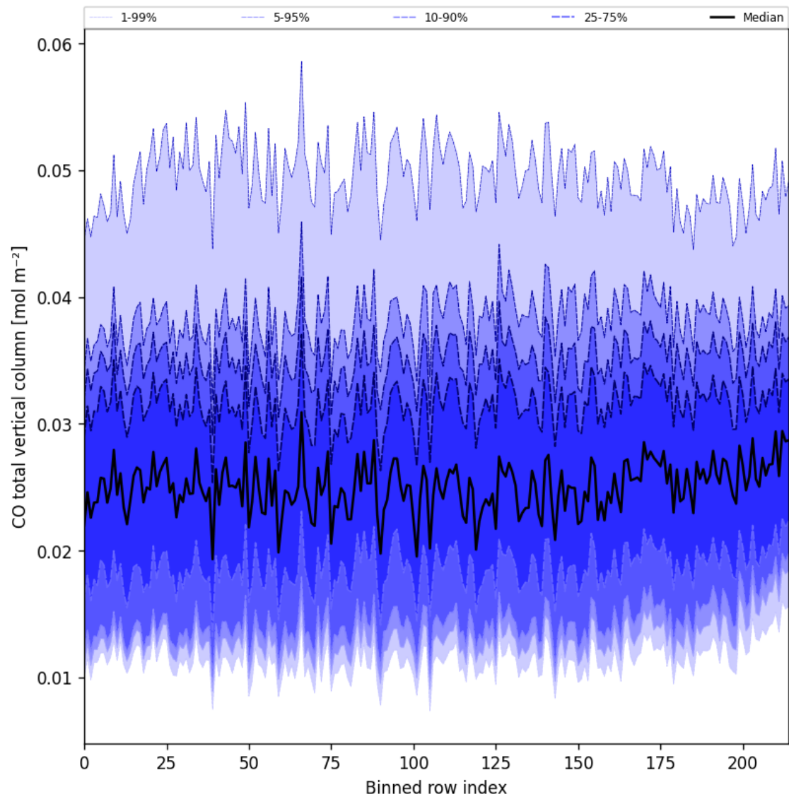
Figure 21: Along track statistics of “CO total vertical column” for 2024-12-02 to 2024-12-03
