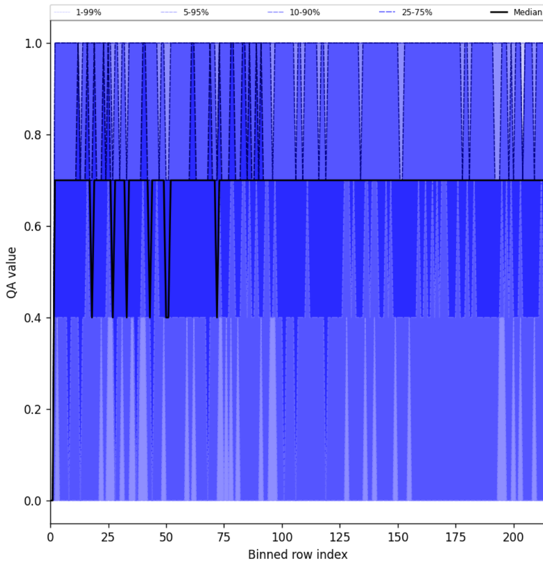
Figure 20: Along track statistics of “QA value” for 2024-12-02 to 2024-12-03
