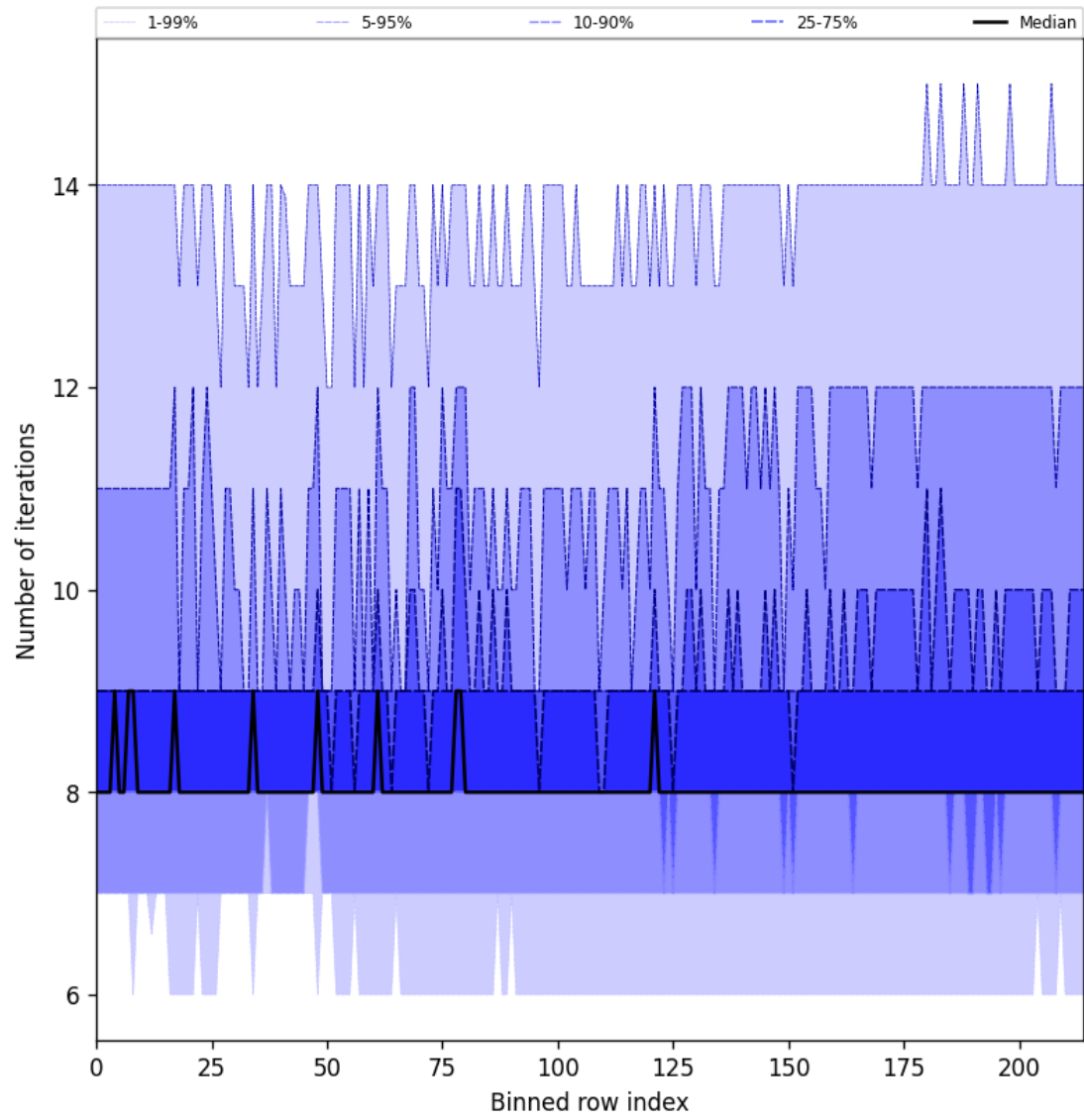
Figure 26: Along track statistics of “Number of iterations” for 2024-12-02 to 2024-12-03
