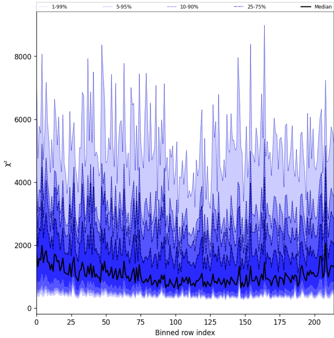
Figure 24: Along track statistics of “ \chi^2 ” for 2024-12-02 to 2024-12-03
