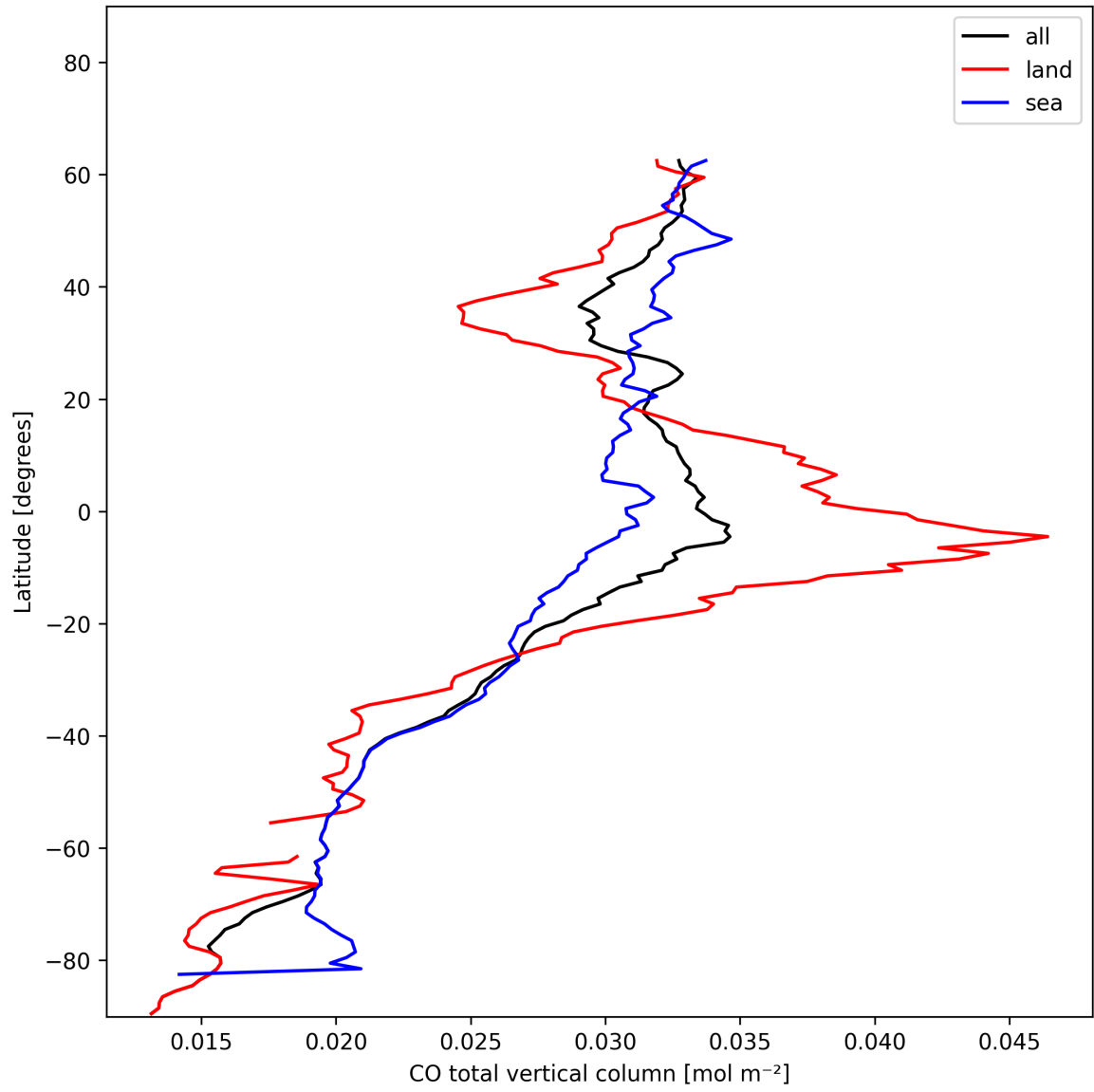
Figure 7: Zonal average of “CO total vertical column” for 2024-12-02 to 2024-12-03.
