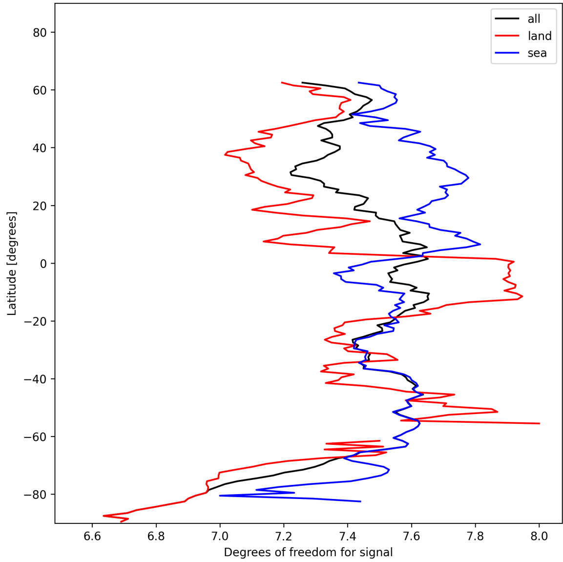
Figure 11: Zonal average of “Degrees of freedom for signal” for 2024-12-02 to 2024-12-03.
