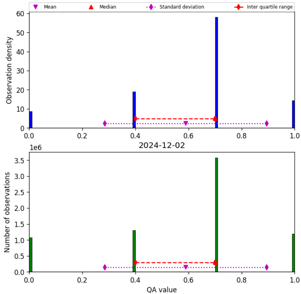
Figure 13: Histogram of “QA value” for 2024-12-02 to 2024-12-03
