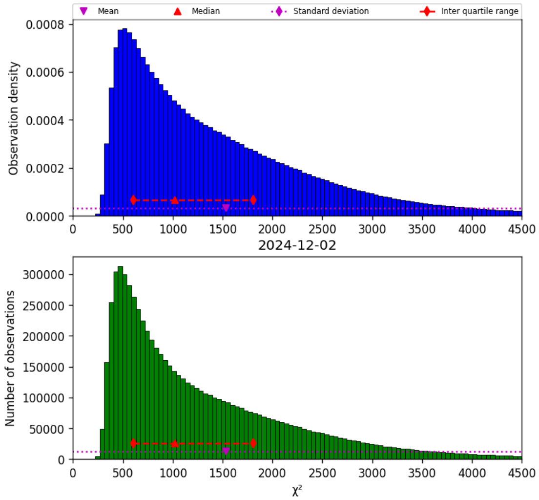
Figure 17: Histogram of " \chi^2 " for 2024-12-02 to 2024-12-03
