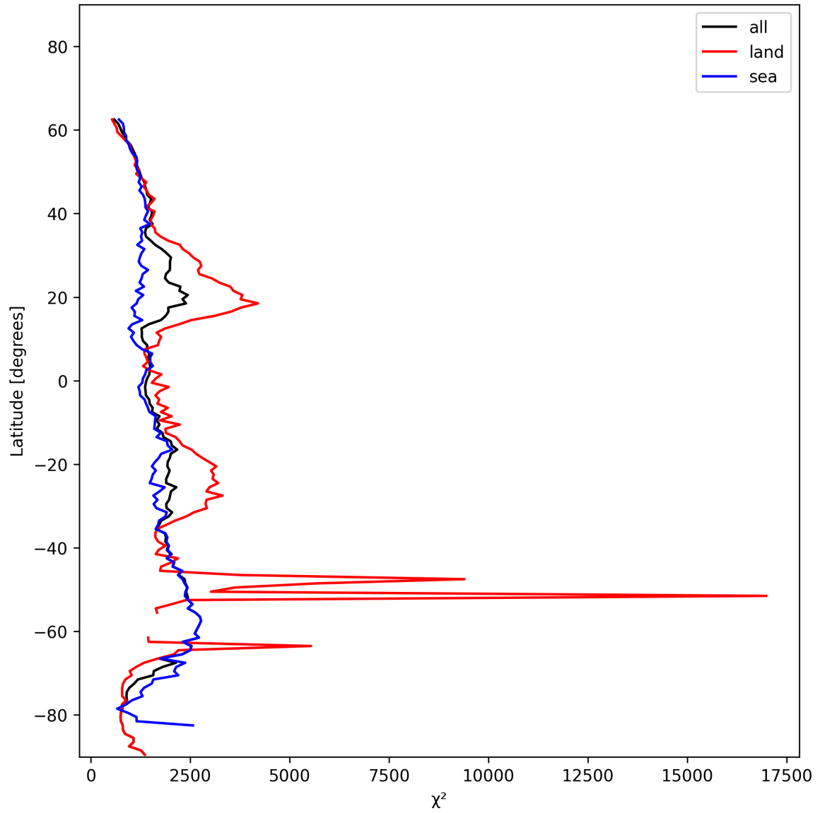
Figure 10: Zonal average of “ \chi^2 ” for 2024-12-02 to 2024-12-03.
