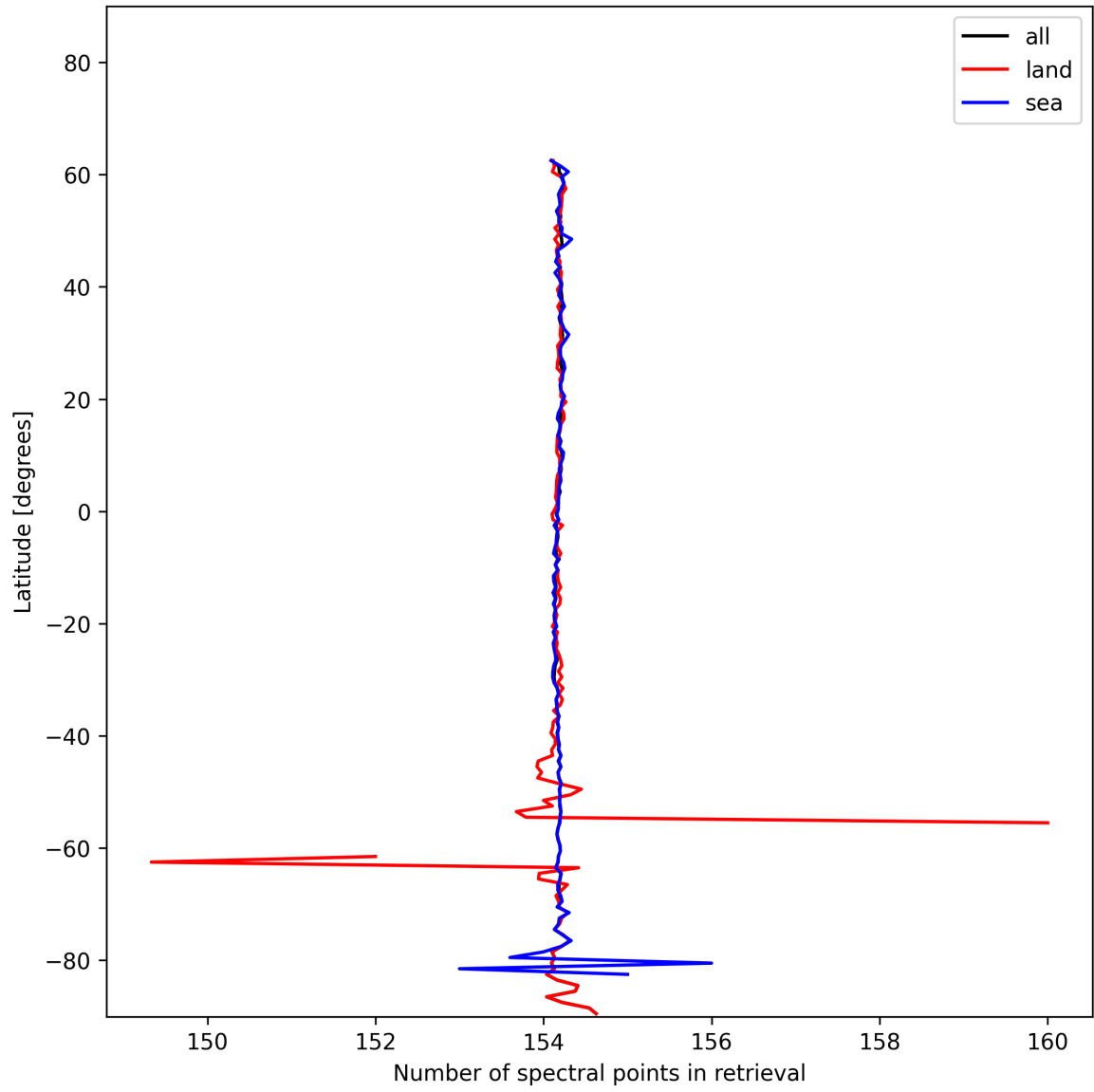
Figure 9: Zonal average of “Number of spectral points in retrieval” for 2024-12-02 to 2024-12-03.
