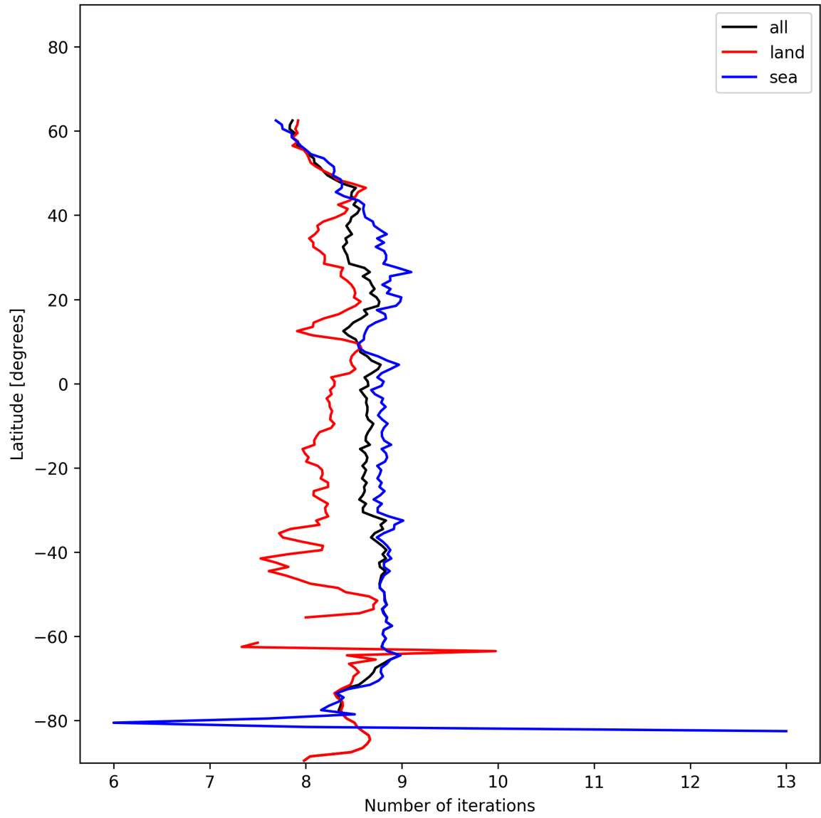
Figure 12: Zonal average of “Number of iterations” for 2024-12-02 to 2024-12-03.
