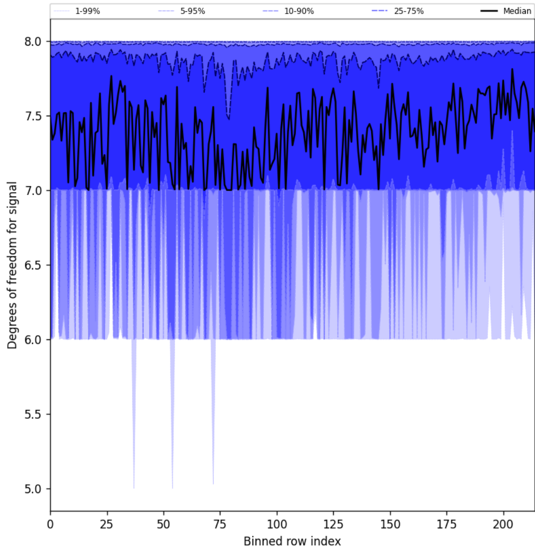
Figure 25: Along track statistics of “Degrees of freedom for signal” for 2024-12-02 to 2024-12-03
