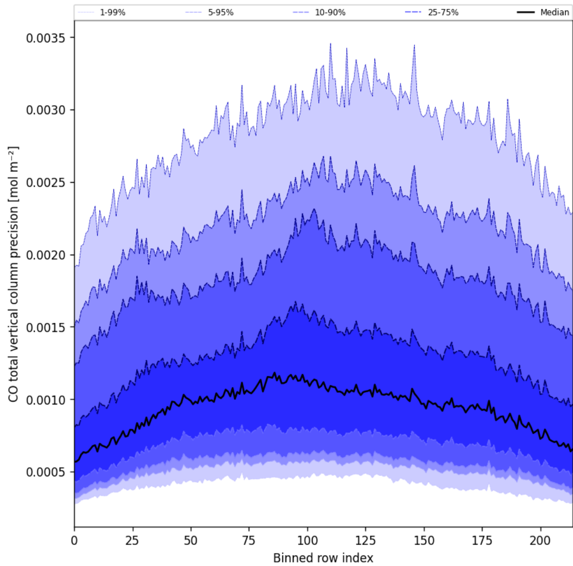
Figure 22: Along track statistics of “CO total vertical column precision” for 2024-12-02 to 2024-12-03
