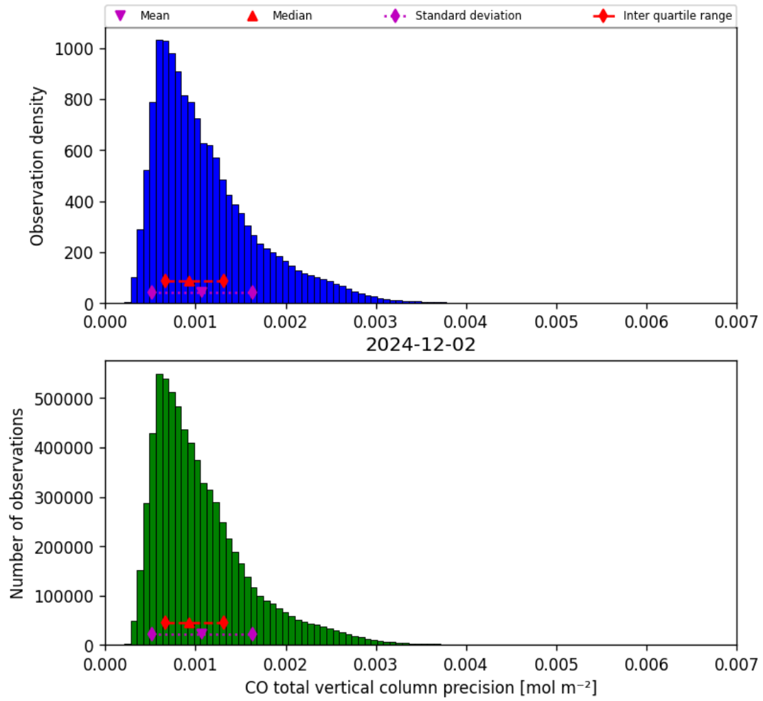
Figure 15: Histogram of “CO total vertical column precision” for 2024-12-02 to 2024-12-03
