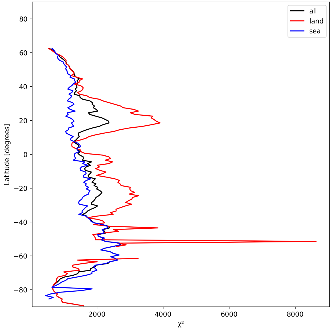
Figure 10: Zonal average of “ \chi^2 ” for 2024-12-04 to 2024-12-04.
