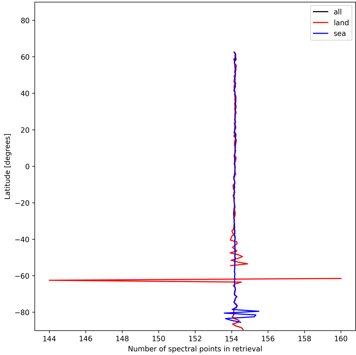
Figure 9: Zonal average of “Number of spectral points in retrieval” for 2024-12-04 to 2024-12-04.
