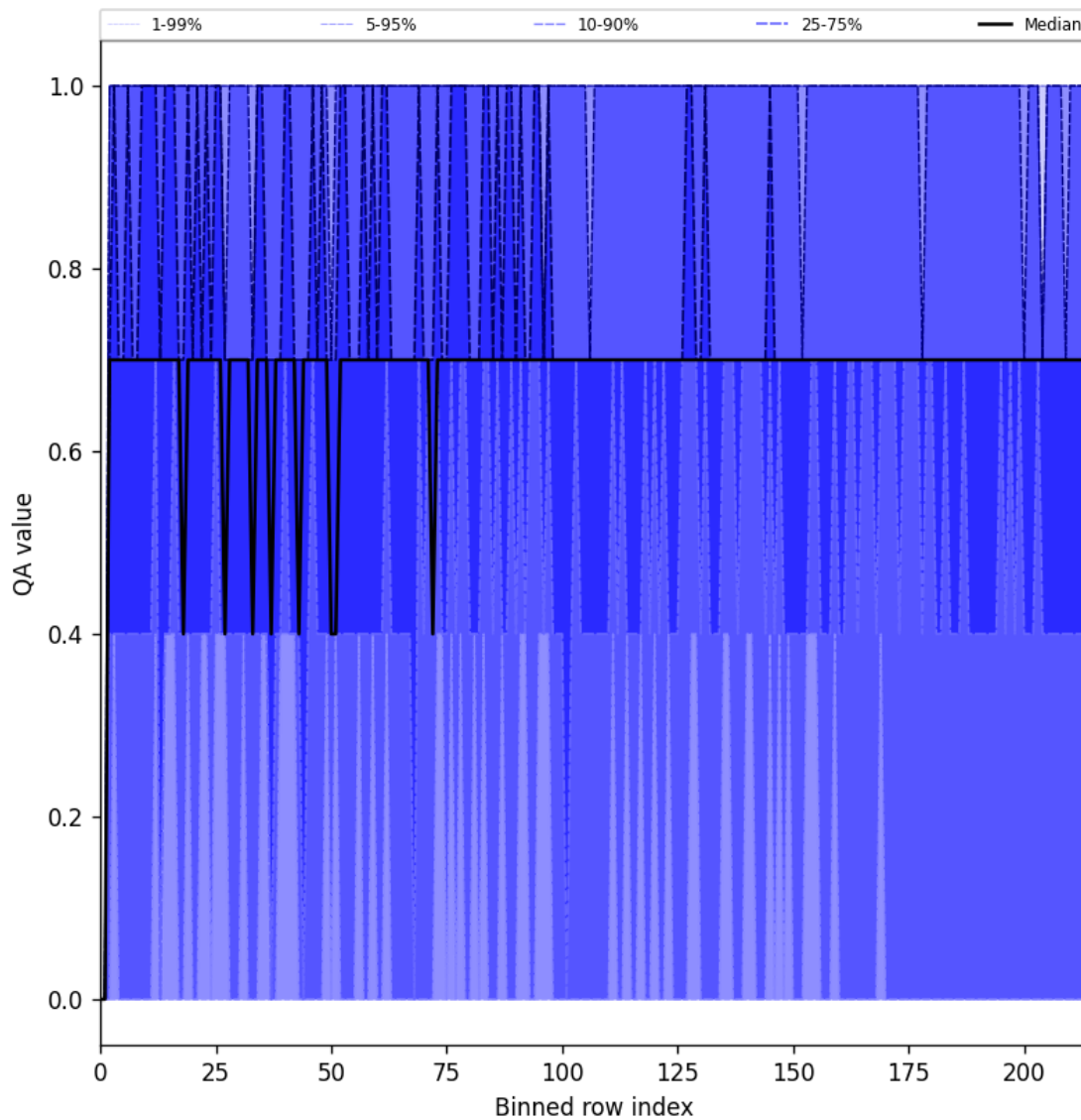
Figure 20: Along track statistics of “QA value” for 2024-12-04 to 2024-12-04
