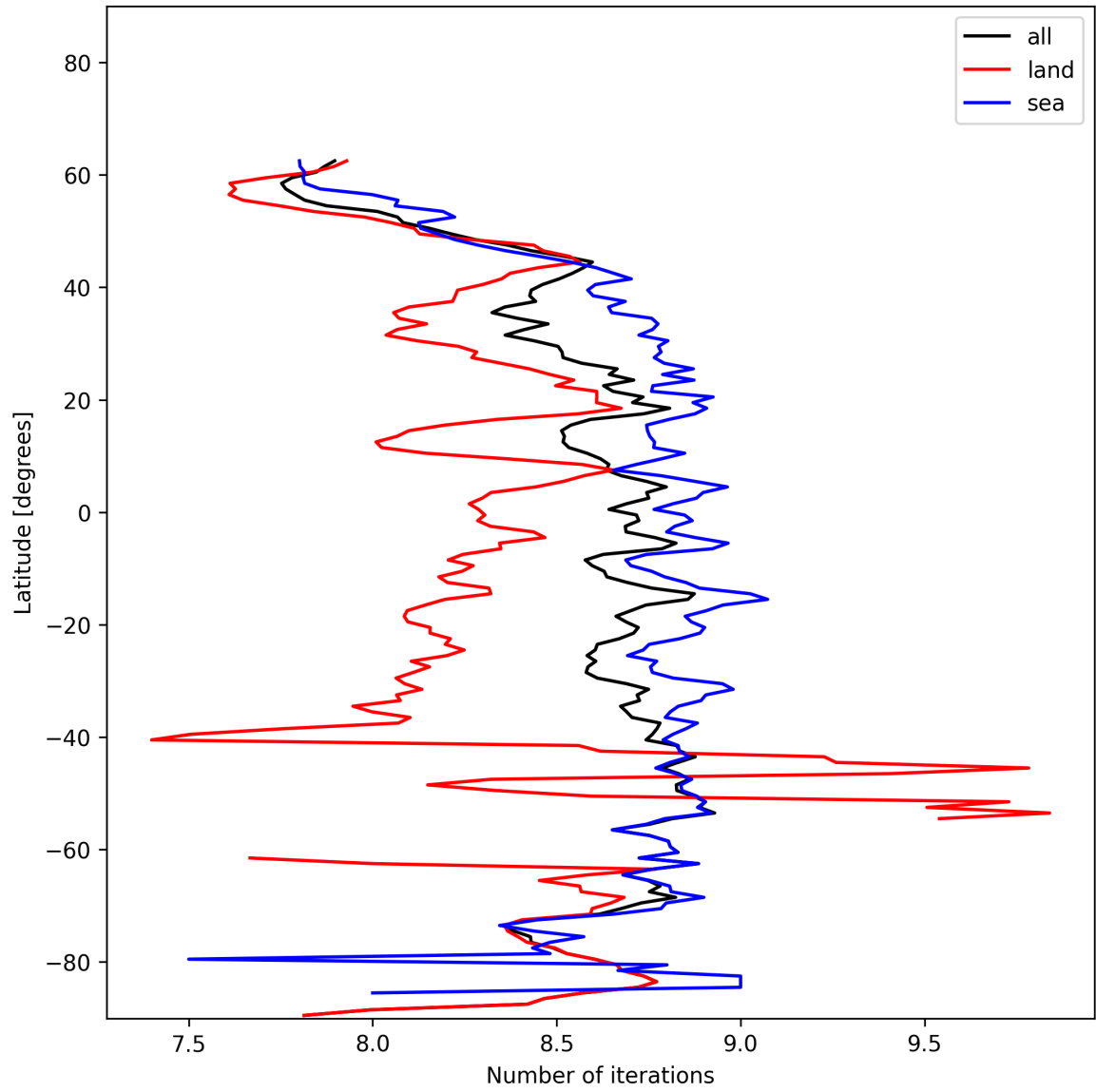
Figure 12: Zonal average of “Number of iterations” for 2024-12-04 to 2024-12-04.
