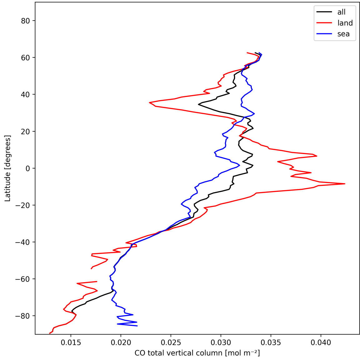
Figure 7: Zonal average of “CO total vertical column” for 2024-12-04 to 2024-12-04.
