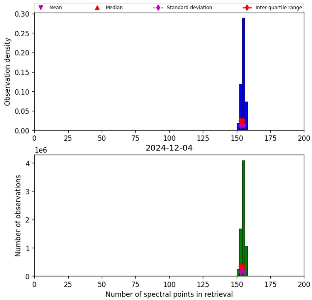
Figure 16: Histogram of “Number of spectral points in retrieval” for 2024-12-04 to 2024-12-04
