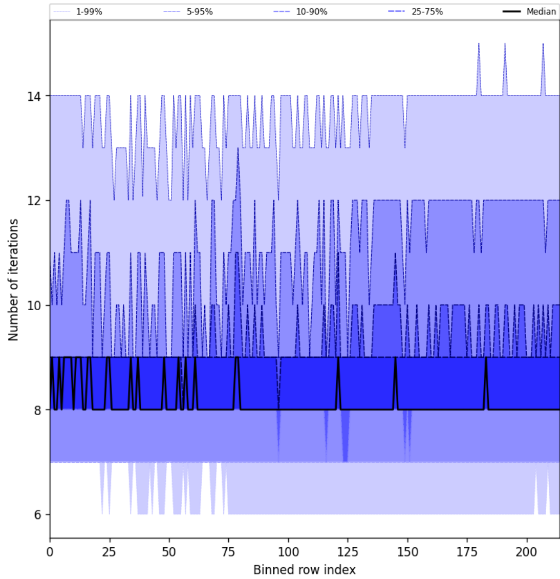
Figure 26: Along track statistics of “Number of iterations” for 2024-12-04 to 2024-12-04
