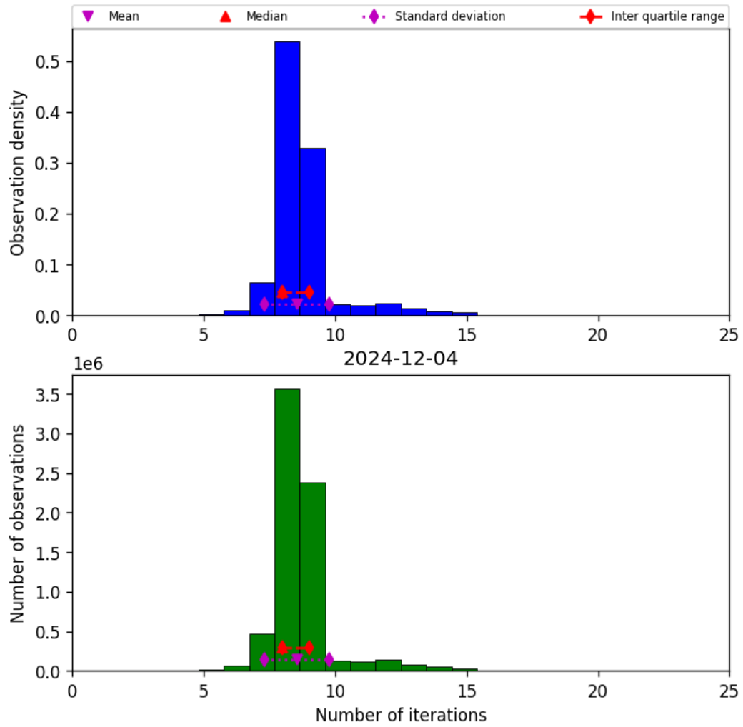
Figure 19: Histogram of “Number of iterations” for 2024-12-04 to 2024-12-04
