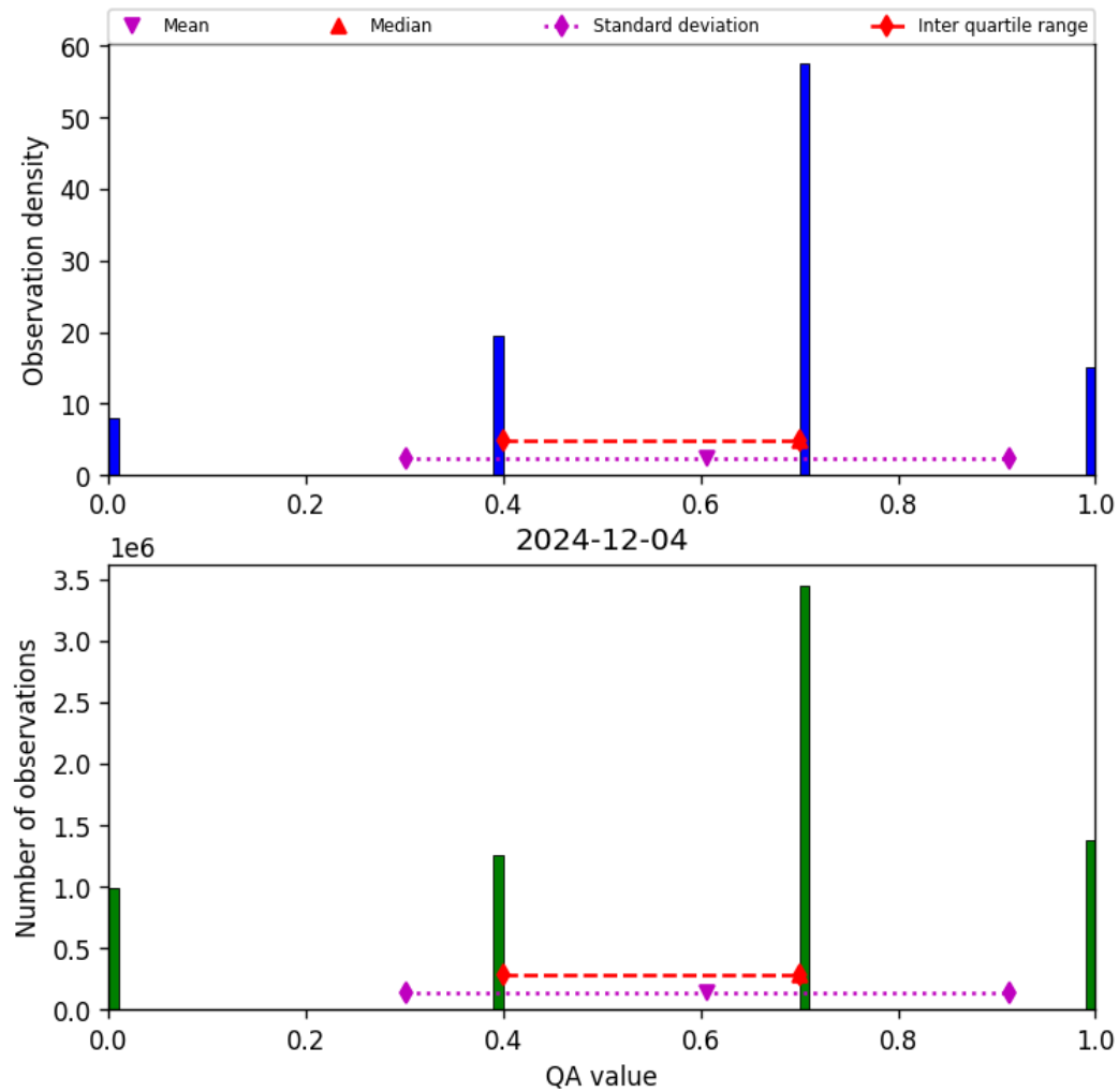
Figure 13: Histogram of “QA value” for 2024-12-04 to 2024-12-04
