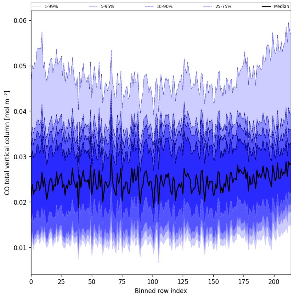
Figure 21: Along track statistics of “CO total vertical column” for 2024-12-04 to 2024-12-04
