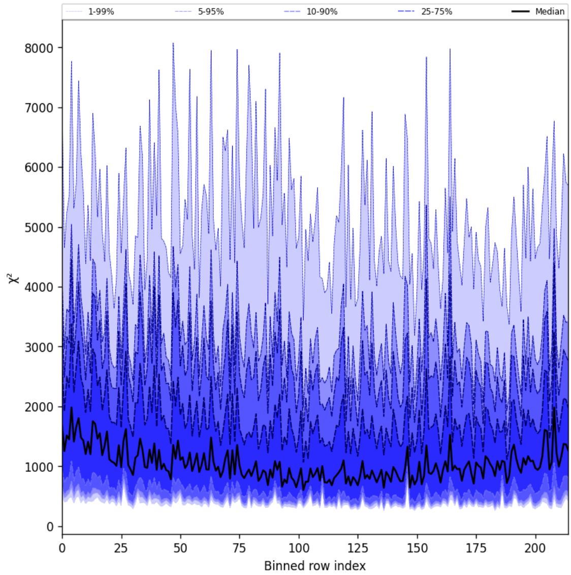
Figure 24: Along track statistics of “ \chi^2 ” for 2024-12-04 to 2024-12-04
