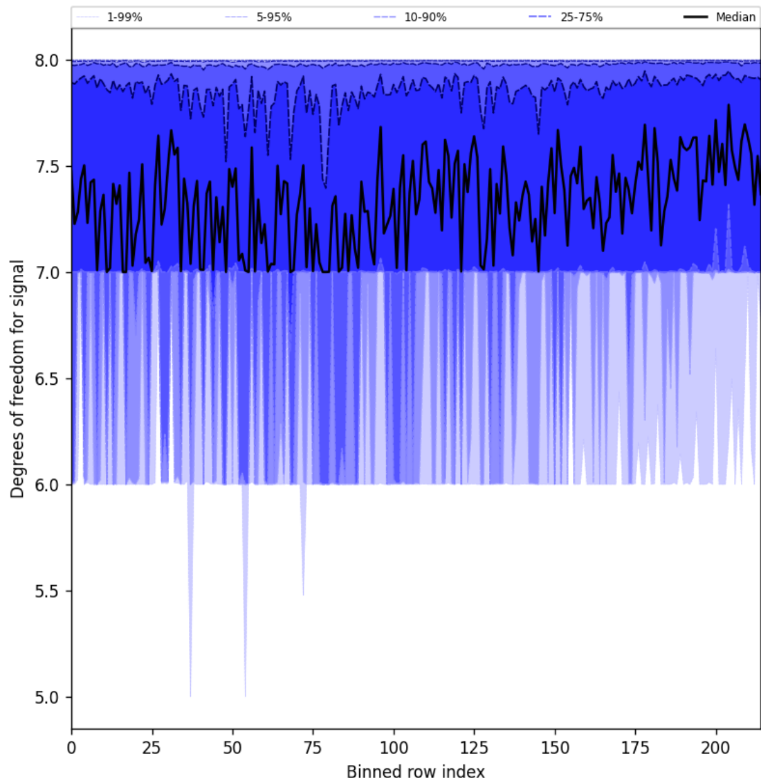
Figure 25: Along track statistics of “Degrees of freedom for signal” for 2024-12-04 to 2024-12-04
