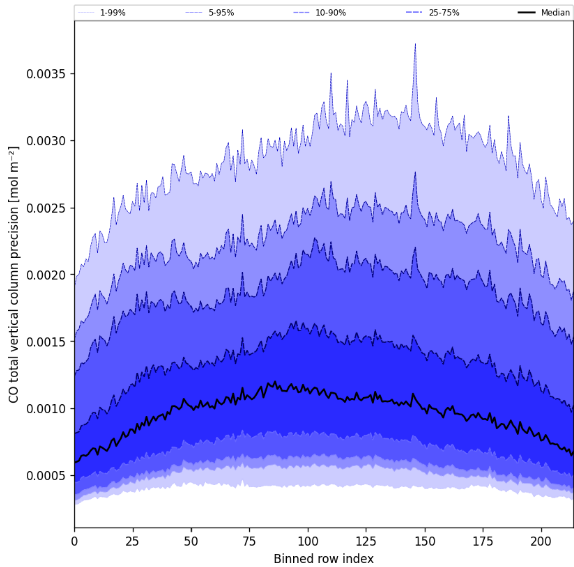
Figure 22: Along track statistics of “CO total vertical column precision” for 2024-12-04 to 2024-12-04
