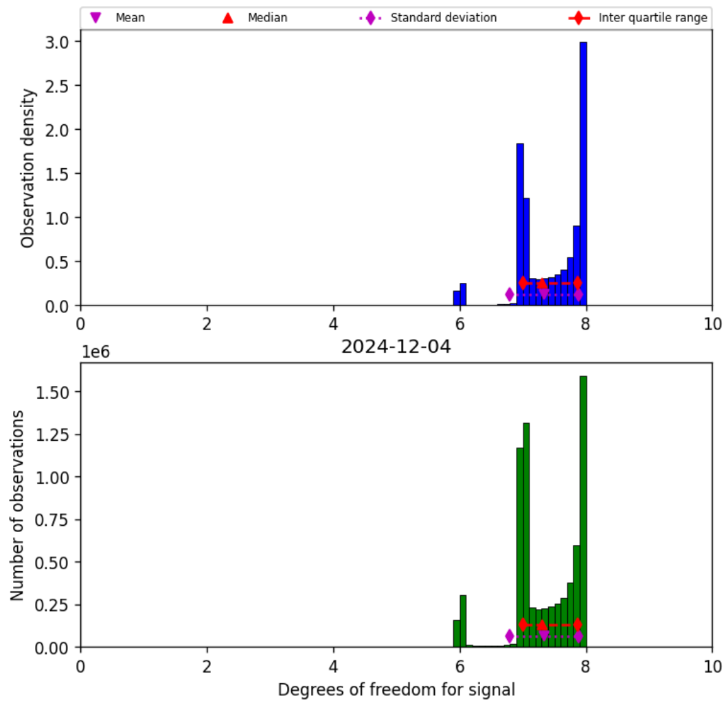
Figure 18: Histogram of “Degrees of freedom for signal” for 2024-12-04 to 2024-12-04
