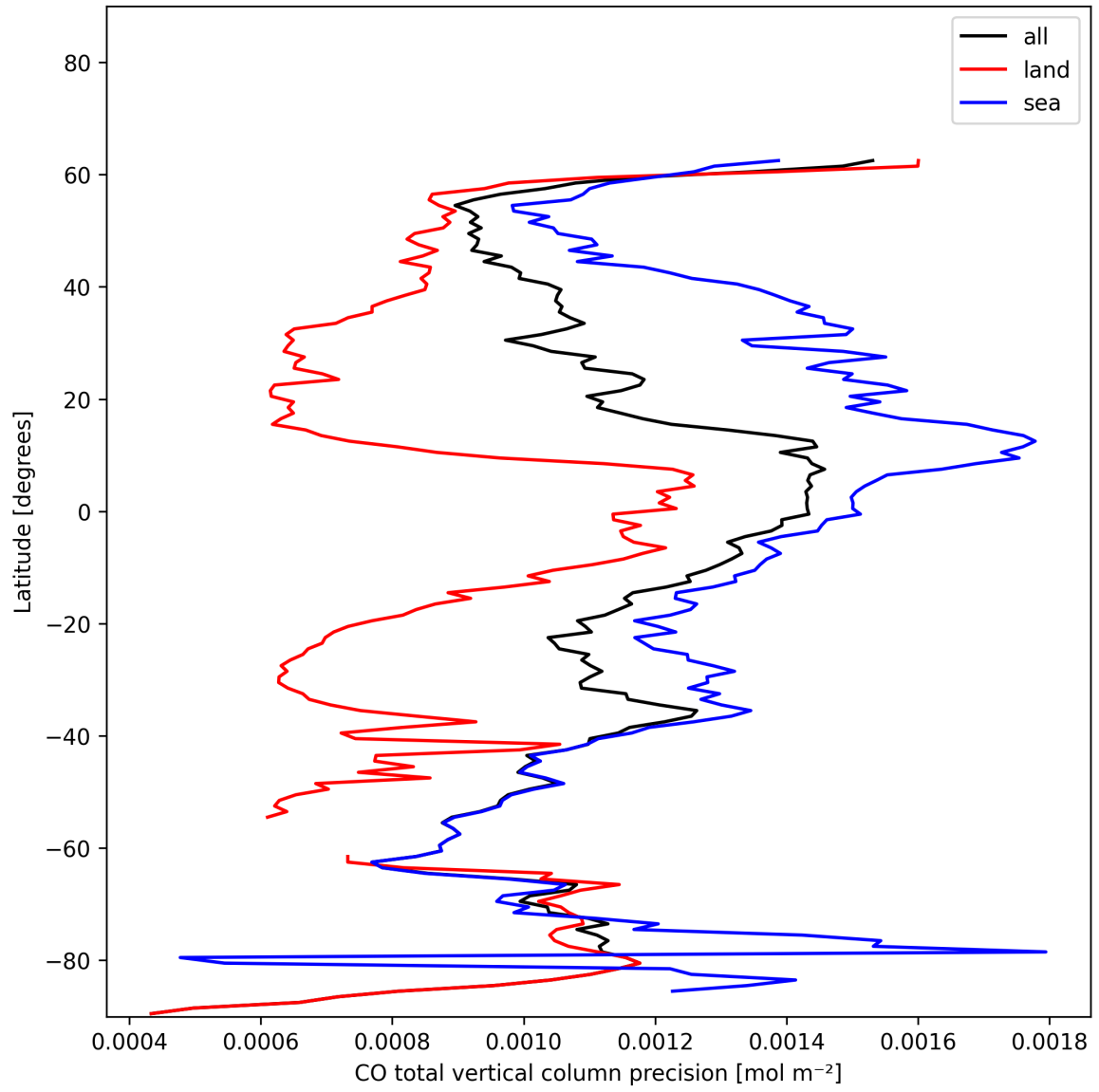
Figure 8: Zonal average of “CO total vertical column precision” for 2024-12-04 to 2024-12-04.
