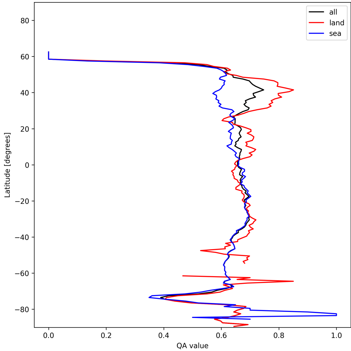
Figure 6: Zonal average of “QA value” for 2024-12-04 to 2024-12-04.
