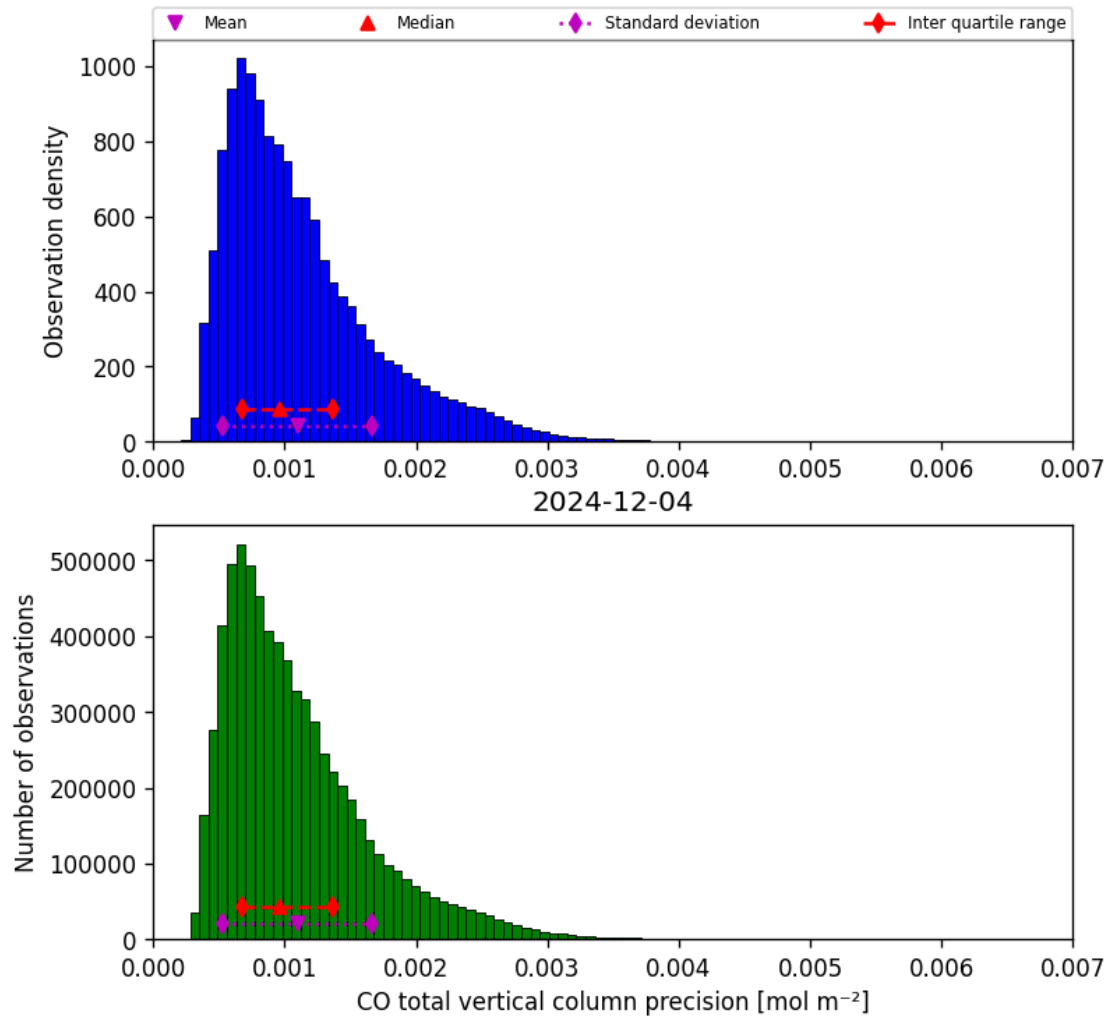
Figure 15: Histogram of “CO total vertical column precision” for 2024-12-04 to 2024-12-04
