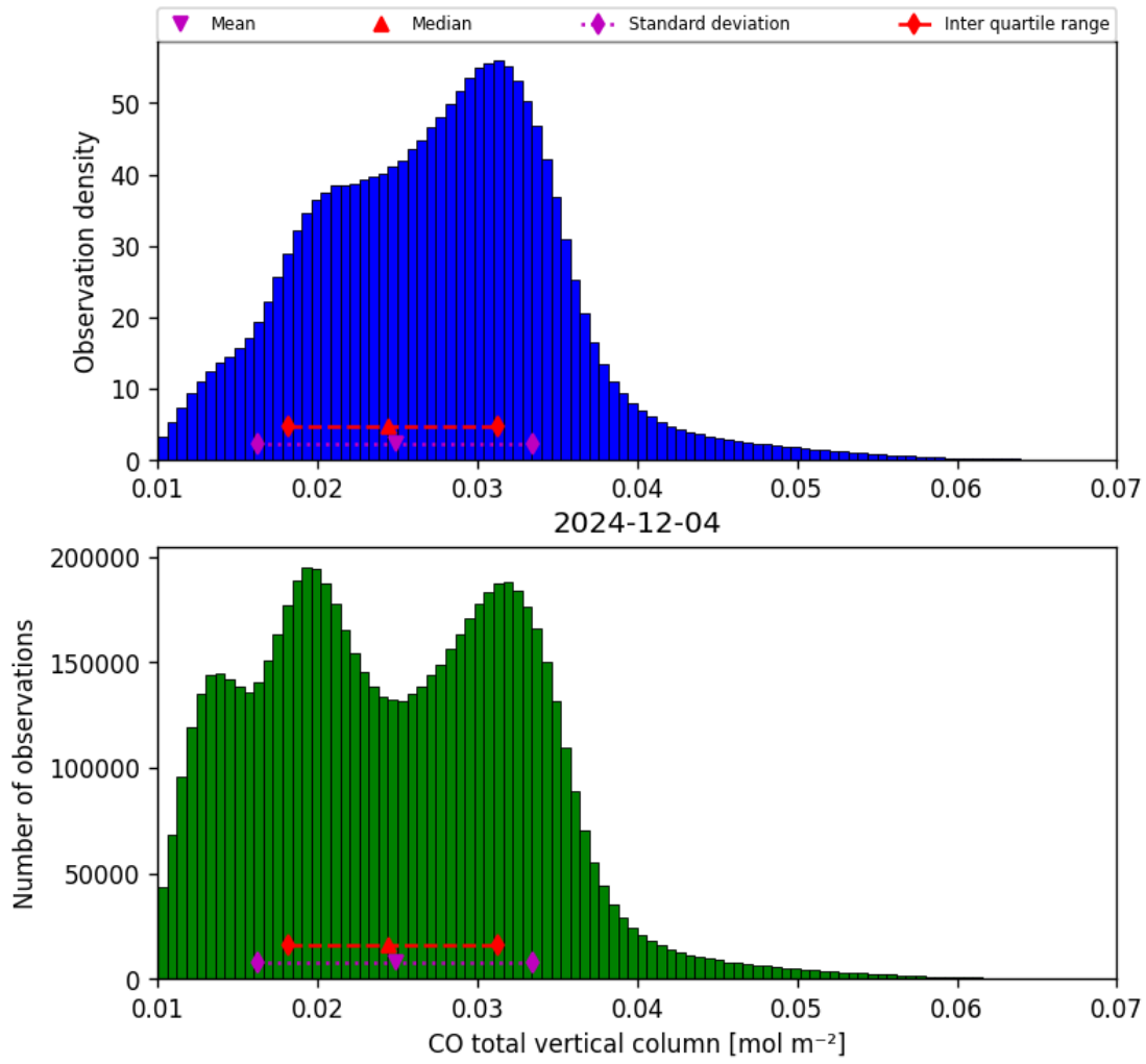
Figure 14: Histogram of “CO total vertical column” for 2024-12-04 to 2024-12-04
