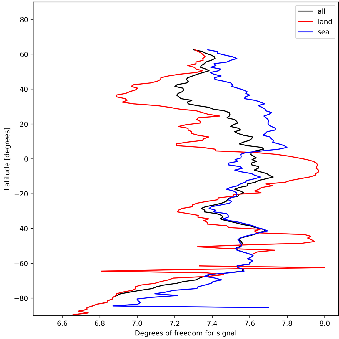
Figure 11: Zonal average of “Degrees of freedom for signal” for 2024-12-04 to 2024-12-04.
