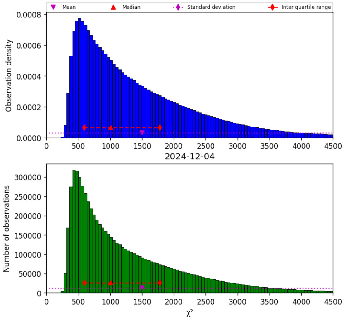
Figure 17: Histogram of " \chi^2 " for 2024-12-04 to 2024-12-04
