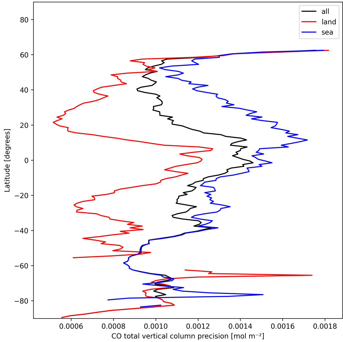
Figure 8: Zonal average of “CO total vertical column precision” for 2024-12-06 to 2024-12-07.
