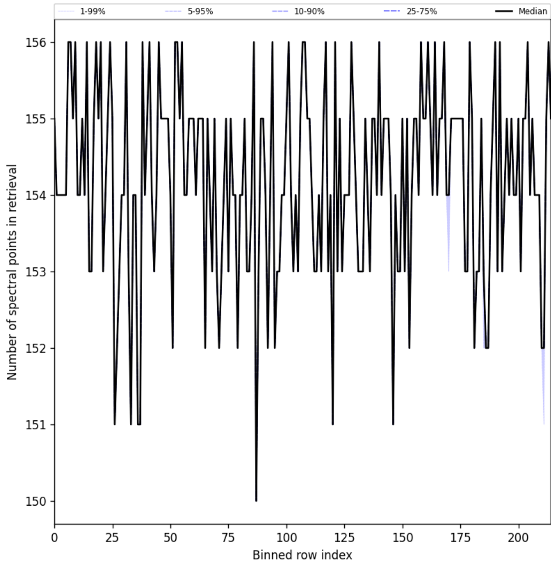
Figure 23: Along track statistics of “Number of spectral points in retrieval” for 2024-12-06 to 2024-12-07
