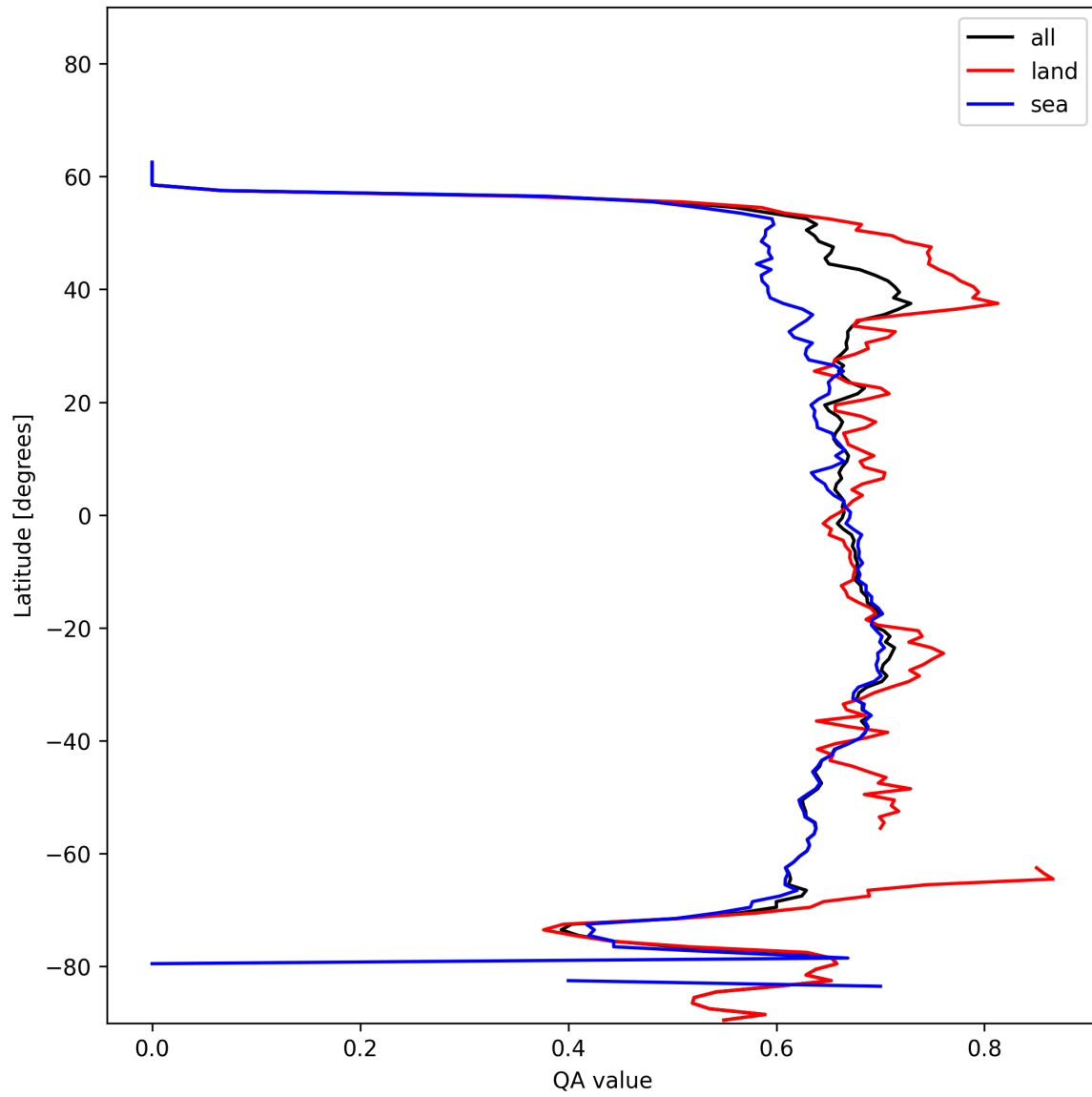
Figure 6: Zonal average of “QA value” for 2024-12-06 to 2024-12-07.
