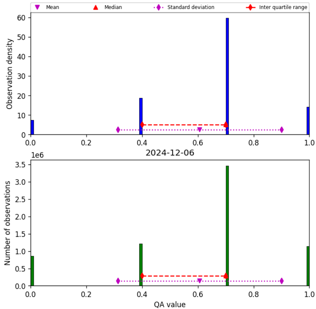
Figure 13: Histogram of “QA value” for 2024-12-06 to 2024-12-07
