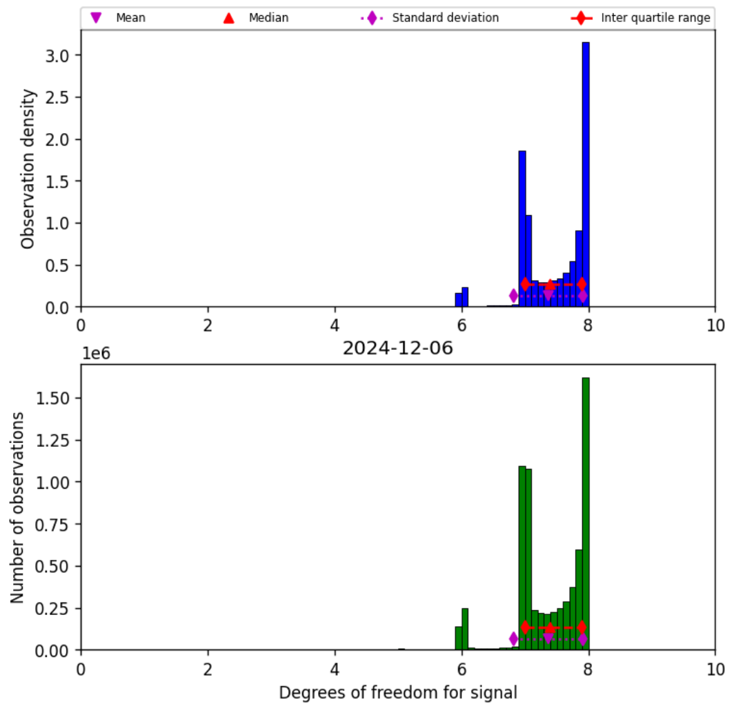
Figure 18: Histogram of “Degrees of freedom for signal” for 2024-12-06 to 2024-12-07
