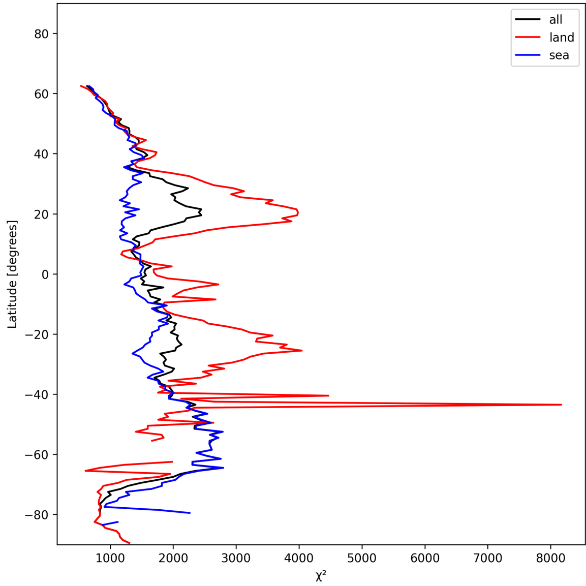
Figure 10: Zonal average of “ \chi^2 ” for 2024-12-06 to 2024-12-07.
