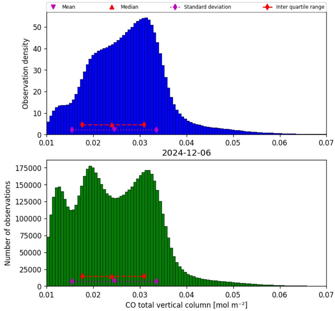
Figure 14: Histogram of “CO total vertical column” for 2024-12-06 to 2024-12-07
