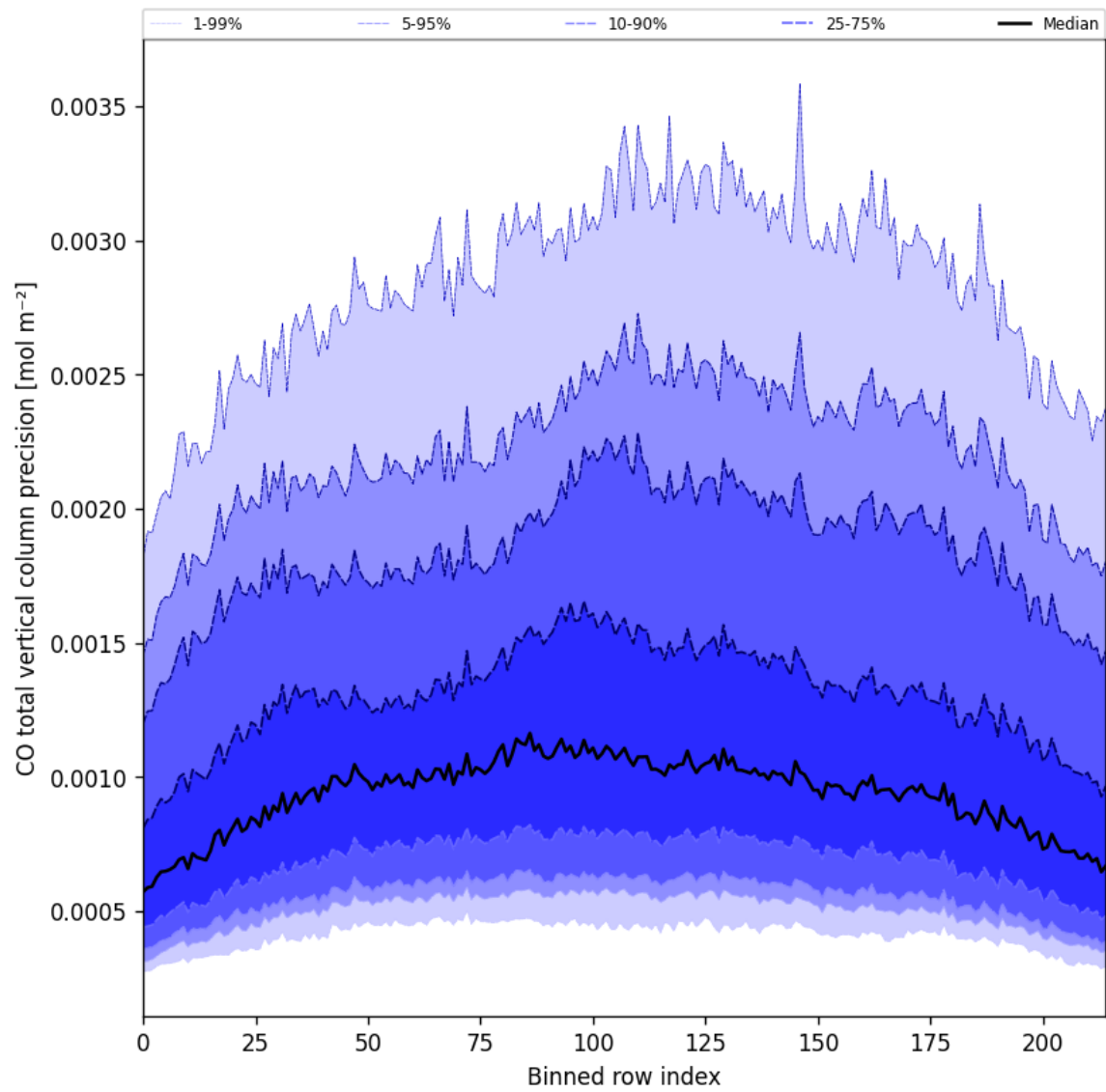
Figure 22: Along track statistics of “CO total vertical column precision” for 2024-12-06 to 2024-12-07
