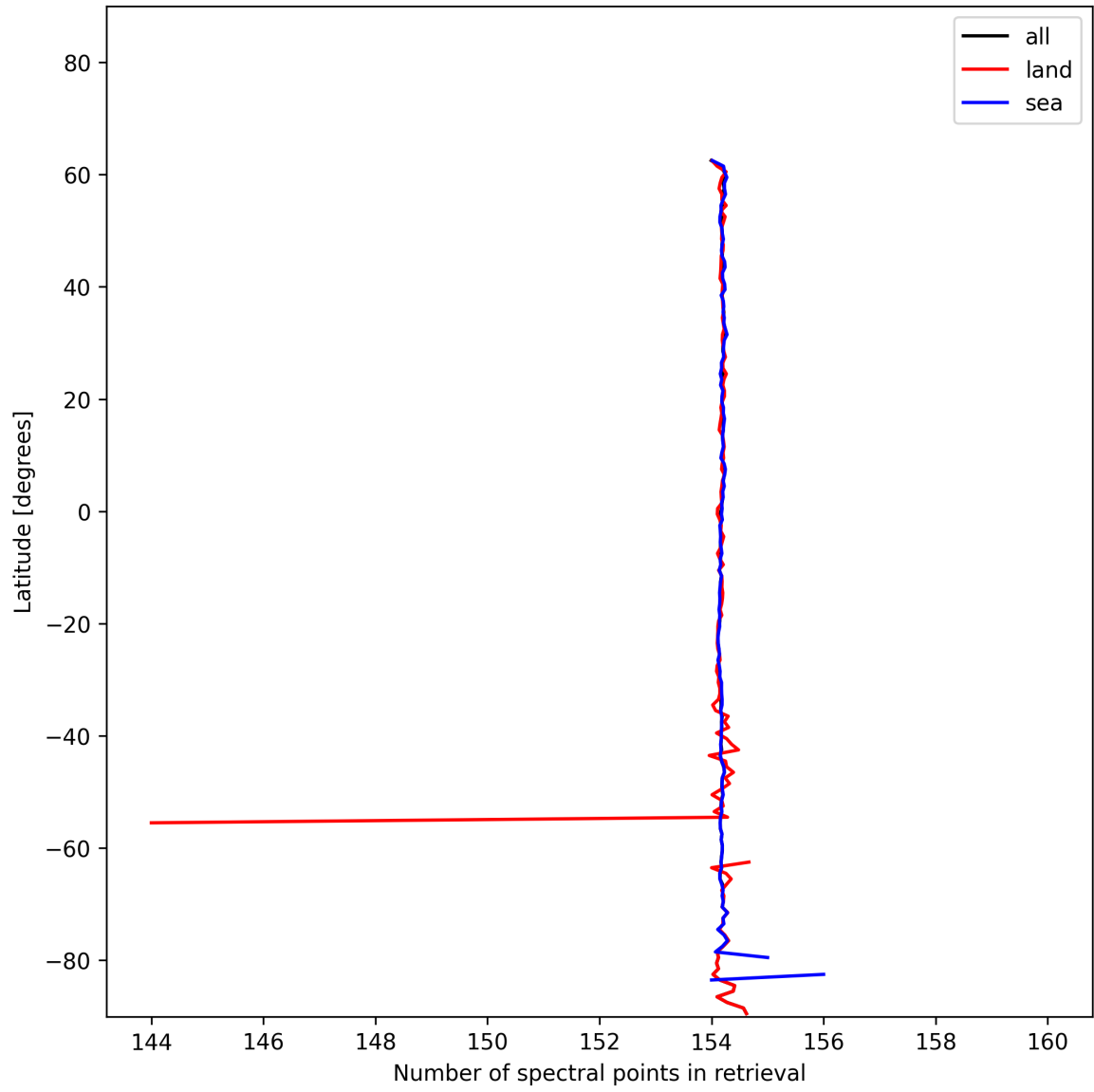
Figure 9: Zonal average of “Number of spectral points in retrieval” for 2024-12-06 to 2024-12-07.
