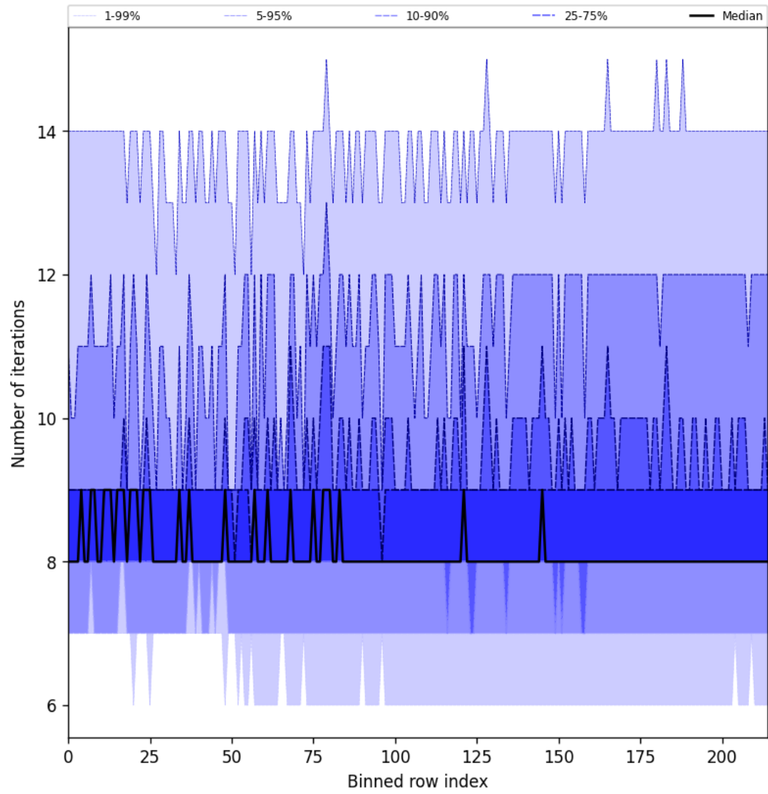
Figure 26: Along track statistics of “Number of iterations” for 2024-12-06 to 2024-12-07
