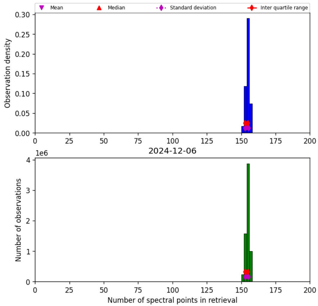
Figure 16: Histogram of "Number of spectral points in retrieval" for 2024-12-06 to 2024-12-07
