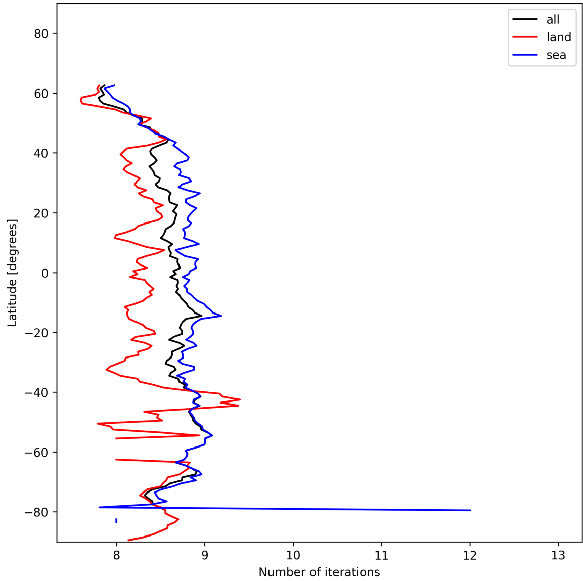
Figure 12: Zonal average of “Number of iterations” for 2024-12-06 to 2024-12-07.
