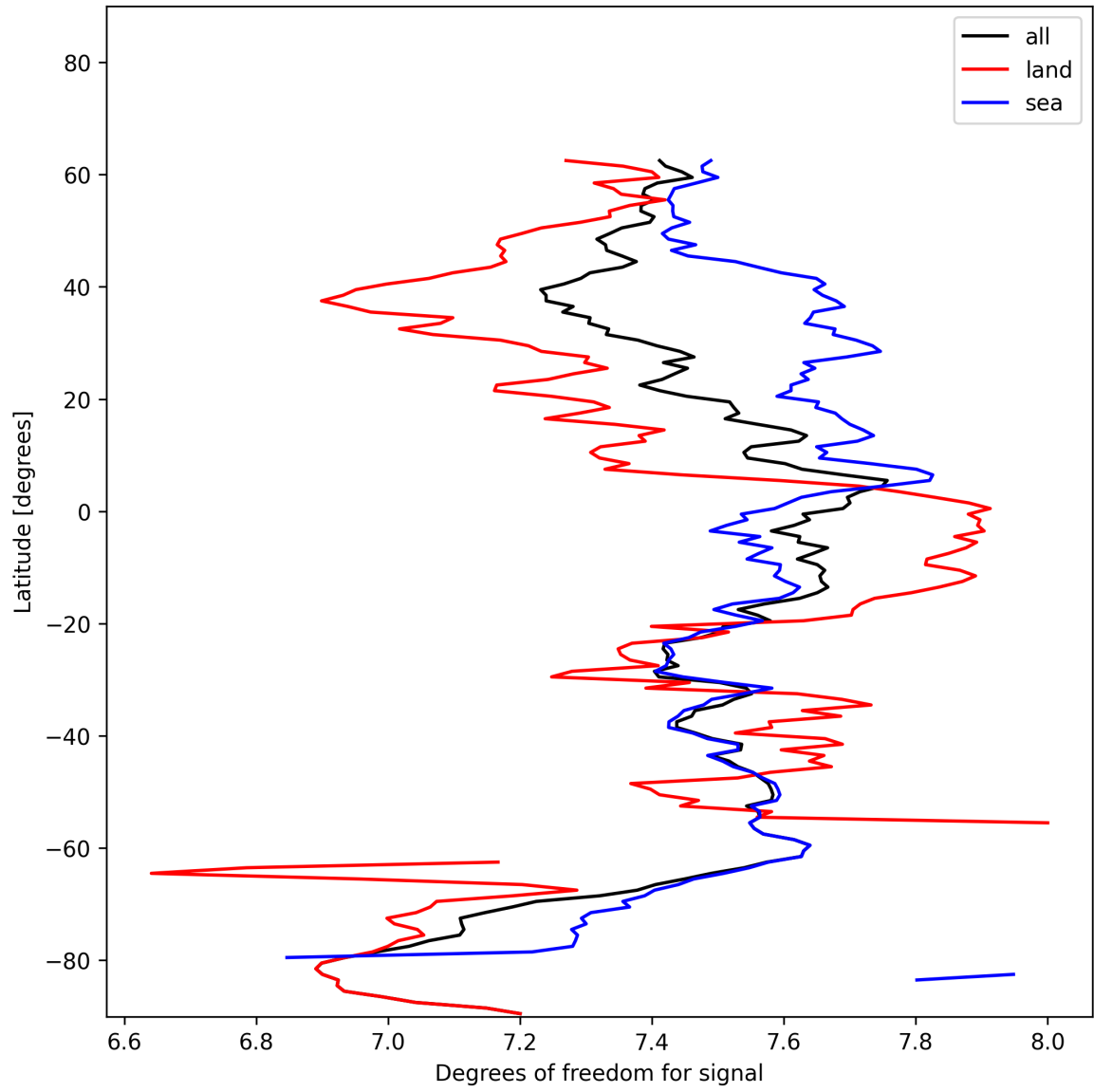
Figure 11: Zonal average of “Degrees of freedom for signal” for 2024-12-06 to 2024-12-07.
