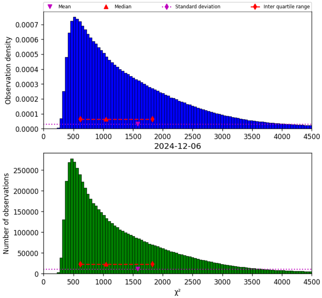
Figure 17: Histogram of " \chi^2 " for 2024-12-06 to 2024-12-07
