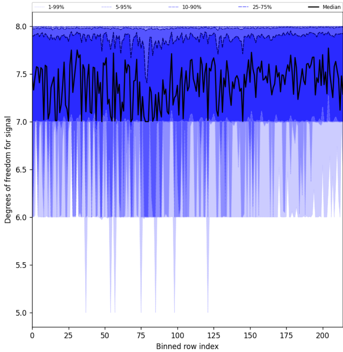
Figure 25: Along track statistics of “Degrees of freedom for signal” for 2024-12-06 to 2024-12-07
