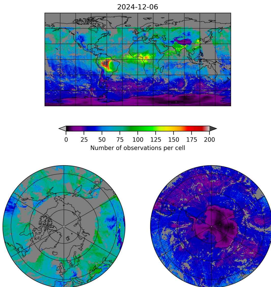
Figure 5: Map of the number of observations for 2024-12-06 to 2024-12-07
