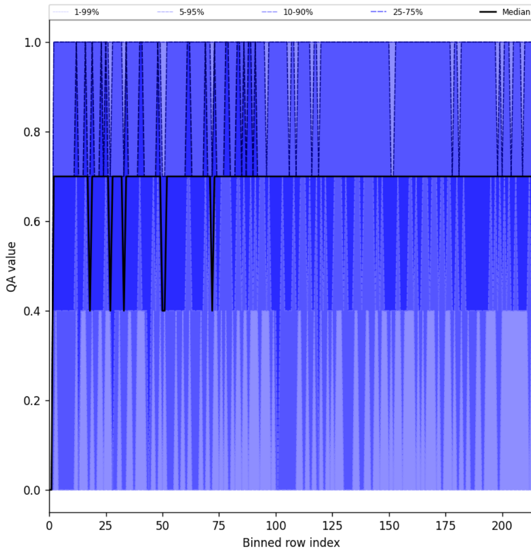
Figure 20: Along track statistics of “QA value” for 2024-12-06 to 2024-12-07
