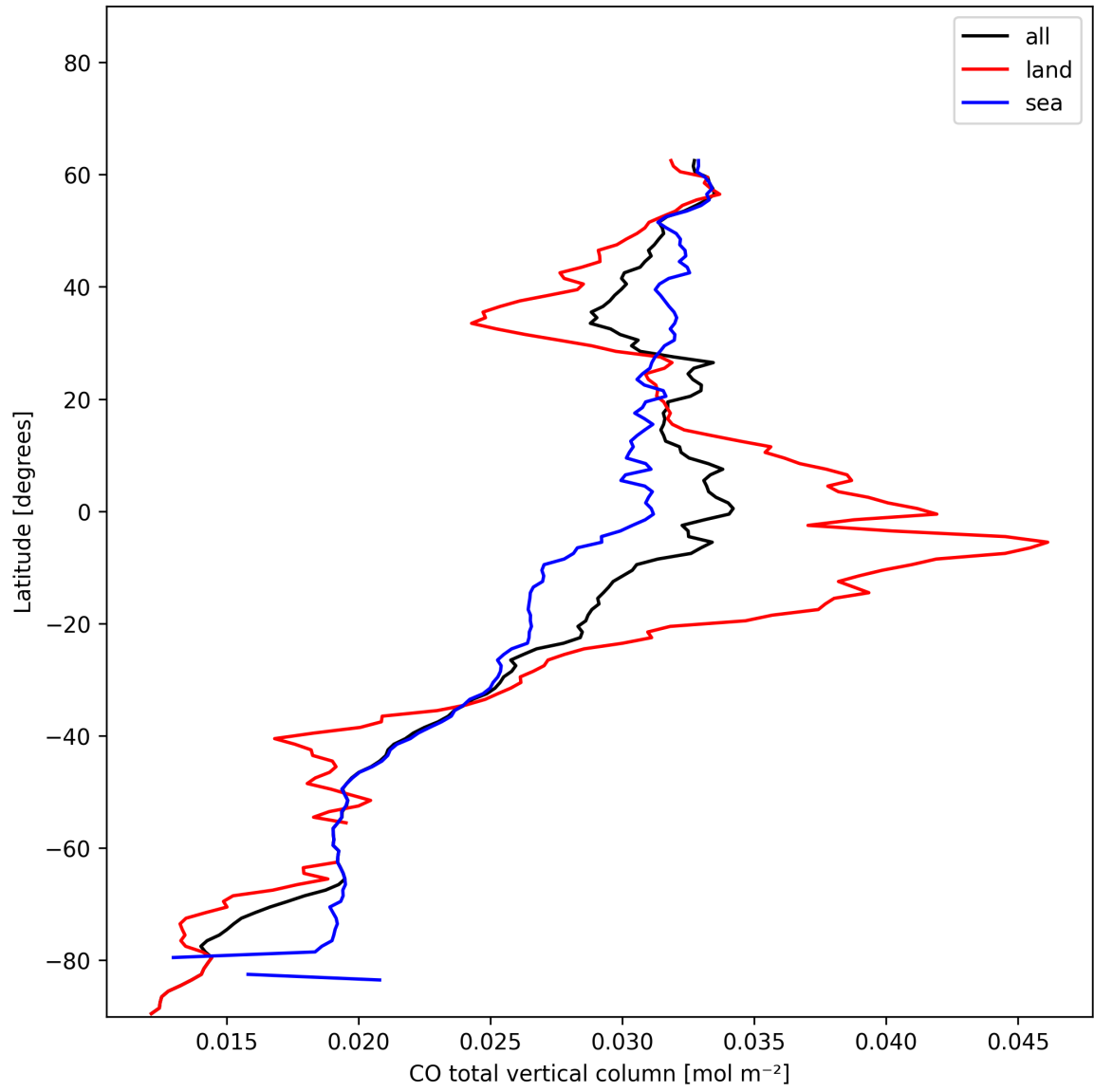
Figure 7: Zonal average of “CO total vertical column” for 2024-12-06 to 2024-12-07.
