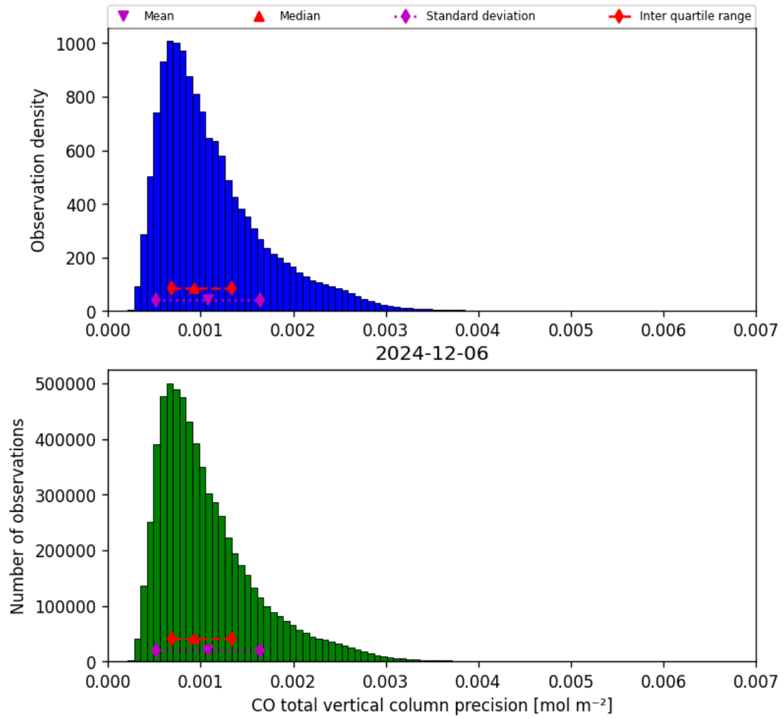
Figure 15: Histogram of “CO total vertical column precision” for 2024-12-06 to 2024-12-07
