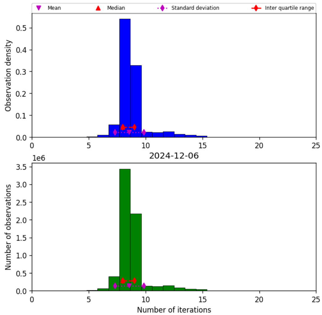
Figure 19: Histogram of “Number of iterations” for 2024-12-06 to 2024-12-07
