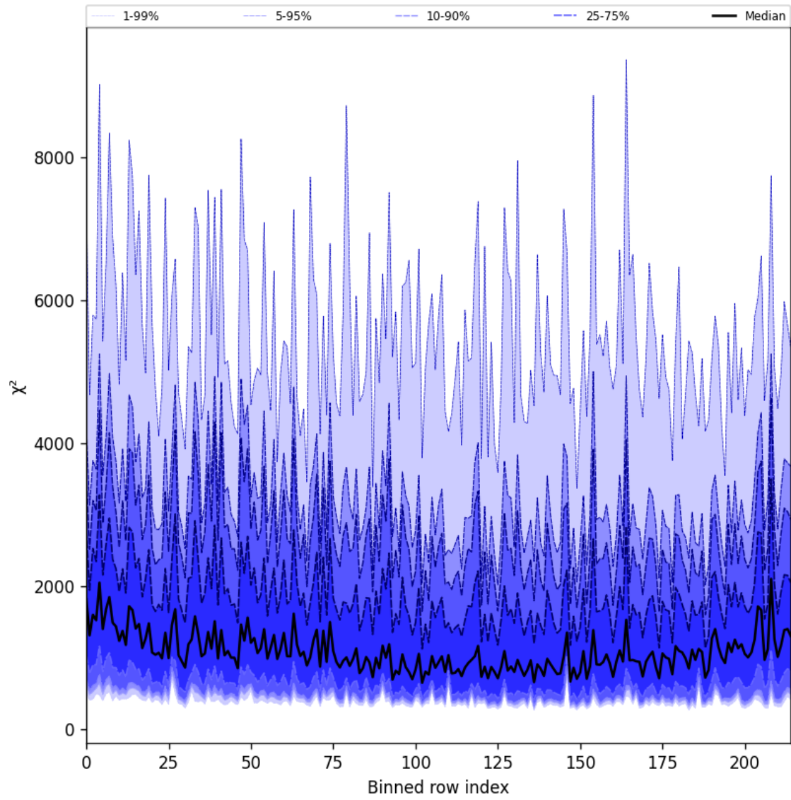
Figure 24: Along track statistics of “ \chi^2 ” for 2024-12-06 to 2024-12-07
