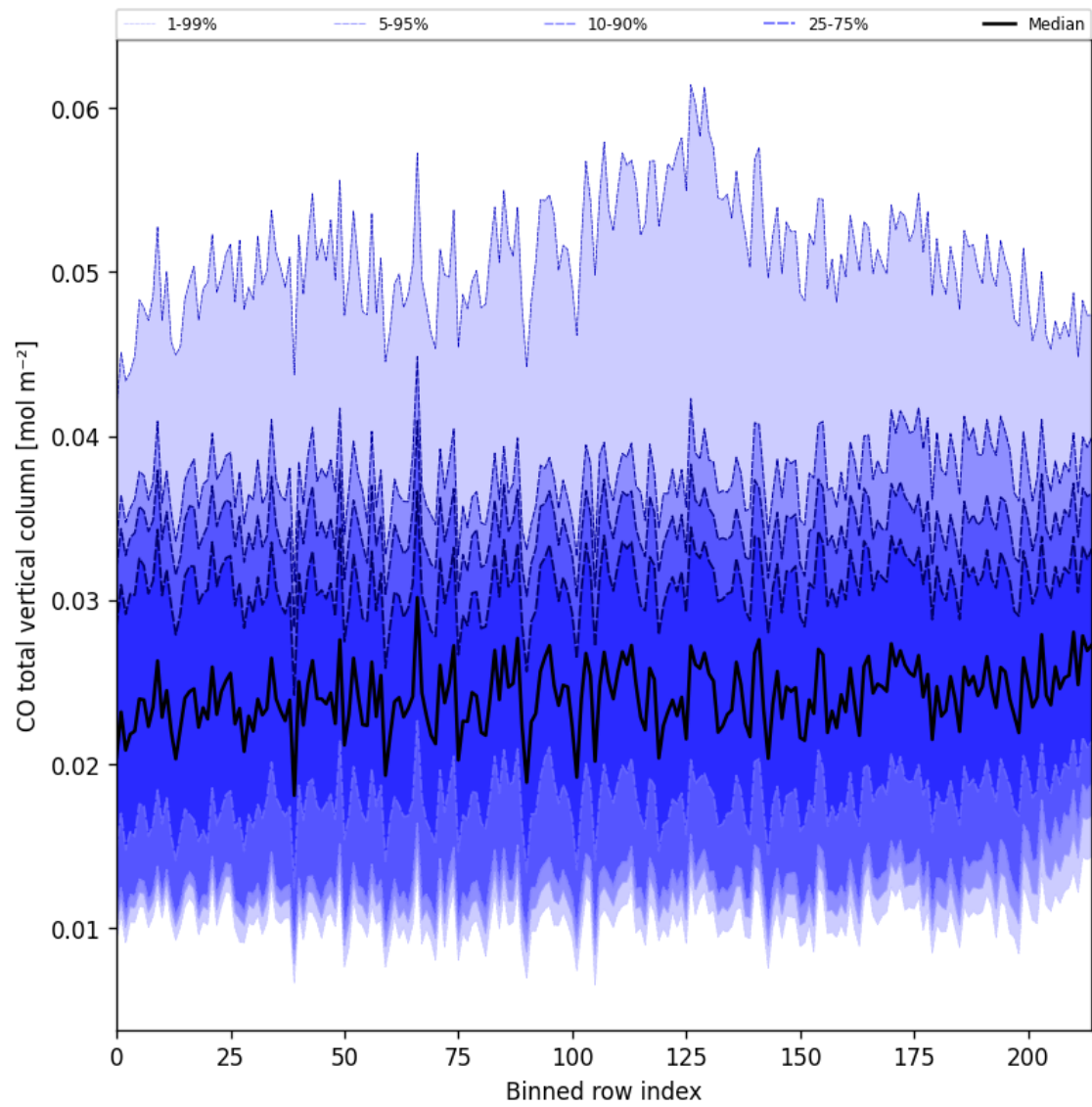
Figure 21: Along track statistics of “CO total vertical column” for 2024-12-06 to 2024-12-07
