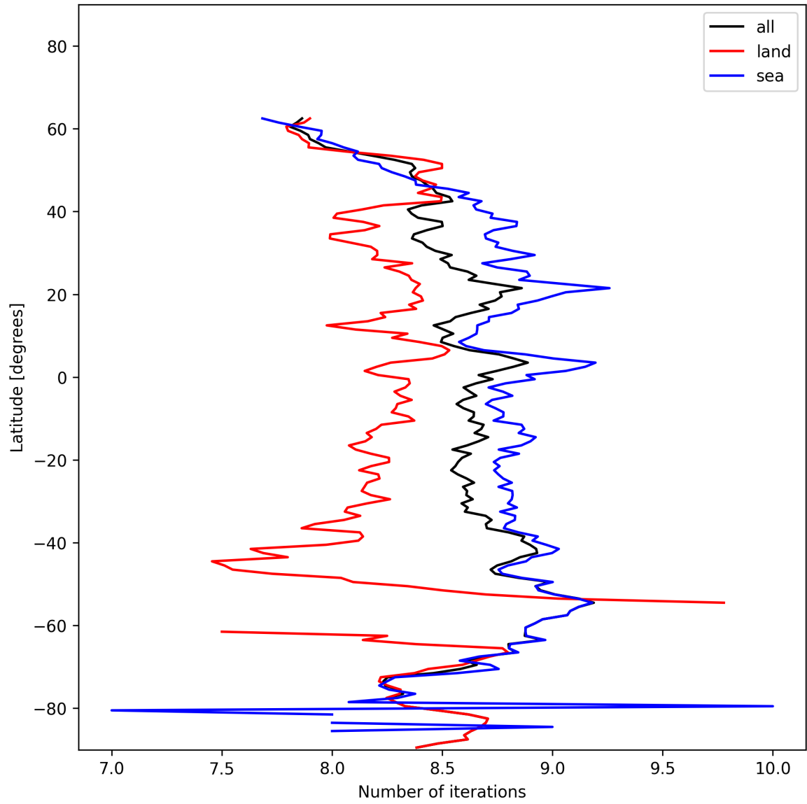
Figure 12: Zonal average of “Number of iterations” for 2024-12-07 to 2024-12-08.
