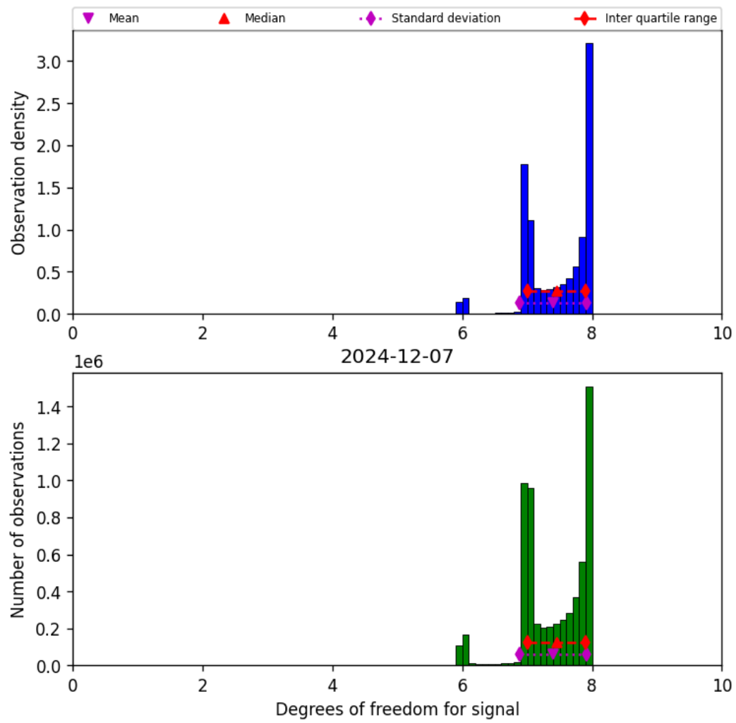
Figure 18: Histogram of “Degrees of freedom for signal” for 2024-12-07 to 2024-12-08
