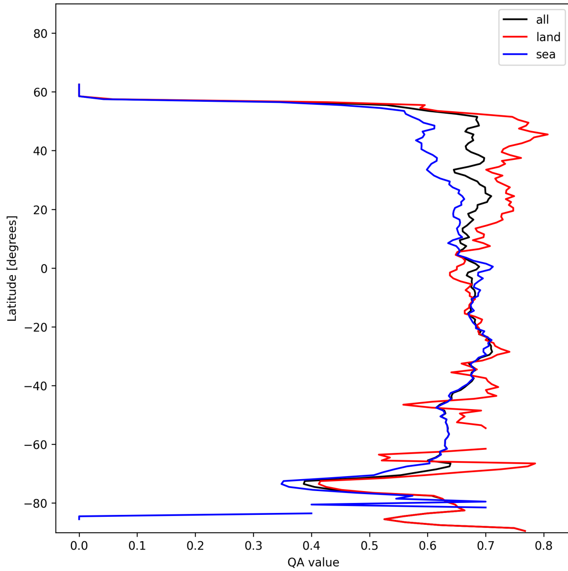
Figure 6: Zonal average of “QA value” for 2024-12-07 to 2024-12-08.
