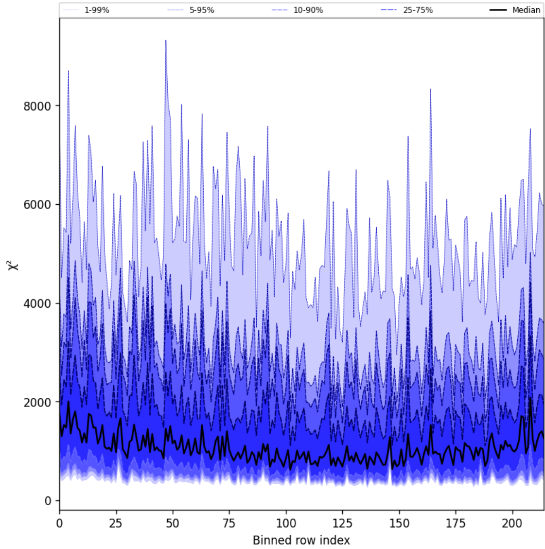
Figure 24: Along track statistics of “ \chi^2 ” for 2024-12-07 to 2024-12-08
