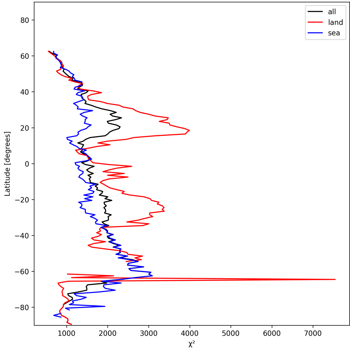
Figure 10: Zonal average of “ \chi^2 ” for 2024-12-07 to 2024-12-08.
