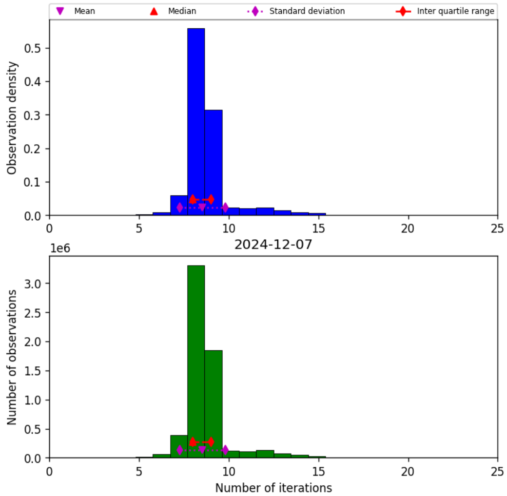
Figure 19: Histogram of “Number of iterations” for 2024-12-07 to 2024-12-08
