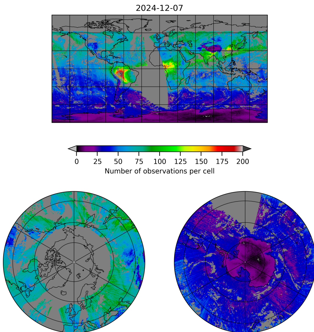
Figure 5: Map of the number of observations for 2024-12-07 to 2024-12-08
