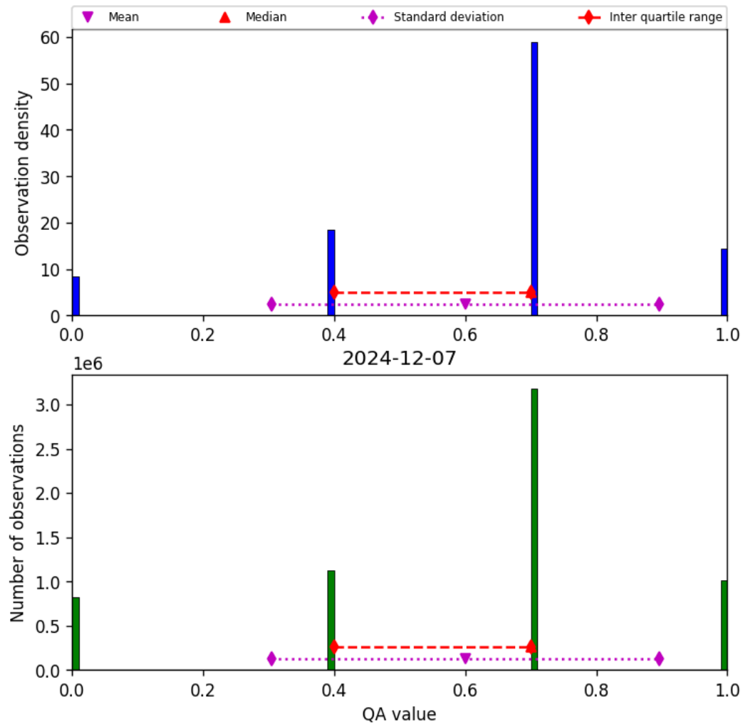
Figure 13: Histogram of “QA value” for 2024-12-07 to 2024-12-08
