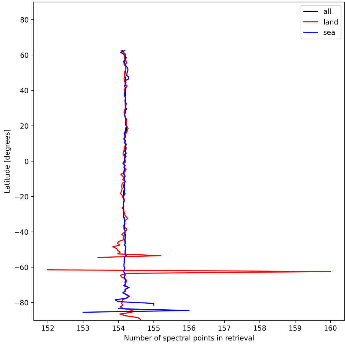
Figure 9: Zonal average of “Number of spectral points in retrieval” for 2024-12-07 to 2024-12-08.
