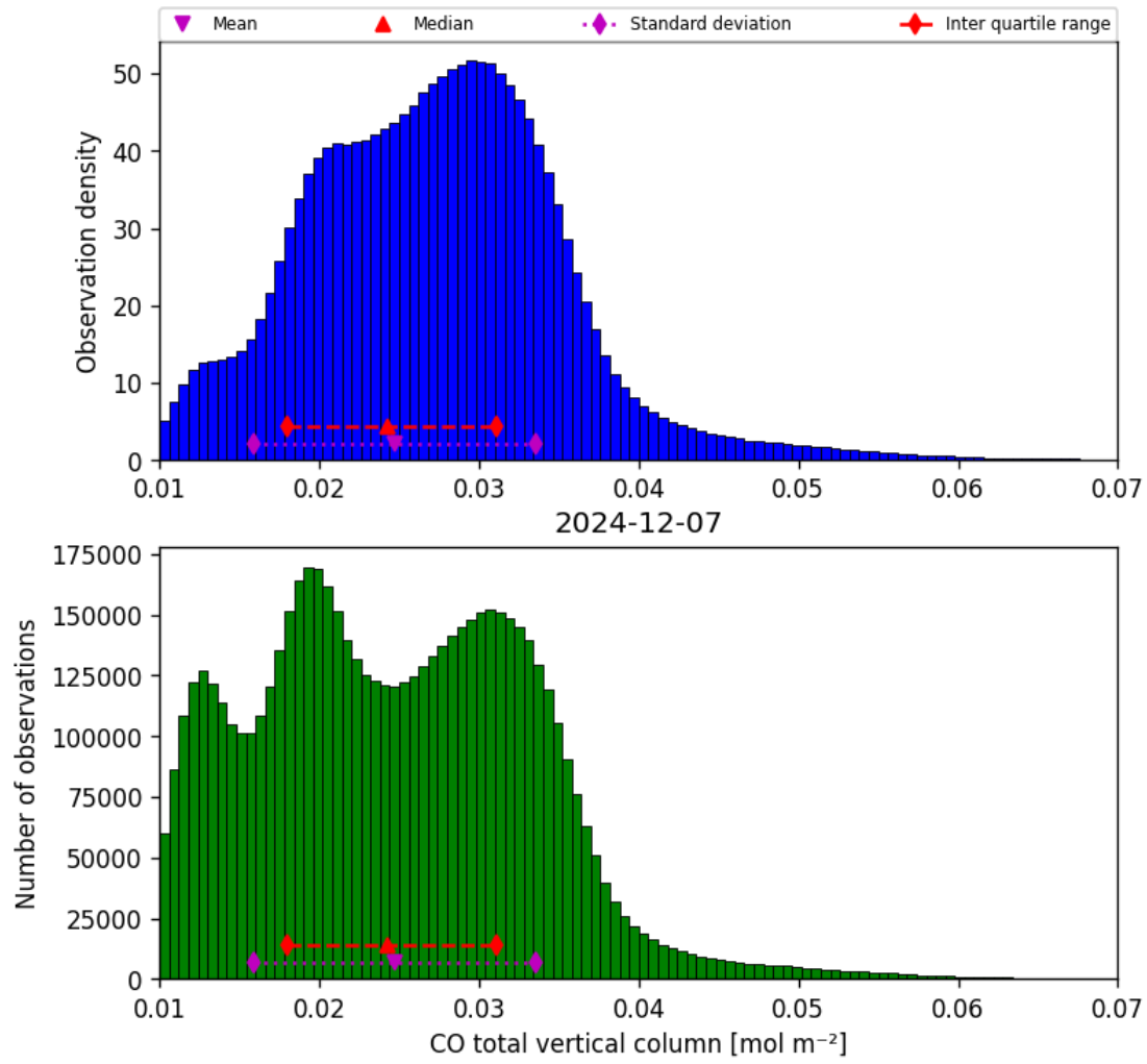
Figure 14: Histogram of “CO total vertical column” for 2024-12-07 to 2024-12-08
