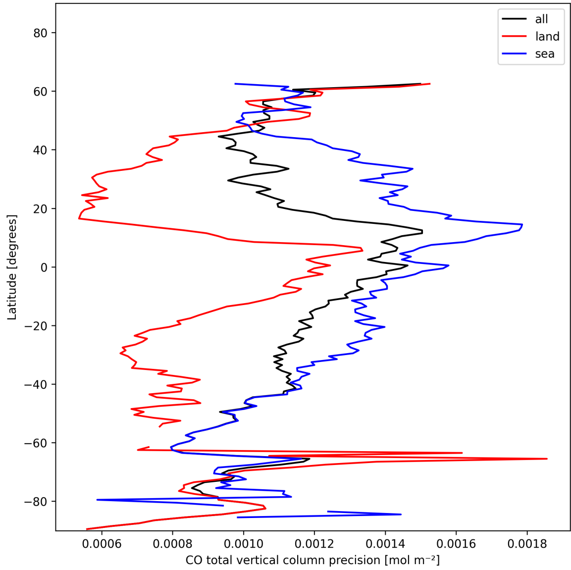
Figure 8: Zonal average of “CO total vertical column precision” for 2024-12-07 to 2024-12-08.
