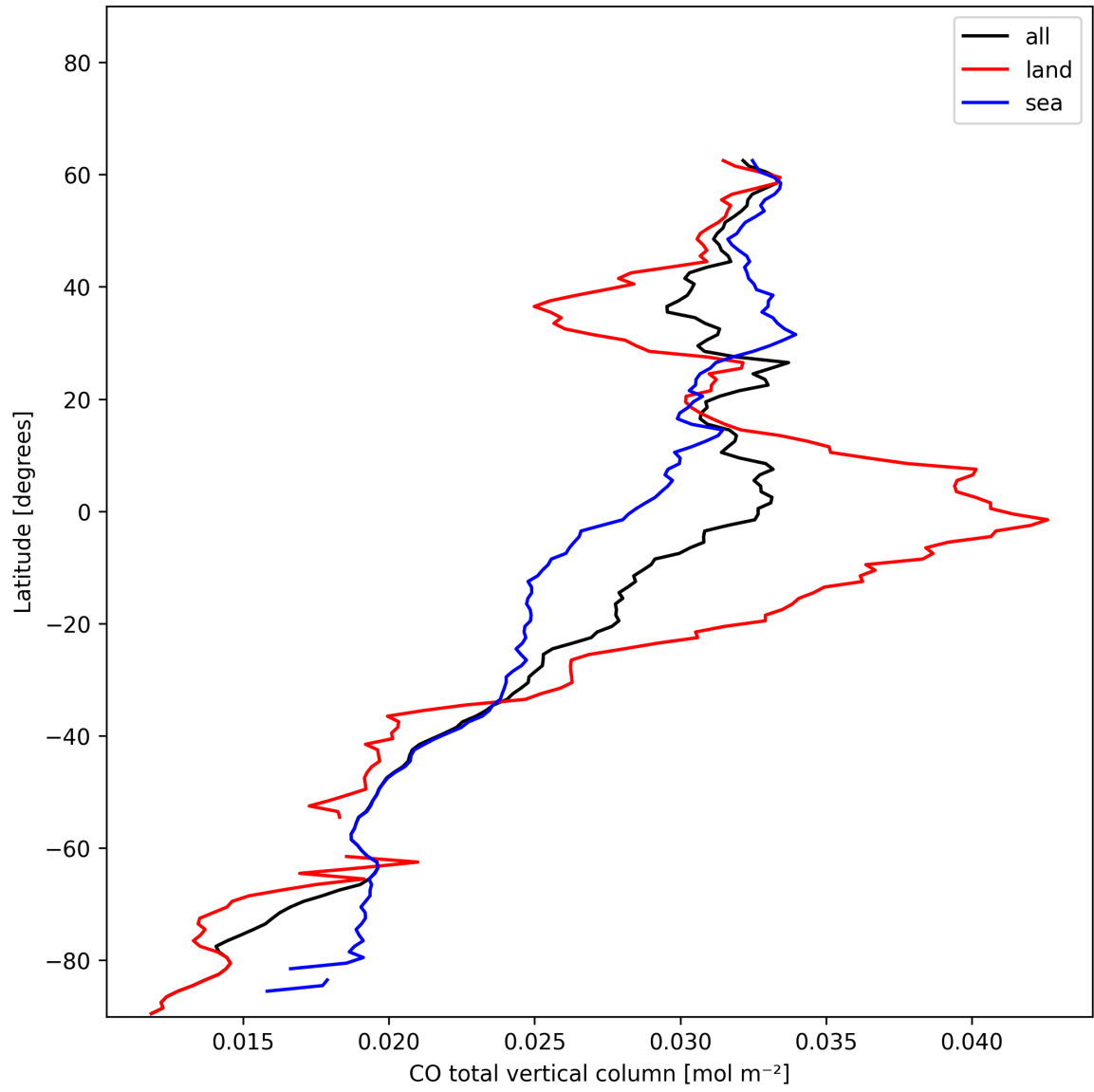
Figure 7: Zonal average of “CO total vertical column” for 2024-12-07 to 2024-12-08.
