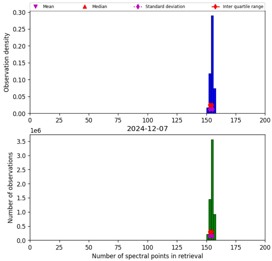
Figure 16: Histogram of “Number of spectral points in retrieval” for 2024-12-07 to 2024-12-08
