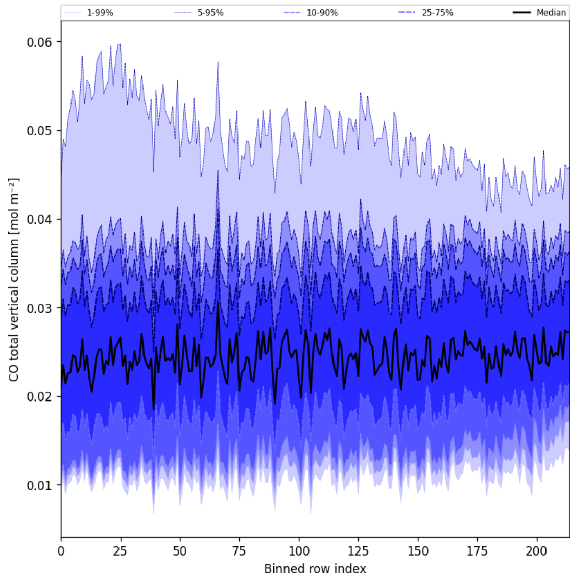
Figure 21: Along track statistics of “CO total vertical column” for 2024-12-07 to 2024-12-08
