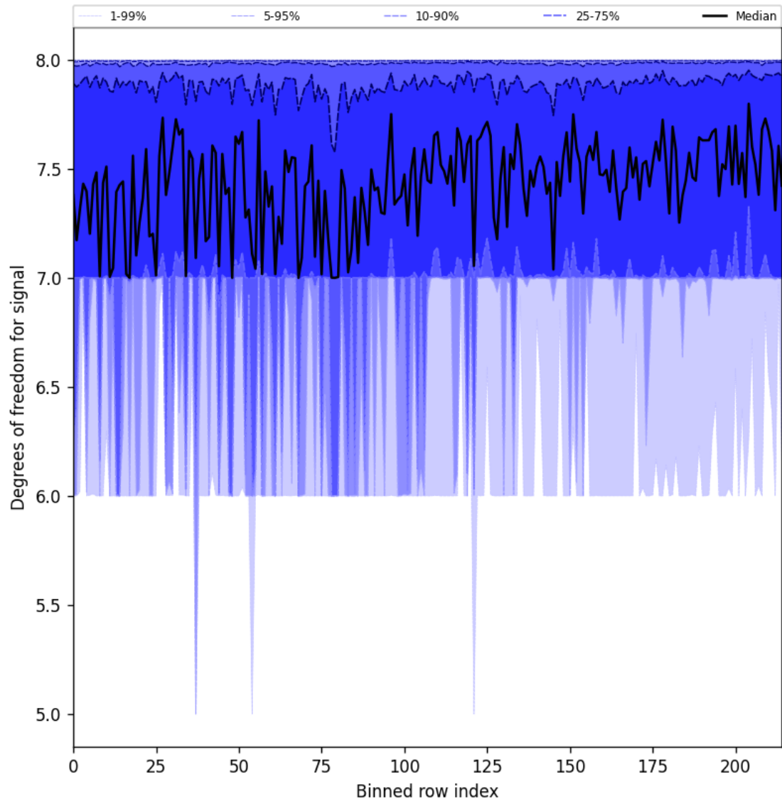
Figure 25: Along track statistics of “Degrees of freedom for signal” for 2024-12-07 to 2024-12-08
