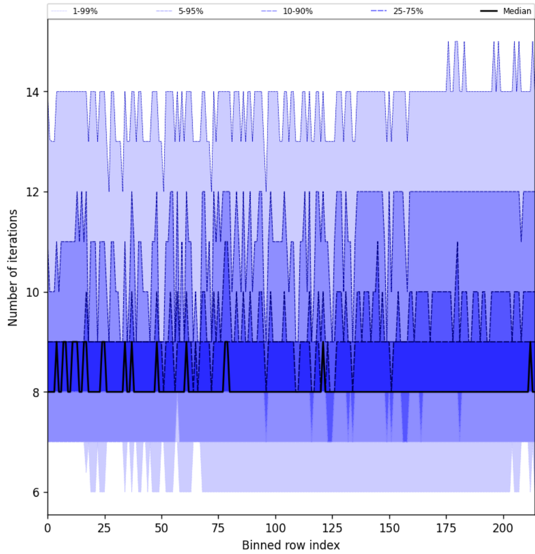
Figure 26: Along track statistics of “Number of iterations” for 2024-12-07 to 2024-12-08
