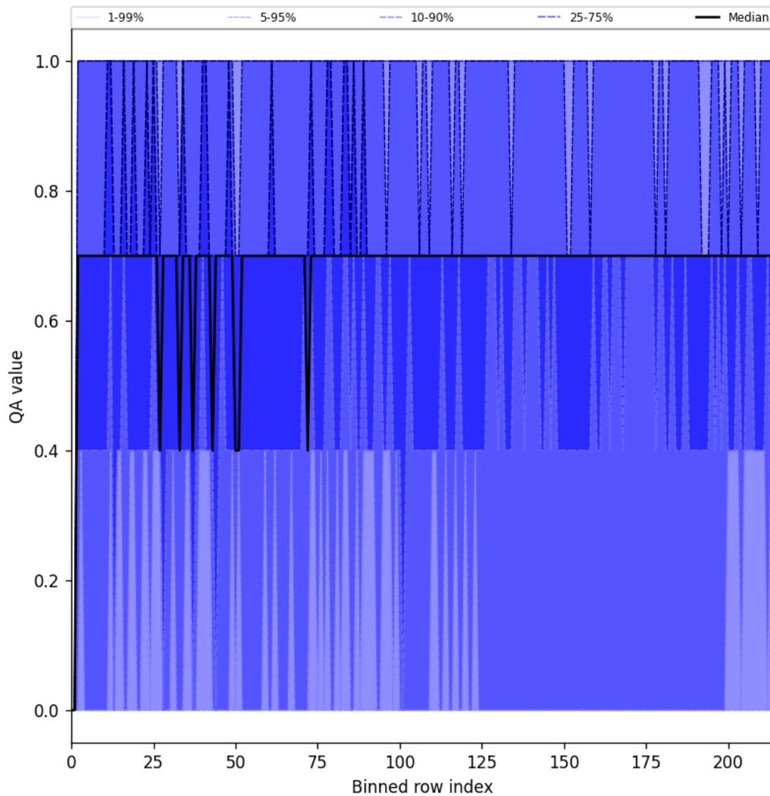
Figure 20: Along track statistics of “QA value” for 2024-12-07 to 2024-12-08
