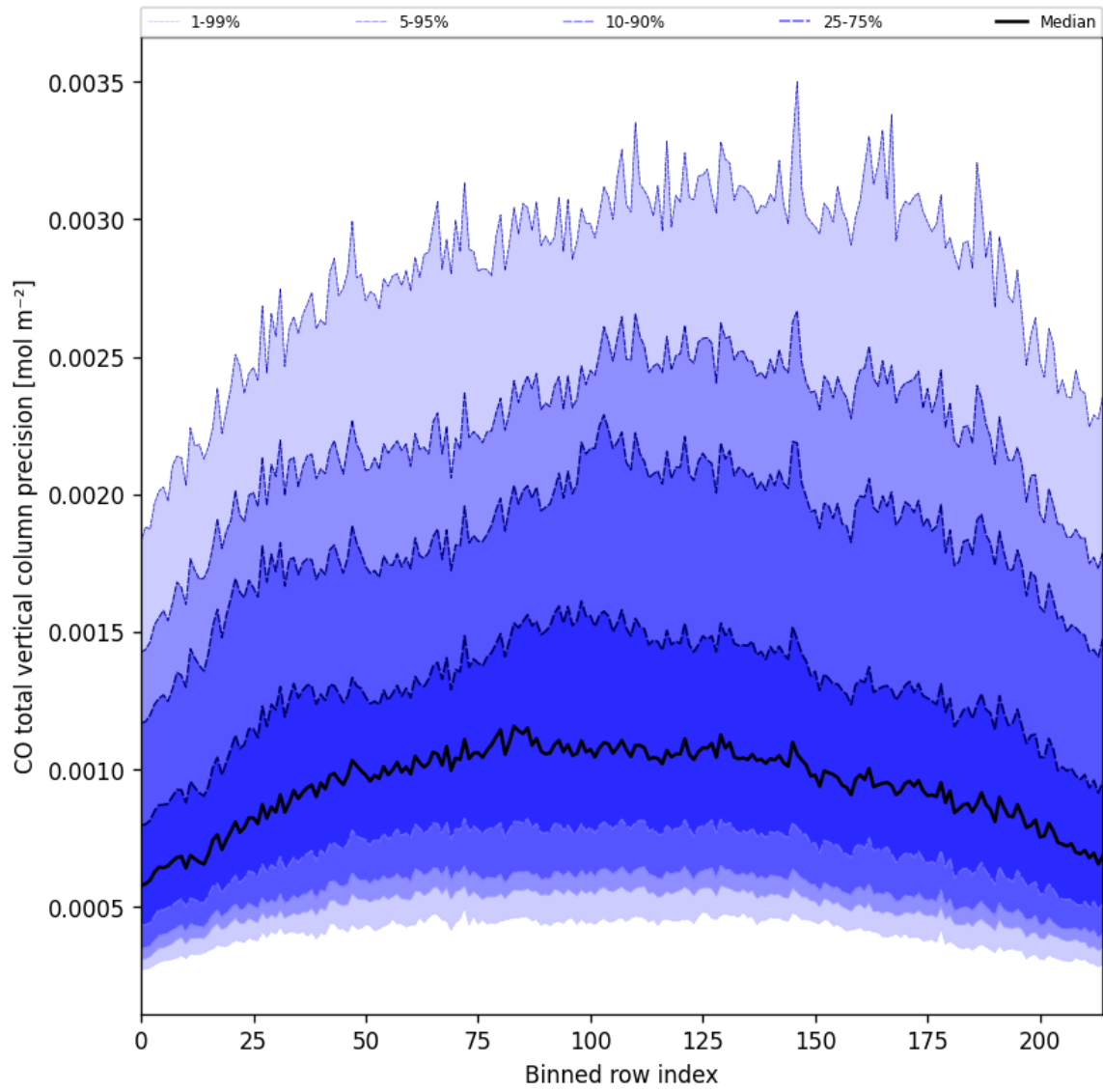
Figure 22: Along track statistics of “CO total vertical column precision” for 2024-12-07 to 2024-12-08
