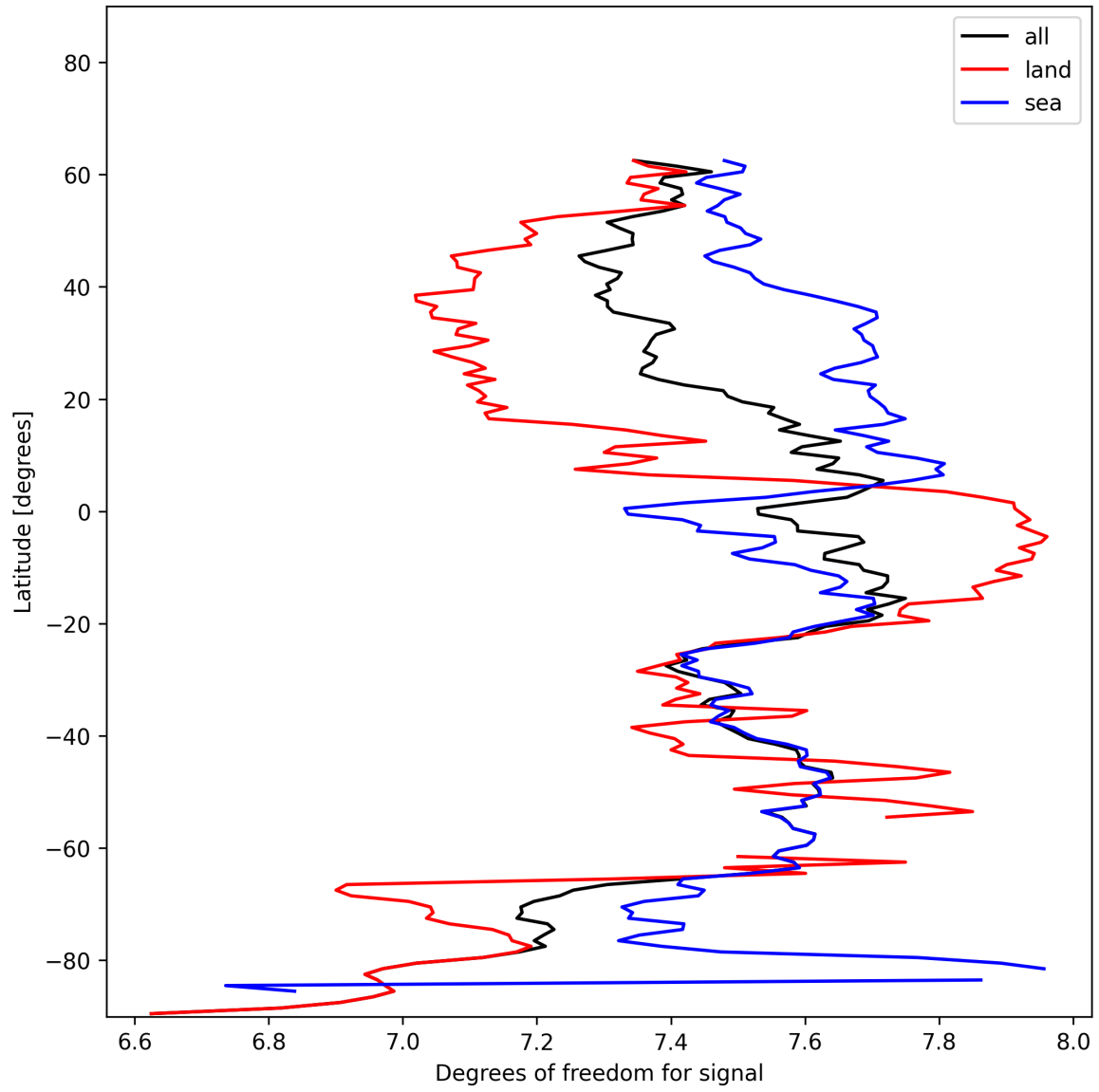
Figure 11: Zonal average of “Degrees of freedom for signal” for 2024-12-07 to 2024-12-08.
