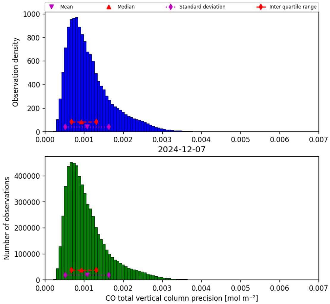
Figure 15: Histogram of “CO total vertical column precision” for 2024-12-07 to 2024-12-08
