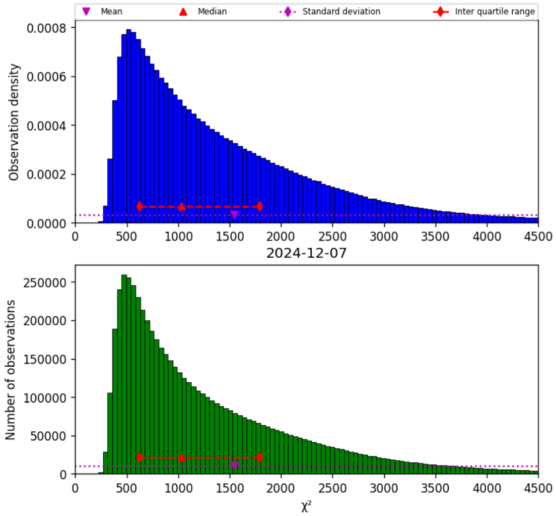
Figure 17: Histogram of “ \chi^2 ” for 2024-12-07 to 2024-12-08
