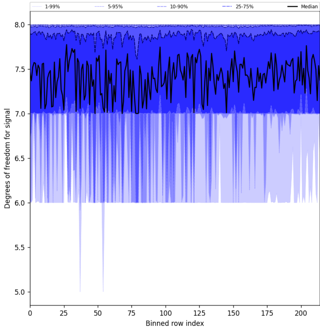
Figure 25: Along track statistics of “Degrees of freedom for signal” for 2024-12-08 to 2024-12-09
