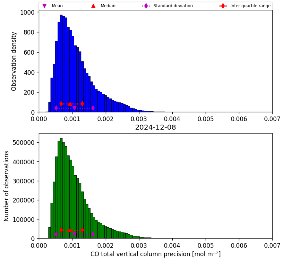
Figure 15: Histogram of “CO total vertical column precision” for 2024-12-08 to 2024-12-09
