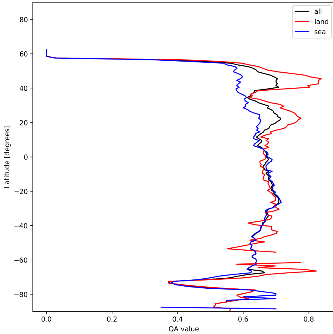
Figure 6: Zonal average of “QA value” for 2024-12-08 to 2024-12-09.
