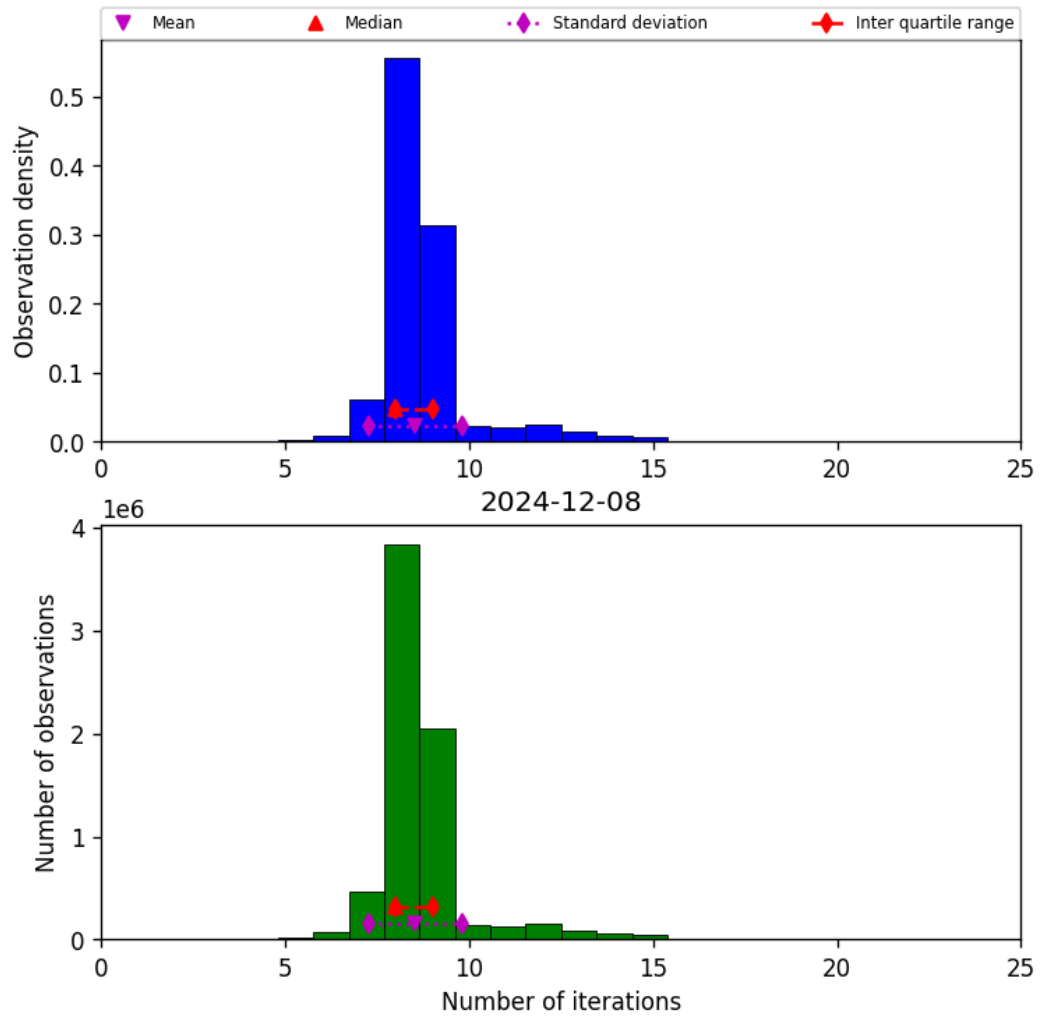
Figure 19: Histogram of “Number of iterations” for 2024-12-08 to 2024-12-09
