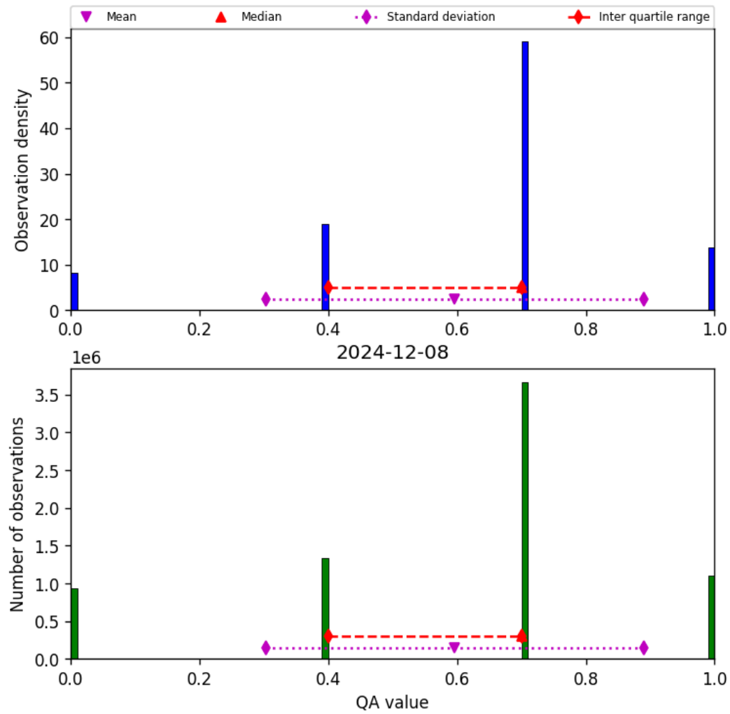
Figure 13: Histogram of “QA value” for 2024-12-08 to 2024-12-09
