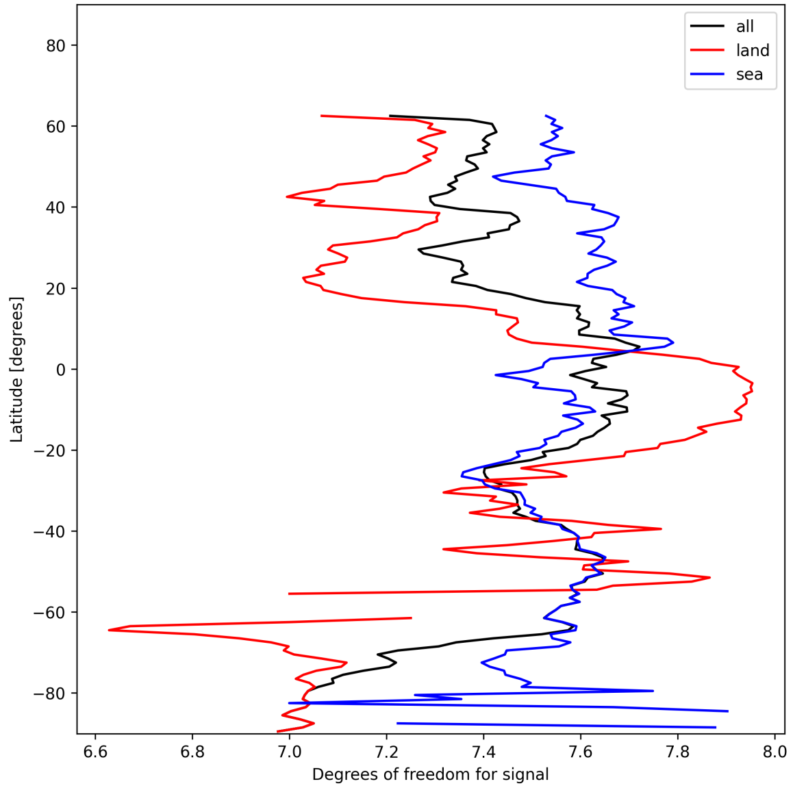
Figure 11: Zonal average of “Degrees of freedom for signal” for 2024-12-08 to 2024-12-09.
