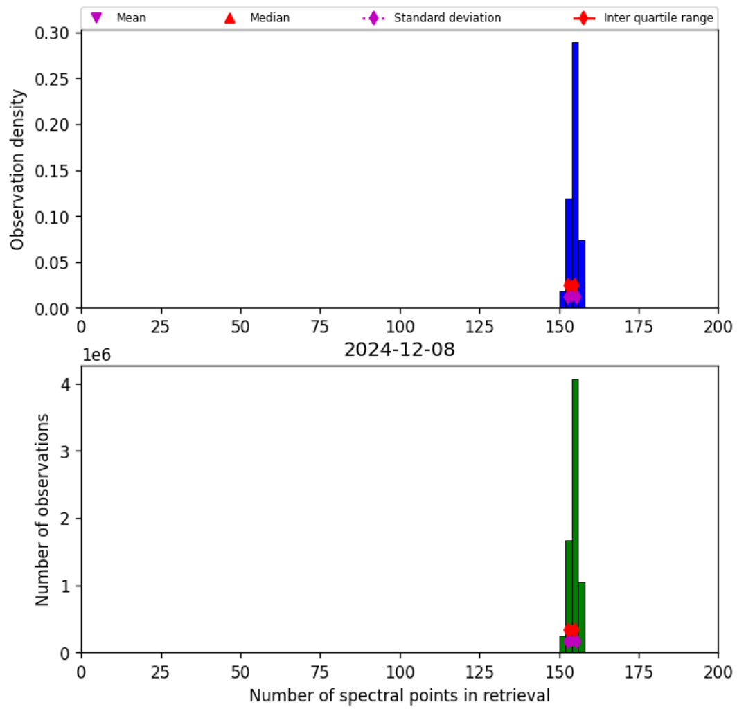
Figure 16: Histogram of “Number of spectral points in retrieval” for 2024-12-08 to 2024-12-09
