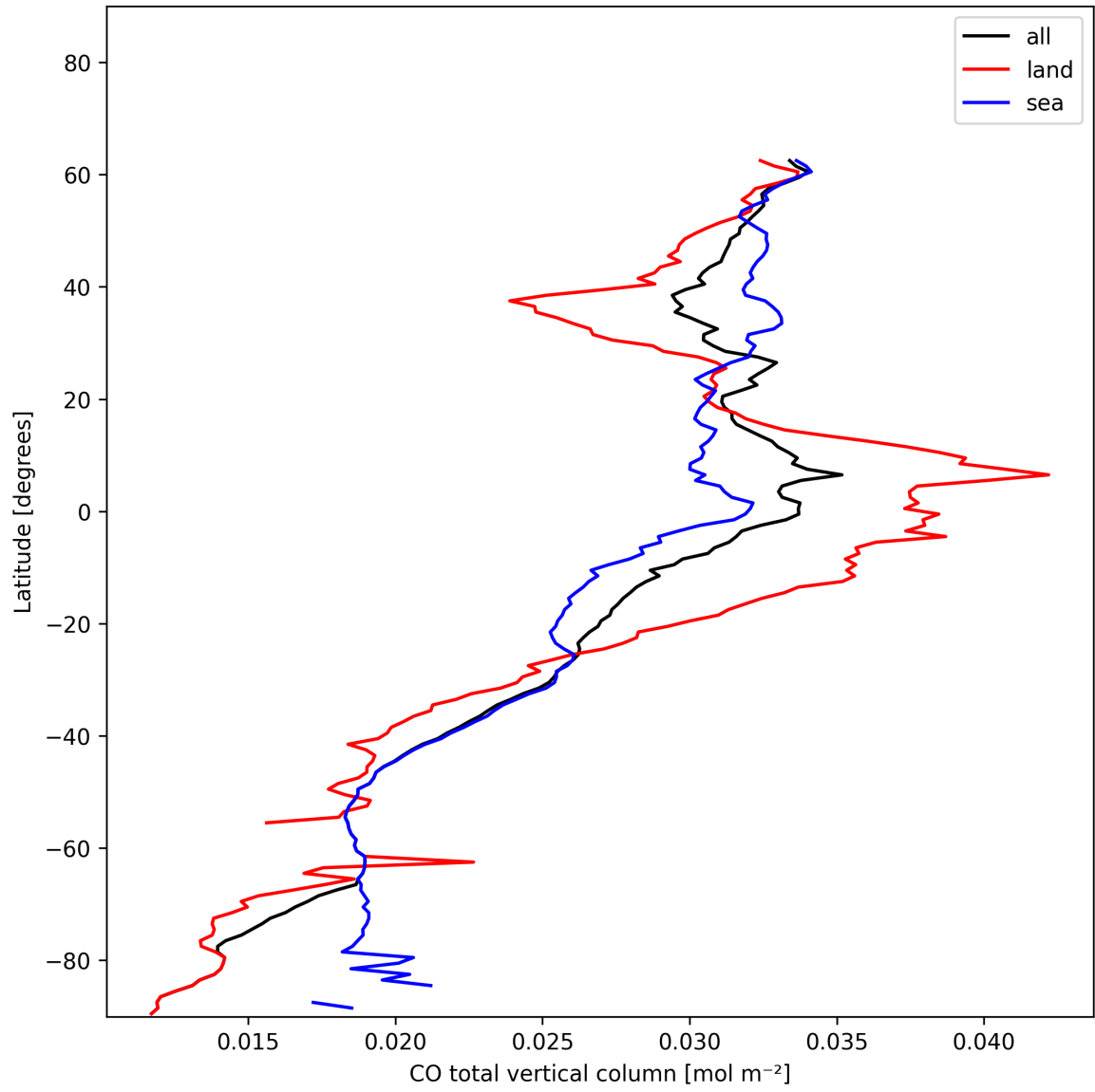
Figure 7: Zonal average of “CO total vertical column” for 2024-12-08 to 2024-12-09.
