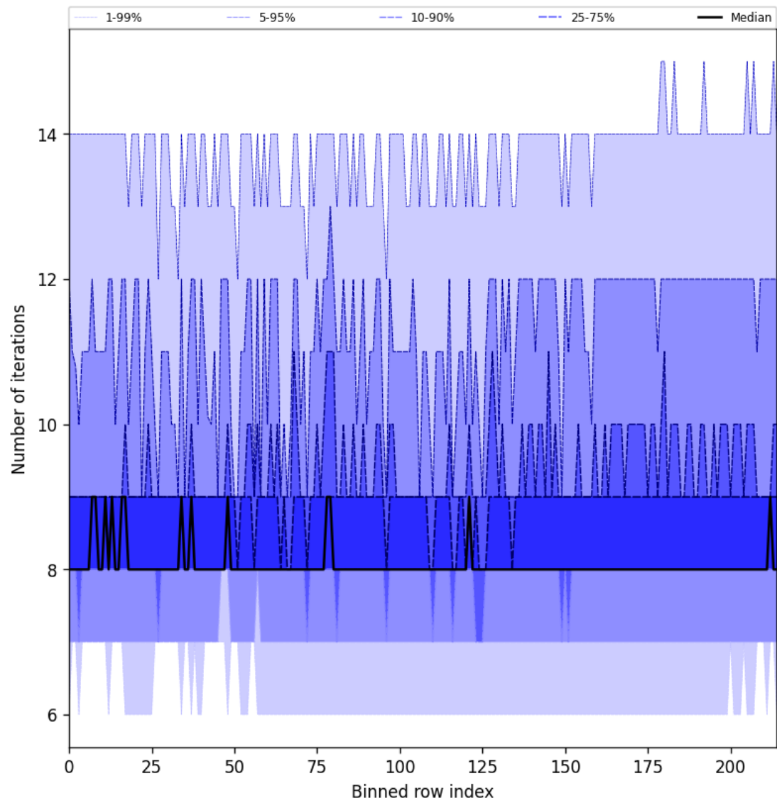
Figure 26: Along track statistics of “Number of iterations” for 2024-12-08 to 2024-12-09
