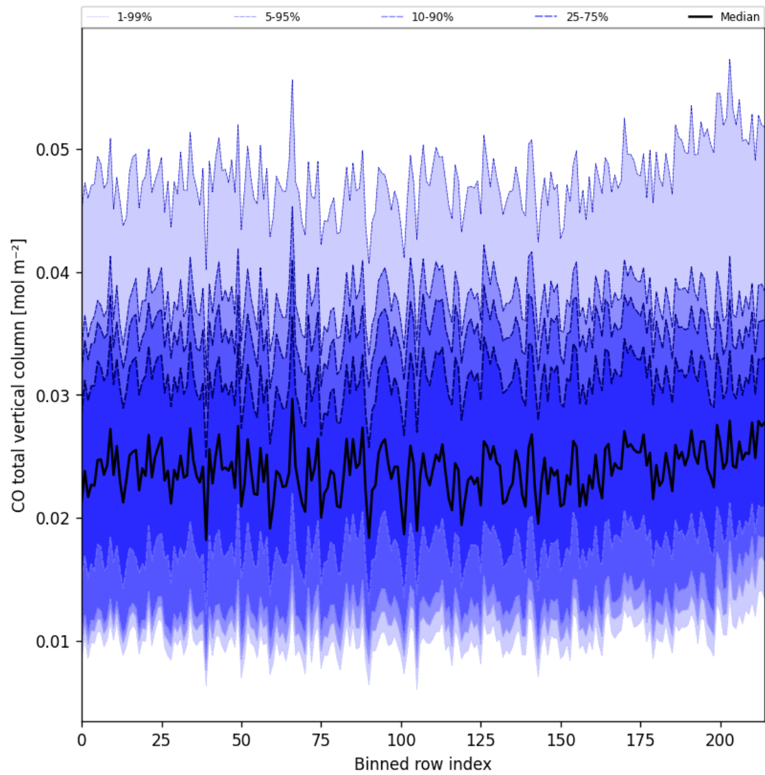
Figure 21: Along track statistics of “CO total vertical column” for 2024-12-08 to 2024-12-09
