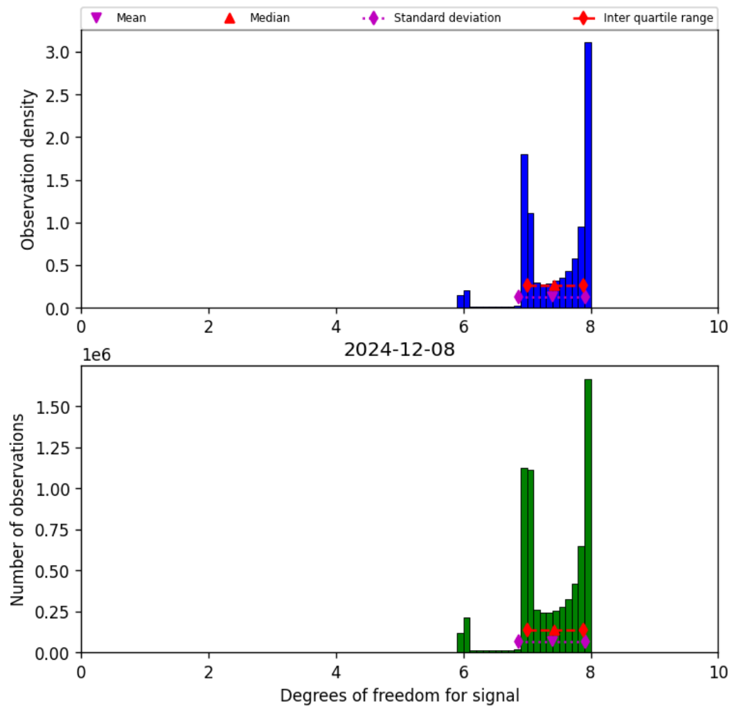
Figure 18: Histogram of “Degrees of freedom for signal” for 2024-12-08 to 2024-12-09
