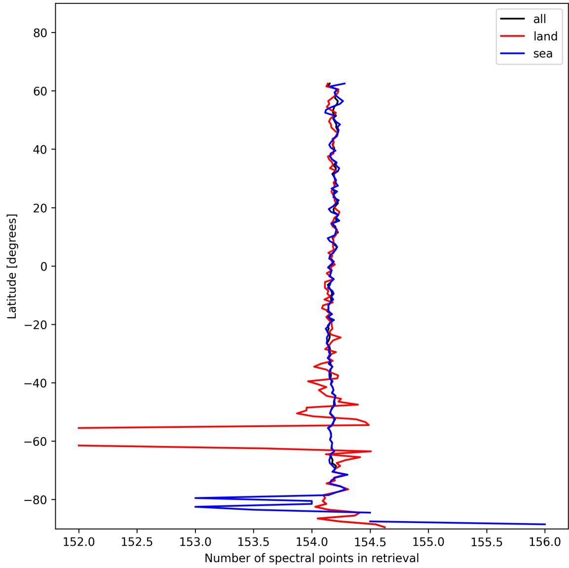
Figure 9: Zonal average of “Number of spectral points in retrieval” for 2024-12-08 to 2024-12-09.
