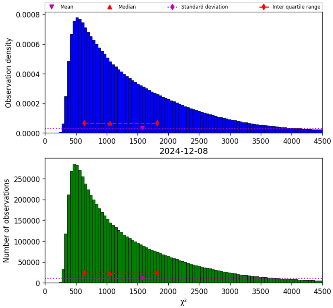
Figure 17: Histogram of " \chi^2 " for 2024-12-08 to 2024-12-09
