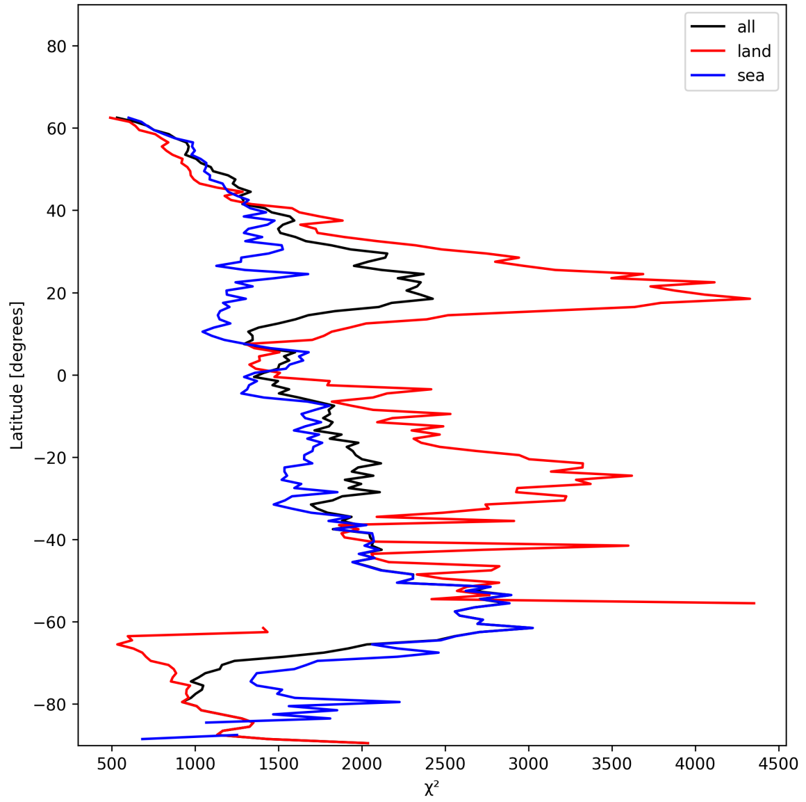
Figure 10: Zonal average of “ \chi^2 ” for 2024-12-08 to 2024-12-09.
