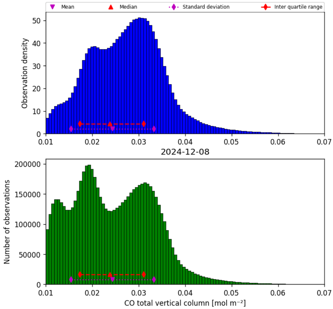
Figure 14: Histogram of “CO total vertical column” for 2024-12-08 to 2024-12-09
