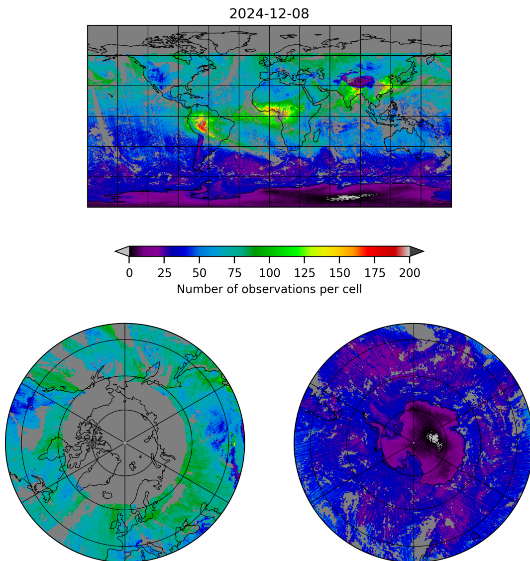
Figure 5: Map of the number of observations for 2024-12-08 to 2024-12-09
