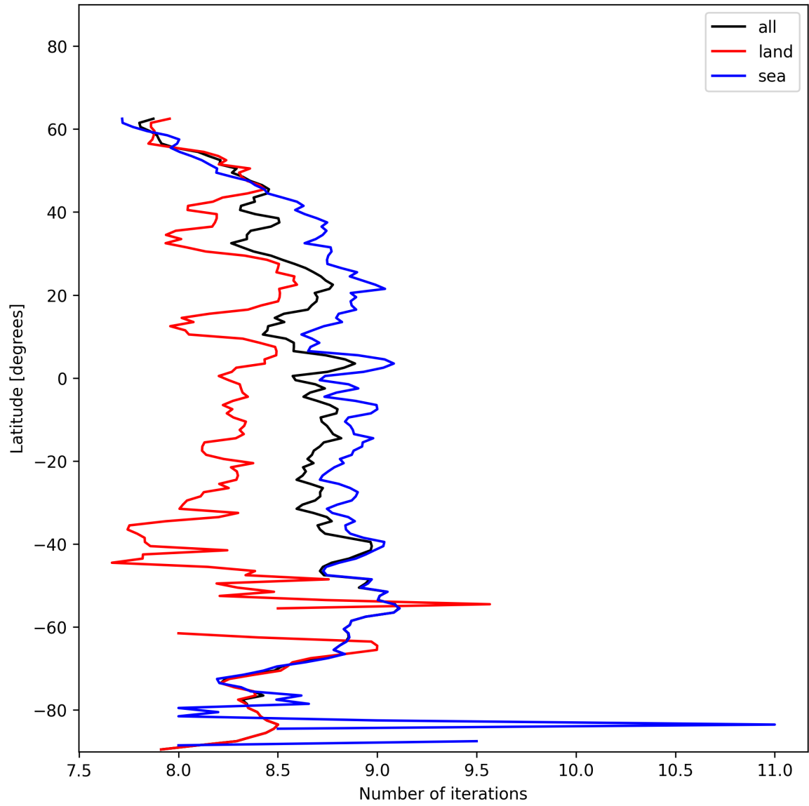
Figure 12: Zonal average of “Number of iterations” for 2024-12-08 to 2024-12-09.
