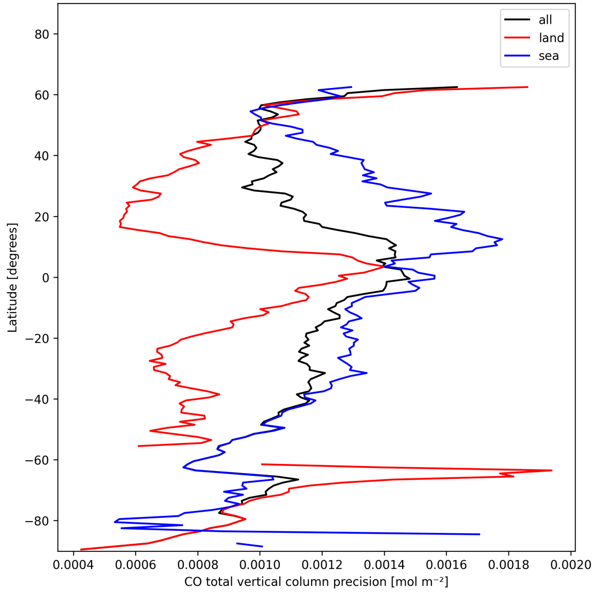
Figure 8: Zonal average of “CO total vertical column precision” for 2024-12-08 to 2024-12-09.
