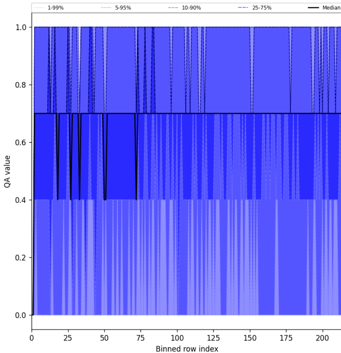
Figure 20: Along track statistics of “QA value” for 2024-12-08 to 2024-12-09
