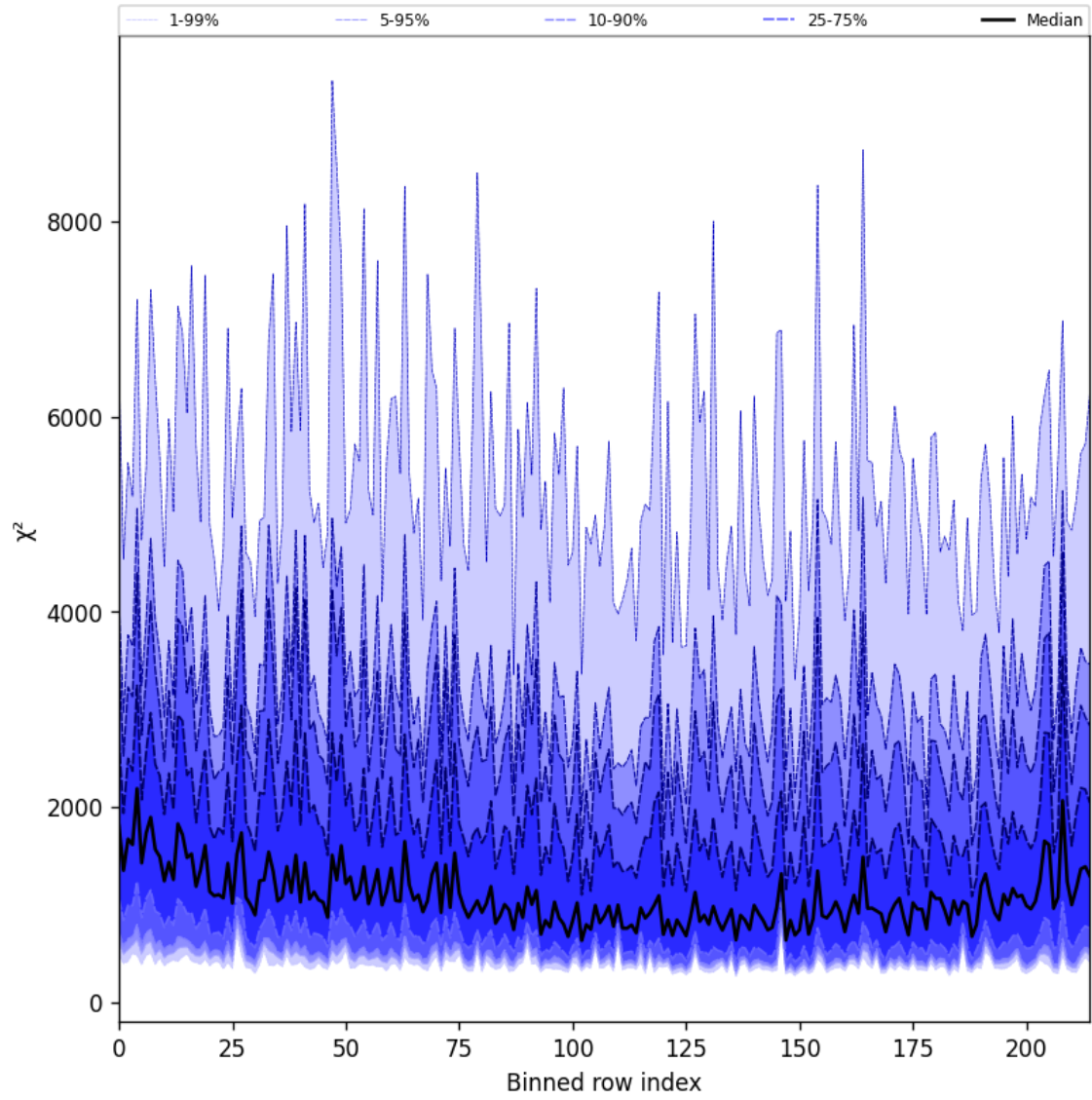
Figure 24: Along track statistics of “ \chi^2 ” for 2024-12-08 to 2024-12-09
