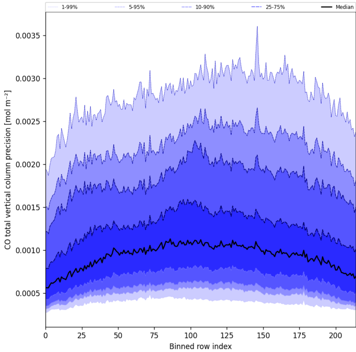
Figure 22: Along track statistics of “CO total vertical column precision” for 2024-12-08 to 2024-12-09
