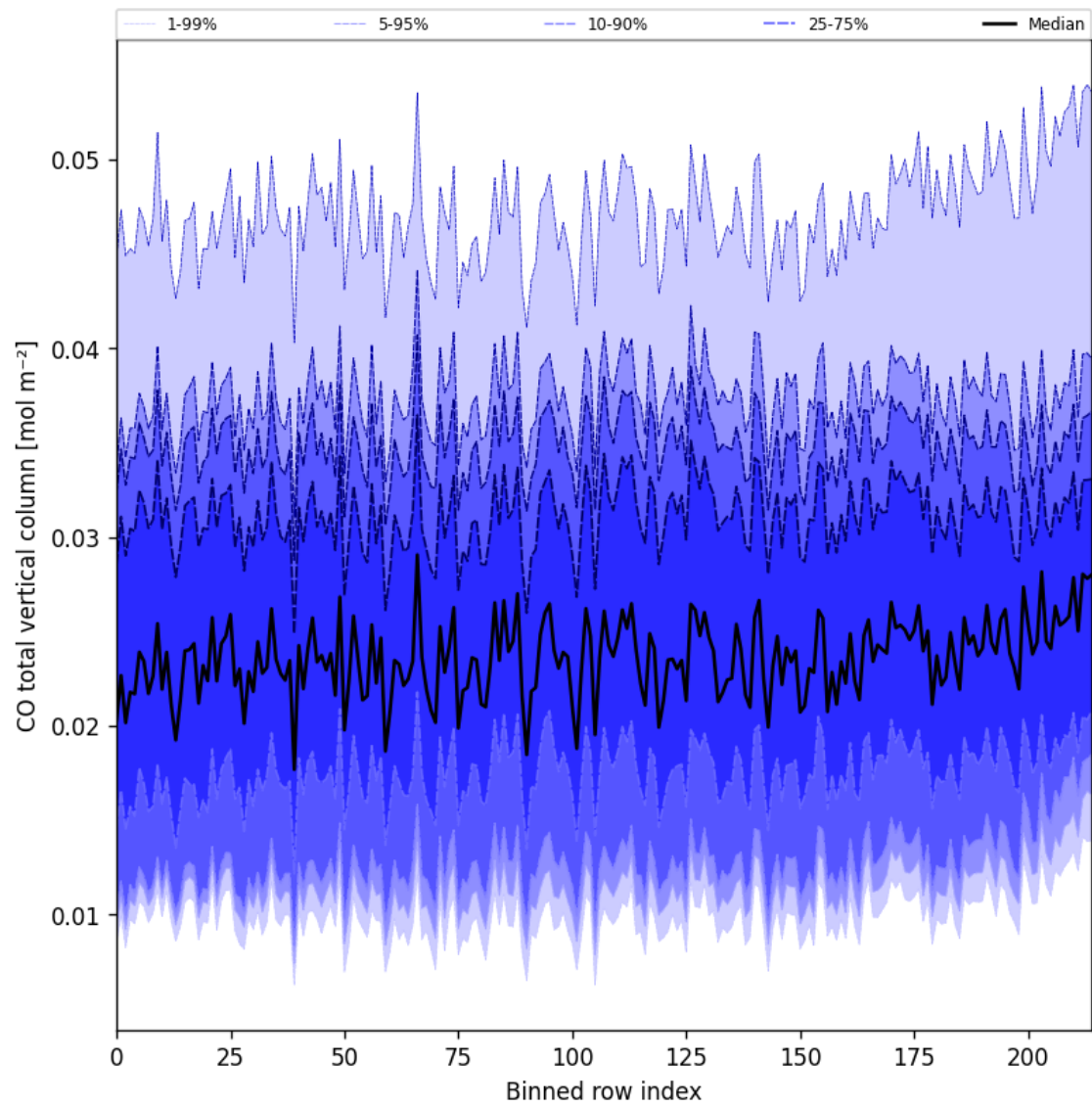
Figure 21: Along track statistics of “CO total vertical column” for 2024-12-10 to 2024-12-11
