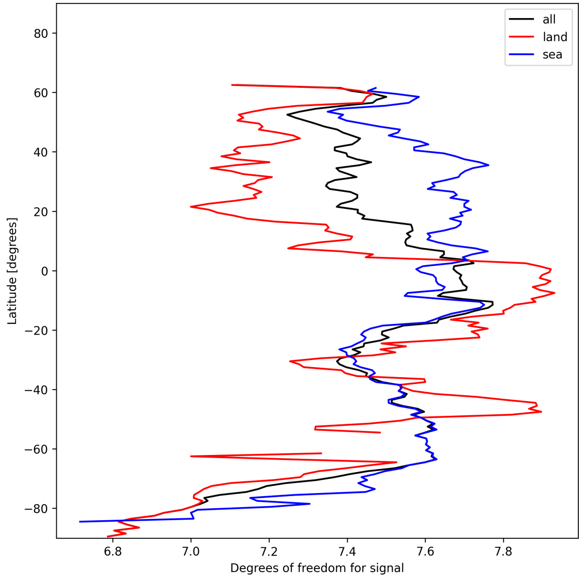
Figure 11: Zonal average of “Degrees of freedom for signal” for 2024-12-10 to 2024-12-11.
