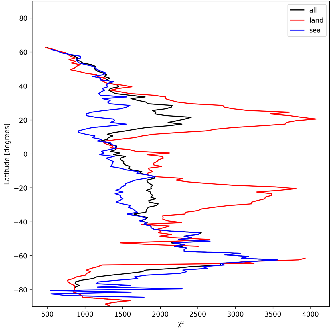
Figure 10: Zonal average of “ \chi^2 ” for 2024-12-10 to 2024-12-11.
