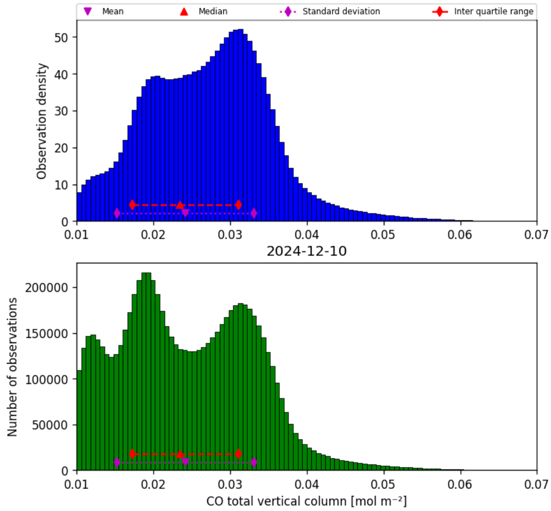
Figure 14: Histogram of “CO total vertical column” for 2024-12-10 to 2024-12-11
