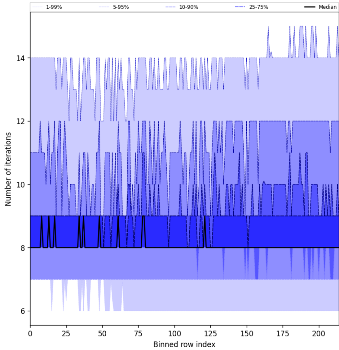
Figure 26: Along track statistics of “Number of iterations” for 2024-12-10 to 2024-12-11
