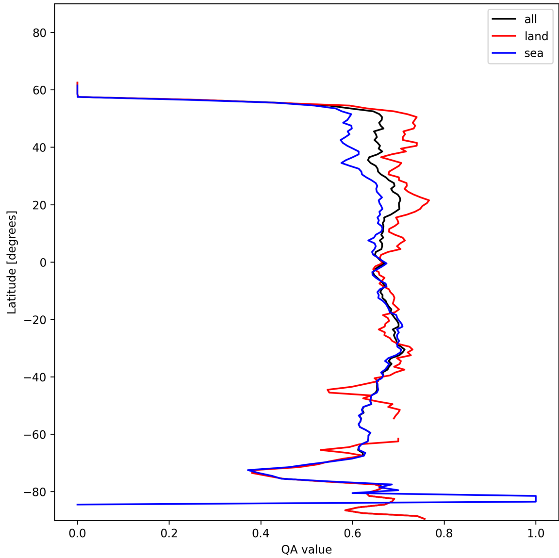
Figure 6: Zonal average of “QA value” for 2024-12-10 to 2024-12-11.
