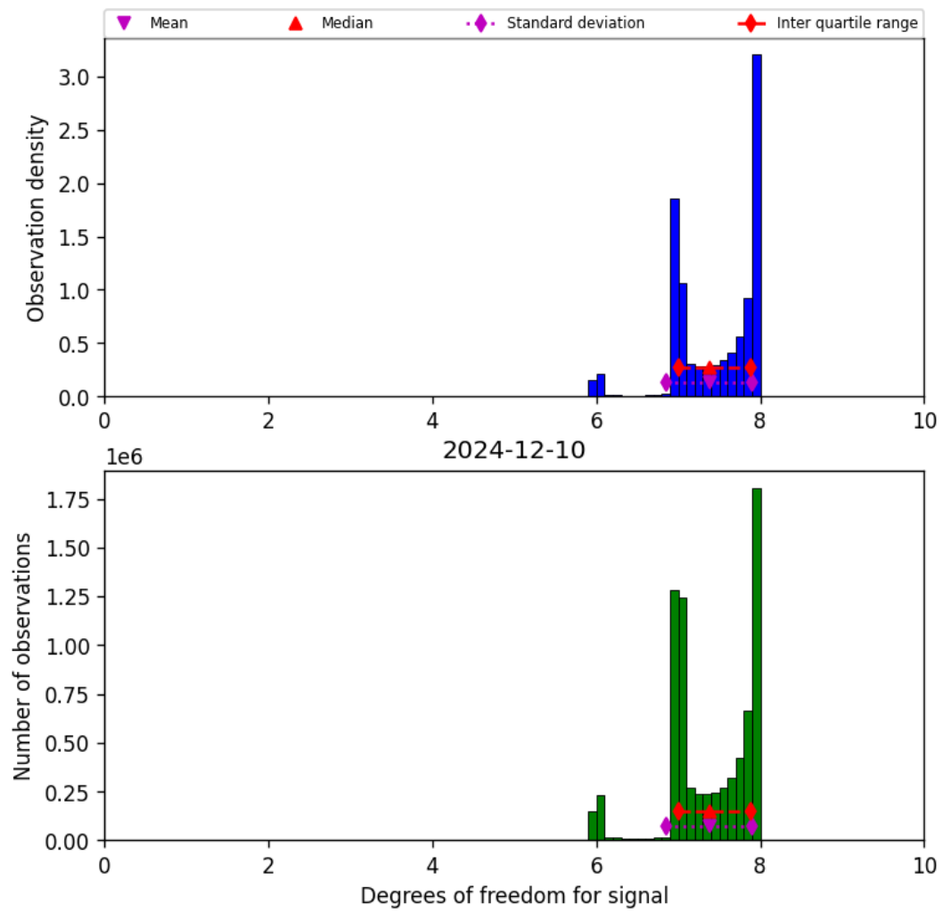
Figure 18: Histogram of “Degrees of freedom for signal” for 2024-12-10 to 2024-12-11
