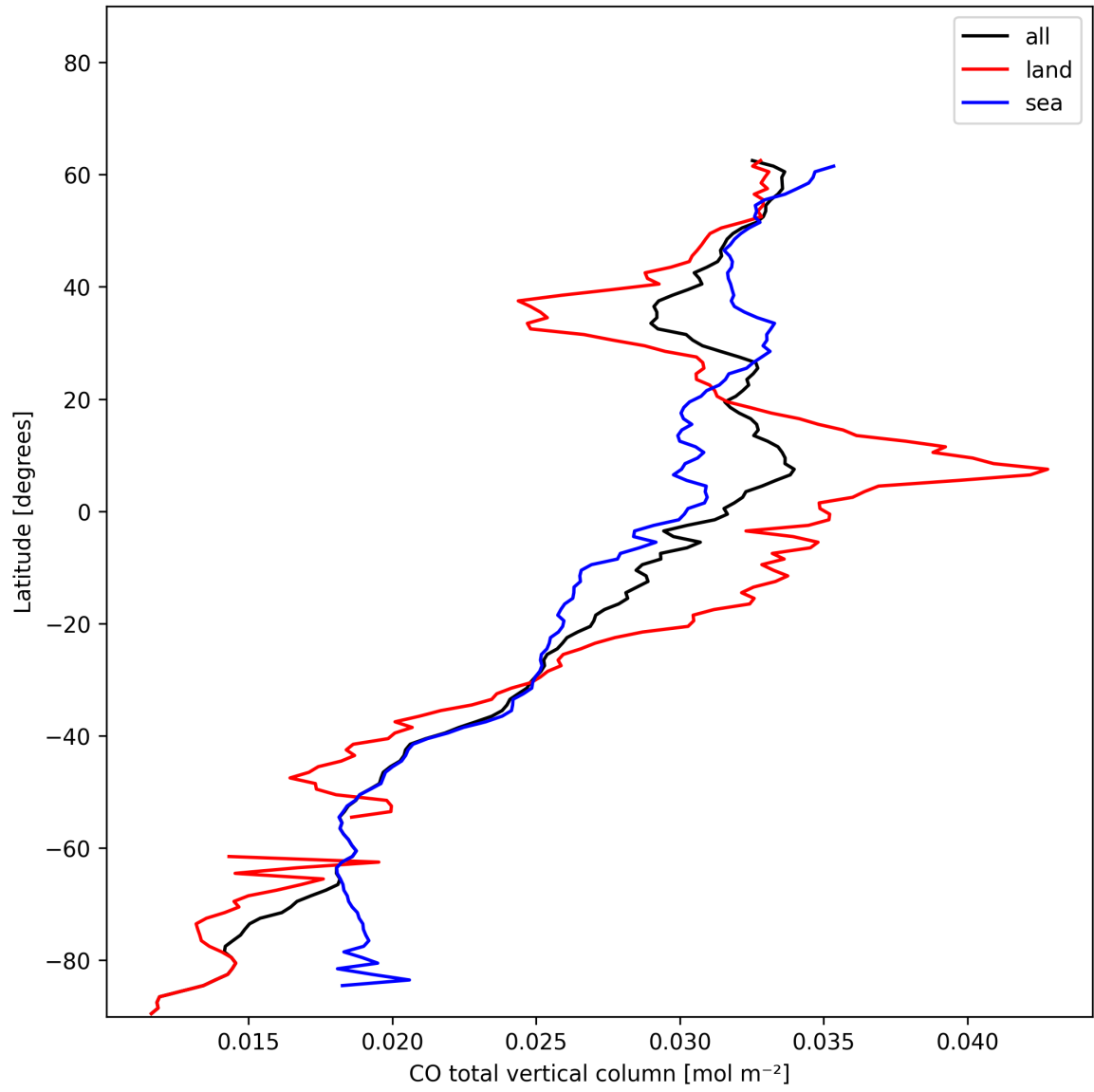
Figure 7: Zonal average of “CO total vertical column” for 2024-12-10 to 2024-12-11.
