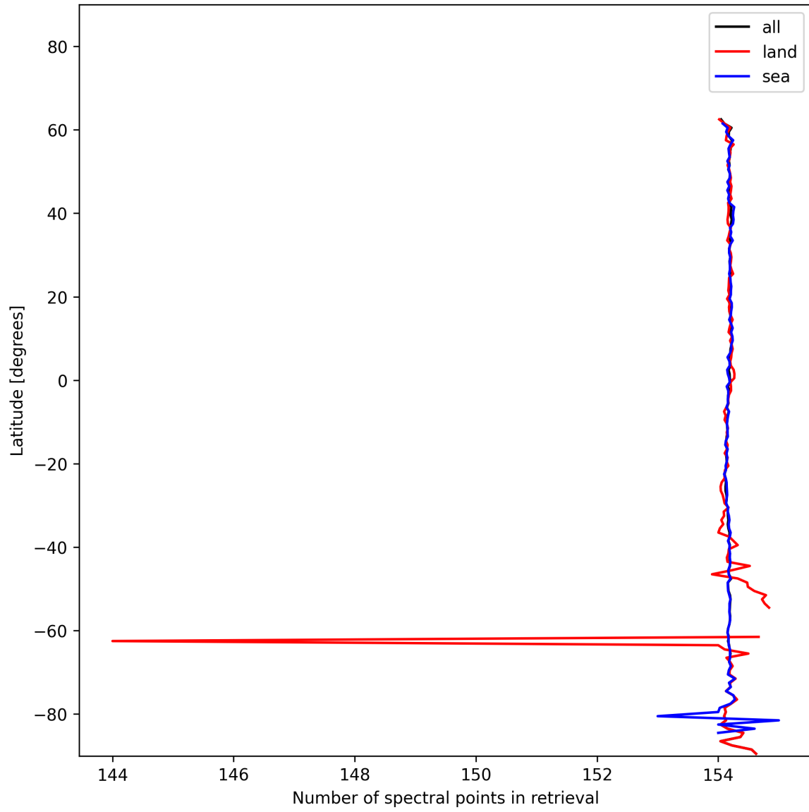
Figure 9: Zonal average of “Number of spectral points in retrieval” for 2024-12-10 to 2024-12-11.
