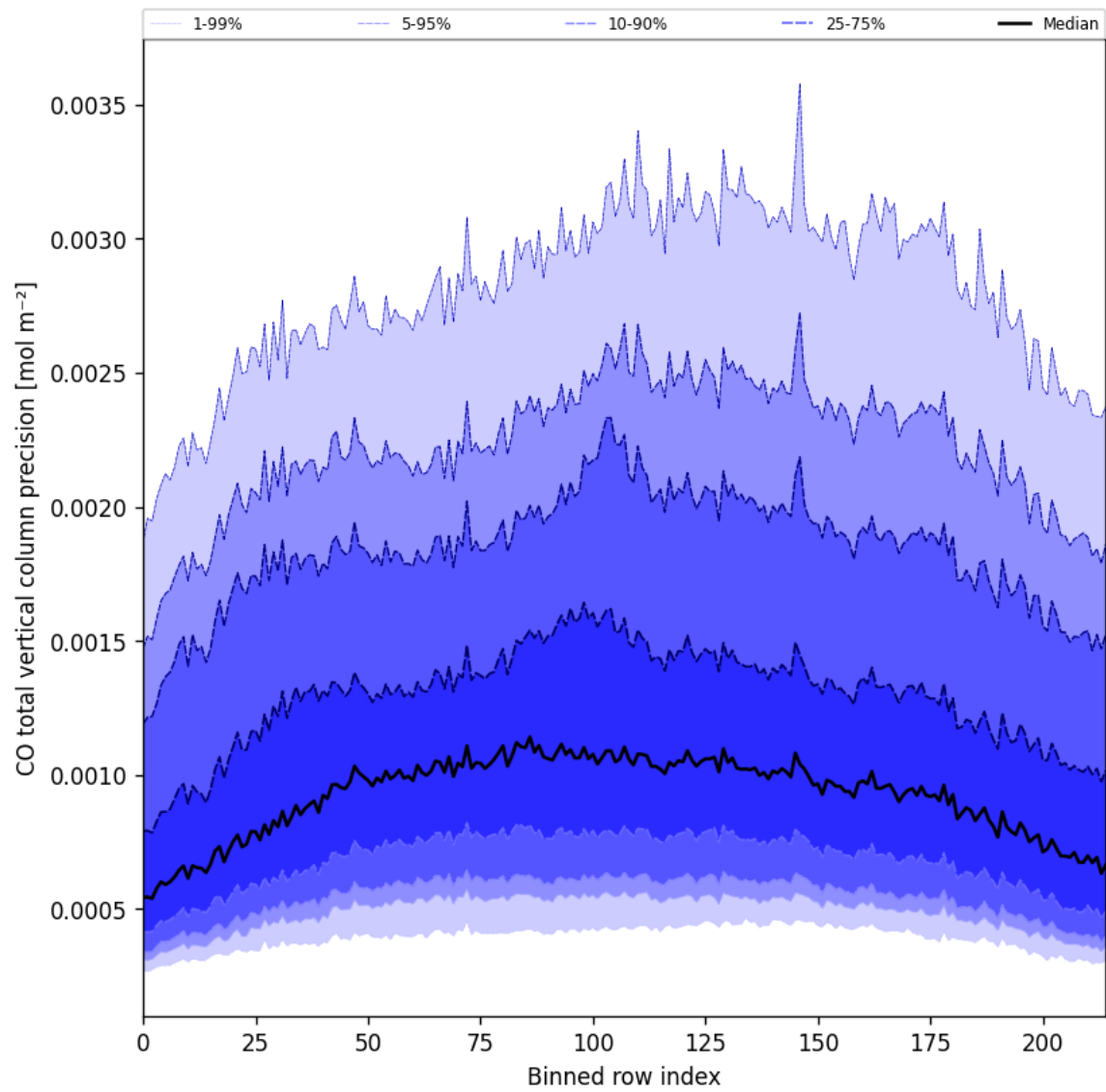
Figure 22: Along track statistics of “CO total vertical column precision” for 2024-12-10 to 2024-12-11
