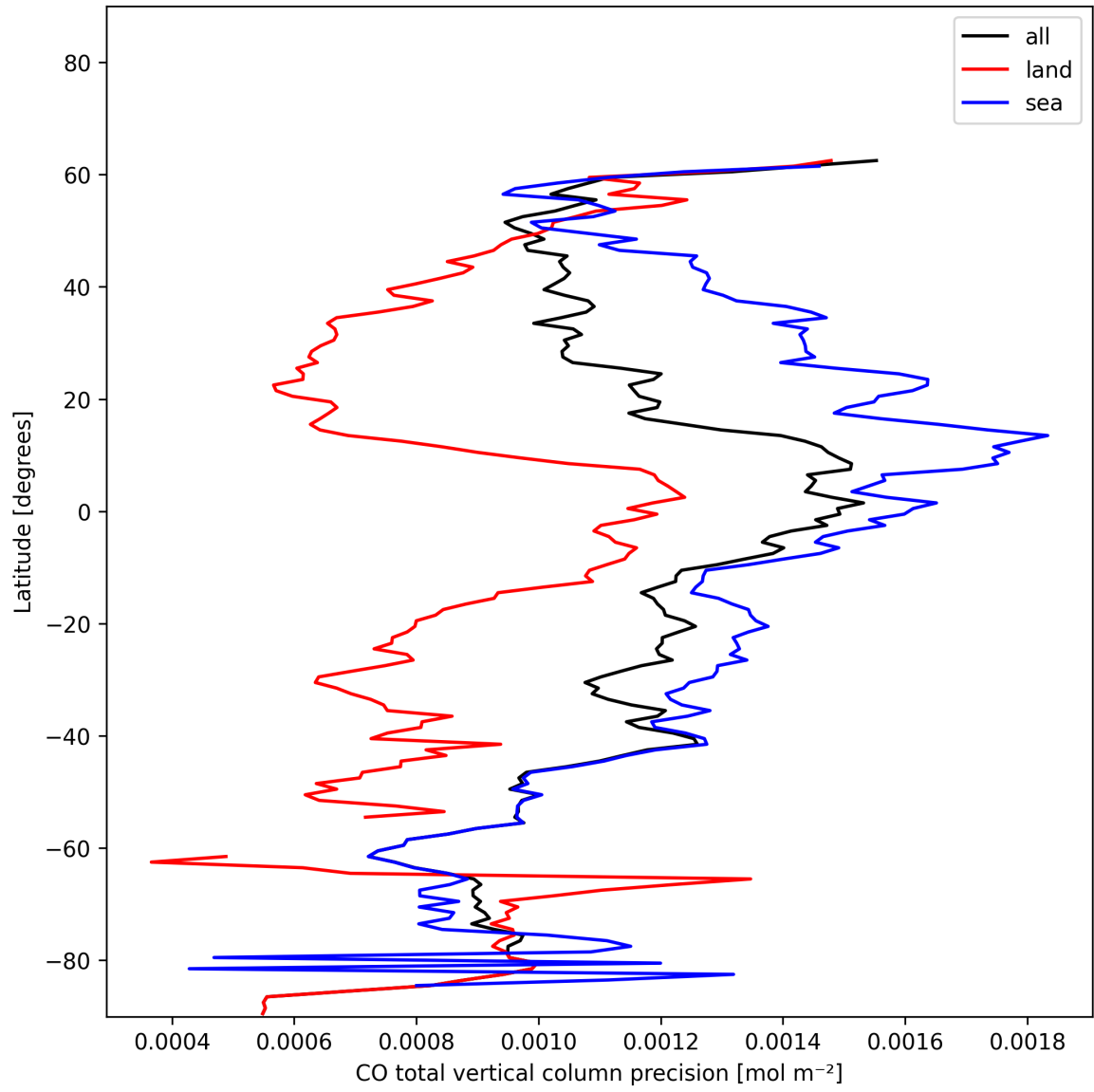
Figure 8: Zonal average of “CO total vertical column precision” for 2024-12-10 to 2024-12-11.
