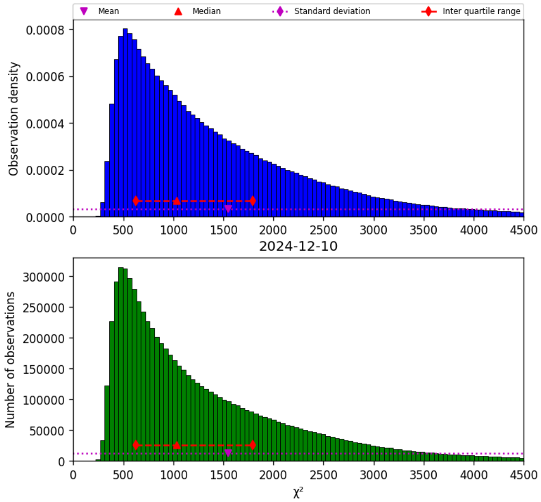
Figure 17: Histogram of " \chi^2 " for 2024-12-10 to 2024-12-11
