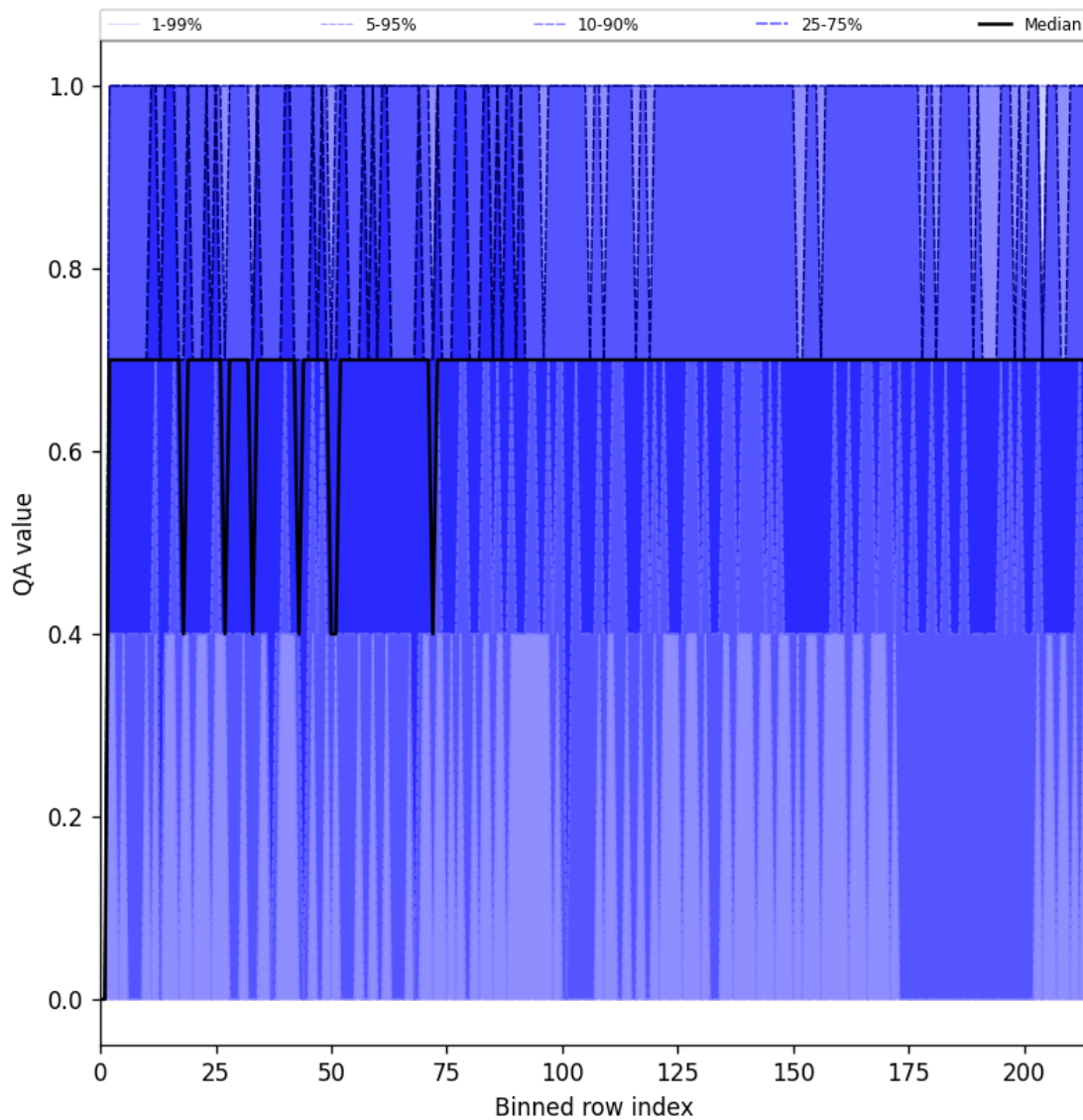
Figure 20: Along track statistics of “QA value” for 2024-12-10 to 2024-12-11
