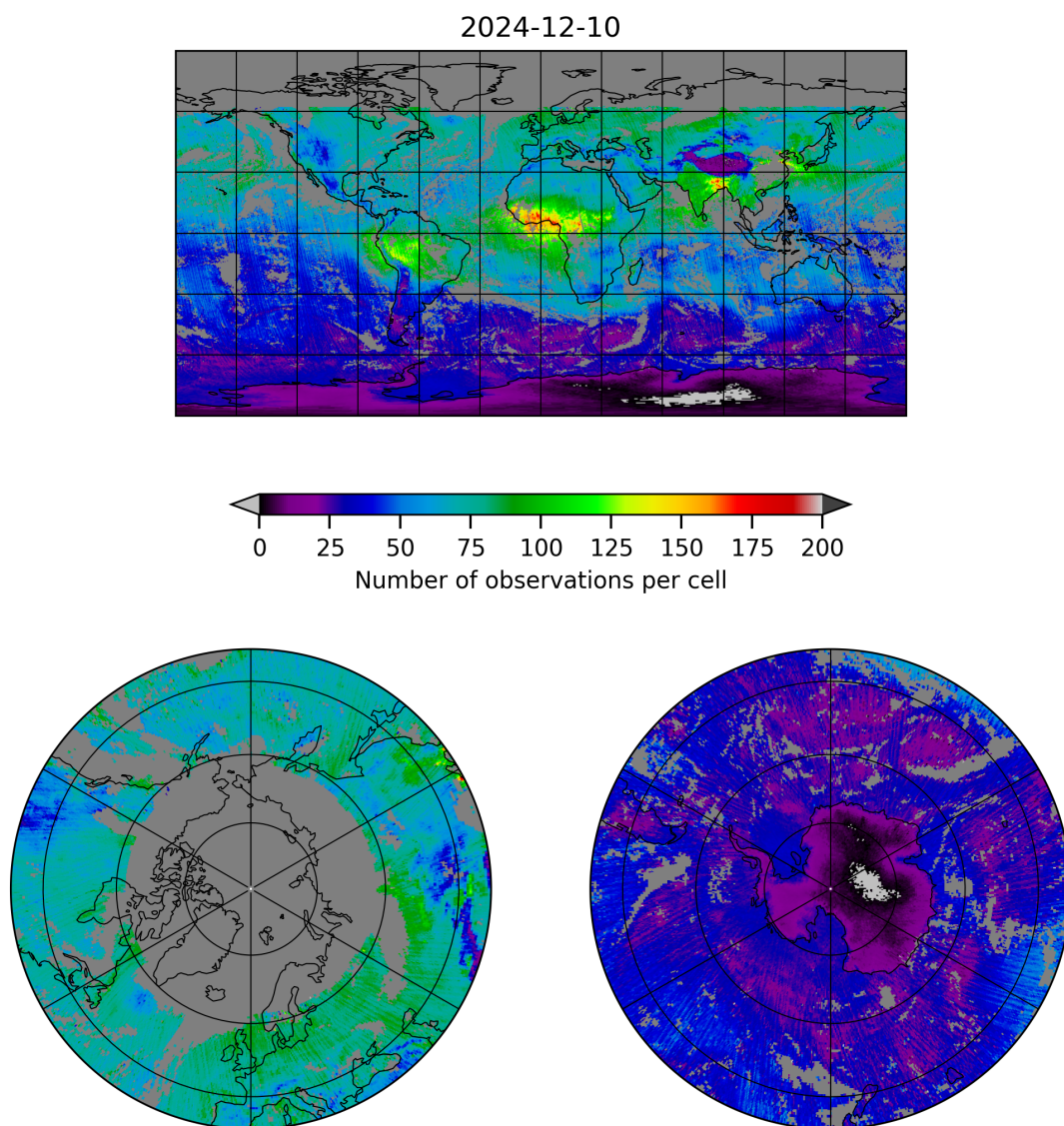
Figure 5: Map of the number of observations for 2024-12-10 to 2024-12-11
