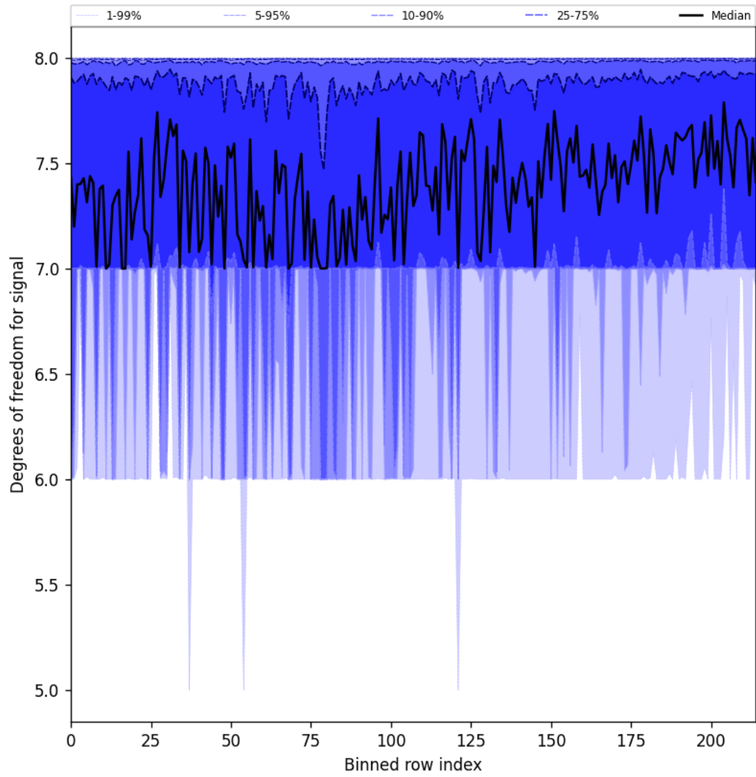
Figure 25: Along track statistics of “Degrees of freedom for signal” for 2024-12-10 to 2024-12-11
