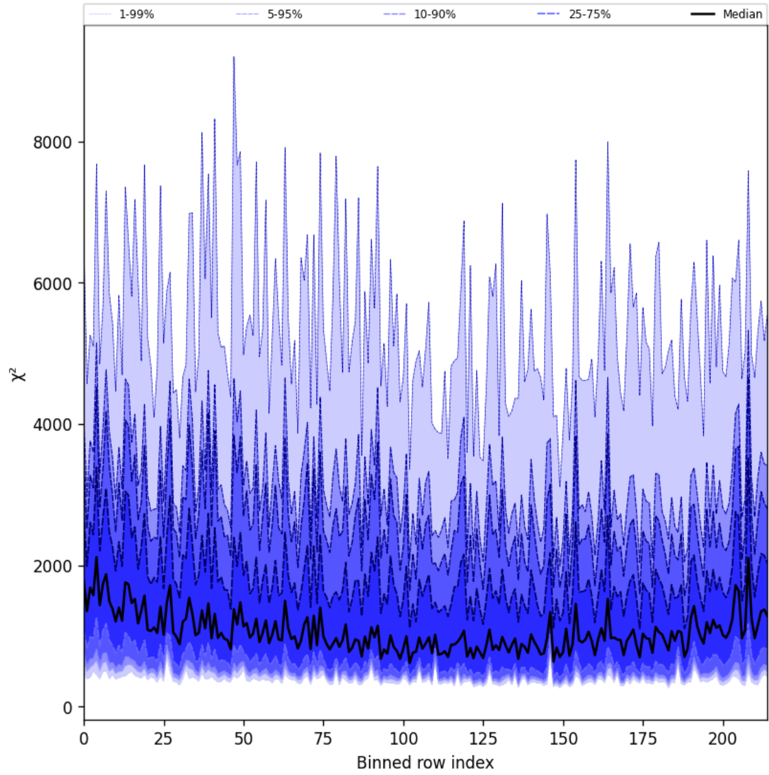
Figure 24: Along track statistics of “ \chi^2 ” for 2024-12-10 to 2024-12-11
