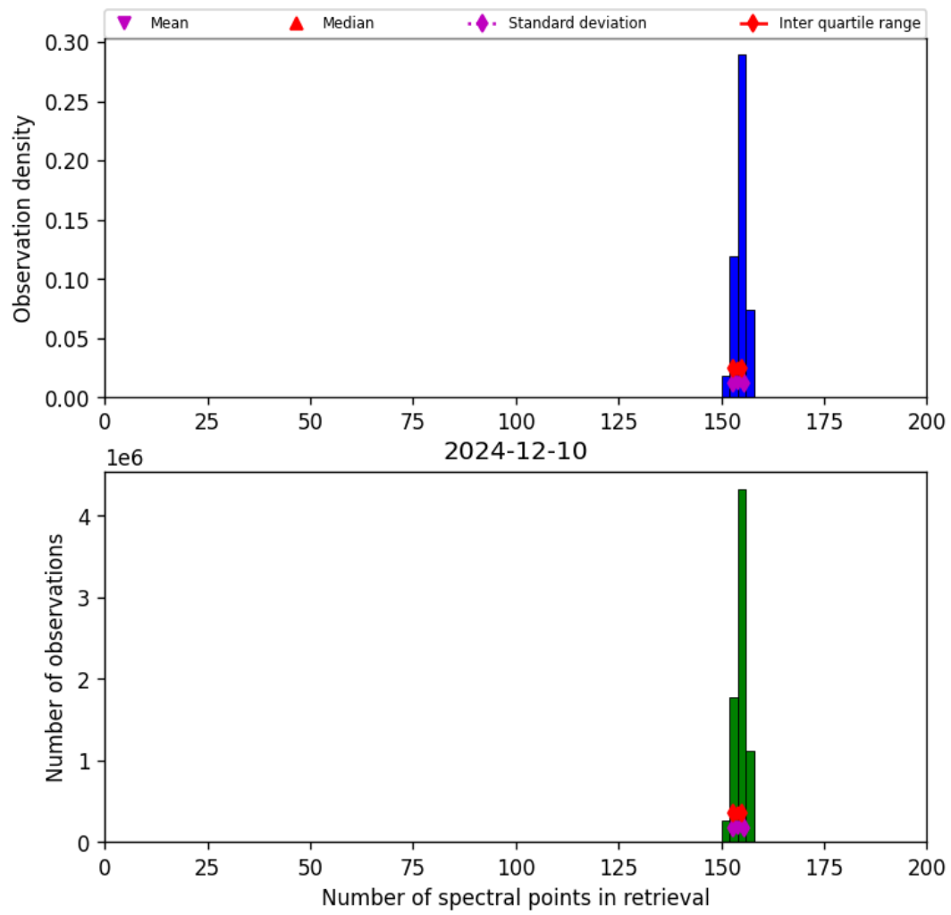
Figure 16: Histogram of “Number of spectral points in retrieval” for 2024-12-10 to 2024-12-11
