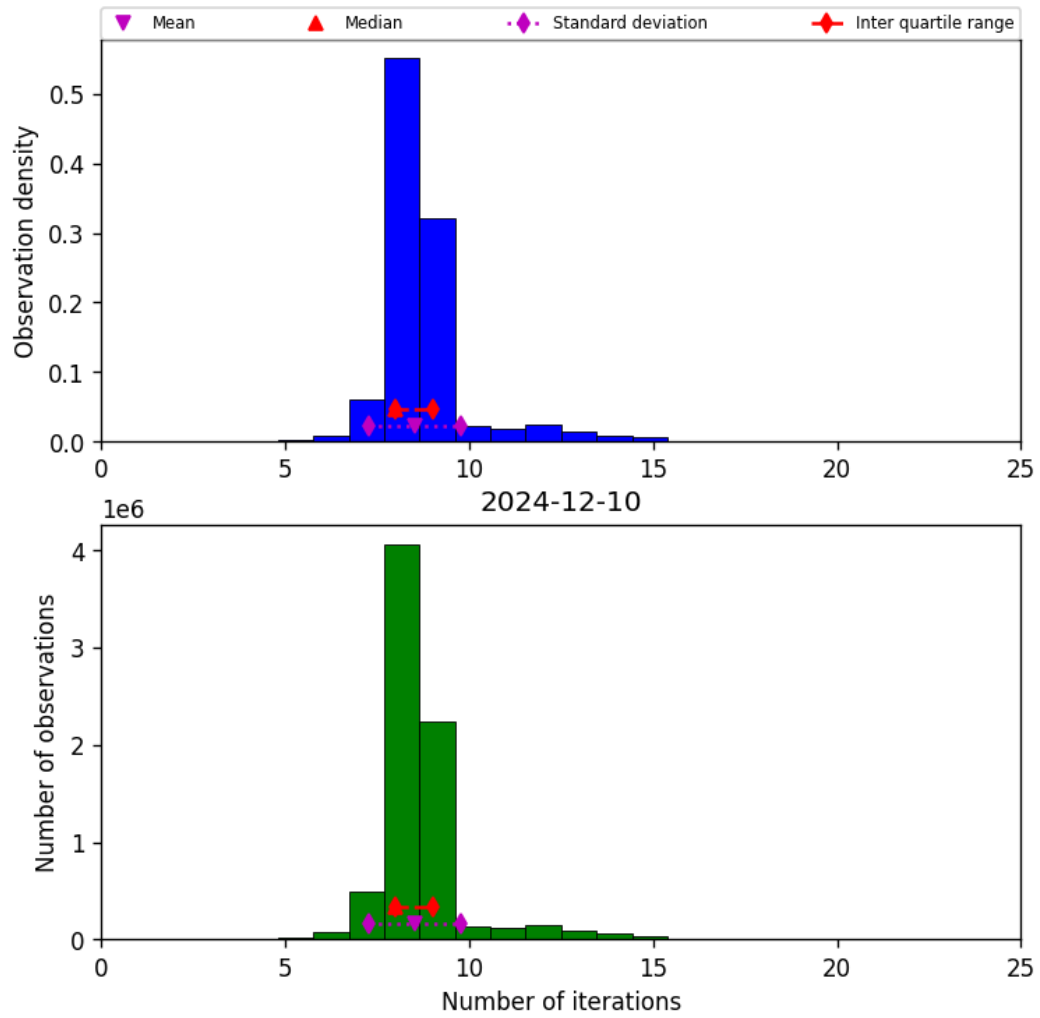
Figure 19: Histogram of “Number of iterations” for 2024-12-10 to 2024-12-11
