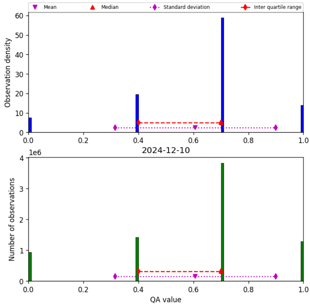
Figure 13: Histogram of “QA value” for 2024-12-10 to 2024-12-11
