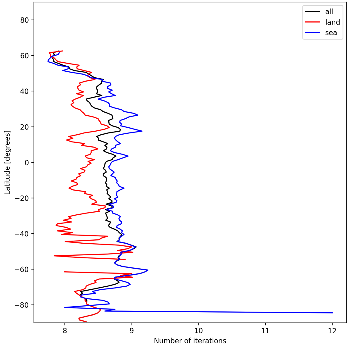
Figure 12: Zonal average of “Number of iterations” for 2024-12-10 to 2024-12-11.
