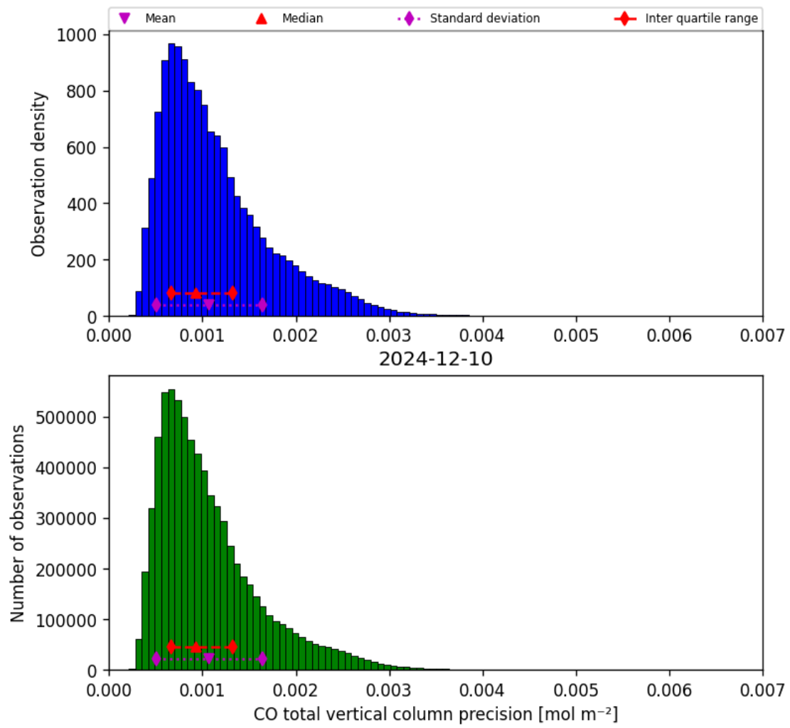
Figure 15: Histogram of “CO total vertical column precision” for 2024-12-10 to 2024-12-11
