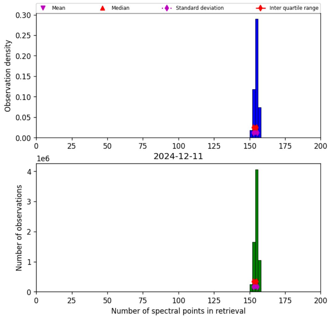
Figure 16: Histogram of “Number of spectral points in retrieval” for 2024-12-11 to 2024-12-12
