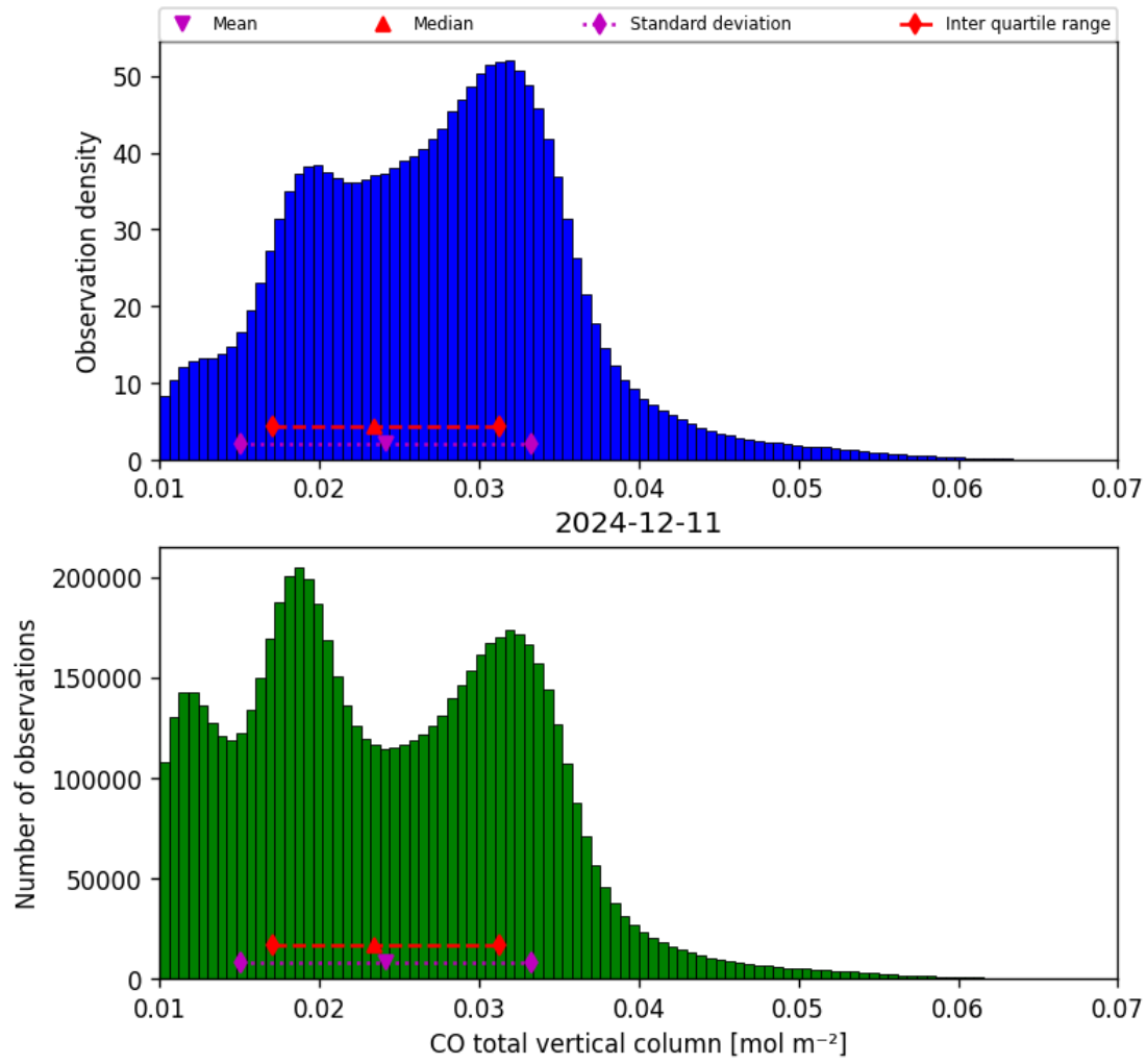
Figure 14: Histogram of “CO total vertical column” for 2024-12-11 to 2024-12-12
