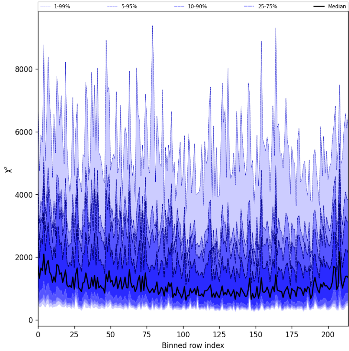
Figure 24: Along track statistics of “ \chi^2 ” for 2024-12-11 to 2024-12-12
