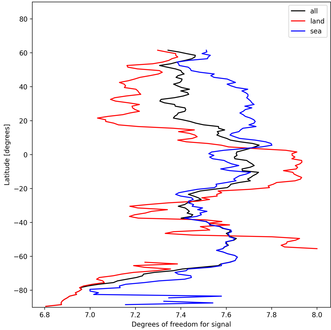
Figure 11: Zonal average of “Degrees of freedom for signal” for 2024-12-11 to 2024-12-12.
