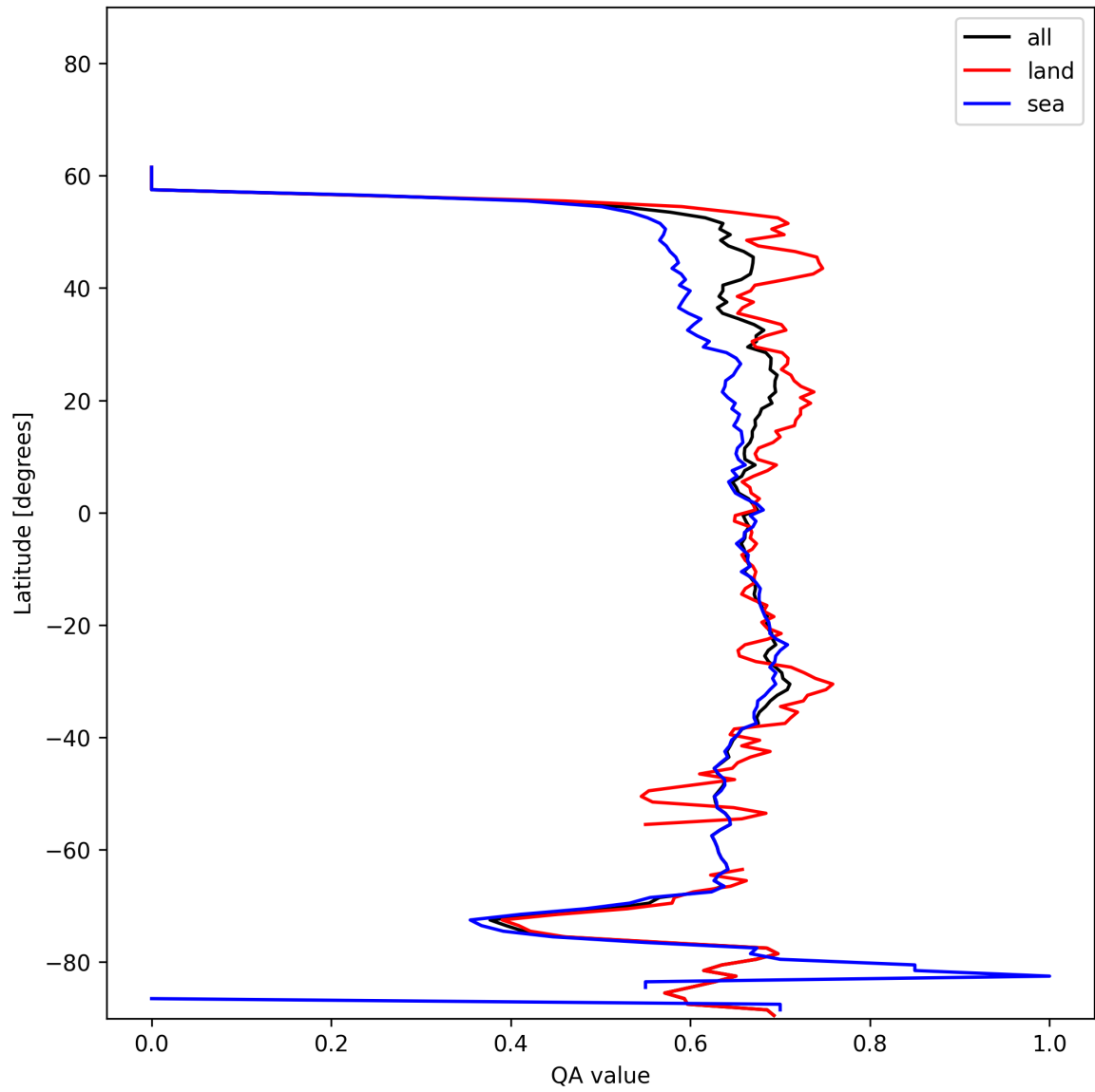
Figure 6: Zonal average of “QA value” for 2024-12-11 to 2024-12-12.
