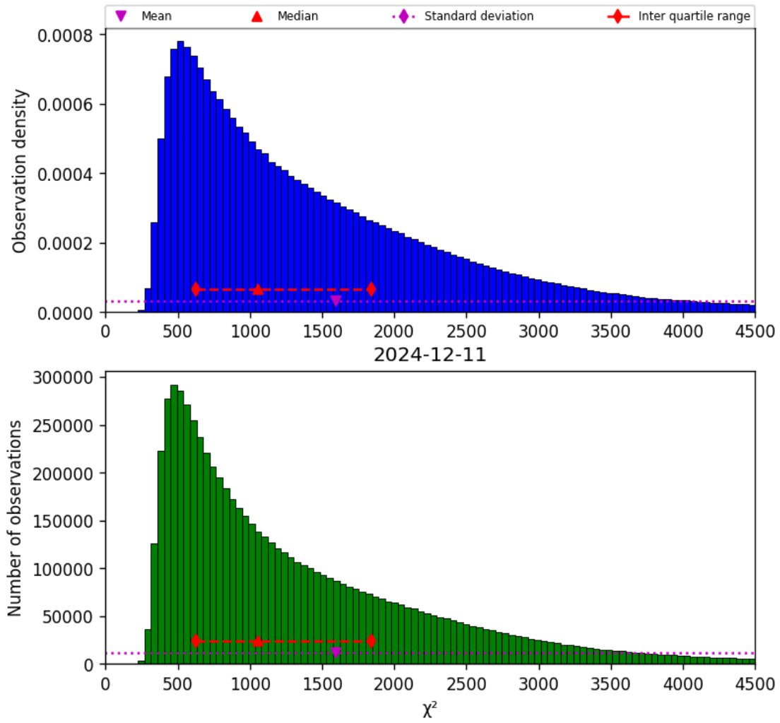
Figure 17: Histogram of “ \chi^2 ” for 2024-12-11 to 2024-12-12
