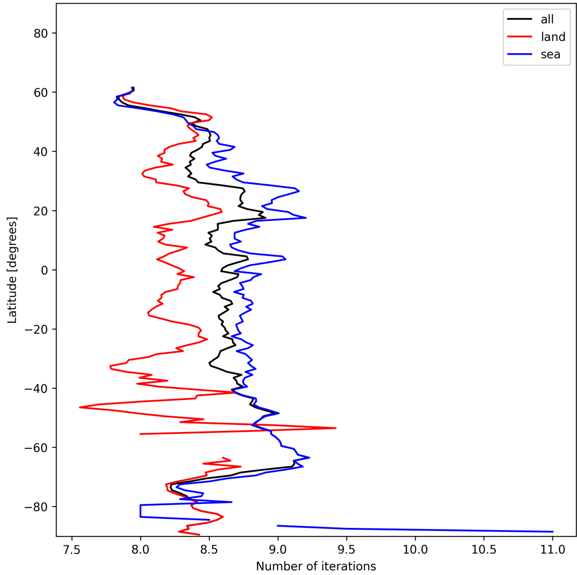
Figure 12: Zonal average of “Number of iterations” for 2024-12-11 to 2024-12-12.
