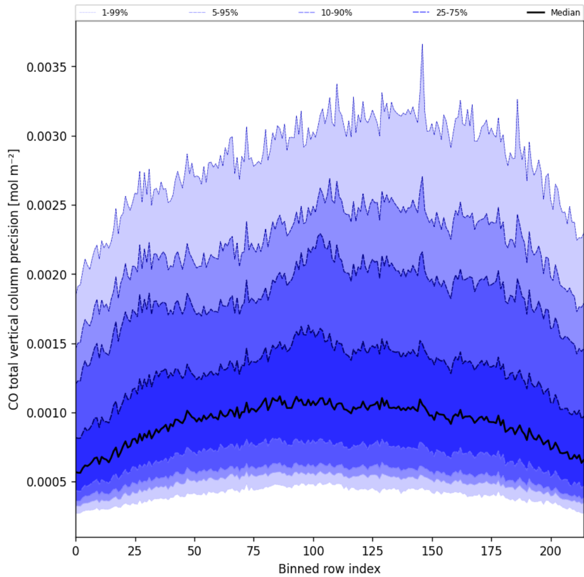
Figure 22: Along track statistics of “CO total vertical column precision” for 2024-12-11 to 2024-12-12
