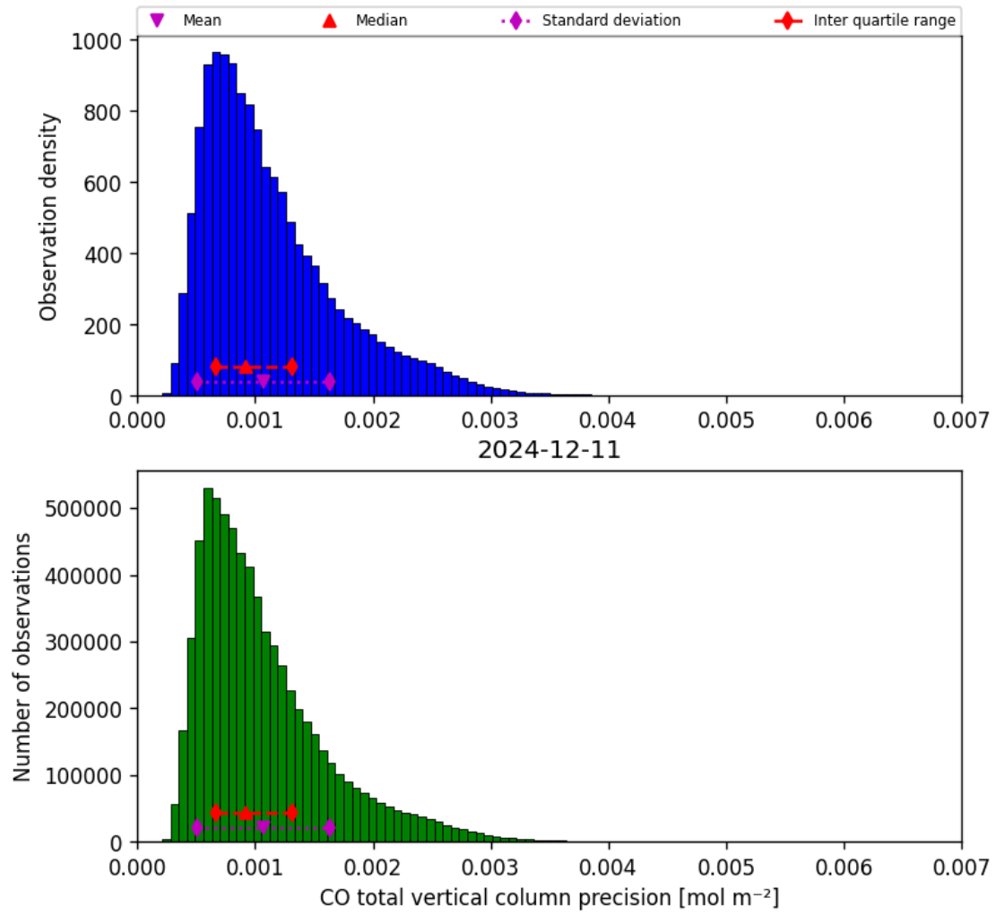
Figure 15: Histogram of “CO total vertical column precision” for 2024-12-11 to 2024-12-12
