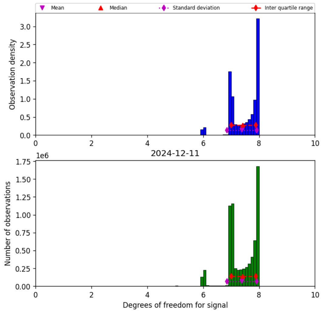
Figure 18: Histogram of “Degrees of freedom for signal” for 2024-12-11 to 2024-12-12
