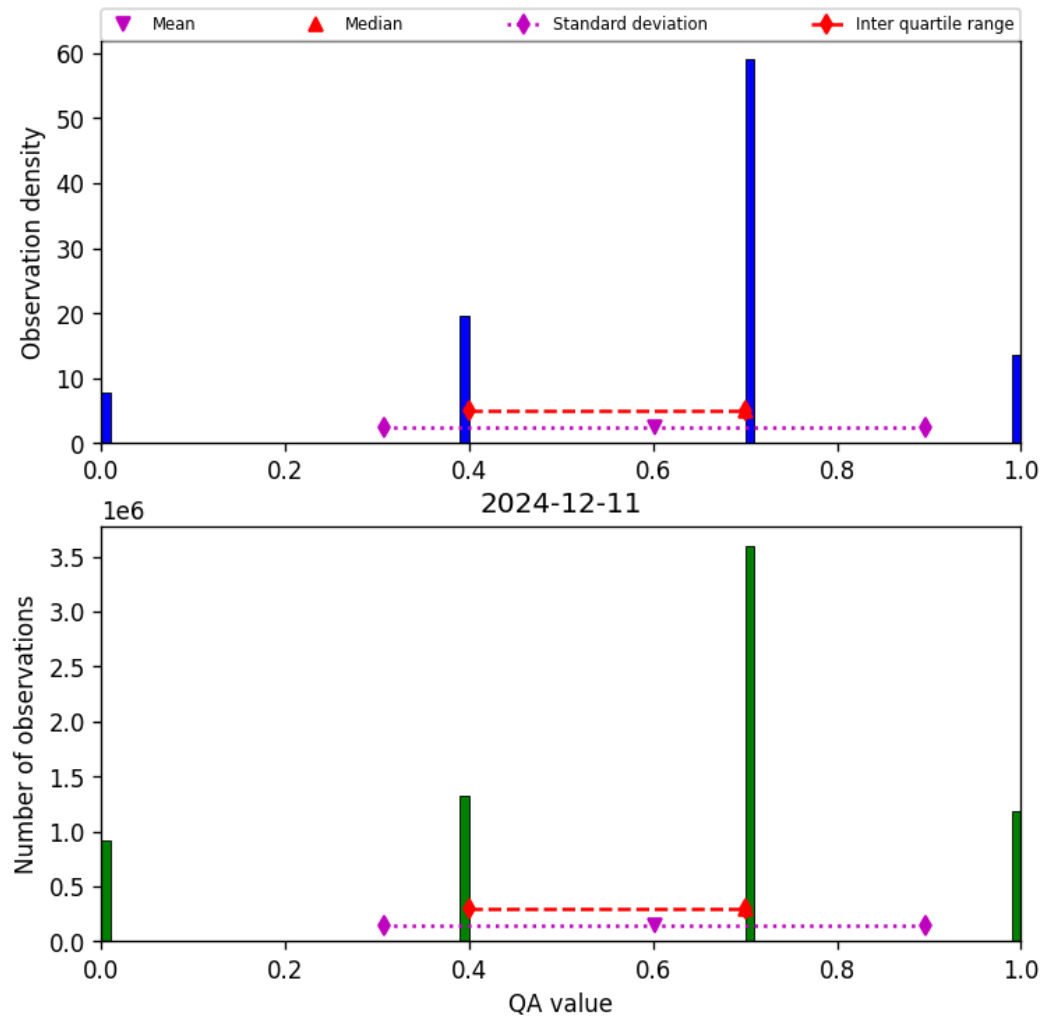
Figure 13: Histogram of “QA value” for 2024-12-11 to 2024-12-12
