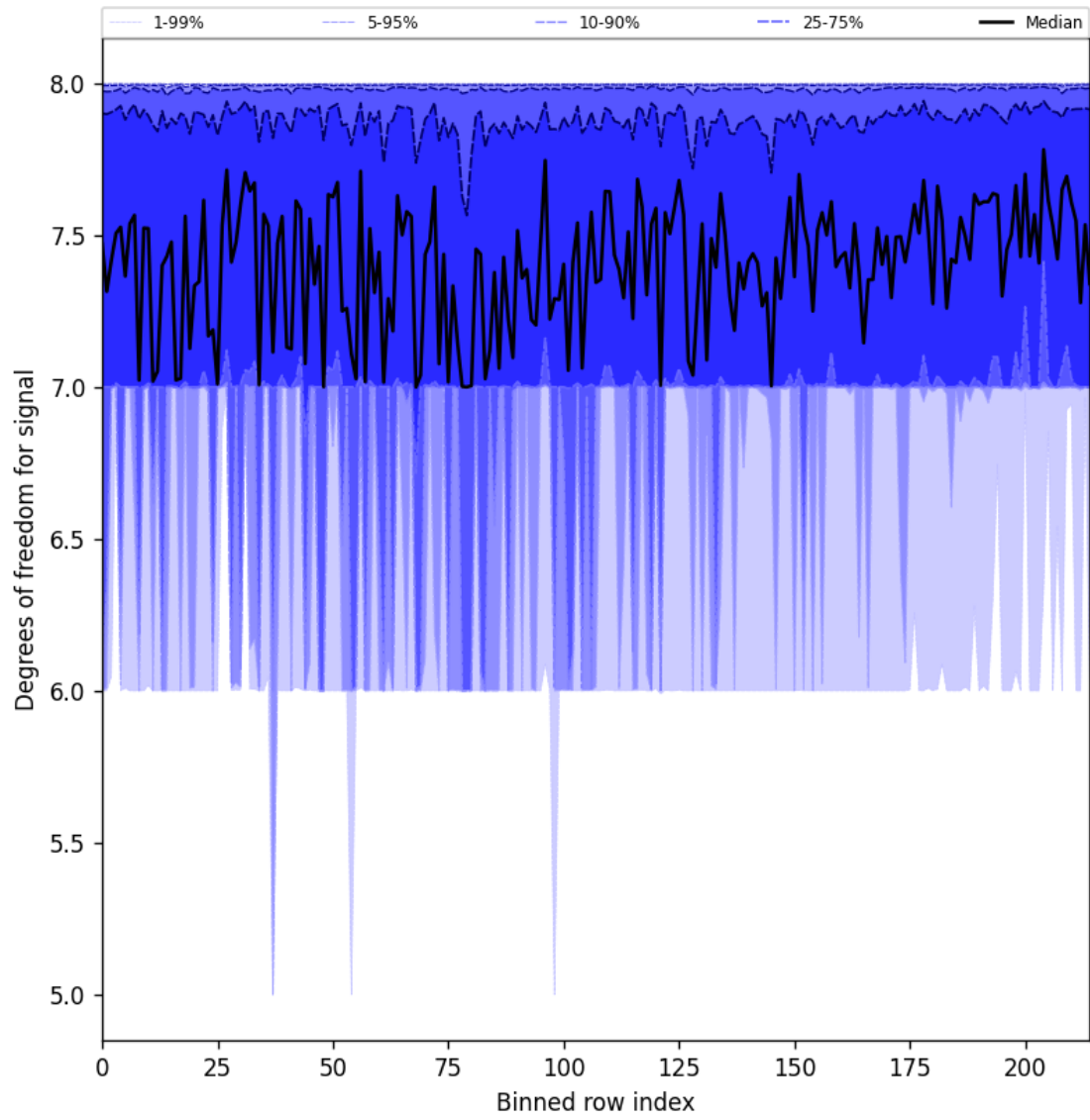
Figure 25: Along track statistics of “Degrees of freedom for signal” for 2024-12-11 to 2024-12-12
