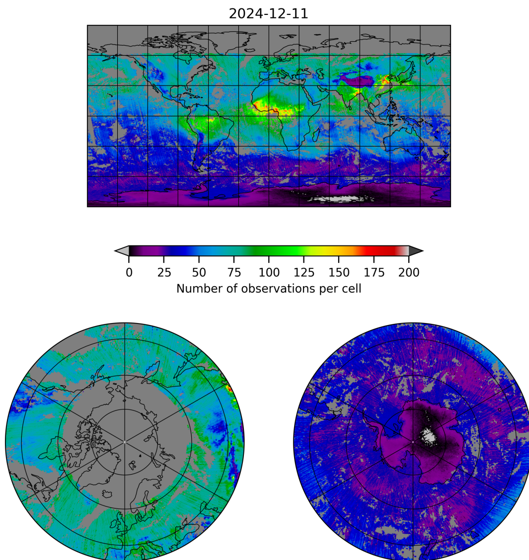
Figure 5: Map of the number of observations for 2024-12-11 to 2024-12-12
