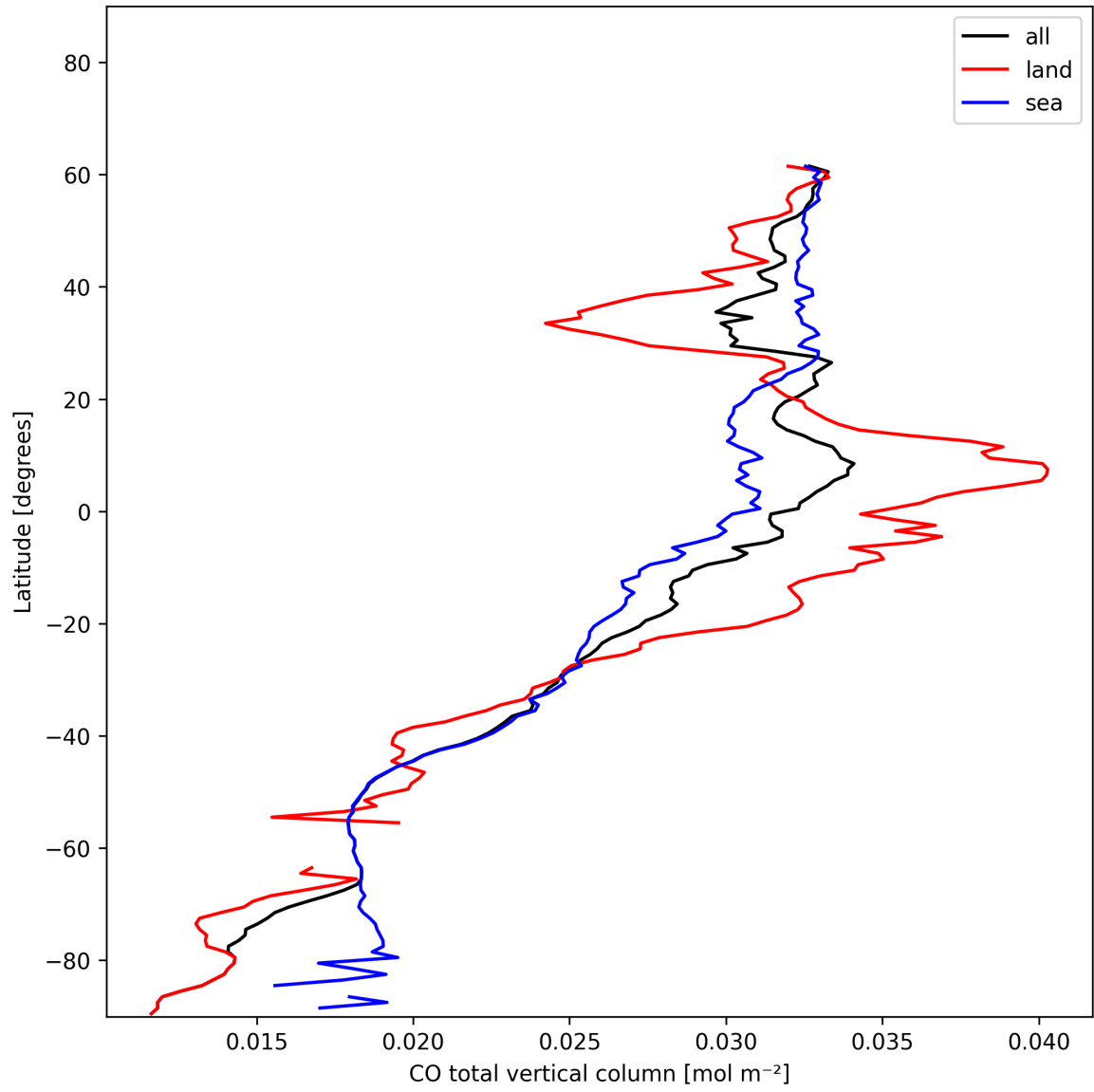
Figure 7: Zonal average of “CO total vertical column” for 2024-12-11 to 2024-12-12.
