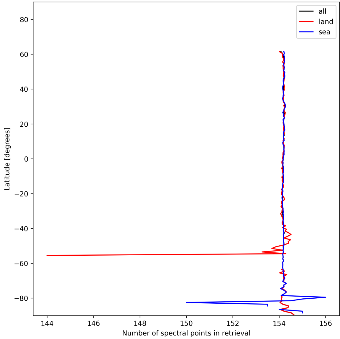
Figure 9: Zonal average of “Number of spectral points in retrieval” for 2024-12-11 to 2024-12-12.
