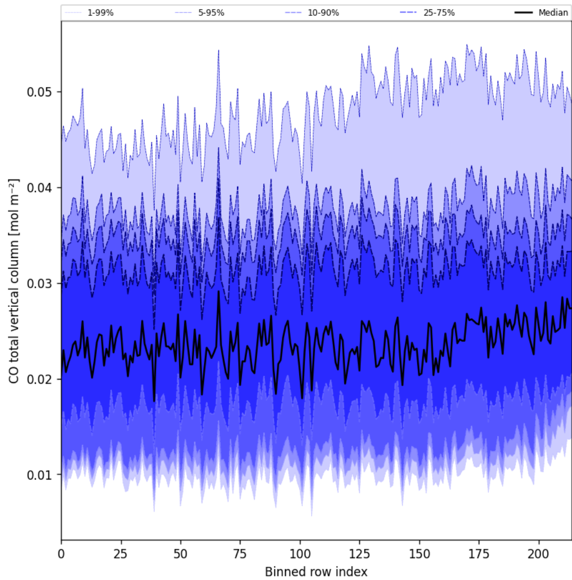
Figure 21: Along track statistics of “CO total vertical column” for 2024-12-11 to 2024-12-12
