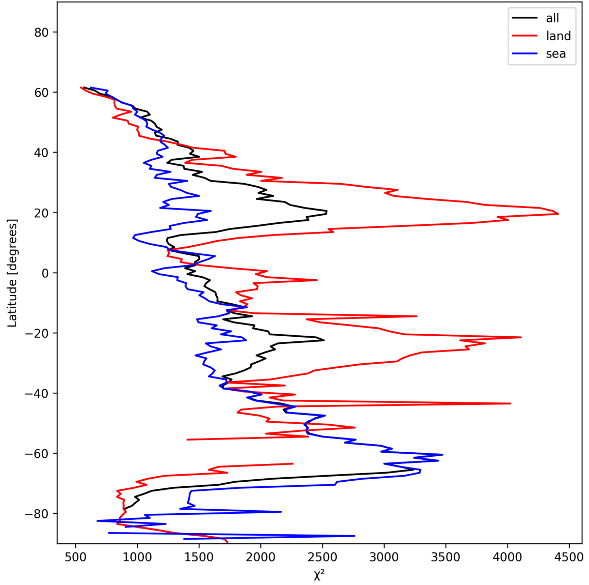
Figure 10: Zonal average of “ \chi^2 ” for 2024-12-11 to 2024-12-12.
