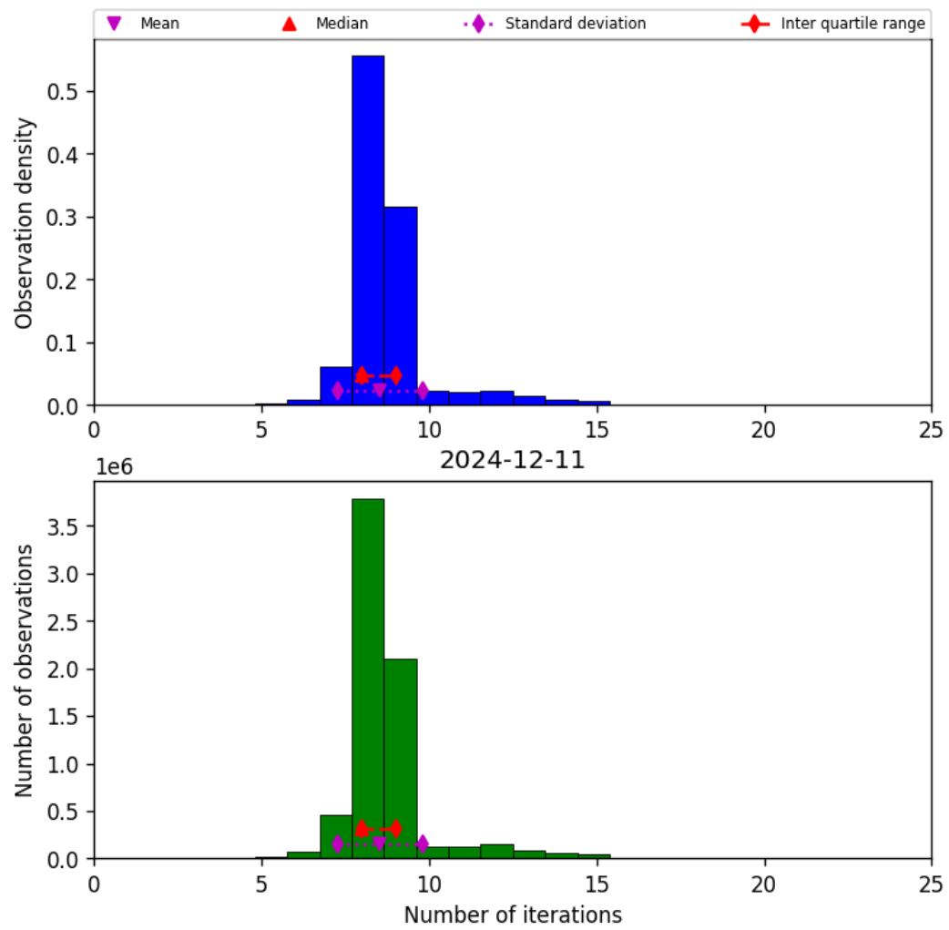
Figure 19: Histogram of “Number of iterations” for 2024-12-11 to 2024-12-12
