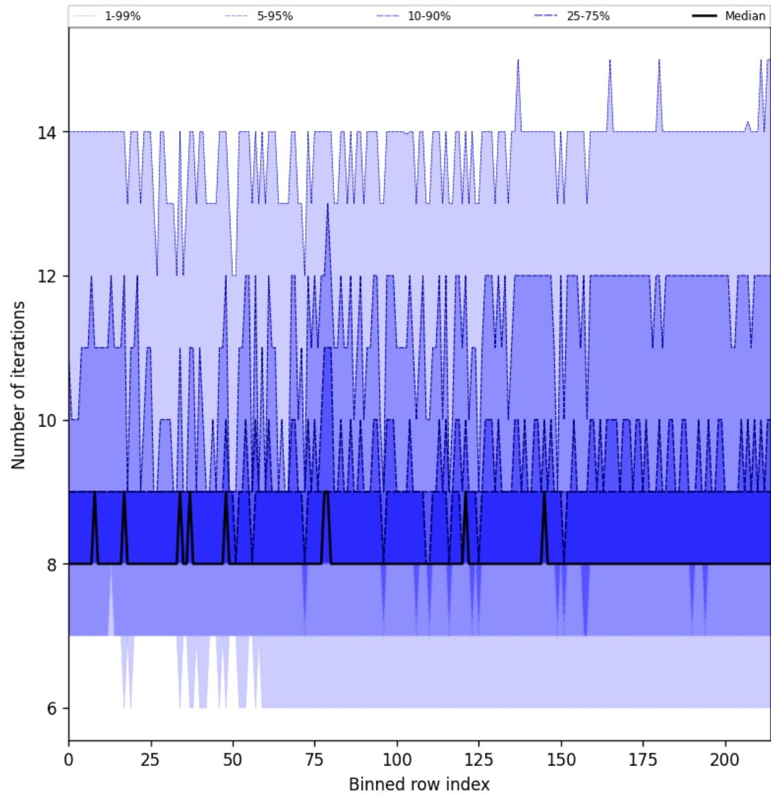
Figure 26: Along track statistics of “Number of iterations” for 2024-12-11 to 2024-12-12
