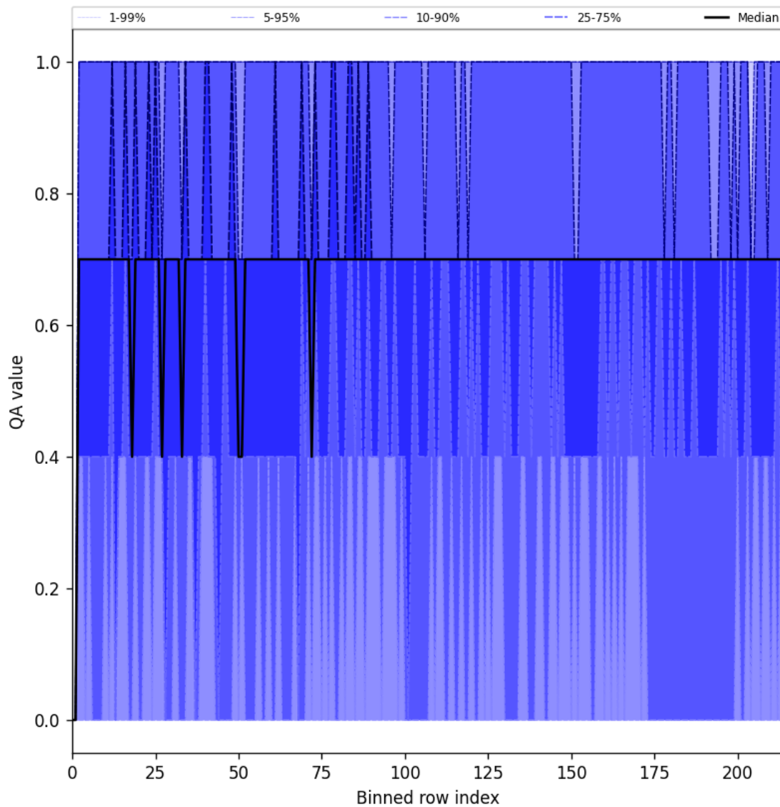
Figure 20: Along track statistics of “QA value” for 2024-12-11 to 2024-12-12
