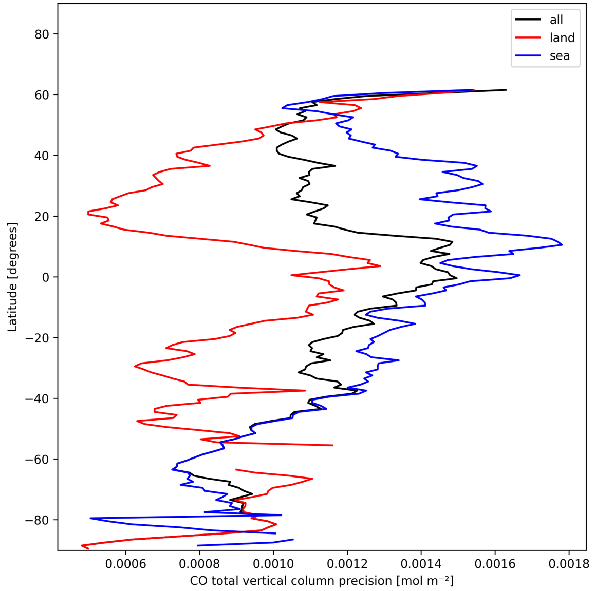
Figure 8: Zonal average of “CO total vertical column precision” for 2024-12-11 to 2024-12-12.
