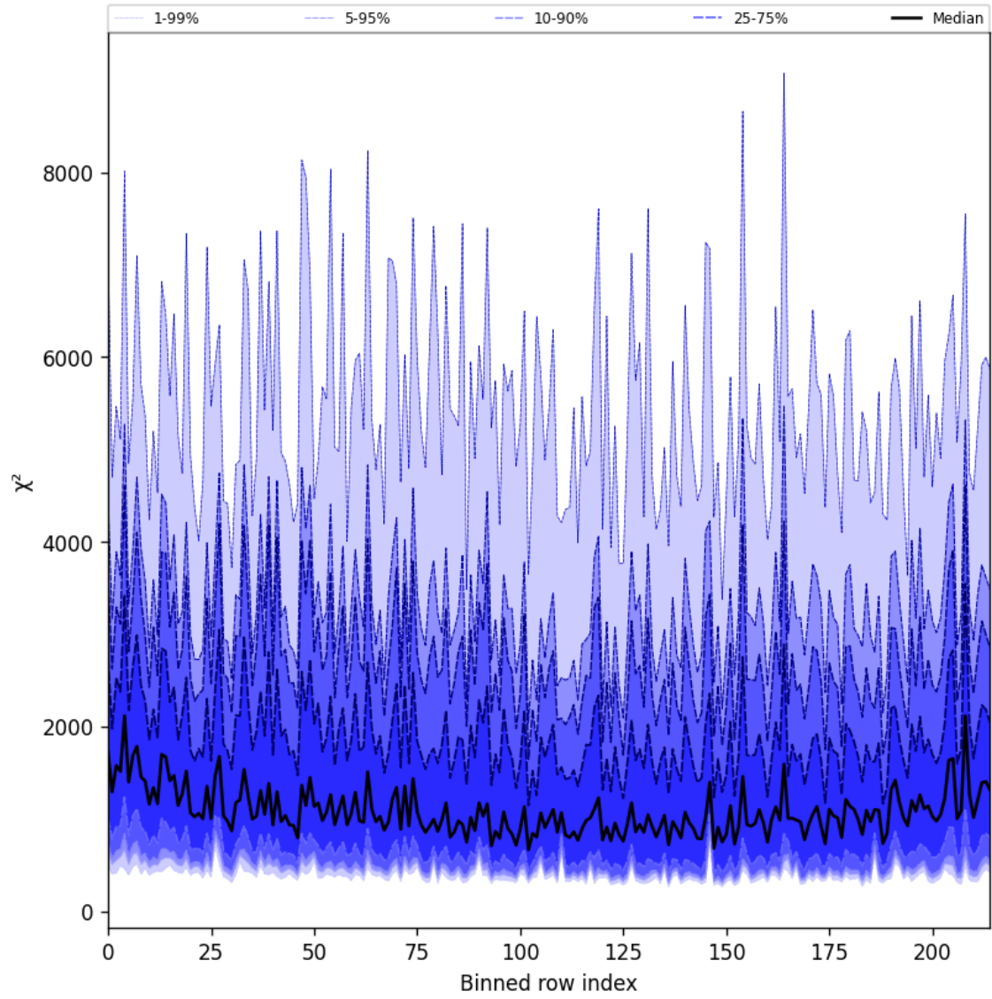
Figure 24: Along track statistics of “ \chi^2 ” for 2024-12-13 to 2024-12-14
