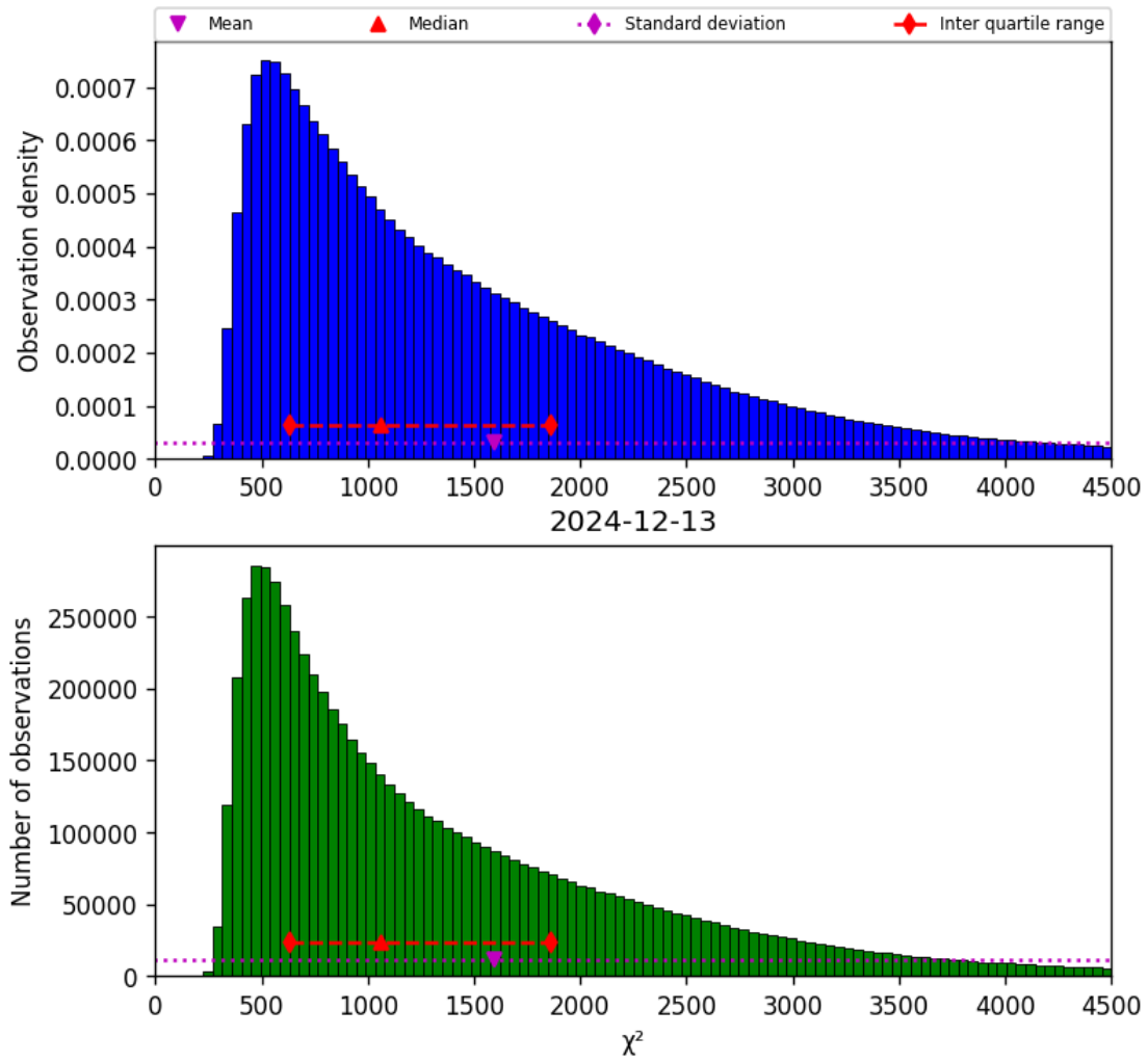
Figure 17: Histogram of “ \chi^2 ” for 2024-12-13 to 2024-12-14
