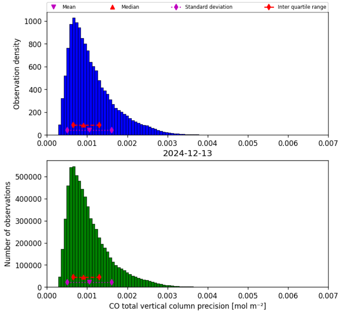
Figure 15: Histogram of “CO total vertical column precision” for 2024-12-13 to 2024-12-14
