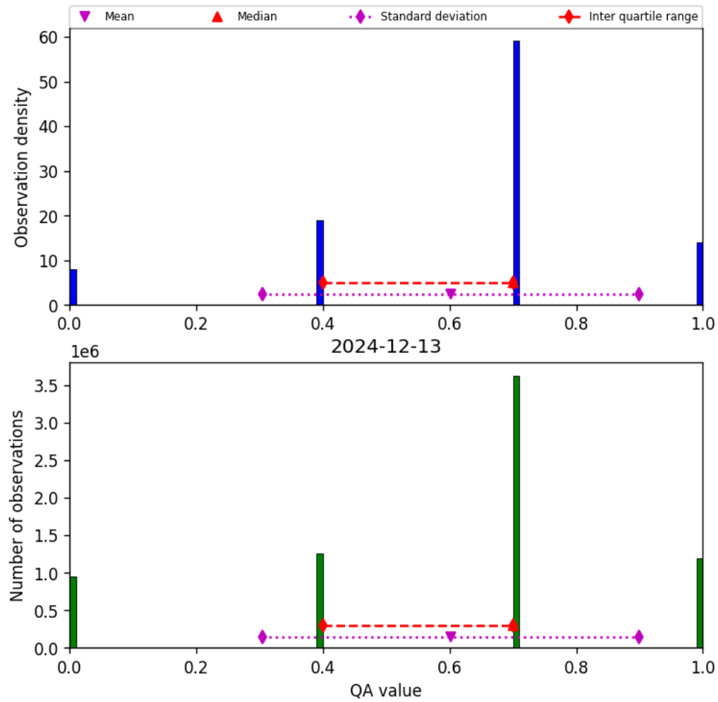
Figure 13: Histogram of “QA value” for 2024-12-13 to 2024-12-14
