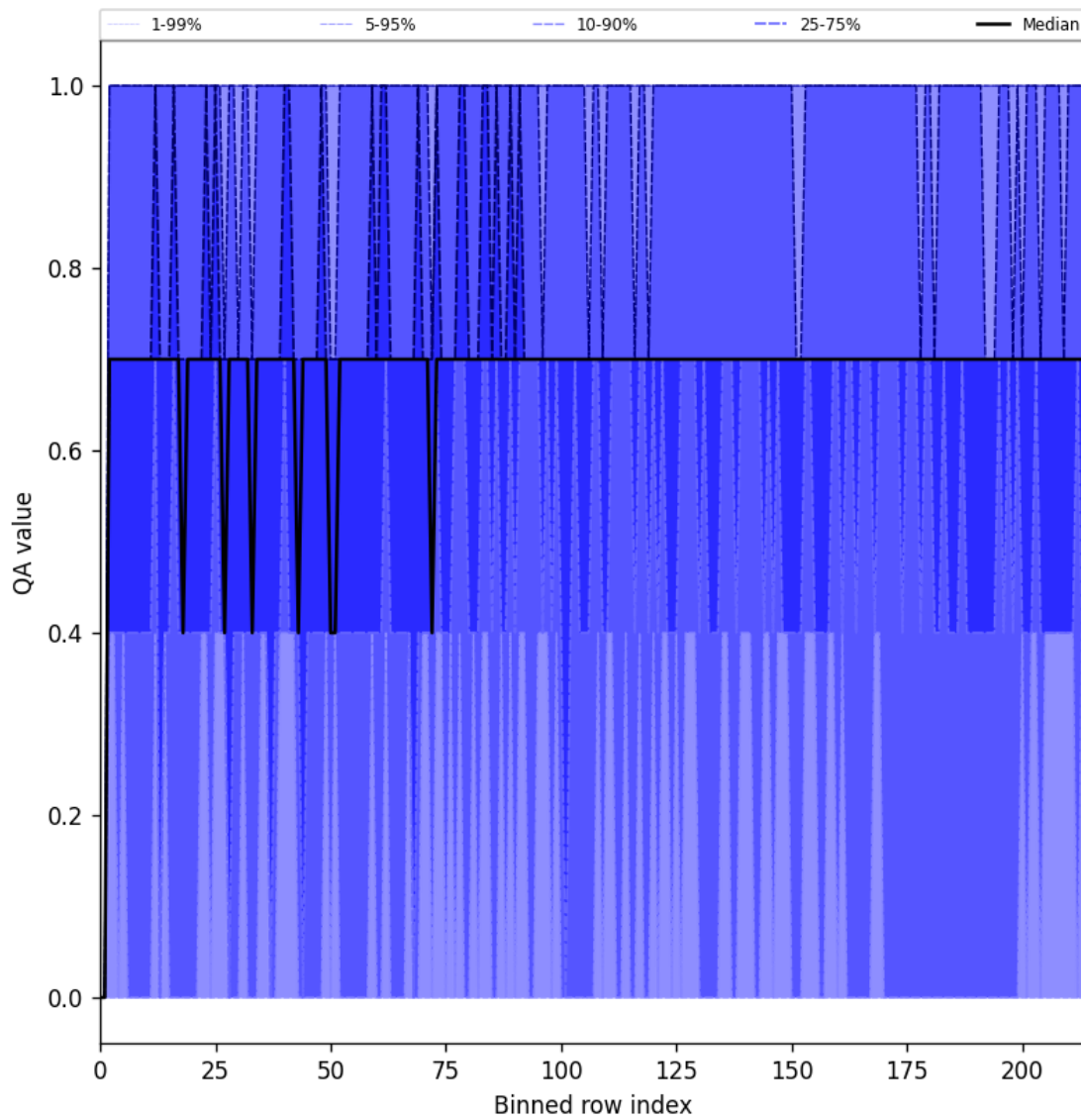
Figure 20: Along track statistics of “QA value” for 2024-12-13 to 2024-12-14
