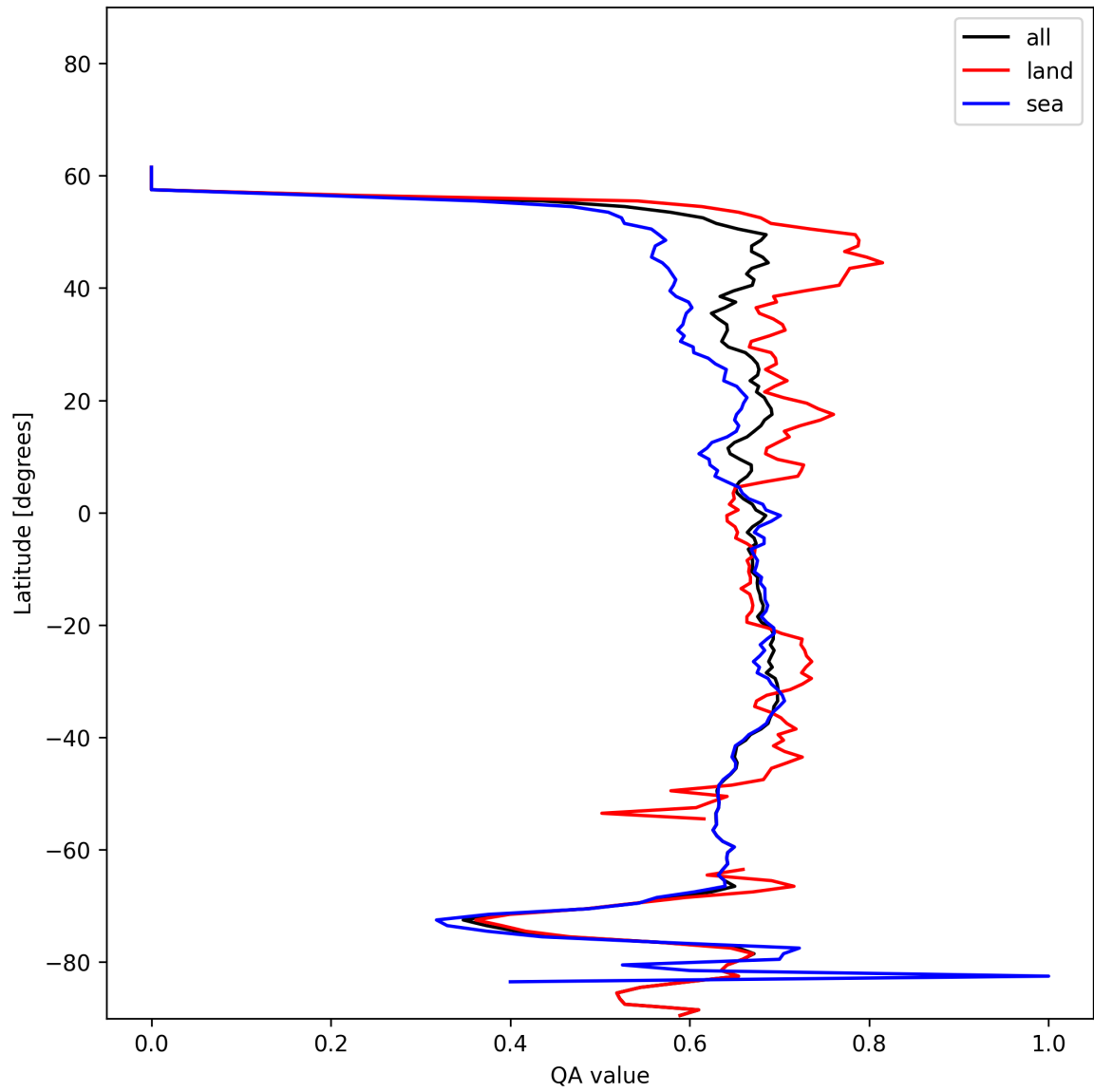
Figure 6: Zonal average of “QA value” for 2024-12-13 to 2024-12-14.
