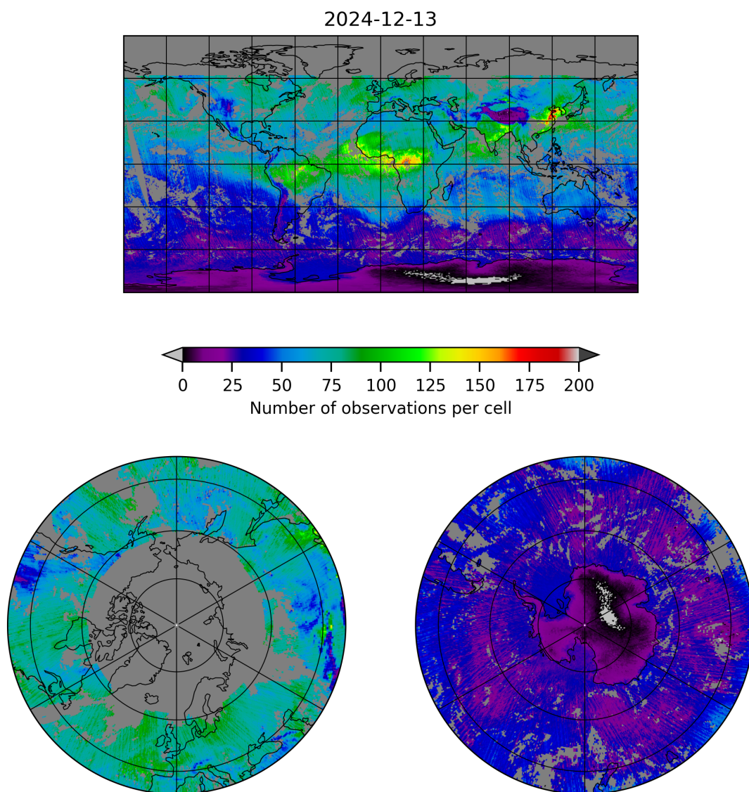
Figure 5: Map of the number of observations for 2024-12-13 to 2024-12-14
