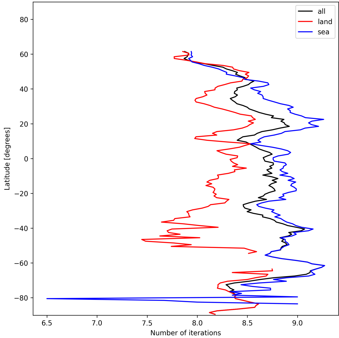
Figure 12: Zonal average of “Number of iterations” for 2024-12-13 to 2024-12-14.
