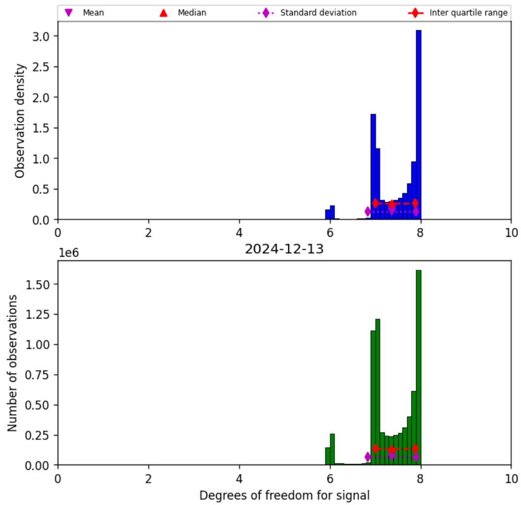
Figure 18: Histogram of “Degrees of freedom for signal” for 2024-12-13 to 2024-12-14
