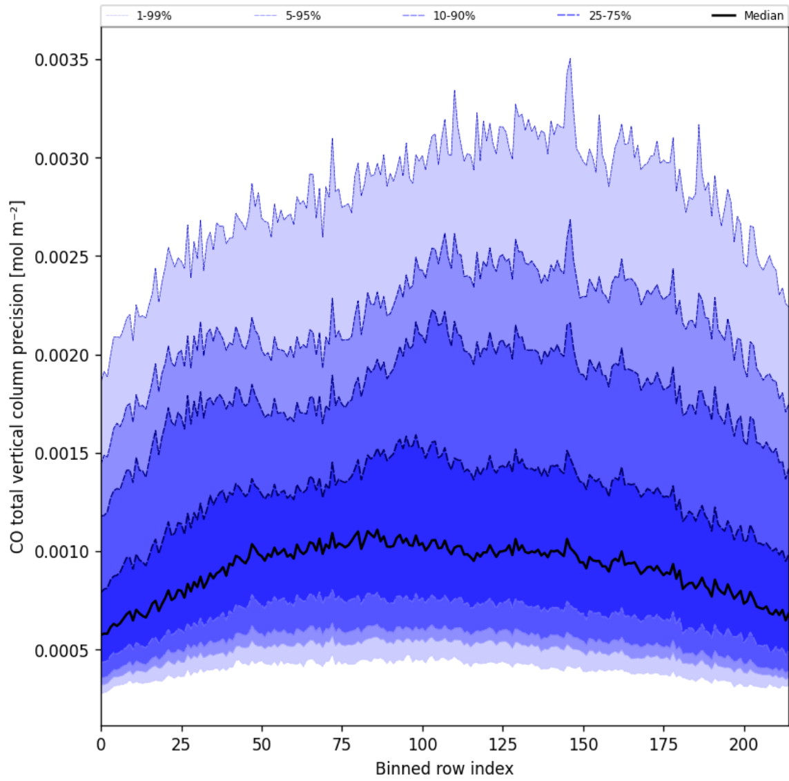
Figure 22: Along track statistics of “CO total vertical column precision” for 2024-12-13 to 2024-12-14
