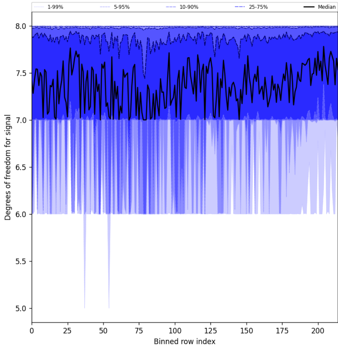
Figure 25: Along track statistics of “Degrees of freedom for signal” for 2024-12-13 to 2024-12-14
