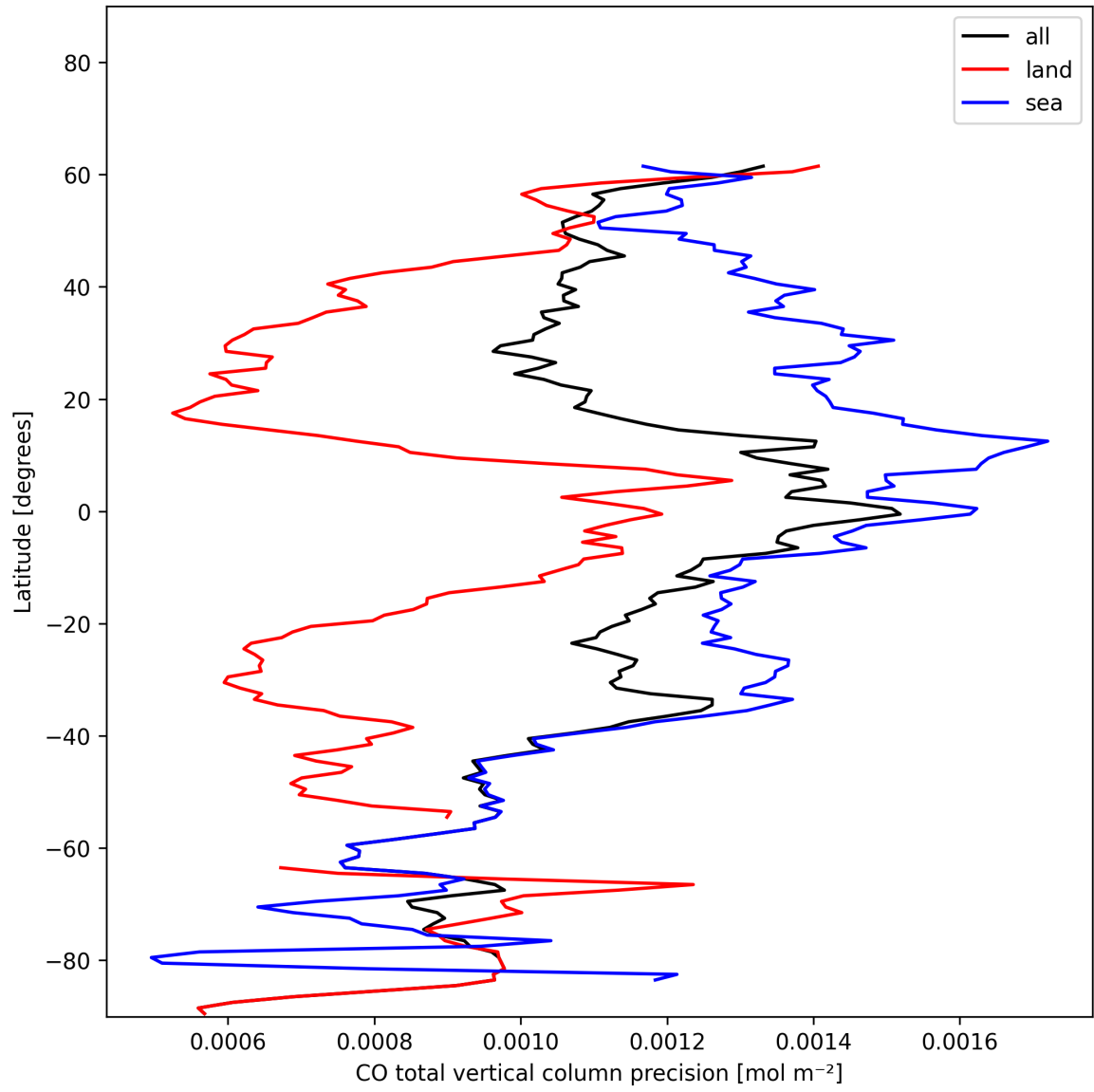
Figure 8: Zonal average of "CO total vertical column precision" for 2024-12-13 to 2024-12-14.
