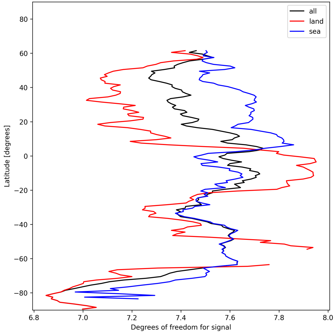
Figure 11: Zonal average of “Degrees of freedom for signal” for 2024-12-13 to 2024-12-14.
