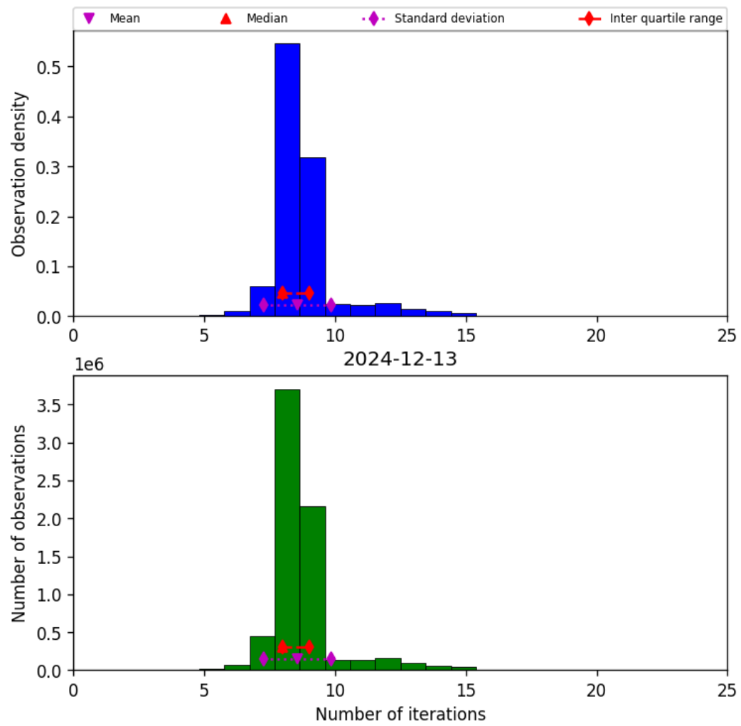
Figure 19: Histogram of “Number of iterations” for 2024-12-13 to 2024-12-14
