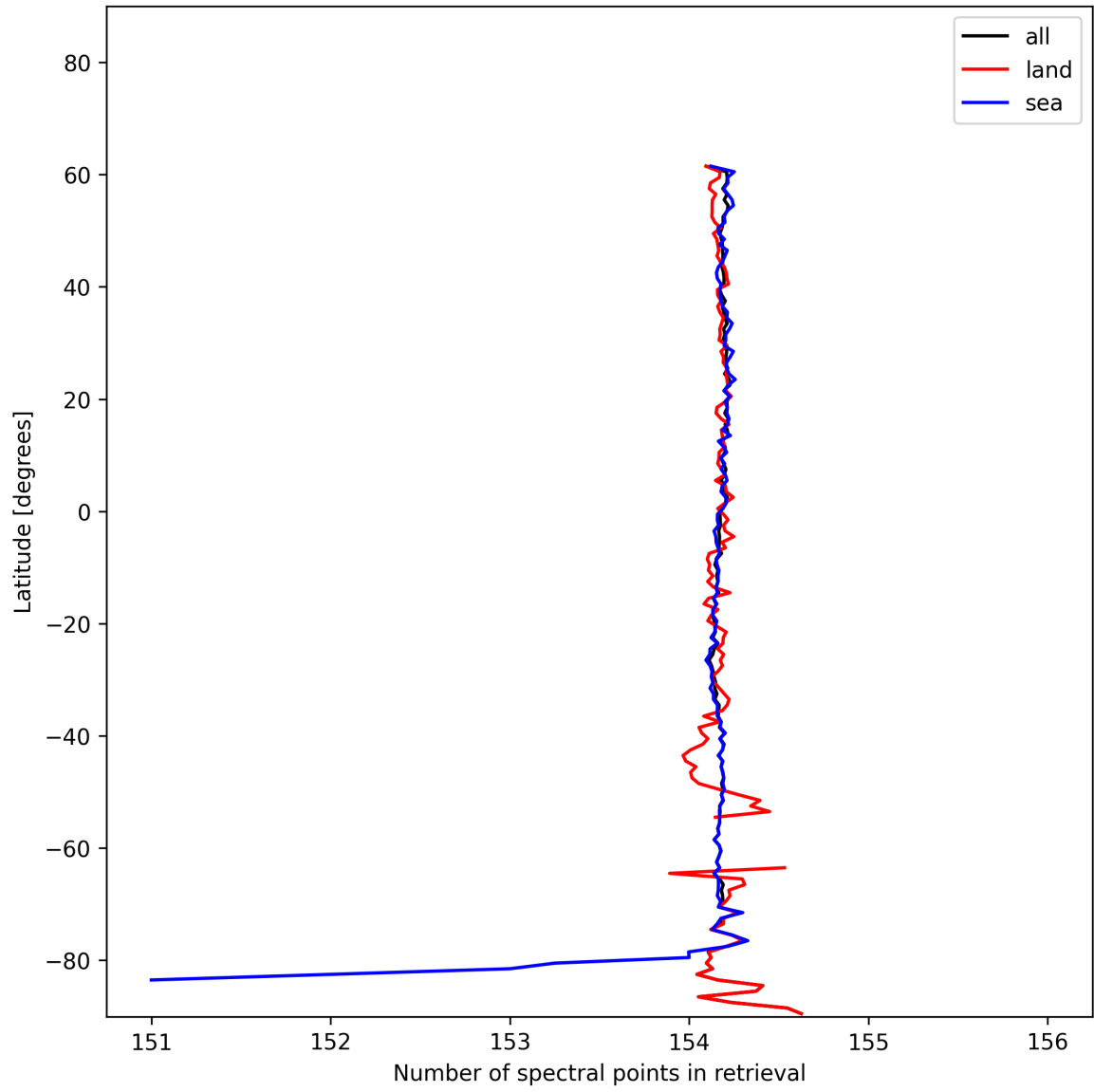
Figure 9: Zonal average of “Number of spectral points in retrieval” for 2024-12-13 to 2024-12-14.
