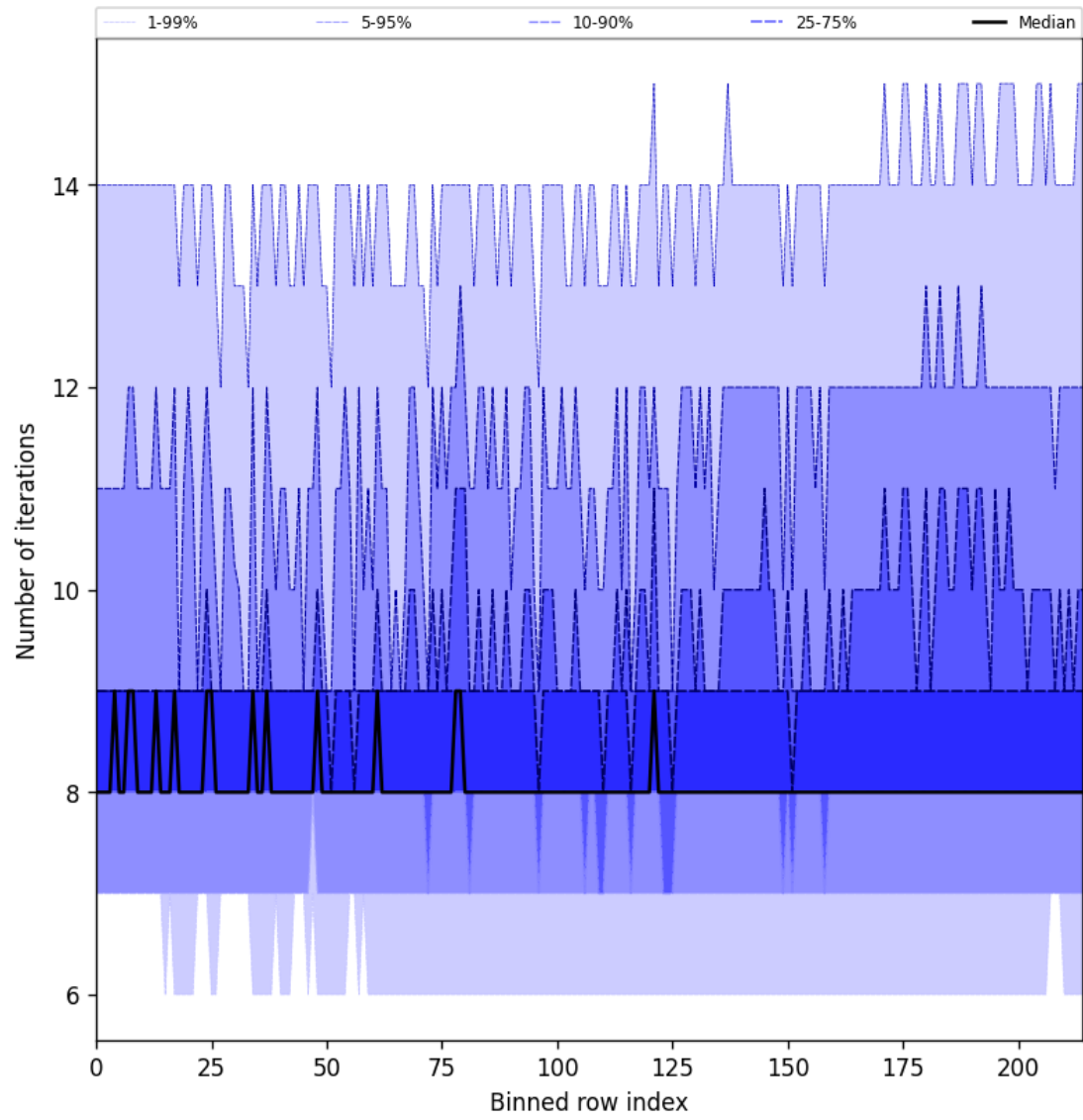
Figure 26: Along track statistics of “Number of iterations” for 2024-12-13 to 2024-12-14
