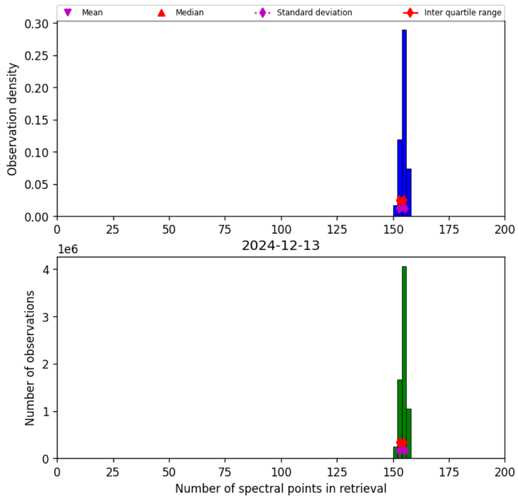
Figure 16: Histogram of “Number of spectral points in retrieval” for 2024-12-13 to 2024-12-14
