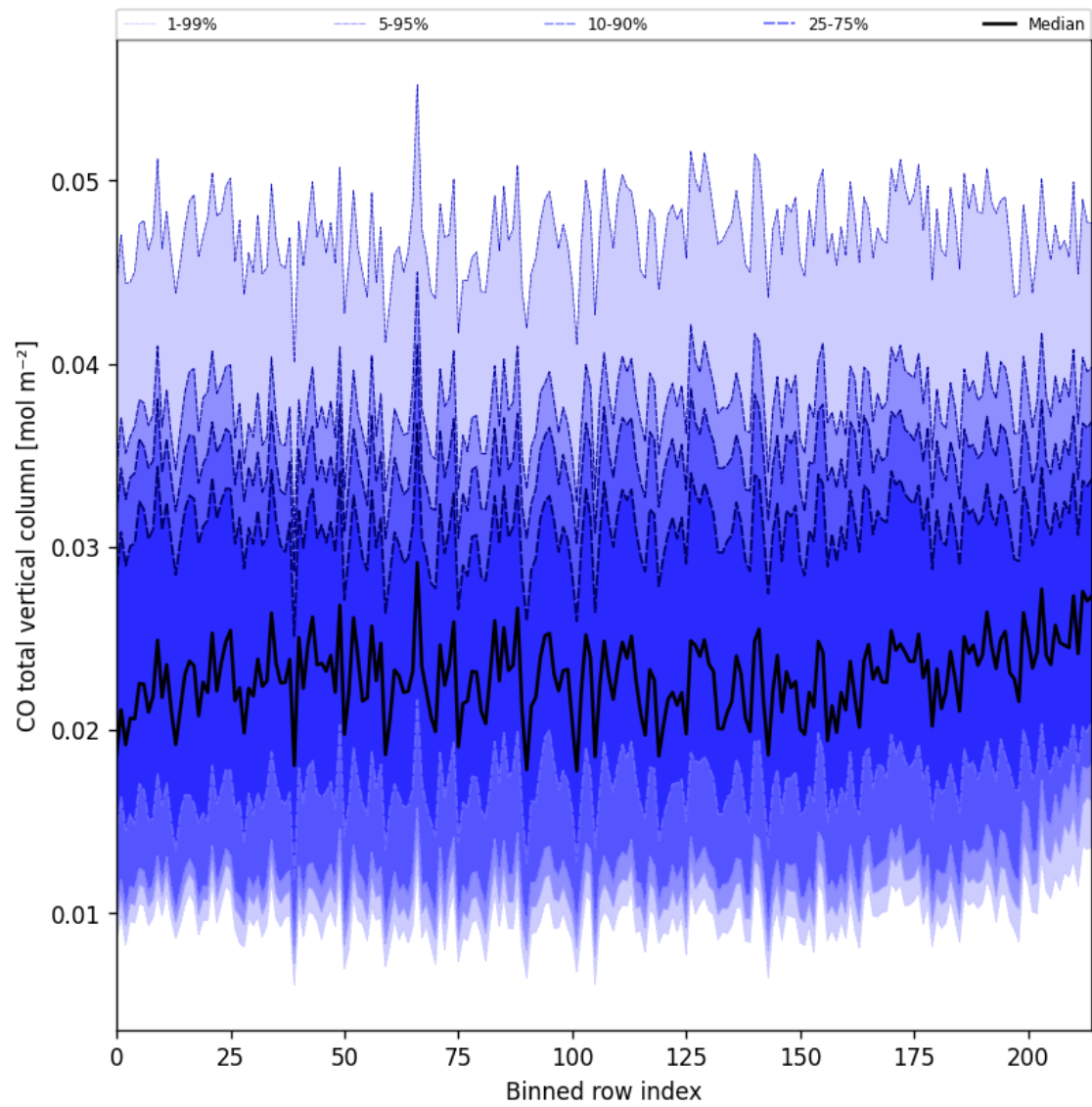
Figure 21: Along track statistics of “CO total vertical column” for 2024-12-13 to 2024-12-14
