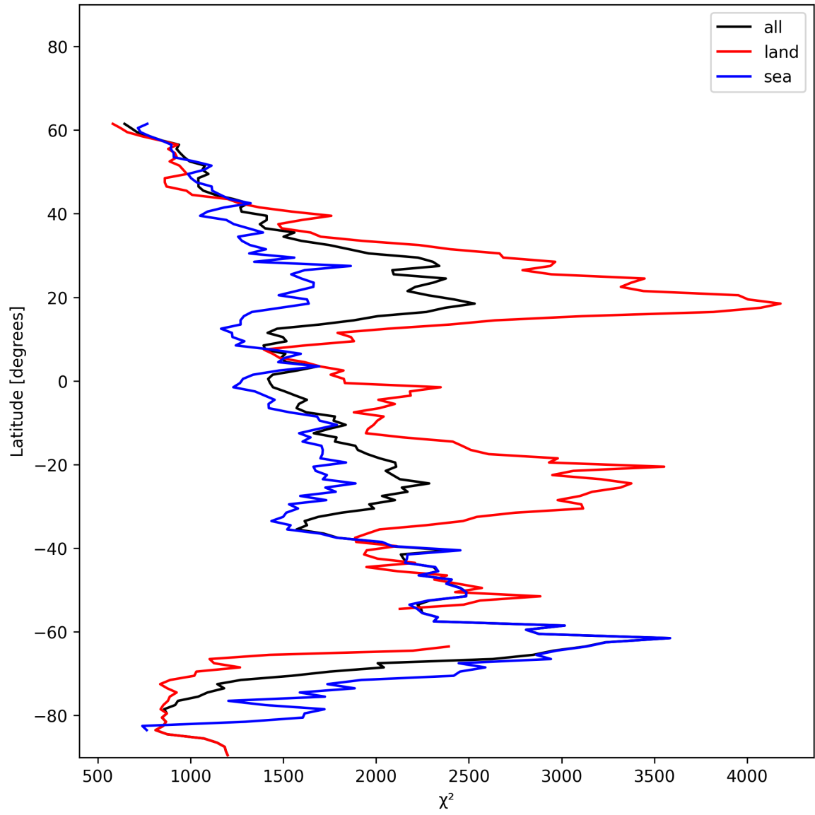
Figure 10: Zonal average of “ \chi^2 ” for 2024-12-13 to 2024-12-14.
