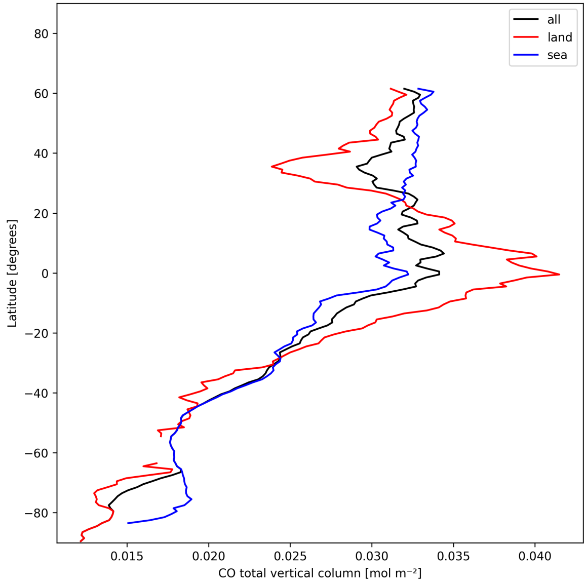
Figure 7: Zonal average of “CO total vertical column” for 2024-12-13 to 2024-12-14.
