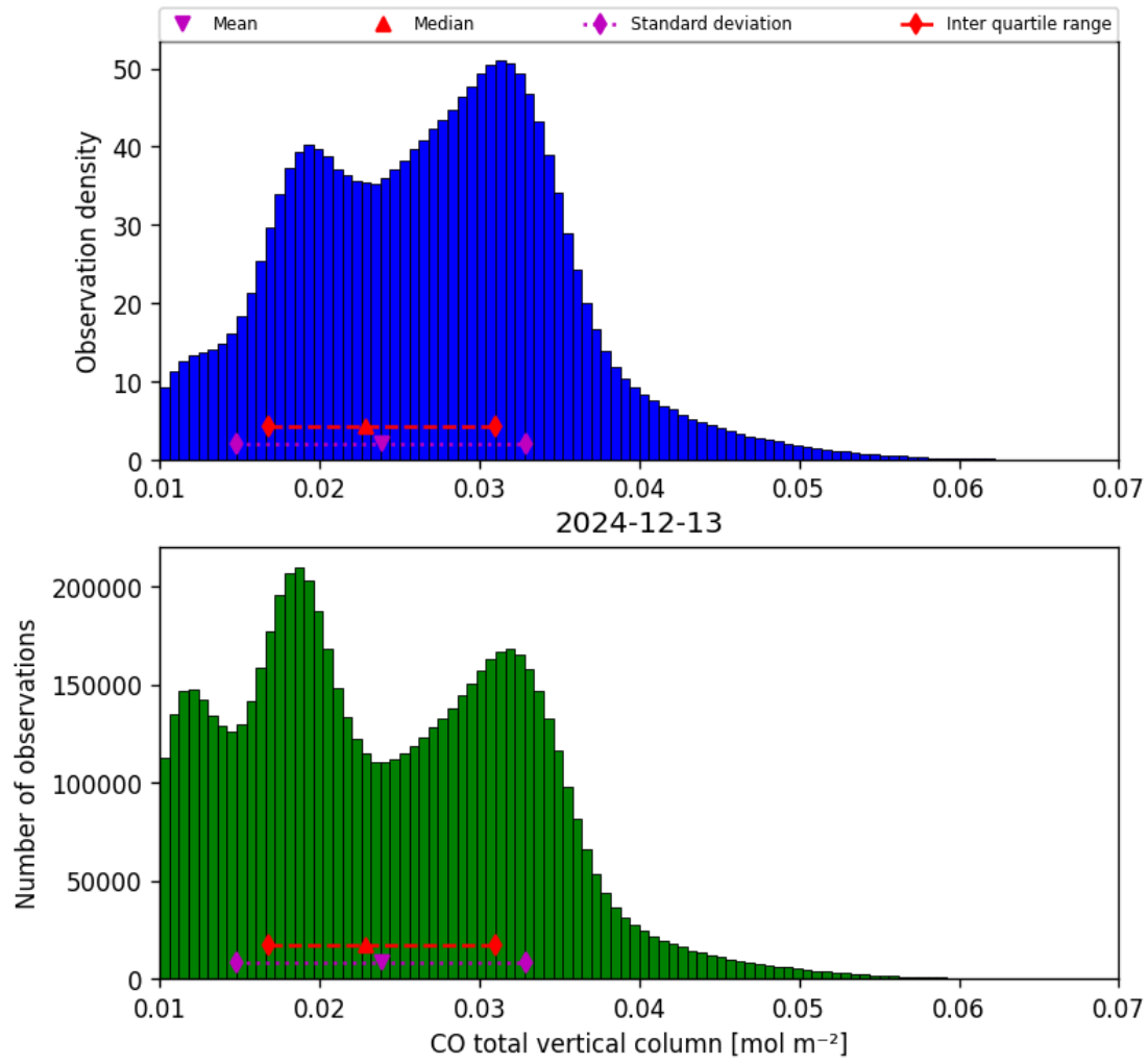
Figure 14: Histogram of “CO total vertical column” for 2024-12-13 to 2024-12-14
