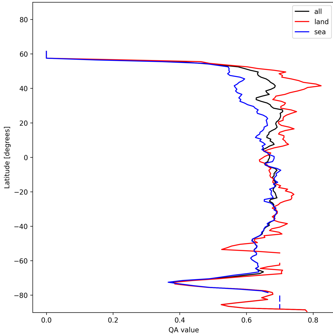
Figure 6: Zonal average of “QA value” for 2024-12-14 to 2024-12-14.
