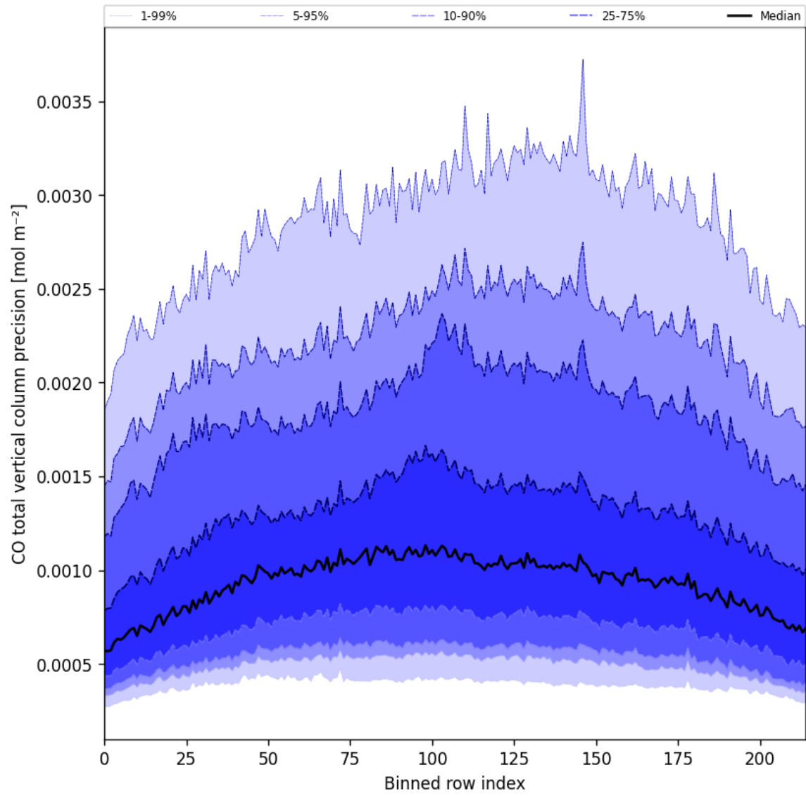
Figure 22: Along track statistics of “CO total vertical column precision” for 2024-12-14 to 2024-12-14
