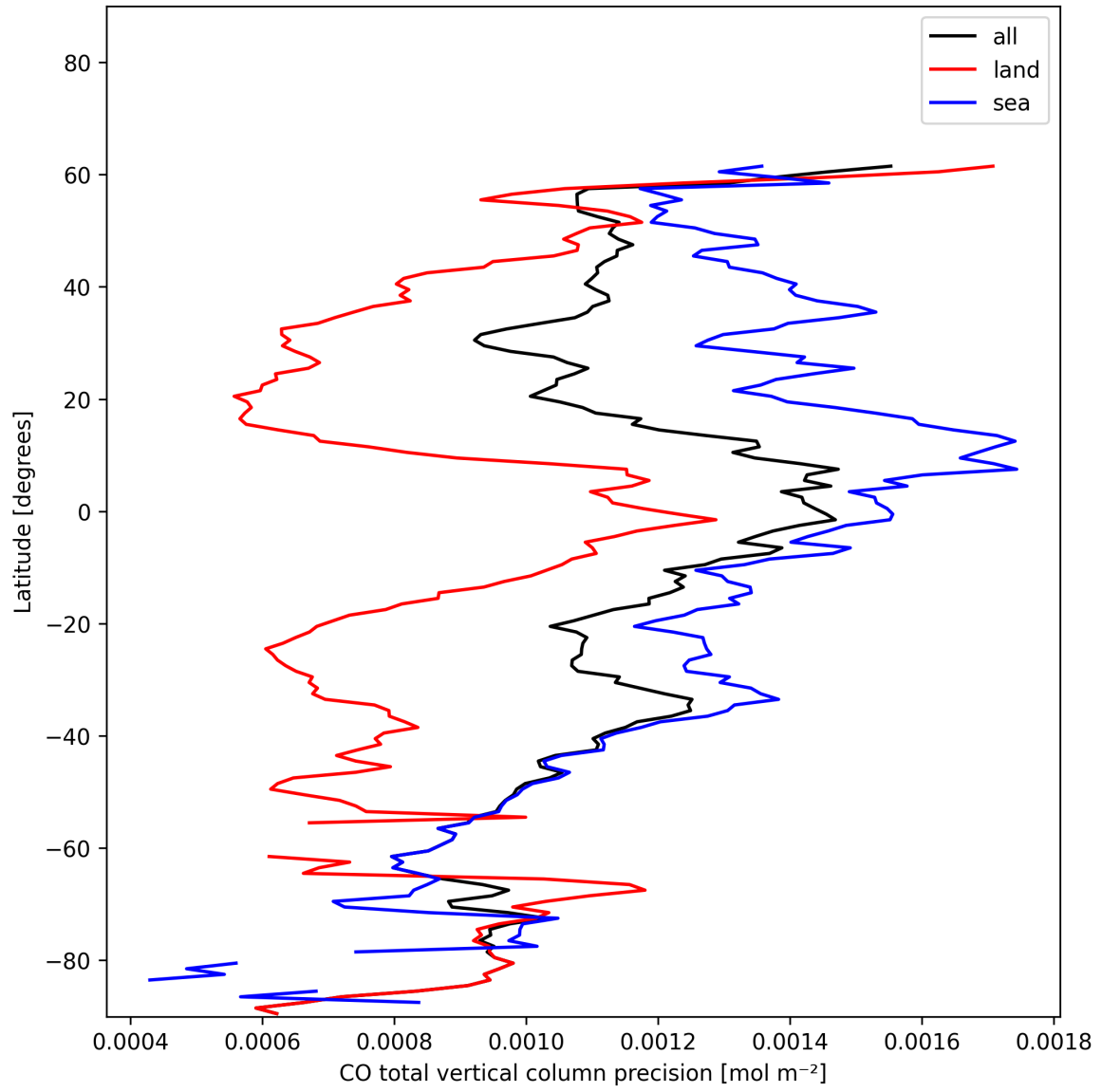
Figure 8: Zonal average of “CO total vertical column precision” for 2024-12-14 to 2024-12-14.
