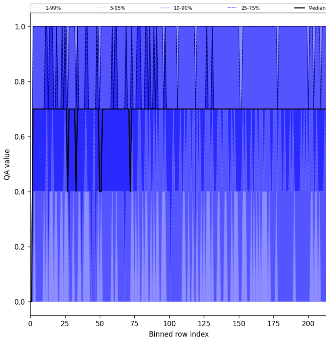
Figure 20: Along track statistics of “QA value” for 2024-12-14 to 2024-12-14
