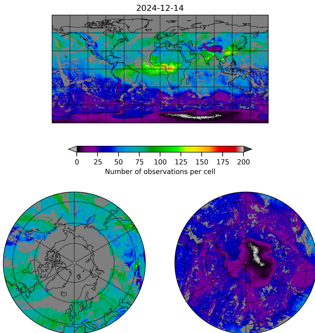
Figure 5: Map of the number of observations for 2024-12-14 to 2024-12-14
