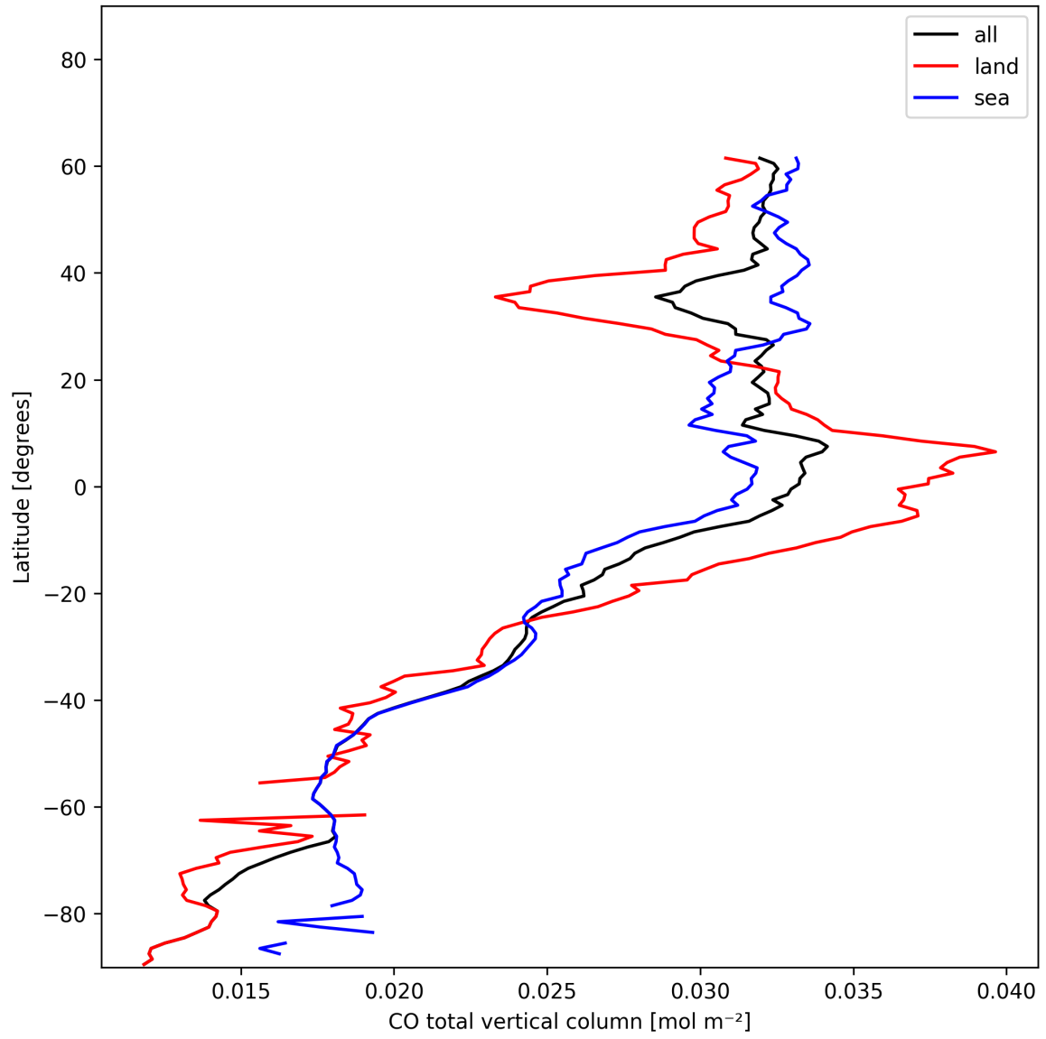
Figure 7: Zonal average of “CO total vertical column” for 2024-12-14 to 2024-12-14.
