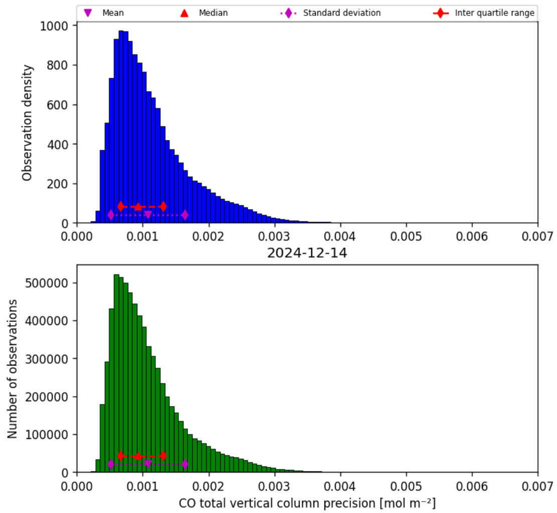
Figure 15: Histogram of “CO total vertical column precision” for 2024-12-14 to 2024-12-14
