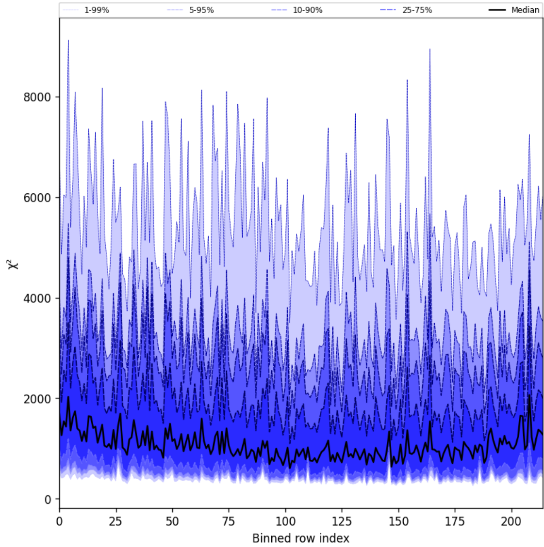
Figure 24: Along track statistics of “ \chi^2 ” for 2024-12-14 to 2024-12-14
