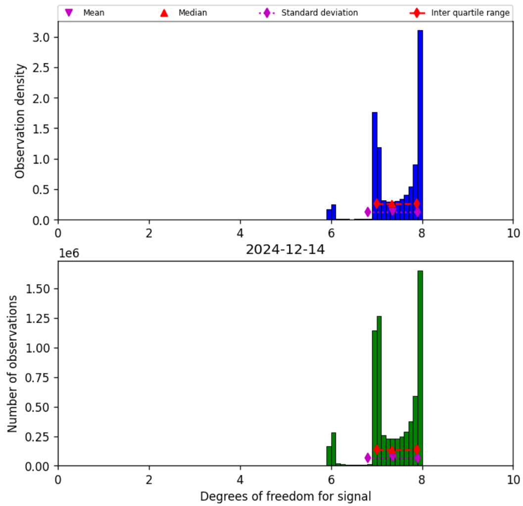
Figure 18: Histogram of “Degrees of freedom for signal” for 2024-12-14 to 2024-12-14
