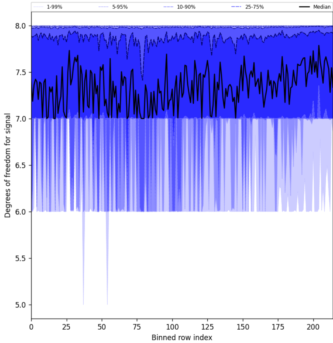
Figure 25: Along track statistics of “Degrees of freedom for signal” for 2024-12-14 to 2024-12-14
