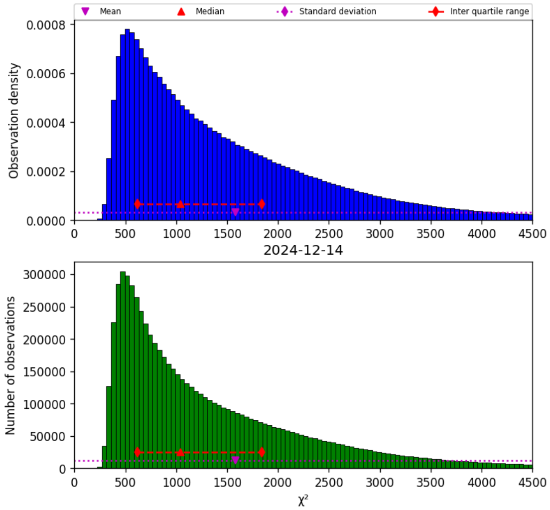
Figure 17: Histogram of " \chi^2 " for 2024-12-14 to 2024-12-14
