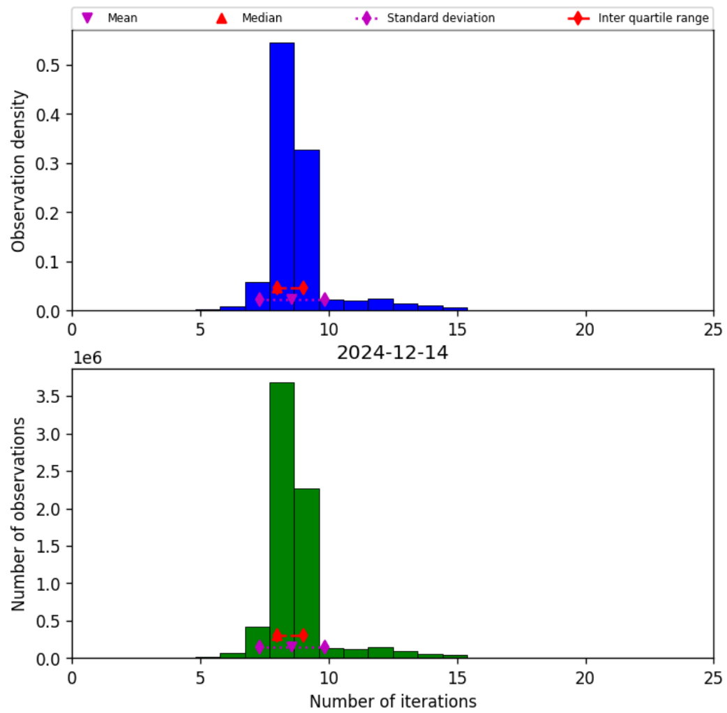
Figure 19: Histogram of “Number of iterations” for 2024-12-14 to 2024-12-14
