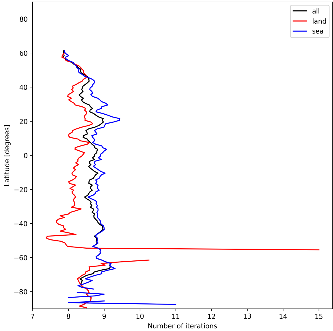
Figure 12: Zonal average of “Number of iterations” for 2024-12-14 to 2024-12-14.
