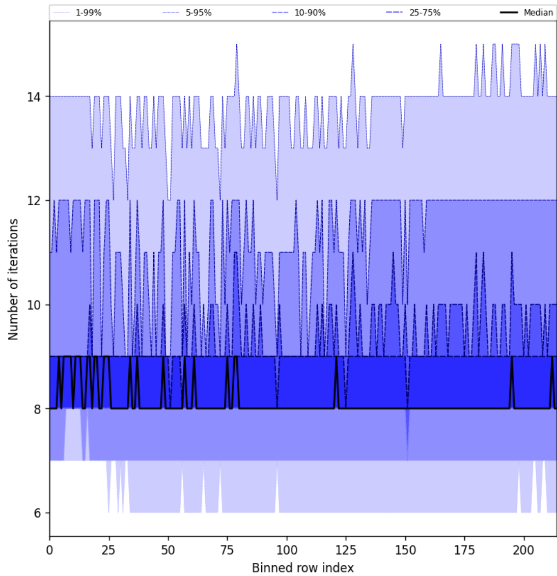
Figure 26: Along track statistics of “Number of iterations” for 2024-12-14 to 2024-12-14
