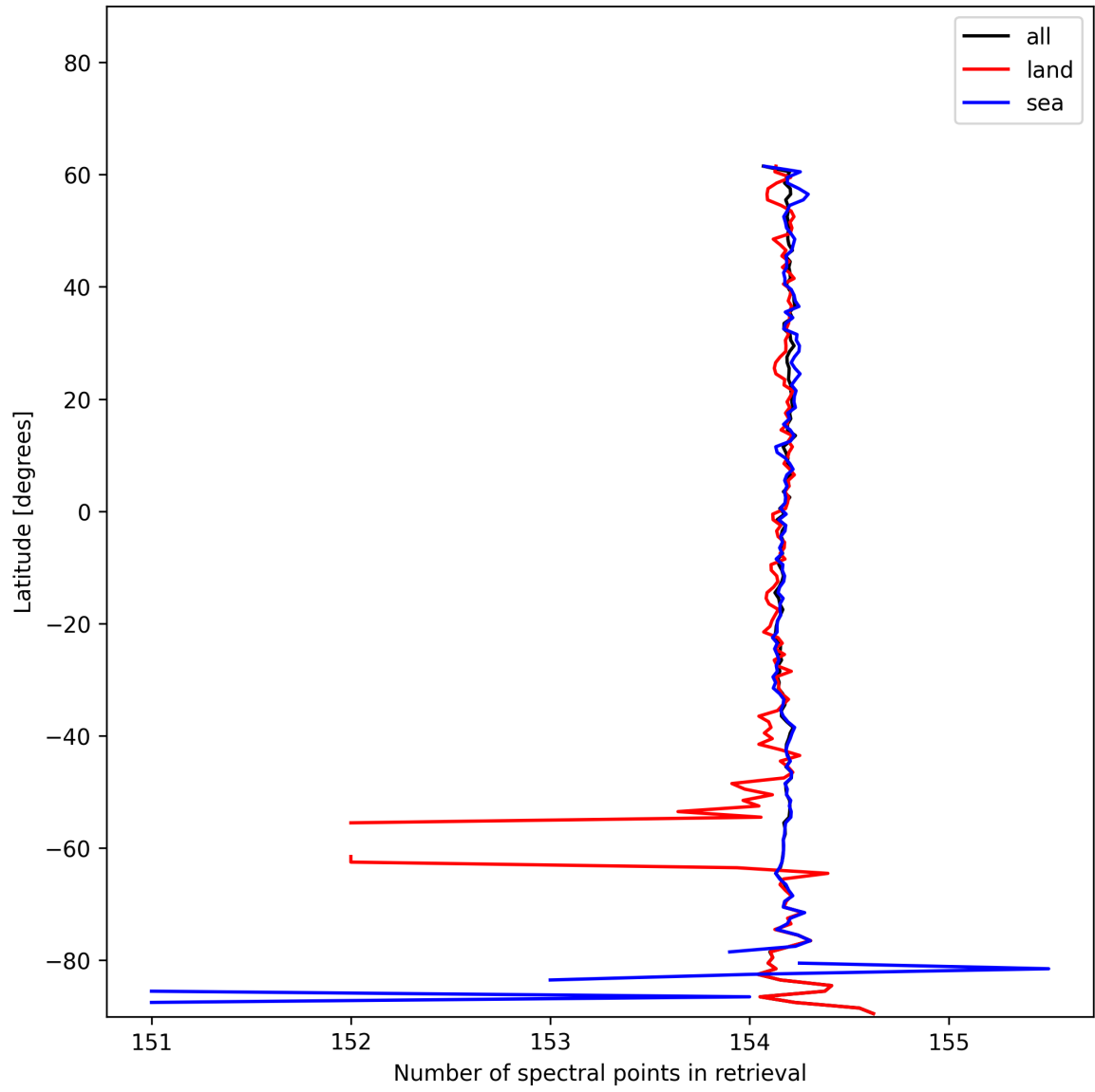
Figure 9: Zonal average of “Number of spectral points in retrieval” for 2024-12-14 to 2024-12-14.
