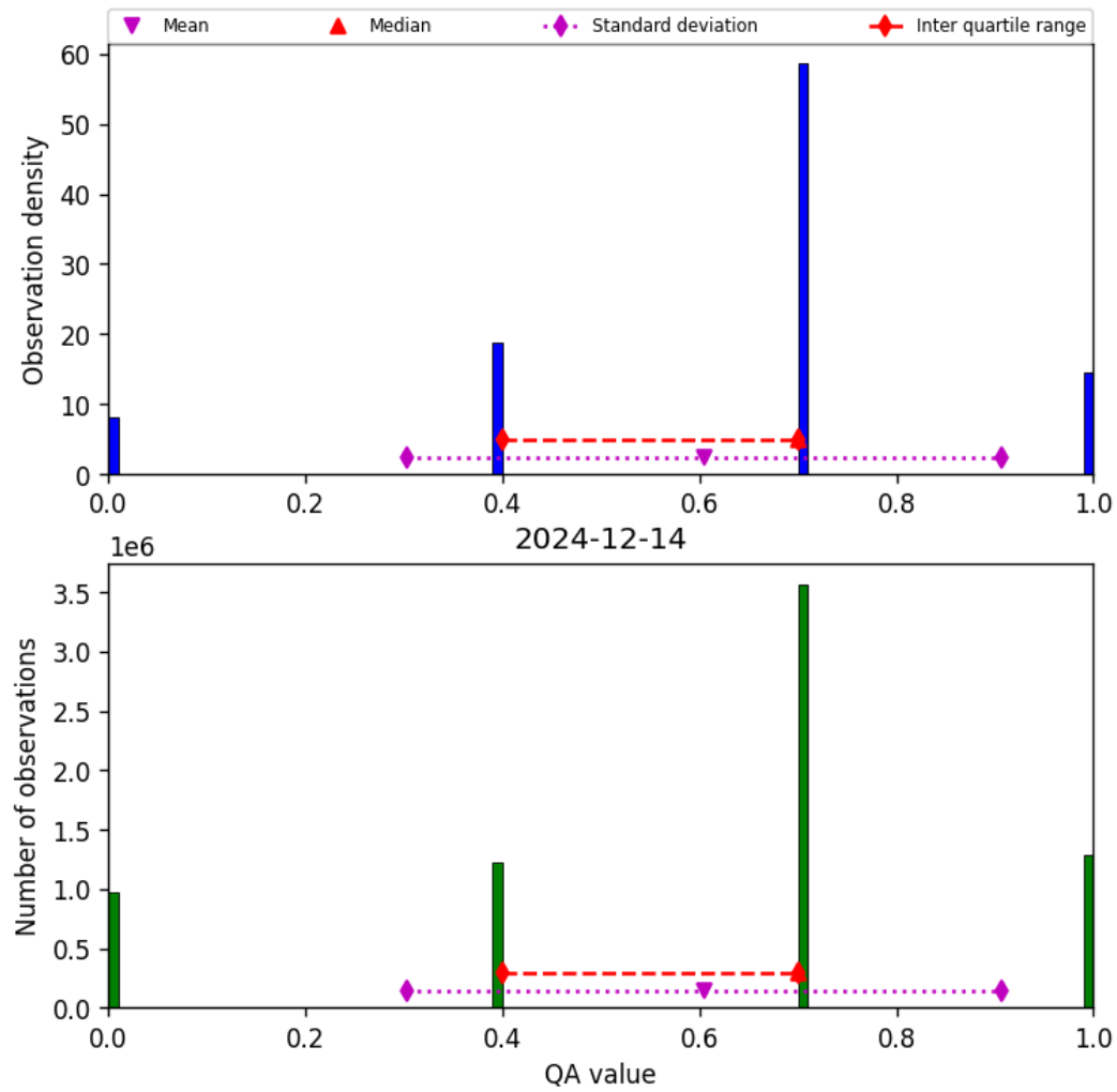
Figure 13: Histogram of “QA value” for 2024-12-14 to 2024-12-14
