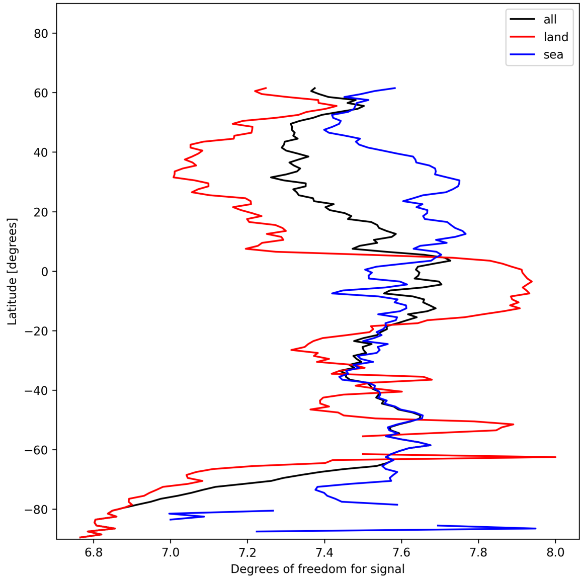
Figure 11: Zonal average of “Degrees of freedom for signal” for 2024-12-14 to 2024-12-14.
