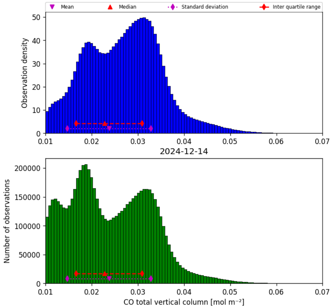
Figure 14: Histogram of “CO total vertical column” for 2024-12-14 to 2024-12-14
