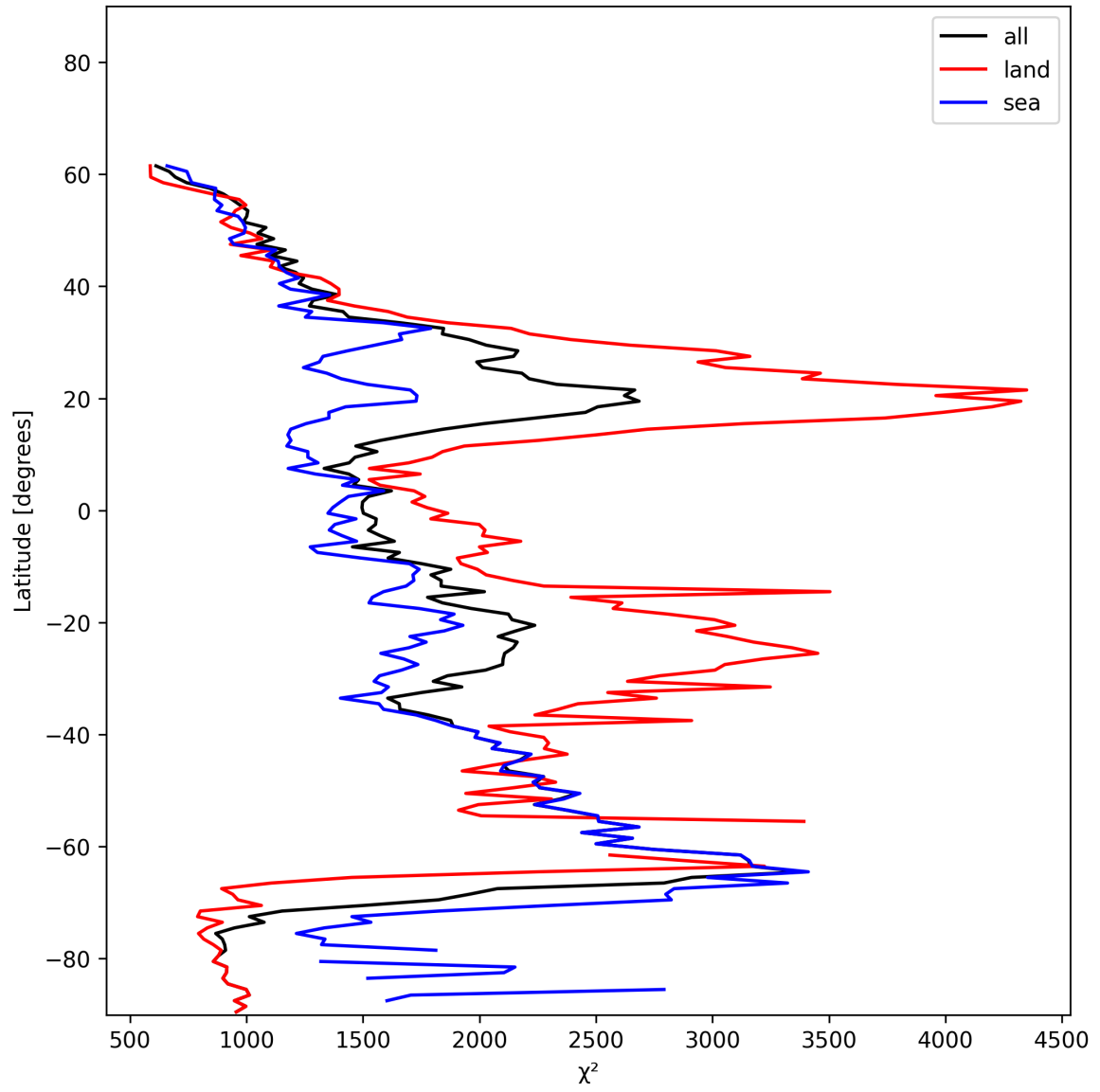
Figure 10: Zonal average of “ \chi^2 ” for 2024-12-14 to 2024-12-14.
