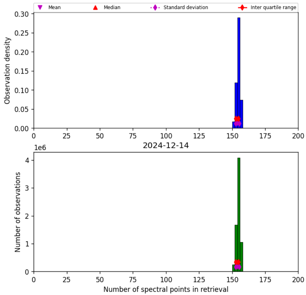
Figure 16: Histogram of “Number of spectral points in retrieval” for 2024-12-14 to 2024-12-14
