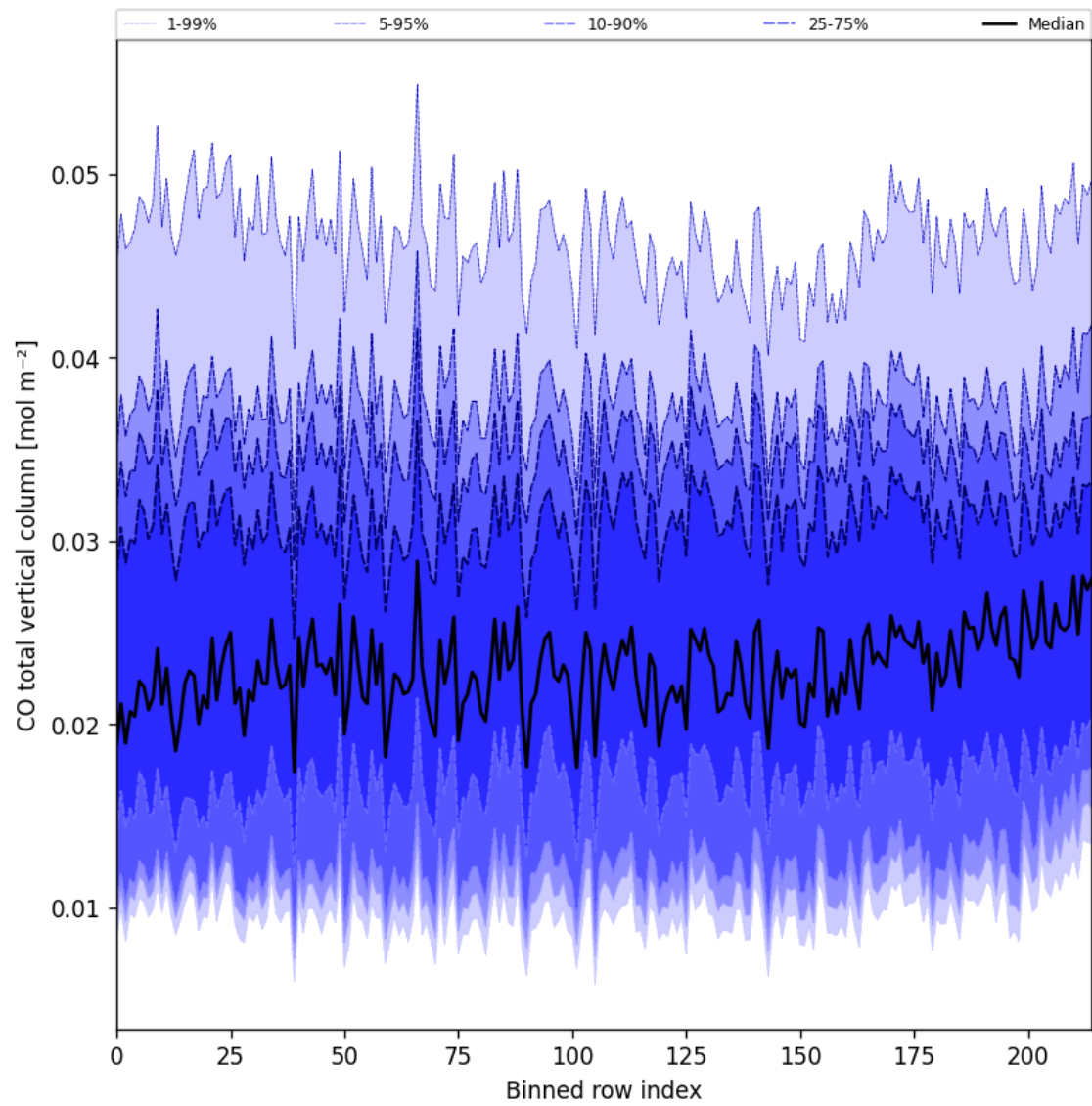
Figure 21: Along track statistics of “CO total vertical column” for 2024-12-14 to 2024-12-14
