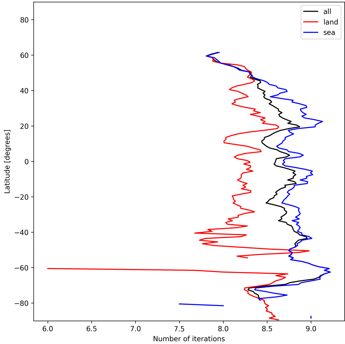
Figure 12: Zonal average of “Number of iterations” for 2024-12-15 to 2024-12-16.
