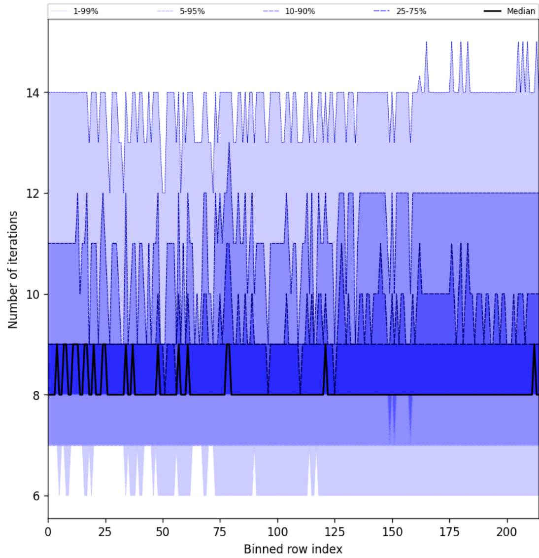
Figure 26: Along track statistics of “Number of iterations” for 2024-12-15 to 2024-12-16
