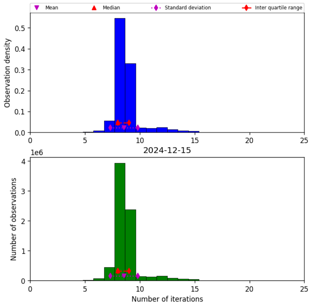
Figure 19: Histogram of “Number of iterations” for 2024-12-15 to 2024-12-16
