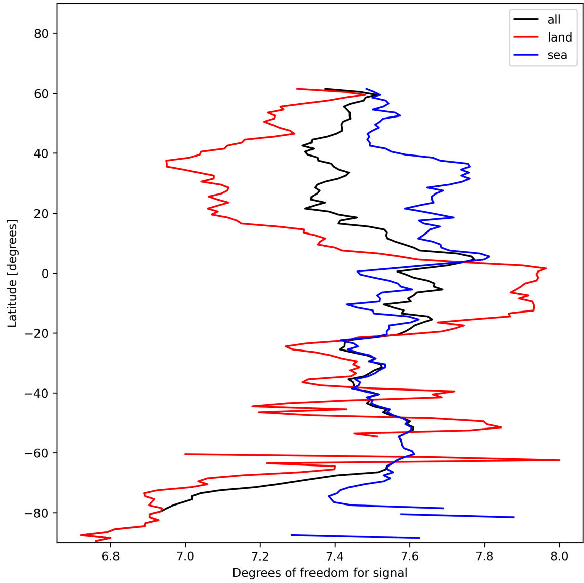
Figure 11: Zonal average of “Degrees of freedom for signal” for 2024-12-15 to 2024-12-16.
