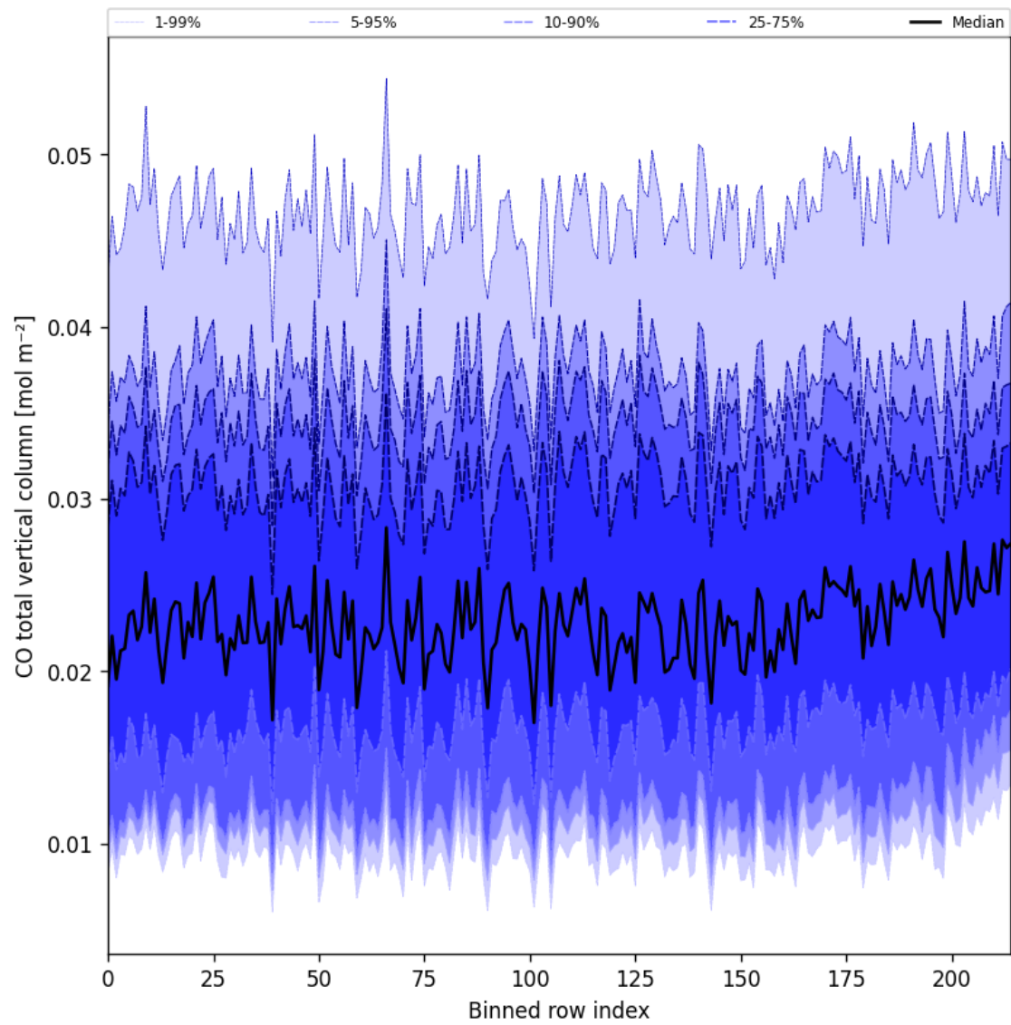
Figure 21: Along track statistics of “CO total vertical column” for 2024-12-15 to 2024-12-16
