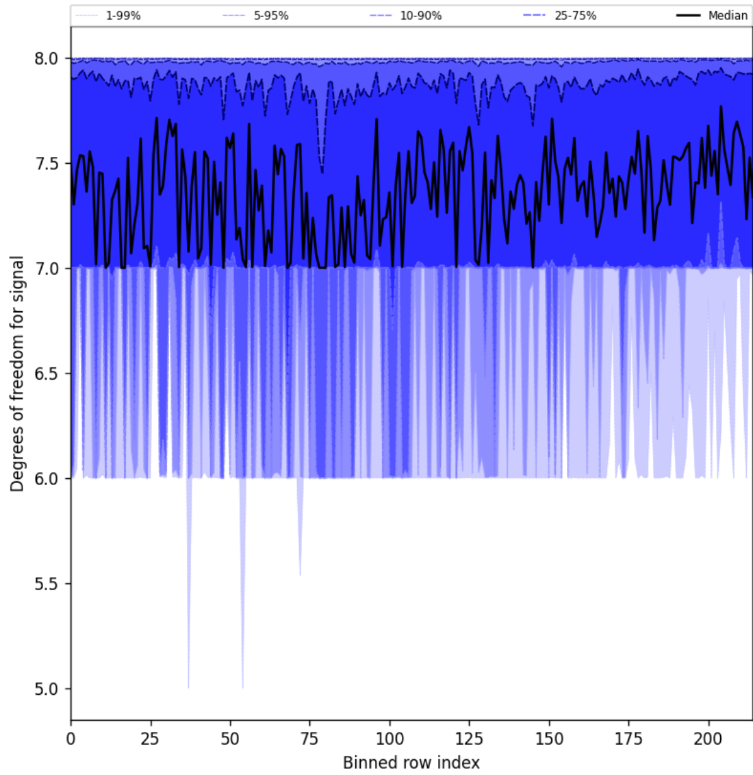
Figure 25: Along track statistics of “Degrees of freedom for signal” for 2024-12-15 to 2024-12-16
