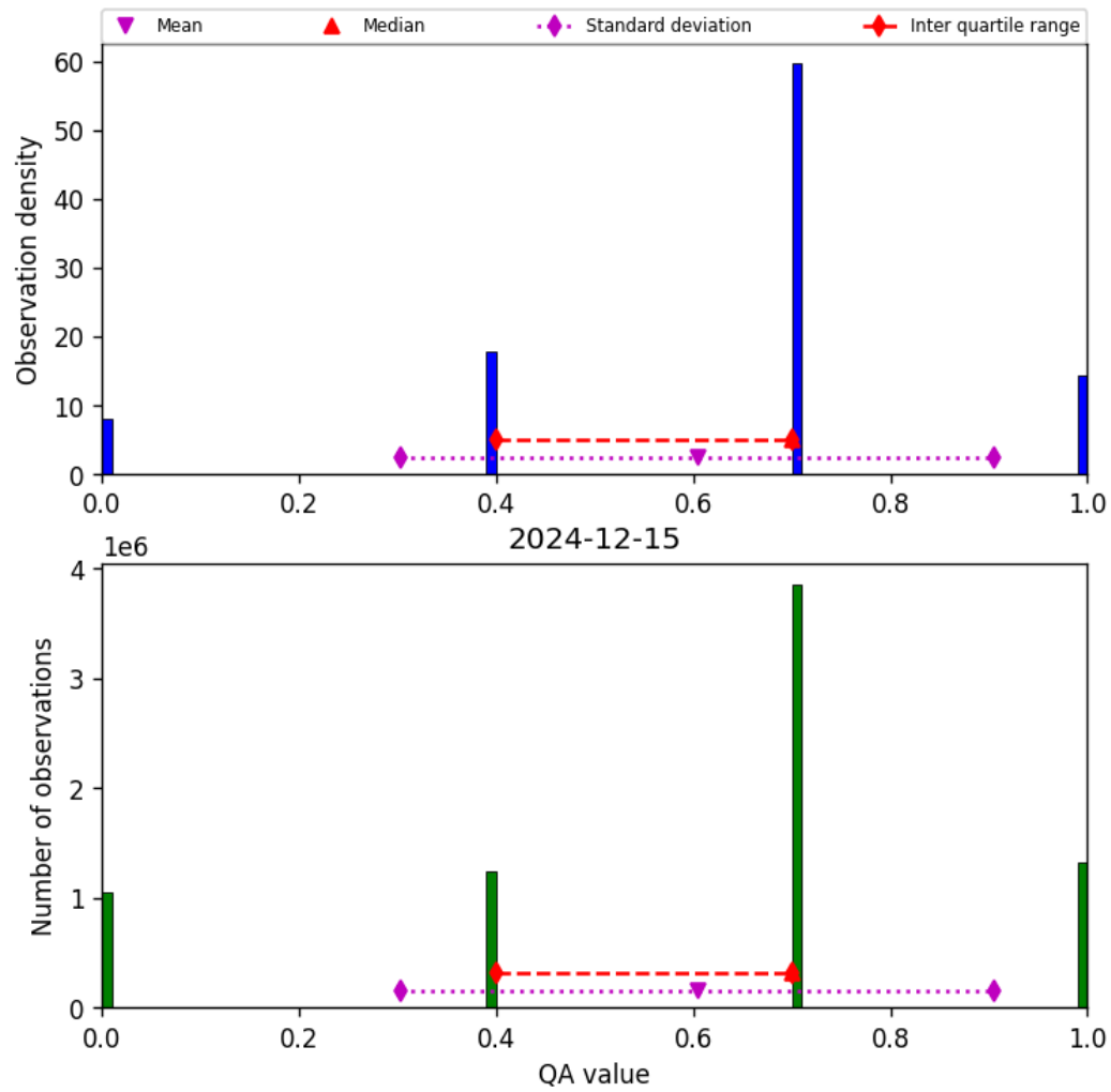
Figure 13: Histogram of “QA value” for 2024-12-15 to 2024-12-16
