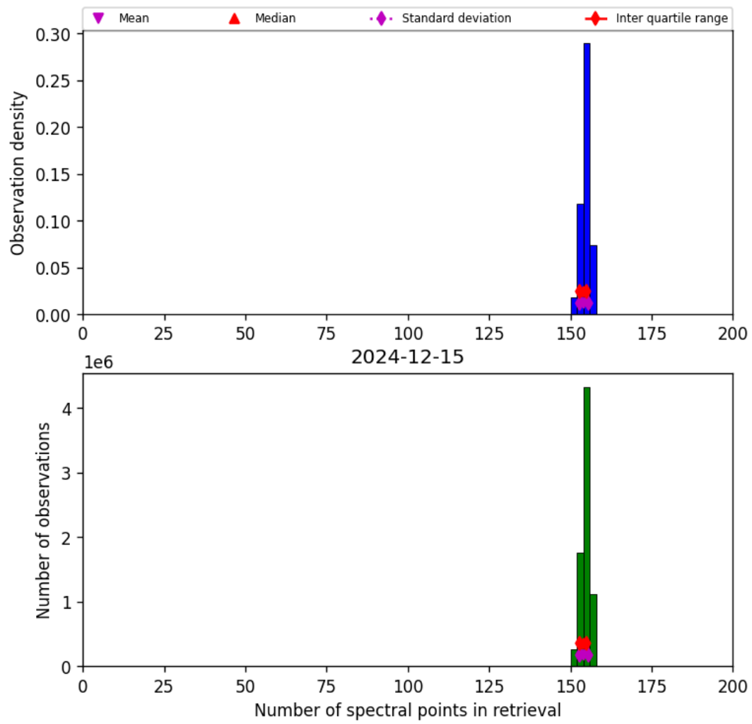
Figure 16: Histogram of “Number of spectral points in retrieval” for 2024-12-15 to 2024-12-16
