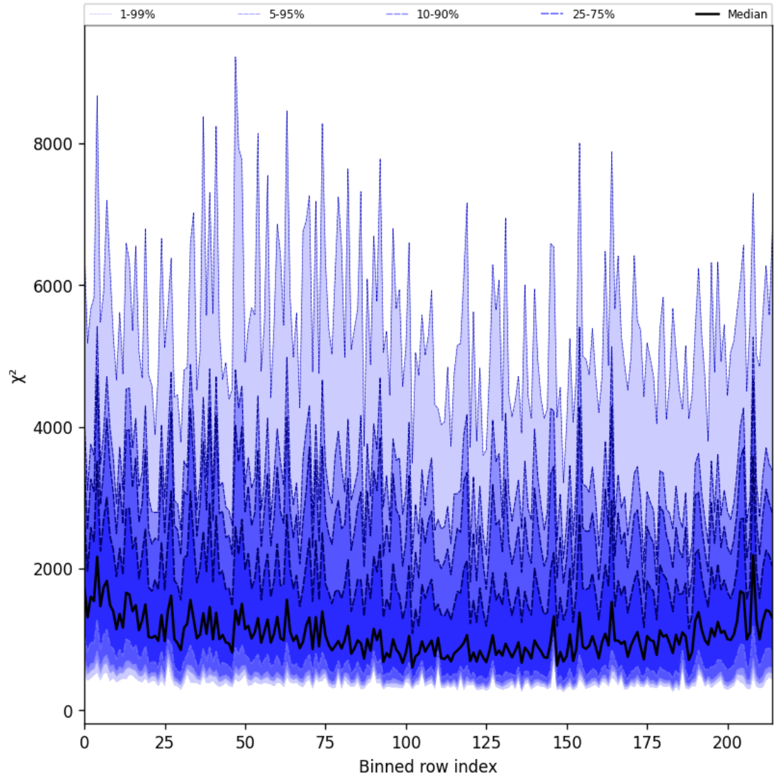
Figure 24: Along track statistics of “ \chi^2 ” for 2024-12-15 to 2024-12-16
