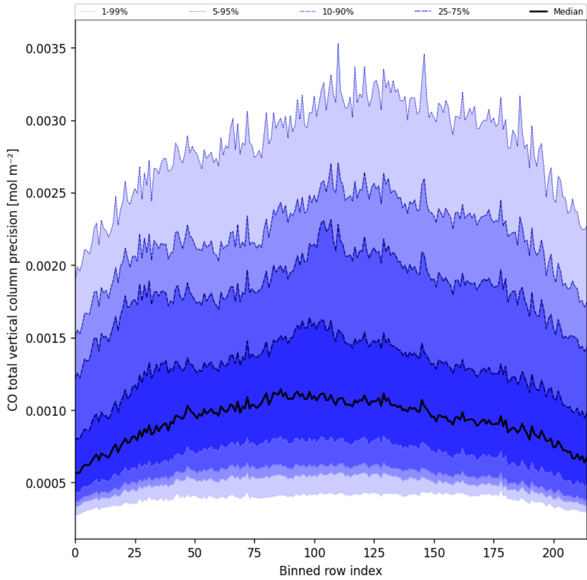
Figure 22: Along track statistics of “CO total vertical column precision” for 2024-12-15 to 2024-12-16
