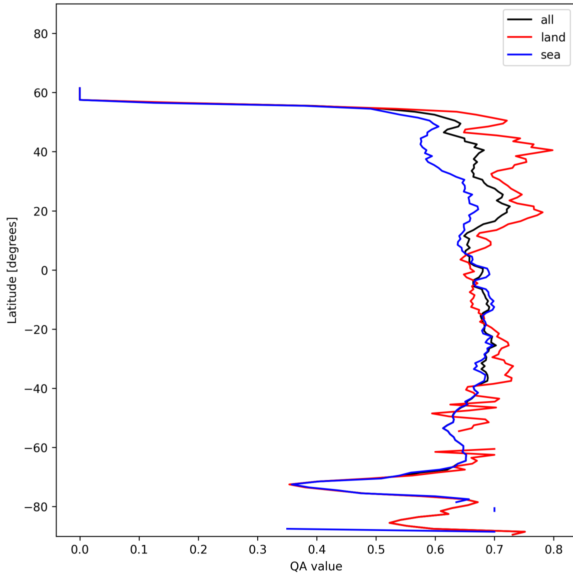
Figure 6: Zonal average of “QA value” for 2024-12-15 to 2024-12-16.
