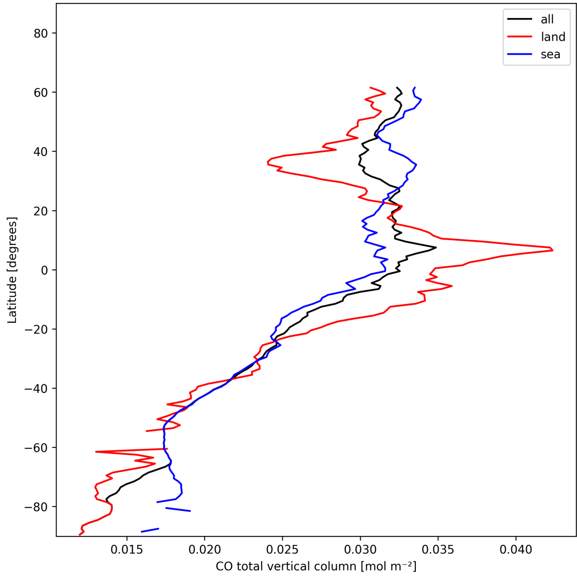
Figure 7: Zonal average of “CO total vertical column” for 2024-12-15 to 2024-12-16.
