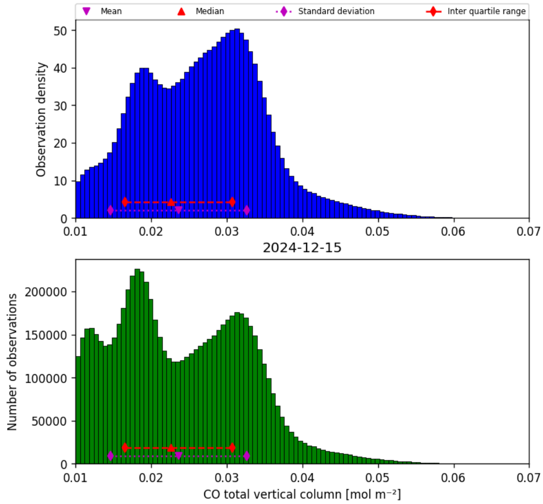
Figure 14: Histogram of “CO total vertical column” for 2024-12-15 to 2024-12-16
