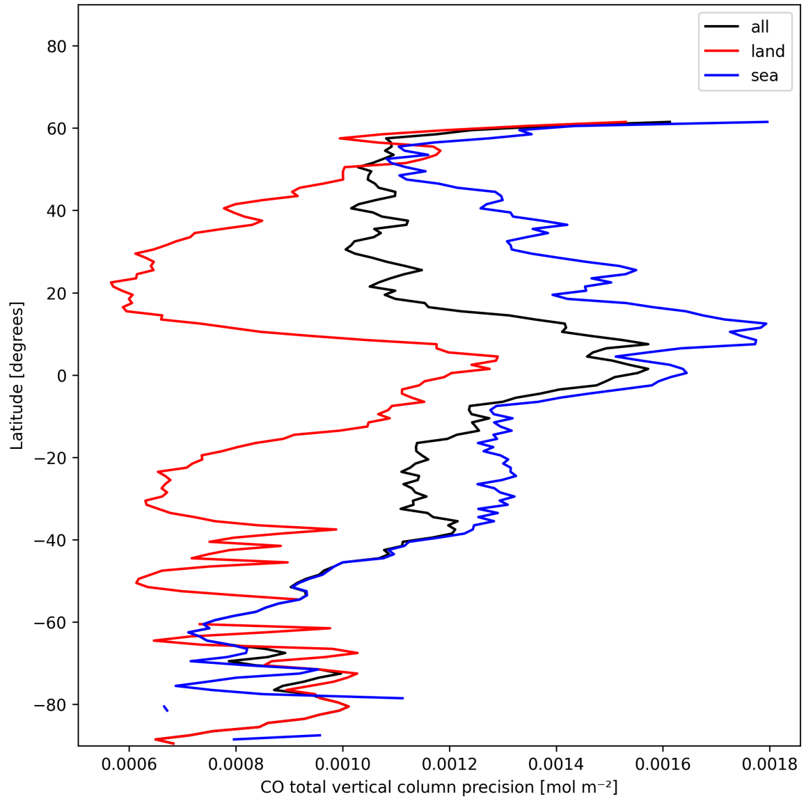
Figure 8: Zonal average of “CO total vertical column precision” for 2024-12-15 to 2024-12-16.
