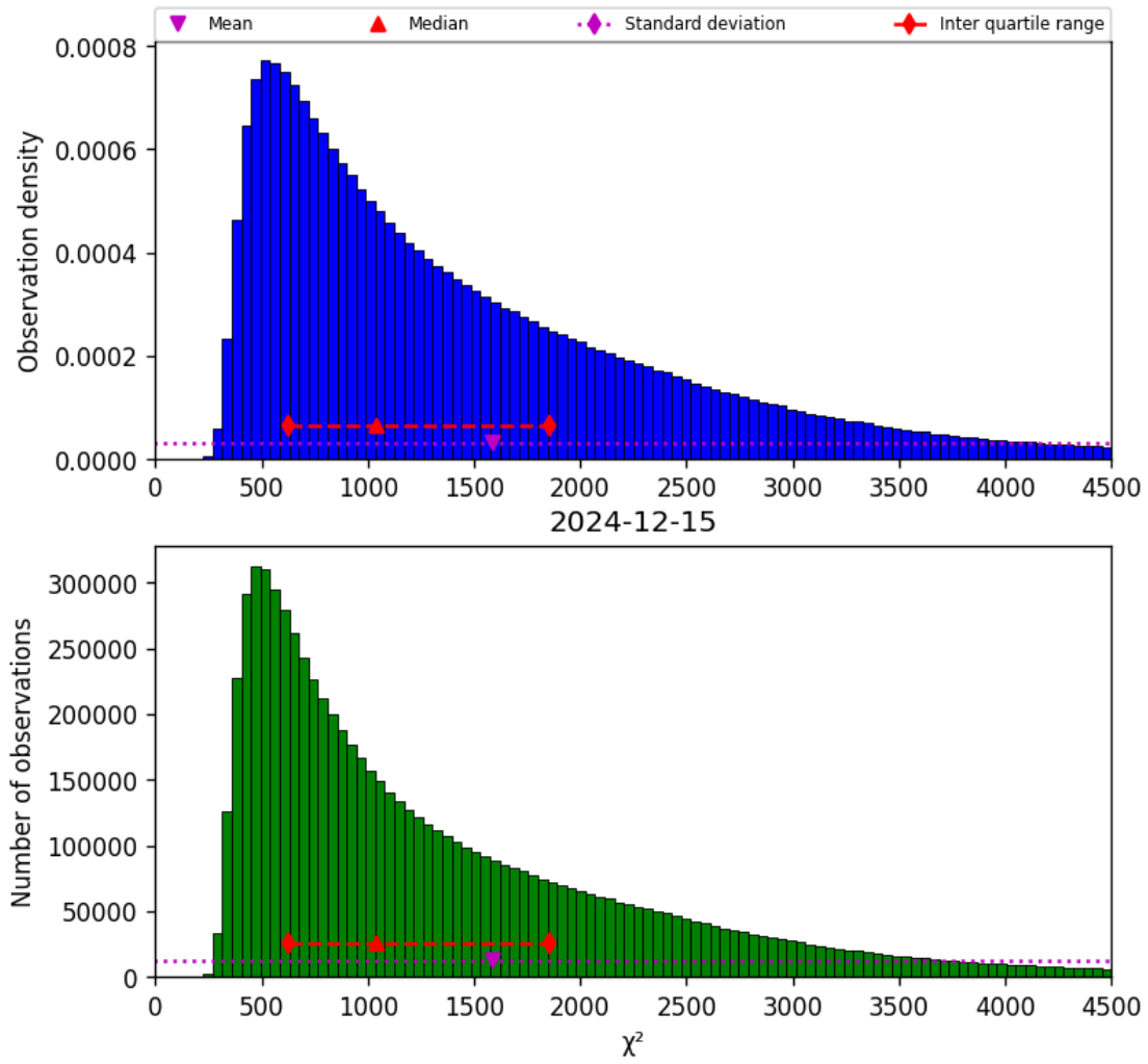
Figure 17: Histogram of “ \chi^2 ” for 2024-12-15 to 2024-12-16
