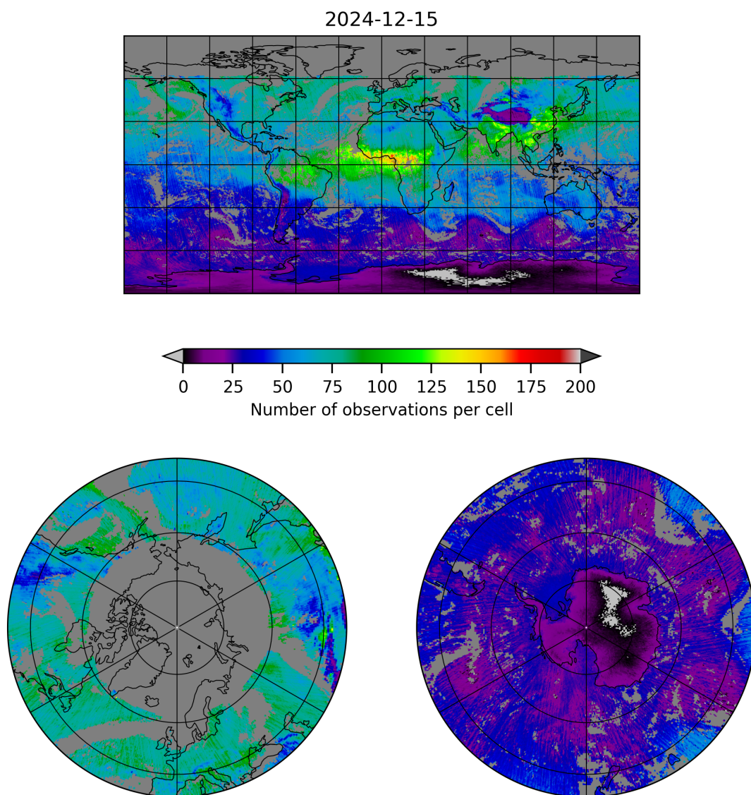
Figure 5: Map of the number of observations for 2024-12-15 to 2024-12-16
