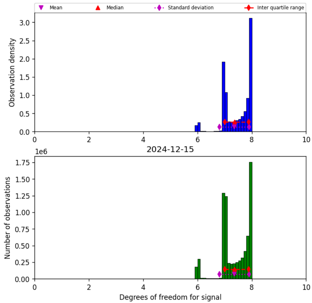
Figure 18: Histogram of “Degrees of freedom for signal” for 2024-12-15 to 2024-12-16
