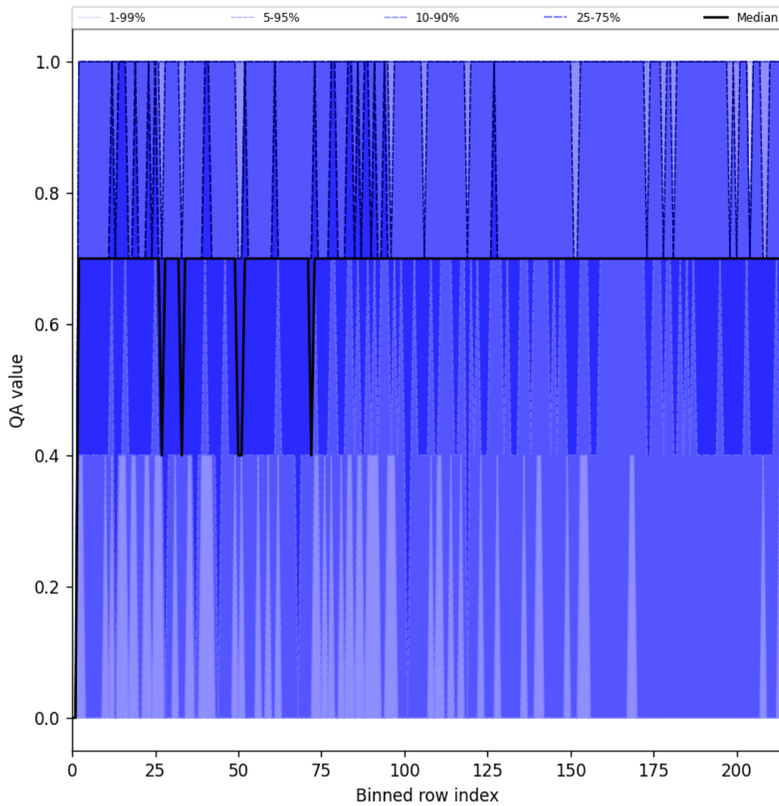
Figure 20: Along track statistics of “QA value” for 2024-12-15 to 2024-12-16
