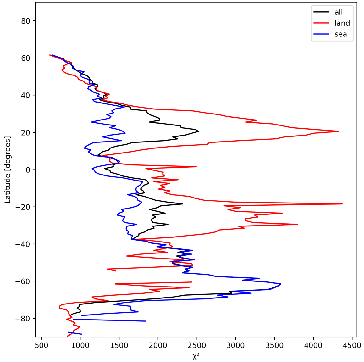
Figure 10: Zonal average of “ \chi^2 ” for 2024-12-15 to 2024-12-16.
