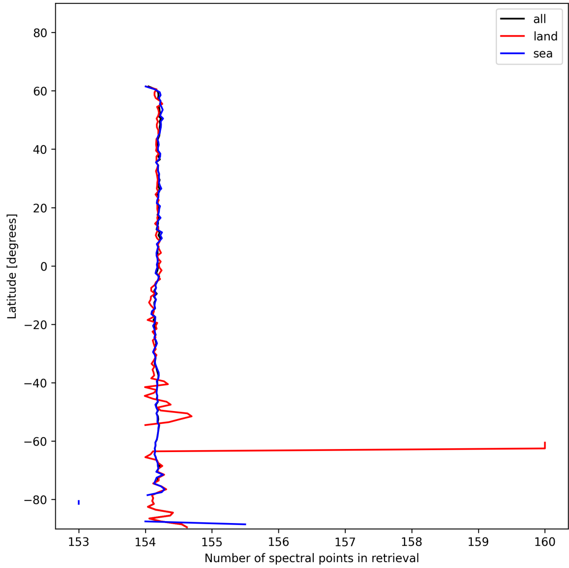
Figure 9: Zonal average of “Number of spectral points in retrieval” for 2024-12-15 to 2024-12-16.
