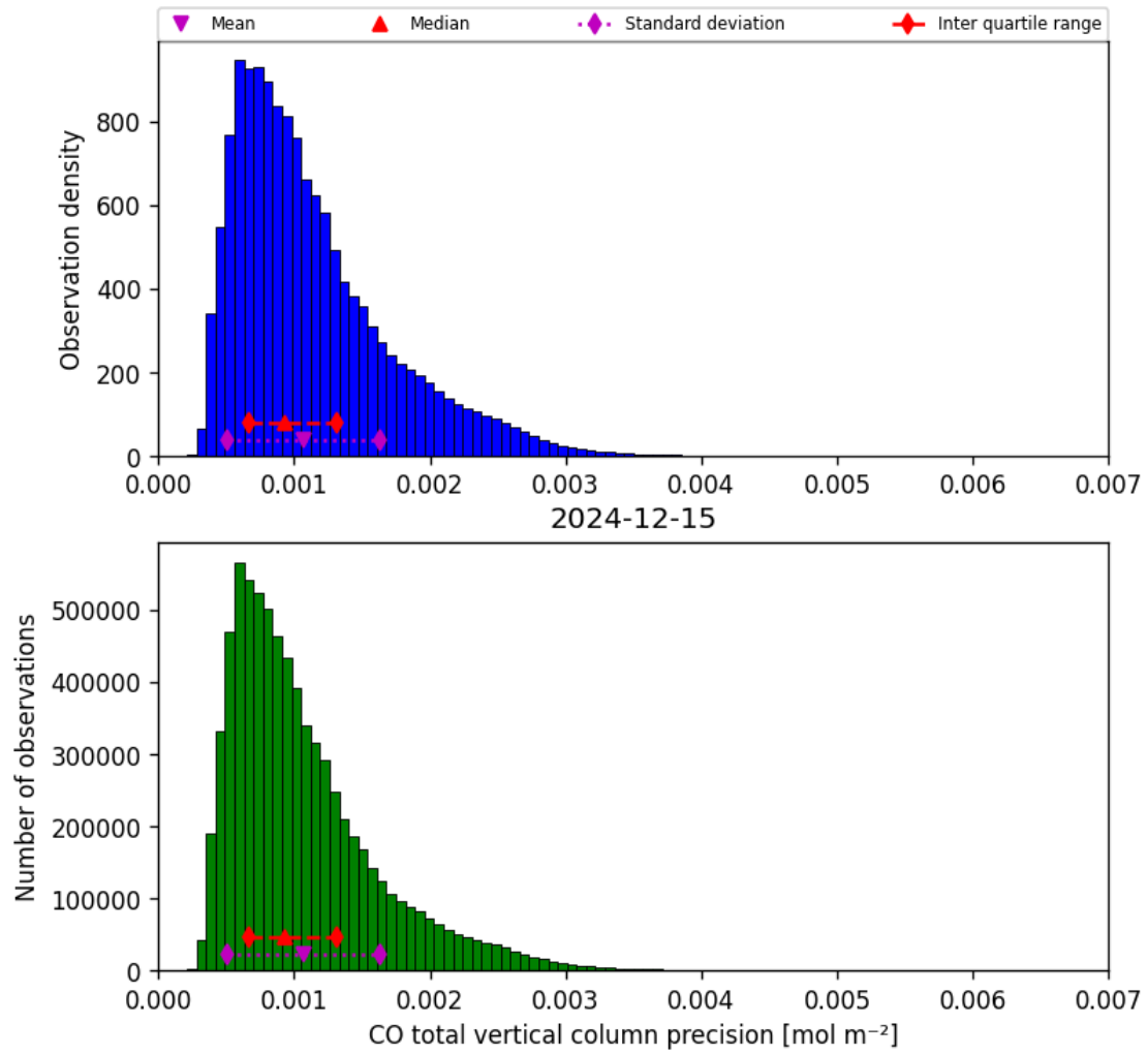
Figure 15: Histogram of “CO total vertical column precision” for 2024-12-15 to 2024-12-16
