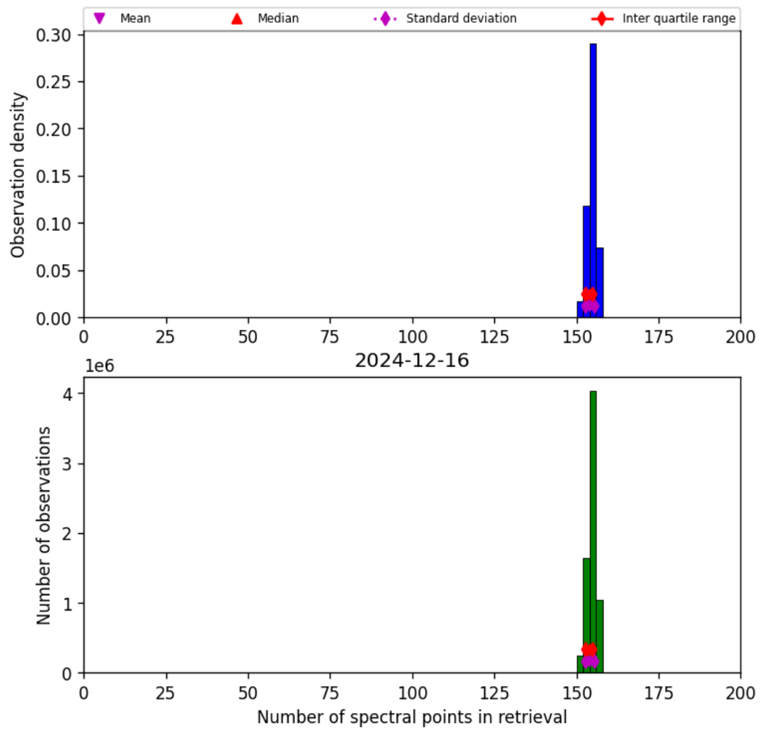
Figure 16: Histogram of “Number of spectral points in retrieval” for 2024-12-16 to 2024-12-17
