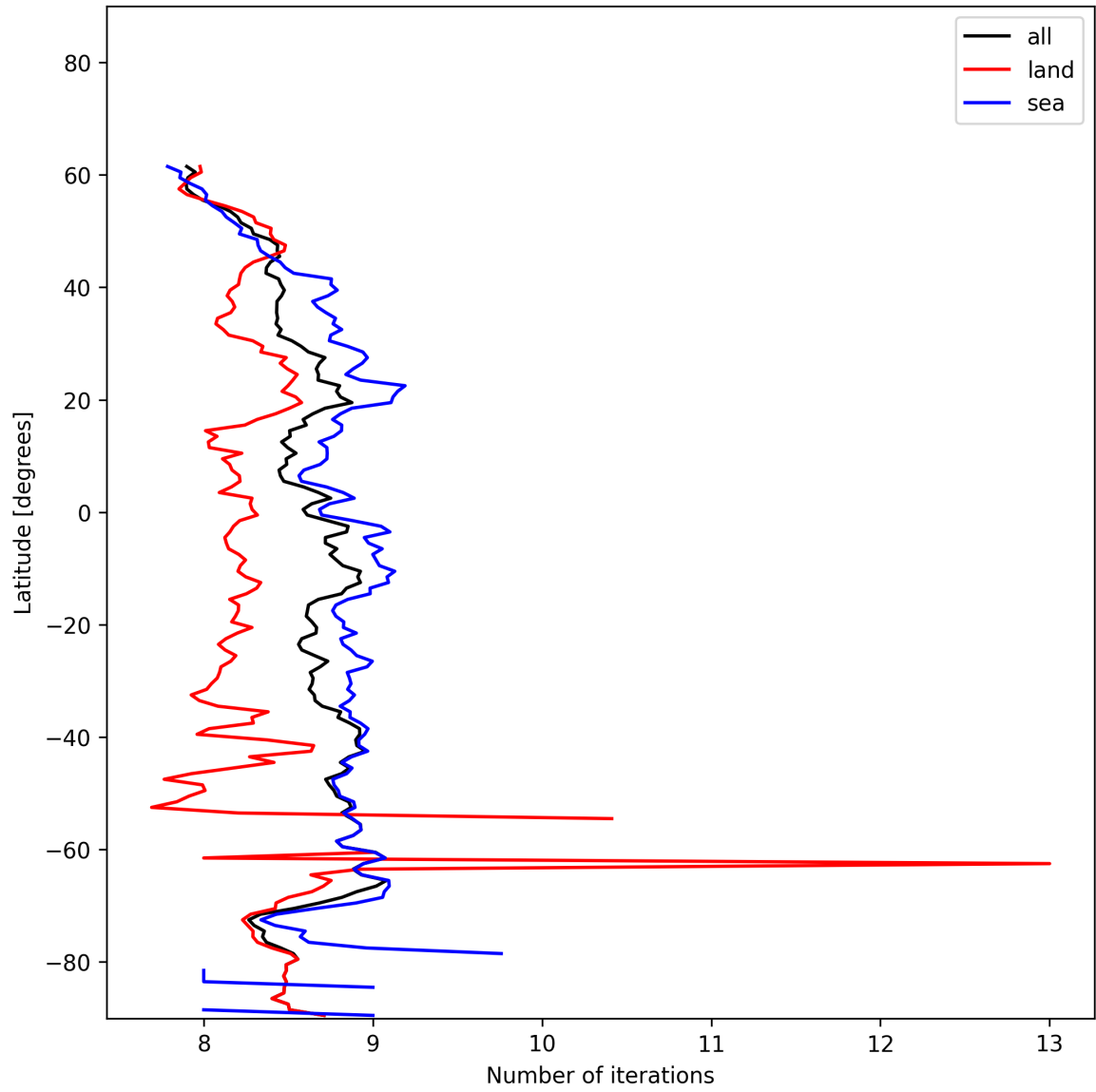
Figure 12: Zonal average of “Number of iterations” for 2024-12-16 to 2024-12-17.
