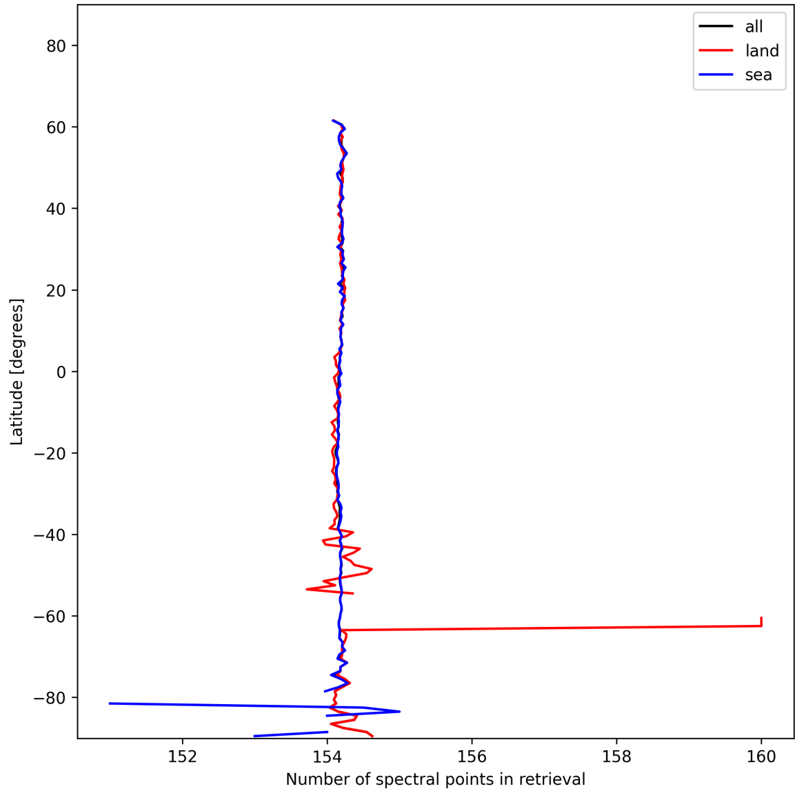
Figure 9: Zonal average of “Number of spectral points in retrieval” for 2024-12-16 to 2024-12-17.
