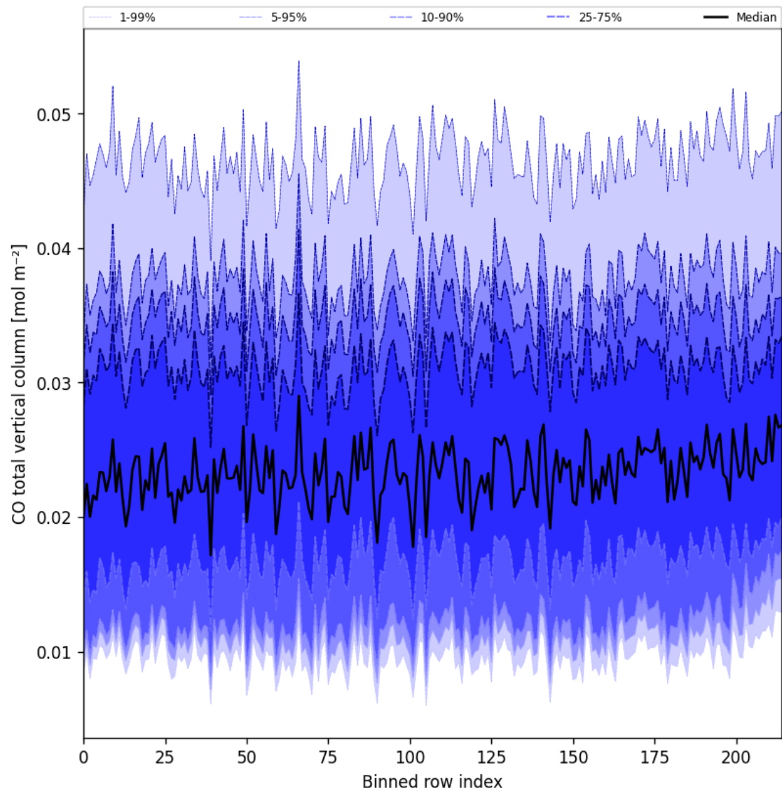
Figure 21: Along track statistics of “CO total vertical column” for 2024-12-16 to 2024-12-17
