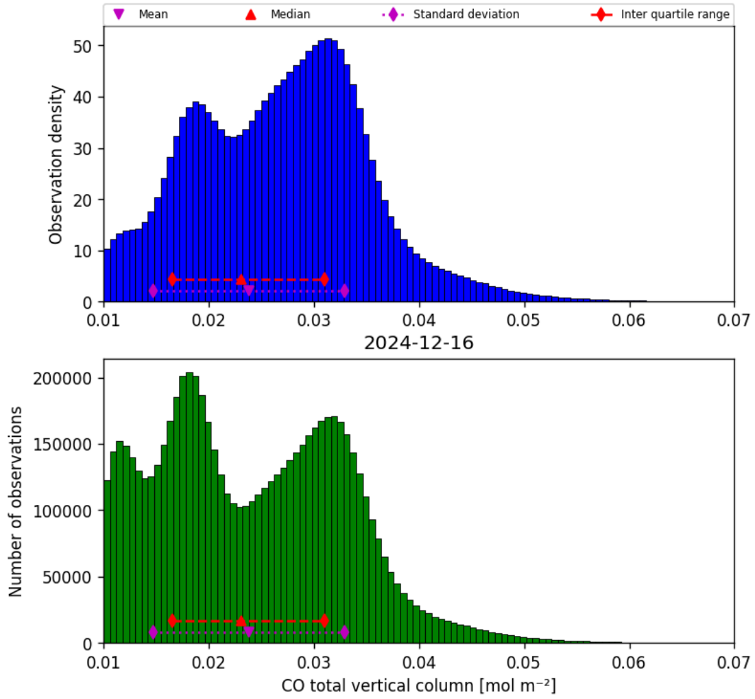
Figure 14: Histogram of “CO total vertical column” for 2024-12-16 to 2024-12-17
