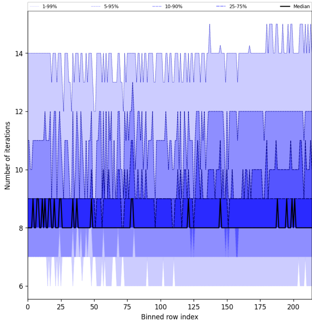
Figure 26: Along track statistics of “Number of iterations” for 2024-12-16 to 2024-12-17
