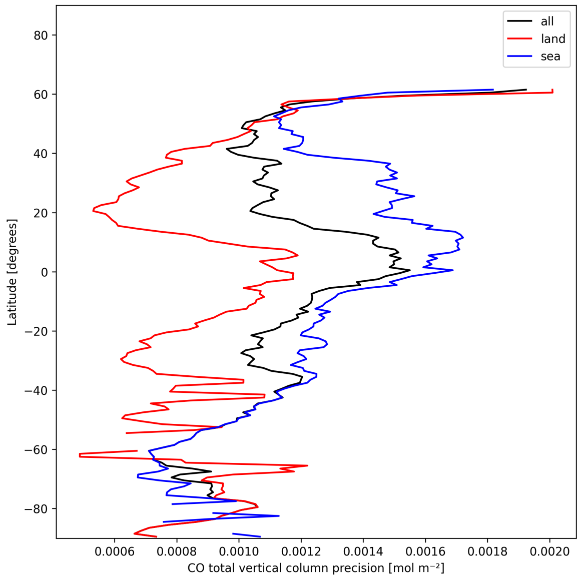
Figure 8: Zonal average of “CO total vertical column precision” for 2024-12-16 to 2024-12-17.
