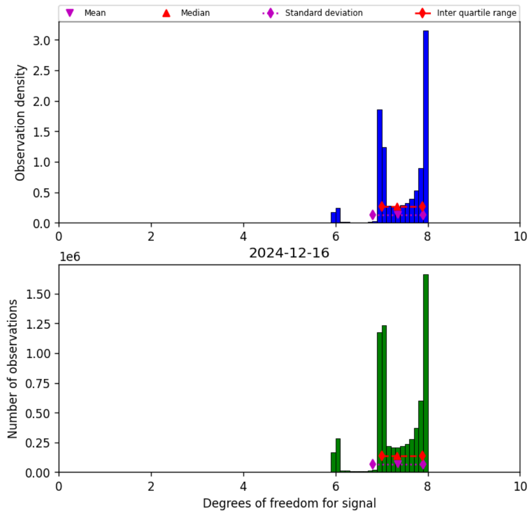
Figure 18: Histogram of “Degrees of freedom for signal” for 2024-12-16 to 2024-12-17
