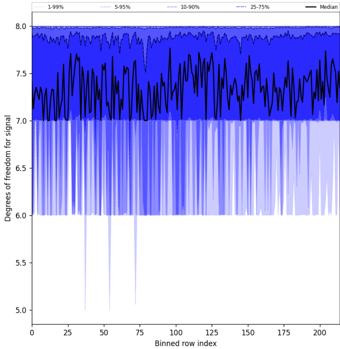
Figure 25: Along track statistics of “Degrees of freedom for signal” for 2024-12-16 to 2024-12-17
