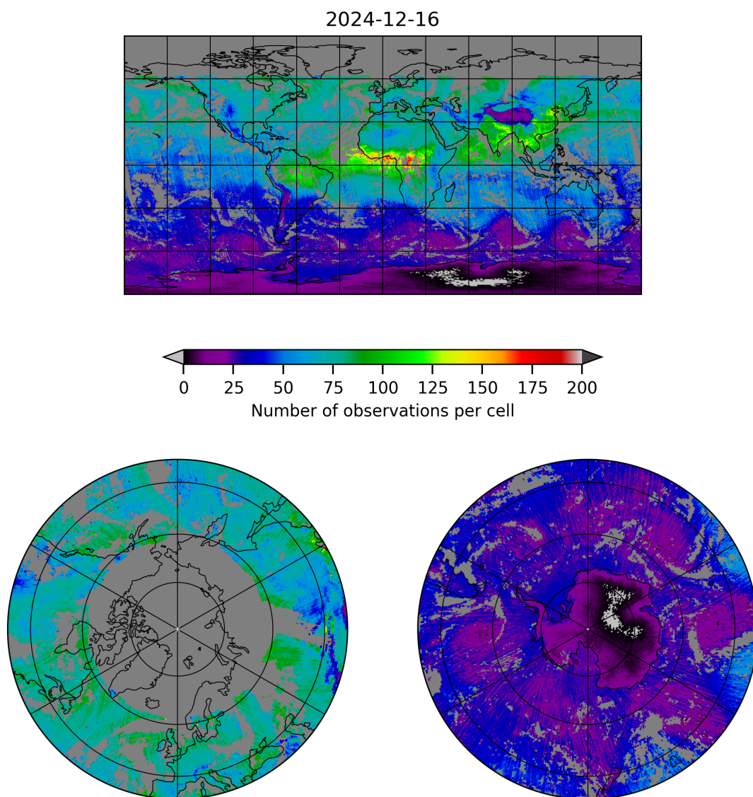
Figure 5: Map of the number of observations for 2024-12-16 to 2024-12-17
