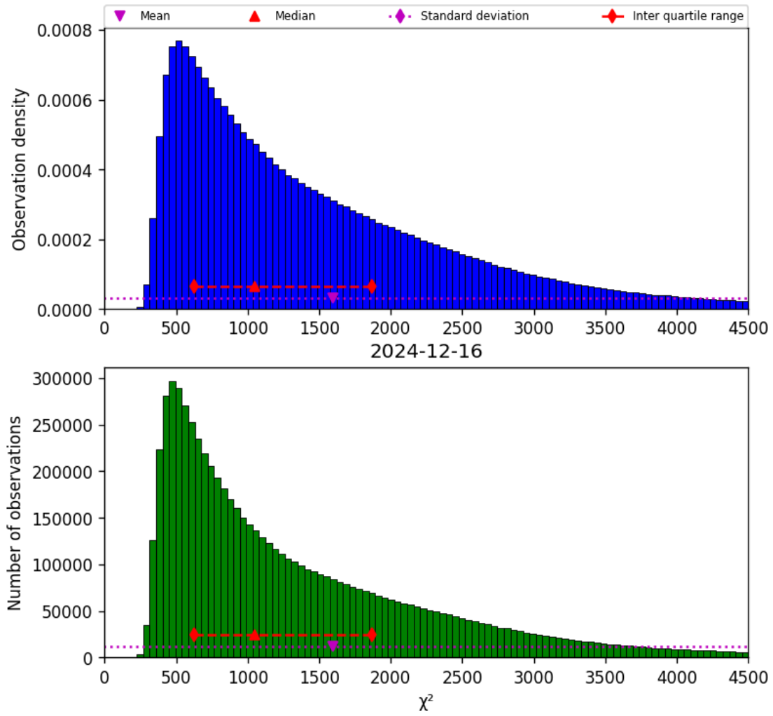
Figure 17: Histogram of “ \chi^2 ” for 2024-12-16 to 2024-12-17
