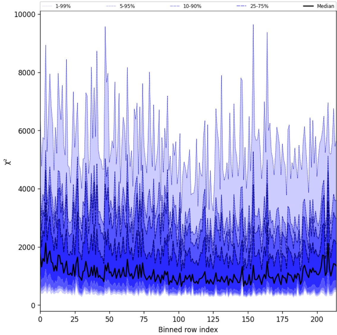
Figure 24: Along track statistics of “ \chi^2 ” for 2024-12-16 to 2024-12-17
