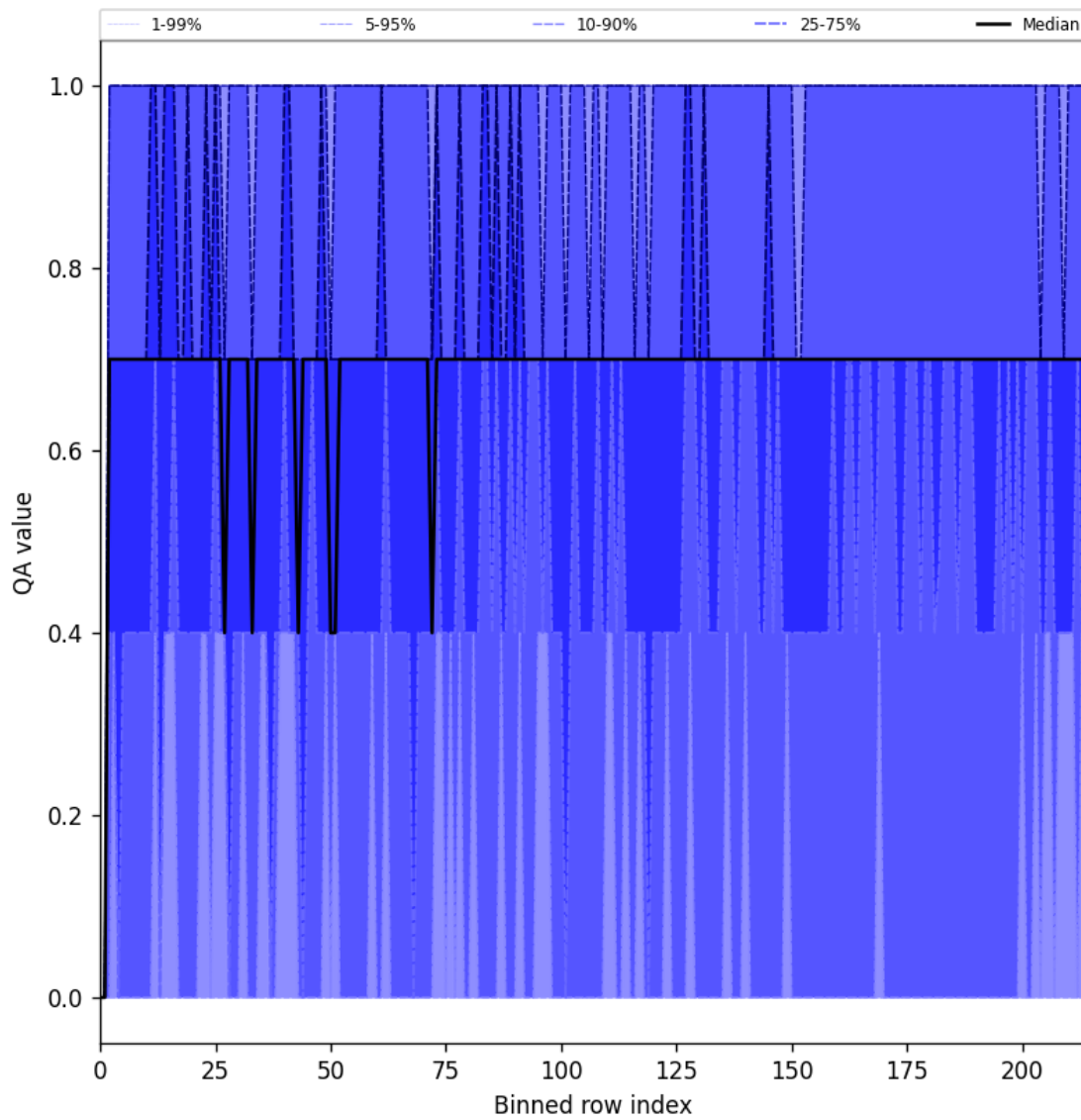
Figure 20: Along track statistics of “QA value” for 2024-12-16 to 2024-12-17
