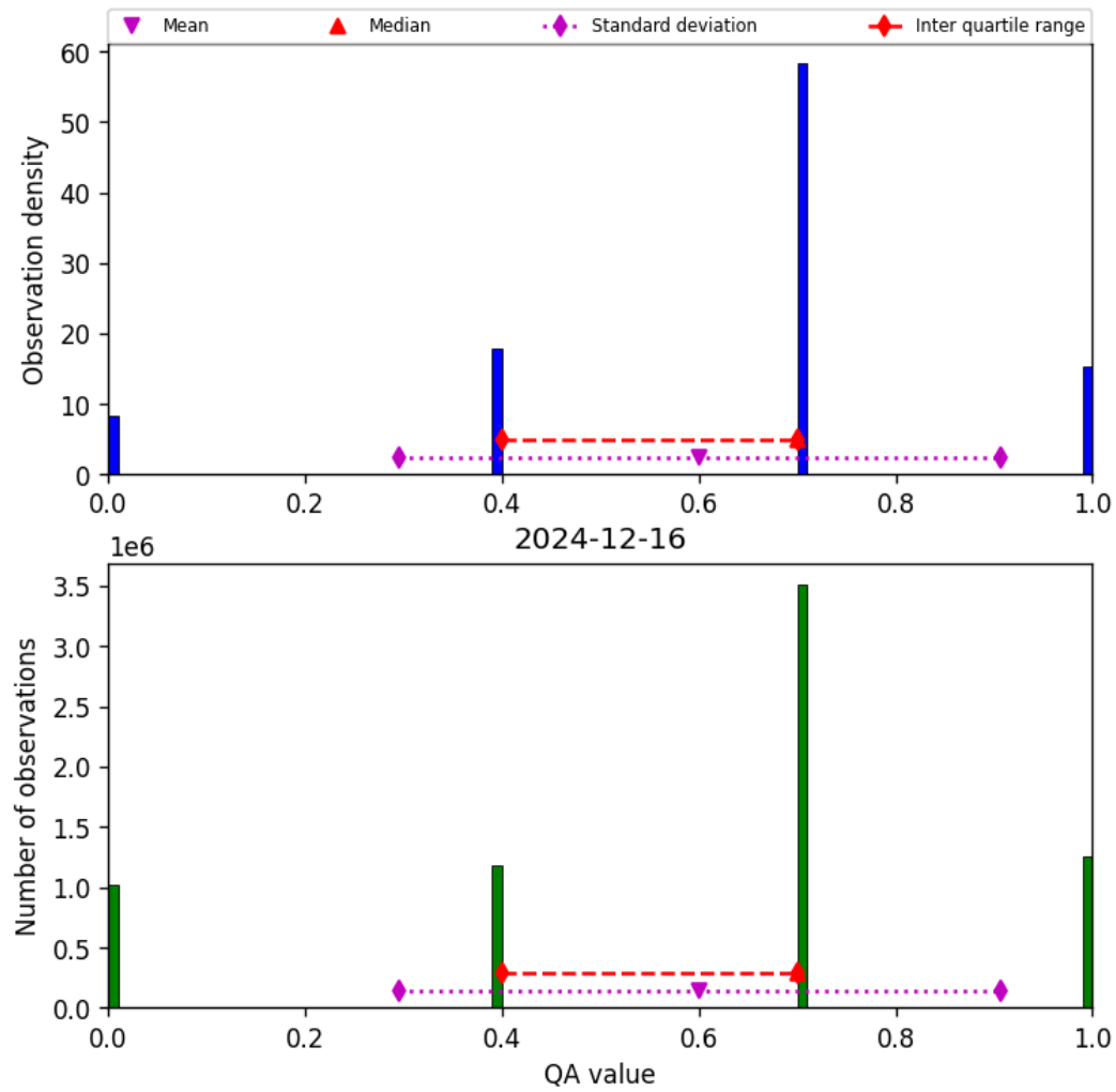
Figure 13: Histogram of “QA value” for 2024-12-16 to 2024-12-17
