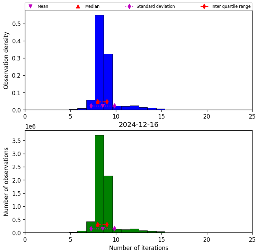
Figure 19: Histogram of “Number of iterations” for 2024-12-16 to 2024-12-17
