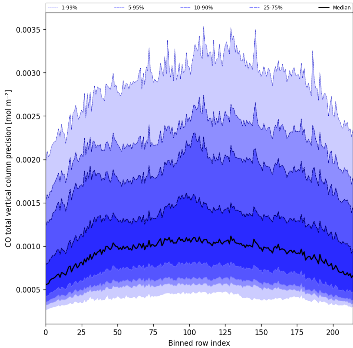
Figure 22: Along track statistics of “CO total vertical column precision” for 2024-12-16 to 2024-12-17
