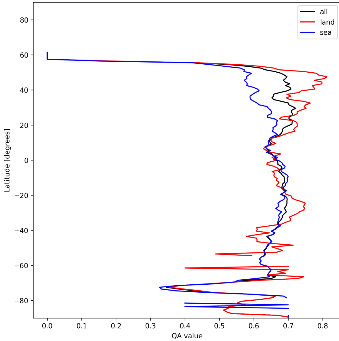
Figure 6: Zonal average of “QA value” for 2024-12-16 to 2024-12-17.
