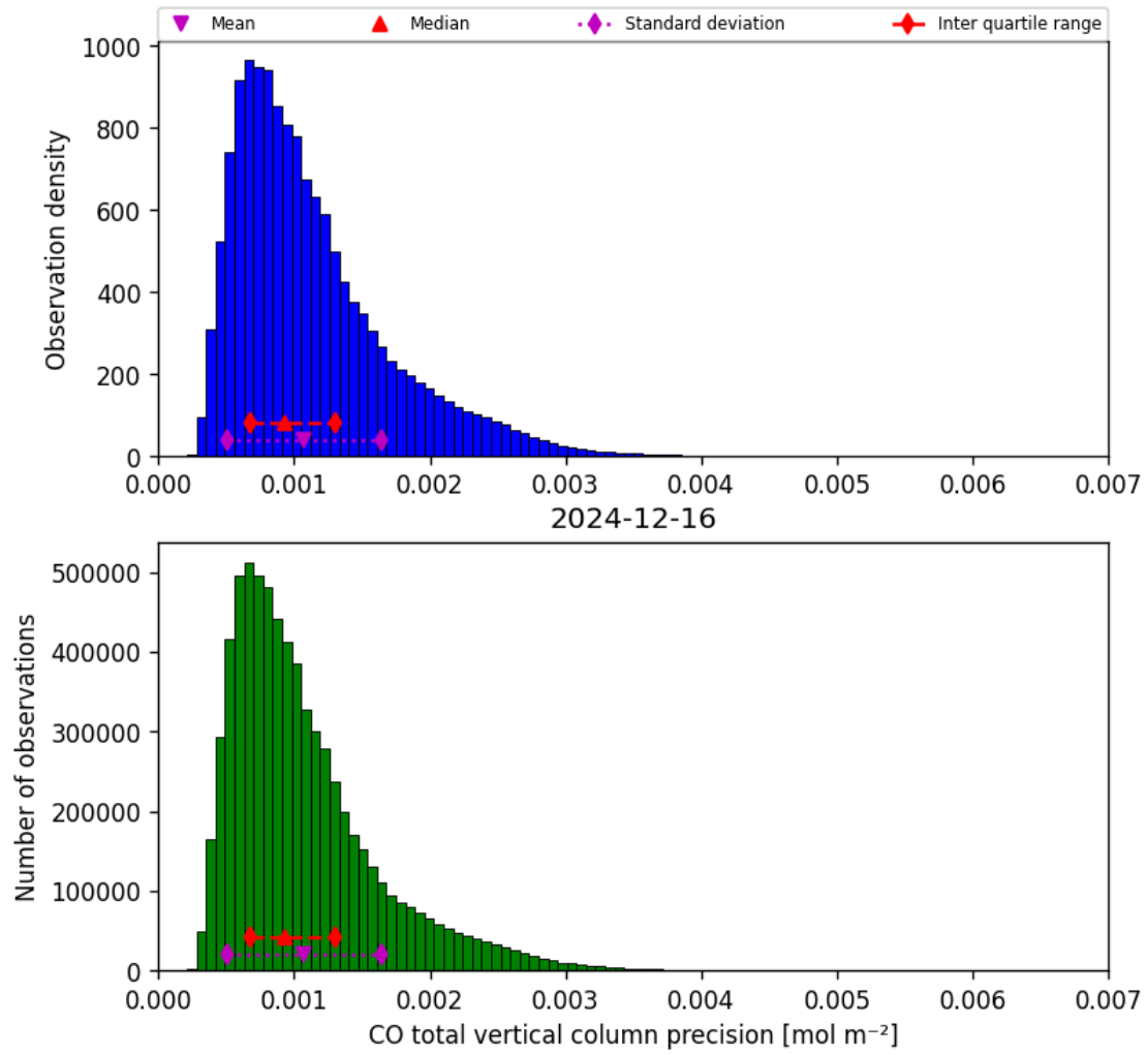
Figure 15: Histogram of “CO total vertical column precision” for 2024-12-16 to 2024-12-17
