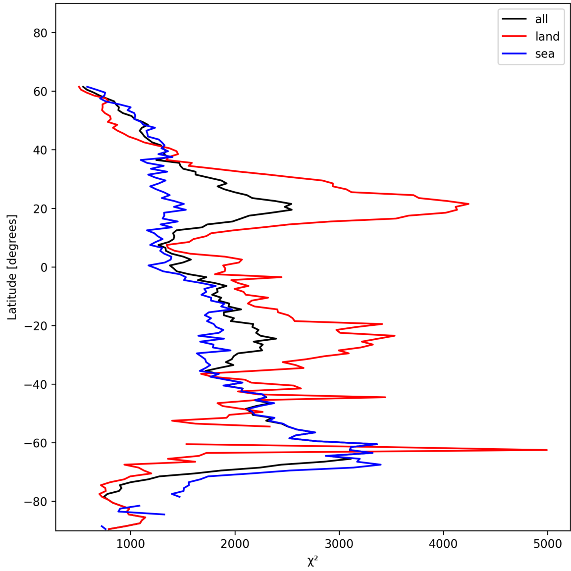
Figure 10: Zonal average of “ \chi^2 ” for 2024-12-16 to 2024-12-17.
