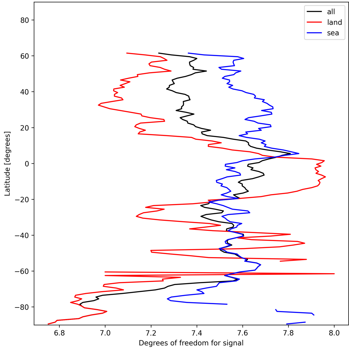
Figure 11: Zonal average of “Degrees of freedom for signal” for 2024-12-16 to 2024-12-17.
