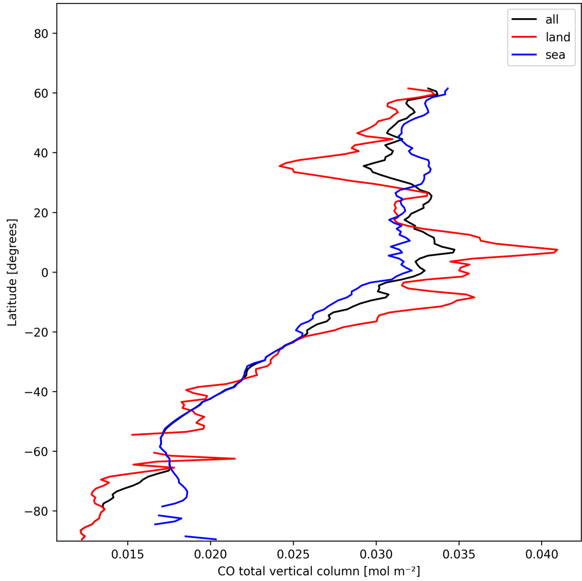
Figure 7: Zonal average of “CO total vertical column” for 2024-12-16 to 2024-12-17.
