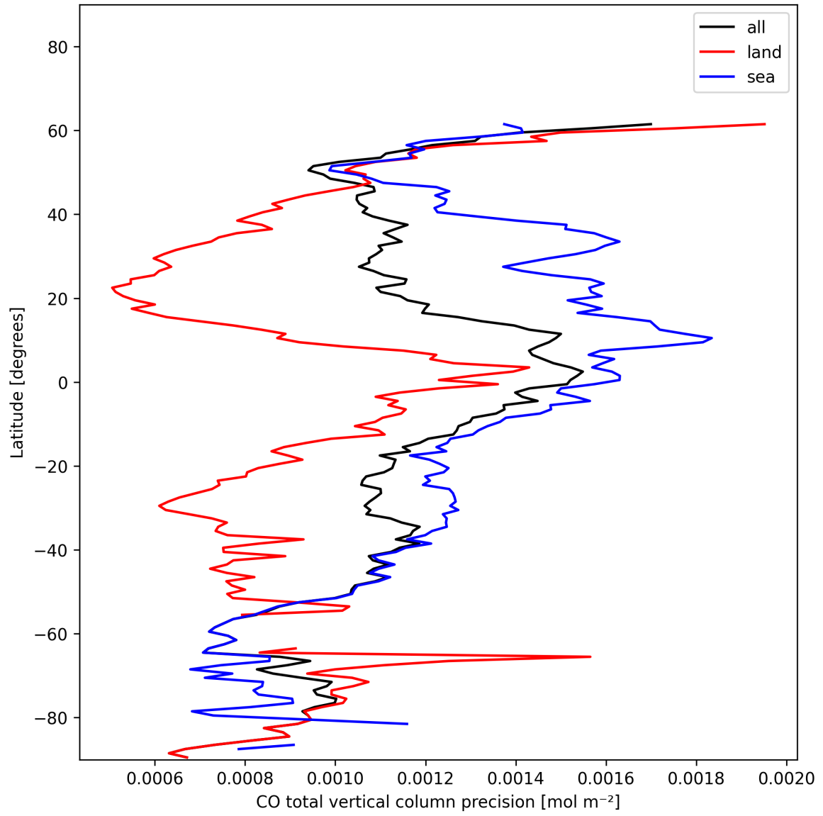
Figure 8: Zonal average of “CO total vertical column precision” for 2024-12-17 to 2024-12-18.
