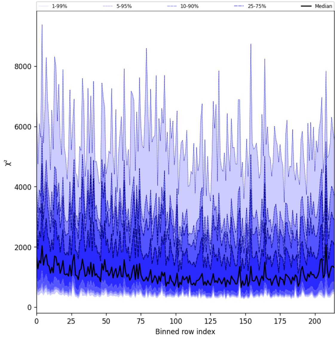
Figure 24: Along track statistics of “ \chi^2 ” for 2024-12-17 to 2024-12-18
