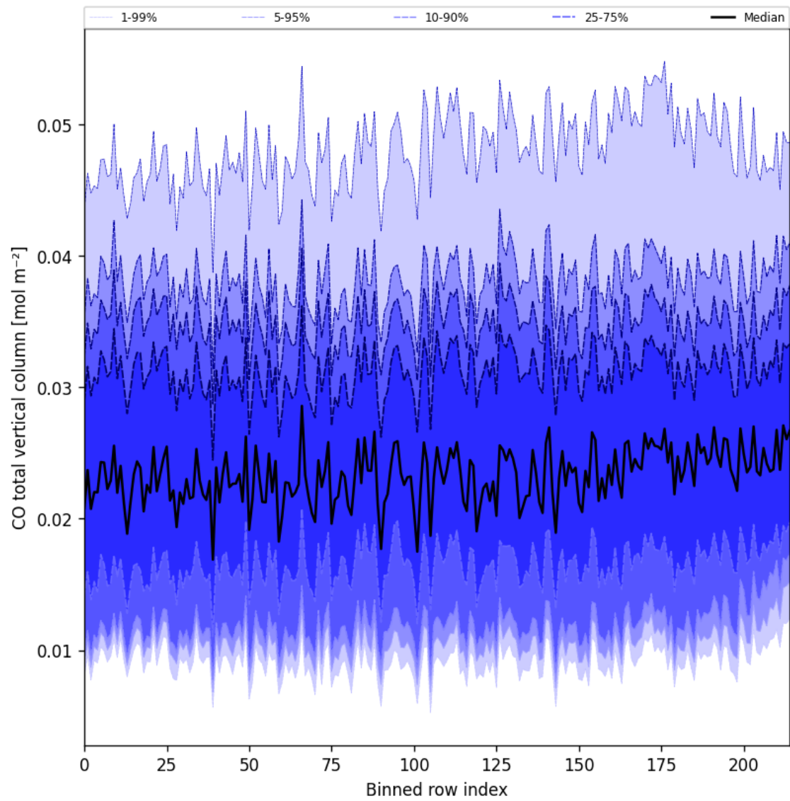
Figure 21: Along track statistics of “CO total vertical column” for 2024-12-17 to 2024-12-18
