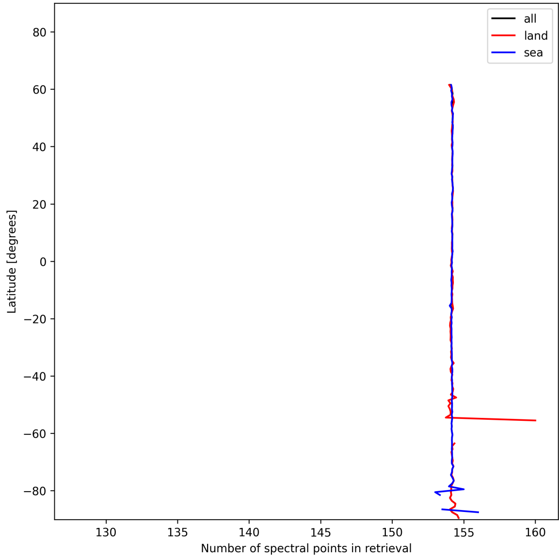
Figure 9: Zonal average of “Number of spectral points in retrieval” for 2024-12-17 to 2024-12-18.
