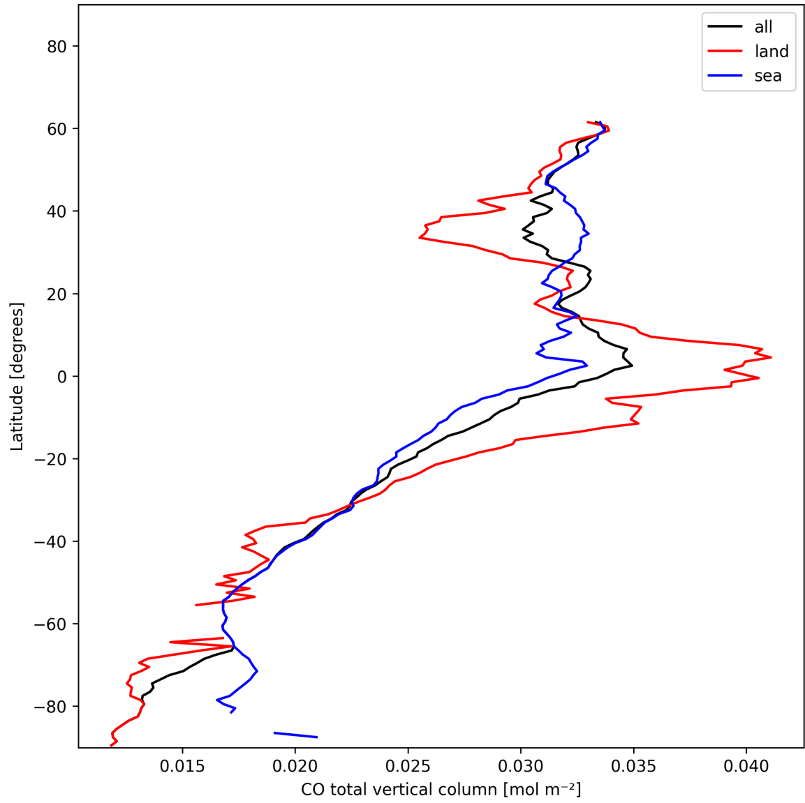
Figure 7: Zonal average of “CO total vertical column” for 2024-12-17 to 2024-12-18.
