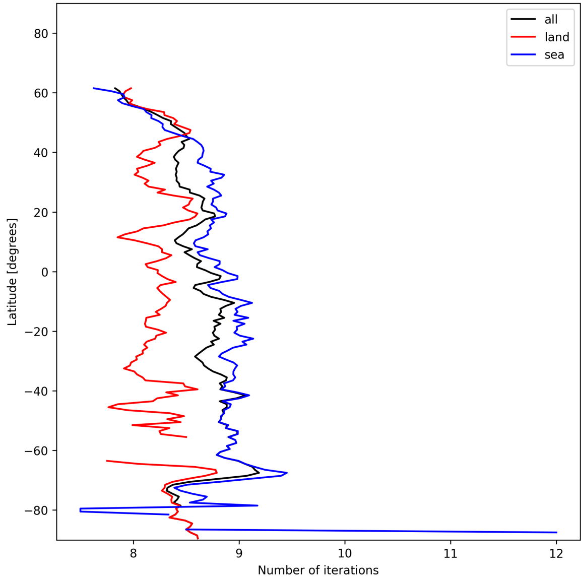
Figure 12: Zonal average of “Number of iterations” for 2024-12-17 to 2024-12-18.
