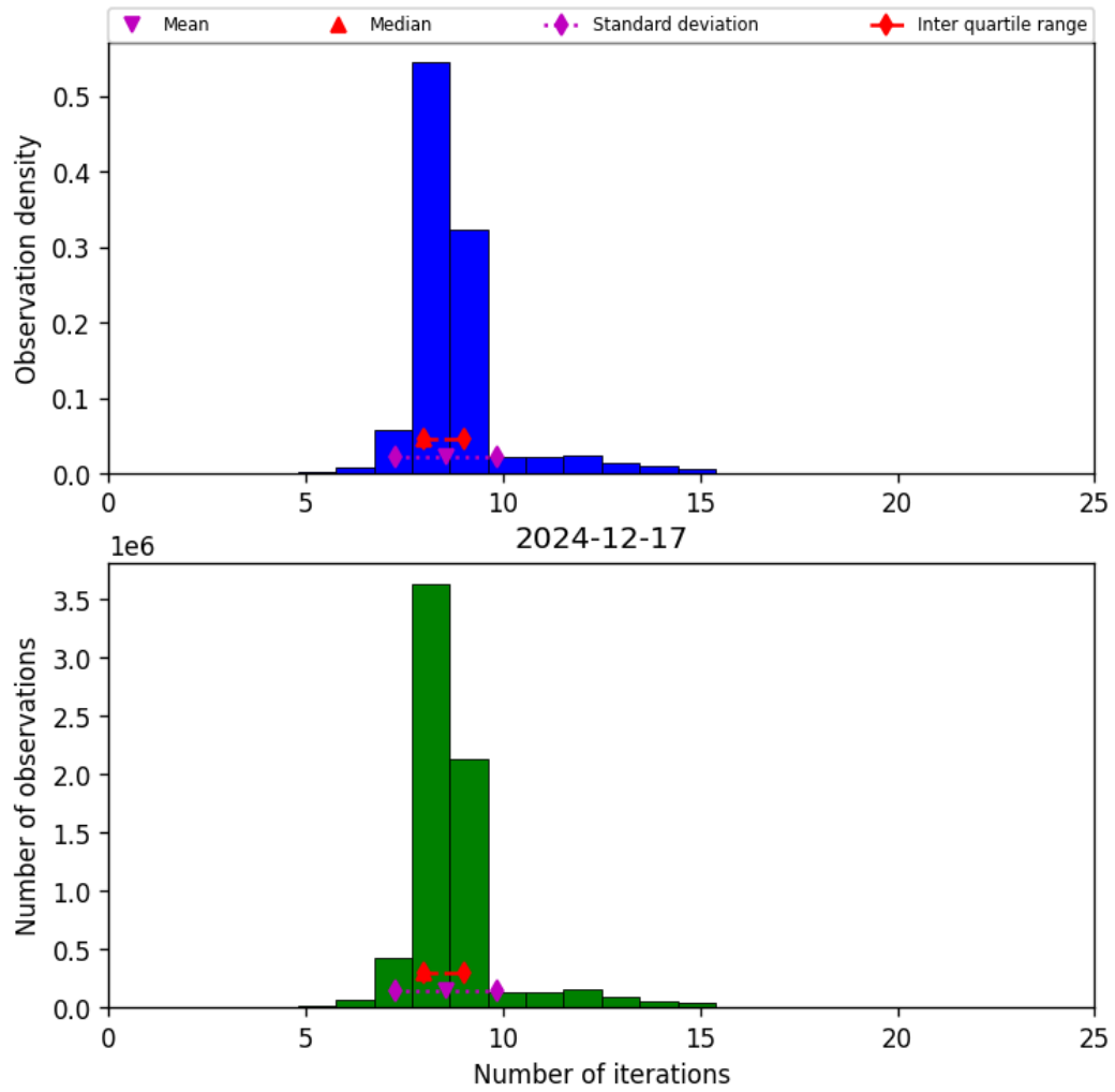
Figure 19: Histogram of “Number of iterations” for 2024-12-17 to 2024-12-18
