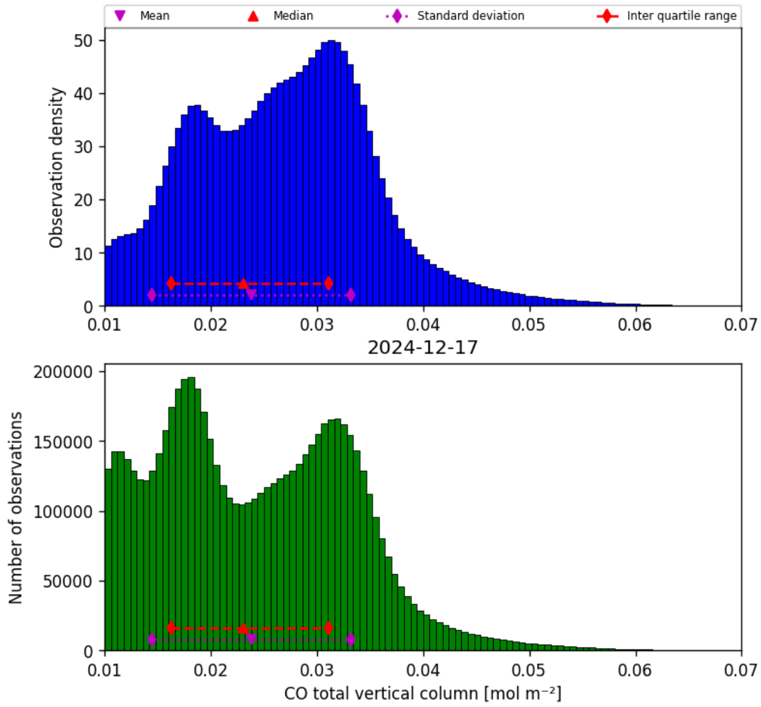
Figure 14: Histogram of “CO total vertical column” for 2024-12-17 to 2024-12-18
