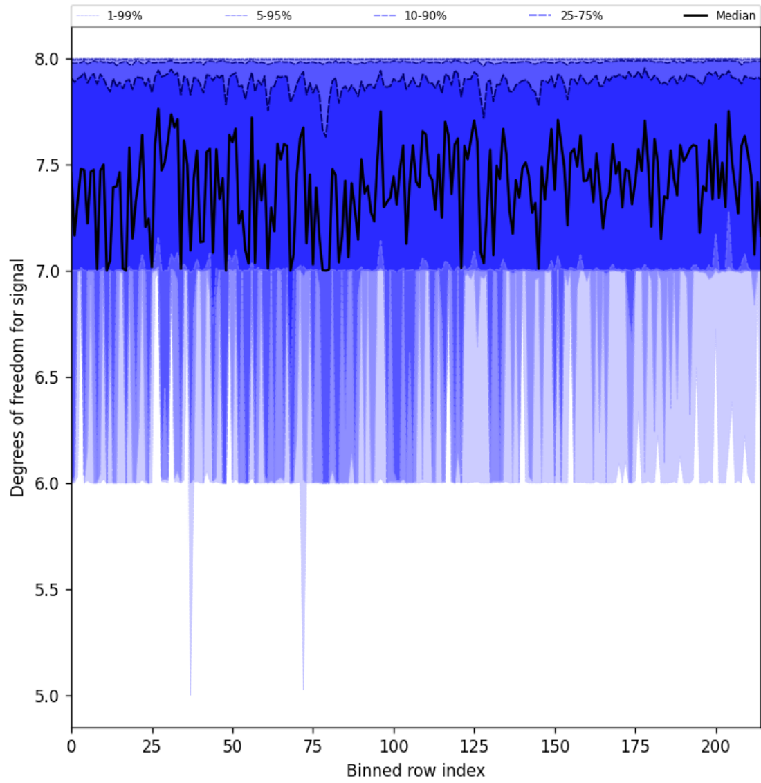
Figure 25: Along track statistics of “Degrees of freedom for signal” for 2024-12-17 to 2024-12-18
