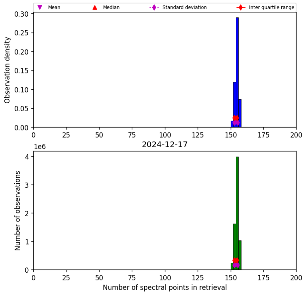
Figure 16: Histogram of “Number of spectral points in retrieval” for 2024-12-17 to 2024-12-18
