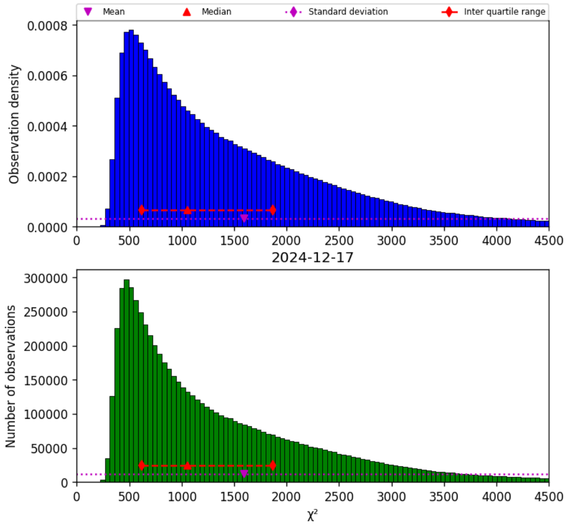
Figure 17: Histogram of “ \chi^2 ” for 2024-12-17 to 2024-12-18
