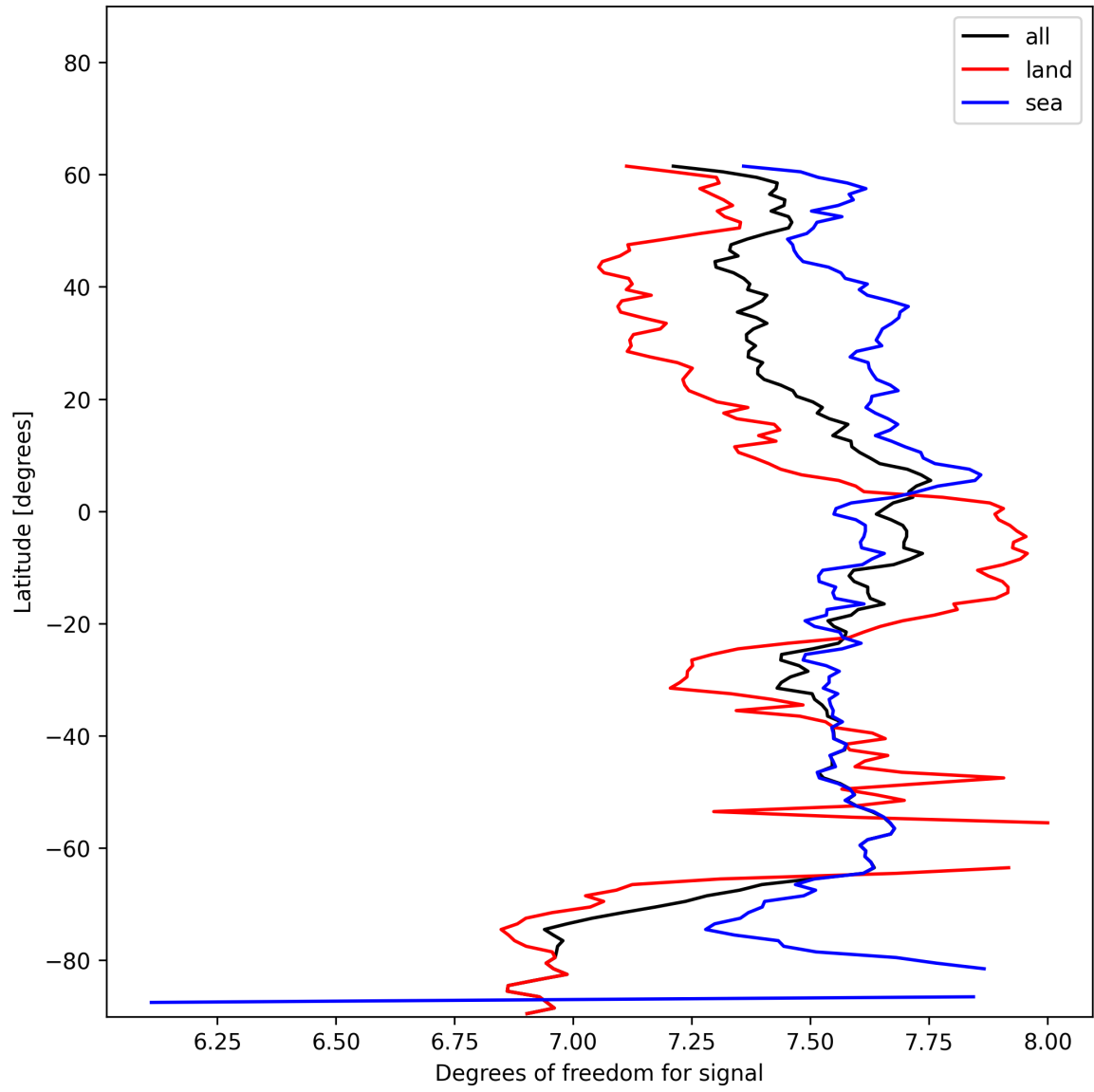
Figure 11: Zonal average of “Degrees of freedom for signal” for 2024-12-17 to 2024-12-18.
