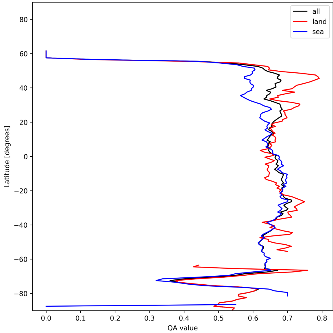
Figure 6: Zonal average of “QA value” for 2024-12-17 to 2024-12-18.
