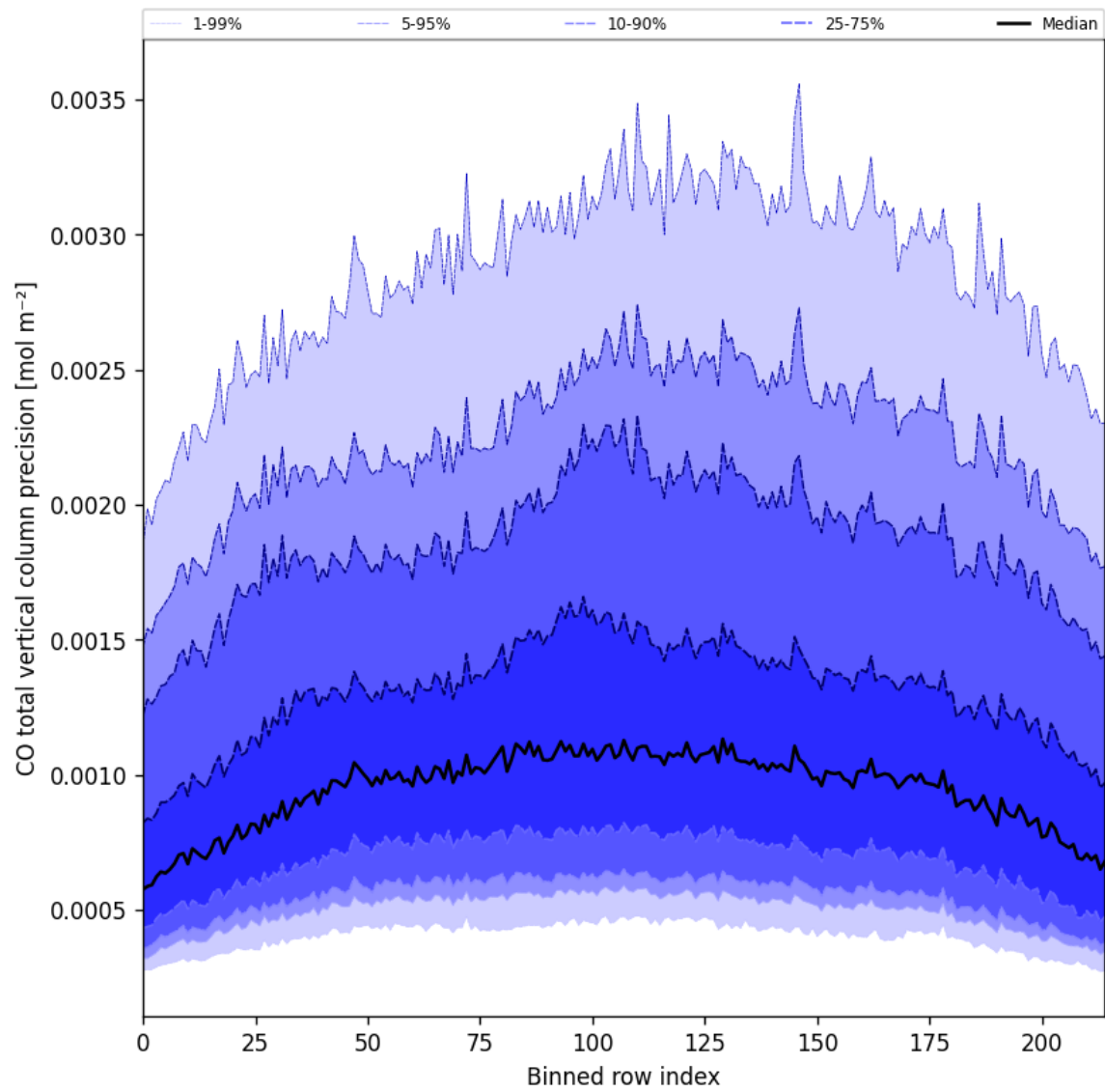
Figure 22: Along track statistics of “CO total vertical column precision” for 2024-12-17 to 2024-12-18
