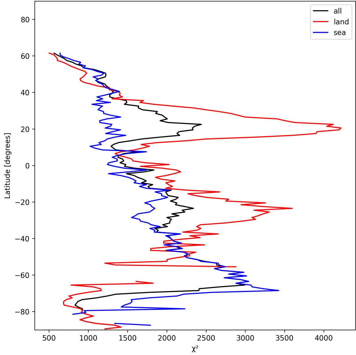
Figure 10: Zonal average of “ \chi^2 ” for 2024-12-17 to 2024-12-18.
