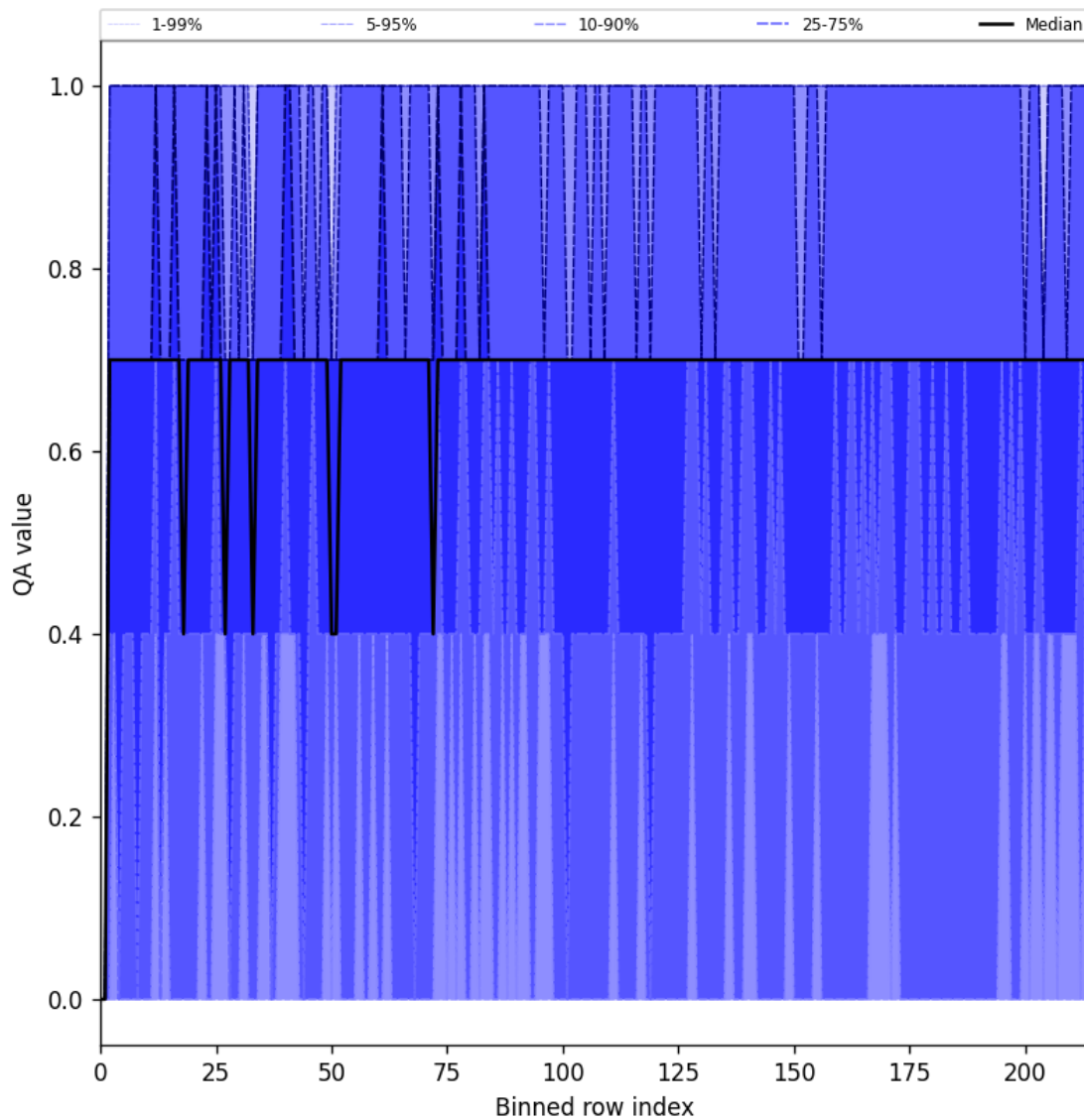
Figure 20: Along track statistics of “QA value” for 2024-12-17 to 2024-12-18
