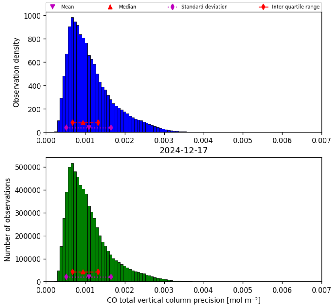
Figure 15: Histogram of “CO total vertical column precision” for 2024-12-17 to 2024-12-18
