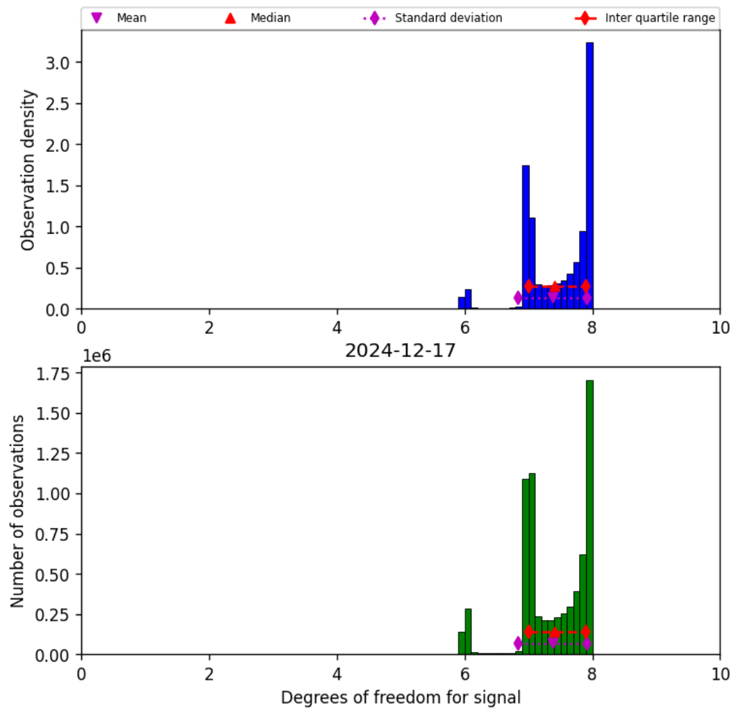
Figure 18: Histogram of “Degrees of freedom for signal” for 2024-12-17 to 2024-12-18
