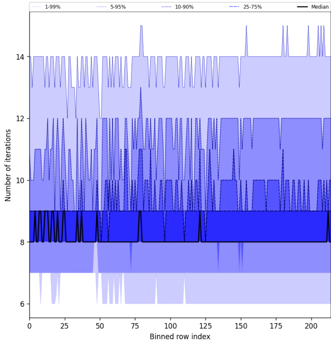
Figure 26: Along track statistics of “Number of iterations” for 2024-12-17 to 2024-12-18
