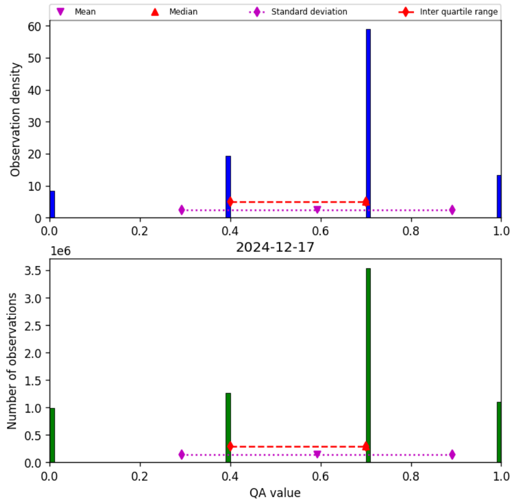
Figure 13: Histogram of “QA value” for 2024-12-17 to 2024-12-18
