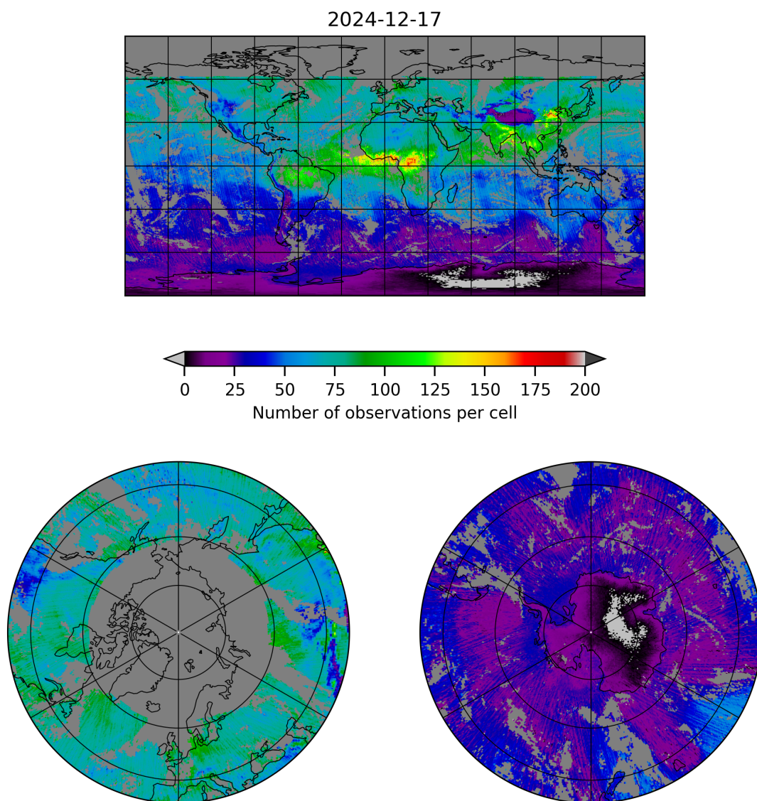
Figure 5: Map of the number of observations for 2024-12-17 to 2024-12-18
