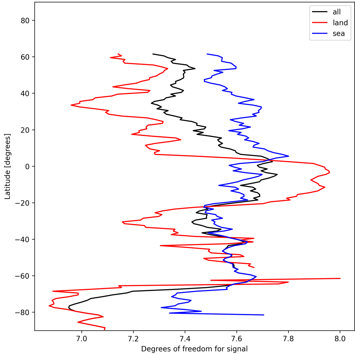
Figure 11: Zonal average of “Degrees of freedom for signal” for 2024-12-18 to 2024-12-19.
