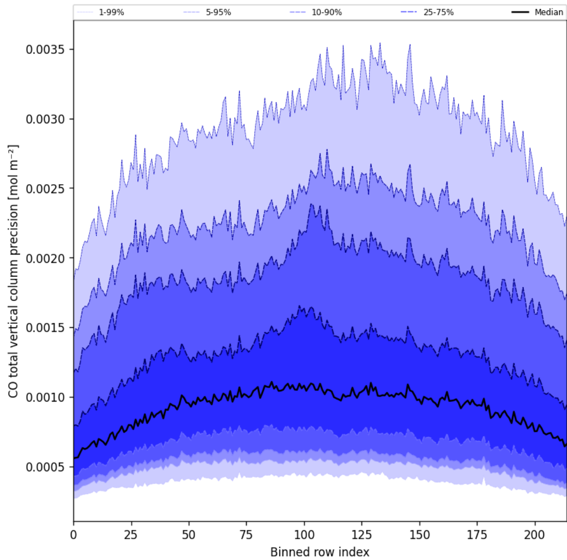
Figure 22: Along track statistics of “CO total vertical column precision” for 2024-12-18 to 2024-12-19
