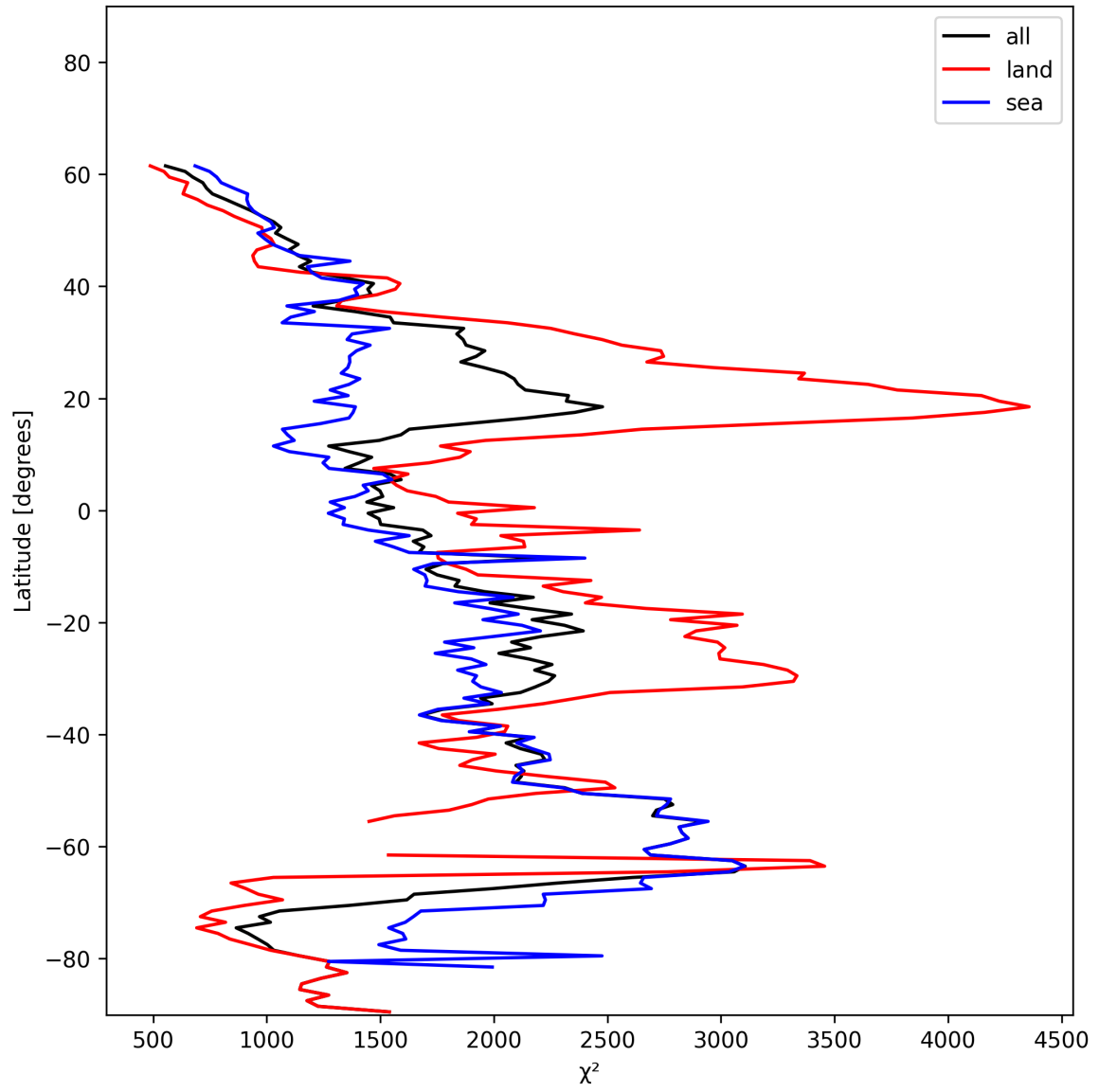
Figure 10: Zonal average of “ \chi^2 ” for 2024-12-18 to 2024-12-19.
