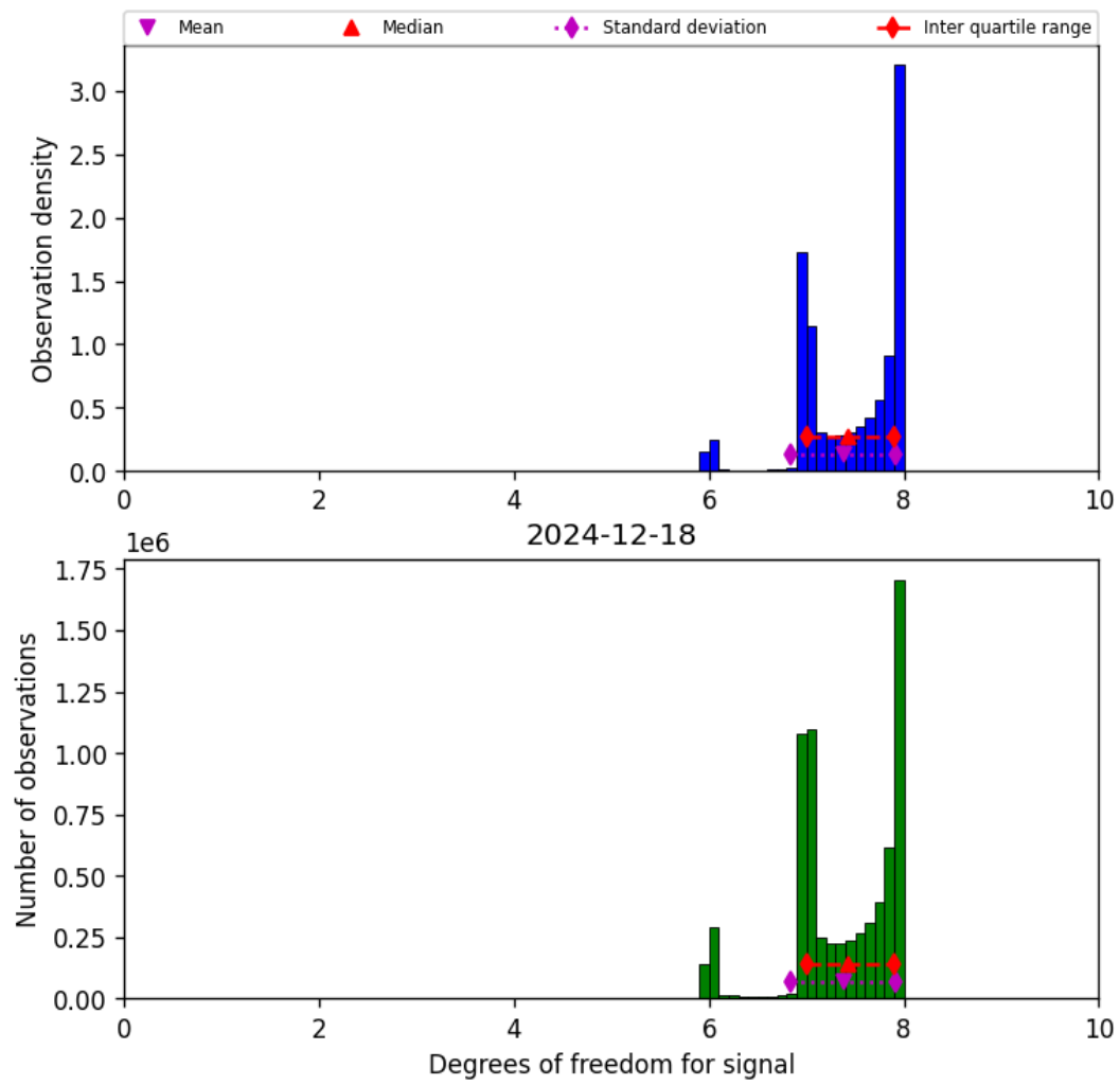
Figure 18: Histogram of “Degrees of freedom for signal” for 2024-12-18 to 2024-12-19
