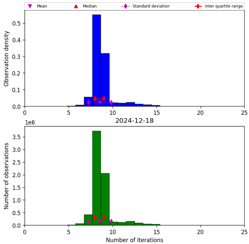
Figure 19: Histogram of “Number of iterations” for 2024-12-18 to 2024-12-19
