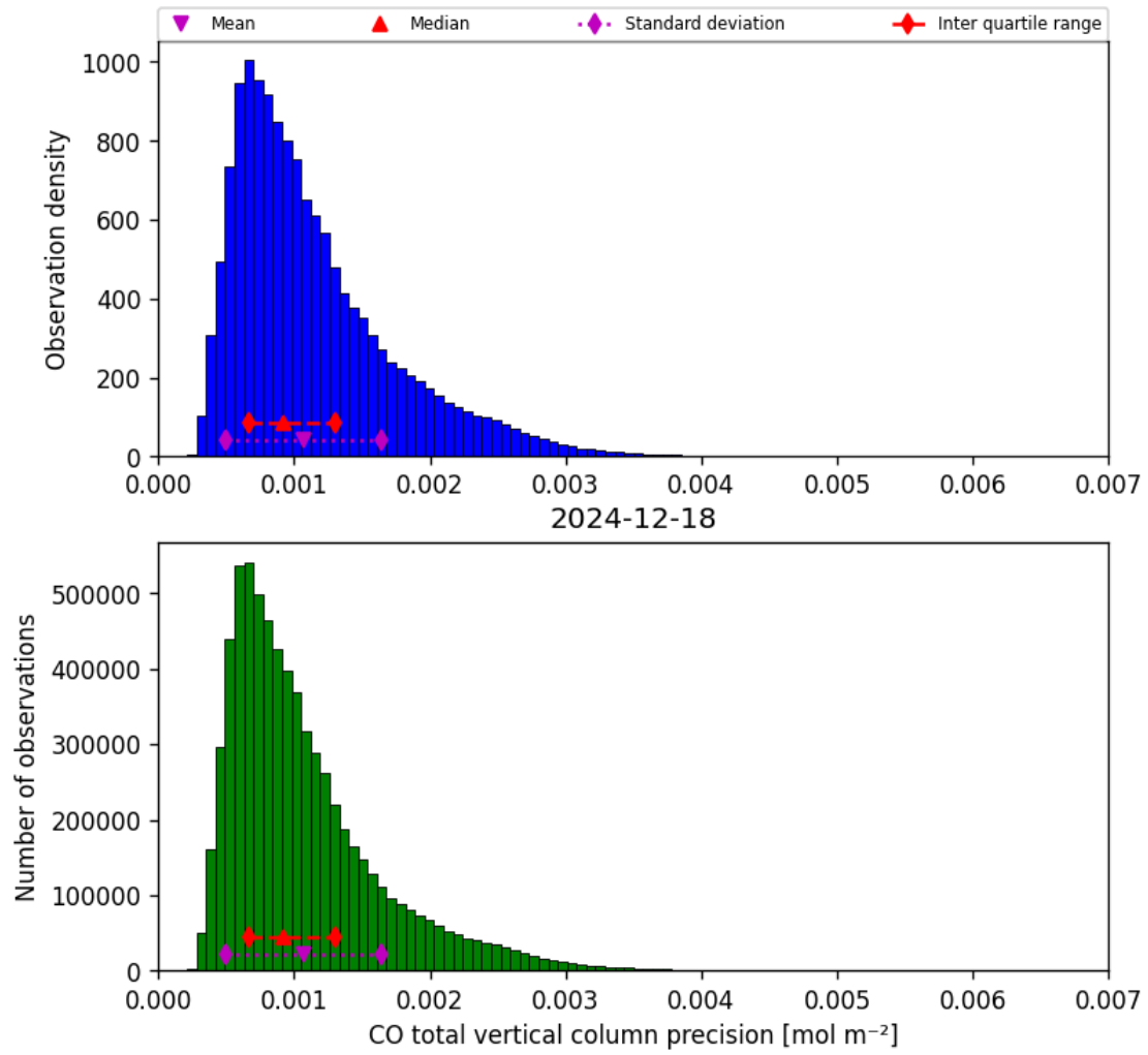
Figure 15: Histogram of “CO total vertical column precision” for 2024-12-18 to 2024-12-19
