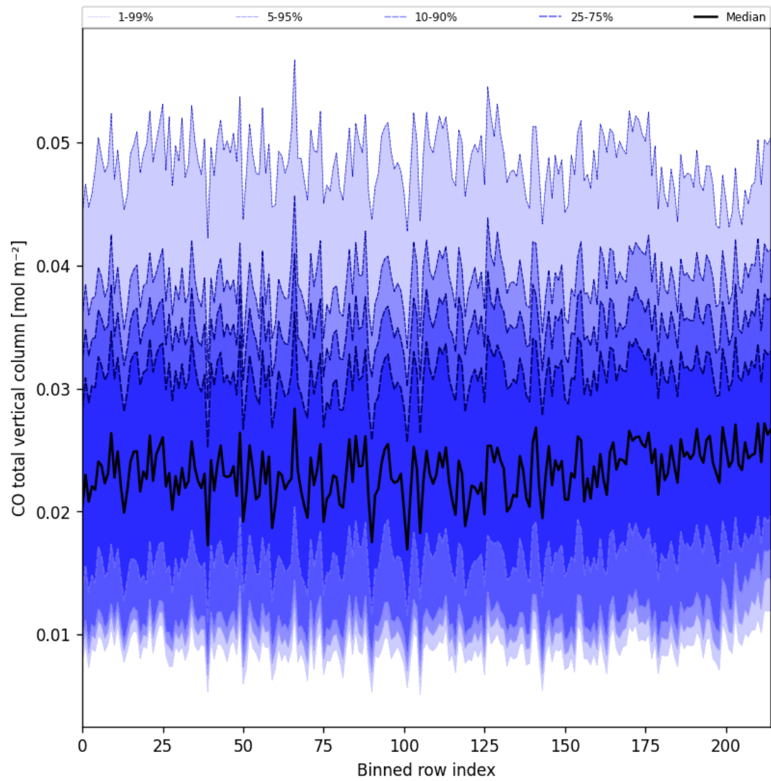
Figure 21: Along track statistics of “CO total vertical column” for 2024-12-18 to 2024-12-19
