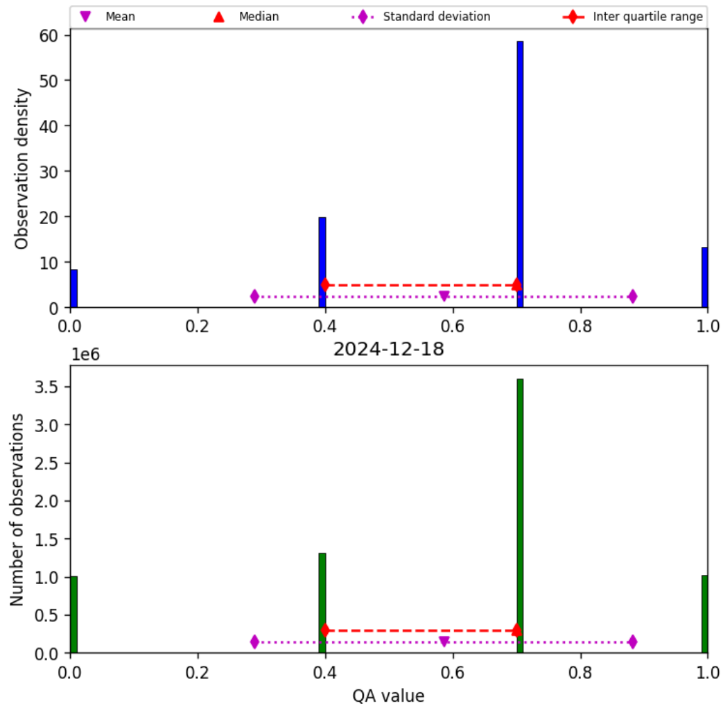
Figure 13: Histogram of “QA value” for 2024-12-18 to 2024-12-19
