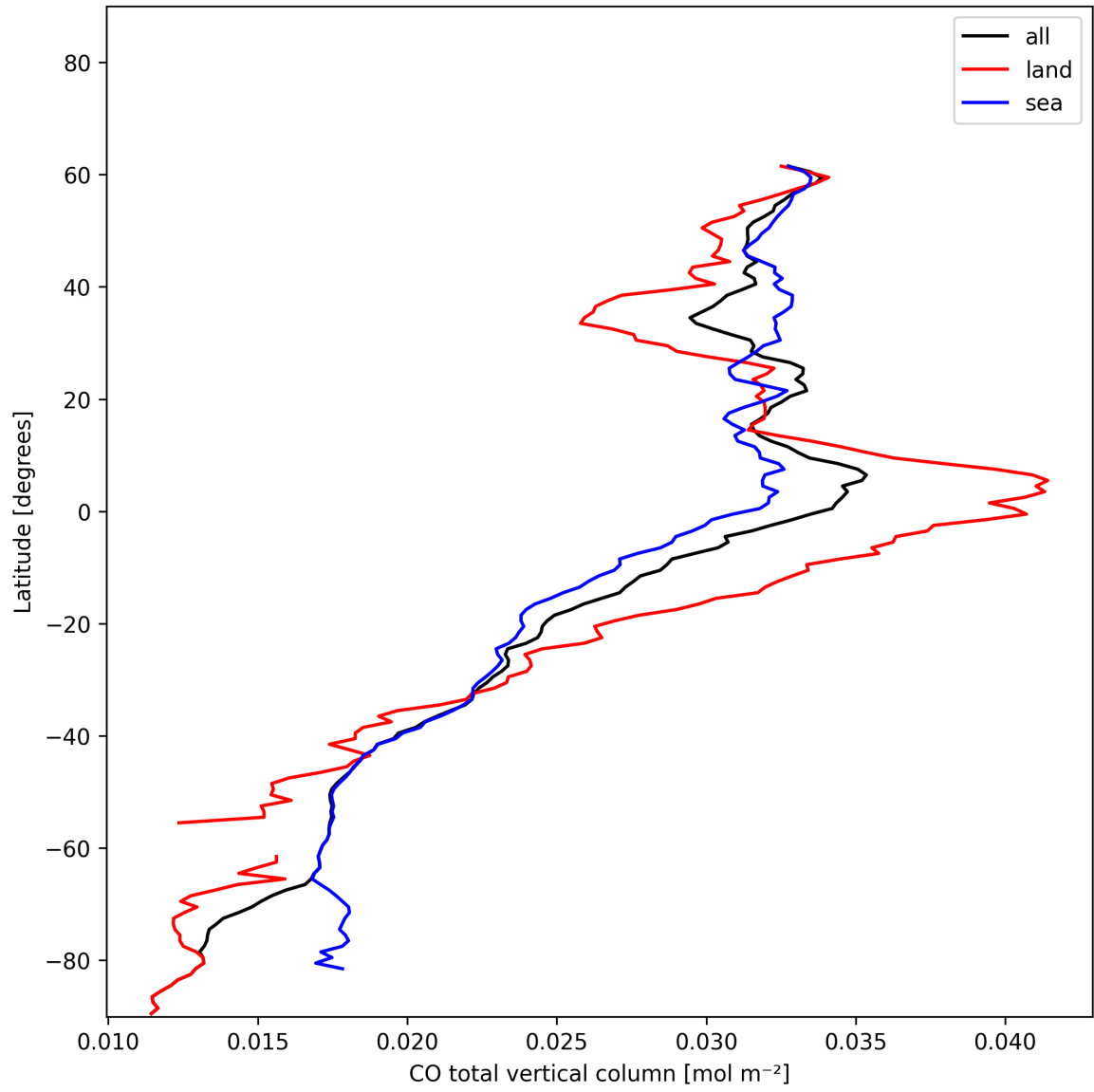
Figure 7: Zonal average of “CO total vertical column” for 2024-12-18 to 2024-12-19.
