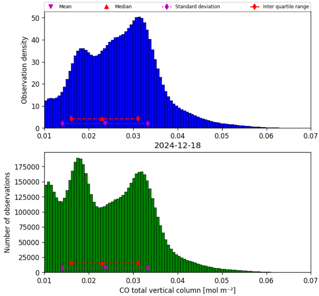
Figure 14: Histogram of “CO total vertical column” for 2024-12-18 to 2024-12-19
