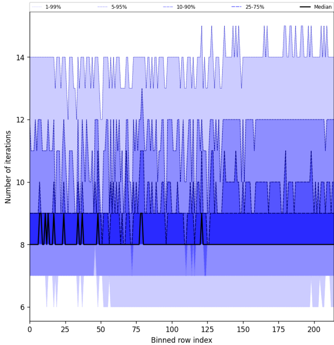
Figure 26: Along track statistics of “Number of iterations” for 2024-12-18 to 2024-12-19
