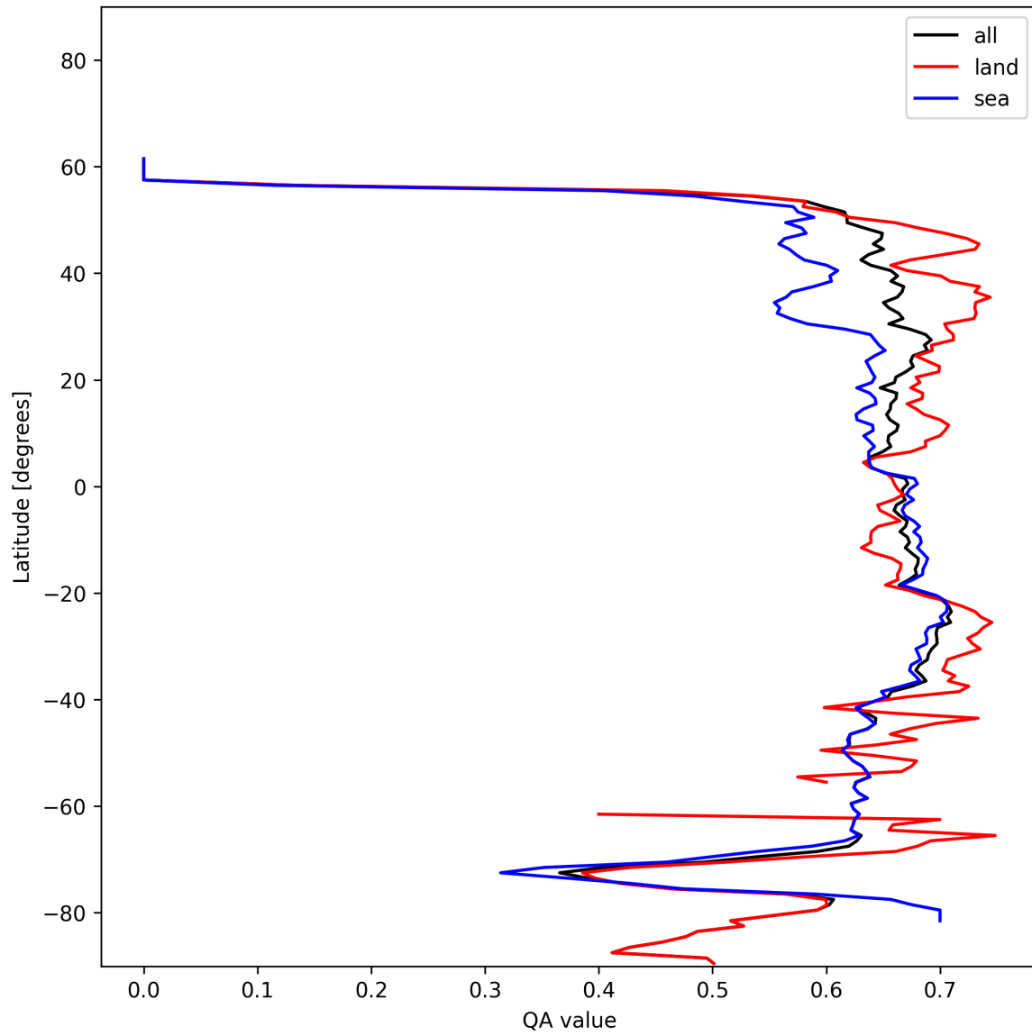
Figure 6: Zonal average of “QA value” for 2024-12-18 to 2024-12-19.
