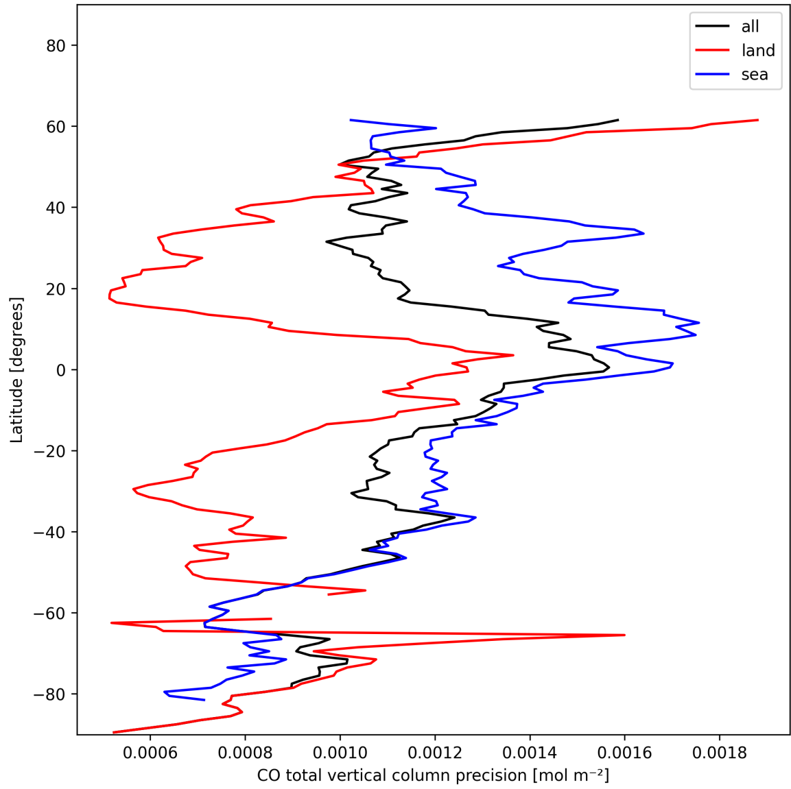
Figure 8: Zonal average of “CO total vertical column precision” for 2024-12-18 to 2024-12-19.
