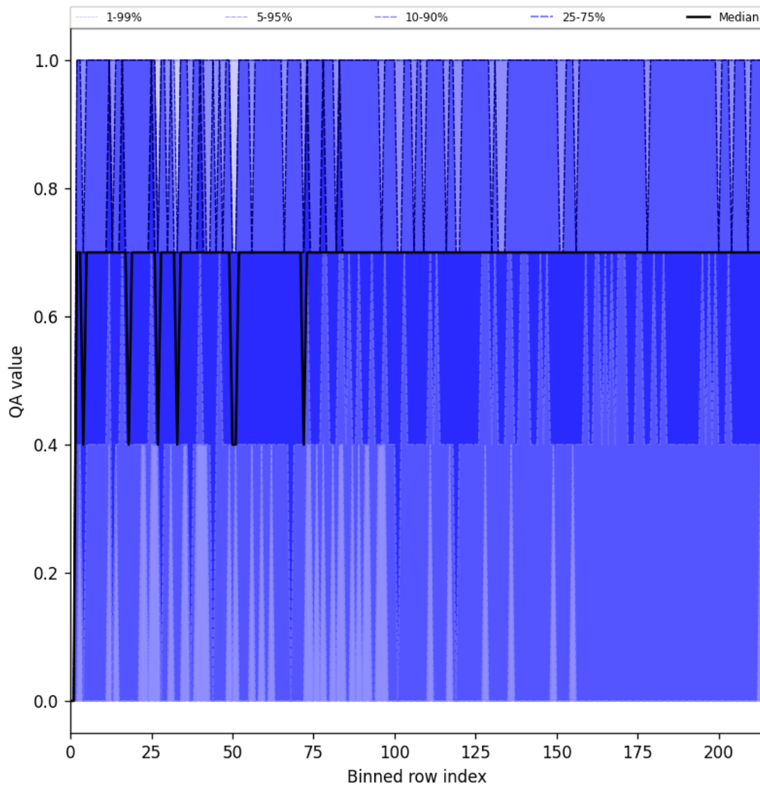
Figure 20: Along track statistics of “QA value” for 2024-12-18 to 2024-12-19
