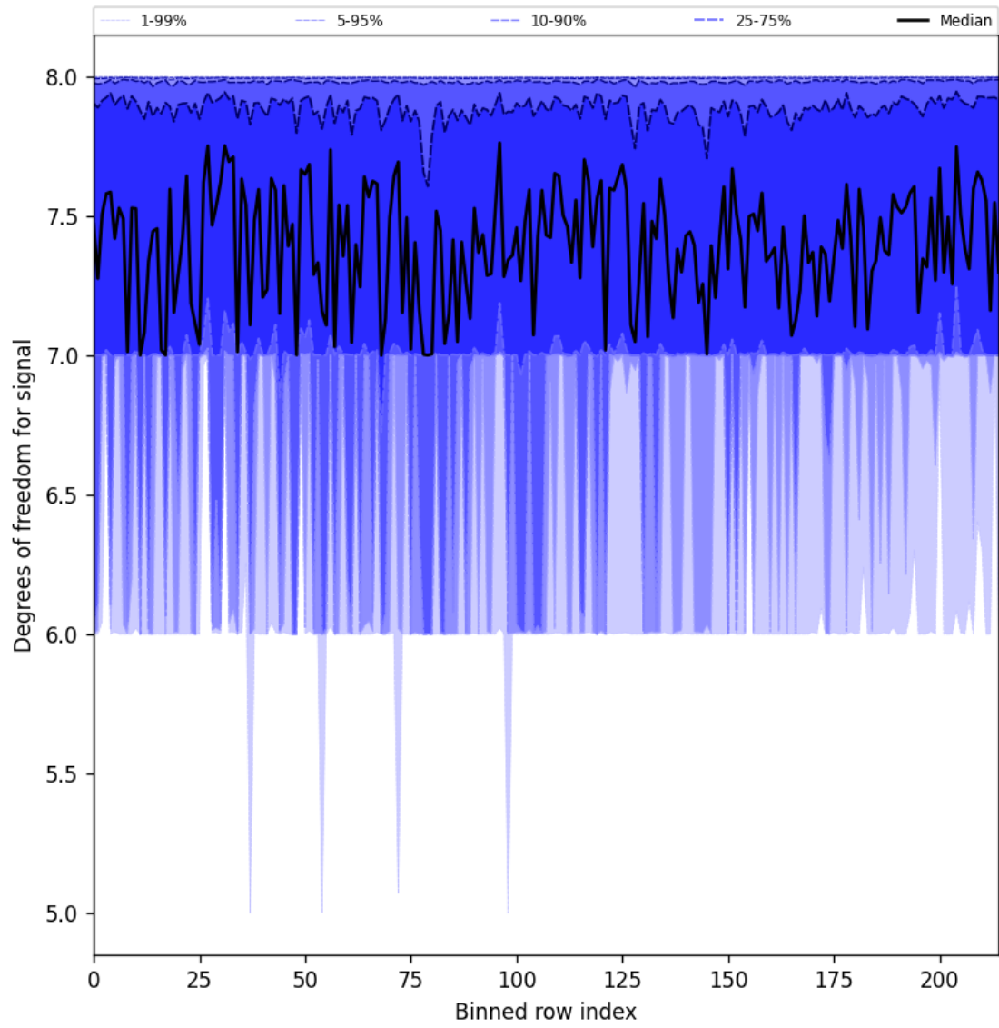
Figure 25: Along track statistics of “Degrees of freedom for signal” for 2024-12-18 to 2024-12-19
