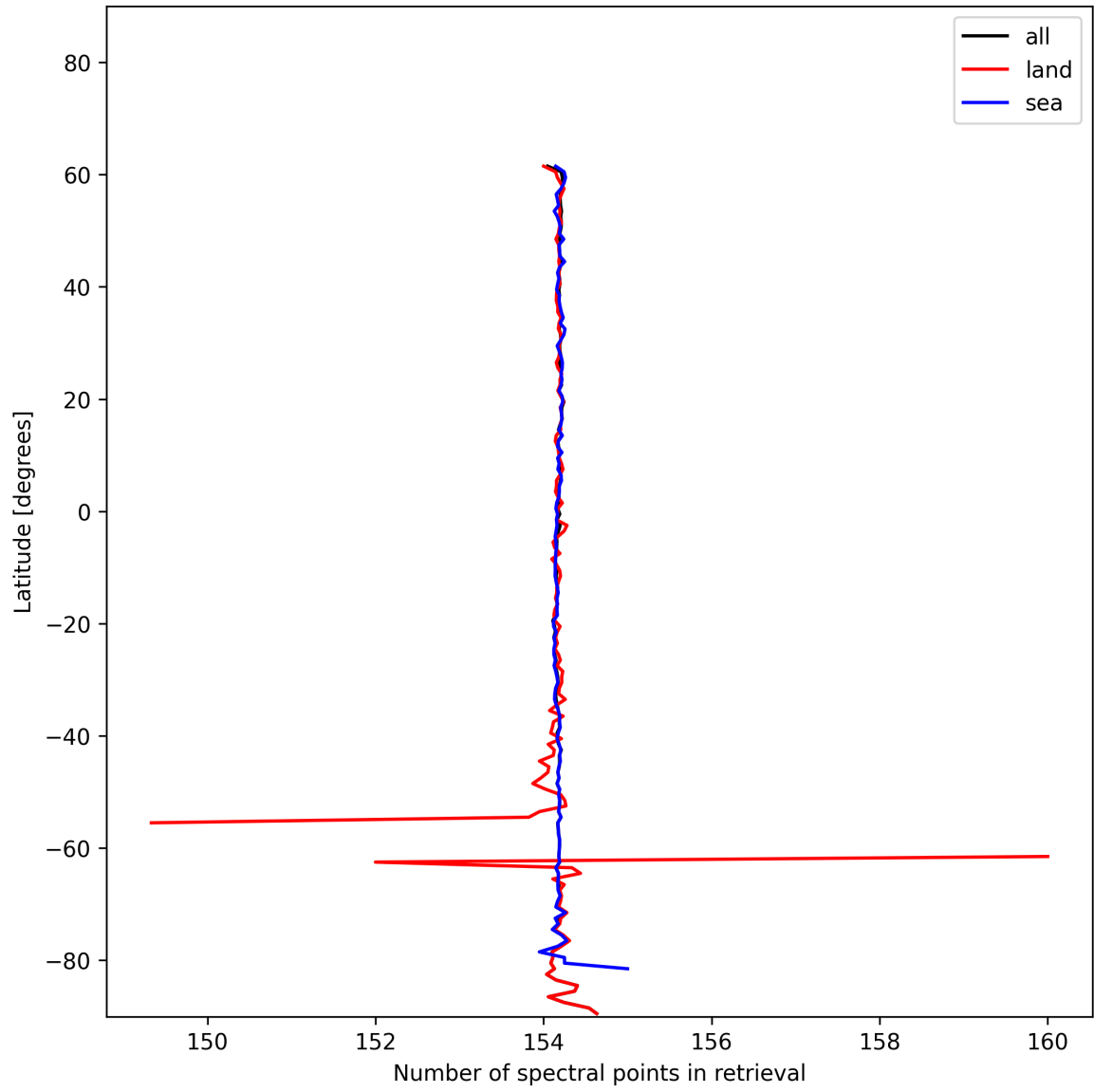
Figure 9: Zonal average of “Number of spectral points in retrieval” for 2024-12-18 to 2024-12-19.
