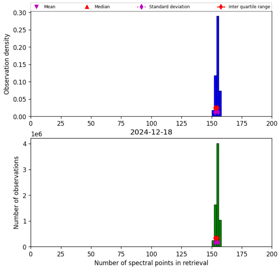
Figure 16: Histogram of "Number of spectral points in retrieval" for 2024-12-18 to 2024-12-19
