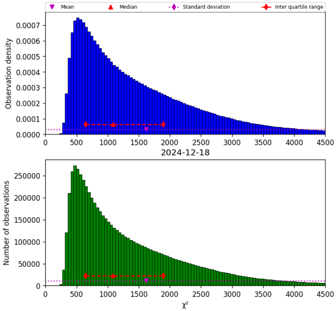
Figure 17: Histogram of “ \chi^2 ” for 2024-12-18 to 2024-12-19
