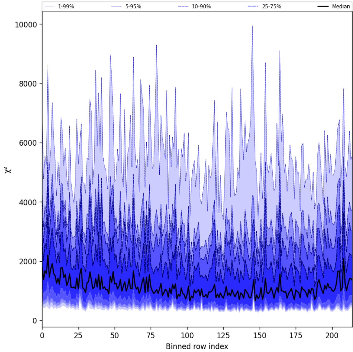
Figure 24: Along track statistics of “ \chi^2 ” for 2024-12-18 to 2024-12-19
