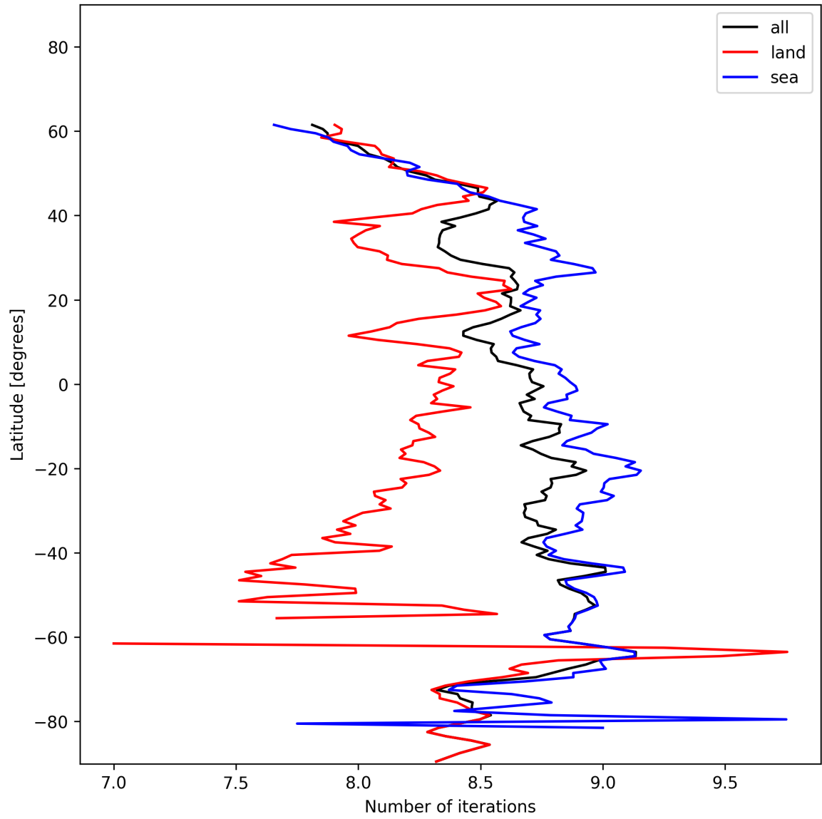
Figure 12: Zonal average of “Number of iterations” for 2024-12-18 to 2024-12-19.
