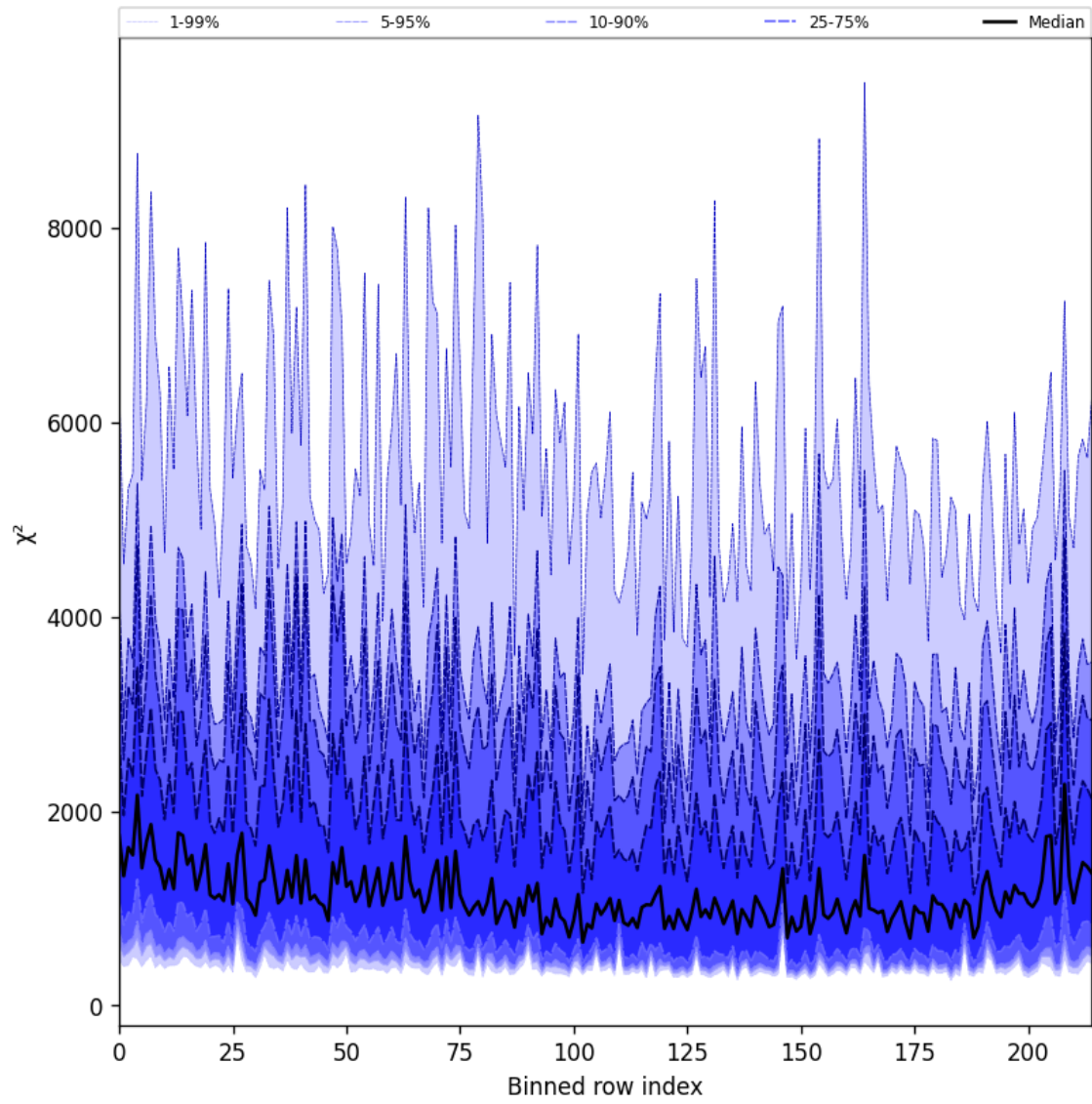
Figure 24: Along track statistics of “ \chi^2 ” for 2024-12-19 to 2024-12-19
