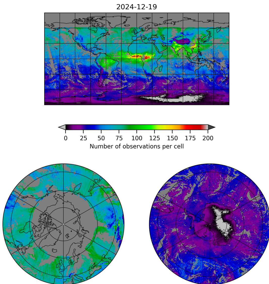
Figure 5: Map of the number of observations for 2024-12-19 to 2024-12-19
