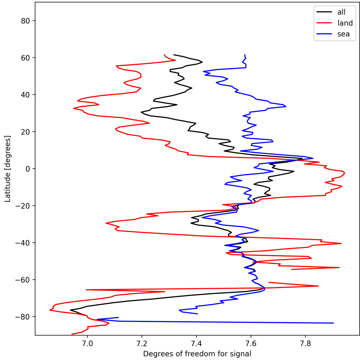
Figure 11: Zonal average of “Degrees of freedom for signal” for 2024-12-19 to 2024-12-19.
