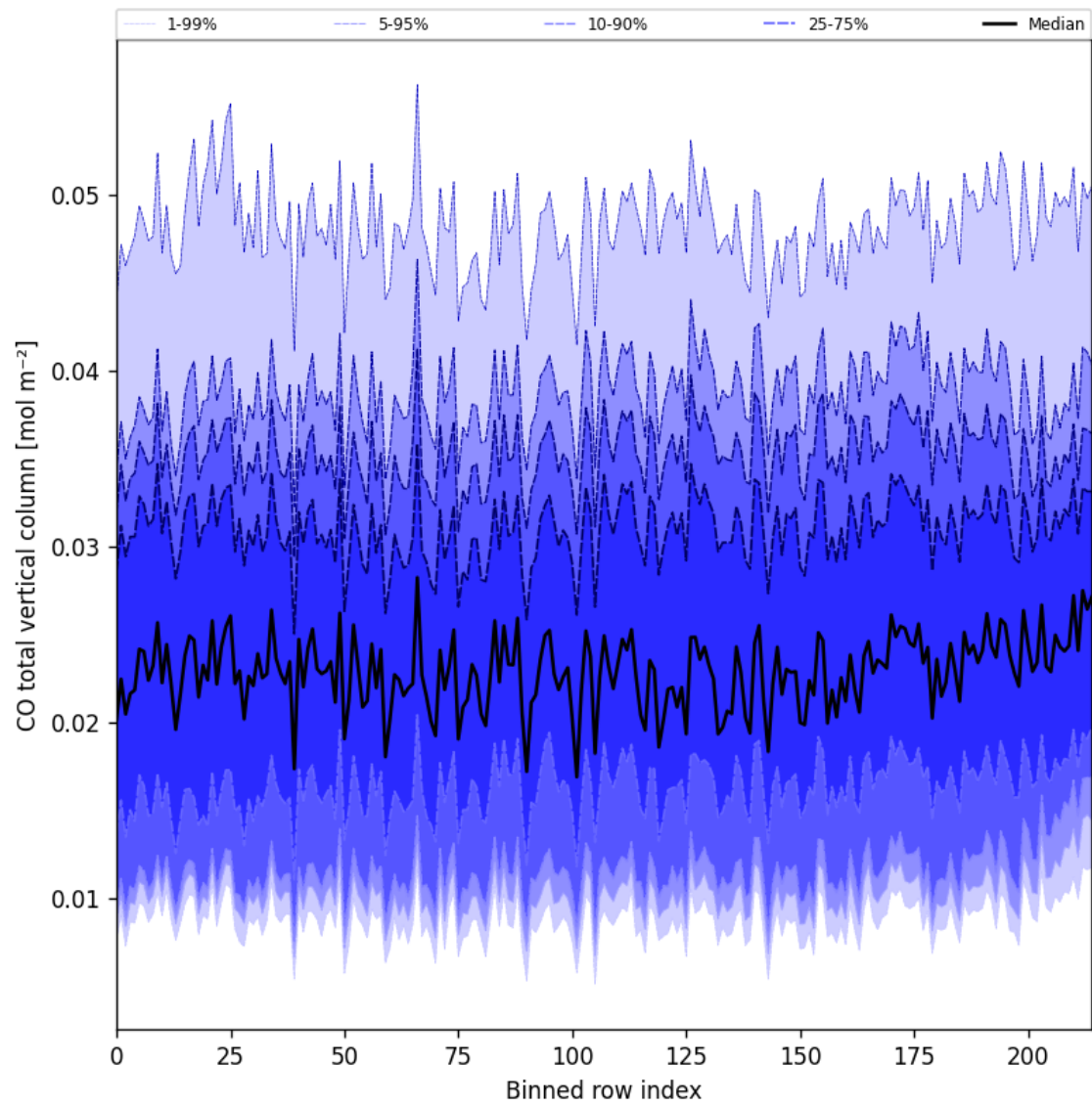
Figure 21: Along track statistics of “CO total vertical column” for 2024-12-19 to 2024-12-19
