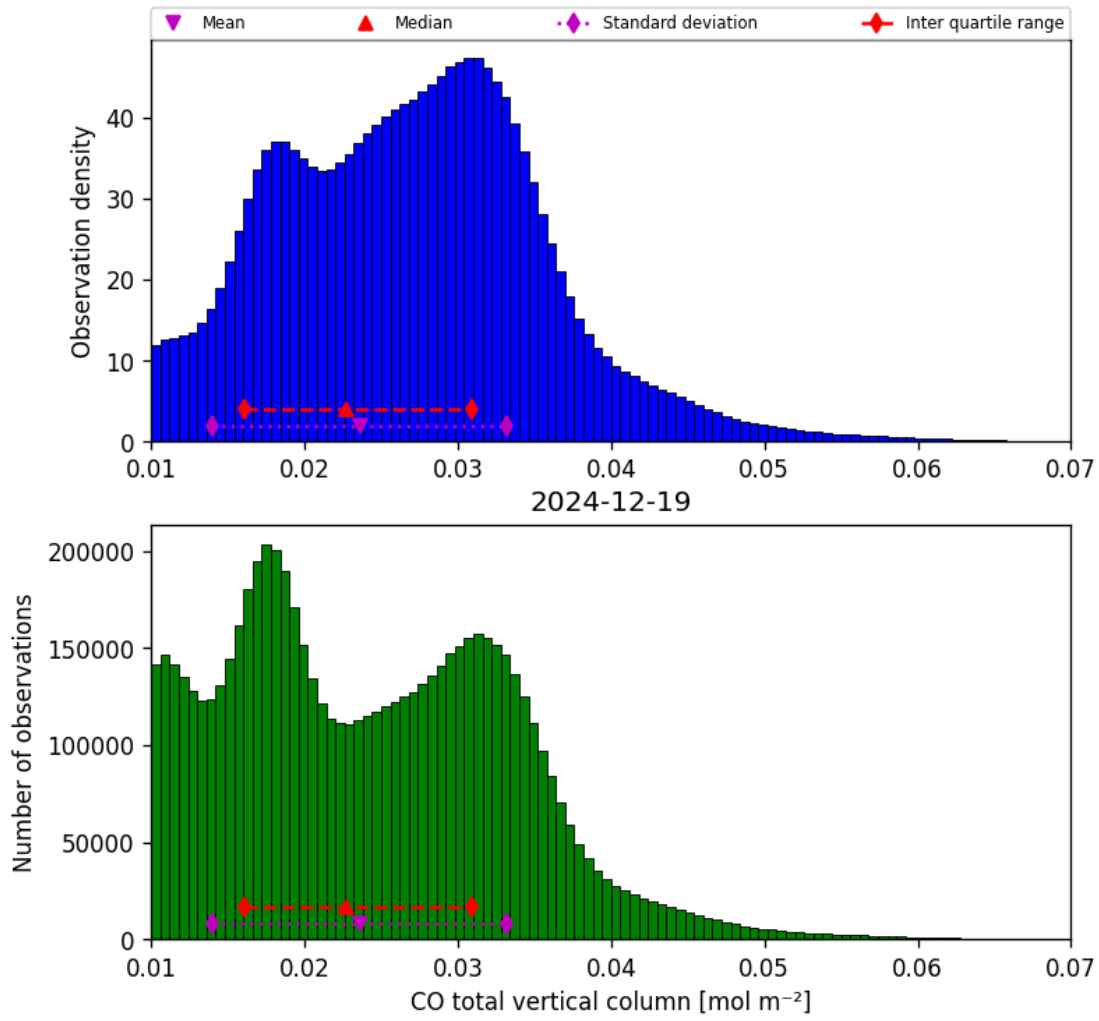
Figure 14: Histogram of “CO total vertical column” for 2024-12-19 to 2024-12-19
