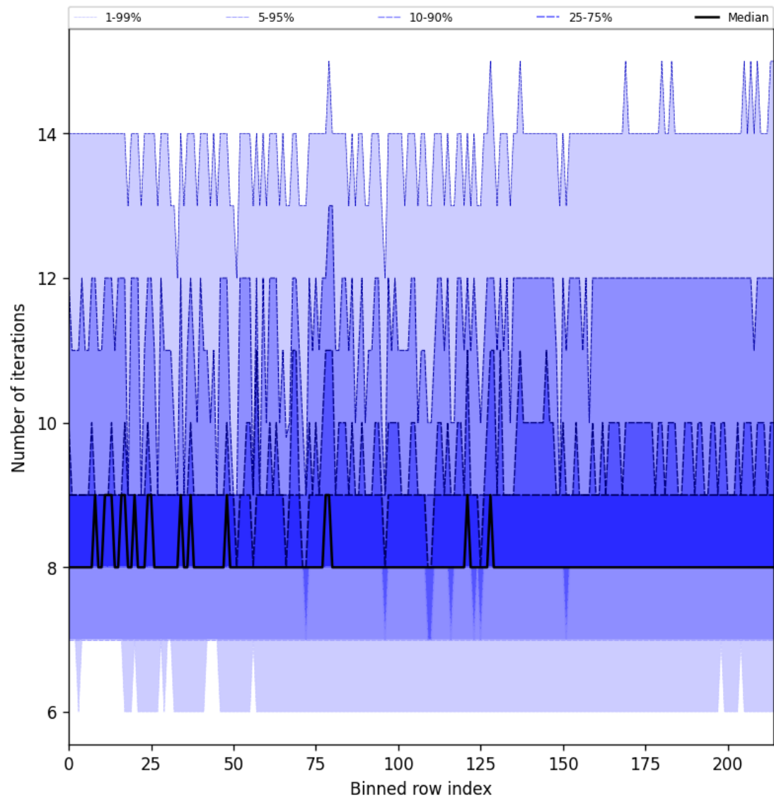
Figure 26: Along track statistics of “Number of iterations” for 2024-12-19 to 2024-12-19
