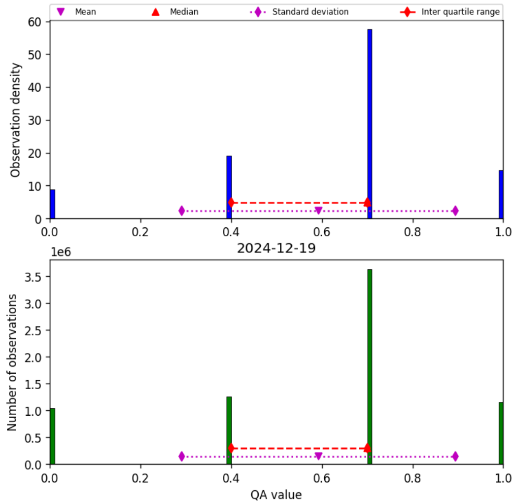
Figure 13: Histogram of “QA value” for 2024-12-19 to 2024-12-19
