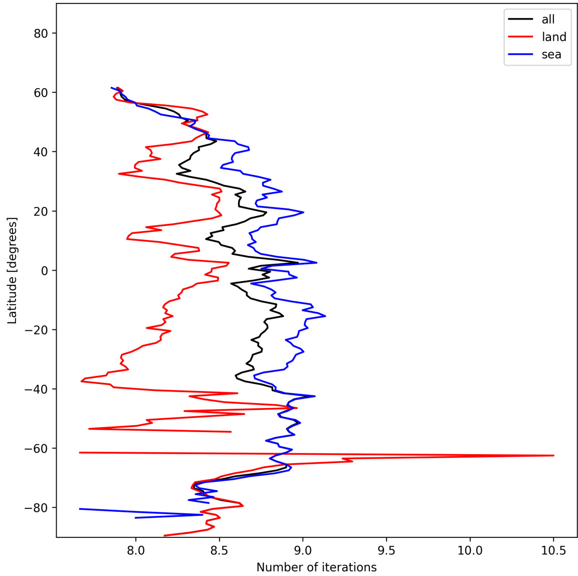
Figure 12: Zonal average of “Number of iterations” for 2024-12-19 to 2024-12-19.
