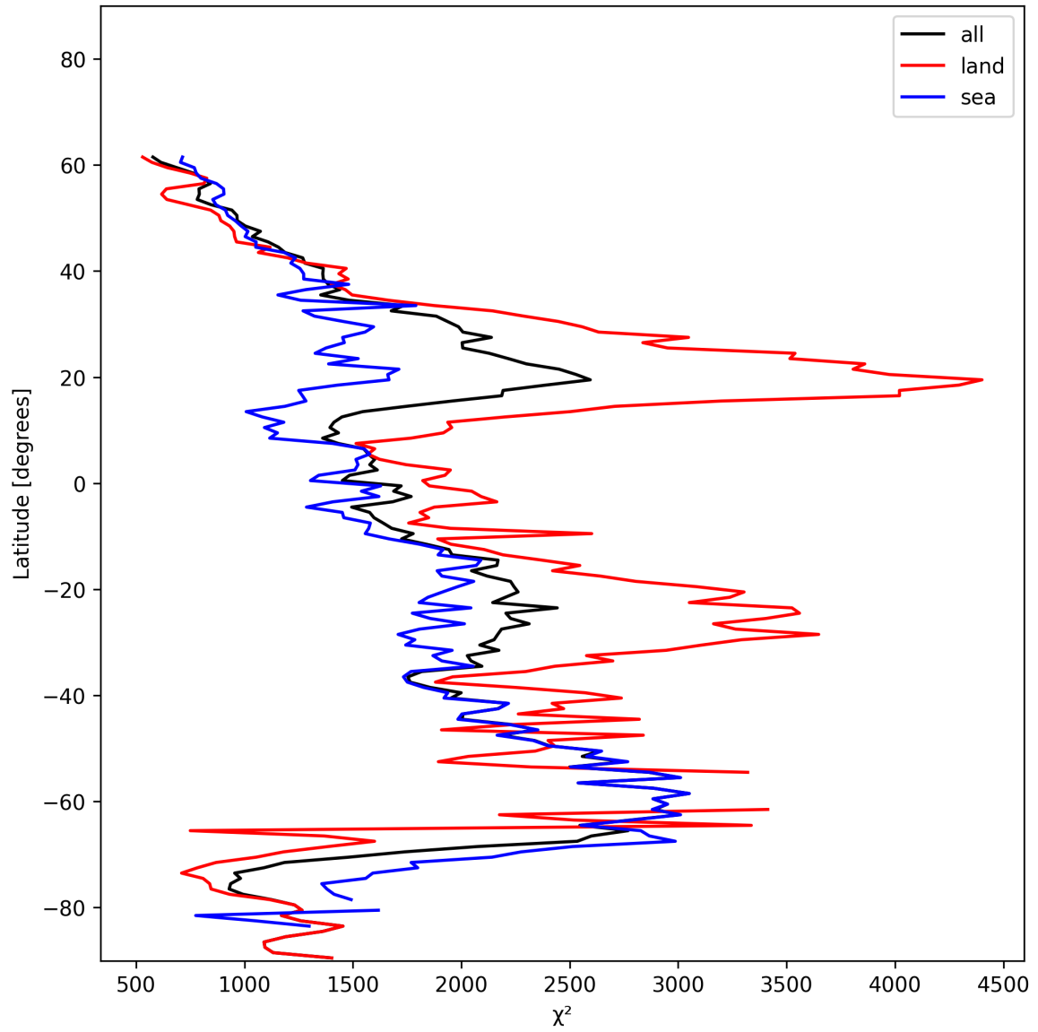
Figure 10: Zonal average of “ \chi^2 ” for 2024-12-19 to 2024-12-19.
