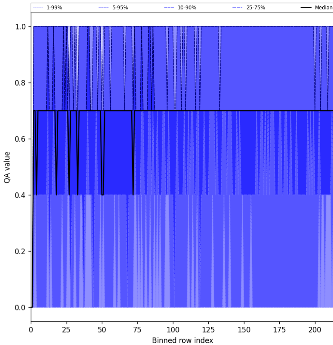
Figure 20: Along track statistics of “QA value” for 2024-12-19 to 2024-12-19
