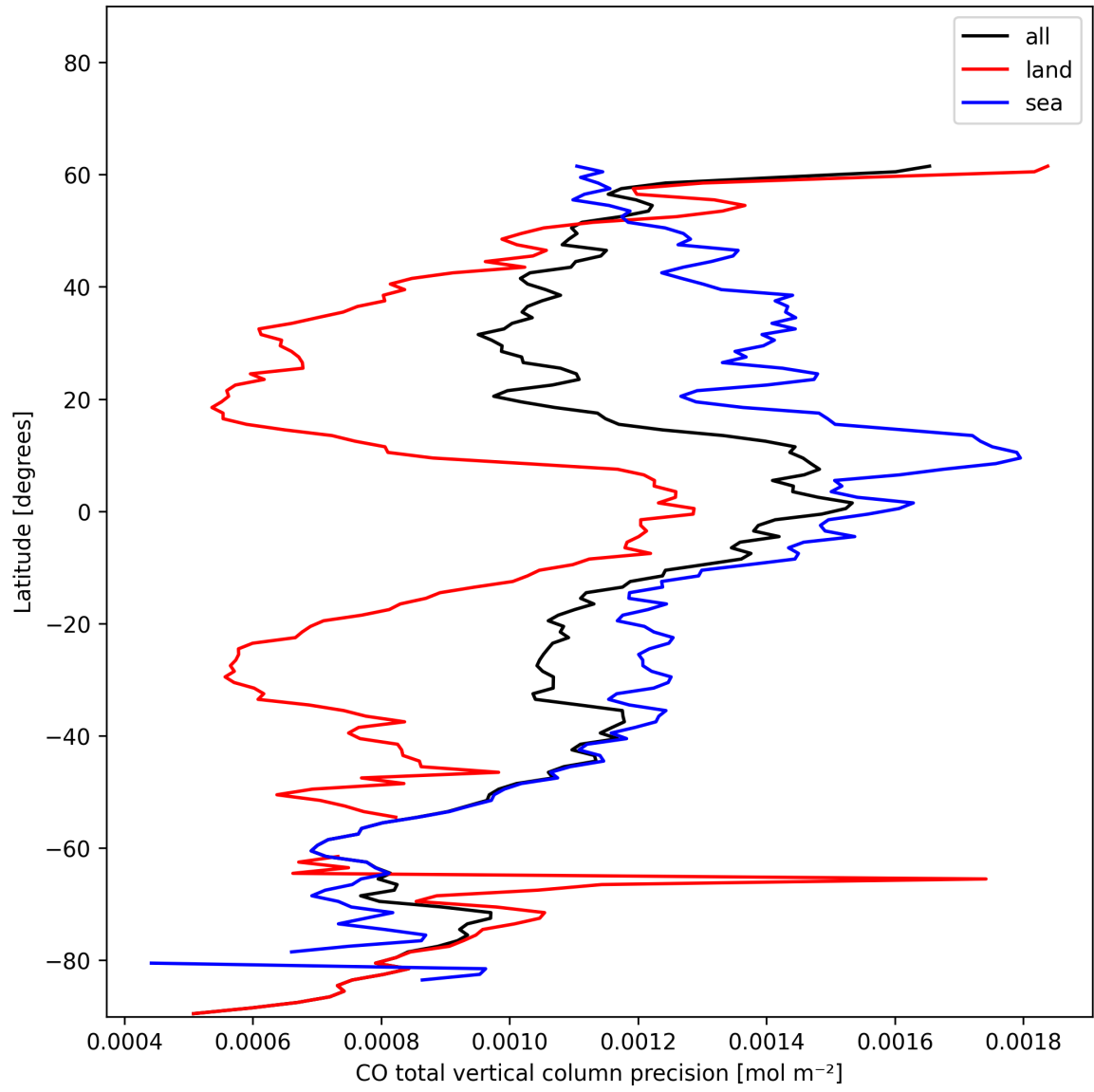
Figure 8: Zonal average of “CO total vertical column precision” for 2024-12-19 to 2024-12-19.
