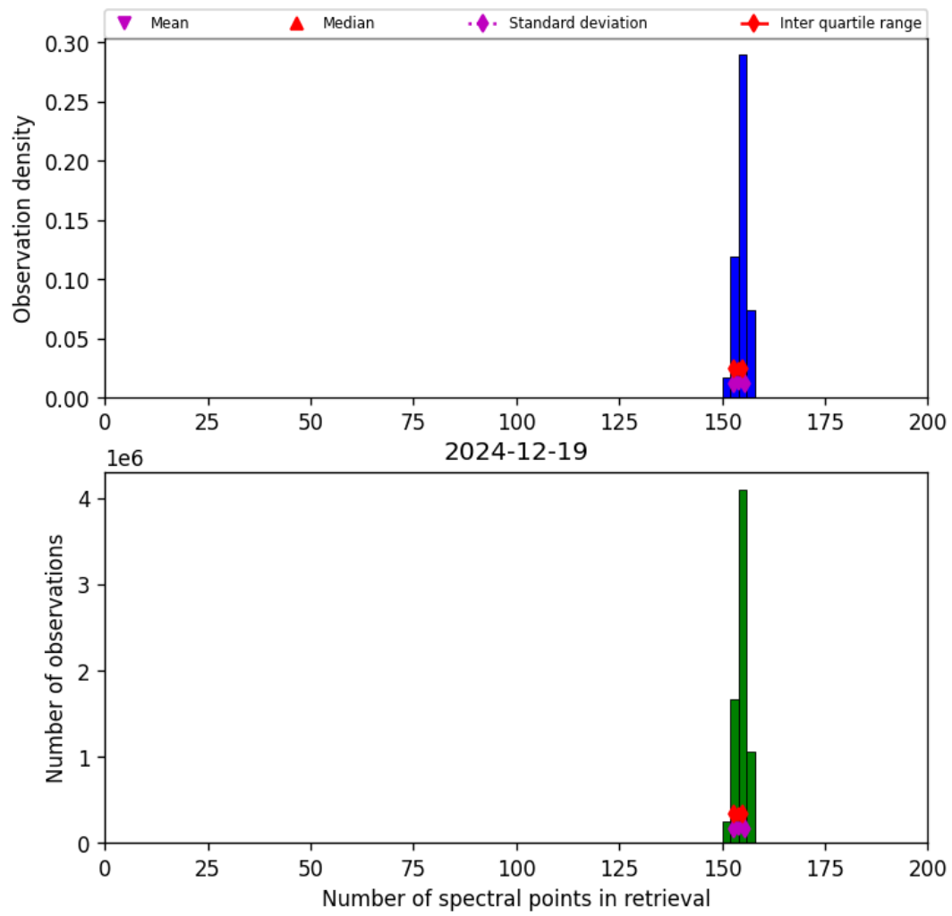
Figure 16: Histogram of “Number of spectral points in retrieval” for 2024-12-19 to 2024-12-19
