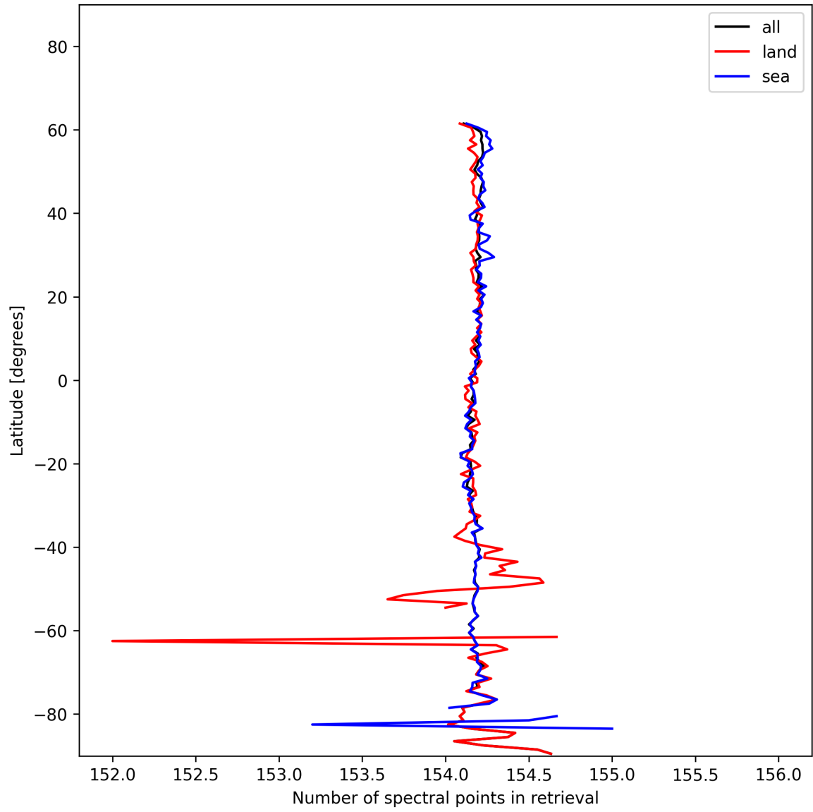
Figure 9: Zonal average of “Number of spectral points in retrieval” for 2024-12-19 to 2024-12-19.
