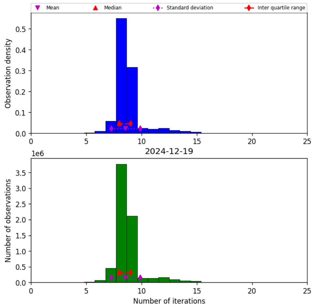
Figure 19: Histogram of “Number of iterations” for 2024-12-19 to 2024-12-19
