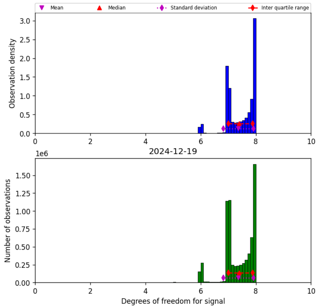
Figure 18: Histogram of “Degrees of freedom for signal” for 2024-12-19 to 2024-12-19
