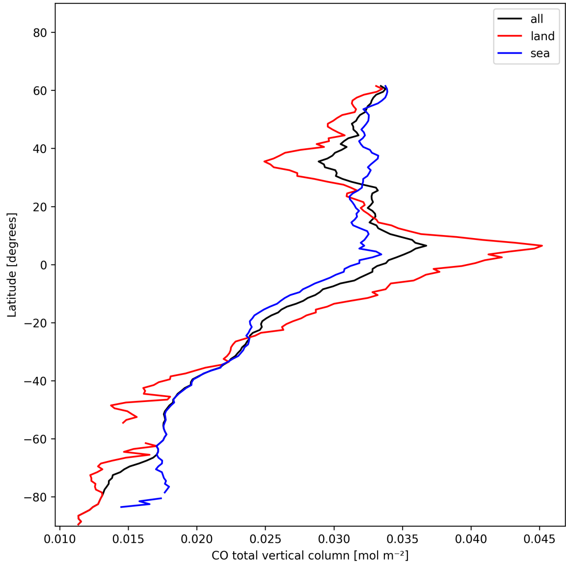
Figure 7: Zonal average of “CO total vertical column” for 2024-12-19 to 2024-12-19.
