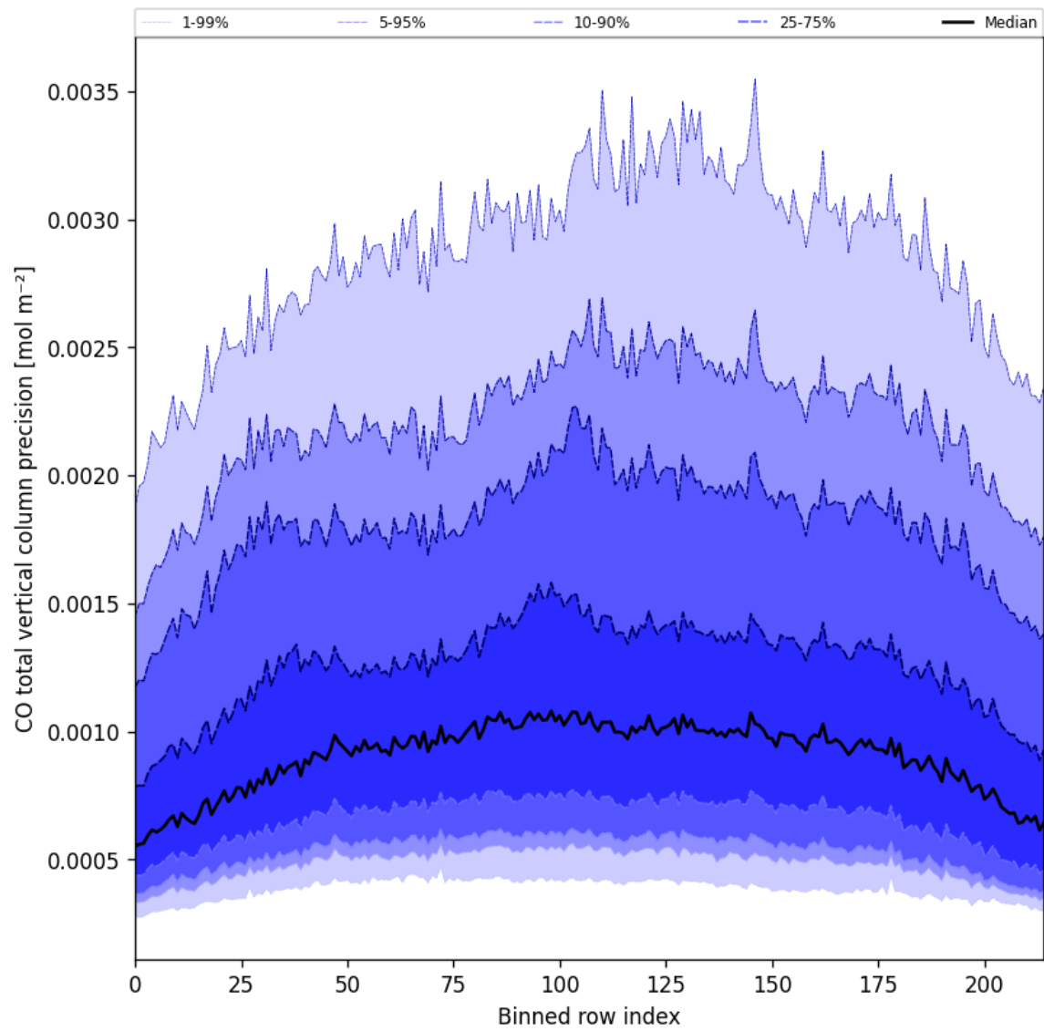
Figure 22: Along track statistics of “CO total vertical column precision” for 2024-12-19 to 2024-12-19
