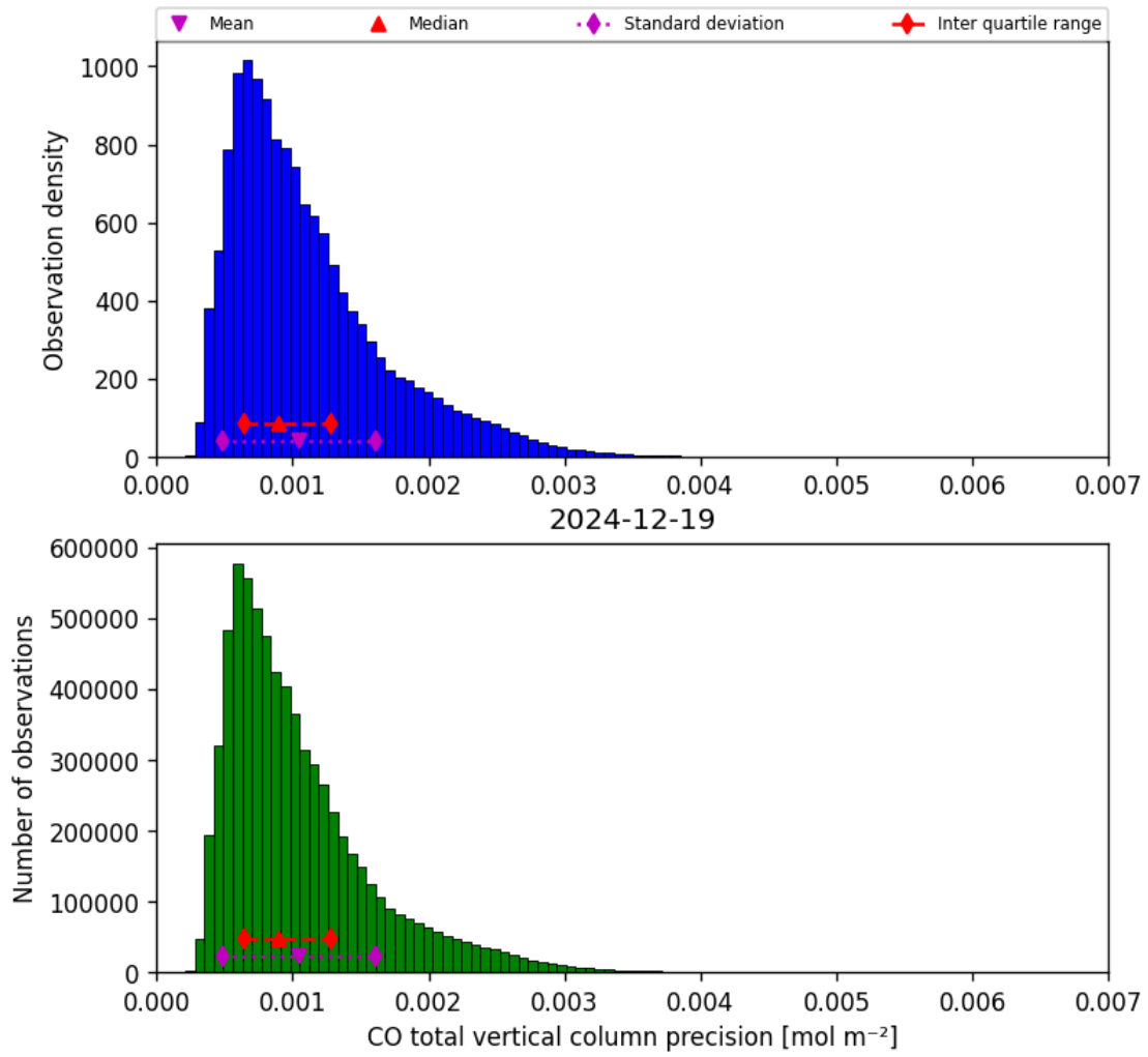
Figure 15: Histogram of “CO total vertical column precision” for 2024-12-19 to 2024-12-19
