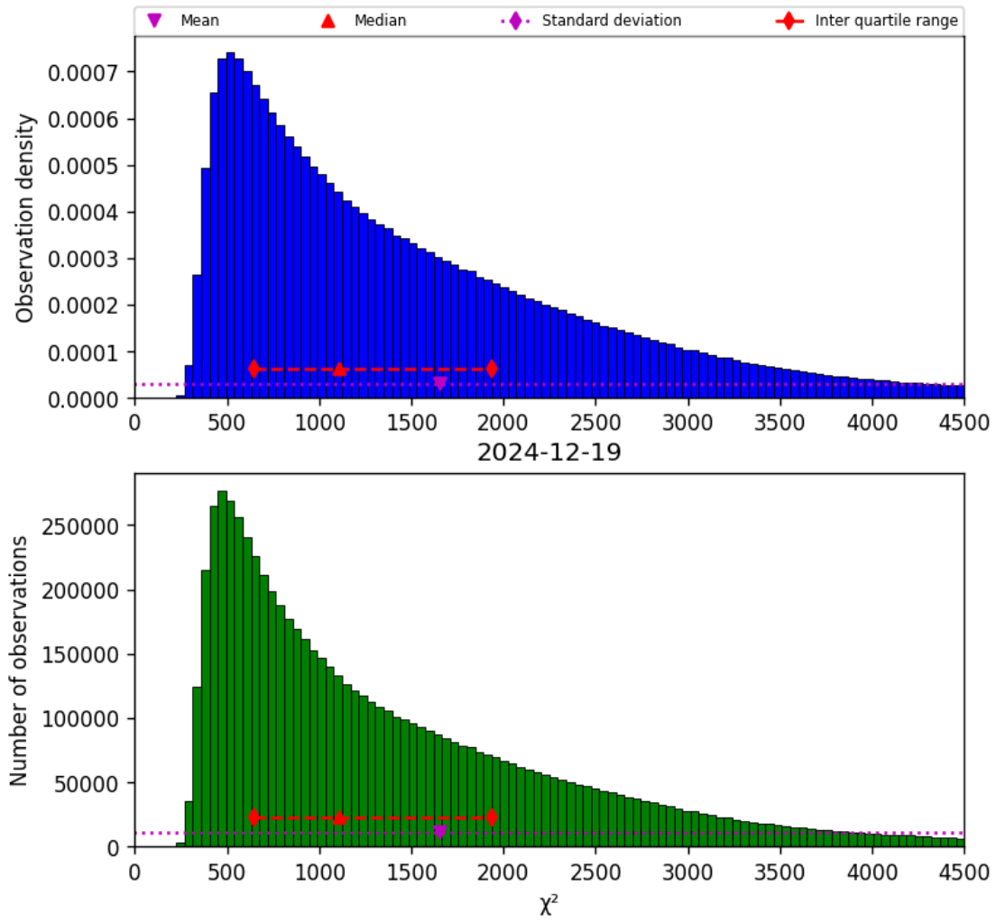
Figure 17: Histogram of " \chi^2 " for 2024-12-19 to 2024-12-19
