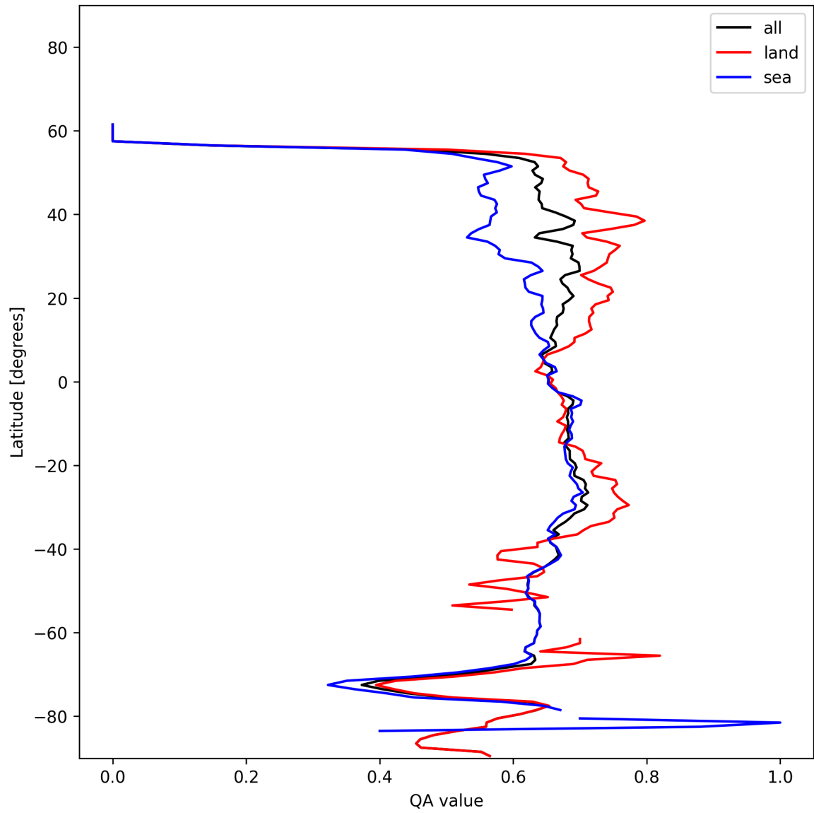
Figure 6: Zonal average of “QA value” for 2024-12-19 to 2024-12-19.
