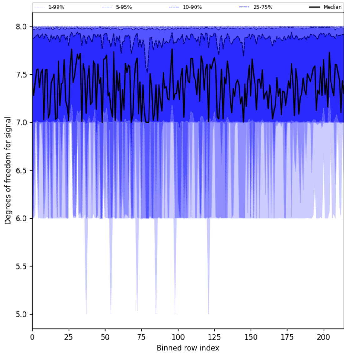
Figure 25: Along track statistics of “Degrees of freedom for signal” for 2024-12-19 to 2024-12-19
