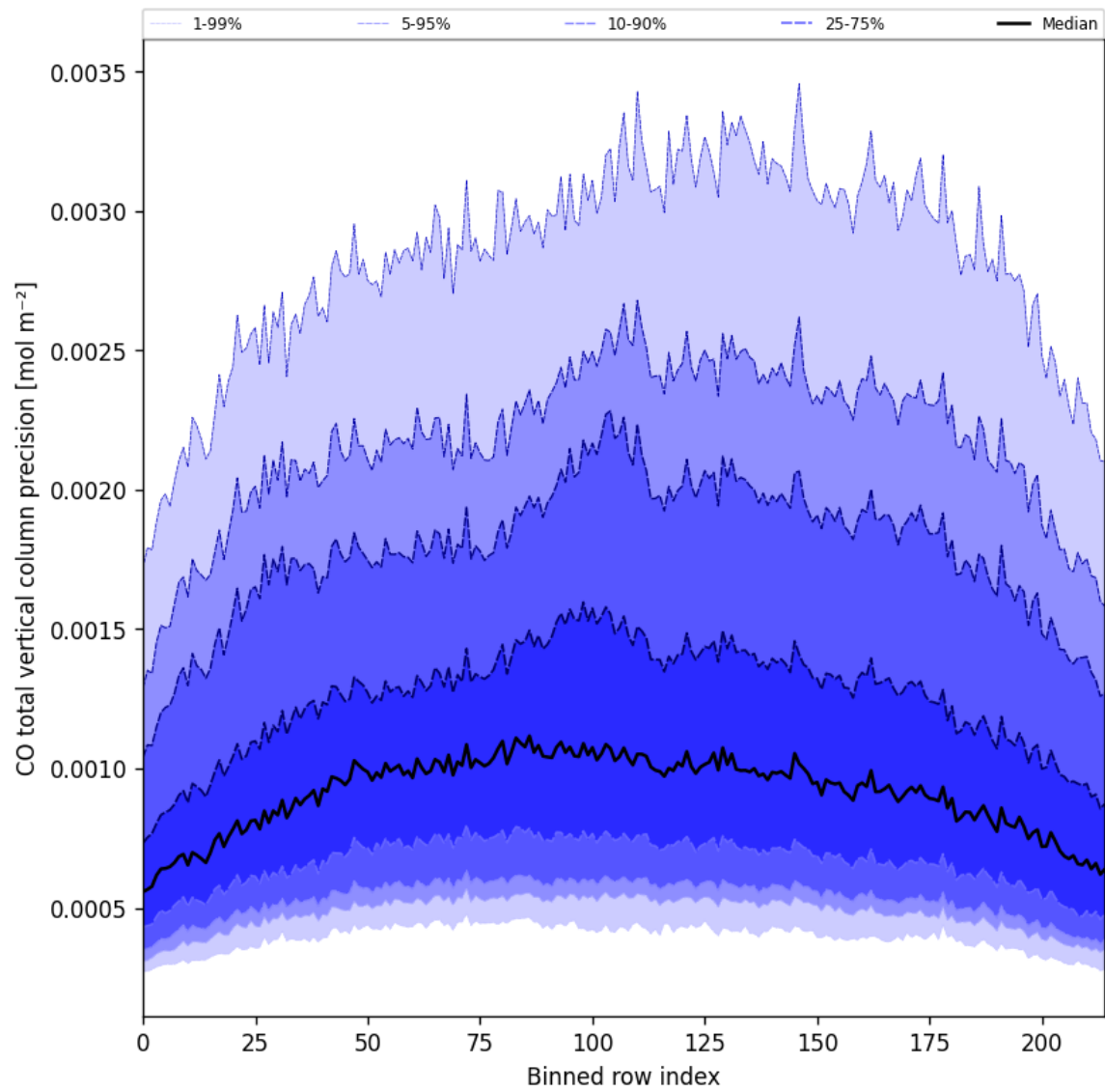
Figure 22: Along track statistics of “CO total vertical column precision” for 2024-12-22 to 2024-12-23
