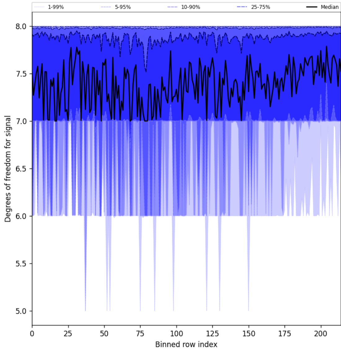
Figure 25: Along track statistics of “Degrees of freedom for signal” for 2024-12-22 to 2024-12-23
