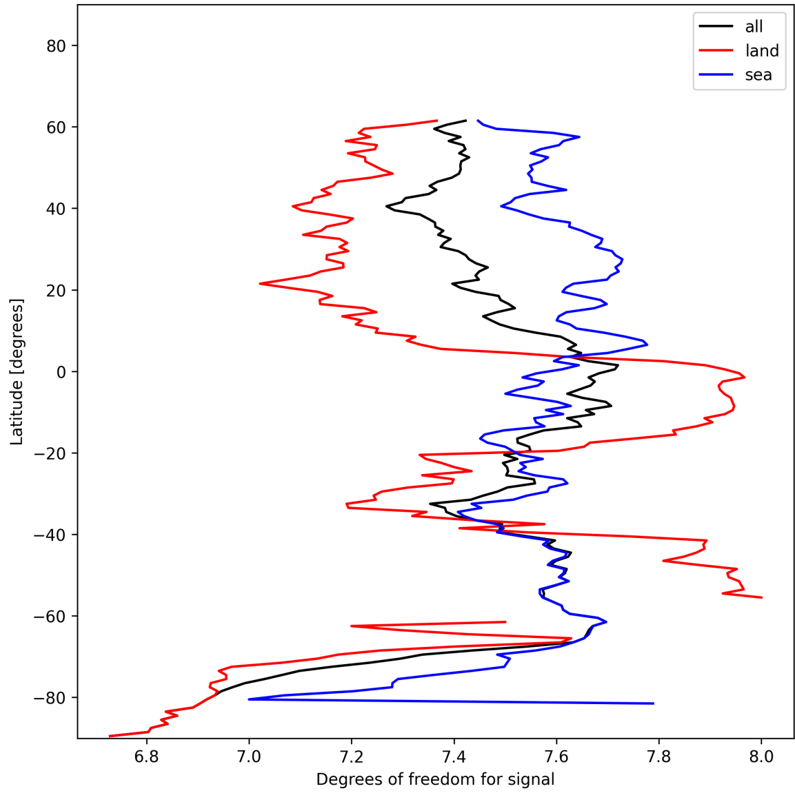
Figure 11: Zonal average of “Degrees of freedom for signal” for 2024-12-22 to 2024-12-23.
