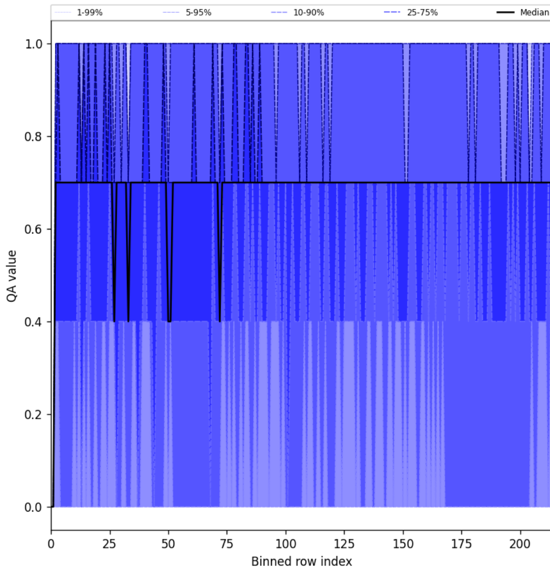
Figure 20: Along track statistics of “QA value” for 2024-12-22 to 2024-12-23
