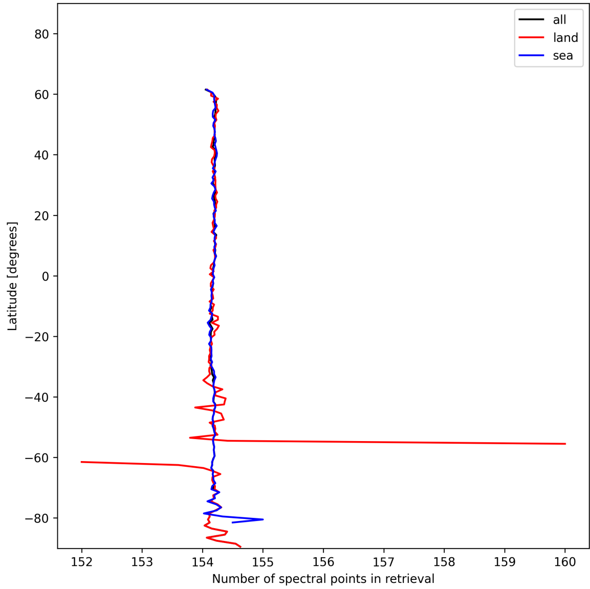
Figure 9: Zonal average of “Number of spectral points in retrieval” for 2024-12-22 to 2024-12-23.
