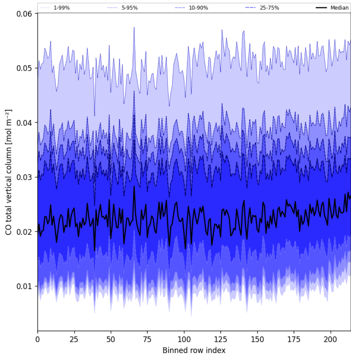
Figure 21: Along track statistics of “CO total vertical column” for 2024-12-22 to 2024-12-23
