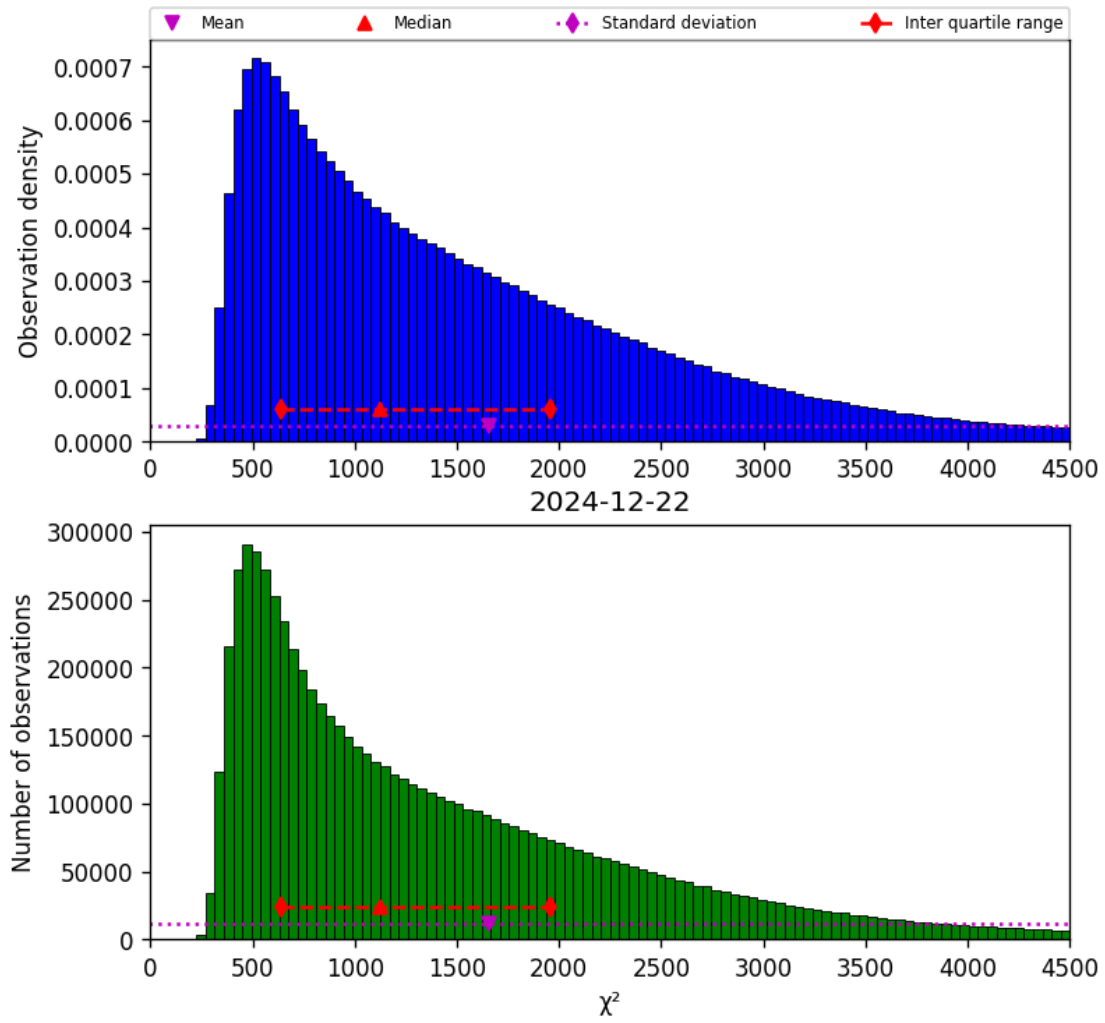
Figure 17: Histogram of “ \chi^2 ” for 2024-12-22 to 2024-12-23
