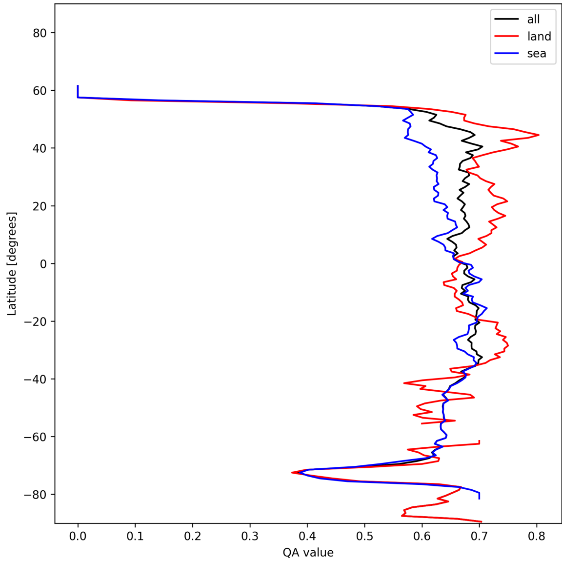
Figure 6: Zonal average of “QA value” for 2024-12-22 to 2024-12-23.
