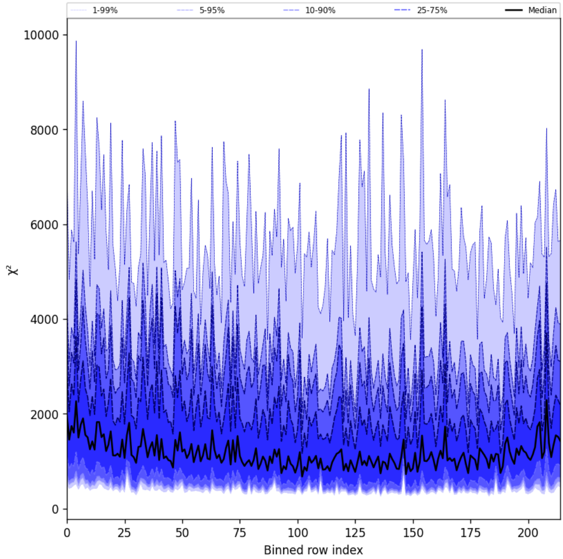
Figure 24: Along track statistics of “ \chi^2 ” for 2024-12-22 to 2024-12-23
