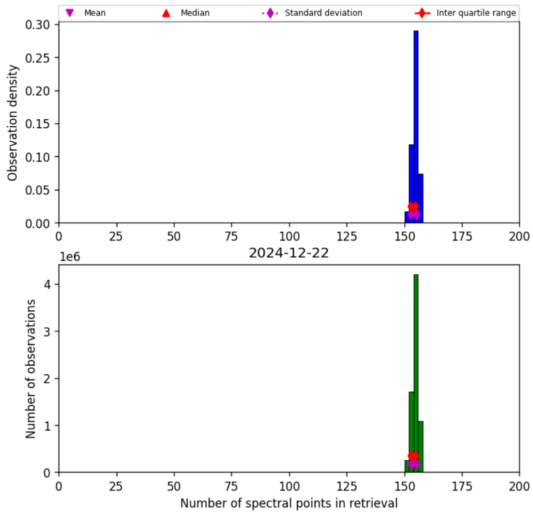
Figure 16: Histogram of “Number of spectral points in retrieval” for 2024-12-22 to 2024-12-23
