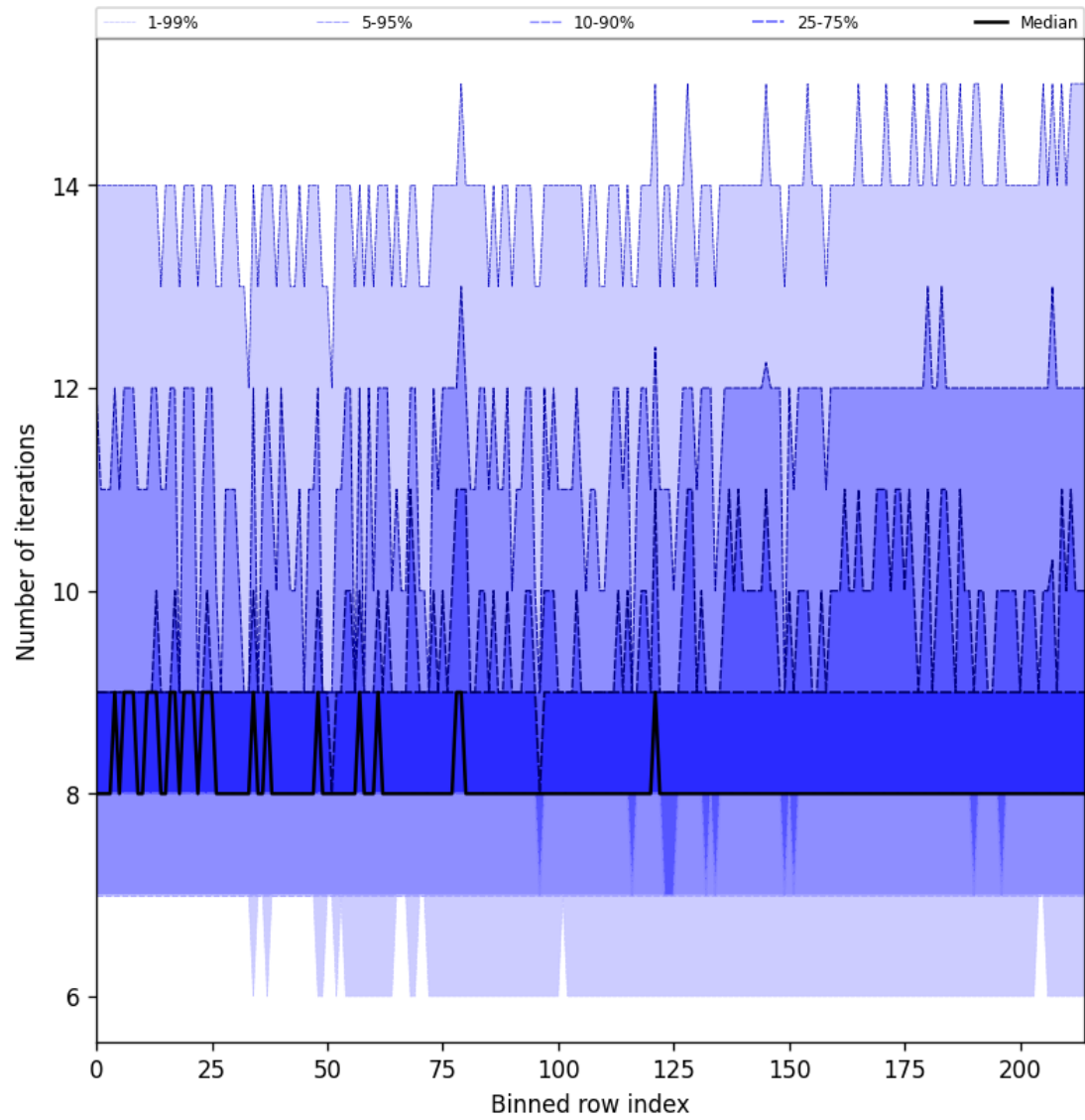
Figure 26: Along track statistics of “Number of iterations” for 2024-12-22 to 2024-12-23
