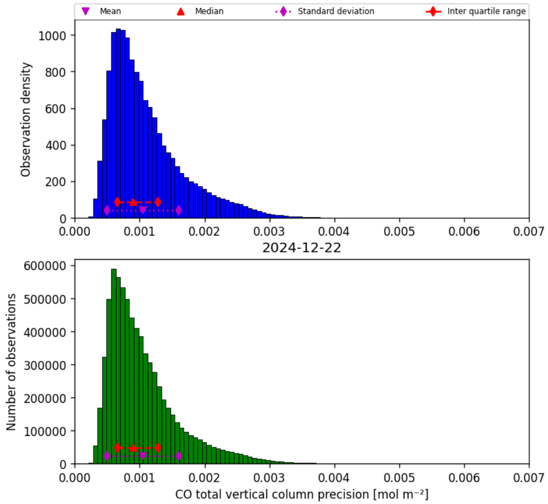
Figure 15: Histogram of “CO total vertical column precision” for 2024-12-22 to 2024-12-23
