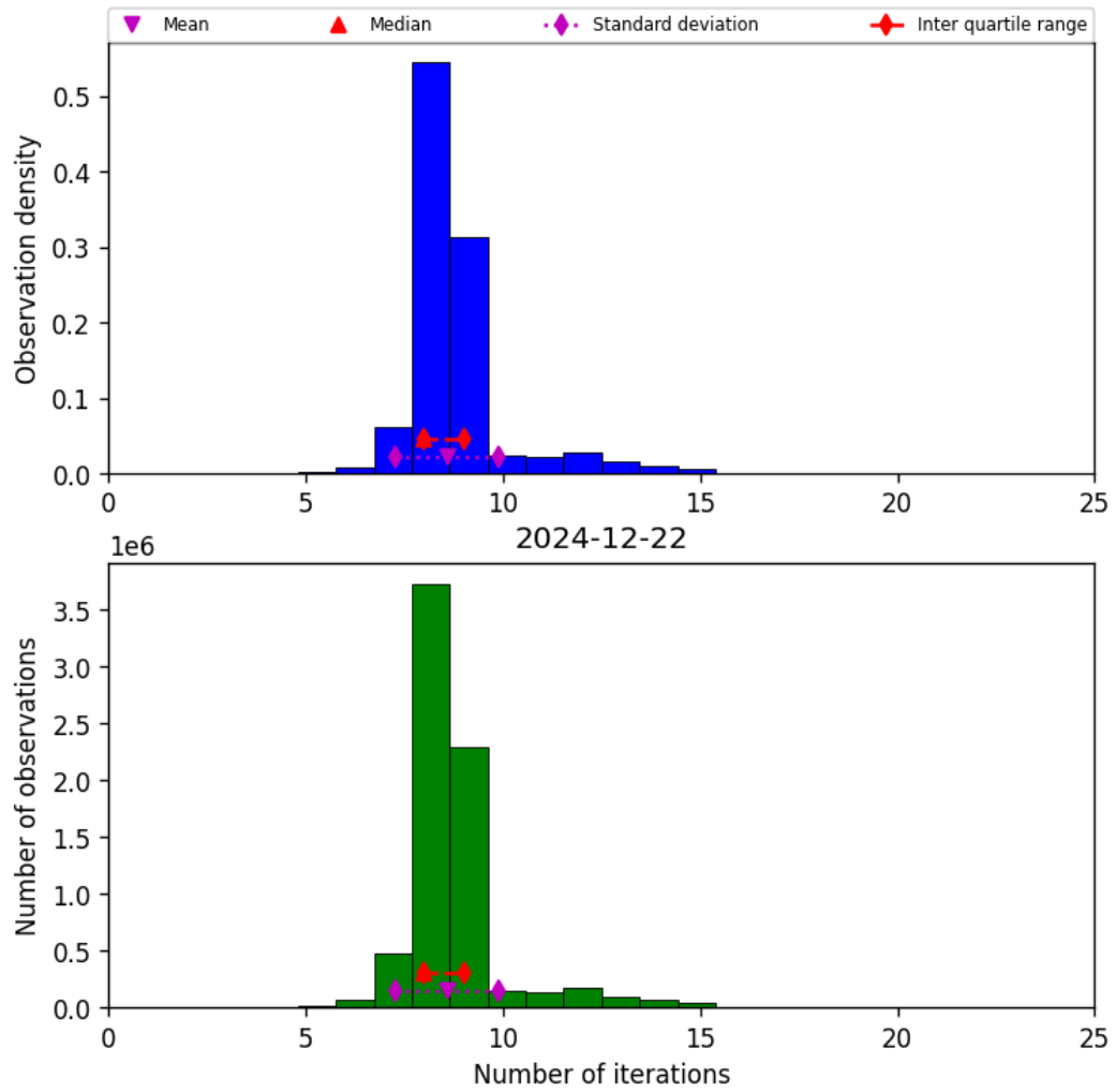
Figure 19: Histogram of “Number of iterations” for 2024-12-22 to 2024-12-23
