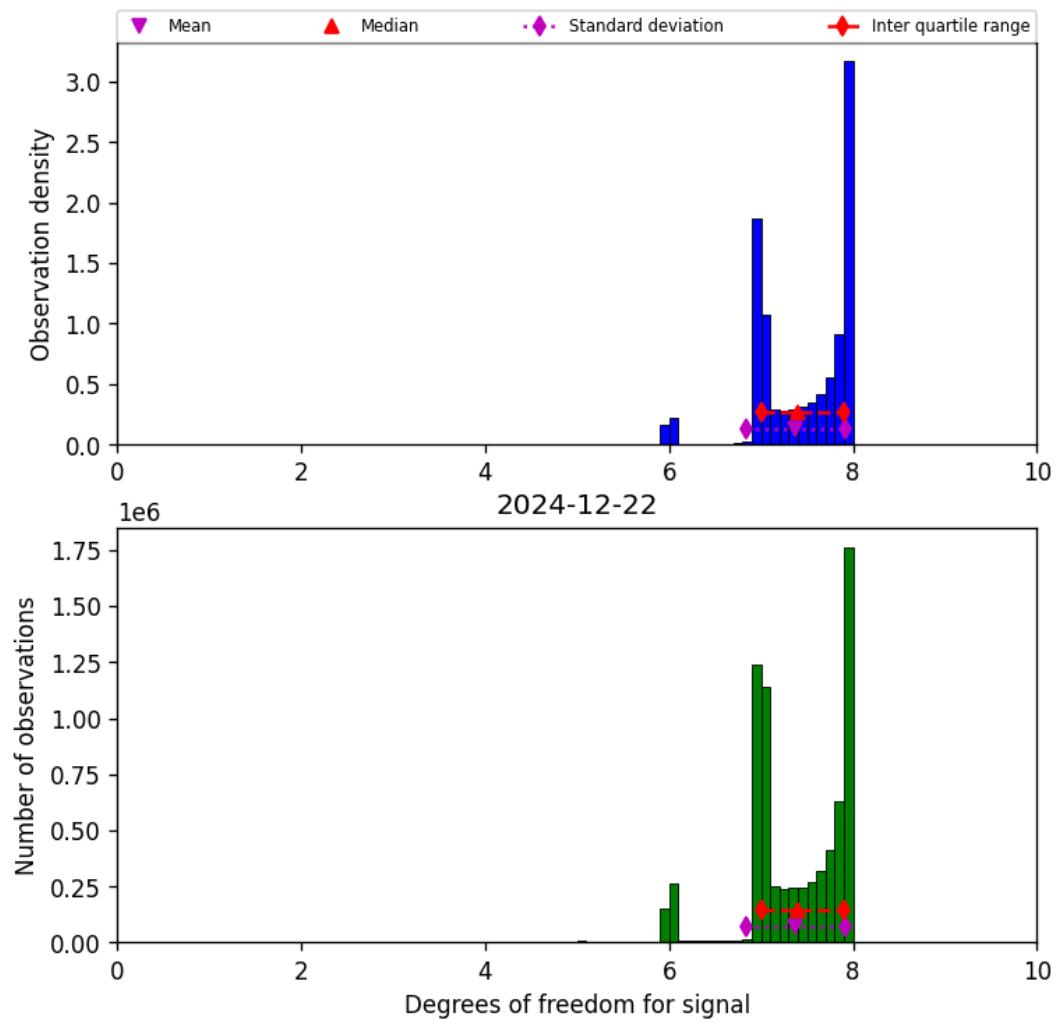
Figure 18: Histogram of “Degrees of freedom for signal” for 2024-12-22 to 2024-12-23
