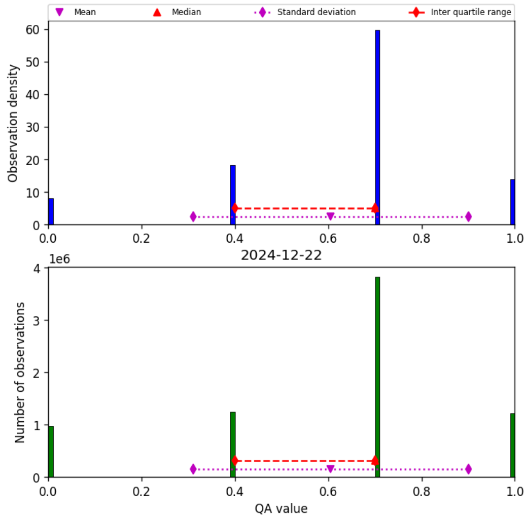
Figure 13: Histogram of “QA value” for 2024-12-22 to 2024-12-23
