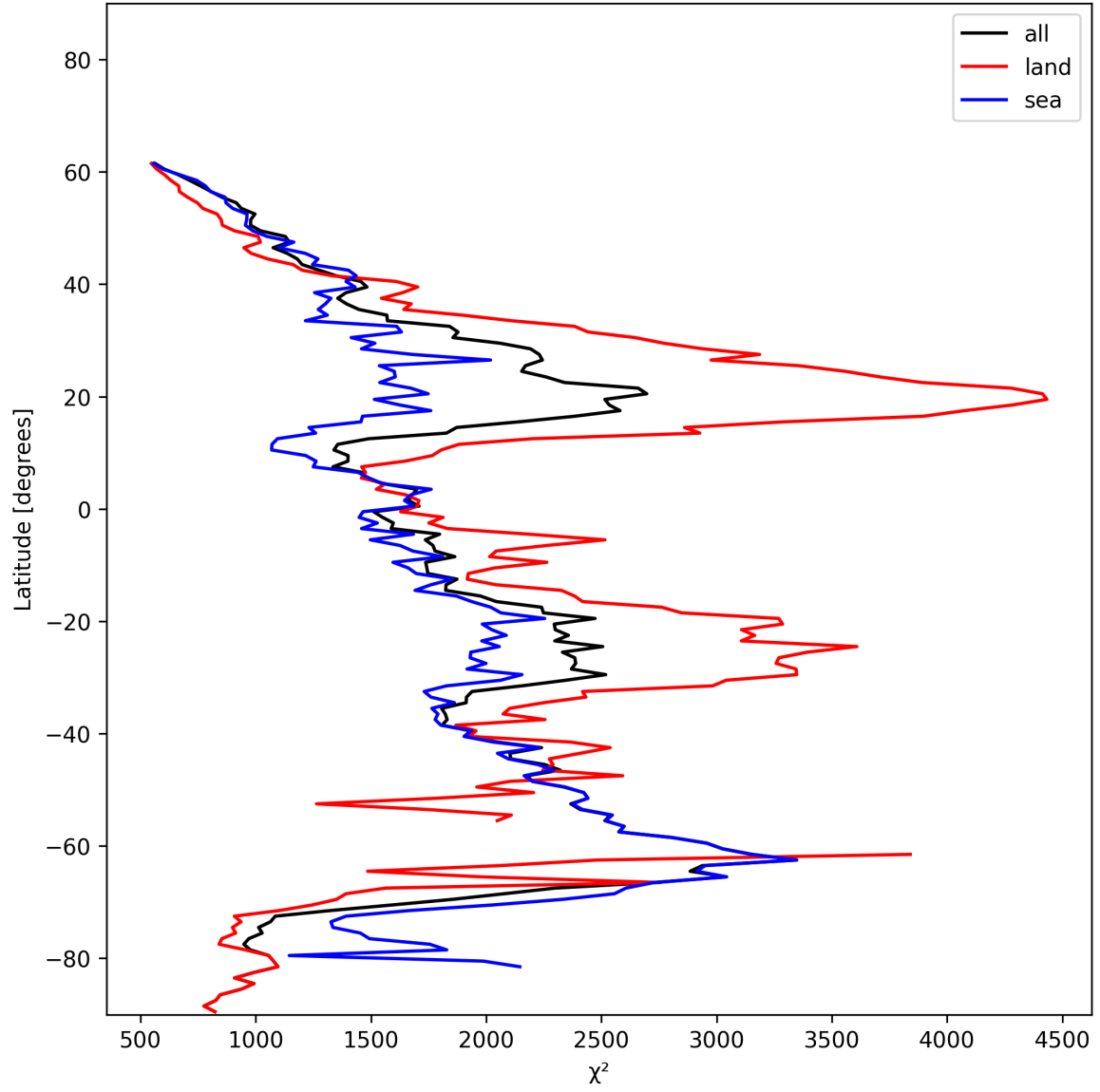
Figure 10: Zonal average of “ \chi^2 ” for 2024-12-22 to 2024-12-23.
