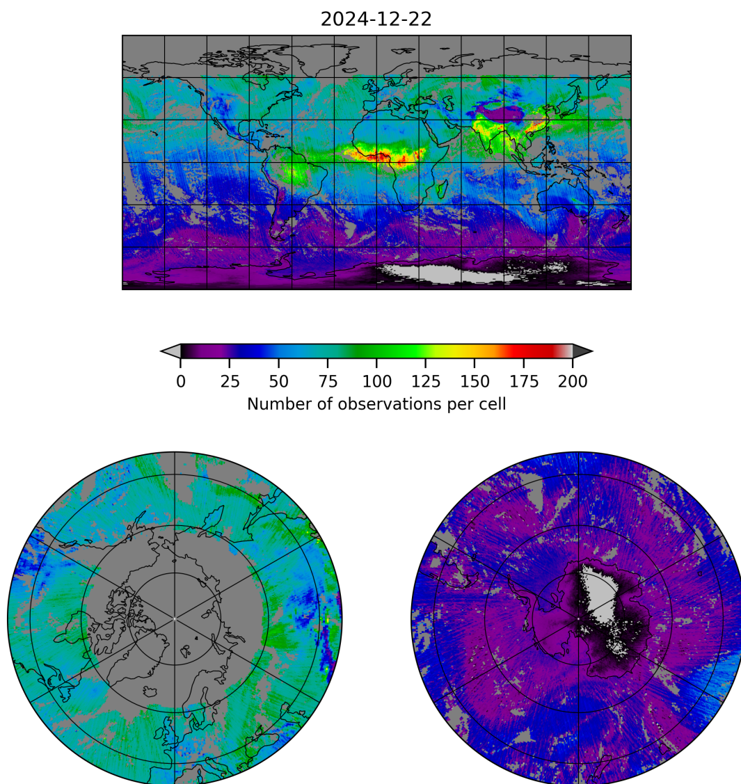
Figure 5: Map of the number of observations for 2024-12-22 to 2024-12-23
