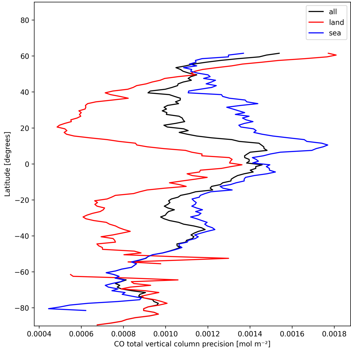
Figure 8: Zonal average of “CO total vertical column precision” for 2024-12-22 to 2024-12-23.
