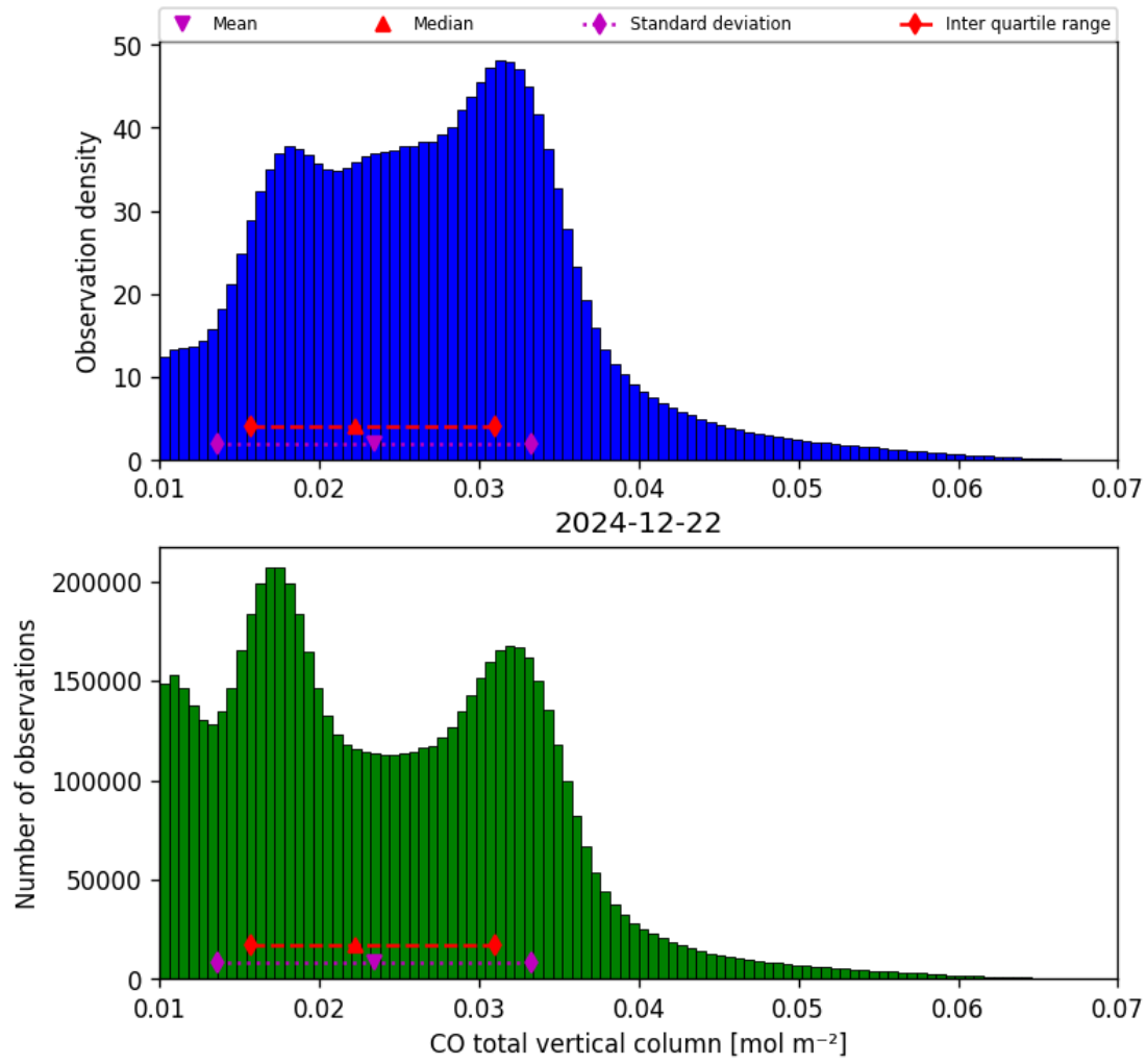
Figure 14: Histogram of “CO total vertical column” for 2024-12-22 to 2024-12-23
