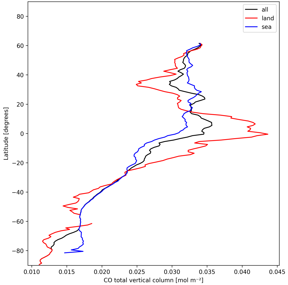
Figure 7: Zonal average of “CO total vertical column” for 2024-12-22 to 2024-12-23.
