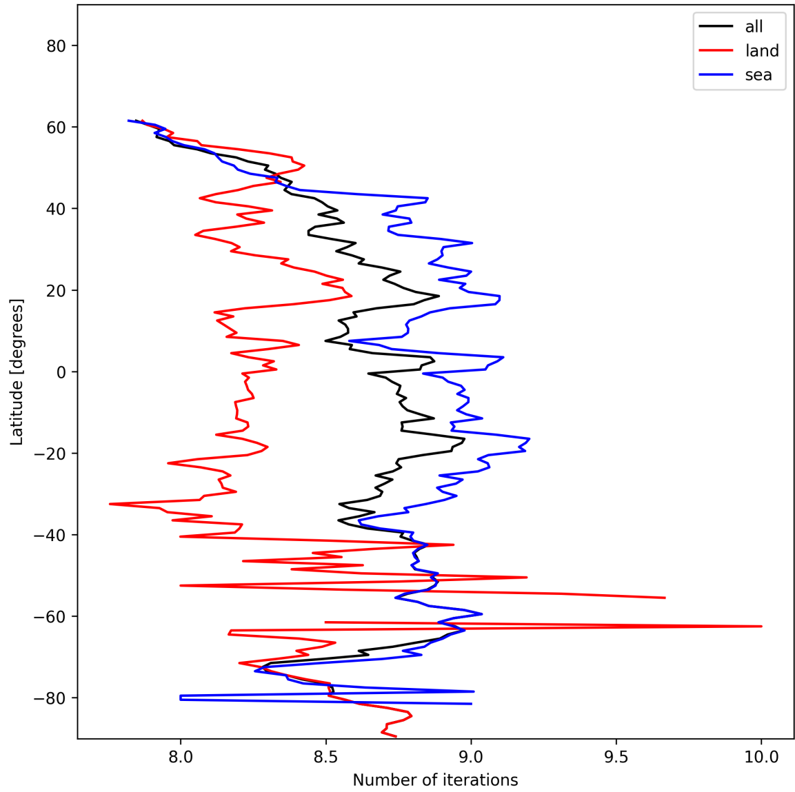
Figure 12: Zonal average of “Number of iterations” for 2024-12-22 to 2024-12-23.
