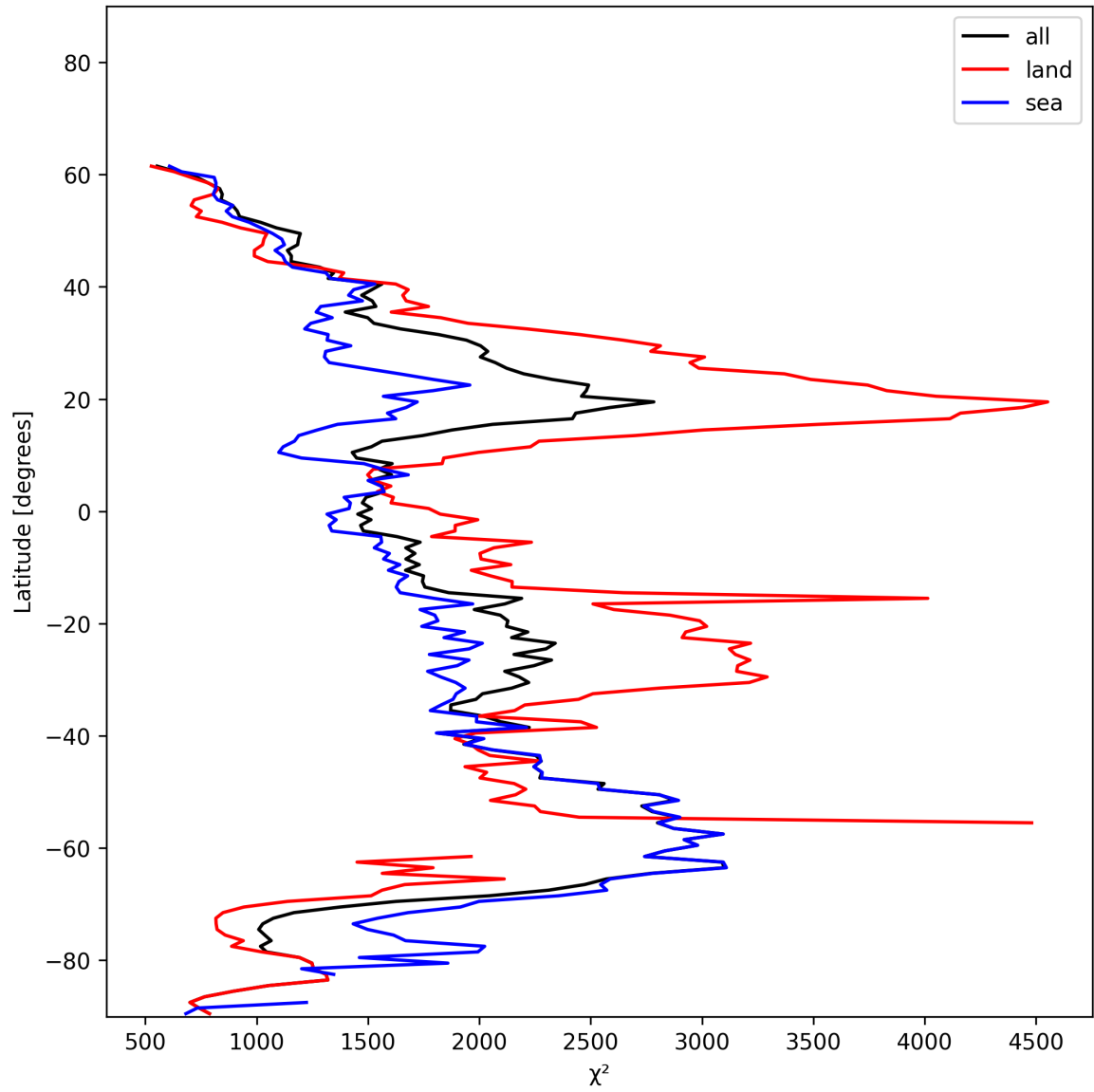
Figure 10: Zonal average of “ \chi^2 ” for 2024-12-23 to 2024-12-24.
