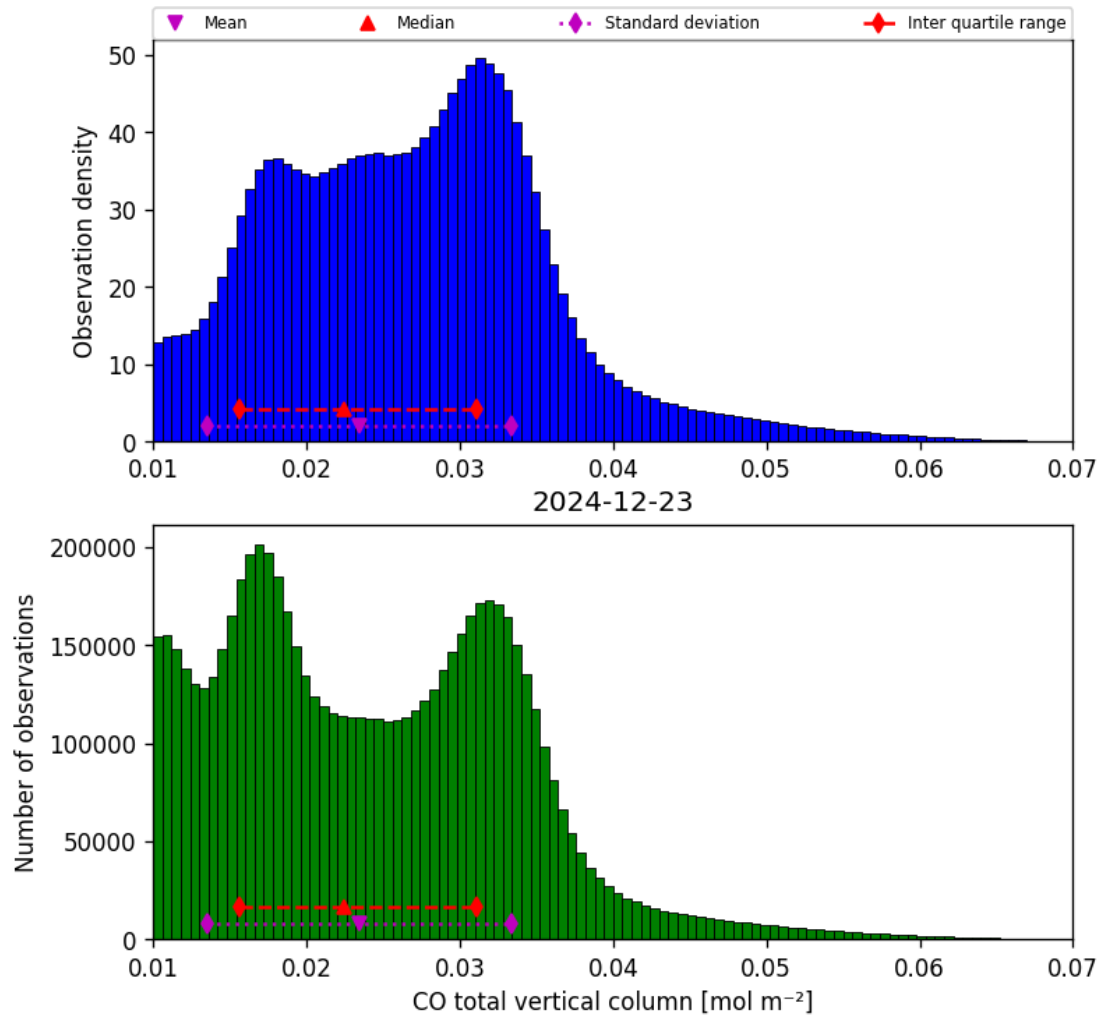
Figure 14: Histogram of “CO total vertical column” for 2024-12-23 to 2024-12-24
