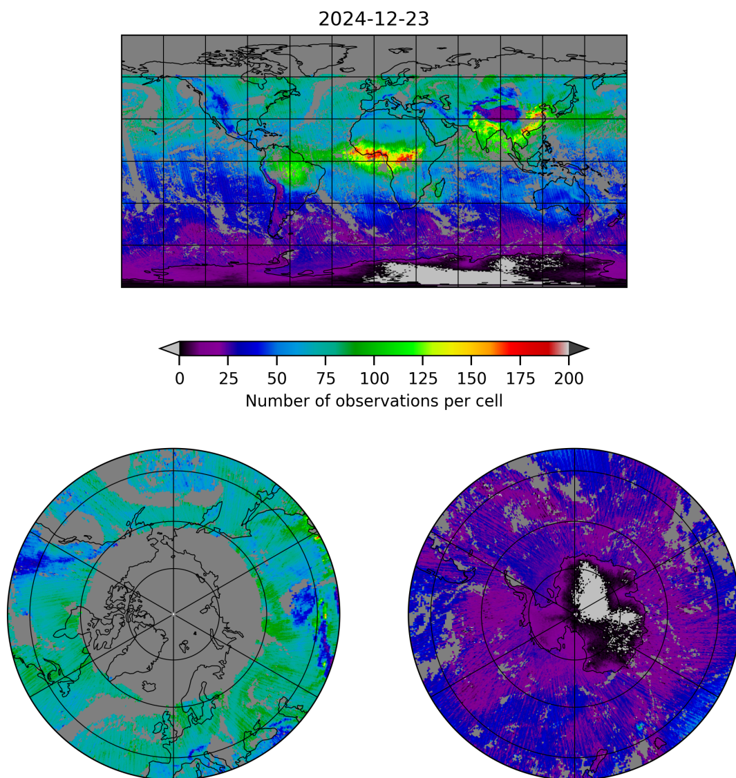
Figure 5: Map of the number of observations for 2024-12-23 to 2024-12-24
