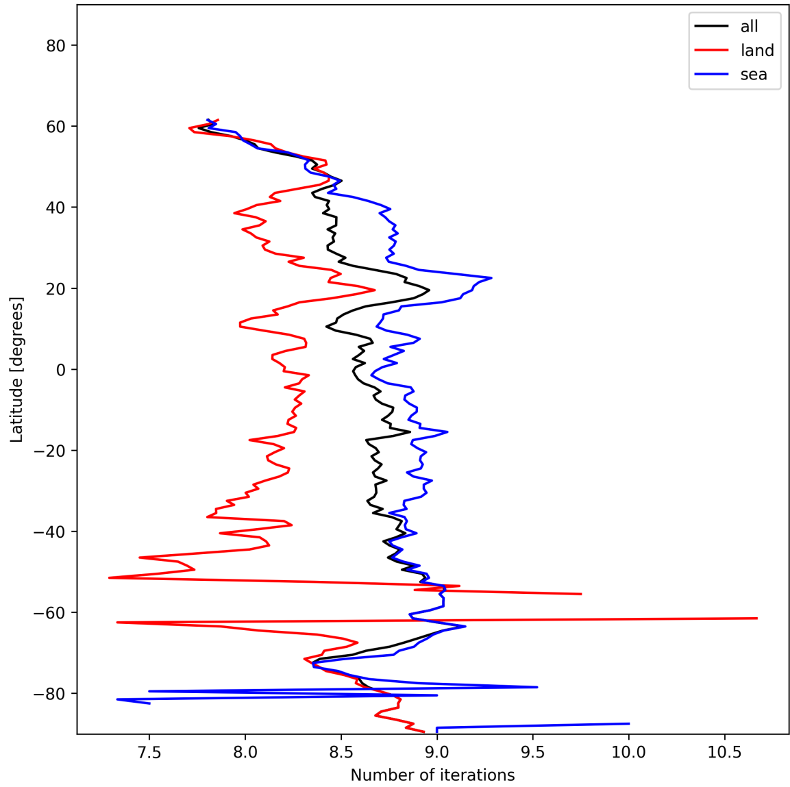
Figure 12: Zonal average of “Number of iterations” for 2024-12-23 to 2024-12-24.
