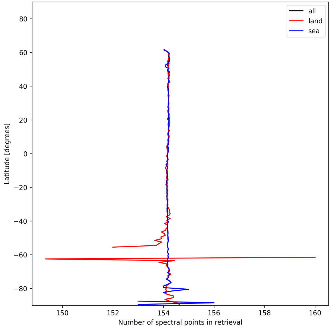
Figure 9: Zonal average of “Number of spectral points in retrieval” for 2024-12-23 to 2024-12-24.
