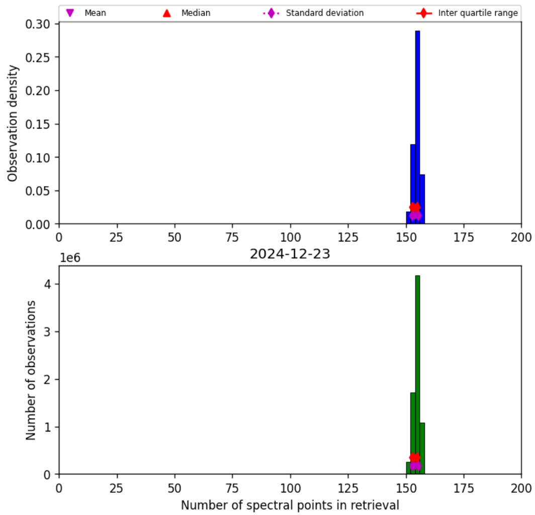
Figure 16: Histogram of “Number of spectral points in retrieval” for 2024-12-23 to 2024-12-24
