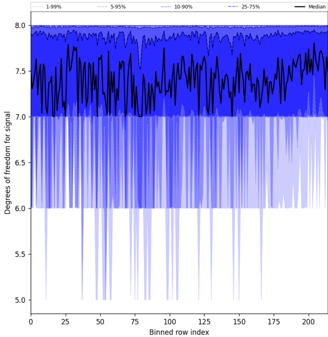
Figure 25: Along track statistics of “Degrees of freedom for signal” for 2024-12-23 to 2024-12-24
