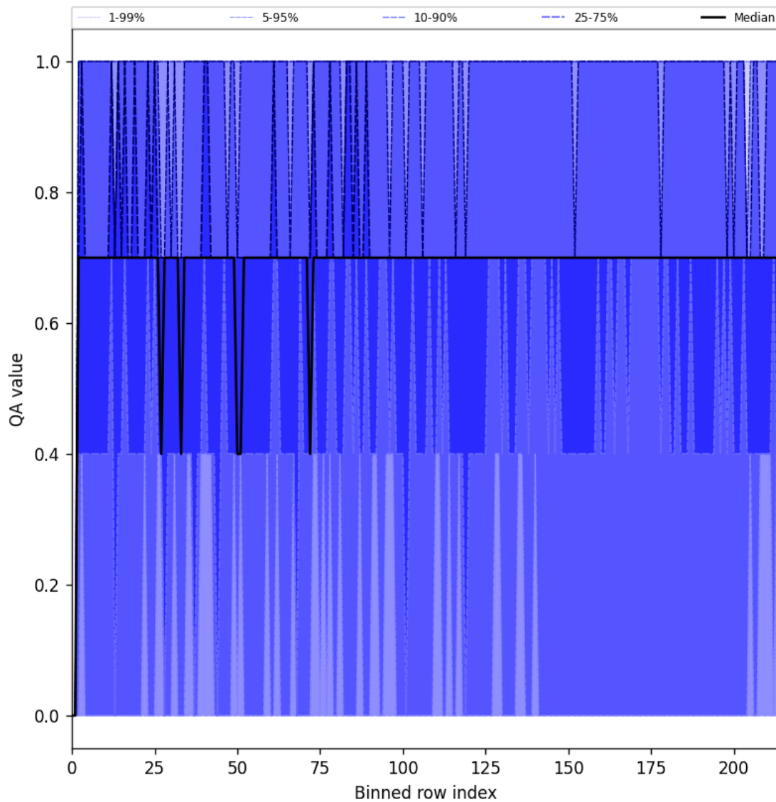
Figure 20: Along track statistics of “QA value” for 2024-12-23 to 2024-12-24
