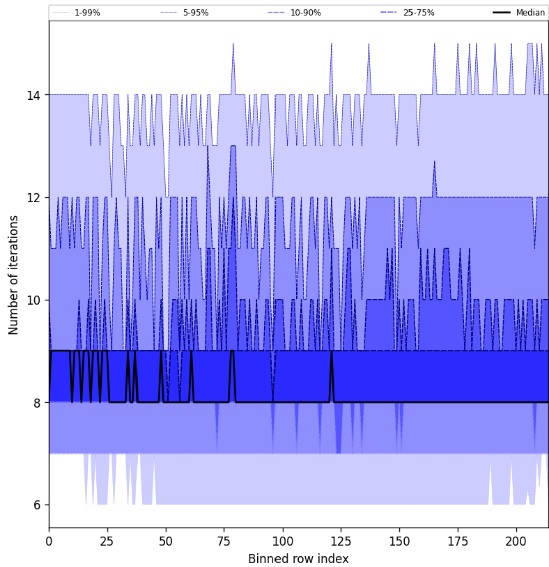
Figure 26: Along track statistics of “Number of iterations” for 2024-12-23 to 2024-12-24
