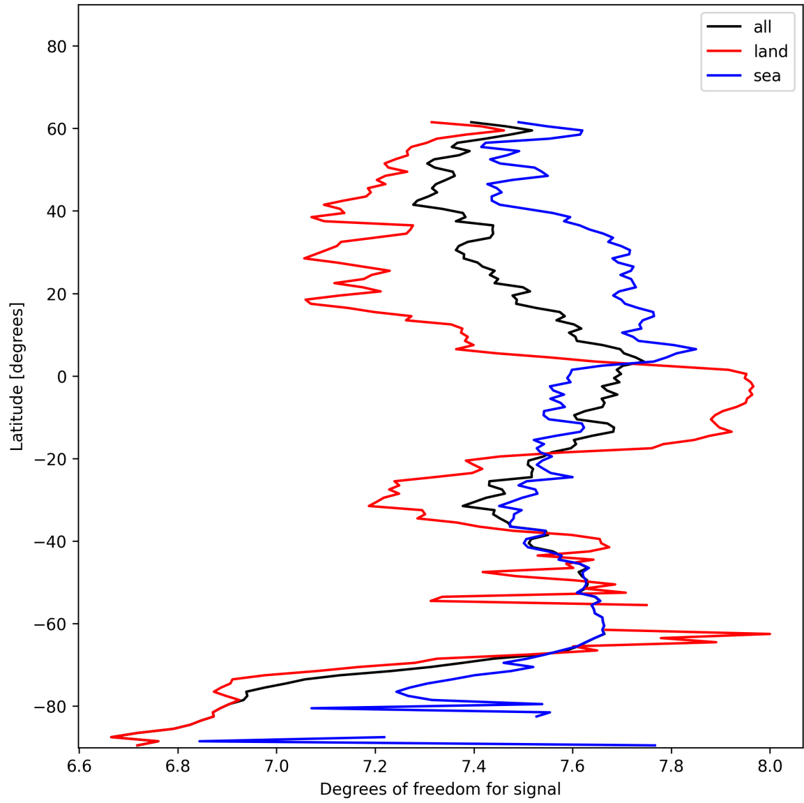
Figure 11: Zonal average of “Degrees of freedom for signal” for 2024-12-23 to 2024-12-24.
