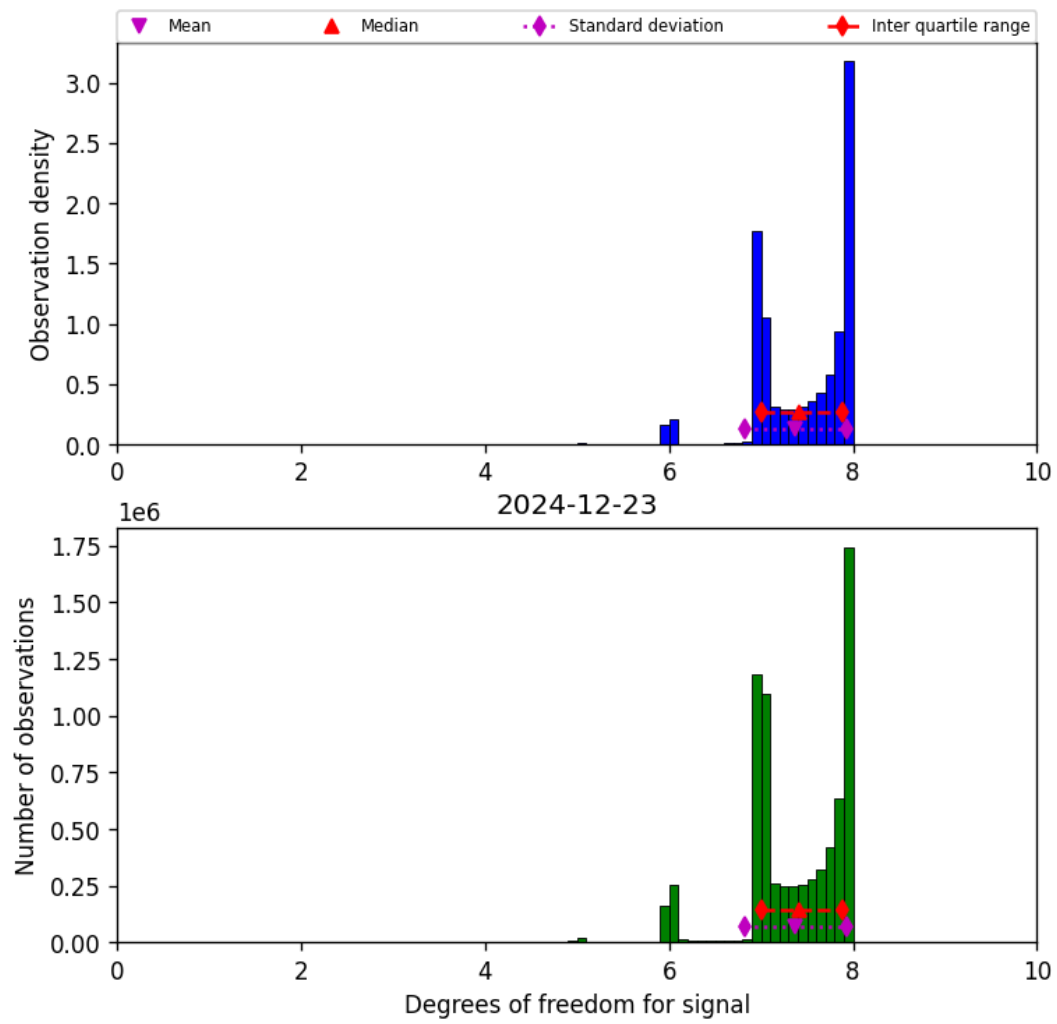
Figure 18: Histogram of “Degrees of freedom for signal” for 2024-12-23 to 2024-12-24
