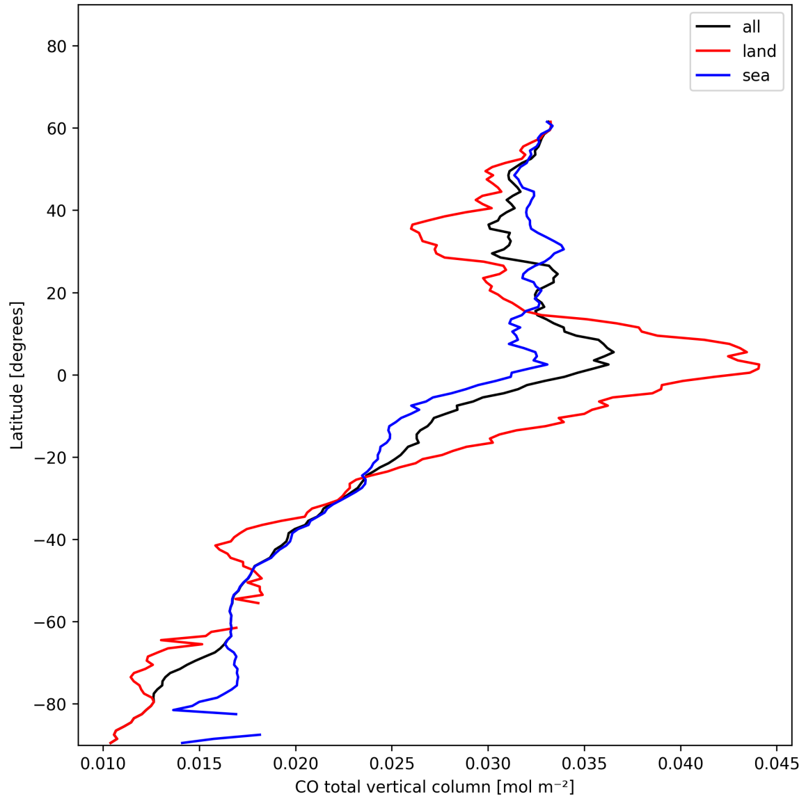
Figure 7: Zonal average of “CO total vertical column” for 2024-12-23 to 2024-12-24.
