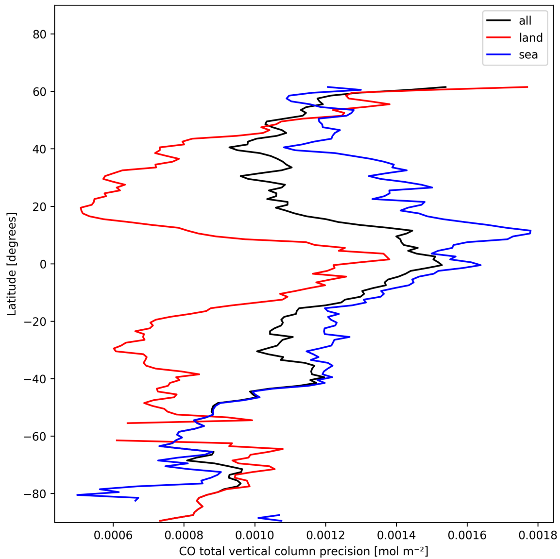
Figure 8: Zonal average of “CO total vertical column precision” for 2024-12-23 to 2024-12-24.
