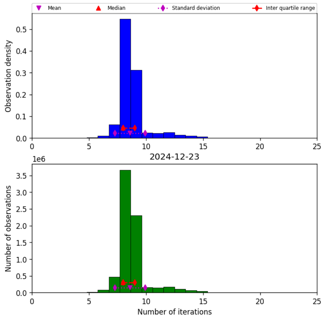
Figure 19: Histogram of “Number of iterations” for 2024-12-23 to 2024-12-24
