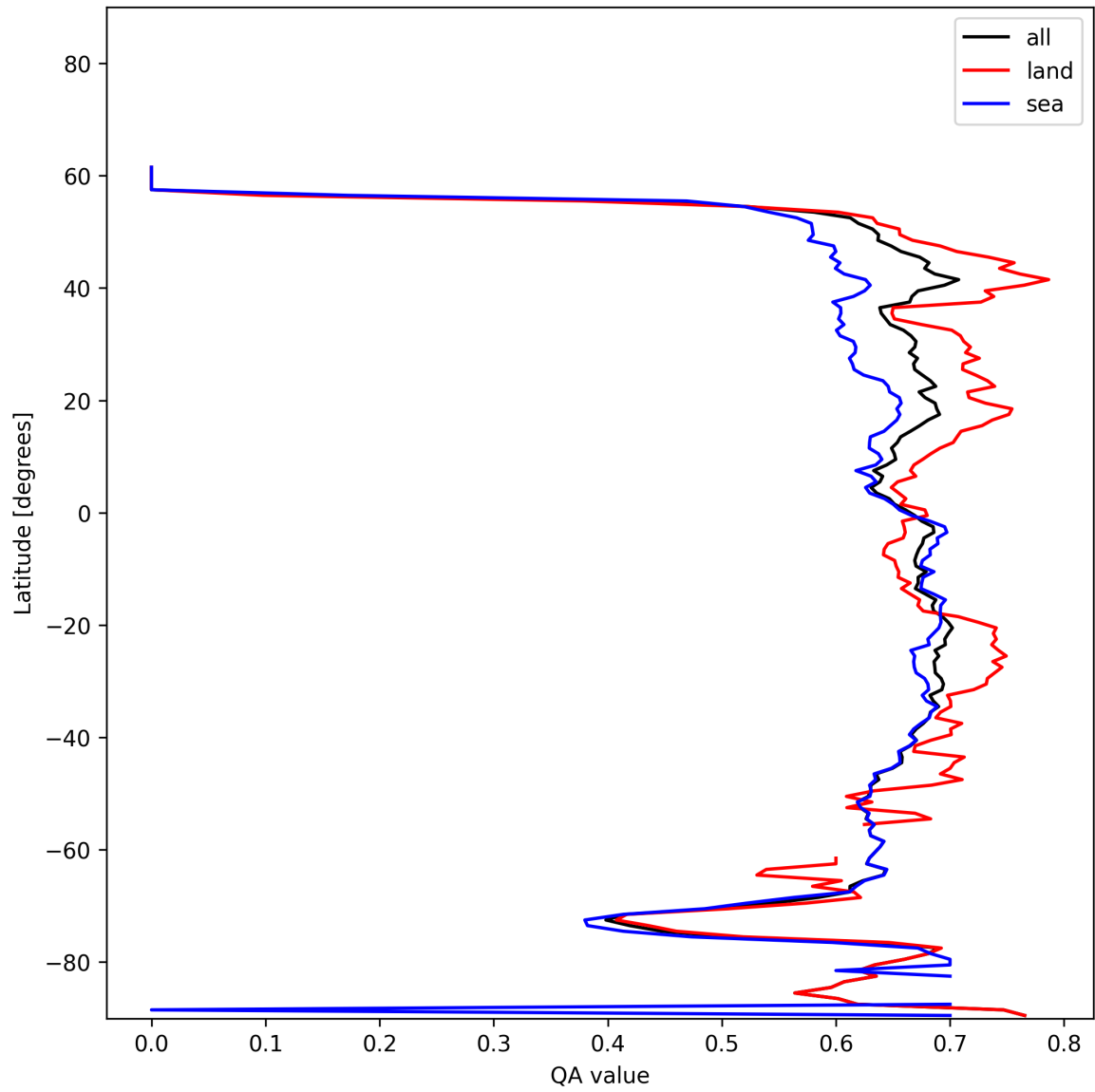
Figure 6: Zonal average of “QA value” for 2024-12-23 to 2024-12-24.
