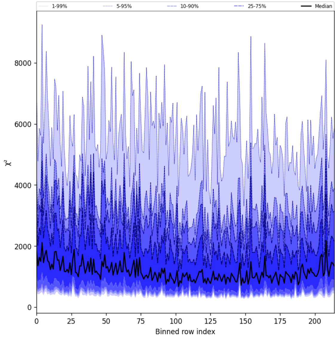
Figure 24: Along track statistics of “ \chi^2 ” for 2024-12-23 to 2024-12-24
