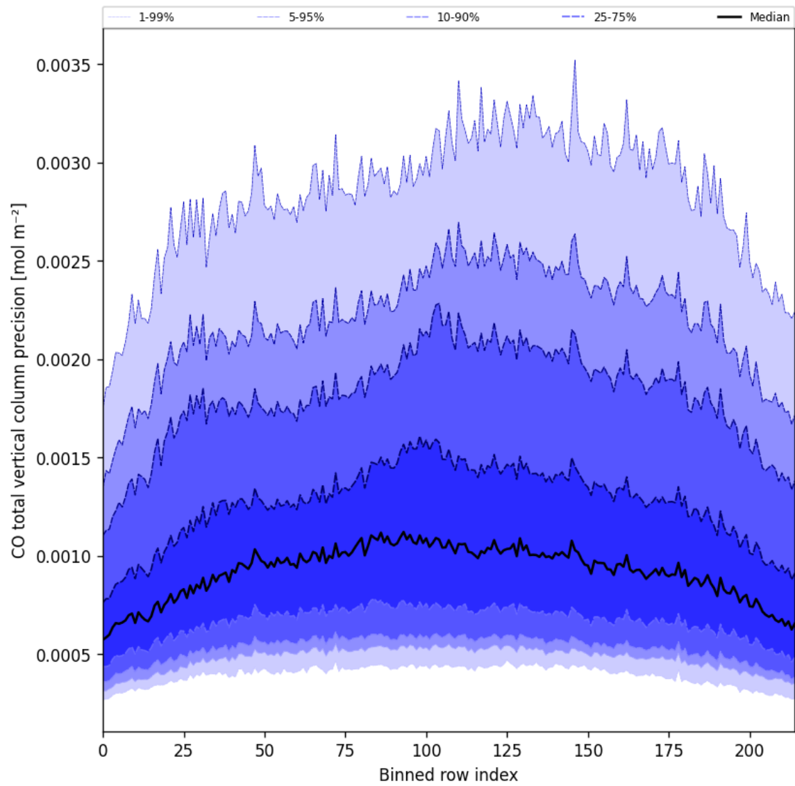
Figure 22: Along track statistics of “CO total vertical column precision” for 2024-12-23 to 2024-12-24
