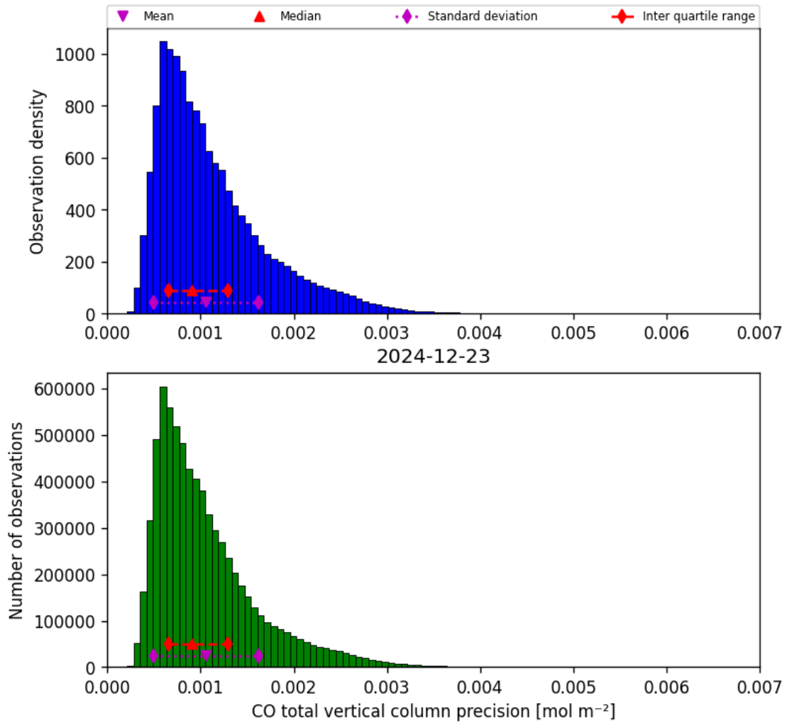
Figure 15: Histogram of “CO total vertical column precision” for 2024-12-23 to 2024-12-24
