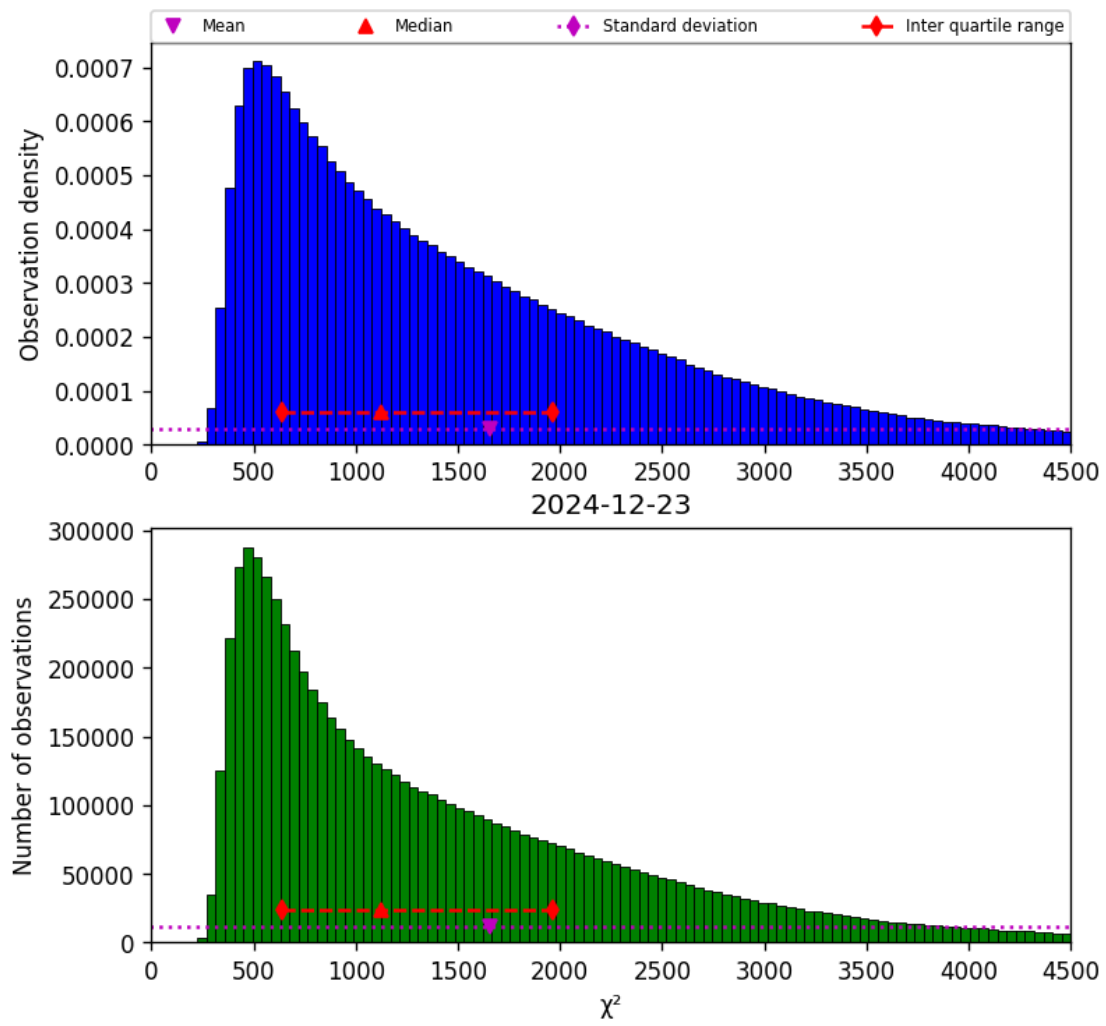
Figure 17: Histogram of “ \chi^2 ” for 2024-12-23 to 2024-12-24
