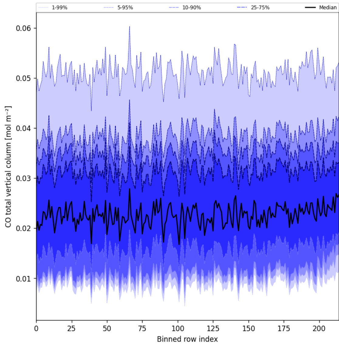
Figure 21: Along track statistics of “CO total vertical column” for 2024-12-23 to 2024-12-24
