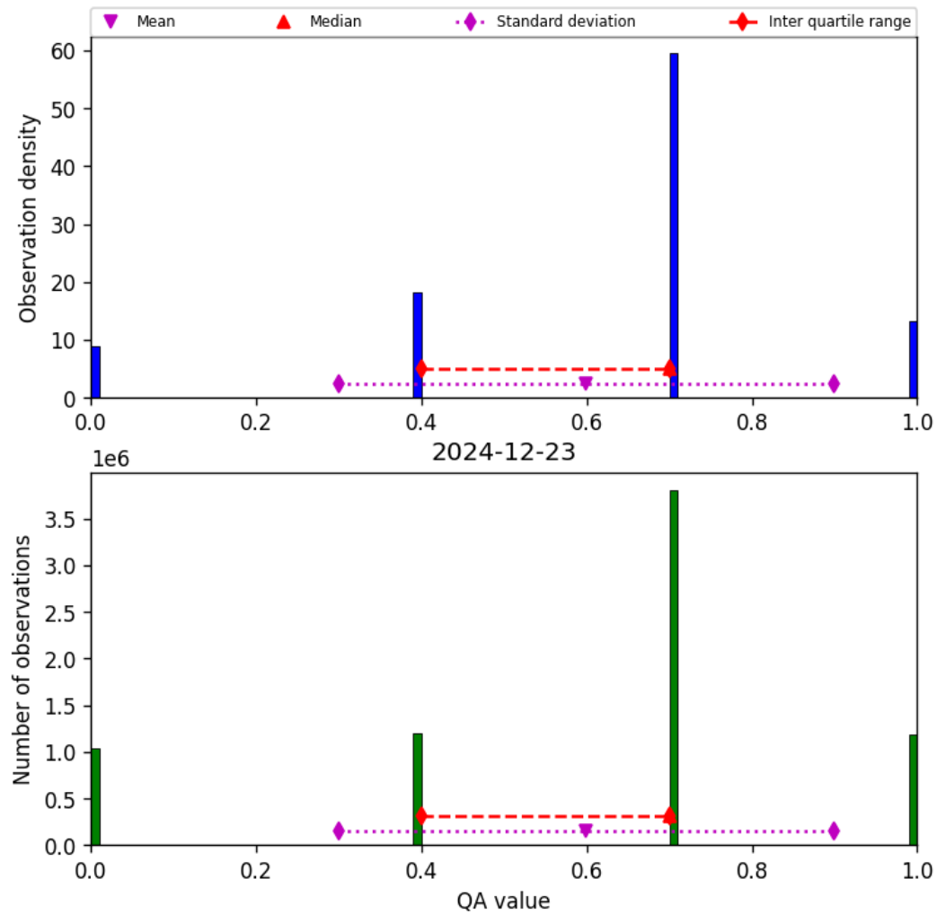
Figure 13: Histogram of “QA value” for 2024-12-23 to 2024-12-24
