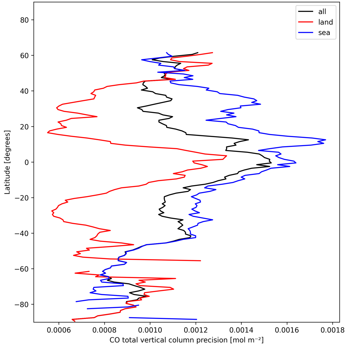
Figure 8: Zonal average of “CO total vertical column precision” for 2024-12-24 to 2024-12-25.
