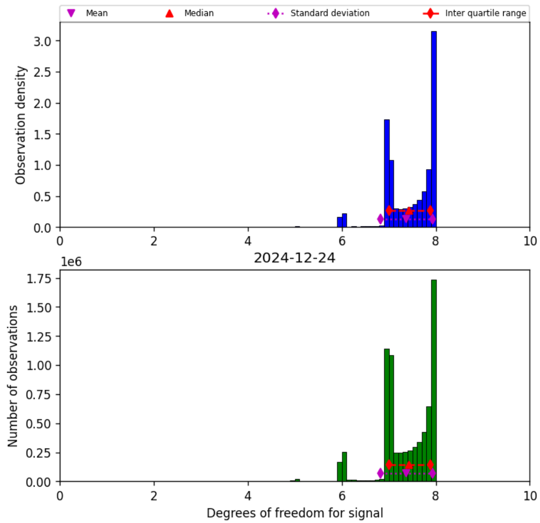
Figure 18: Histogram of “Degrees of freedom for signal” for 2024-12-24 to 2024-12-25
