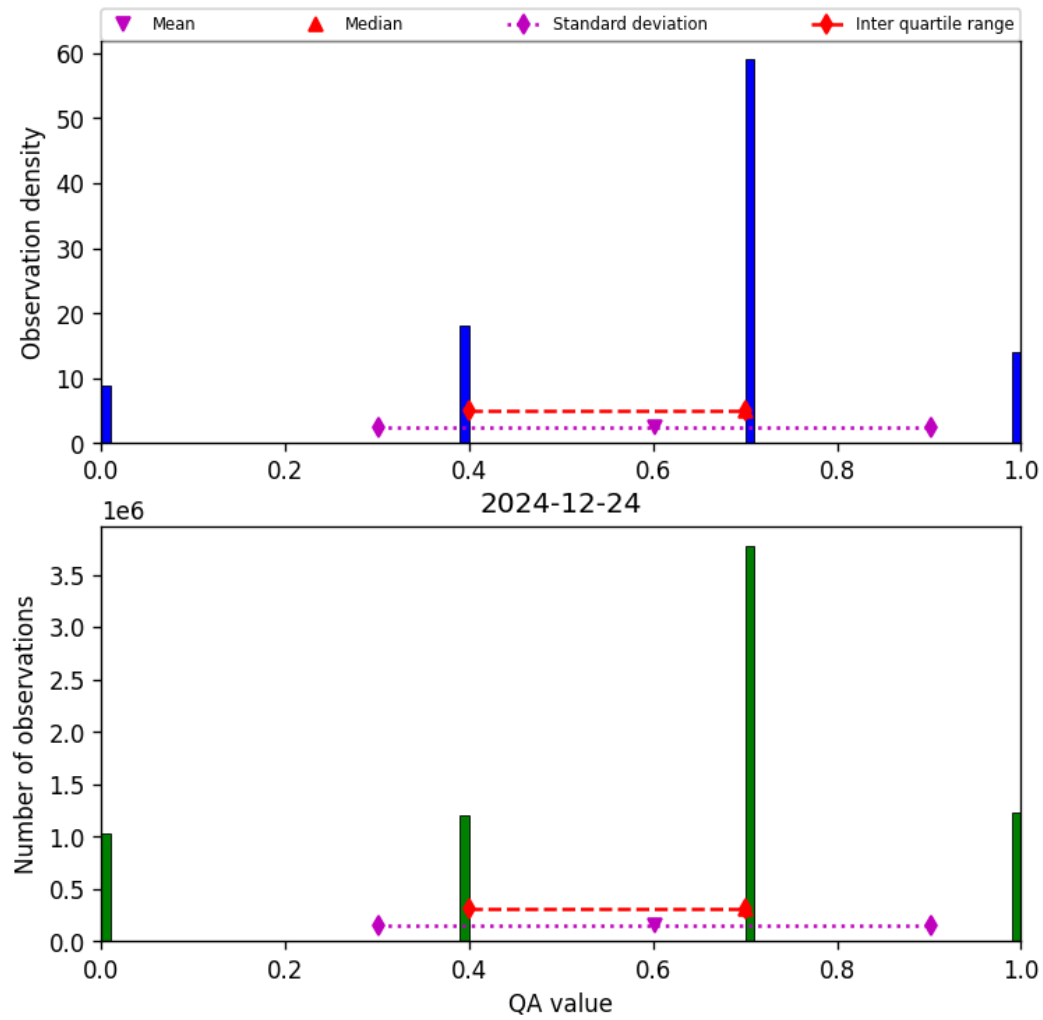
Figure 13: Histogram of “QA value” for 2024-12-24 to 2024-12-25
