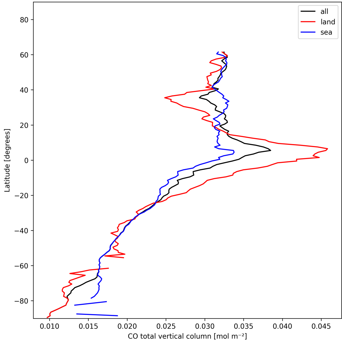
Figure 7: Zonal average of “CO total vertical column” for 2024-12-24 to 2024-12-25.
