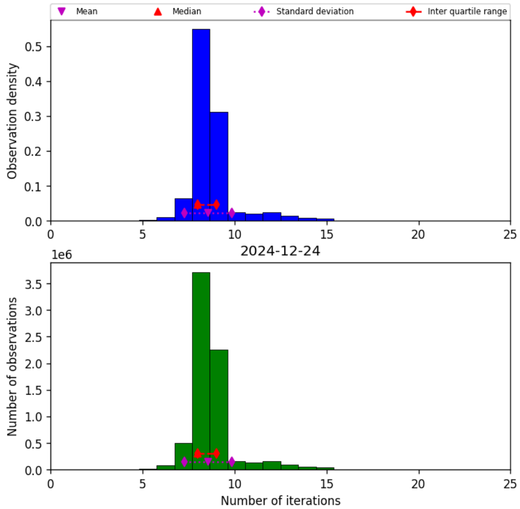
Figure 19: Histogram of “Number of iterations” for 2024-12-24 to 2024-12-25
