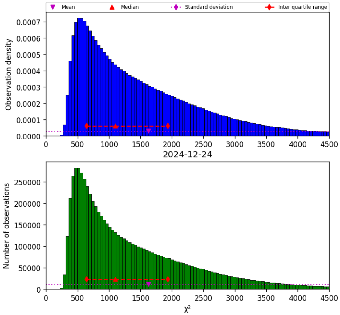
Figure 17: Histogram of “ \chi^2 ” for 2024-12-24 to 2024-12-25
