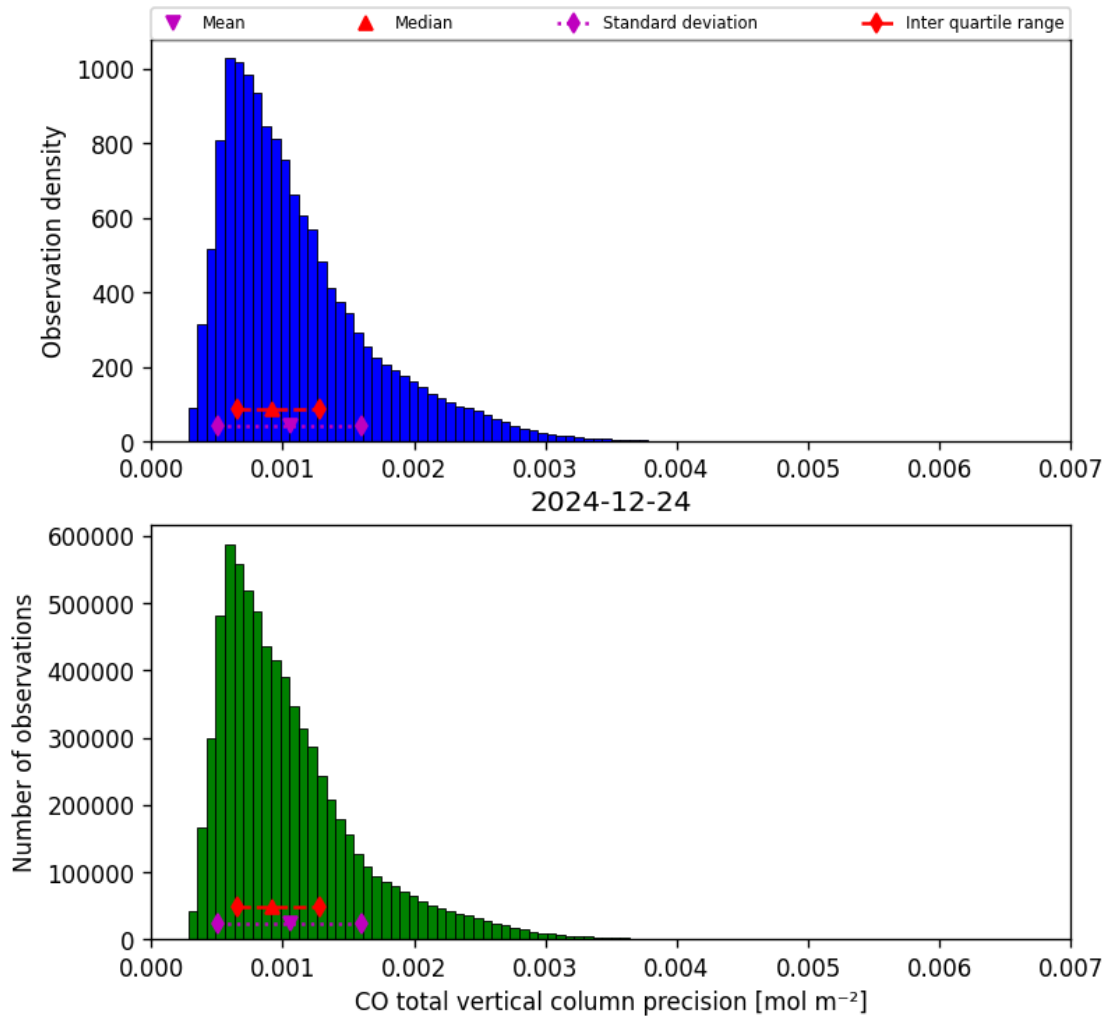
Figure 15: Histogram of “CO total vertical column precision” for 2024-12-24 to 2024-12-25
