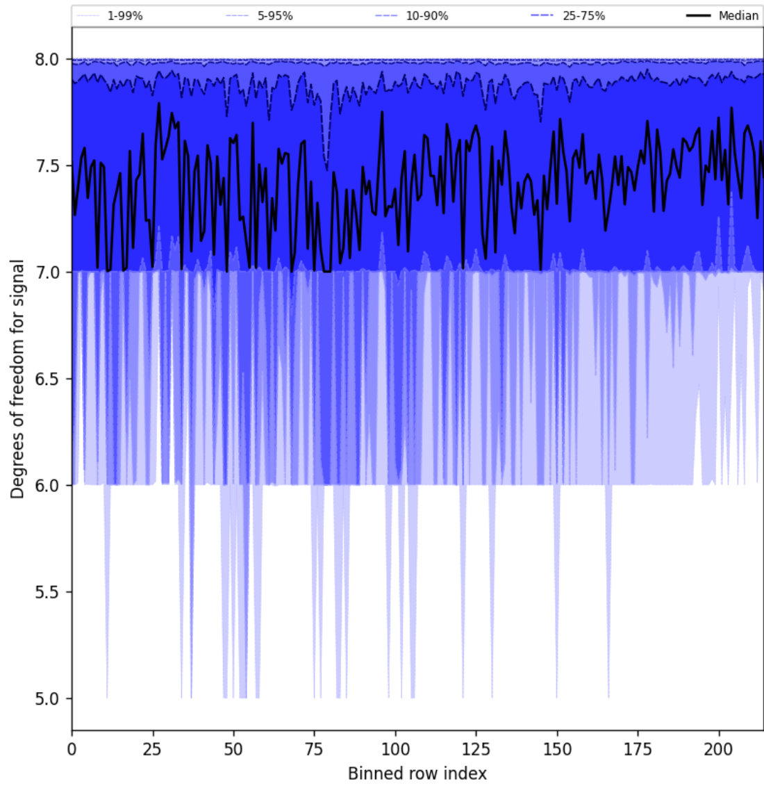
Figure 25: Along track statistics of “Degrees of freedom for signal” for 2024-12-24 to 2024-12-25
