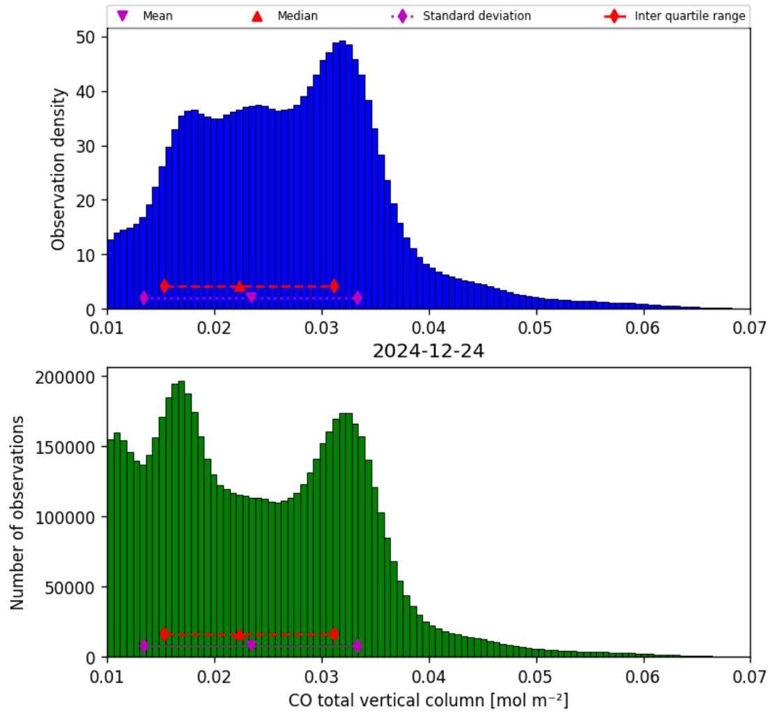
Figure 14: Histogram of “CO total vertical column” for 2024-12-24 to 2024-12-25
