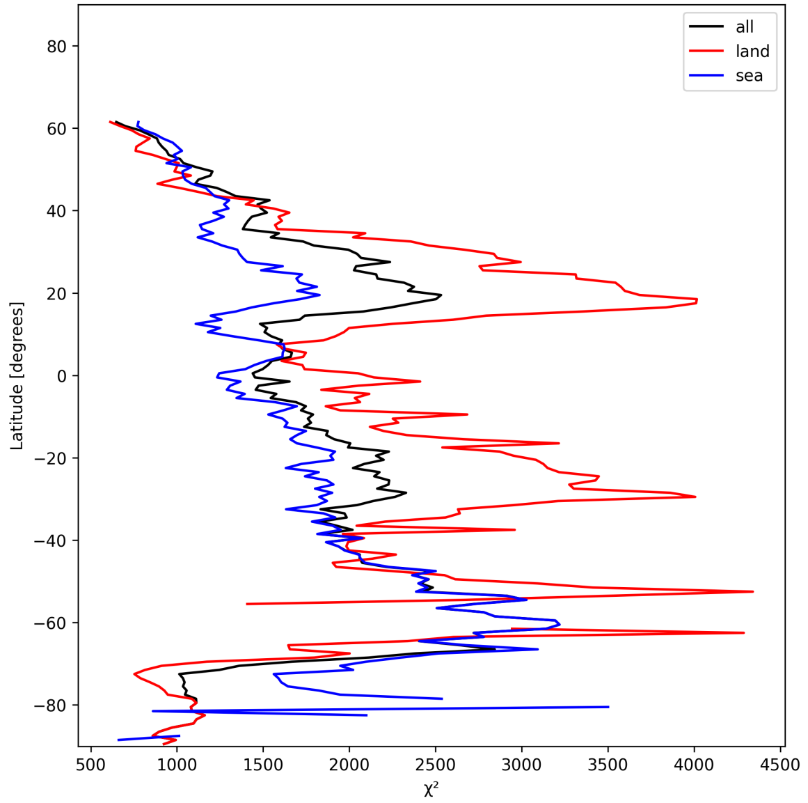
Figure 10: Zonal average of “ \chi^2 ” for 2024-12-24 to 2024-12-25.
