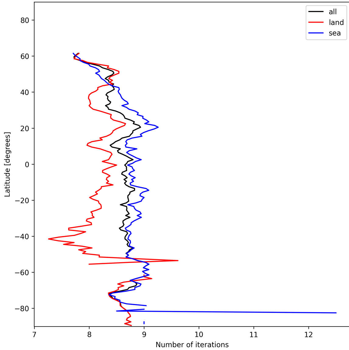
Figure 12: Zonal average of “Number of iterations” for 2024-12-24 to 2024-12-25.
