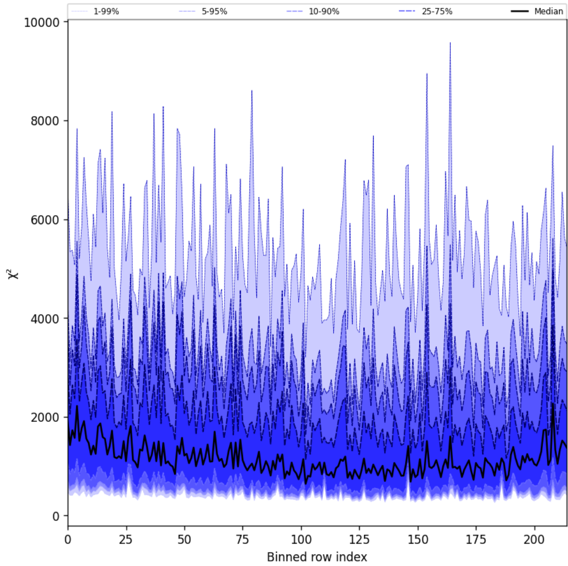
Figure 24: Along track statistics of “ \chi^2 ” for 2024-12-24 to 2024-12-25
