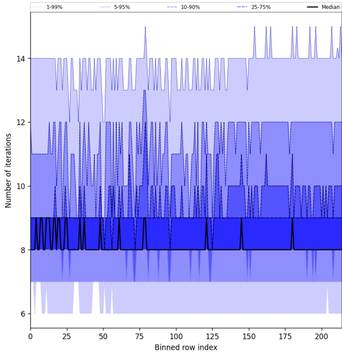
Figure 26: Along track statistics of “Number of iterations” for 2024-12-24 to 2024-12-25
