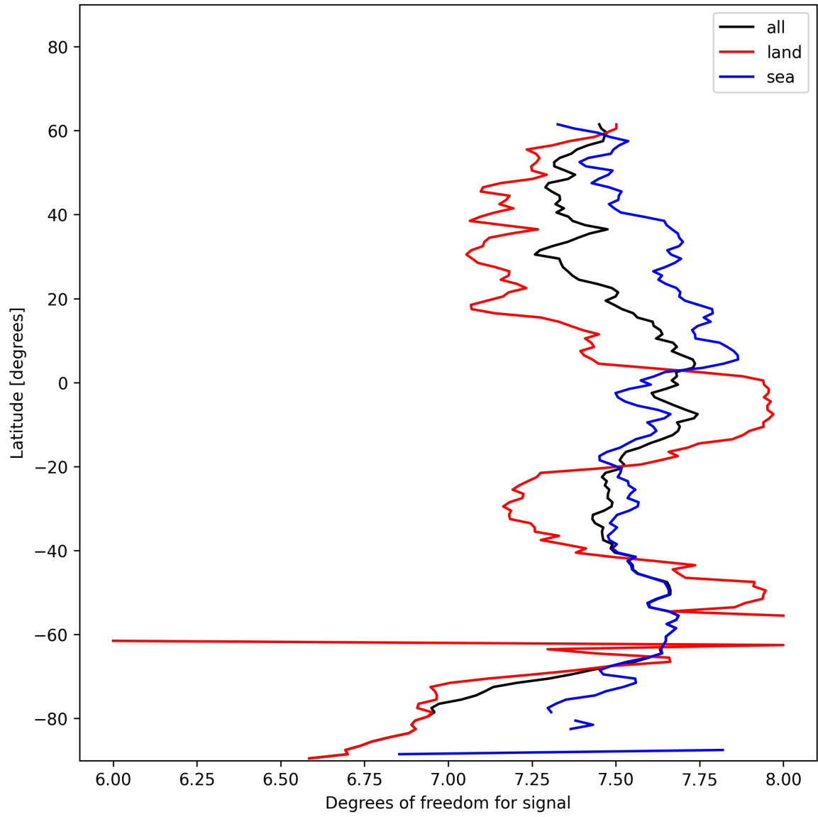
Figure 11: Zonal average of “Degrees of freedom for signal” for 2024-12-24 to 2024-12-25.
