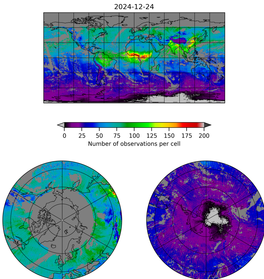
Figure 5: Map of the number of observations for 2024-12-24 to 2024-12-25
