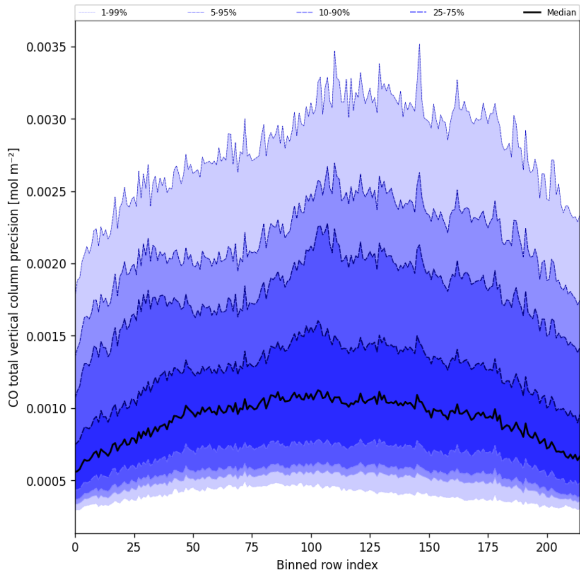
Figure 22: Along track statistics of “CO total vertical column precision” for 2024-12-24 to 2024-12-25
