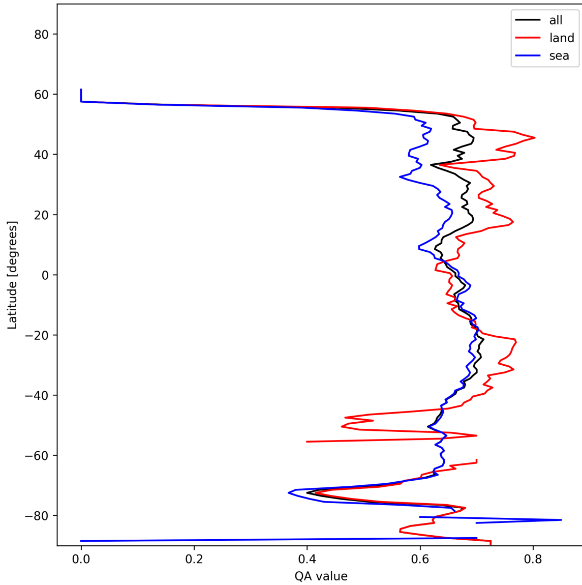
Figure 6: Zonal average of “QA value” for 2024-12-24 to 2024-12-25.
