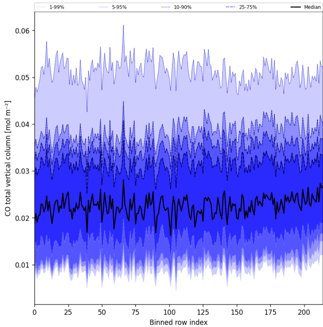
Figure 21: Along track statistics of “CO total vertical column” for 2024-12-24 to 2024-12-25
