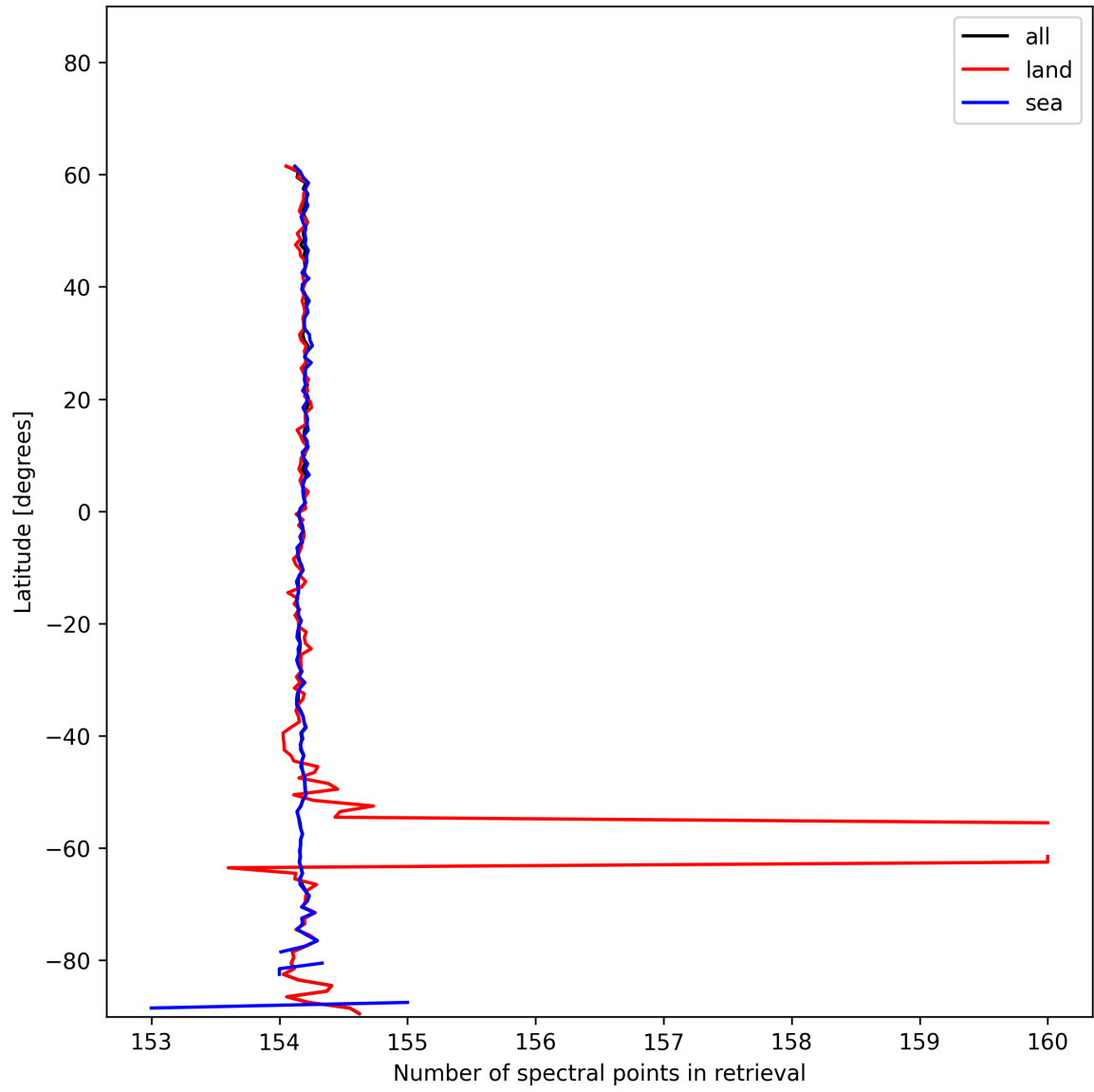
Figure 9: Zonal average of “Number of spectral points in retrieval” for 2024-12-24 to 2024-12-25.
