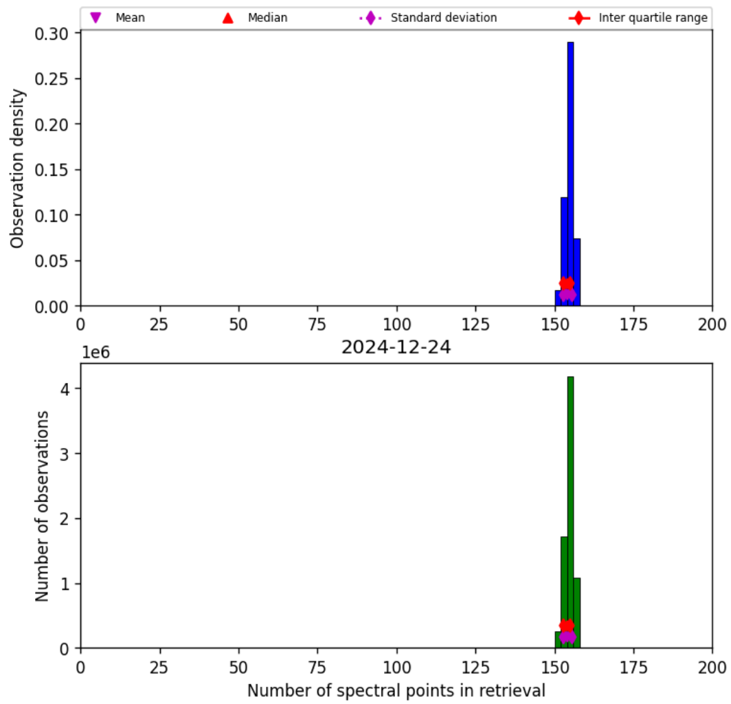
Figure 16: Histogram of “Number of spectral points in retrieval” for 2024-12-24 to 2024-12-25
