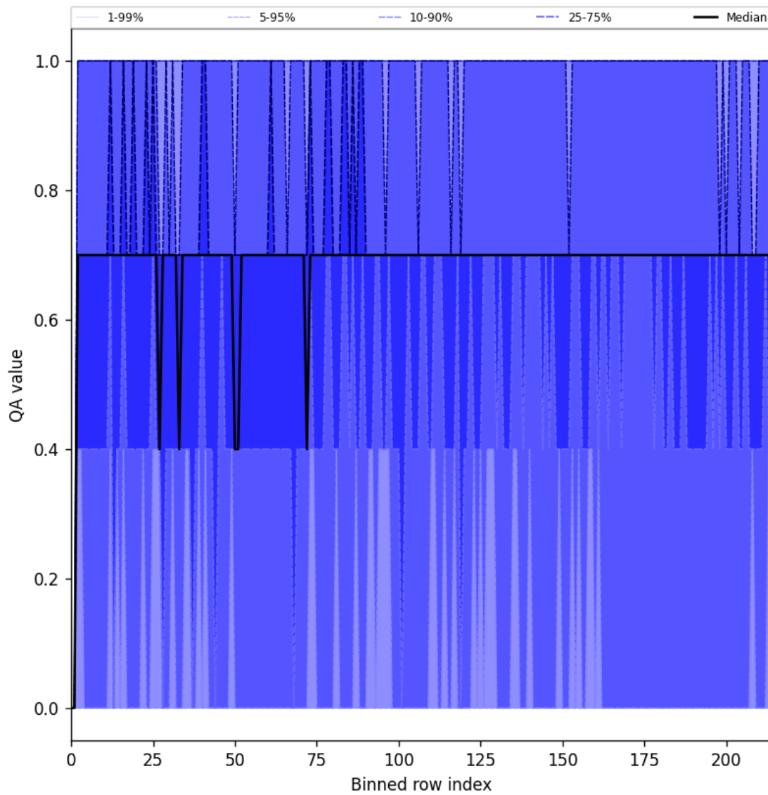
Figure 20: Along track statistics of “QA value” for 2024-12-24 to 2024-12-25
