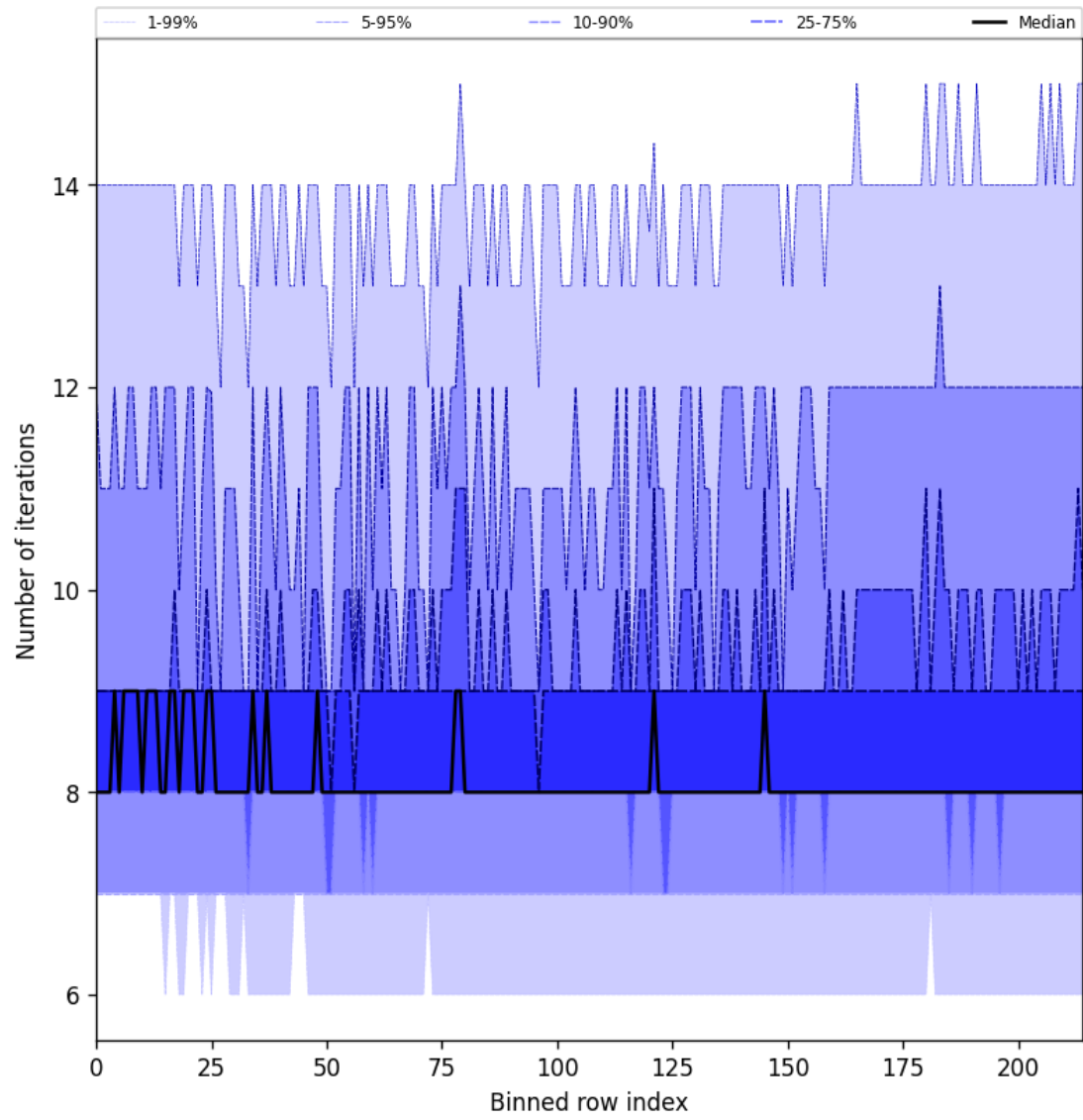
Figure 26: Along track statistics of “Number of iterations” for 2024-12-25 to 2024-12-25
