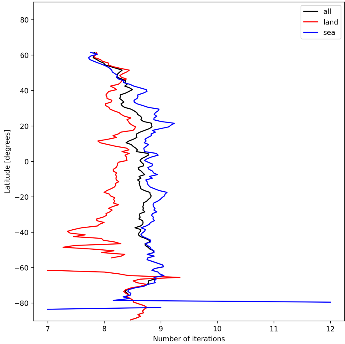
Figure 12: Zonal average of “Number of iterations” for 2024-12-25 to 2024-12-25.
