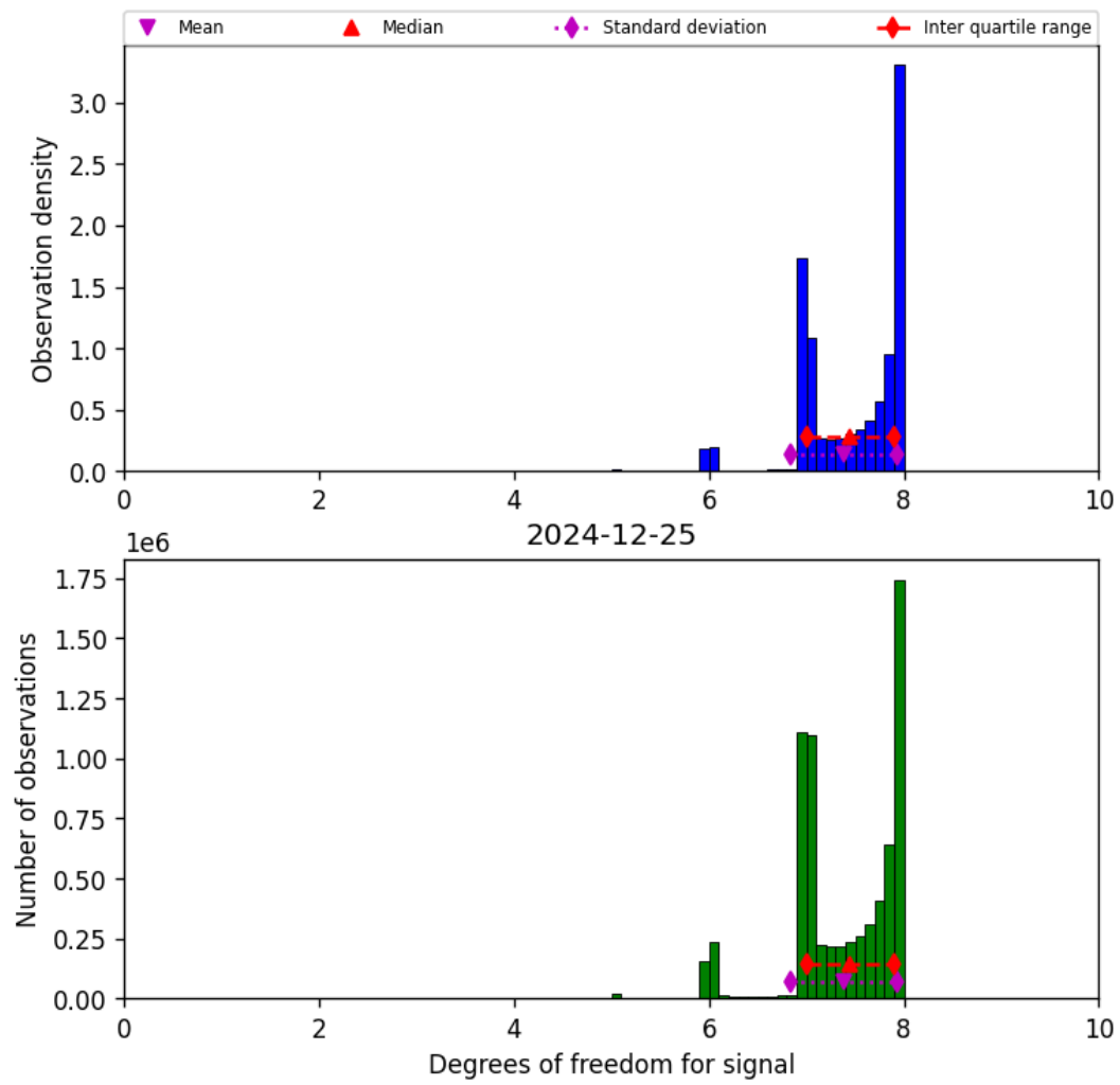
Figure 18: Histogram of “Degrees of freedom for signal” for 2024-12-25 to 2024-12-25
