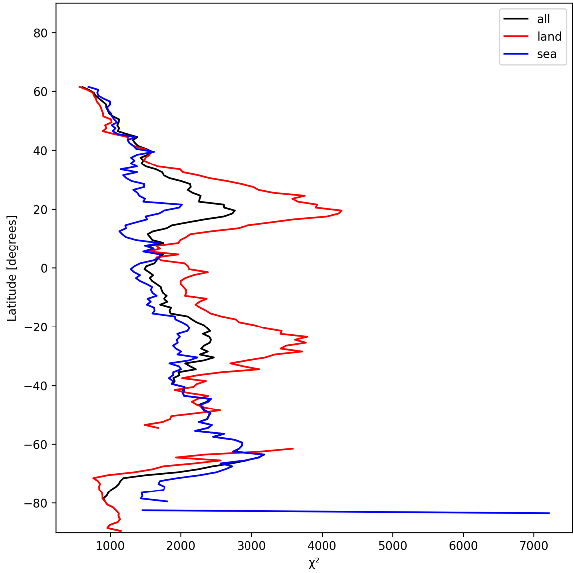
Figure 10: Zonal average of “ \chi^2 ” for 2024-12-25 to 2024-12-25.
