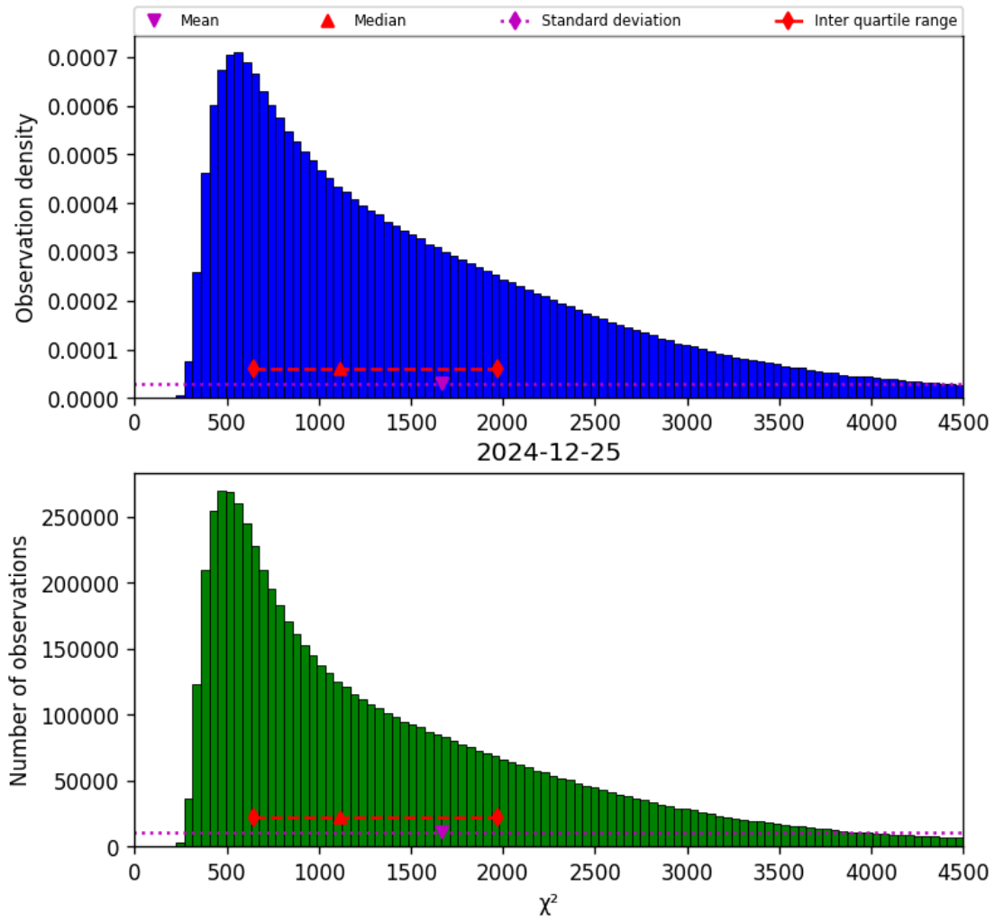
Figure 17: Histogram of “ \chi^2 ” for 2024-12-25 to 2024-12-25
