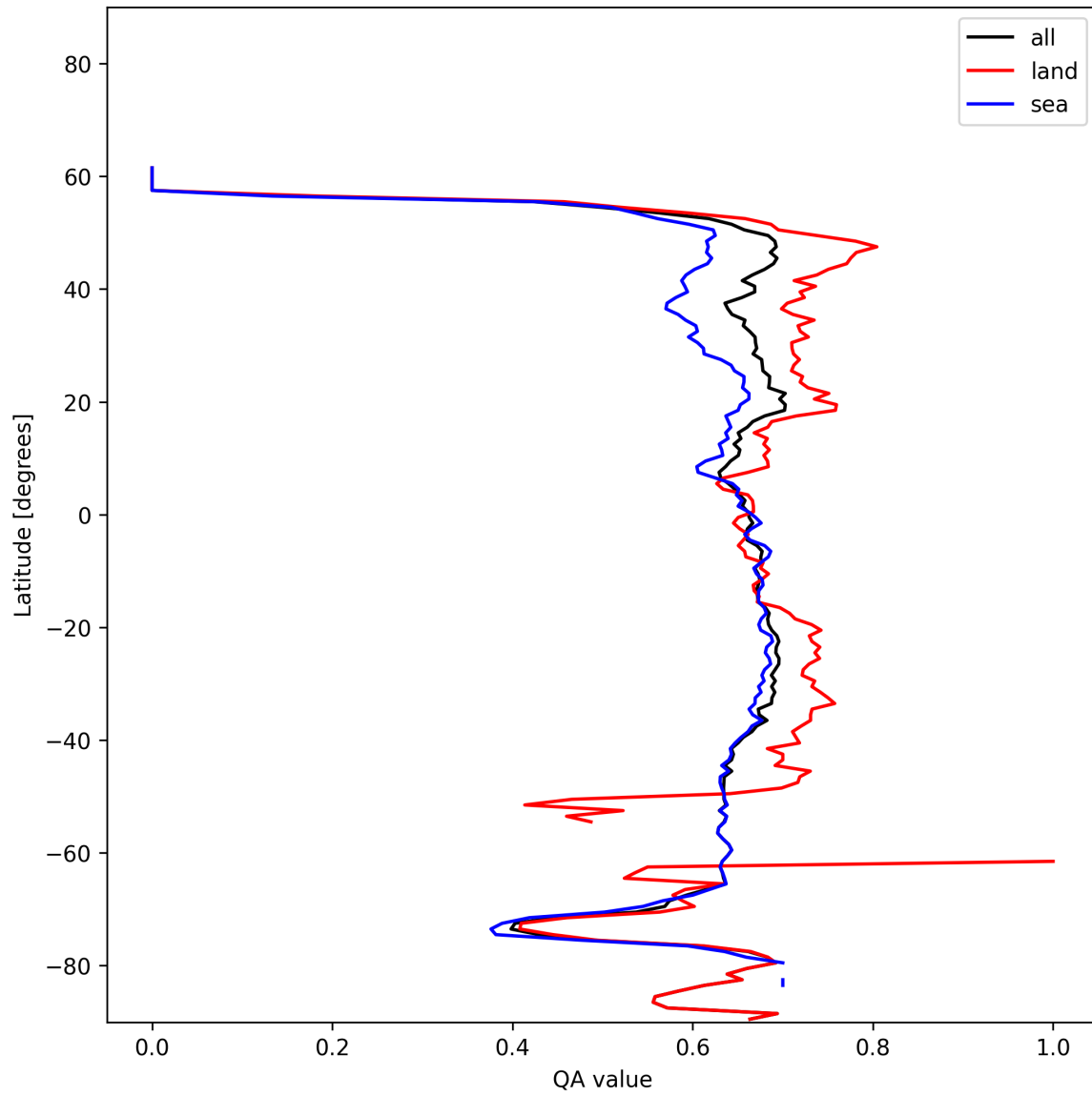
Figure 6: Zonal average of “QA value” for 2024-12-25 to 2024-12-25.
