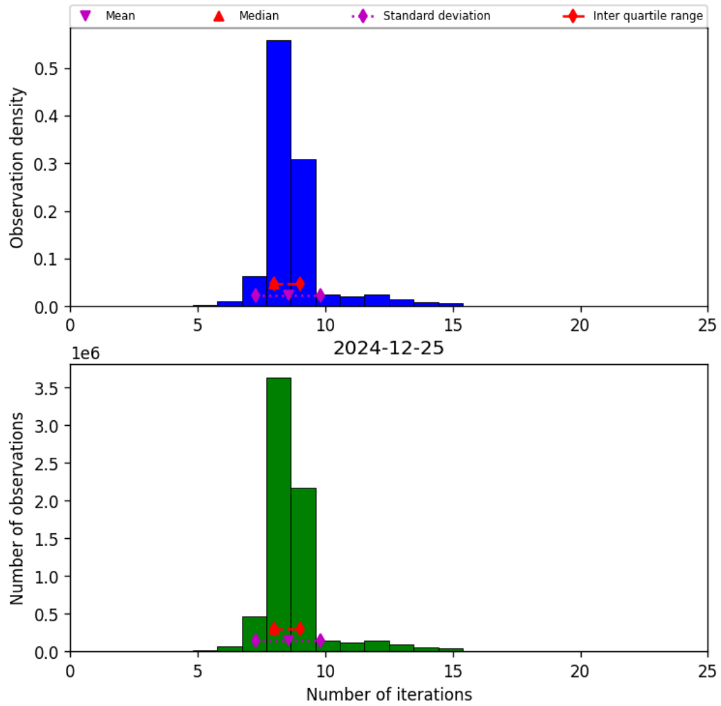
Figure 19: Histogram of “Number of iterations” for 2024-12-25 to 2024-12-25
