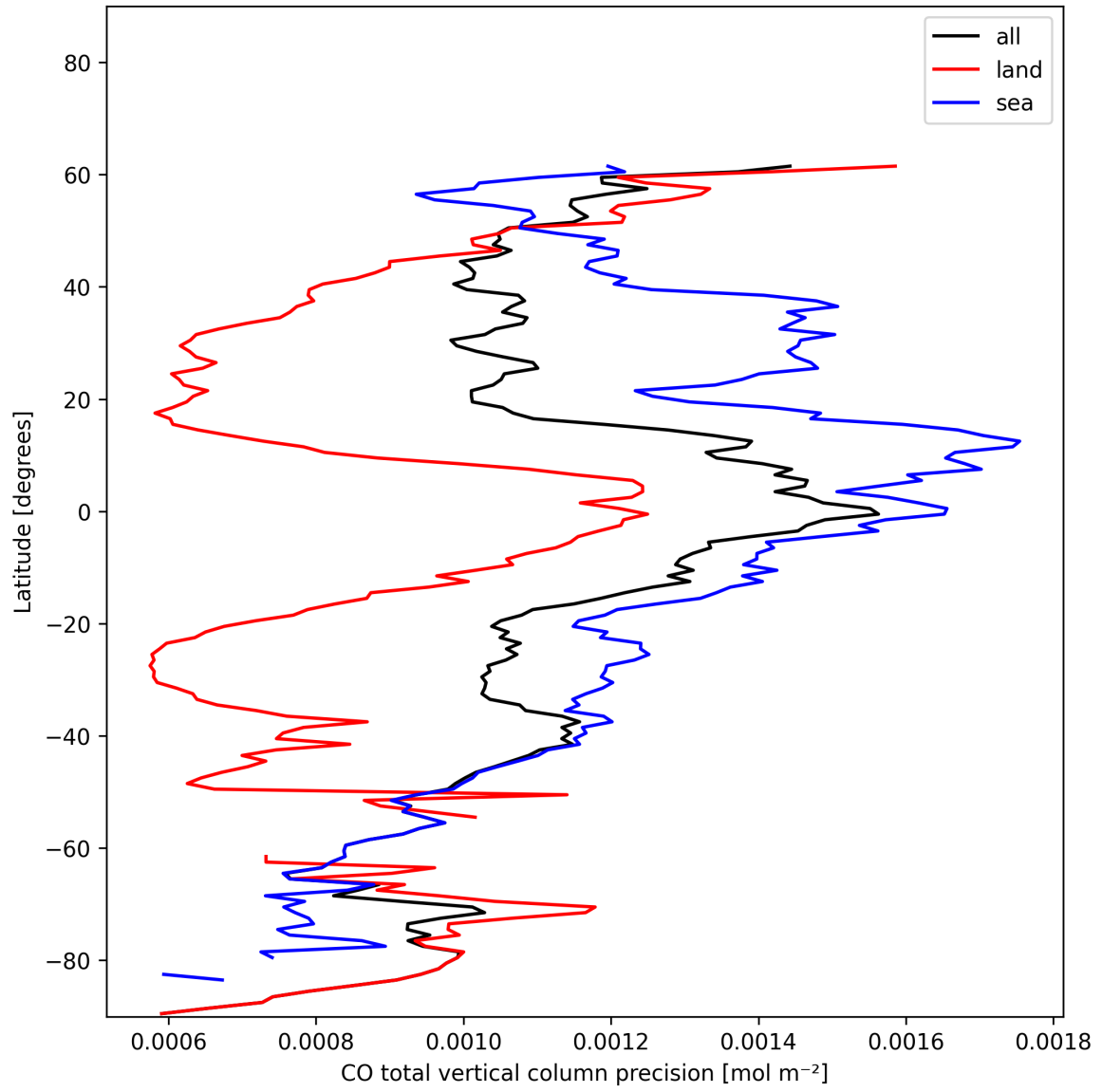
Figure 8: Zonal average of “CO total vertical column precision” for 2024-12-25 to 2024-12-25.
