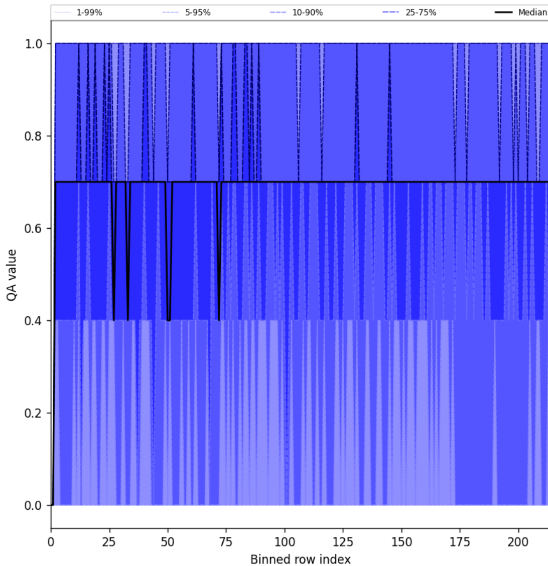
Figure 20: Along track statistics of “QA value” for 2024-12-25 to 2024-12-25
