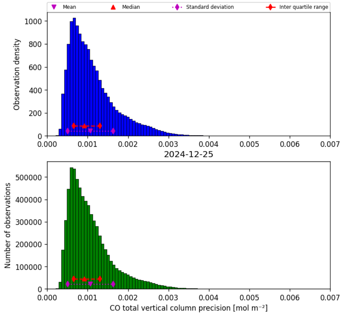
Figure 15: Histogram of “CO total vertical column precision” for 2024-12-25 to 2024-12-25
