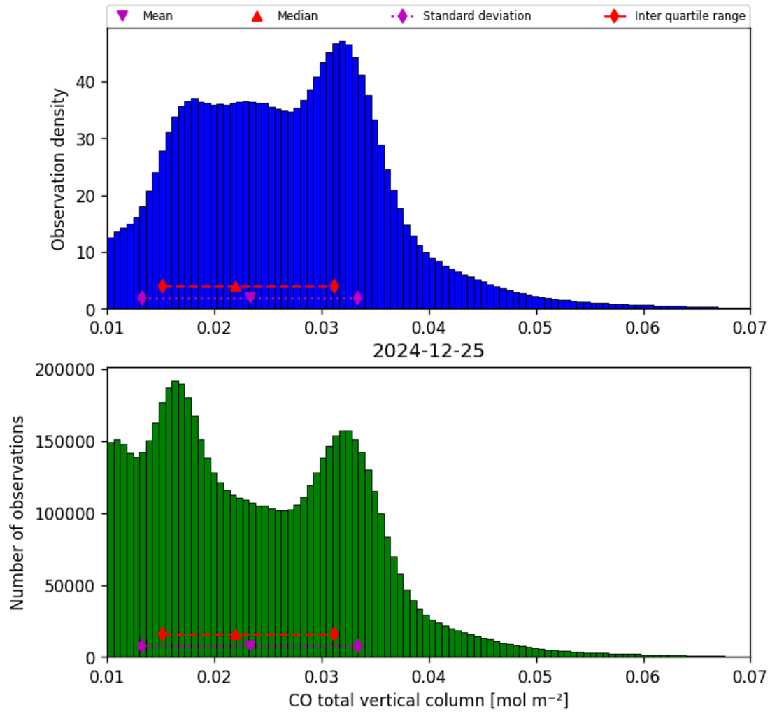
Figure 14: Histogram of “CO total vertical column” for 2024-12-25 to 2024-12-25
