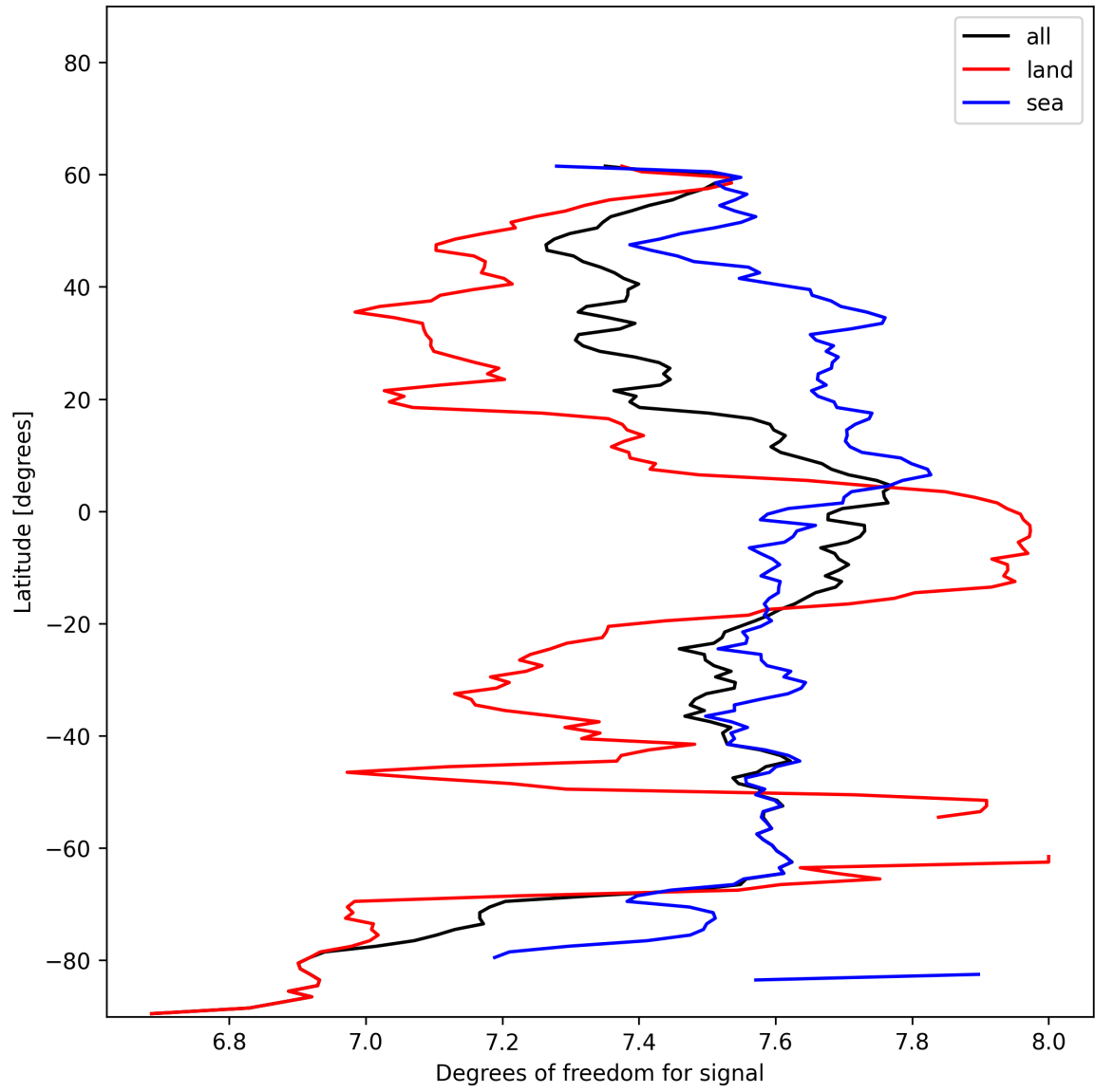
Figure 11: Zonal average of “Degrees of freedom for signal” for 2024-12-25 to 2024-12-25.
