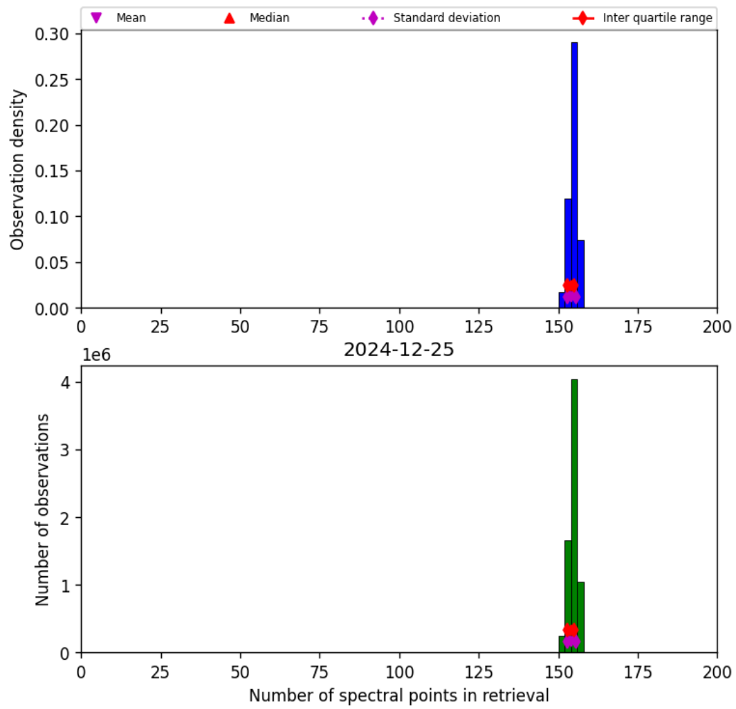
Figure 16: Histogram of “Number of spectral points in retrieval” for 2024-12-25 to 2024-12-25
