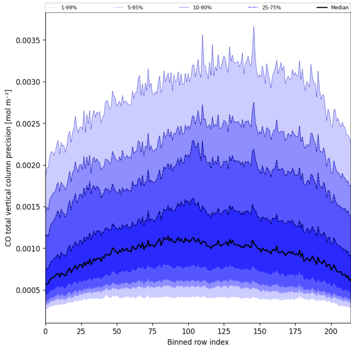
Figure 22: Along track statistics of “CO total vertical column precision” for 2024-12-25 to 2024-12-25
