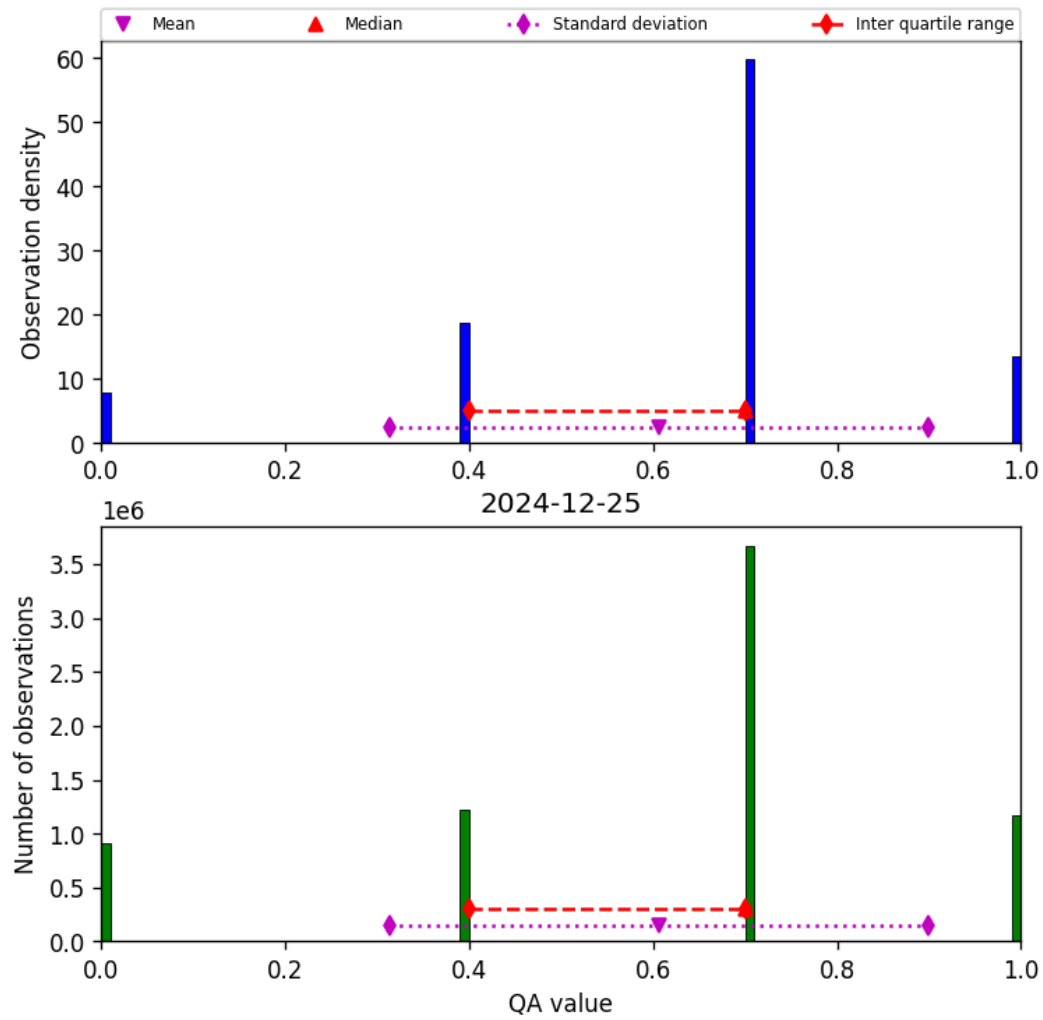
Figure 13: Histogram of “QA value” for 2024-12-25 to 2024-12-25
