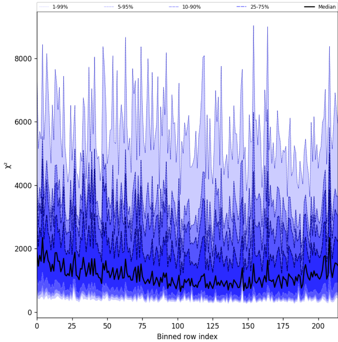
Figure 24: Along track statistics of “ \chi^2 ” for 2024-12-25 to 2024-12-25
