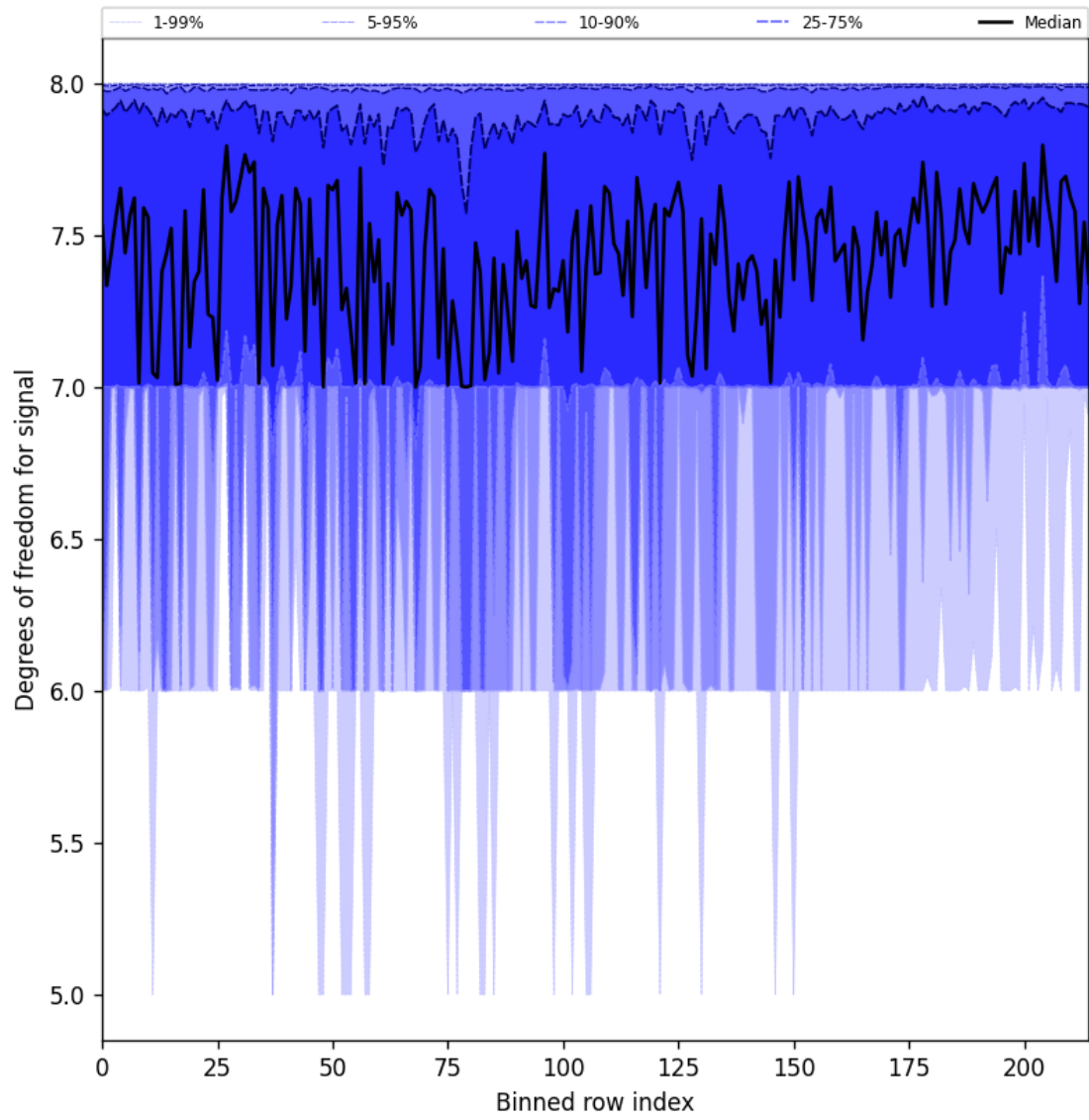
Figure 25: Along track statistics of “Degrees of freedom for signal” for 2024-12-25 to 2024-12-25
