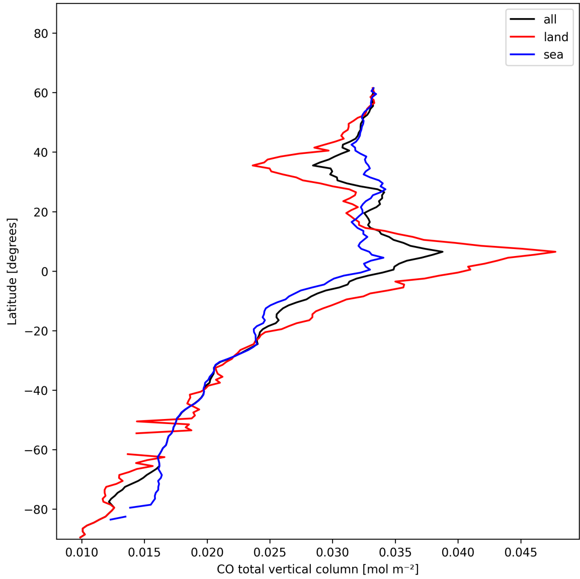
Figure 7: Zonal average of “CO total vertical column” for 2024-12-25 to 2024-12-25.
