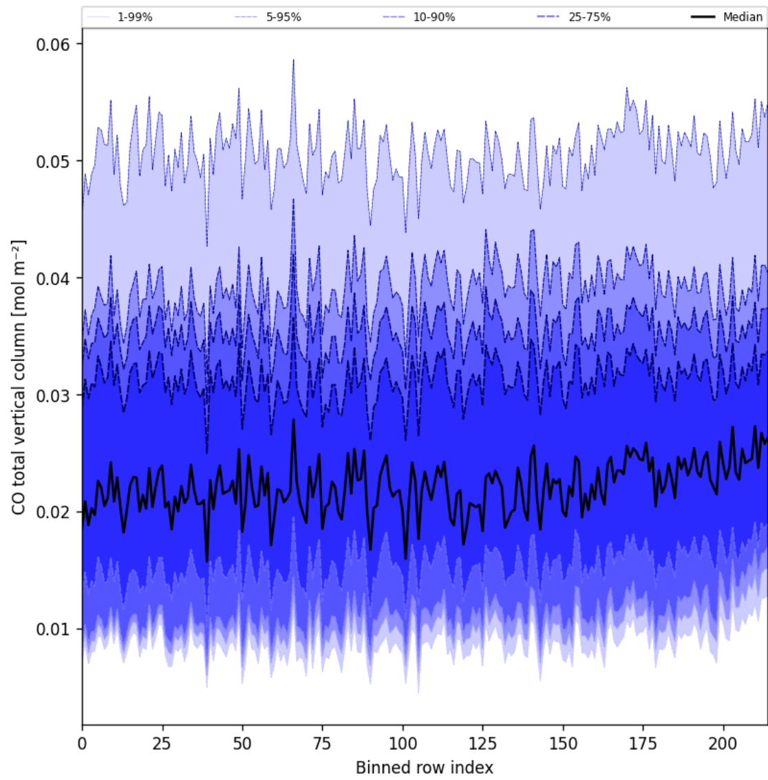
Figure 21: Along track statistics of “CO total vertical column” for 2024-12-25 to 2024-12-25
