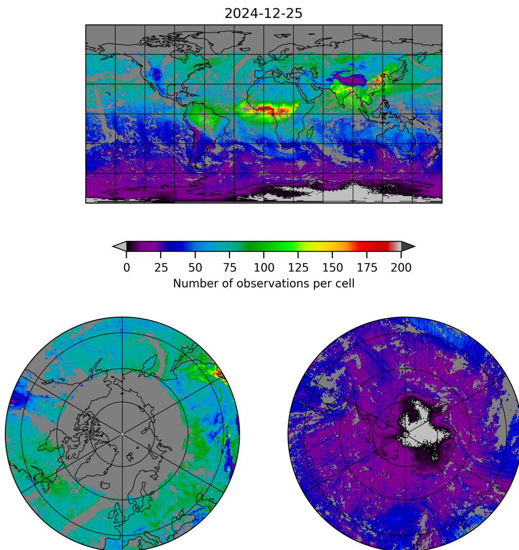
Figure 5: Map of the number of observations for 2024-12-25 to 2024-12-25
