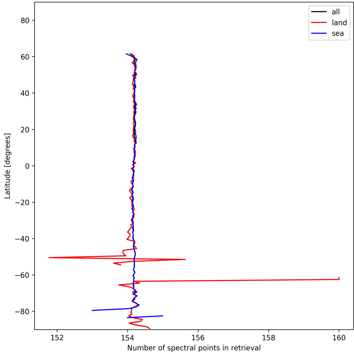
Figure 9: Zonal average of “Number of spectral points in retrieval” for 2024-12-25 to 2024-12-25.
