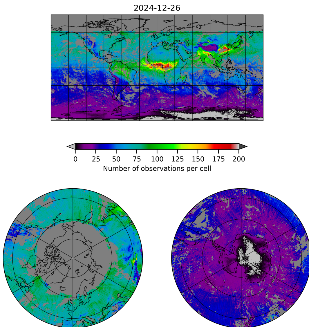
Figure 5: Map of the number of observations for 2024-12-26 to 2024-12-27
