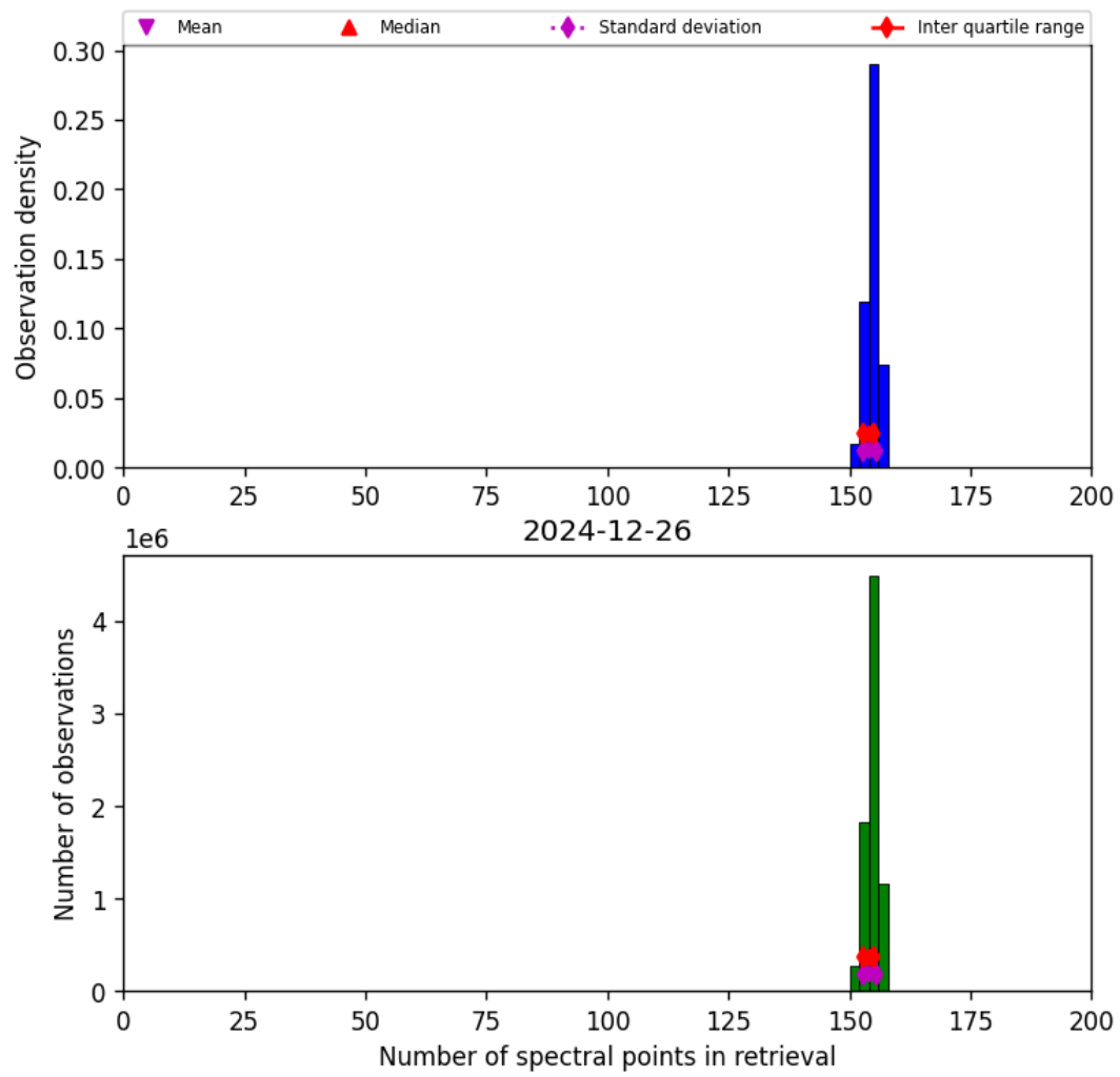
Figure 16: Histogram of “Number of spectral points in retrieval” for 2024-12-26 to 2024-12-27
