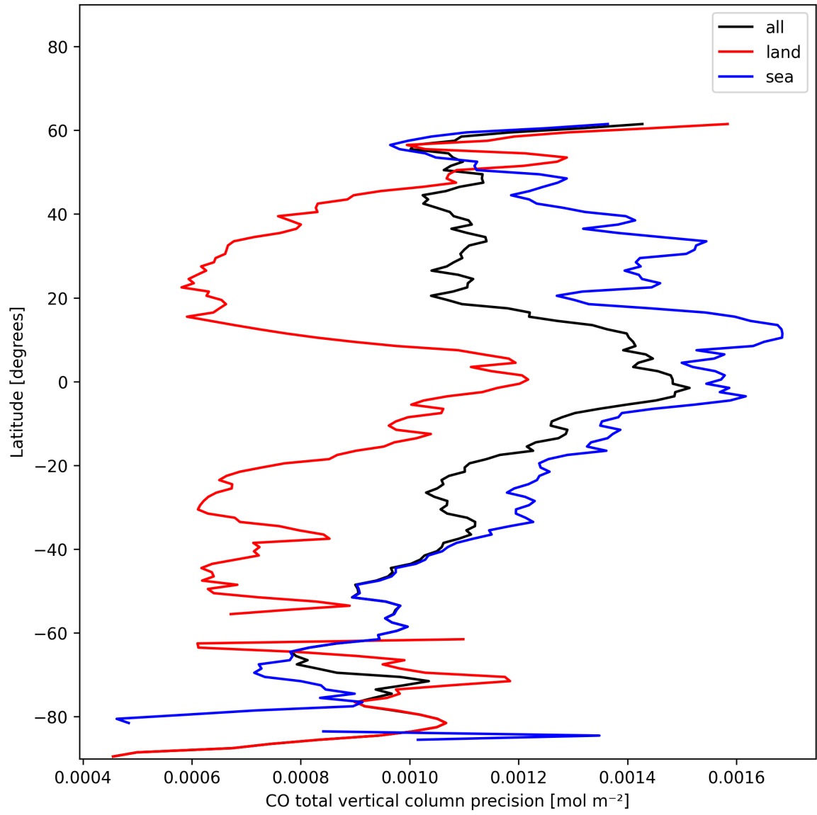
Figure 8: Zonal average of “CO total vertical column precision” for 2024-12-26 to 2024-12-27.
