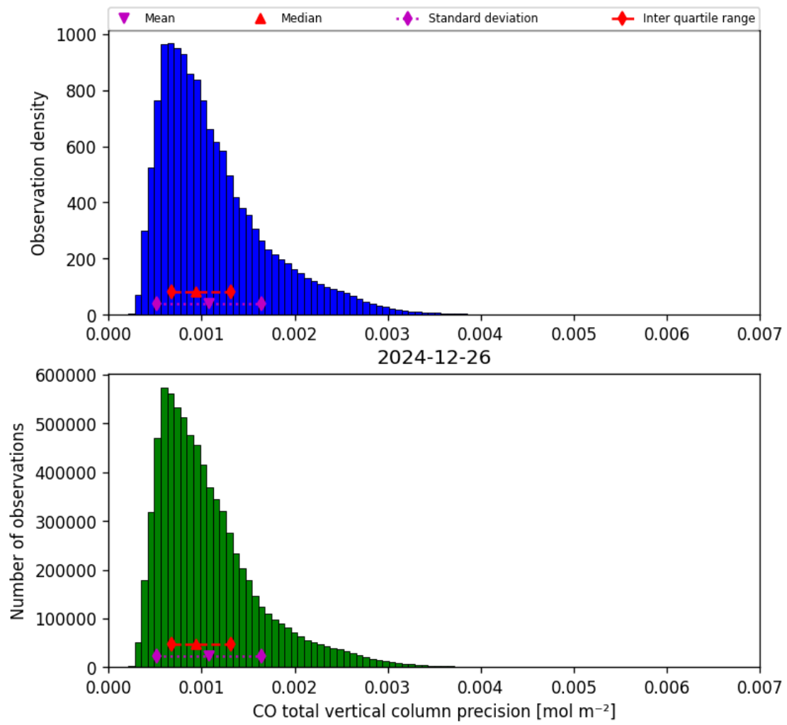
Figure 15: Histogram of “CO total vertical column precision” for 2024-12-26 to 2024-12-27
