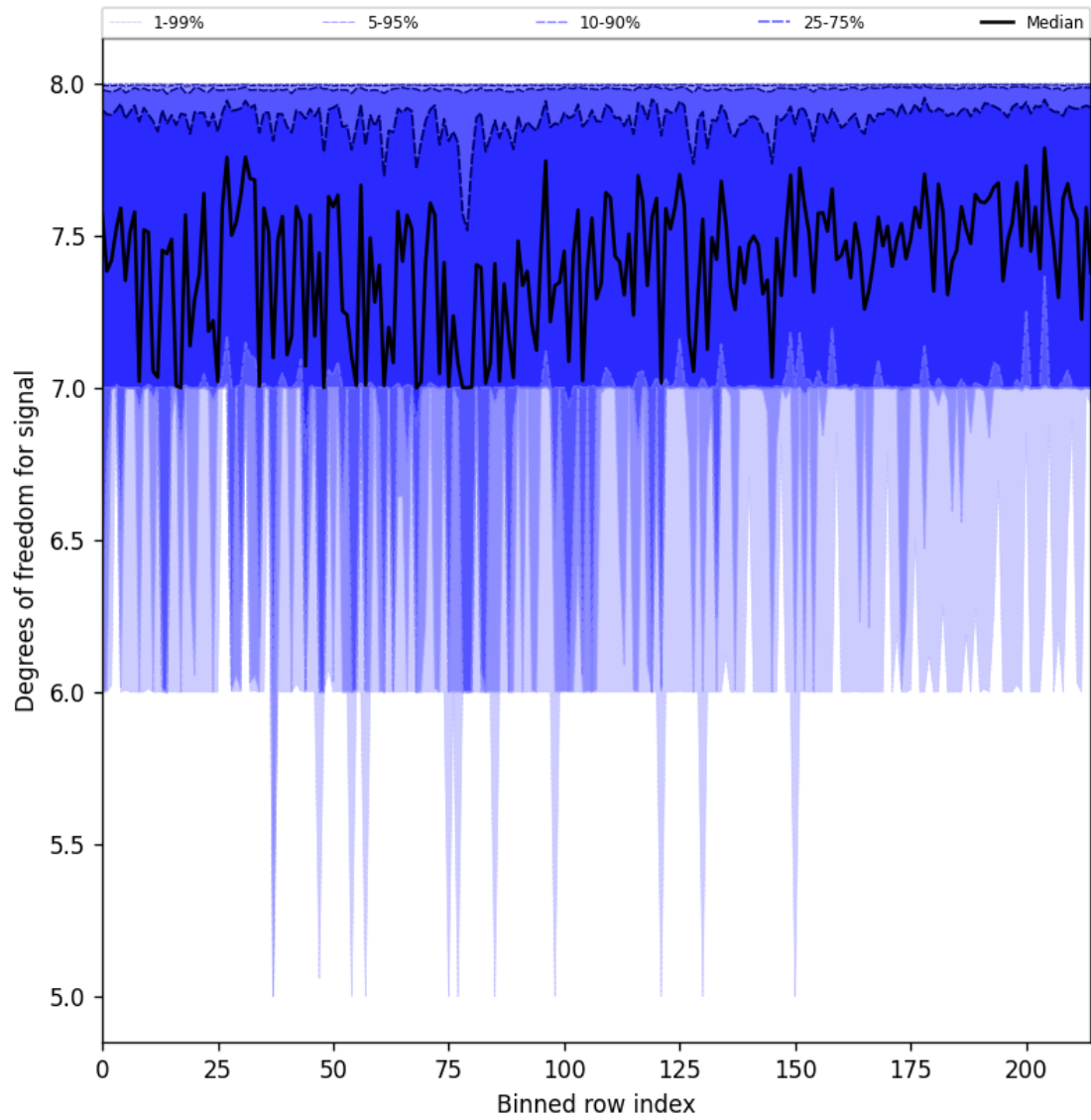
Figure 25: Along track statistics of “Degrees of freedom for signal” for 2024-12-26 to 2024-12-27
