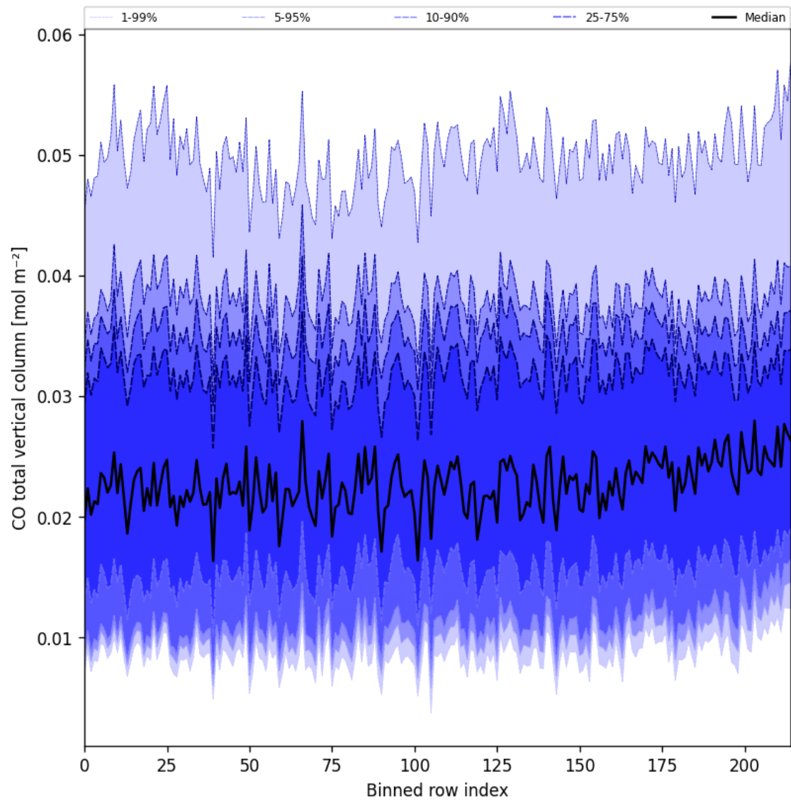
Figure 21: Along track statistics of “CO total vertical column” for 2024-12-26 to 2024-12-27
