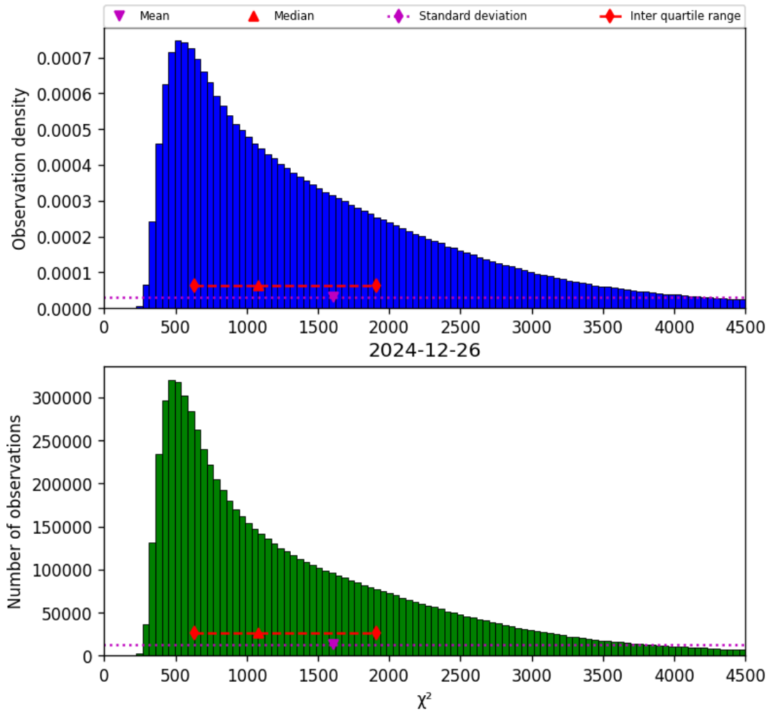
Figure 17: Histogram of “ \chi^2 ” for 2024-12-26 to 2024-12-27
