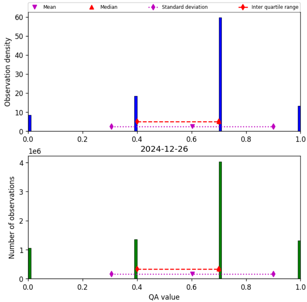
Figure 13: Histogram of “QA value” for 2024-12-26 to 2024-12-27
