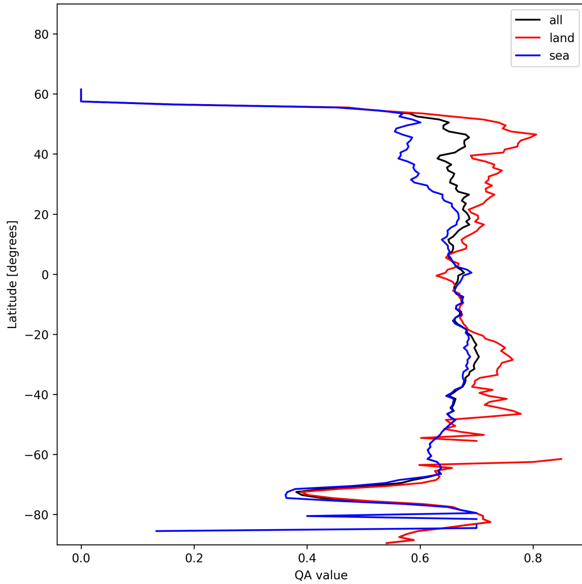
Figure 6: Zonal average of “QA value” for 2024-12-26 to 2024-12-27.
