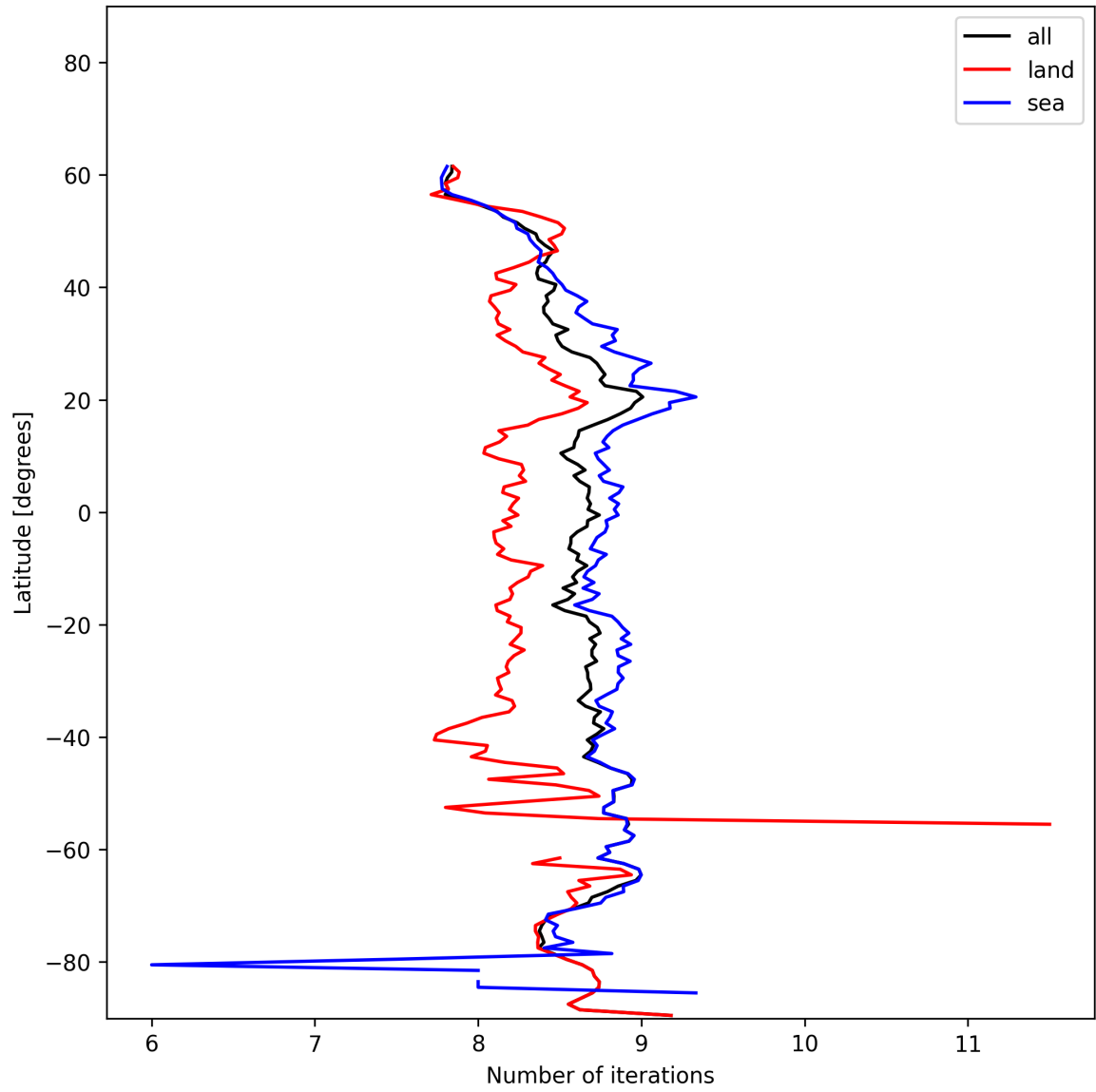
Figure 12: Zonal average of “Number of iterations” for 2024-12-26 to 2024-12-27.
