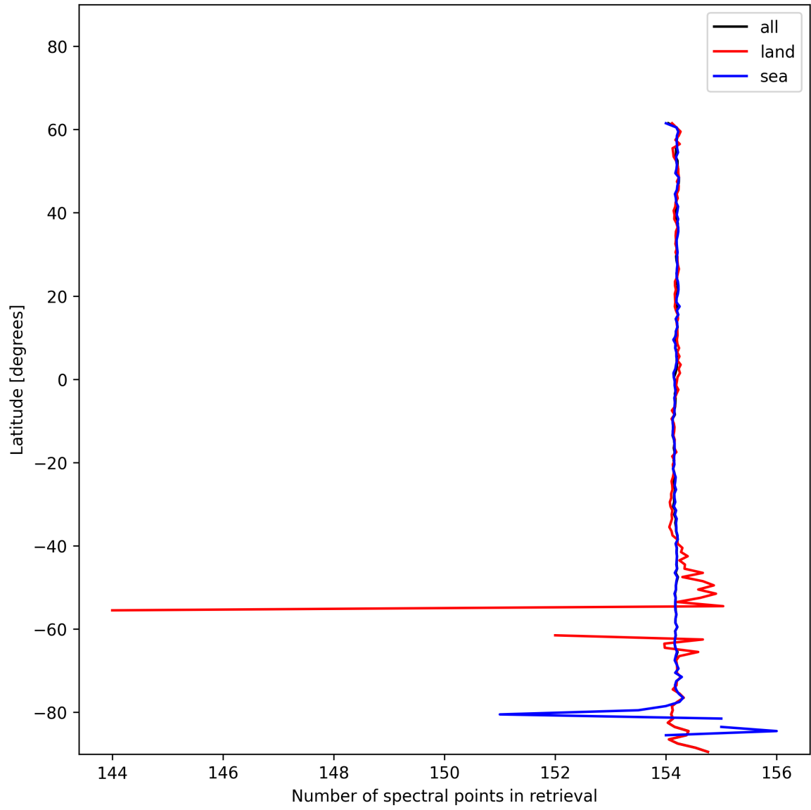
Figure 9: Zonal average of “Number of spectral points in retrieval” for 2024-12-26 to 2024-12-27.
