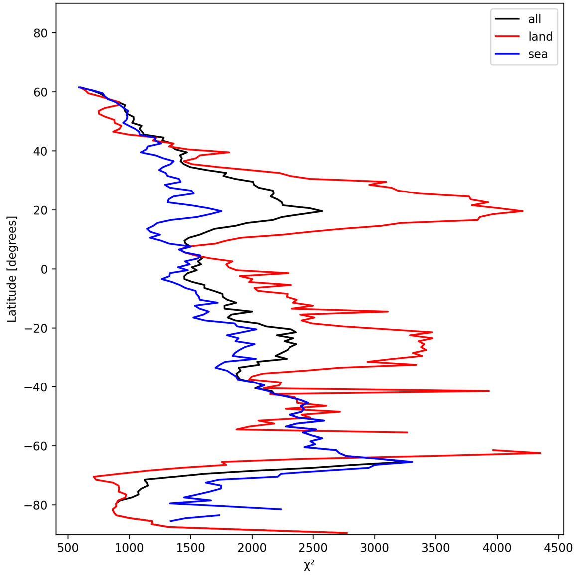
Figure 10: Zonal average of “ \chi^2 ” for 2024-12-26 to 2024-12-27.
