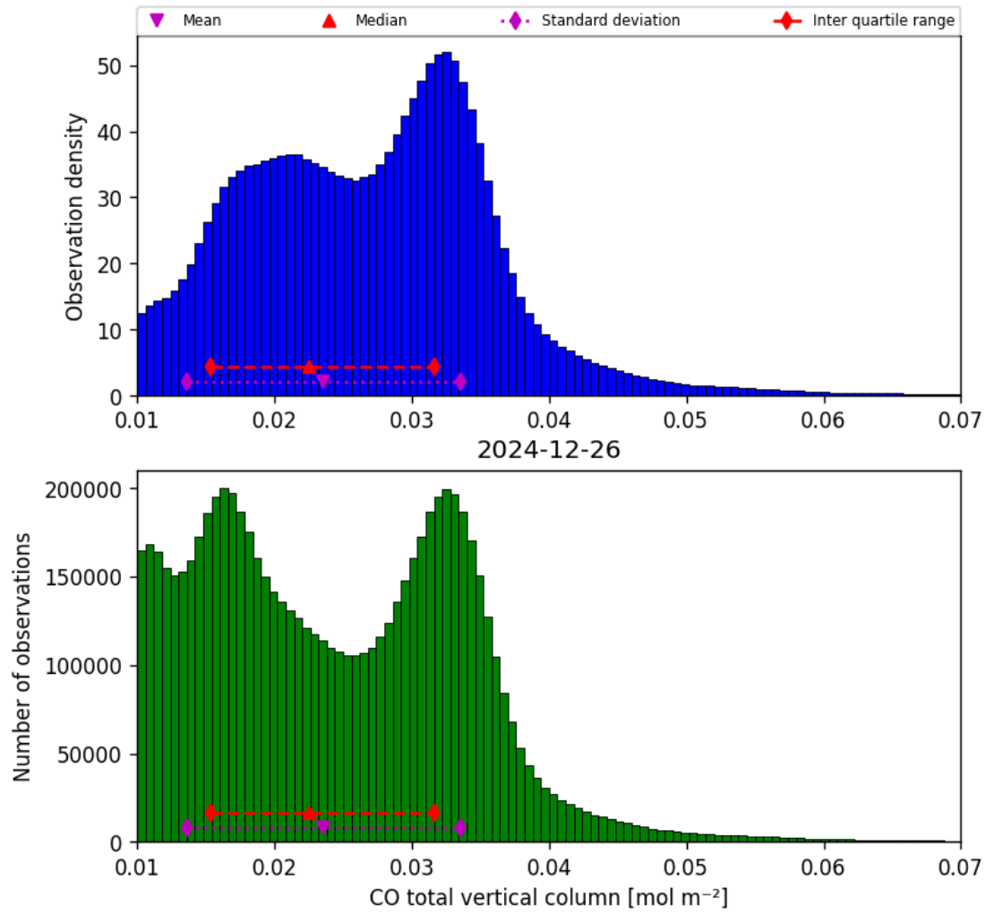
Figure 14: Histogram of “CO total vertical column” for 2024-12-26 to 2024-12-27
