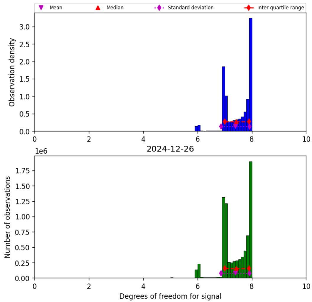
Figure 18: Histogram of “Degrees of freedom for signal” for 2024-12-26 to 2024-12-27
