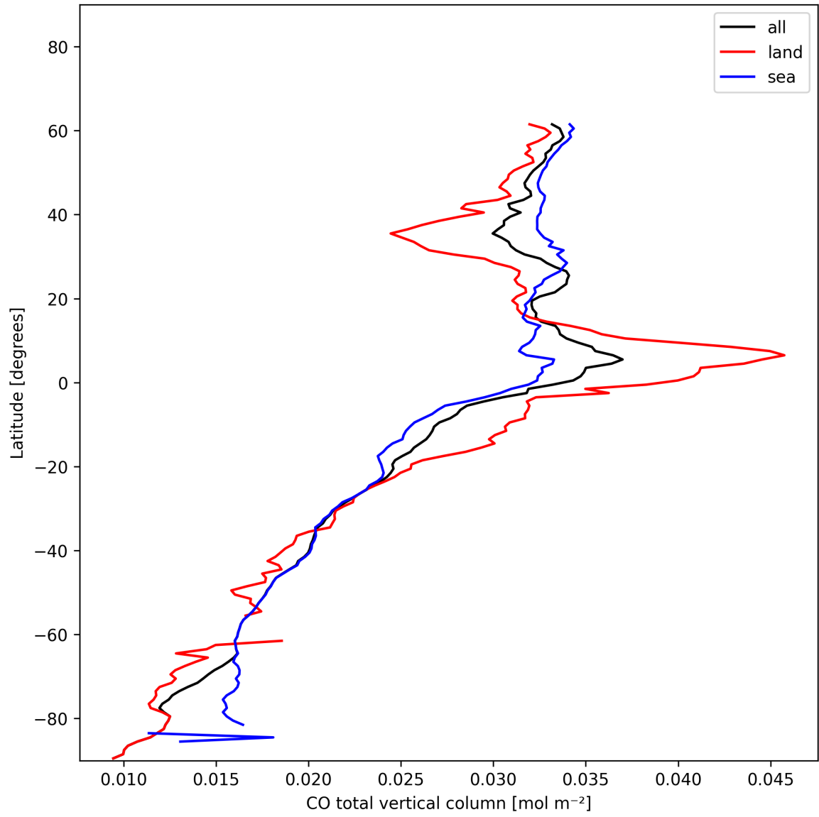
Figure 7: Zonal average of “CO total vertical column” for 2024-12-26 to 2024-12-27.
