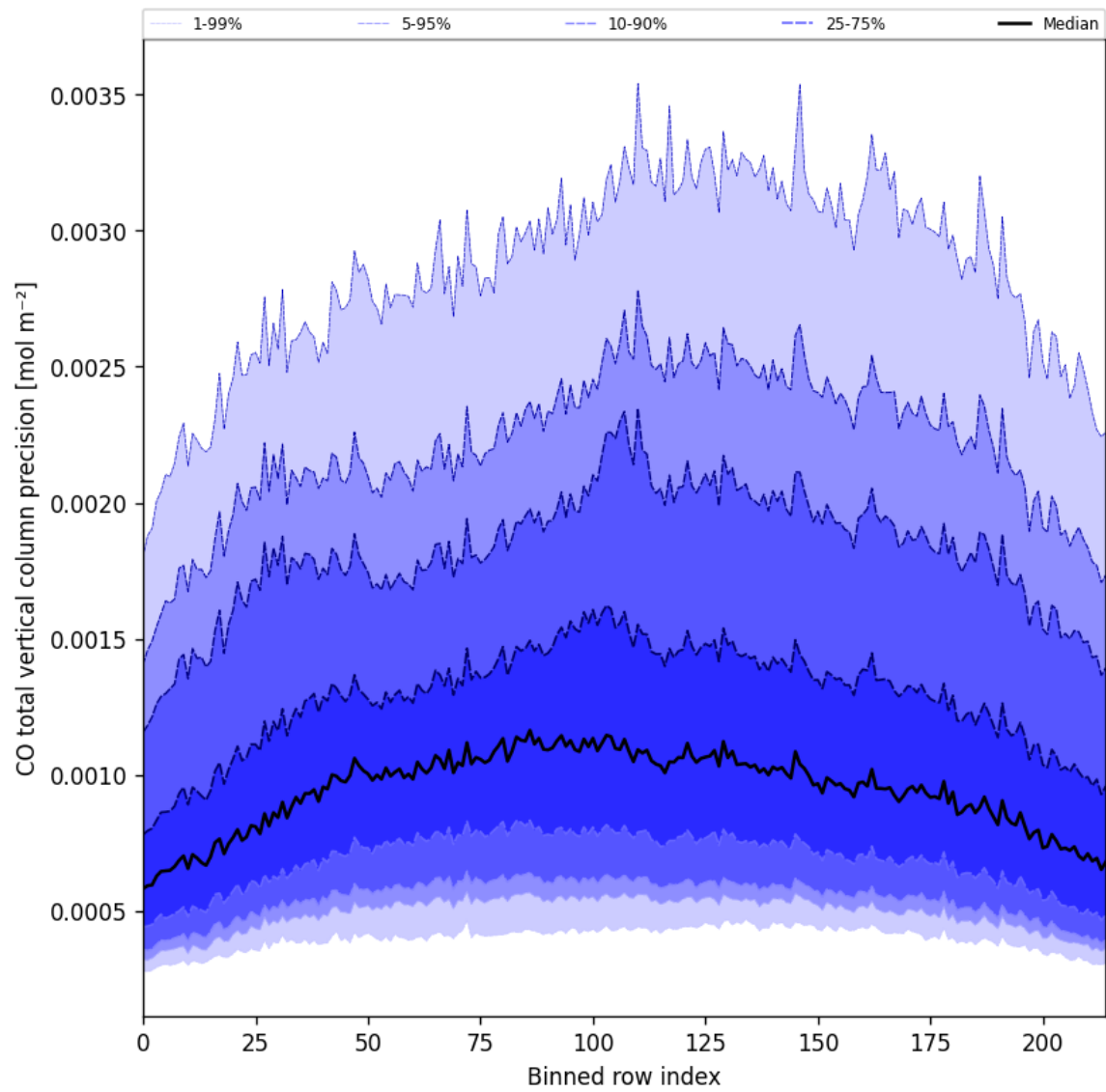
Figure 22: Along track statistics of “CO total vertical column precision” for 2024-12-26 to 2024-12-27
