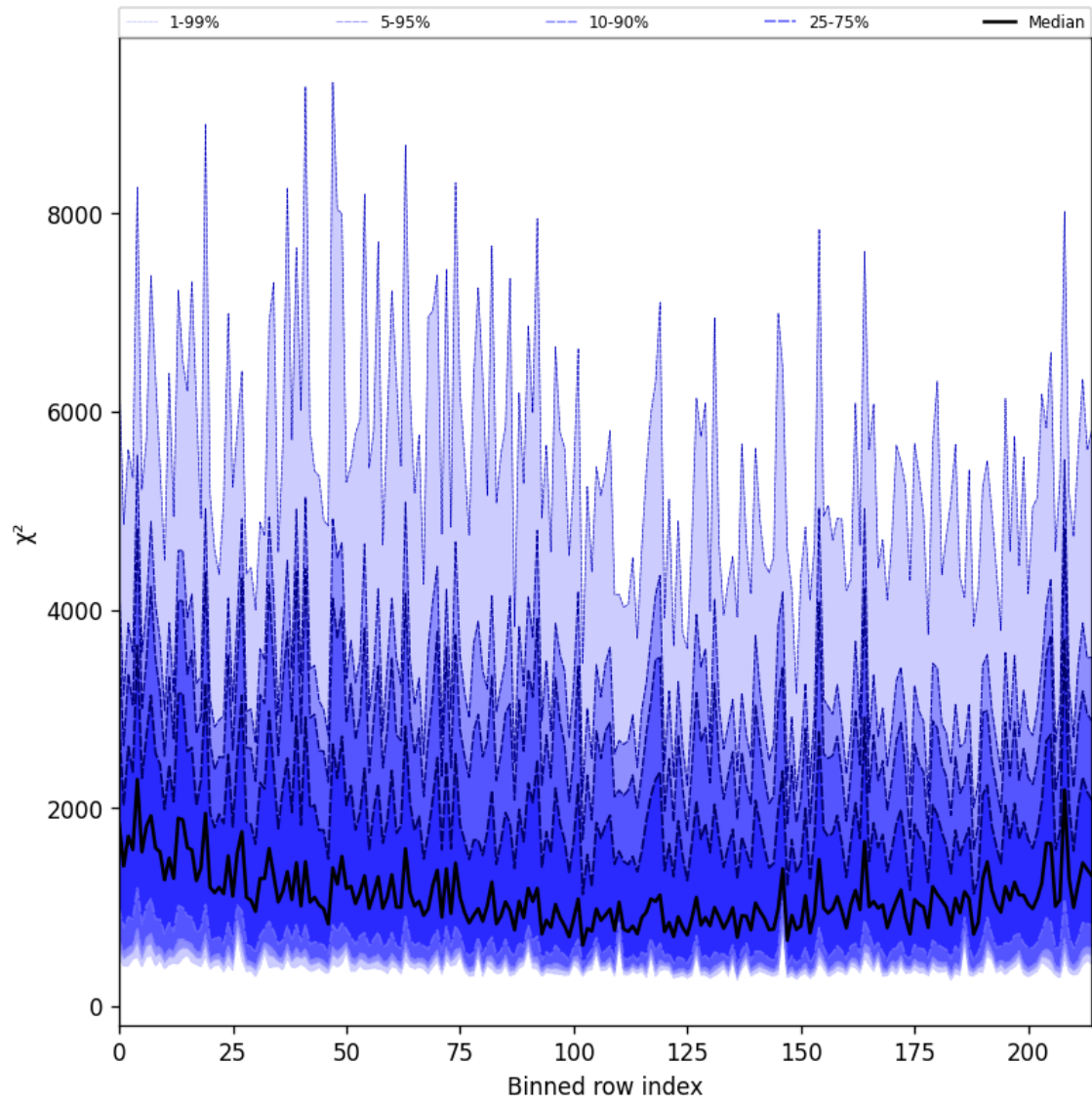
Figure 24: Along track statistics of “ \chi^2 ” for 2024-12-26 to 2024-12-27
