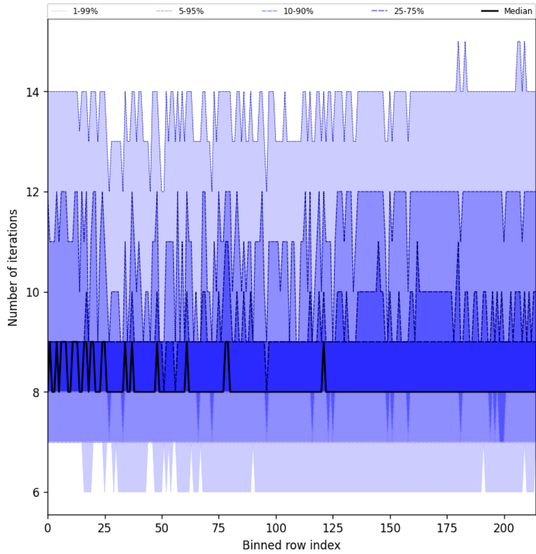
Figure 26: Along track statistics of “Number of iterations” for 2024-12-26 to 2024-12-27
