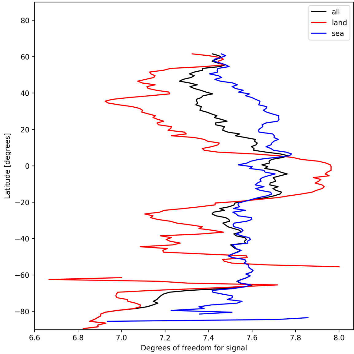
Figure 11: Zonal average of “Degrees of freedom for signal” for 2024-12-26 to 2024-12-27.
