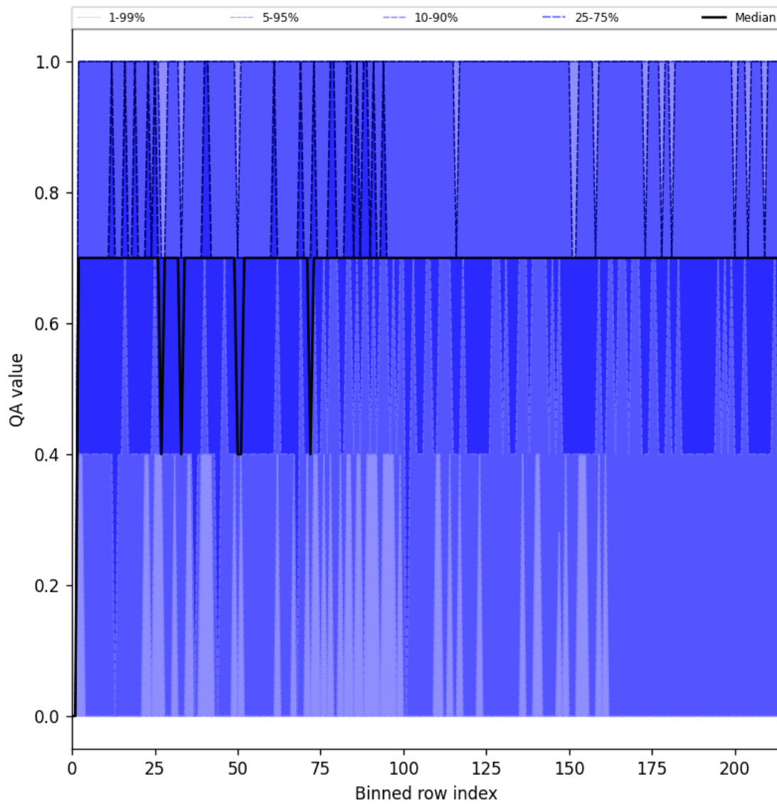
Figure 20: Along track statistics of “QA value” for 2024-12-26 to 2024-12-27
