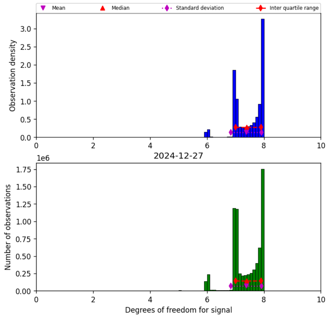
Figure 18: Histogram of “Degrees of freedom for signal” for 2024-12-27 to 2024-12-28
