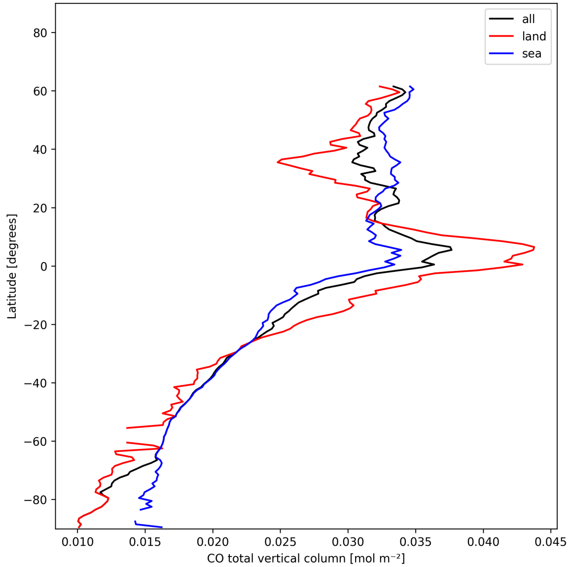
Figure 7: Zonal average of “CO total vertical column” for 2024-12-27 to 2024-12-28.
