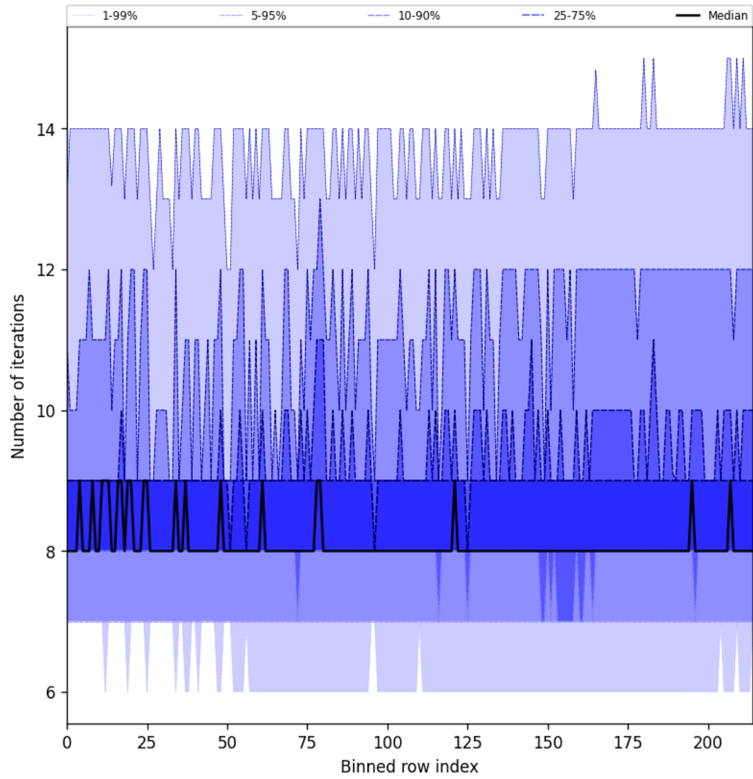
Figure 26: Along track statistics of “Number of iterations” for 2024-12-27 to 2024-12-28
