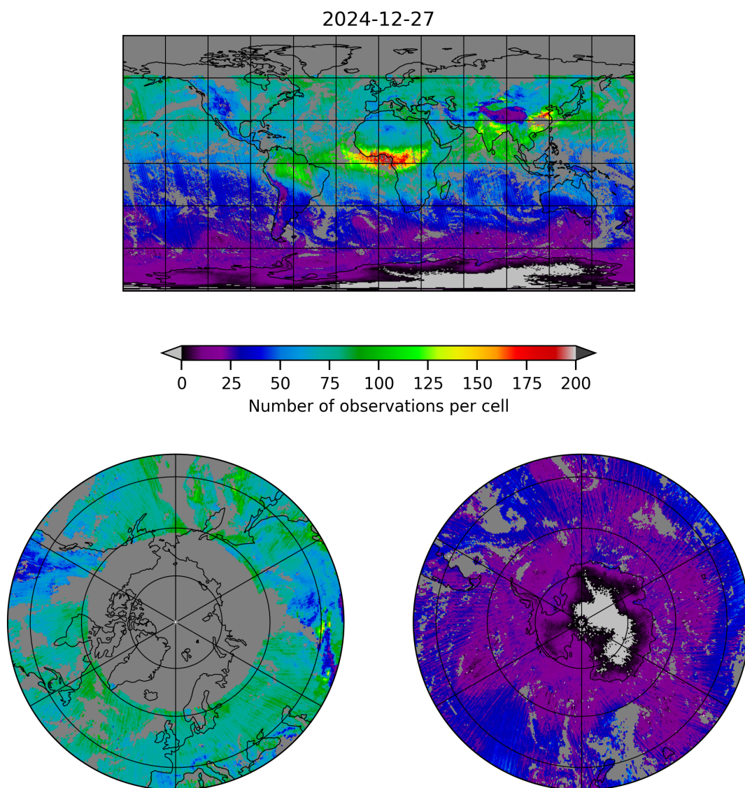
Figure 5: Map of the number of observations for 2024-12-27 to 2024-12-28
