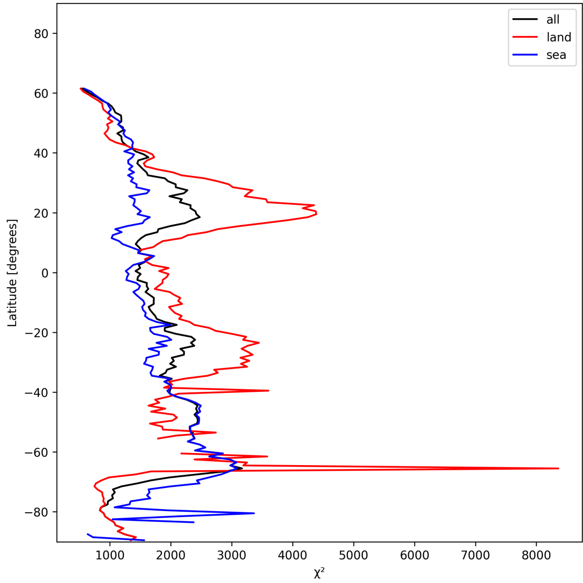
Figure 10: Zonal average of “ \chi^2 ” for 2024-12-27 to 2024-12-28.
