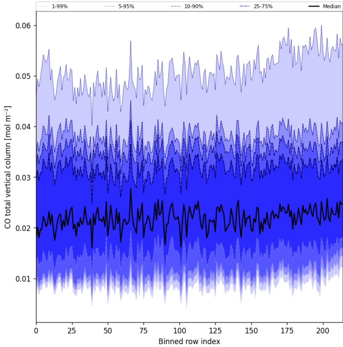
Figure 21: Along track statistics of “CO total vertical column” for 2024-12-27 to 2024-12-28
