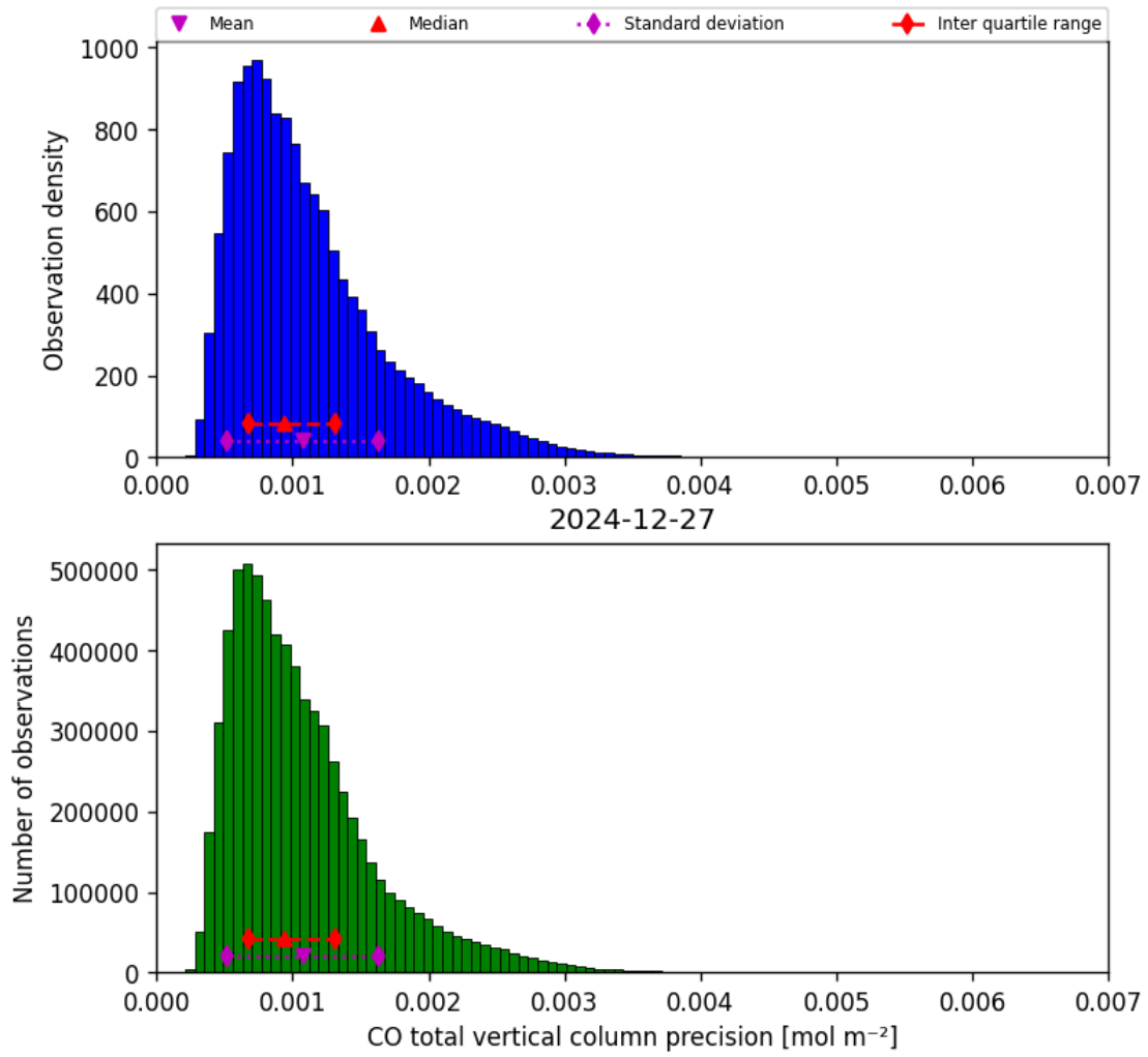
Figure 15: Histogram of “CO total vertical column precision” for 2024-12-27 to 2024-12-28
