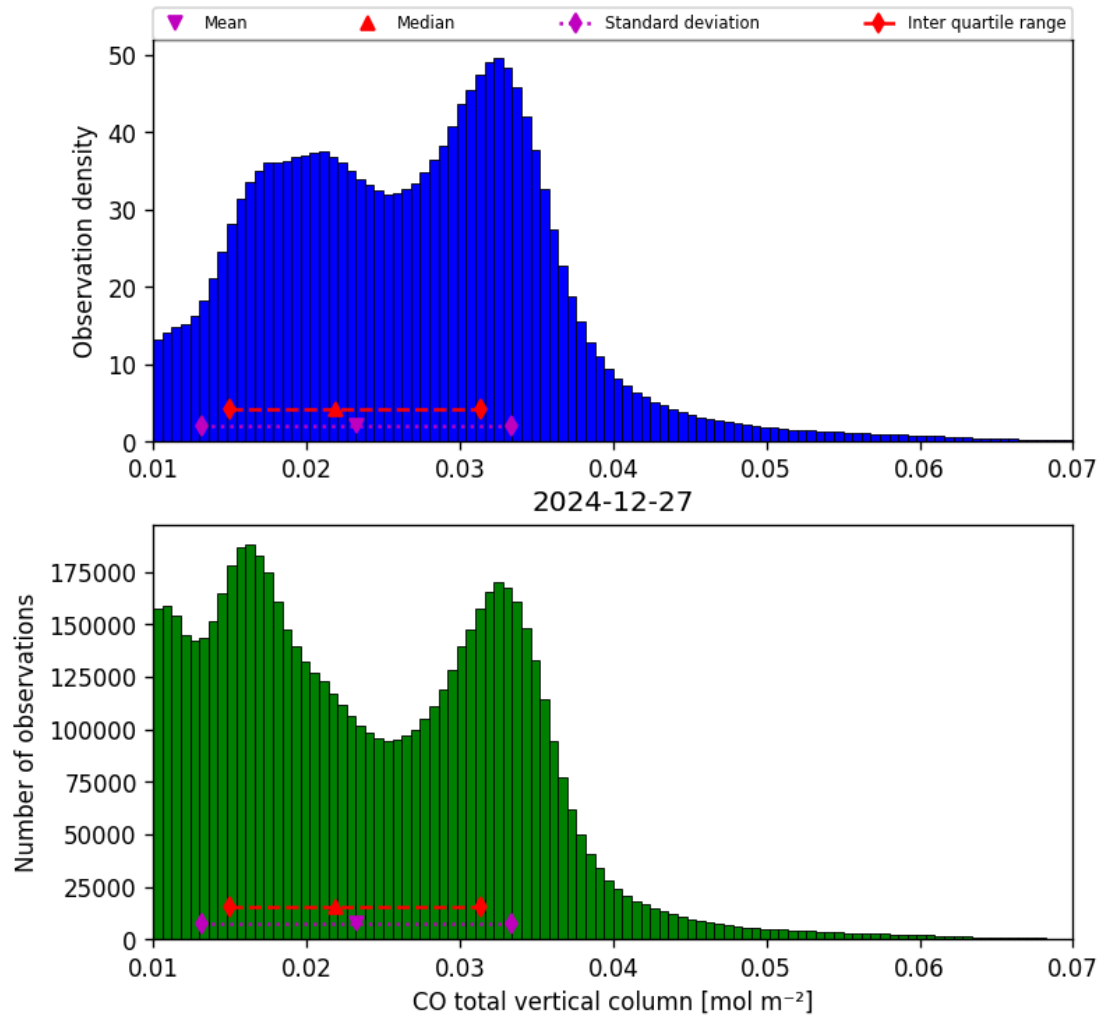
Figure 14: Histogram of “CO total vertical column” for 2024-12-27 to 2024-12-28
