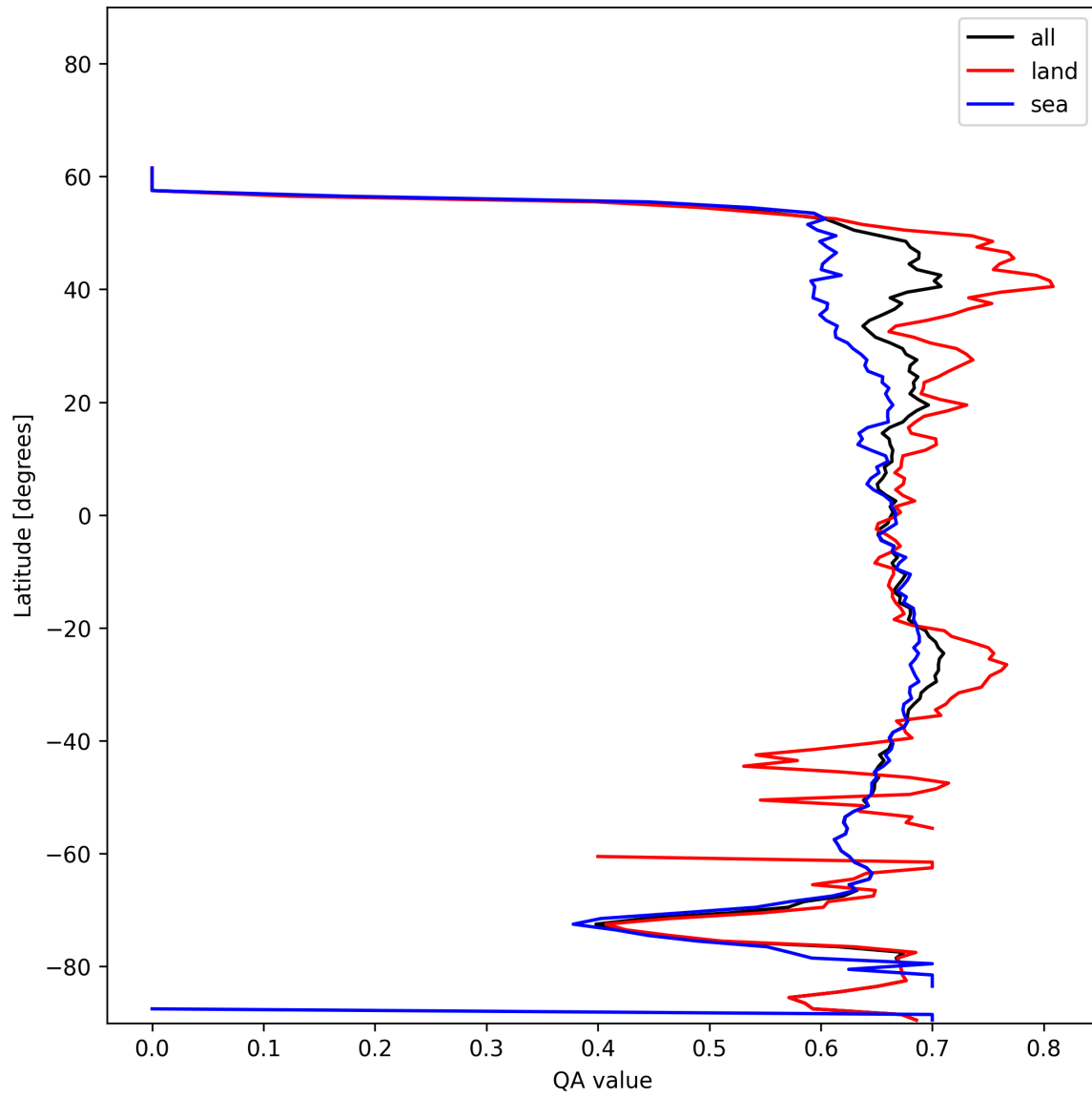
Figure 6: Zonal average of “QA value” for 2024-12-27 to 2024-12-28.
