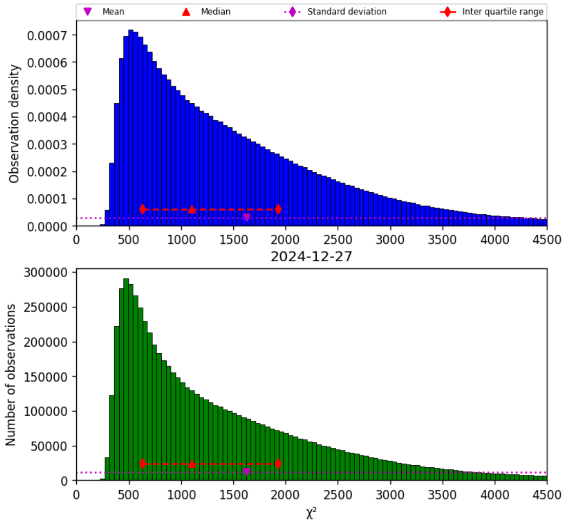
Figure 17: Histogram of “ \chi^2 ” for 2024-12-27 to 2024-12-28
