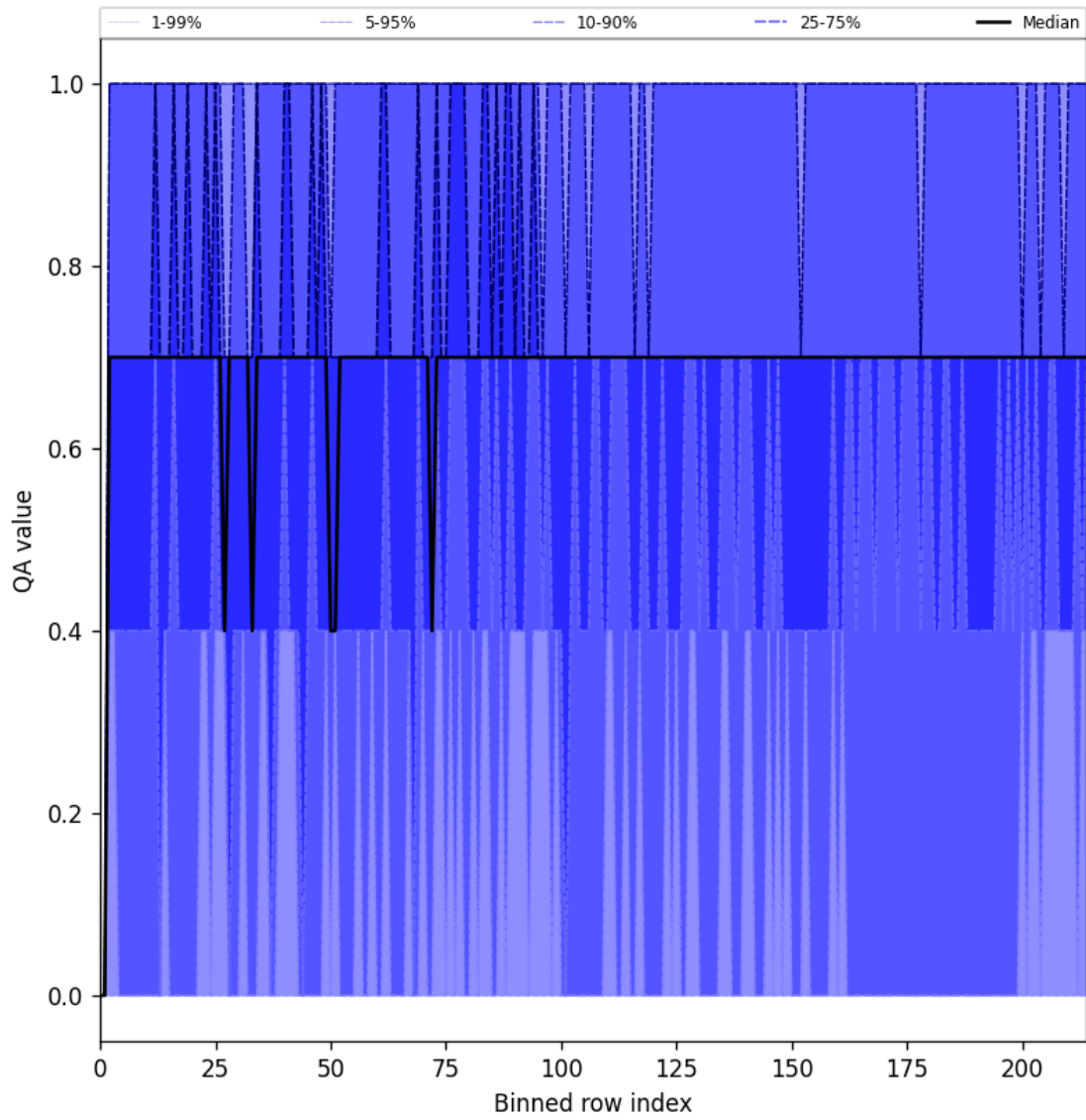
Figure 20: Along track statistics of “QA value” for 2024-12-27 to 2024-12-28
