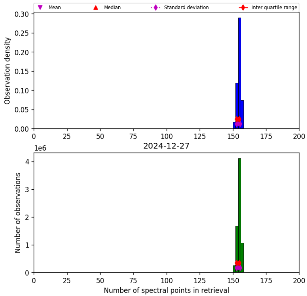
Figure 16: Histogram of “Number of spectral points in retrieval” for 2024-12-27 to 2024-12-28
