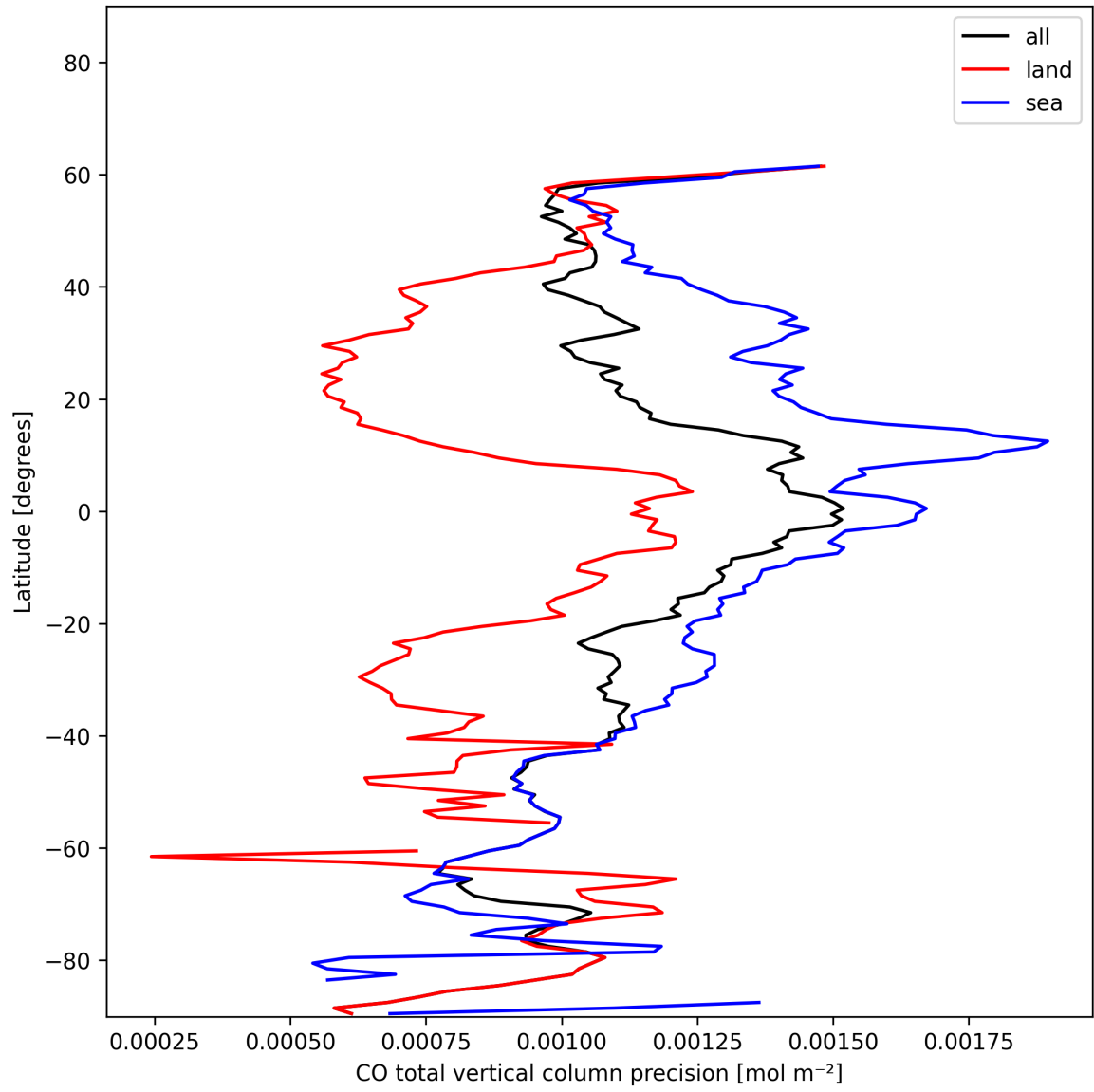
Figure 8: Zonal average of “CO total vertical column precision” for 2024-12-27 to 2024-12-28.
