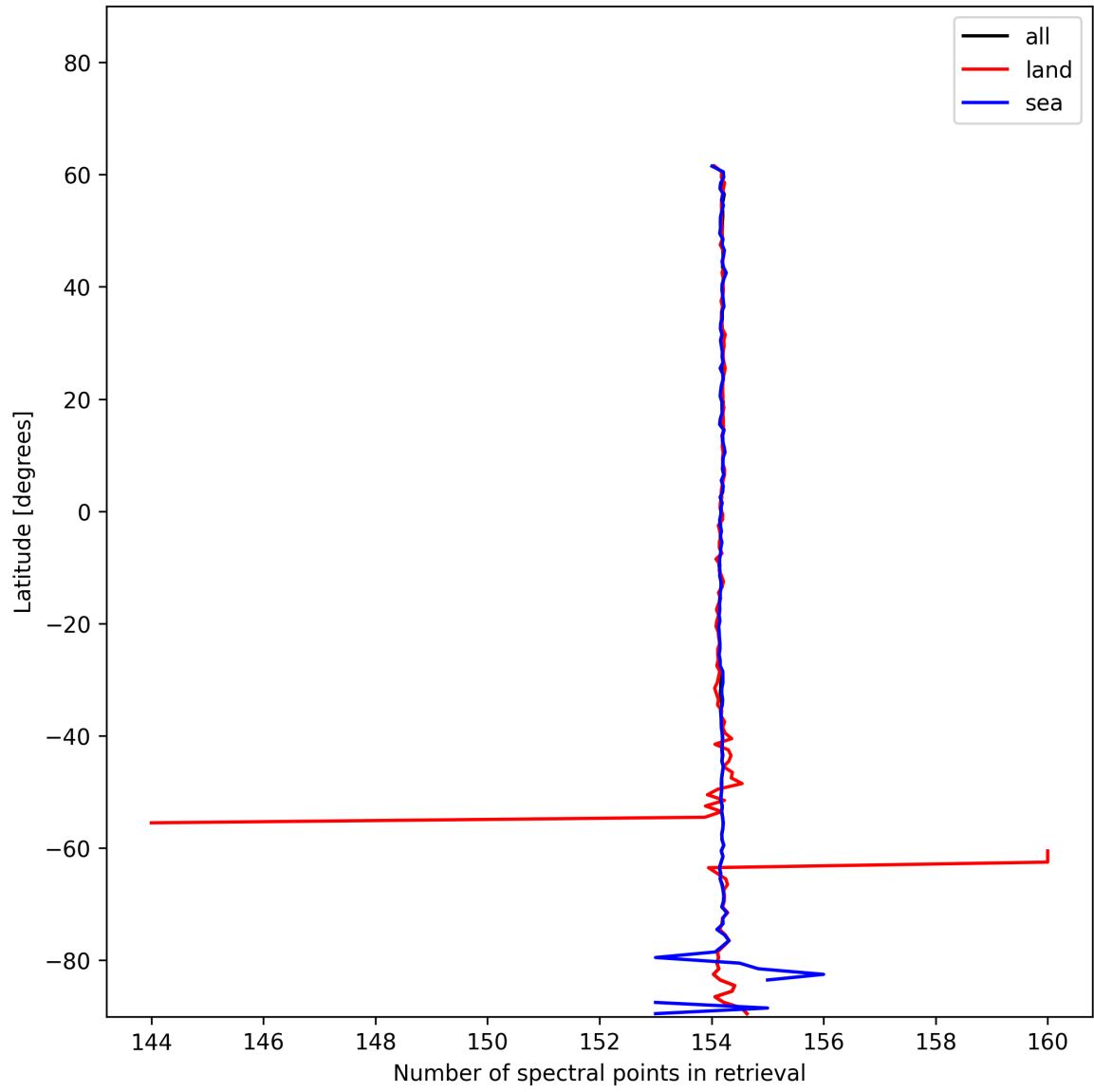
Figure 9: Zonal average of “Number of spectral points in retrieval” for 2024-12-27 to 2024-12-28.
