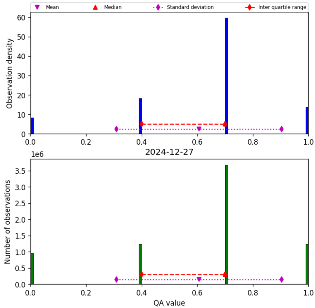
Figure 13: Histogram of “QA value” for 2024-12-27 to 2024-12-28
