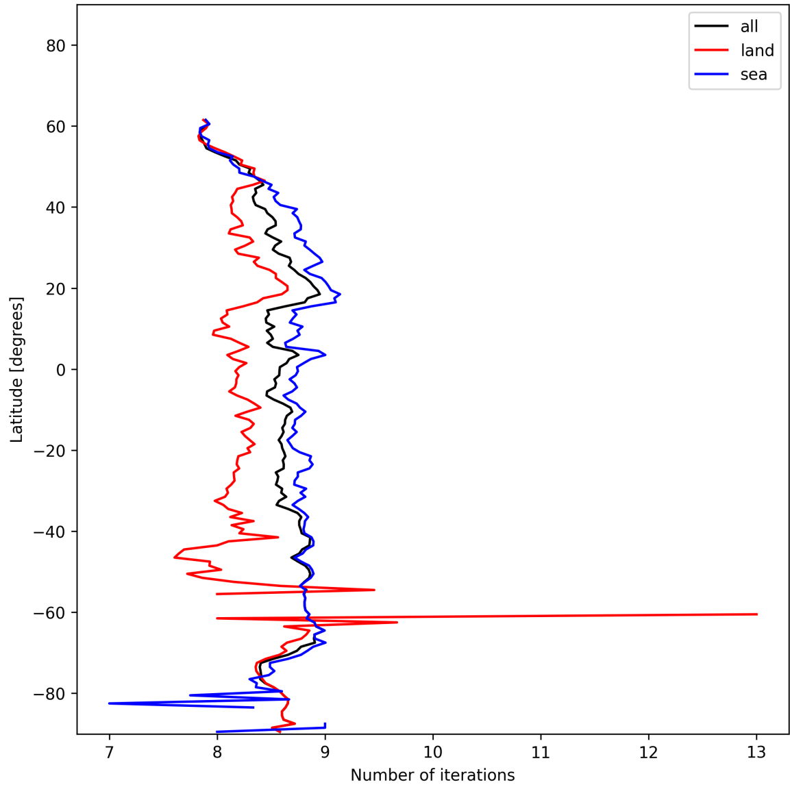
Figure 12: Zonal average of “Number of iterations” for 2024-12-27 to 2024-12-28.
