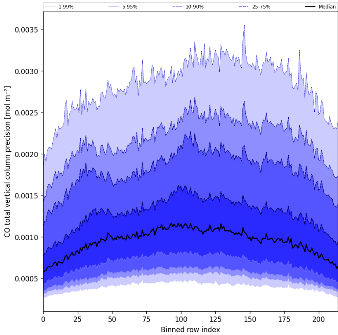
Figure 22: Along track statistics of “CO total vertical column precision” for 2024-12-27 to 2024-12-28
