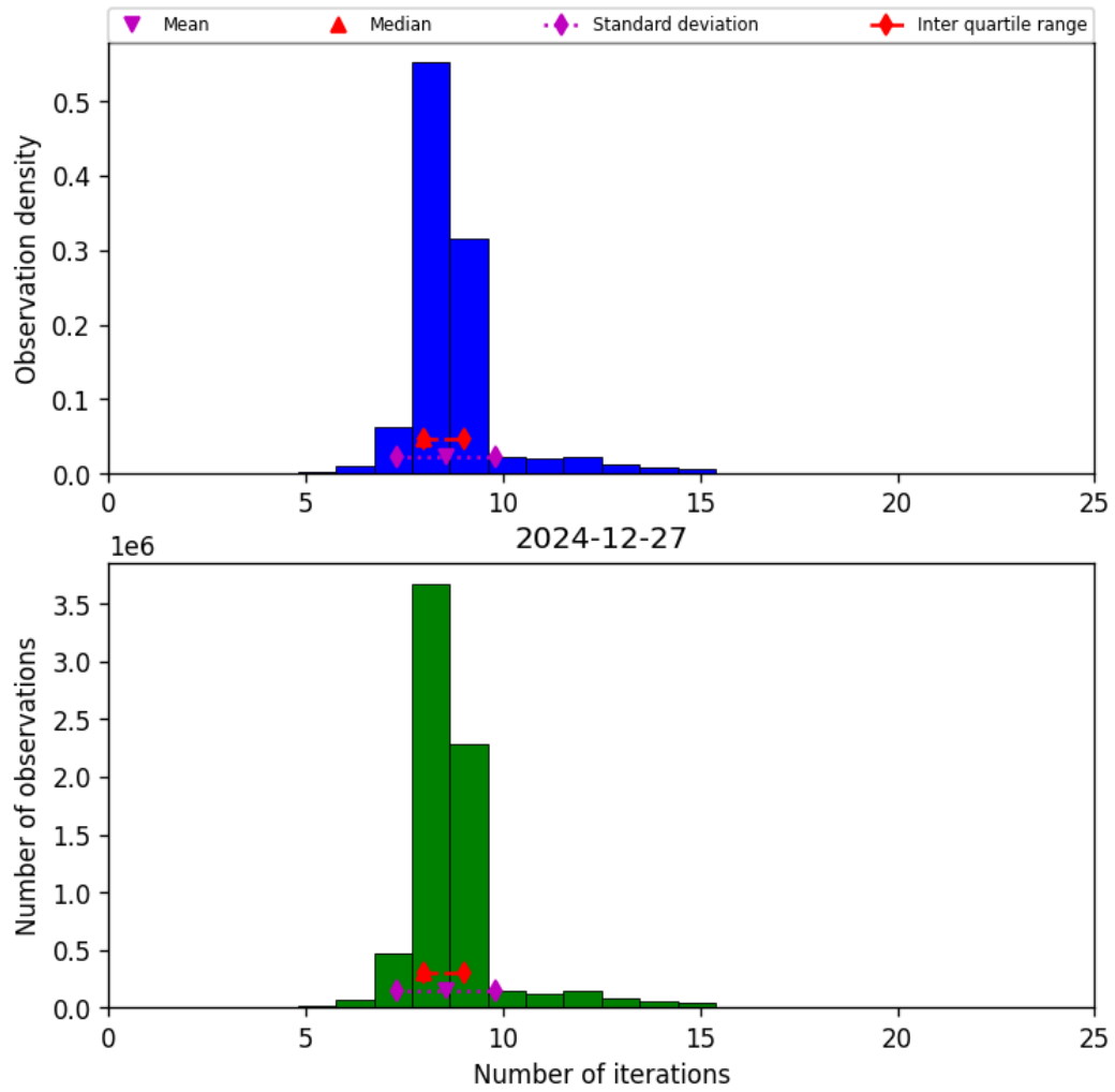
Figure 19: Histogram of “Number of iterations” for 2024-12-27 to 2024-12-28
