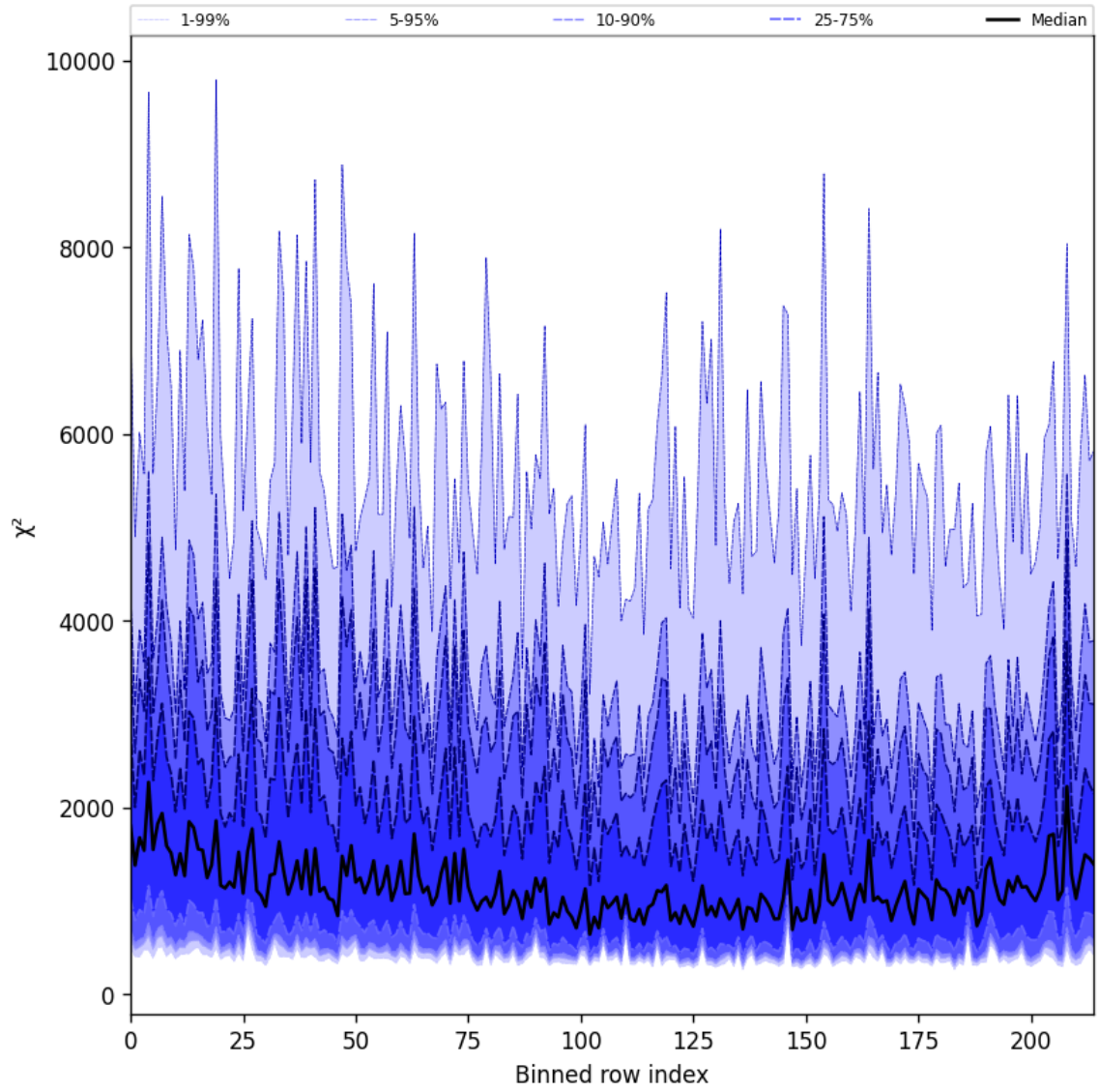
Figure 24: Along track statistics of “ \chi^2 ” for 2024-12-27 to 2024-12-28
