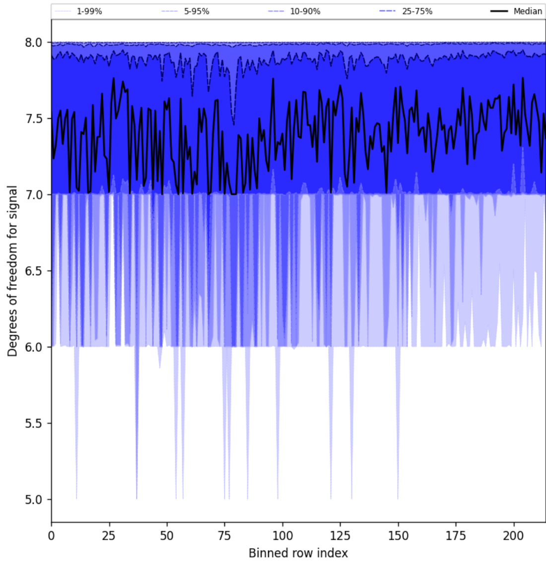
Figure 25: Along track statistics of “Degrees of freedom for signal” for 2024-12-27 to 2024-12-28
