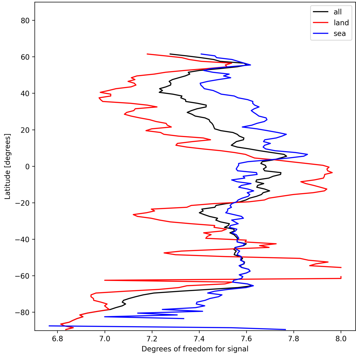
Figure 11: Zonal average of “Degrees of freedom for signal” for 2024-12-27 to 2024-12-28.
