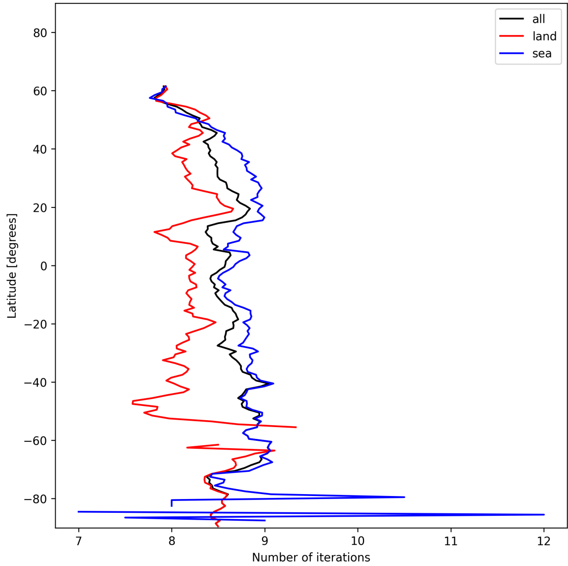
Figure 12: Zonal average of “Number of iterations” for 2024-12-28 to 2024-12-29.
