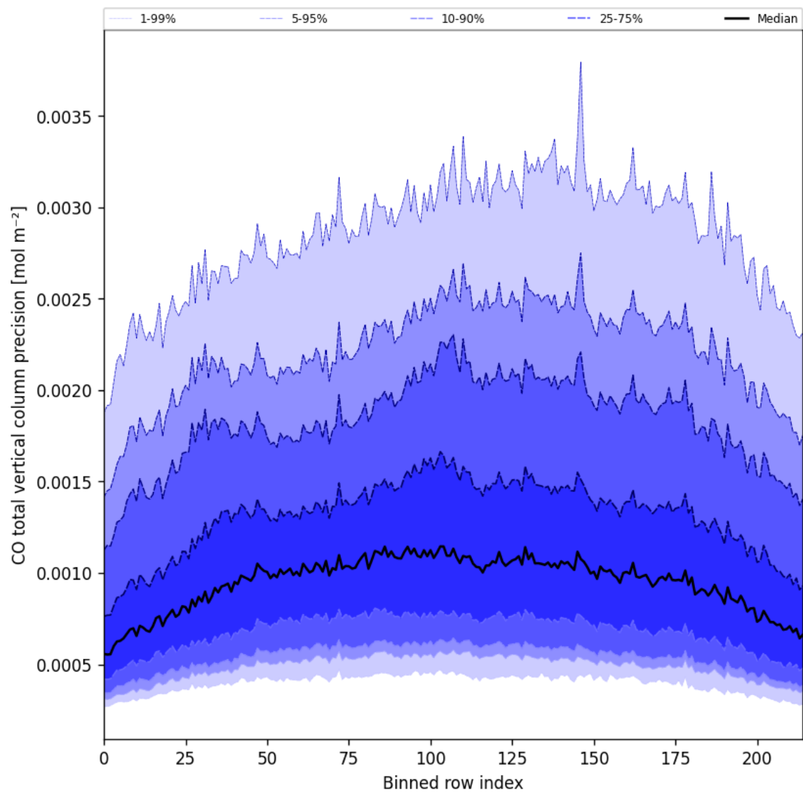
Figure 22: Along track statistics of “CO total vertical column precision” for 2024-12-28 to 2024-12-29
