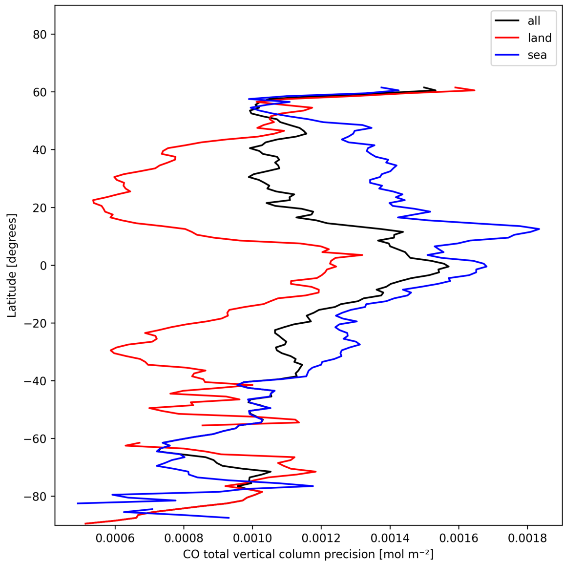
Figure 8: Zonal average of “CO total vertical column precision” for 2024-12-28 to 2024-12-29.
