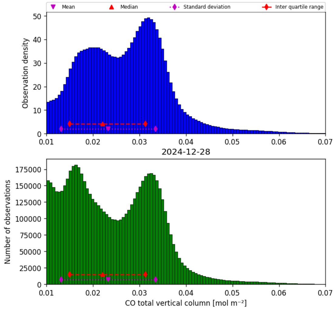
Figure 14: Histogram of “CO total vertical column” for 2024-12-28 to 2024-12-29
