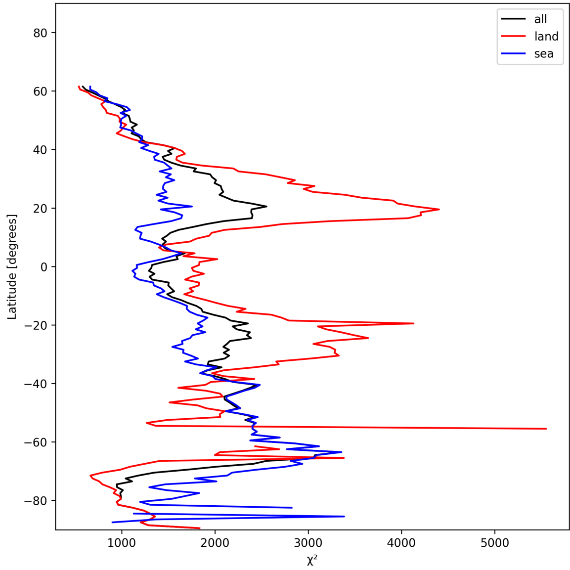
Figure 10: Zonal average of “ \chi^2 ” for 2024-12-28 to 2024-12-29.
