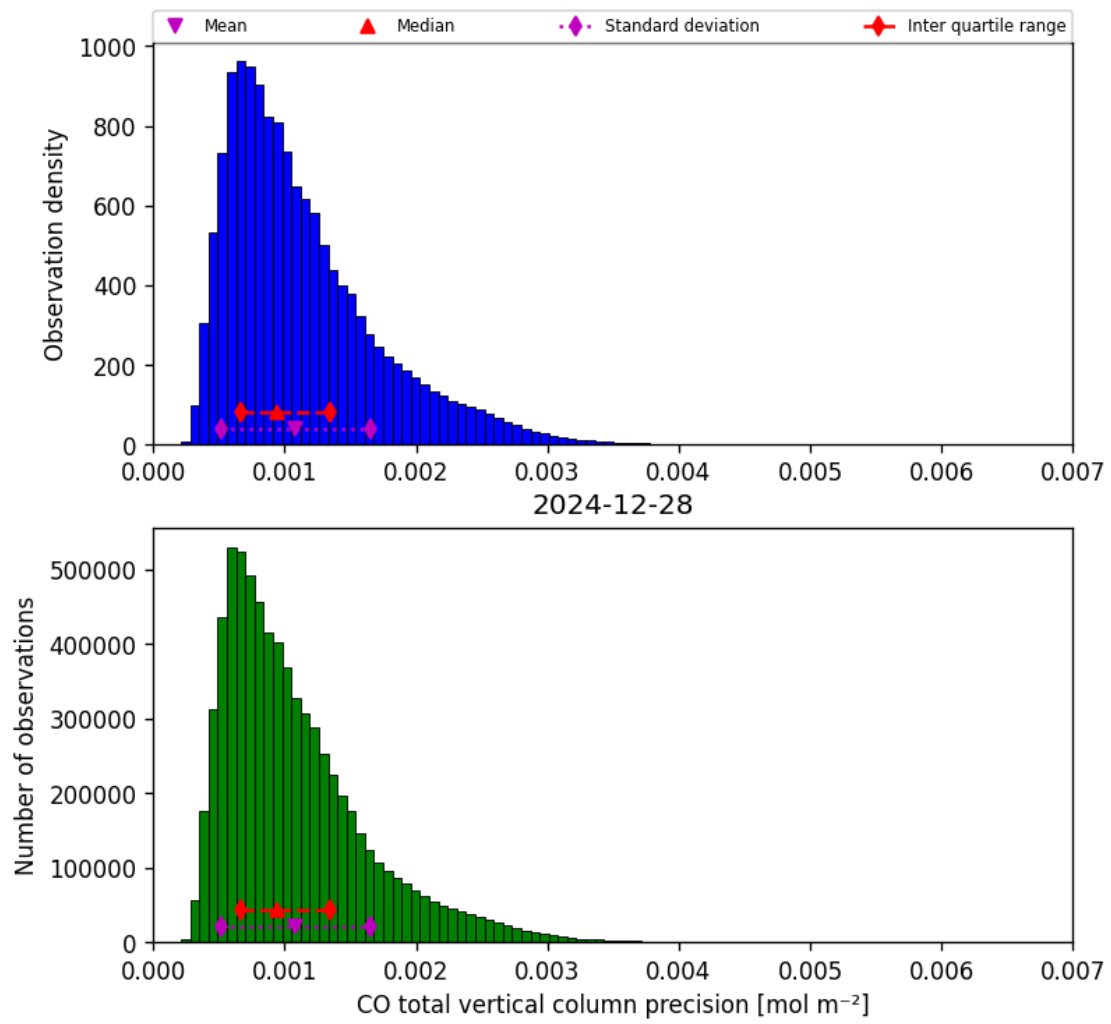
Figure 15: Histogram of “CO total vertical column precision” for 2024-12-28 to 2024-12-29
