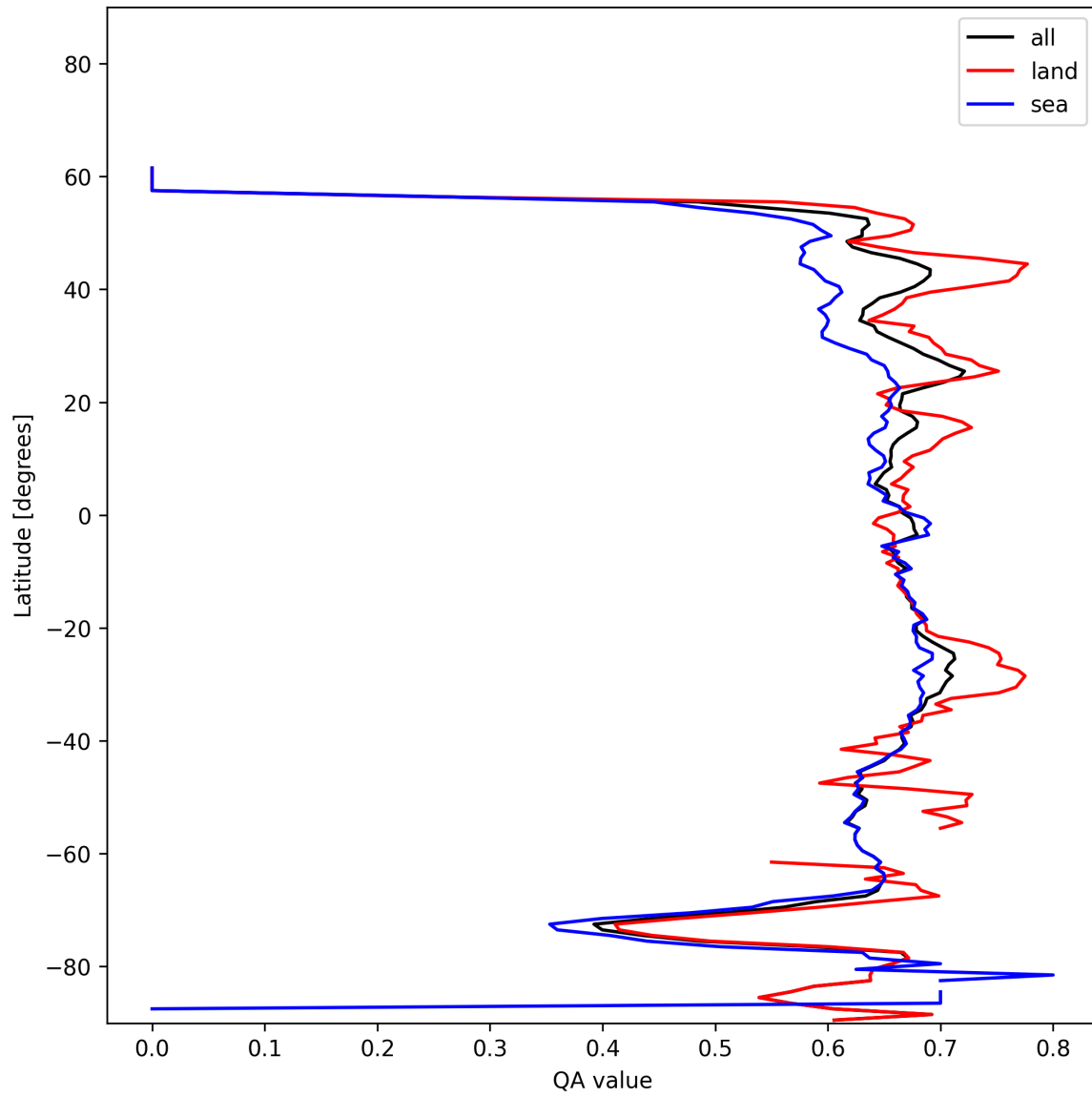
Figure 6: Zonal average of “QA value” for 2024-12-28 to 2024-12-29.
