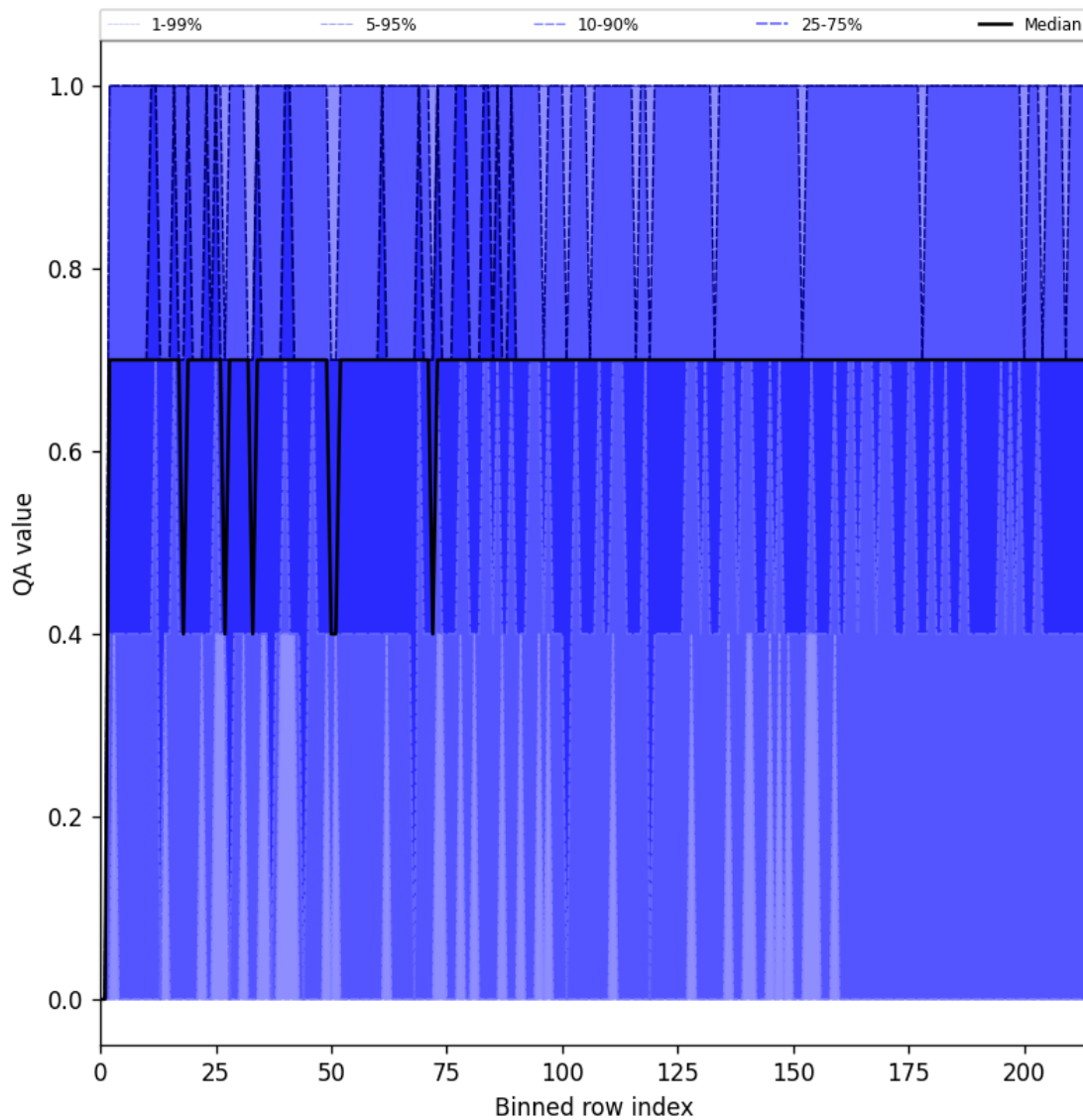
Figure 20: Along track statistics of “QA value” for 2024-12-28 to 2024-12-29
