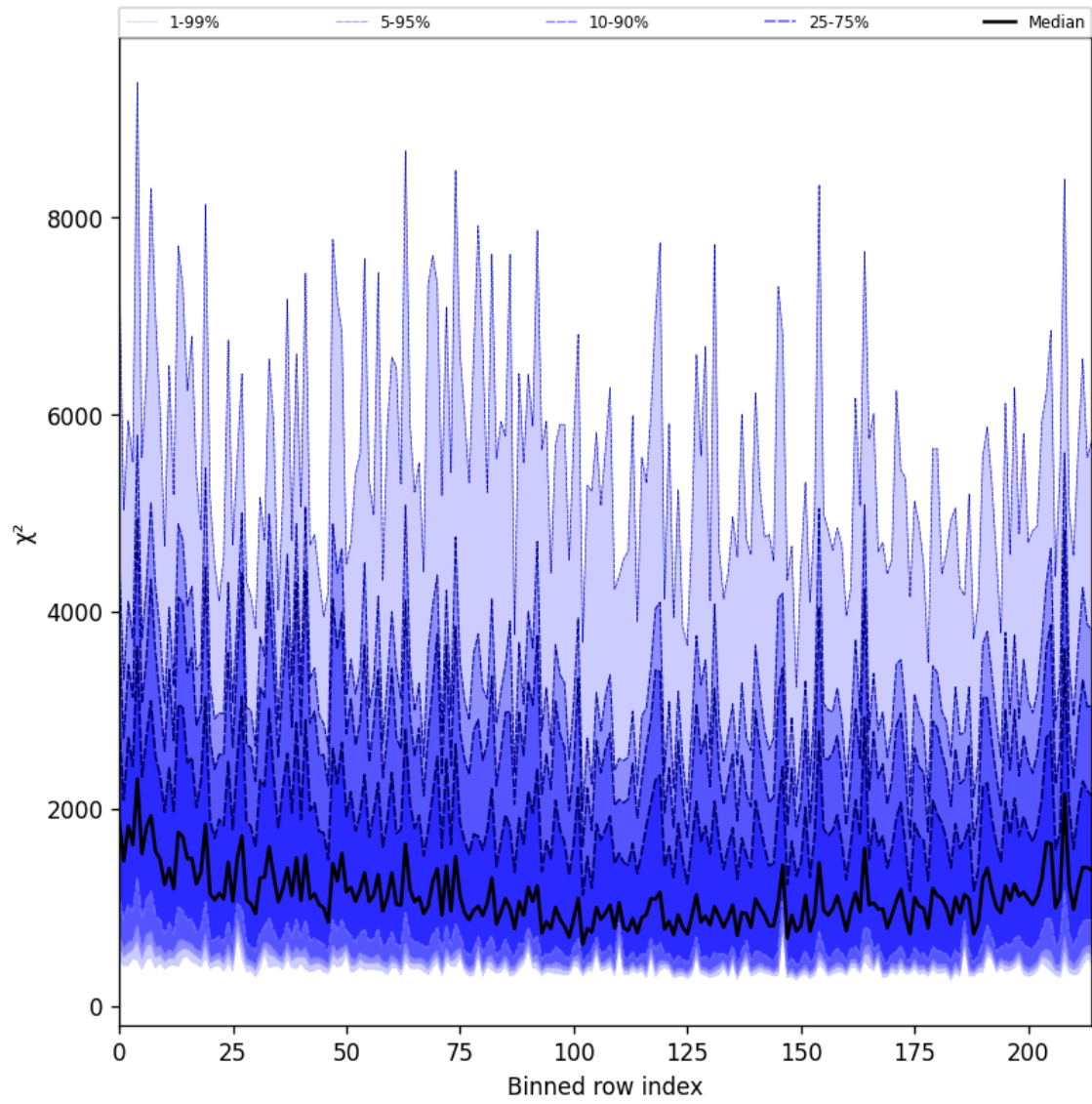
Figure 24: Along track statistics of “ \chi^2 ” for 2024-12-28 to 2024-12-29
