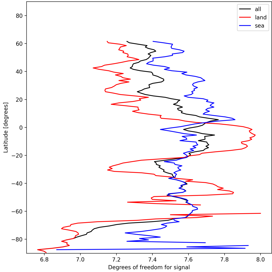
Figure 11: Zonal average of “Degrees of freedom for signal” for 2024-12-28 to 2024-12-29.
