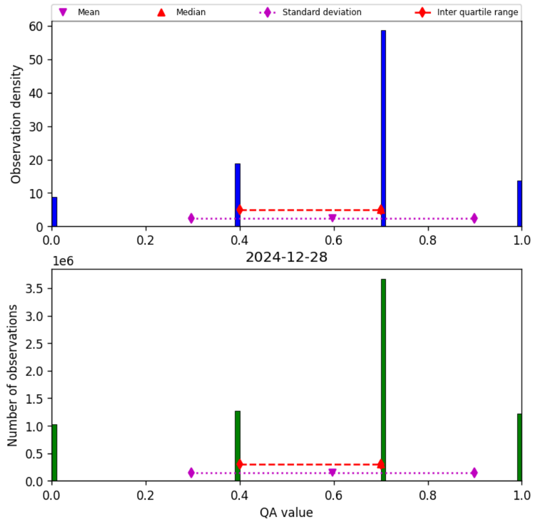
Figure 13: Histogram of “QA value” for 2024-12-28 to 2024-12-29
