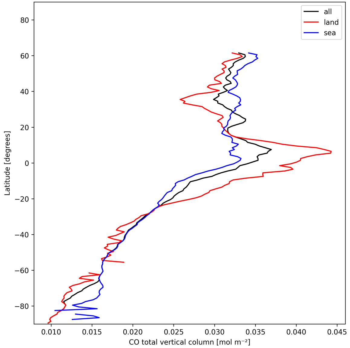
Figure 7: Zonal average of “CO total vertical column” for 2024-12-28 to 2024-12-29.
