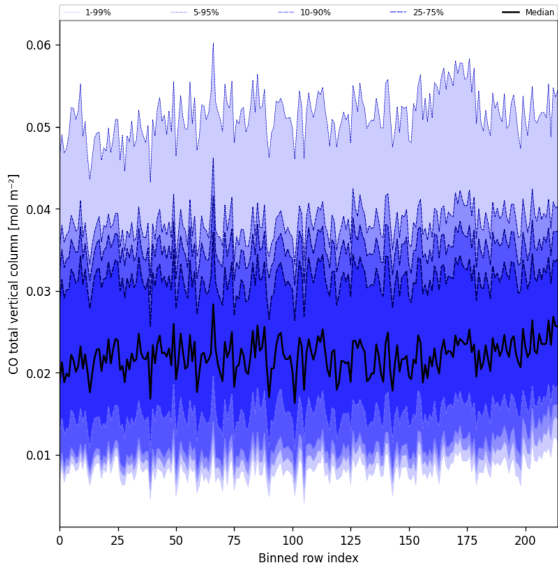
Figure 21: Along track statistics of “CO total vertical column” for 2024-12-28 to 2024-12-29
