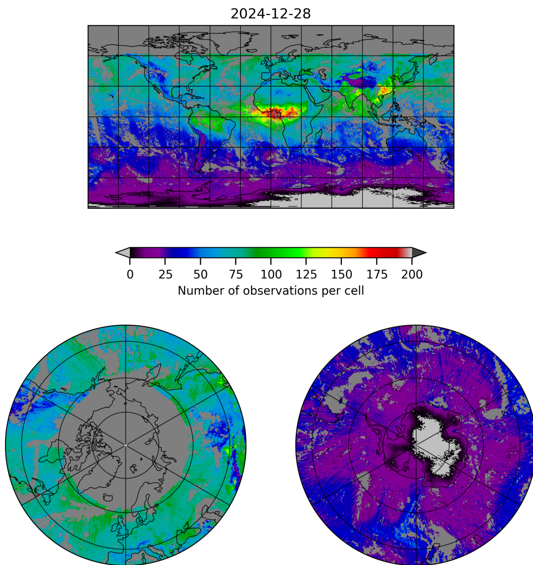
Figure 5: Map of the number of observations for 2024-12-28 to 2024-12-29
