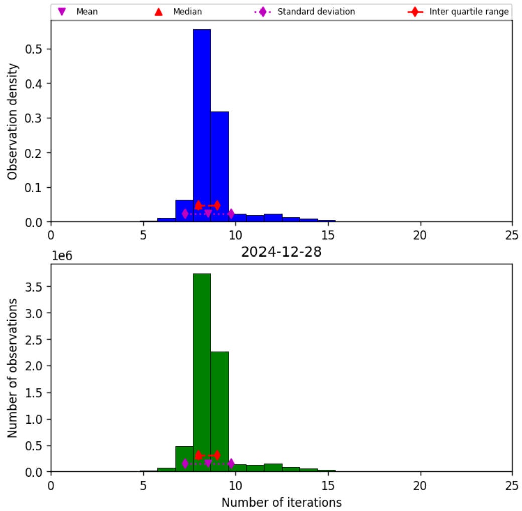
Figure 19: Histogram of “Number of iterations” for 2024-12-28 to 2024-12-29
