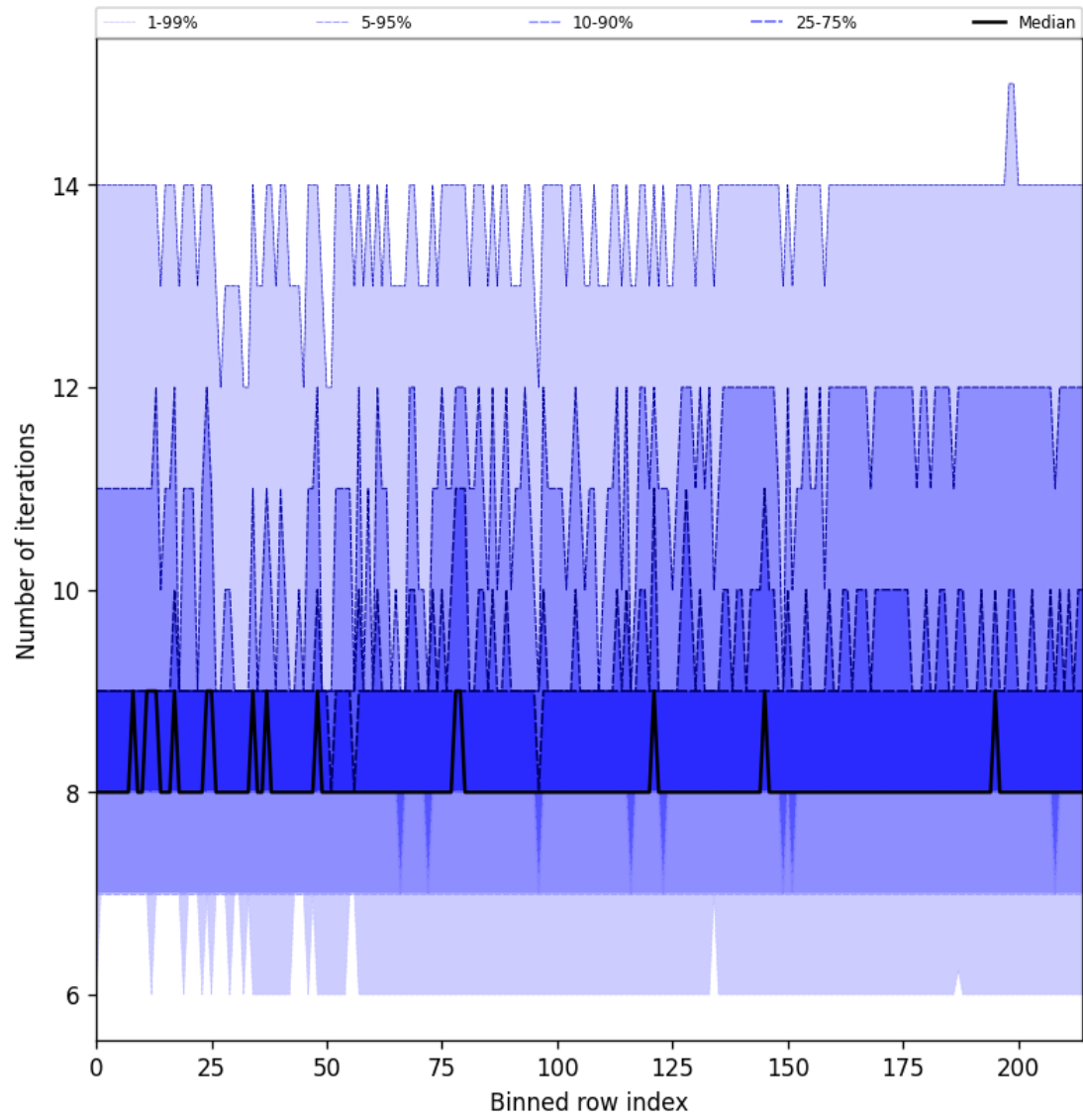
Figure 26: Along track statistics of “Number of iterations” for 2024-12-28 to 2024-12-29
