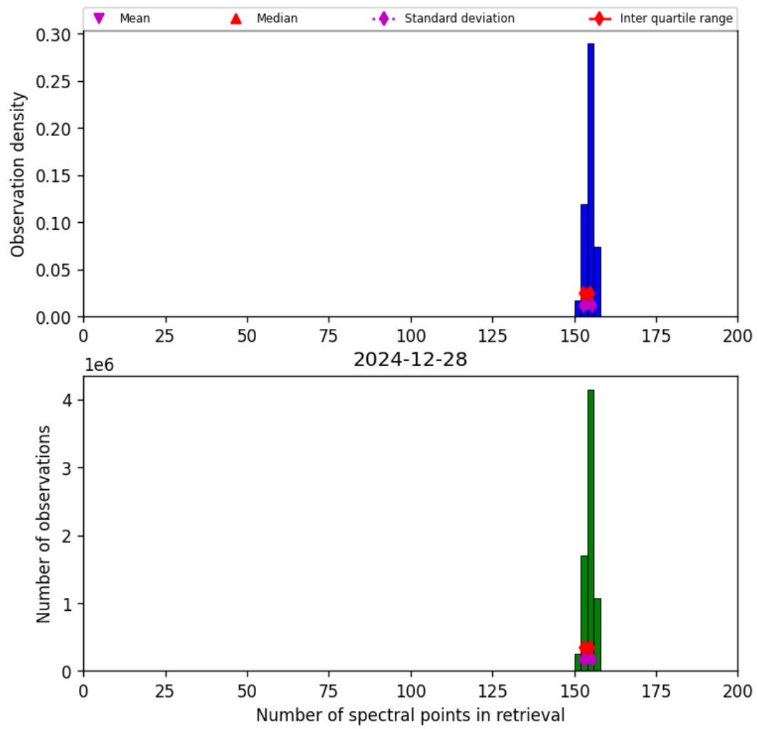
Figure 16: Histogram of “Number of spectral points in retrieval” for 2024-12-28 to 2024-12-29
