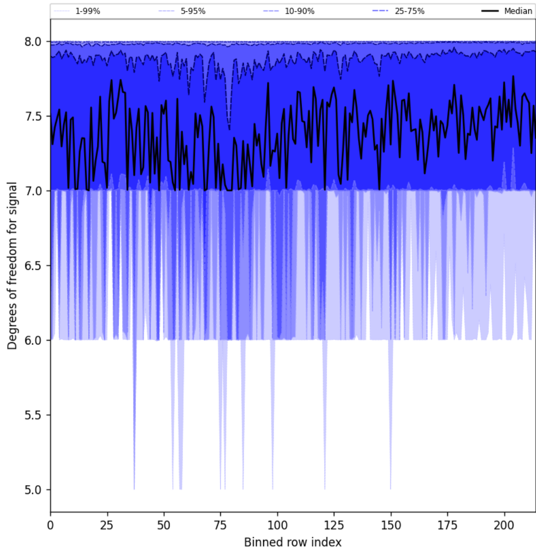
Figure 25: Along track statistics of “Degrees of freedom for signal” for 2024-12-28 to 2024-12-29
