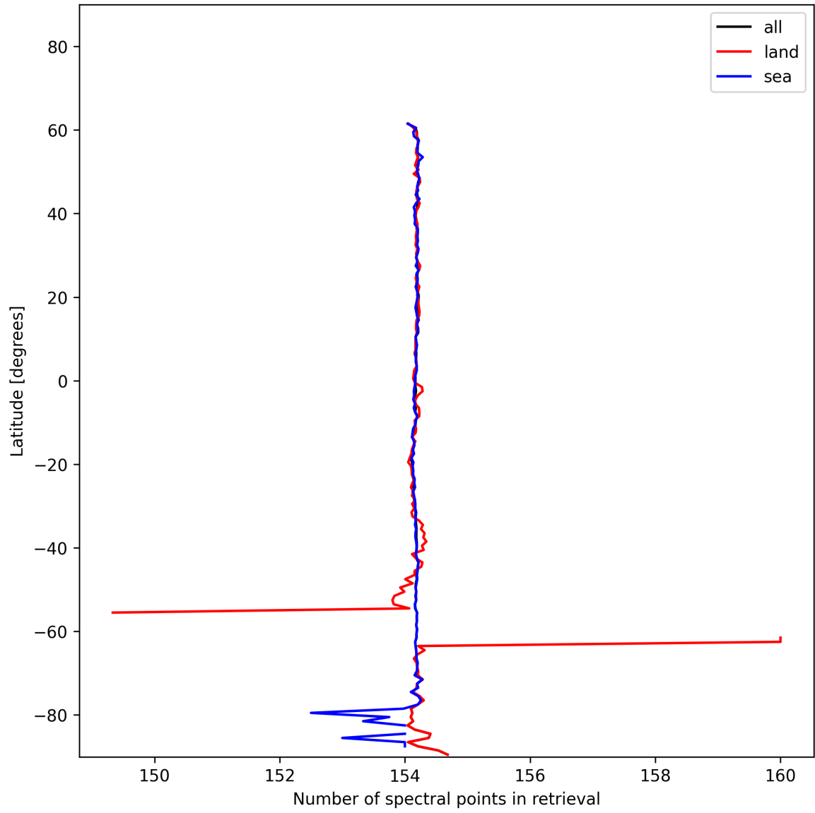
Figure 9: Zonal average of “Number of spectral points in retrieval” for 2024-12-28 to 2024-12-29.
