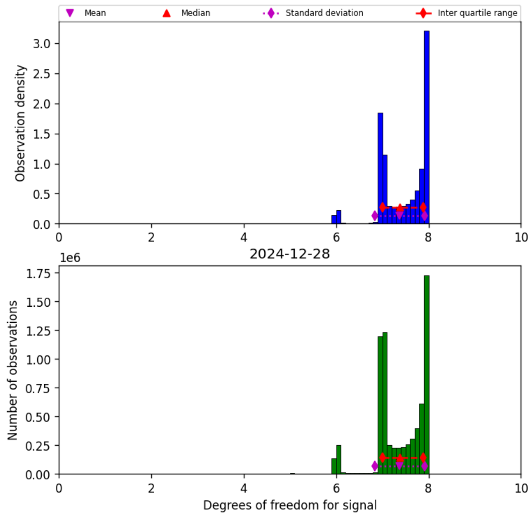
Figure 18: Histogram of “Degrees of freedom for signal” for 2024-12-28 to 2024-12-29
