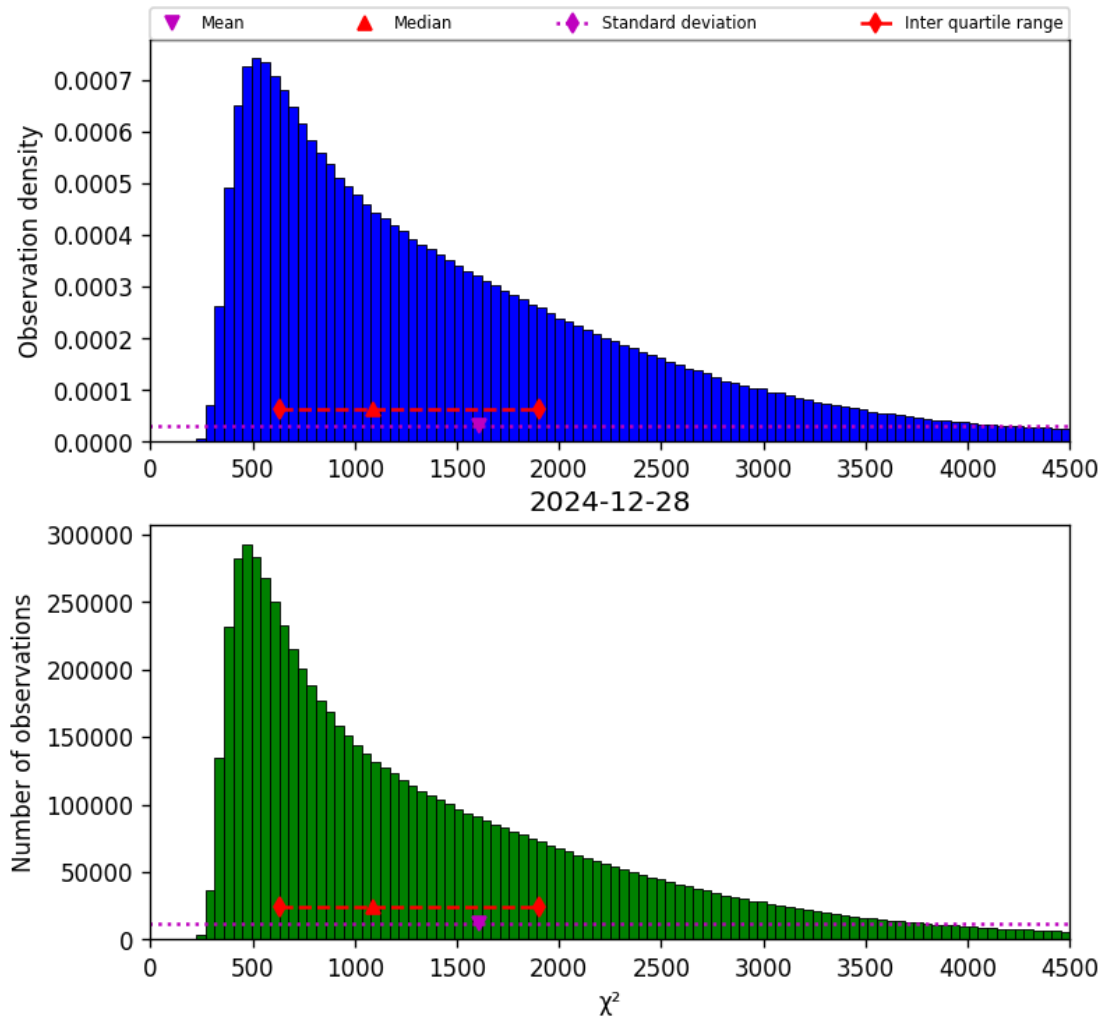
Figure 17: Histogram of “ \chi^2 ” for 2024-12-28 to 2024-12-29
