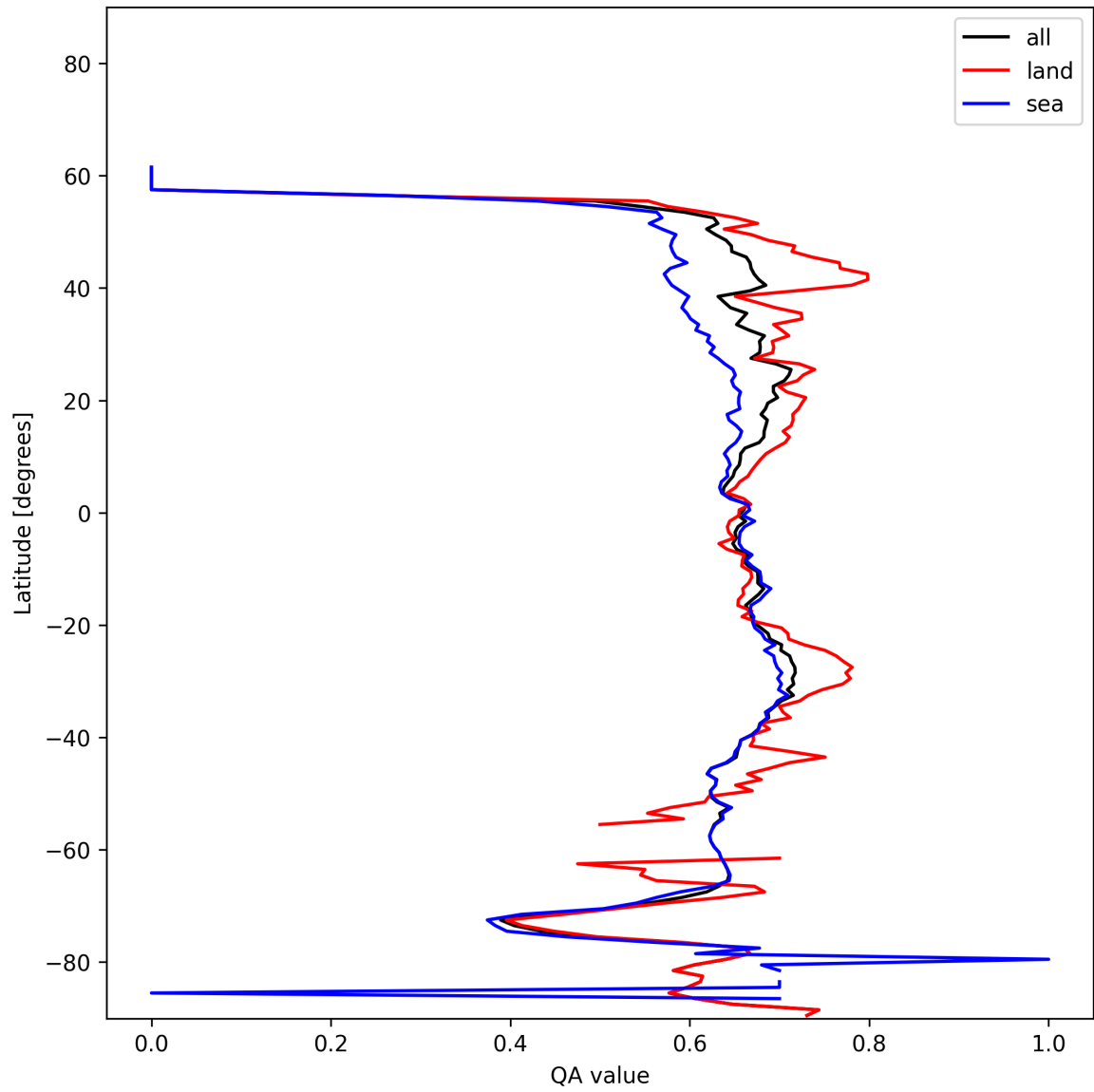
Figure 6: Zonal average of “QA value” for 2024-12-29 to 2024-12-30.
