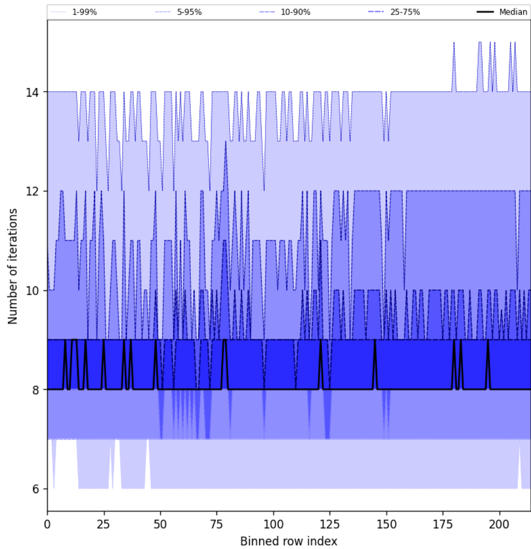
Figure 26: Along track statistics of “Number of iterations” for 2024-12-29 to 2024-12-30
