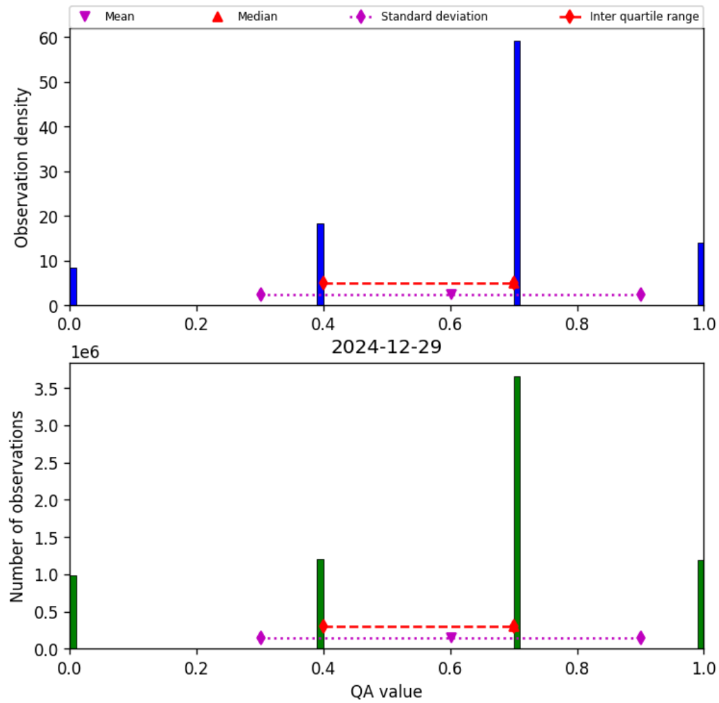
Figure 13: Histogram of “QA value” for 2024-12-29 to 2024-12-30
