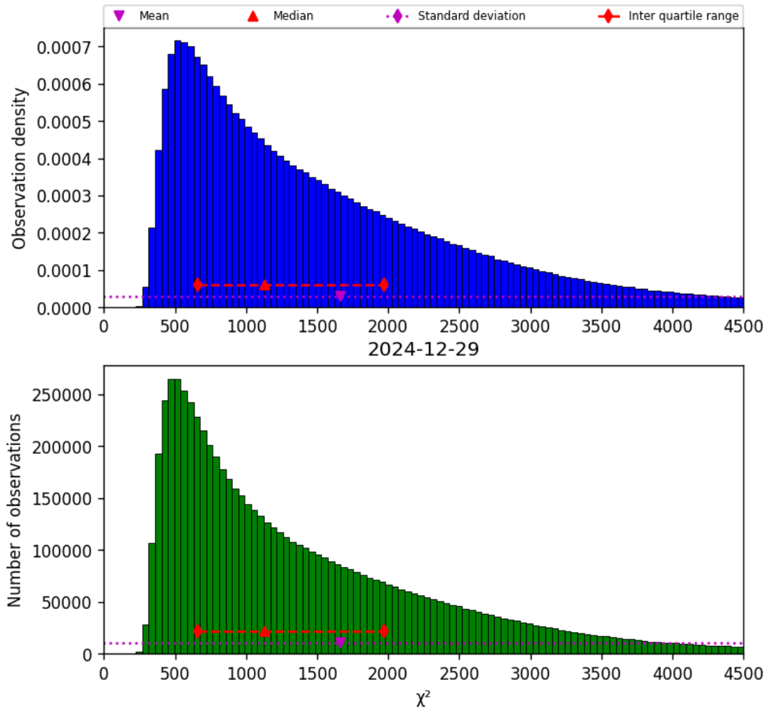
Figure 17: Histogram of “ \chi^2 ” for 2024-12-29 to 2024-12-30
