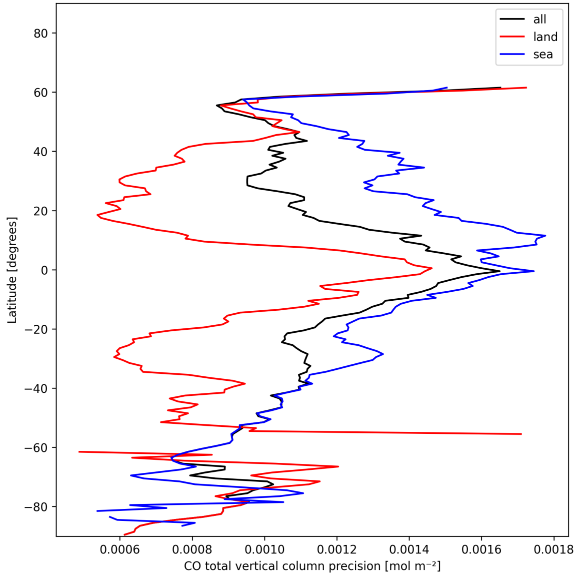
Figure 8: Zonal average of “CO total vertical column precision” for 2024-12-29 to 2024-12-30.
