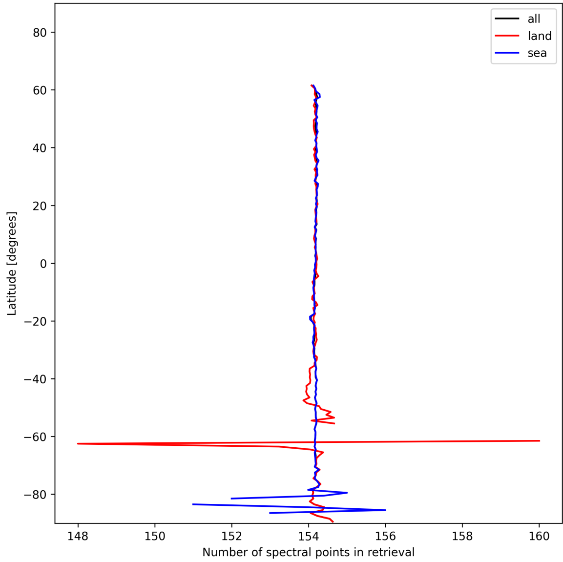
Figure 9: Zonal average of “Number of spectral points in retrieval” for 2024-12-29 to 2024-12-30.
