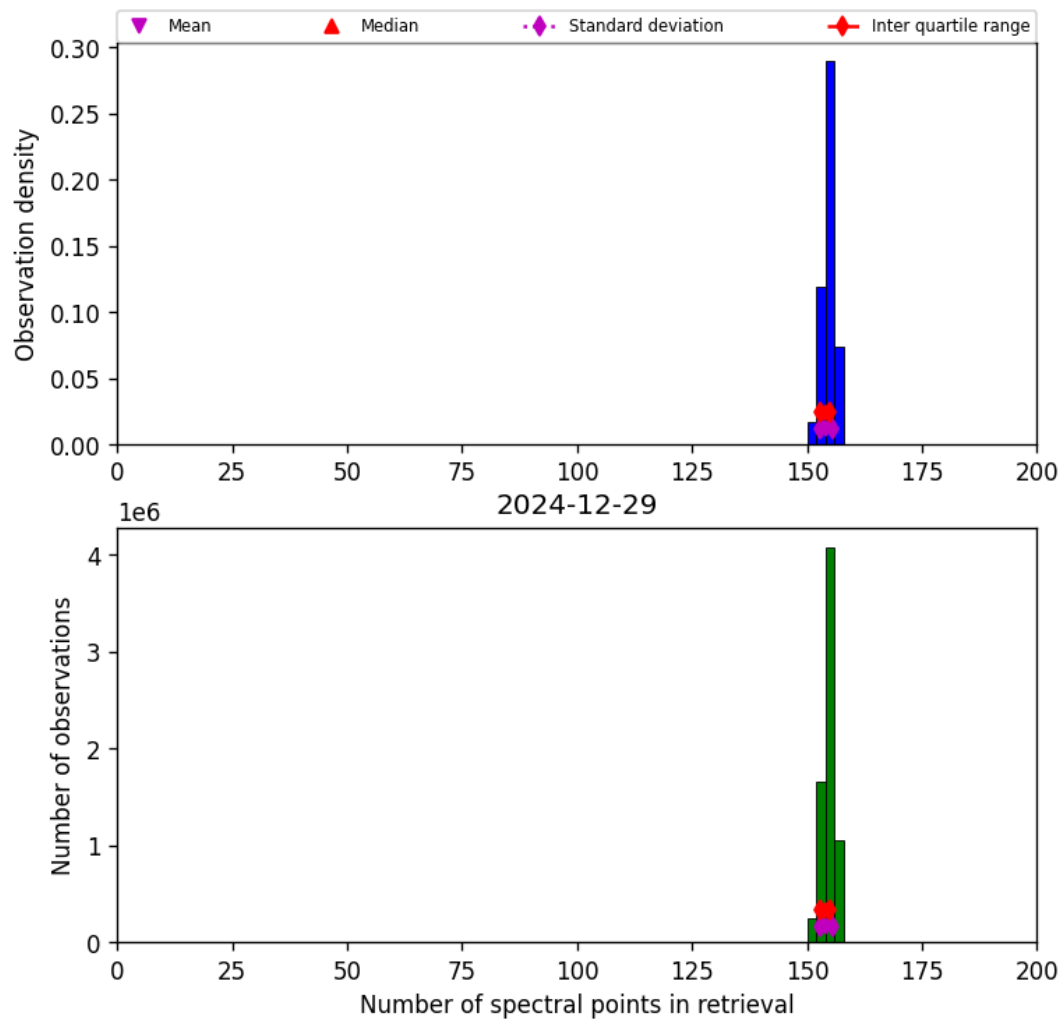
Figure 16: Histogram of “Number of spectral points in retrieval” for 2024-12-29 to 2024-12-30
