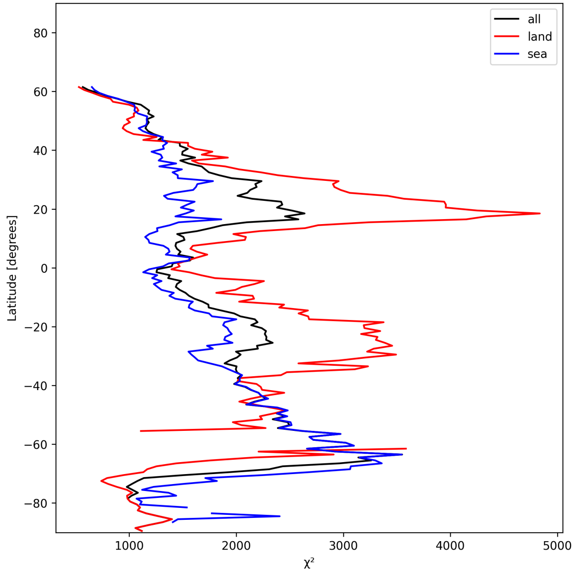
Figure 10: Zonal average of “ \chi^2 ” for 2024-12-29 to 2024-12-30.
