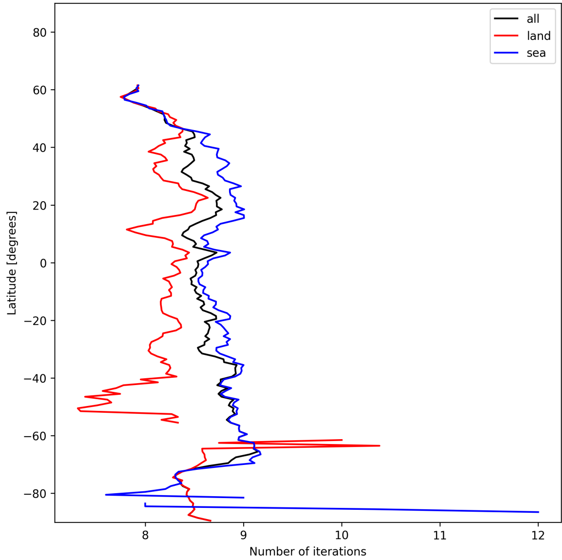
Figure 12: Zonal average of “Number of iterations” for 2024-12-29 to 2024-12-30.
