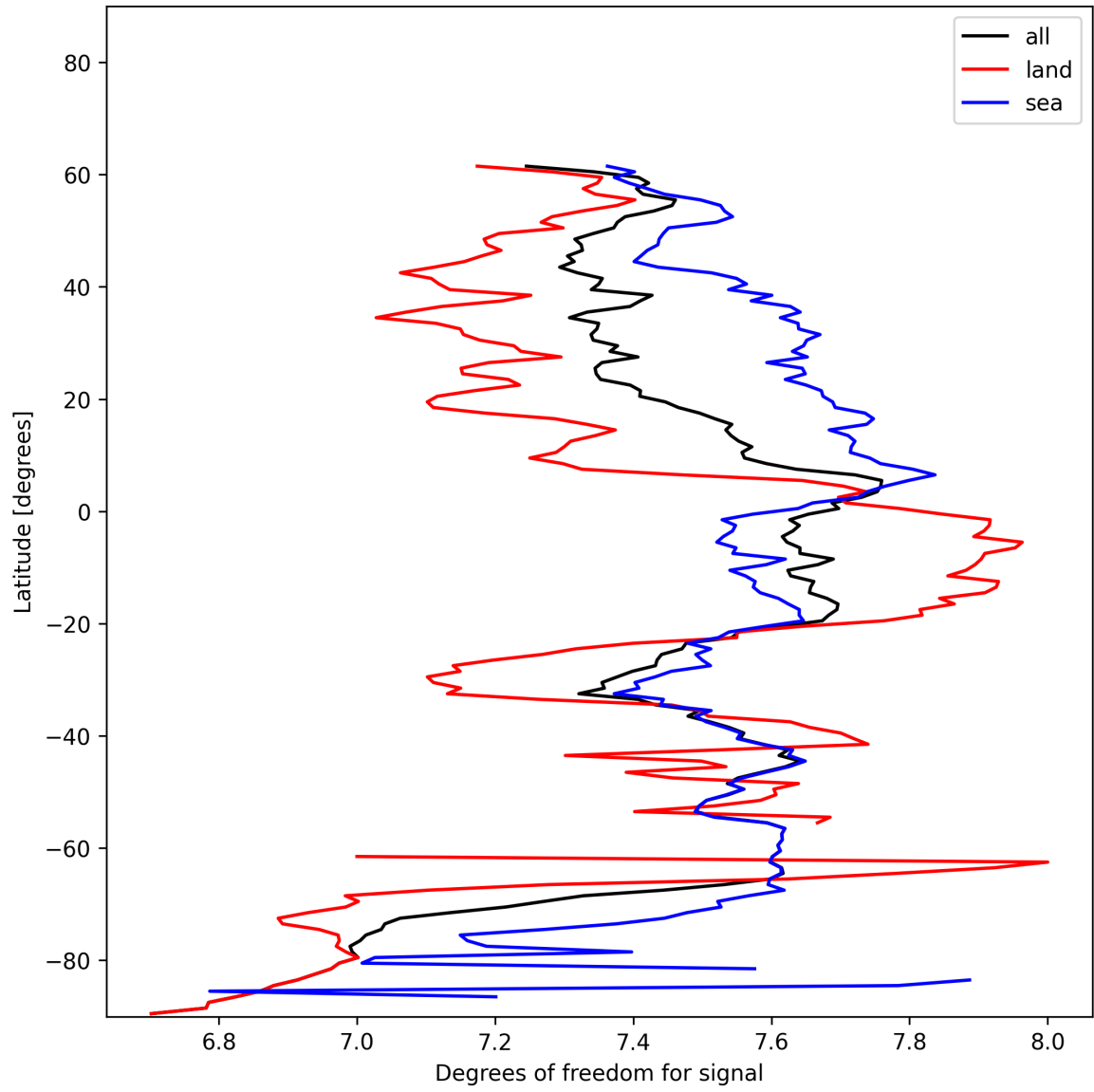
Figure 11: Zonal average of “Degrees of freedom for signal” for 2024-12-29 to 2024-12-30.
