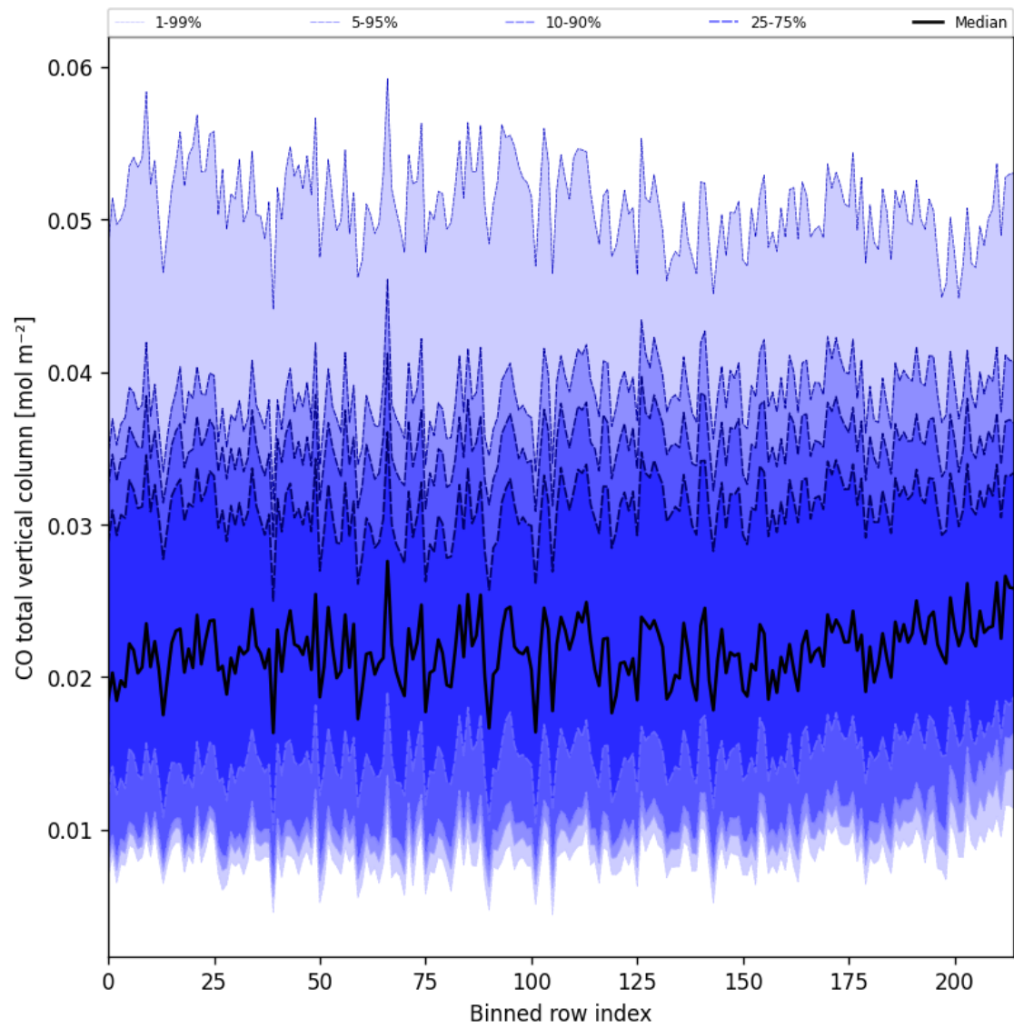
Figure 21: Along track statistics of “CO total vertical column” for 2024-12-29 to 2024-12-30
