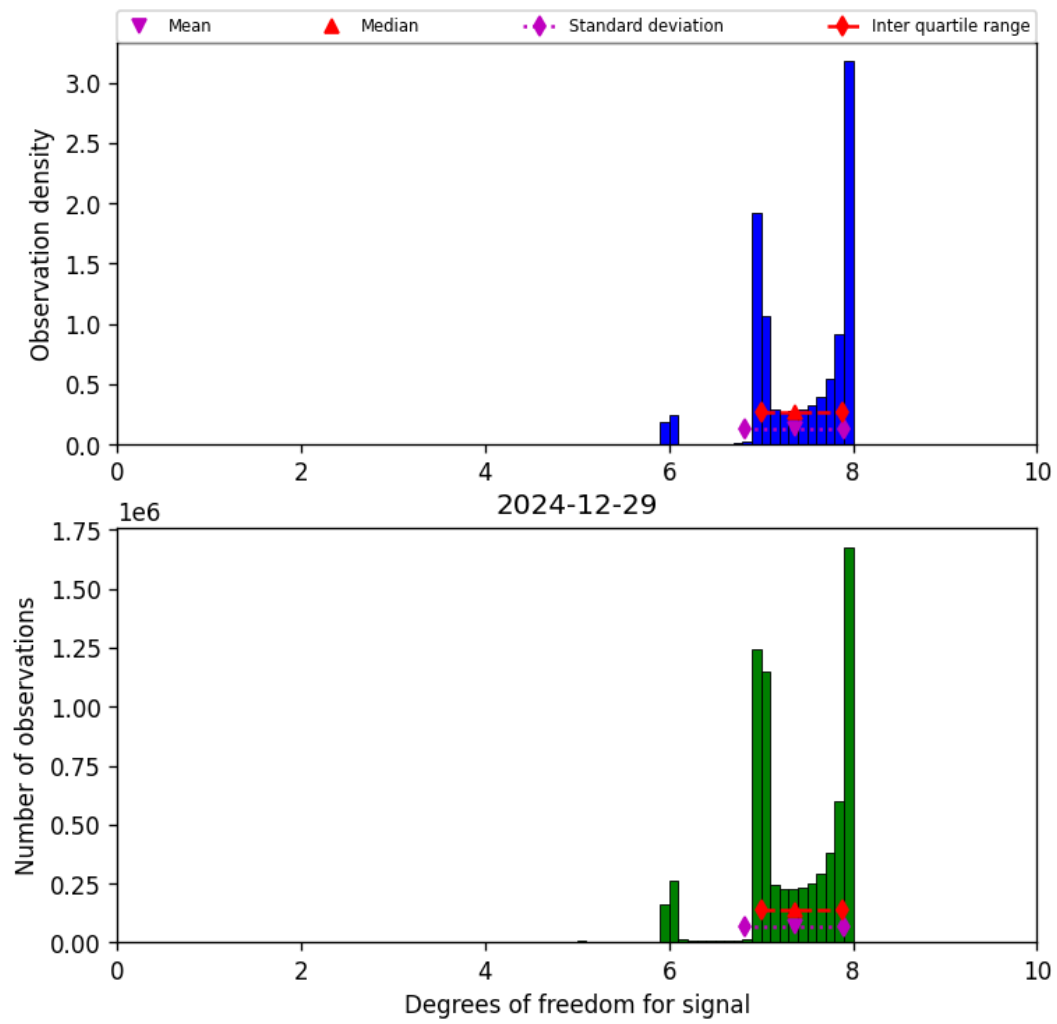
Figure 18: Histogram of “Degrees of freedom for signal” for 2024-12-29 to 2024-12-30
