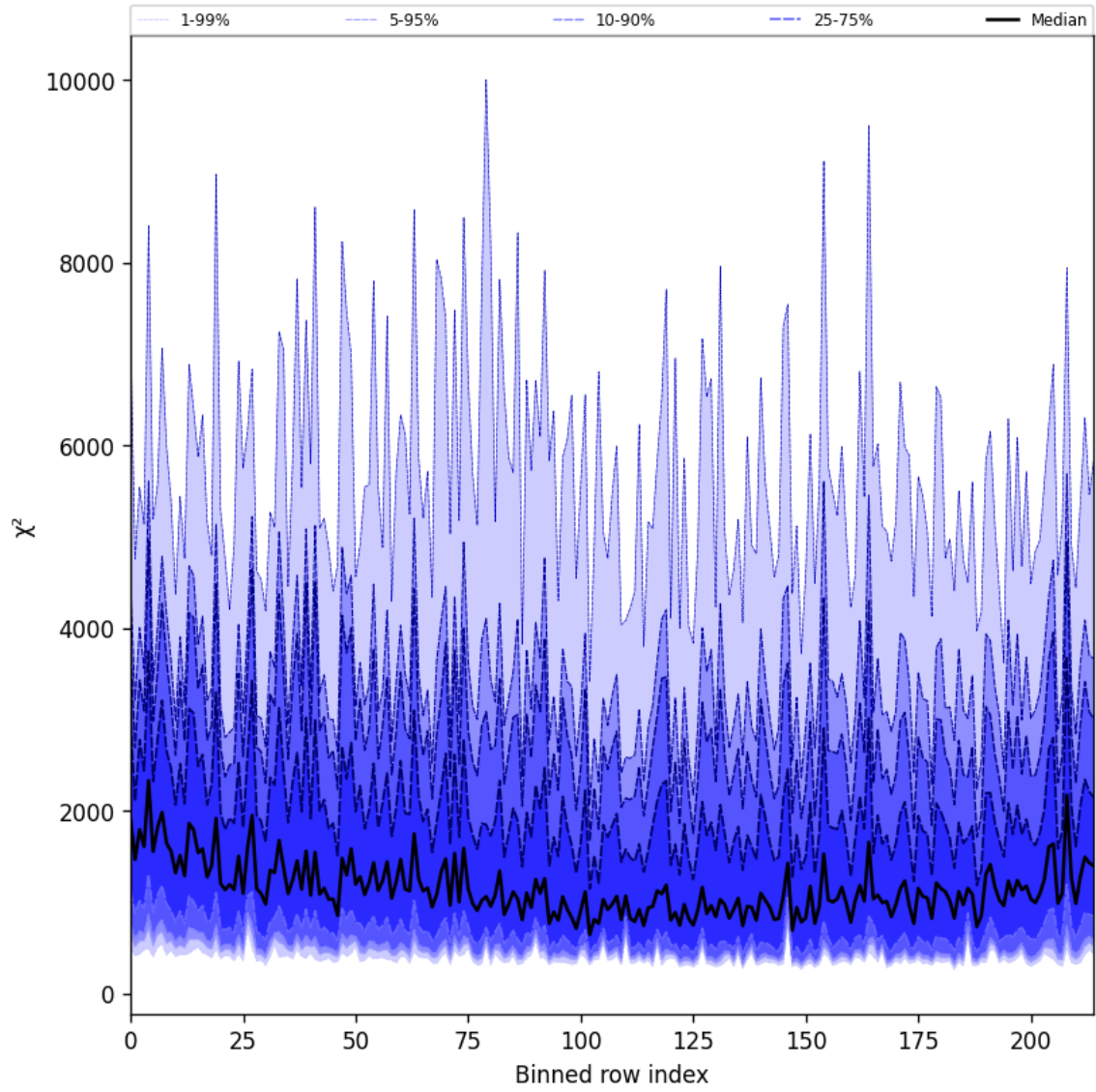
Figure 24: Along track statistics of “ \chi^2 ” for 2024-12-29 to 2024-12-30
