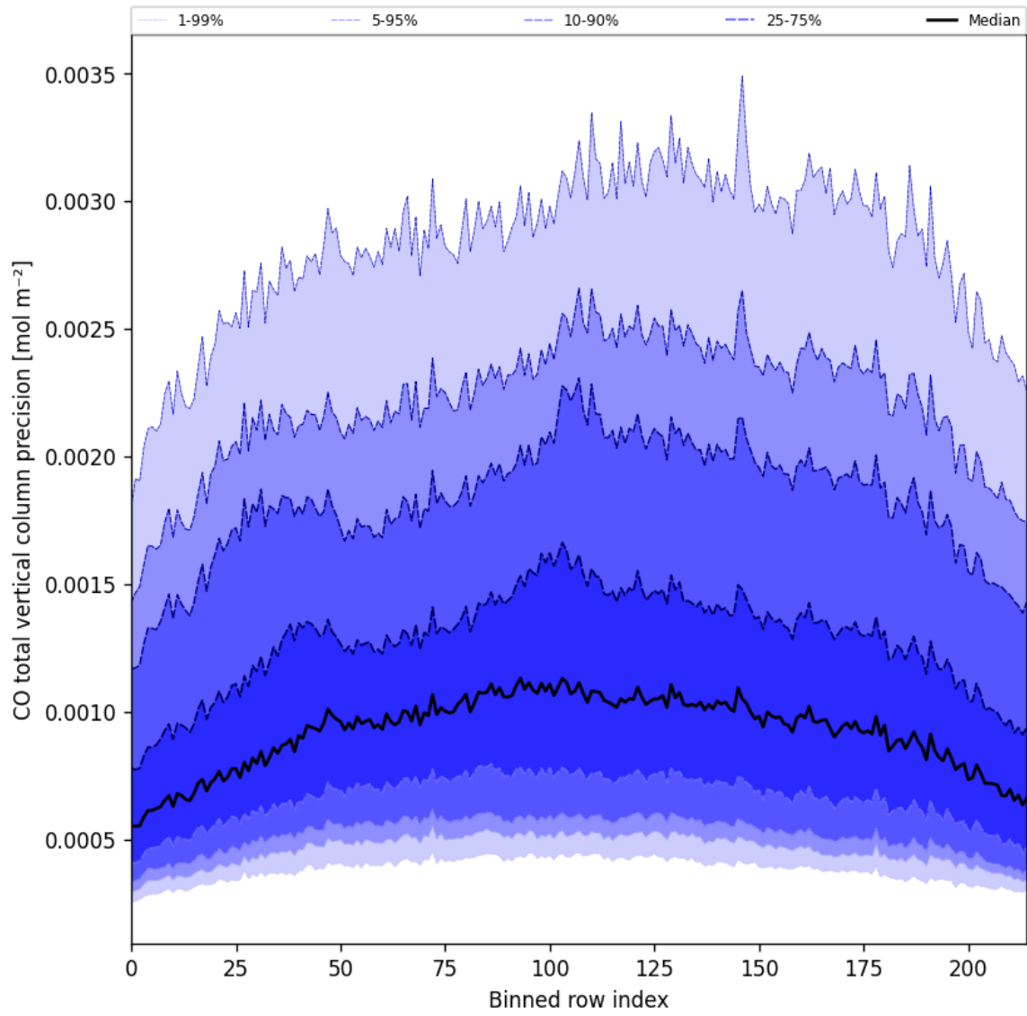
Figure 22: Along track statistics of “CO total vertical column precision” for 2024-12-29 to 2024-12-30
