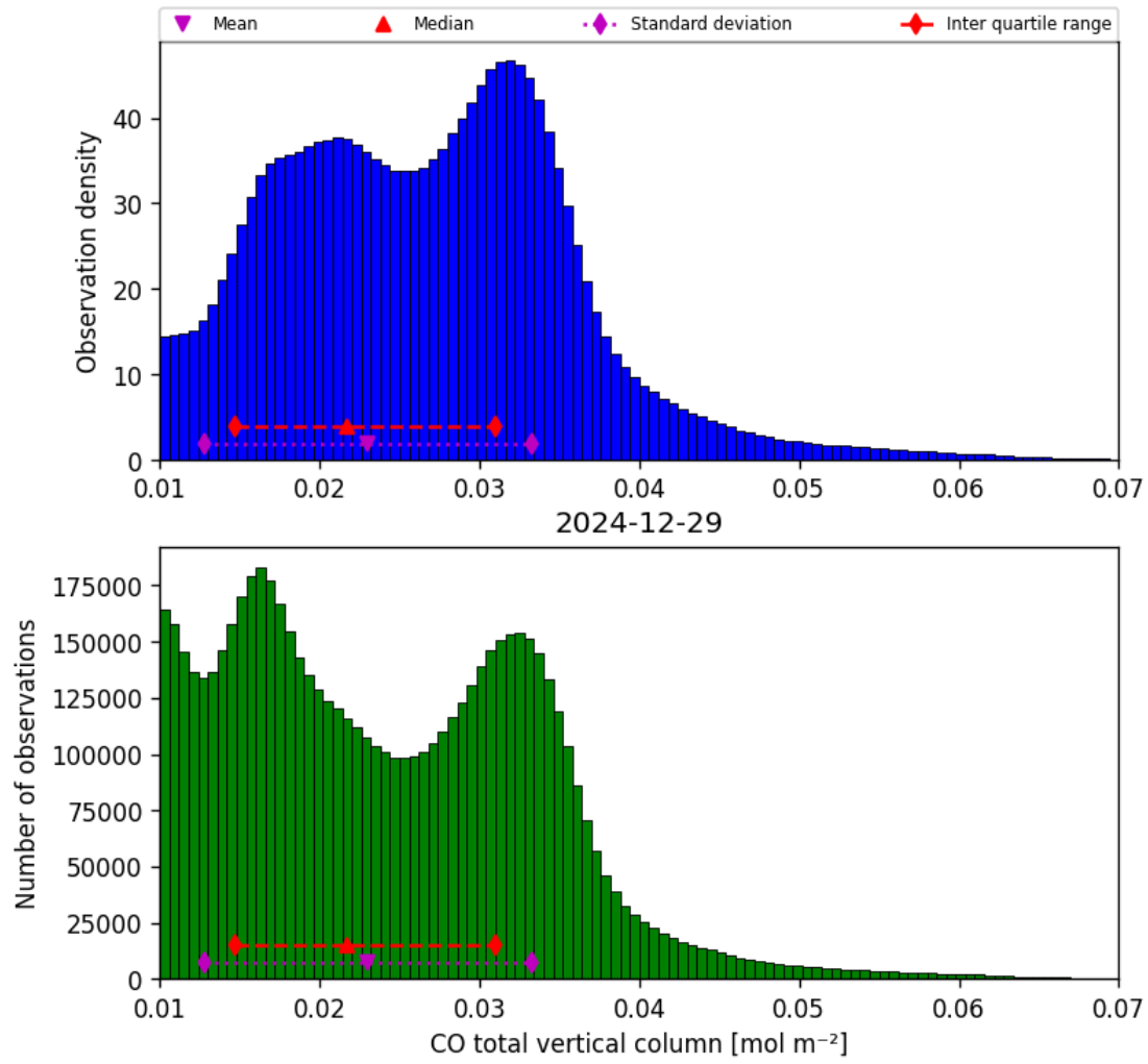
Figure 14: Histogram of “CO total vertical column” for 2024-12-29 to 2024-12-30
