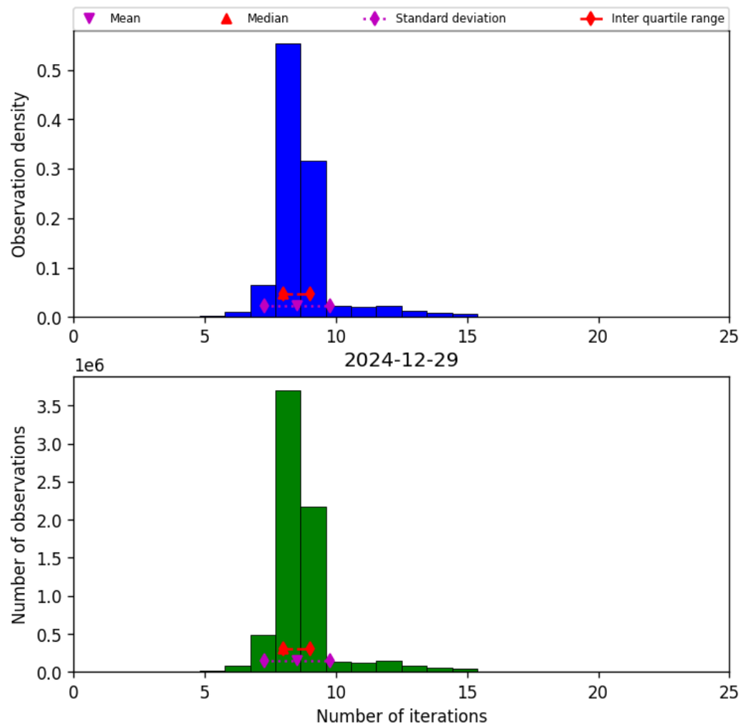
Figure 19: Histogram of “Number of iterations” for 2024-12-29 to 2024-12-30
