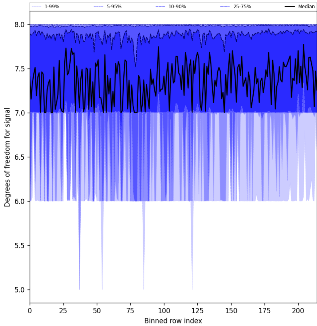
Figure 25: Along track statistics of “Degrees of freedom for signal” for 2024-12-29 to 2024-12-30
