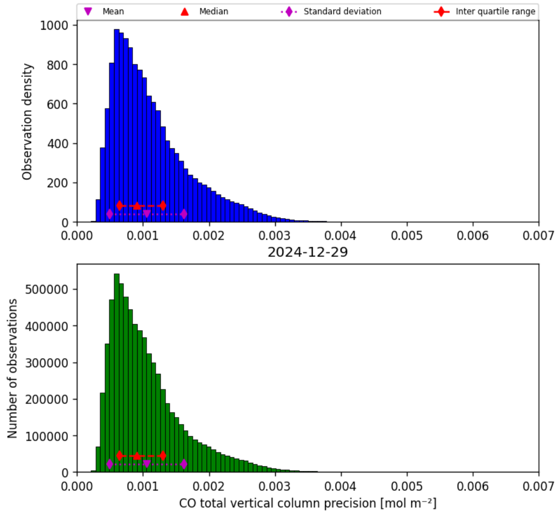
Figure 15: Histogram of “CO total vertical column precision” for 2024-12-29 to 2024-12-30
