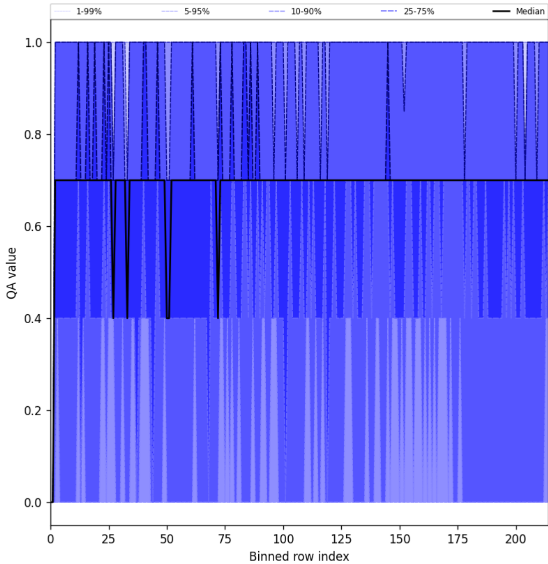
Figure 20: Along track statistics of “QA value” for 2024-12-29 to 2024-12-30
