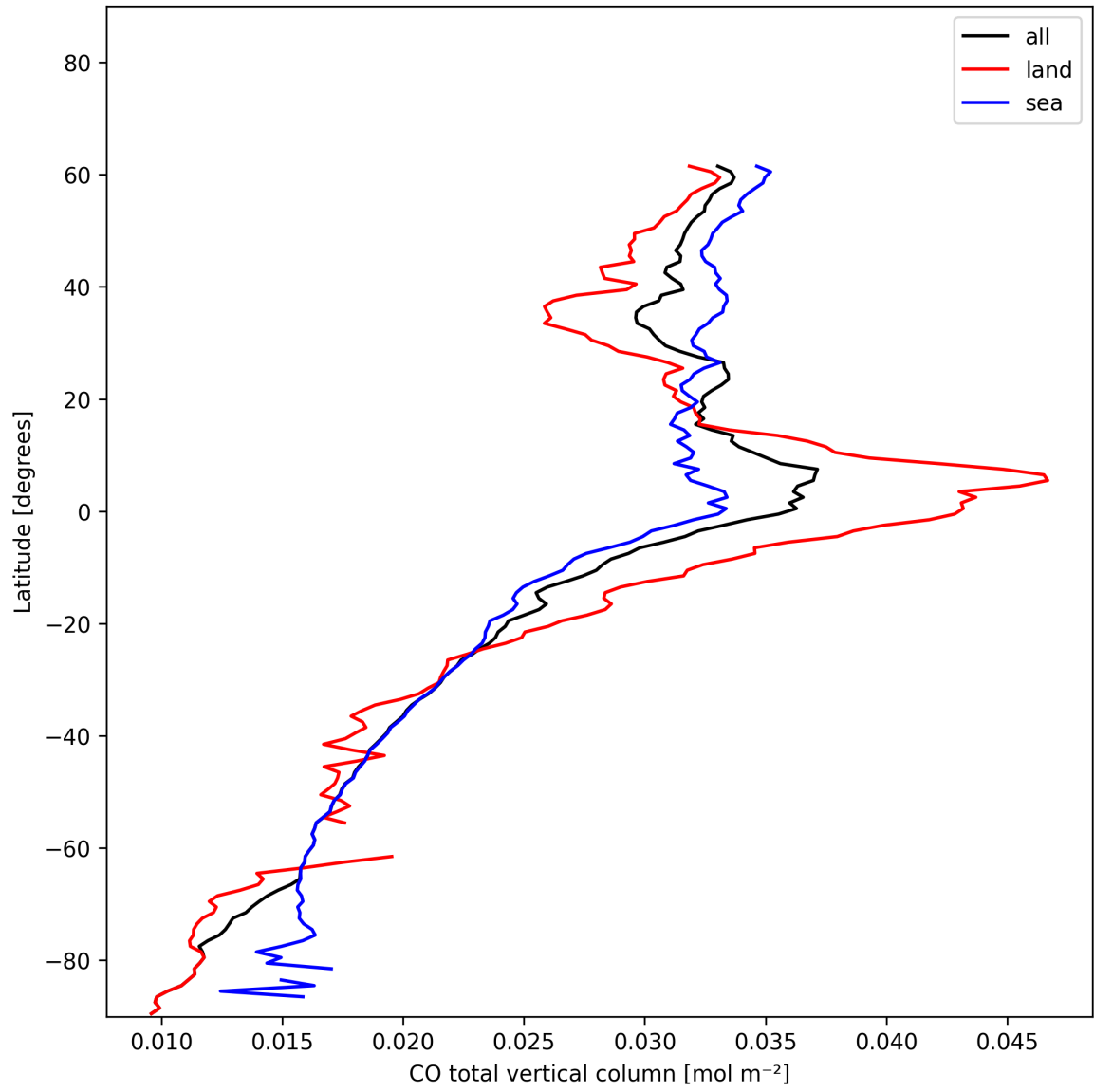
Figure 7: Zonal average of “CO total vertical column” for 2024-12-29 to 2024-12-30.
