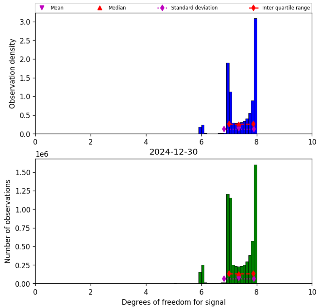
Figure 18: Histogram of “Degrees of freedom for signal” for 2024-12-30 to 2024-12-30
