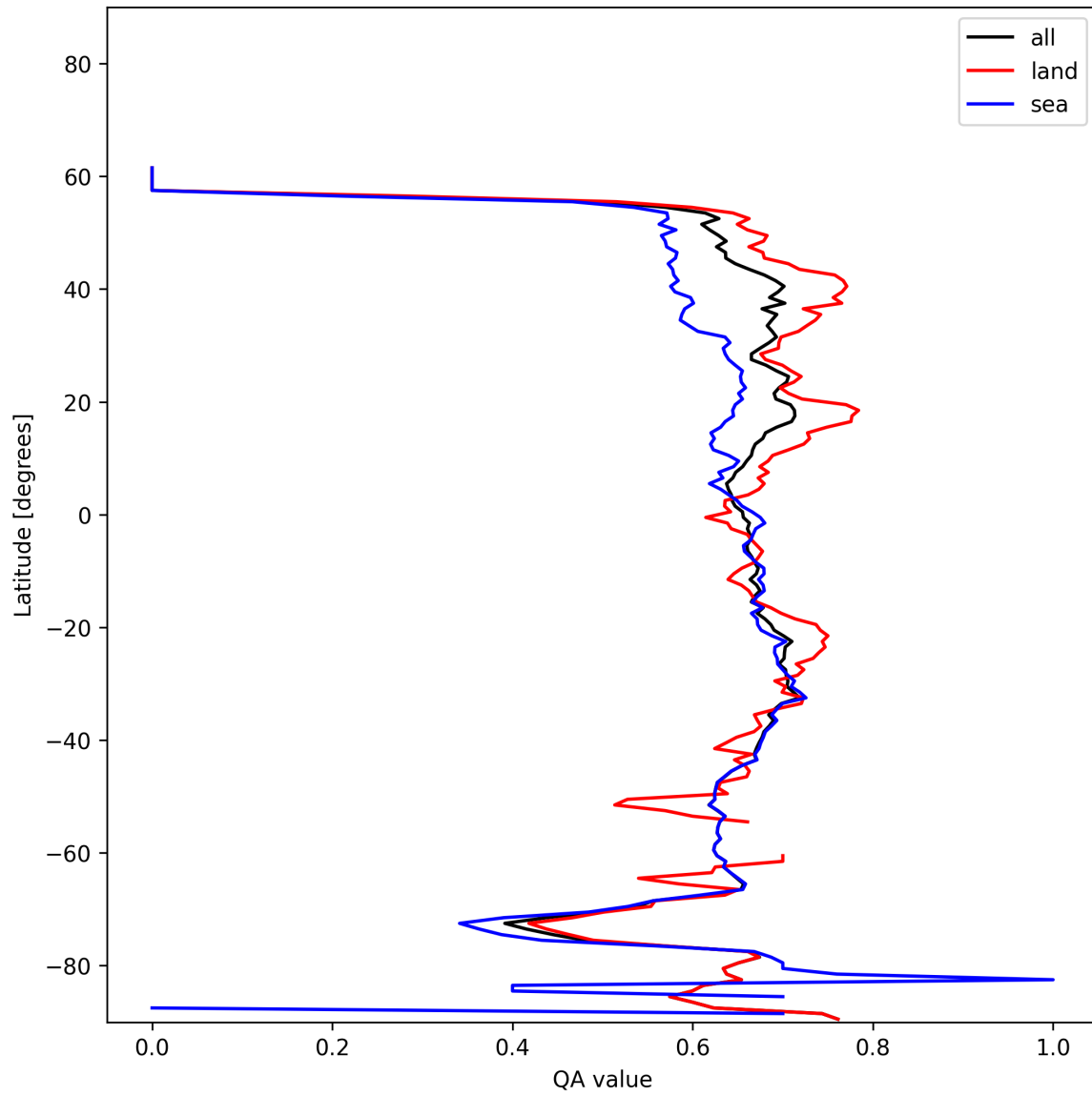
Figure 6: Zonal average of “QA value” for 2024-12-30 to 2024-12-30.
