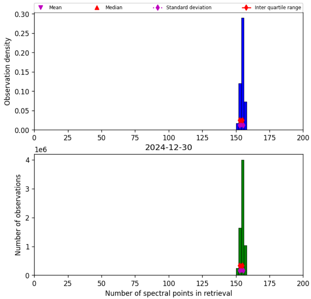
Figure 16: Histogram of “Number of spectral points in retrieval” for 2024-12-30 to 2024-12-30
