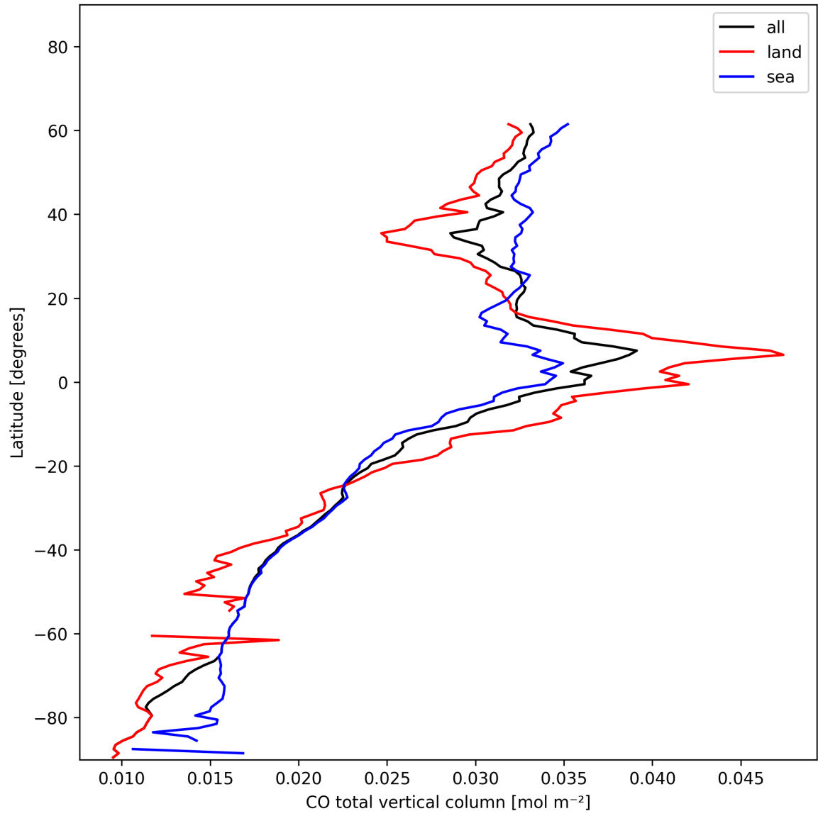
Figure 7: Zonal average of “CO total vertical column” for 2024-12-30 to 2024-12-30.
