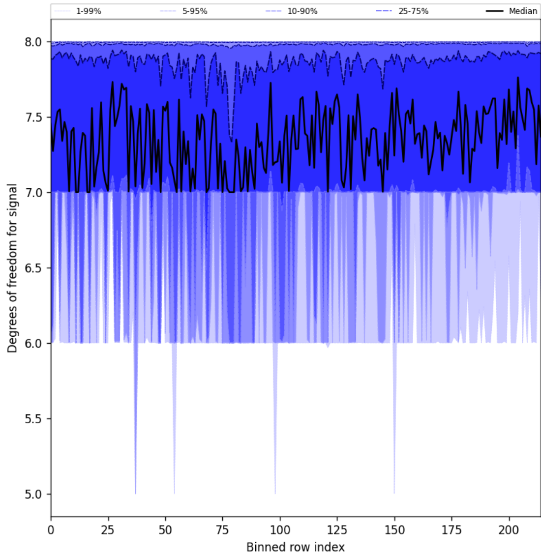
Figure 25: Along track statistics of “Degrees of freedom for signal” for 2024-12-30 to 2024-12-30
