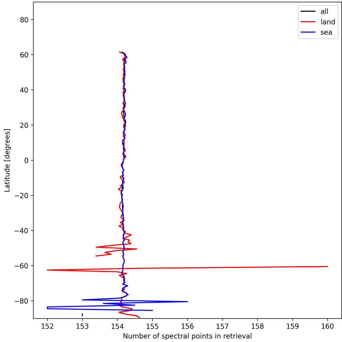
Figure 9: Zonal average of “Number of spectral points in retrieval” for 2024-12-30 to 2024-12-30.
