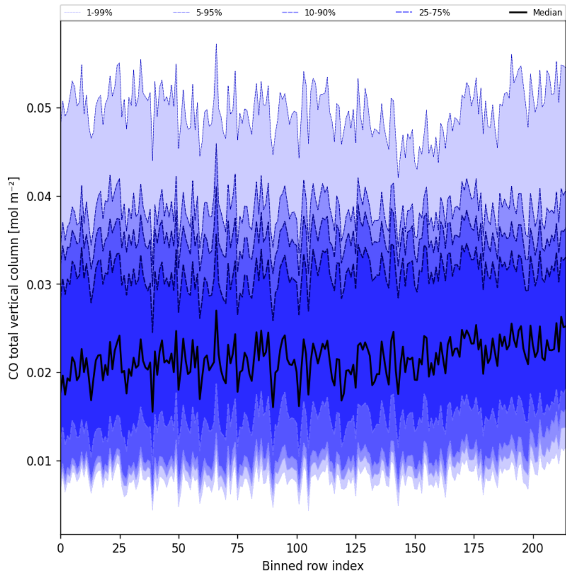
Figure 21: Along track statistics of “CO total vertical column” for 2024-12-30 to 2024-12-30
