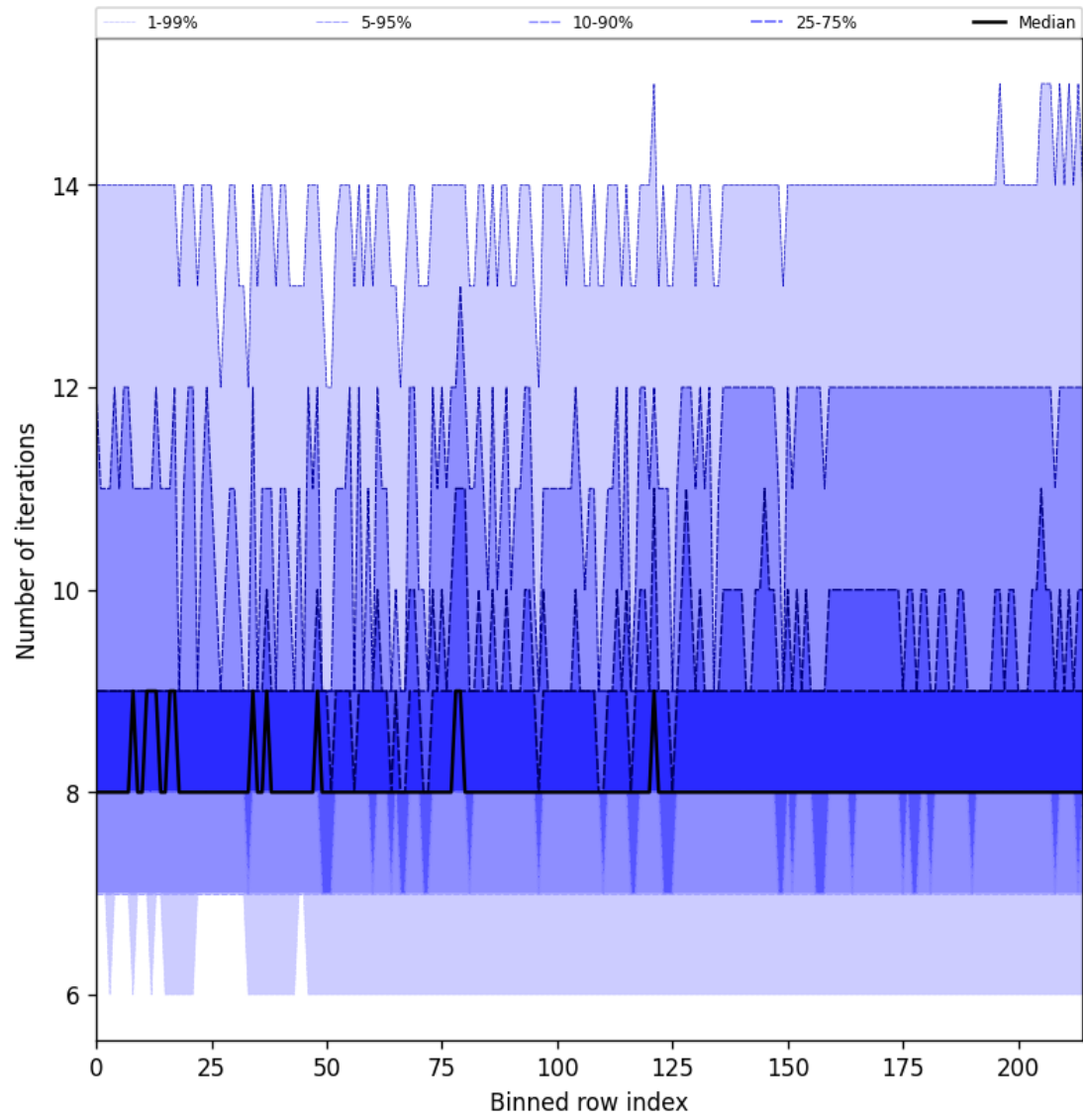
Figure 26: Along track statistics of “Number of iterations” for 2024-12-30 to 2024-12-30
