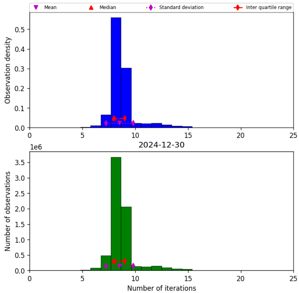
Figure 19: Histogram of “Number of iterations” for 2024-12-30 to 2024-12-30
