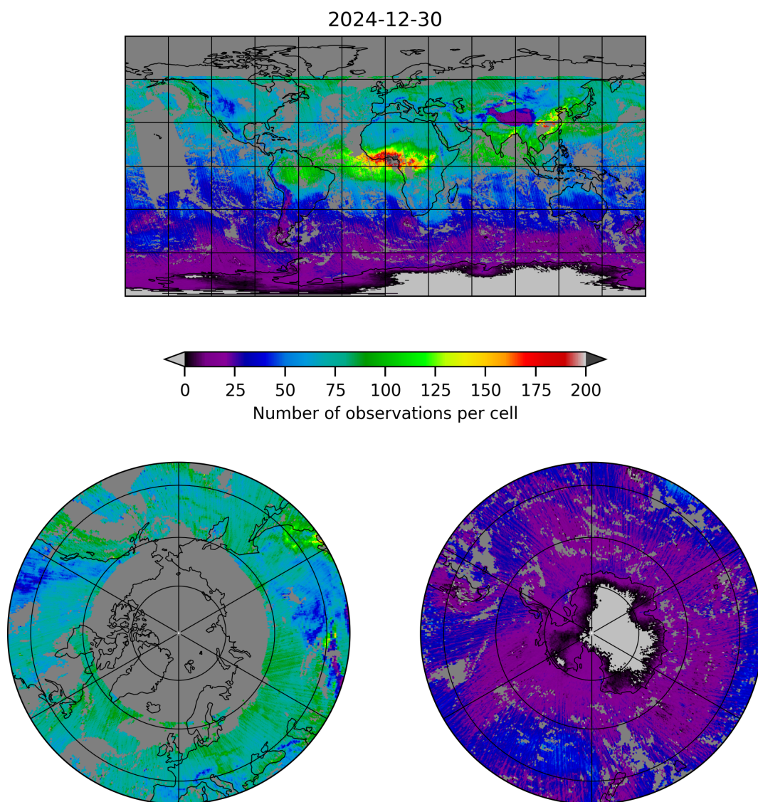
Figure 5: Map of the number of observations for 2024-12-30 to 2024-12-30
