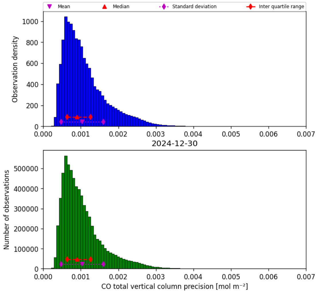
Figure 15: Histogram of “CO total vertical column precision” for 2024-12-30 to 2024-12-30
