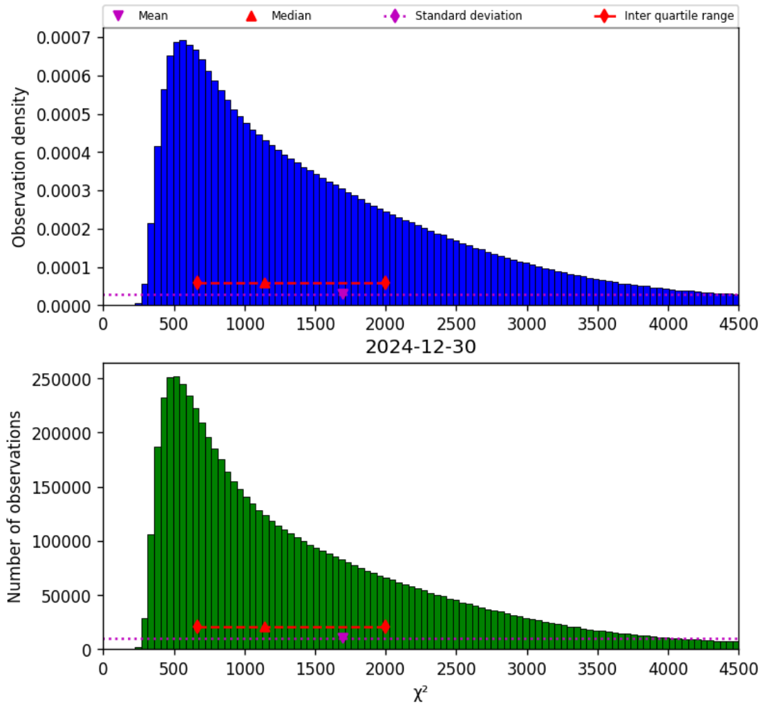
Figure 17: Histogram of “ \chi^2 ” for 2024-12-30 to 2024-12-30
