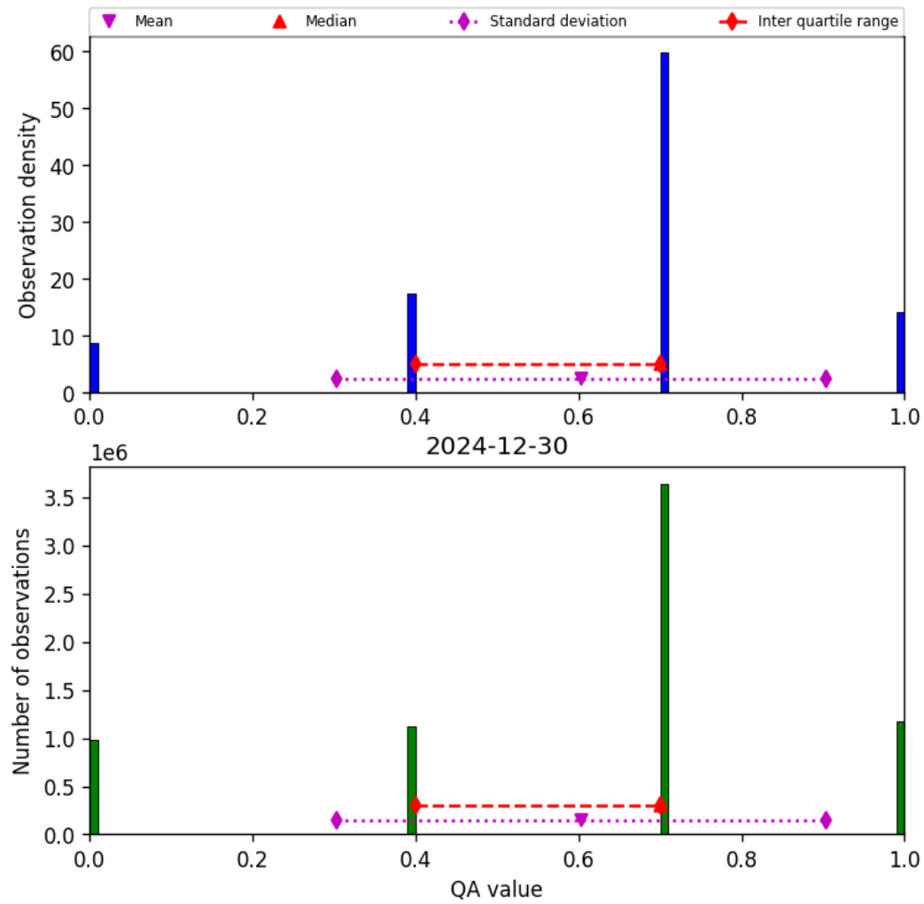
Figure 13: Histogram of “QA value” for 2024-12-30 to 2024-12-30
