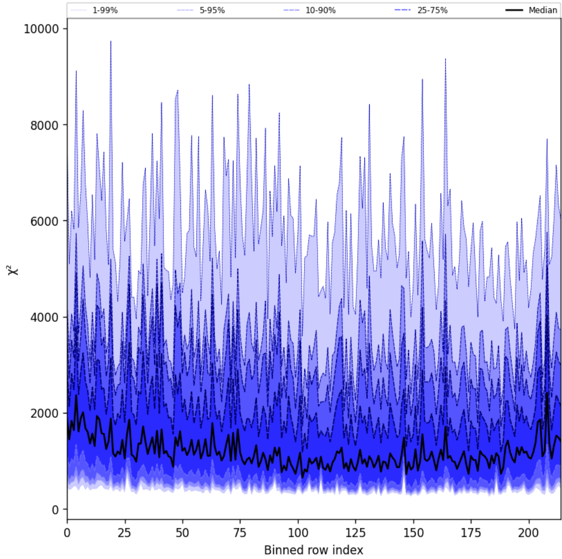
Figure 24: Along track statistics of “ \chi^2 ” for 2024-12-30 to 2024-12-30
