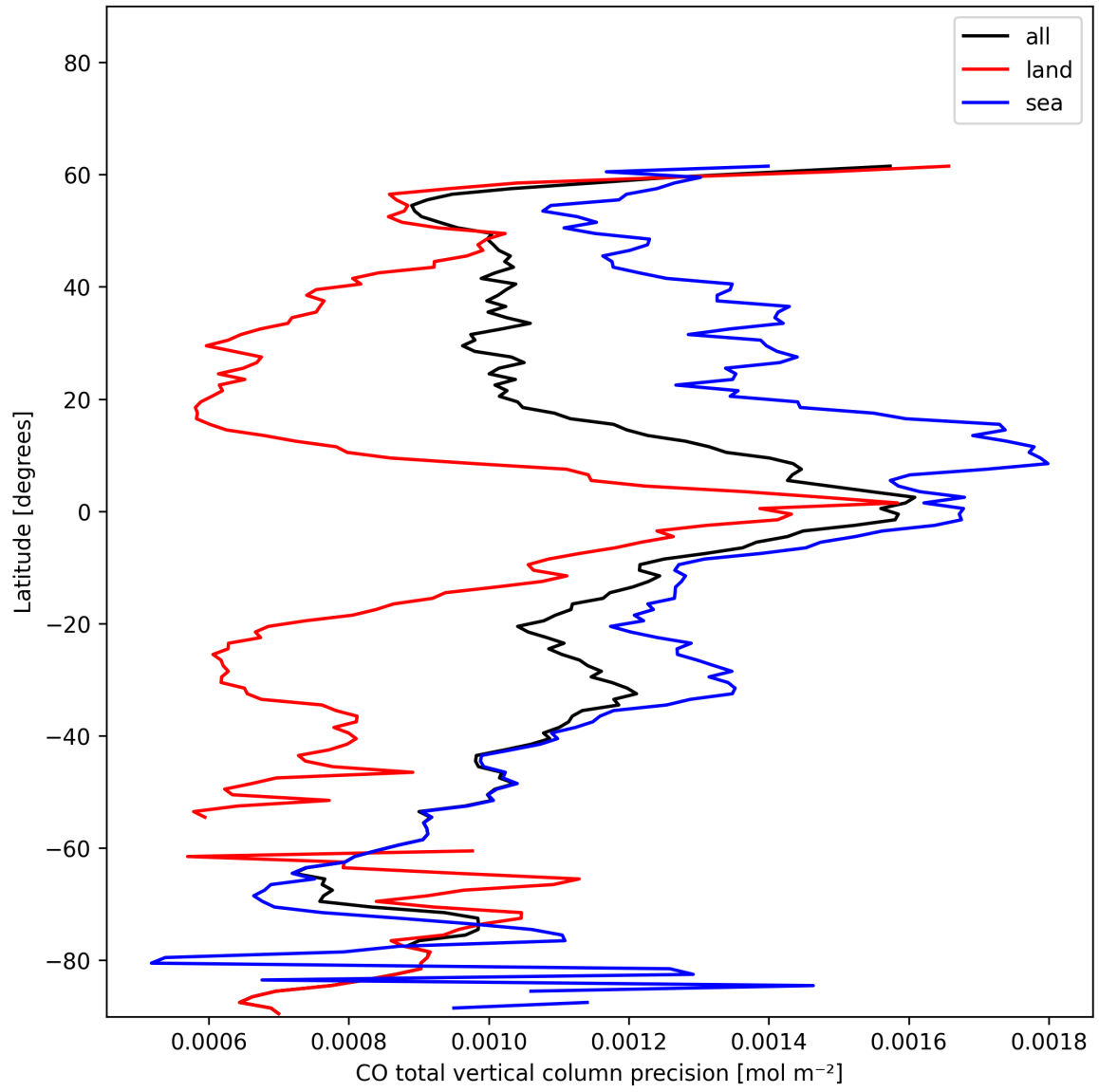
Figure 8: Zonal average of "CO total vertical column precision" for 2024-12-30 to 2024-12-30.
