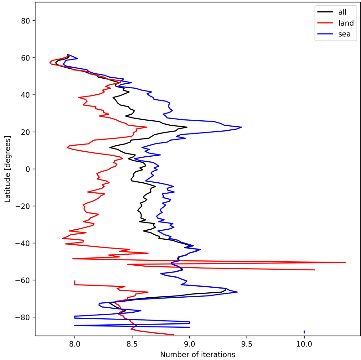
Figure 12: Zonal average of “Number of iterations” for 2024-12-30 to 2024-12-30.
