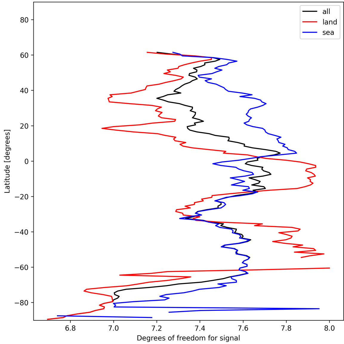
Figure 11: Zonal average of “Degrees of freedom for signal” for 2024-12-30 to 2024-12-30.
