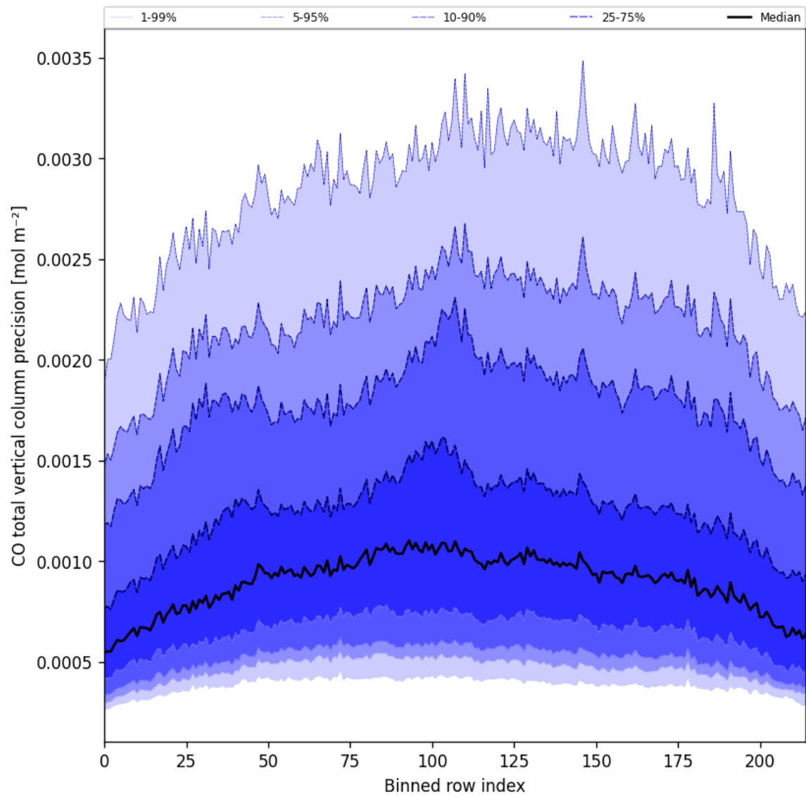
Figure 22: Along track statistics of “CO total vertical column precision” for 2024-12-30 to 2024-12-30
