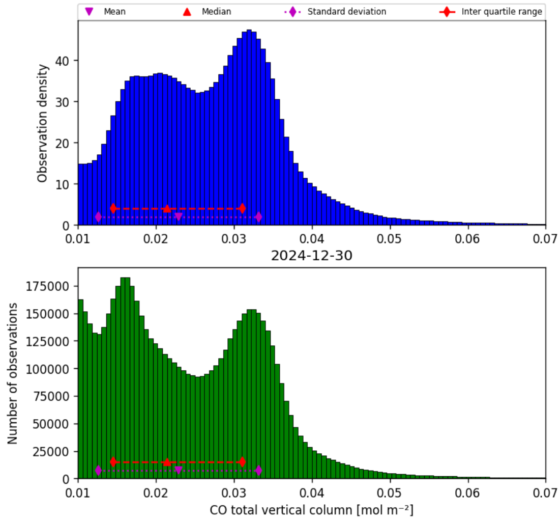
Figure 14: Histogram of “CO total vertical column” for 2024-12-30 to 2024-12-30
