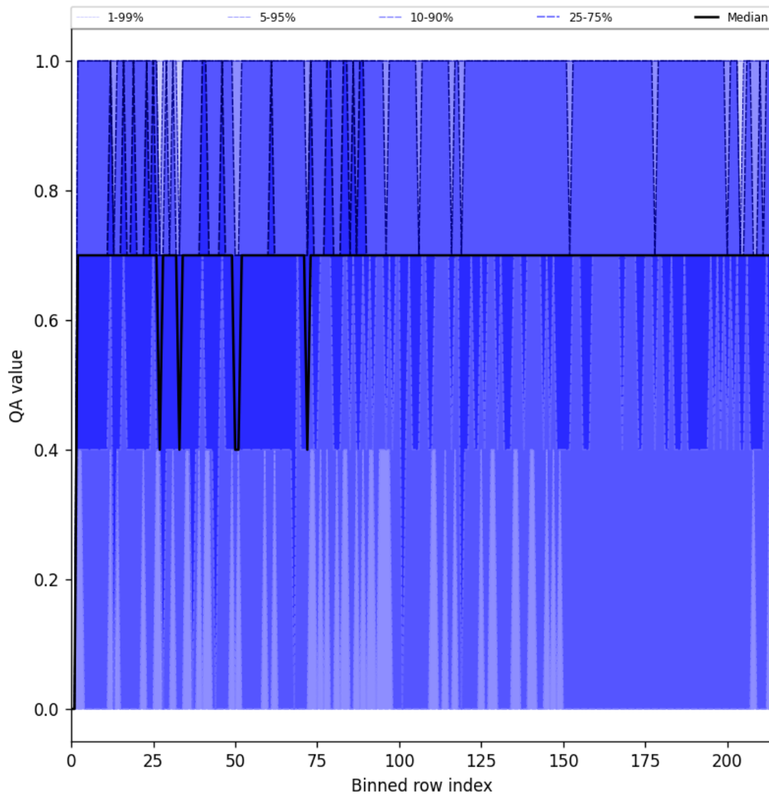
Figure 20: Along track statistics of “QA value” for 2024-12-30 to 2024-12-30
