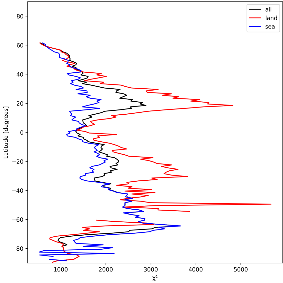
Figure 10: Zonal average of “ \chi^2 ” for 2024-12-30 to 2024-12-30.
