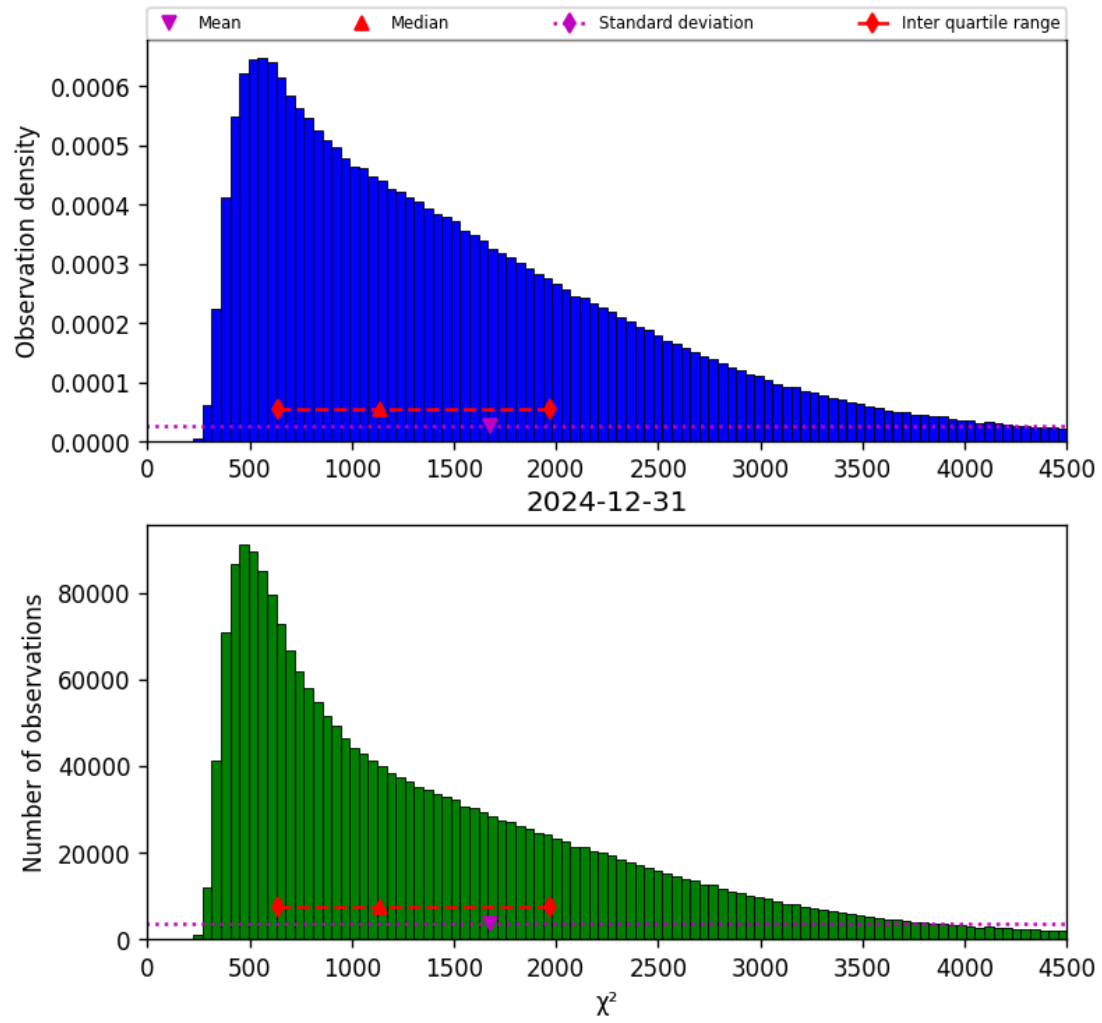
Figure 17: Histogram of " \chi^2 " for 2024-12-31 to 2024-12-31
