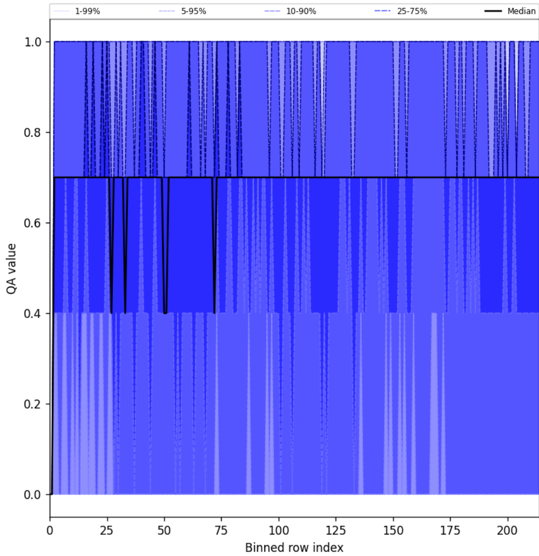
Figure 20: Along track statistics of “QA value” for 2024-12-31 to 2024-12-31
