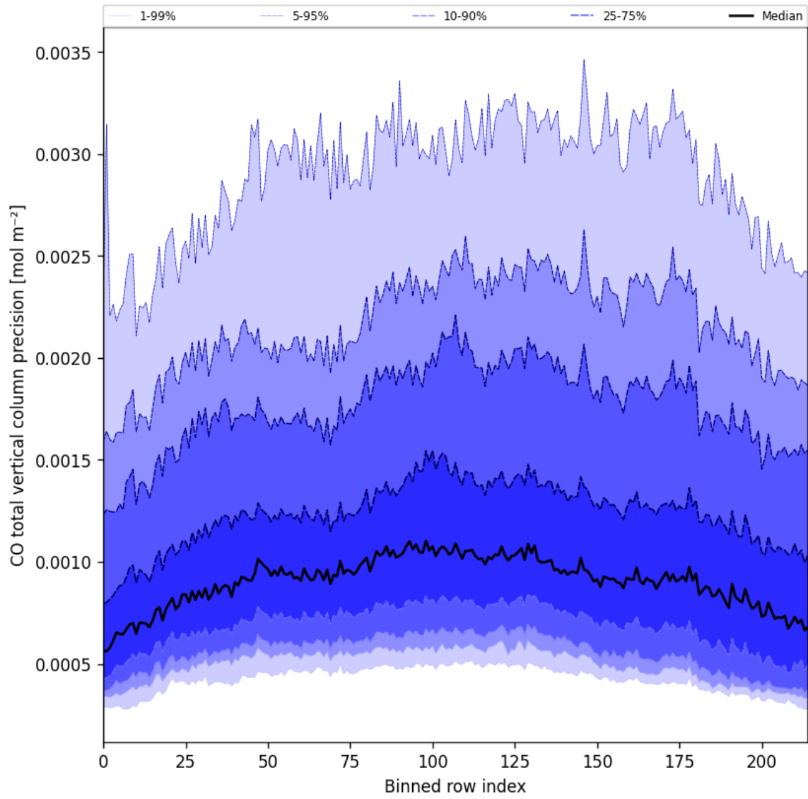
Figure 22: Along track statistics of “CO total vertical column precision” for 2024-12-31 to 2024-12-31
