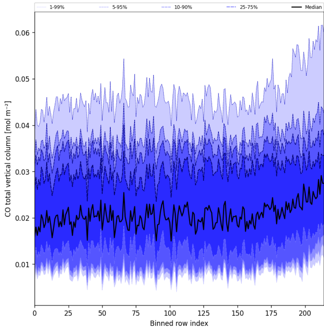
Figure 21: Along track statistics of “CO total vertical column” for 2024-12-31 to 2024-12-31
