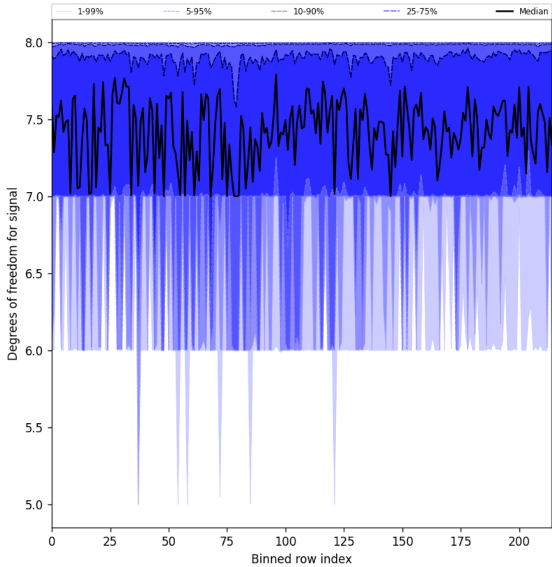
Figure 25: Along track statistics of “Degrees of freedom for signal” for 2024-12-31 to 2024-12-31
