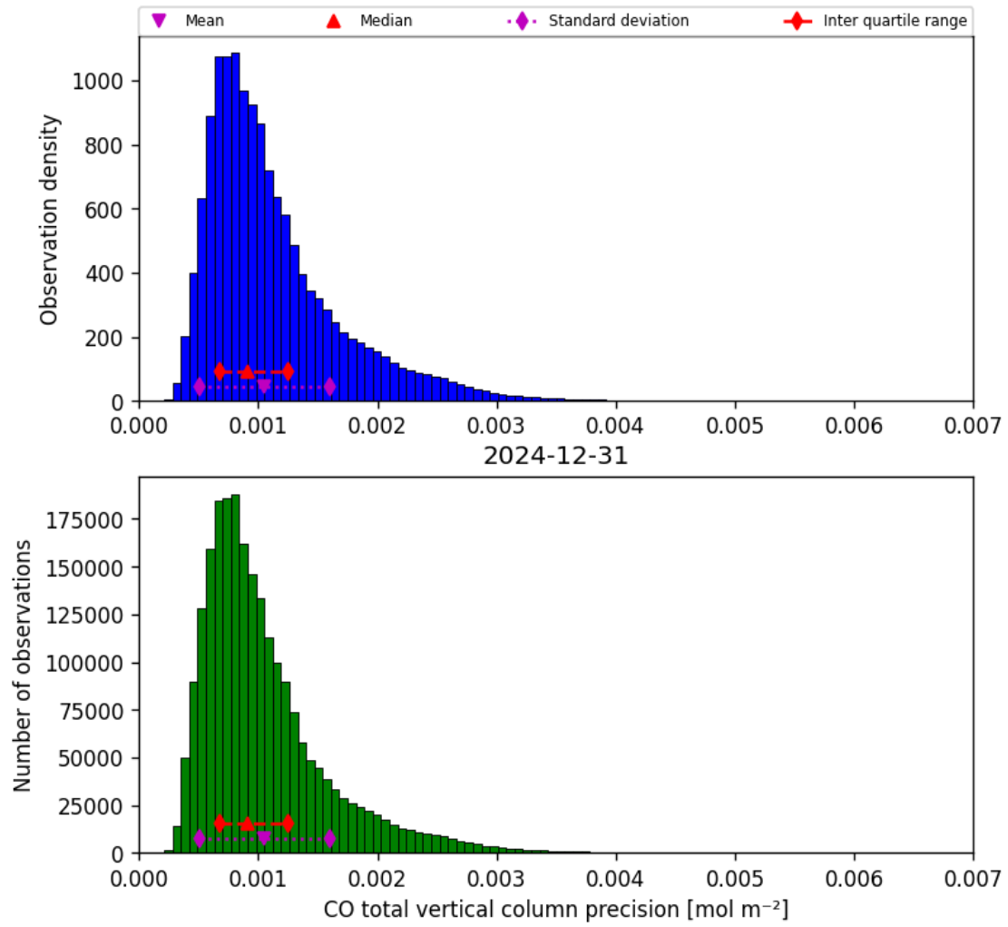
Figure 15: Histogram of “CO total vertical column precision” for 2024-12-31 to 2024-12-31
