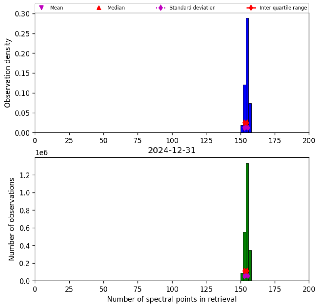
Figure 16: Histogram of “Number of spectral points in retrieval” for 2024-12-31 to 2024-12-31
