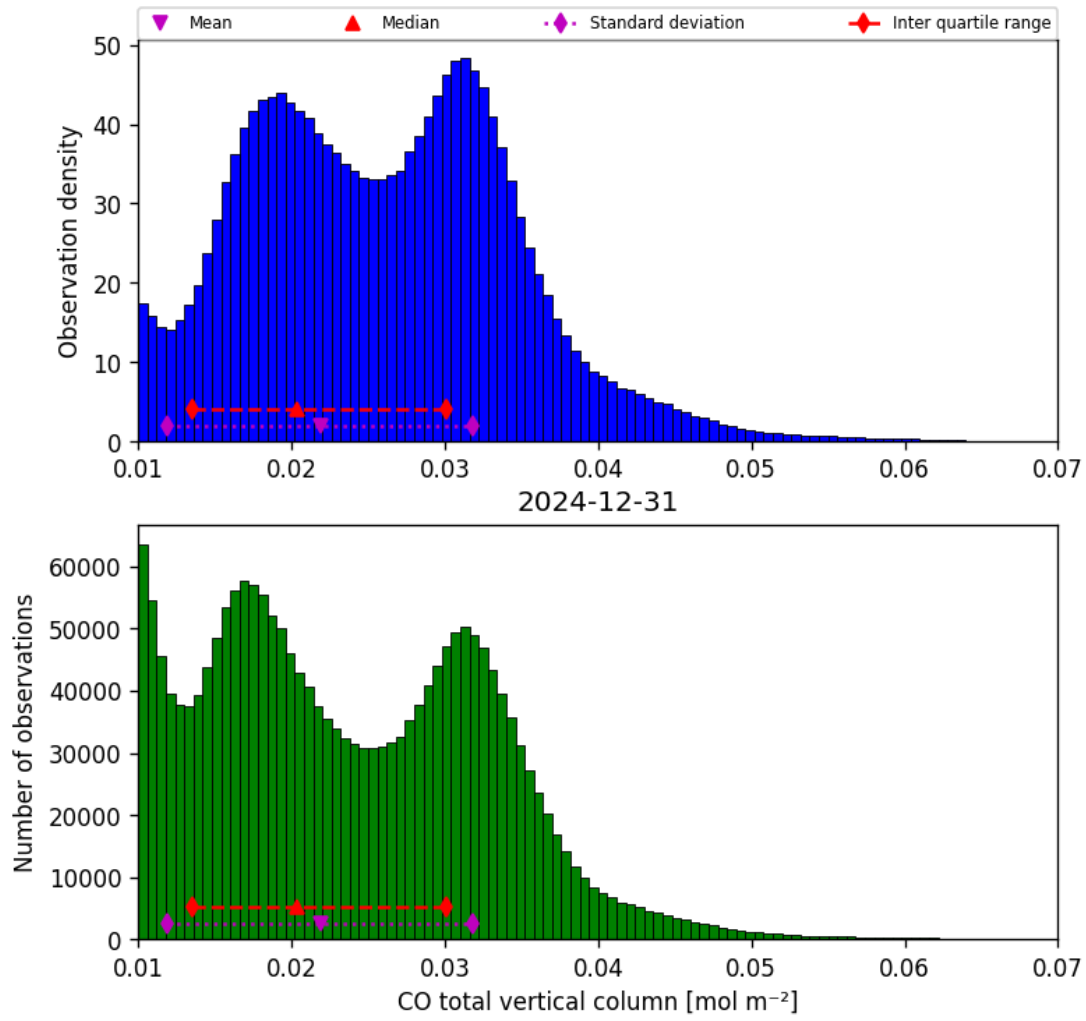
Figure 14: Histogram of “CO total vertical column” for 2024-12-31 to 2024-12-31
