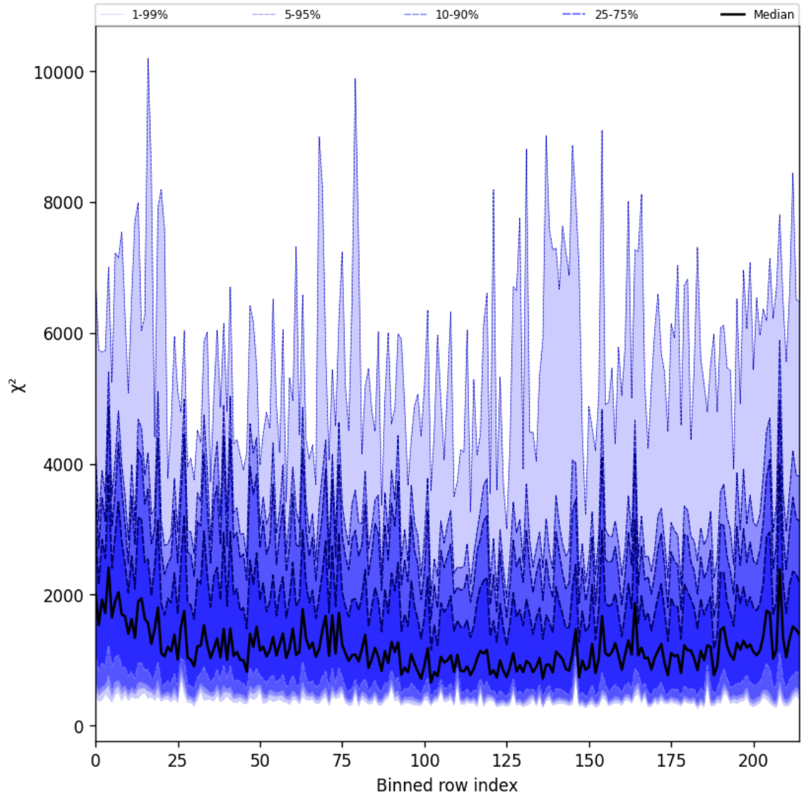
Figure 24: Along track statistics of “ \chi^2 ” for 2024-12-31 to 2024-12-31
