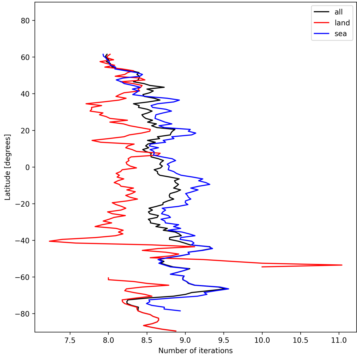
Figure 12: Zonal average of “Number of iterations” for 2024-12-31 to 2024-12-31.
