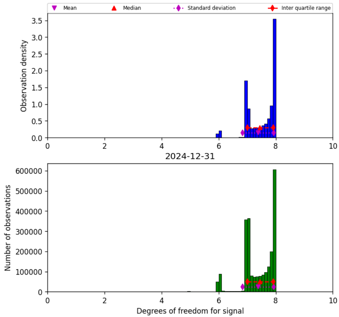
Figure 18: Histogram of “Degrees of freedom for signal” for 2024-12-31 to 2024-12-31
