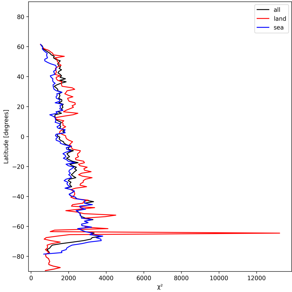
Figure 10: Zonal average of “ \chi^2 ” for 2024-12-31 to 2024-12-31.
