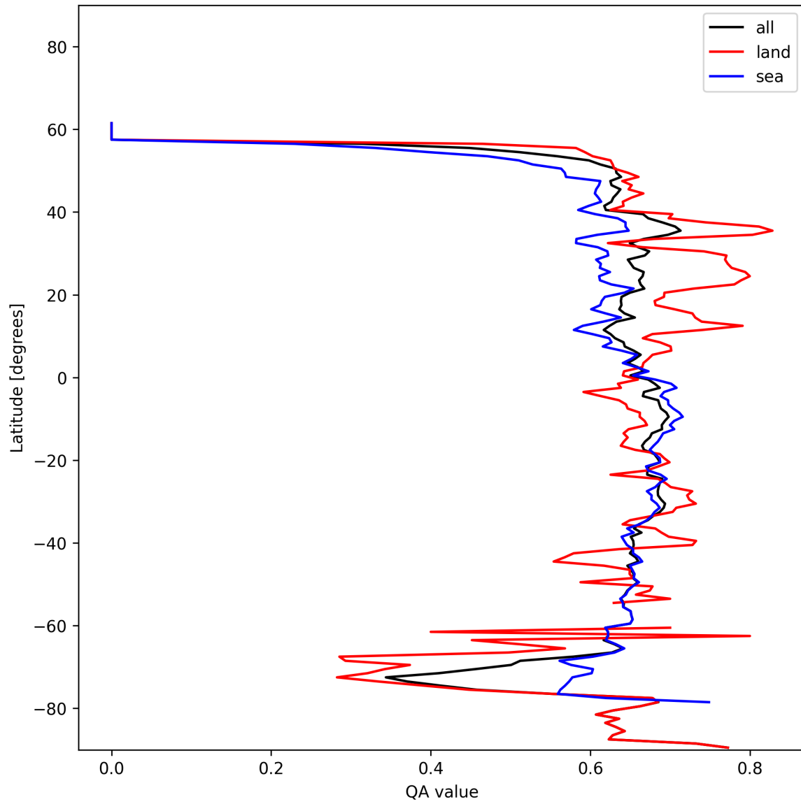
Figure 6: Zonal average of “QA value” for 2024-12-31 to 2024-12-31.
