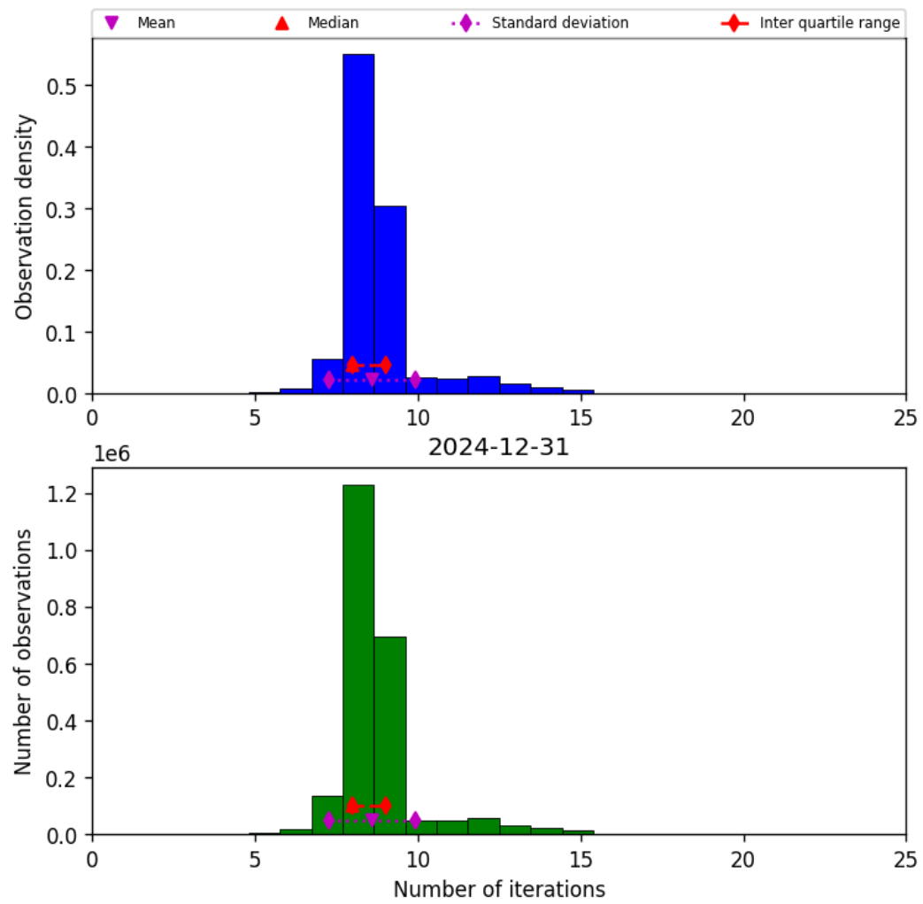
Figure 19: Histogram of “Number of iterations” for 2024-12-31 to 2024-12-31
