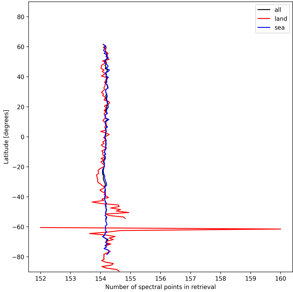
Figure 9: Zonal average of “Number of spectral points in retrieval” for 2024-12-31 to 2024-12-31.
