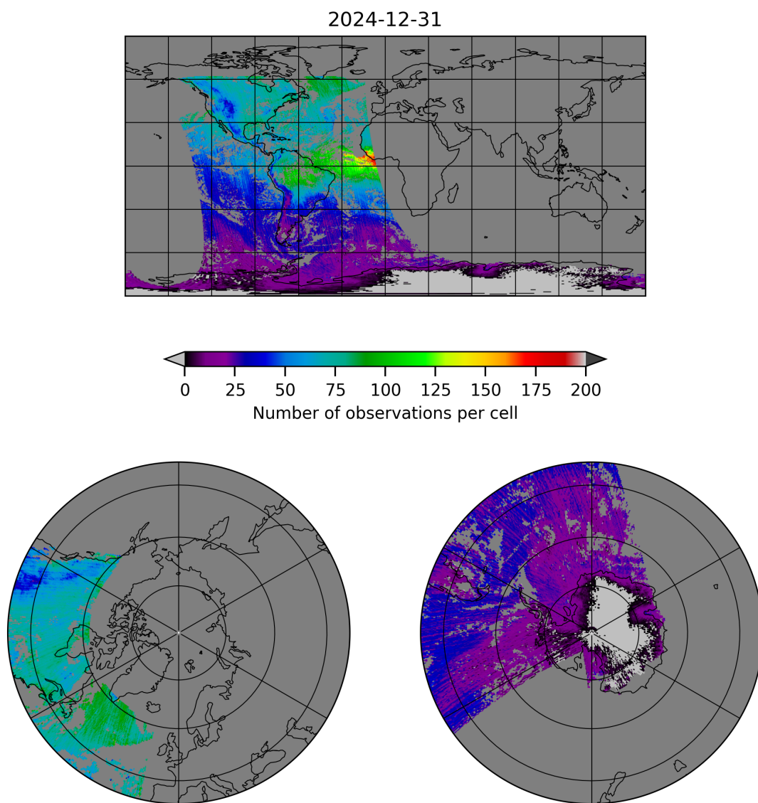
Figure 5: Map of the number of observations for 2024-12-31 to 2024-12-31
