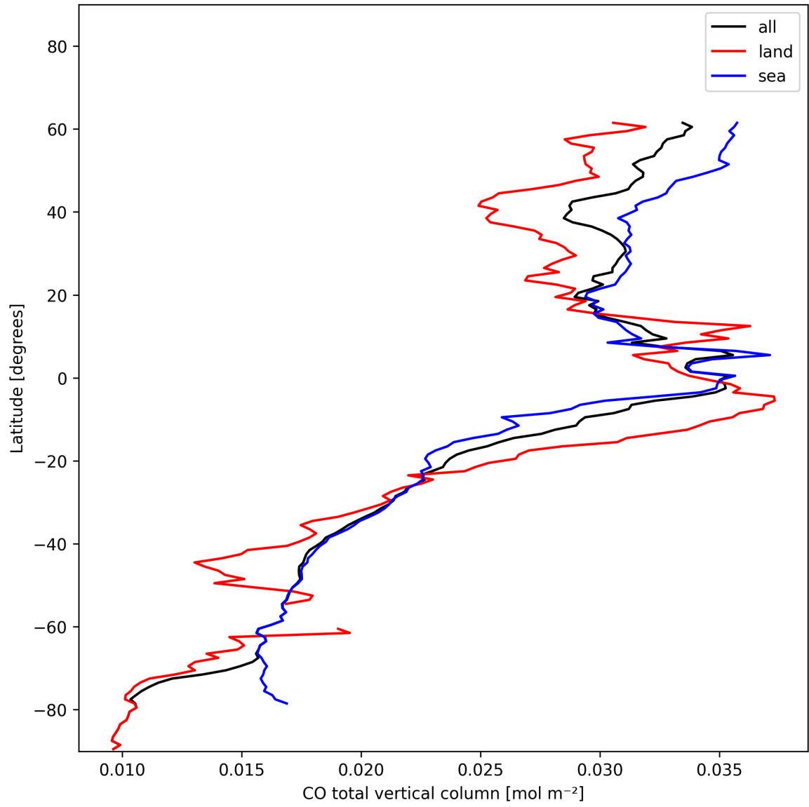
Figure 7: Zonal average of “CO total vertical column” for 2024-12-31 to 2024-12-31.
