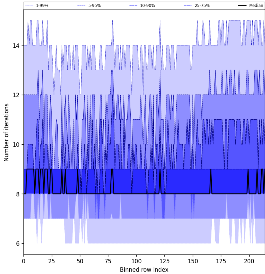
Figure 26: Along track statistics of “Number of iterations” for 2024-12-31 to 2024-12-31
