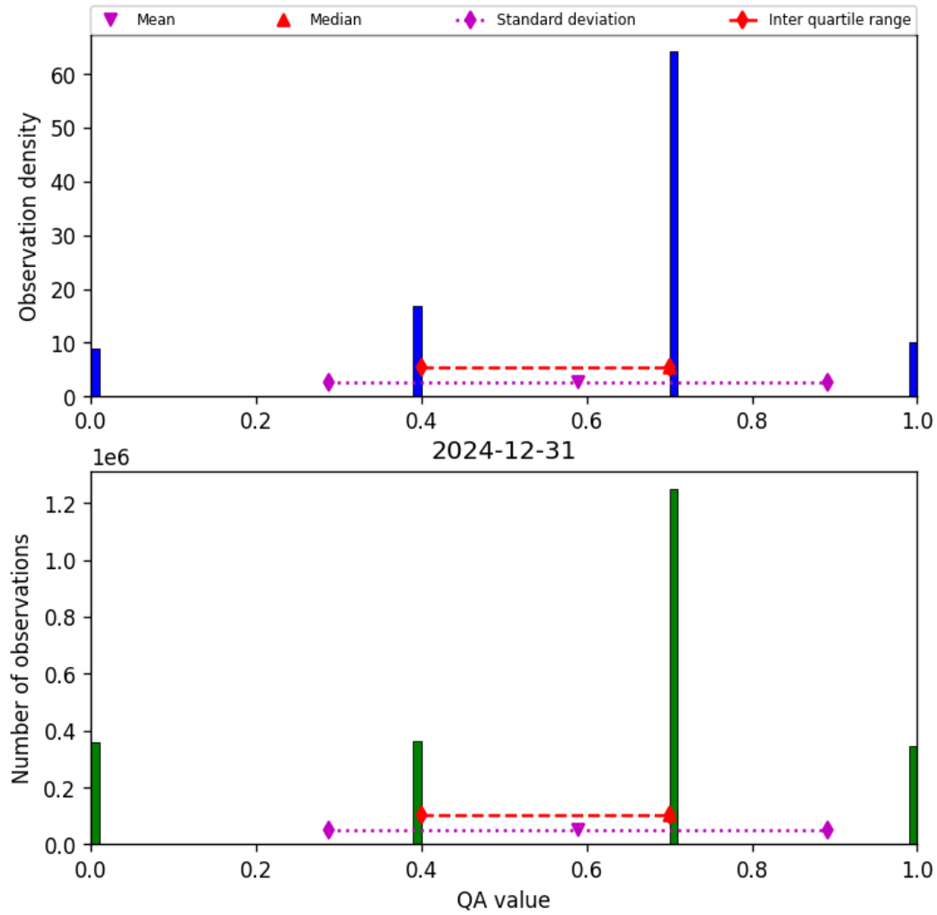
Figure 13: Histogram of “QA value” for 2024-12-31 to 2024-12-31
