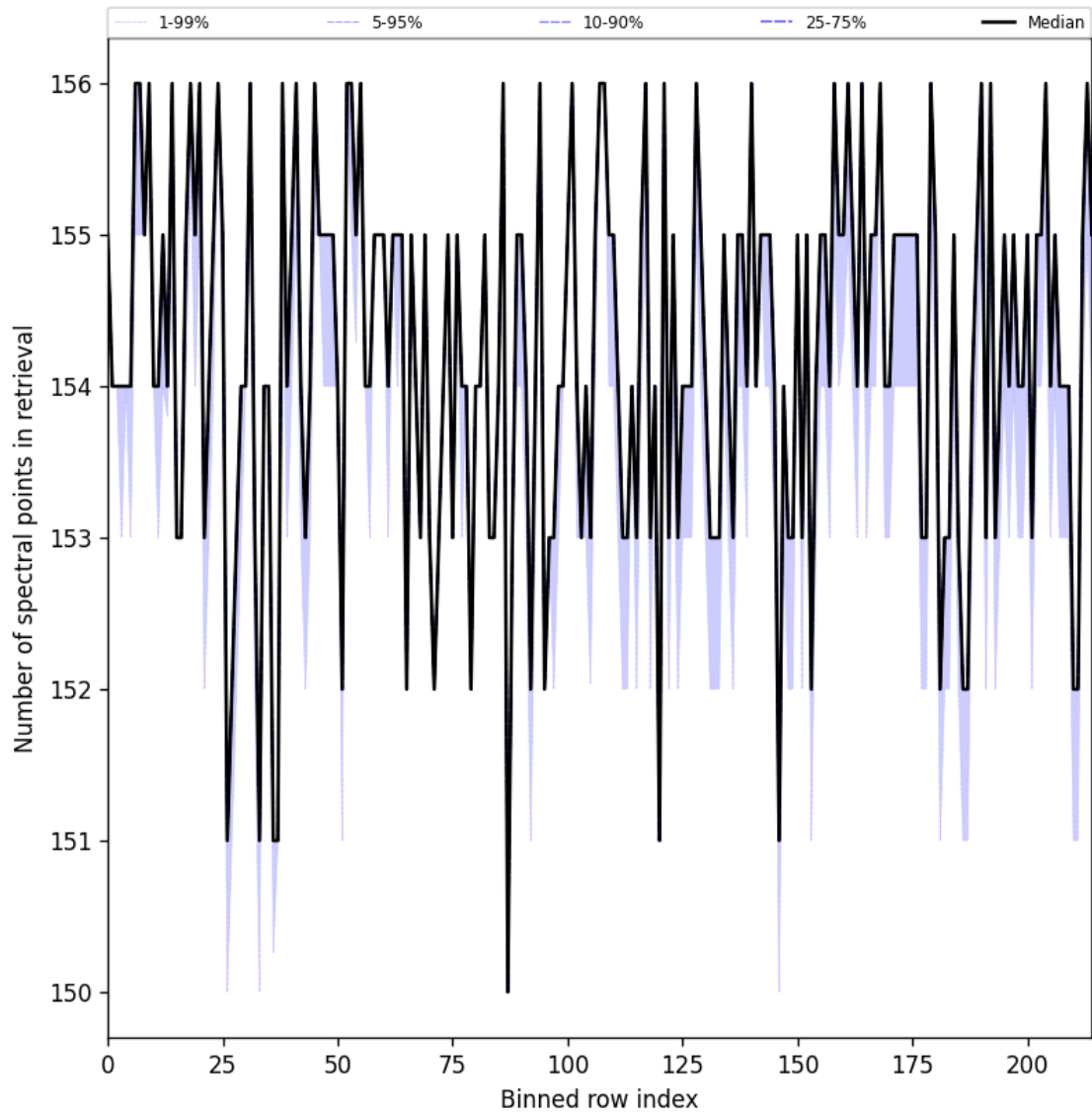
Figure 23: Along track statistics of “Number of spectral points in retrieval” for 2024-12-31 to 2024-12-31
