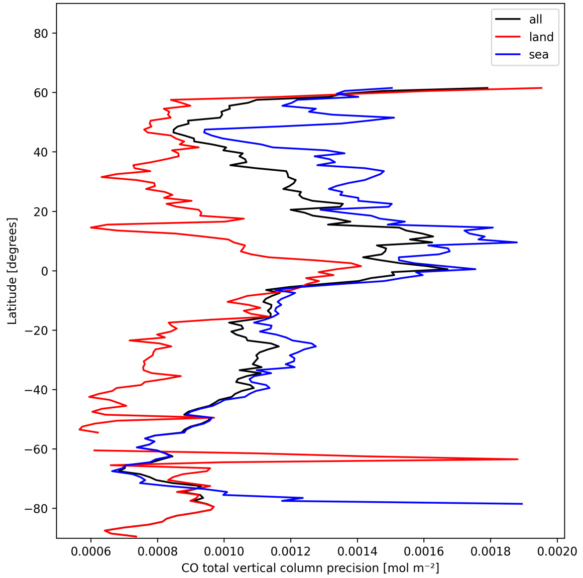
Figure 8: Zonal average of “CO total vertical column precision” for 2024-12-31 to 2024-12-31.
