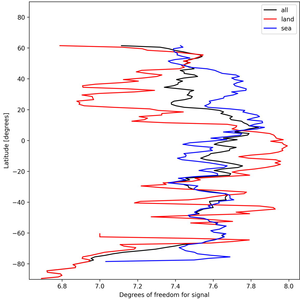
Figure 11: Zonal average of “Degrees of freedom for signal” for 2024-12-31 to 2024-12-31.
