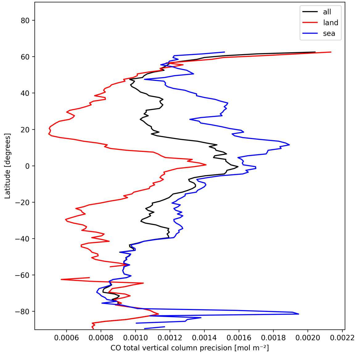
Figure 8: Zonal average of “CO total vertical column precision” for 2025-01-02 to 2025-01-03.
