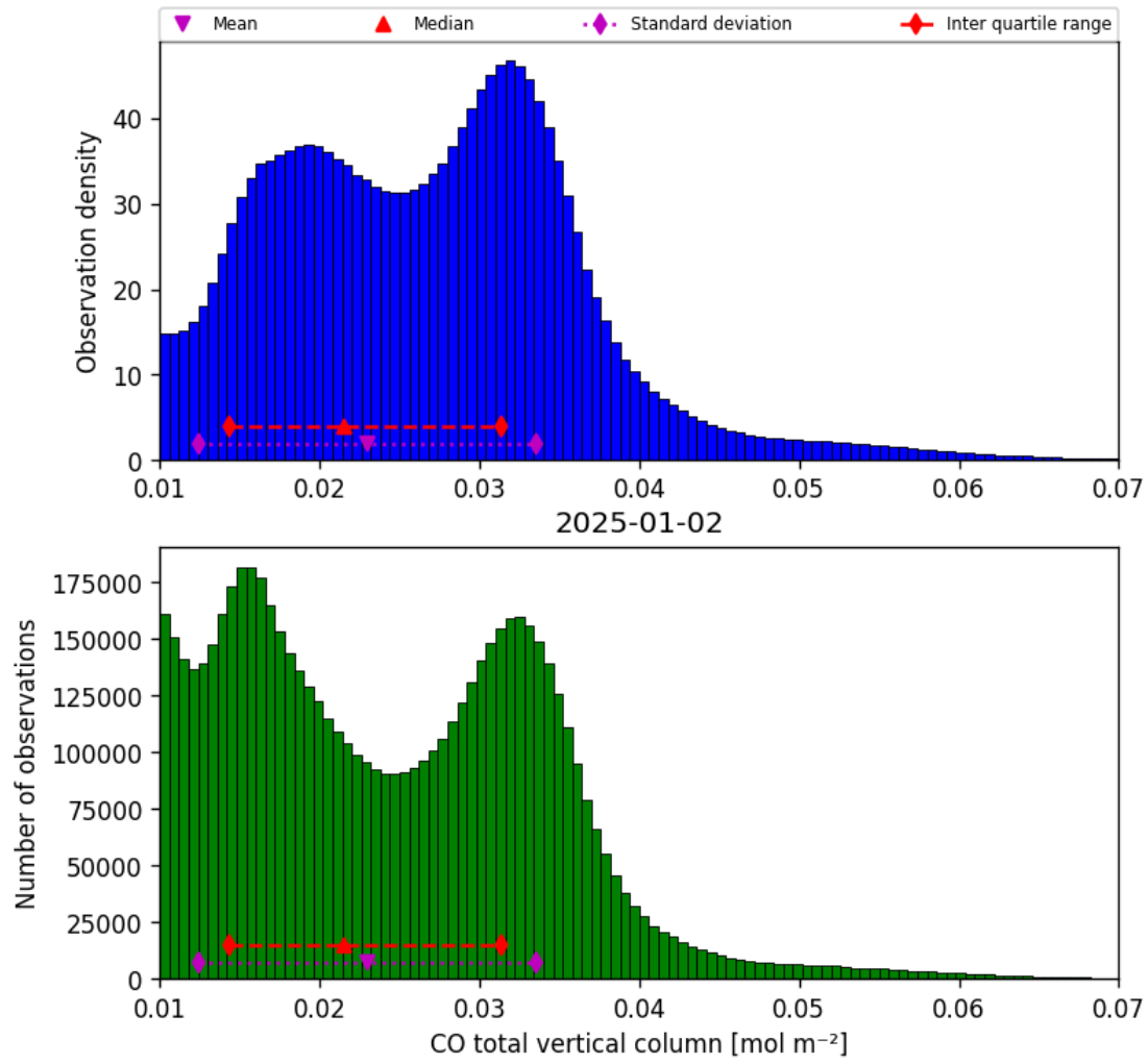
Figure 14: Histogram of “CO total vertical column” for 2025-01-02 to 2025-01-03
