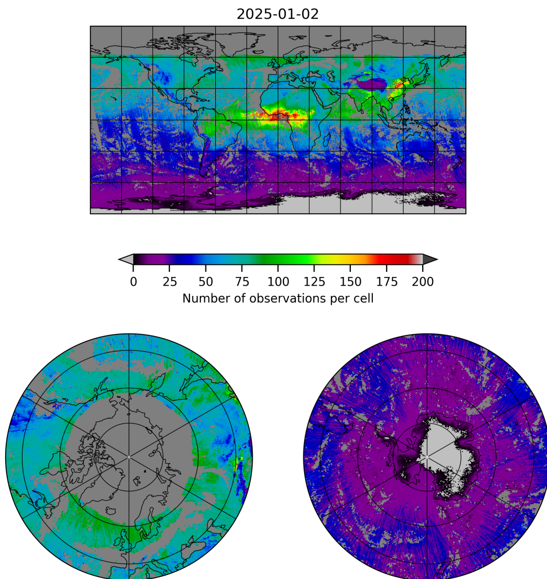
Figure 5: Map of the number of observations for 2025-01-02 to 2025-01-03
