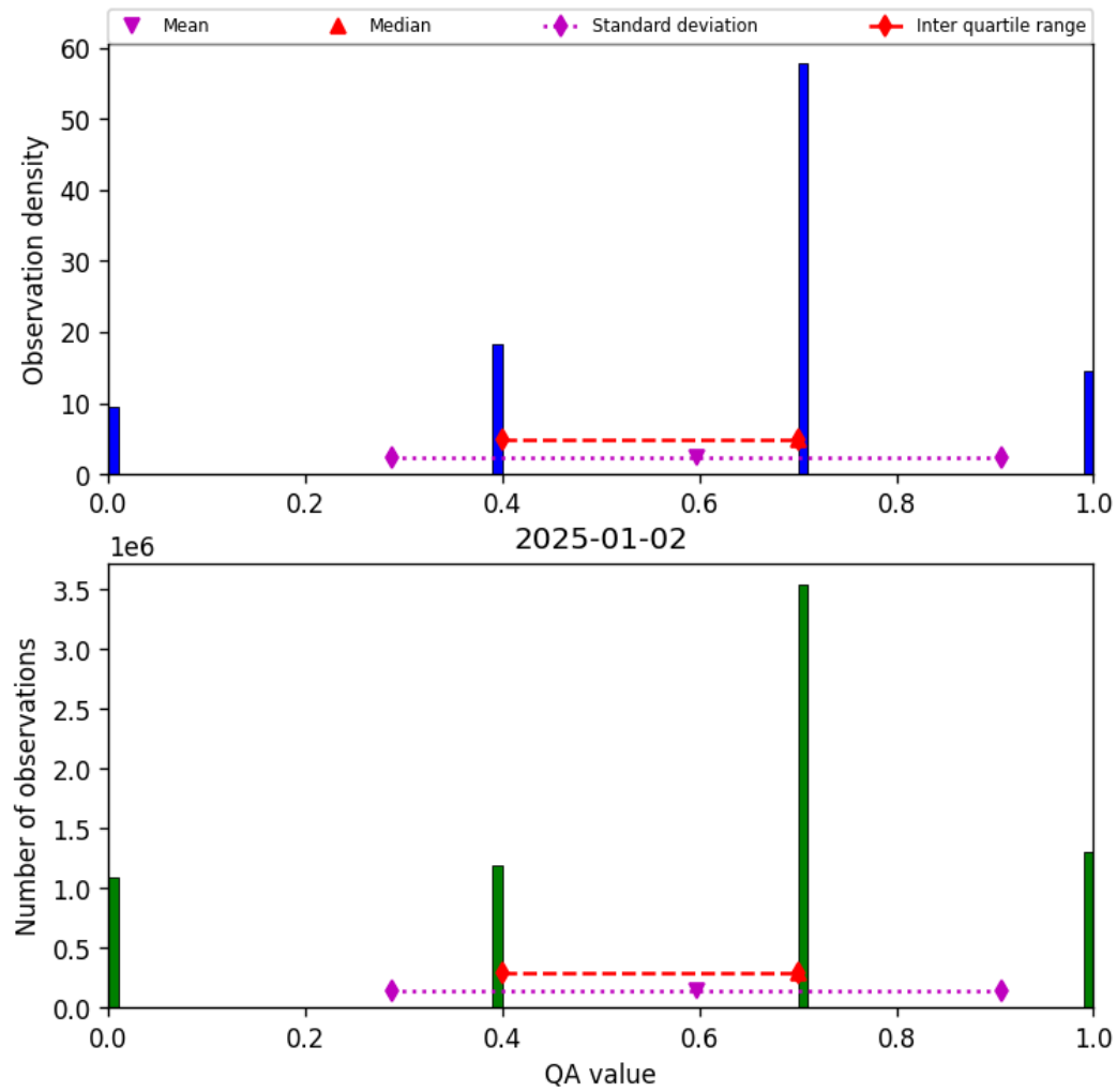
Figure 13: Histogram of “QA value” for 2025-01-02 to 2025-01-03
