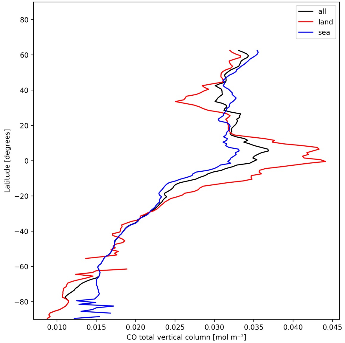
Figure 7: Zonal average of “CO total vertical column” for 2025-01-02 to 2025-01-03.
