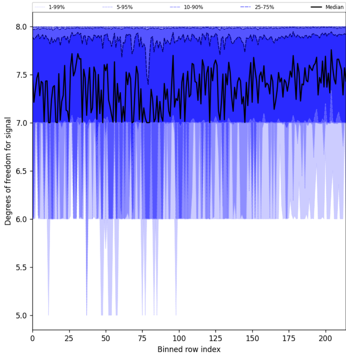
Figure 25: Along track statistics of “Degrees of freedom for signal” for 2025-01-02 to 2025-01-03
