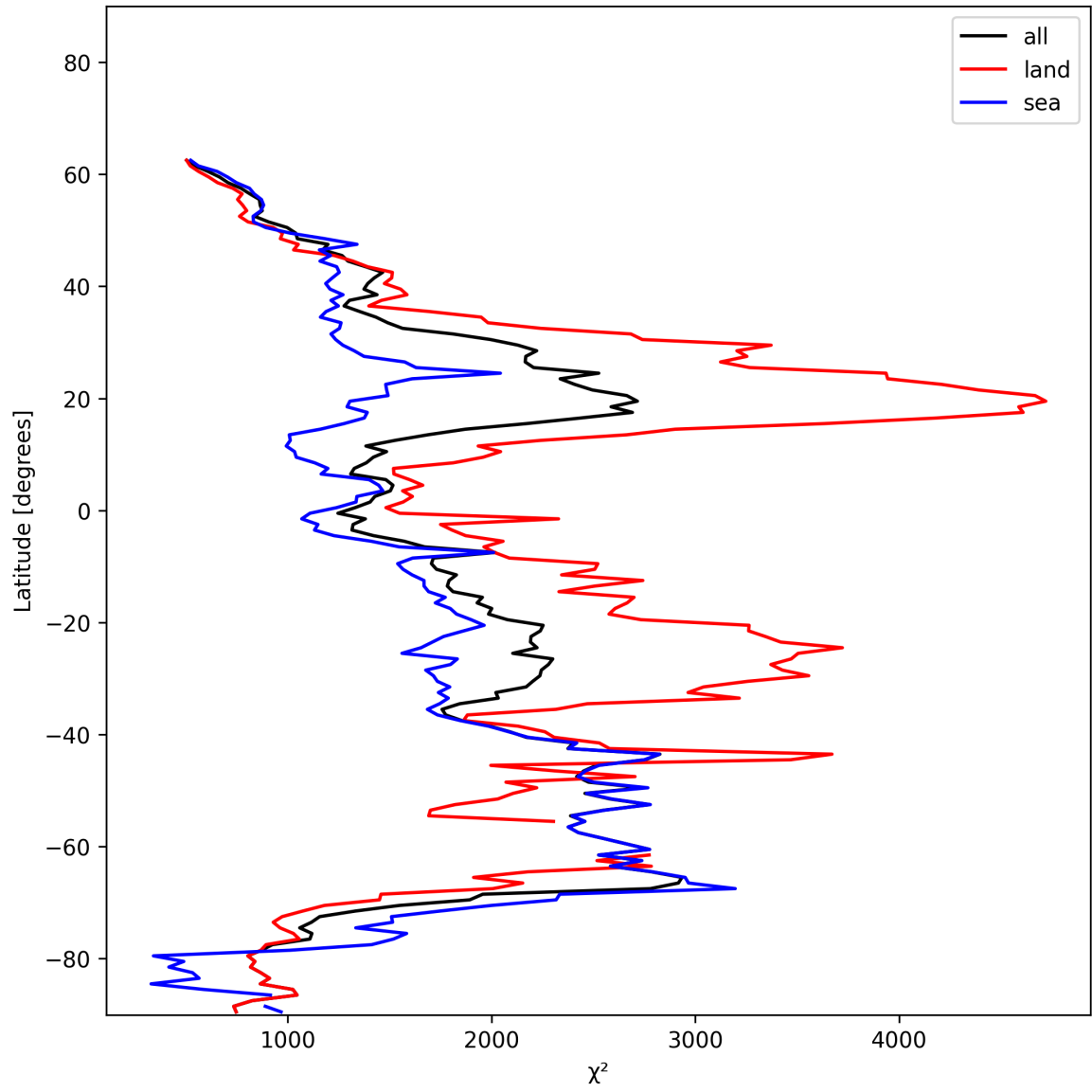
Figure 10: Zonal average of “ \chi^2 ” for 2025-01-02 to 2025-01-03.
