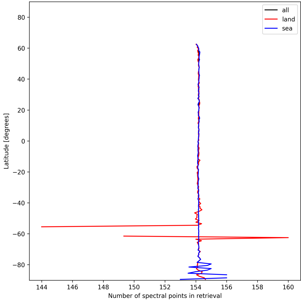
Figure 9: Zonal average of “Number of spectral points in retrieval” for 2025-01-02 to 2025-01-03.
