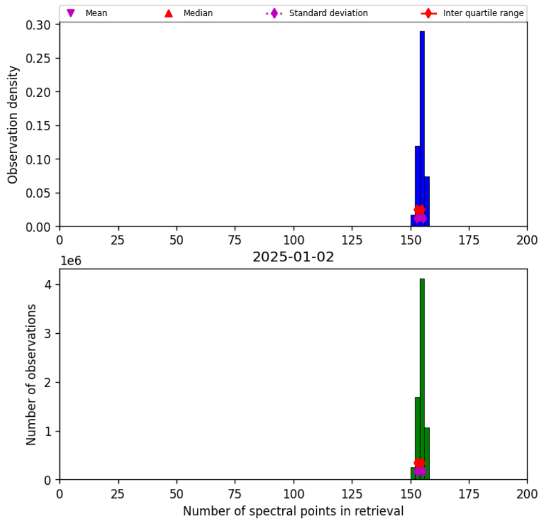
Figure 16: Histogram of “Number of spectral points in retrieval” for 2025-01-02 to 2025-01-03
