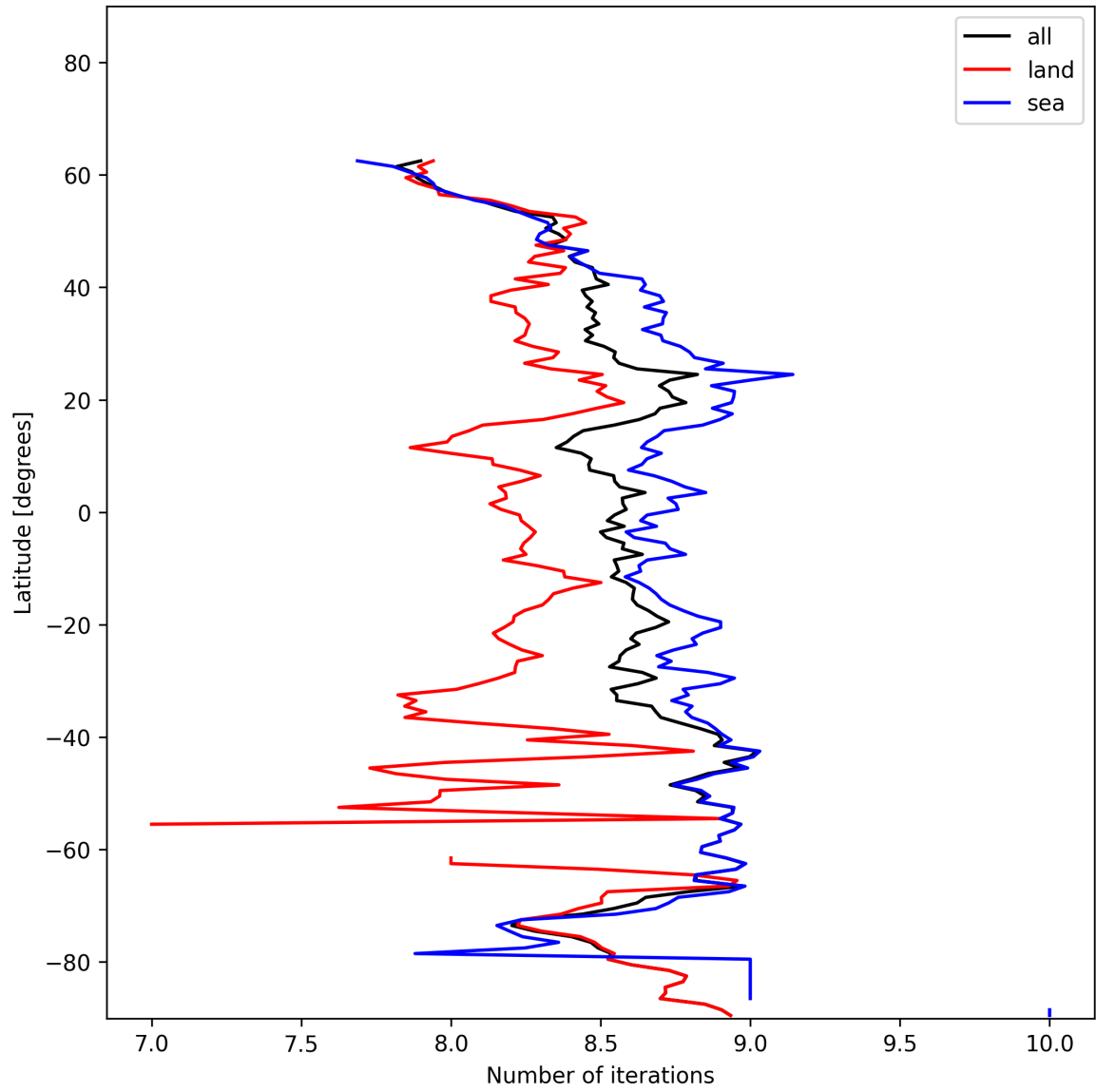
Figure 12: Zonal average of “Number of iterations” for 2025-01-02 to 2025-01-03.
