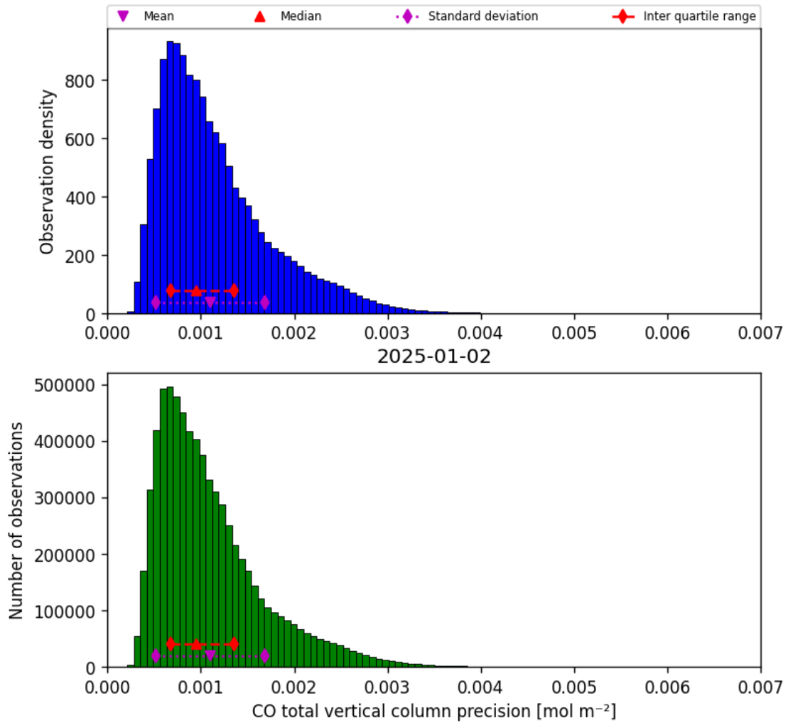
Figure 15: Histogram of “CO total vertical column precision” for 2025-01-02 to 2025-01-03
