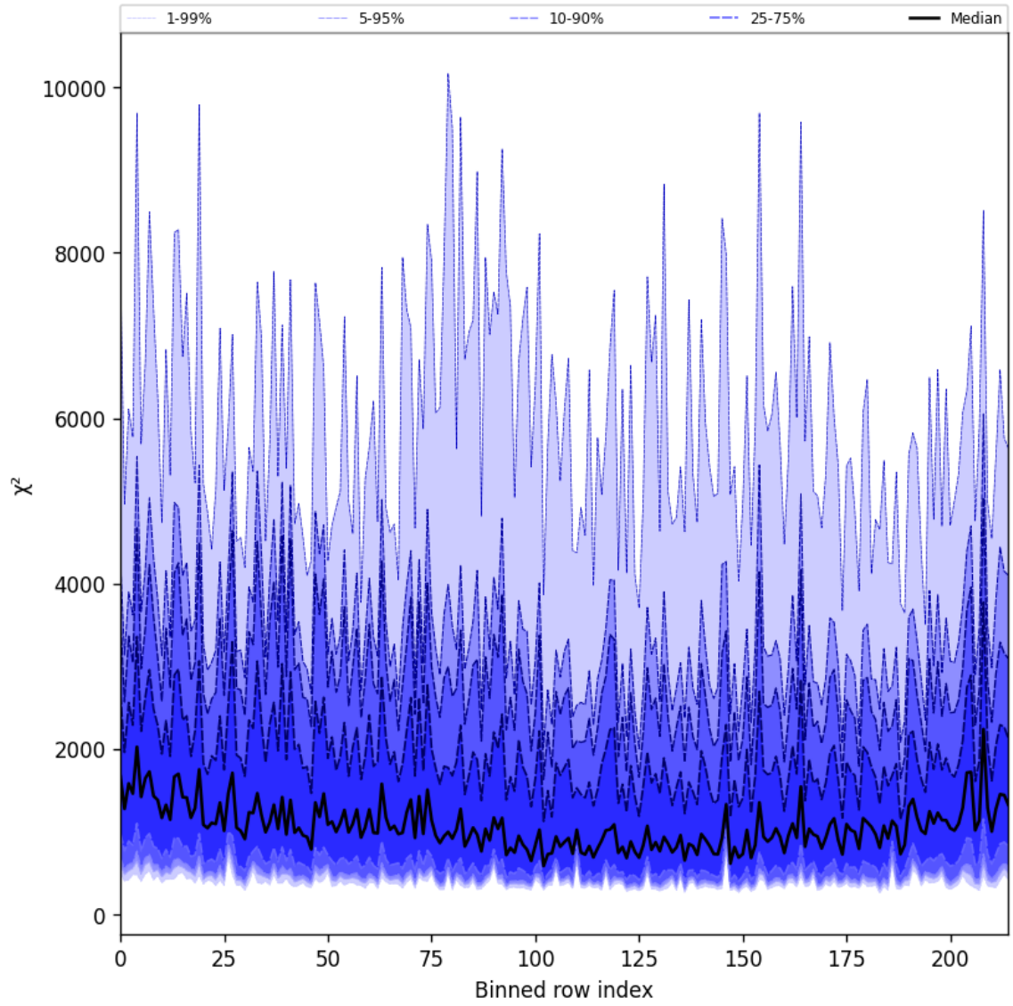
Figure 24: Along track statistics of “ \chi^2 ” for 2025-01-02 to 2025-01-03
