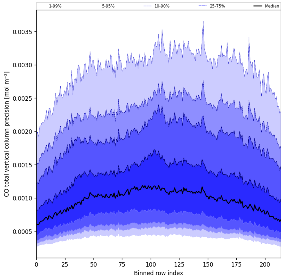
Figure 22: Along track statistics of “CO total vertical column precision” for 2025-01-02 to 2025-01-03
