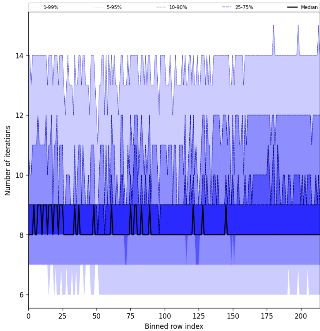
Figure 26: Along track statistics of “Number of iterations” for 2025-01-02 to 2025-01-03
