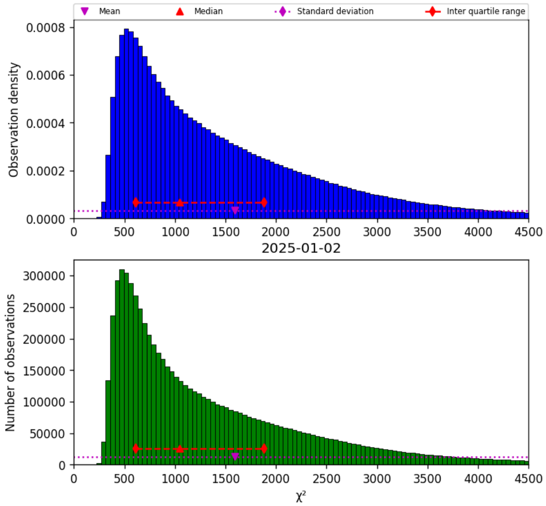
Figure 17: Histogram of " \chi^2 " for 2025-01-02 to 2025-01-03
