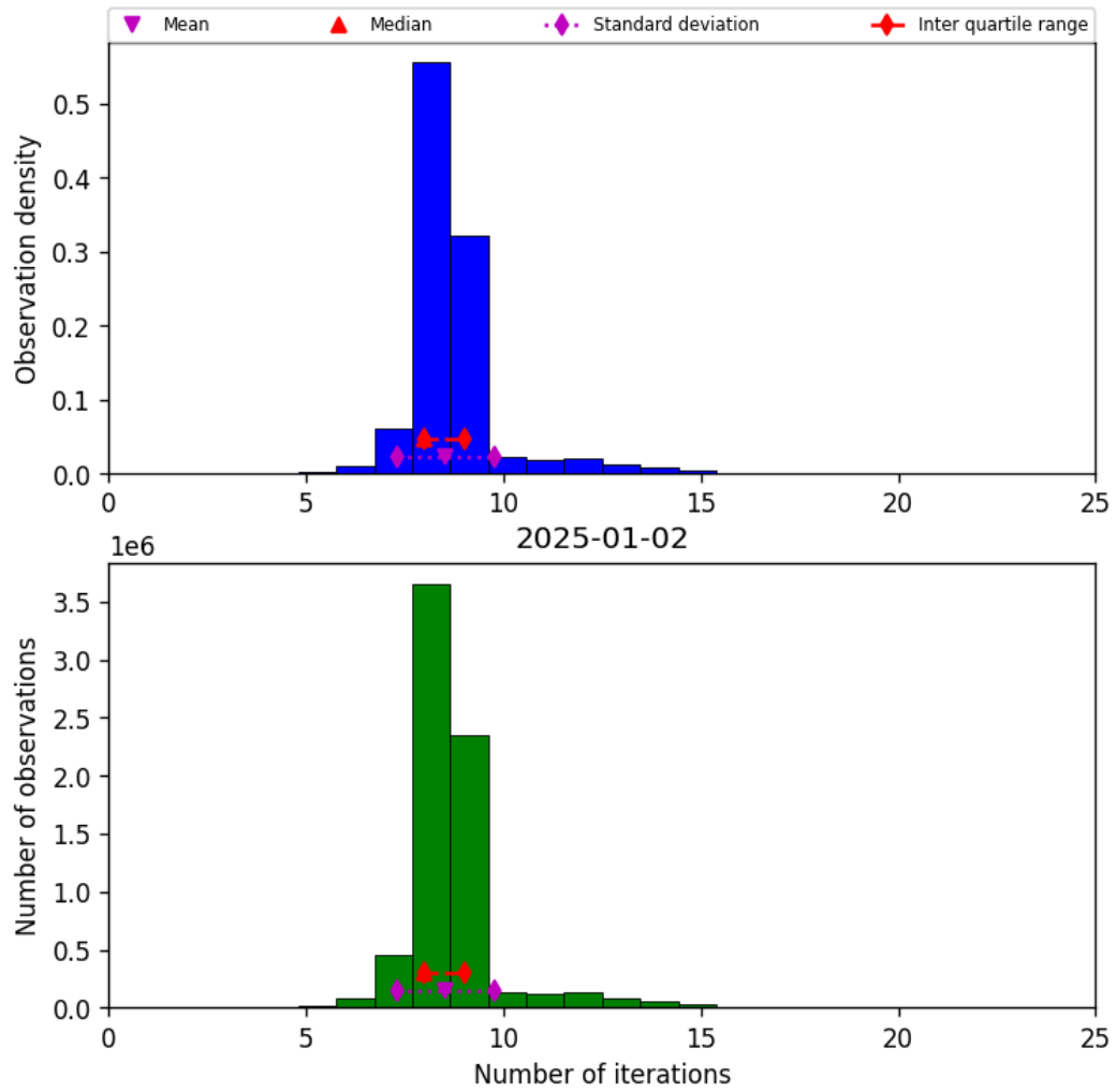
Figure 19: Histogram of “Number of iterations” for 2025-01-02 to 2025-01-03
