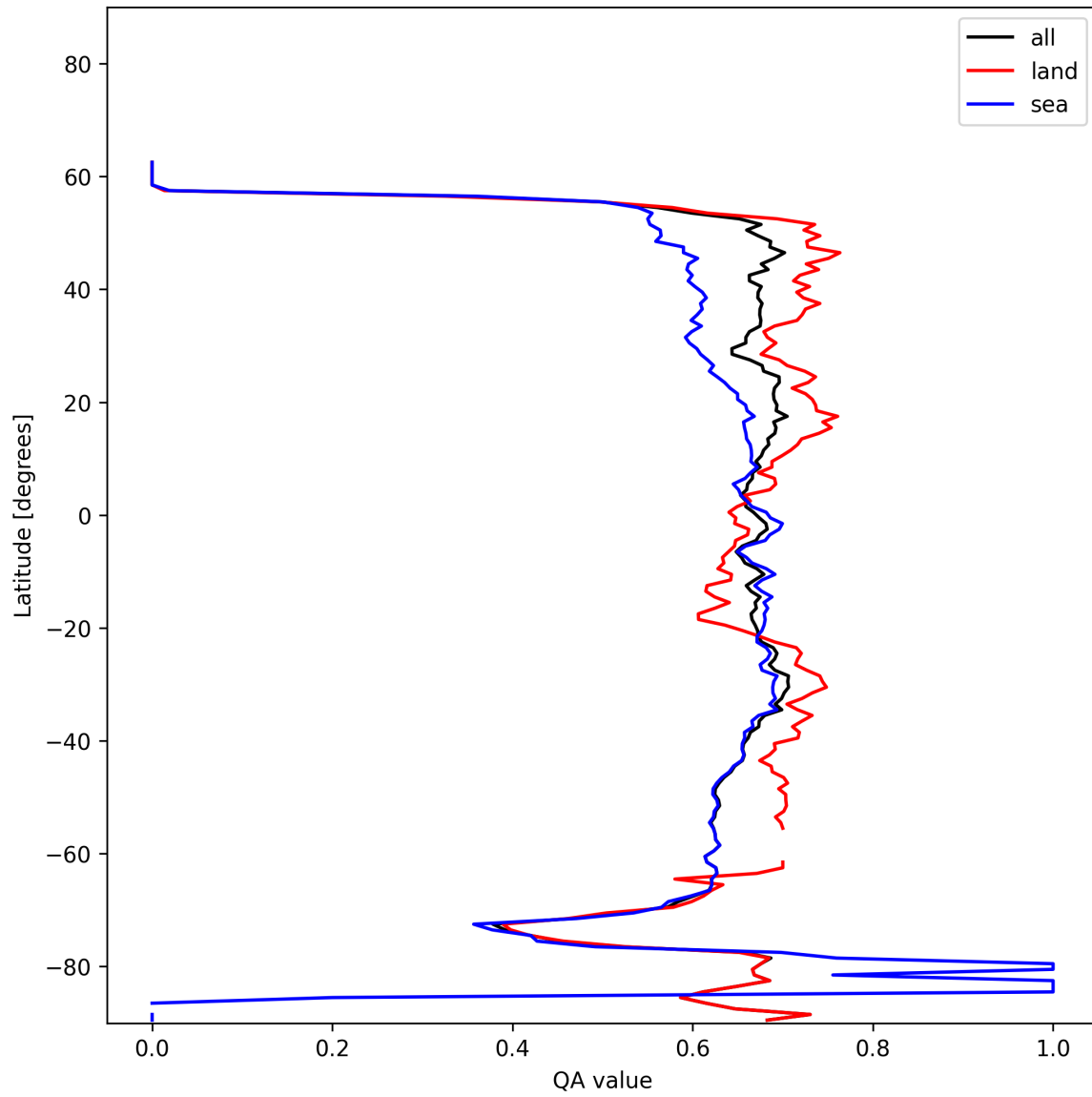
Figure 6: Zonal average of “QA value” for 2025-01-02 to 2025-01-03.
