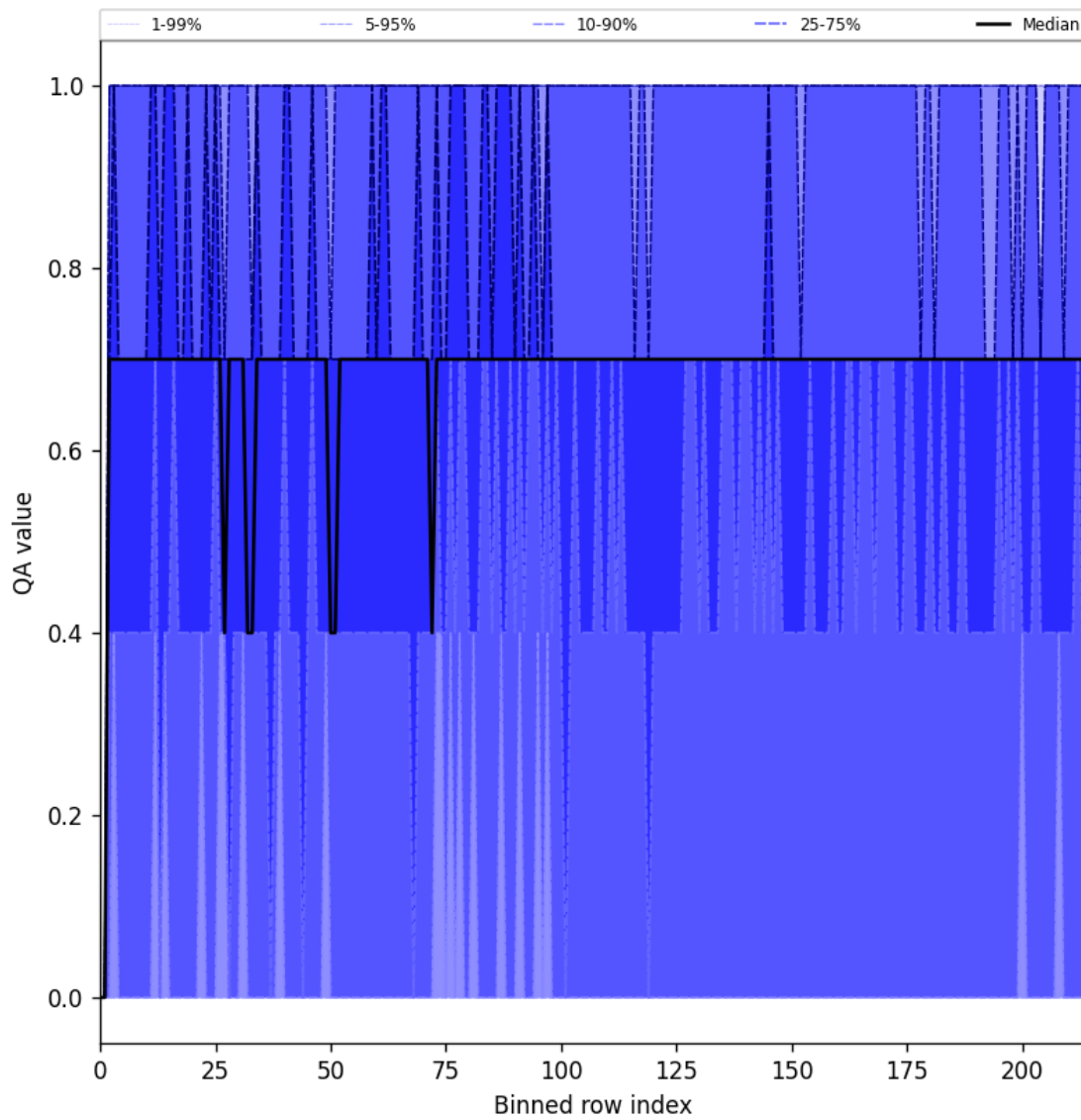
Figure 20: Along track statistics of “QA value” for 2025-01-02 to 2025-01-03
