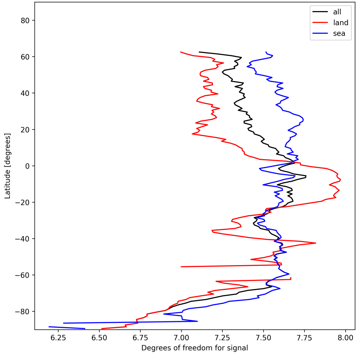
Figure 11: Zonal average of “Degrees of freedom for signal” for 2025-01-02 to 2025-01-03.
