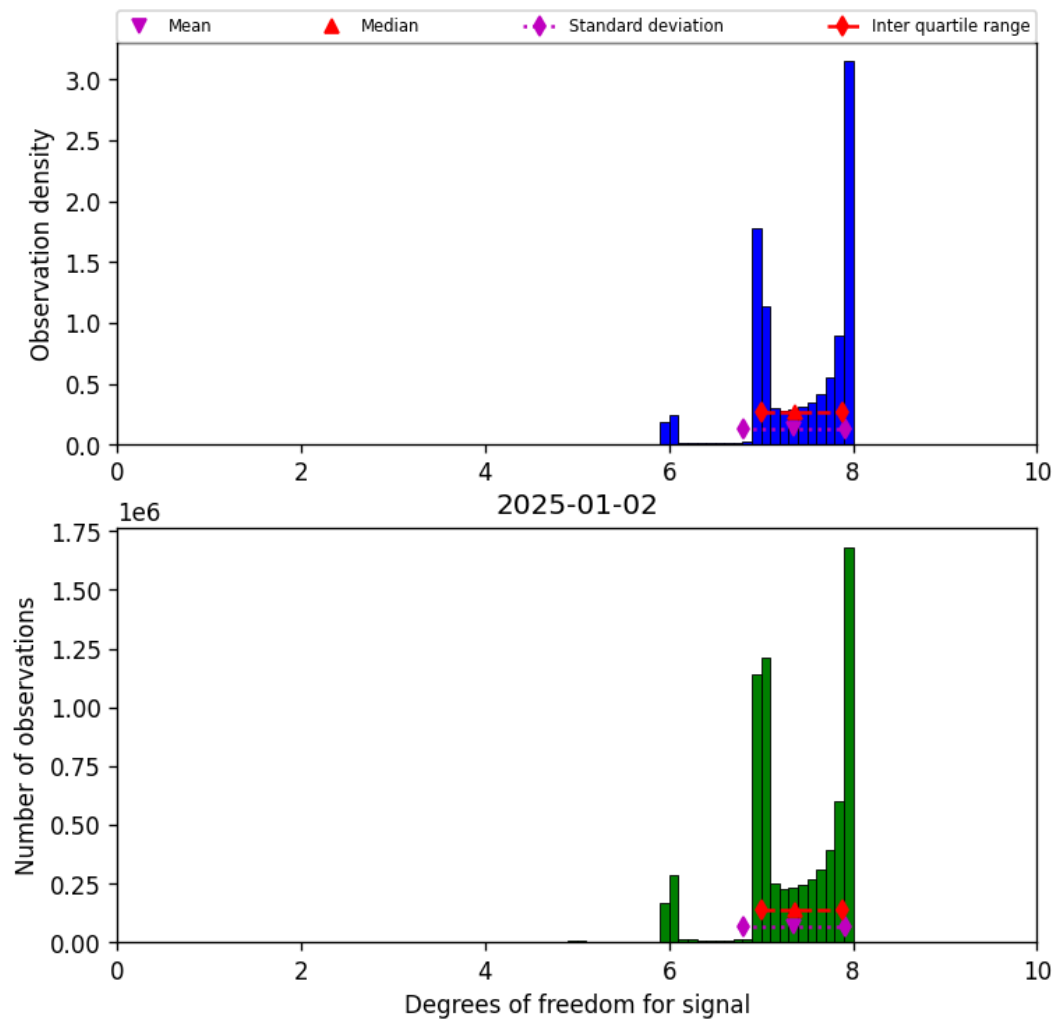
Figure 18: Histogram of “Degrees of freedom for signal” for 2025-01-02 to 2025-01-03
