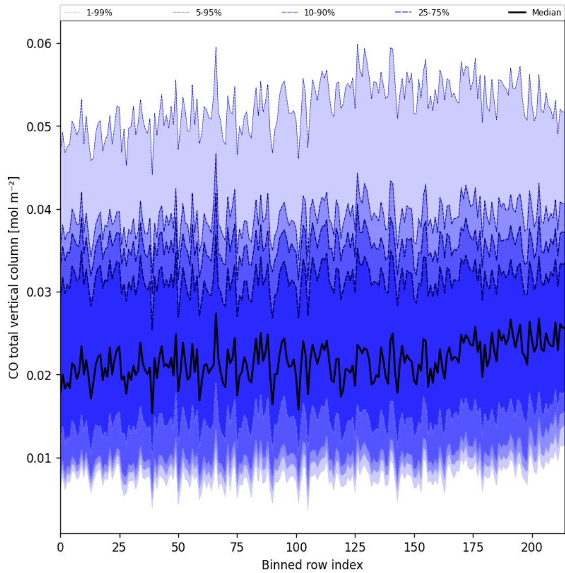
Figure 21: Along track statistics of “CO total vertical column” for 2025-01-02 to 2025-01-03
