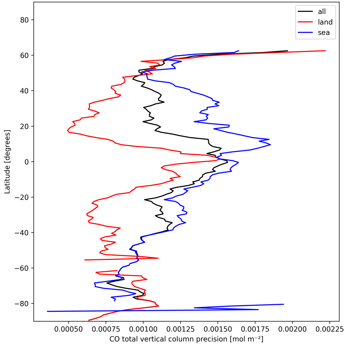
Figure 8: Zonal average of “CO total vertical column precision” for 2025-01-03 to 2025-01-04.
