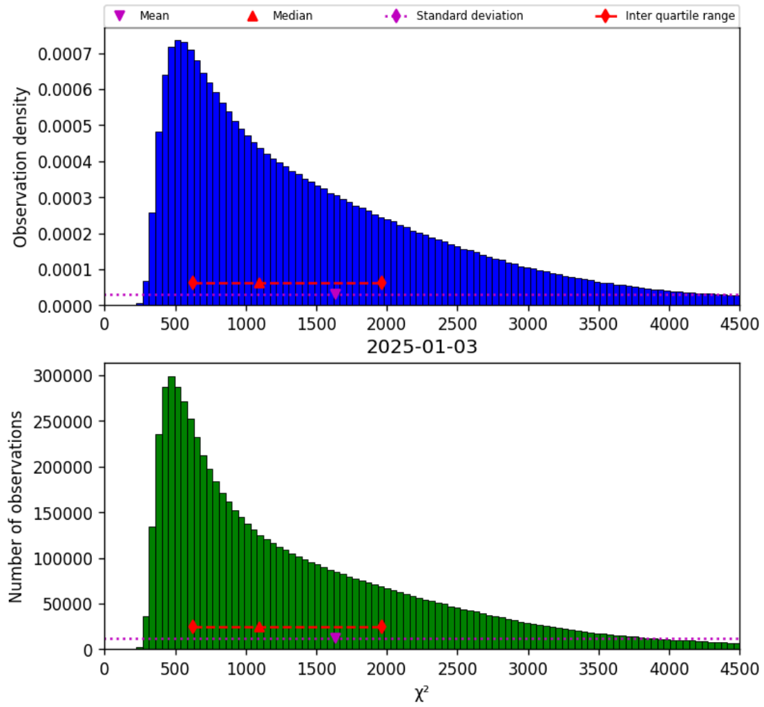
Figure 17: Histogram of “ \chi^2 ” for 2025-01-03 to 2025-01-04
