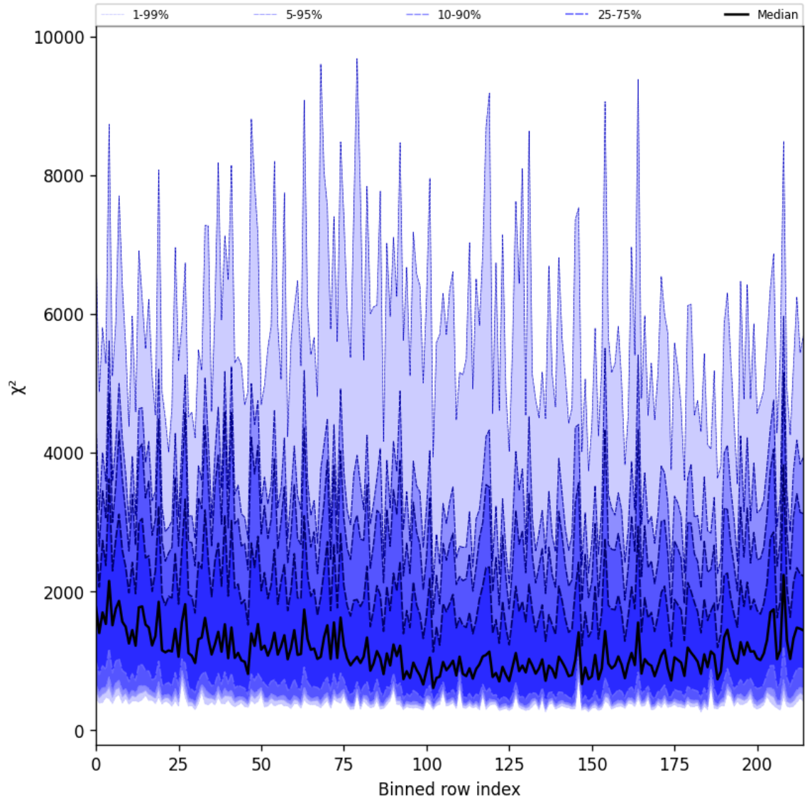
Figure 24: Along track statistics of “ \chi^2 ” for 2025-01-03 to 2025-01-04
