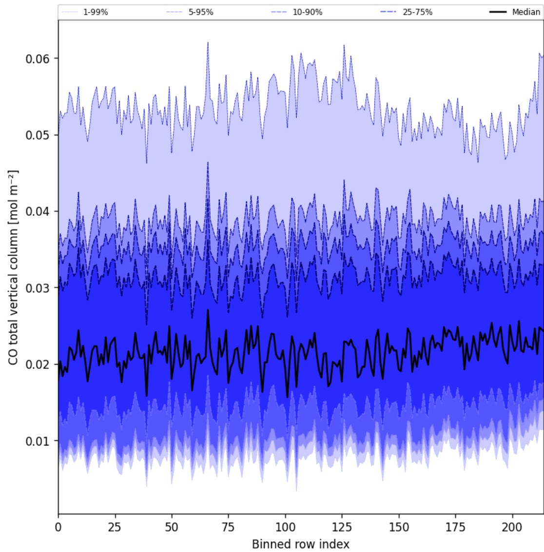
Figure 21: Along track statistics of “CO total vertical column” for 2025-01-03 to 2025-01-04
