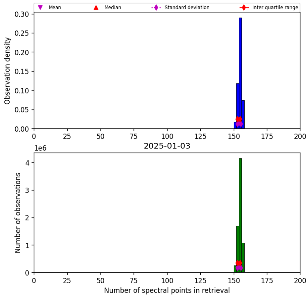
Figure 16: Histogram of “Number of spectral points in retrieval” for 2025-01-03 to 2025-01-04
