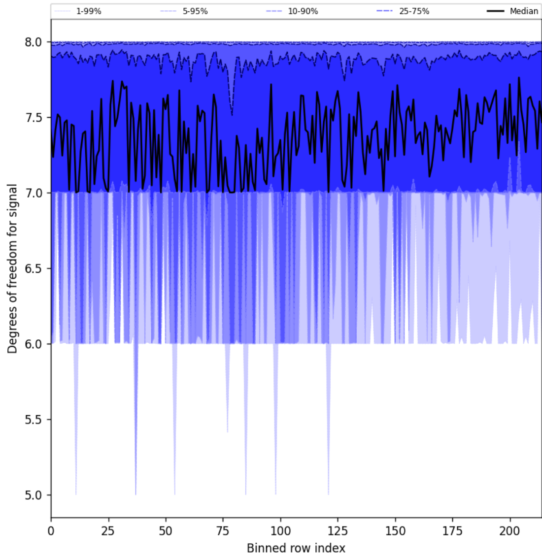
Figure 25: Along track statistics of “Degrees of freedom for signal” for 2025-01-03 to 2025-01-04
