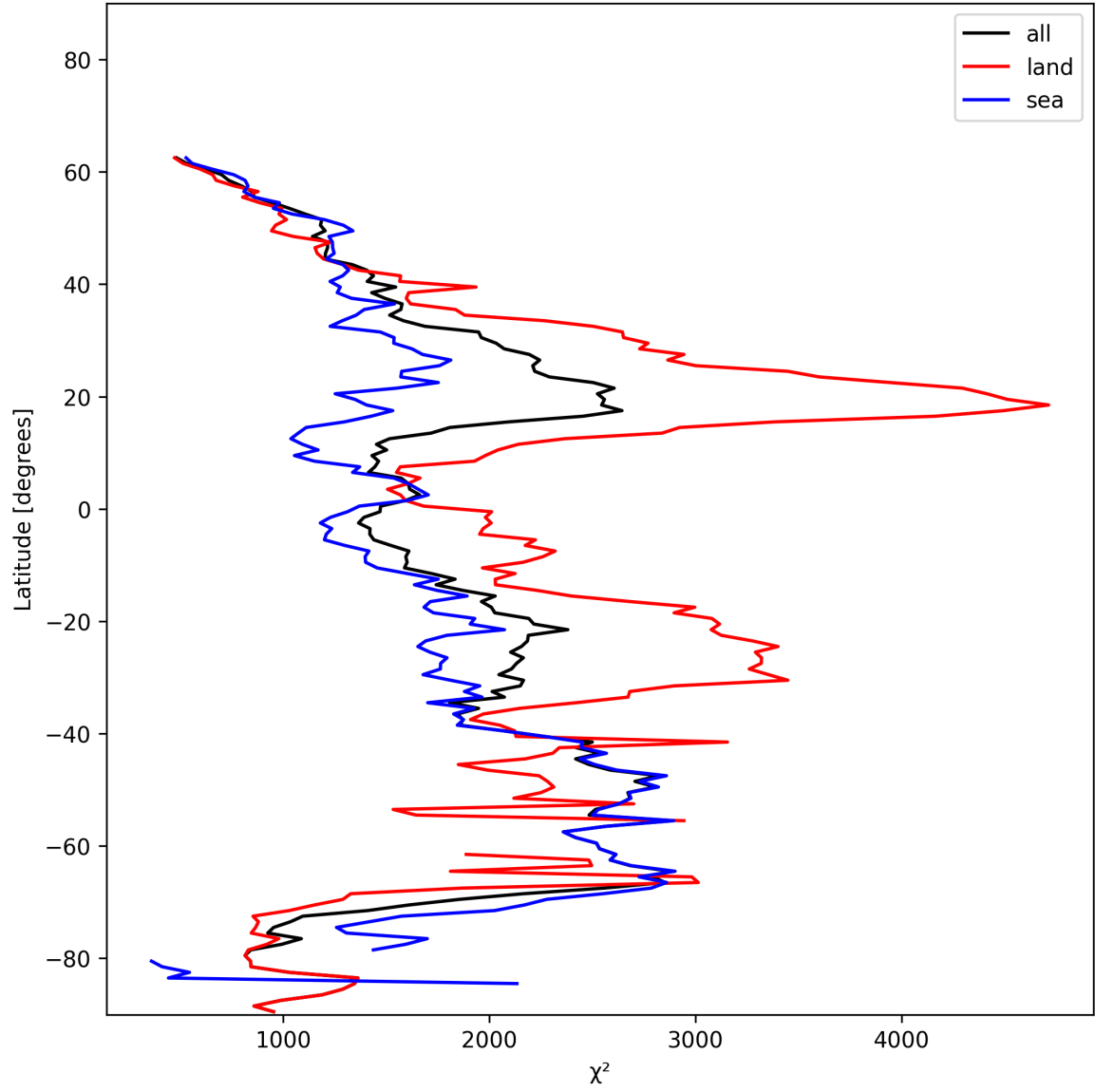
Figure 10: Zonal average of “ \chi^2 ” for 2025-01-03 to 2025-01-04.
