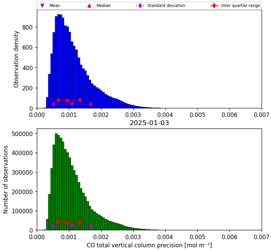
Figure 15: Histogram of “CO total vertical column precision” for 2025-01-03 to 2025-01-04
