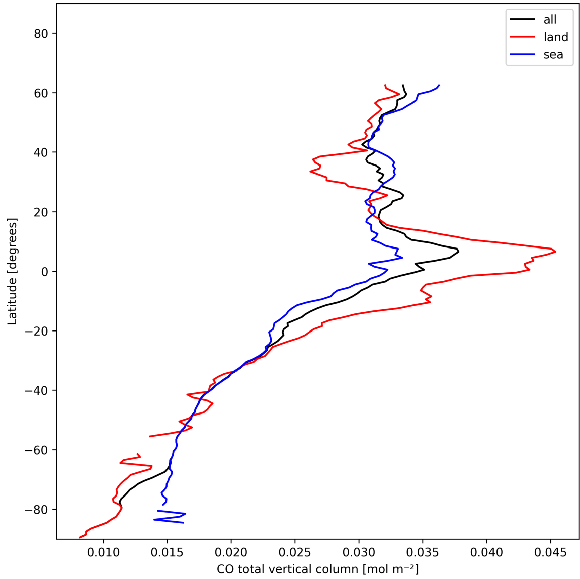
Figure 7: Zonal average of “CO total vertical column” for 2025-01-03 to 2025-01-04.
