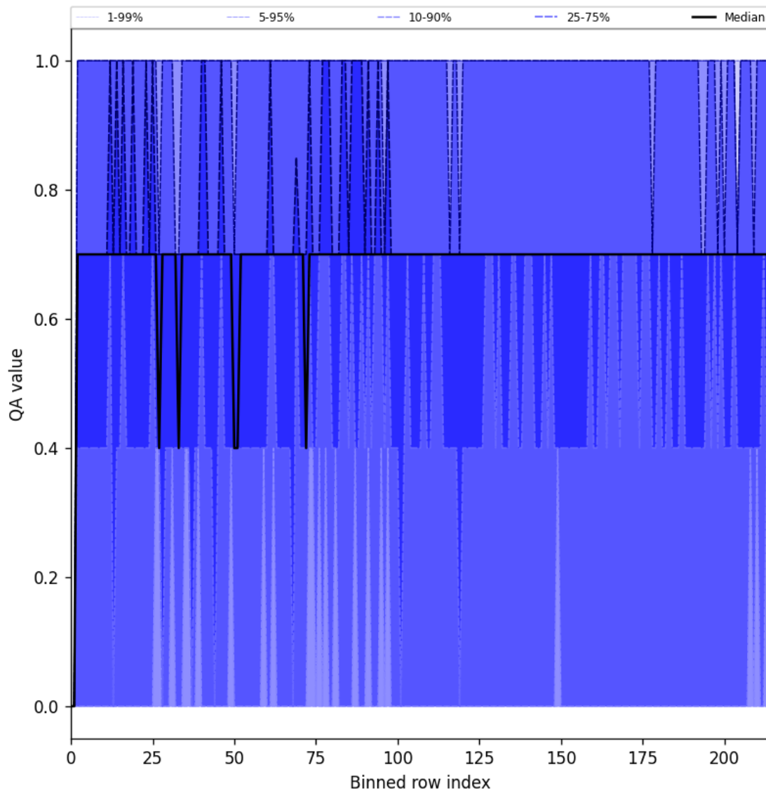
Figure 20: Along track statistics of “QA value” for 2025-01-03 to 2025-01-04
