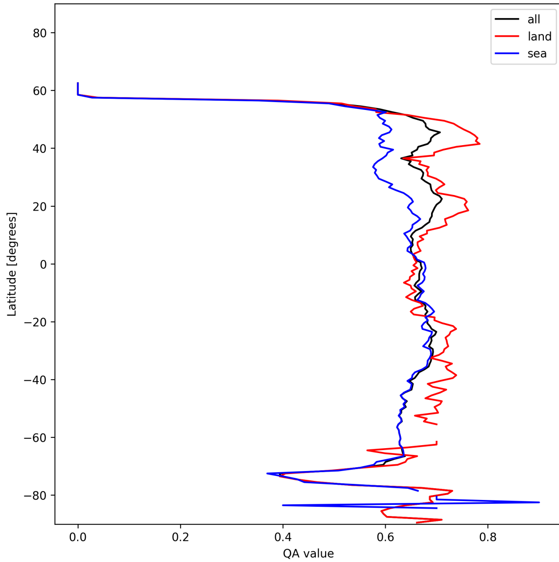
Figure 6: Zonal average of “QA value” for 2025-01-03 to 2025-01-04.
