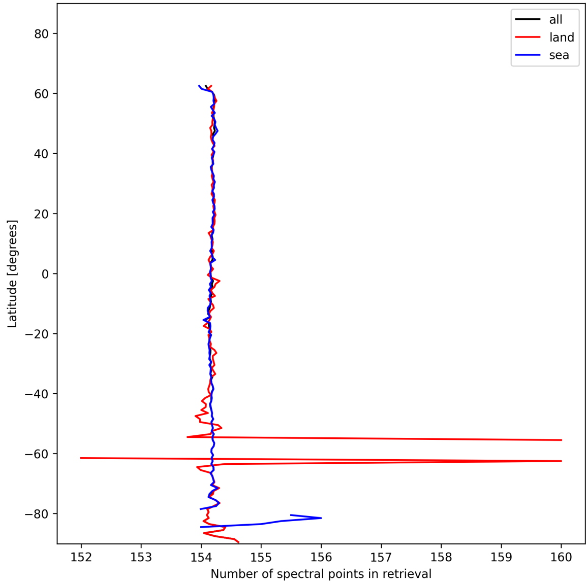
Figure 9: Zonal average of “Number of spectral points in retrieval” for 2025-01-03 to 2025-01-04.
