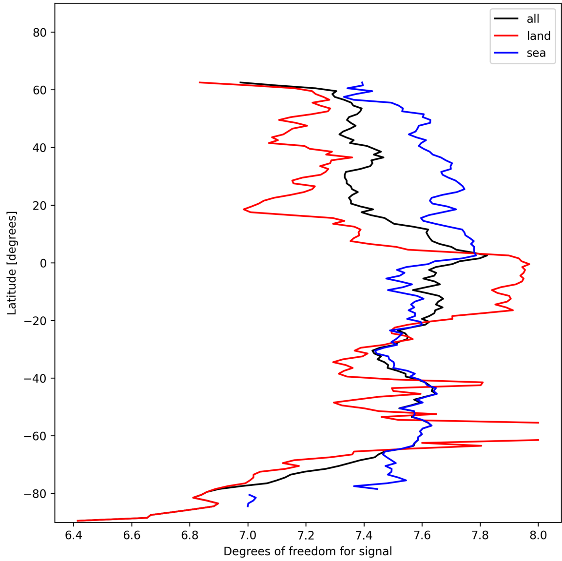
Figure 11: Zonal average of “Degrees of freedom for signal” for 2025-01-03 to 2025-01-04.
