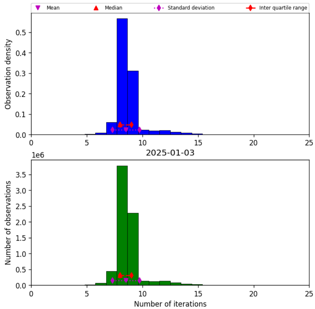
Figure 19: Histogram of “Number of iterations” for 2025-01-03 to 2025-01-04
