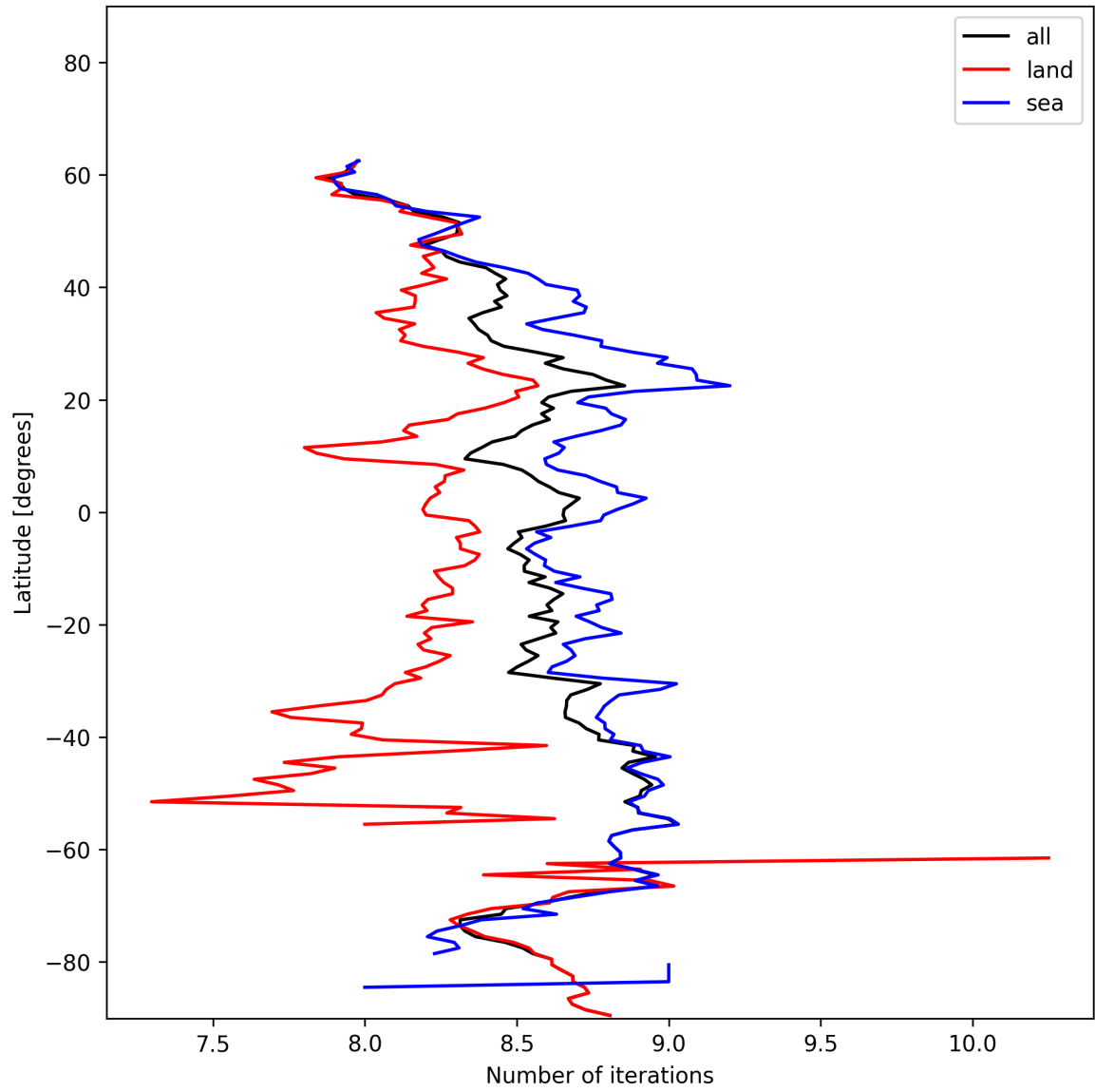
Figure 12: Zonal average of “Number of iterations” for 2025-01-03 to 2025-01-04.
