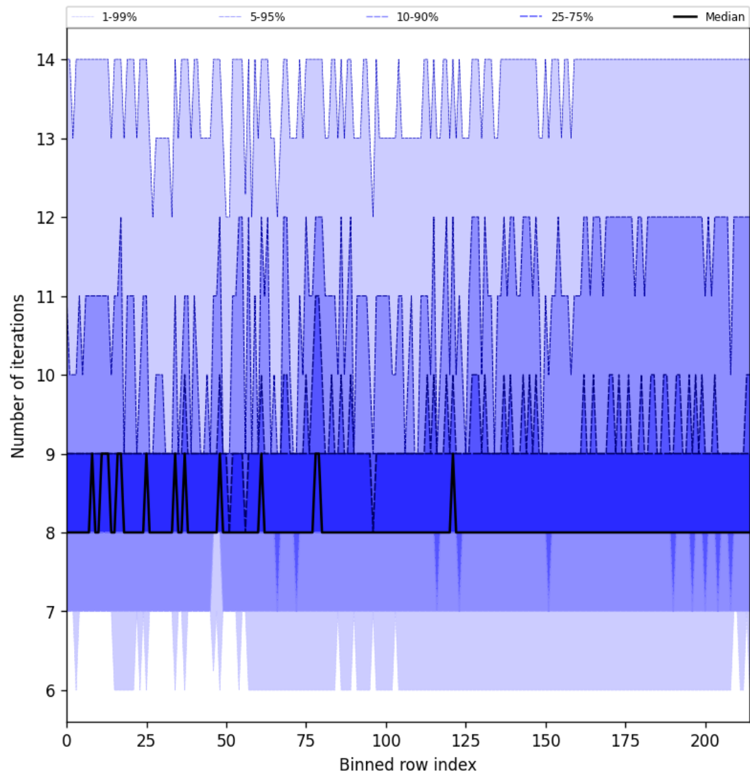
Figure 26: Along track statistics of “Number of iterations” for 2025-01-03 to 2025-01-04
