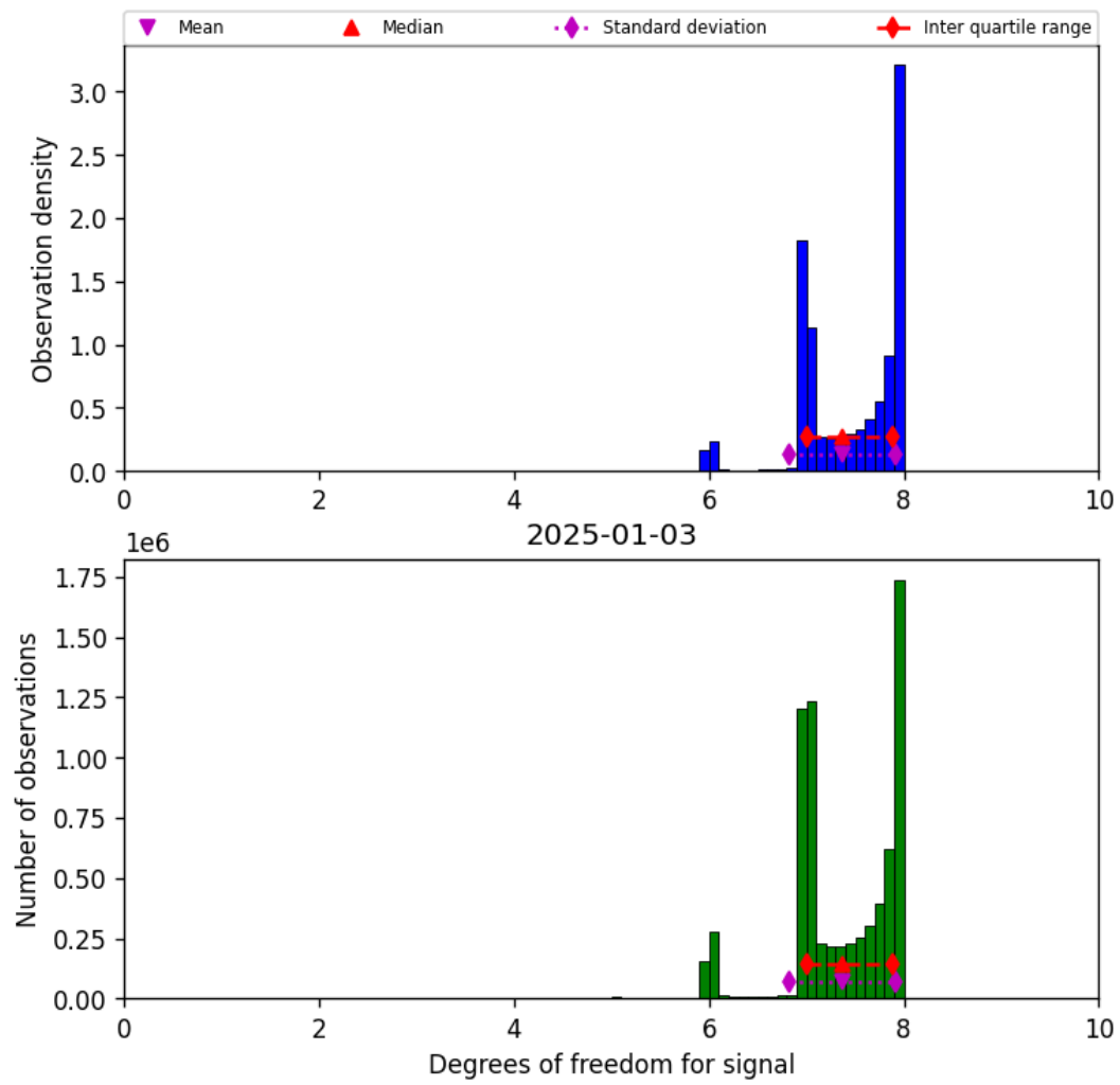
Figure 18: Histogram of “Degrees of freedom for signal” for 2025-01-03 to 2025-01-04
