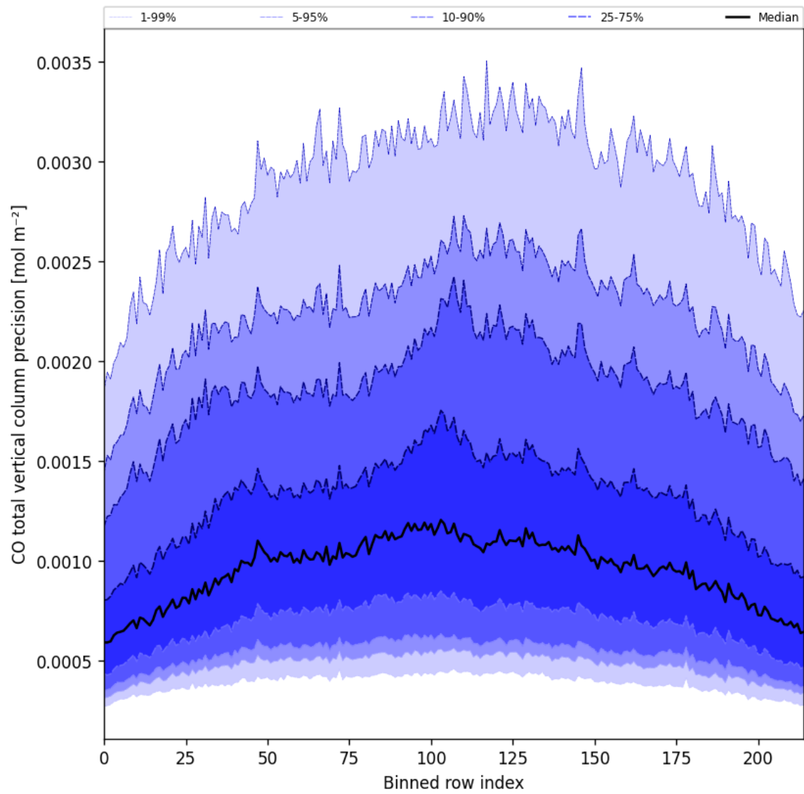
Figure 22: Along track statistics of “CO total vertical column precision” for 2025-01-03 to 2025-01-04
