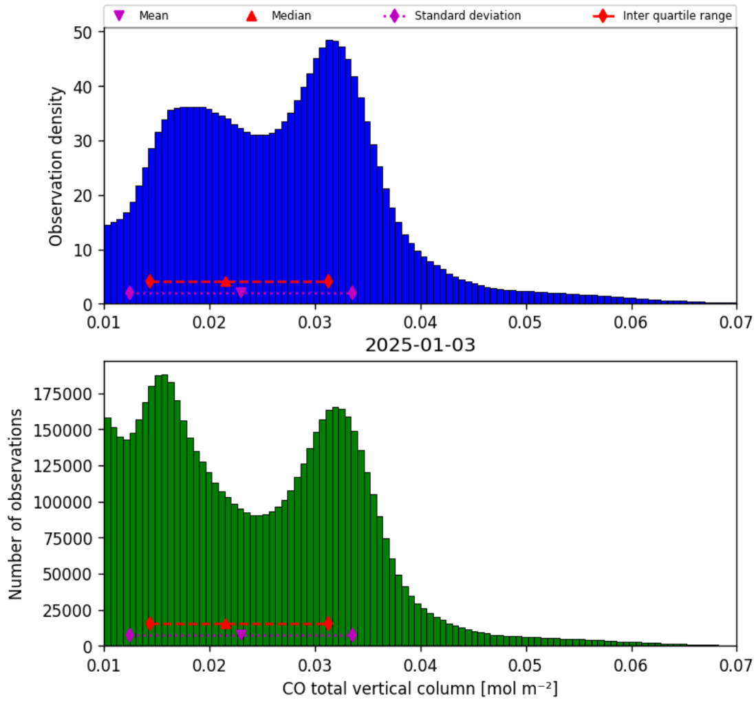
Figure 14: Histogram of “CO total vertical column” for 2025-01-03 to 2025-01-04
