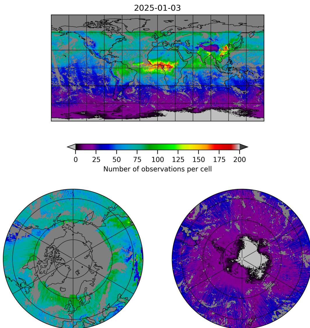
Figure 5: Map of the number of observations for 2025-01-03 to 2025-01-04
