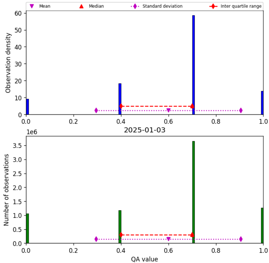
Figure 13: Histogram of “QA value” for 2025-01-03 to 2025-01-04
