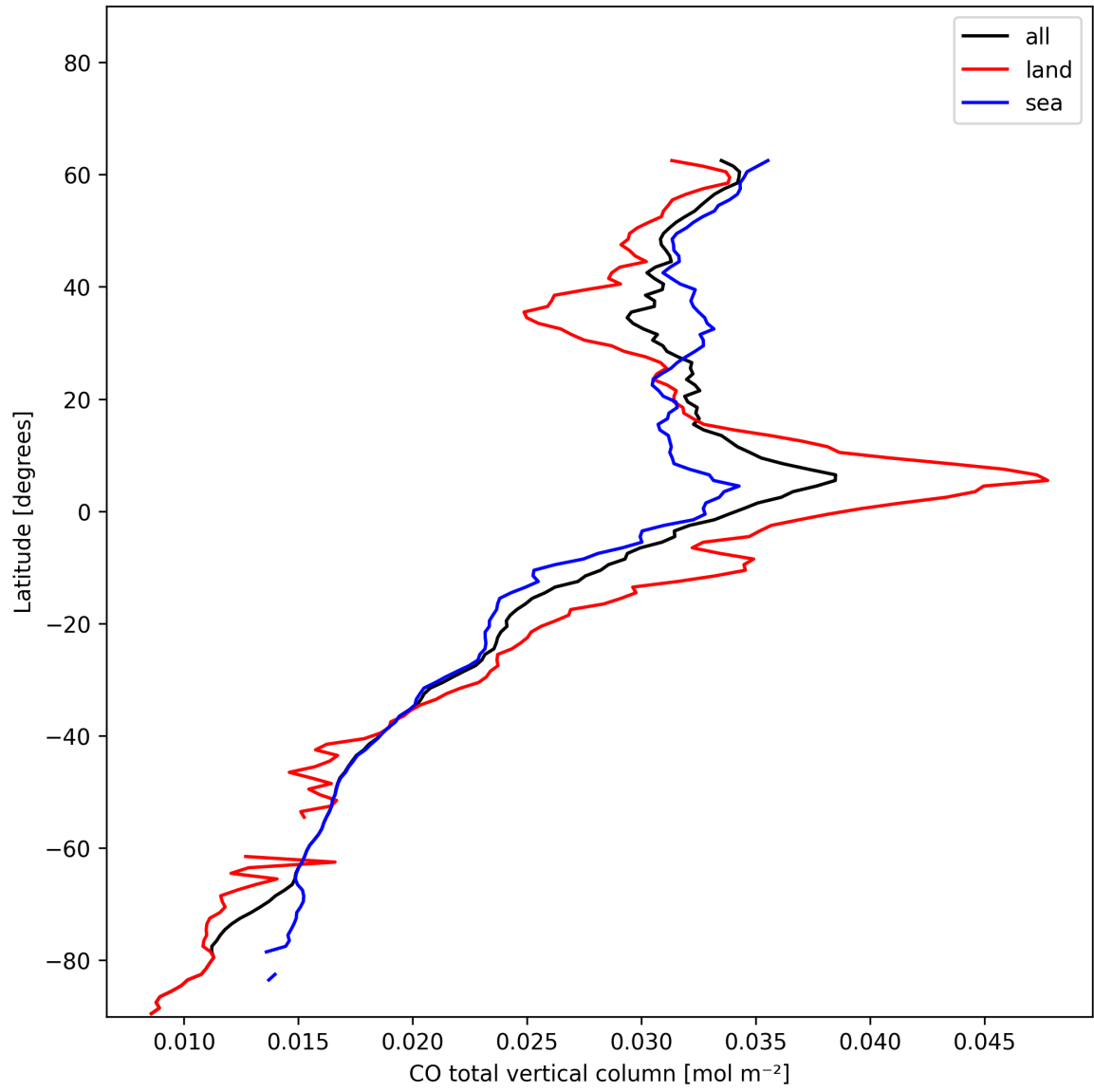
Figure 7: Zonal average of “CO total vertical column” for 2025-01-04 to 2025-01-04.
