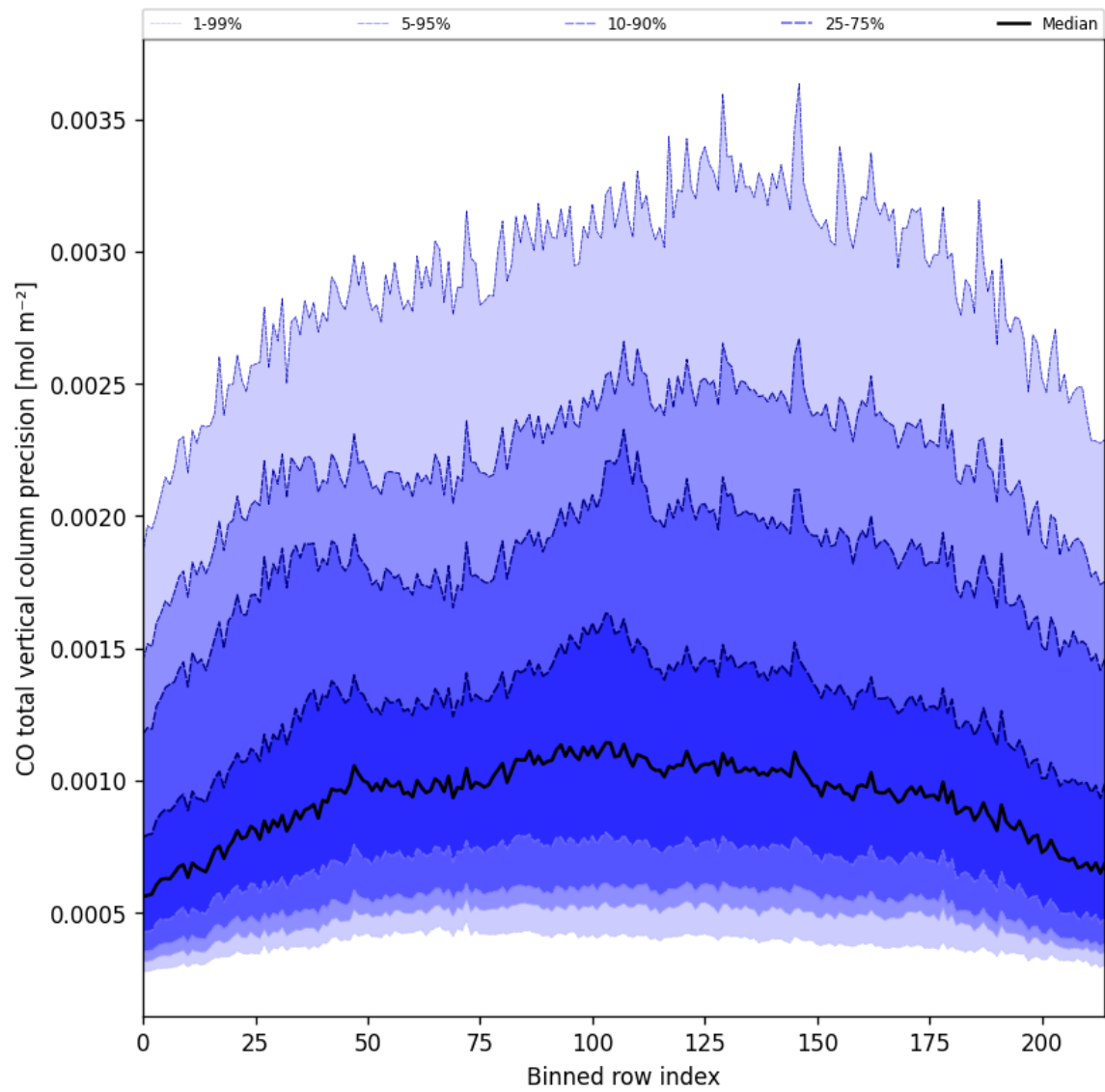
Figure 22: Along track statistics of “CO total vertical column precision” for 2025-01-04 to 2025-01-04
