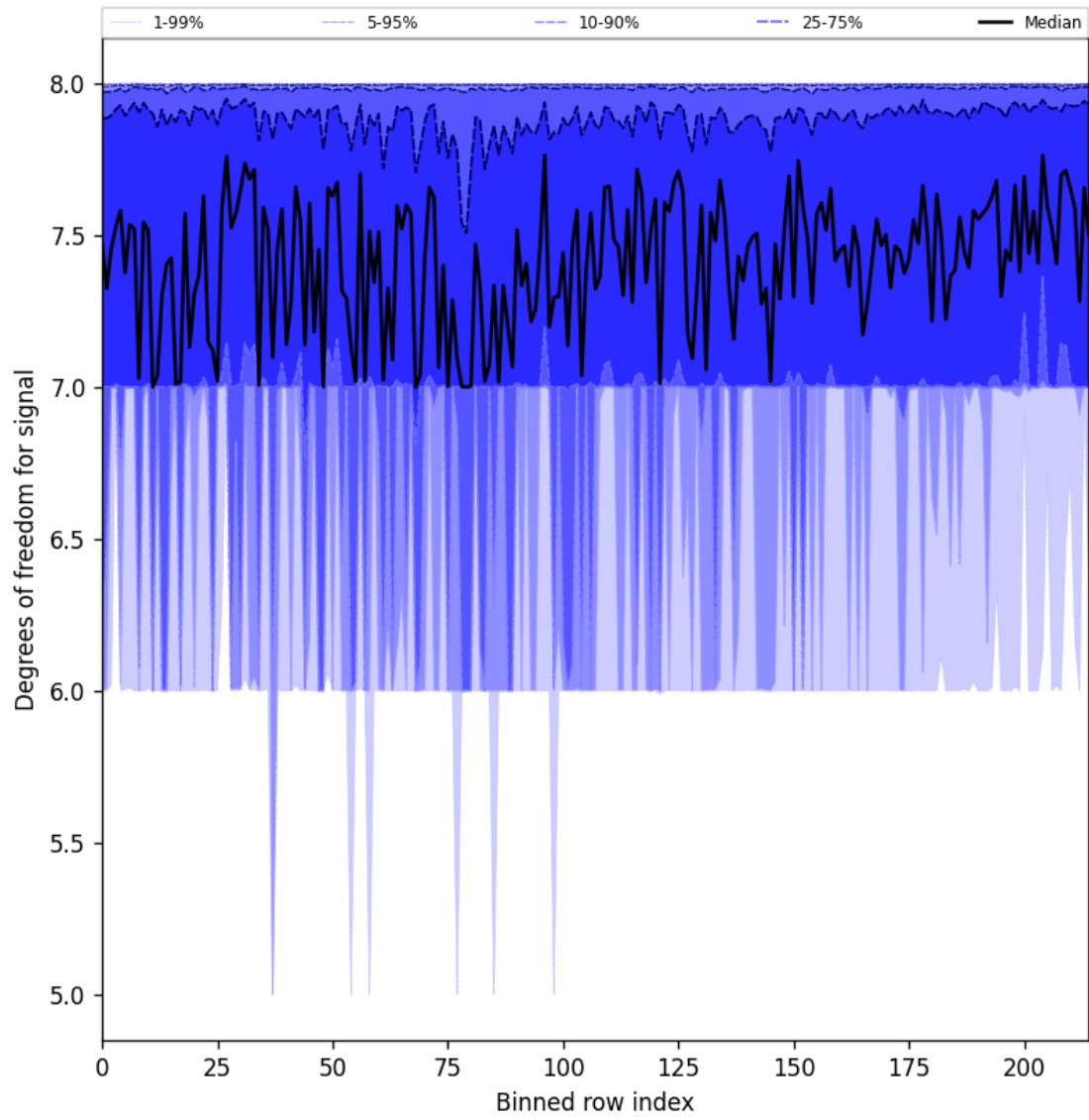
Figure 25: Along track statistics of “Degrees of freedom for signal” for 2025-01-04 to 2025-01-04
