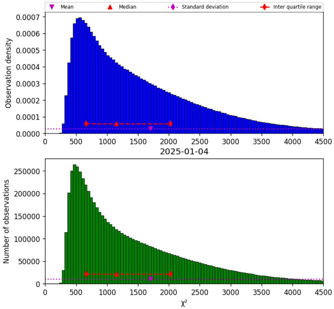
Figure 17: Histogram of " \chi^2 " for 2025-01-04 to 2025-01-04
