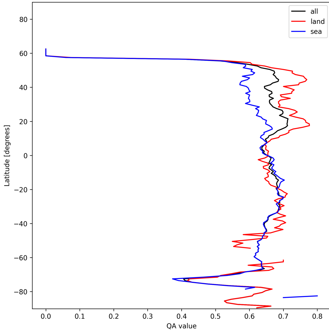
Figure 6: Zonal average of “QA value” for 2025-01-04 to 2025-01-04.
