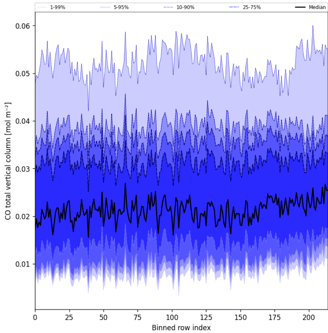
Figure 21: Along track statistics of “CO total vertical column” for 2025-01-04 to 2025-01-04
