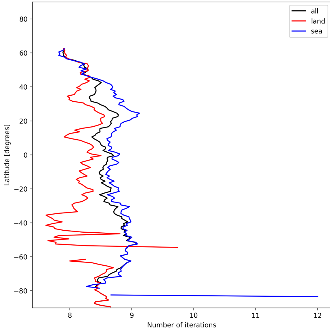
Figure 12: Zonal average of “Number of iterations” for 2025-01-04 to 2025-01-04.
