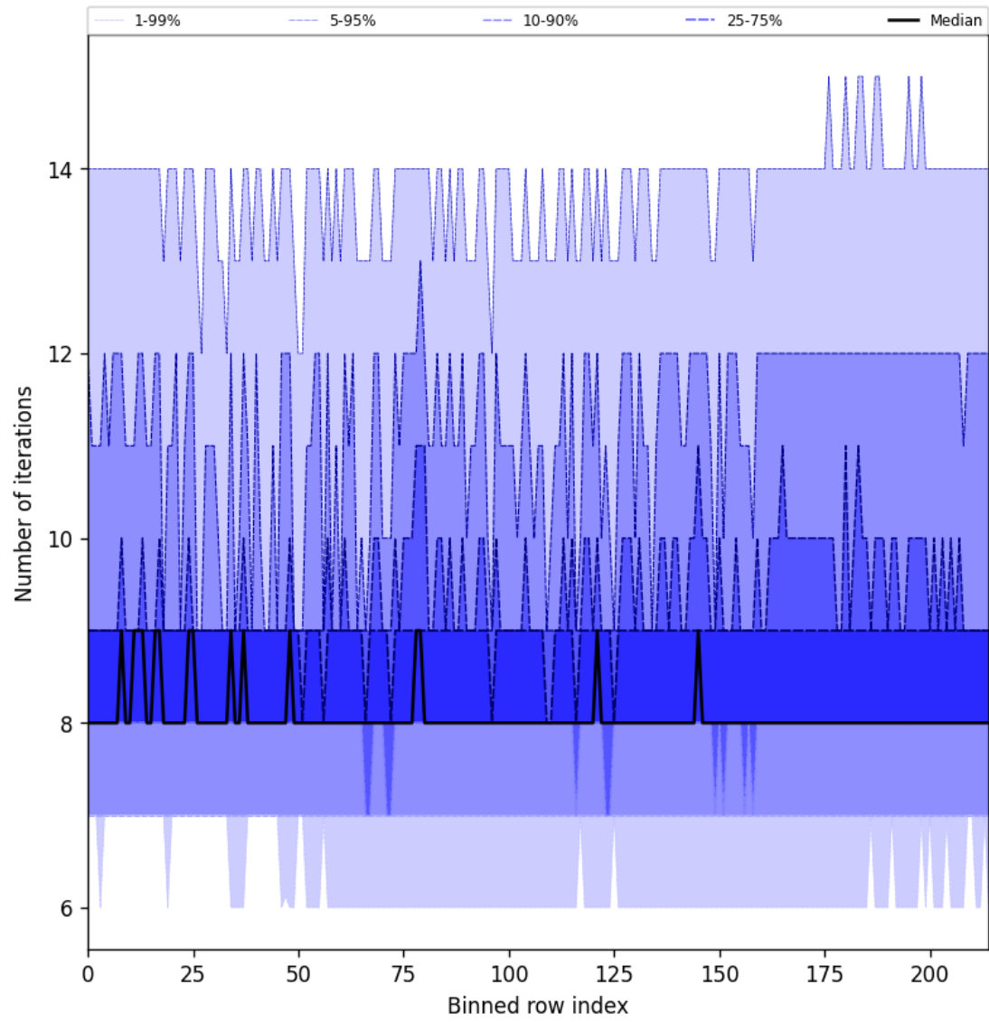
Figure 26: Along track statistics of “Number of iterations” for 2025-01-04 to 2025-01-04
