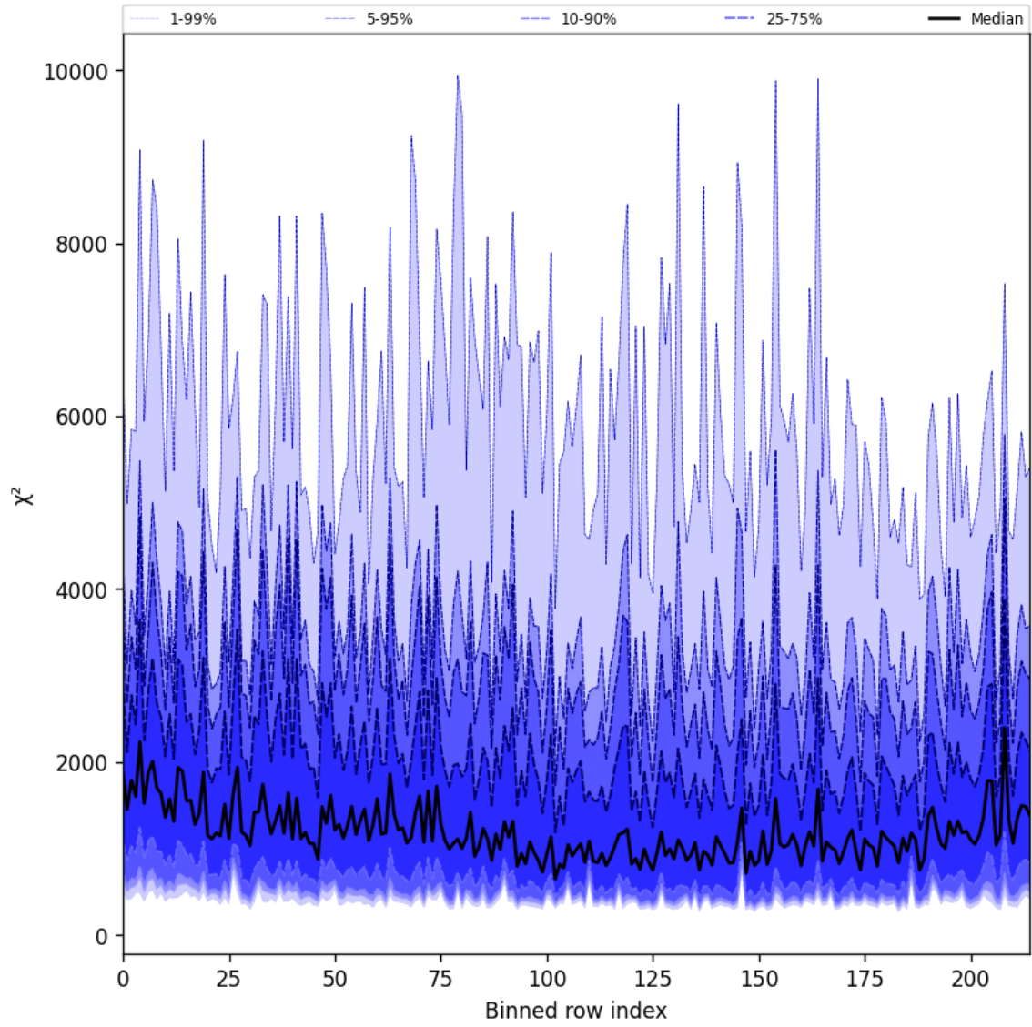
Figure 24: Along track statistics of “ \chi^2 ” for 2025-01-04 to 2025-01-04
