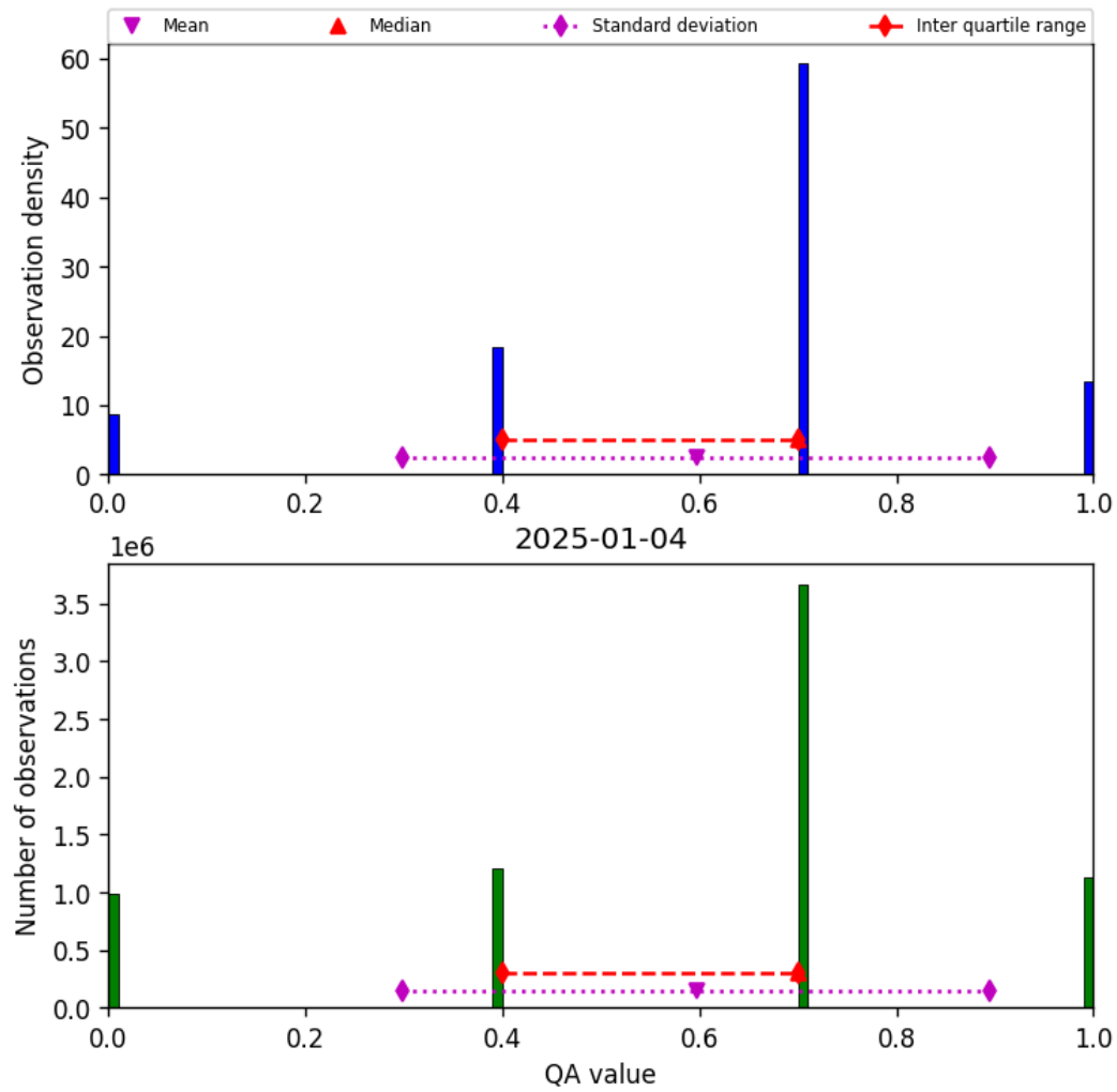
Figure 13: Histogram of “QA value” for 2025-01-04 to 2025-01-04
