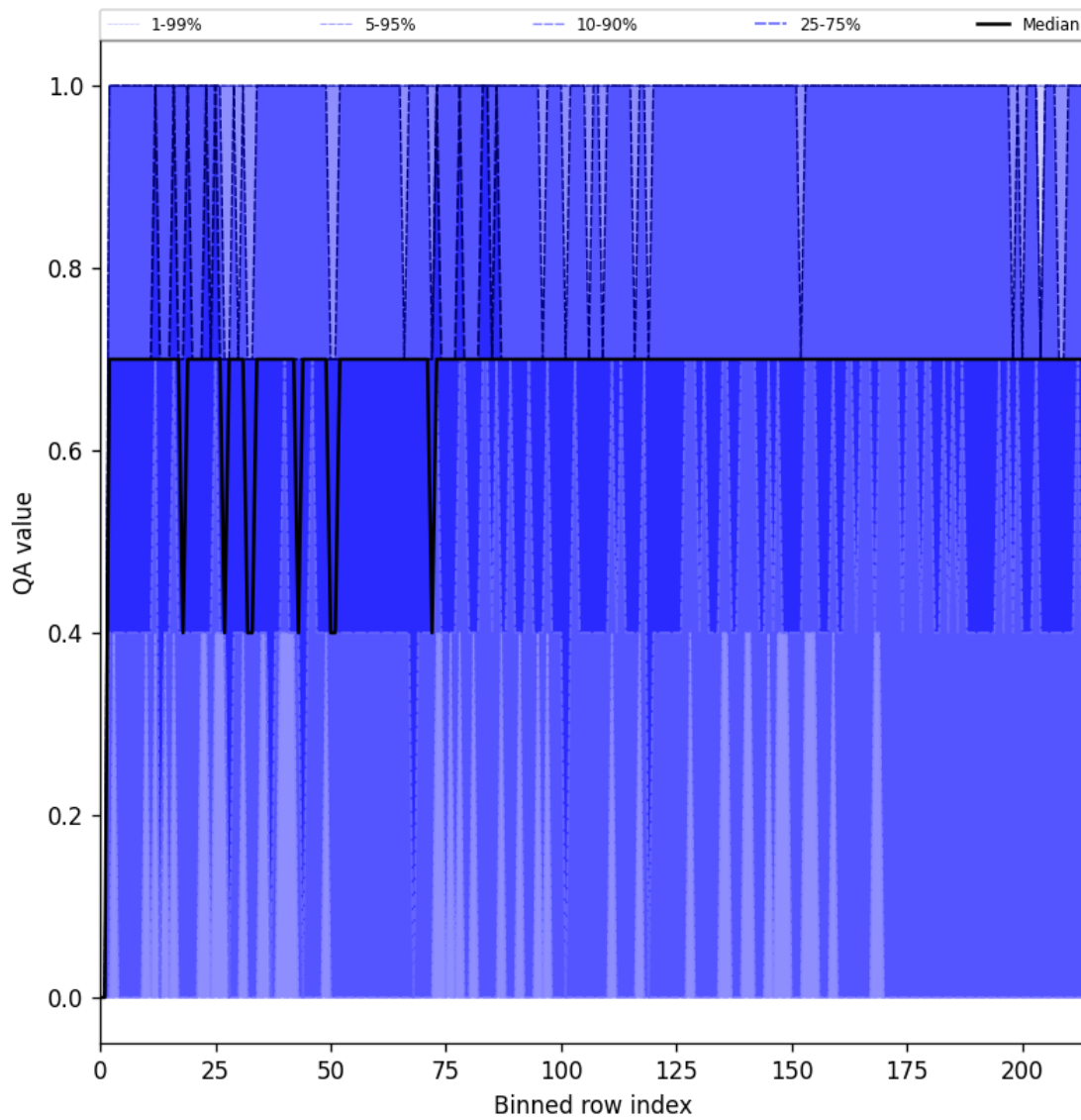
Figure 20: Along track statistics of “QA value” for 2025-01-04 to 2025-01-04
