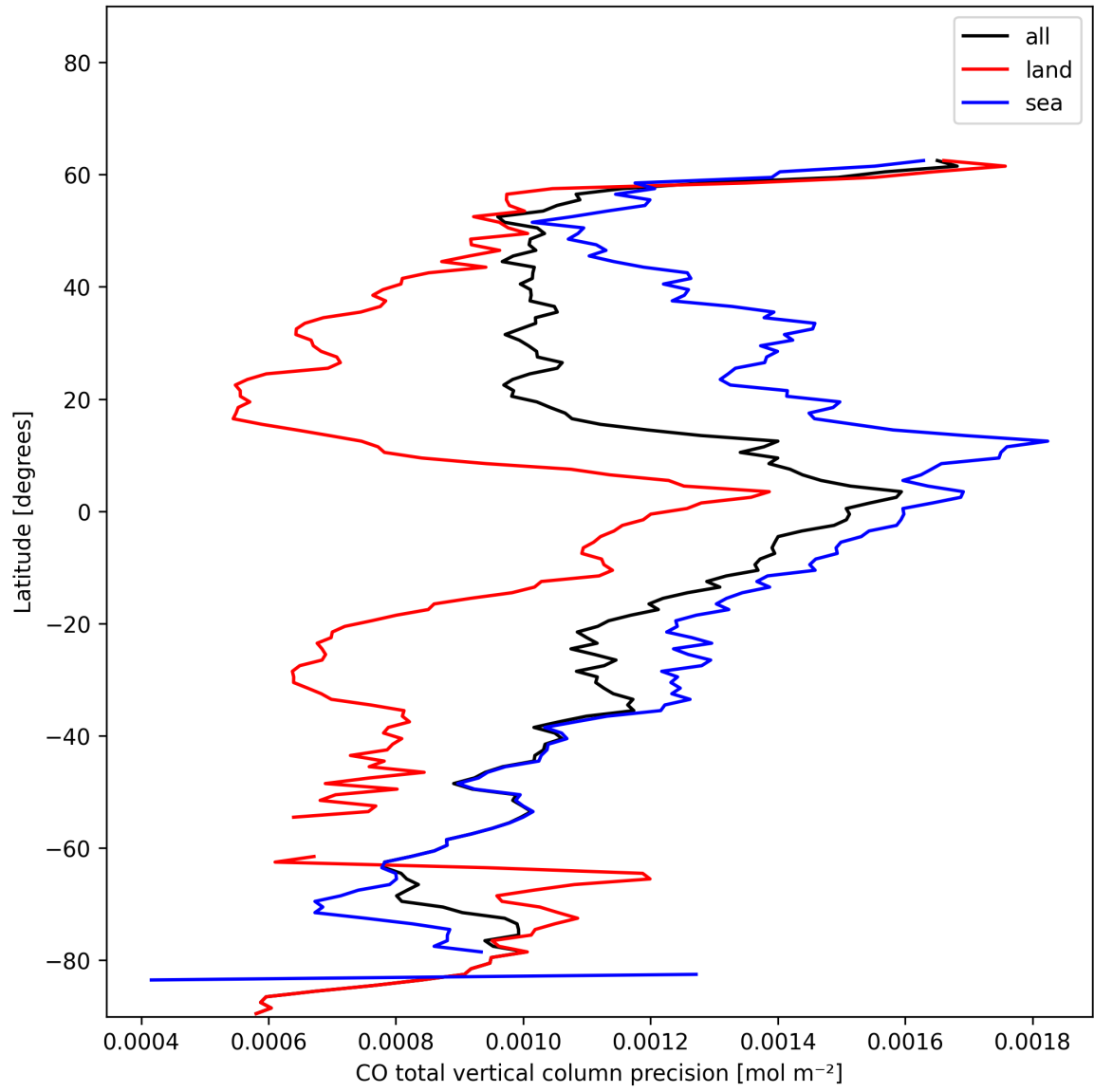
Figure 8: Zonal average of “CO total vertical column precision” for 2025-01-04 to 2025-01-04.
