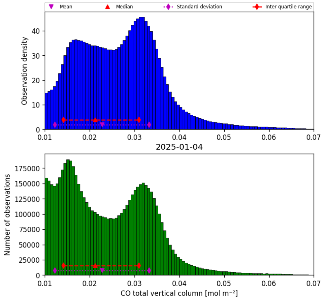
Figure 14: Histogram of “CO total vertical column” for 2025-01-04 to 2025-01-04
