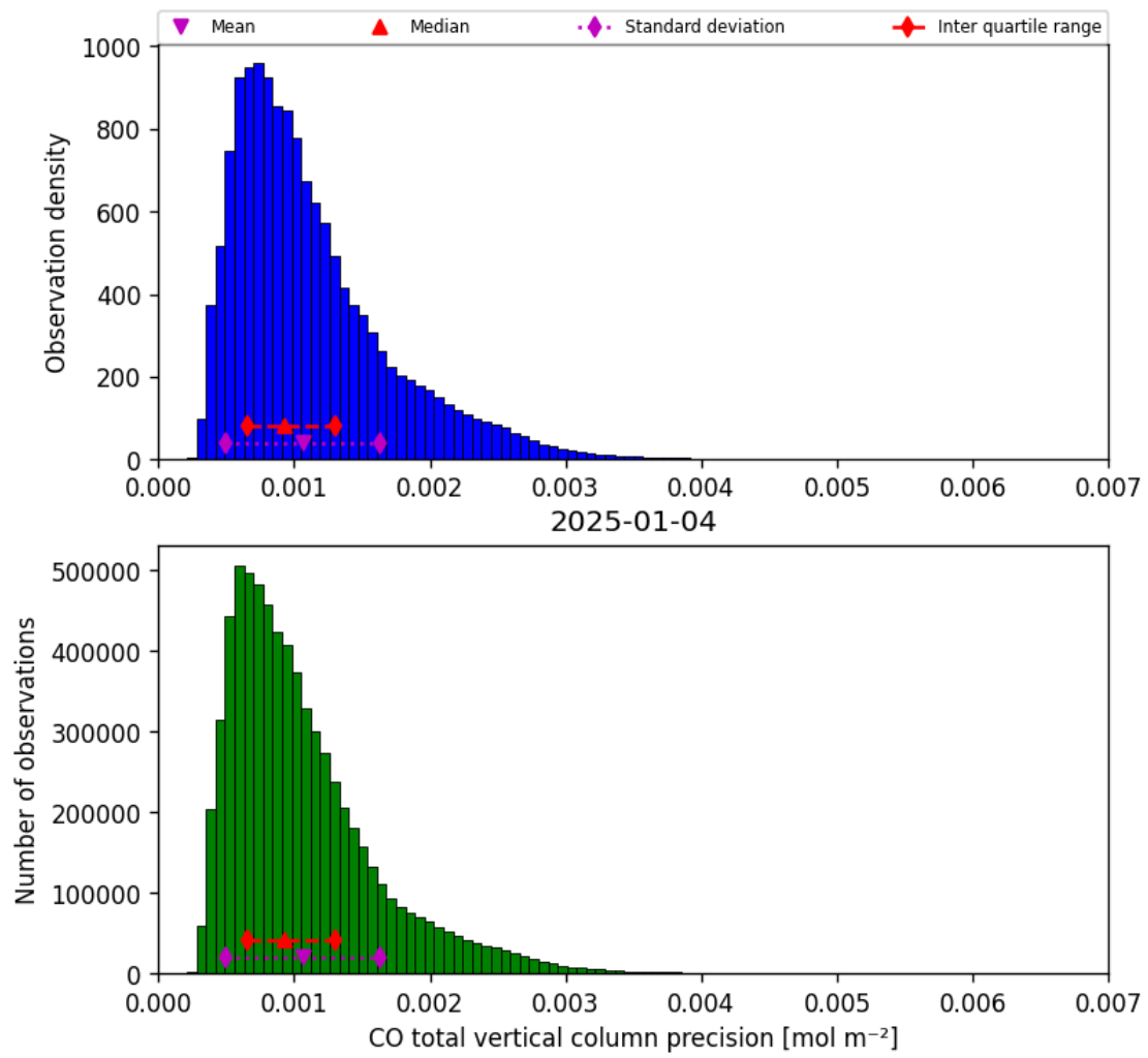
Figure 15: Histogram of “CO total vertical column precision” for 2025-01-04 to 2025-01-04
