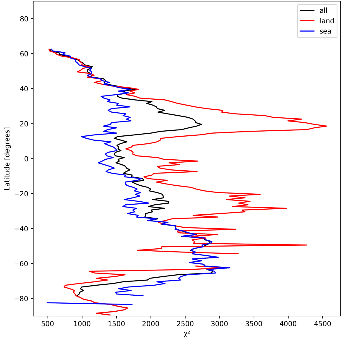
Figure 10: Zonal average of “ \chi^2 ” for 2025-01-04 to 2025-01-04.
