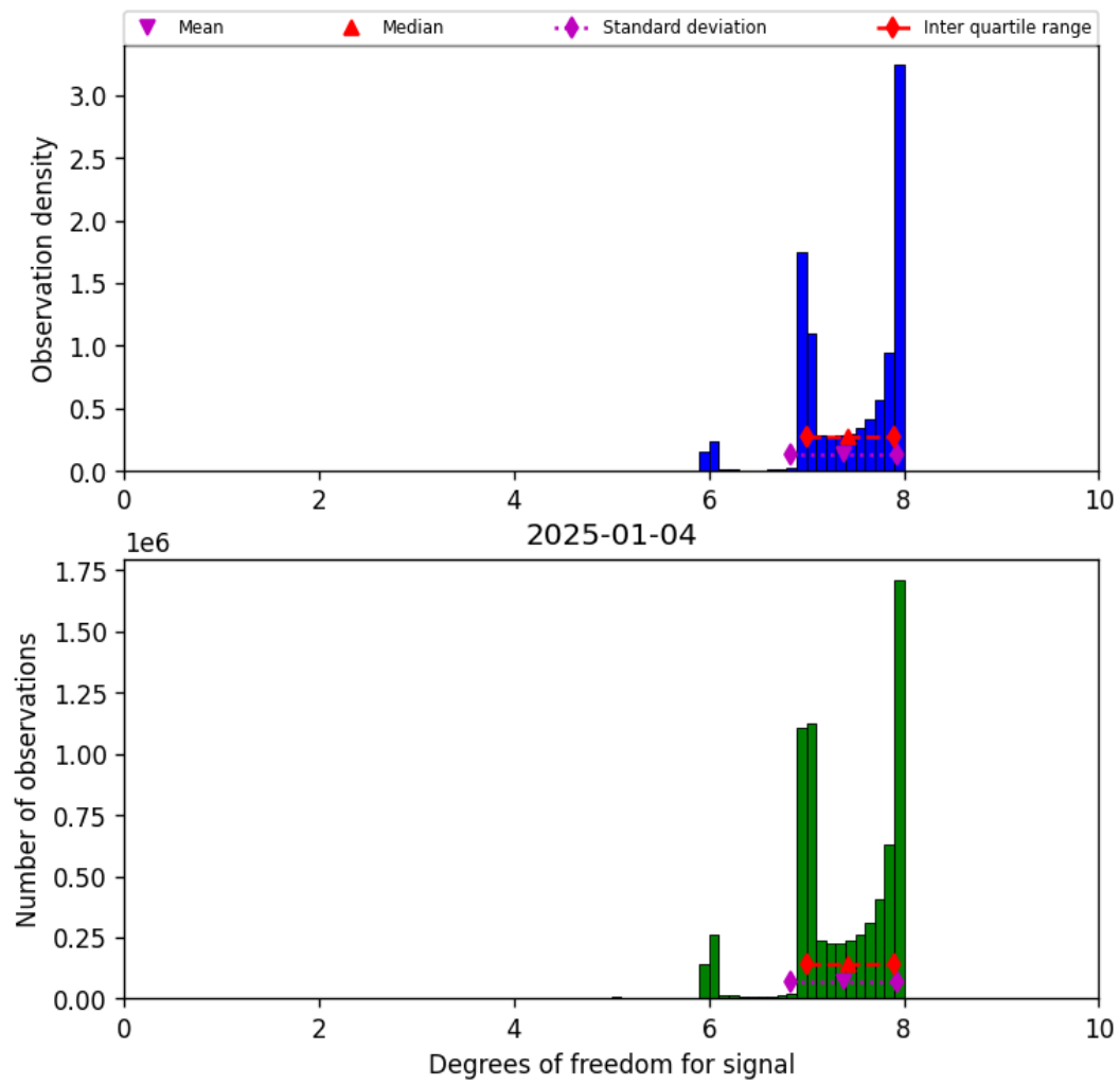
Figure 18: Histogram of “Degrees of freedom for signal” for 2025-01-04 to 2025-01-04
