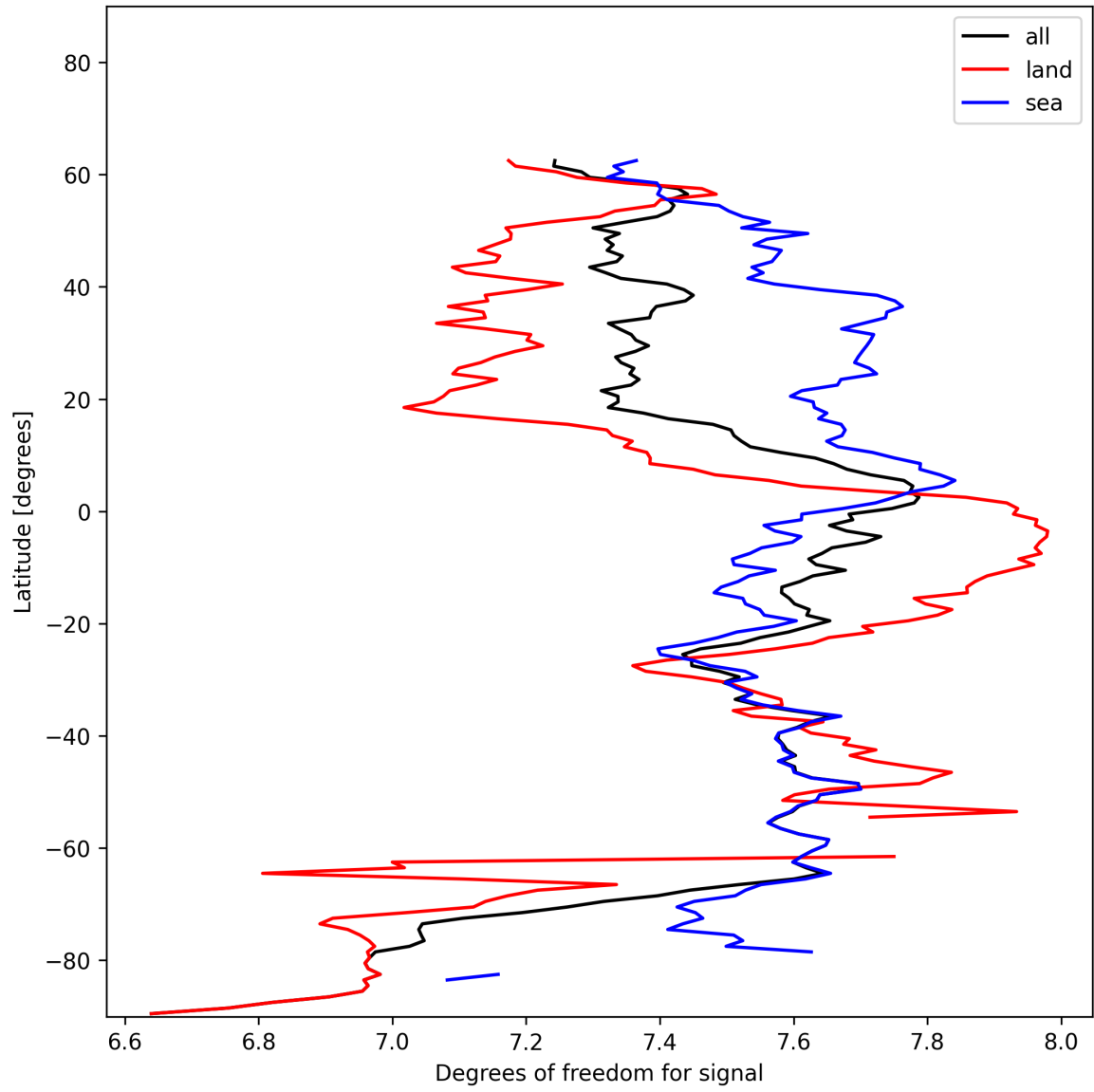
Figure 11: Zonal average of “Degrees of freedom for signal” for 2025-01-04 to 2025-01-04.
