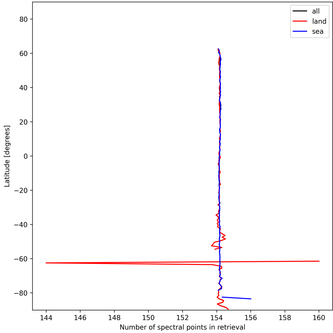
Figure 9: Zonal average of “Number of spectral points in retrieval” for 2025-01-04 to 2025-01-04.
