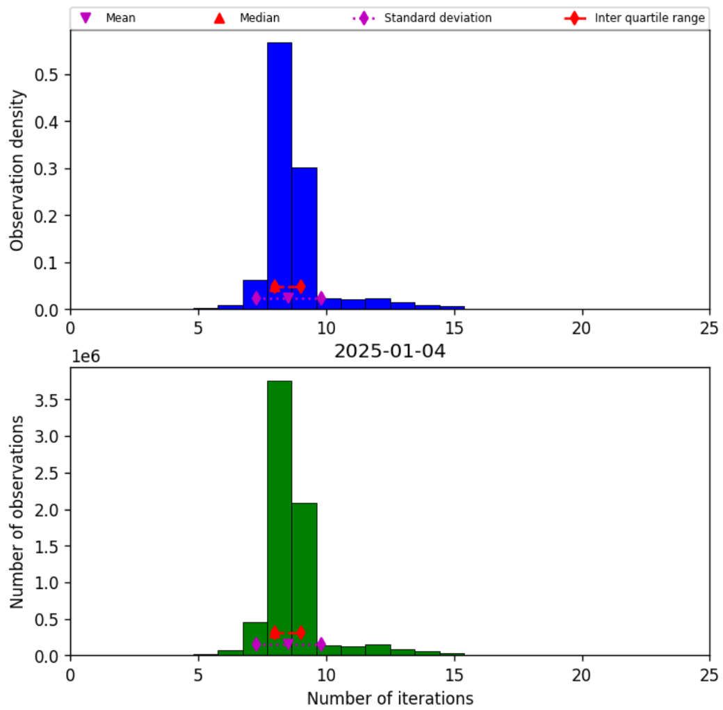
Figure 19: Histogram of “Number of iterations” for 2025-01-04 to 2025-01-04
