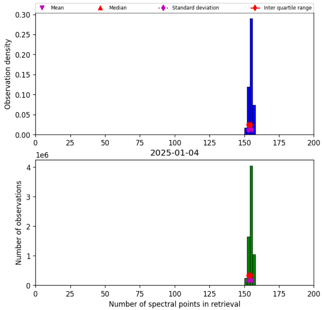
Figure 16: Histogram of “Number of spectral points in retrieval” for 2025-01-04 to 2025-01-04
