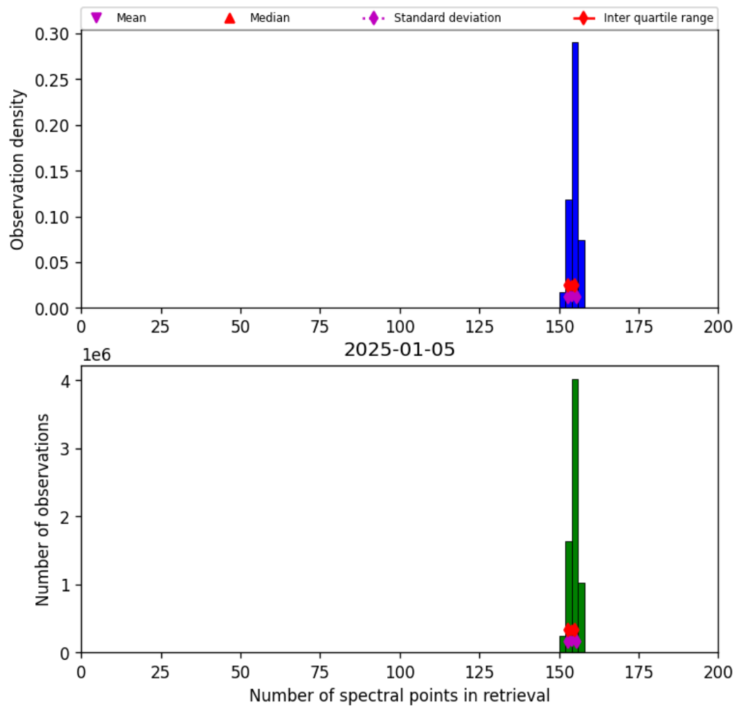
Figure 16: Histogram of “Number of spectral points in retrieval” for 2025-01-05 to 2025-01-05
