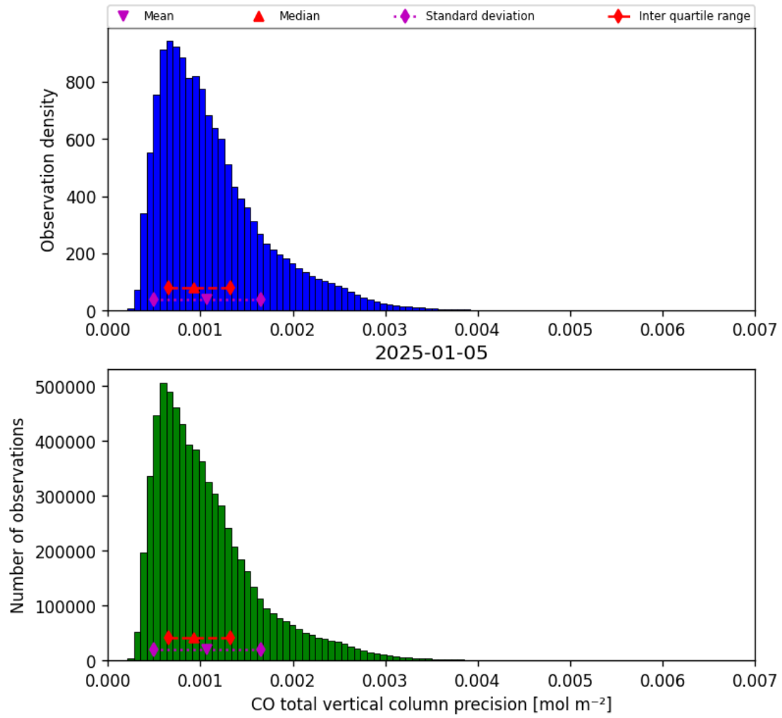
Figure 15: Histogram of “CO total vertical column precision” for 2025-01-05 to 2025-01-05
