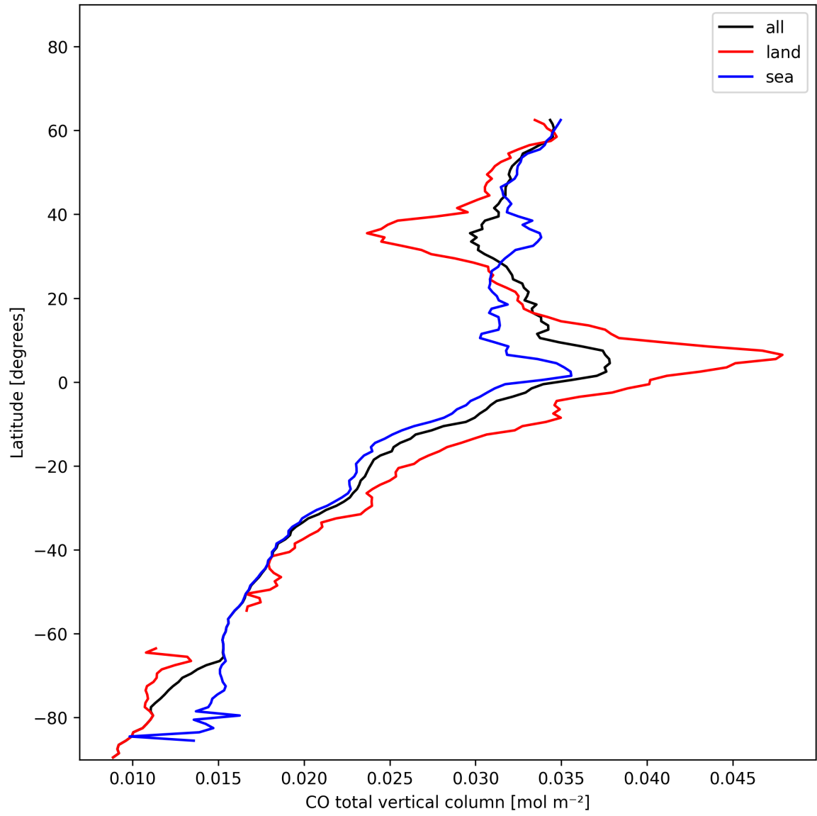
Figure 7: Zonal average of “CO total vertical column” for 2025-01-05 to 2025-01-05.
