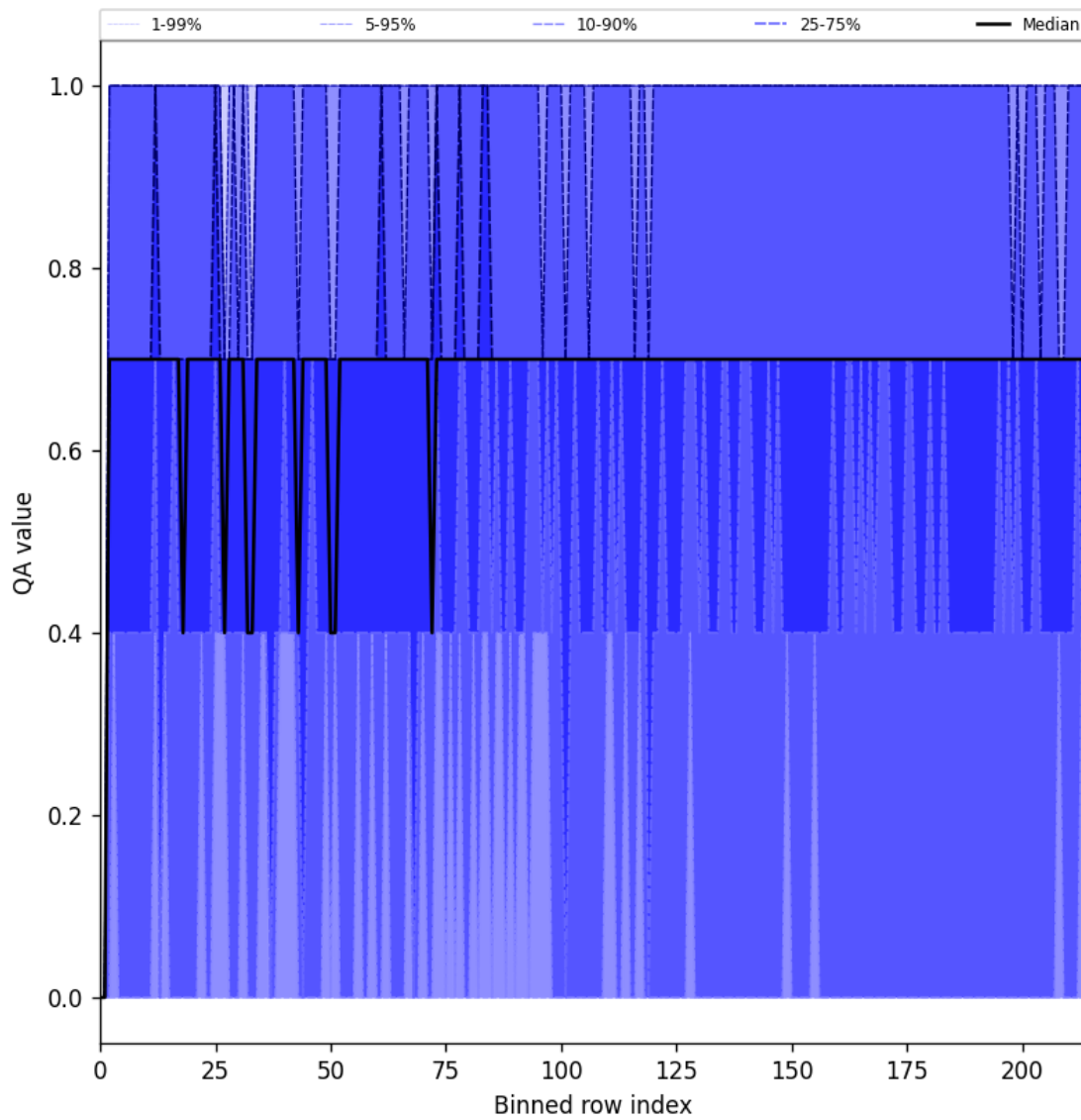
Figure 20: Along track statistics of “QA value” for 2025-01-05 to 2025-01-05
