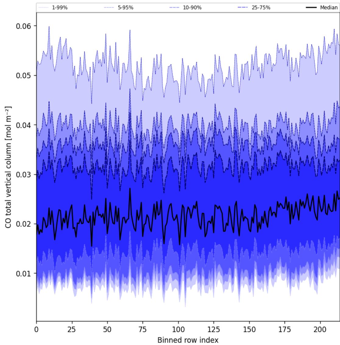
Figure 21: Along track statistics of “CO total vertical column” for 2025-01-05 to 2025-01-05
