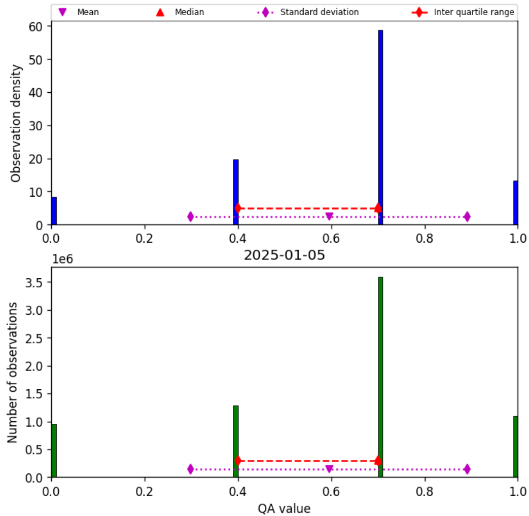
Figure 13: Histogram of “QA value” for 2025-01-05 to 2025-01-05
