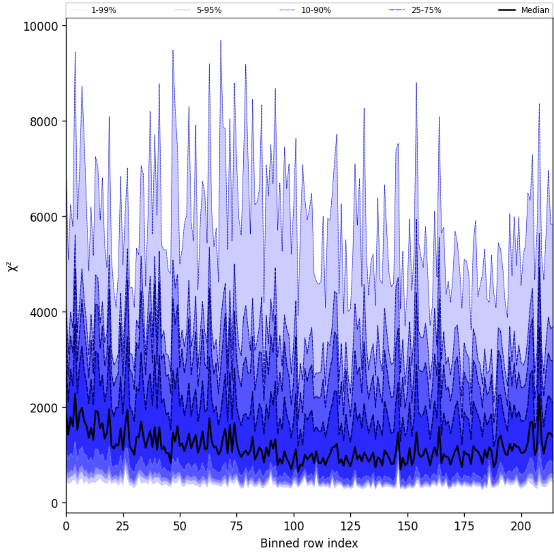
Figure 24: Along track statistics of “ \chi^2 ” for 2025-01-05 to 2025-01-05
