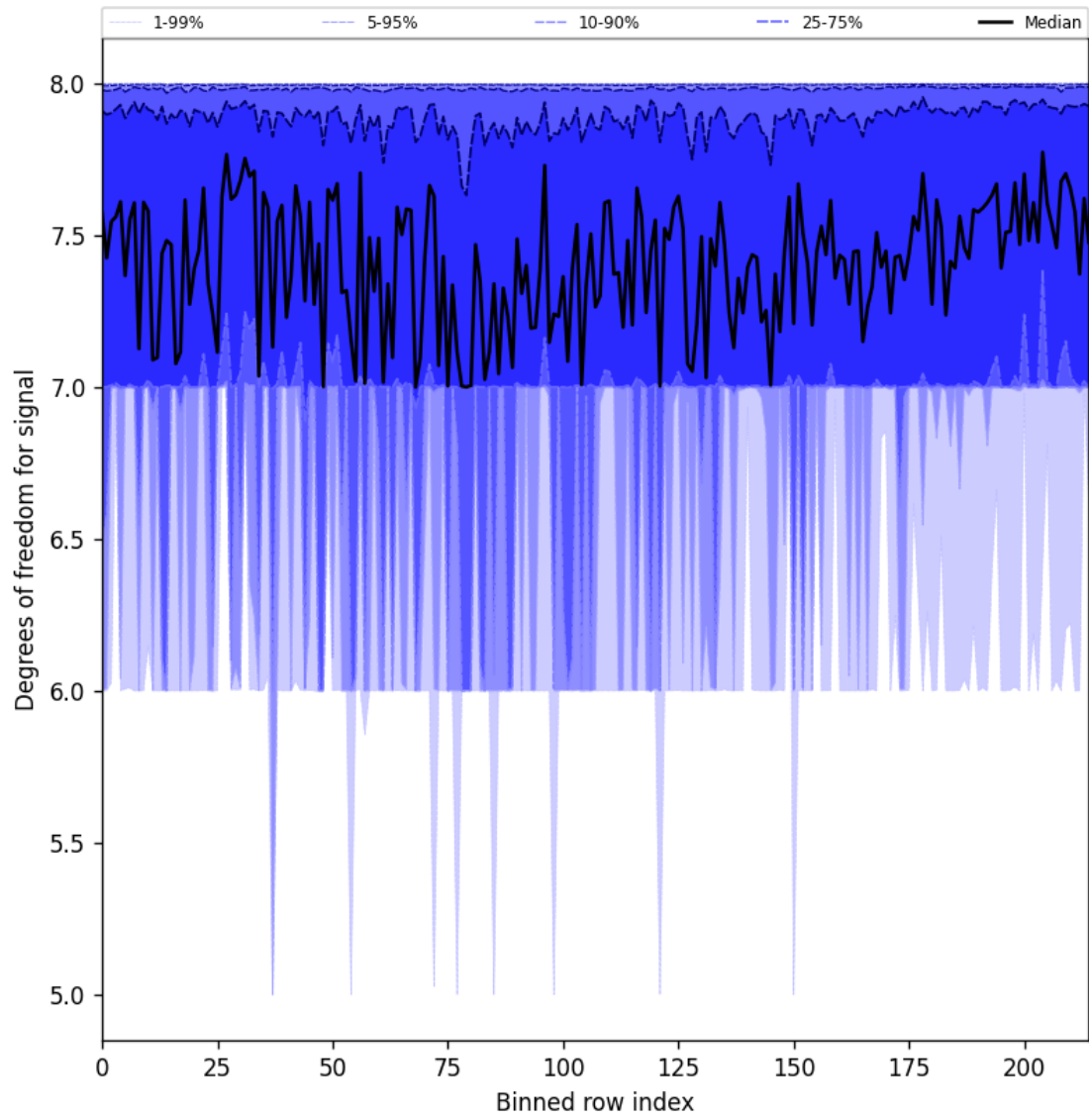
Figure 25: Along track statistics of “Degrees of freedom for signal” for 2025-01-05 to 2025-01-05
