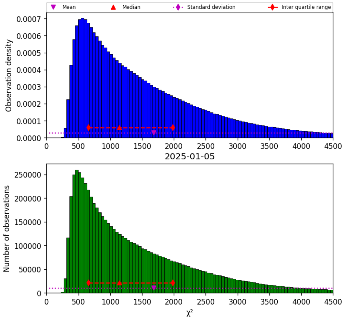
Figure 17: Histogram of " \chi^2 " for 2025-01-05 to 2025-01-05
