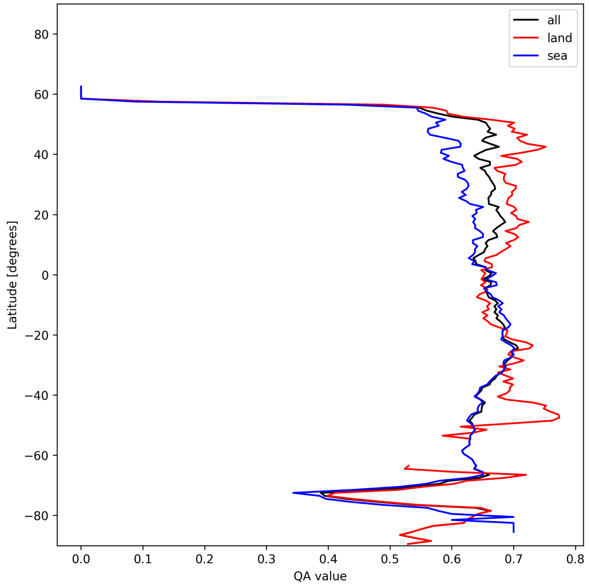
Figure 6: Zonal average of “QA value” for 2025-01-05 to 2025-01-05.
