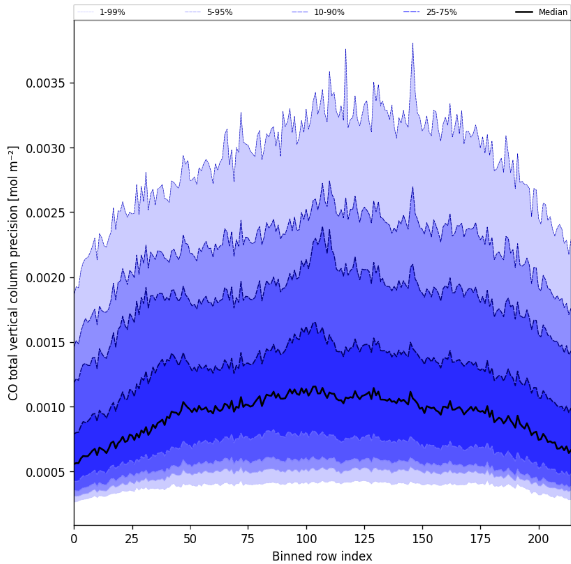
Figure 22: Along track statistics of “CO total vertical column precision” for 2025-01-05 to 2025-01-05
