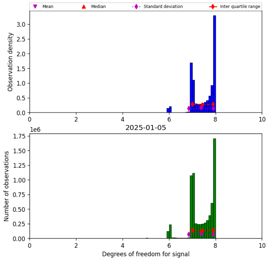
Figure 18: Histogram of “Degrees of freedom for signal” for 2025-01-05 to 2025-01-05
