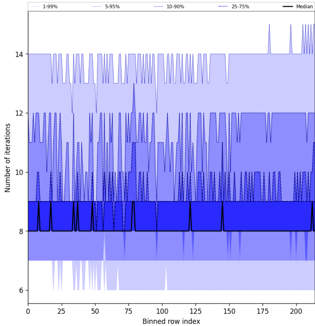
Figure 26: Along track statistics of “Number of iterations” for 2025-01-05 to 2025-01-05
