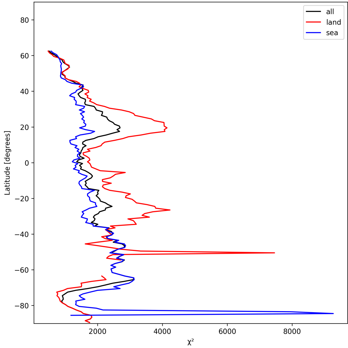
Figure 10: Zonal average of “ \chi^2 ” for 2025-01-05 to 2025-01-05.
