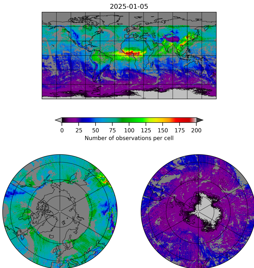
Figure 5: Map of the number of observations for 2025-01-05 to 2025-01-05
