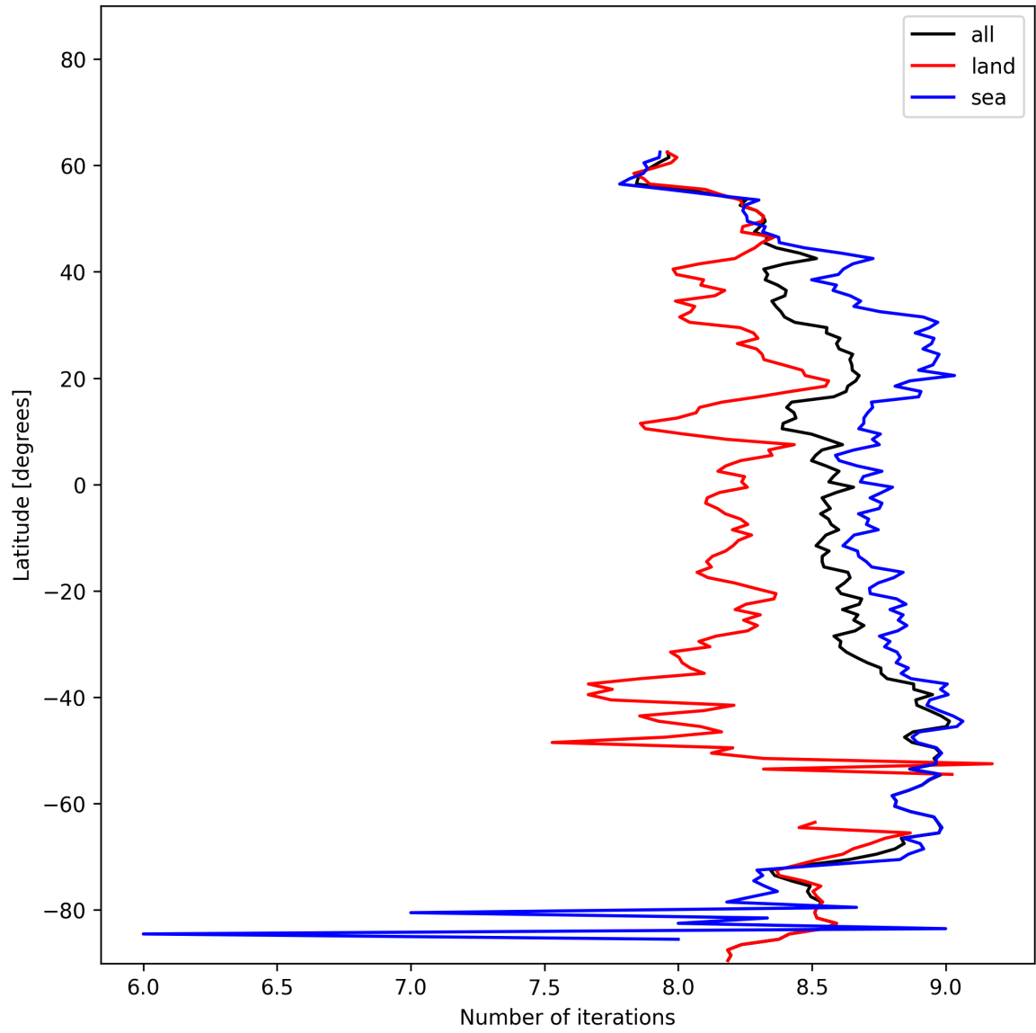
Figure 12: Zonal average of “Number of iterations” for 2025-01-05 to 2025-01-05.
