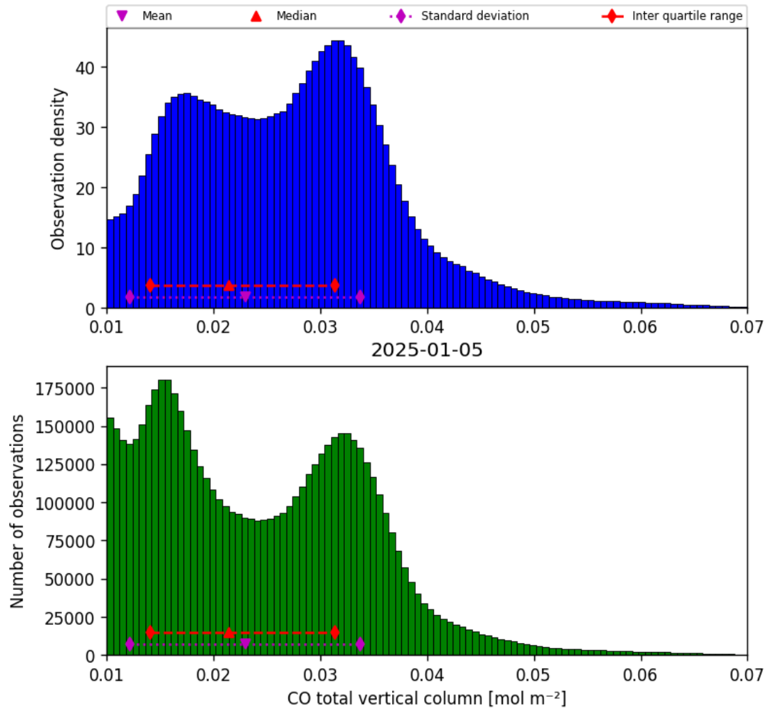
Figure 14: Histogram of “CO total vertical column” for 2025-01-05 to 2025-01-05
