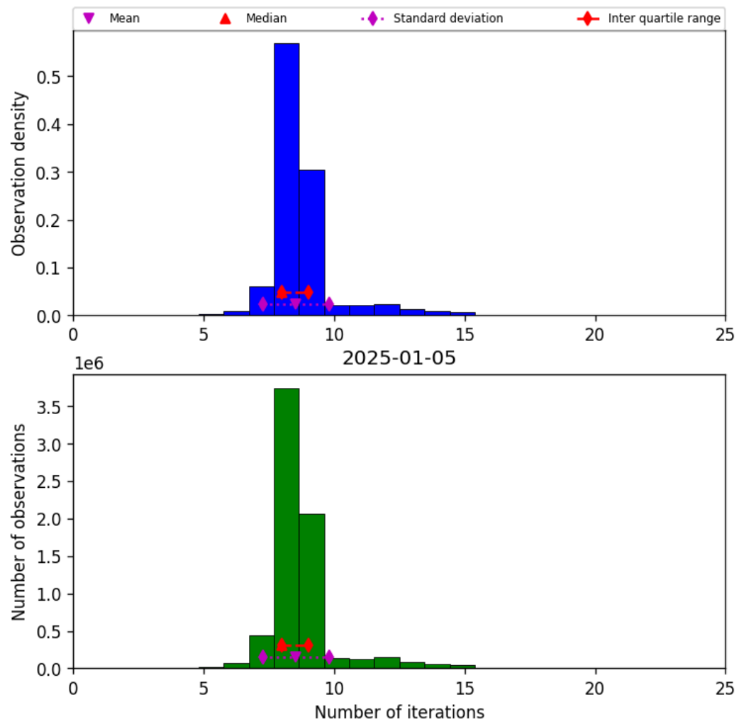
Figure 19: Histogram of “Number of iterations” for 2025-01-05 to 2025-01-05
