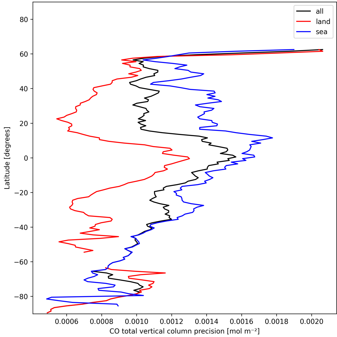
Figure 8: Zonal average of “CO total vertical column precision” for 2025-01-05 to 2025-01-05.
