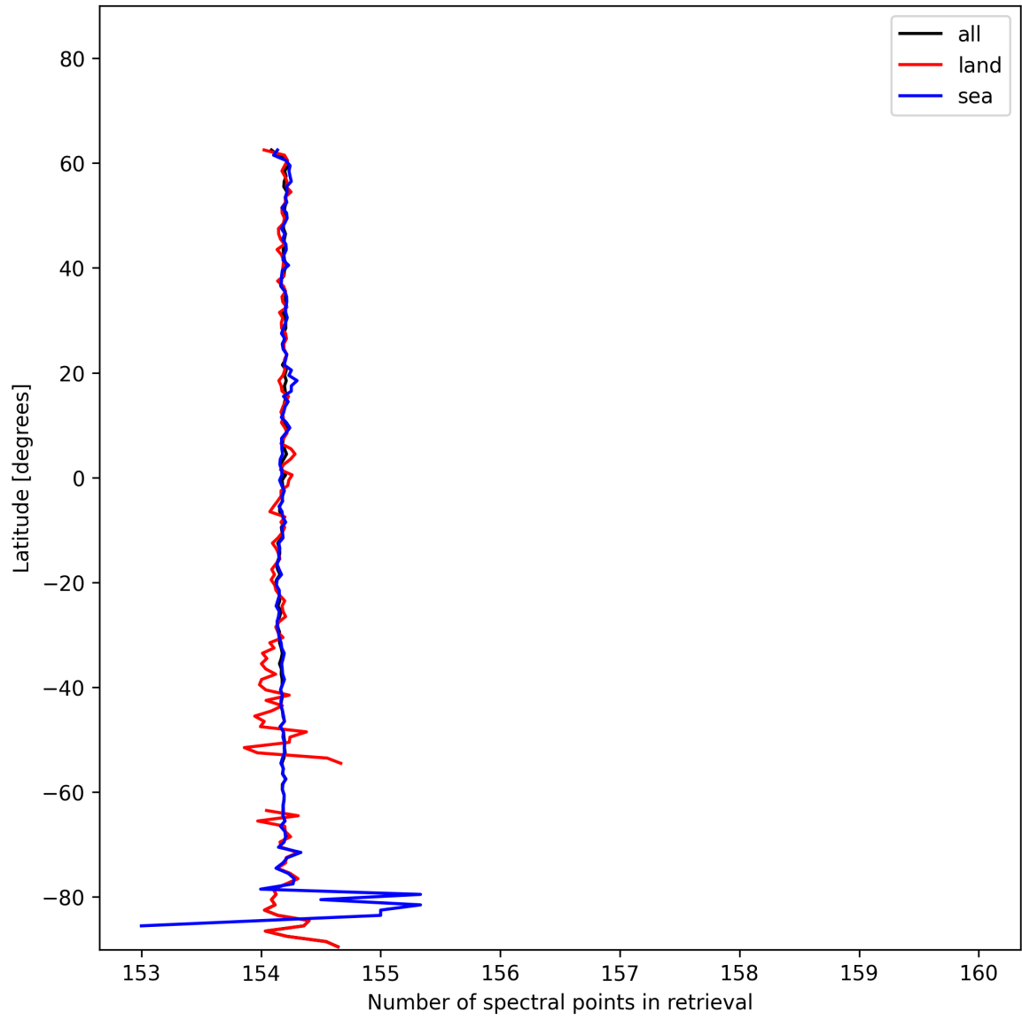
Figure 9: Zonal average of “Number of spectral points in retrieval” for 2025-01-05 to 2025-01-05.
