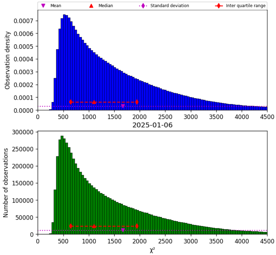
Figure 17: Histogram of " \chi^2 " for 2025-01-06 to 2025-01-07
