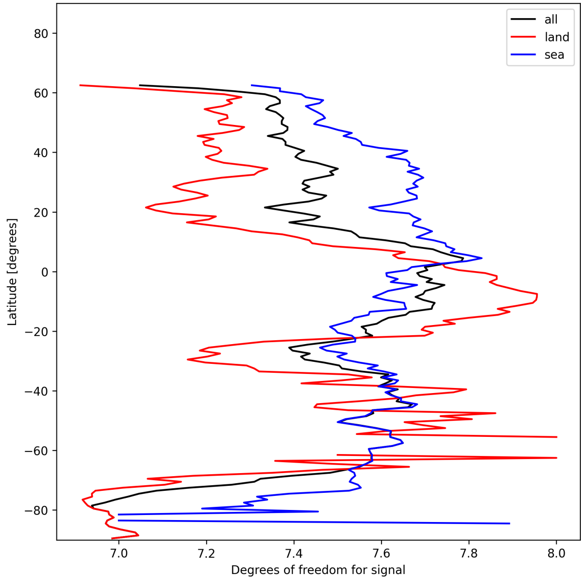
Figure 11: Zonal average of “Degrees of freedom for signal” for 2025-01-06 to 2025-01-07.
