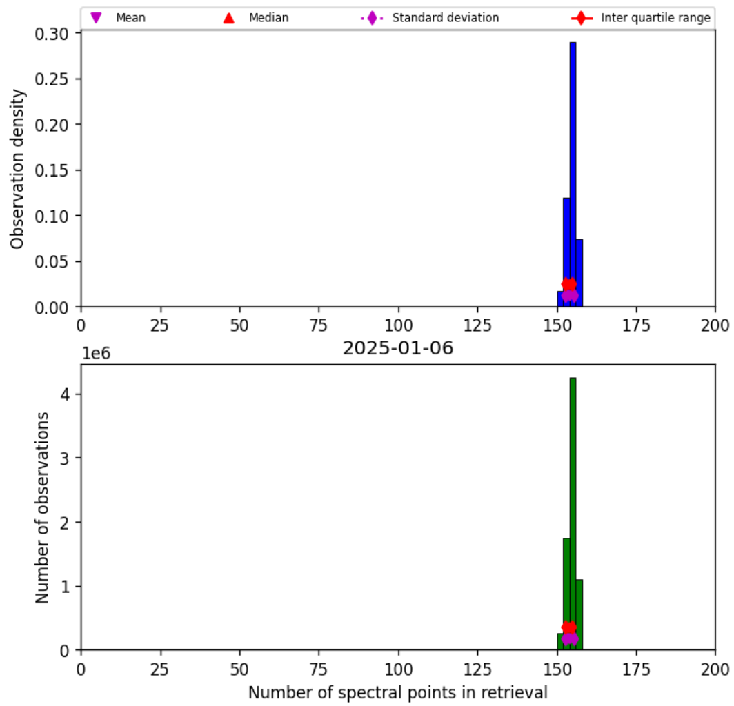
Figure 16: Histogram of “Number of spectral points in retrieval” for 2025-01-06 to 2025-01-07
