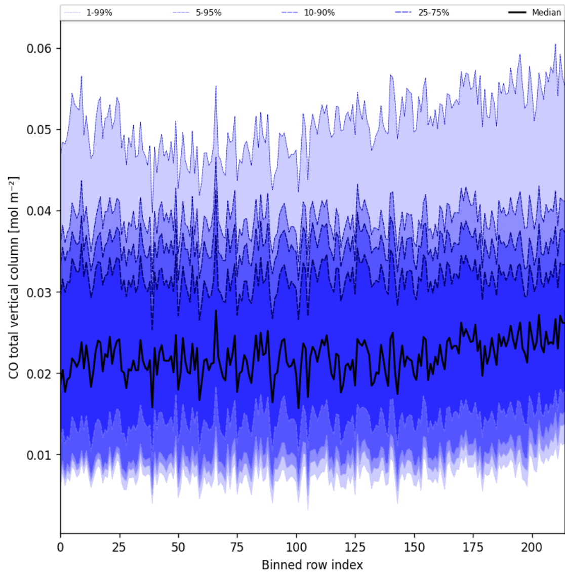
Figure 21: Along track statistics of “CO total vertical column” for 2025-01-06 to 2025-01-07
