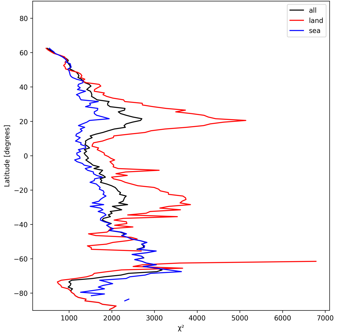
Figure 10: Zonal average of “ \chi^2 ” for 2025-01-06 to 2025-01-07.
