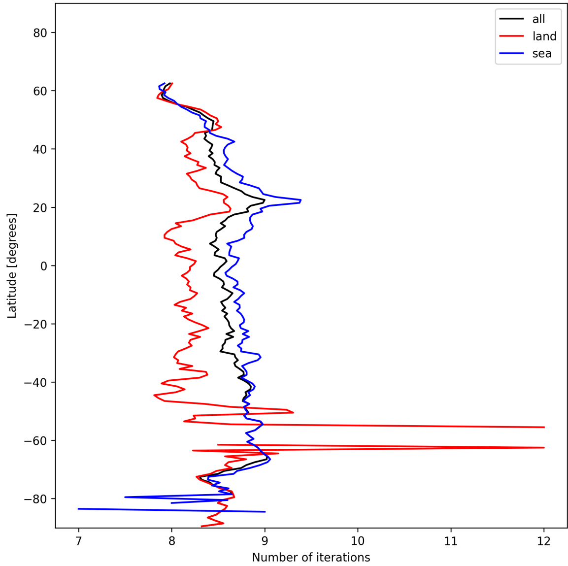
Figure 12: Zonal average of “Number of iterations” for 2025-01-06 to 2025-01-07.
