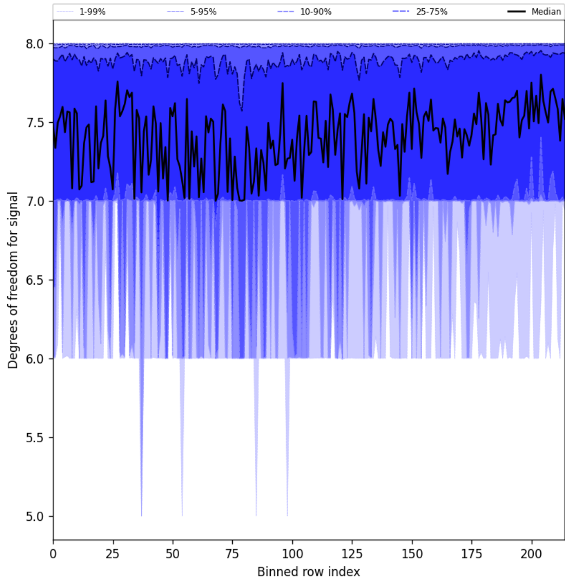
Figure 25: Along track statistics of “Degrees of freedom for signal” for 2025-01-06 to 2025-01-07
