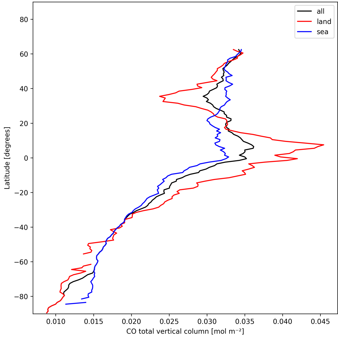
Figure 7: Zonal average of “CO total vertical column” for 2025-01-06 to 2025-01-07.
