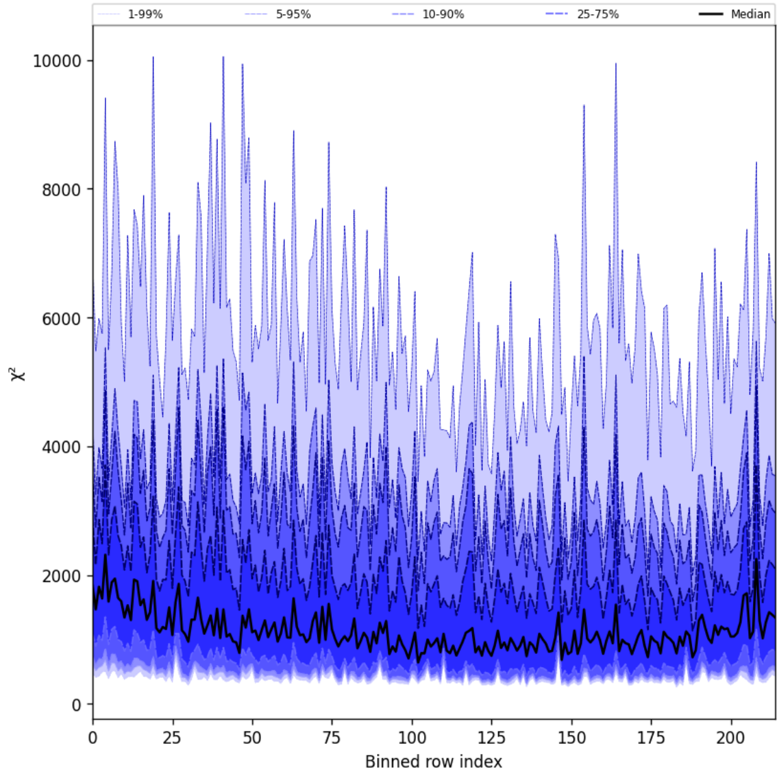
Figure 24: Along track statistics of “ \chi^2 ” for 2025-01-06 to 2025-01-07
