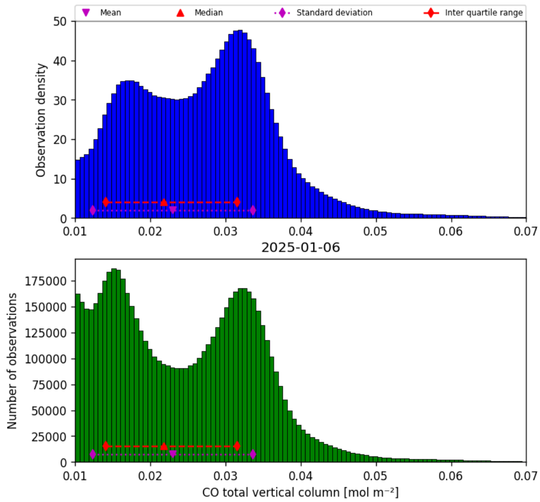
Figure 14: Histogram of “CO total vertical column” for 2025-01-06 to 2025-01-07
