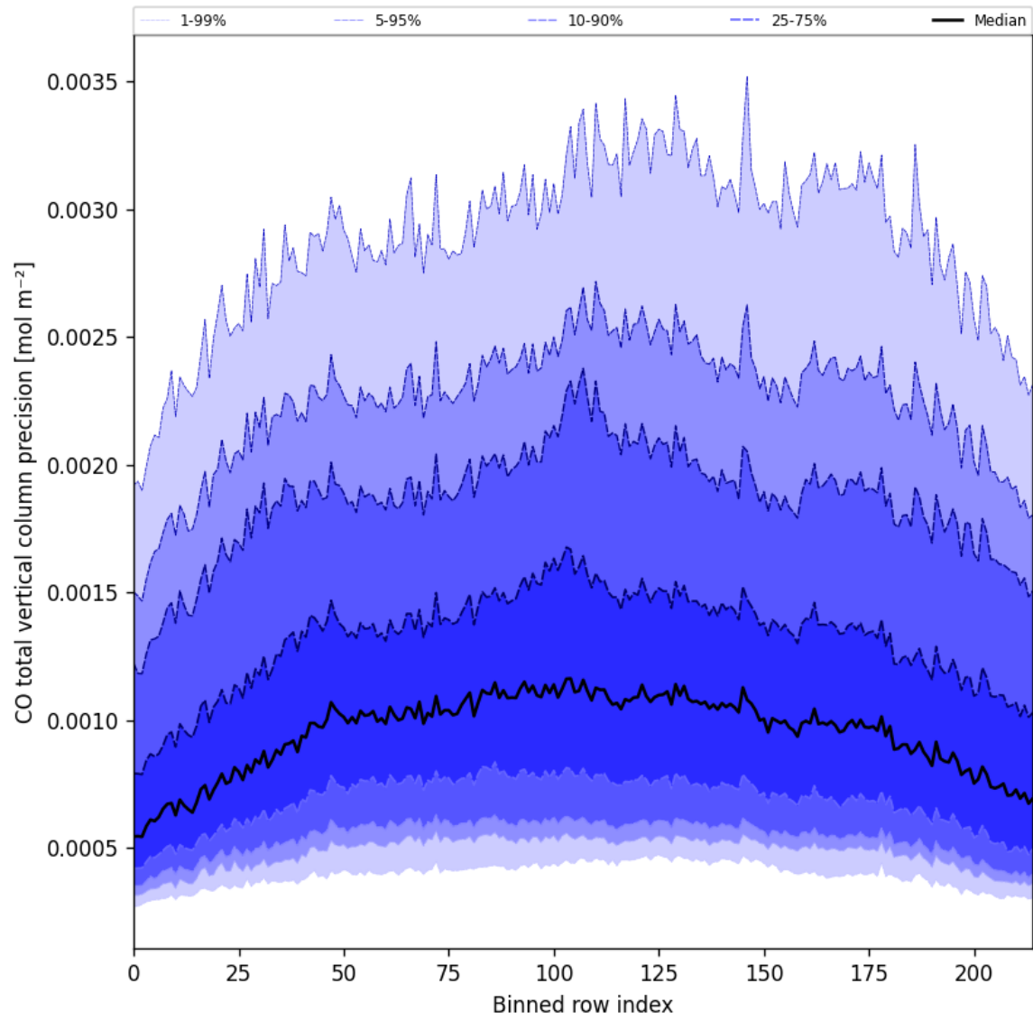
Figure 22: Along track statistics of “CO total vertical column precision” for 2025-01-06 to 2025-01-07
