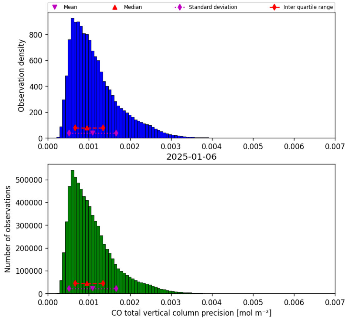
Figure 15: Histogram of “CO total vertical column precision” for 2025-01-06 to 2025-01-07
