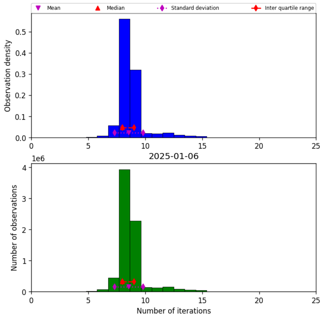
Figure 19: Histogram of “Number of iterations” for 2025-01-06 to 2025-01-07
