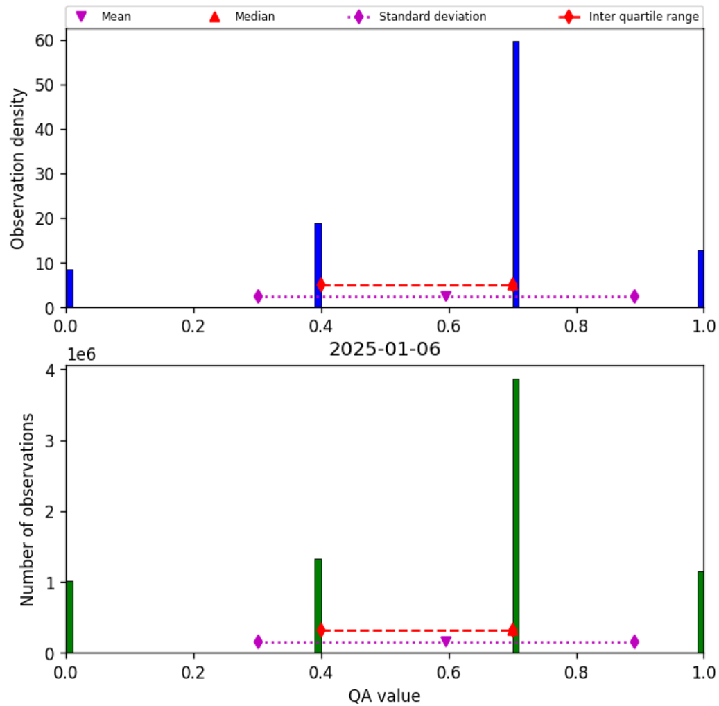
Figure 13: Histogram of “QA value” for 2025-01-06 to 2025-01-07
