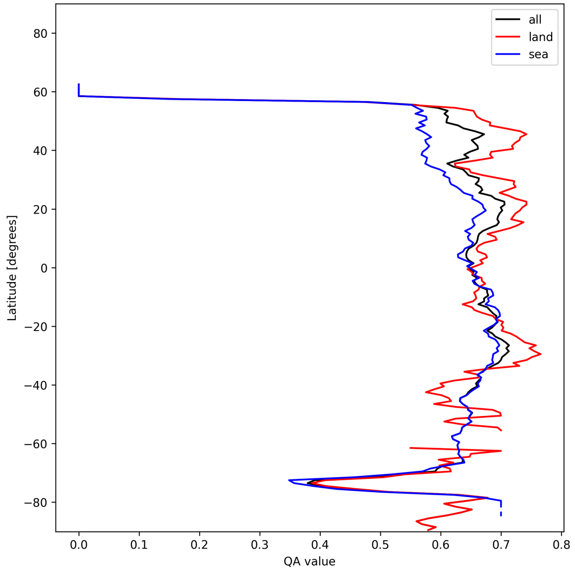
Figure 6: Zonal average of “QA value” for 2025-01-06 to 2025-01-07.
