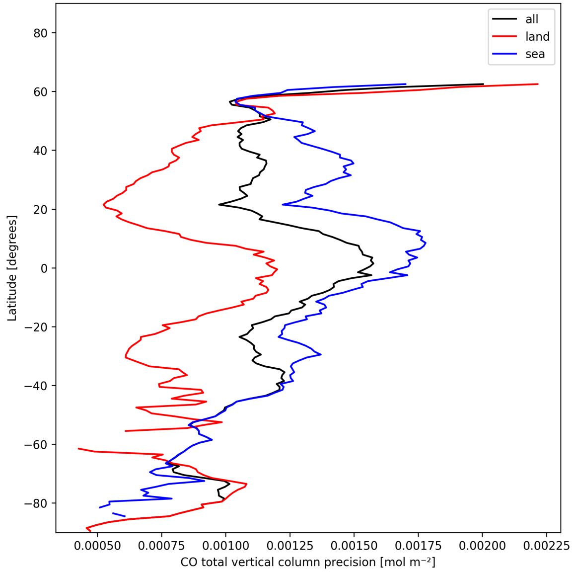
Figure 8: Zonal average of “CO total vertical column precision” for 2025-01-06 to 2025-01-07.
