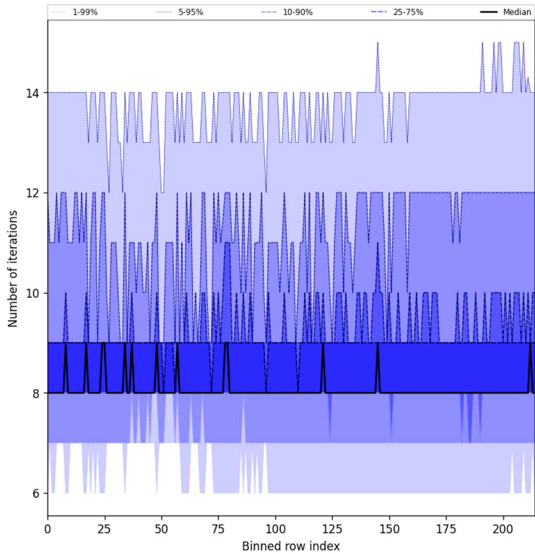
Figure 26: Along track statistics of “Number of iterations” for 2025-01-06 to 2025-01-07
