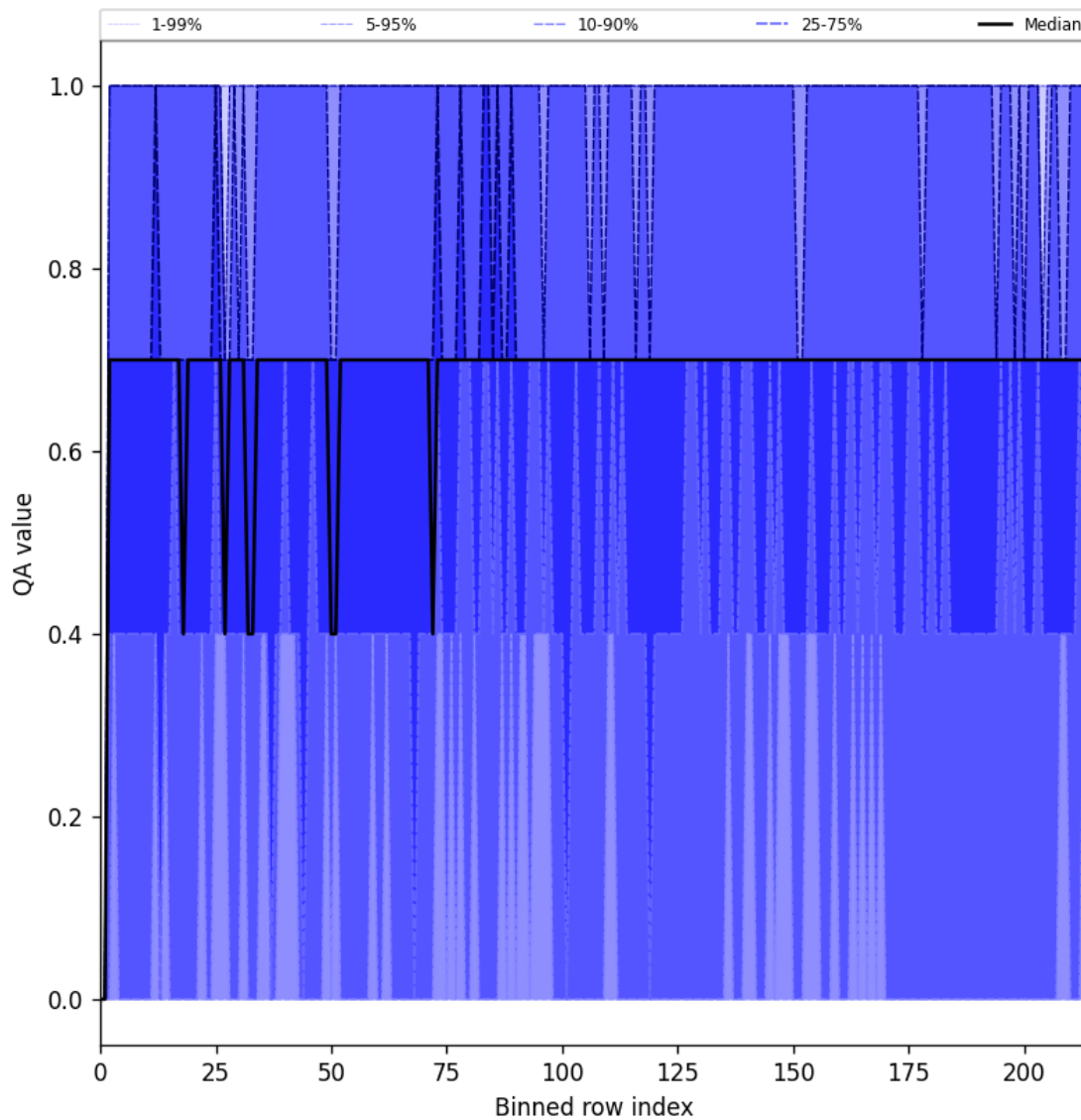
Figure 20: Along track statistics of “QA value” for 2025-01-06 to 2025-01-07
