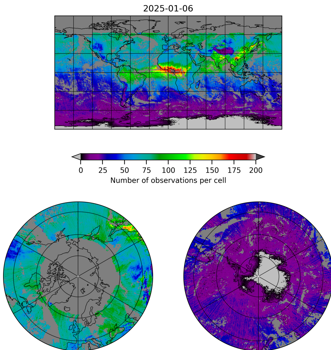
Figure 5: Map of the number of observations for 2025-01-06 to 2025-01-07
