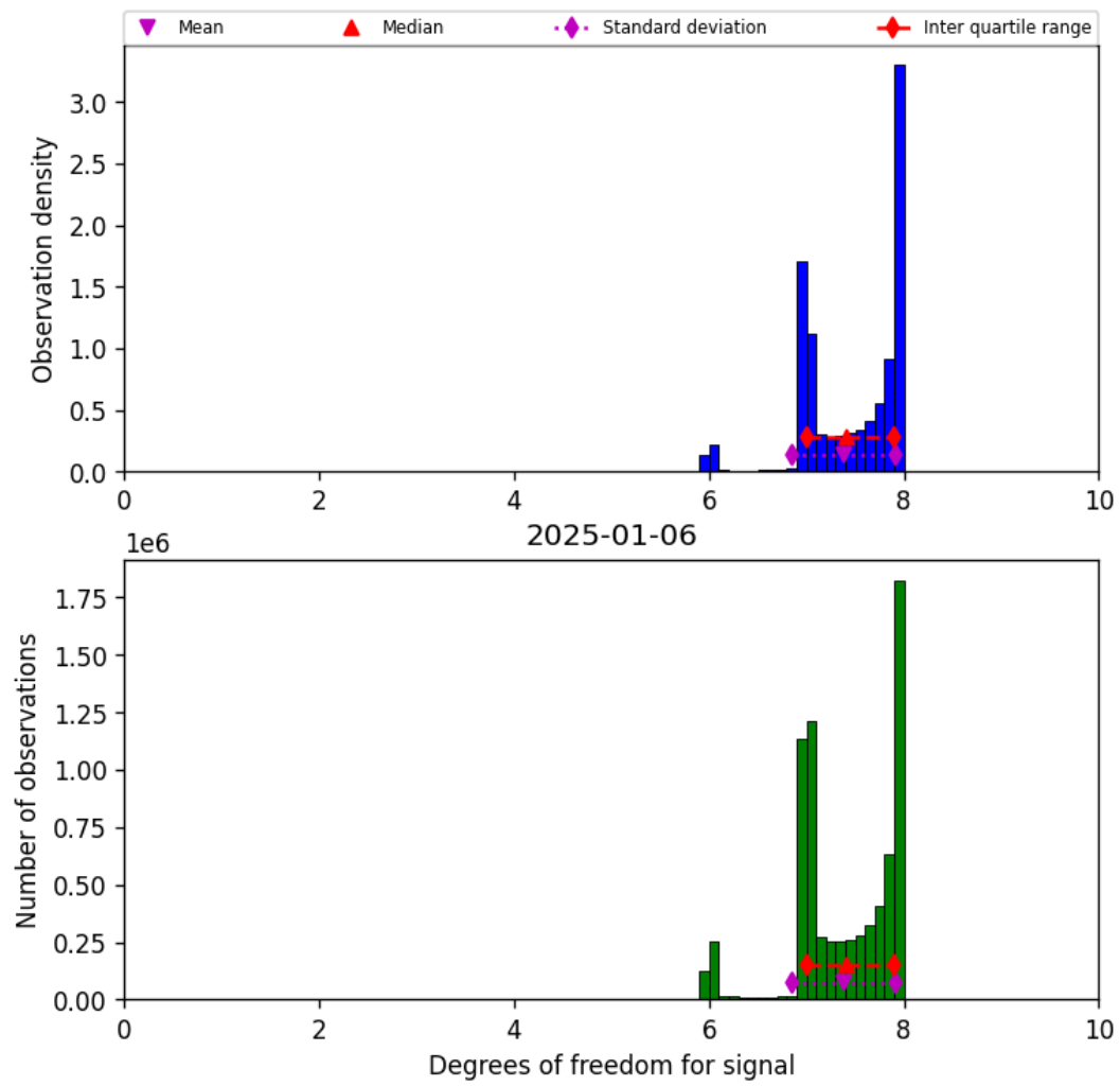
Figure 18: Histogram of “Degrees of freedom for signal” for 2025-01-06 to 2025-01-07
