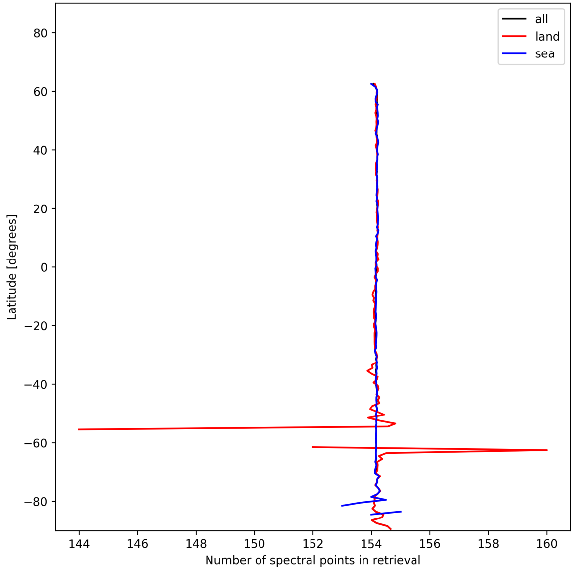
Figure 9: Zonal average of “Number of spectral points in retrieval” for 2025-01-06 to 2025-01-07.
