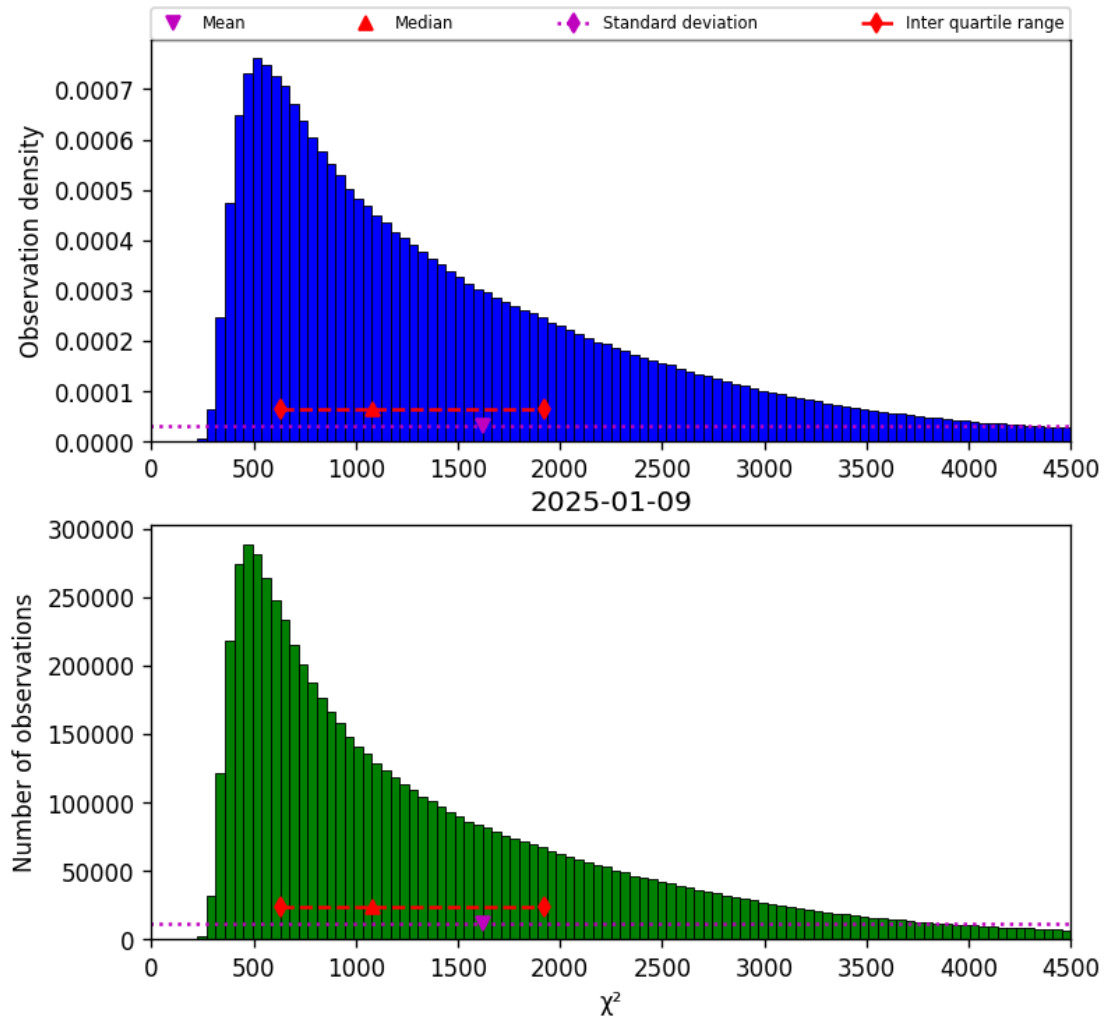
Figure 17: Histogram of " \chi^2 " for 2025-01-09 to 2025-01-10
