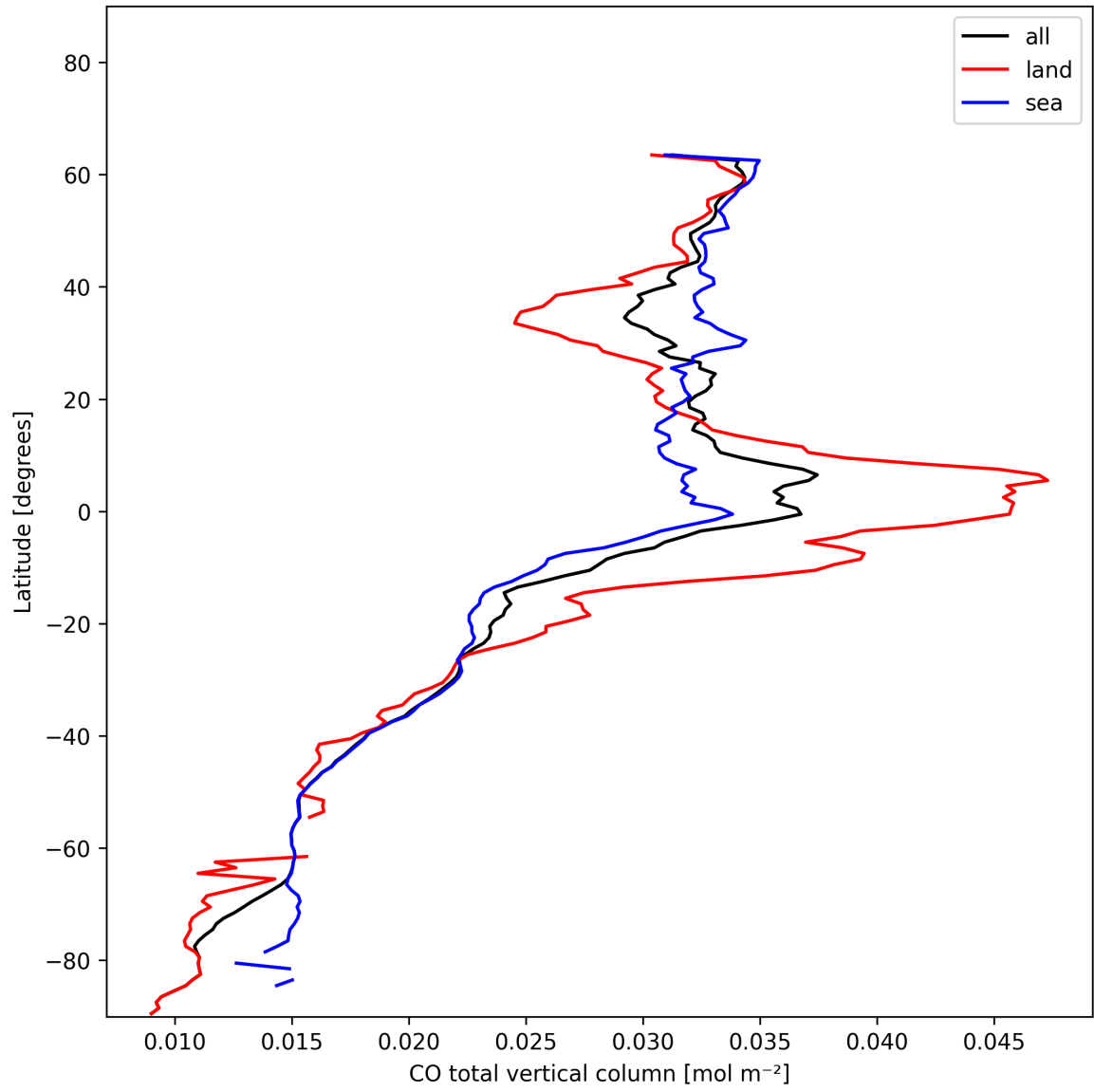
Figure 7: Zonal average of “CO total vertical column” for 2025-01-09 to 2025-01-10.
