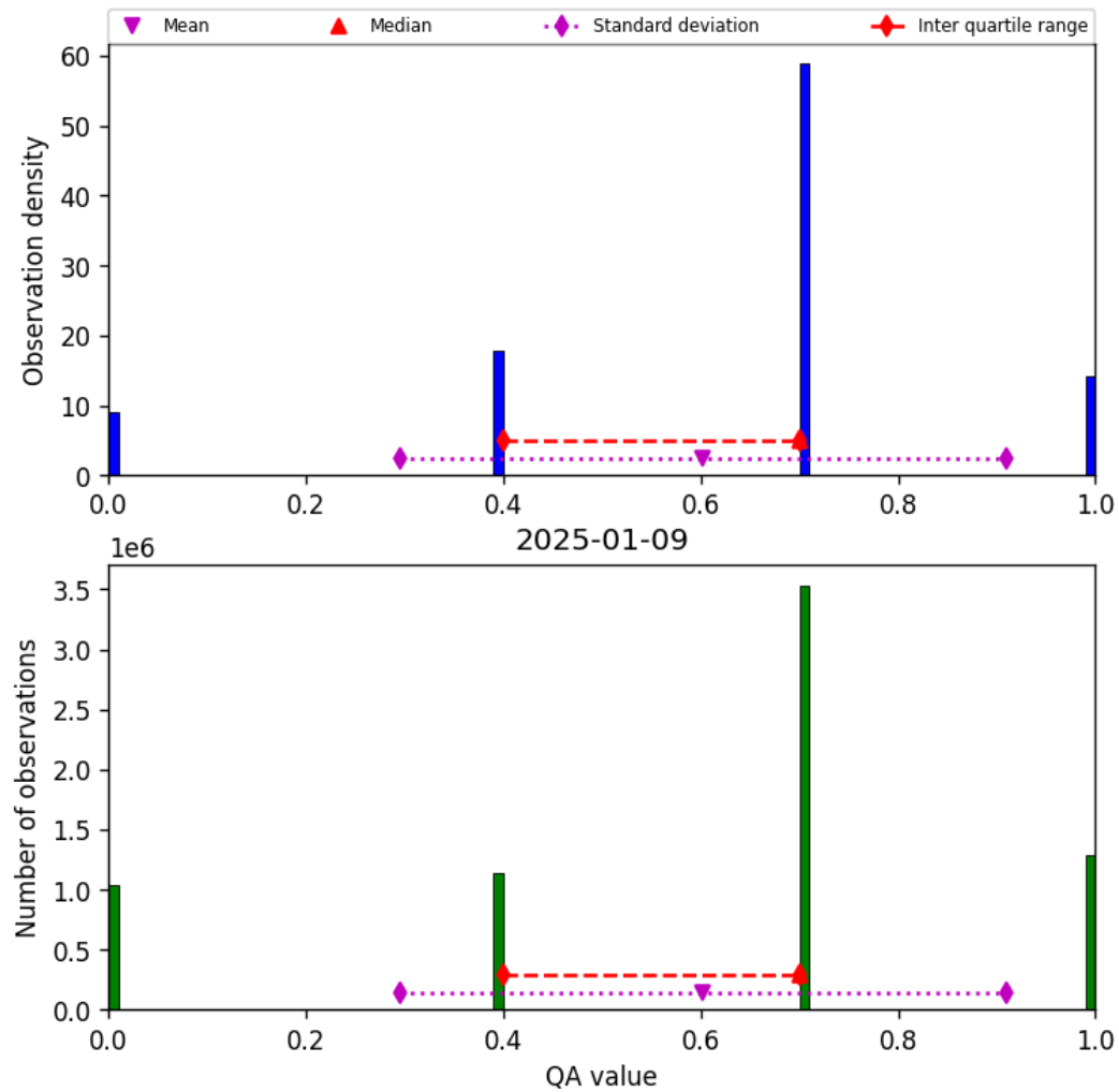
Figure 13: Histogram of “QA value” for 2025-01-09 to 2025-01-10
