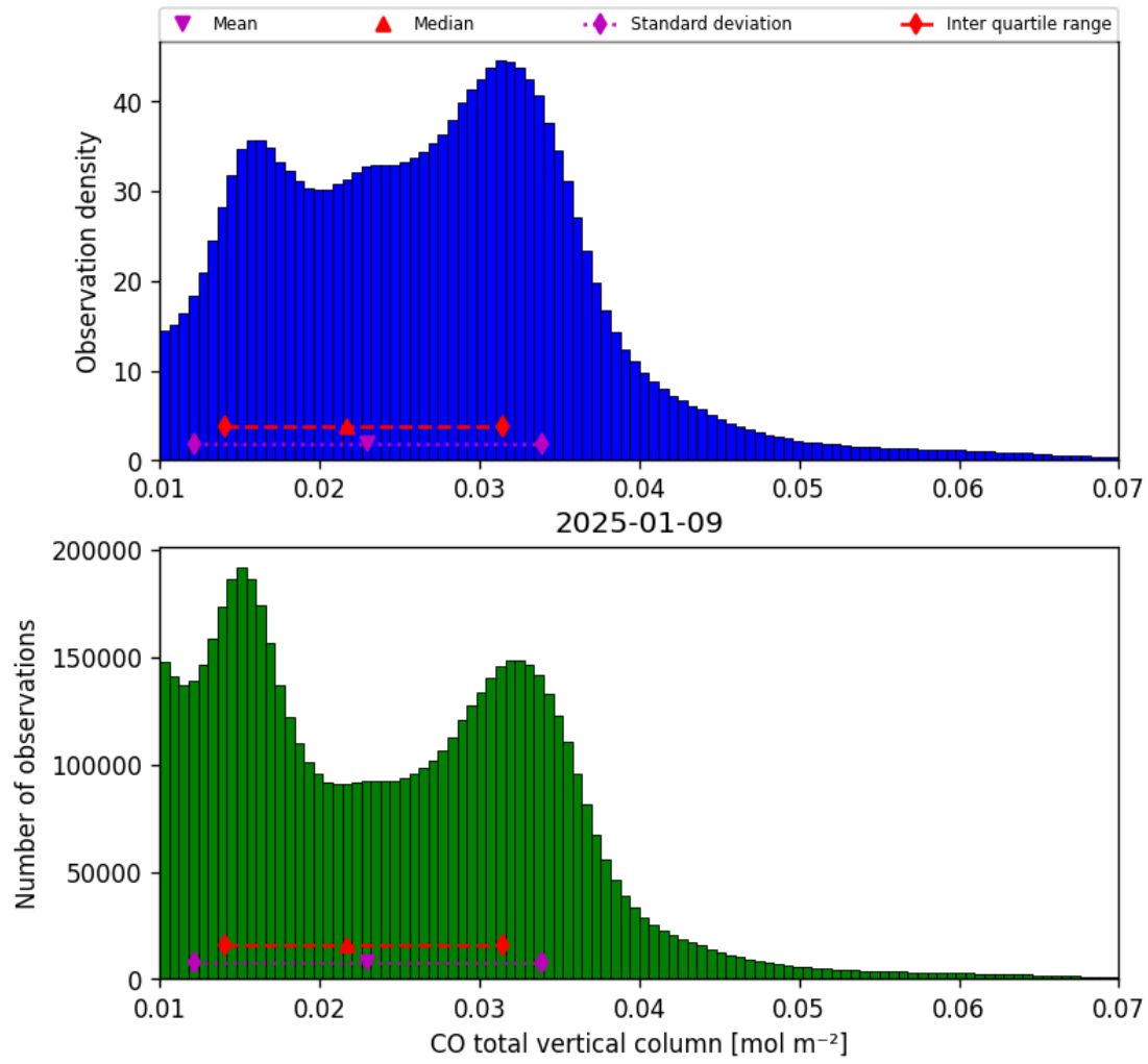
Figure 14: Histogram of “CO total vertical column” for 2025-01-09 to 2025-01-10
