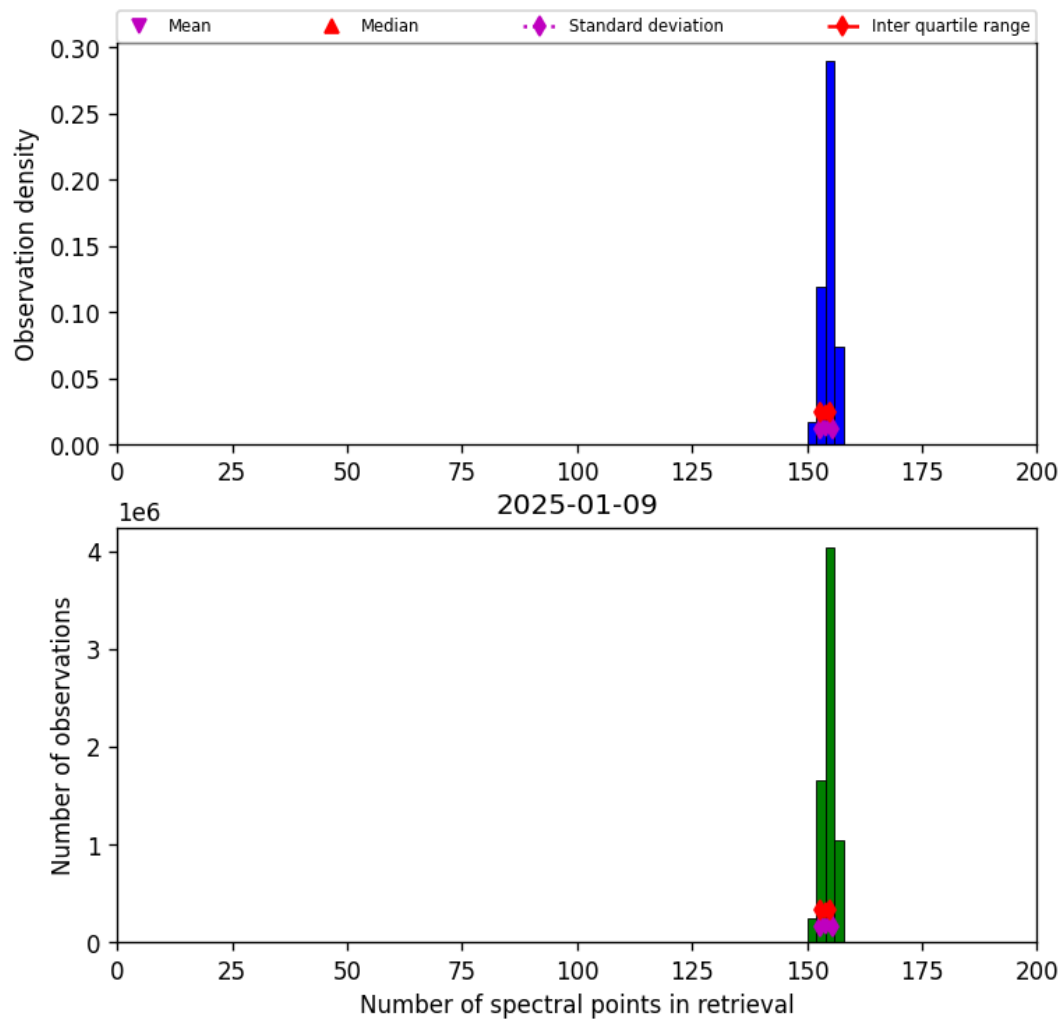
Figure 16: Histogram of “Number of spectral points in retrieval” for 2025-01-09 to 2025-01-10
