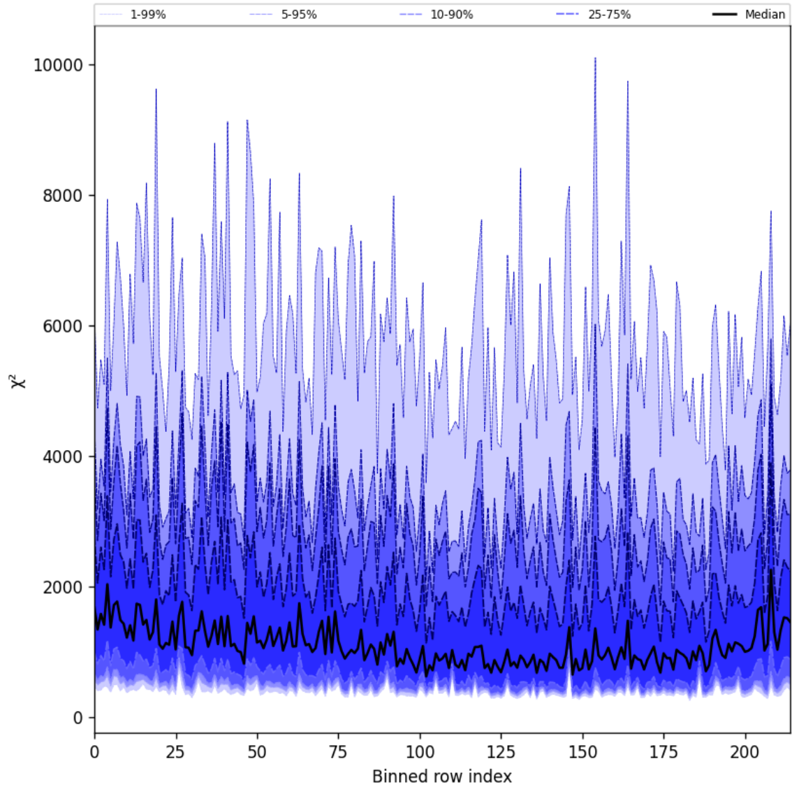
Figure 24: Along track statistics of “ \chi^2 ” for 2025-01-09 to 2025-01-10
