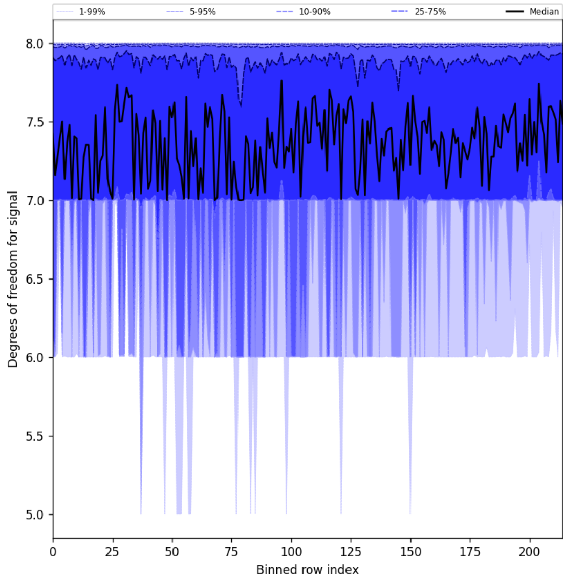
Figure 25: Along track statistics of “Degrees of freedom for signal” for 2025-01-09 to 2025-01-10
