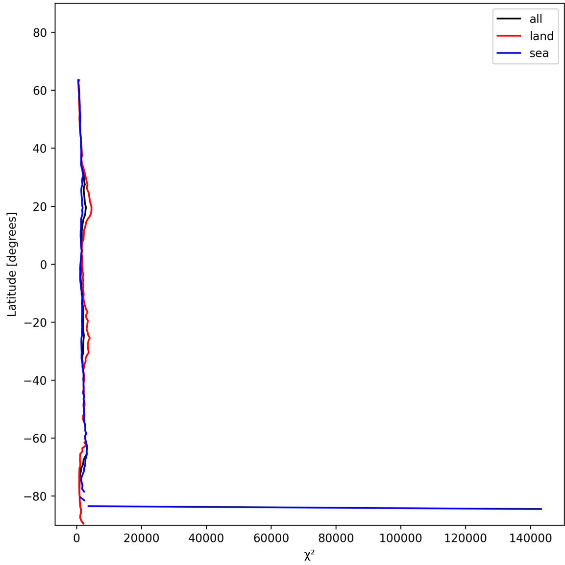
Figure 10: Zonal average of “ \chi^2 ” for 2025-01-09 to 2025-01-10.
