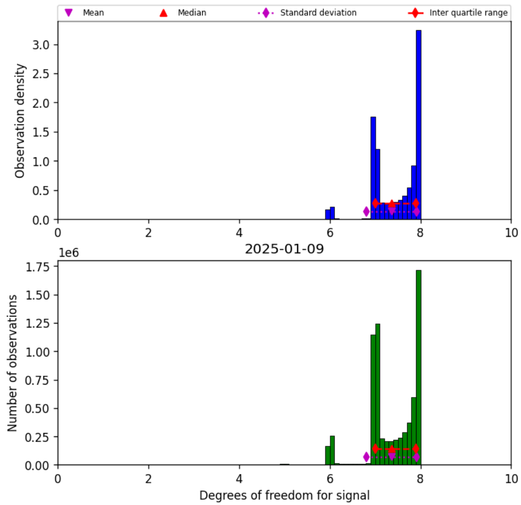
Figure 18: Histogram of “Degrees of freedom for signal” for 2025-01-09 to 2025-01-10
