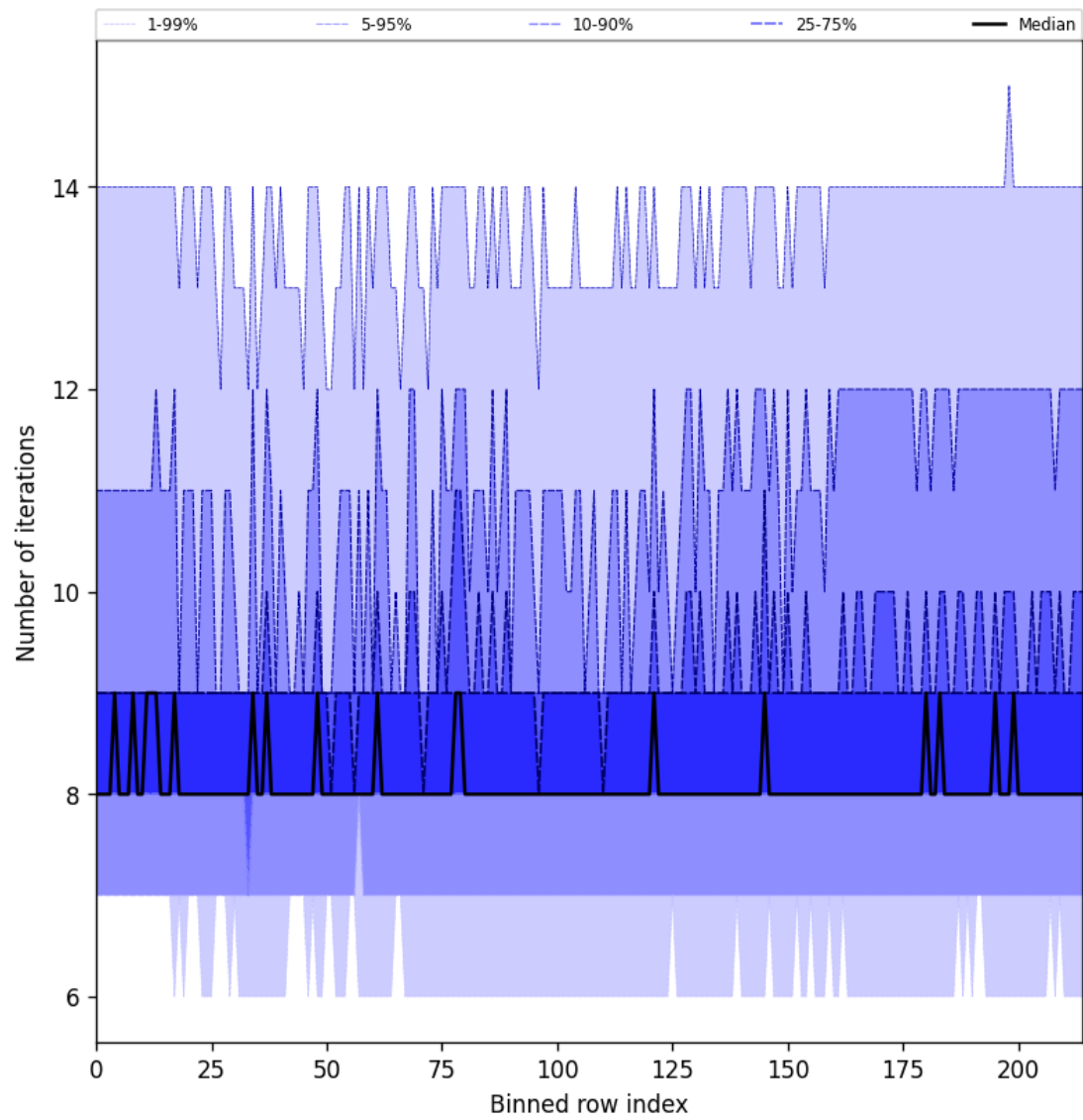
Figure 26: Along track statistics of “Number of iterations” for 2025-01-09 to 2025-01-10
