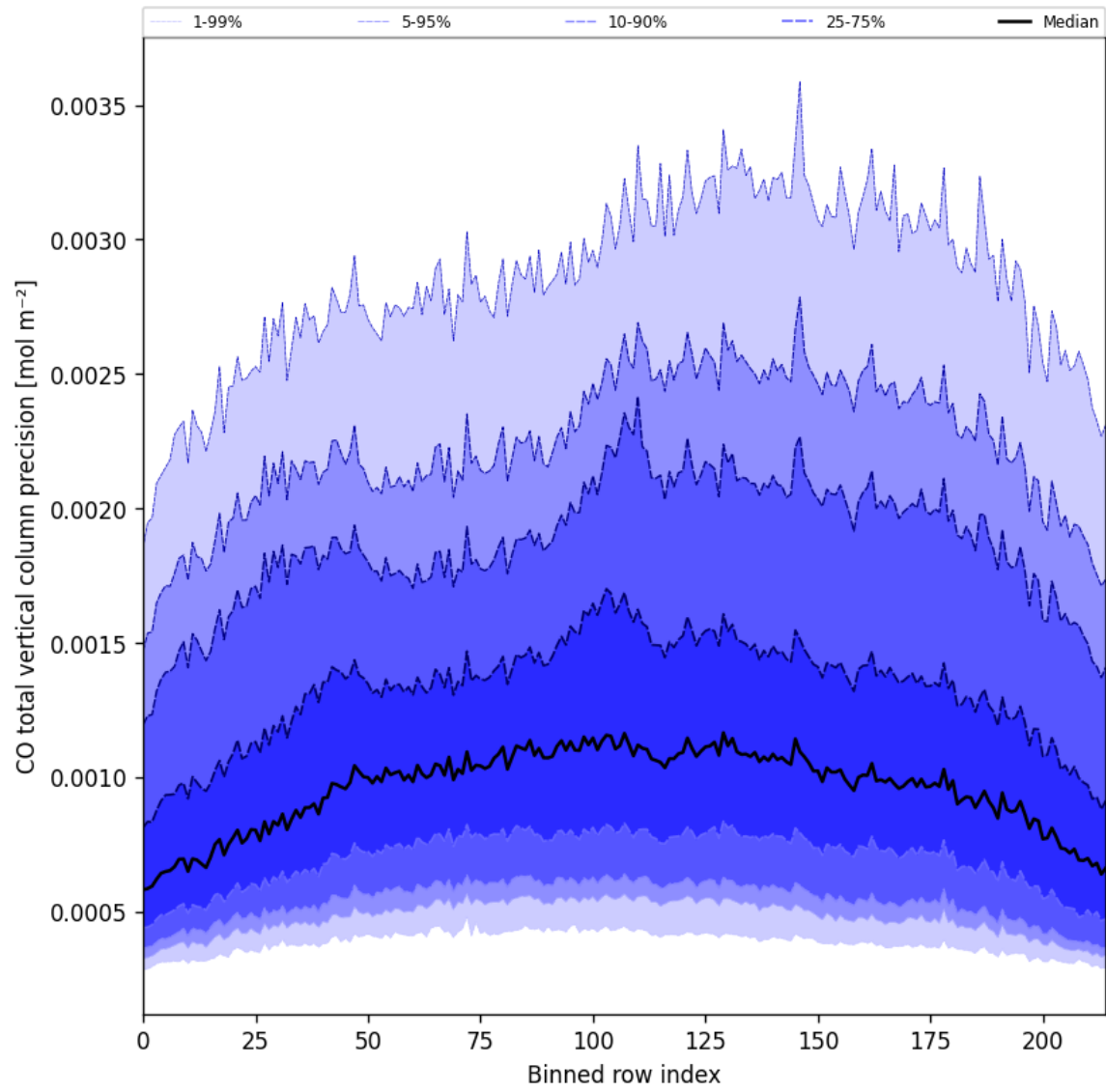
Figure 22: Along track statistics of “CO total vertical column precision” for 2025-01-09 to 2025-01-10
