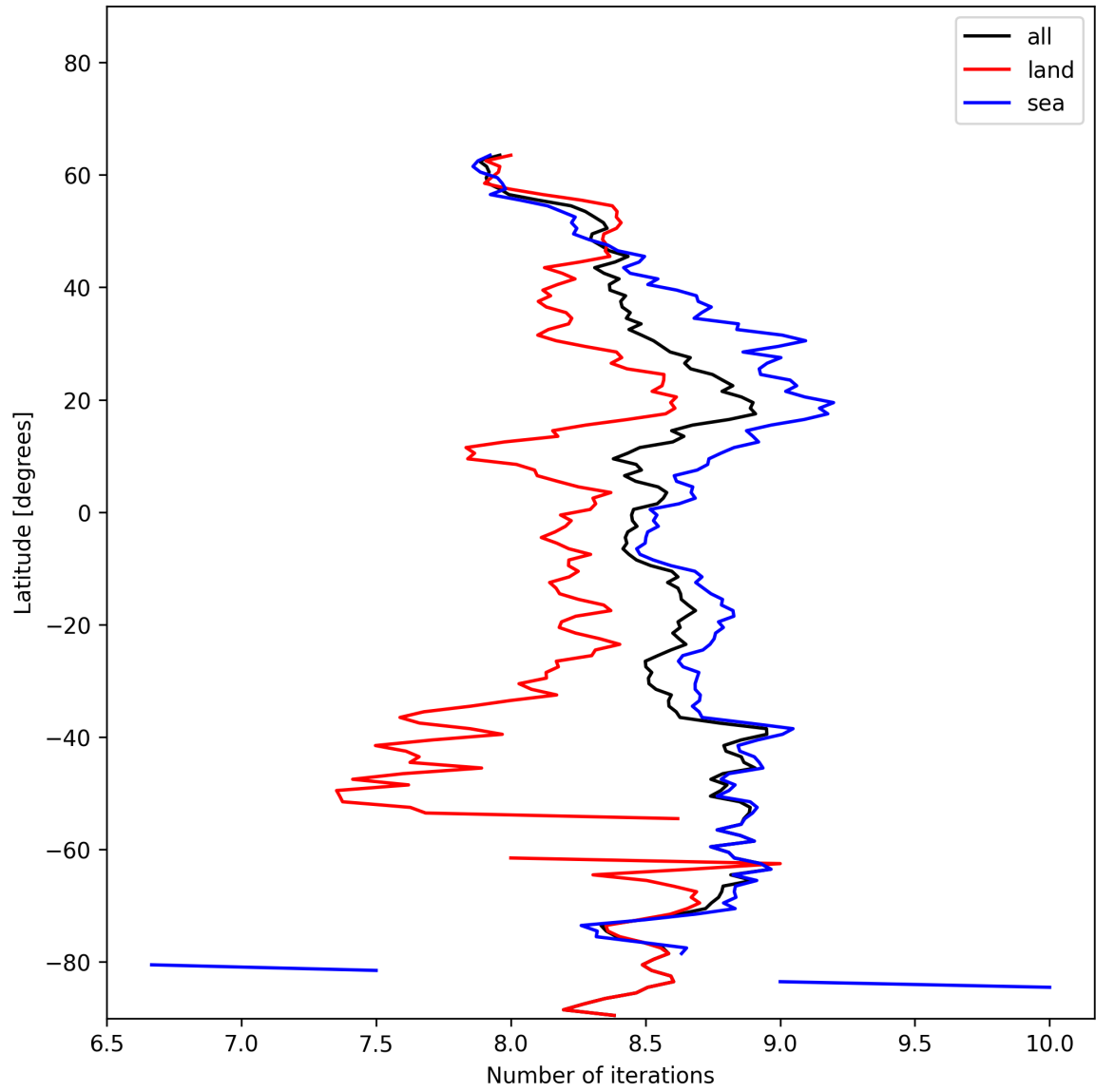
Figure 12: Zonal average of “Number of iterations” for 2025-01-09 to 2025-01-10.
