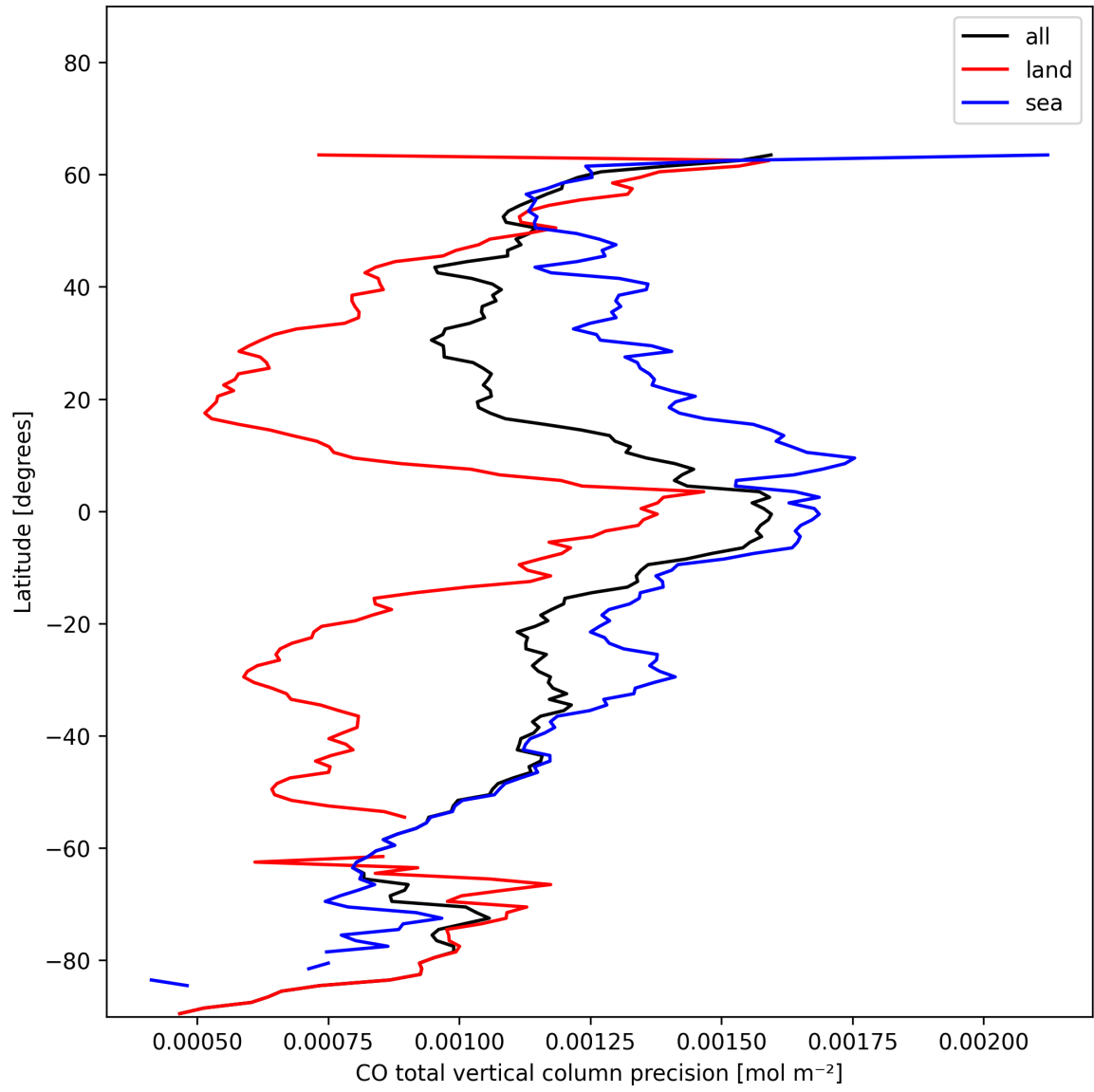
Figure 8: Zonal average of “CO total vertical column precision” for 2025-01-09 to 2025-01-10.
