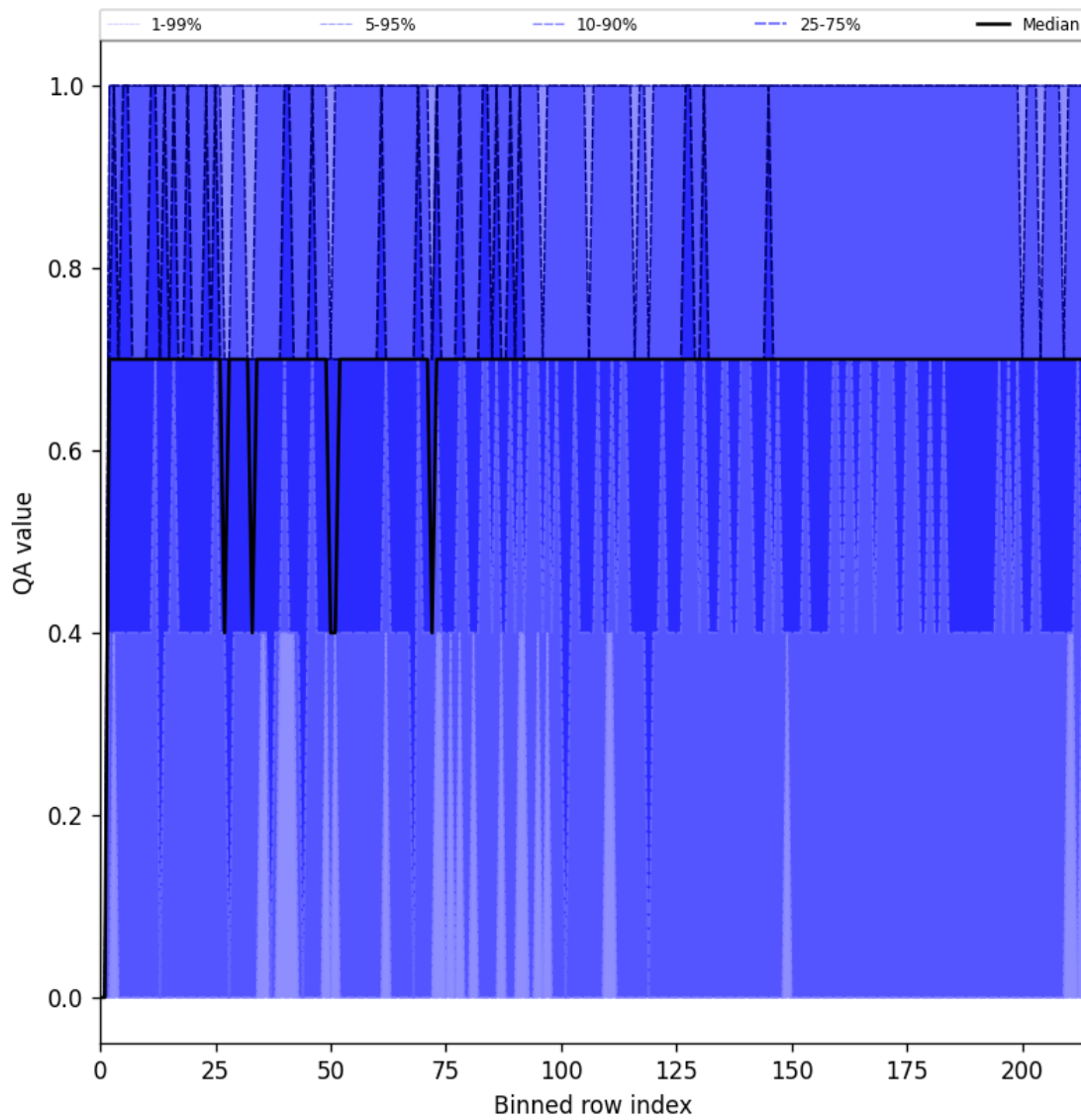
Figure 20: Along track statistics of “QA value” for 2025-01-09 to 2025-01-10
