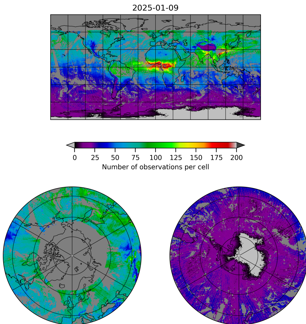
Figure 5: Map of the number of observations for 2025-01-09 to 2025-01-10
