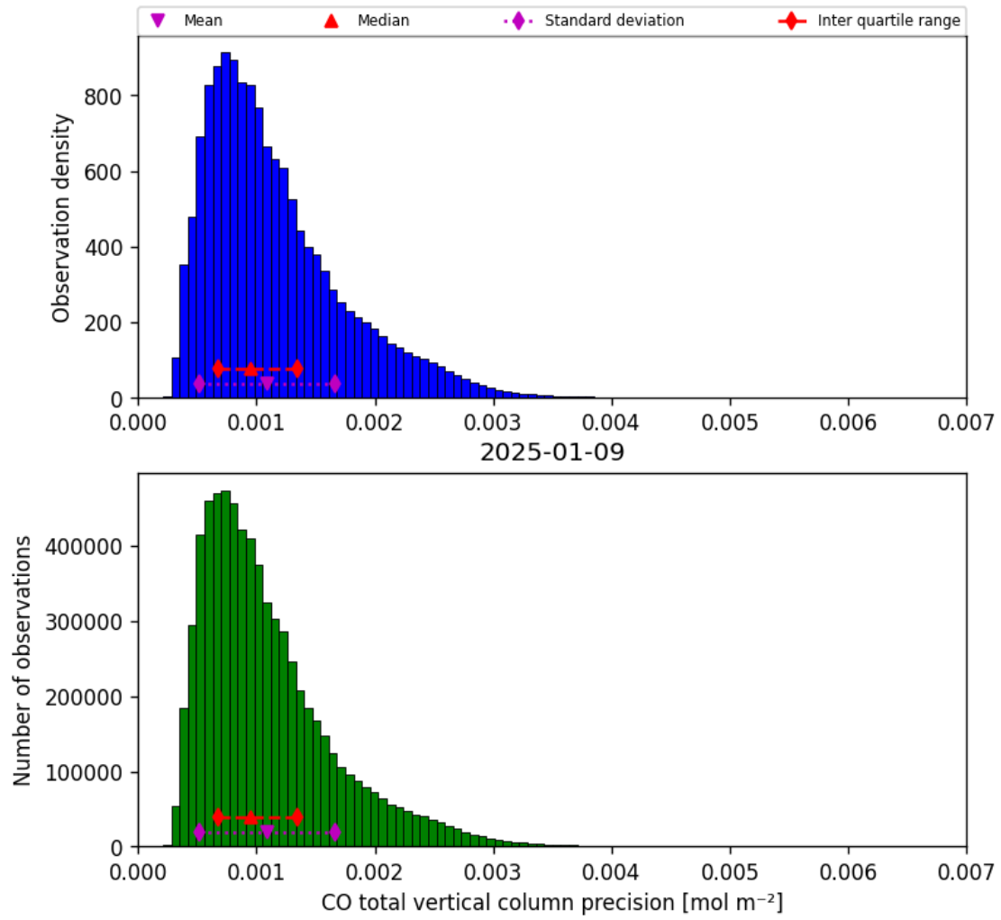
Figure 15: Histogram of “CO total vertical column precision” for 2025-01-09 to 2025-01-10
