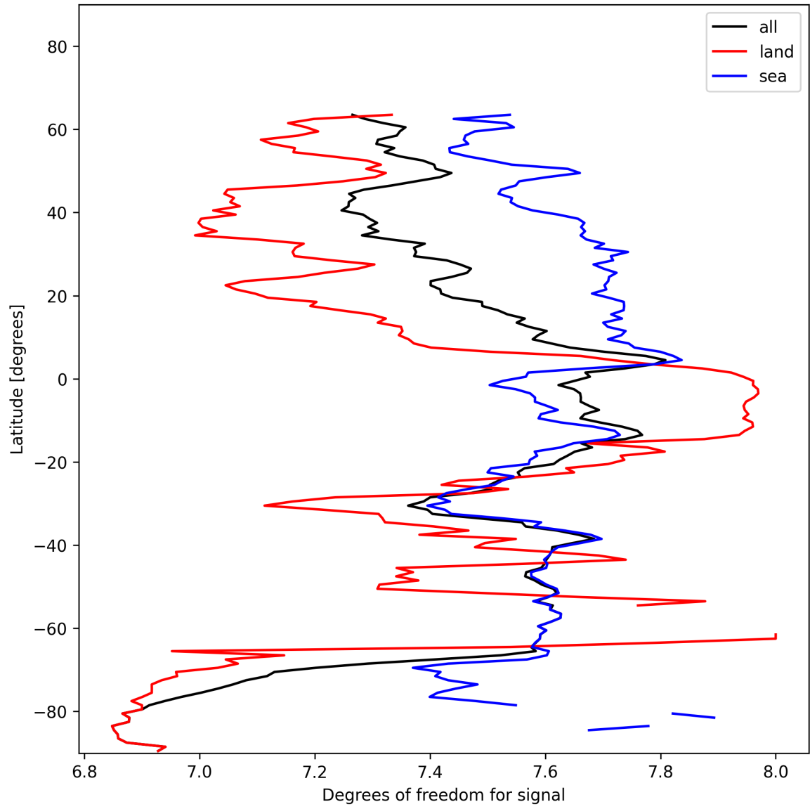
Figure 11: Zonal average of “Degrees of freedom for signal” for 2025-01-09 to 2025-01-10.
