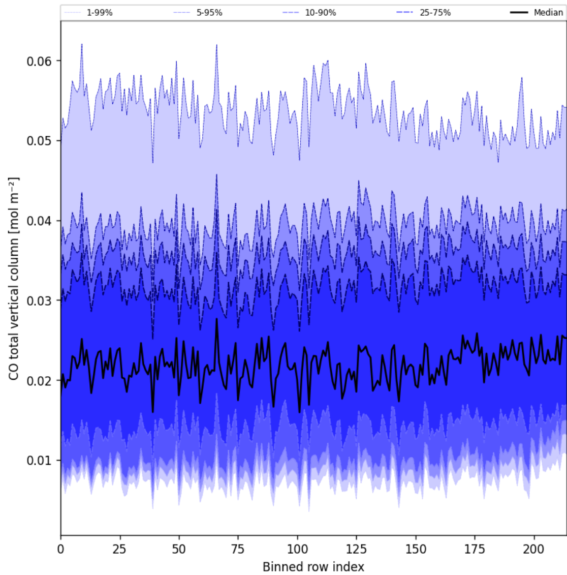
Figure 21: Along track statistics of “CO total vertical column” for 2025-01-09 to 2025-01-10
