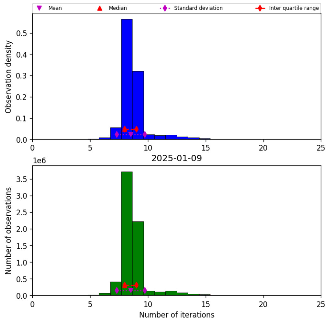
Figure 19: Histogram of “Number of iterations” for 2025-01-09 to 2025-01-10
