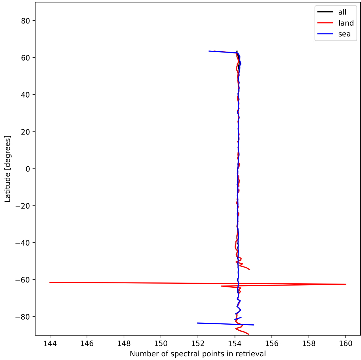
Figure 9: Zonal average of “Number of spectral points in retrieval” for 2025-01-09 to 2025-01-10.
