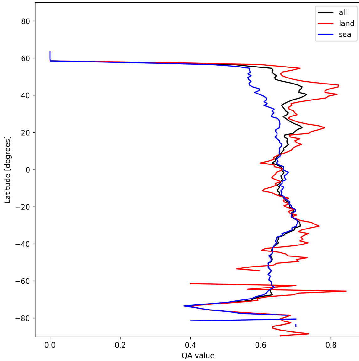
Figure 6: Zonal average of “QA value” for 2025-01-09 to 2025-01-10.
